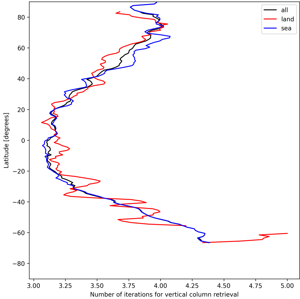
Figure 19: Zonal average of “Number of iterations for vertical column retrieval” for 2025-05-29 to 2025-05-31.
