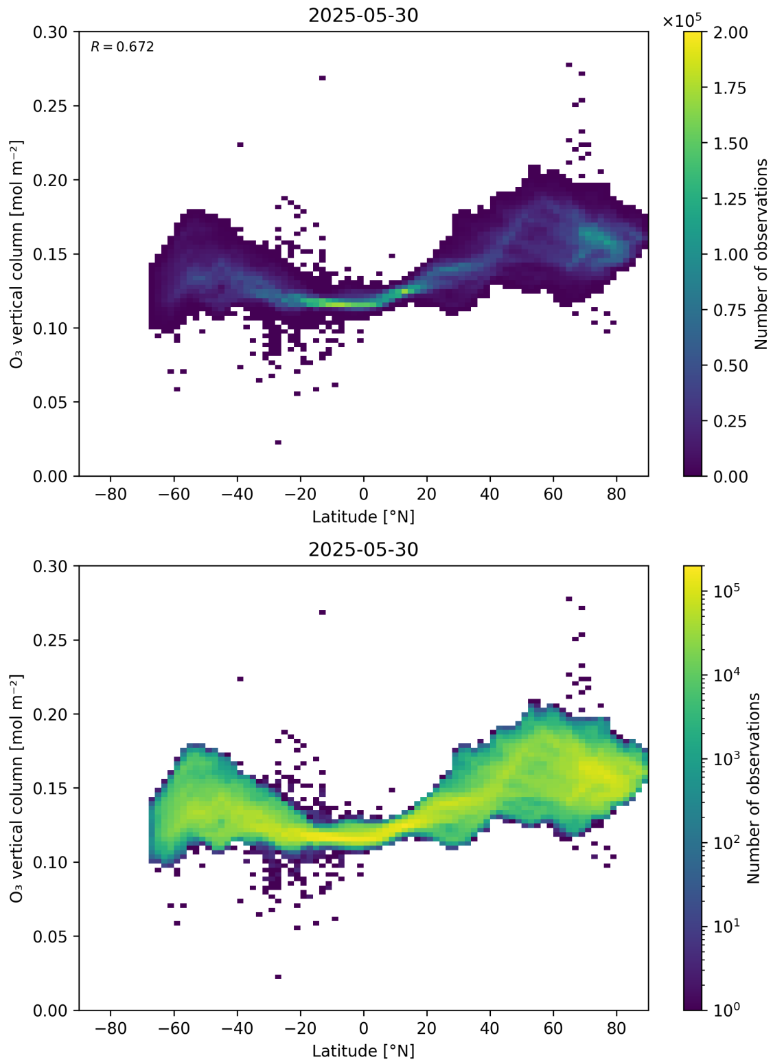
Figure 36: Scatter density plot of “Latitude” against “O 3 vertical column” for 2025-05-29 to 2025-05-31.
