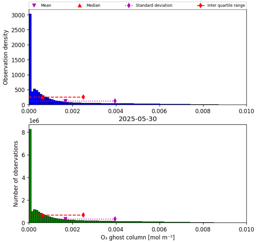
Figure 25: Histogram of “O 3 ghost column” for 2025-05-29 to 2025-05-31
