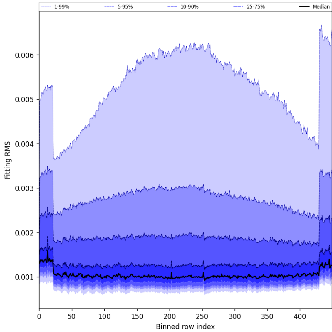
Figure 30: Along track statistics of “Fitting RMS” for 2025-05-29 to 2025-05-31
