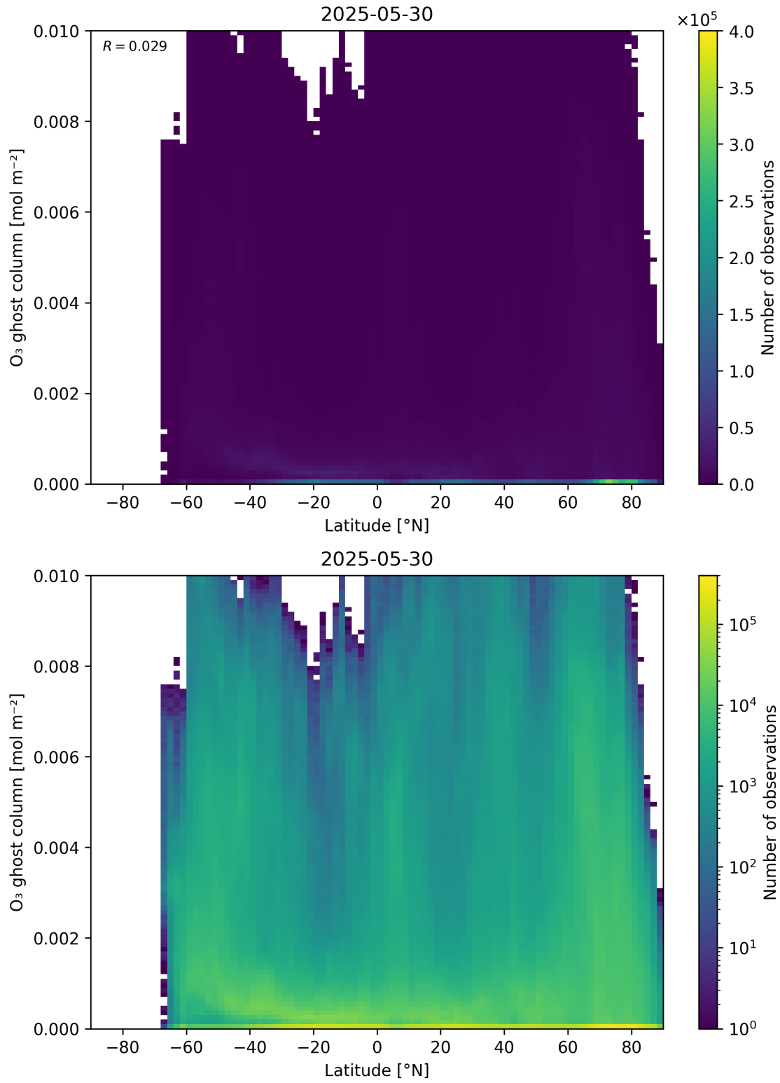
Figure 35: Scatter density plot of “Latitude” against “O 3 ghost column” for 2025-05-29 to 2025-05-31.
