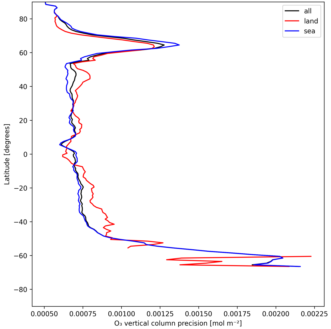
Figure 15: Zonal average of “O 3 vertical column precision” for 2025-05-29 to 2025-05-31.
