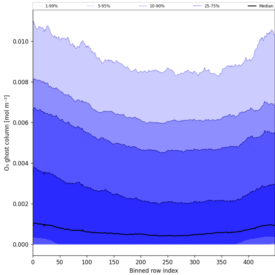
Figure 32: Along track statistics of "O 3 ghost column" for 2025-05-29 to 2025-05-31
