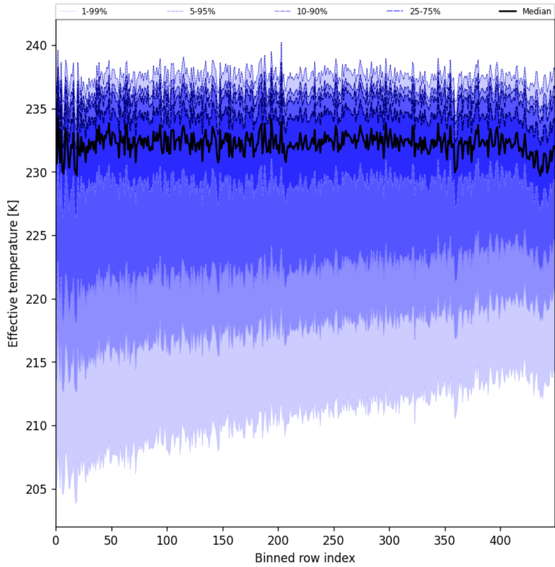
Figure 31: Along track statistics of “Effective temperature” for 2025-05-29 to 2025-05-31
