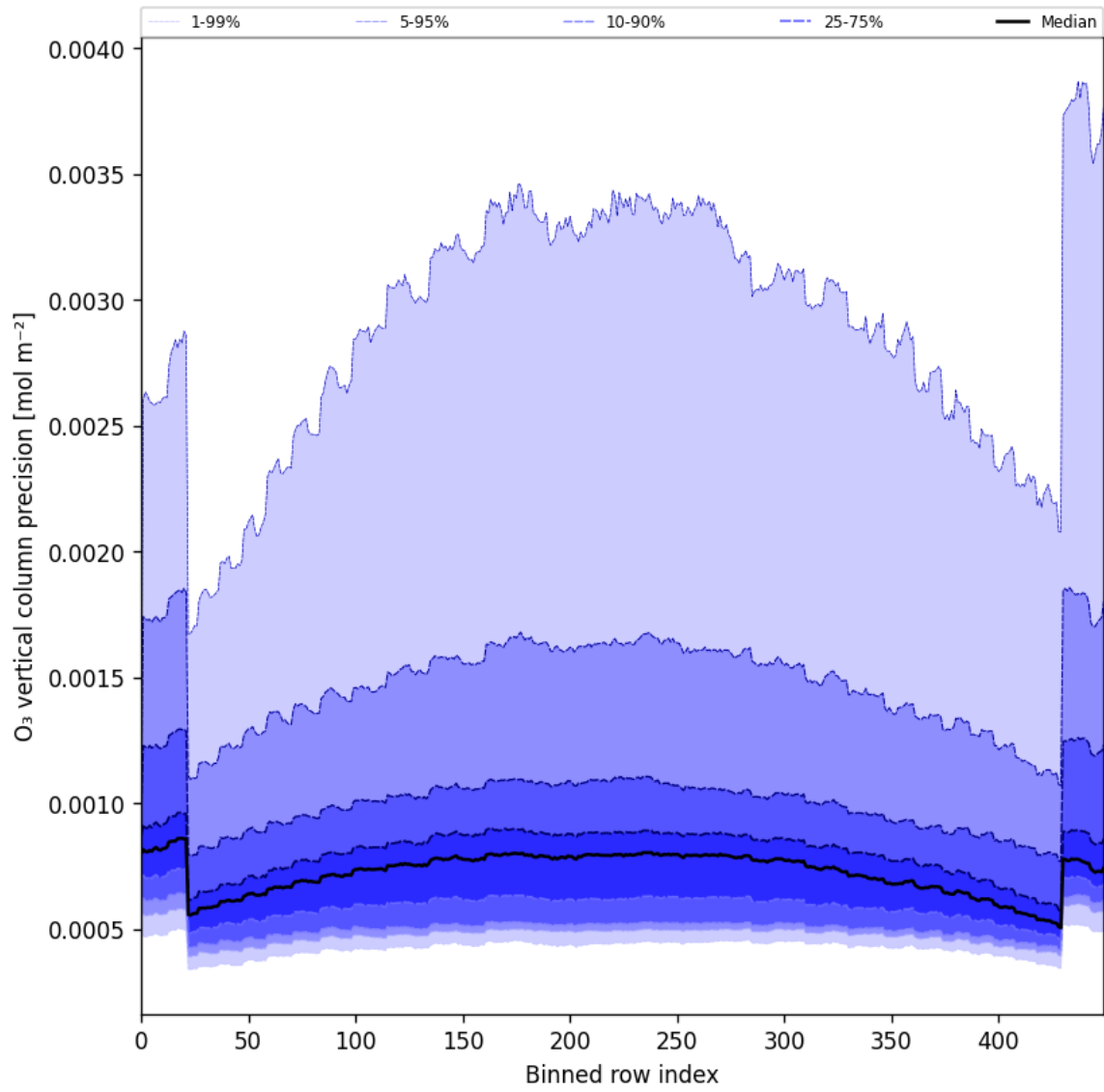
Figure 29: Along track statistics of “O 3 vertical column precision” for 2025-05-29 to 2025-05-31
