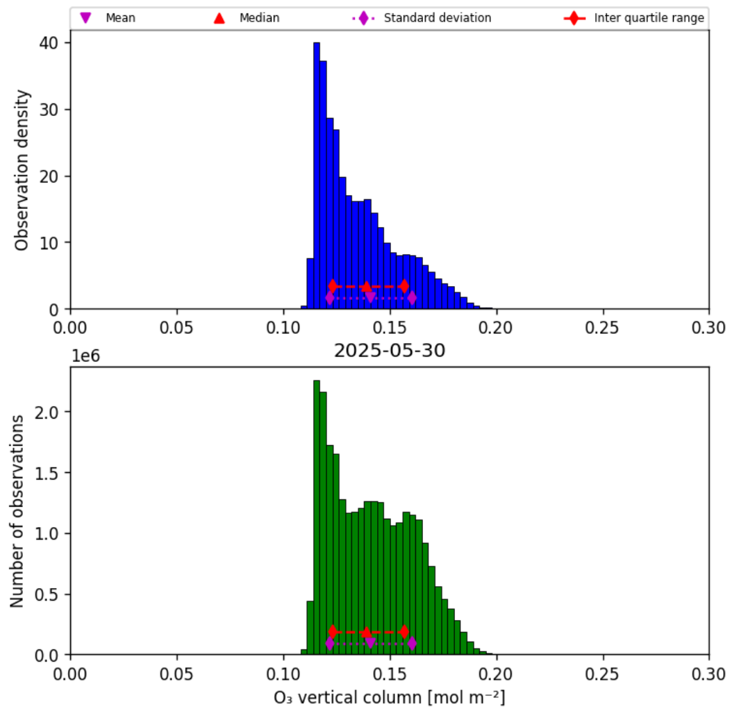
Figure 21: Histogram of “O 3 vertical column” for 2025-05-29 to 2025-05-31
