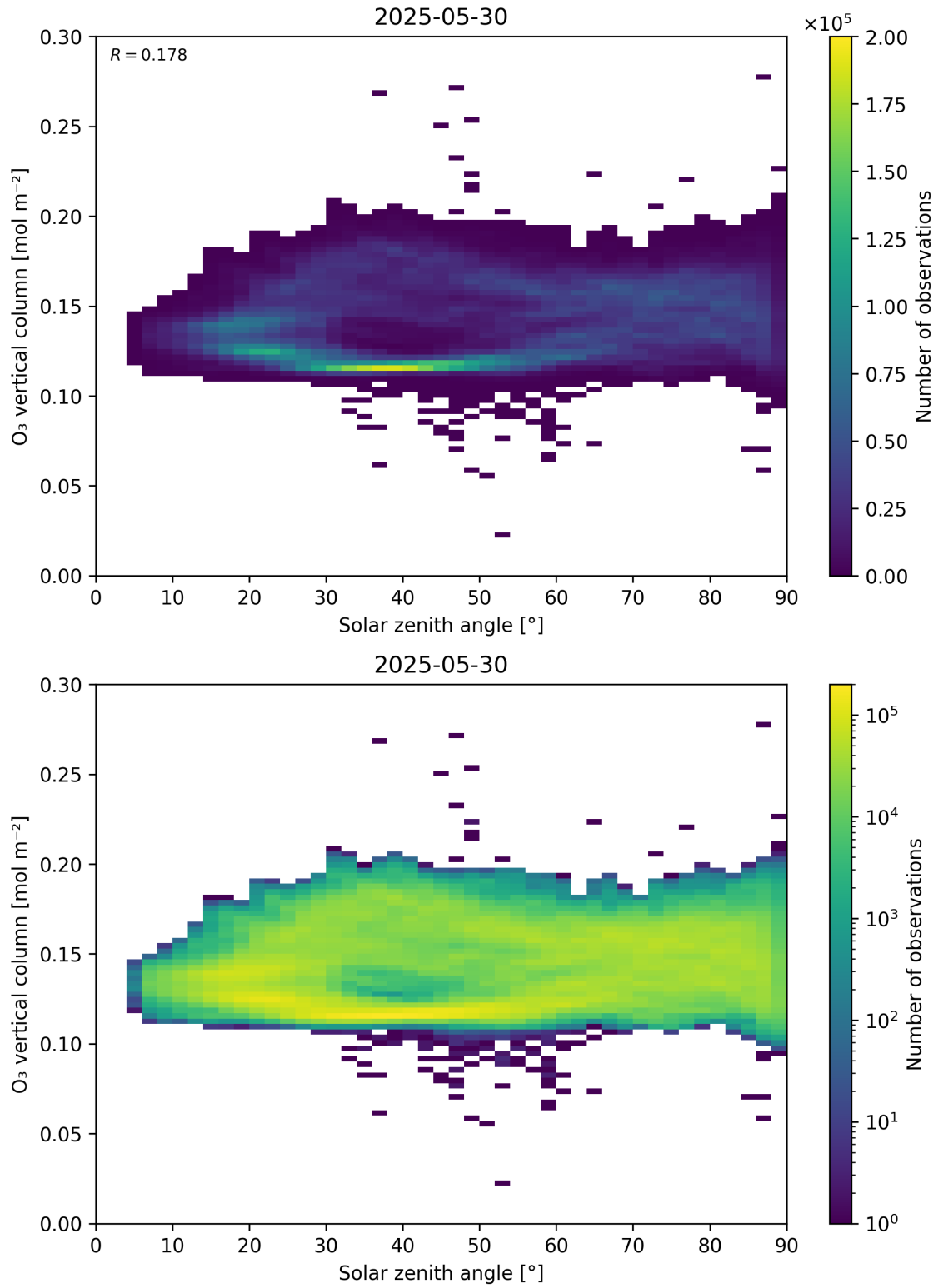
Figure 47: Scatter density plot of “Solar zenith angle” against “O 3 vertical column” for 2025-05-29 to 2025-05-31.
