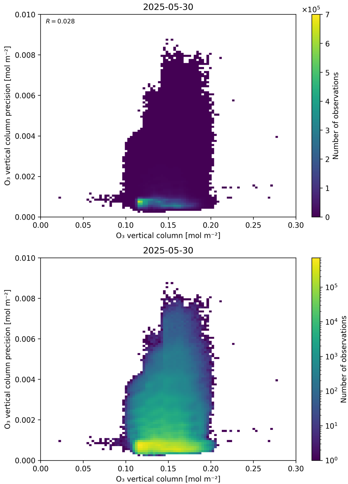
Figure 41: Scatter density plot of “O 3 vertical column” against “O 3 vertical column precision” for 2025-05-29 to 2025-05-31.
