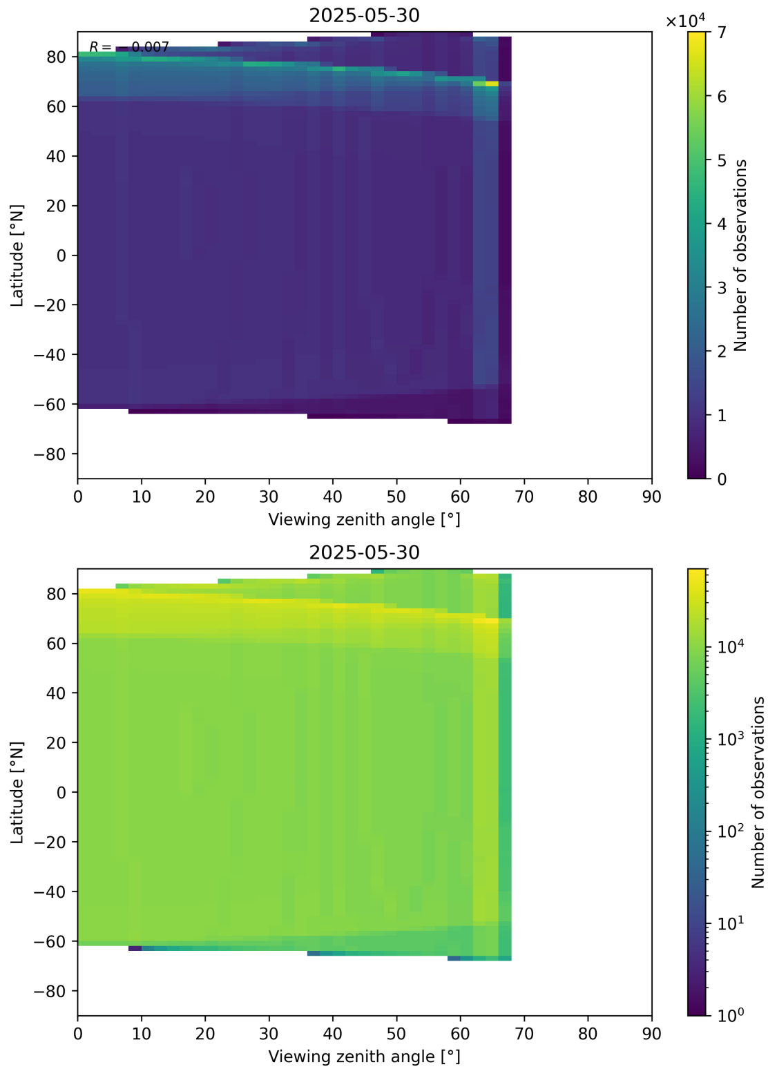
Figure 49: Scatter density plot of “Viewing zenith angle” against “Latitude” for 2025-05-29 to 2025-05-31.
