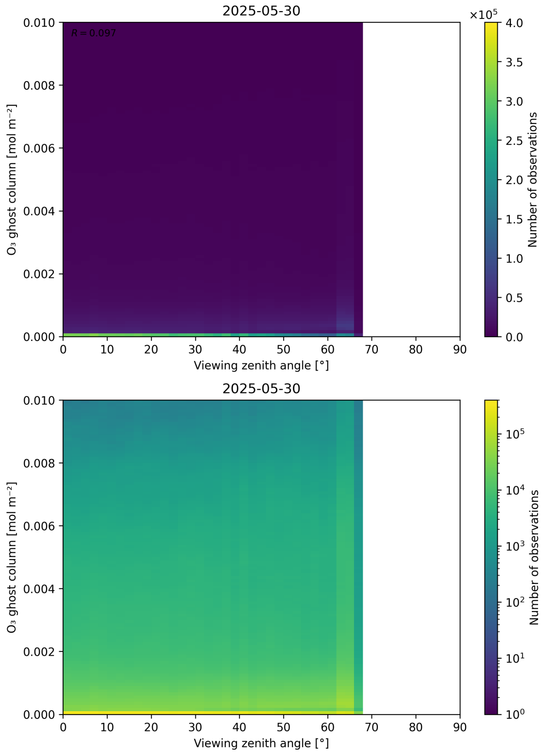
Figure 51: Scatter density plot of “Viewing zenith angle” against “O 3 ghost column” for 2025-05-29 to 2025-05-31.
