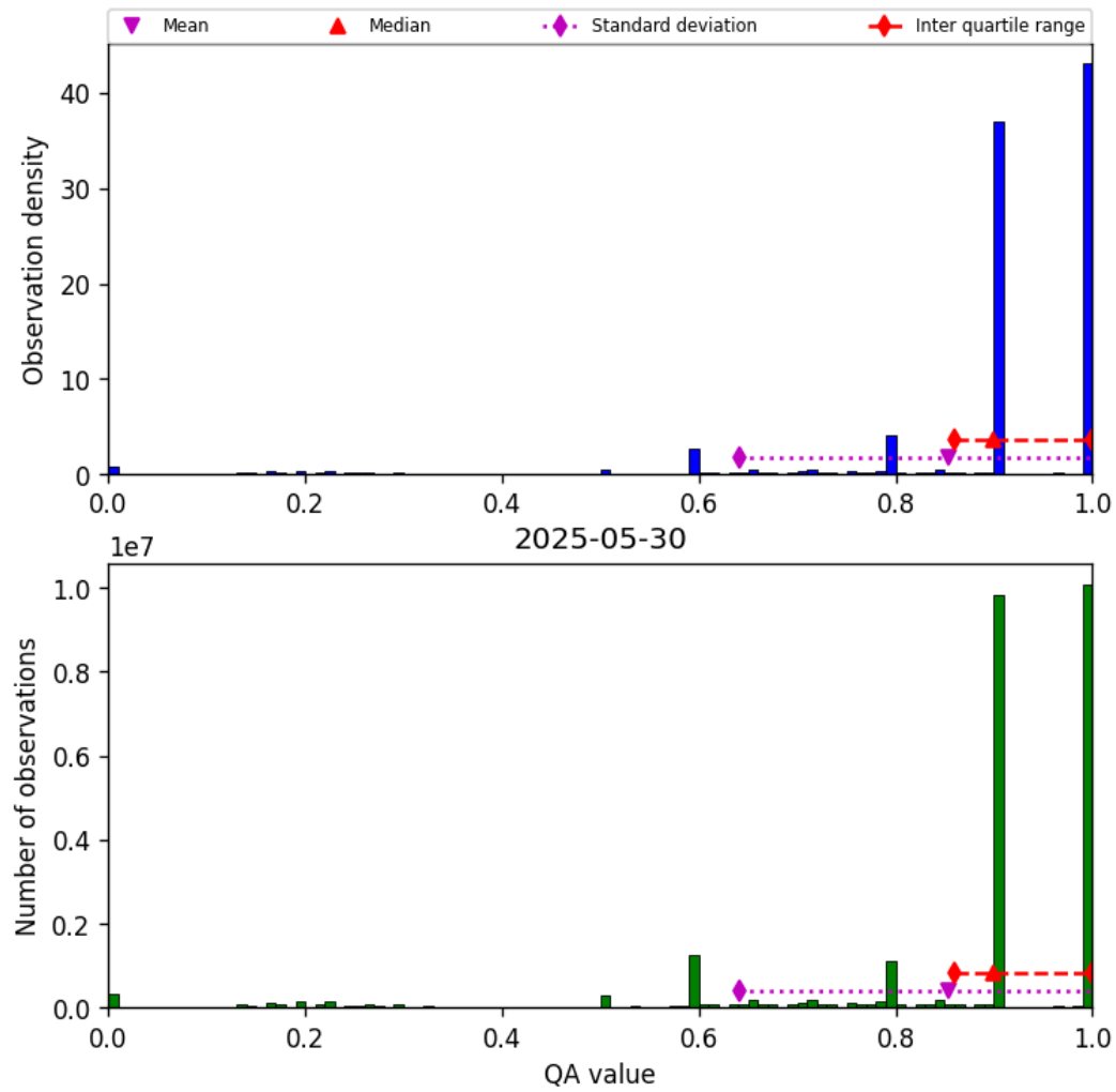
Figure 20: Histogram of “QA value” for 2025-05-29 to 2025-05-31
