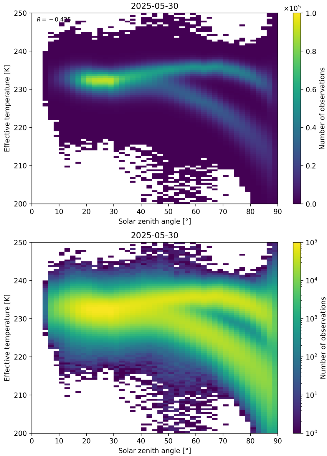
Figure 45: Scatter density plot of “Solar zenith angle” against “Effective temperature” for 2025-05-29 to 2025-05-31.
