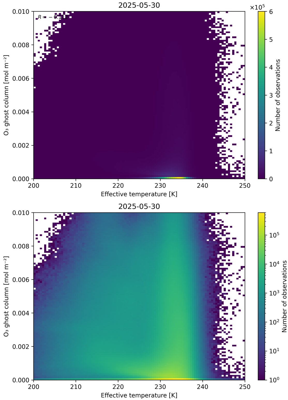
Figure 38: Scatter density plot of “Effective temperature” against “O 3 ghost column” for 2025-05-29 to 2025-05-31.
