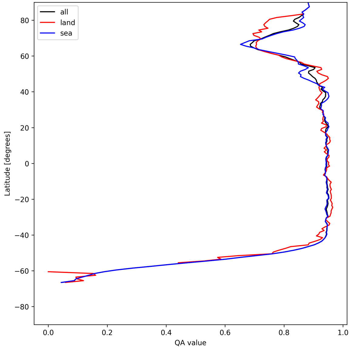
Figure 13: Zonal average of “QA value” for 2025-05-29 to 2025-05-31.
