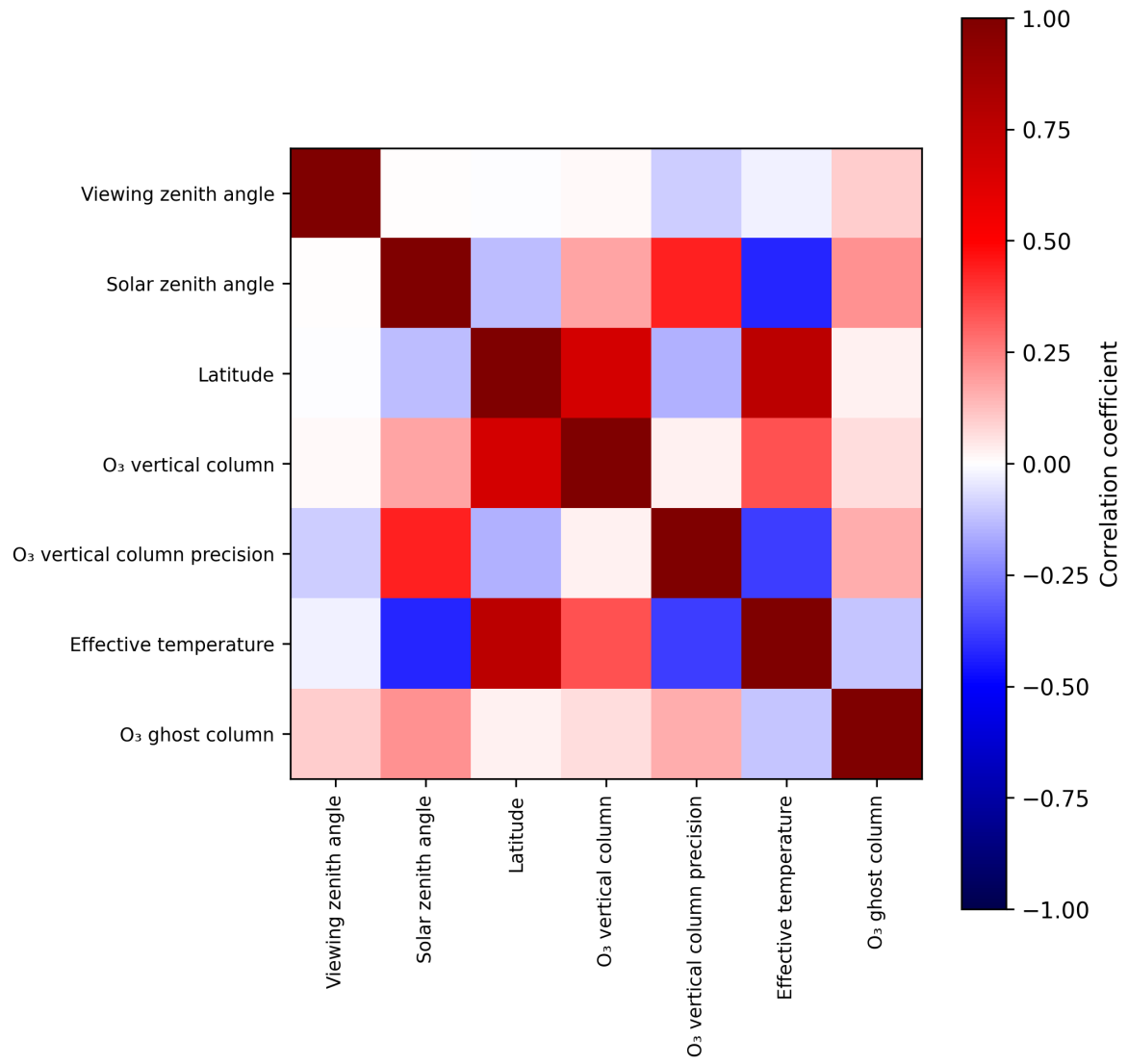
Figure 2: Map of correlation matrix for 2025-05-29 to 2025-05-31.
