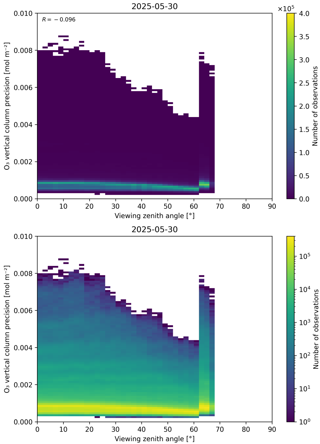
Figure 53: Scatter density plot of “Viewing zenith angle” against “O 3 vertical column precision” for 2025-05-29 to 2025-05-31.
