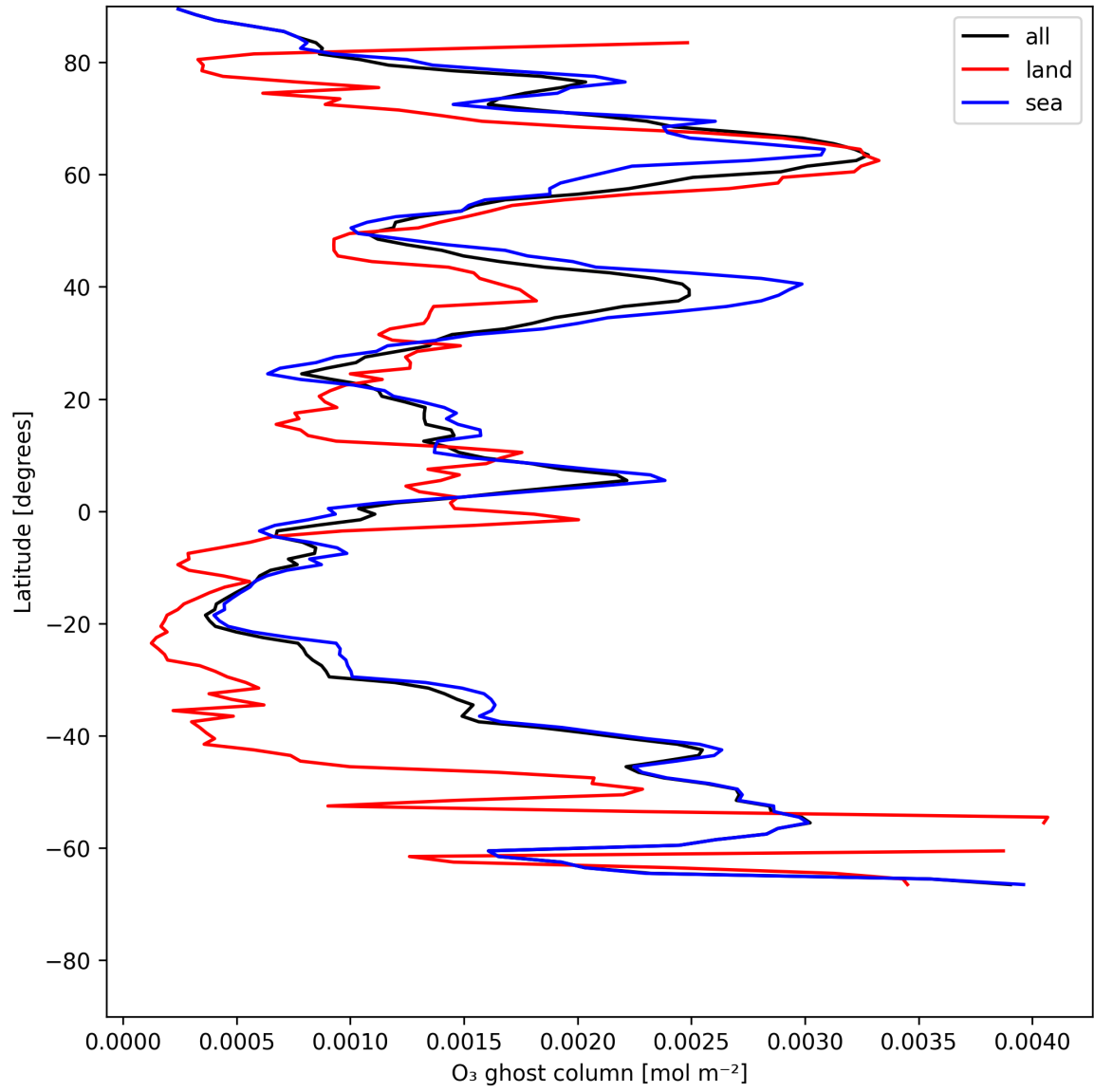
Figure 18: Zonal average of "O 3 ghost column" for 2025-05-29 to 2025-05-31.
