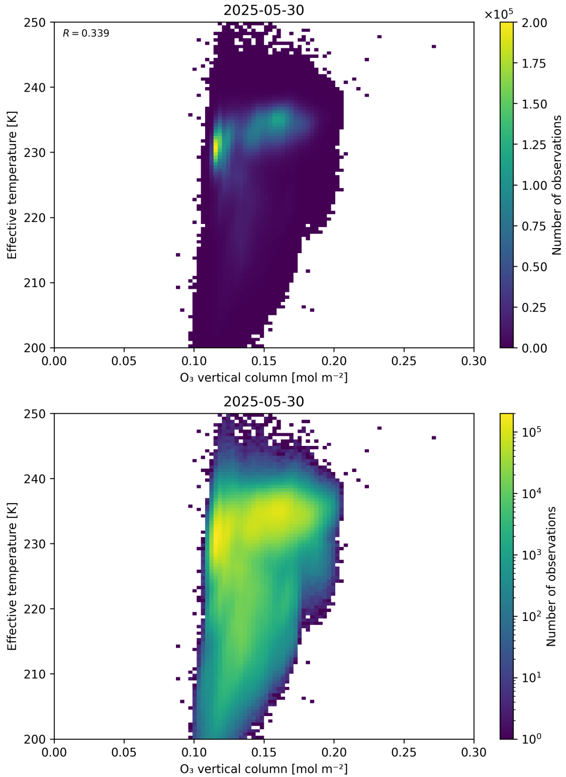
Figure 39: Scatter density plot of “O 3 vertical column” against “Effective temperature” for 2025-05-29 to 2025-05-31.
