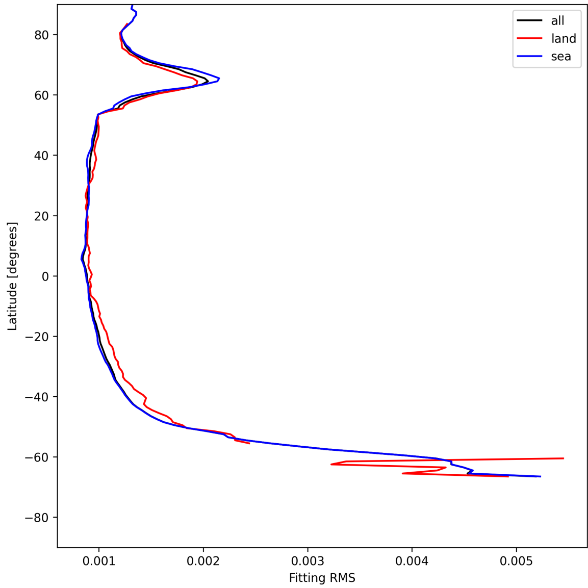
Figure 16: Zonal average of “Fitting RMS” for 2025-05-29 to 2025-05-31.
