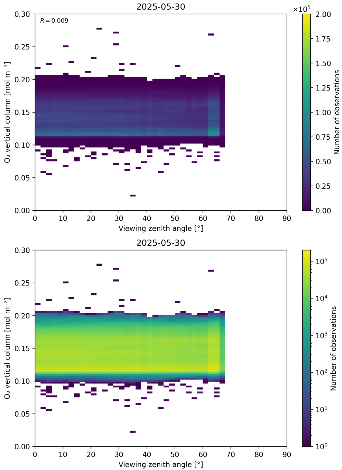
Figure 52: Scatter density plot of “Viewing zenith angle” against “O 3 vertical column” for 2025-05-29 to 2025-05-31.
