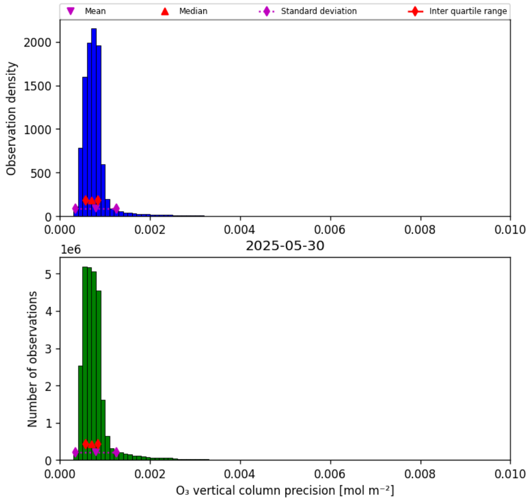
Figure 22: Histogram of “O 3 vertical column precision” for 2025-05-29 to 2025-05-31
