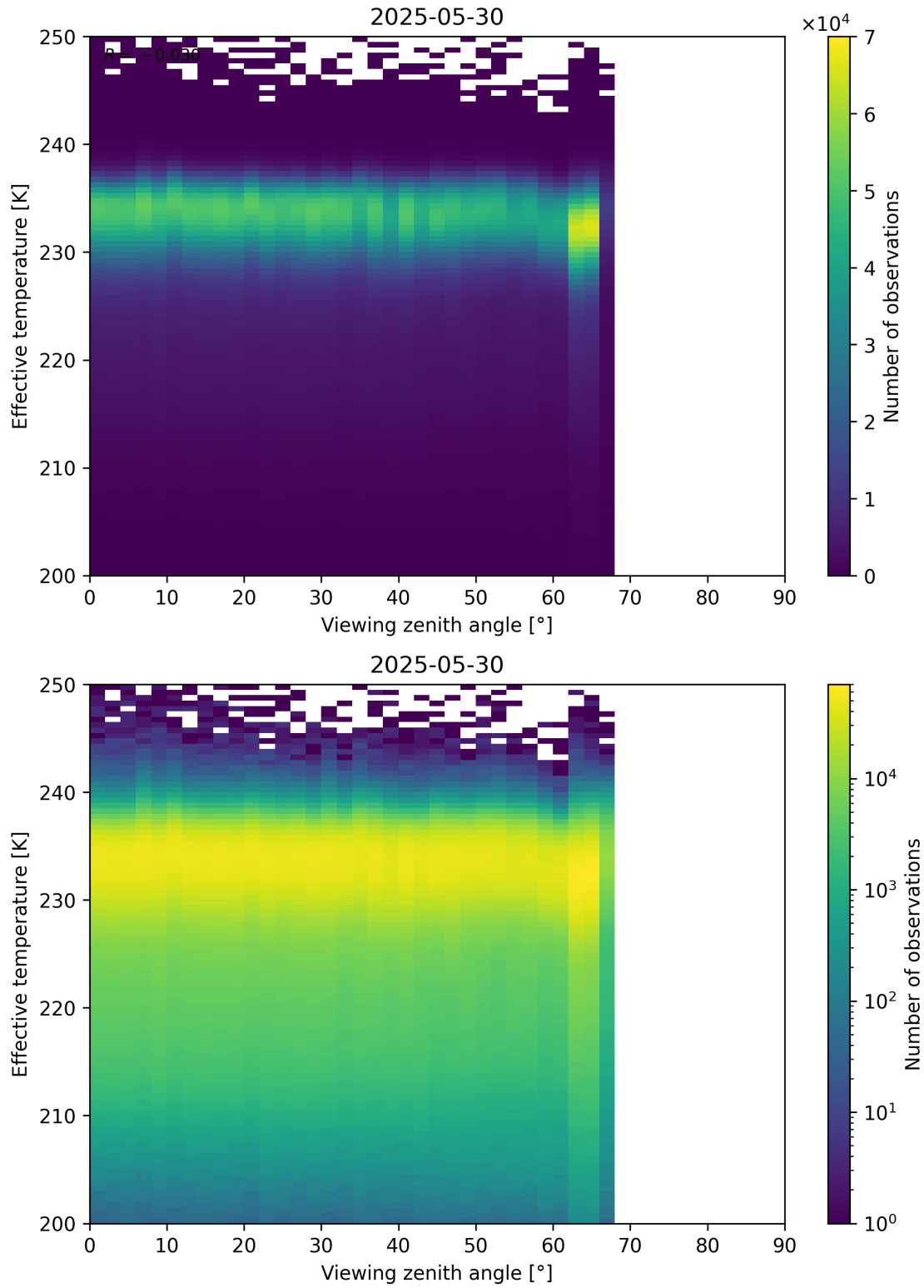
Figure 50: Scatter density plot of “Viewing zenith angle” against “Effective temperature” for 2025-05-29 to 2025-05-31.
