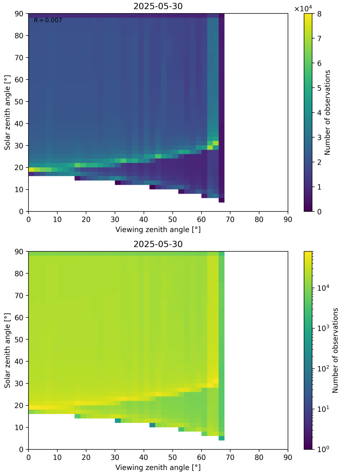
Figure 54: Scatter density plot of “Viewing zenith angle” against “Solar zenith angle” for 2025-05-29 to 2025-05-31.
