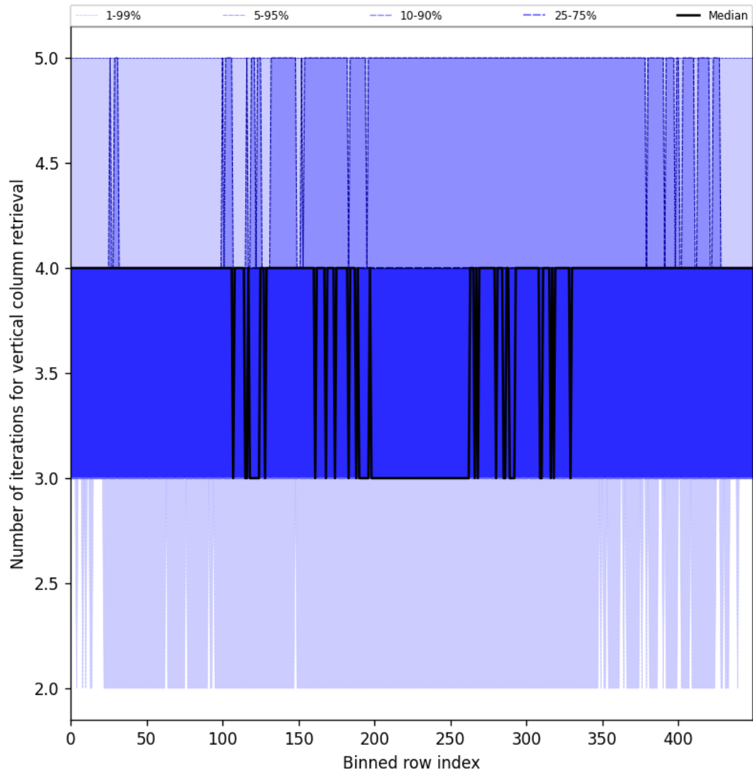
Figure 33: Along track statistics of “Number of iterations for vertical column retrieval” for 2025-05-29 to 2025-05-31
