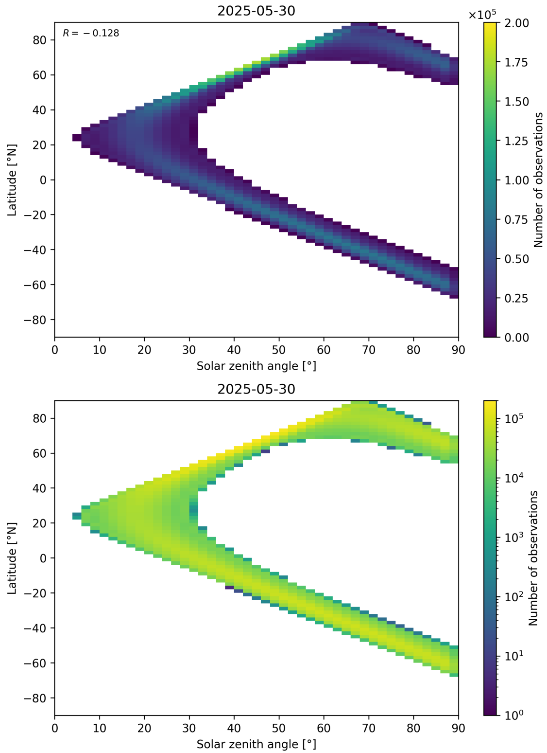
Figure 44: Scatter density plot of “Solar zenith angle” against “Latitude” for 2025-05-29 to 2025-05-31.
