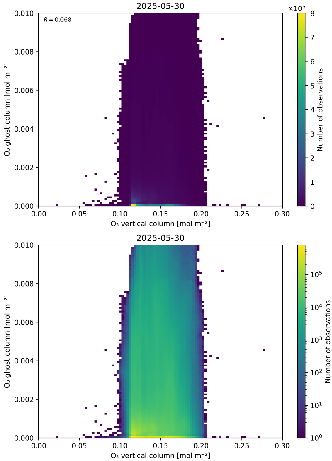
Figure 40: Scatter density plot of “O 3 vertical column” against “O 3 ghost column” for 2025-05-29 to 2025-05-31.
