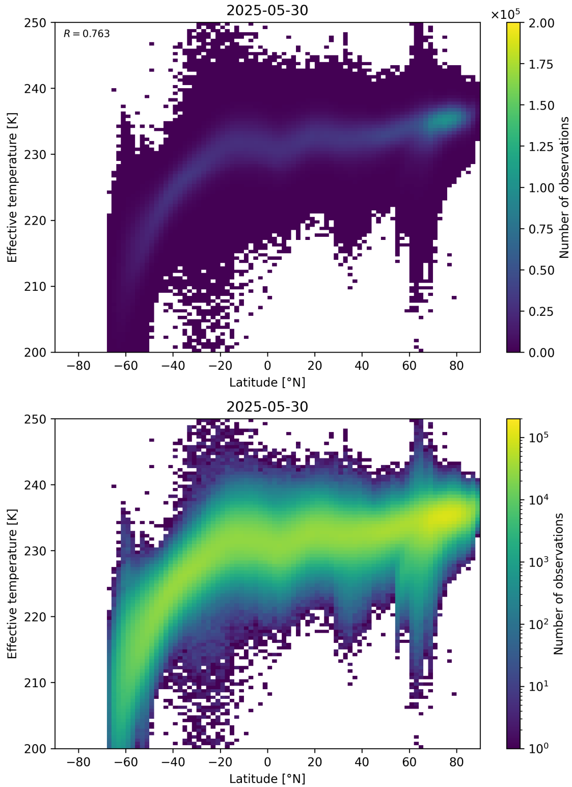
Figure 34: Scatter density plot of “Latitude” against “Effective temperature” for 2025-05-29 to 2025-05-31.
