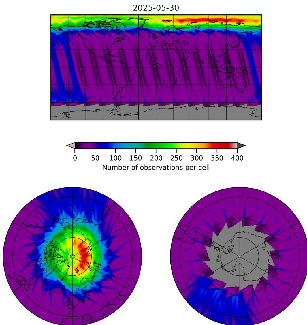
Figure 12: Map of the number of observations for 2025-05-29 to 2025-05-31
