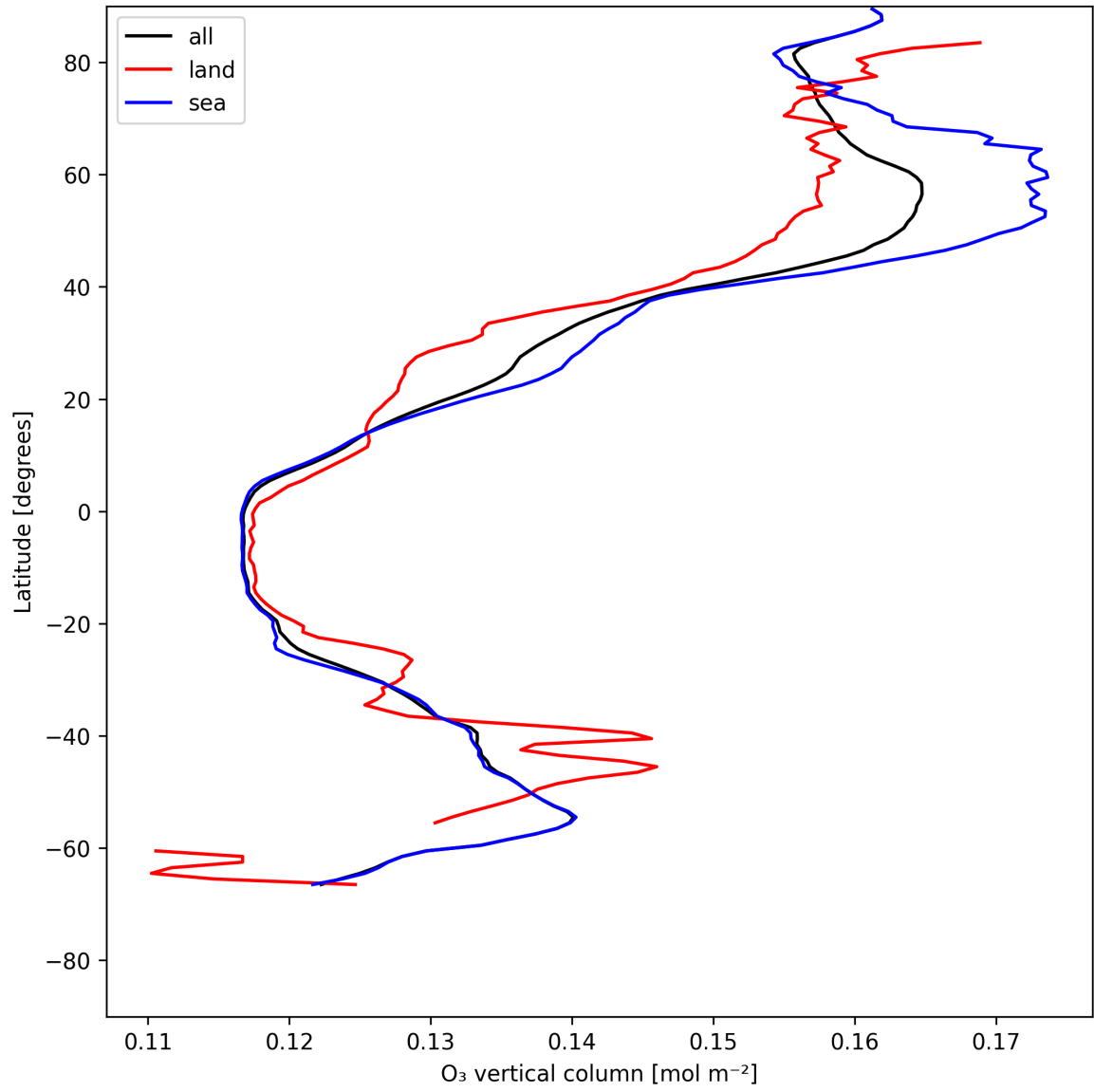
Figure 14: Zonal average of “O 3 vertical column” for 2025-05-29 to 2025-05-31.
