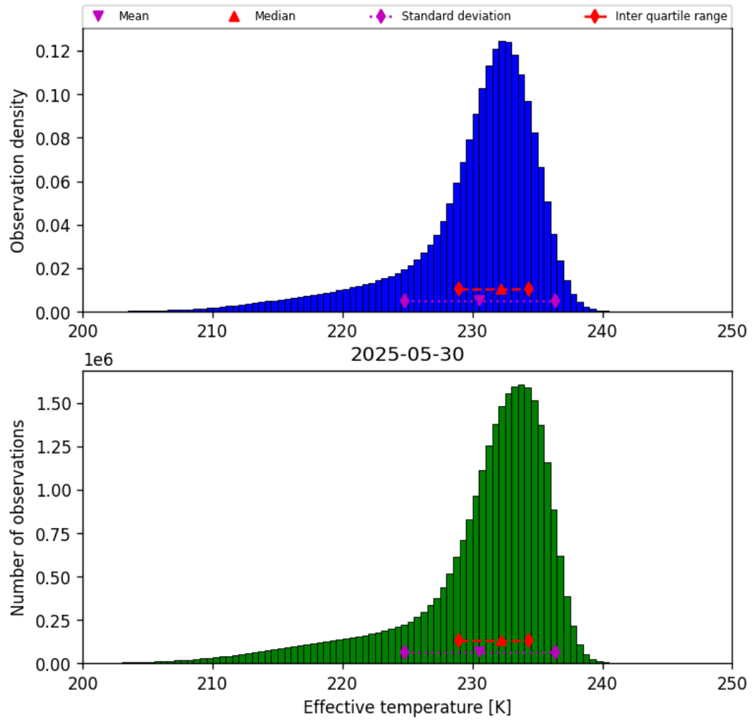
Figure 24: Histogram of “Effective temperature” for 2025-05-29 to 2025-05-31
