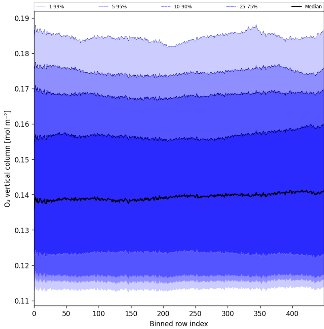
Figure 28: Along track statistics of “O 3 vertical column” for 2025-05-29 to 2025-05-31
