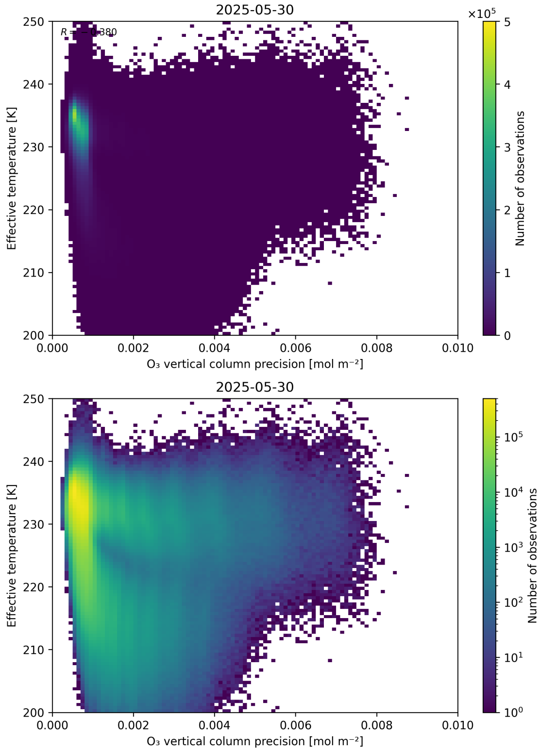
Figure 42: Scatter density plot of “O 3 vertical column precision” against “Effective temperature” for 2025-05-29 to 2025-05-31.
