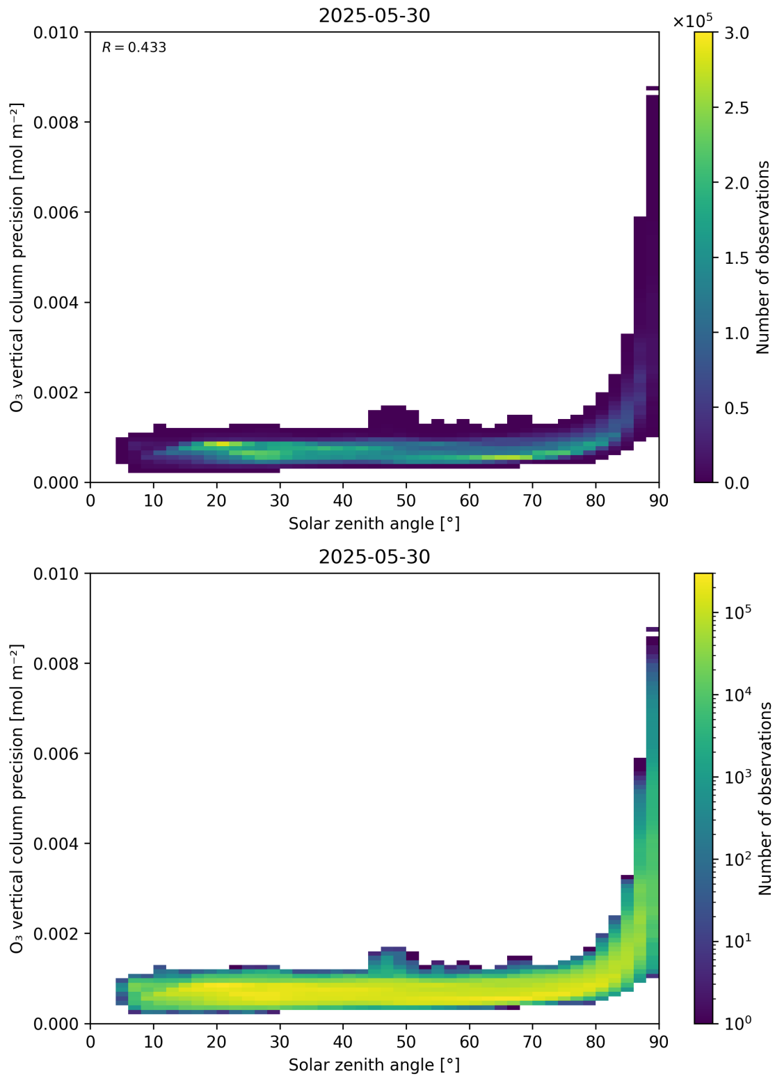
Figure 48: Scatter density plot of “Solar zenith angle” against “O 3 vertical column precision” for 2025-05-29 to 2025-05-31.
