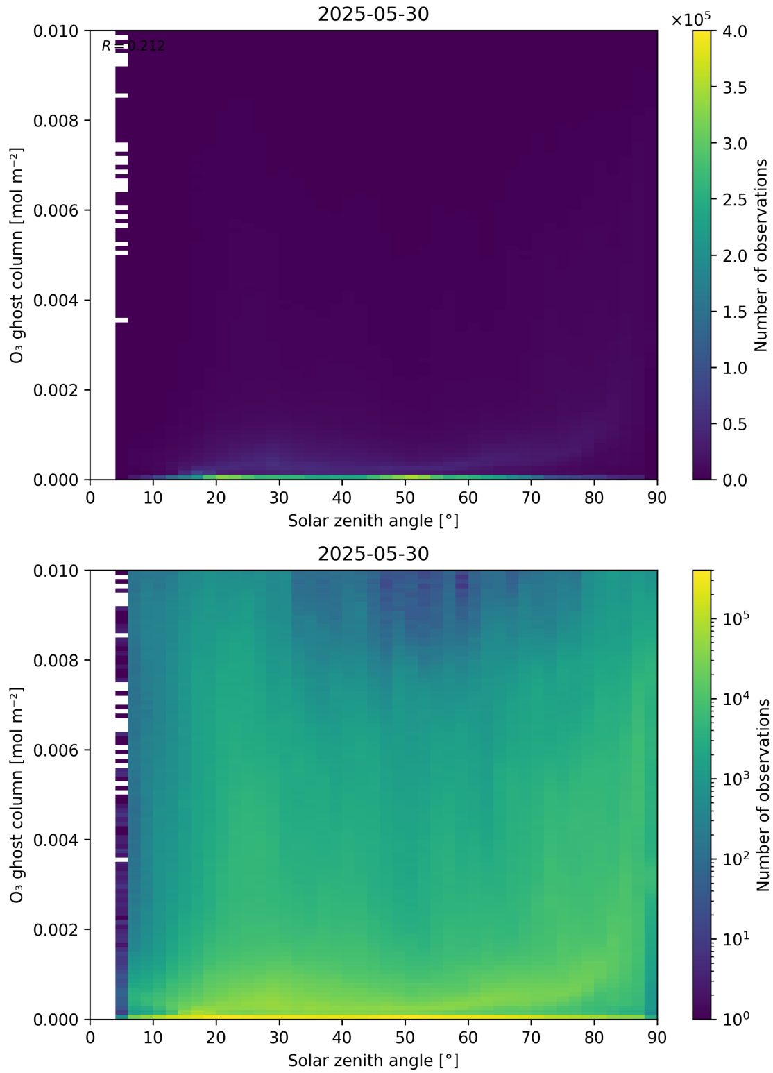
Figure 46: Scatter density plot of “Solar zenith angle” against “O 3 ghost column” for 2025-05-29 to 2025-05-31.
