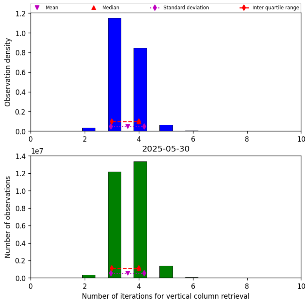
Figure 26: Histogram of “Number of iterations for vertical column retrieval” for 2025-05-29 to 2025-05-31
