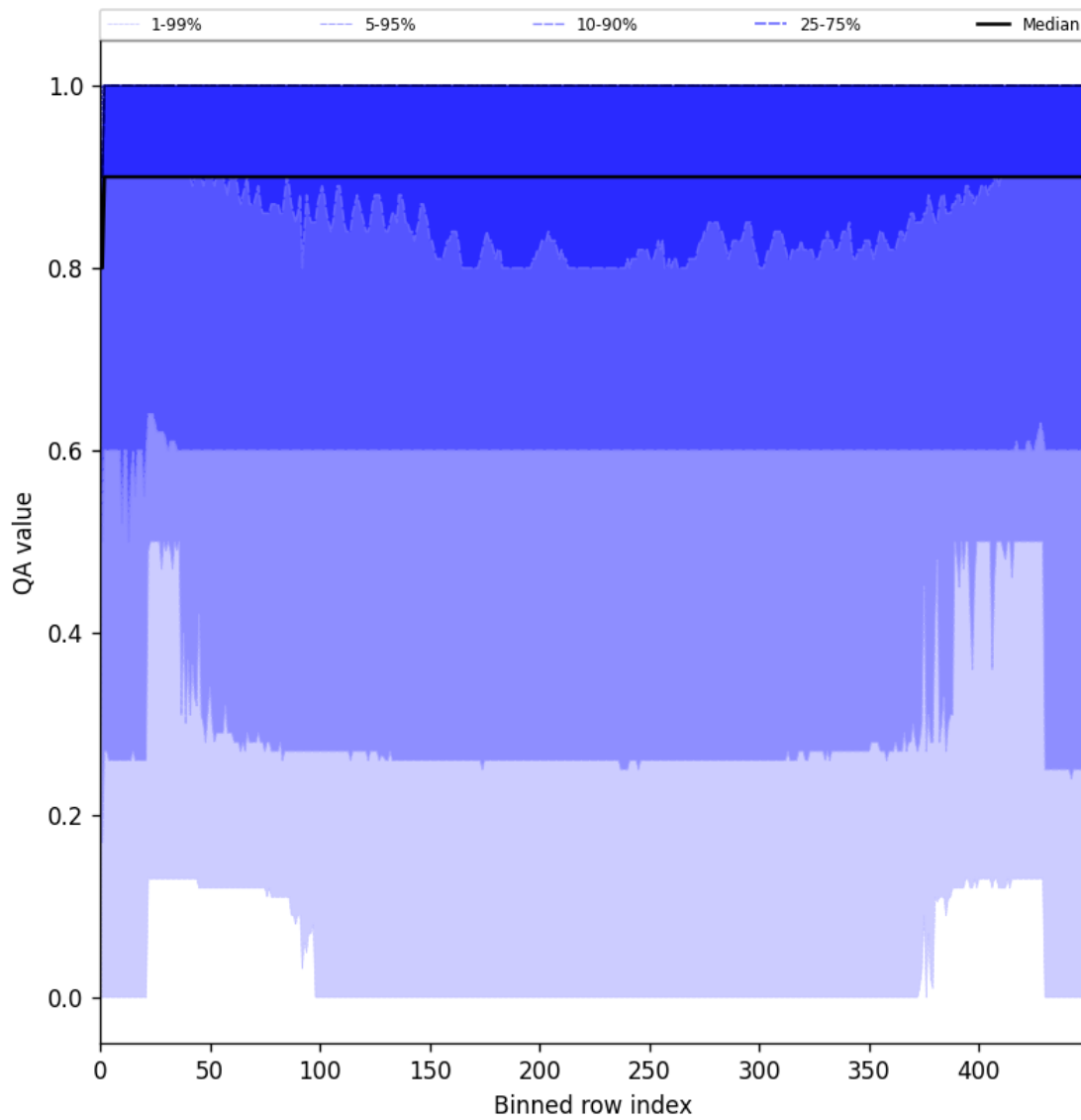
Figure 27: Along track statistics of “QA value” for 2025-05-29 to 2025-05-31
