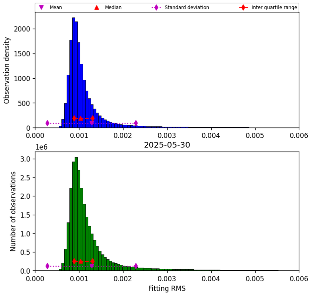
Figure 23: Histogram of “Fitting RMS” for 2025-05-29 to 2025-05-31
