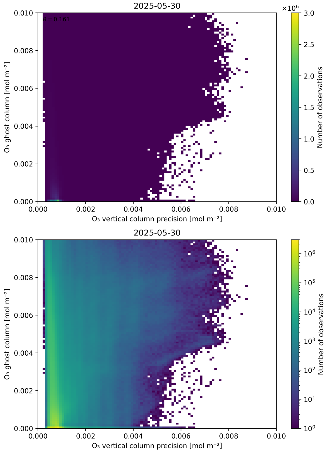
Figure 43: Scatter density plot of “ \text{O}_3 vertical column precision” against “ \text{O}_3 ghost column” for 2025-05-29 to 2025-05-31.
