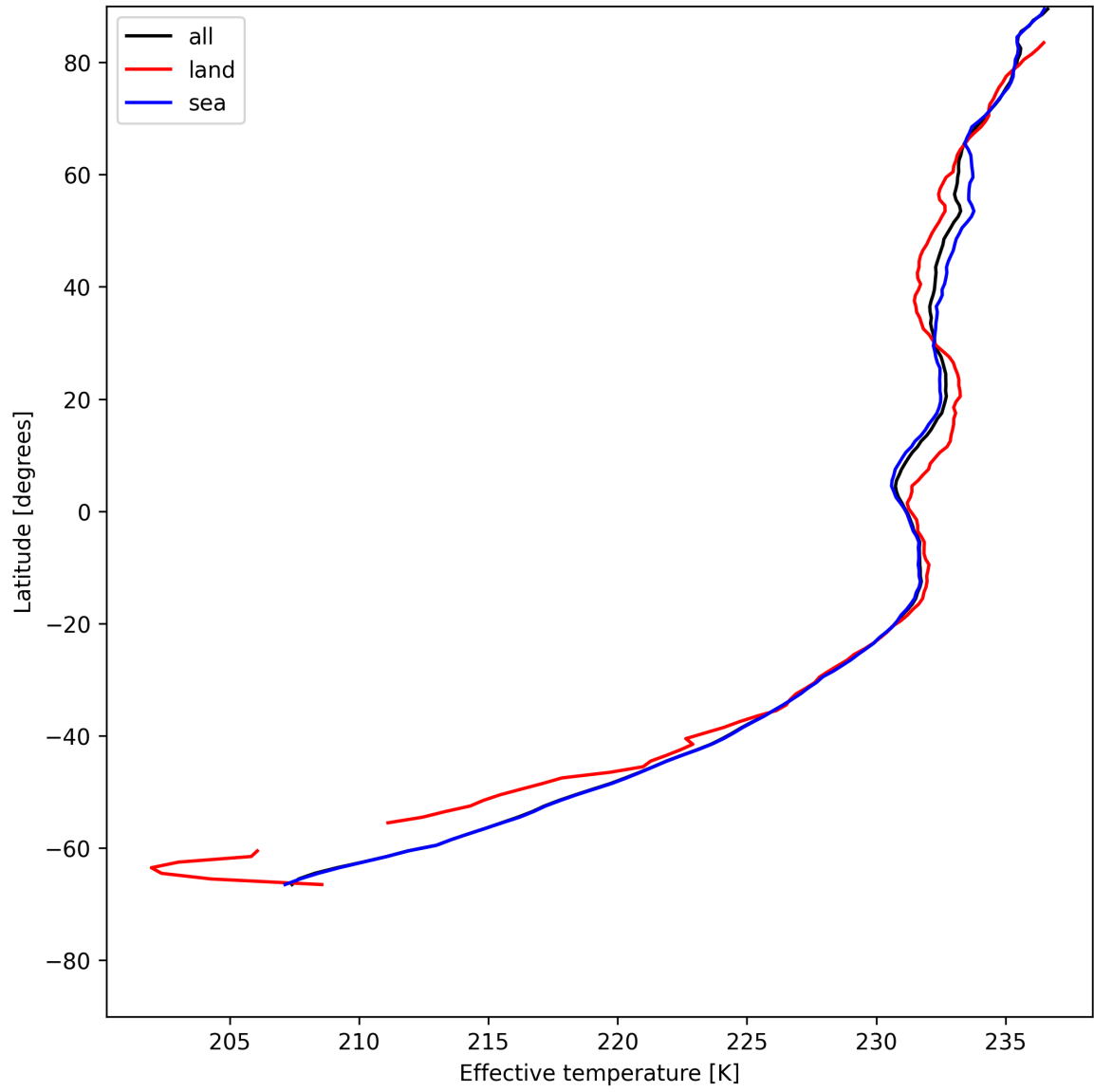
Figure 17: Zonal average of "Effective temperature" for 2025-05-29 to 2025-05-31.
