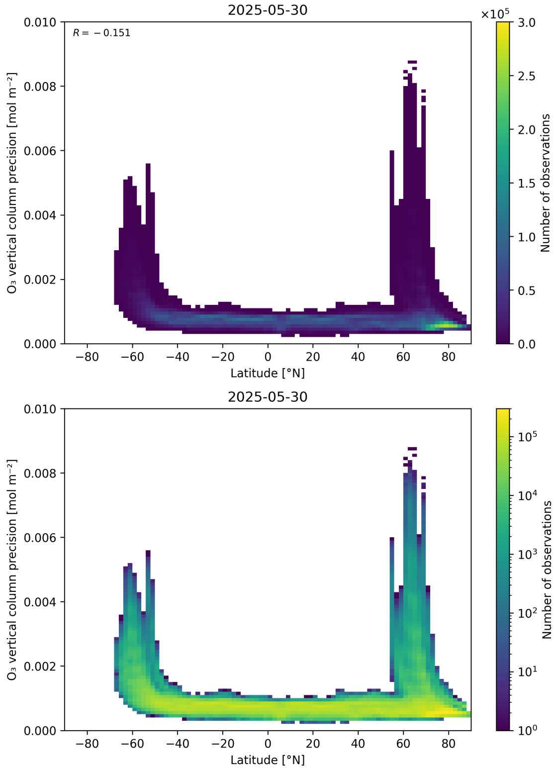
Figure 37: Scatter density plot of “Latitude” against “O 3 vertical column precision” for 2025-05-29 to 2025-05-31.
