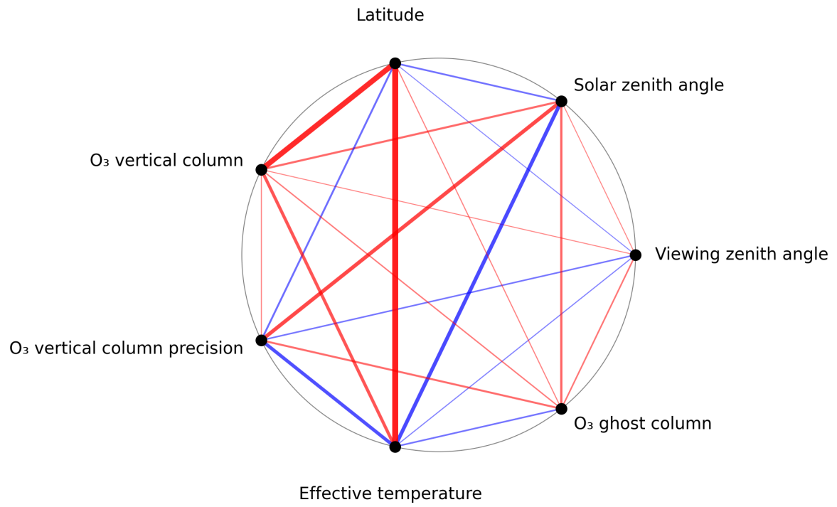
Figure 1: Map of correlation graph for 2025-05-29 to 2025-05-31.
