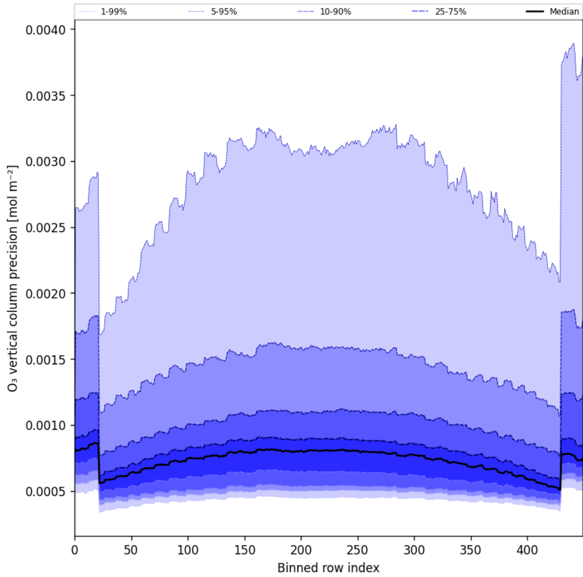
Figure 29: Along track statistics of “O 3 vertical column precision” for 2025-05-31 to 2025-06-01
