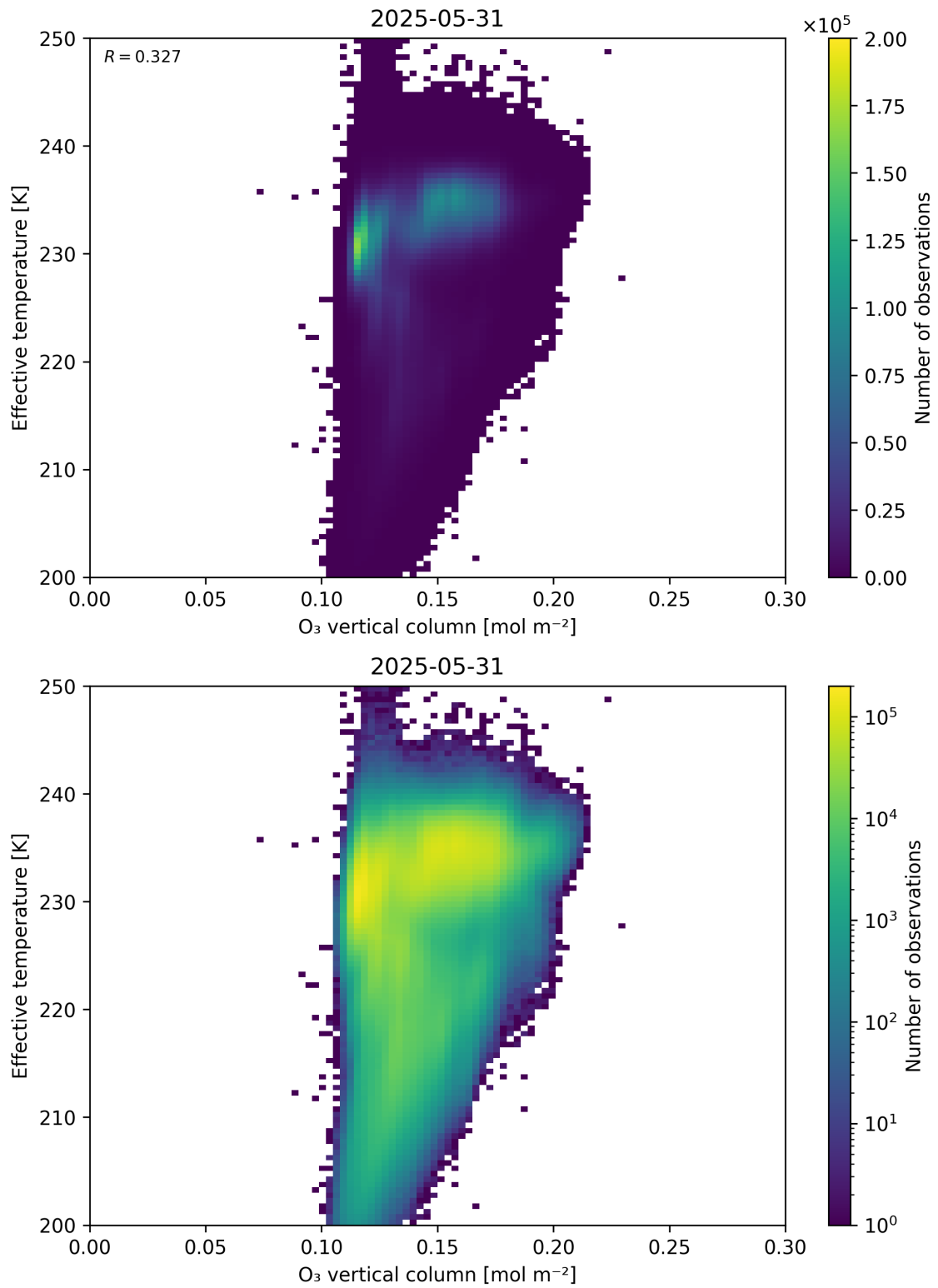
Figure 39: Scatter density plot of “O 3 vertical column” against “Effective temperature” for 2025-05-31 to 2025-06-01.
