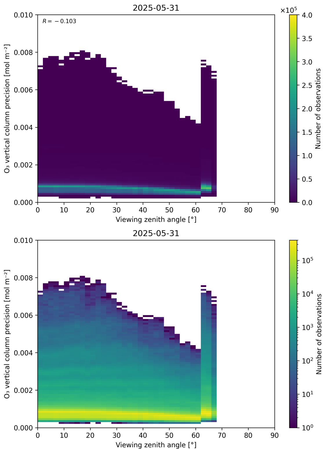
Figure 53: Scatter density plot of “Viewing zenith angle” against “O 3 vertical column precision” for 2025-05-31 to 2025-06-01.
