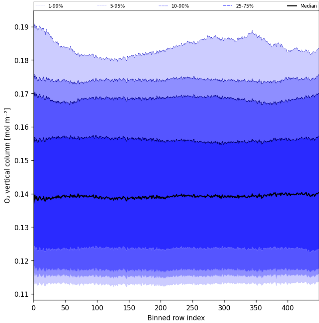
Figure 28: Along track statistics of “O 3 vertical column” for 2025-05-31 to 2025-06-01
