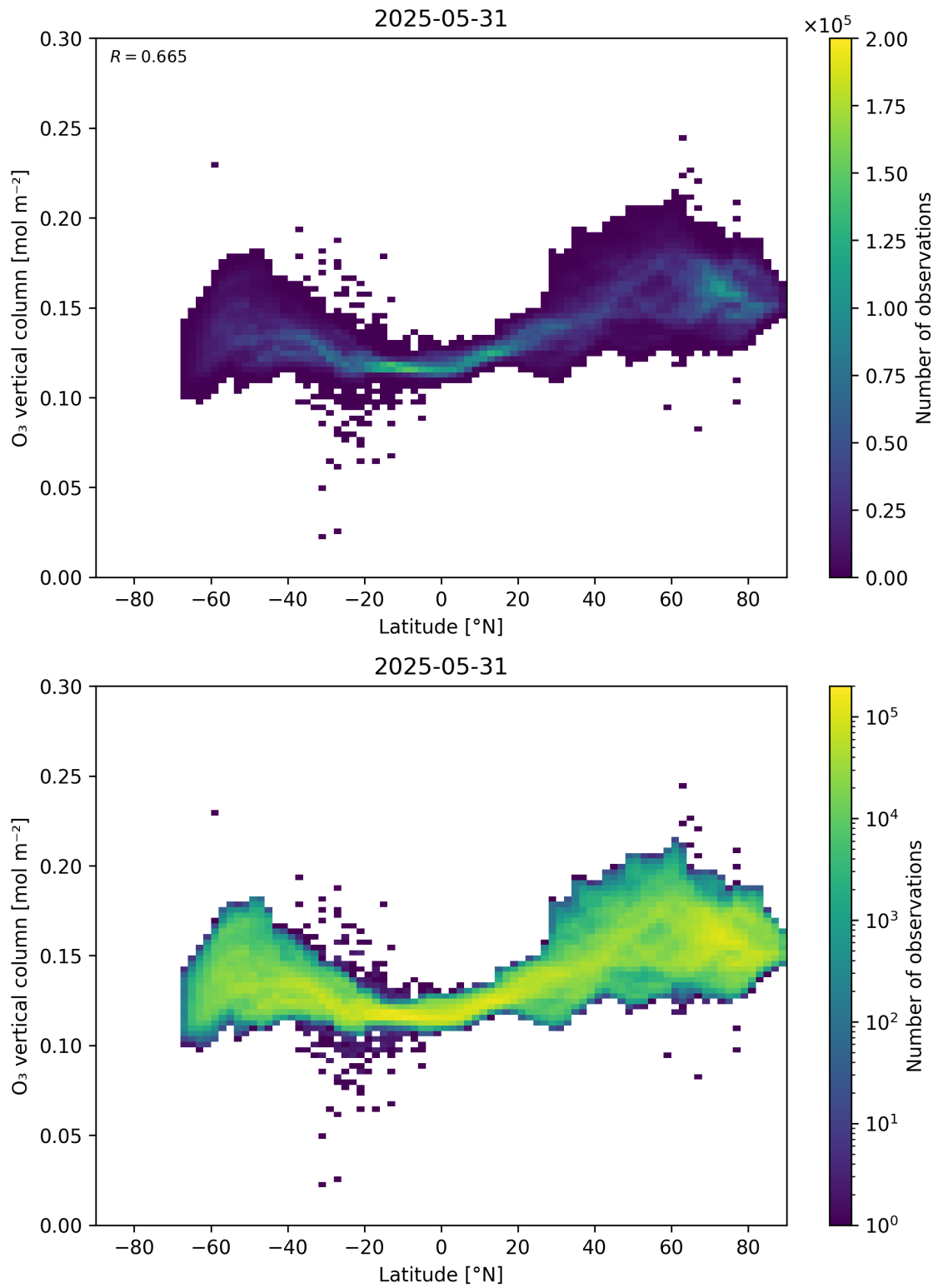
Figure 36: Scatter density plot of “Latitude” against “O 3 vertical column” for 2025-05-31 to 2025-06-01.
