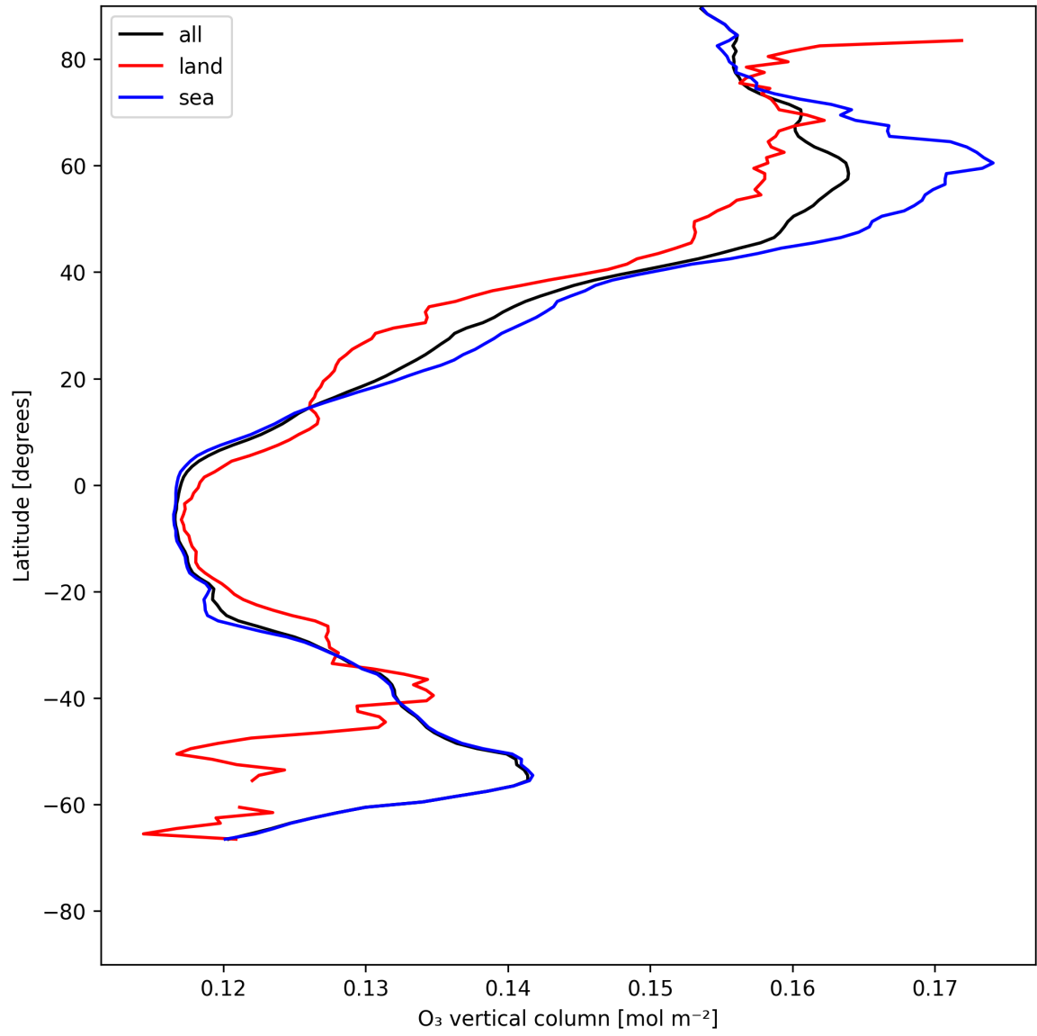
Figure 14: Zonal average of “O 3 vertical column” for 2025-05-31 to 2025-06-01.
