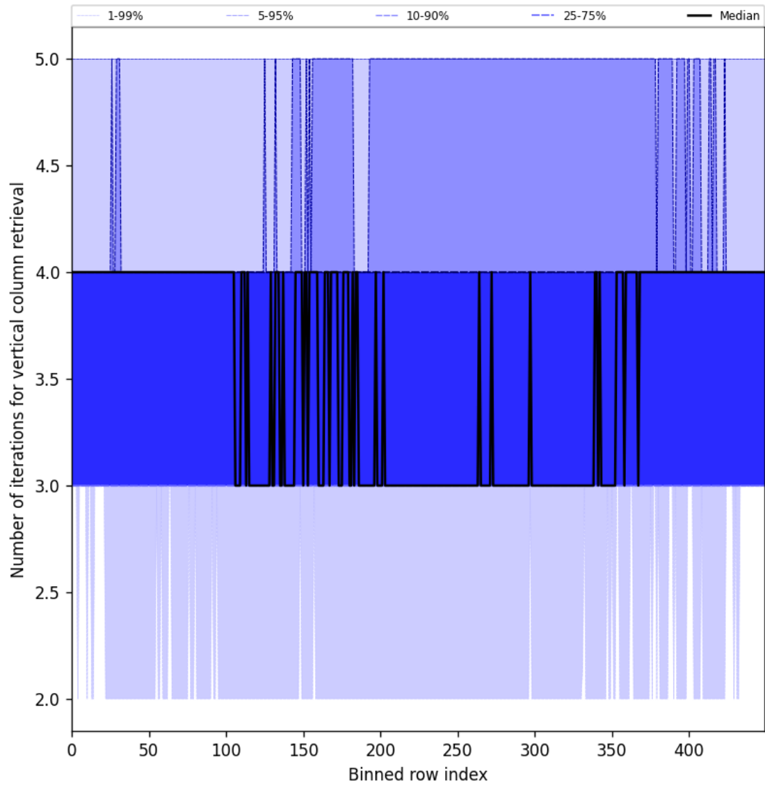
Figure 33: Along track statistics of “Number of iterations for vertical column retrieval” for 2025-05-31 to 2025-06-01
