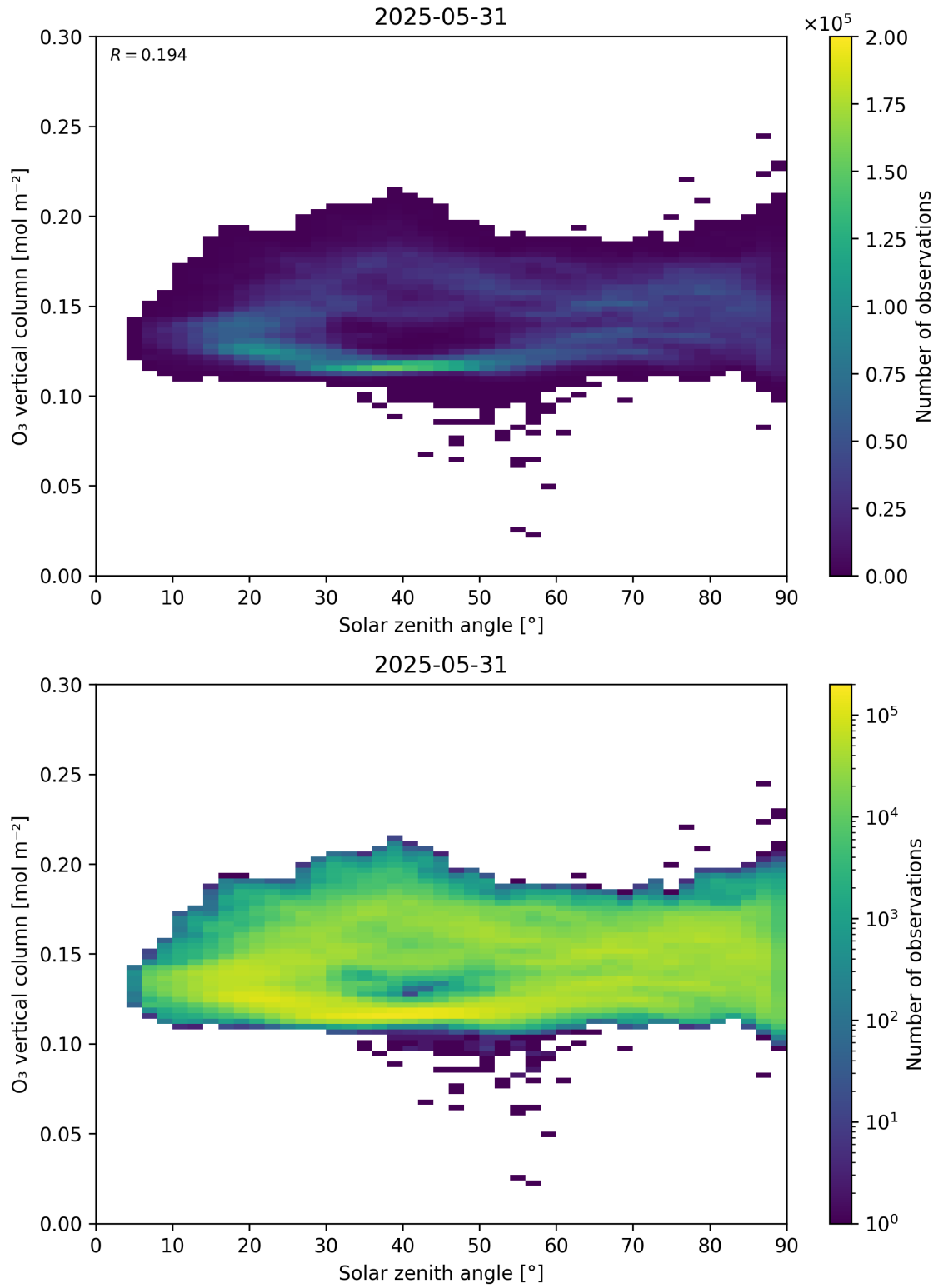
Figure 47: Scatter density plot of “Solar zenith angle” against “O 3 vertical column” for 2025-05-31 to 2025-06-01.
