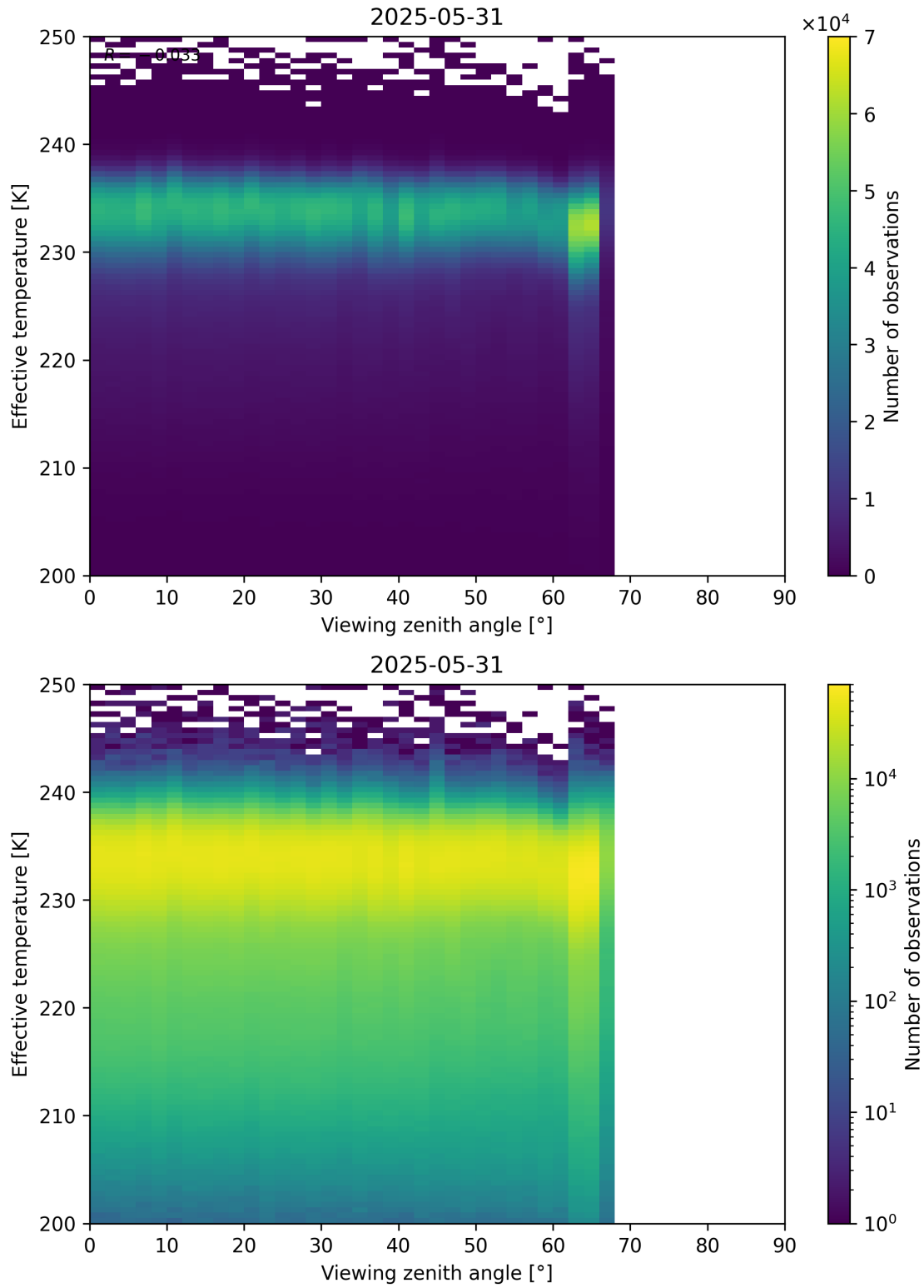
Figure 50: Scatter density plot of “Viewing zenith angle” against “Effective temperature” for 2025-05-31 to 2025-06-01.
