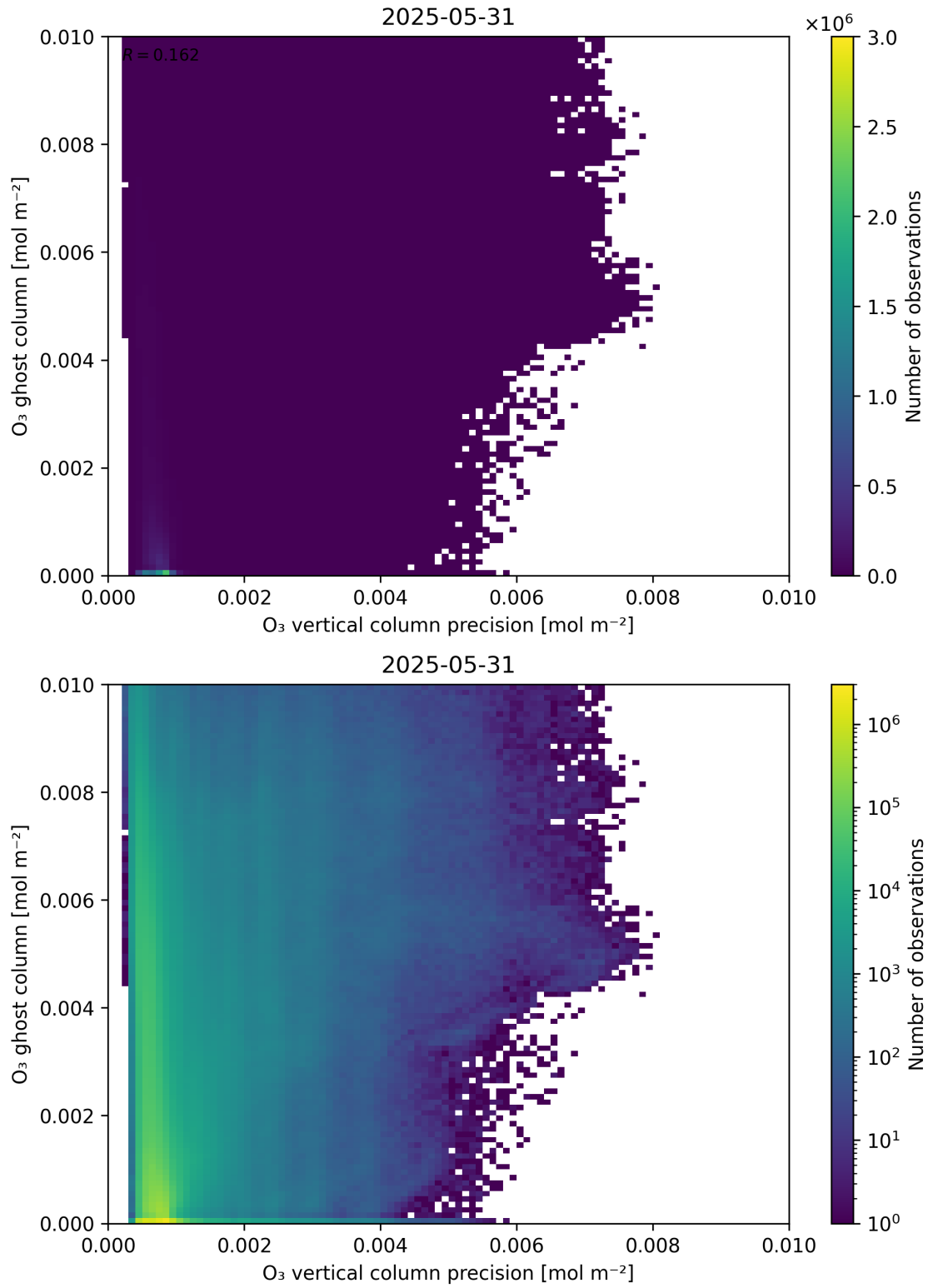
Figure 43: Scatter density plot of “ \text{O}_3 vertical column precision” against “ \text{O}_3 ghost column” for 2025-05-31 to 2025-06-01.
