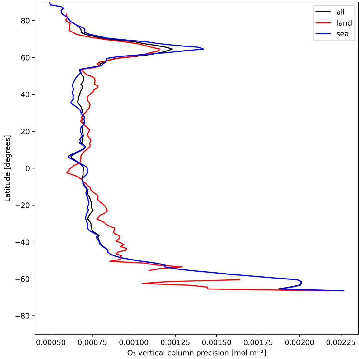
Figure 15: Zonal average of “O 3 vertical column precision” for 2025-05-31 to 2025-06-01.
