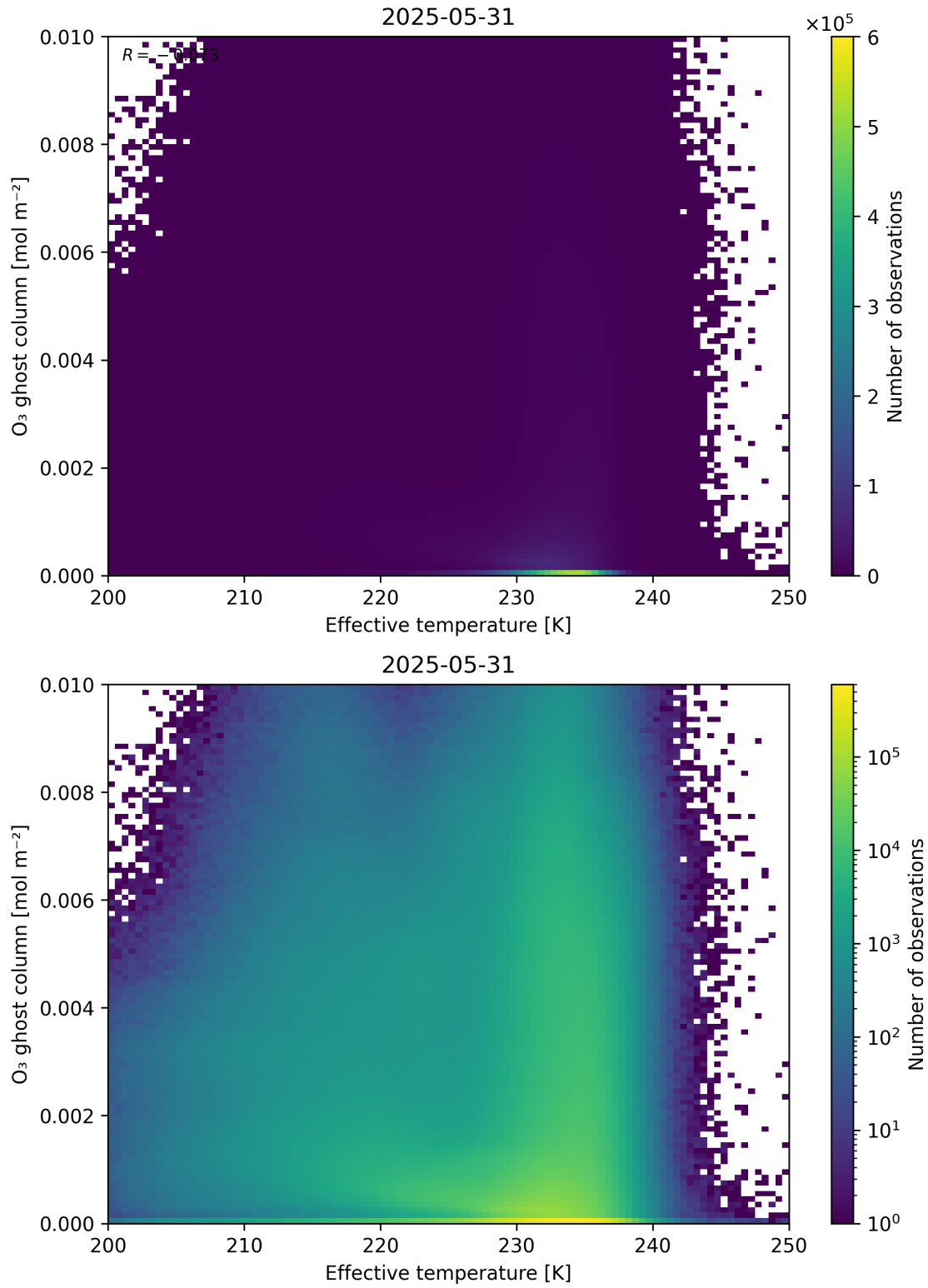
Figure 38: Scatter density plot of “Effective temperature” against “O 3 ghost column” for 2025-05-31 to 2025-06-01.
