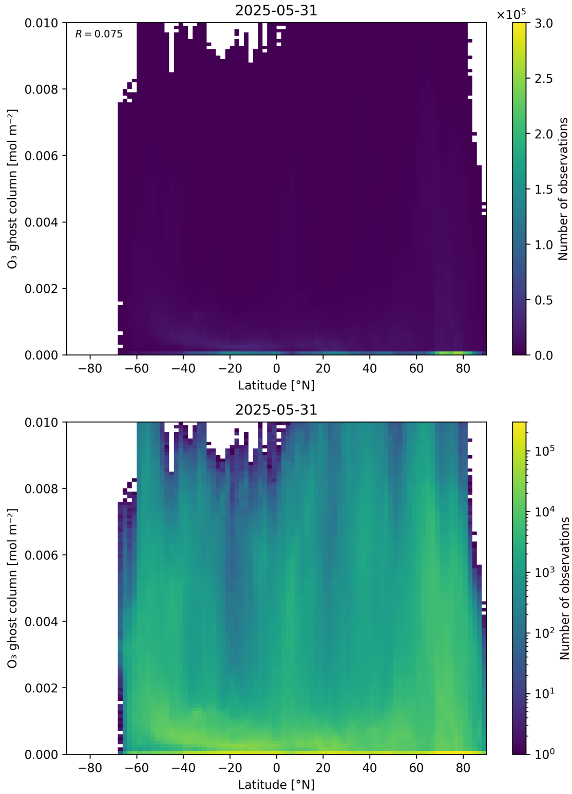
Figure 35: Scatter density plot of “Latitude” against “O 3 ghost column” for 2025-05-31 to 2025-06-01.
