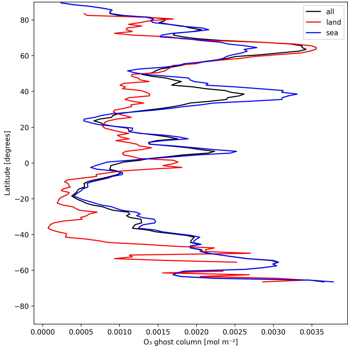
Figure 18: Zonal average of "O 3 ghost column" for 2025-05-31 to 2025-06-01.
