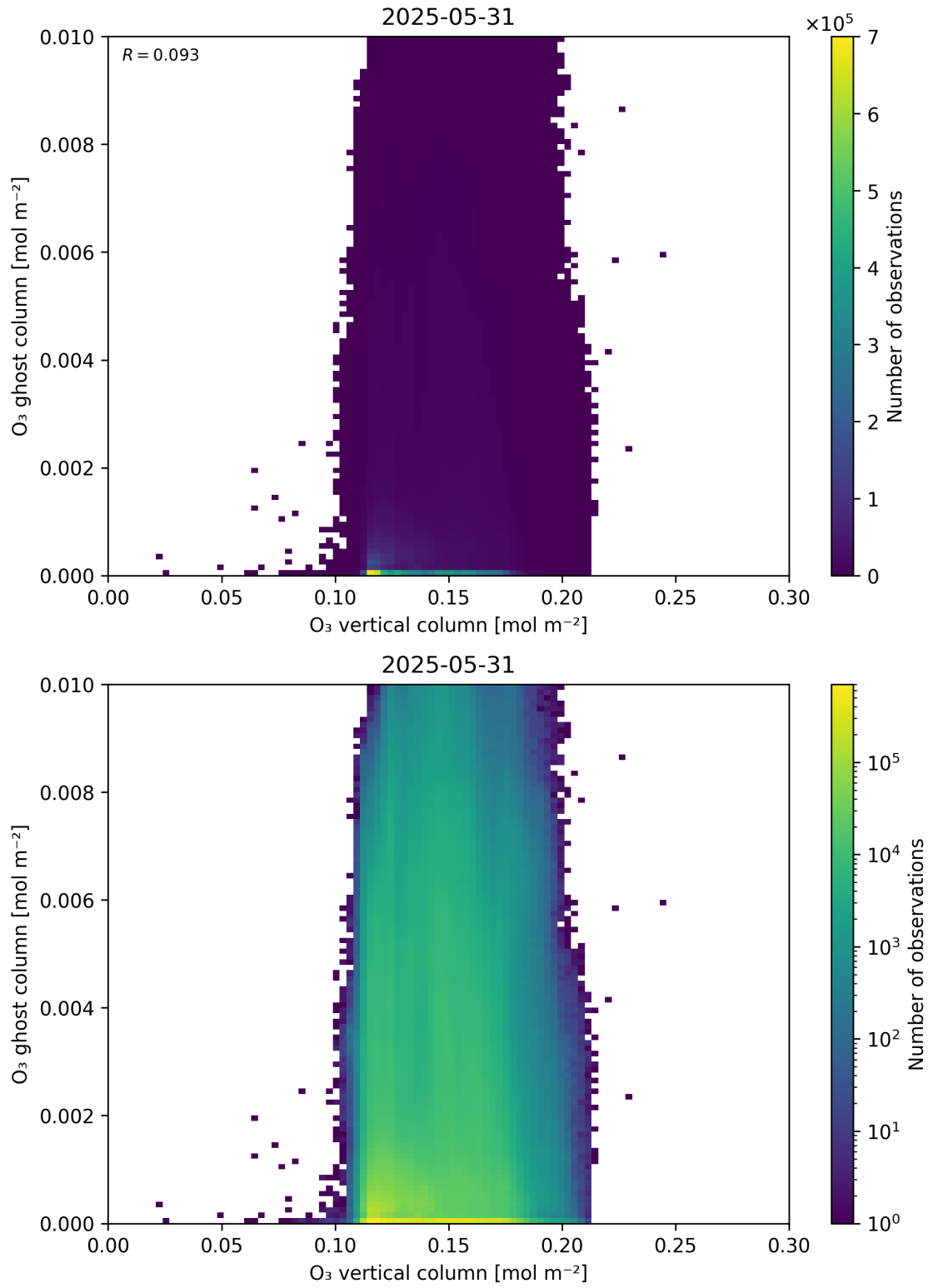
Figure 40: Scatter density plot of “O 3 vertical column” against “O 3 ghost column” for 2025-05-31 to 2025-06-01.
