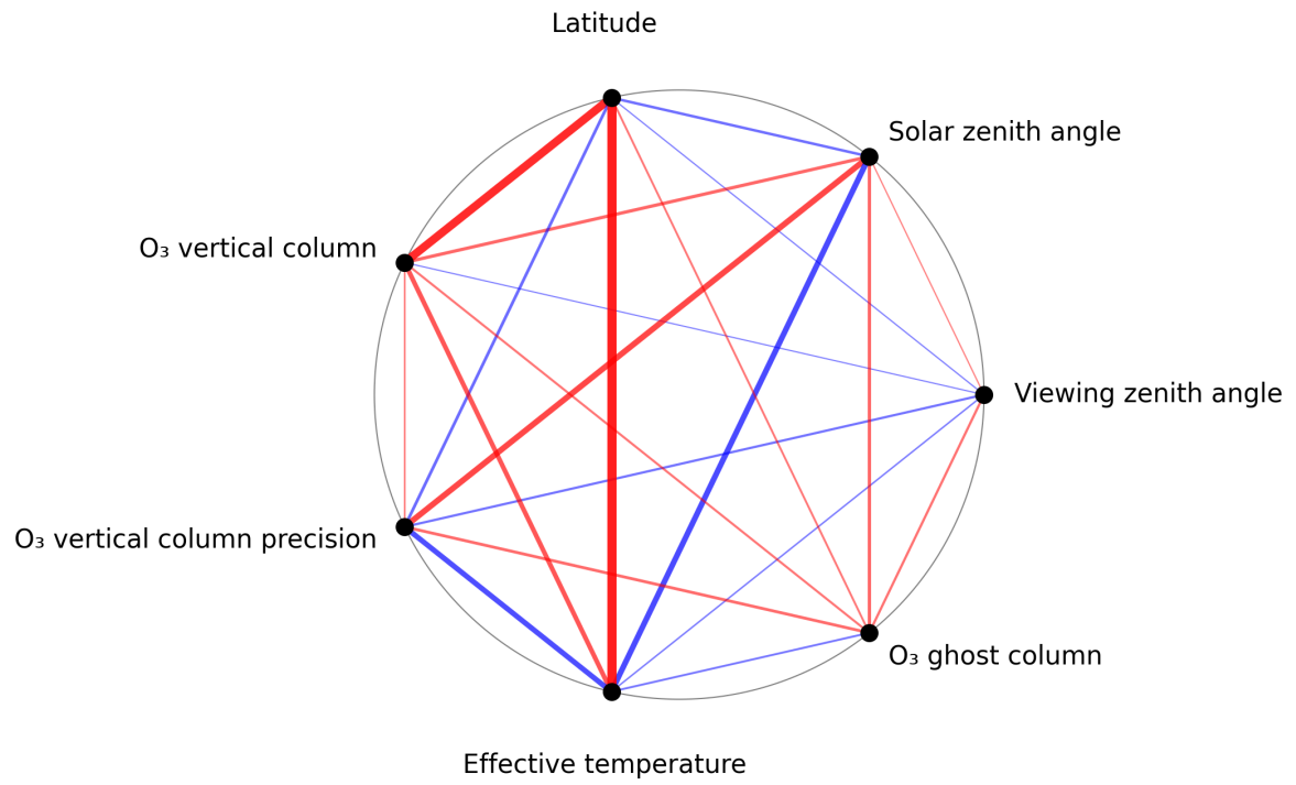
Figure 1: Map of correlation graph for 2025-05-31 to 2025-06-01.
