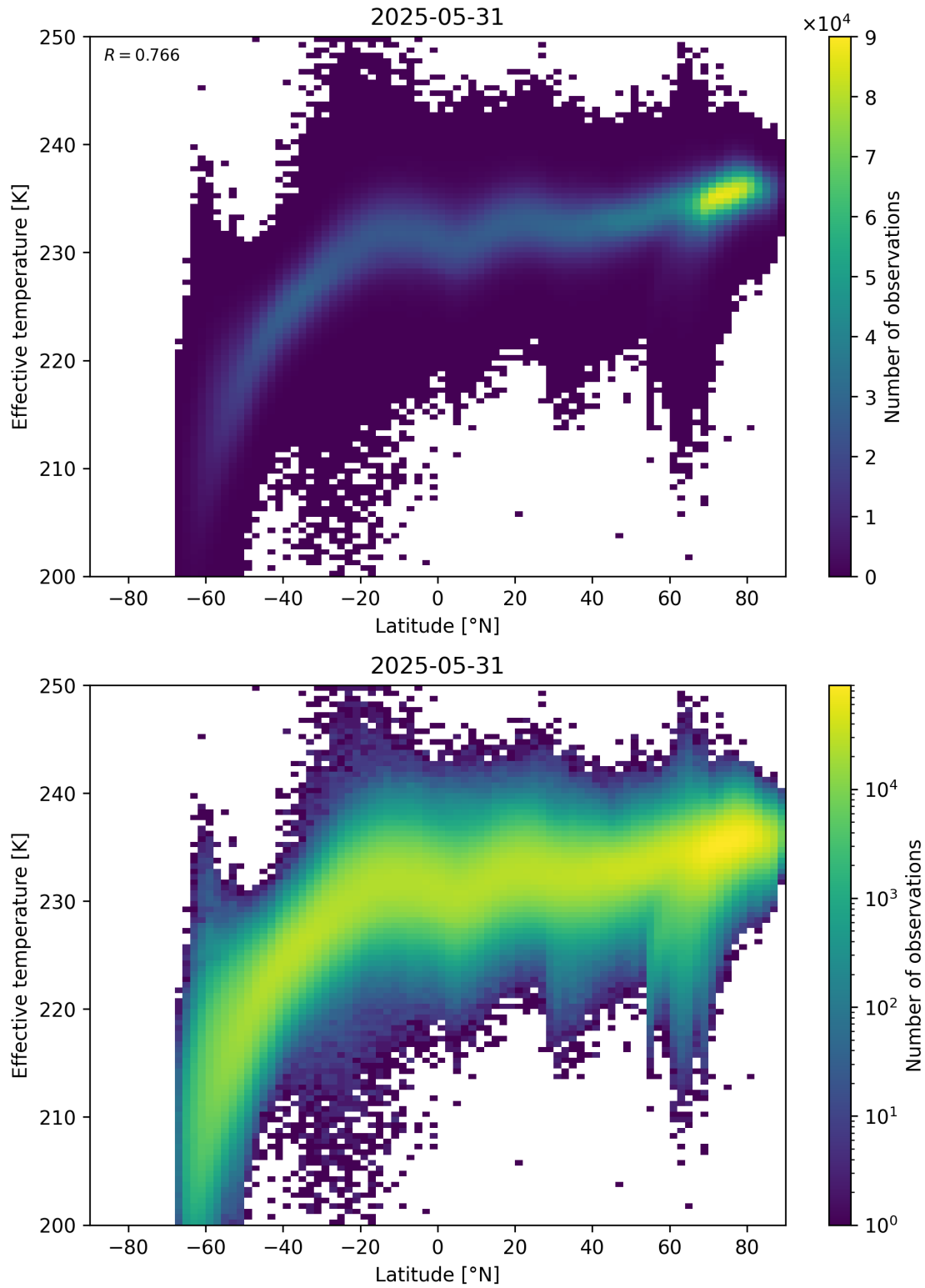
Figure 34: Scatter density plot of “Latitude” against “Effective temperature” for 2025-05-31 to 2025-06-01.
