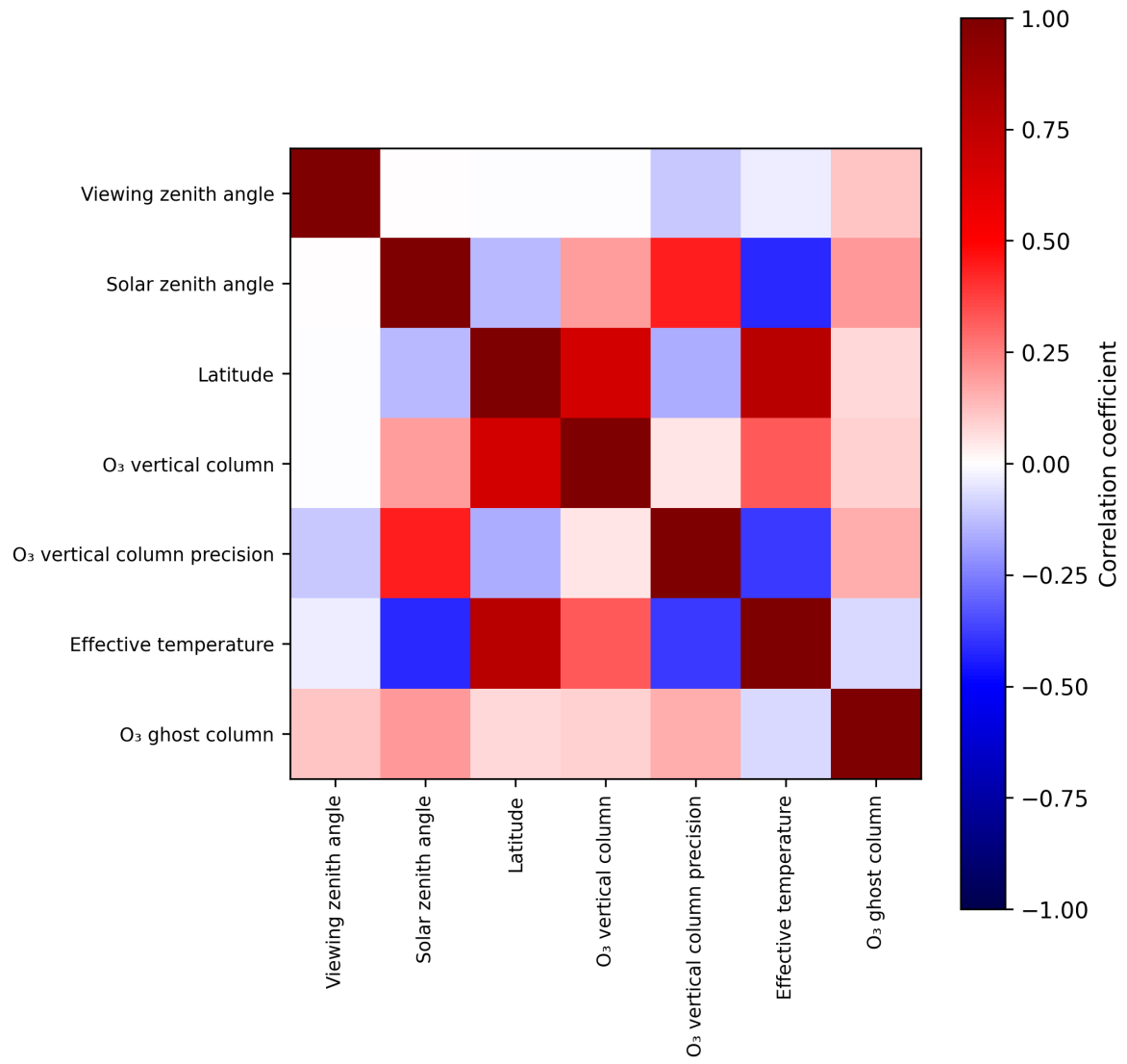
Figure 2: Map of correlation matrix for 2025-05-31 to 2025-06-01.
