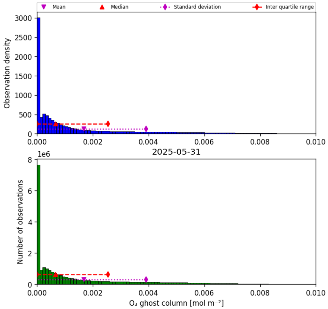
Figure 25: Histogram of “O 3 ghost column” for 2025-05-31 to 2025-06-01
