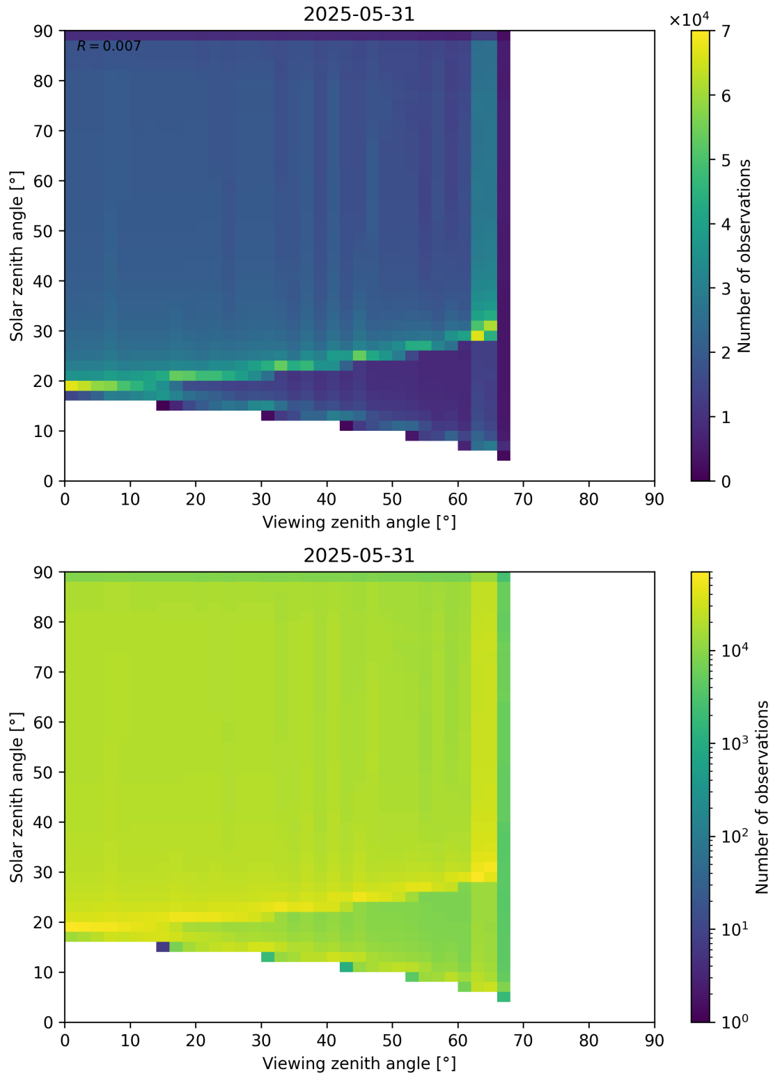
Figure 54: Scatter density plot of “Viewing zenith angle” against “Solar zenith angle” for 2025-05-31 to 2025-06-01.
