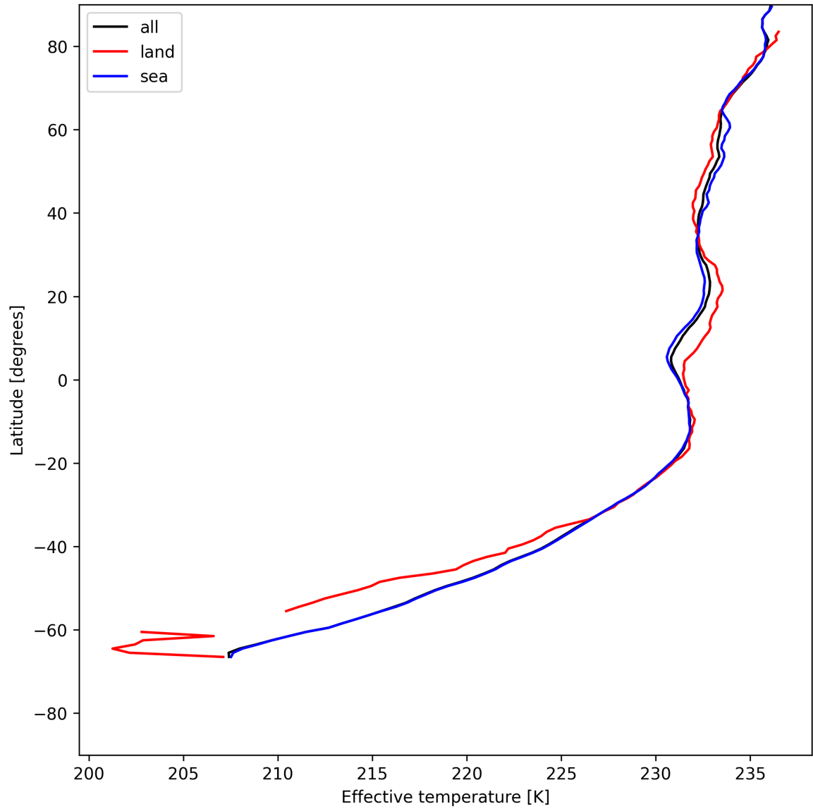
Figure 17: Zonal average of “Effective temperature” for 2025-05-31 to 2025-06-01.
