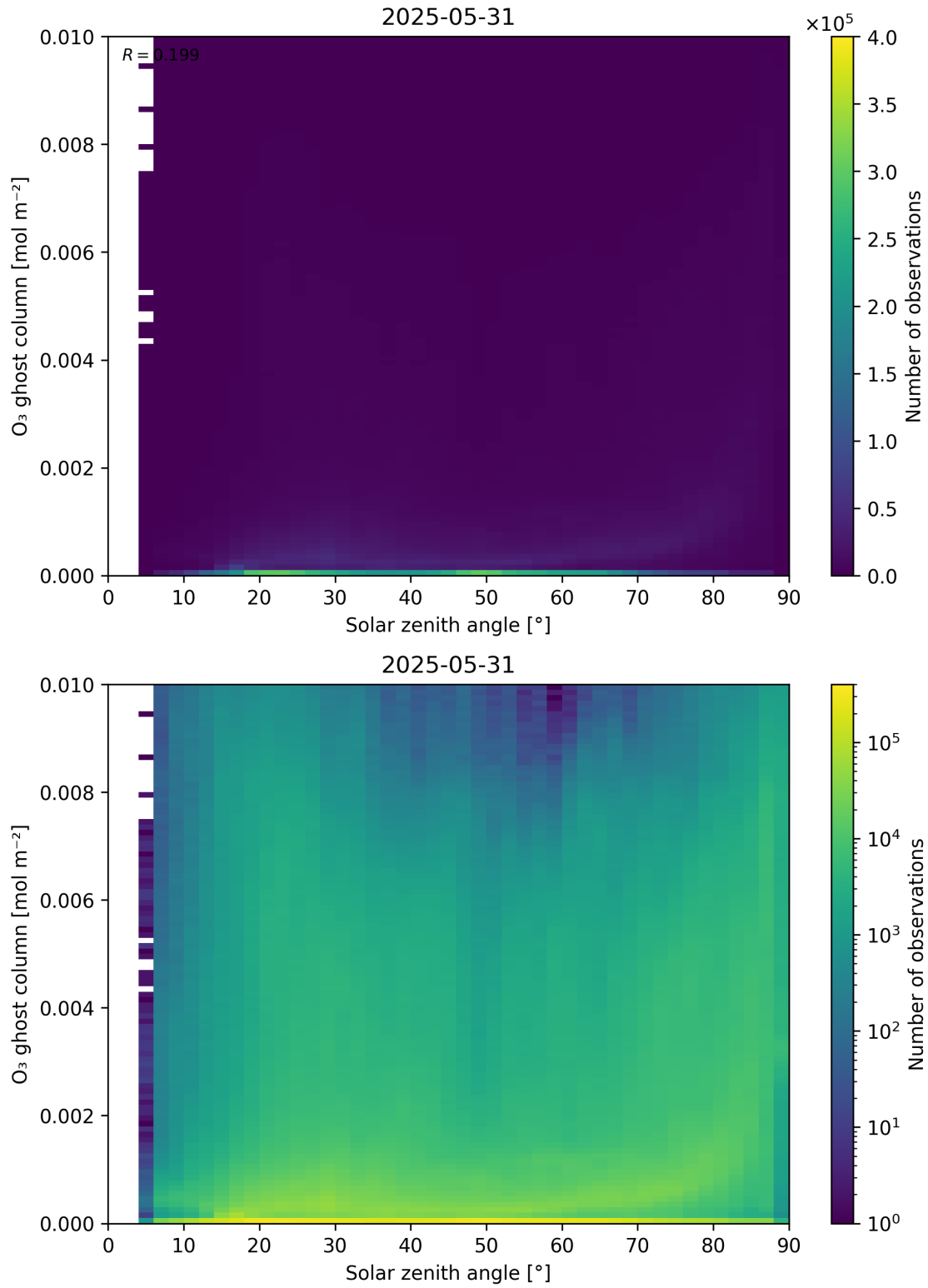
Figure 46: Scatter density plot of “Solar zenith angle” against “O 3 ghost column” for 2025-05-31 to 2025-06-01.
