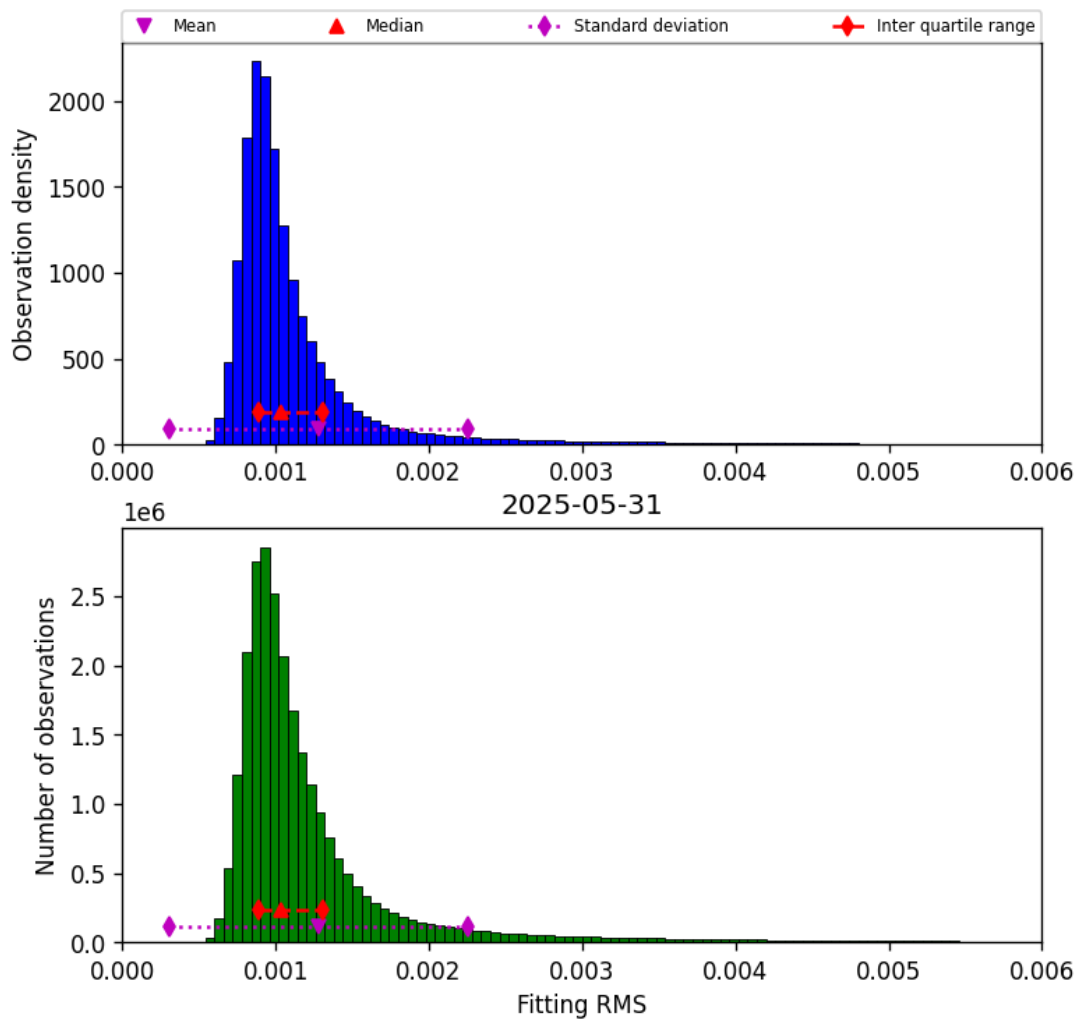
Figure 23: Histogram of “Fitting RMS” for 2025-05-31 to 2025-06-01
