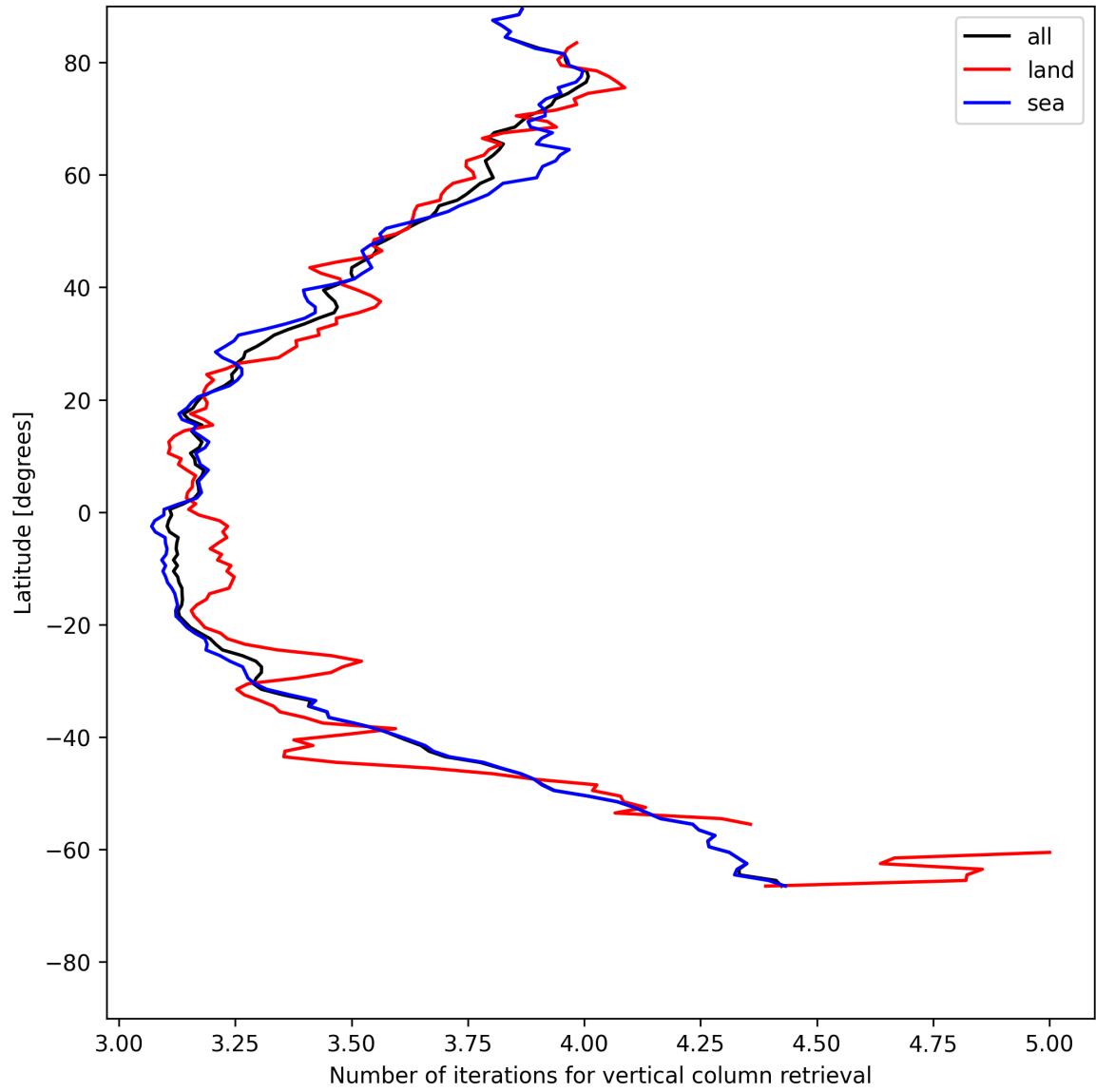
Figure 19: Zonal average of “Number of iterations for vertical column retrieval” for 2025-05-31 to 2025-06-01.
