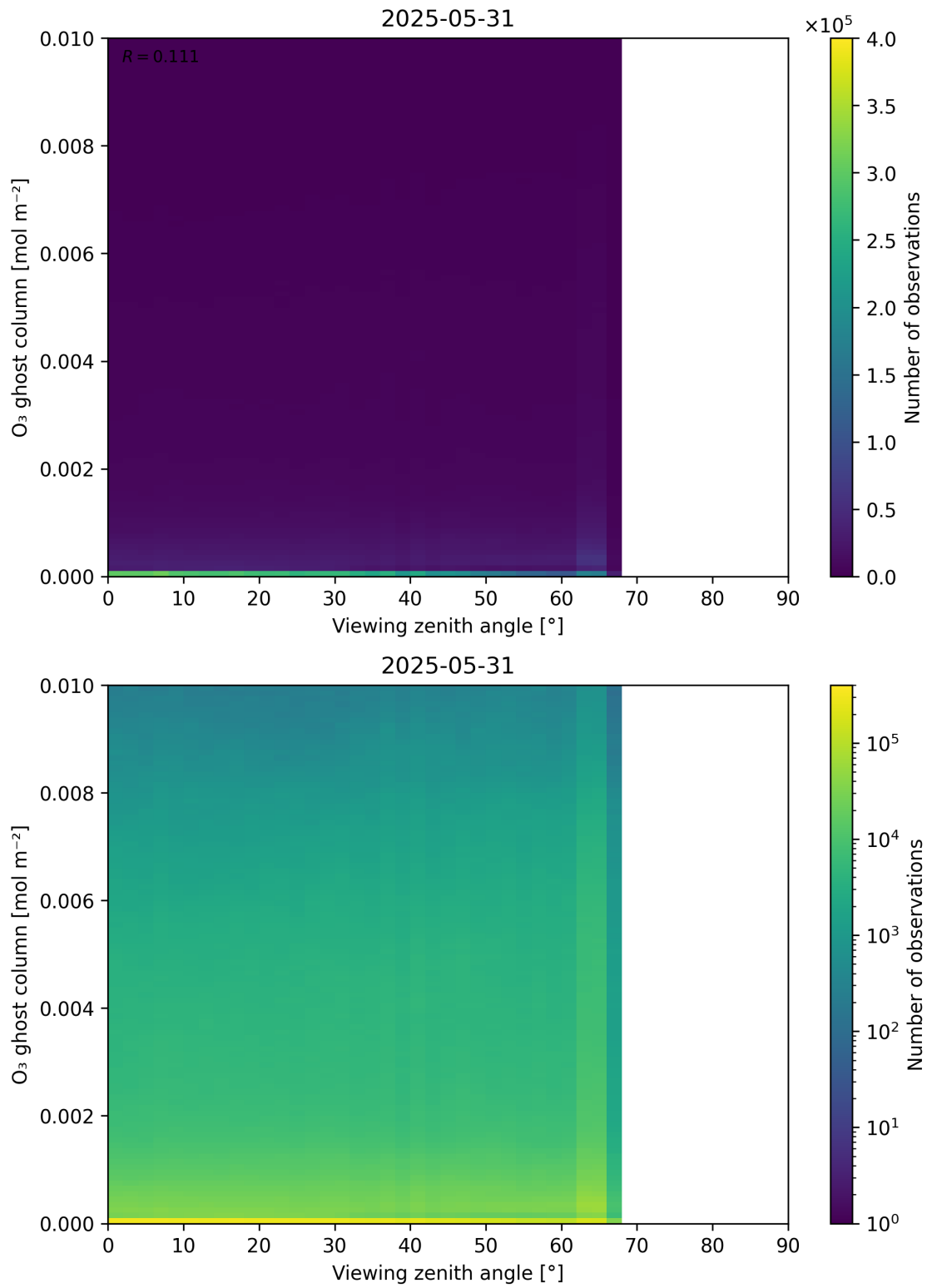
Figure 51: Scatter density plot of “Viewing zenith angle” against “O 3 ghost column” for 2025-05-31 to 2025-06-01.
