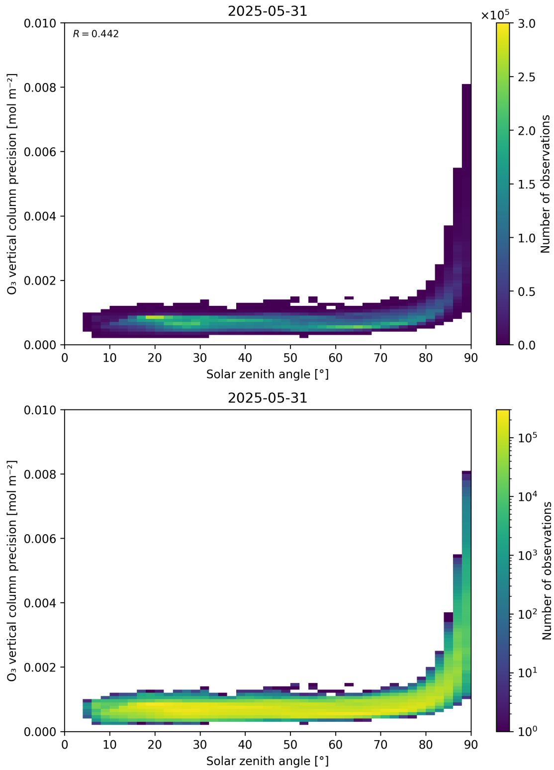
Figure 48: Scatter density plot of “Solar zenith angle” against “O 3 vertical column precision” for 2025-05-31 to 2025-06-01.
