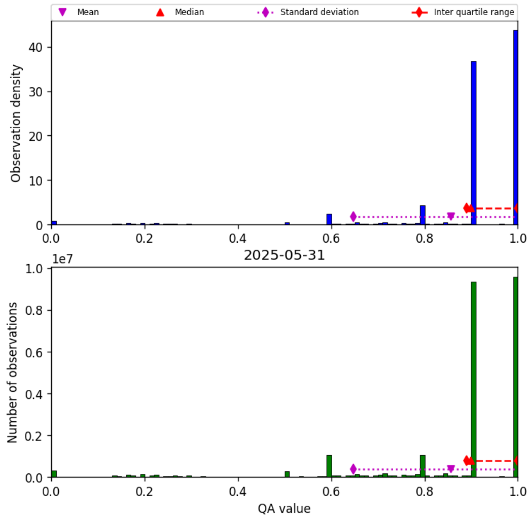
Figure 20: Histogram of “QA value” for 2025-05-31 to 2025-06-01
