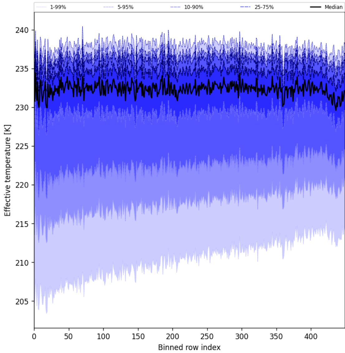
Figure 31: Along track statistics of “Effective temperature” for 2025-05-31 to 2025-06-01
