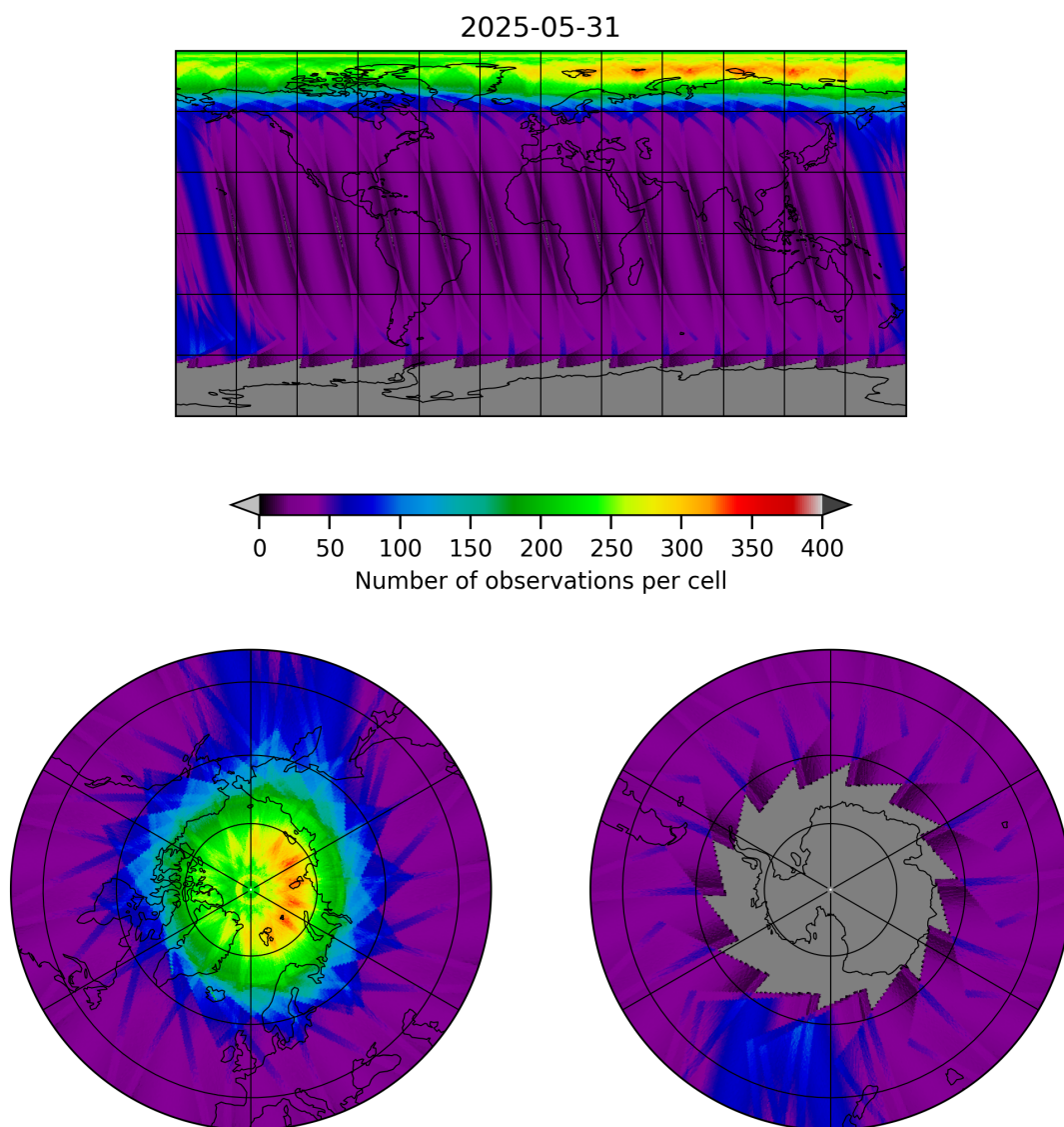
Figure 12: Map of the number of observations for 2025-05-31 to 2025-06-01
