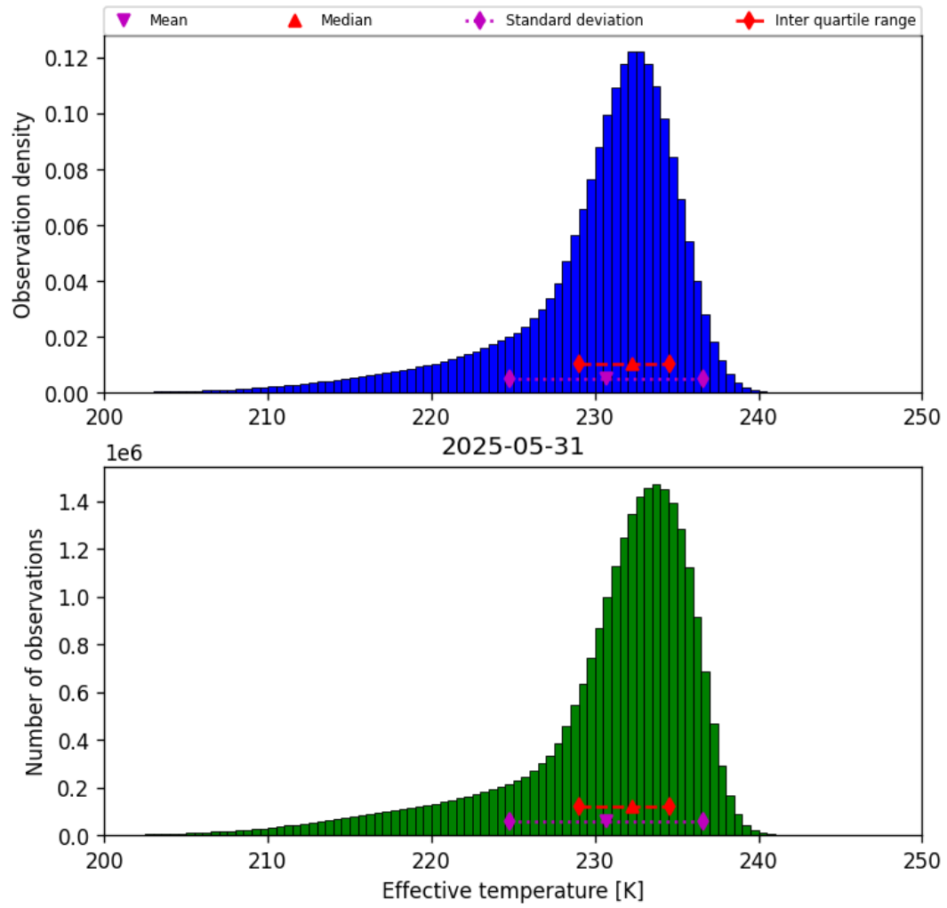
Figure 24: Histogram of “Effective temperature” for 2025-05-31 to 2025-06-01
