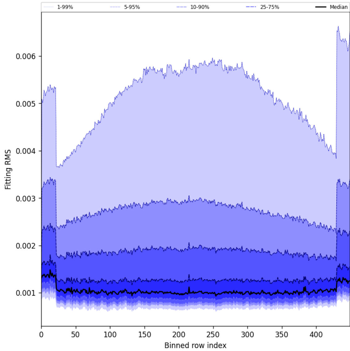
Figure 30: Along track statistics of “Fitting RMS” for 2025-05-31 to 2025-06-01
