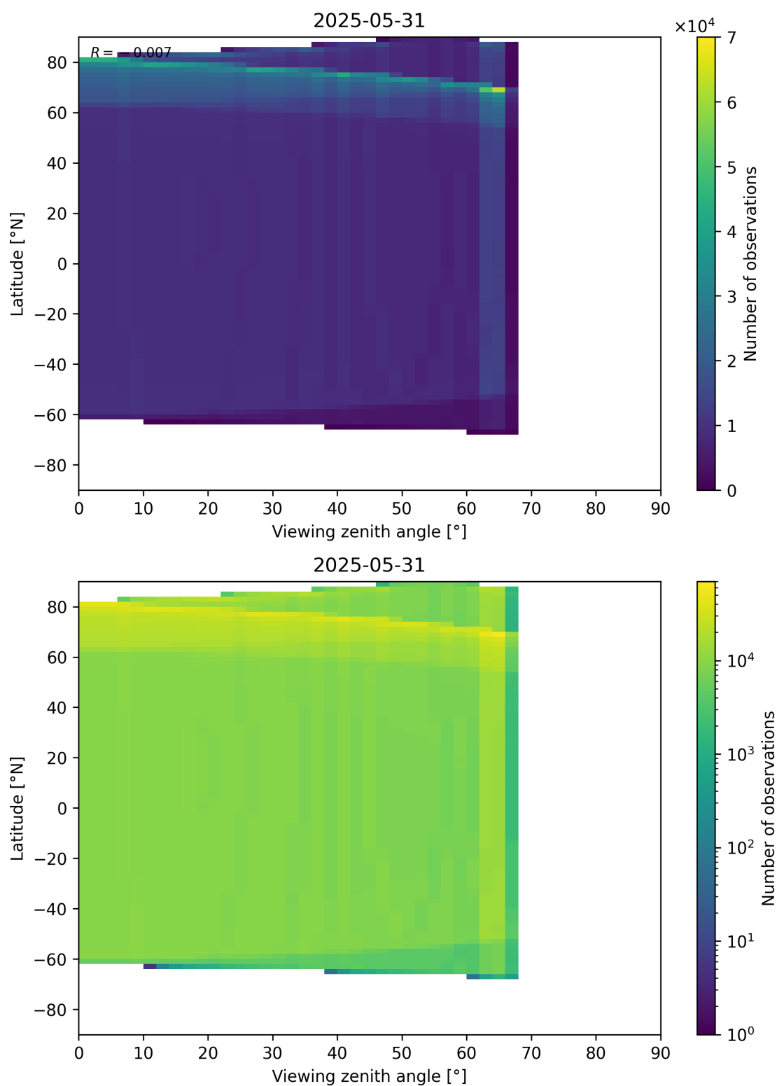
Figure 49: Scatter density plot of “Viewing zenith angle” against “Latitude” for 2025-05-31 to 2025-06-01.
