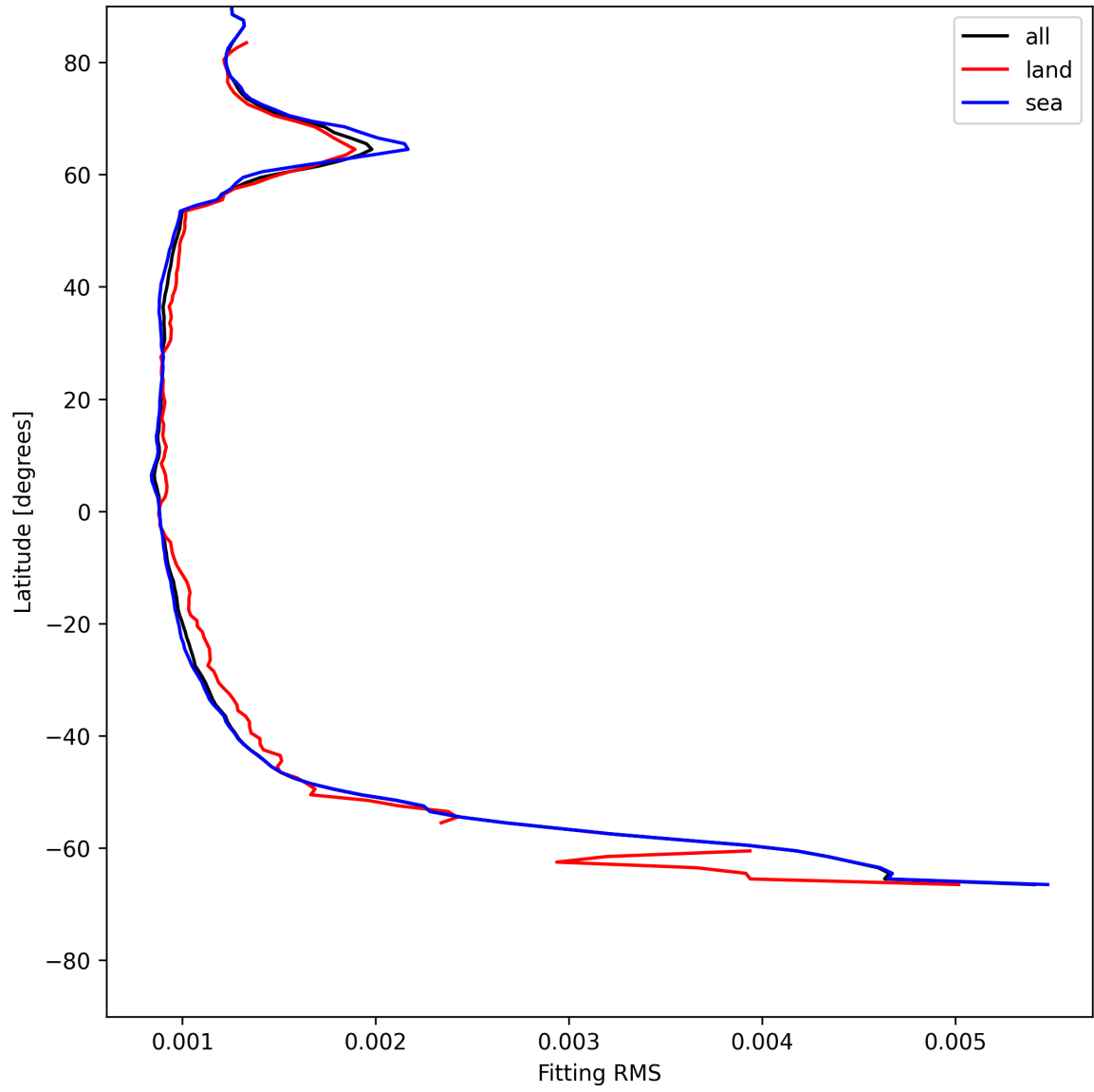
Figure 16: Zonal average of “Fitting RMS” for 2025-05-31 to 2025-06-01.
