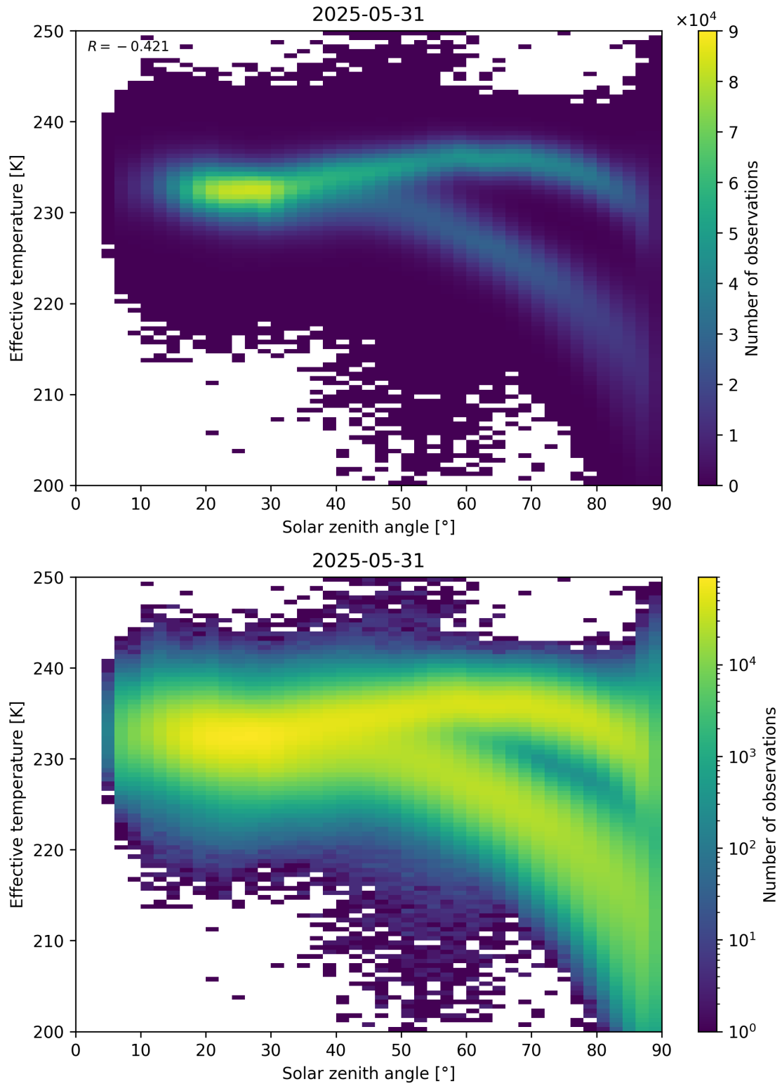
Figure 45: Scatter density plot of “Solar zenith angle” against “Effective temperature” for 2025-05-31 to 2025-06-01.
