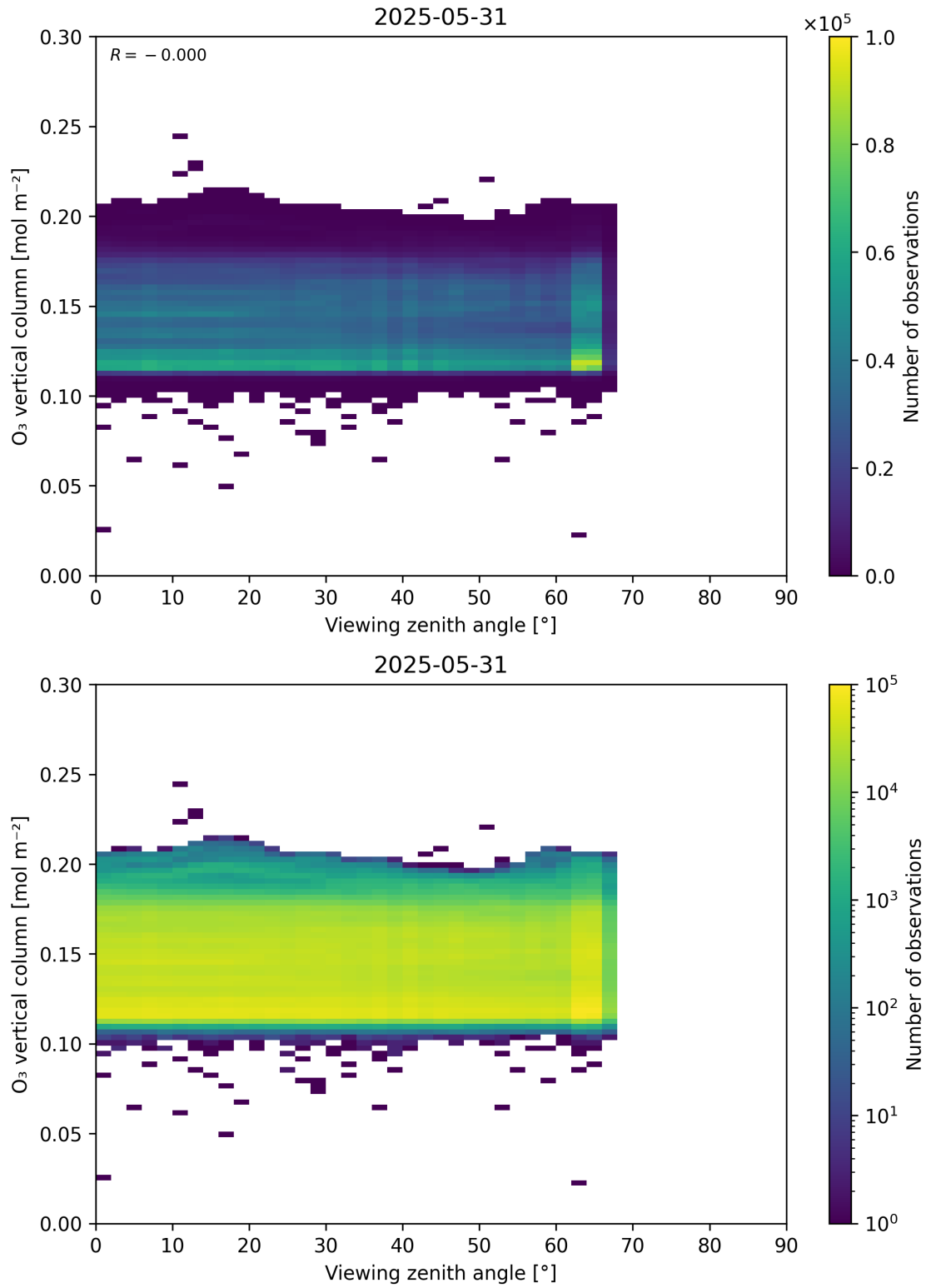
Figure 52: Scatter density plot of “Viewing zenith angle” against “O 3 vertical column” for 2025-05-31 to 2025-06-01.
