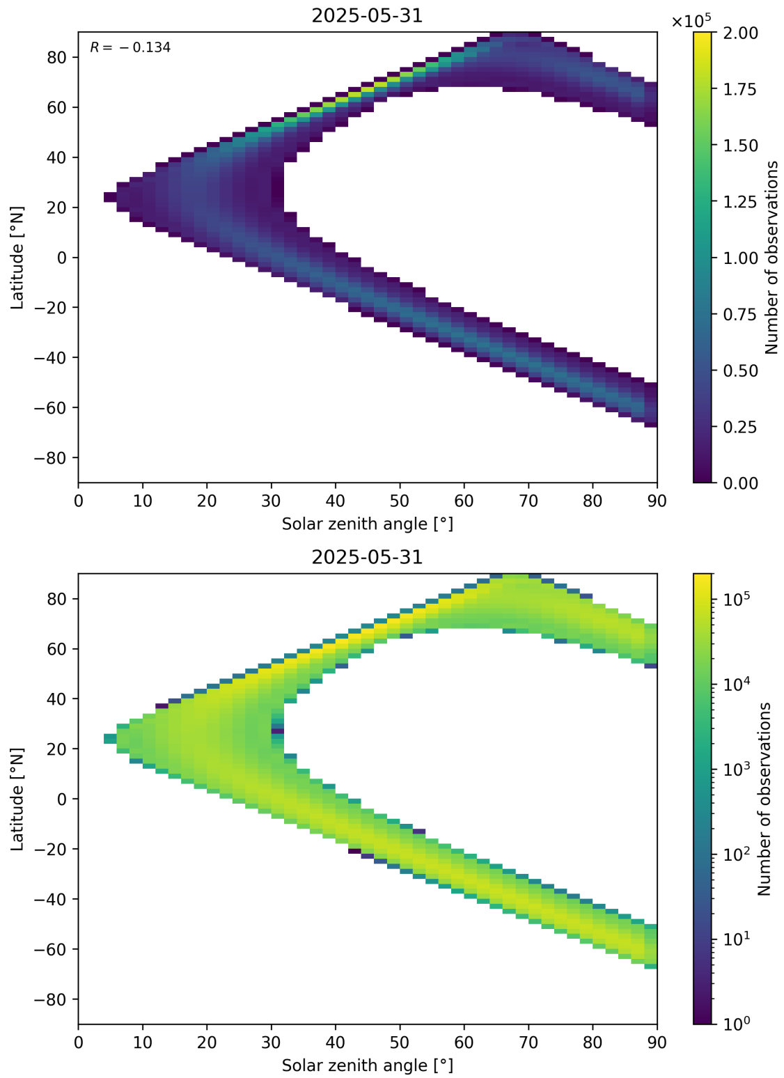
Figure 44: Scatter density plot of “Solar zenith angle” against “Latitude” for 2025-05-31 to 2025-06-01.
