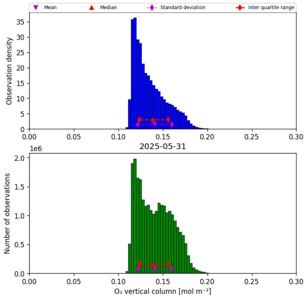
Figure 21: Histogram of “O 3 vertical column” for 2025-05-31 to 2025-06-01
