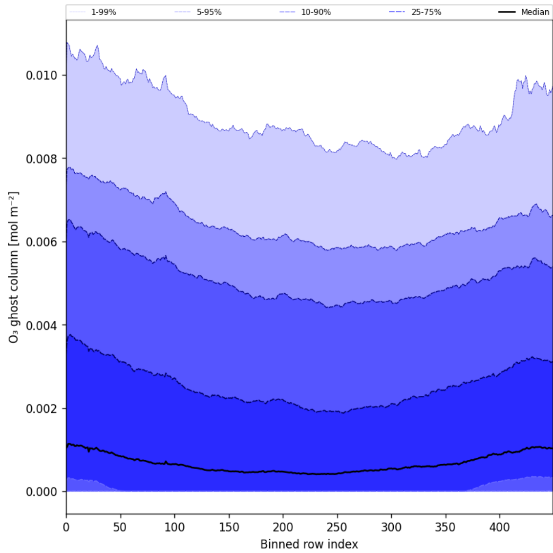
Figure 32: Along track statistics of “O 3 ghost column” for 2025-05-31 to 2025-06-01
