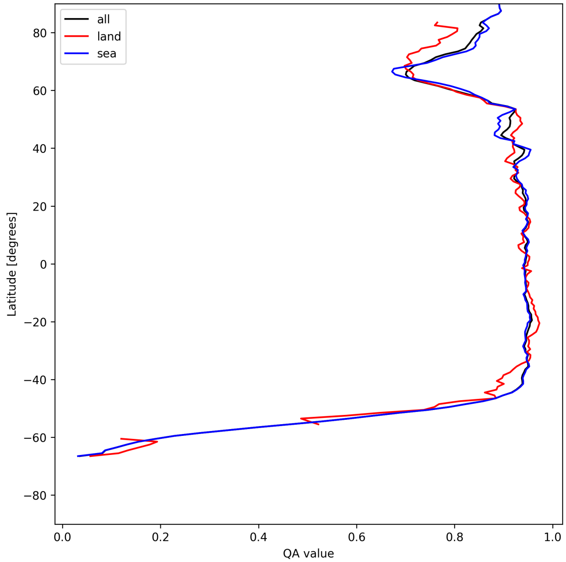
Figure 13: Zonal average of “QA value” for 2025-05-31 to 2025-06-01.
