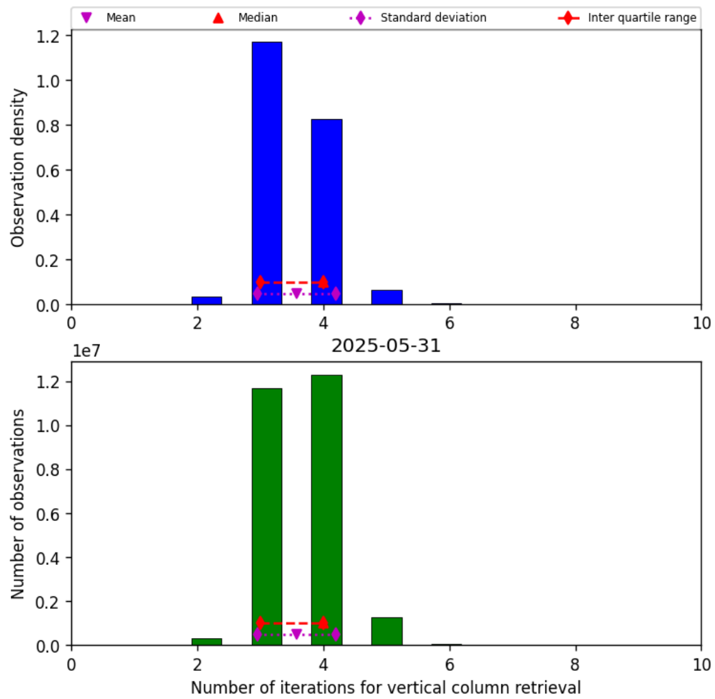
Figure 26: Histogram of “Number of iterations for vertical column retrieval” for 2025-05-31 to 2025-06-01
