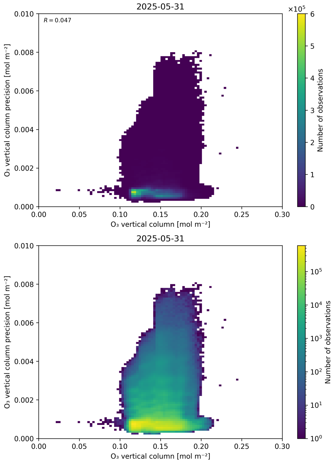
Figure 41: Scatter density plot of “O 3 vertical column” against “O 3 vertical column precision” for 2025-05-31 to 2025-06-01.
