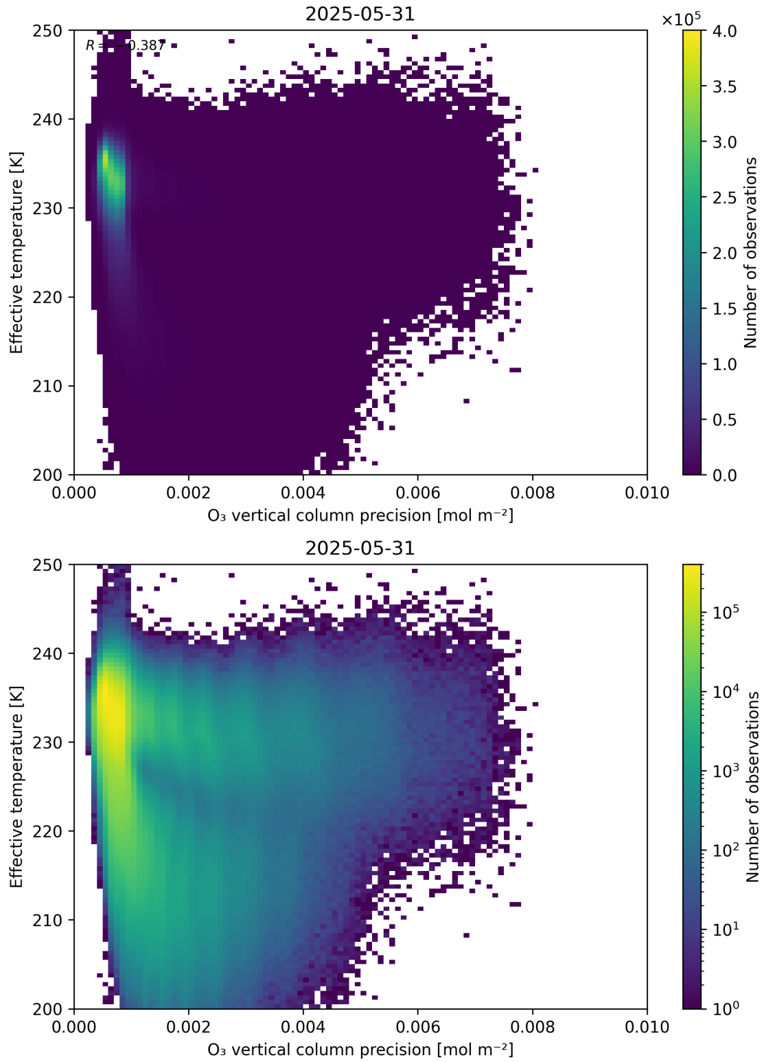
Figure 42: Scatter density plot of “O 3 vertical column precision” against “Effective temperature” for 2025-05-31 to 2025-06-01.
