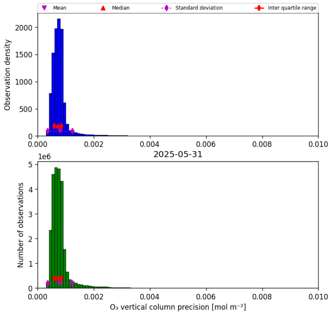
Figure 22: Histogram of “O 3 vertical column precision” for 2025-05-31 to 2025-06-01
