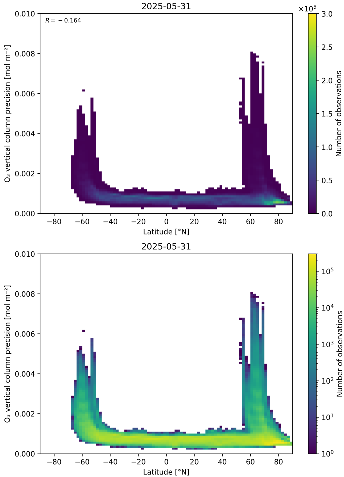
Figure 37: Scatter density plot of “Latitude” against “O 3 vertical column precision” for 2025-05-31 to 2025-06-01.
