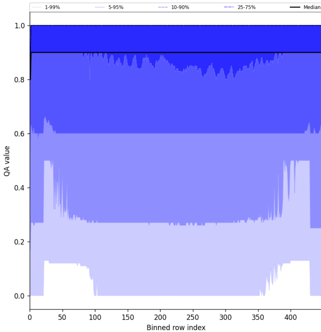
Figure 27: Along track statistics of “QA value” for 2025-05-31 to 2025-06-01
