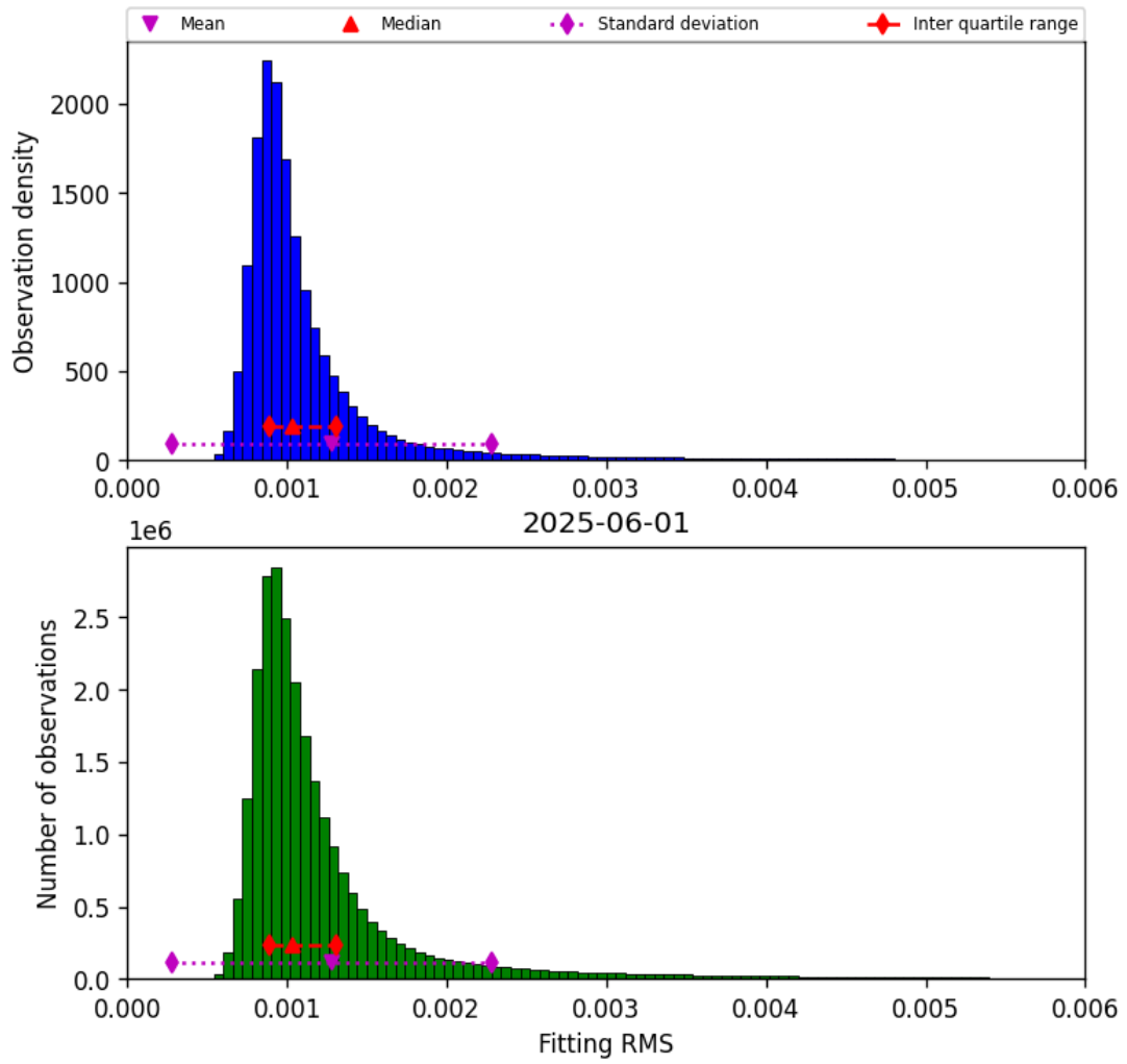
Figure 23: Histogram of “Fitting RMS” for 2025-06-01 to 2025-06-02
