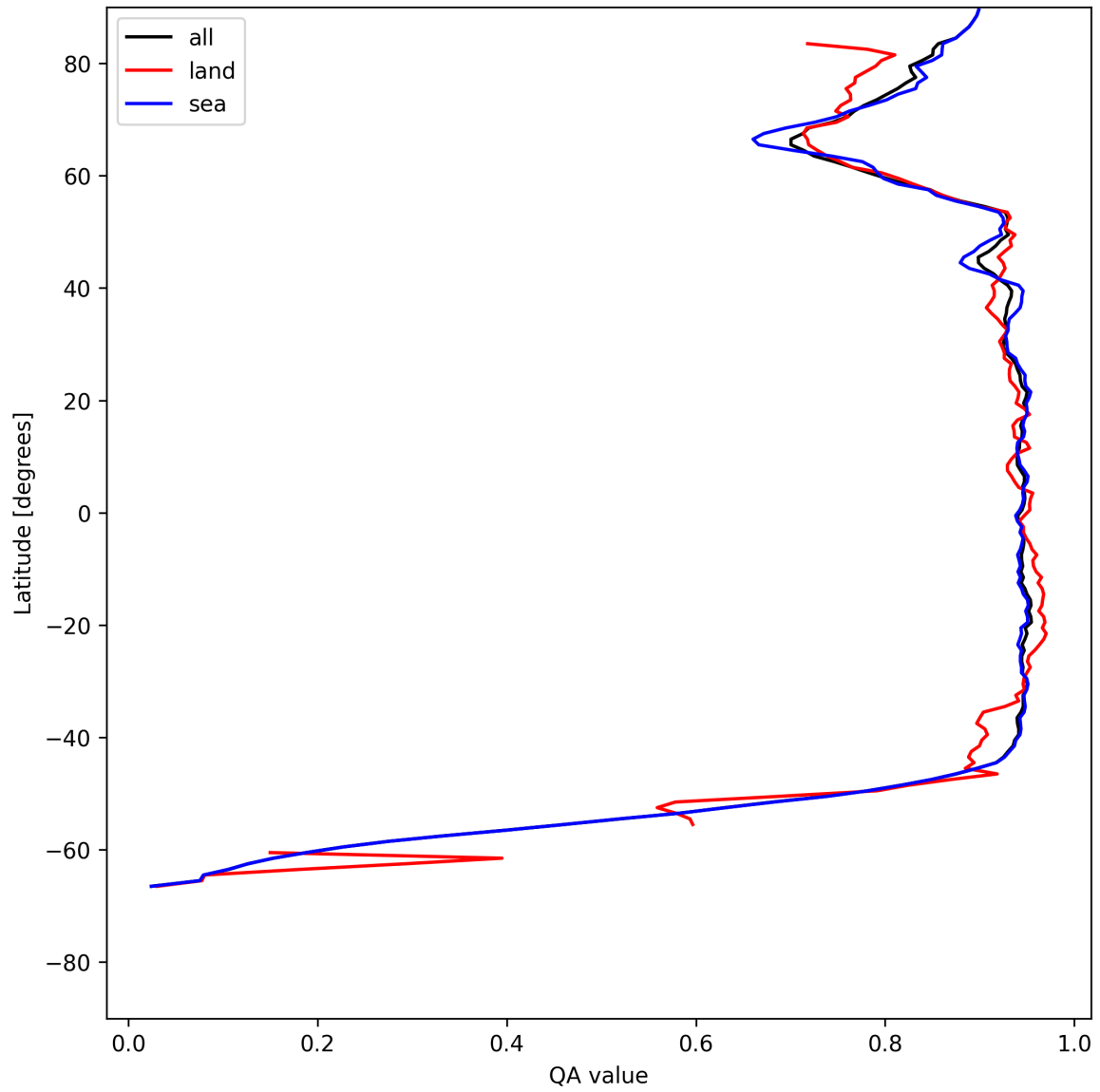
Figure 13: Zonal average of “QA value” for 2025-06-01 to 2025-06-02.
