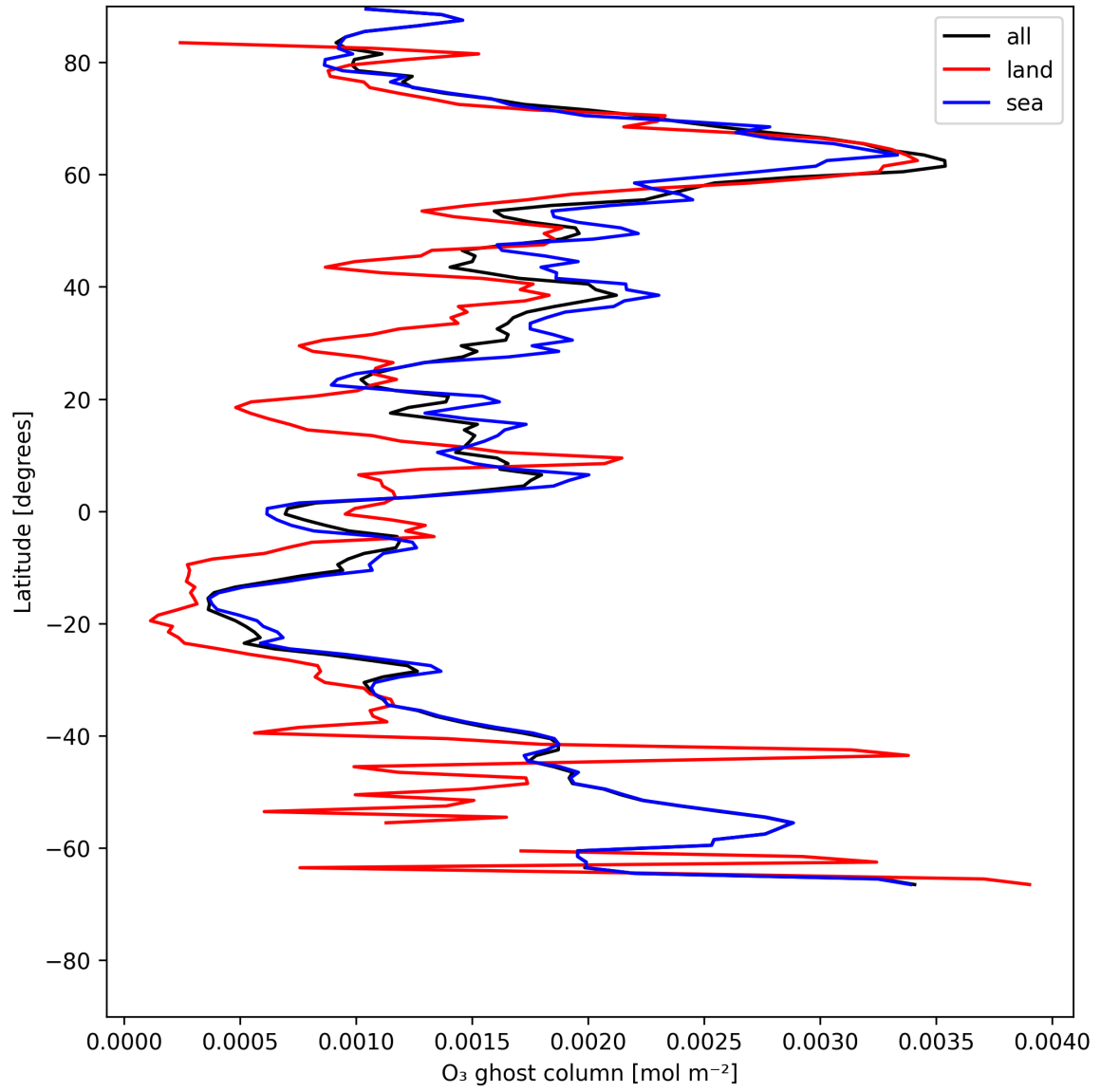
Figure 18: Zonal average of "O 3 ghost column" for 2025-06-01 to 2025-06-02.
