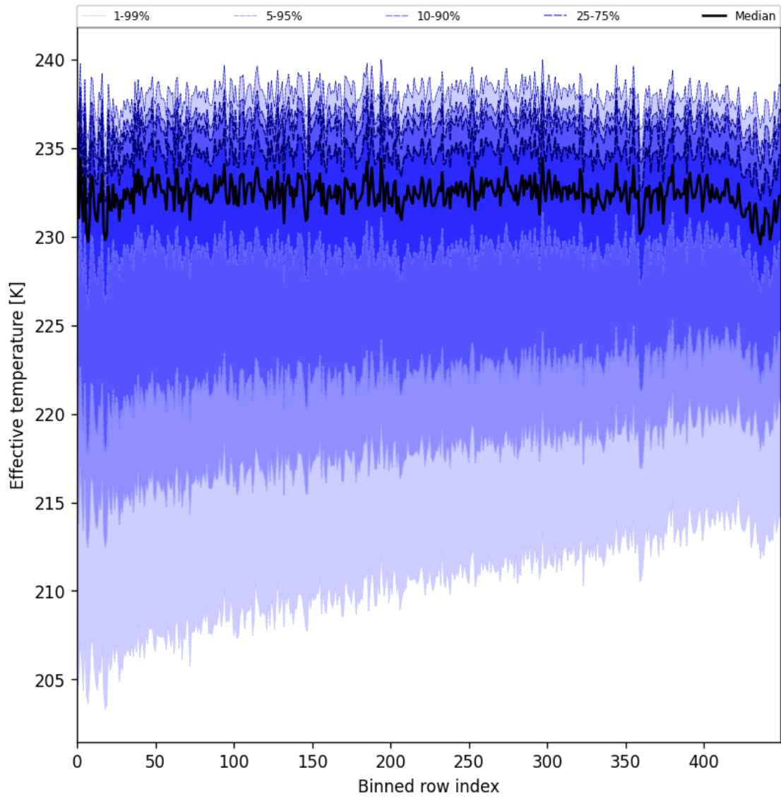
Figure 31: Along track statistics of “Effective temperature” for 2025-06-01 to 2025-06-02
