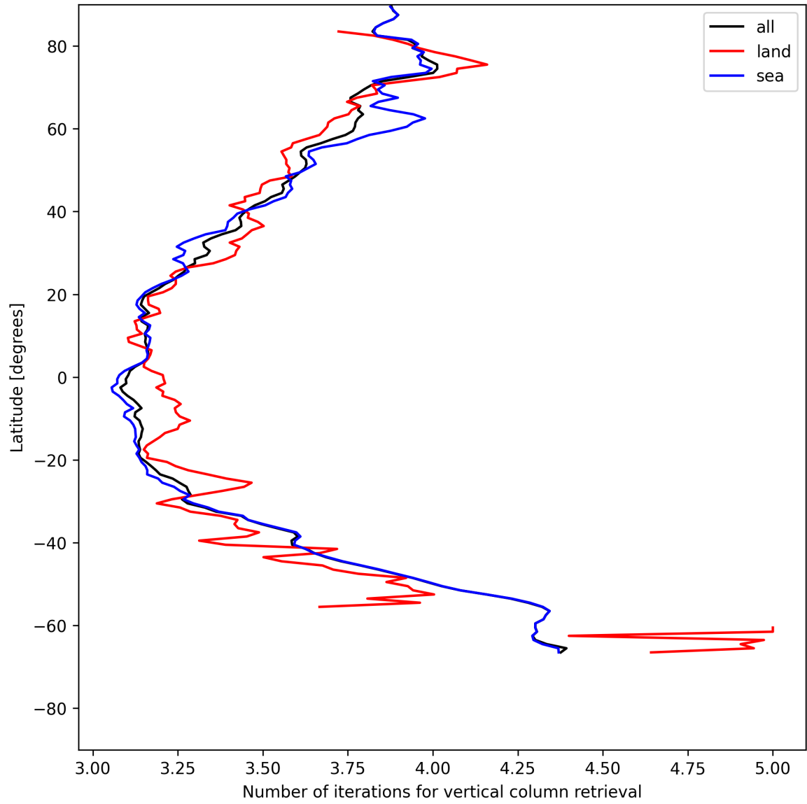
Figure 19: Zonal average of “Number of iterations for vertical column retrieval” for 2025-06-01 to 2025-06-02.
