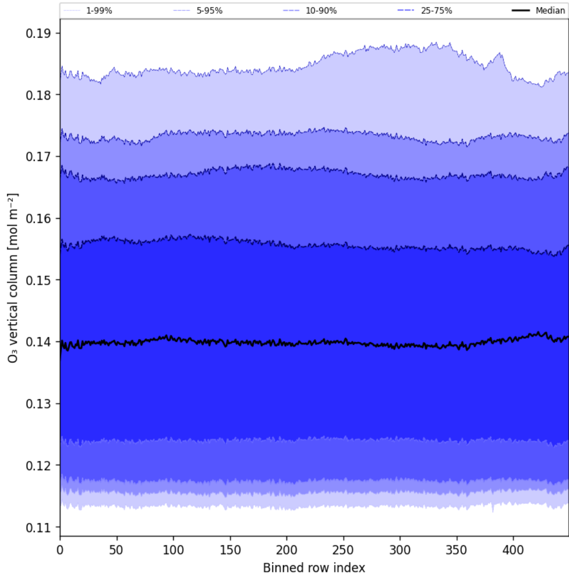
Figure 28: Along track statistics of “O 3 vertical column” for 2025-06-01 to 2025-06-02
