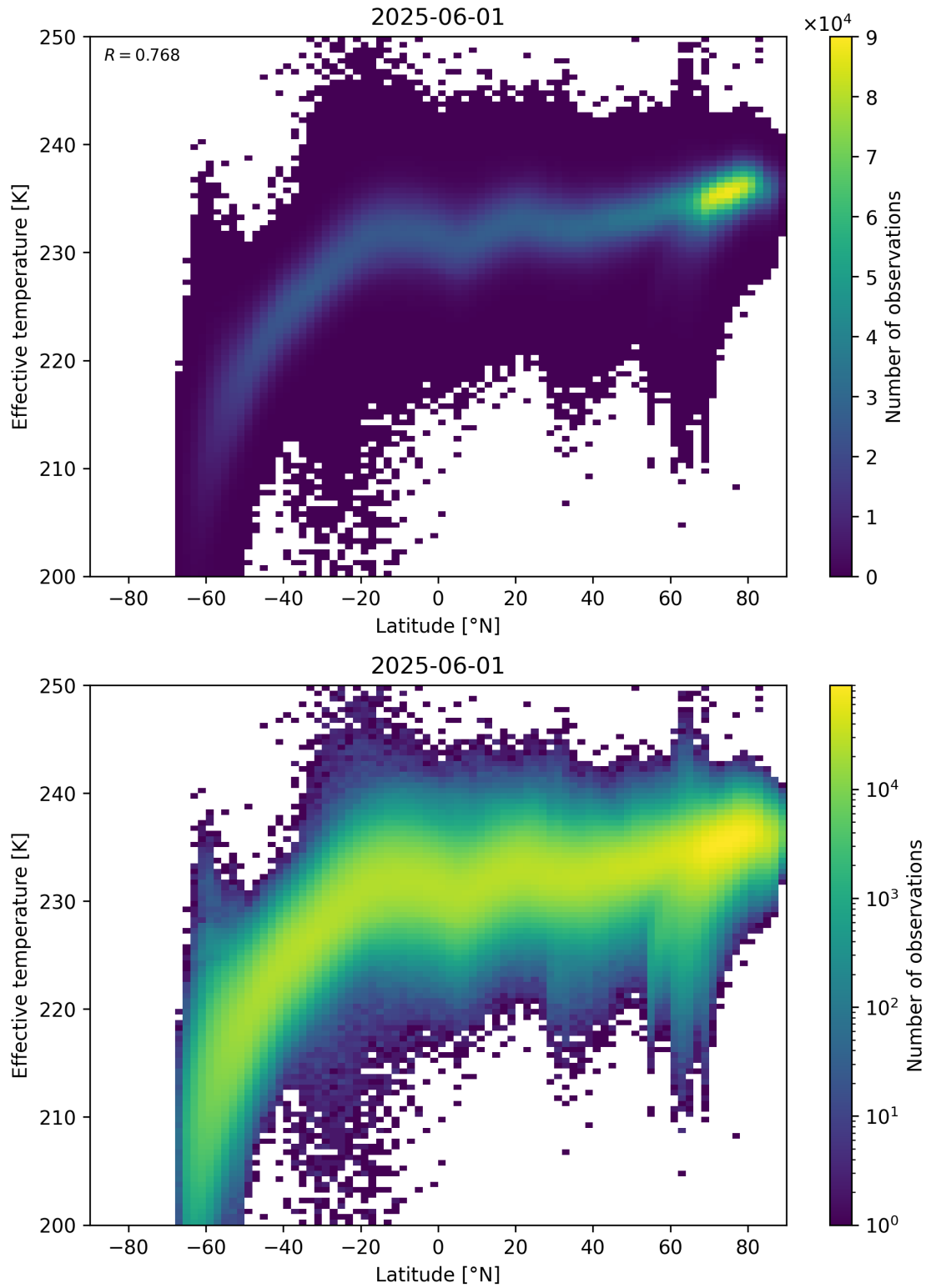
Figure 34: Scatter density plot of “Latitude” against “Effective temperature” for 2025-06-01 to 2025-06-02.
