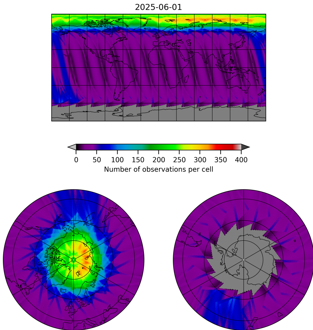
Figure 12: Map of the number of observations for 2025-06-01 to 2025-06-02
