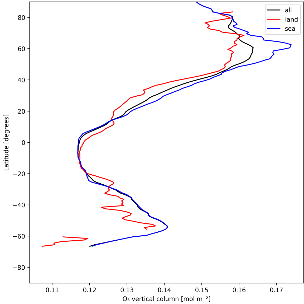
Figure 14: Zonal average of “O 3 vertical column” for 2025-06-01 to 2025-06-02.
