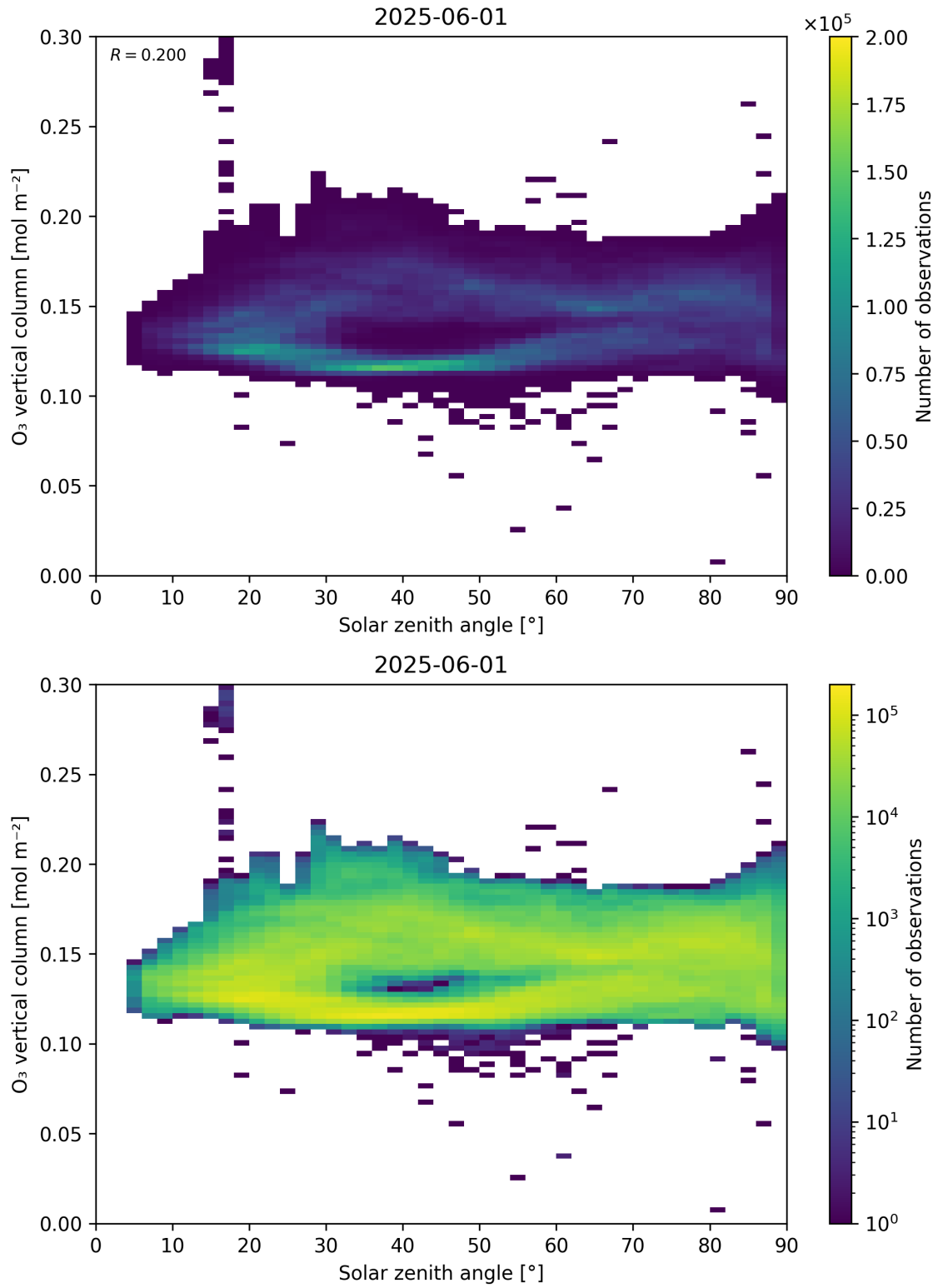
Figure 47: Scatter density plot of “Solar zenith angle” against “O 3 vertical column” for 2025-06-01 to 2025-06-02.
