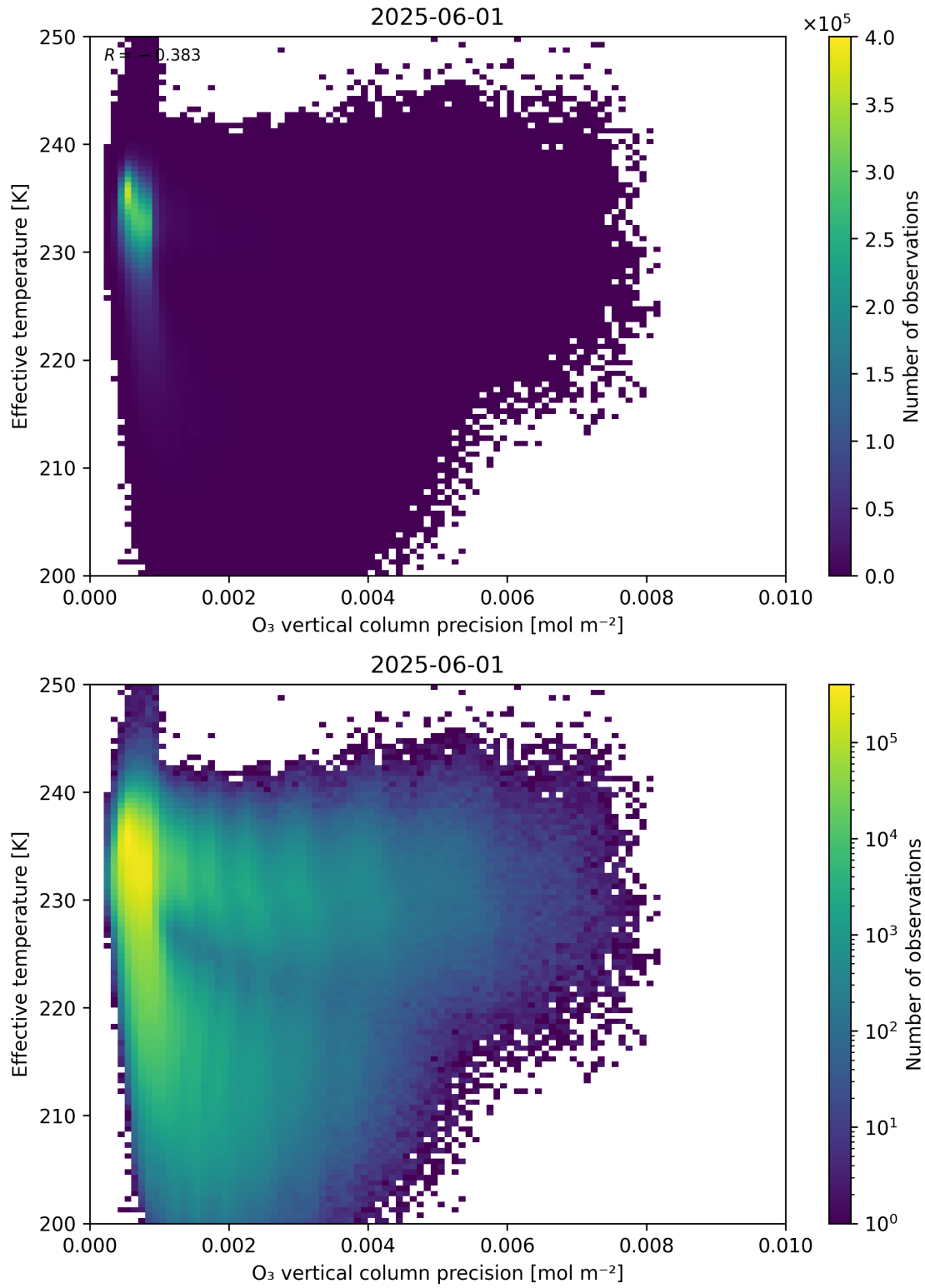
Figure 42: Scatter density plot of “O 3 vertical column precision” against “Effective temperature” for 2025-06-01 to 2025-06-02.
