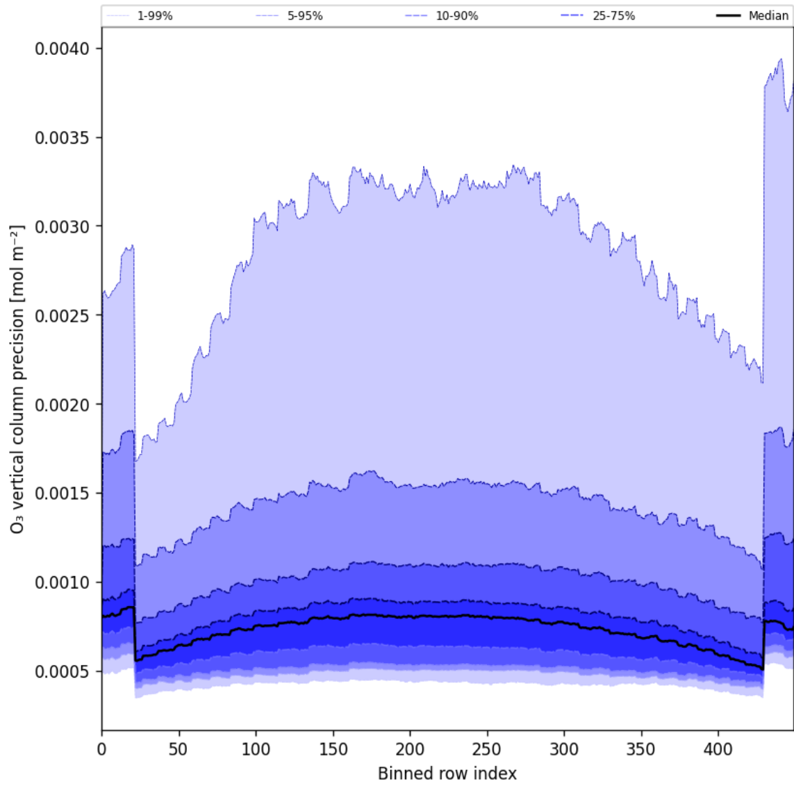
Figure 29: Along track statistics of “O 3 vertical column precision” for 2025-06-01 to 2025-06-02
