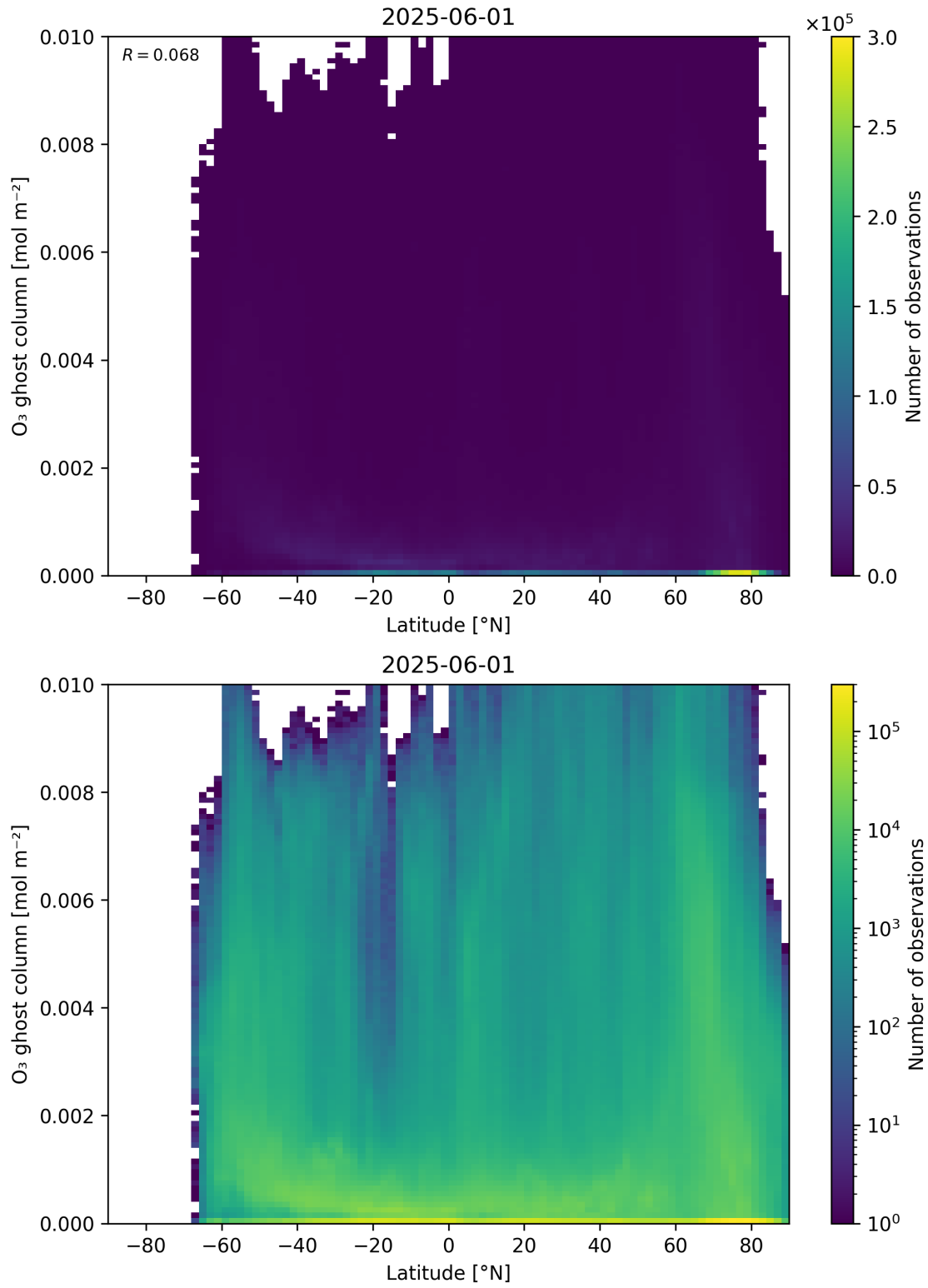
Figure 35: Scatter density plot of “Latitude” against “O 3 ghost column” for 2025-06-01 to 2025-06-02.
