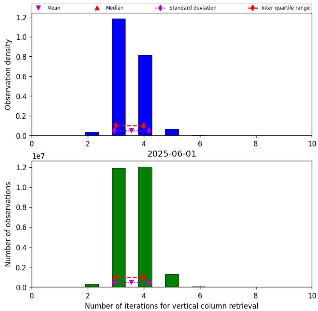
Figure 26: Histogram of “Number of iterations for vertical column retrieval” for 2025-06-01 to 2025-06-02
