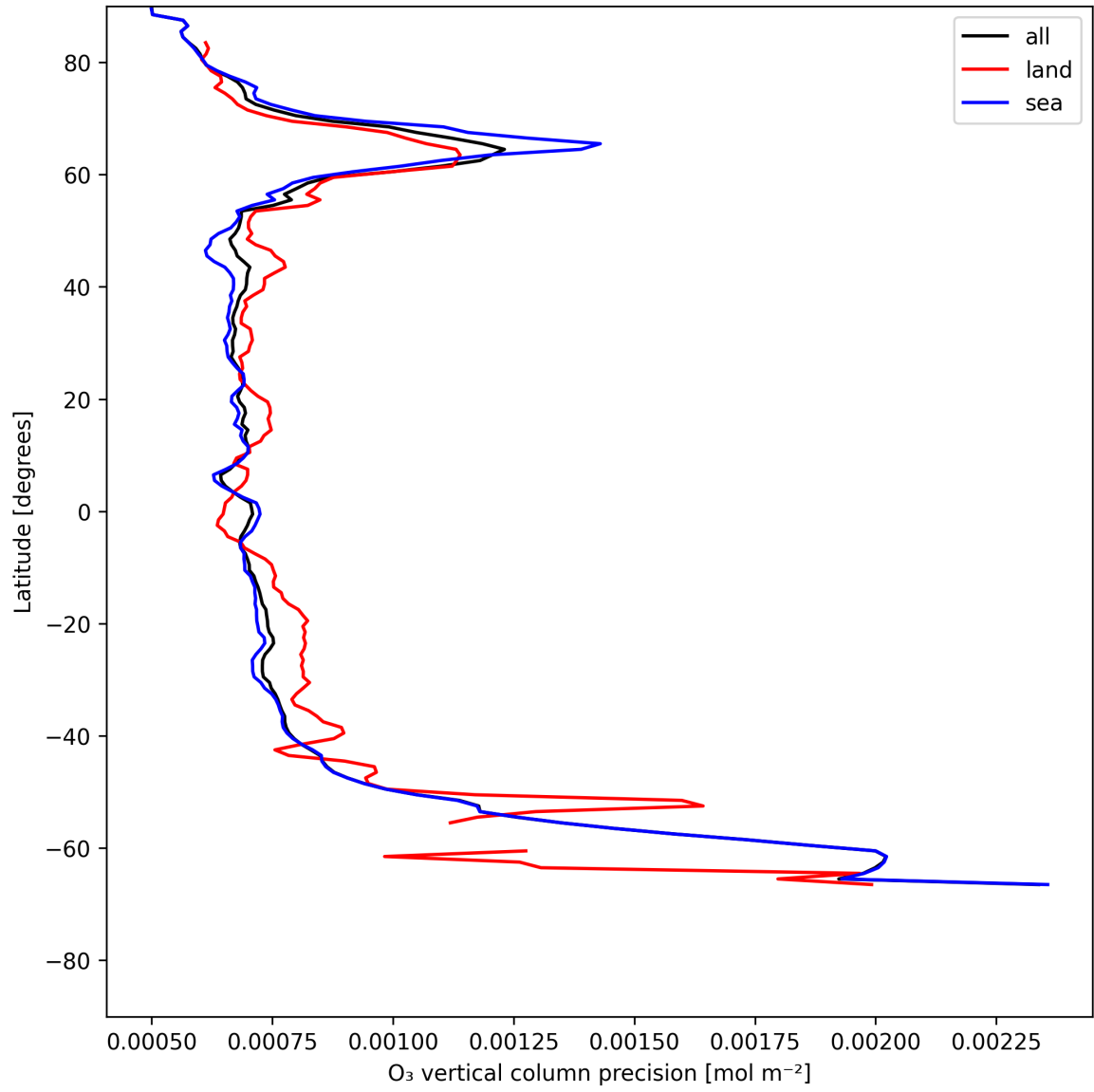
Figure 15: Zonal average of “O 3 vertical column precision” for 2025-06-01 to 2025-06-02.
