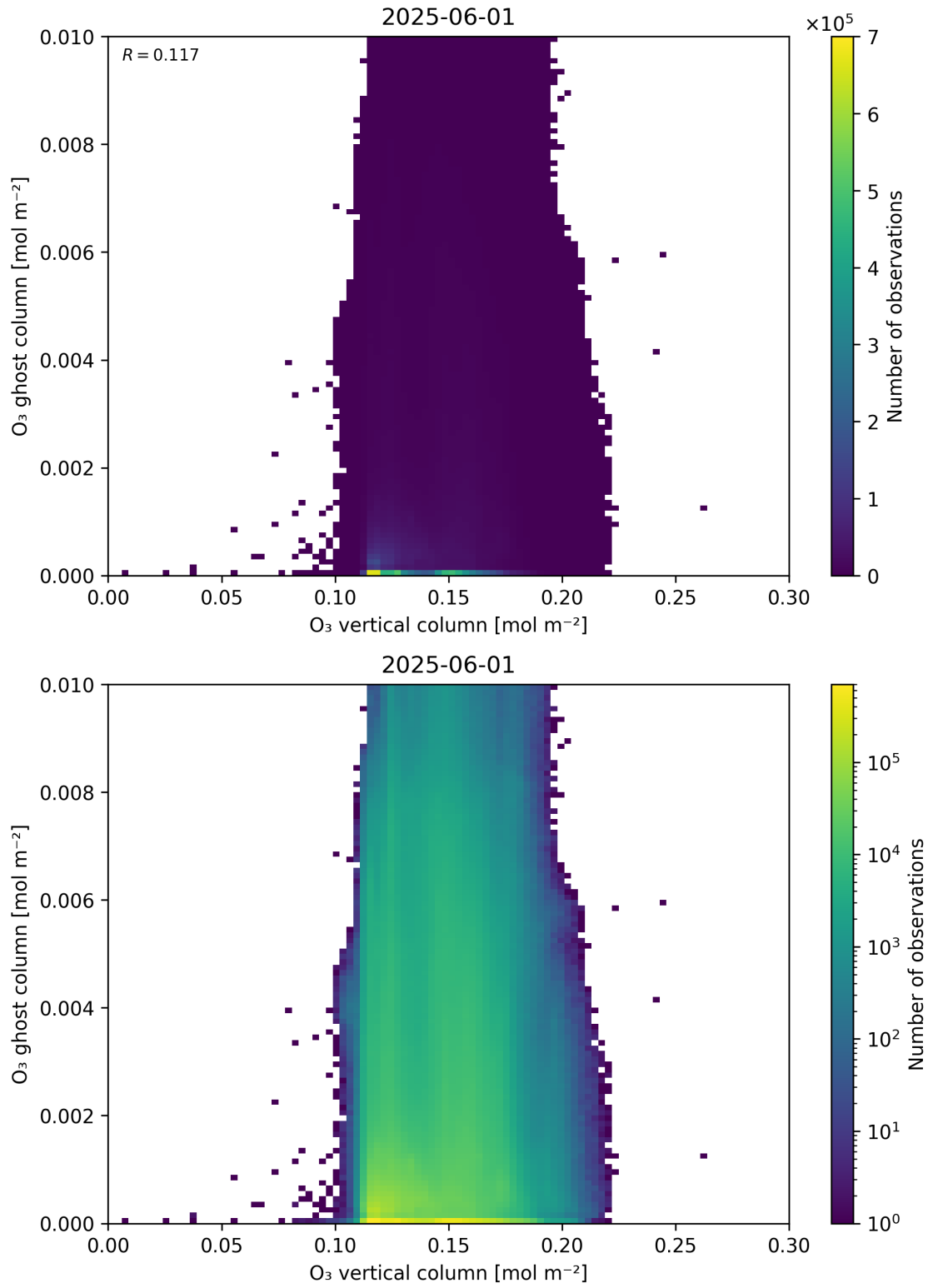
Figure 40: Scatter density plot of “O 3 vertical column” against “O 3 ghost column” for 2025-06-01 to 2025-06-02.
