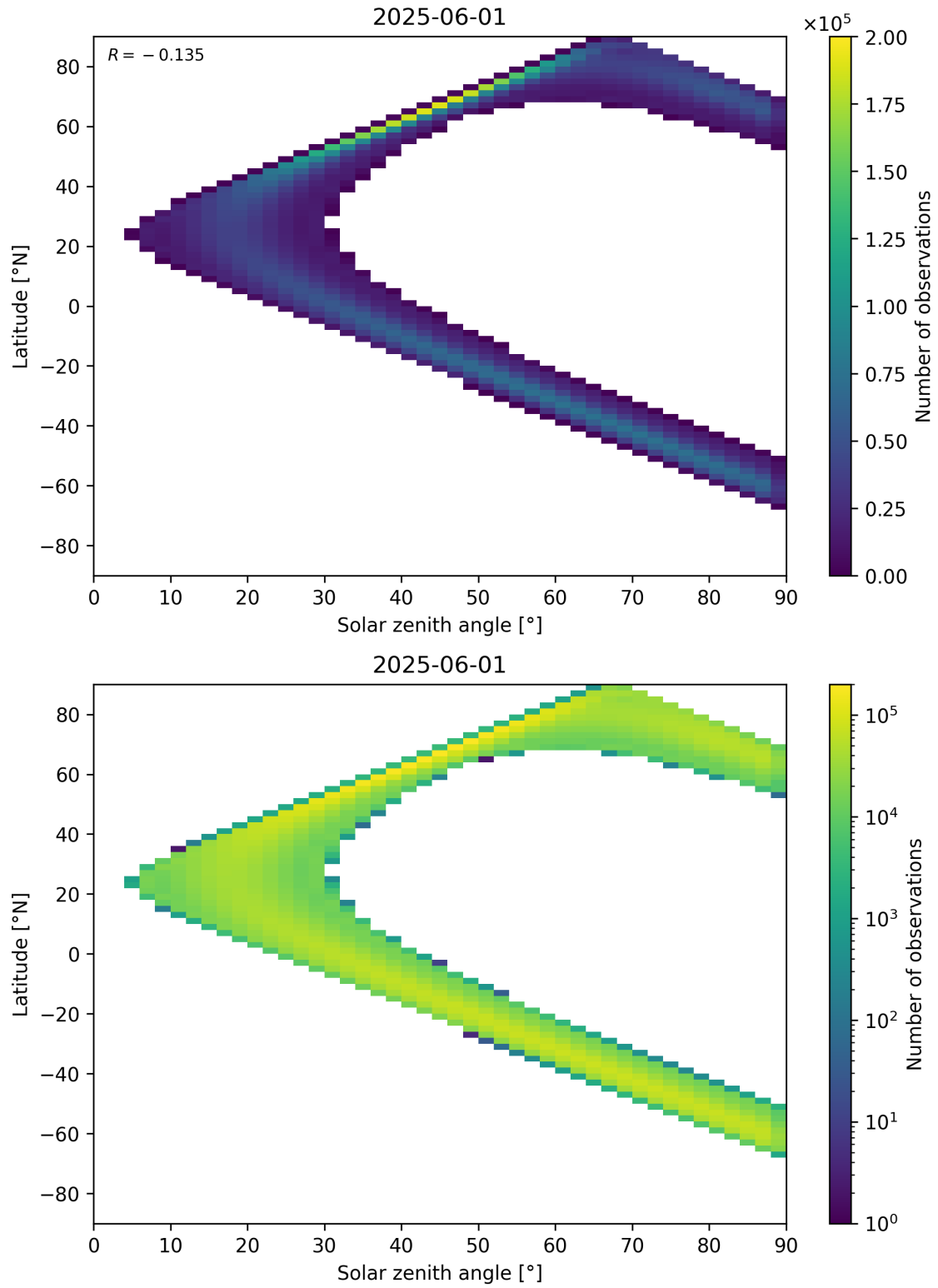
Figure 44: Scatter density plot of “Solar zenith angle” against “Latitude” for 2025-06-01 to 2025-06-02.
