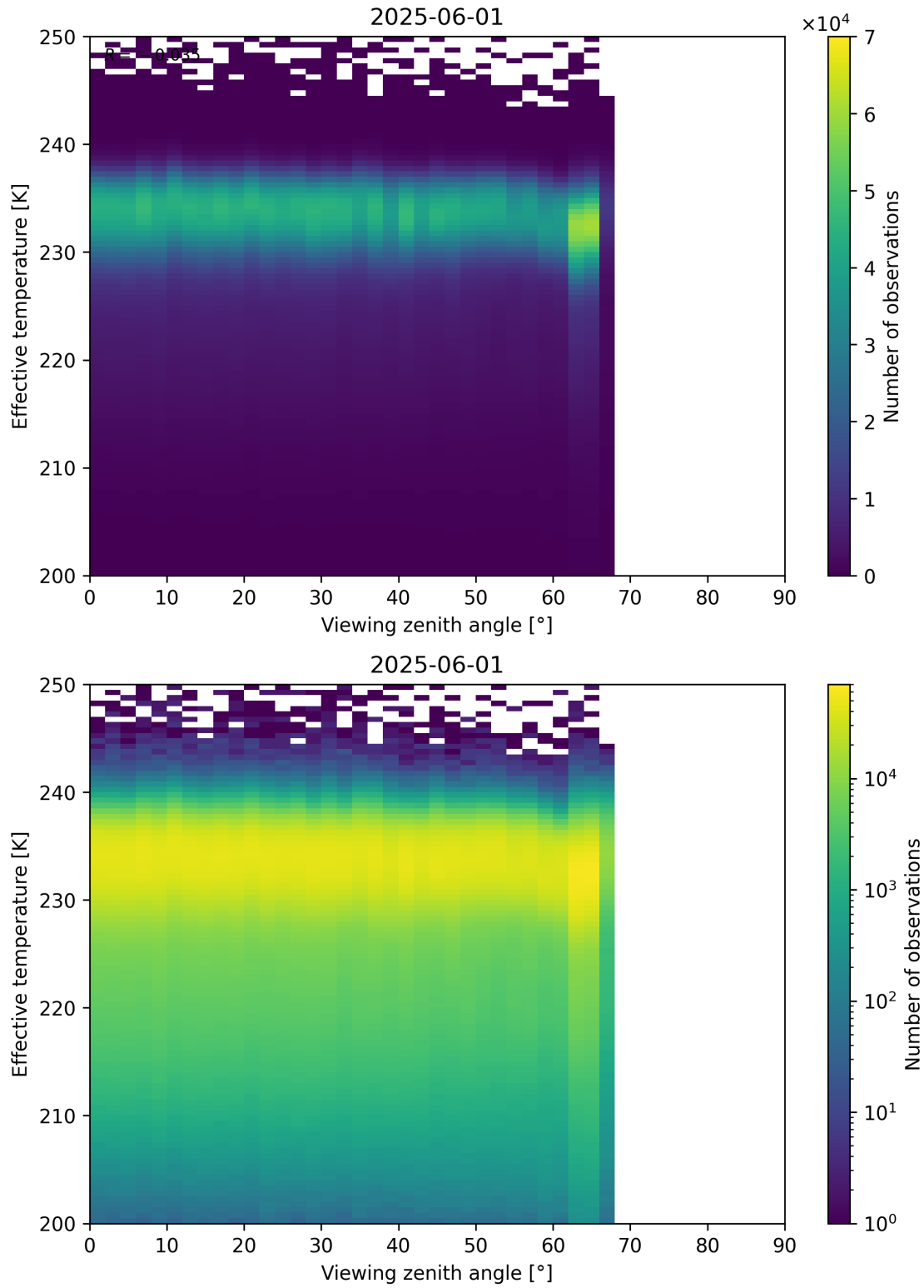
Figure 50: Scatter density plot of “Viewing zenith angle” against “Effective temperature” for 2025-06-01 to 2025-06-02.
