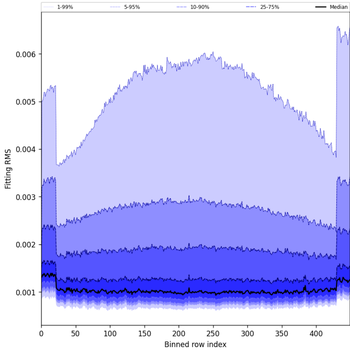
Figure 30: Along track statistics of “Fitting RMS” for 2025-06-01 to 2025-06-02
