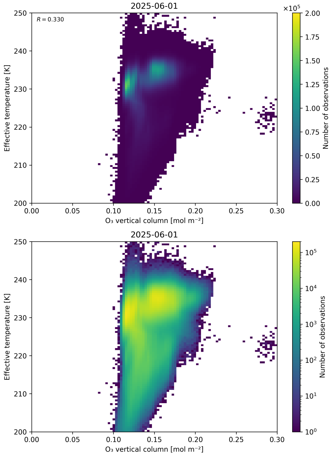
Figure 39: Scatter density plot of “O 3 vertical column” against “Effective temperature” for 2025-06-01 to 2025-06-02.
