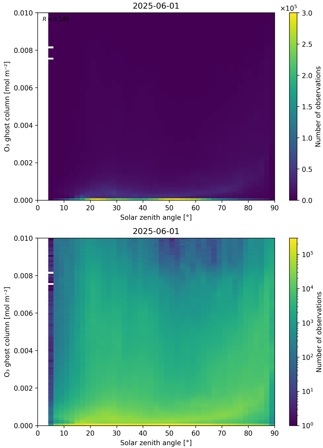
Figure 46: Scatter density plot of “Solar zenith angle” against “O 3 ghost column” for 2025-06-01 to 2025-06-02.
