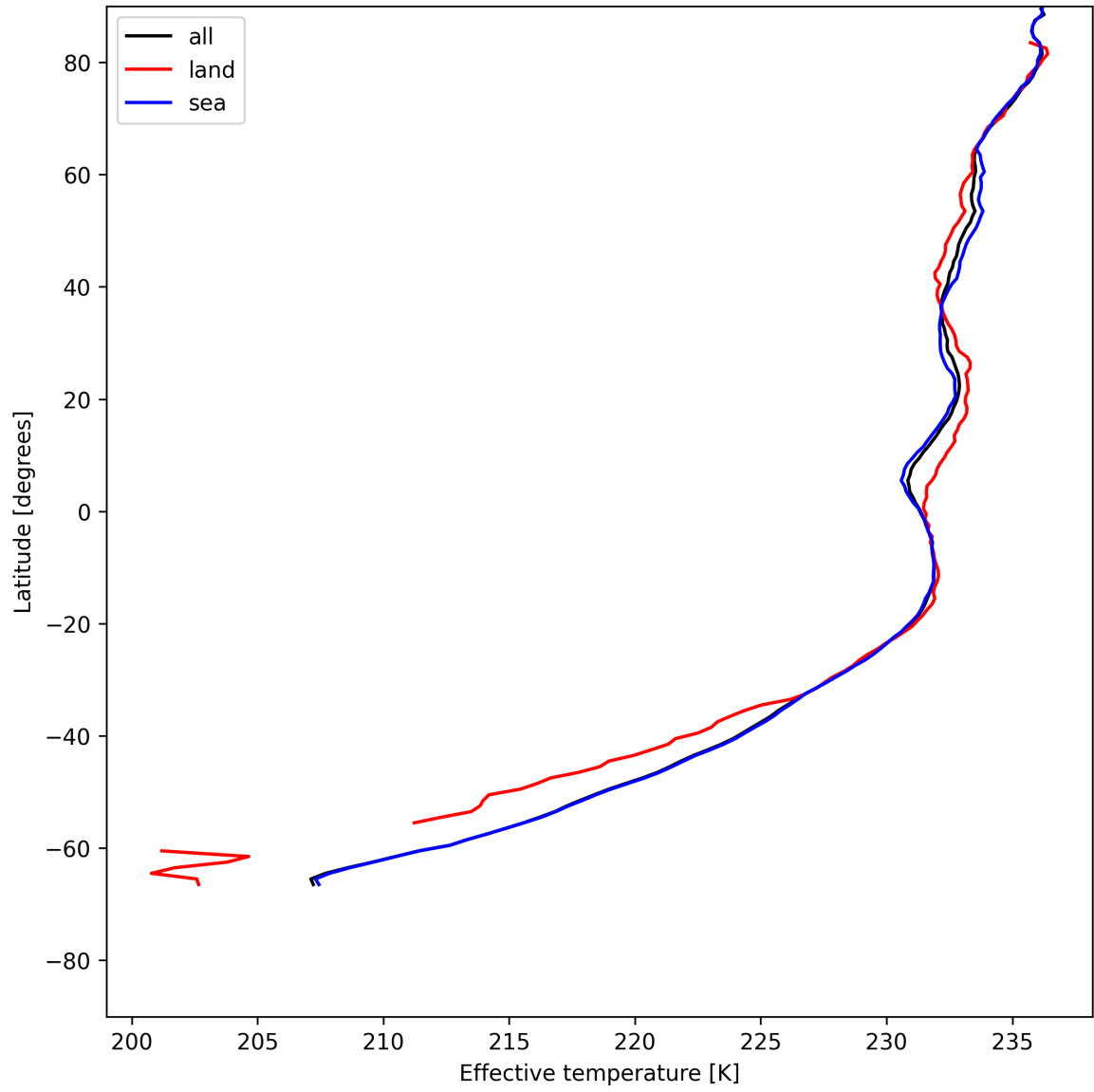
Figure 17: Zonal average of "Effective temperature" for 2025-06-01 to 2025-06-02.
