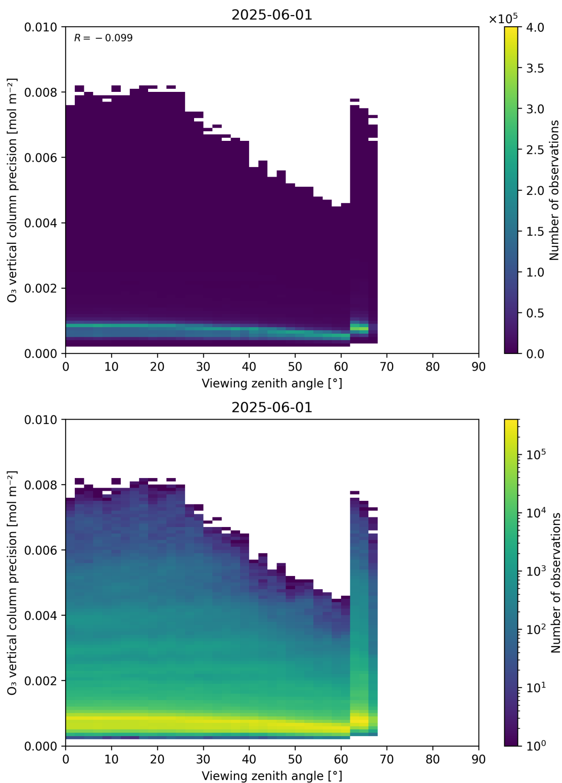
Figure 53: Scatter density plot of “Viewing zenith angle” against “O 3 vertical column precision” for 2025-06-01 to 2025-06-02.
