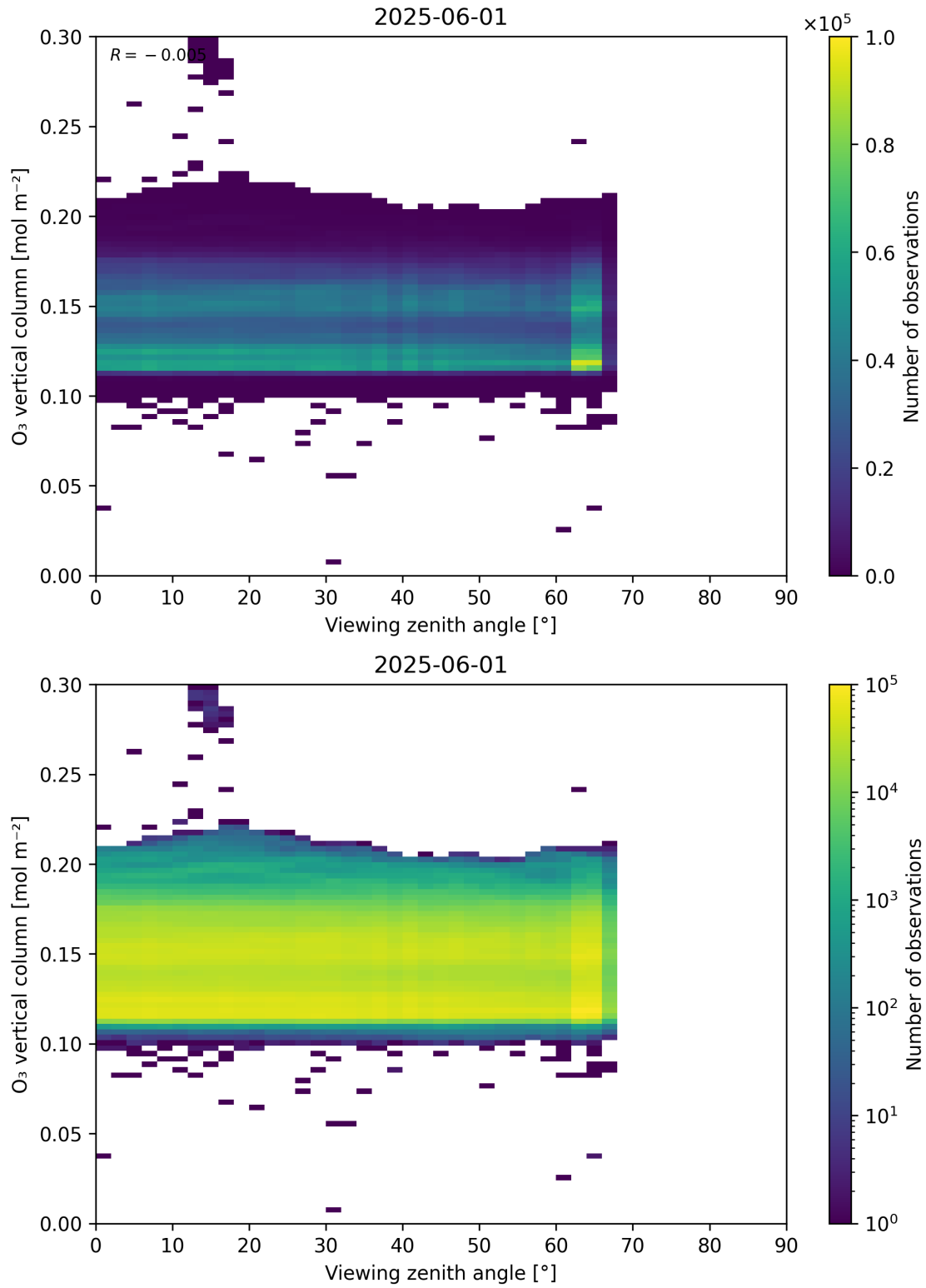
Figure 52: Scatter density plot of “Viewing zenith angle” against “O 3 vertical column” for 2025-06-01 to 2025-06-02.
