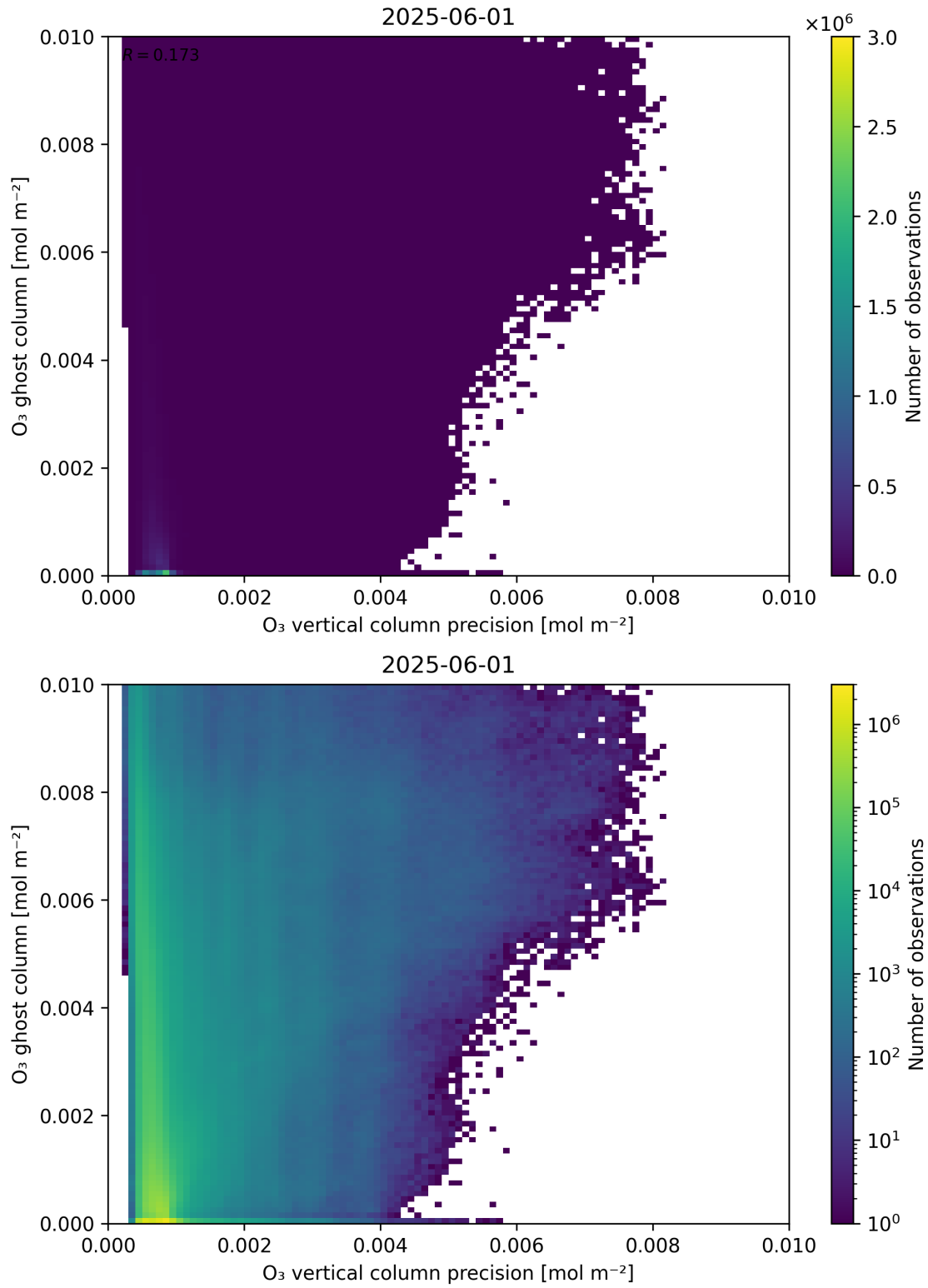
Figure 43: Scatter density plot of “ O_3 vertical column precision” against “ O_3 ghost column” for 2025-06-01 to 2025-06-02.
