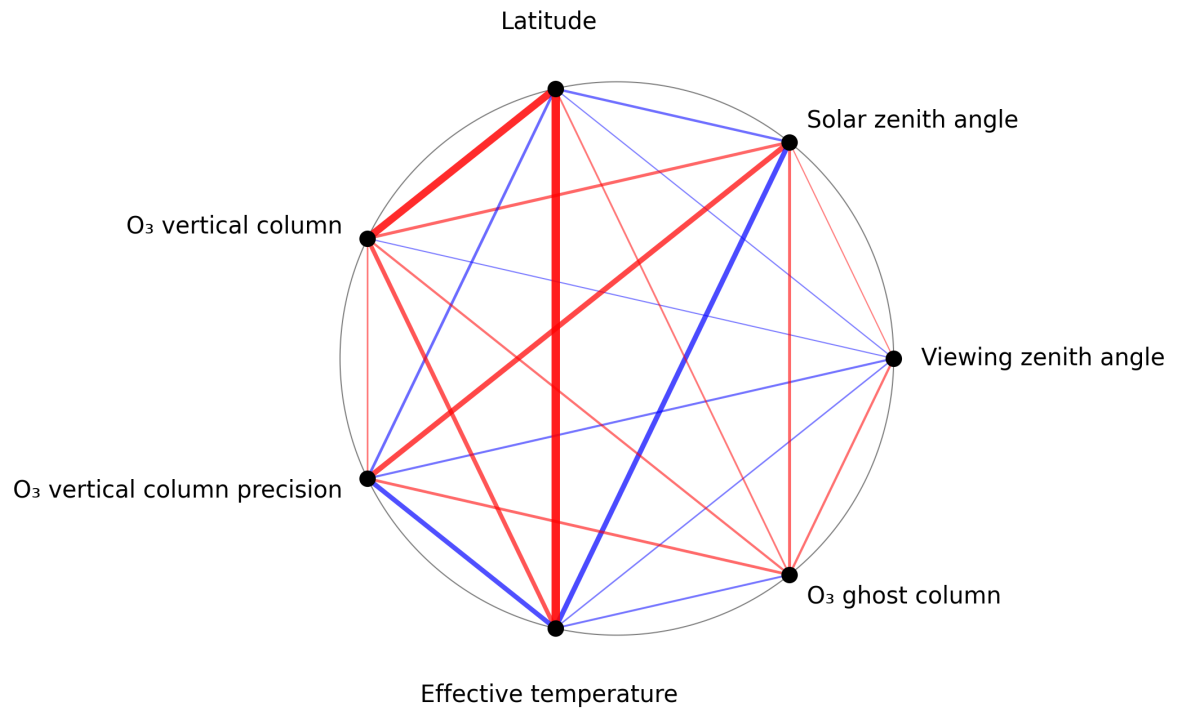
Figure 1: Map of correlation graph for 2025-06-01 to 2025-06-02.
