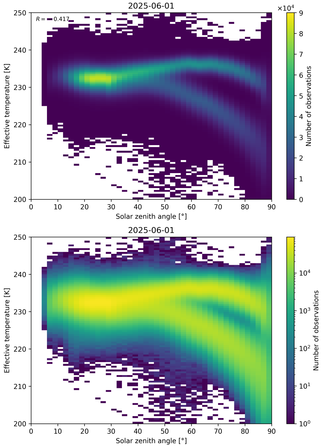
Figure 45: Scatter density plot of “Solar zenith angle” against “Effective temperature” for 2025-06-01 to 2025-06-02.
