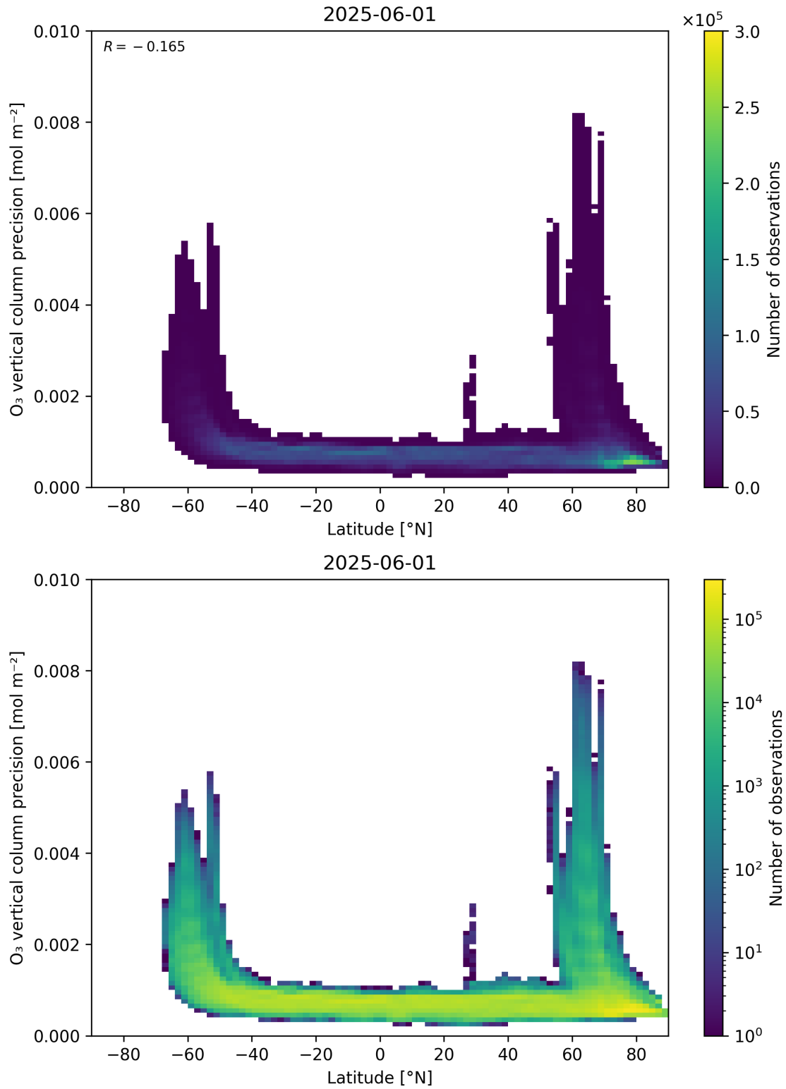
Figure 37: Scatter density plot of “Latitude” against “O 3 vertical column precision” for 2025-06-01 to 2025-06-02.
