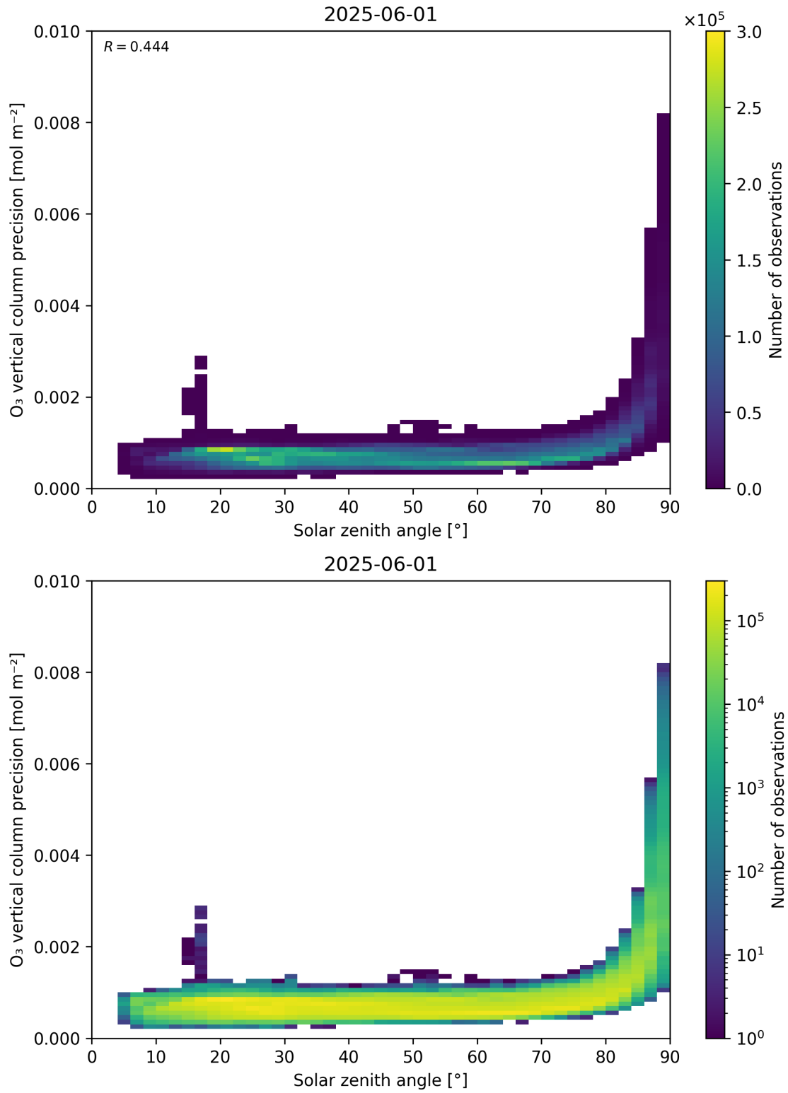
Figure 48: Scatter density plot of “Solar zenith angle” against “O 3 vertical column precision” for 2025-06-01 to 2025-06-02.
