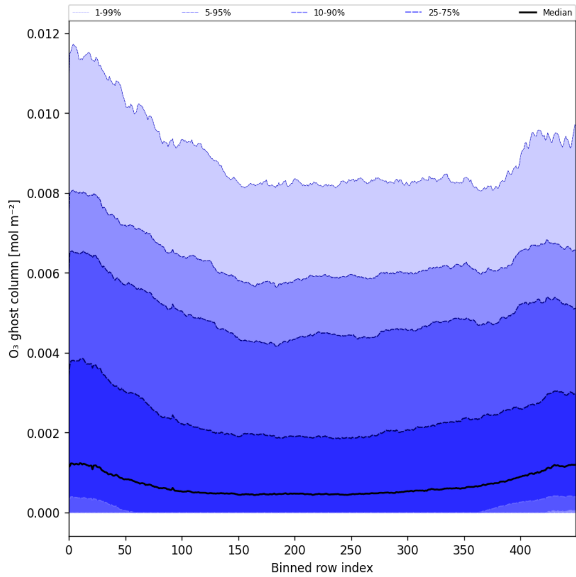
Figure 32: Along track statistics of “O 3 ghost column” for 2025-06-01 to 2025-06-02
