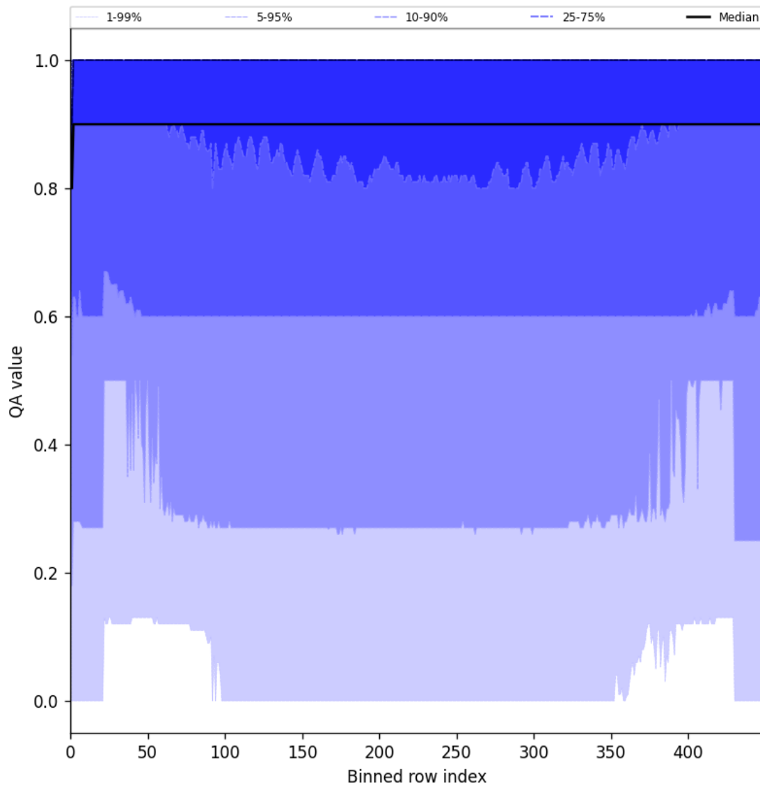
Figure 27: Along track statistics of “QA value” for 2025-06-01 to 2025-06-02
