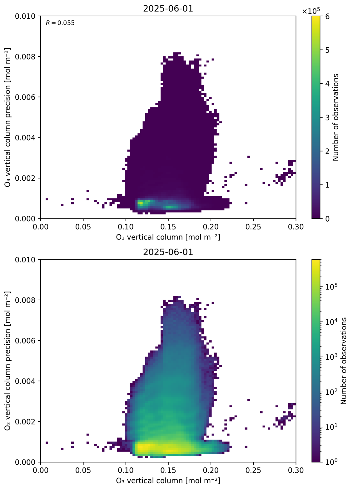
Figure 41: Scatter density plot of “O 3 vertical column” against “O 3 vertical column precision” for 2025-06-01 to 2025-06-02.
