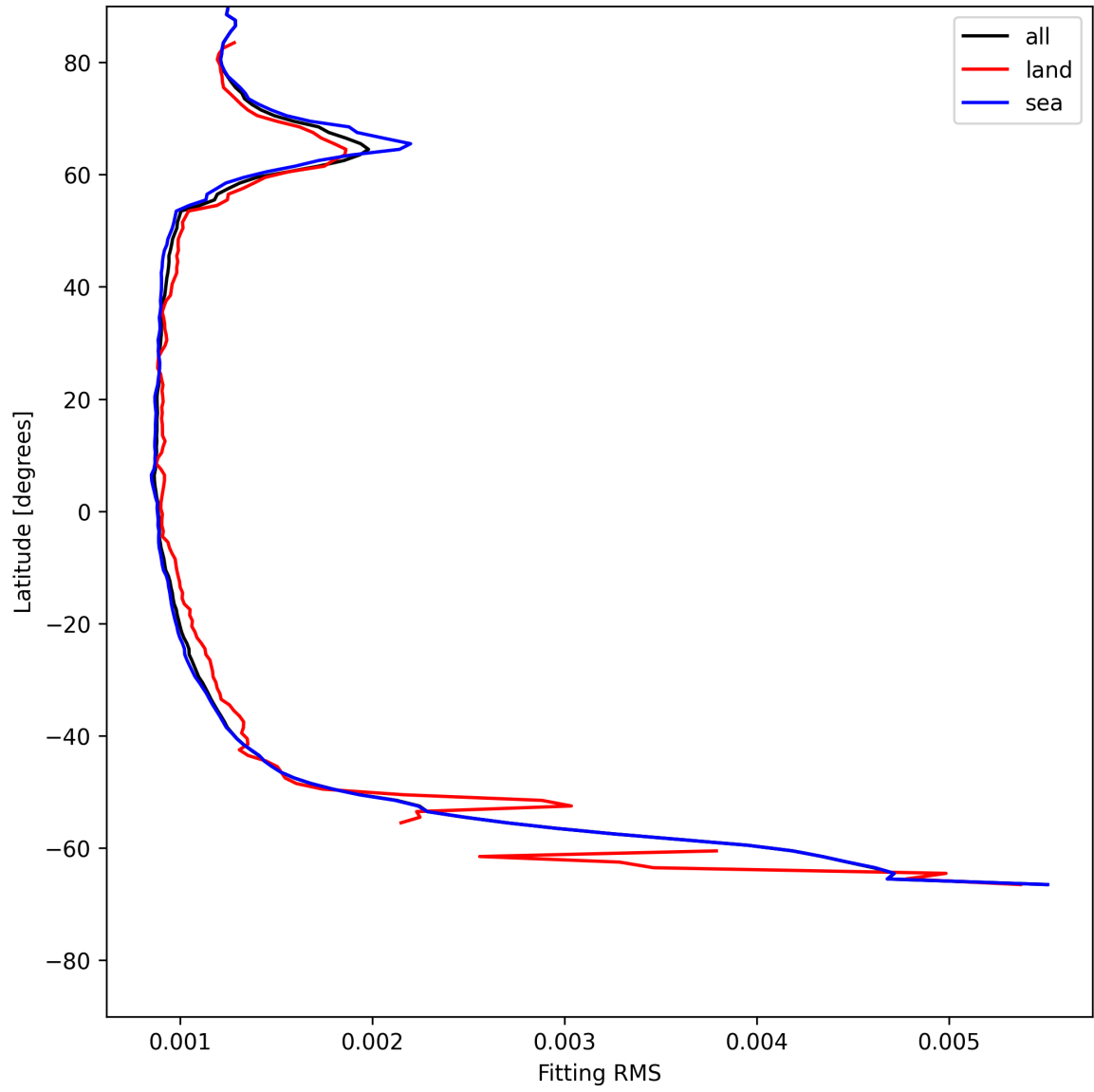
Figure 16: Zonal average of “Fitting RMS” for 2025-06-01 to 2025-06-02.
