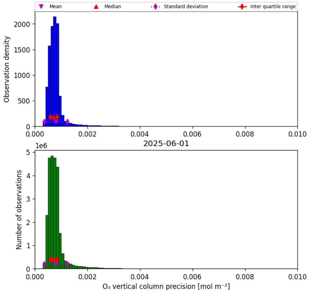
Figure 22: Histogram of “O 3 vertical column precision” for 2025-06-01 to 2025-06-02
