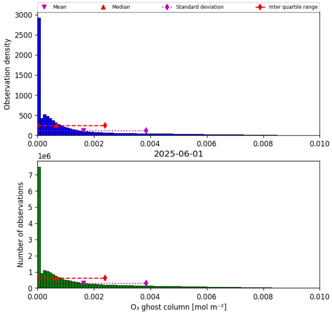
Figure 25: Histogram of “O 3 ghost column” for 2025-06-01 to 2025-06-02
