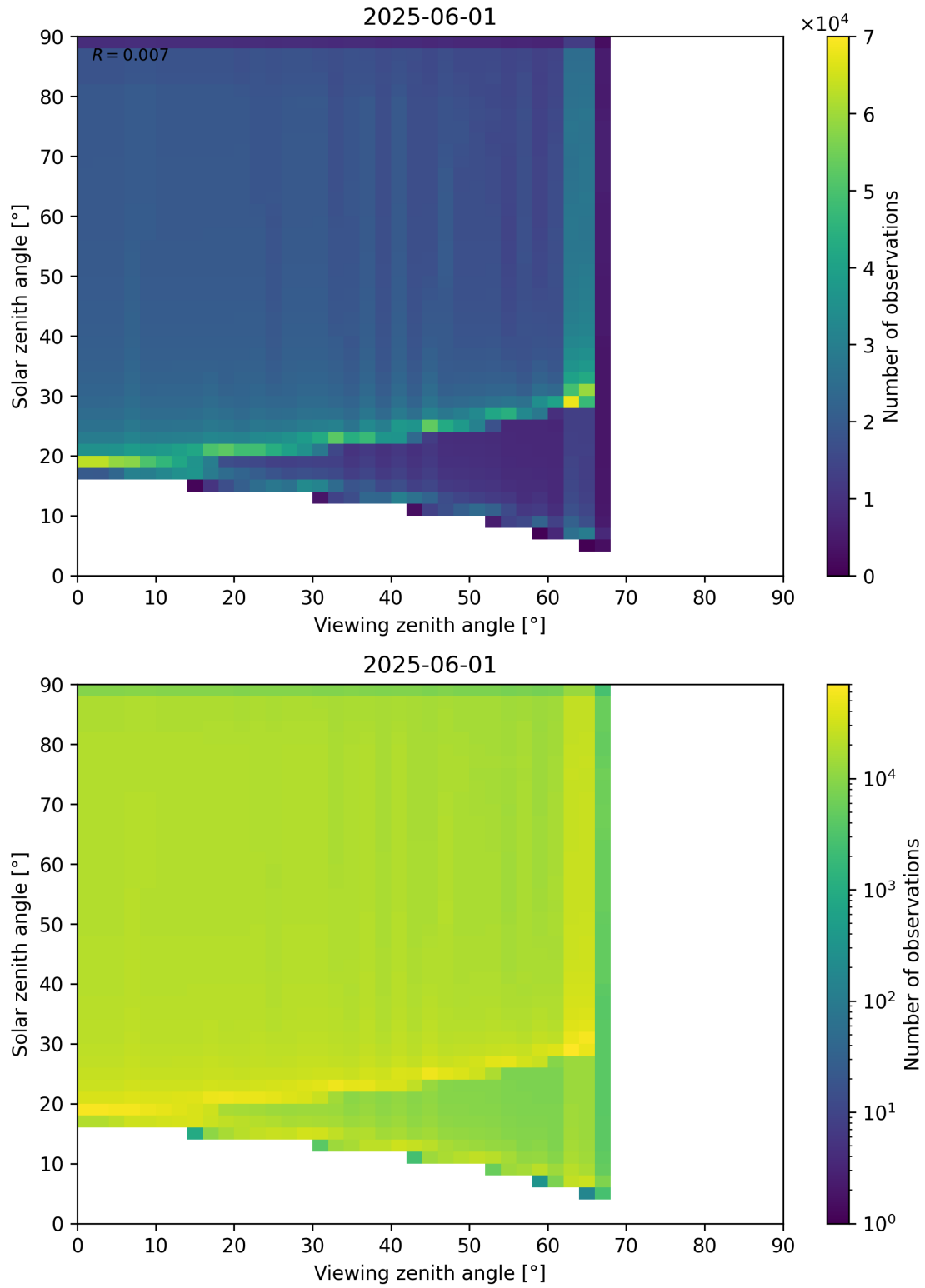
Figure 54: Scatter density plot of “Viewing zenith angle” against “Solar zenith angle” for 2025-06-01 to 2025-06-02.
