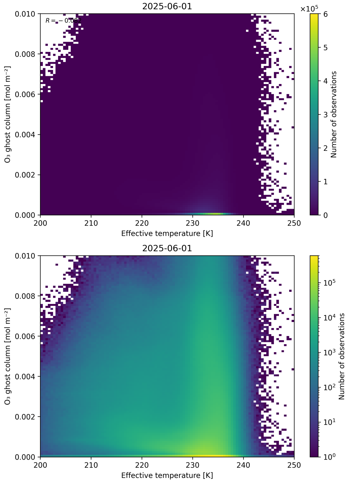
Figure 38: Scatter density plot of “Effective temperature” against “O 3 ghost column” for 2025-06-01 to 2025-06-02.
