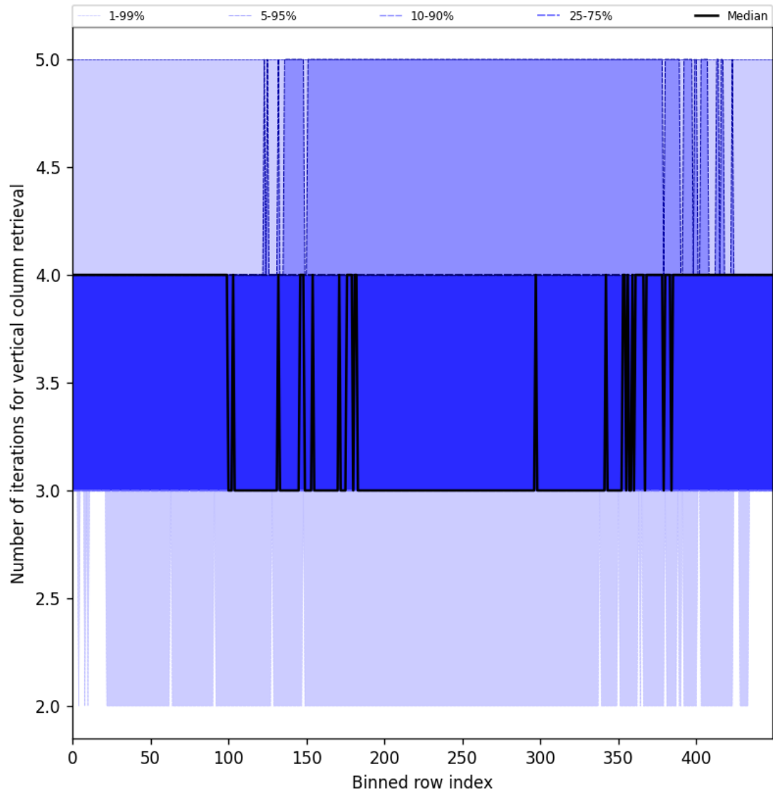
Figure 33: Along track statistics of “Number of iterations for vertical column retrieval” for 2025-06-01 to 2025-06-02
