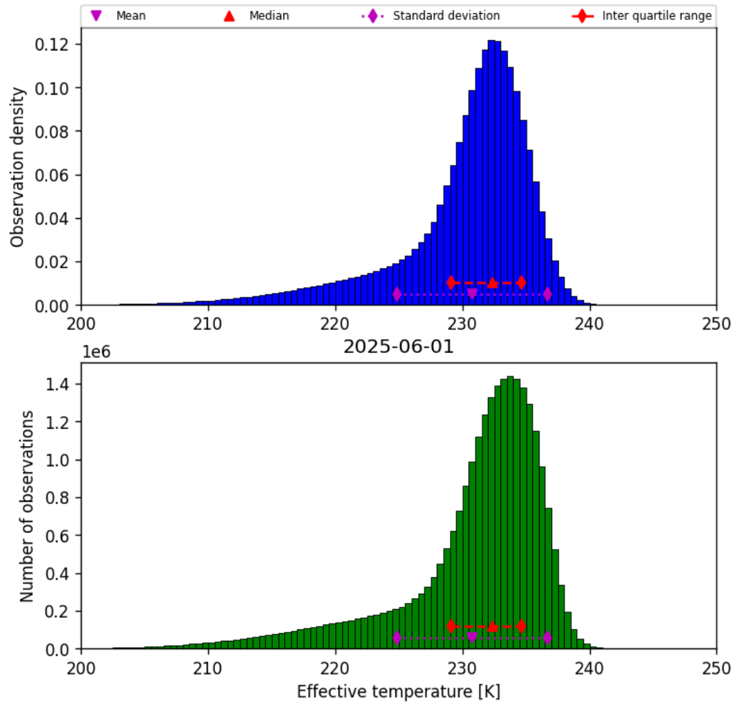
Figure 24: Histogram of “Effective temperature” for 2025-06-01 to 2025-06-02
