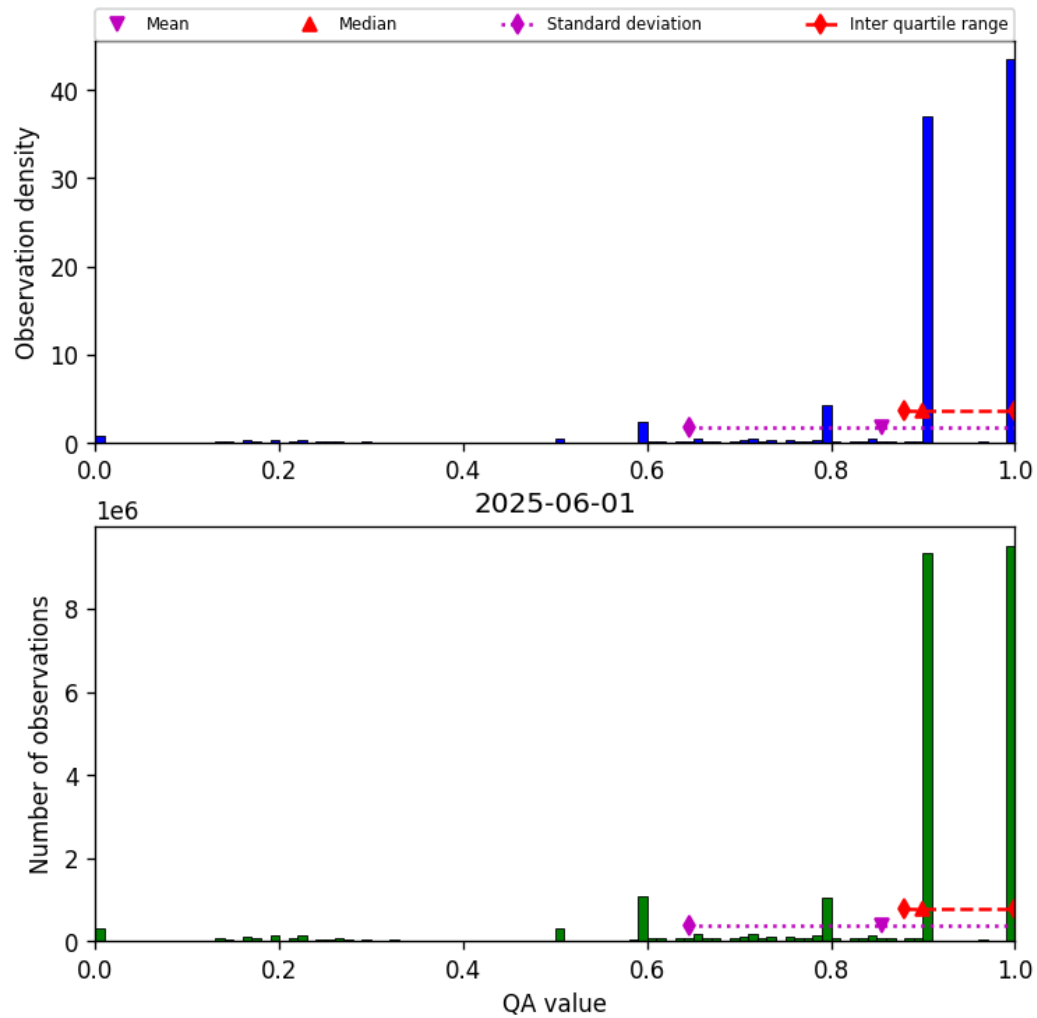
Figure 20: Histogram of “QA value” for 2025-06-01 to 2025-06-02
