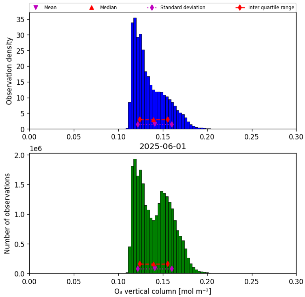
Figure 21: Histogram of “O 3 vertical column” for 2025-06-01 to 2025-06-02
