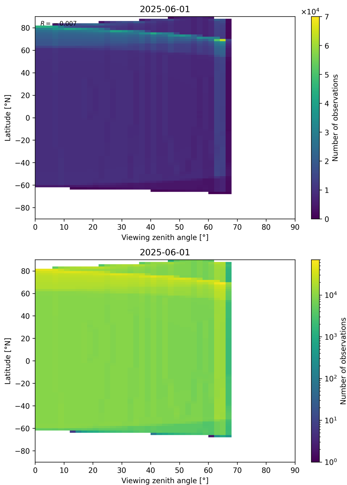
Figure 49: Scatter density plot of “Viewing zenith angle” against “Latitude” for 2025-06-01 to 2025-06-02.
