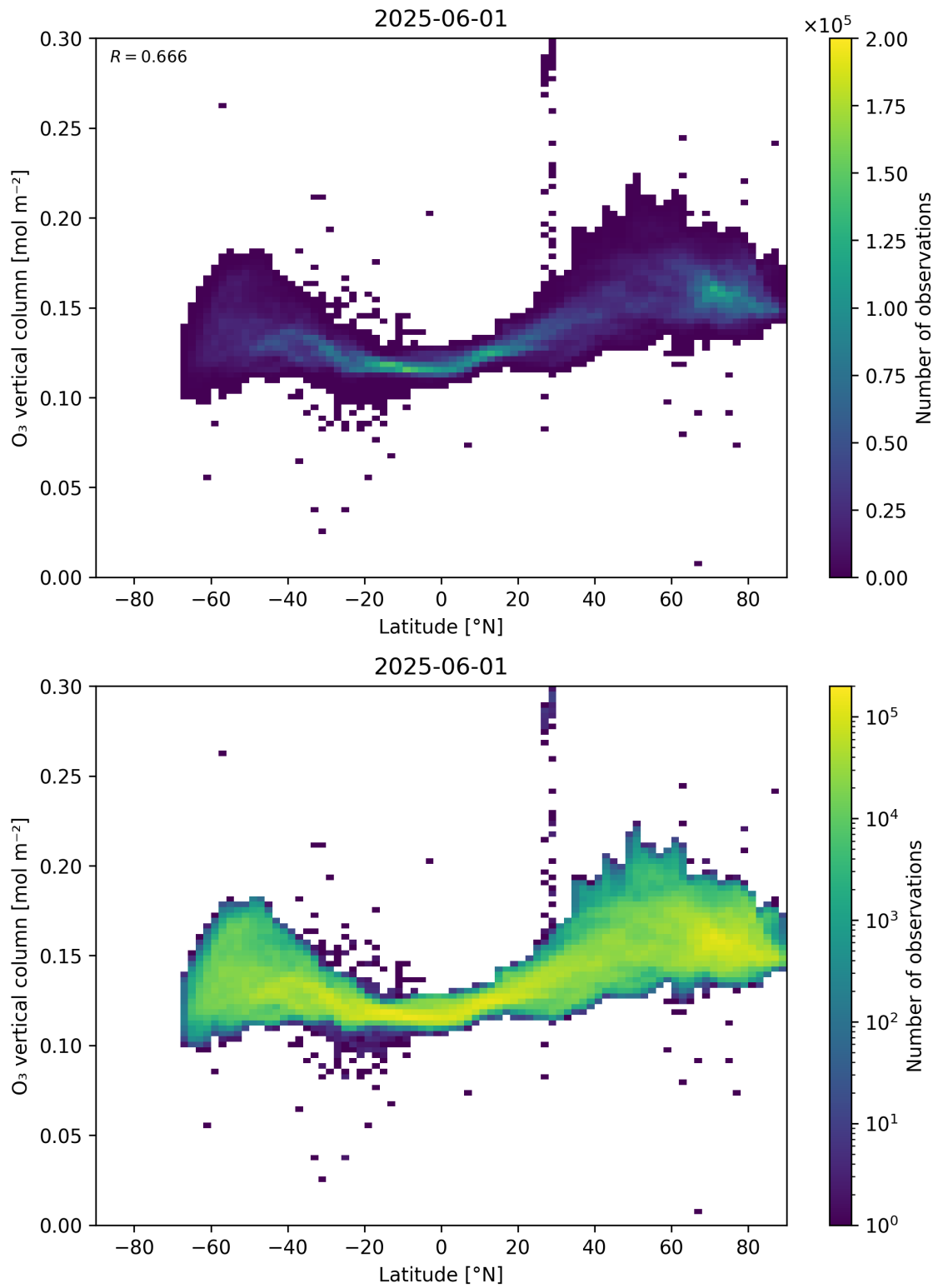
Figure 36: Scatter density plot of “Latitude” against “O 3 vertical column” for 2025-06-01 to 2025-06-02.
