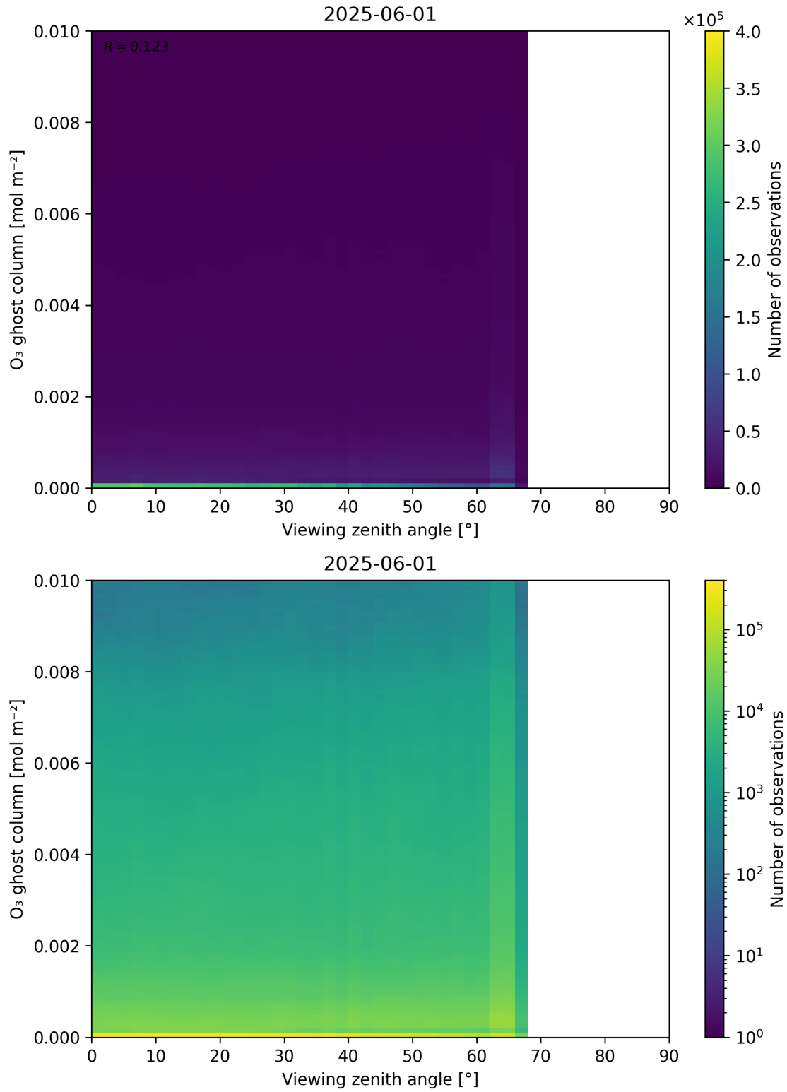
Figure 51: Scatter density plot of “Viewing zenith angle” against “O 3 ghost column” for 2025-06-01 to 2025-06-02.
