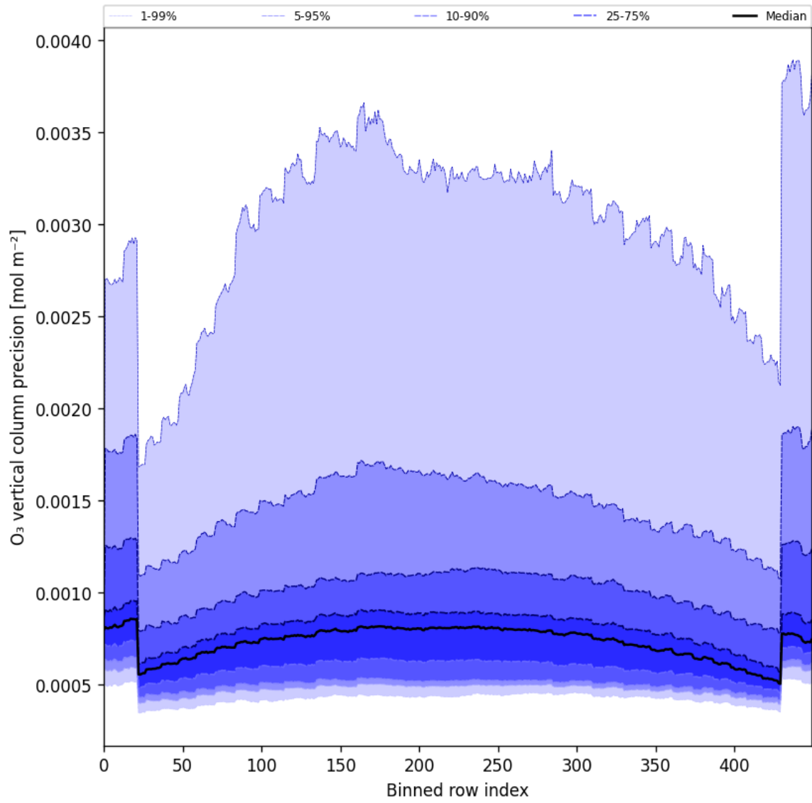
Figure 29: Along track statistics of “O 3 vertical column precision” for 2025-06-01 to 2025-06-03
