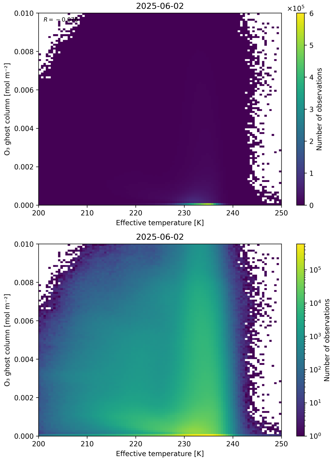
Figure 38: Scatter density plot of “Effective temperature” against “O 3 ghost column” for 2025-06-01 to 2025-06-03.
