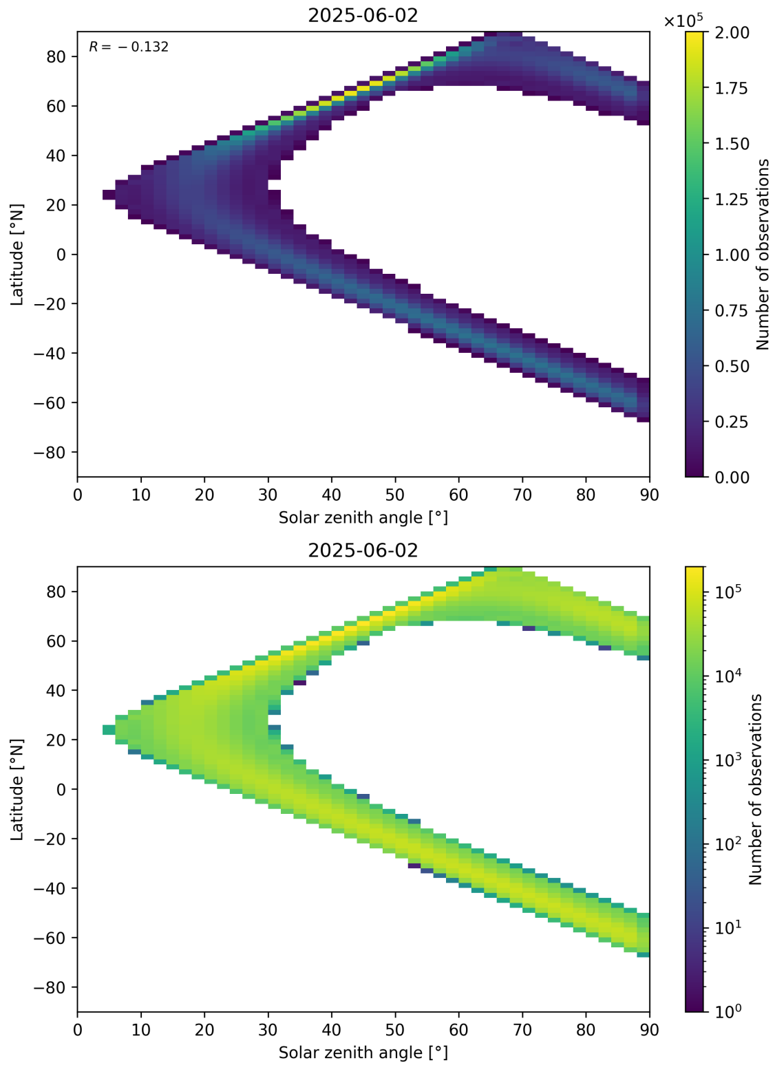
Figure 44: Scatter density plot of “Solar zenith angle” against “Latitude” for 2025-06-01 to 2025-06-03.
