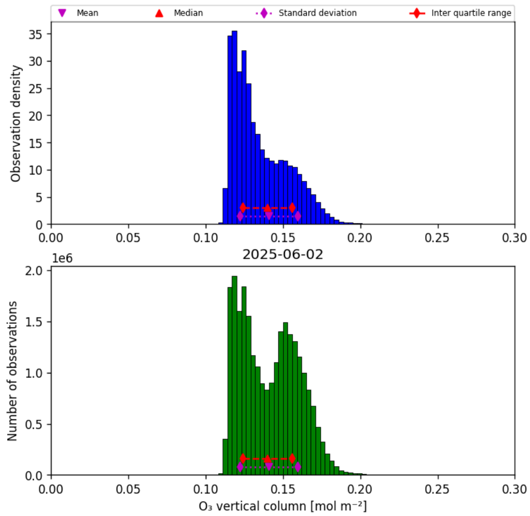
Figure 21: Histogram of “O 3 vertical column” for 2025-06-01 to 2025-06-03
