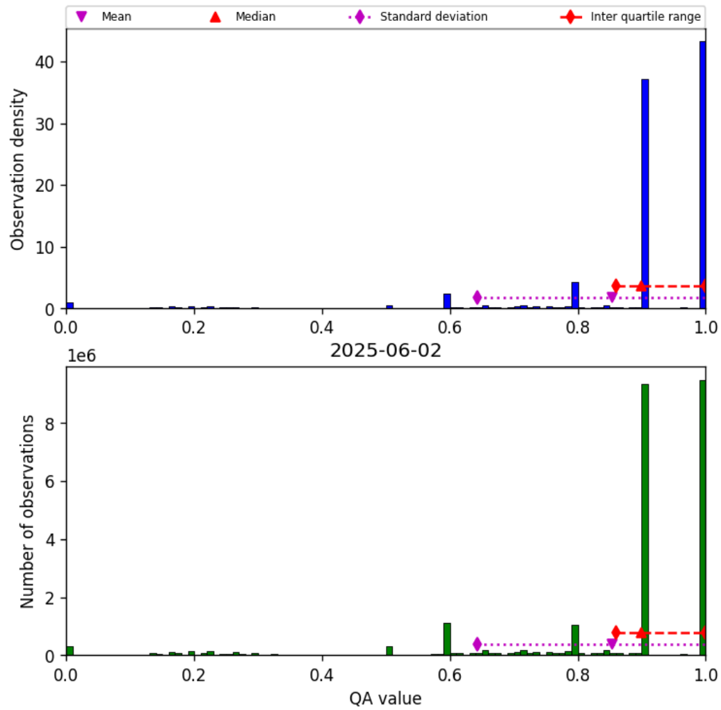
Figure 20: Histogram of “QA value” for 2025-06-01 to 2025-06-03
