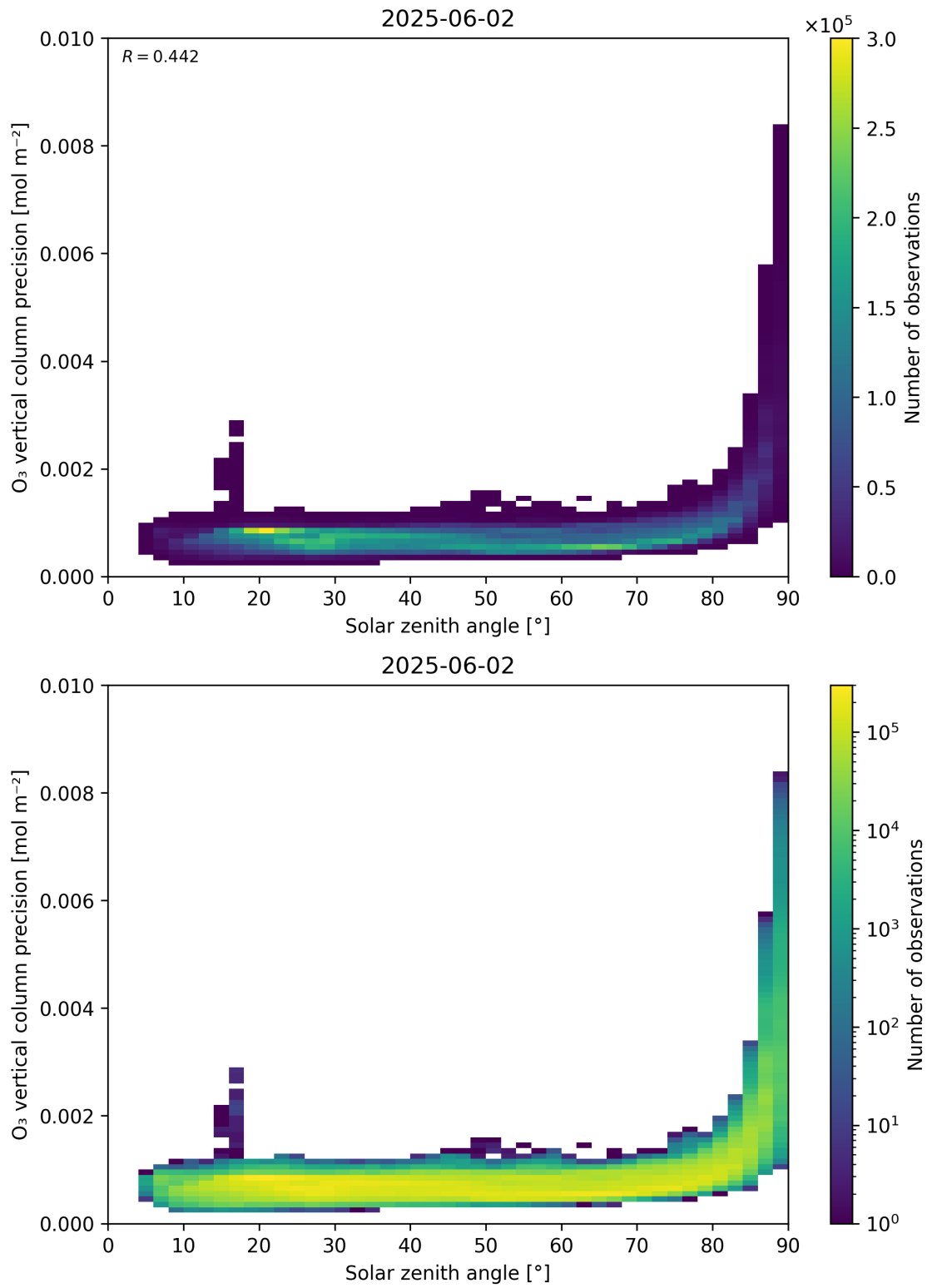
Figure 48: Scatter density plot of “Solar zenith angle” against “O 3 vertical column precision” for 2025-06-01 to 2025-06-03.
