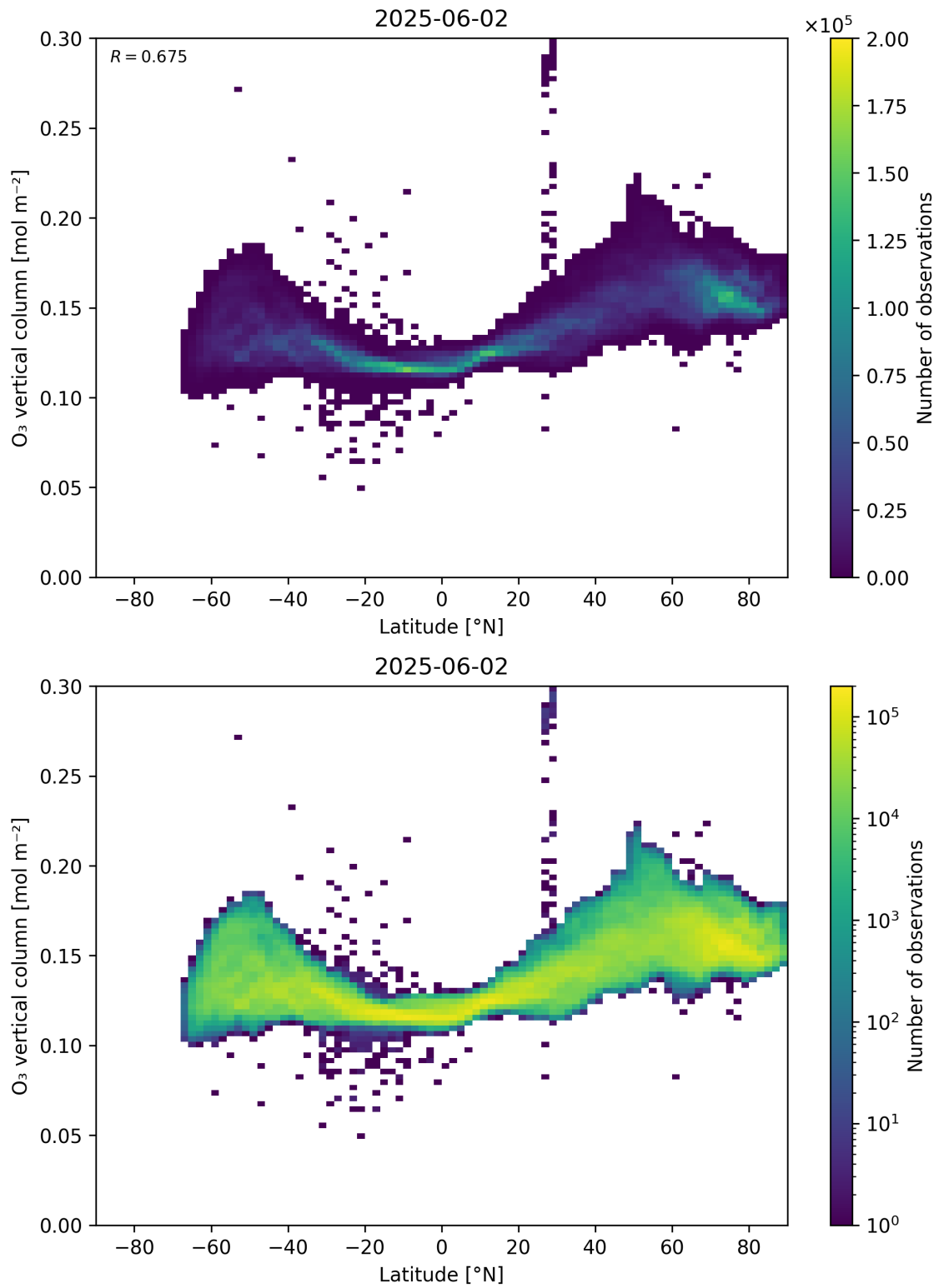
Figure 36: Scatter density plot of “Latitude” against “O 3 vertical column” for 2025-06-01 to 2025-06-03.
