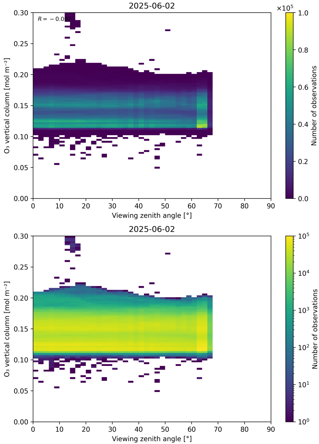
Figure 52: Scatter density plot of “Viewing zenith angle” against “O 3 vertical column” for 2025-06-01 to 2025-06-03.
