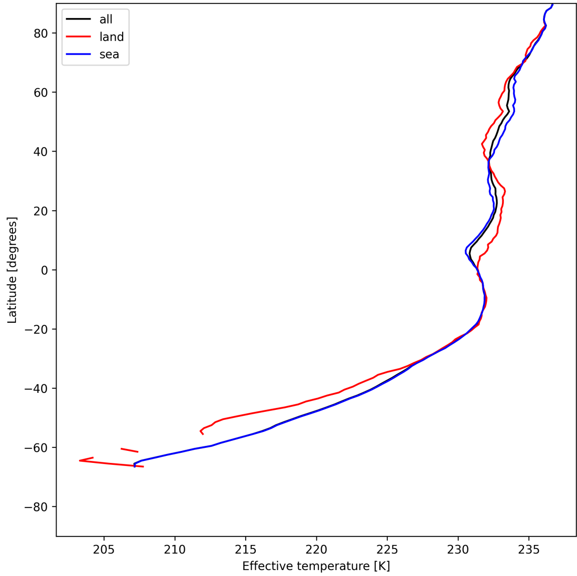
Figure 17: Zonal average of "Effective temperature" for 2025-06-01 to 2025-06-03.
