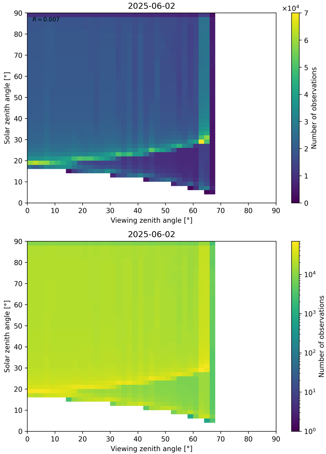
Figure 54: Scatter density plot of “Viewing zenith angle” against “Solar zenith angle” for 2025-06-01 to 2025-06-03.
