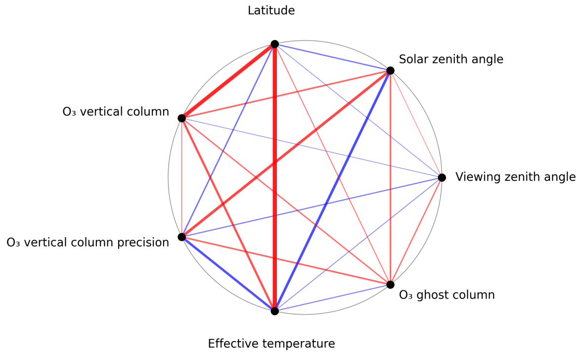
Figure 1: Map of correlation graph for 2025-06-01 to 2025-06-03.
