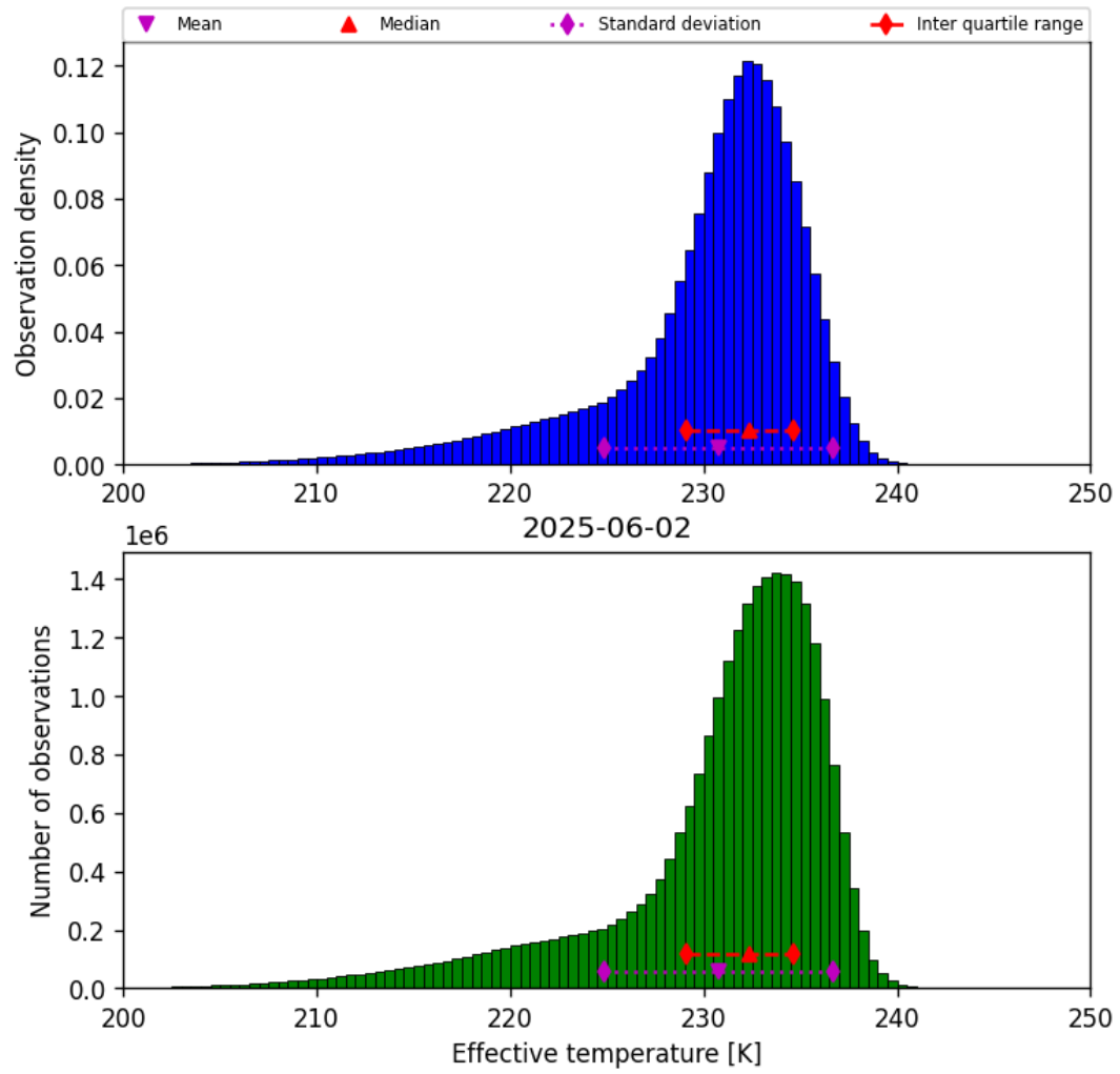
Figure 24: Histogram of “Effective temperature” for 2025-06-01 to 2025-06-03
