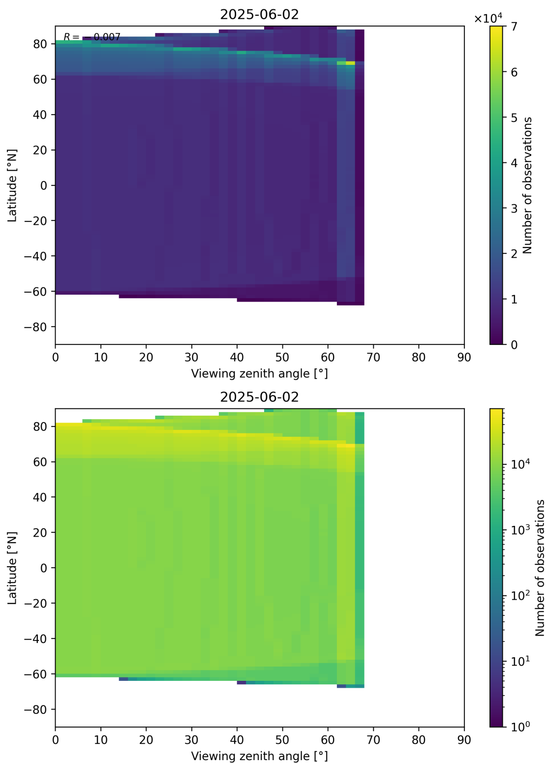
Figure 49: Scatter density plot of “Viewing zenith angle” against “Latitude” for 2025-06-01 to 2025-06-03.
