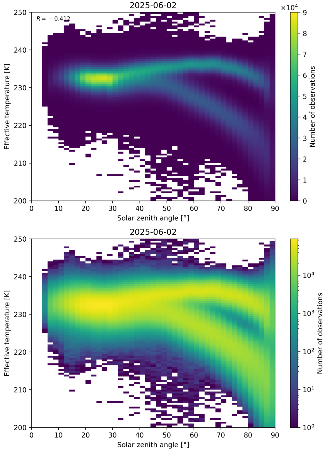
Figure 45: Scatter density plot of “Solar zenith angle” against “Effective temperature” for 2025-06-01 to 2025-06-03.
