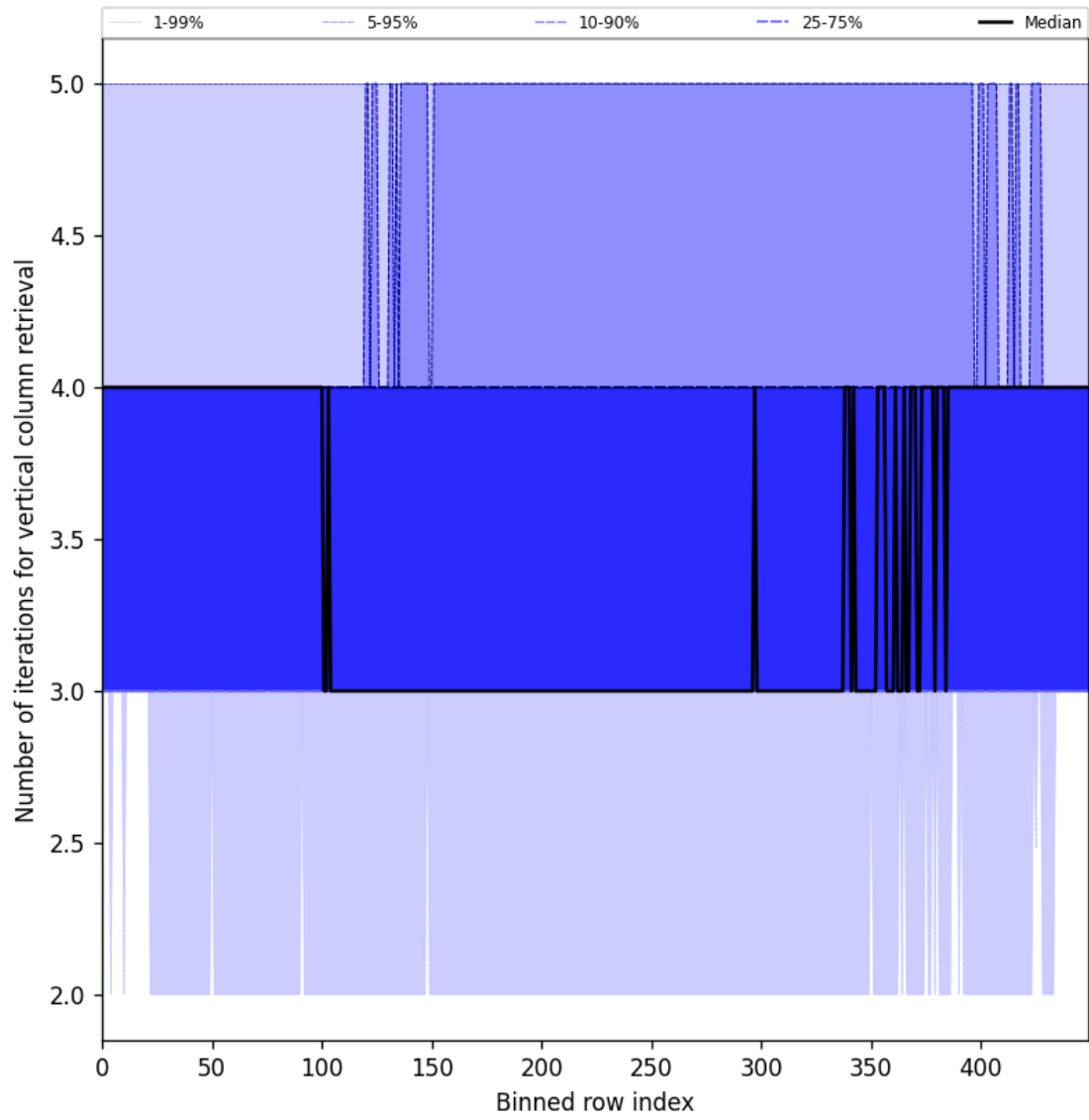
Figure 33: Along track statistics of “Number of iterations for vertical column retrieval” for 2025-06-01 to 2025-06-03
