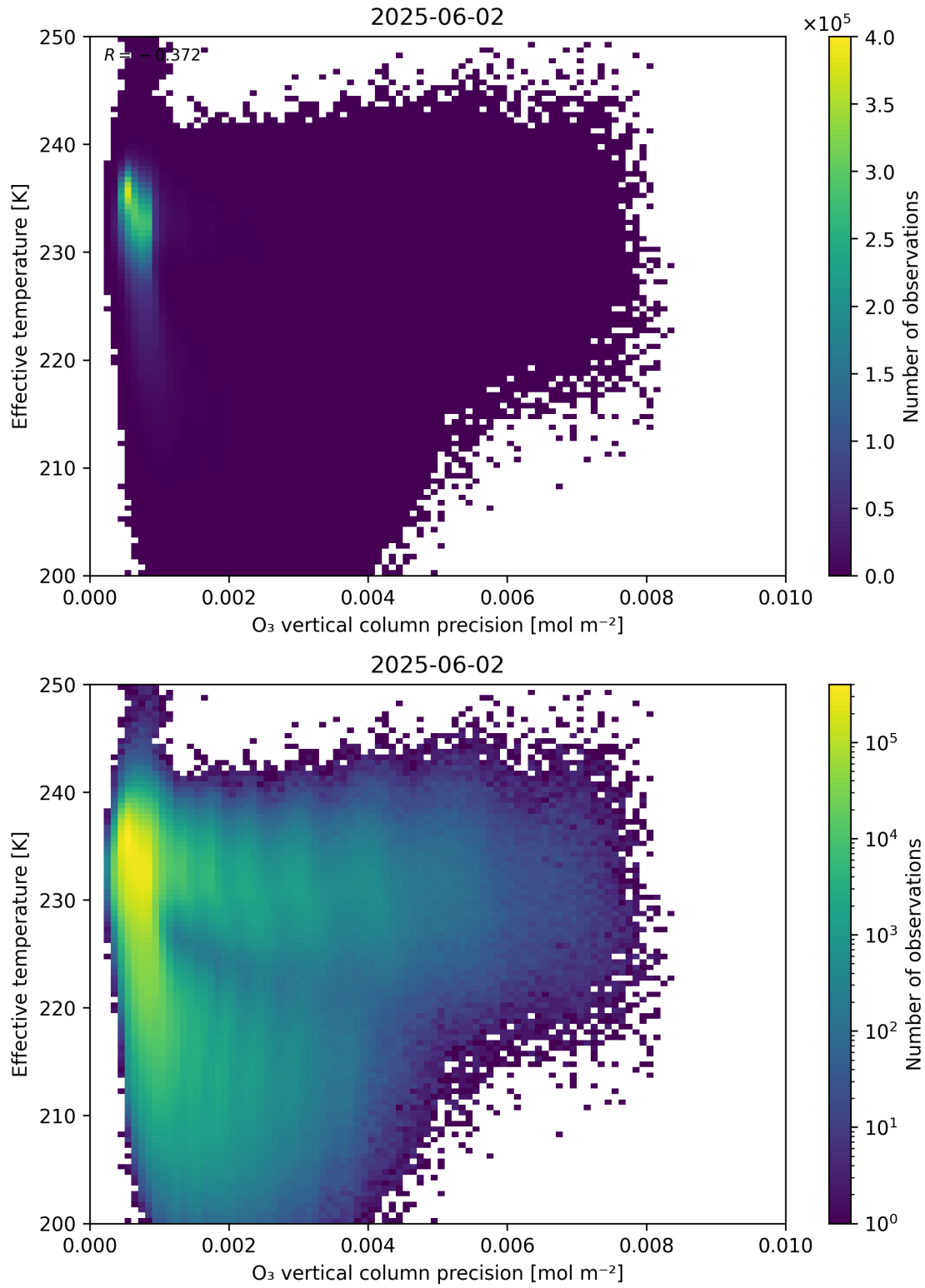
Figure 42: Scatter density plot of “O 3 vertical column precision” against “Effective temperature” for 2025-06-01 to 2025-06-03.
