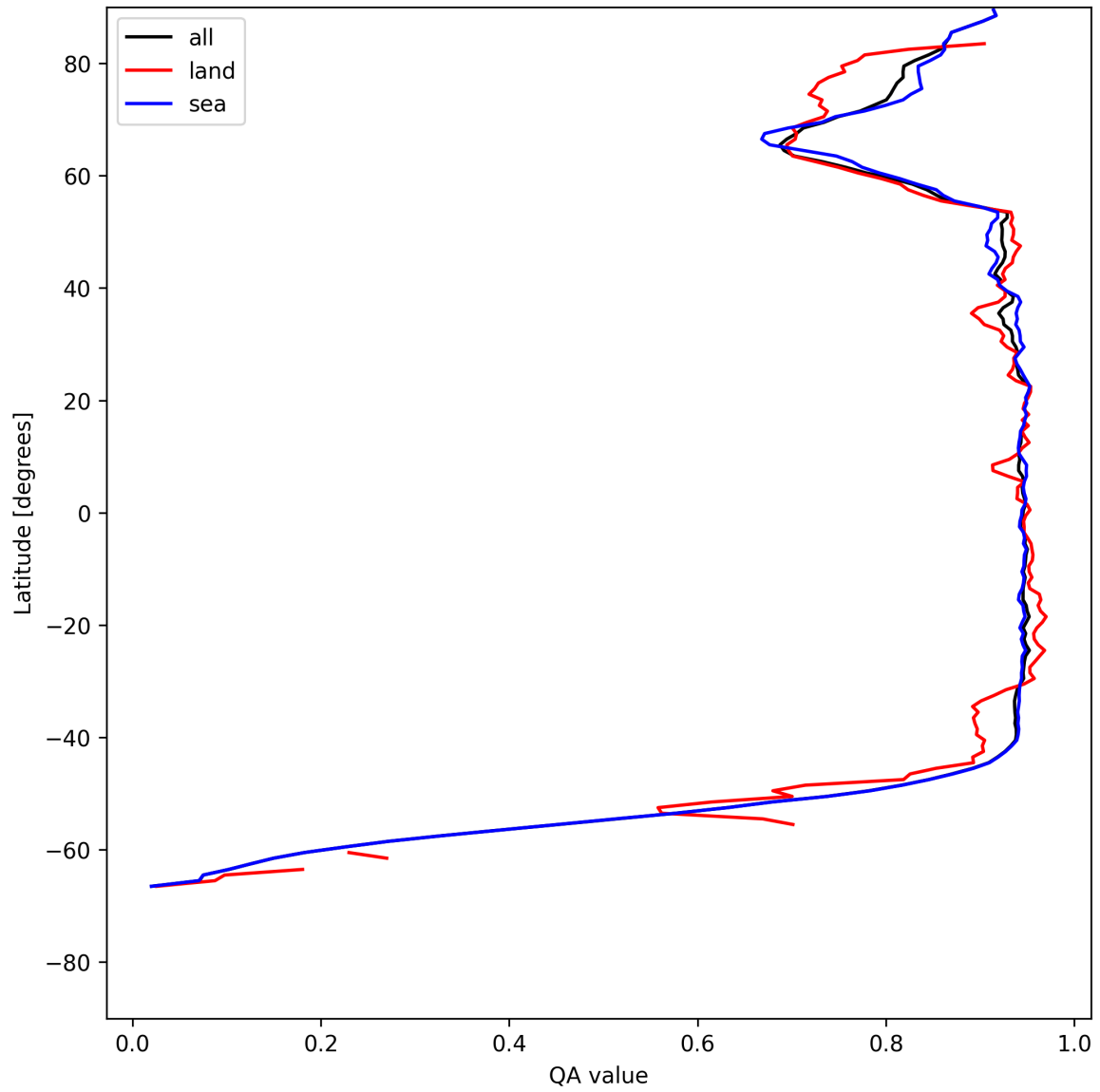
Figure 13: Zonal average of “QA value” for 2025-06-01 to 2025-06-03.
