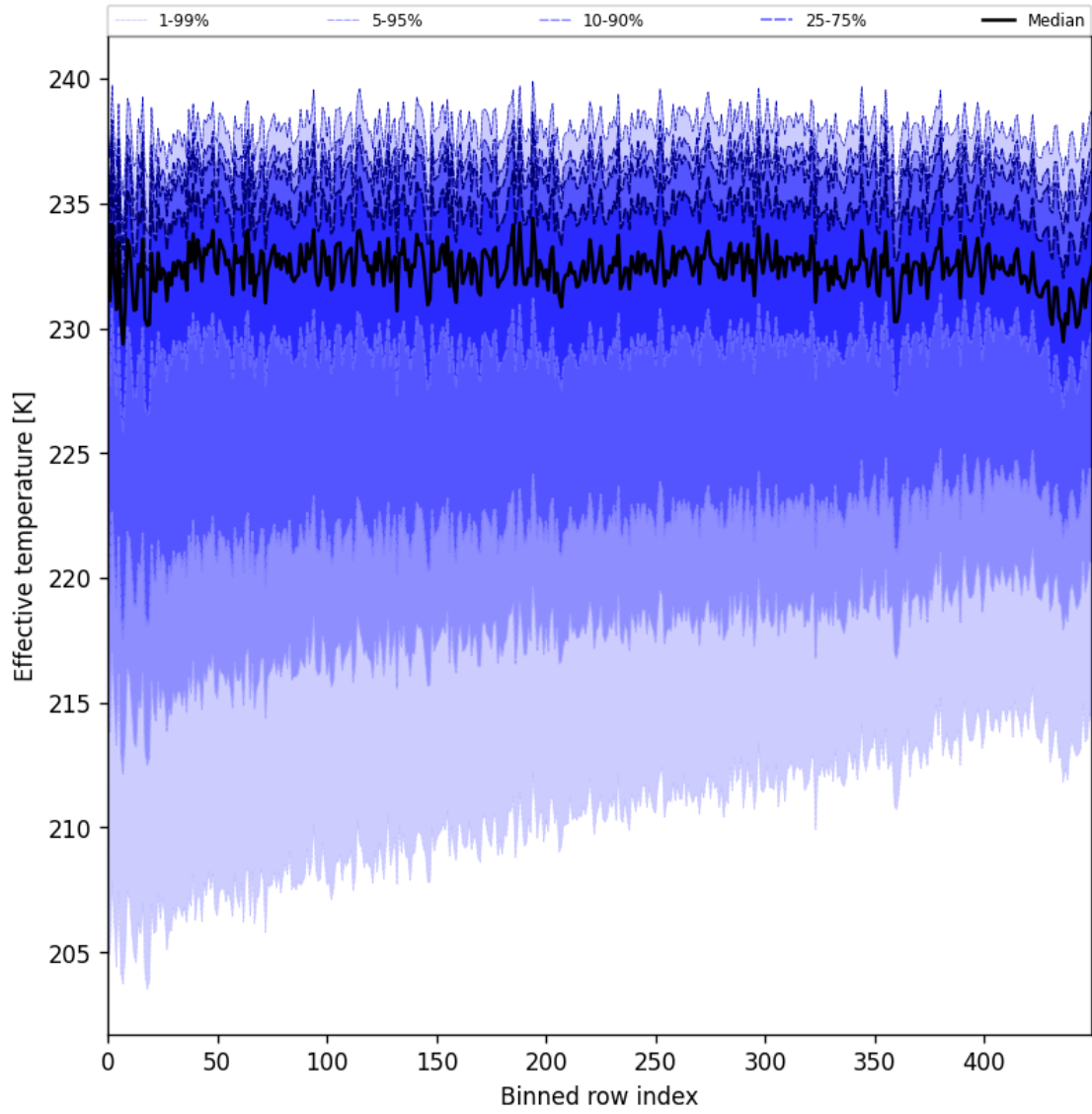
Figure 31: Along track statistics of “Effective temperature” for 2025-06-01 to 2025-06-03
