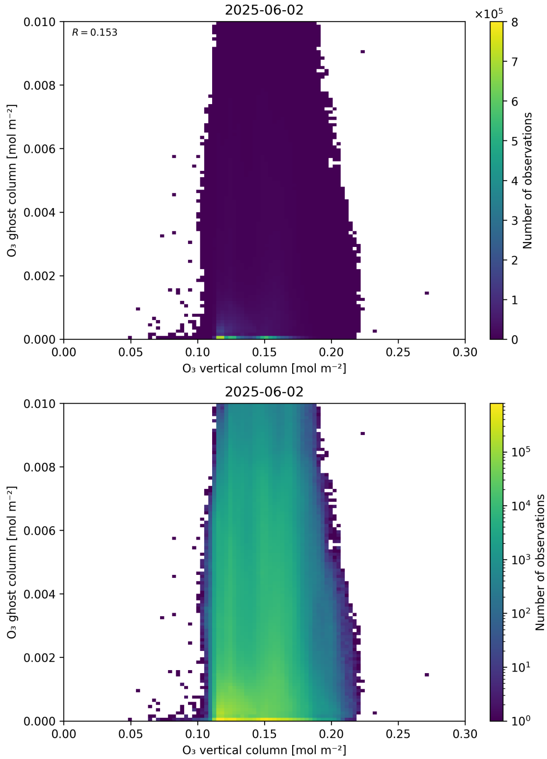
Figure 40: Scatter density plot of “O 3 vertical column” against “O 3 ghost column” for 2025-06-01 to 2025-06-03.
