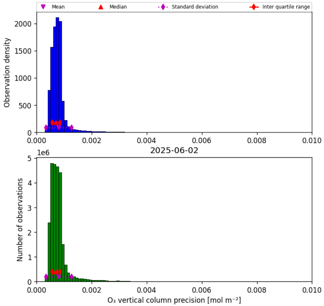
Figure 22: Histogram of “O 3 vertical column precision” for 2025-06-01 to 2025-06-03
