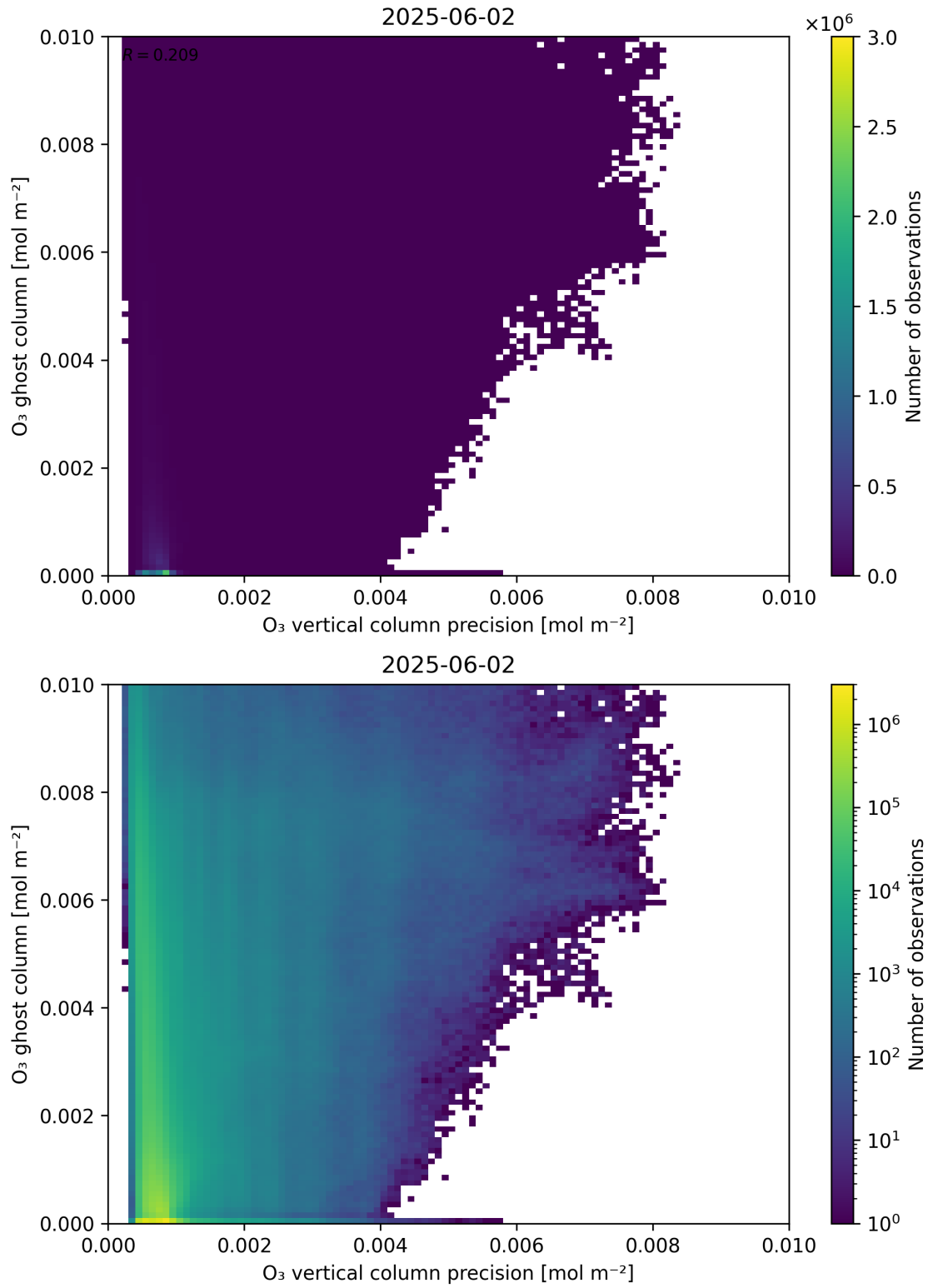
Figure 43: Scatter density plot of “ \text{O}_3 vertical column precision” against “ \text{O}_3 ghost column” for 2025-06-01 to 2025-06-03.
