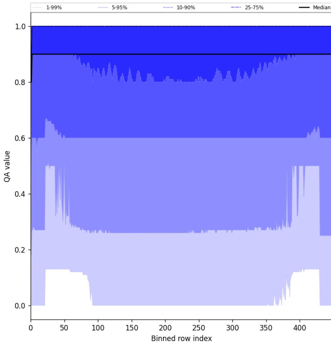
Figure 27: Along track statistics of “QA value” for 2025-06-01 to 2025-06-03
