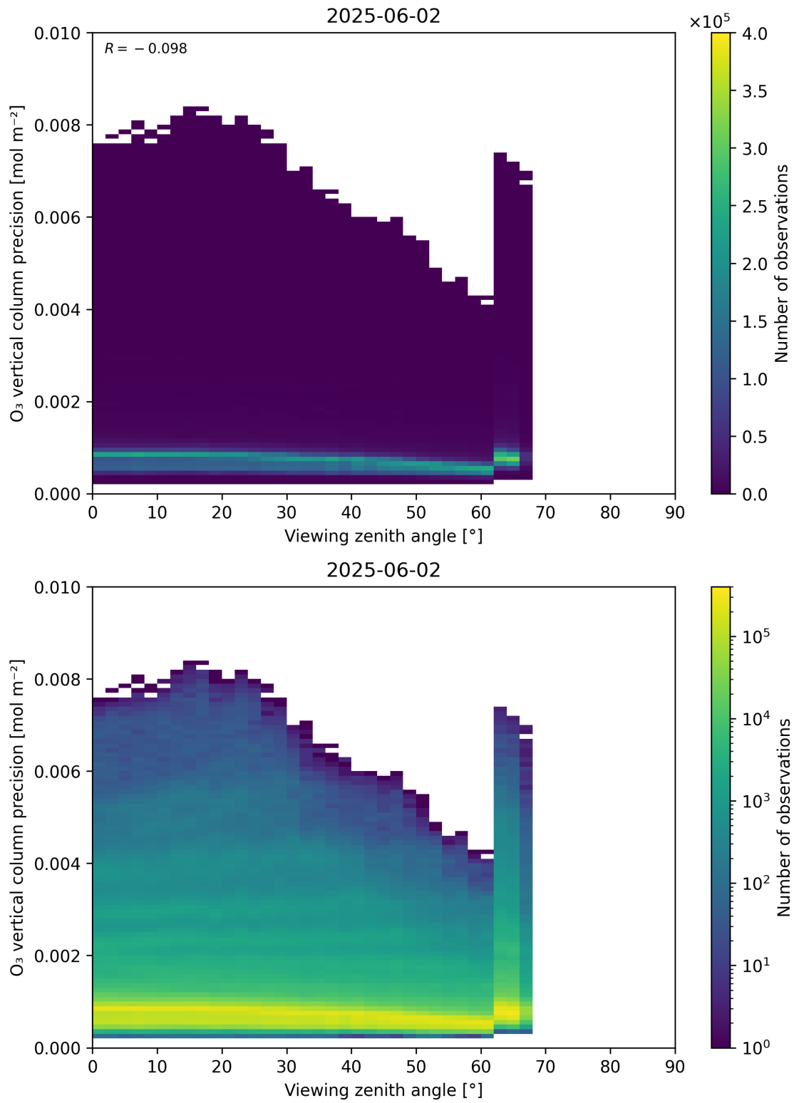
Figure 53: Scatter density plot of “Viewing zenith angle” against “O 3 vertical column precision” for 2025-06-01 to 2025-06-03.
