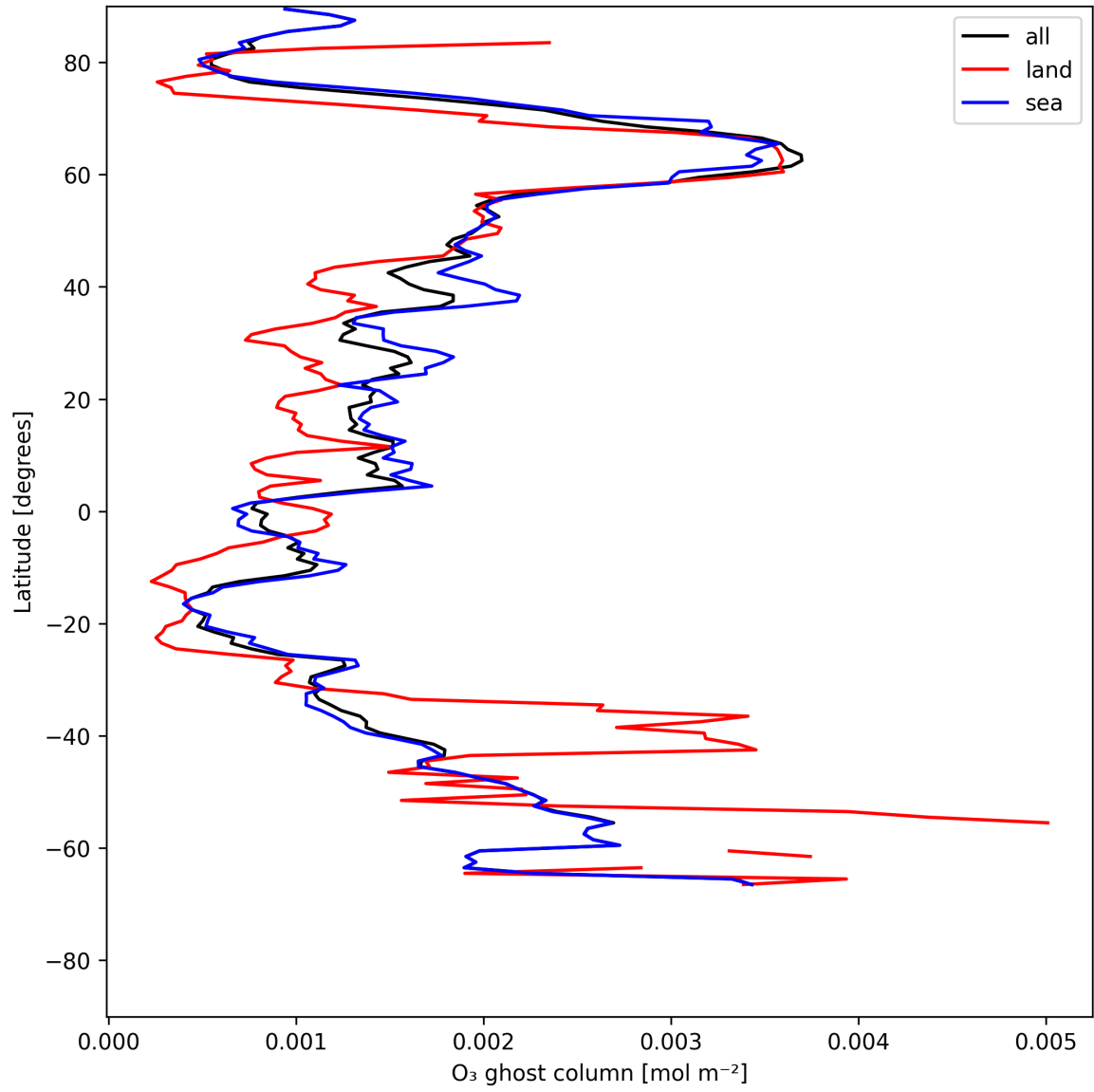
Figure 18: Zonal average of "O 3 ghost column" for 2025-06-01 to 2025-06-03.
