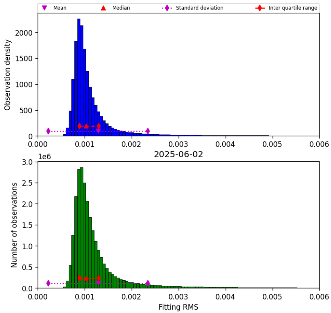
Figure 23: Histogram of “Fitting RMS” for 2025-06-01 to 2025-06-03
