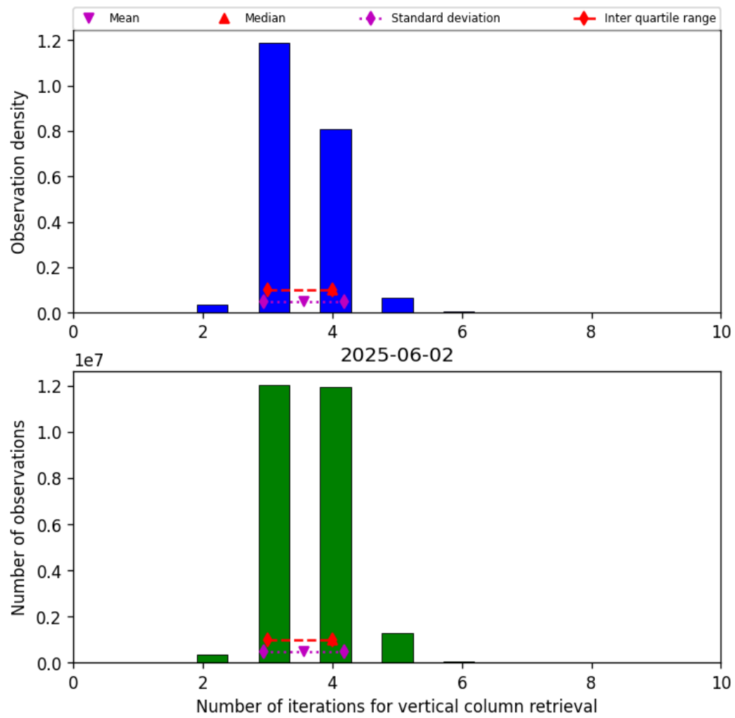
Figure 26: Histogram of “Number of iterations for vertical column retrieval” for 2025-06-01 to 2025-06-03
