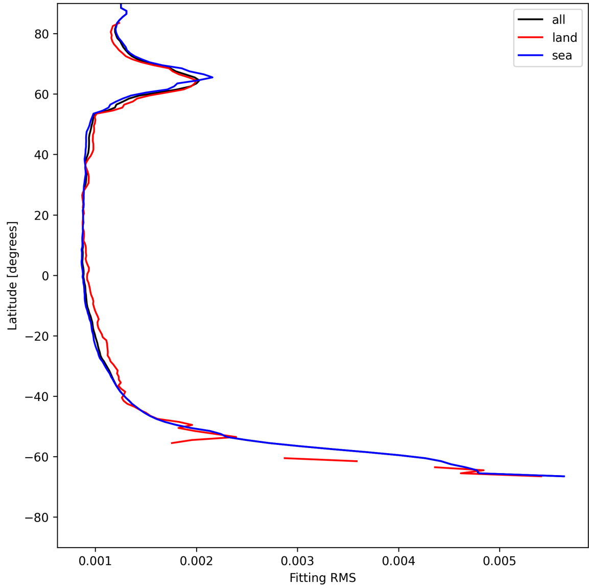
Figure 16: Zonal average of “Fitting RMS” for 2025-06-01 to 2025-06-03.
