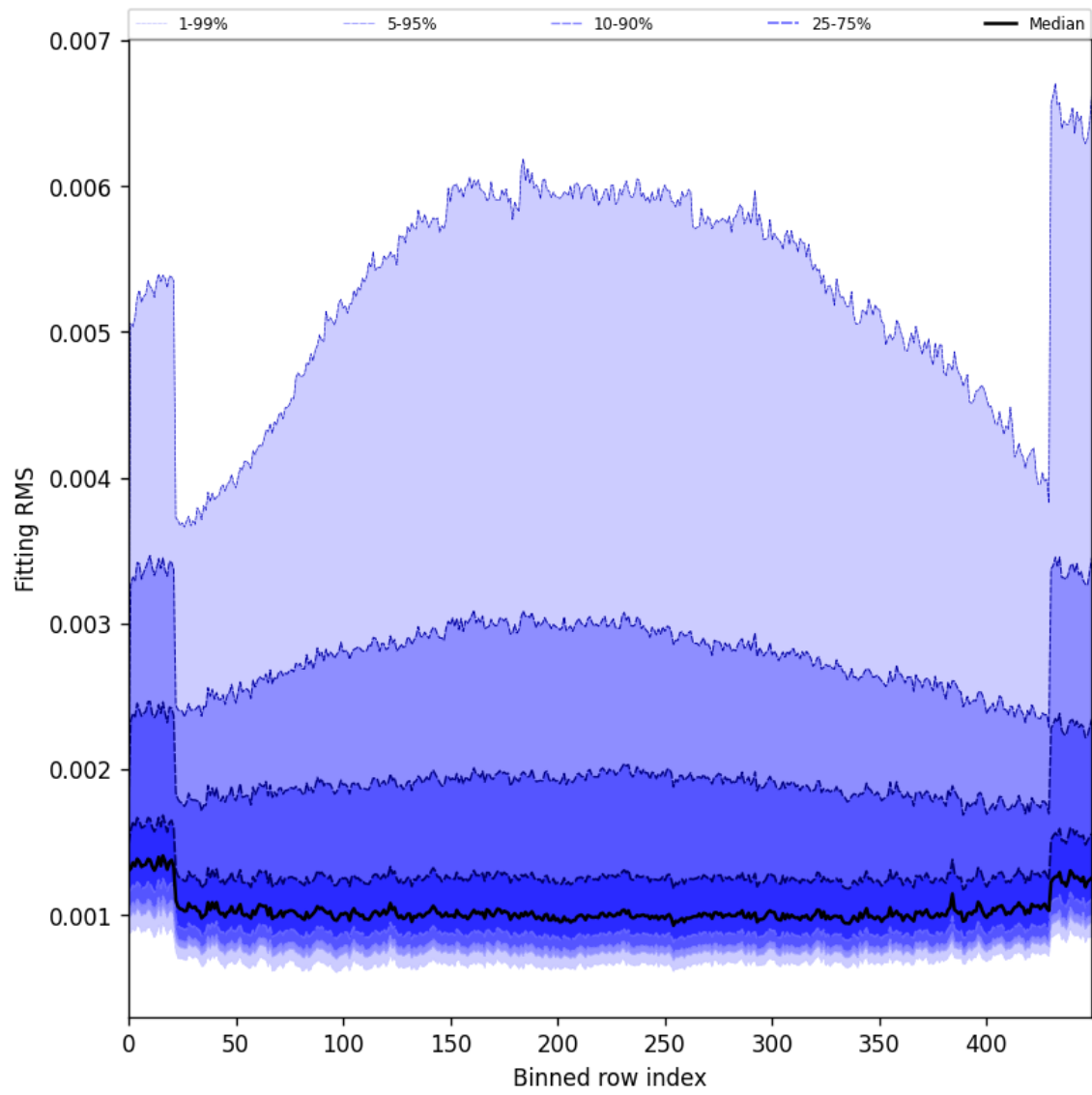
Figure 30: Along track statistics of “Fitting RMS” for 2025-06-01 to 2025-06-03
