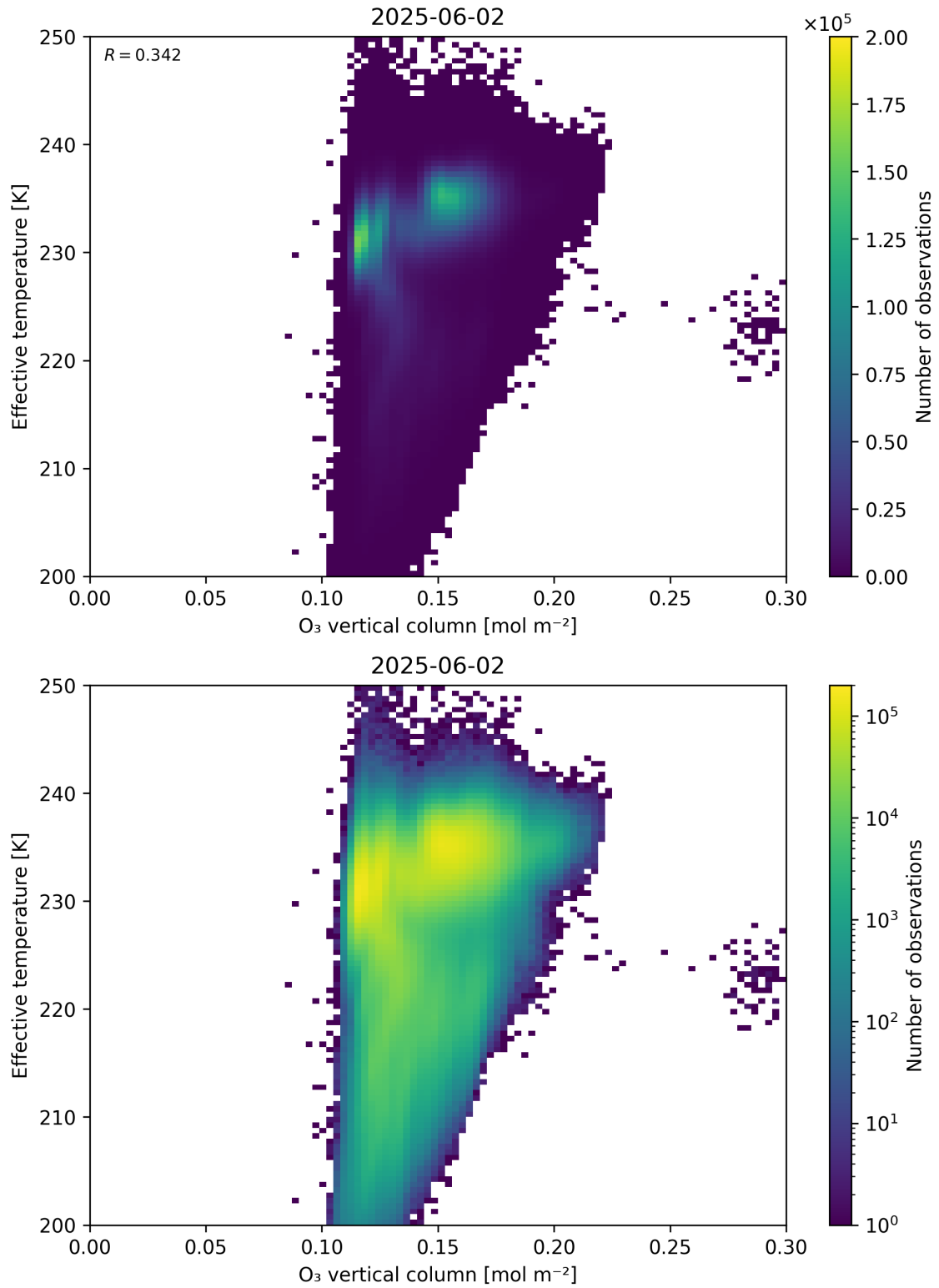
Figure 39: Scatter density plot of “O 3 vertical column” against “Effective temperature” for 2025-06-01 to 2025-06-03.
