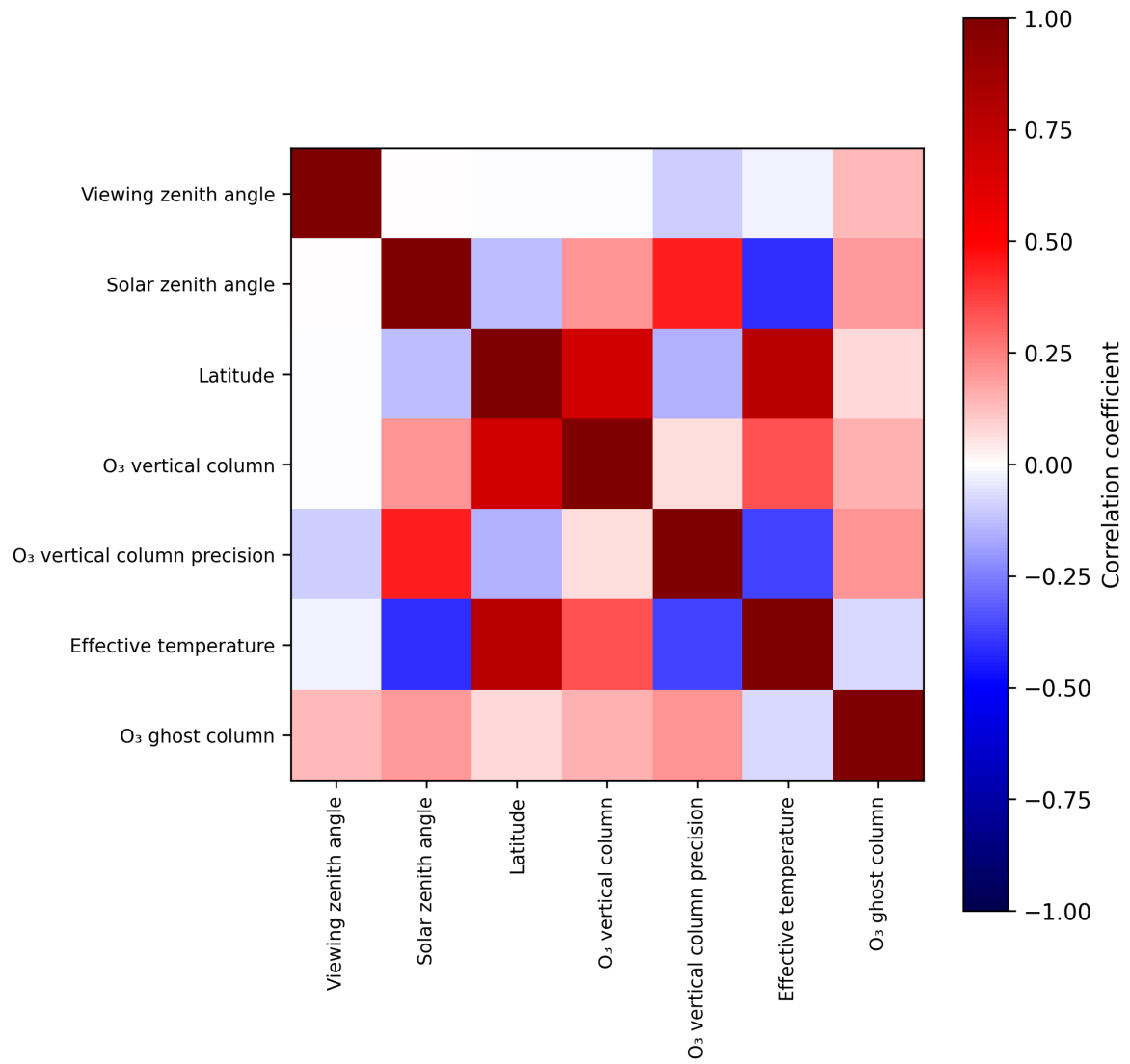
Figure 2: Map of correlation matrix for 2025-06-01 to 2025-06-03.
