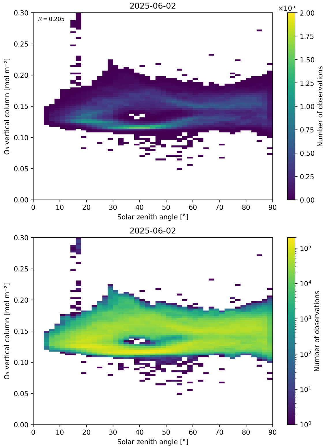
Figure 47: Scatter density plot of “Solar zenith angle” against “O 3 vertical column” for 2025-06-01 to 2025-06-03.
