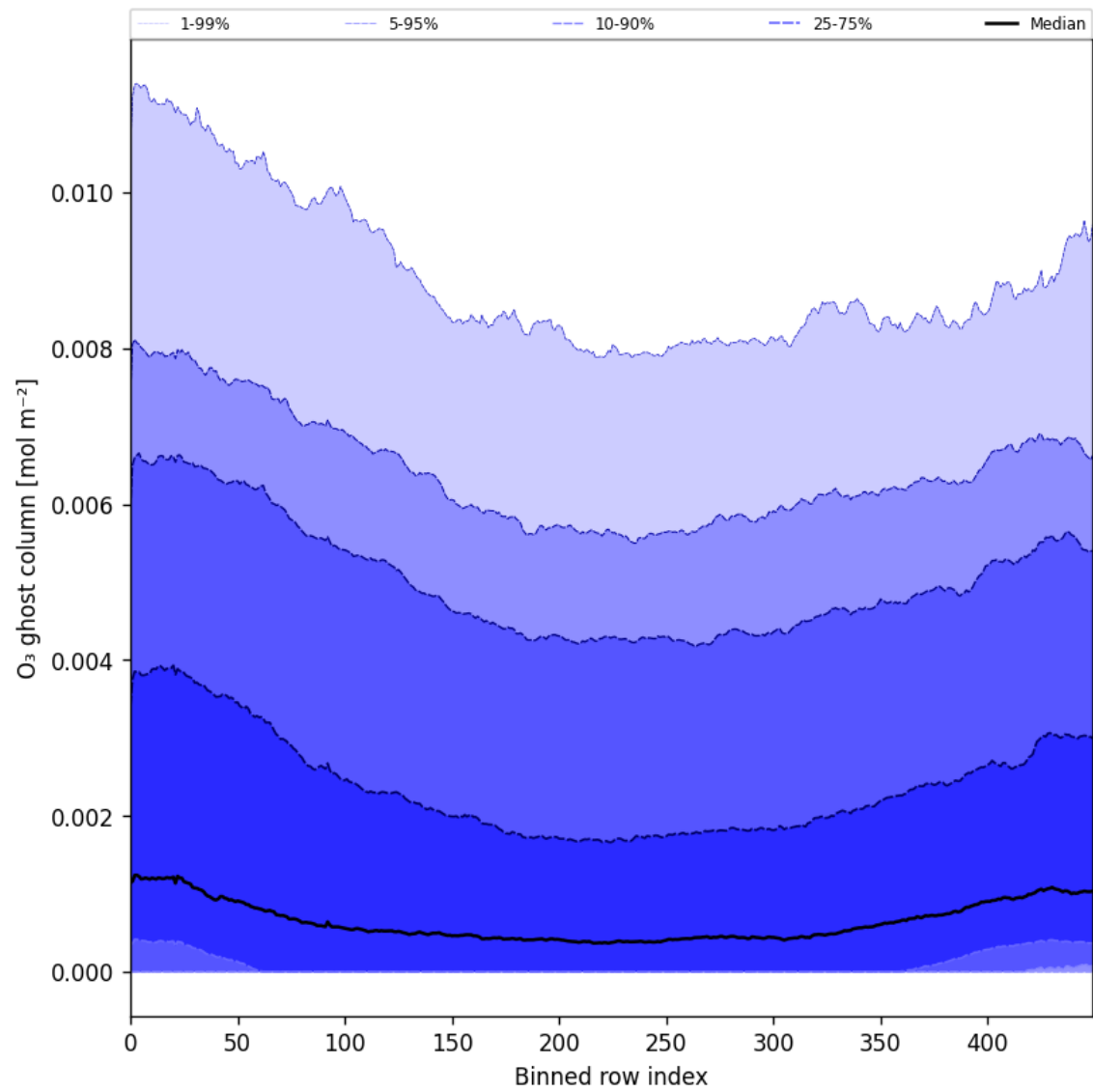
Figure 32: Along track statistics of "O 3 ghost column" for 2025-06-01 to 2025-06-03
