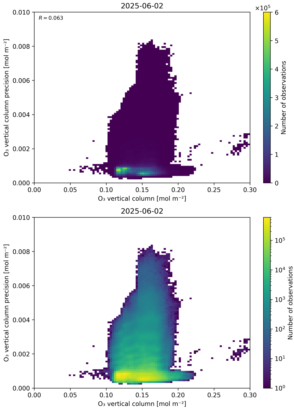
Figure 41: Scatter density plot of “O 3 vertical column” against “O 3 vertical column precision” for 2025-06-01 to 2025-06-03.
