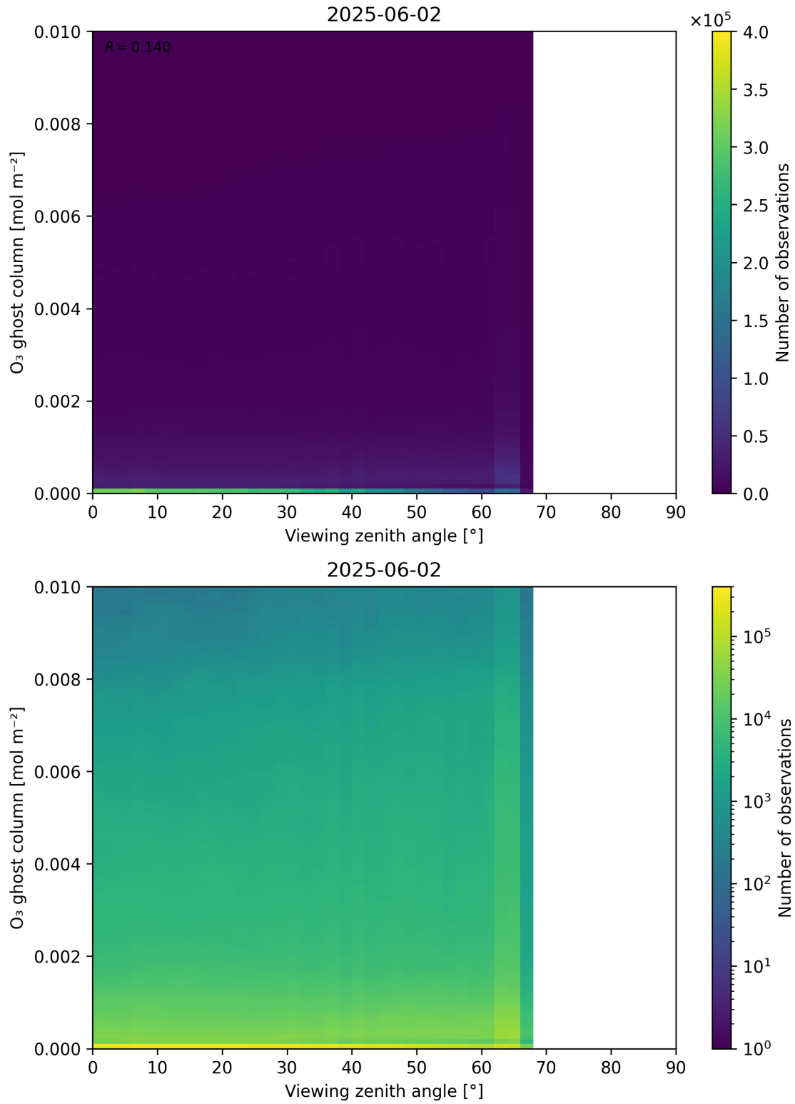
Figure 51: Scatter density plot of “Viewing zenith angle” against “O 3 ghost column” for 2025-06-01 to 2025-06-03.
