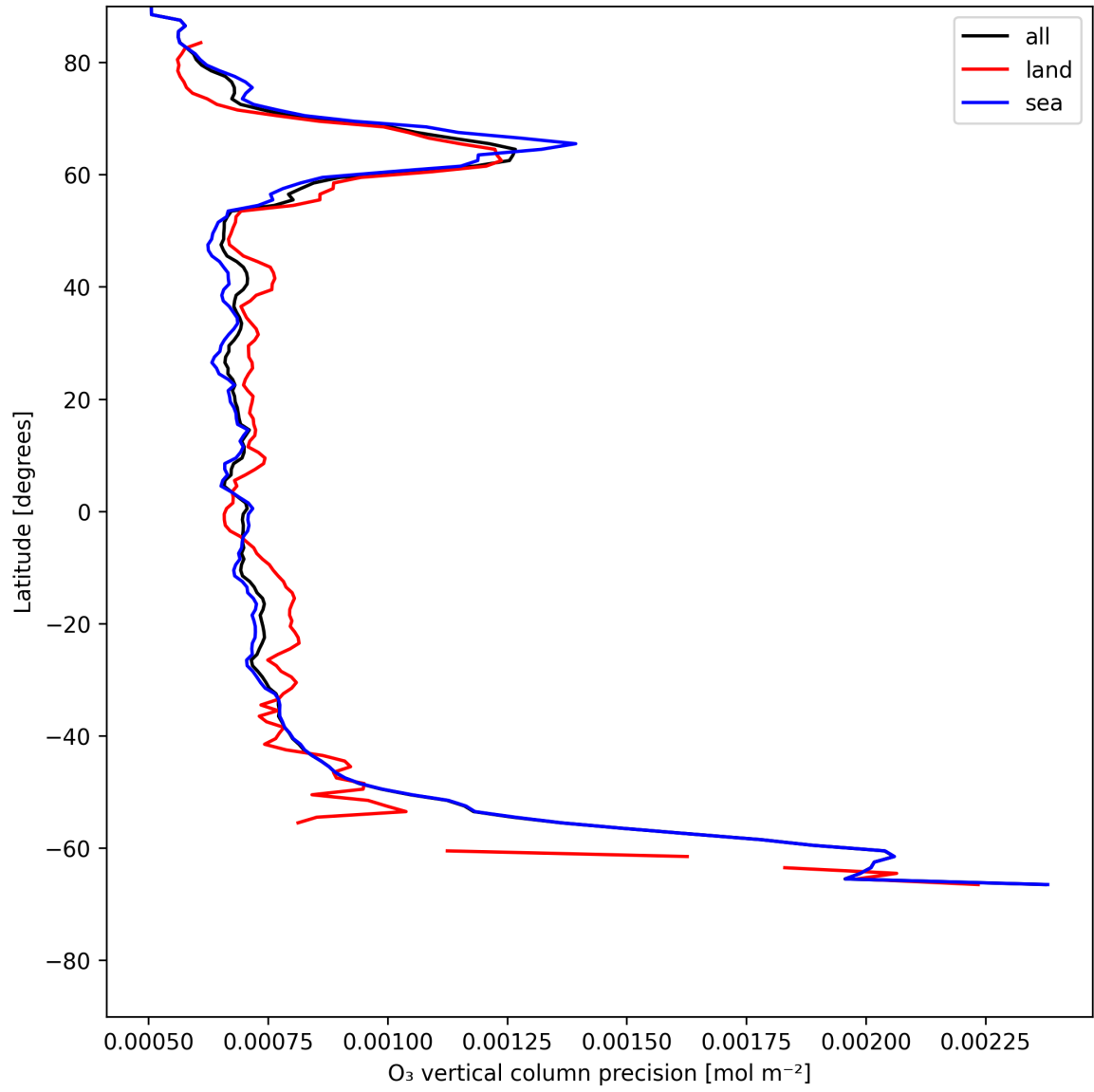
Figure 15: Zonal average of “O 3 vertical column precision” for 2025-06-01 to 2025-06-03.
