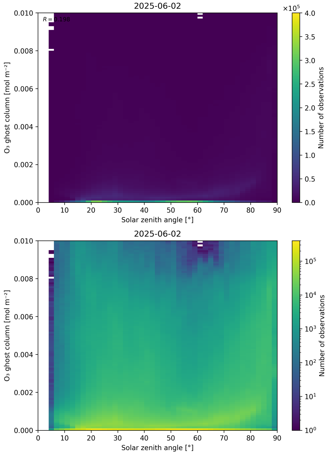
Figure 46: Scatter density plot of “Solar zenith angle” against “O 3 ghost column” for 2025-06-01 to 2025-06-03.
