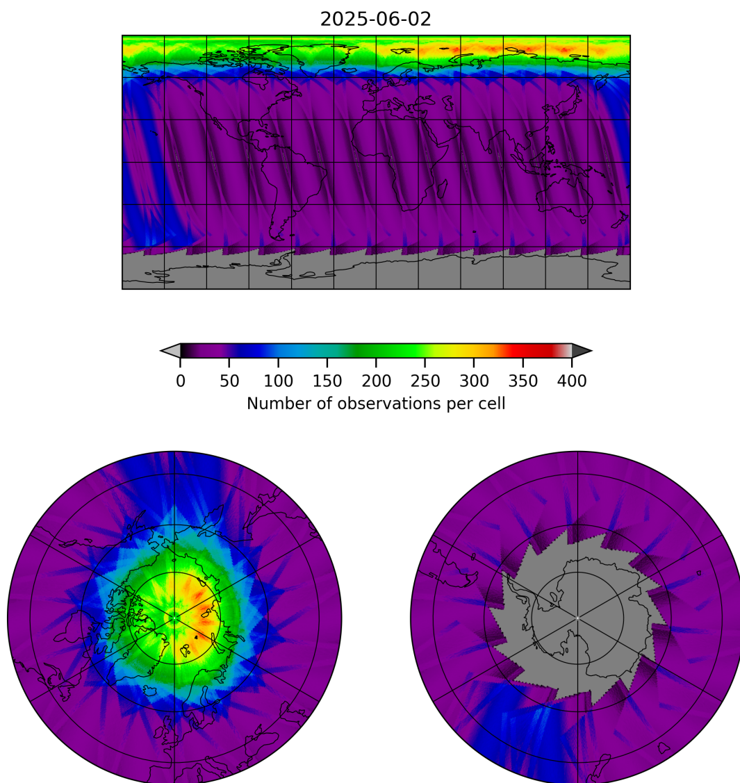
Figure 12: Map of the number of observations for 2025-06-01 to 2025-06-03
