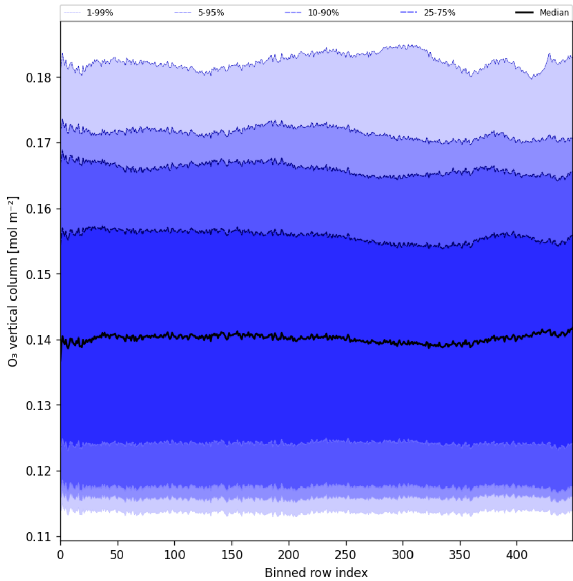
Figure 28: Along track statistics of “O 3 vertical column” for 2025-06-01 to 2025-06-03
