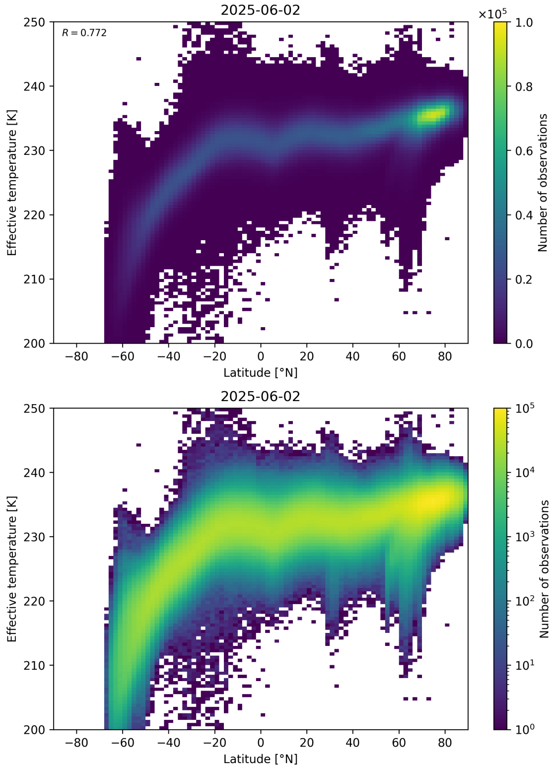
Figure 34: Scatter density plot of “Latitude” against “Effective temperature” for 2025-06-01 to 2025-06-03.
