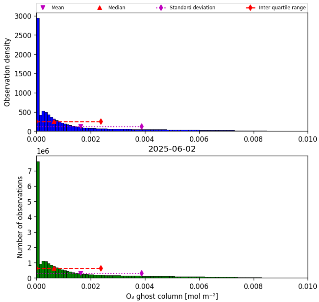
Figure 25: Histogram of “O 3 ghost column” for 2025-06-01 to 2025-06-03
