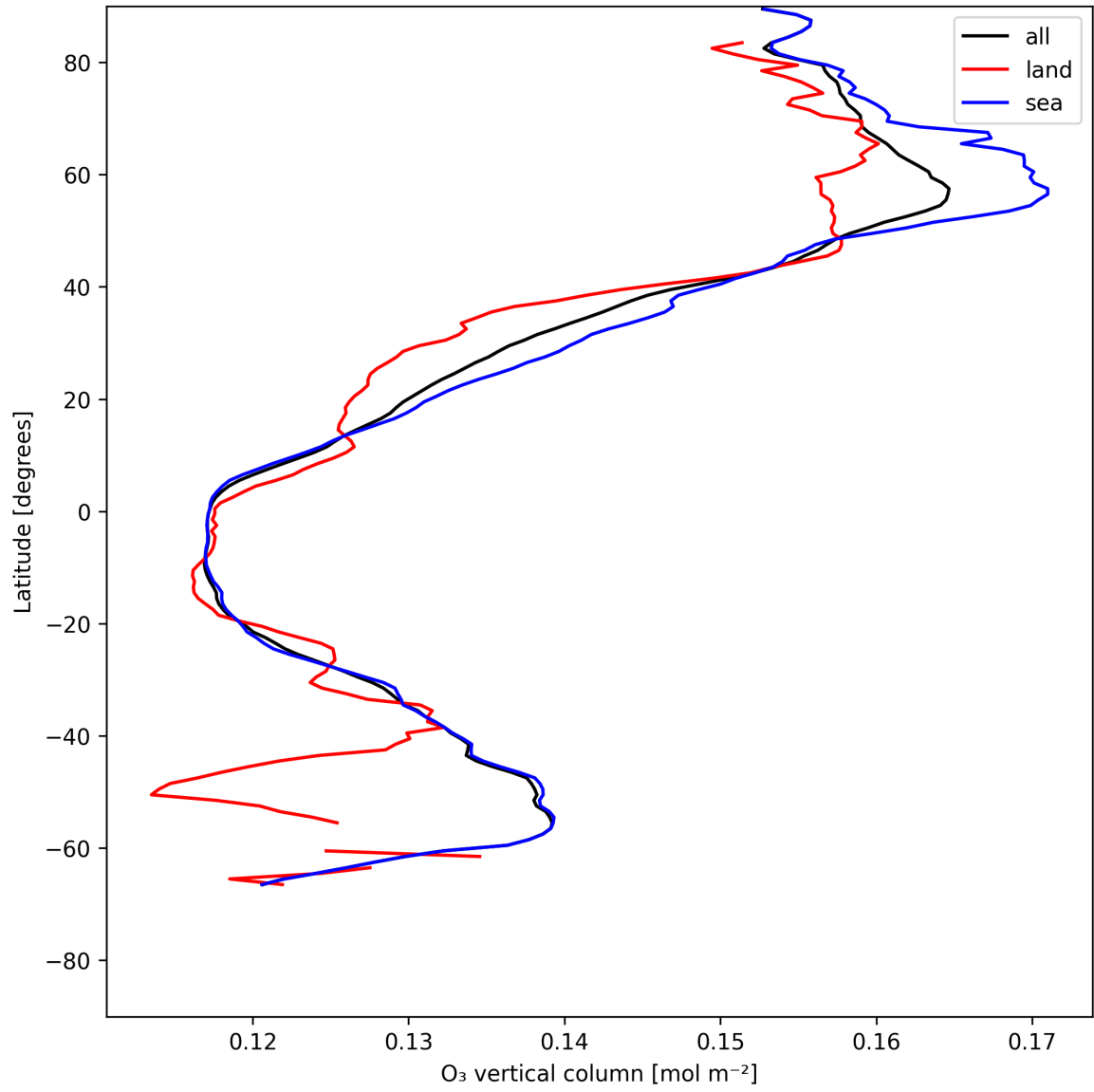
Figure 14: Zonal average of “O 3 vertical column” for 2025-06-01 to 2025-06-03.
