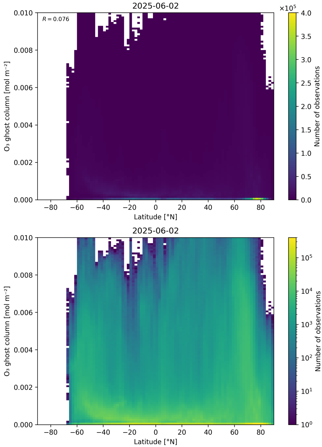
Figure 35: Scatter density plot of “Latitude” against “O 3 ghost column” for 2025-06-01 to 2025-06-03.
