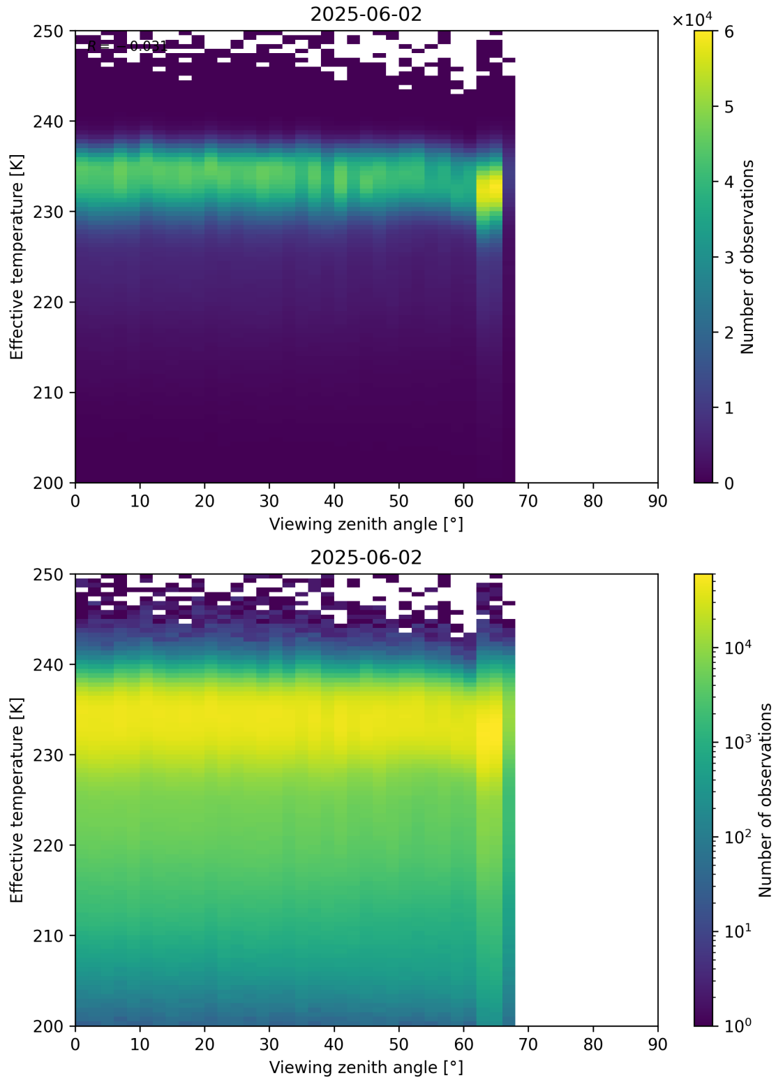
Figure 50: Scatter density plot of “Viewing zenith angle” against “Effective temperature” for 2025-06-01 to 2025-06-03.
