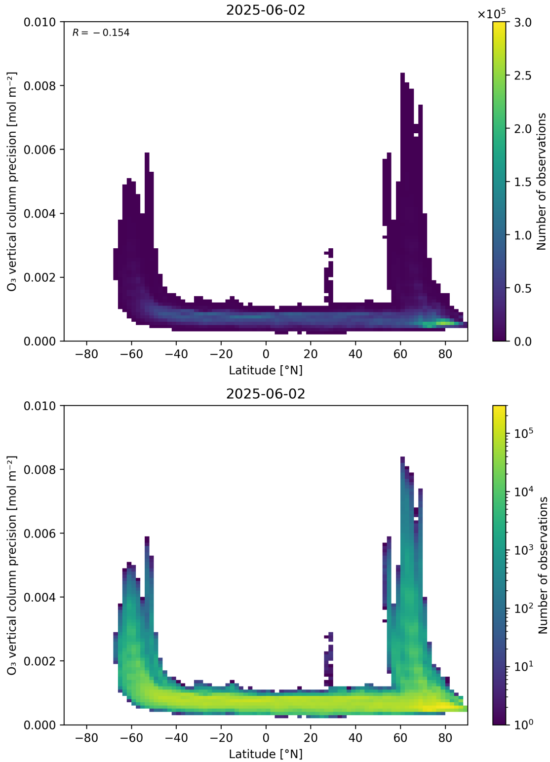
Figure 37: Scatter density plot of “Latitude” against “O 3 vertical column precision” for 2025-06-01 to 2025-06-03.
