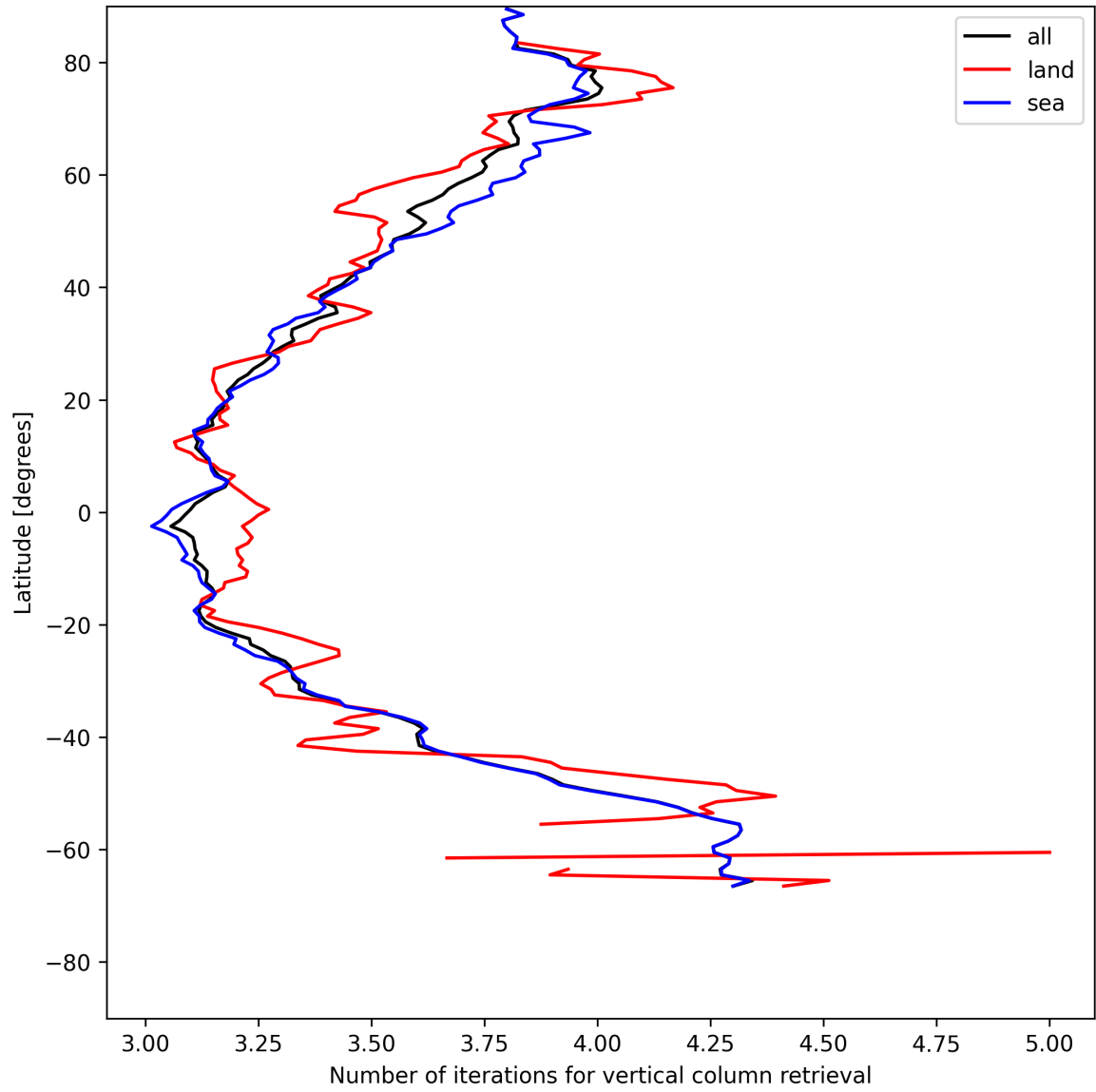
Figure 19: Zonal average of “Number of iterations for vertical column retrieval” for 2025-06-01 to 2025-06-03.
