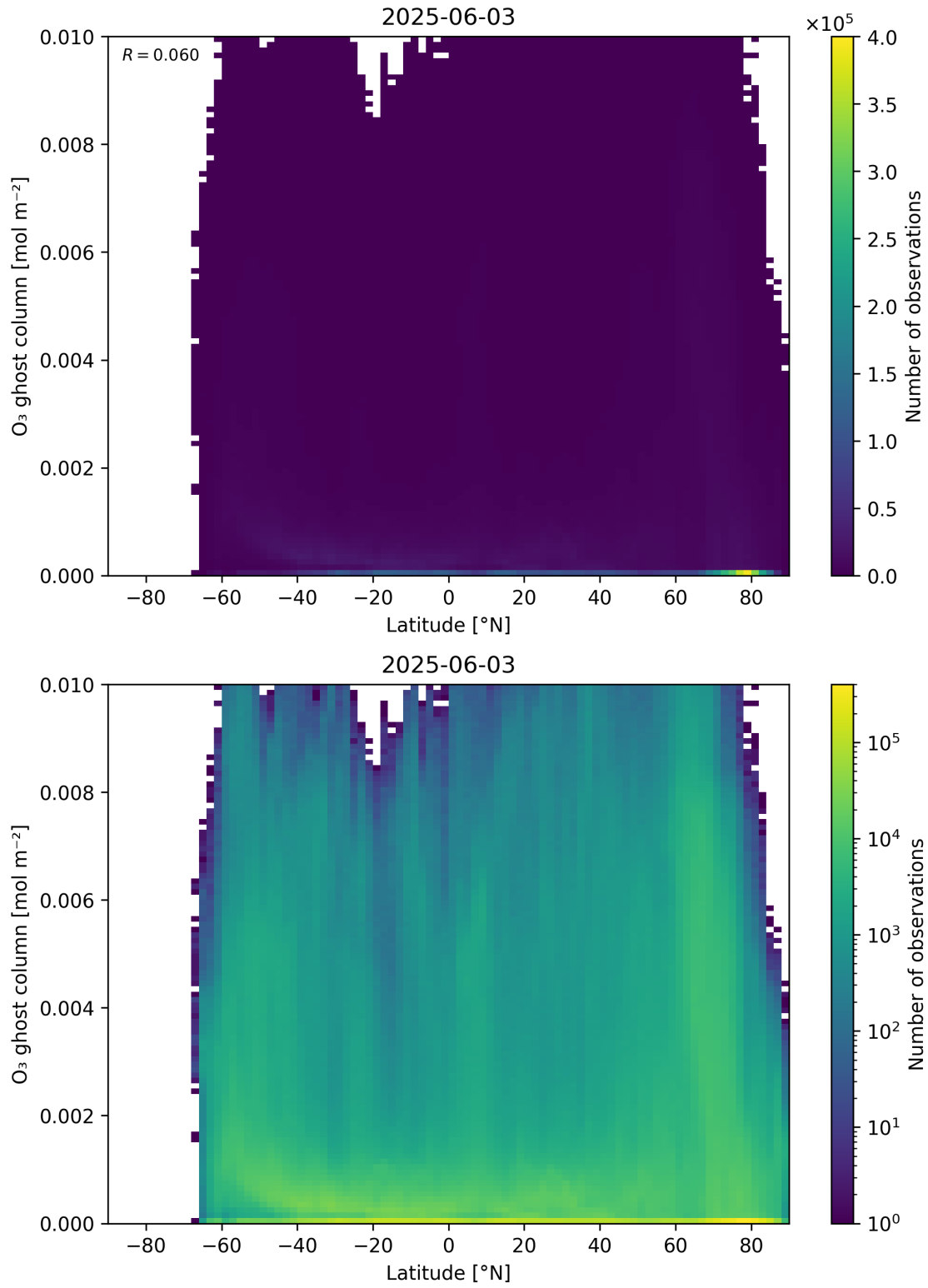
Figure 35: Scatter density plot of “Latitude” against “O 3 ghost column” for 2025-06-02 to 2025-06-04.
