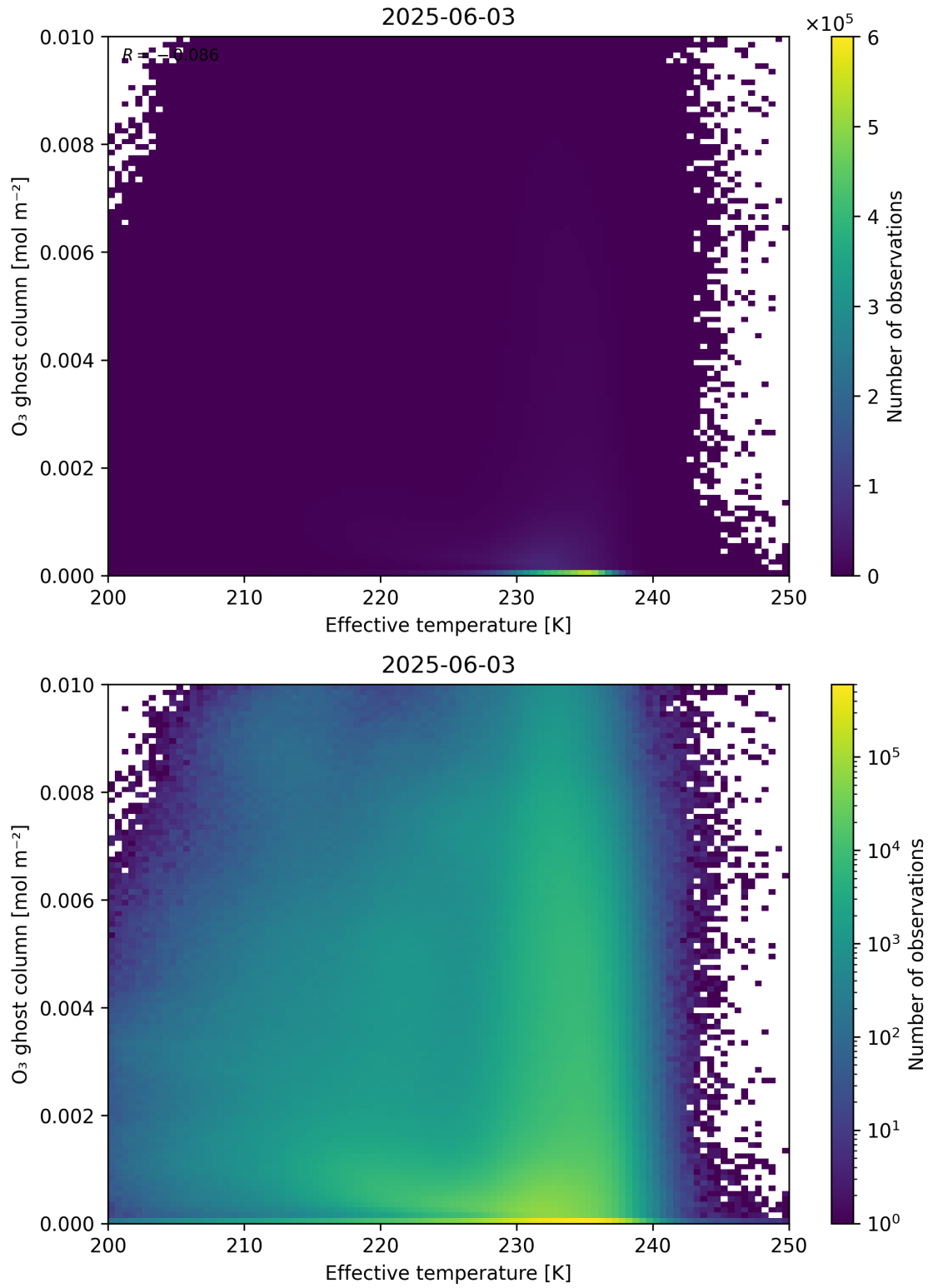
Figure 38: Scatter density plot of “Effective temperature” against “O 3 ghost column” for 2025-06-02 to 2025-06-04.
