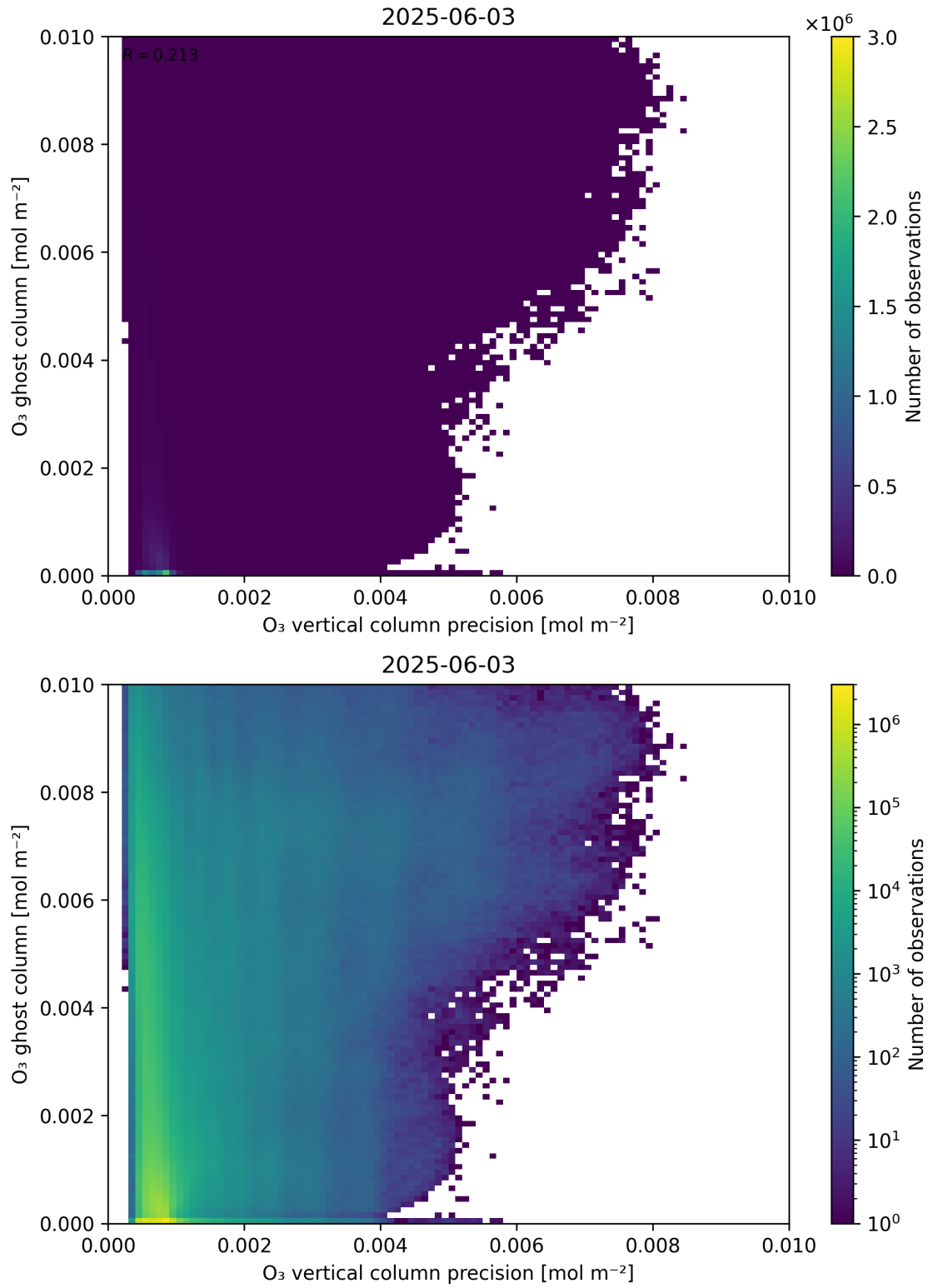
Figure 43: Scatter density plot of “ \text{O}_3 vertical column precision” against “ \text{O}_3 ghost column” for 2025-06-02 to 2025-06-04.
