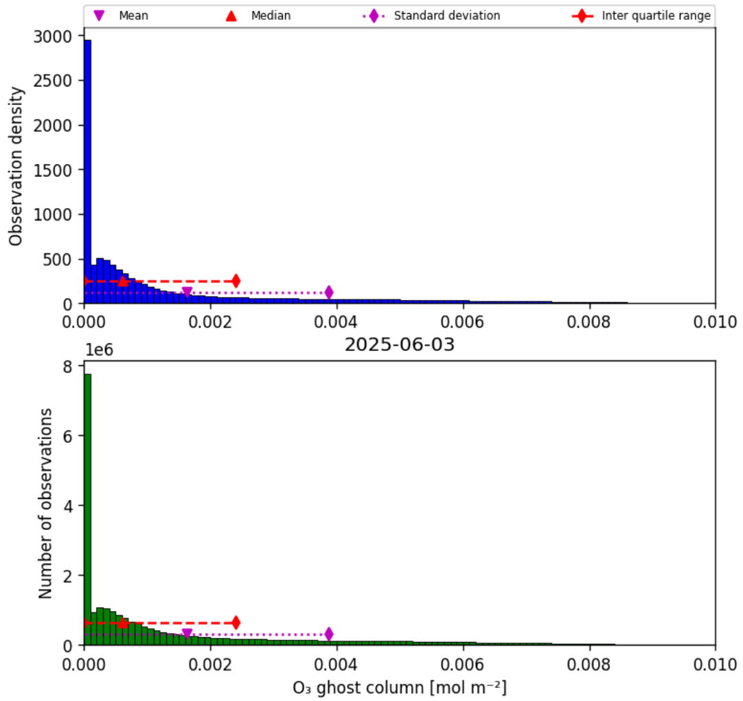
Figure 25: Histogram of “O 3 ghost column” for 2025-06-02 to 2025-06-04
