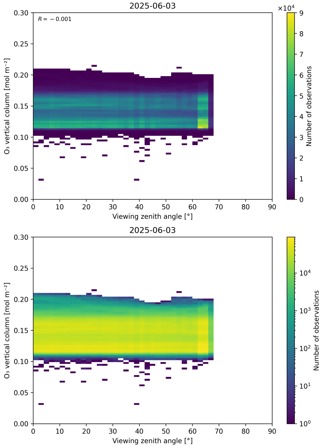
Figure 52: Scatter density plot of “Viewing zenith angle” against “O 3 vertical column” for 2025-06-02 to 2025-06-04.
