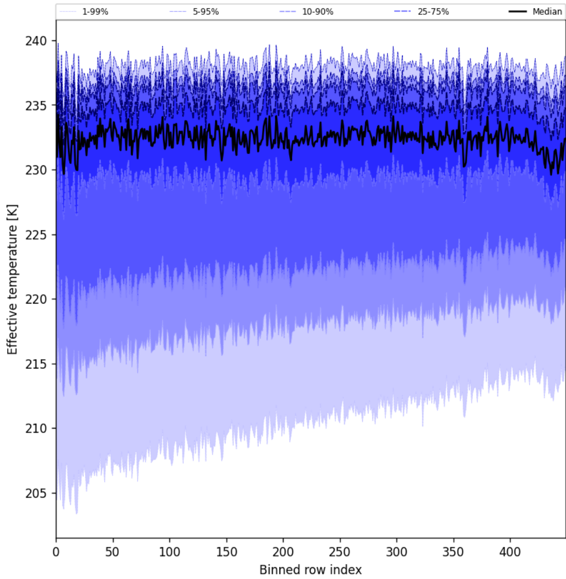
Figure 31: Along track statistics of “Effective temperature” for 2025-06-02 to 2025-06-04
