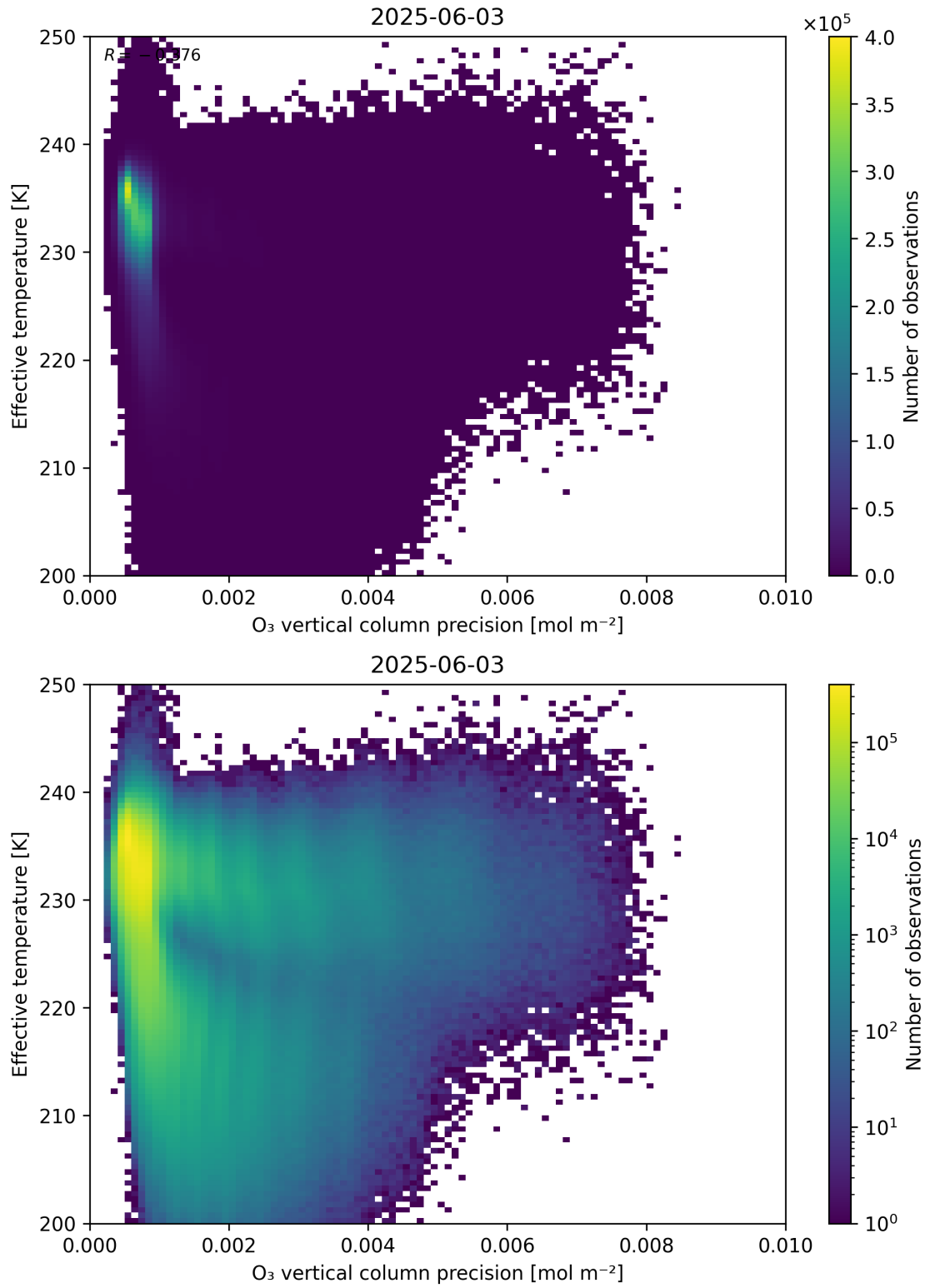
Figure 42: Scatter density plot of “O 3 vertical column precision” against “Effective temperature” for 2025-06-02 to 2025-06-04.
