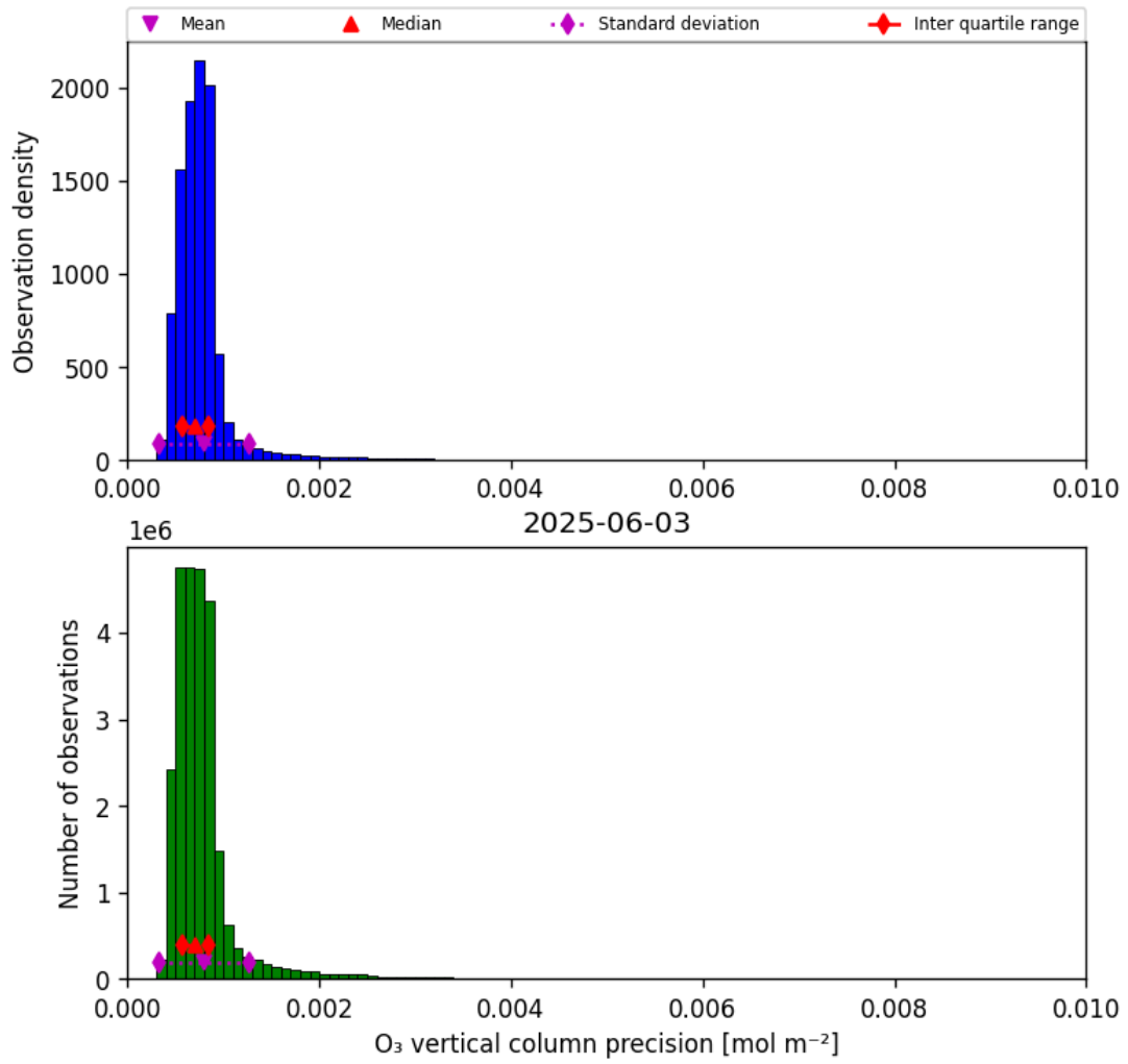
Figure 22: Histogram of “O 3 vertical column precision” for 2025-06-02 to 2025-06-04
