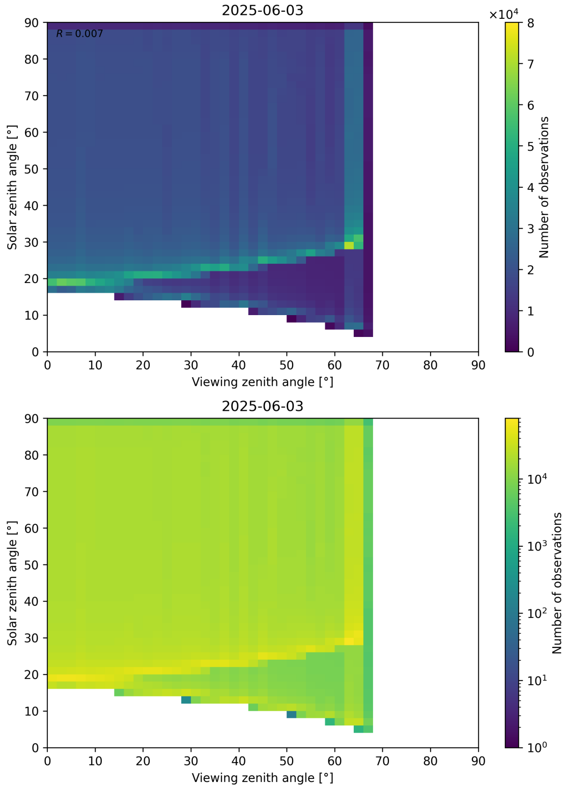
Figure 54: Scatter density plot of “Viewing zenith angle” against “Solar zenith angle” for 2025-06-02 to 2025-06-04.
