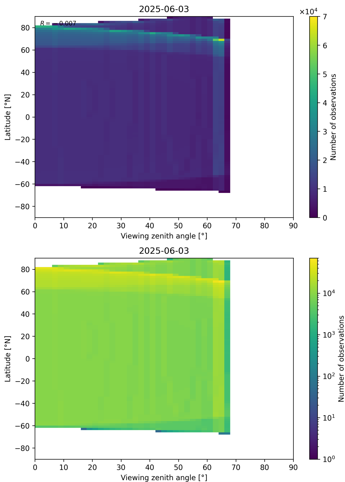
Figure 49: Scatter density plot of “Viewing zenith angle” against “Latitude” for 2025-06-02 to 2025-06-04.
