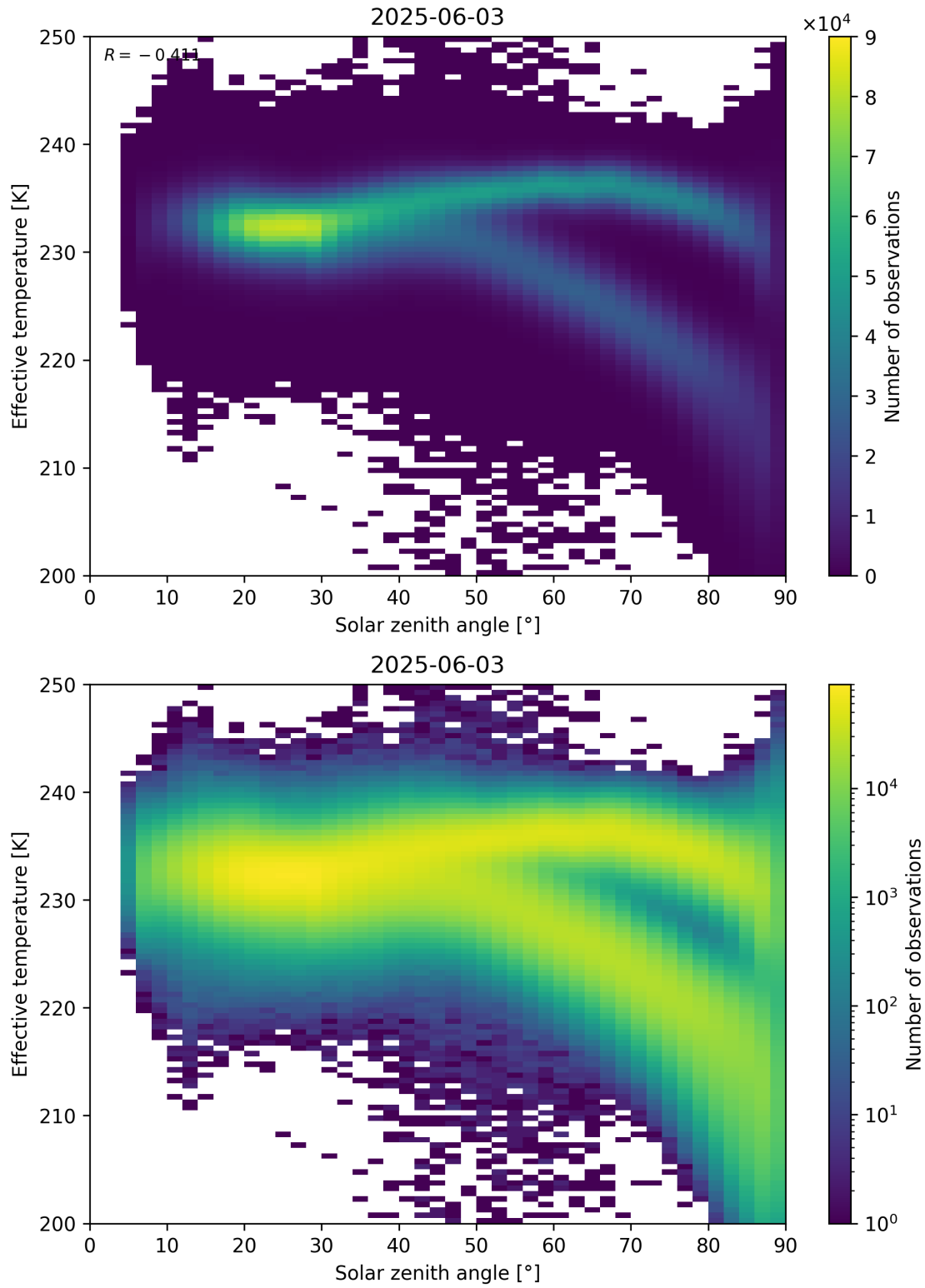
Figure 45: Scatter density plot of “Solar zenith angle” against “Effective temperature” for 2025-06-02 to 2025-06-04.
