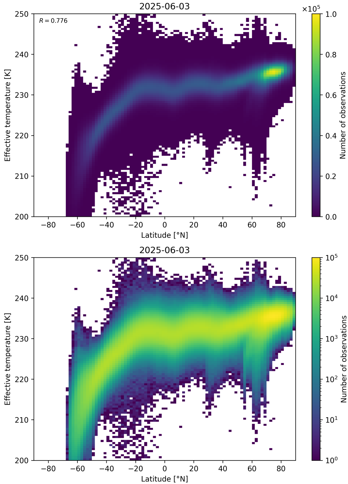
Figure 34: Scatter density plot of “Latitude” against “Effective temperature” for 2025-06-02 to 2025-06-04.
