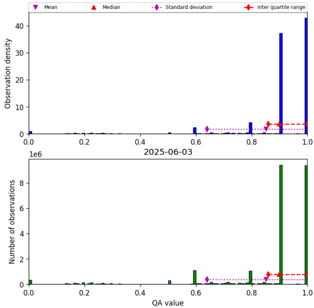
Figure 20: Histogram of “QA value” for 2025-06-02 to 2025-06-04
