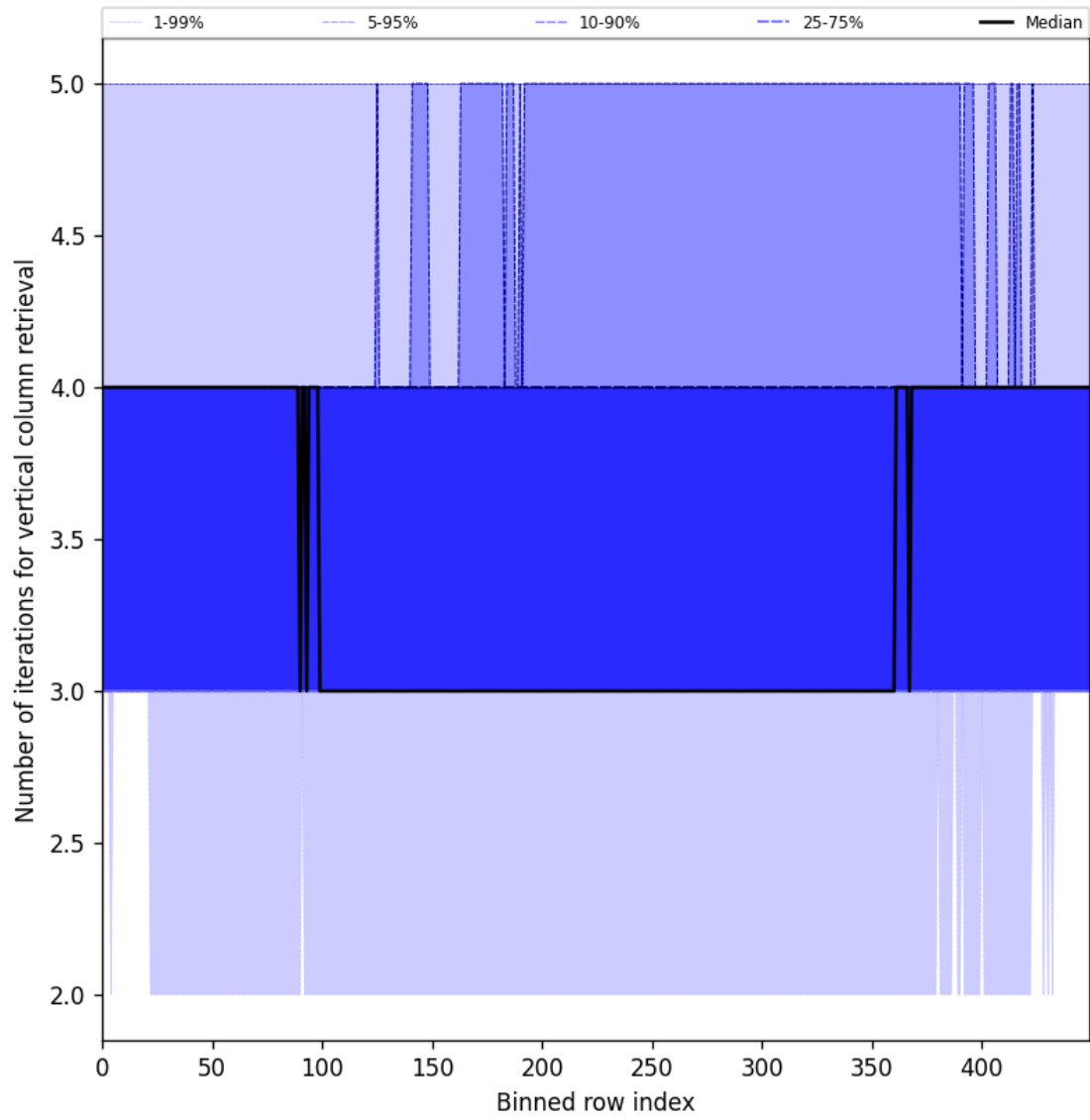
Figure 33: Along track statistics of “Number of iterations for vertical column retrieval” for 2025-06-02 to 2025-06-04
