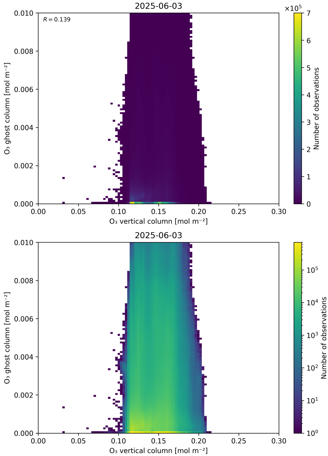
Figure 40: Scatter density plot of “O 3 vertical column” against “O 3 ghost column” for 2025-06-02 to 2025-06-04.
