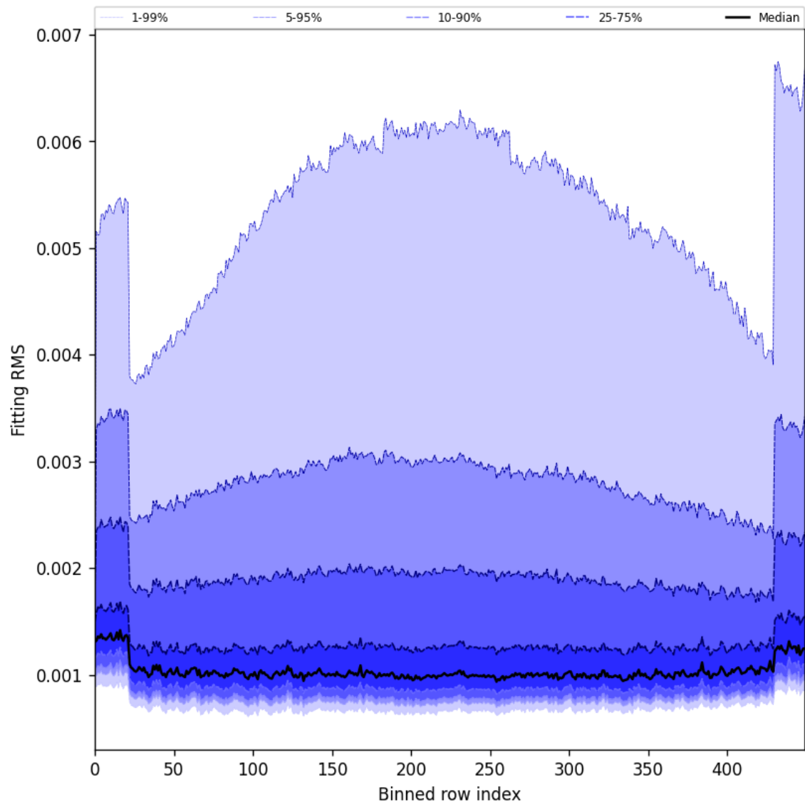
Figure 30: Along track statistics of “Fitting RMS” for 2025-06-02 to 2025-06-04
