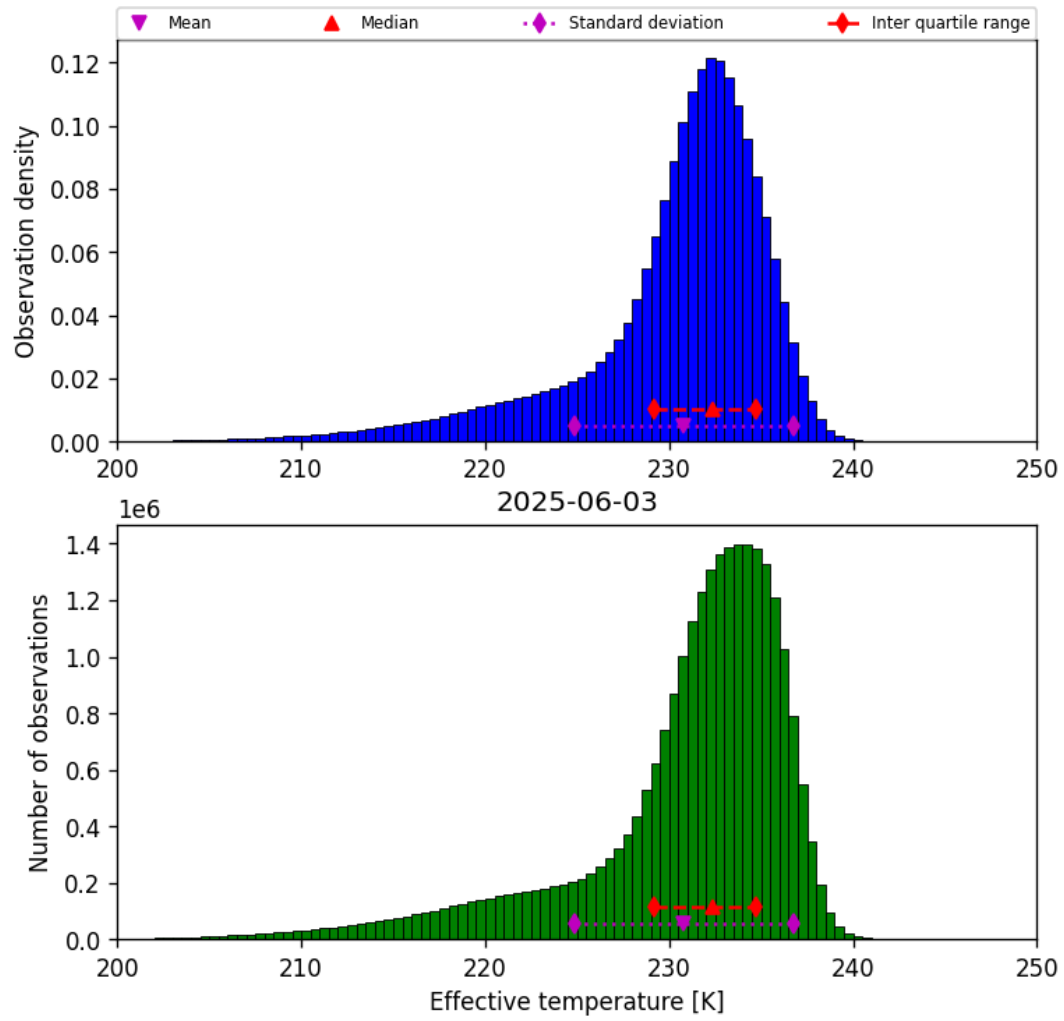
Figure 24: Histogram of “Effective temperature” for 2025-06-02 to 2025-06-04
