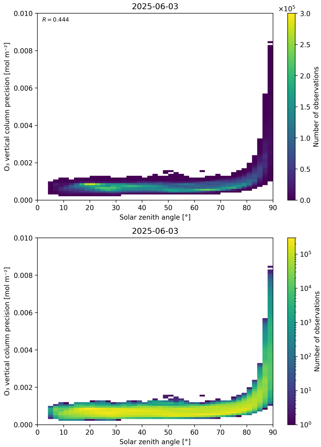
Figure 48: Scatter density plot of “Solar zenith angle” against “O 3 vertical column precision” for 2025-06-02 to 2025-06-04.
