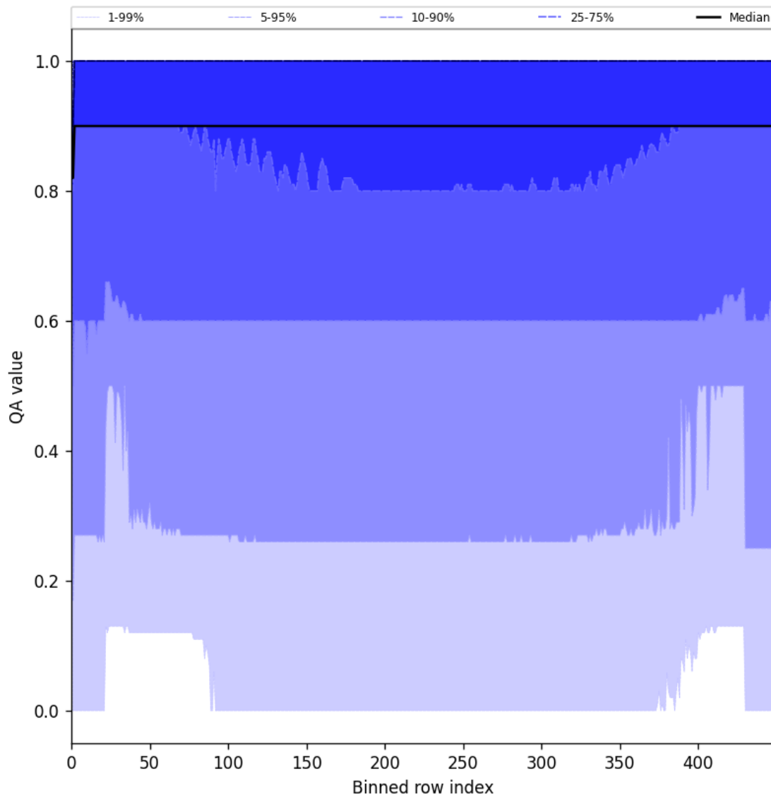
Figure 27: Along track statistics of “QA value” for 2025-06-02 to 2025-06-04
