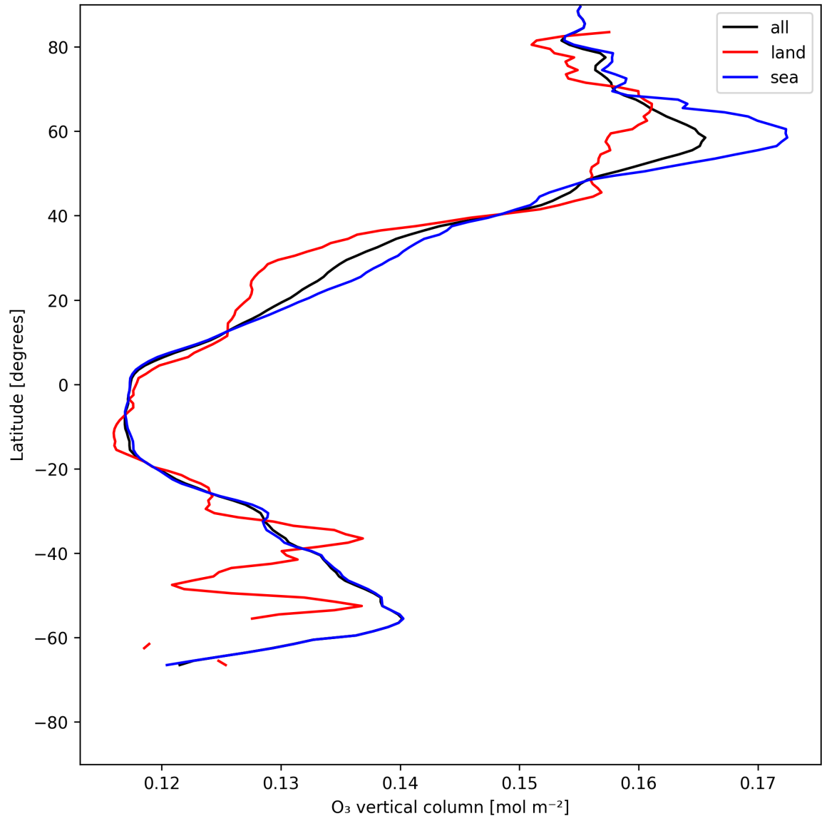
Figure 14: Zonal average of “O 3 vertical column” for 2025-06-02 to 2025-06-04.
