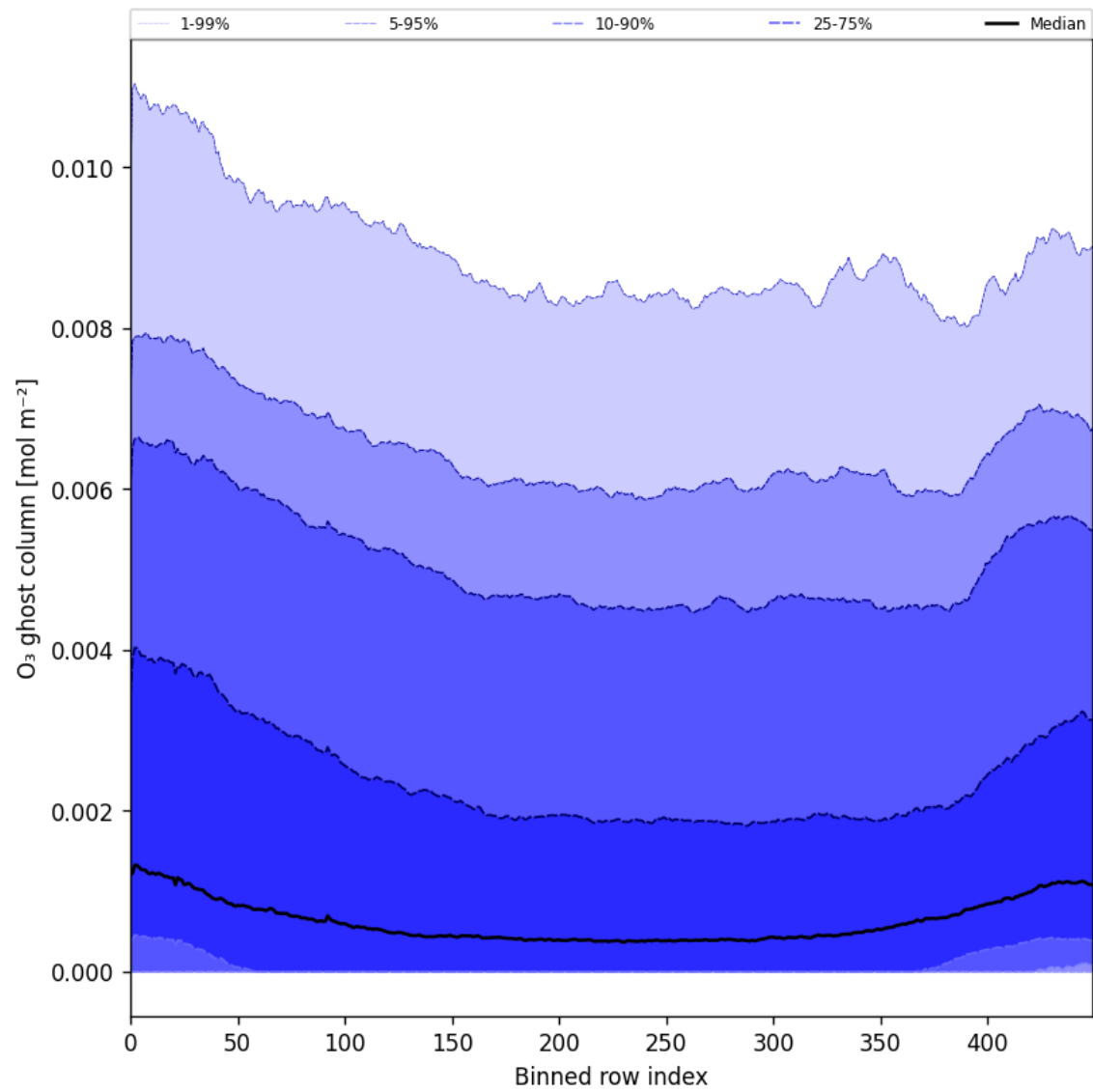
Figure 32: Along track statistics of “O 3 ghost column” for 2025-06-02 to 2025-06-04
