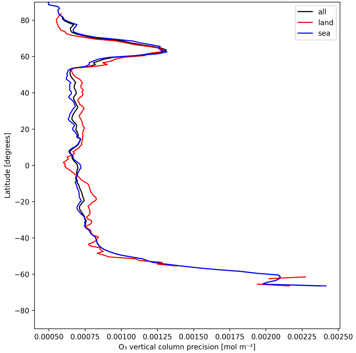
Figure 15: Zonal average of “O 3 vertical column precision” for 2025-06-02 to 2025-06-04.
