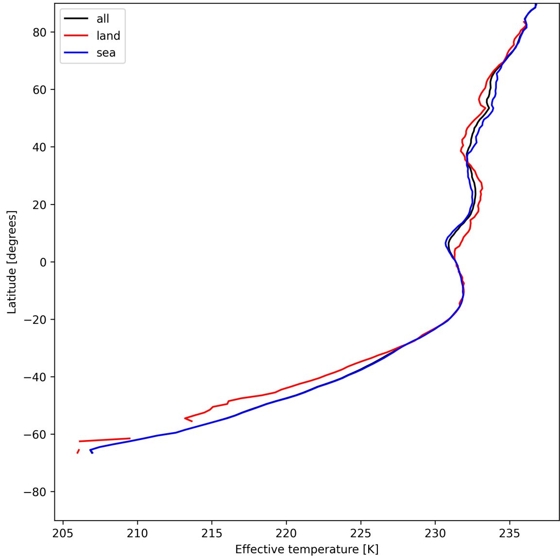
Figure 17: Zonal average of "Effective temperature" for 2025-06-02 to 2025-06-04.
