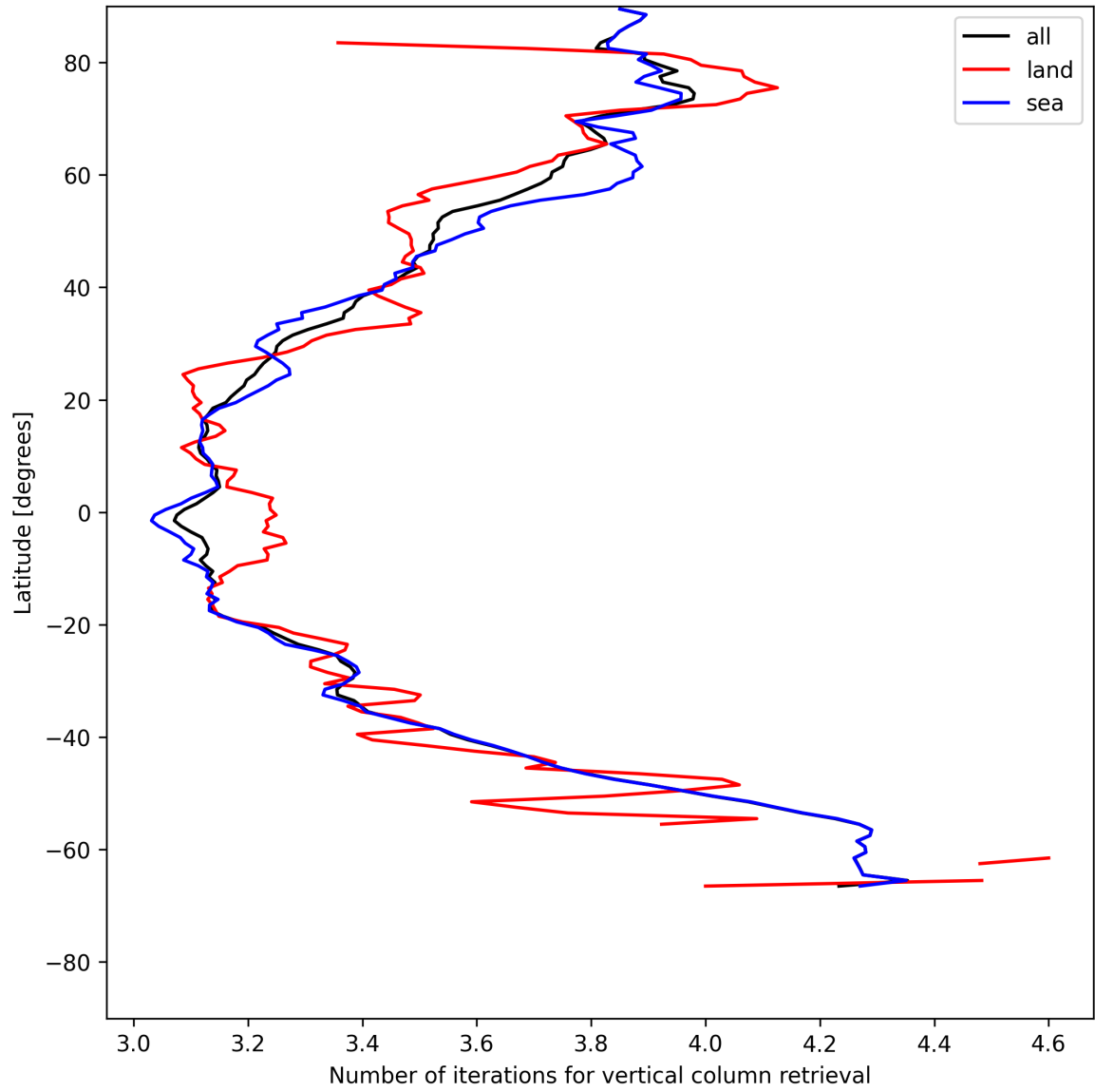
Figure 19: Zonal average of “Number of iterations for vertical column retrieval” for 2025-06-02 to 2025-06-04.
