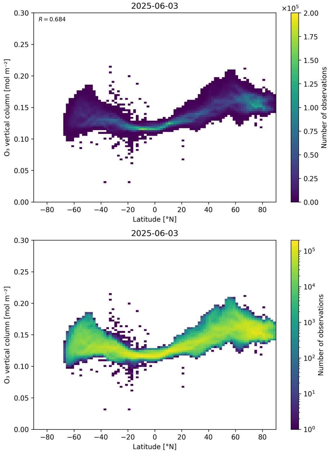
Figure 36: Scatter density plot of “Latitude” against “O 3 vertical column” for 2025-06-02 to 2025-06-04.
