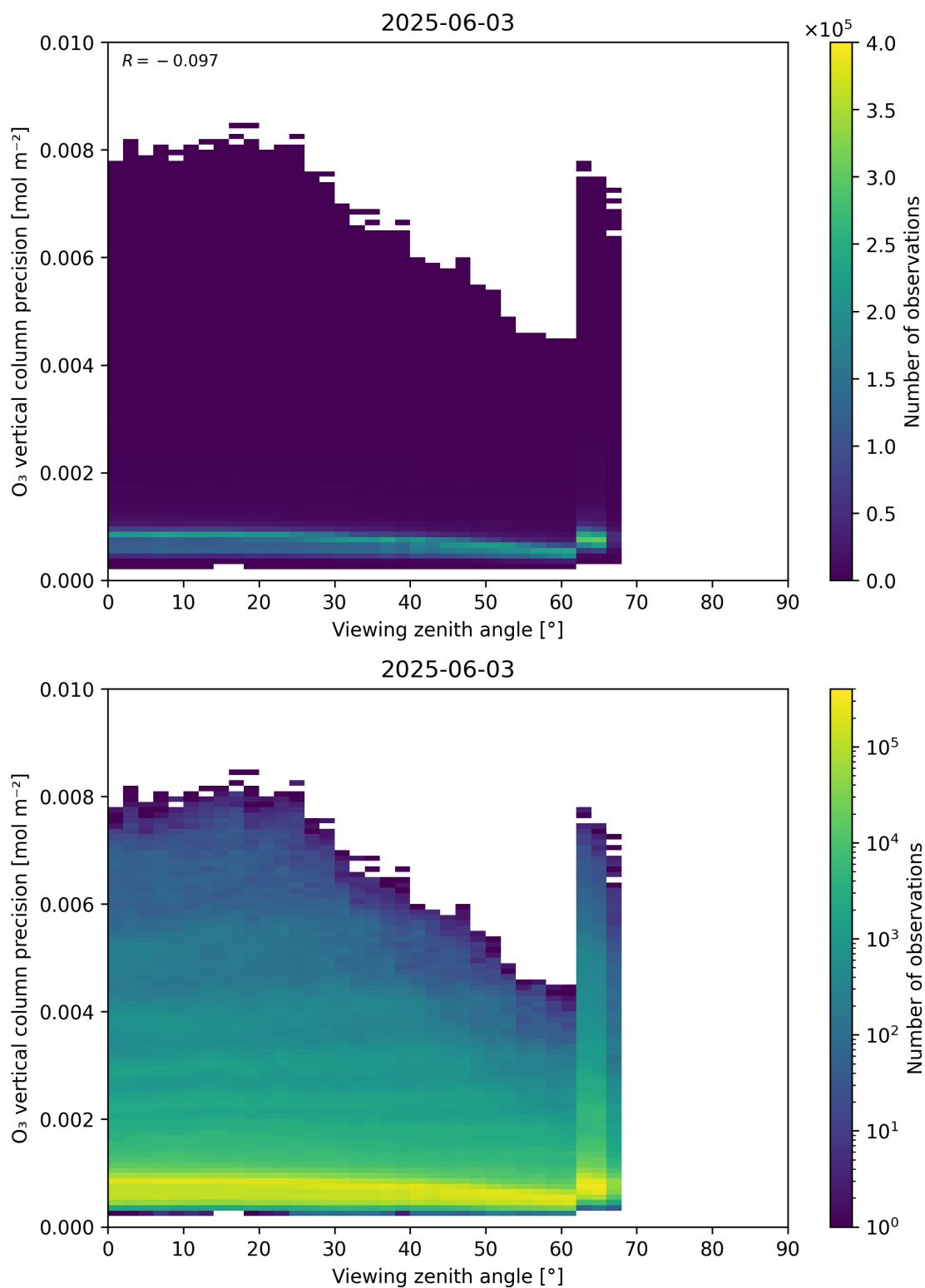
Figure 53: Scatter density plot of “Viewing zenith angle” against “O 3 vertical column precision” for 2025-06-02 to 2025-06-04.
