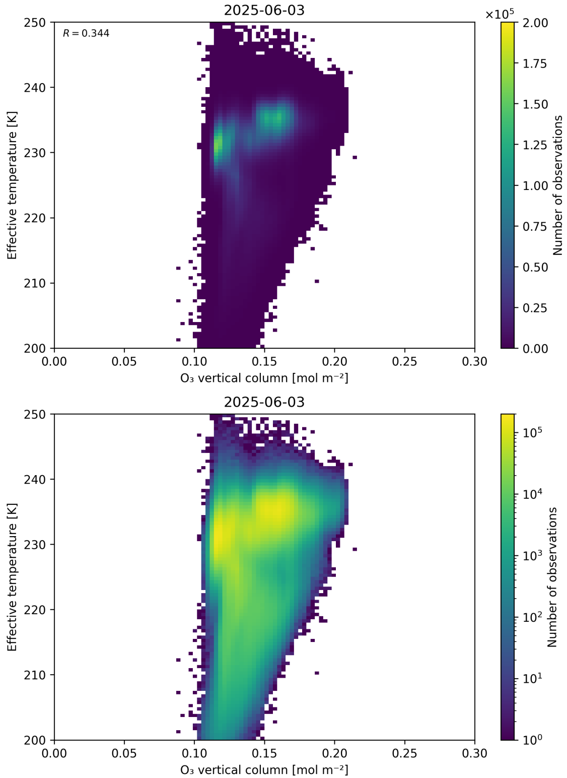
Figure 39: Scatter density plot of “O 3 vertical column” against “Effective temperature” for 2025-06-02 to 2025-06-04.
