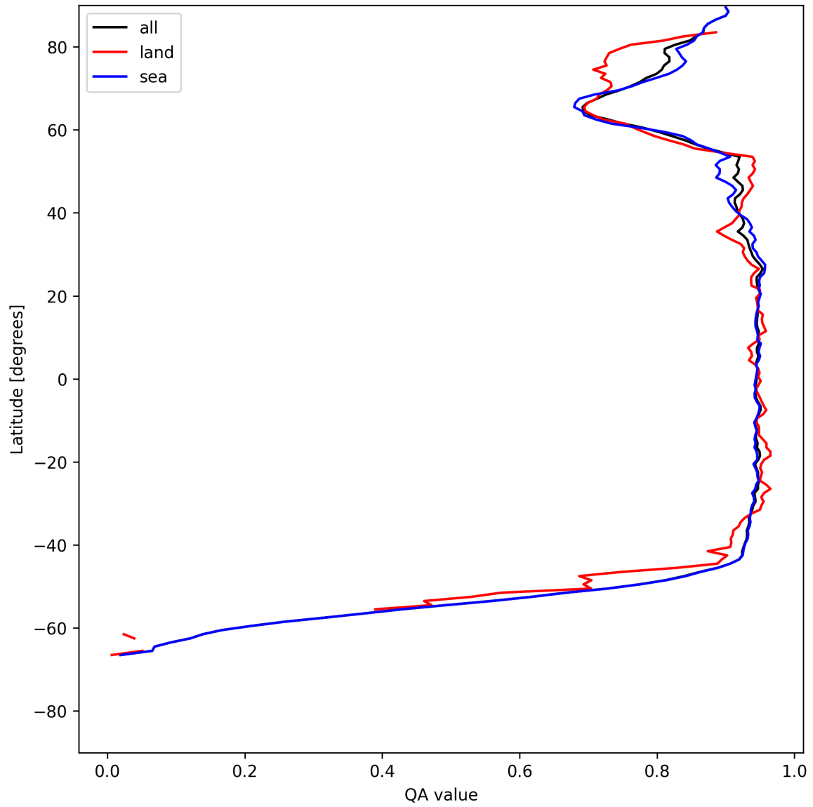
Figure 13: Zonal average of “QA value” for 2025-06-02 to 2025-06-04.
