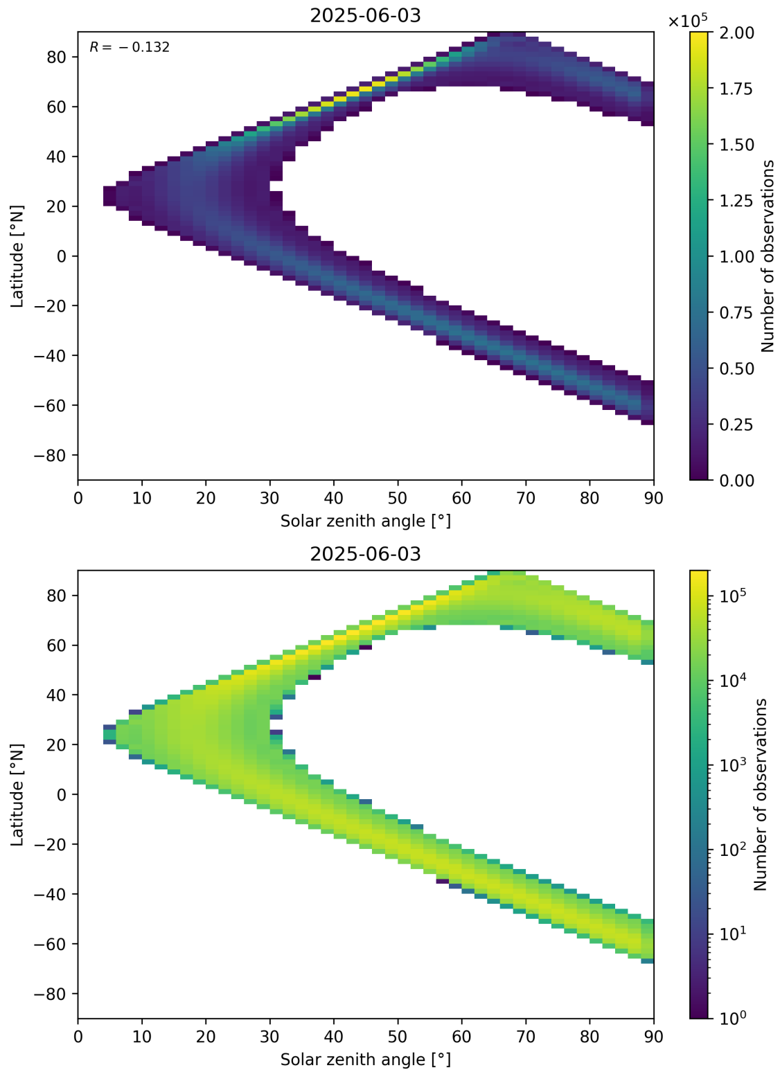
Figure 44: Scatter density plot of “Solar zenith angle” against “Latitude” for 2025-06-02 to 2025-06-04.
