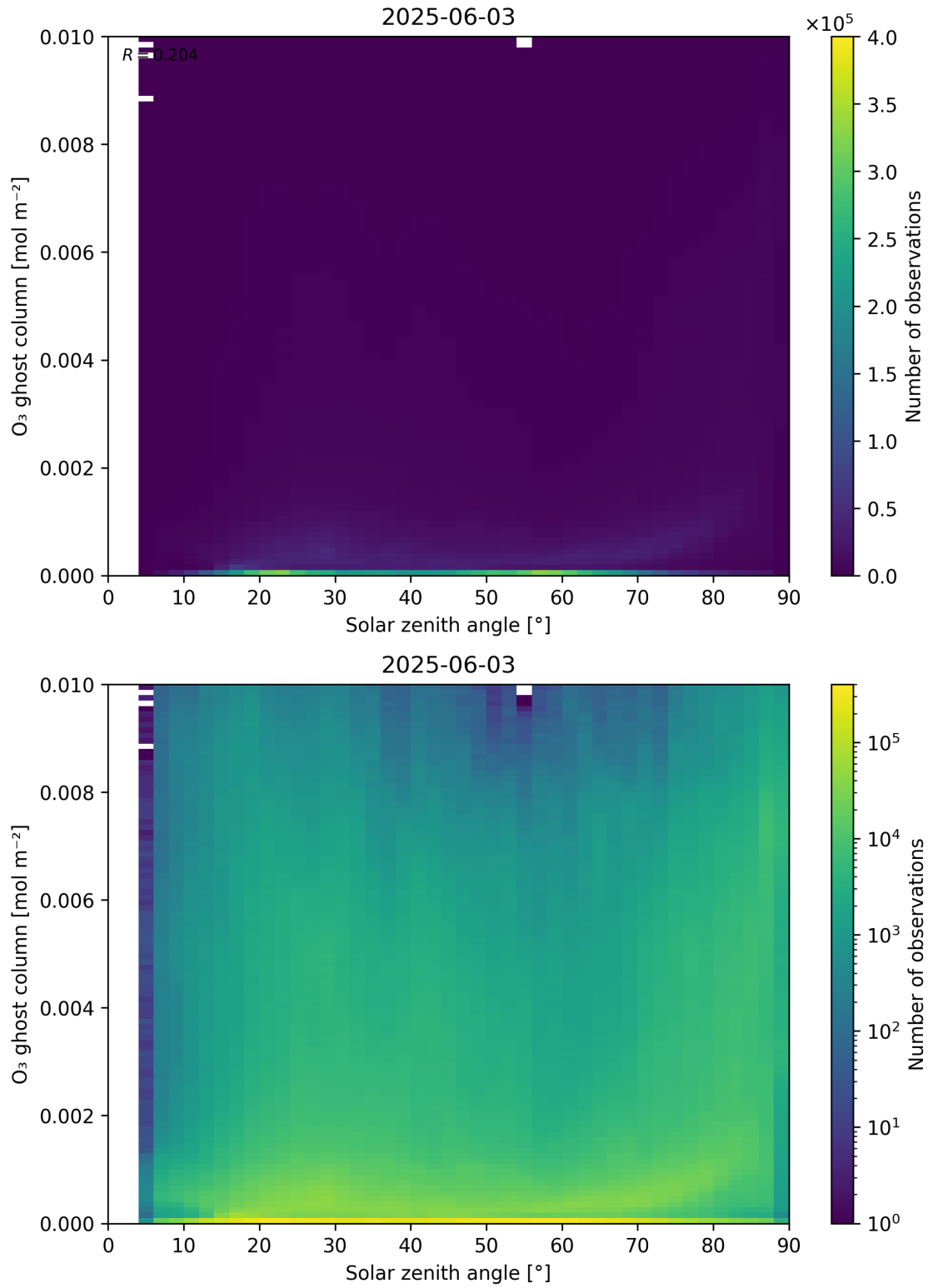
Figure 46: Scatter density plot of “Solar zenith angle” against “O 3 ghost column” for 2025-06-02 to 2025-06-04.
