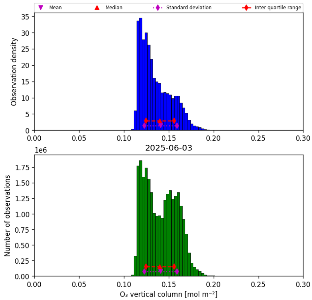
Figure 21: Histogram of “O 3 vertical column” for 2025-06-02 to 2025-06-04
