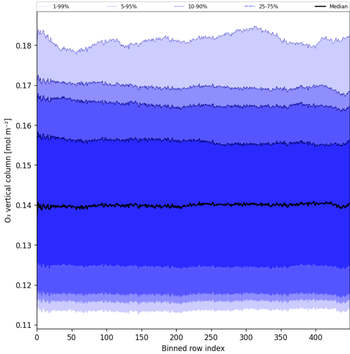
Figure 28: Along track statistics of “O 3 vertical column” for 2025-06-02 to 2025-06-04
