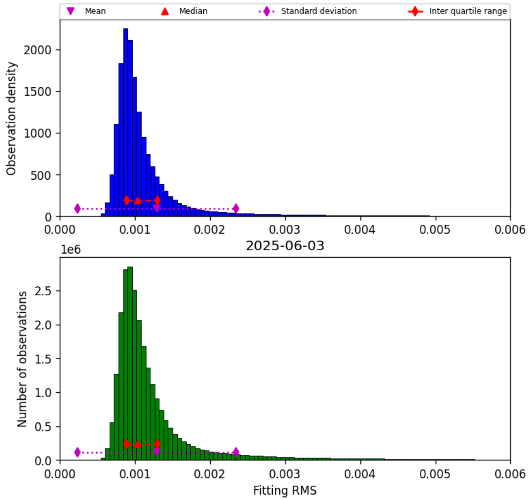
Figure 23: Histogram of “Fitting RMS” for 2025-06-02 to 2025-06-04
