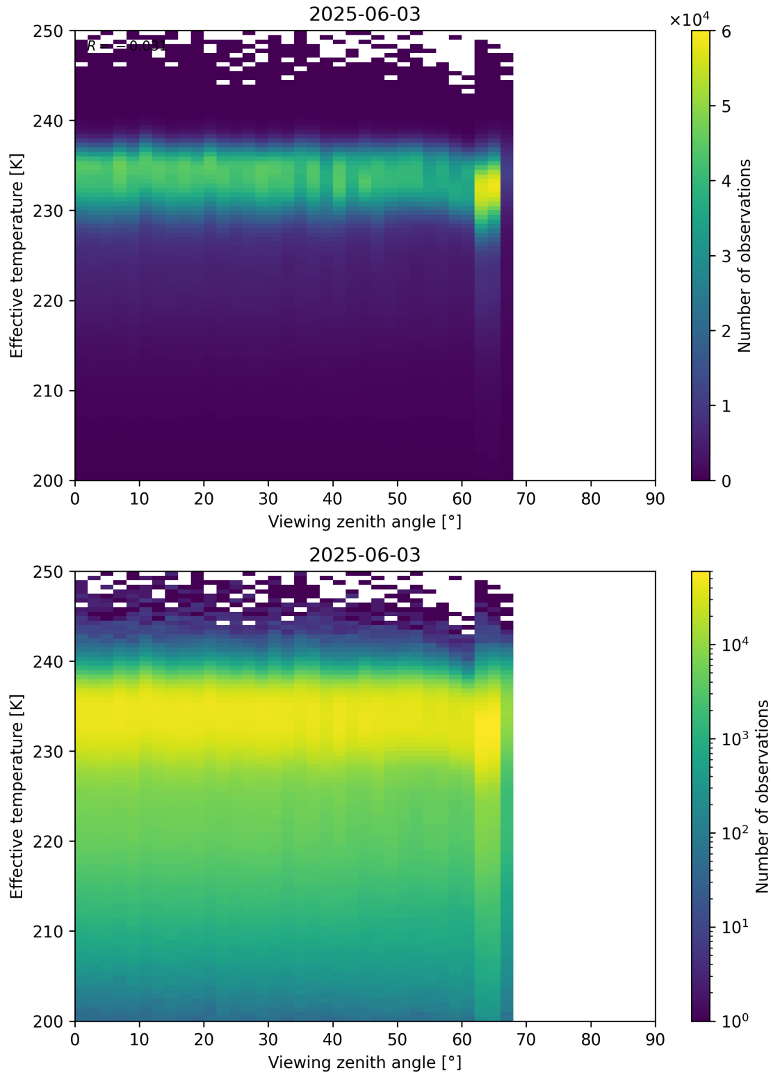
Figure 50: Scatter density plot of “Viewing zenith angle” against “Effective temperature” for 2025-06-02 to 2025-06-04.
