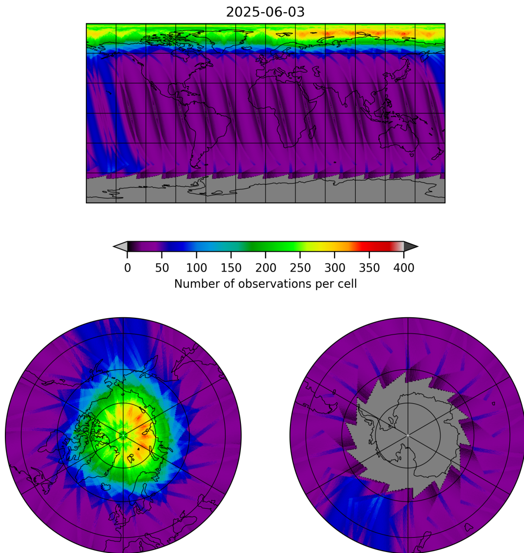
Figure 12: Map of the number of observations for 2025-06-02 to 2025-06-04
