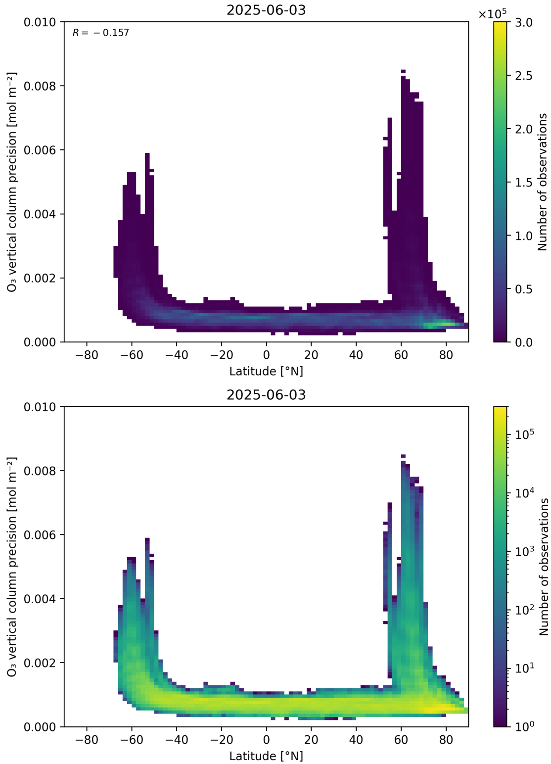
Figure 37: Scatter density plot of “Latitude” against “O 3 vertical column precision” for 2025-06-02 to 2025-06-04.
