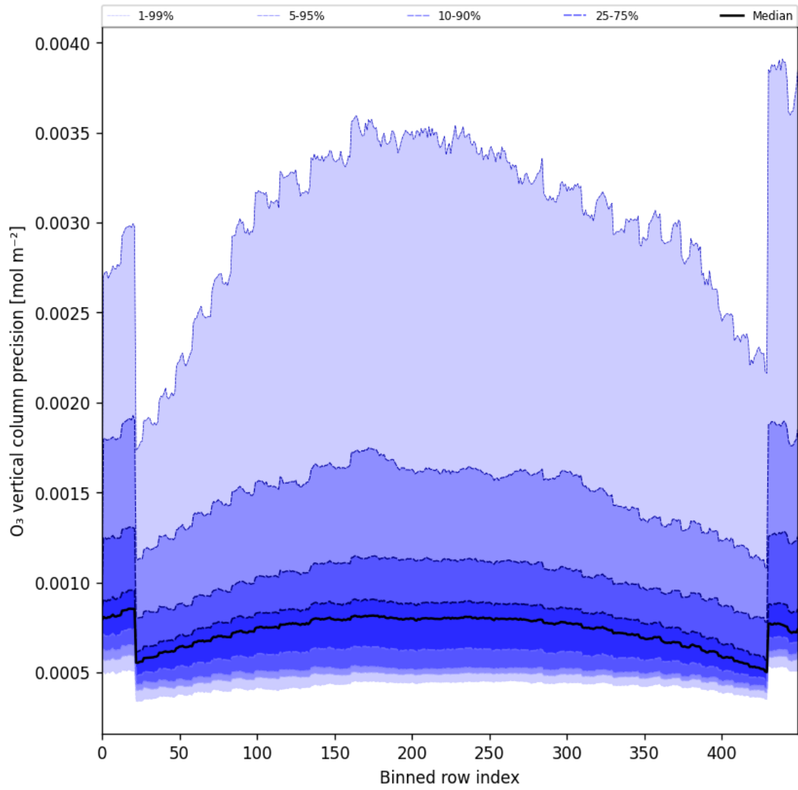
Figure 29: Along track statistics of “O 3 vertical column precision” for 2025-06-02 to 2025-06-04
