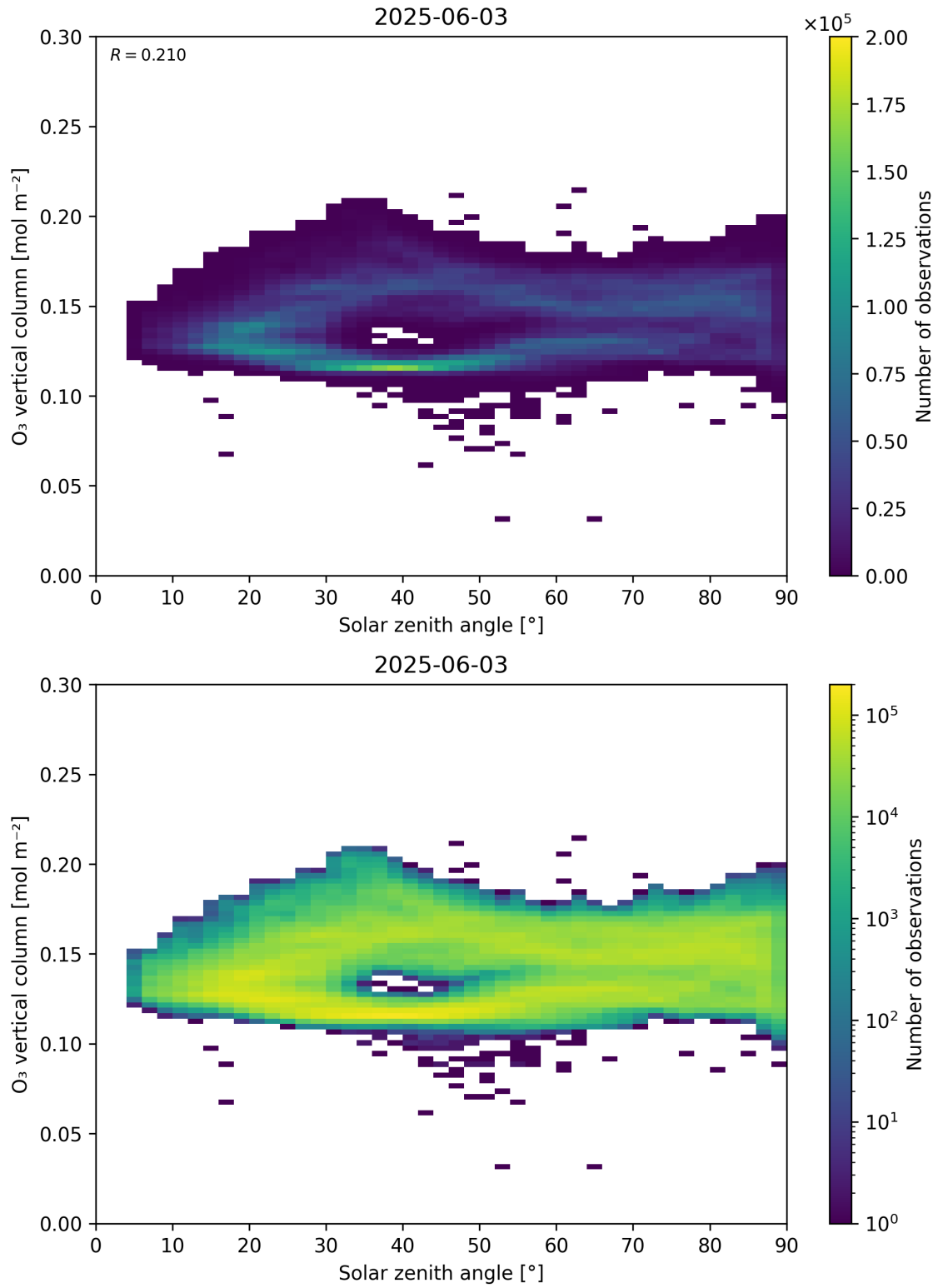
Figure 47: Scatter density plot of “Solar zenith angle” against “O 3 vertical column” for 2025-06-02 to 2025-06-04.
