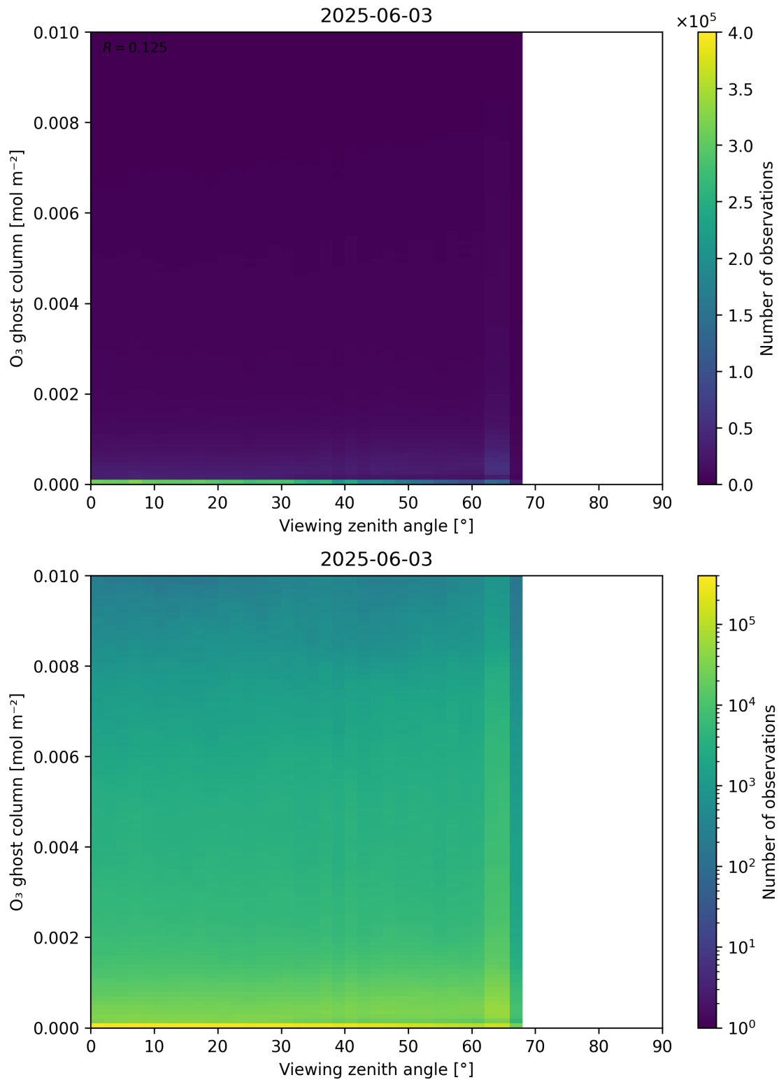
Figure 51: Scatter density plot of “Viewing zenith angle” against “O 3 ghost column” for 2025-06-02 to 2025-06-04.
