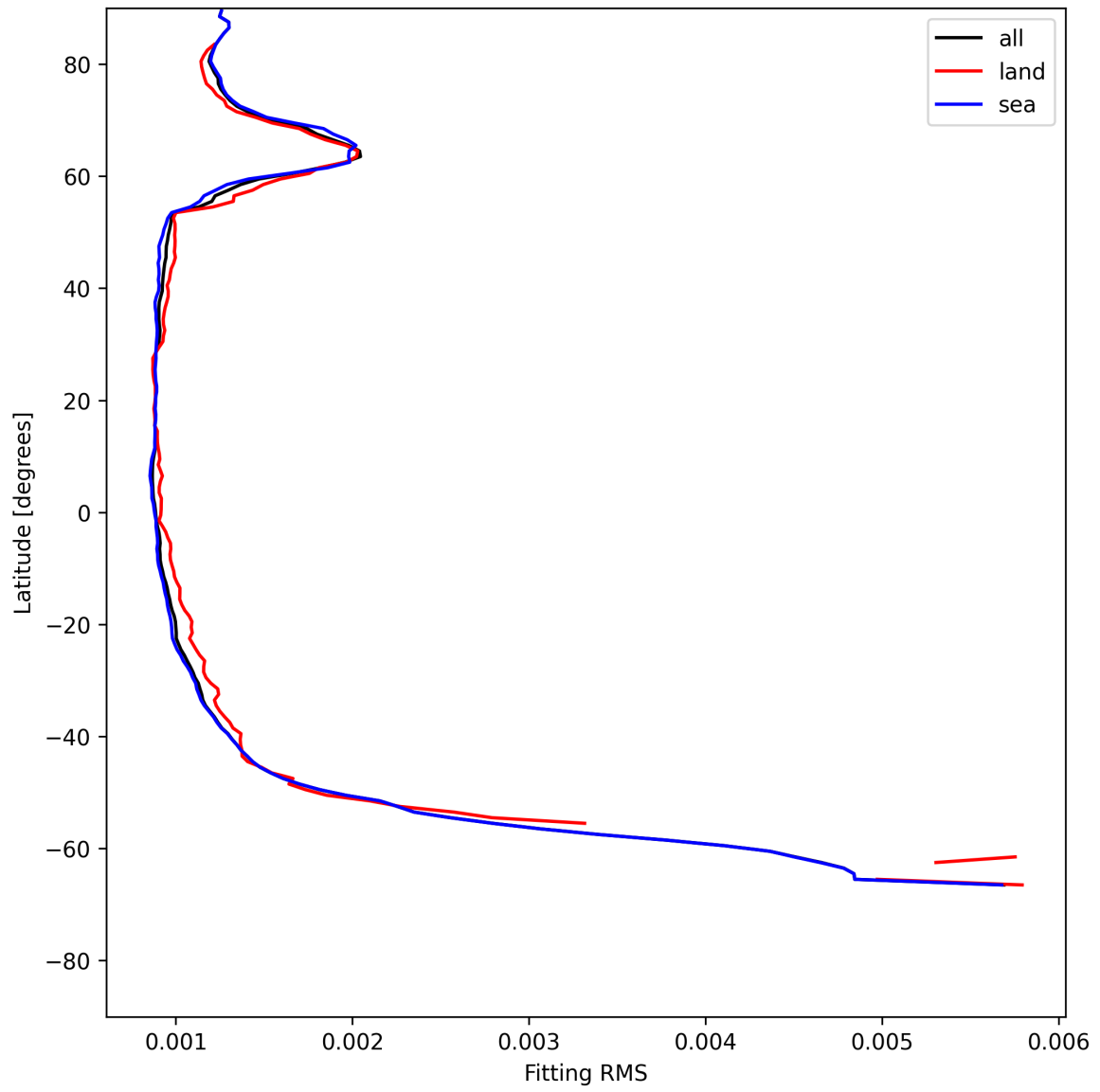
Figure 16: Zonal average of “Fitting RMS” for 2025-06-02 to 2025-06-04.
