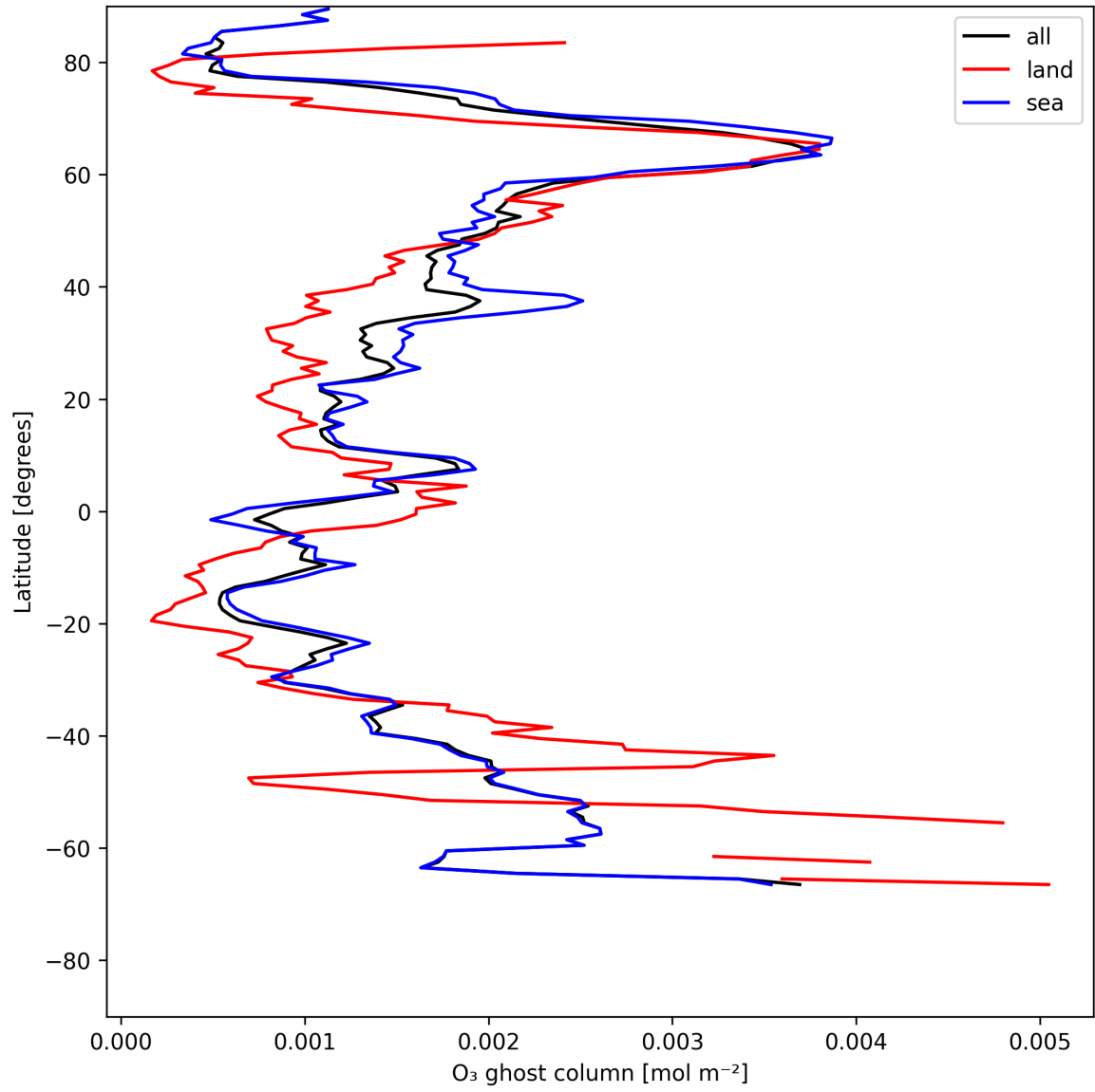
Figure 18: Zonal average of “O 3 ghost column” for 2025-06-02 to 2025-06-04.
