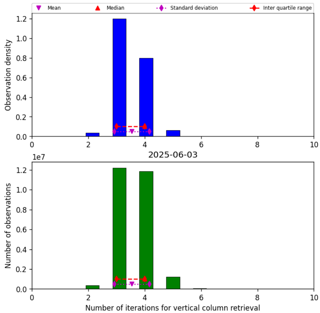
Figure 26: Histogram of “Number of iterations for vertical column retrieval” for 2025-06-02 to 2025-06-04
