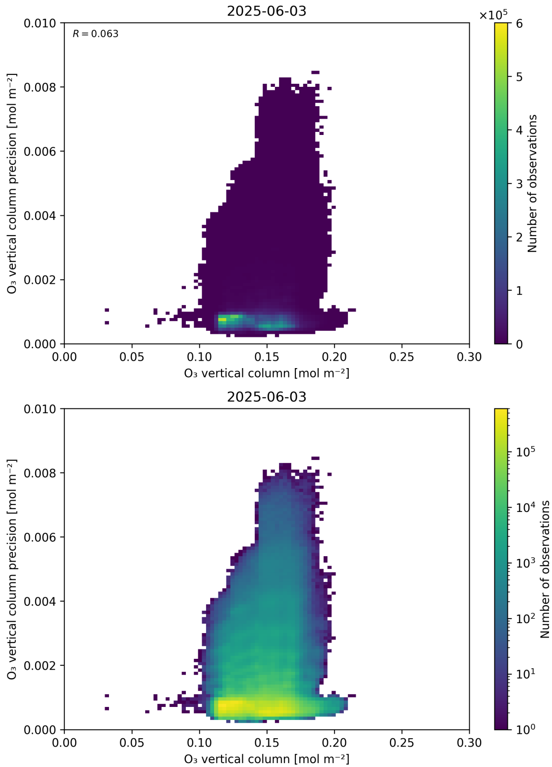
Figure 41: Scatter density plot of “O 3 vertical column” against “O 3 vertical column precision” for 2025-06-02 to 2025-06-04.
