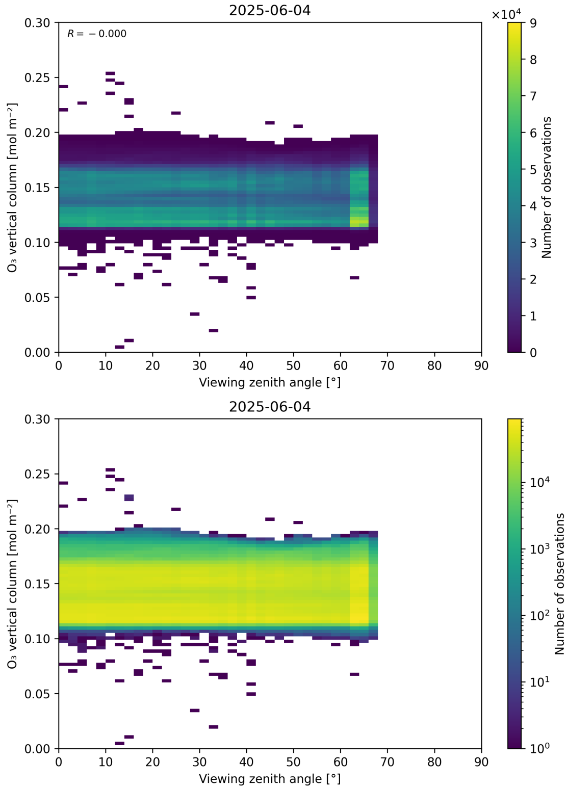
Figure 52: Scatter density plot of “Viewing zenith angle” against “O 3 vertical column” for 2025-06-03 to 2025-06-05.
