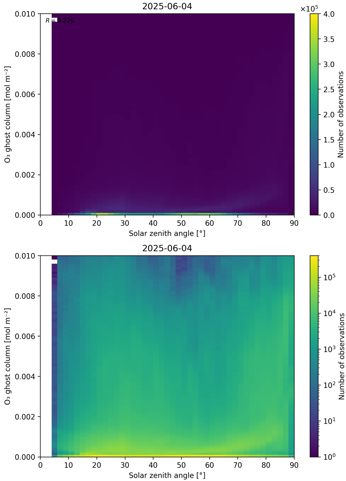
Figure 46: Scatter density plot of “Solar zenith angle” against “O 3 ghost column” for 2025-06-03 to 2025-06-05.
