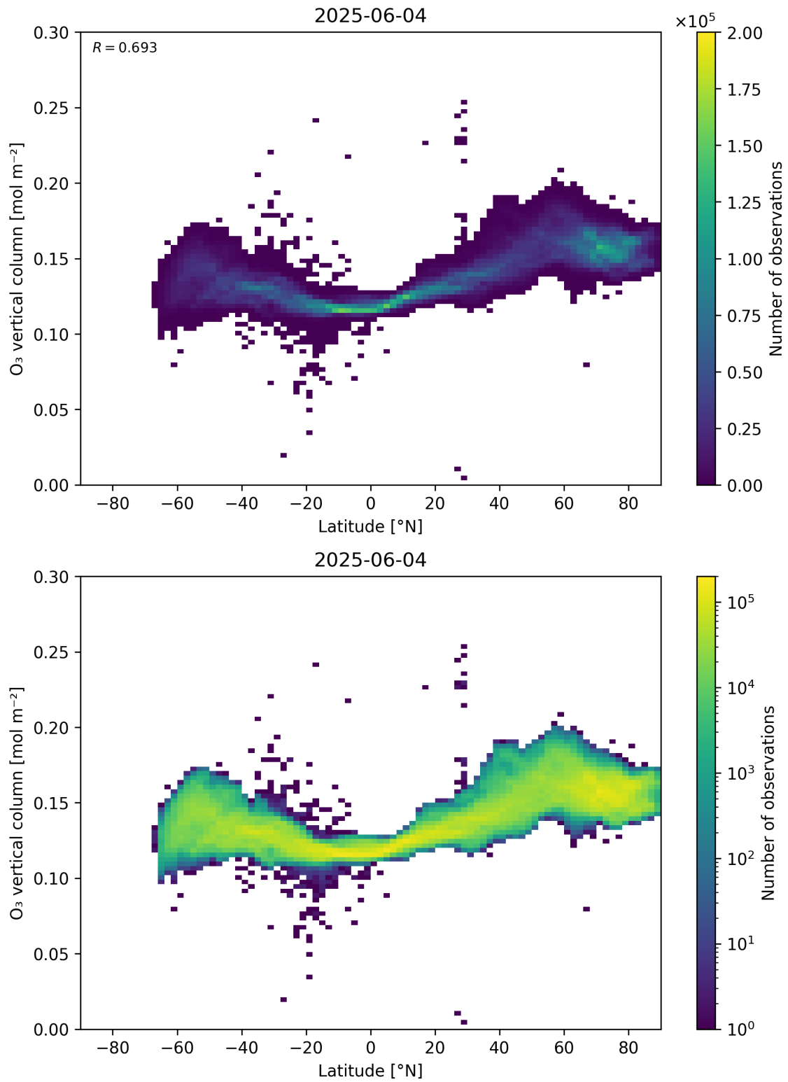
Figure 36: Scatter density plot of “Latitude” against “O 3 vertical column” for 2025-06-03 to 2025-06-05.
