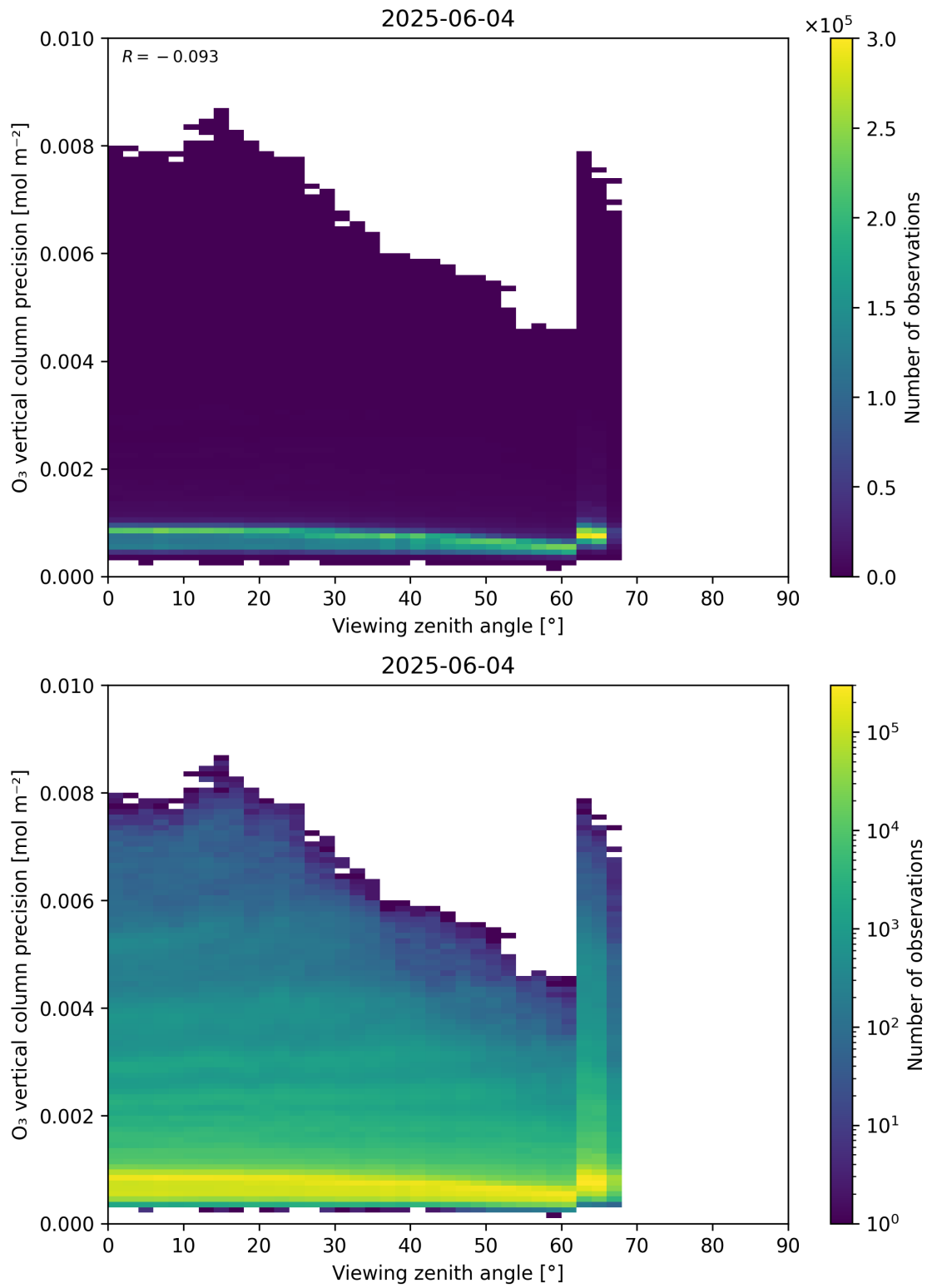
Figure 53: Scatter density plot of “Viewing zenith angle” against “O 3 vertical column precision” for 2025-06-03 to 2025-06-05.
