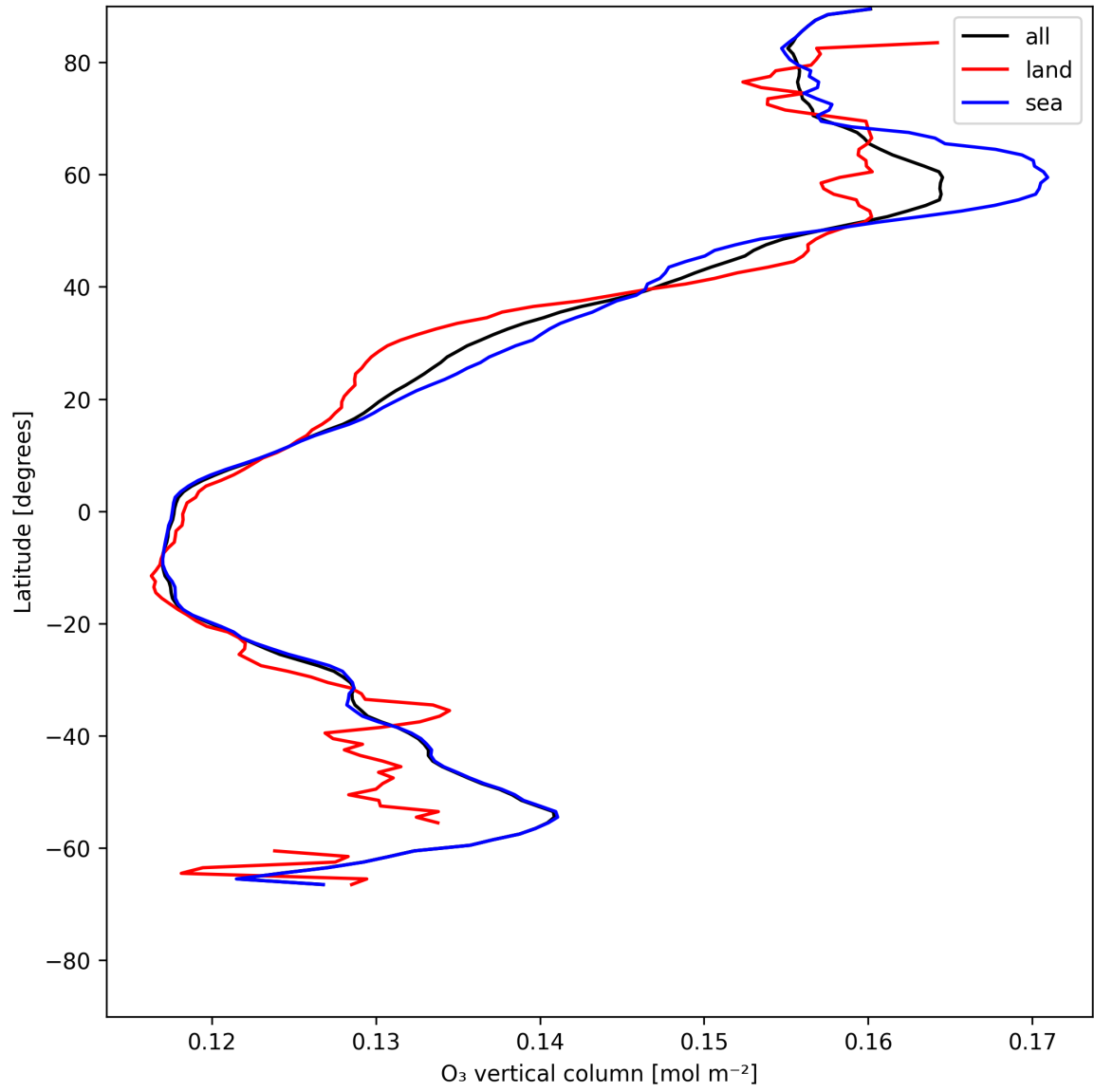
Figure 14: Zonal average of “O 3 vertical column” for 2025-06-03 to 2025-06-05.
