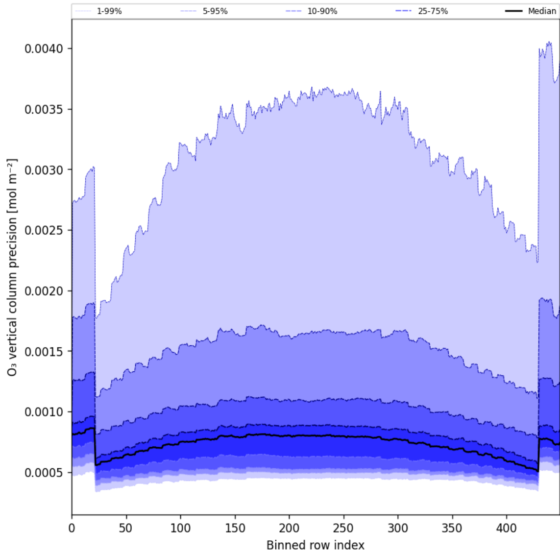
Figure 29: Along track statistics of “O 3 vertical column precision” for 2025-06-03 to 2025-06-05
