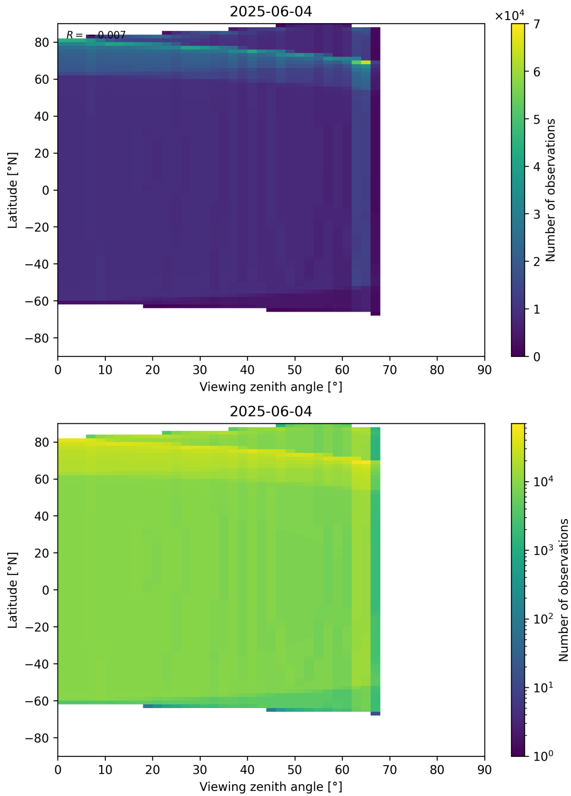
Figure 49: Scatter density plot of “Viewing zenith angle” against “Latitude” for 2025-06-03 to 2025-06-05.
