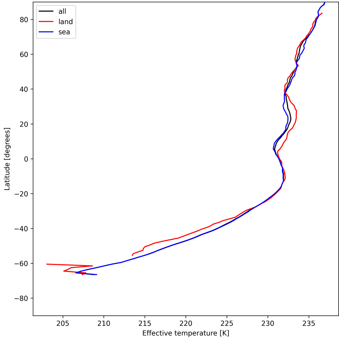
Figure 17: Zonal average of “Effective temperature” for 2025-06-03 to 2025-06-05.
