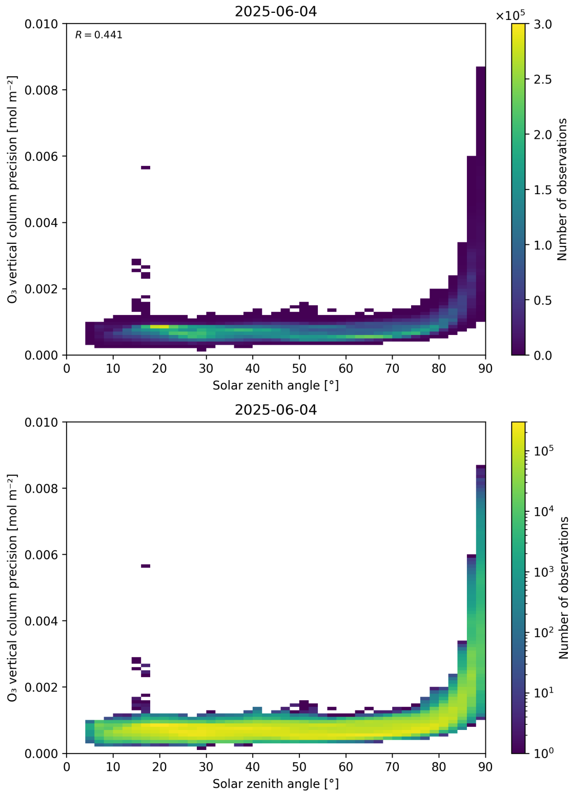
Figure 48: Scatter density plot of “Solar zenith angle” against “O 3 vertical column precision” for 2025-06-03 to 2025-06-05.
