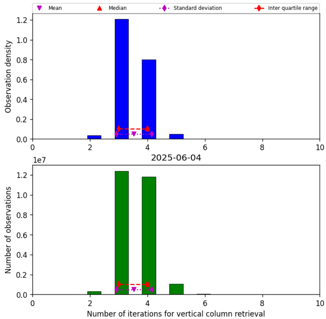
Figure 26: Histogram of “Number of iterations for vertical column retrieval” for 2025-06-03 to 2025-06-05
