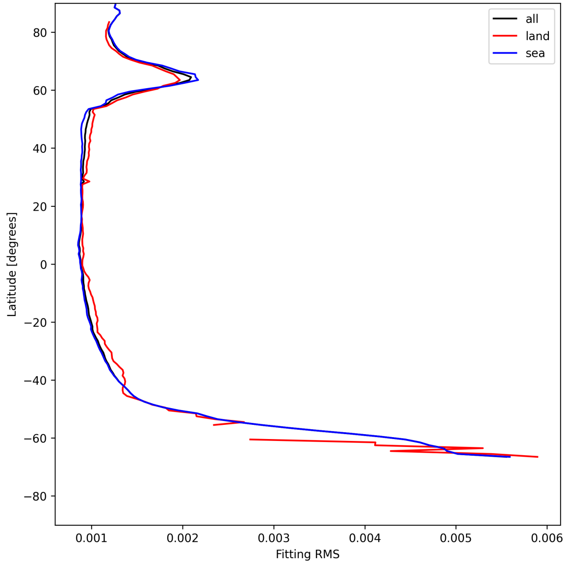
Figure 16: Zonal average of “Fitting RMS” for 2025-06-03 to 2025-06-05.
