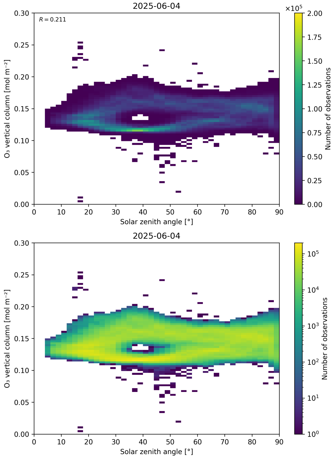
Figure 47: Scatter density plot of “Solar zenith angle” against “O 3 vertical column” for 2025-06-03 to 2025-06-05.
