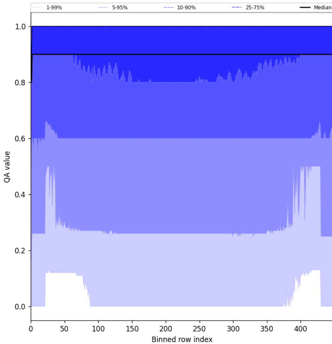
Figure 27: Along track statistics of “QA value” for 2025-06-03 to 2025-06-05
