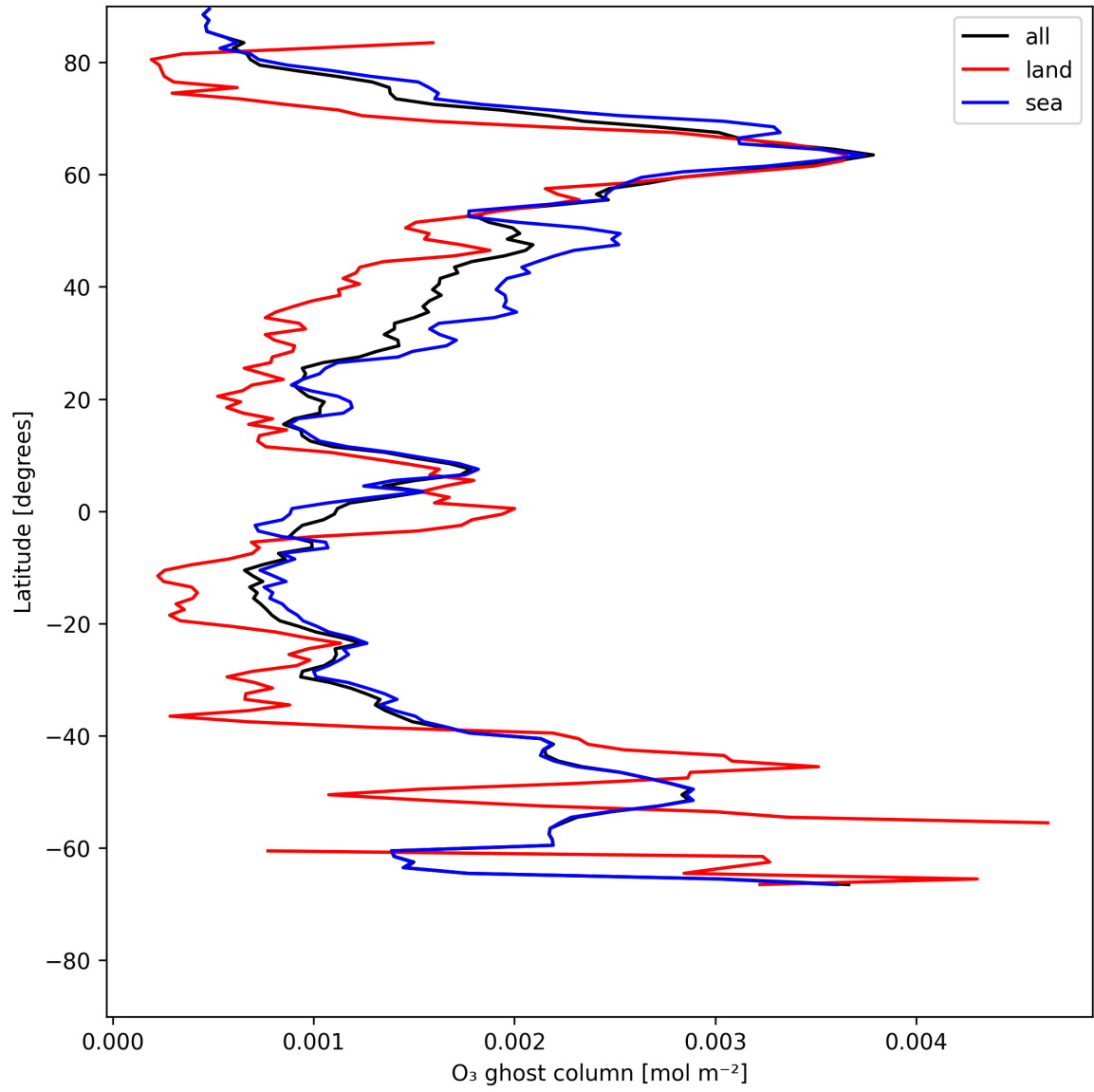
Figure 18: Zonal average of "O 3 ghost column" for 2025-06-03 to 2025-06-05.
