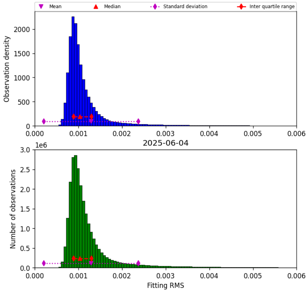
Figure 23: Histogram of “Fitting RMS” for 2025-06-03 to 2025-06-05
