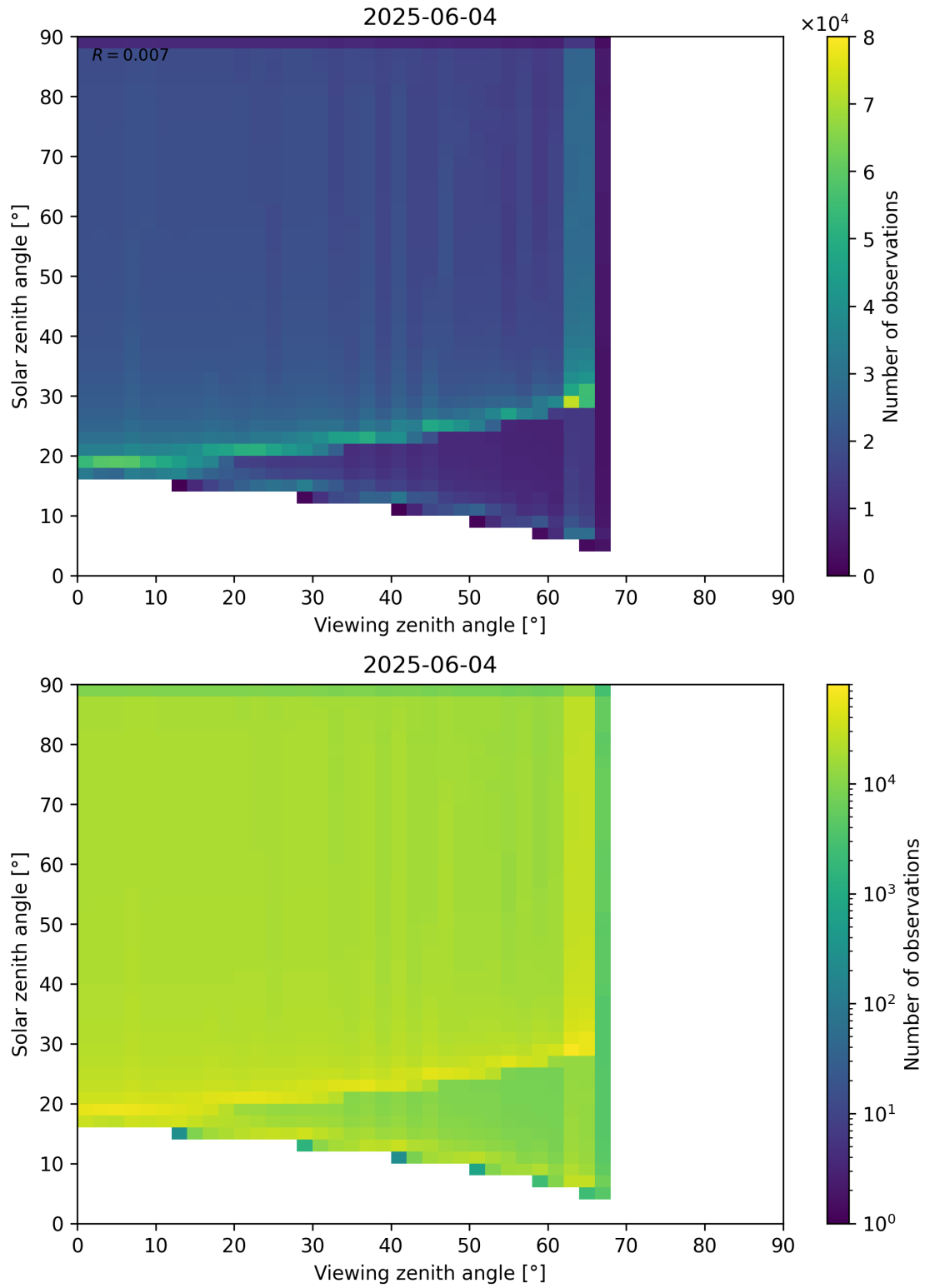
Figure 54: Scatter density plot of “Viewing zenith angle” against “Solar zenith angle” for 2025-06-03 to 2025-06-05.
