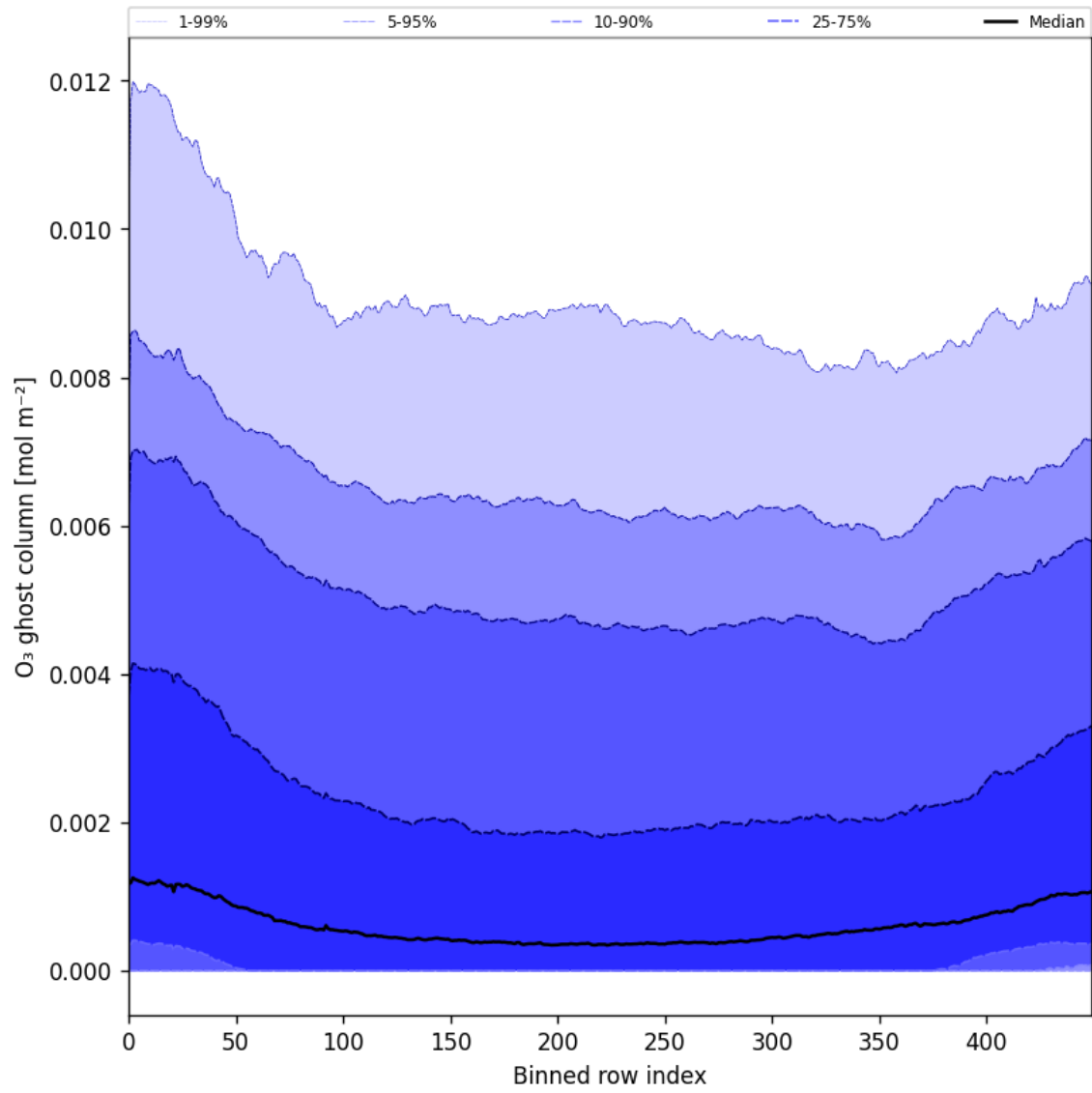
Figure 32: Along track statistics of “O 3 ghost column” for 2025-06-03 to 2025-06-05
