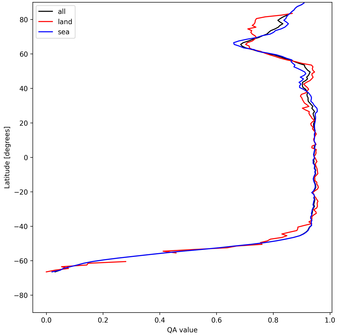
Figure 13: Zonal average of “QA value” for 2025-06-03 to 2025-06-05.
