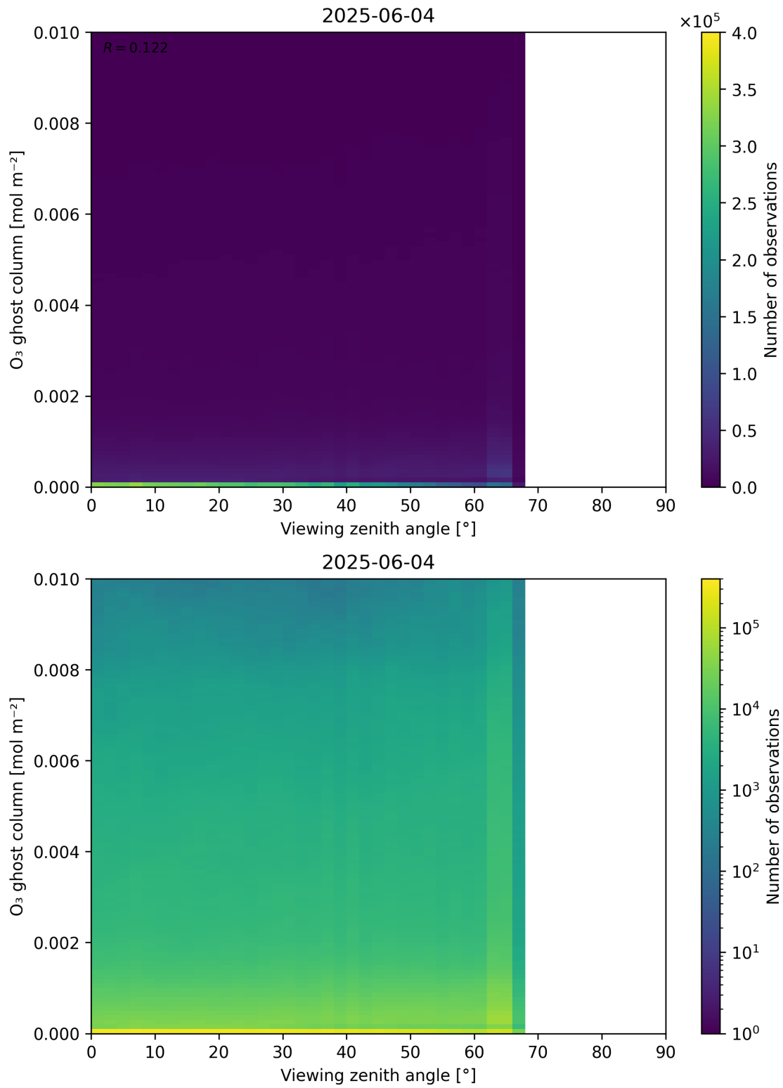
Figure 51: Scatter density plot of “Viewing zenith angle” against “O 3 ghost column” for 2025-06-03 to 2025-06-05.
