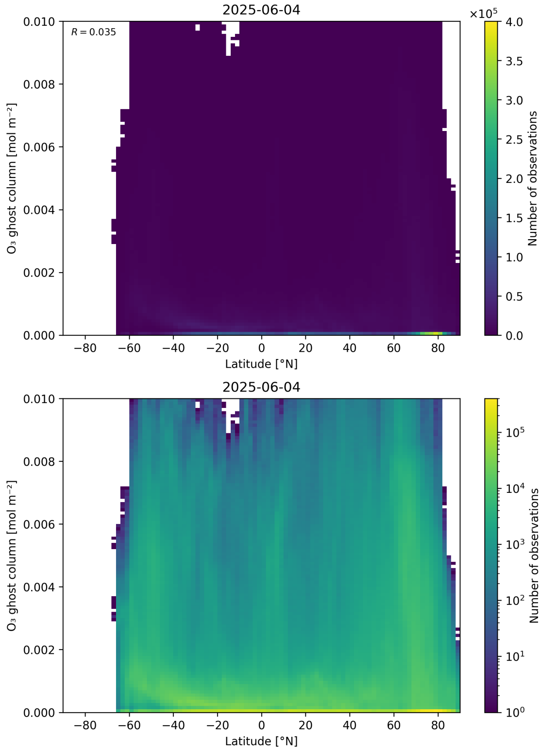
Figure 35: Scatter density plot of “Latitude” against “O 3 ghost column” for 2025-06-03 to 2025-06-05.
