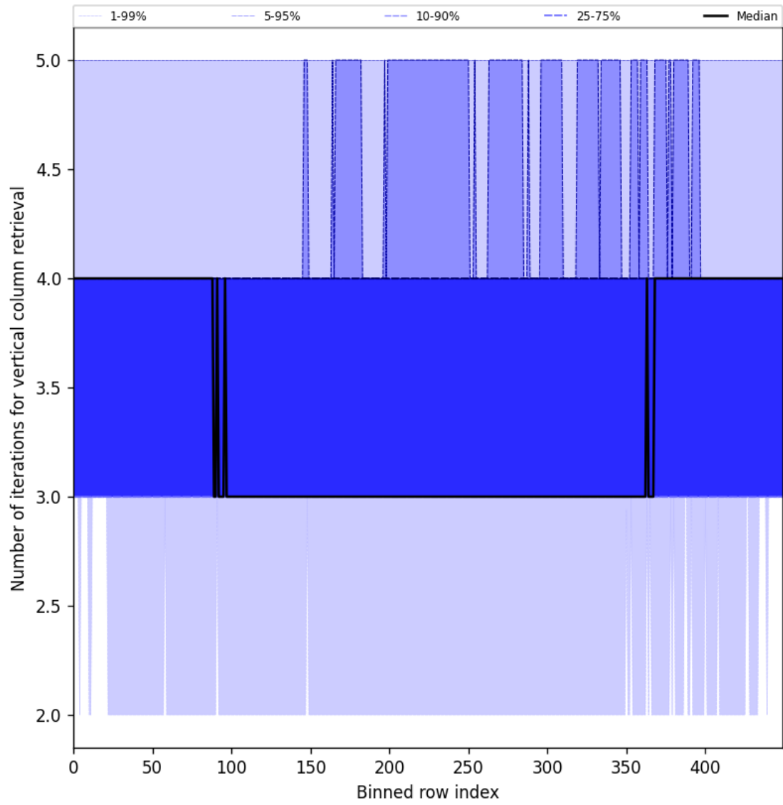
Figure 33: Along track statistics of “Number of iterations for vertical column retrieval” for 2025-06-03 to 2025-06-05
