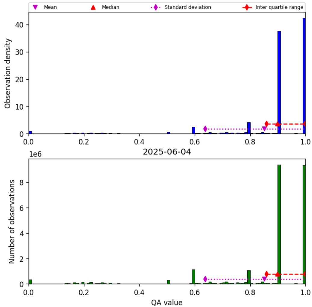
Figure 20: Histogram of “QA value” for 2025-06-03 to 2025-06-05
