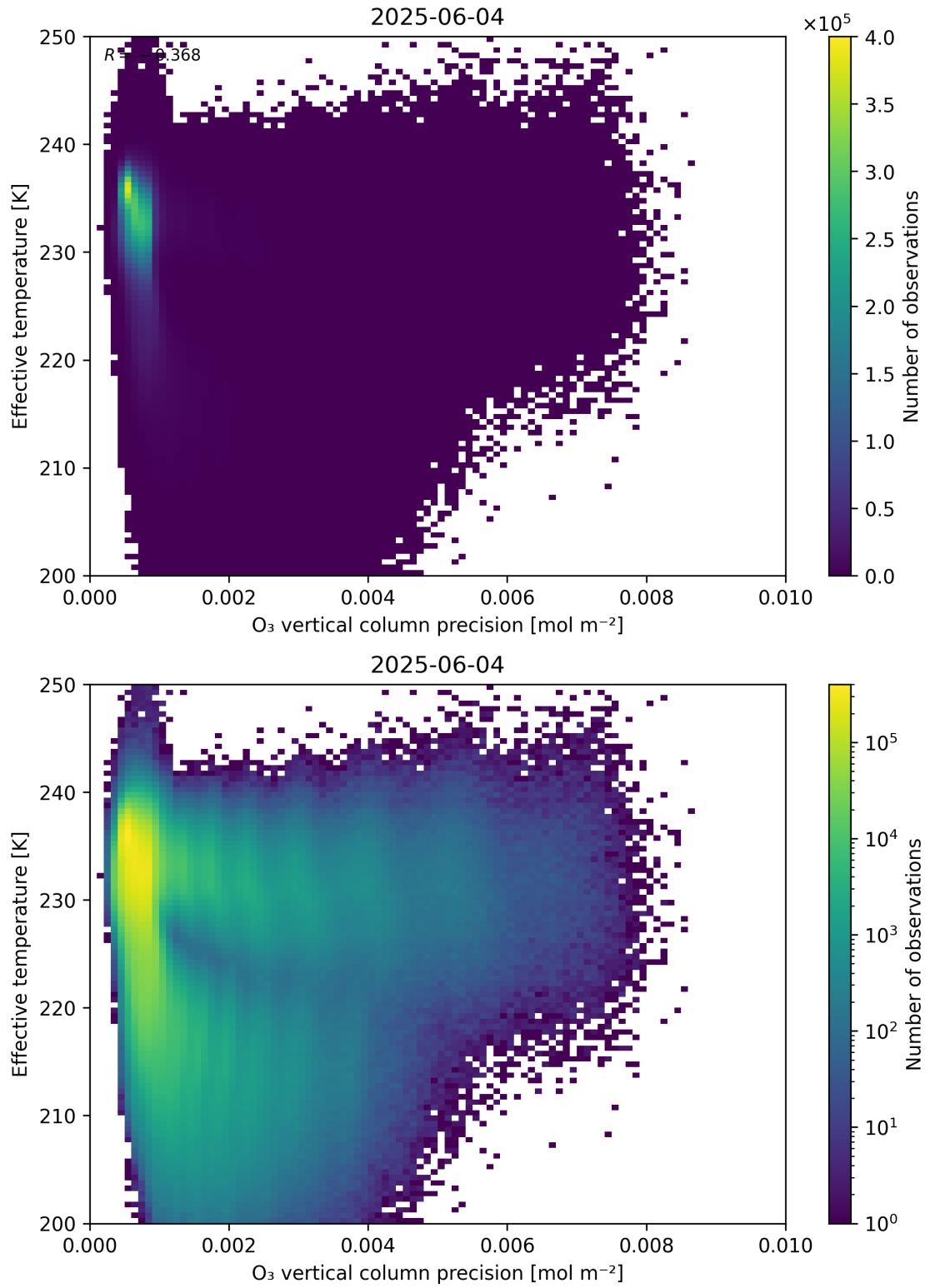
Figure 42: Scatter density plot of “O 3 vertical column precision” against “Effective temperature” for 2025-06-03 to 2025-06-05.
