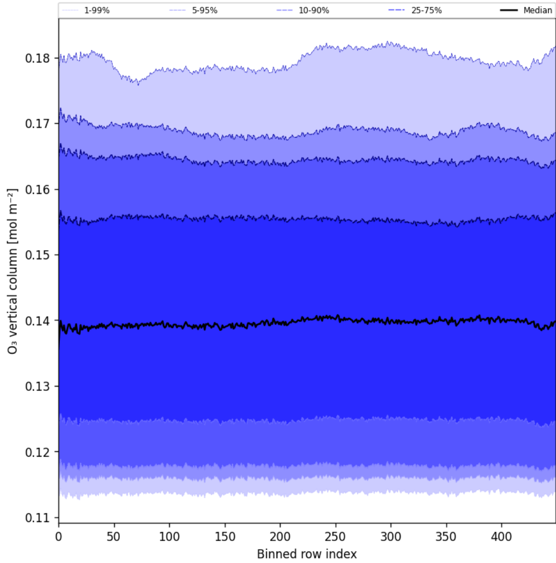
Figure 28: Along track statistics of “O 3 vertical column” for 2025-06-03 to 2025-06-05
