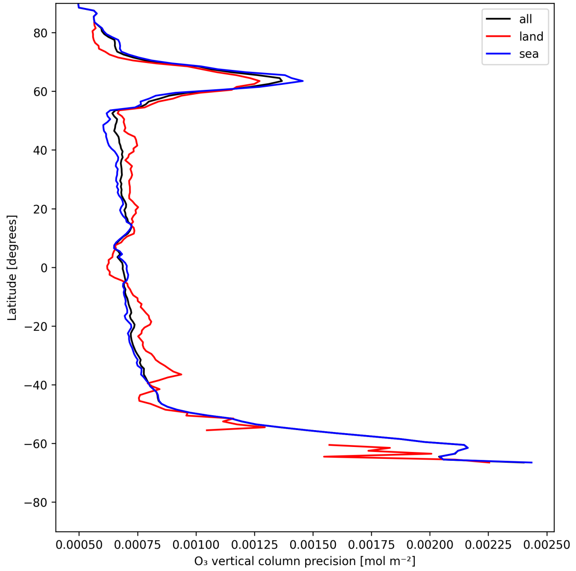
Figure 15: Zonal average of “O 3 vertical column precision” for 2025-06-03 to 2025-06-05.
