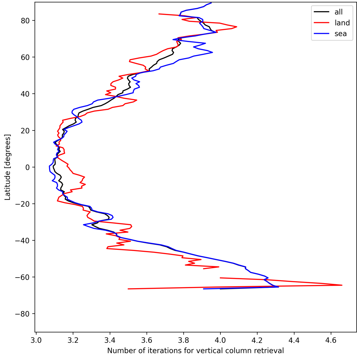
Figure 19: Zonal average of “Number of iterations for vertical column retrieval” for 2025-06-03 to 2025-06-05.
