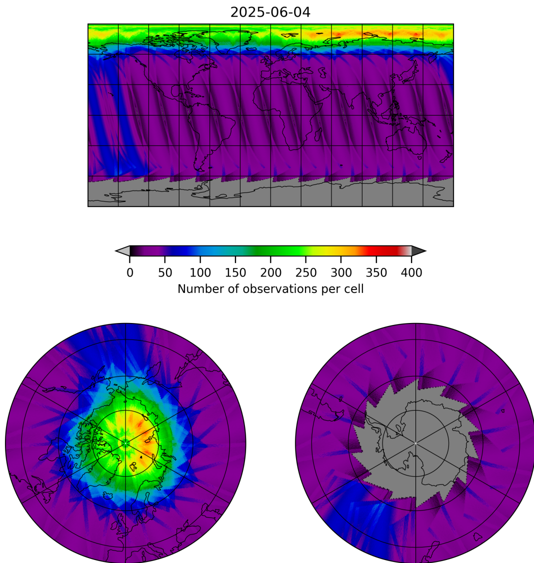
Figure 12: Map of the number of observations for 2025-06-03 to 2025-06-05
