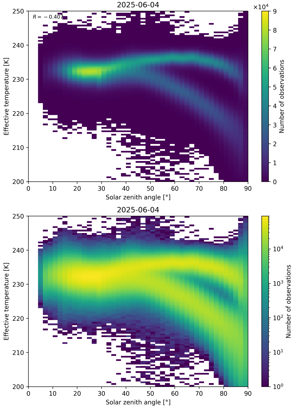
Figure 45: Scatter density plot of “Solar zenith angle” against “Effective temperature” for 2025-06-03 to 2025-06-05.
