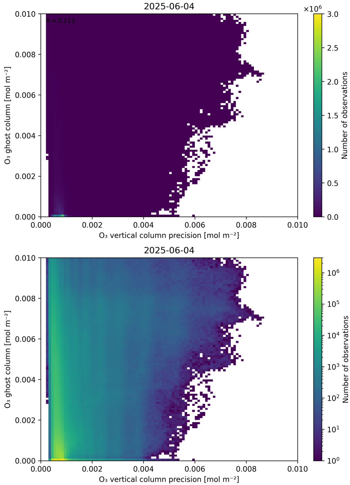
Figure 43: Scatter density plot of “ \text{O}_3 vertical column precision” against “ \text{O}_3 ghost column” for 2025-06-03 to 2025-06-05.
