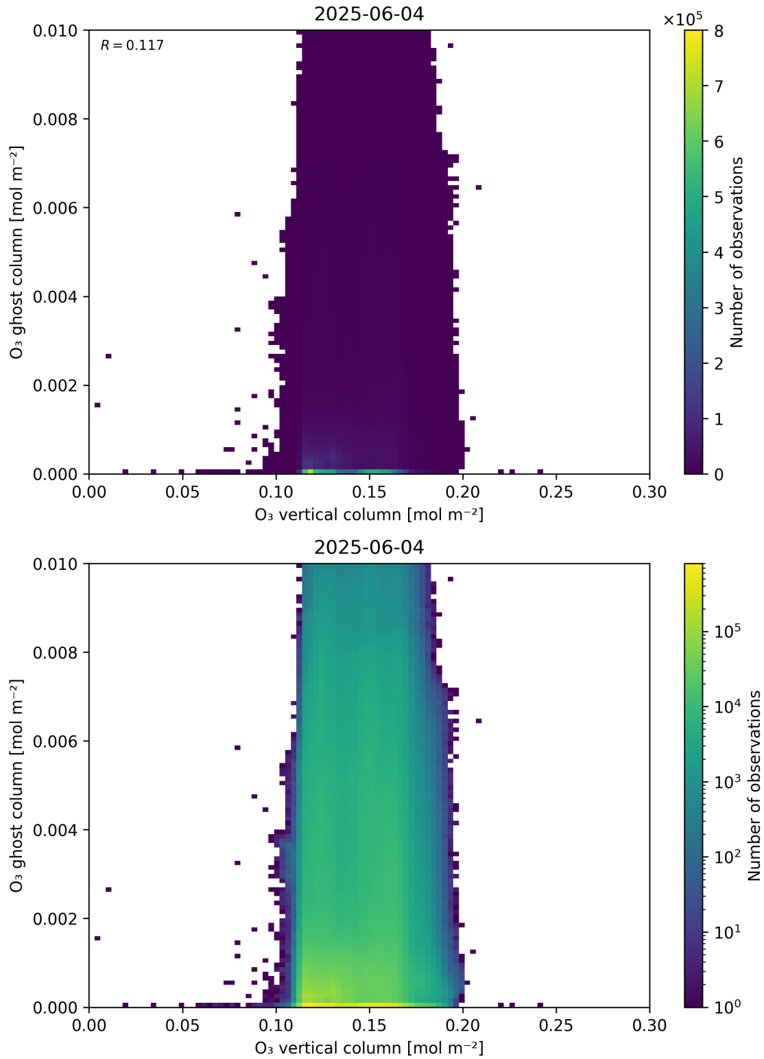
Figure 40: Scatter density plot of “O 3 vertical column” against “O 3 ghost column” for 2025-06-03 to 2025-06-05.
