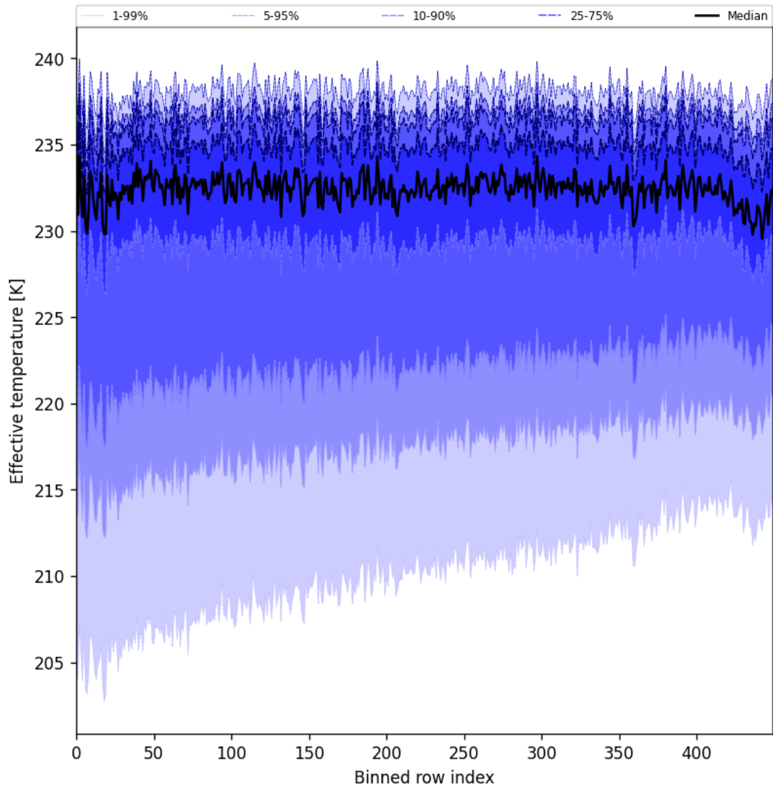
Figure 31: Along track statistics of “Effective temperature” for 2025-06-03 to 2025-06-05
