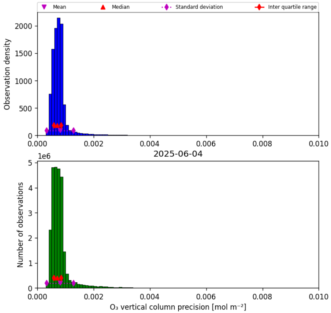
Figure 22: Histogram of "O 3 vertical column precision" for 2025-06-03 to 2025-06-05
