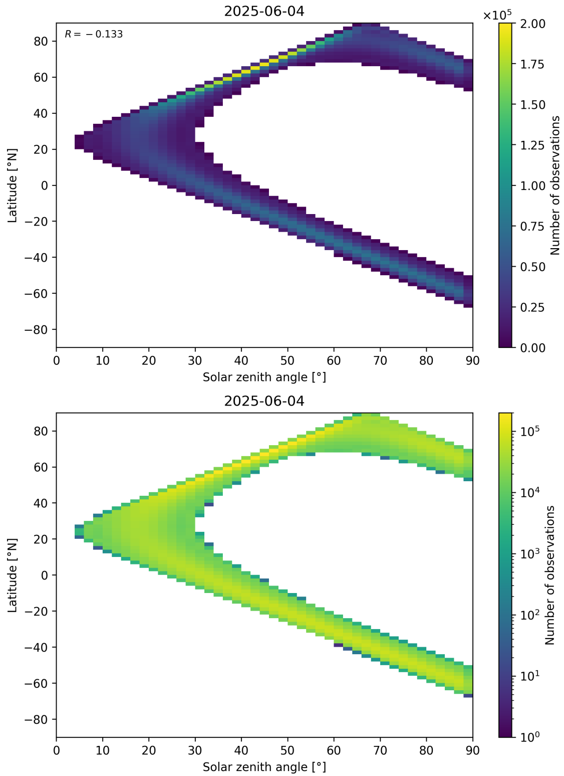
Figure 44: Scatter density plot of “Solar zenith angle” against “Latitude” for 2025-06-03 to 2025-06-05.
