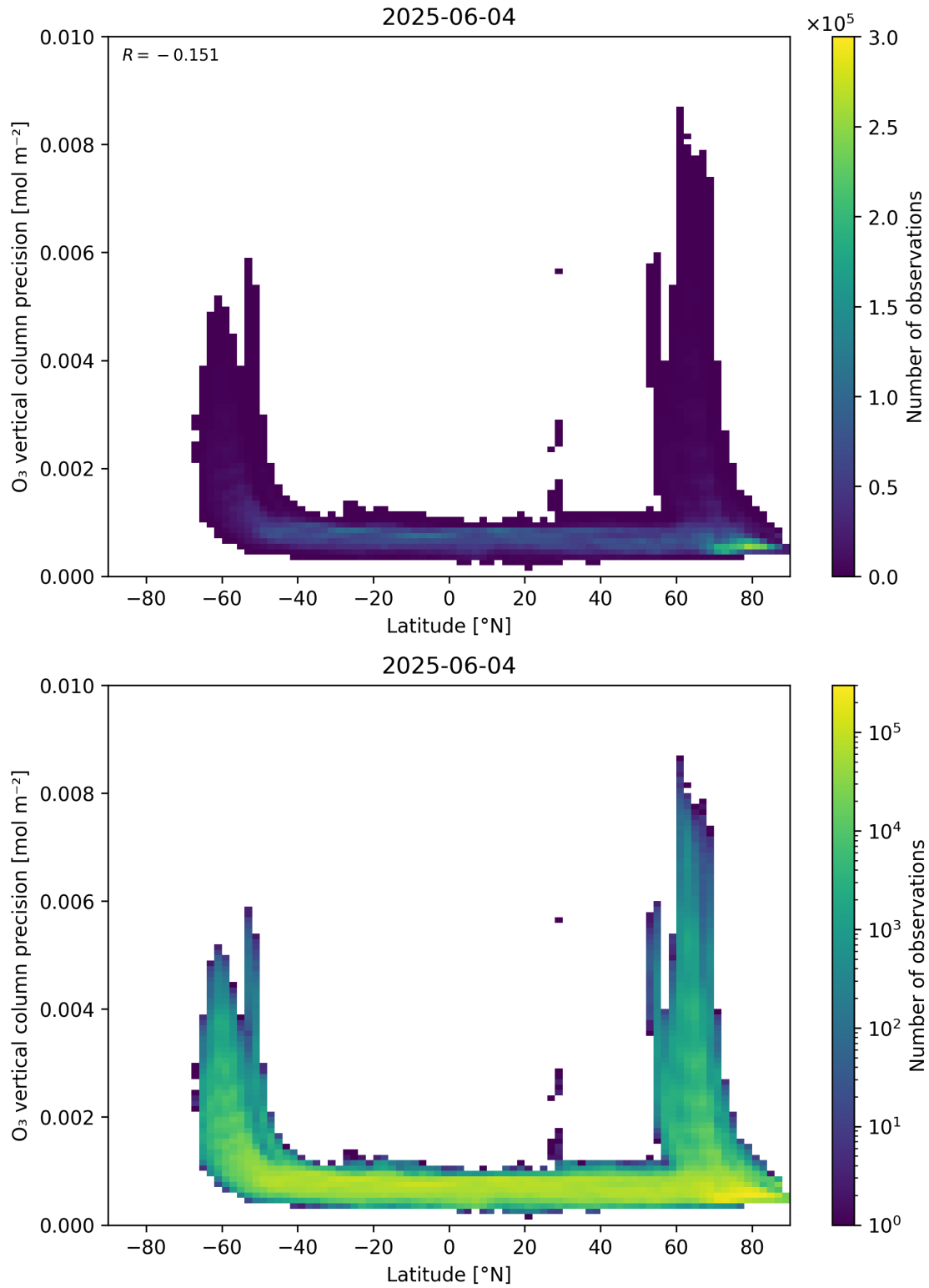
Figure 37: Scatter density plot of “Latitude” against “O 3 vertical column precision” for 2025-06-03 to 2025-06-05.
