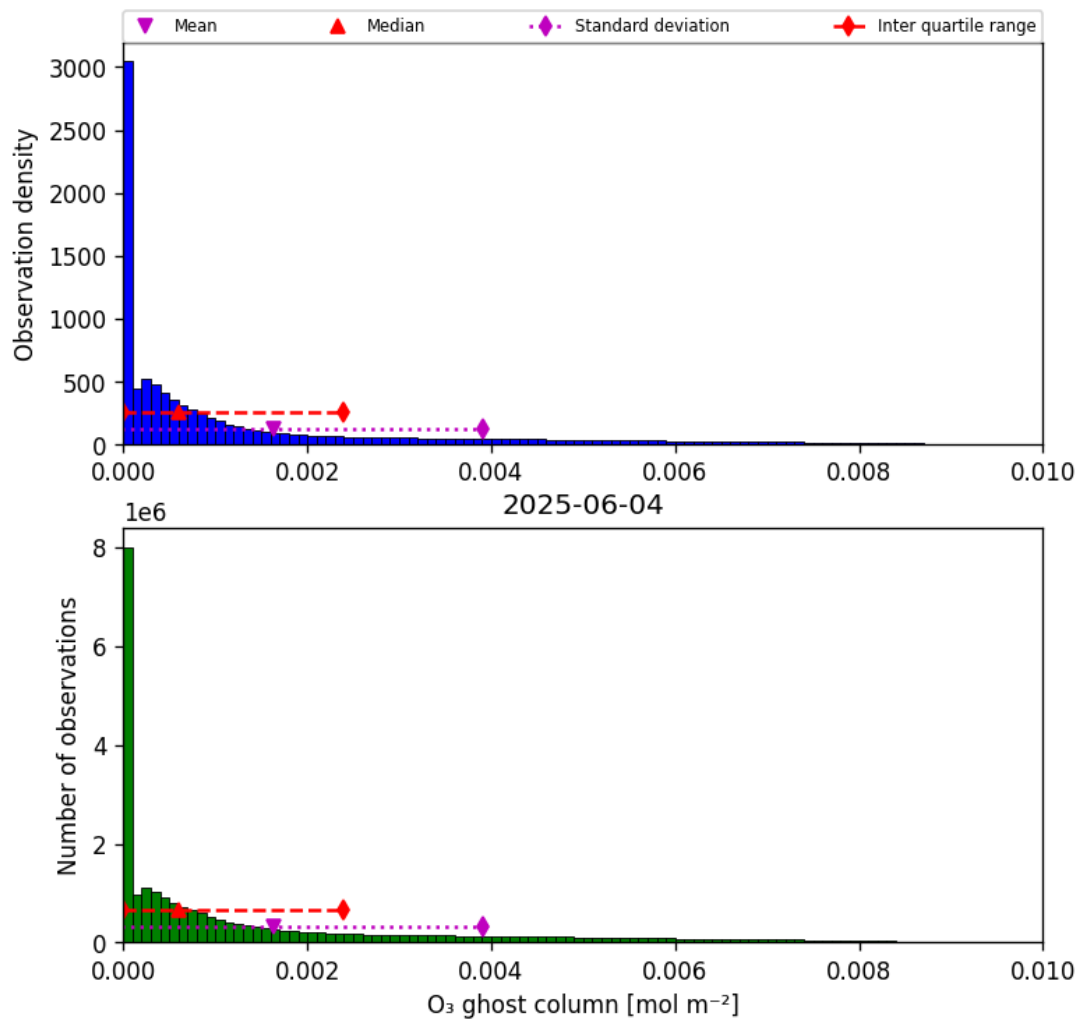
Figure 25: Histogram of “O 3 ghost column” for 2025-06-03 to 2025-06-05
