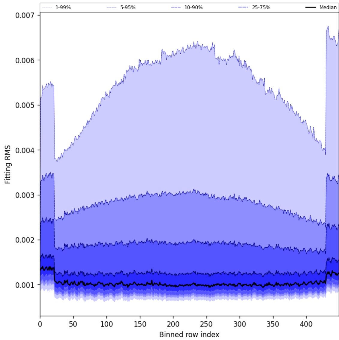
Figure 30: Along track statistics of “Fitting RMS” for 2025-06-03 to 2025-06-05
