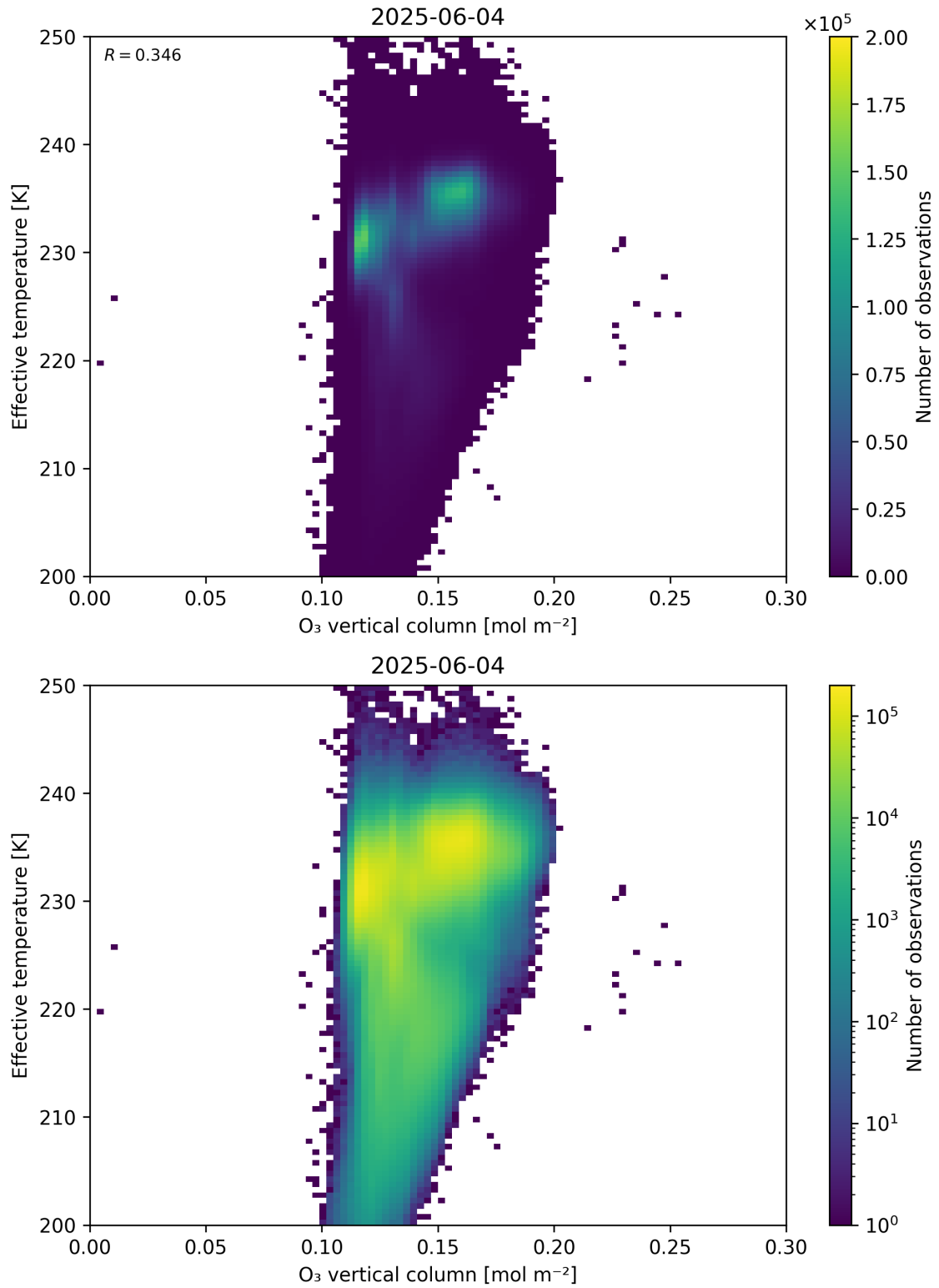
Figure 39: Scatter density plot of “O 3 vertical column” against “Effective temperature” for 2025-06-03 to 2025-06-05.
