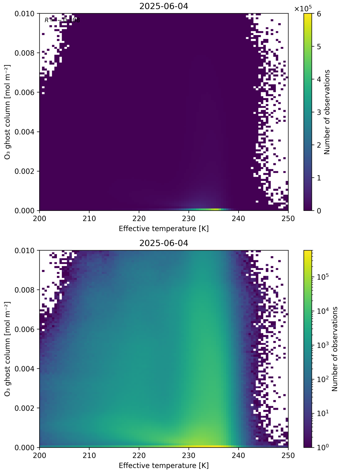
Figure 38: Scatter density plot of “Effective temperature” against “O 3 ghost column” for 2025-06-03 to 2025-06-05.
