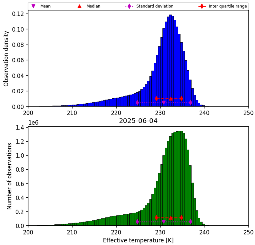
Figure 24: Histogram of “Effective temperature” for 2025-06-03 to 2025-06-05
