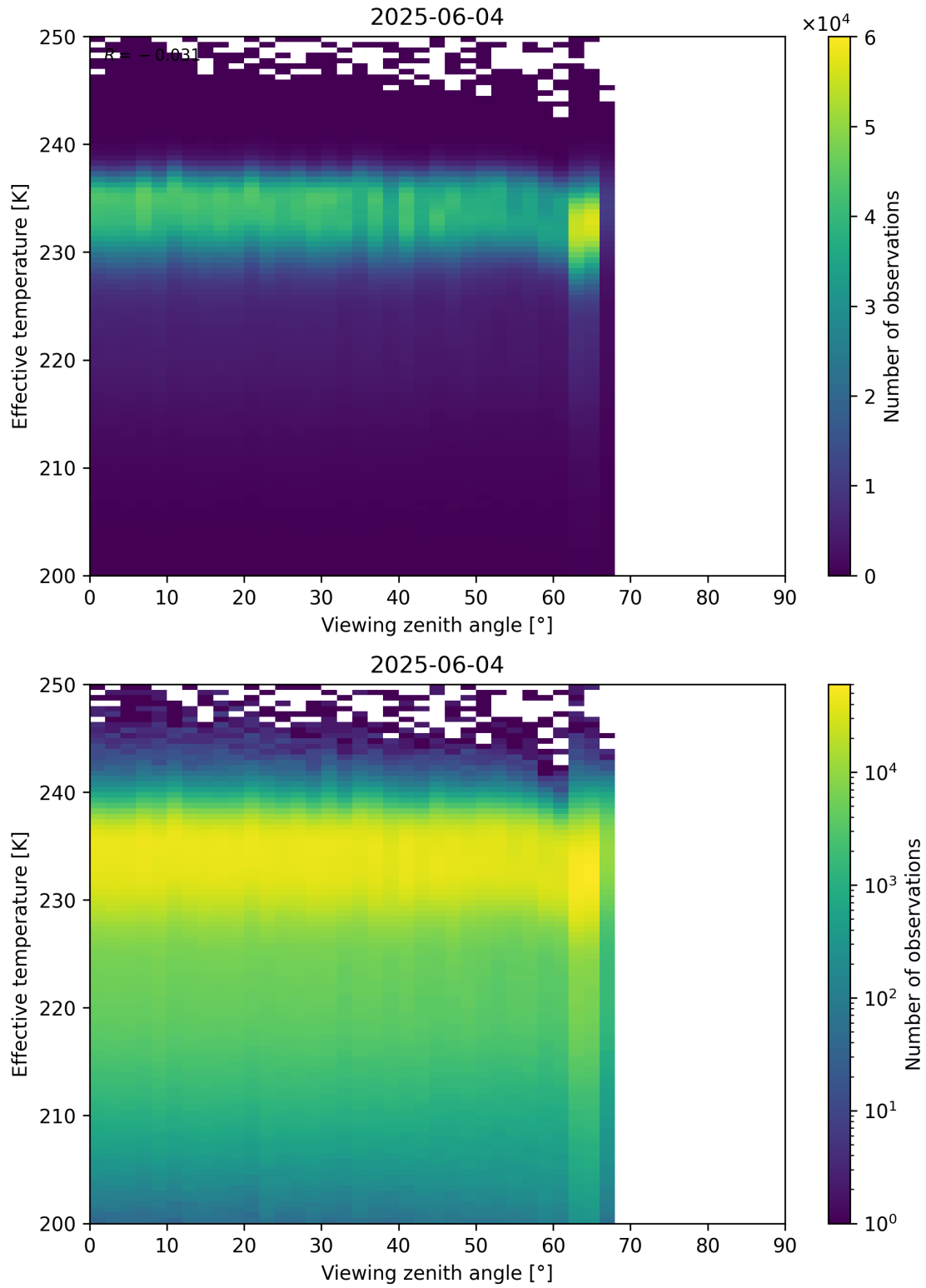
Figure 50: Scatter density plot of “Viewing zenith angle” against “Effective temperature” for 2025-06-03 to 2025-06-05.
