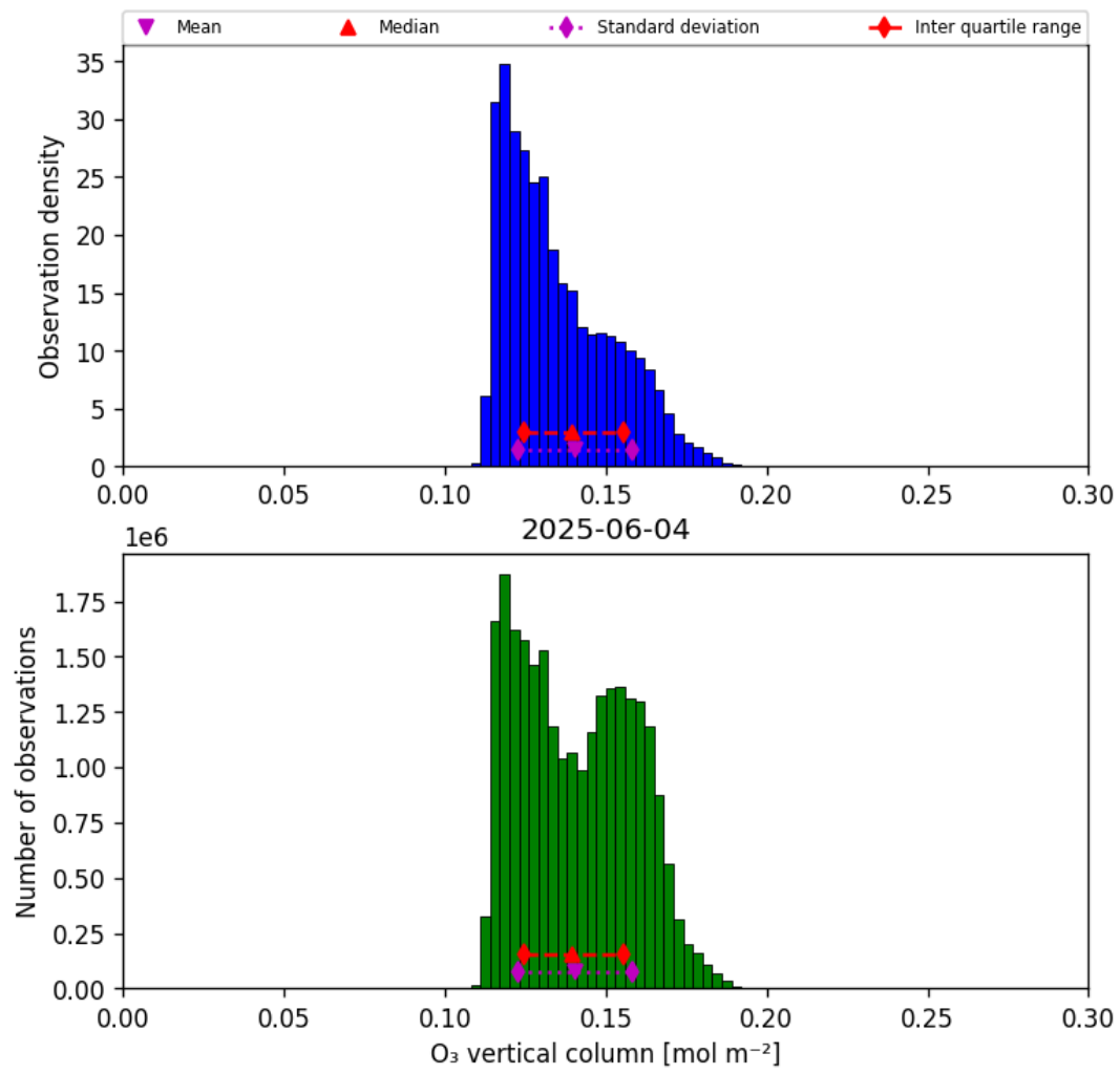
Figure 21: Histogram of “O 3 vertical column” for 2025-06-03 to 2025-06-05
