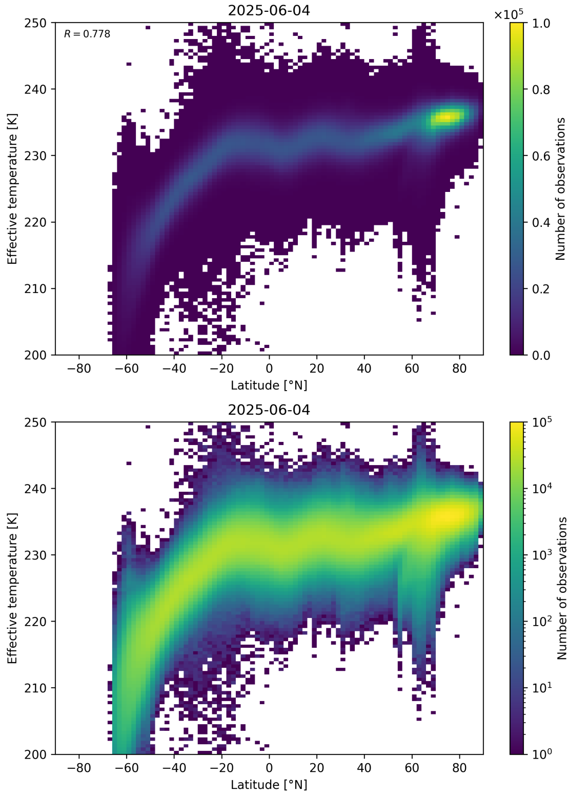
Figure 34: Scatter density plot of “Latitude” against “Effective temperature” for 2025-06-03 to 2025-06-05.
