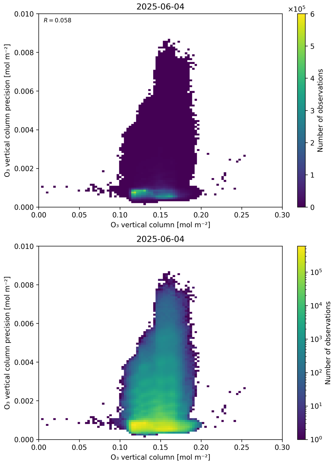
Figure 41: Scatter density plot of “O 3 vertical column” against “O 3 vertical column precision” for 2025-06-03 to 2025-06-05.
