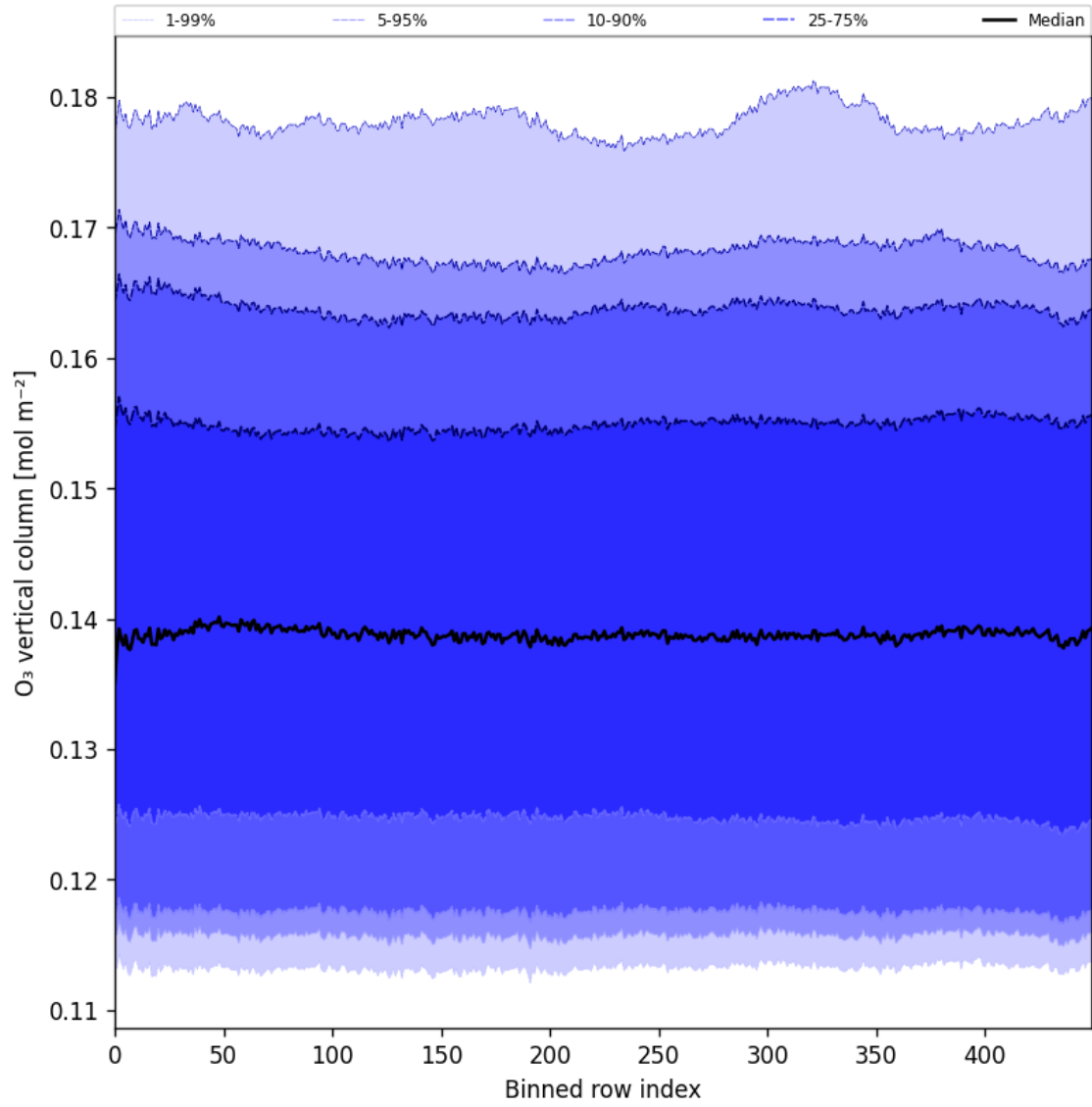
Figure 28: Along track statistics of “O 3 vertical column” for 2025-06-04 to 2025-06-06
