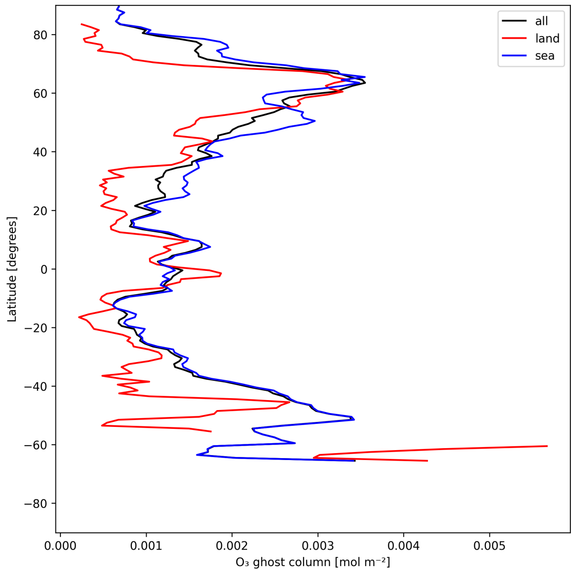
Figure 18: Zonal average of “O 3 ghost column” for 2025-06-04 to 2025-06-06.
