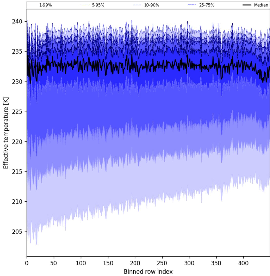
Figure 31: Along track statistics of “Effective temperature” for 2025-06-04 to 2025-06-06
