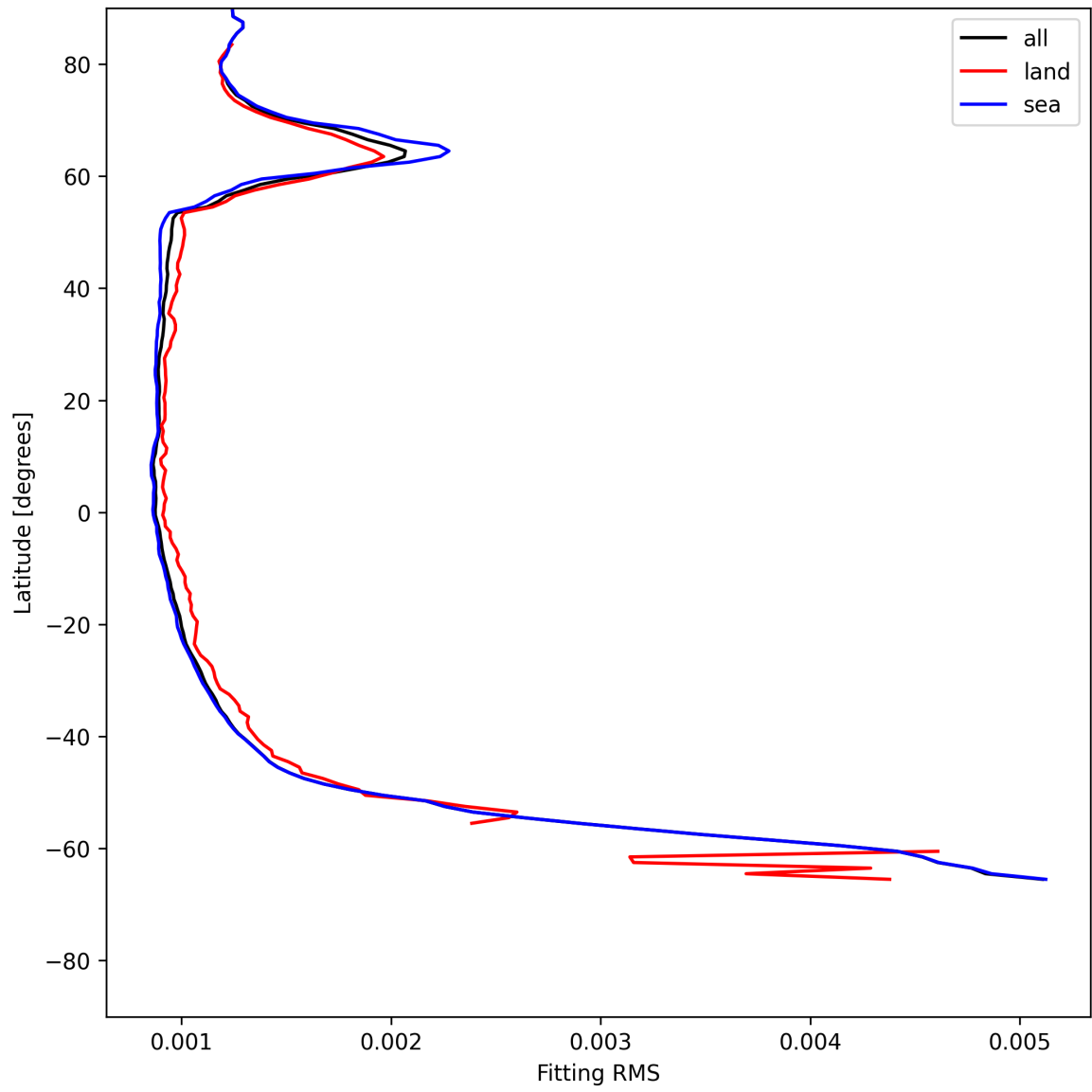
Figure 16: Zonal average of “Fitting RMS” for 2025-06-04 to 2025-06-06.
