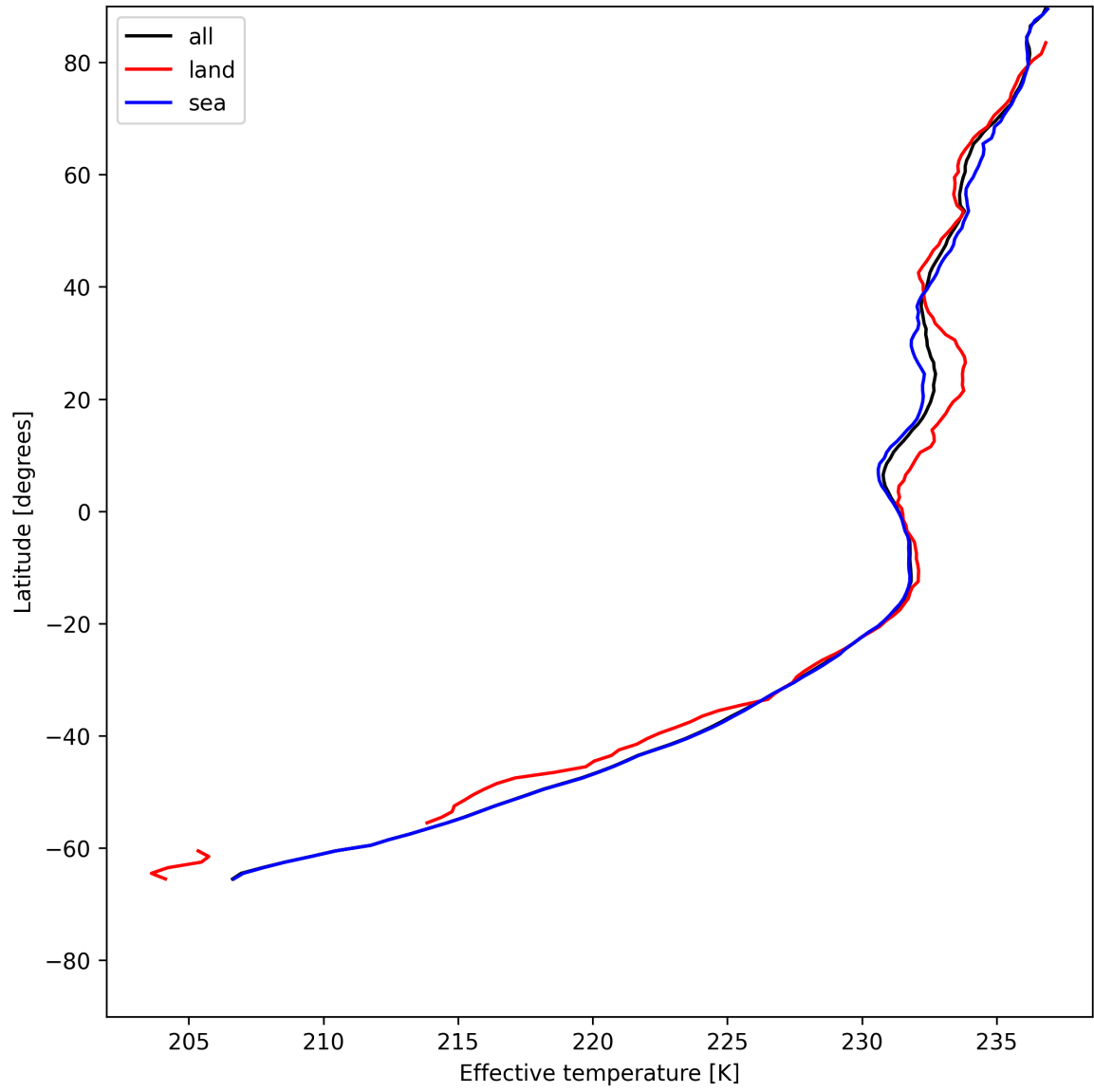
Figure 17: Zonal average of "Effective temperature" for 2025-06-04 to 2025-06-06.
