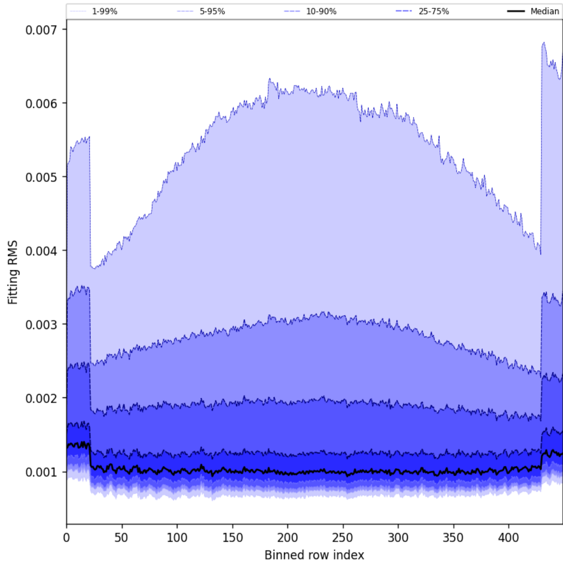
Figure 30: Along track statistics of “Fitting RMS” for 2025-06-04 to 2025-06-06
