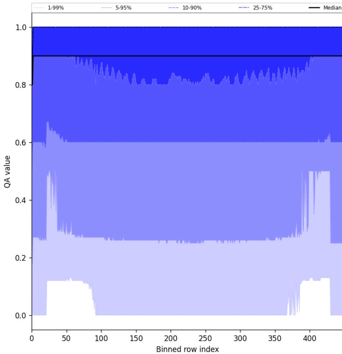
Figure 27: Along track statistics of “QA value” for 2025-06-04 to 2025-06-06
