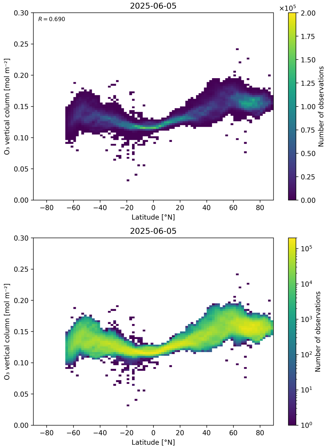
Figure 36: Scatter density plot of “Latitude” against “O 3 vertical column” for 2025-06-04 to 2025-06-06.
