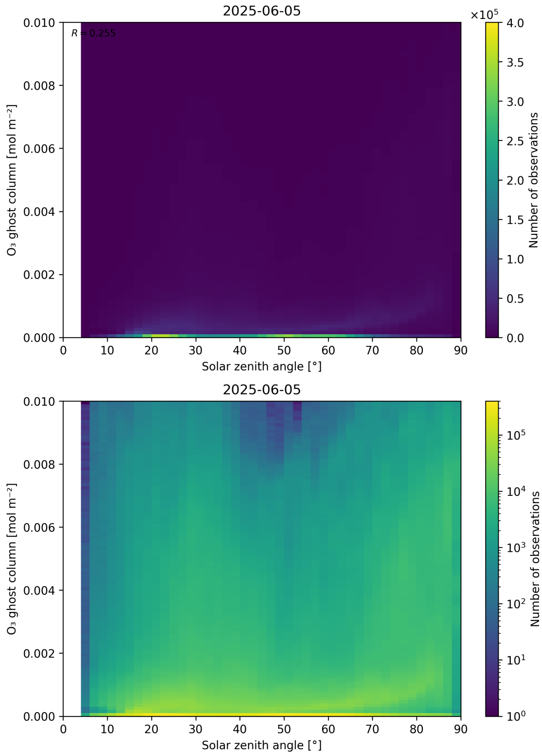
Figure 46: Scatter density plot of “Solar zenith angle” against “O 3 ghost column” for 2025-06-04 to 2025-06-06.
