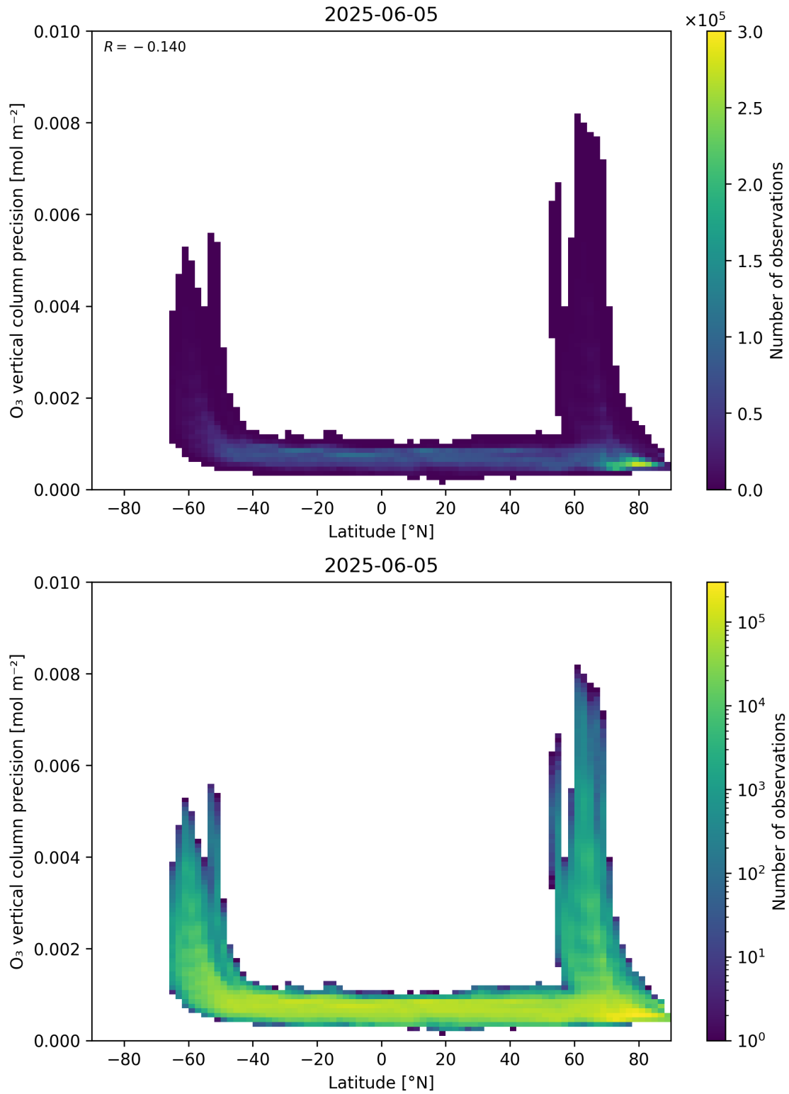
Figure 37: Scatter density plot of “Latitude” against “O 3 vertical column precision” for 2025-06-04 to 2025-06-06.
