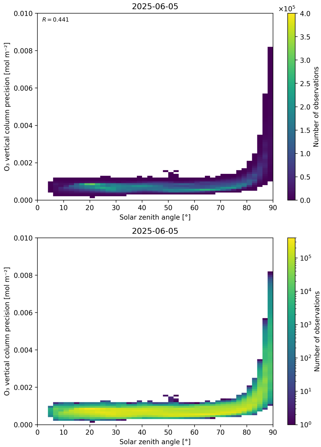
Figure 48: Scatter density plot of “Solar zenith angle” against “O 3 vertical column precision” for 2025-06-04 to 2025-06-06.
