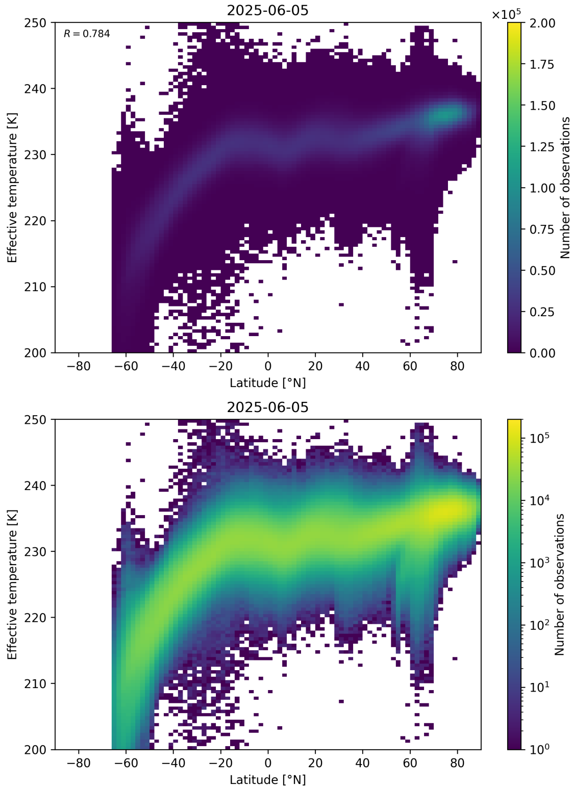
Figure 34: Scatter density plot of “Latitude” against “Effective temperature” for 2025-06-04 to 2025-06-06.
