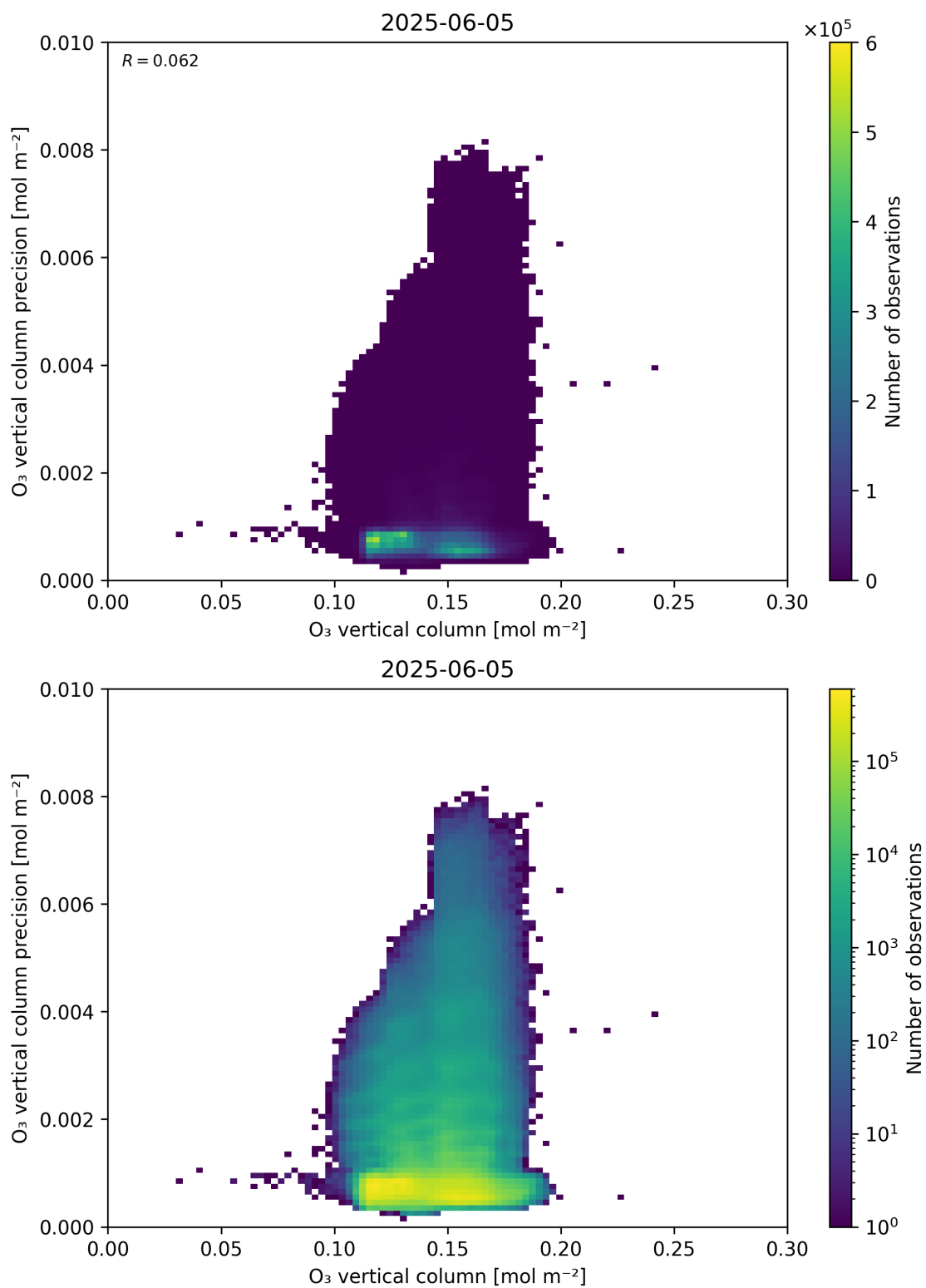
Figure 41: Scatter density plot of “O 3 vertical column” against “O 3 vertical column precision” for 2025-06-04 to 2025-06-06.
