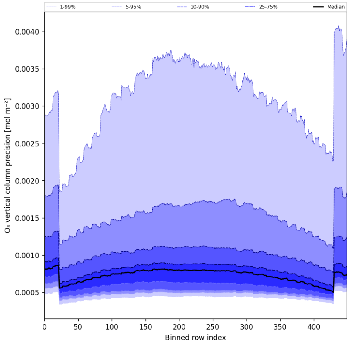
Figure 29: Along track statistics of “O 3 vertical column precision” for 2025-06-04 to 2025-06-06
