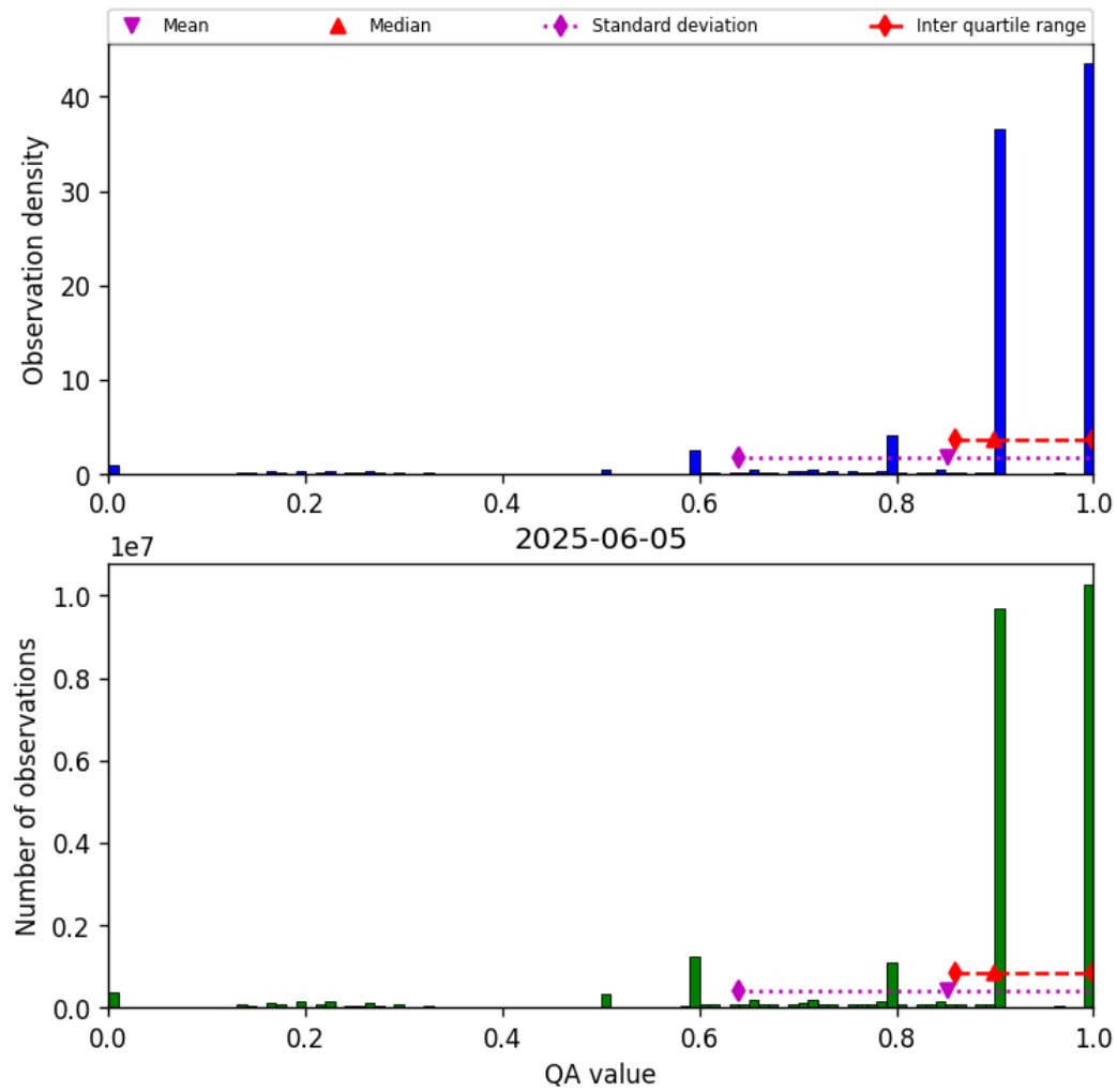
Figure 20: Histogram of “QA value” for 2025-06-04 to 2025-06-06
