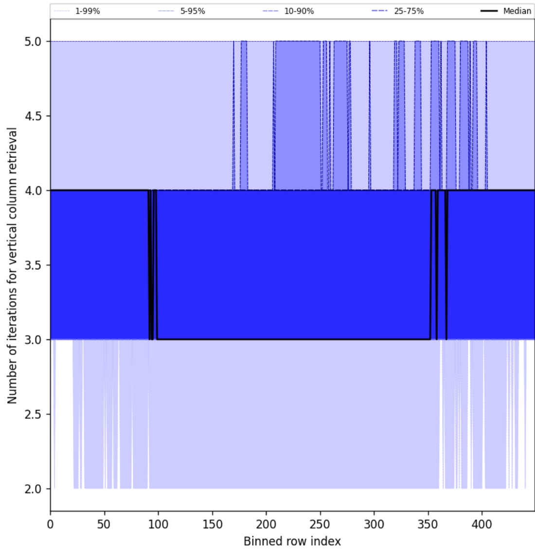
Figure 33: Along track statistics of “Number of iterations for vertical column retrieval” for 2025-06-04 to 2025-06-06
