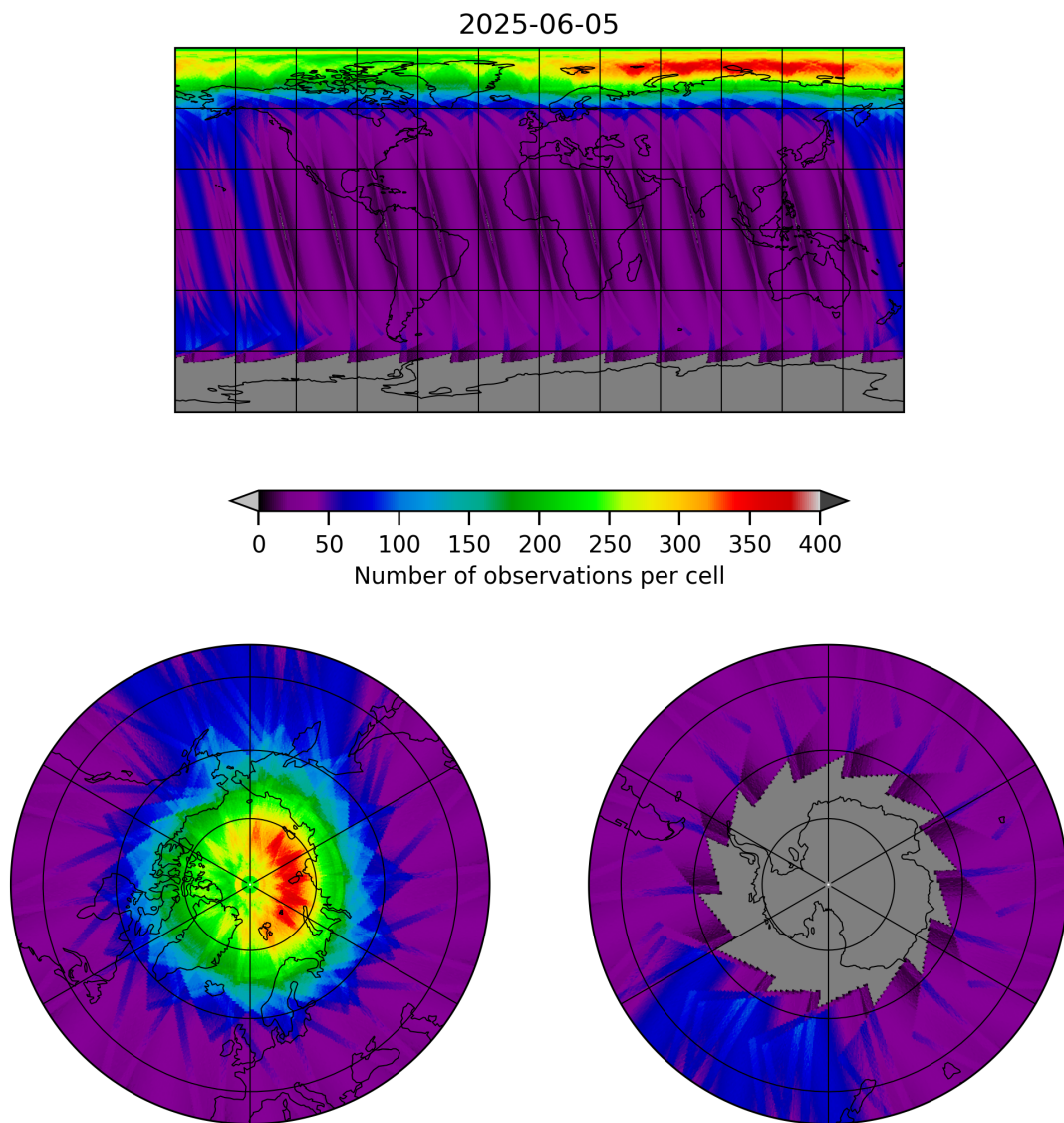
Figure 12: Map of the number of observations for 2025-06-04 to 2025-06-06
