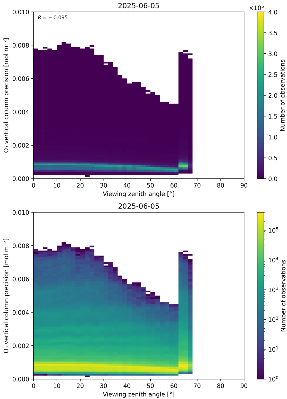
Figure 53: Scatter density plot of “Viewing zenith angle” against “O 3 vertical column precision” for 2025-06-04 to 2025-06-06.
