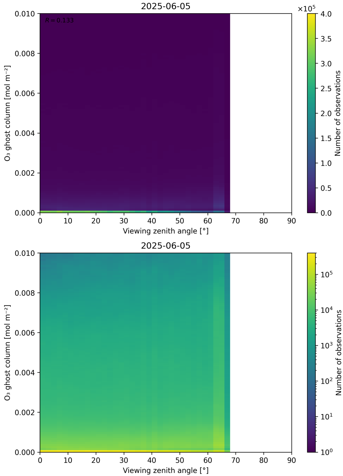
Figure 51: Scatter density plot of “Viewing zenith angle” against “O 3 ghost column” for 2025-06-04 to 2025-06-06.
