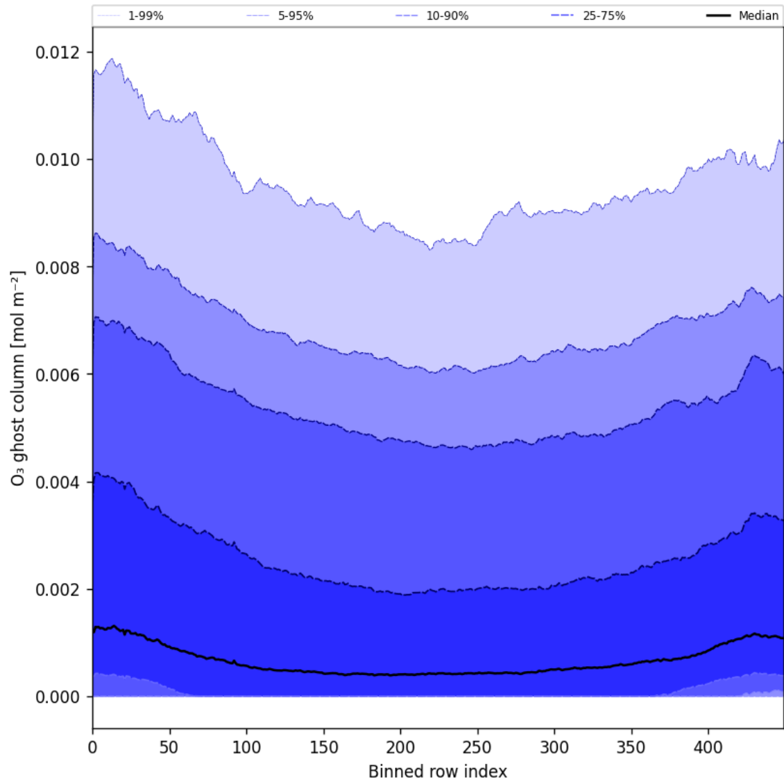
Figure 32: Along track statistics of “O 3 ghost column” for 2025-06-04 to 2025-06-06
