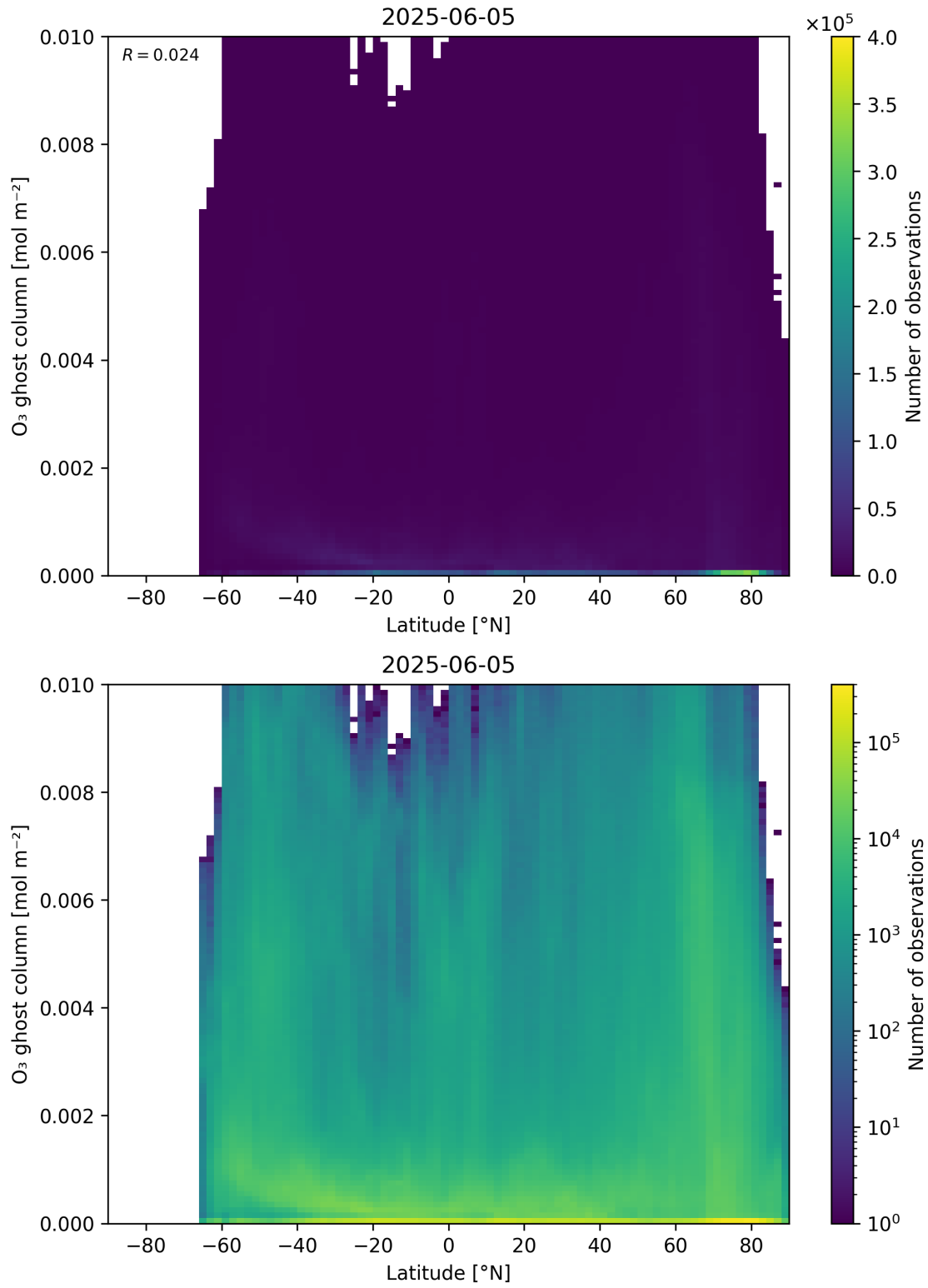
Figure 35: Scatter density plot of “Latitude” against “O 3 ghost column” for 2025-06-04 to 2025-06-06.
