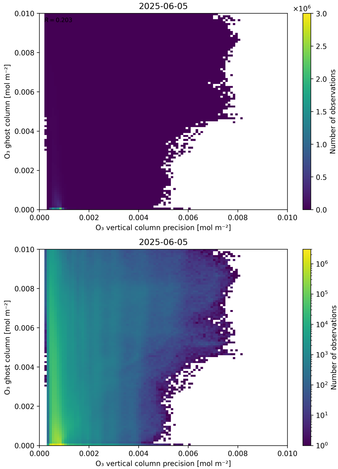
Figure 43: Scatter density plot of “ \text{O}_3 vertical column precision” against “ \text{O}_3 ghost column” for 2025-06-04 to 2025-06-06.
