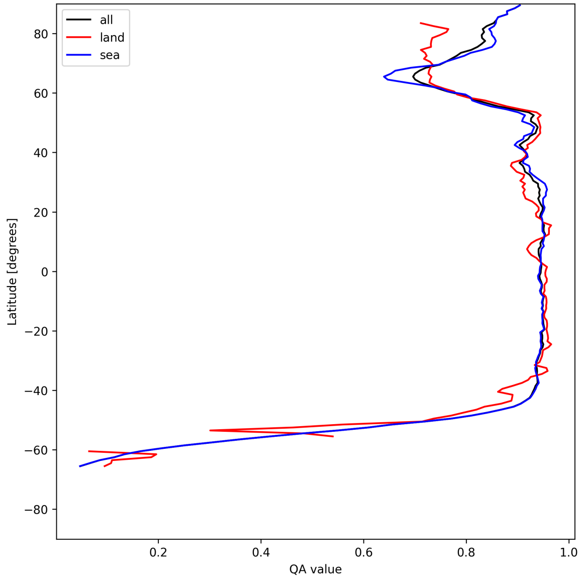
Figure 13: Zonal average of “QA value” for 2025-06-04 to 2025-06-06.
