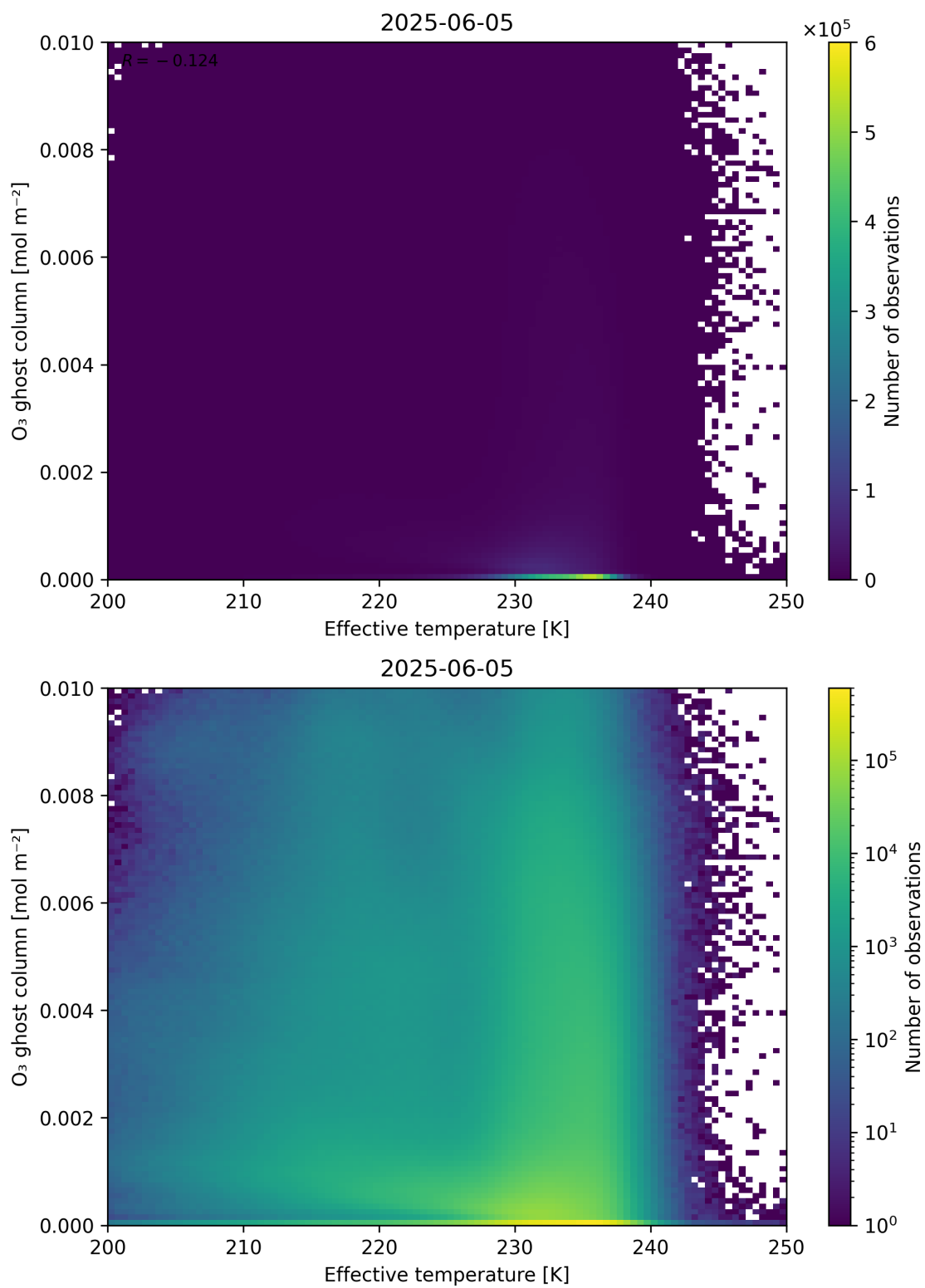
Figure 38: Scatter density plot of “Effective temperature” against “O 3 ghost column” for 2025-06-04 to 2025-06-06.
