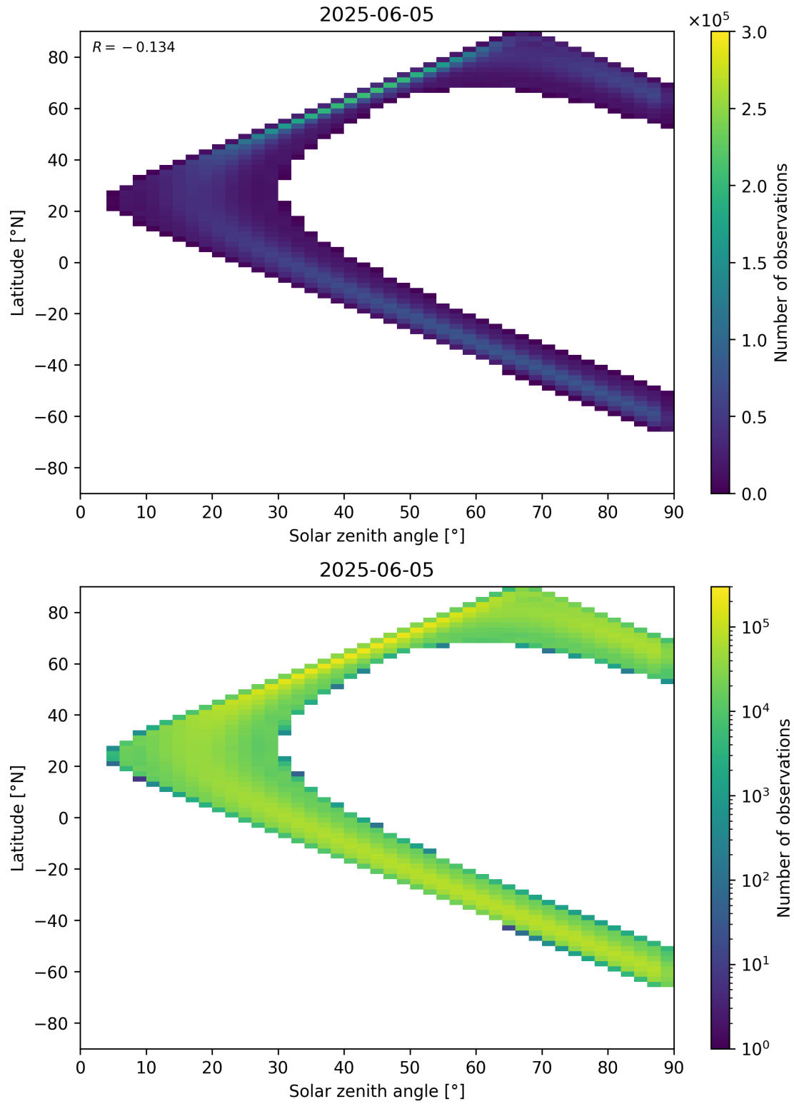
Figure 44: Scatter density plot of “Solar zenith angle” against “Latitude” for 2025-06-04 to 2025-06-06.
