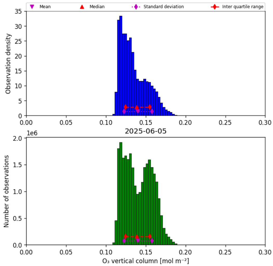
Figure 21: Histogram of “O 3 vertical column” for 2025-06-04 to 2025-06-06
