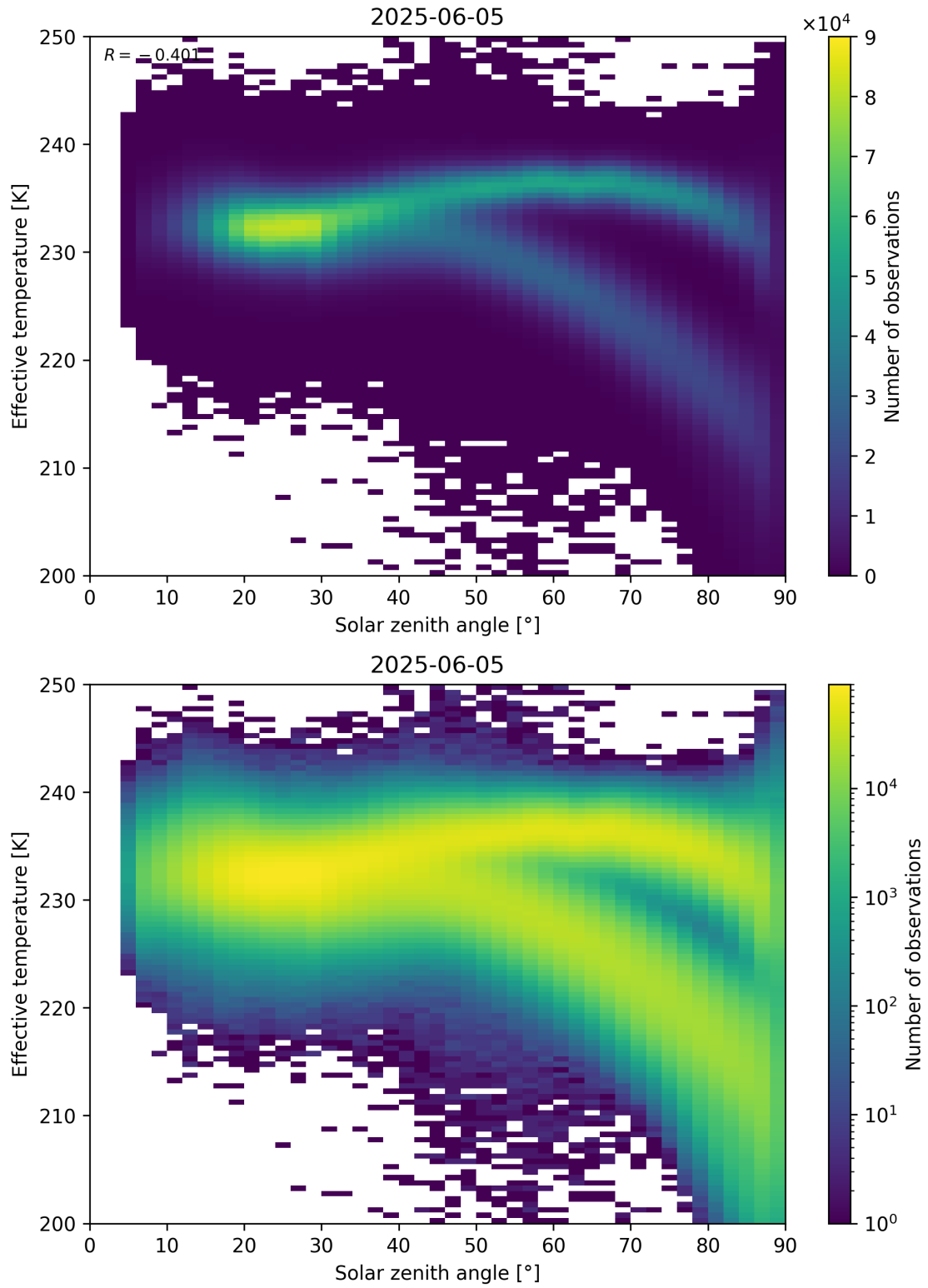
Figure 45: Scatter density plot of “Solar zenith angle” against “Effective temperature” for 2025-06-04 to 2025-06-06.
