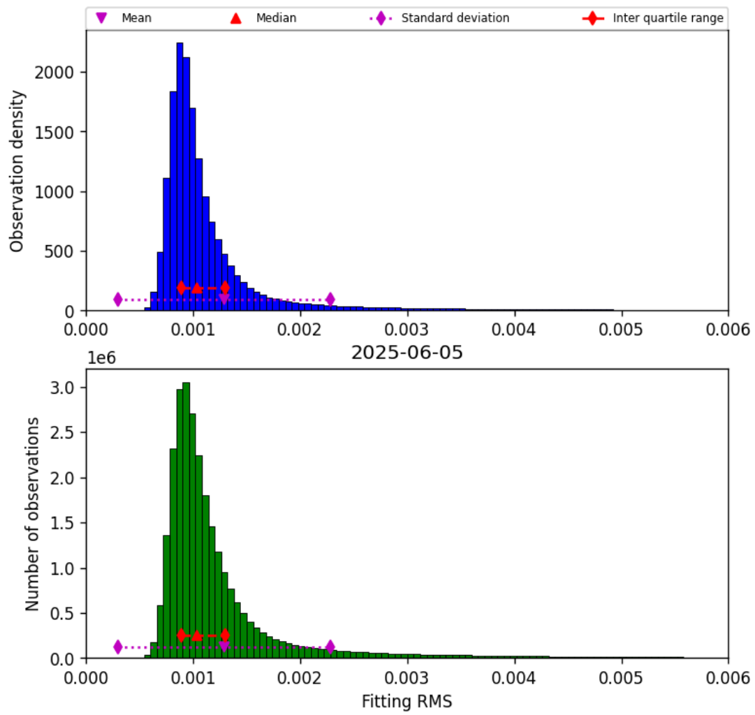
Figure 23: Histogram of “Fitting RMS” for 2025-06-04 to 2025-06-06
