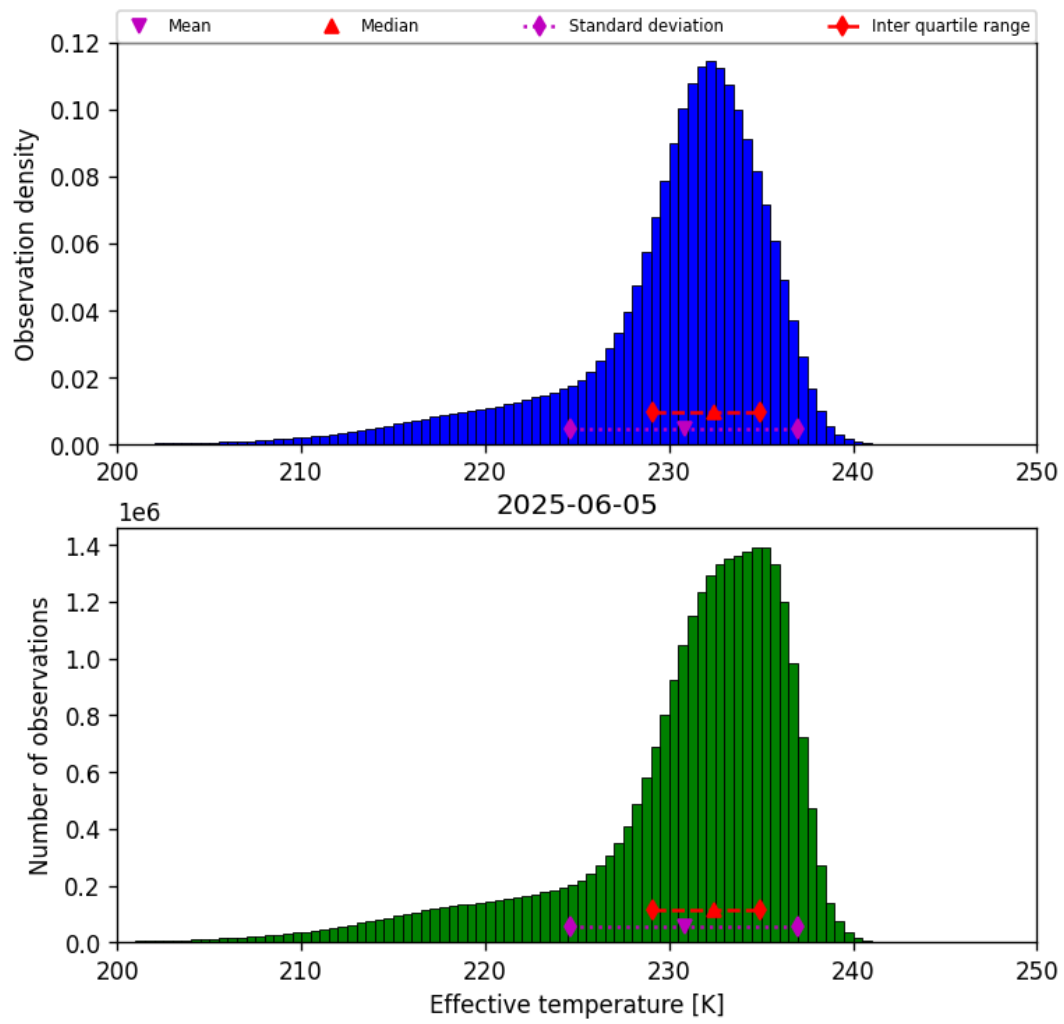
Figure 24: Histogram of “Effective temperature” for 2025-06-04 to 2025-06-06
