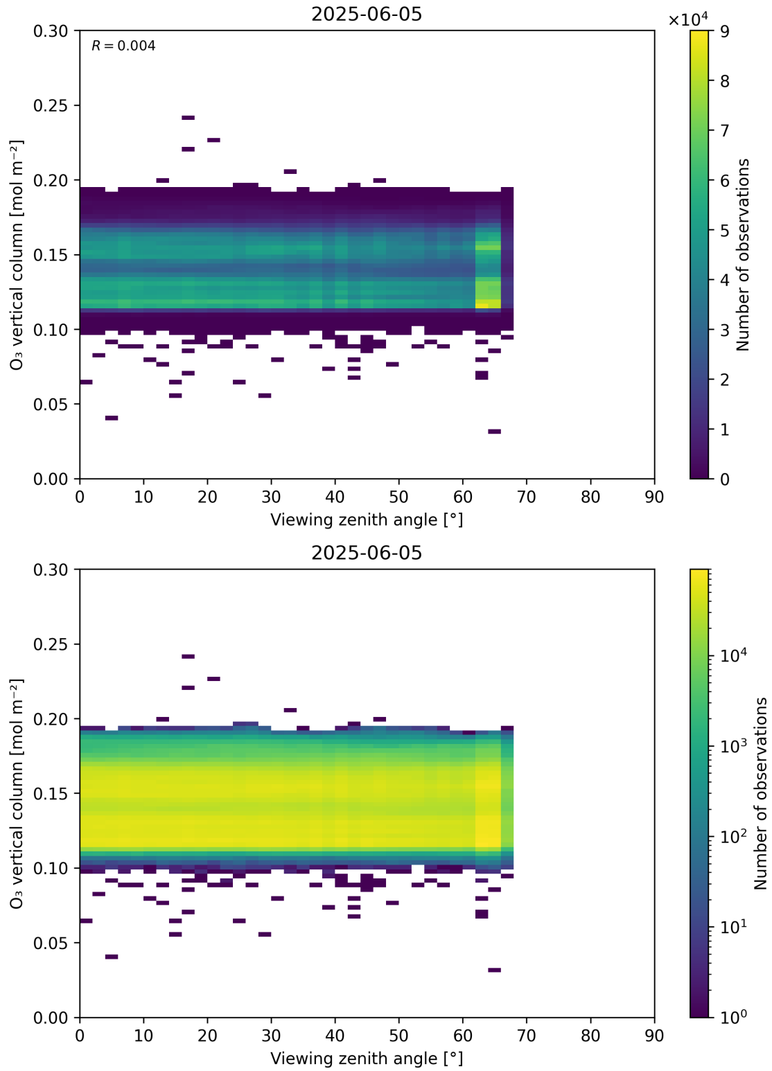
Figure 52: Scatter density plot of “Viewing zenith angle” against “O 3 vertical column” for 2025-06-04 to 2025-06-06.
