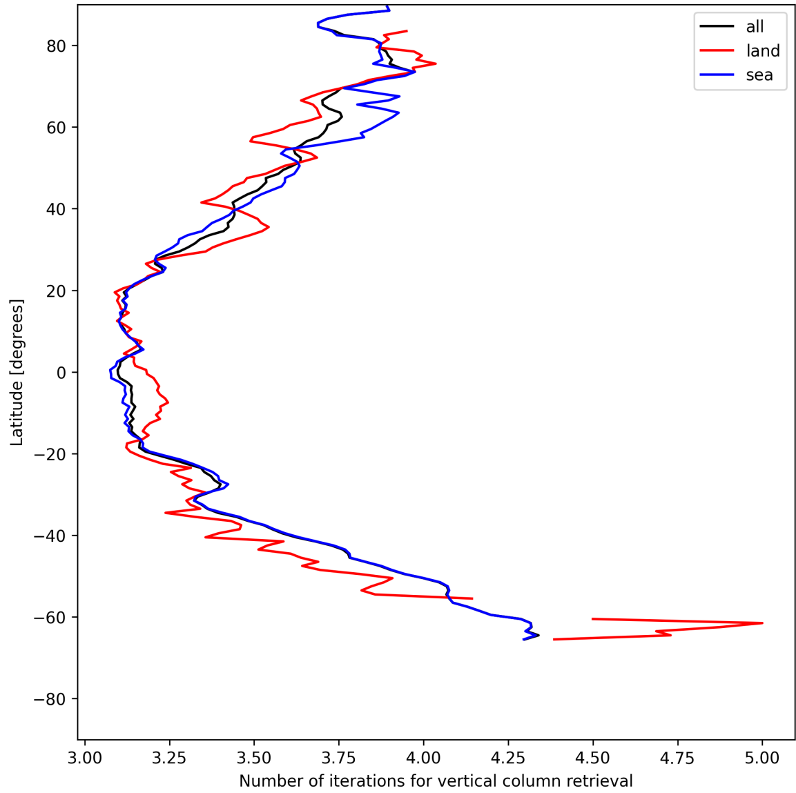
Figure 19: Zonal average of “Number of iterations for vertical column retrieval” for 2025-06-04 to 2025-06-06.
