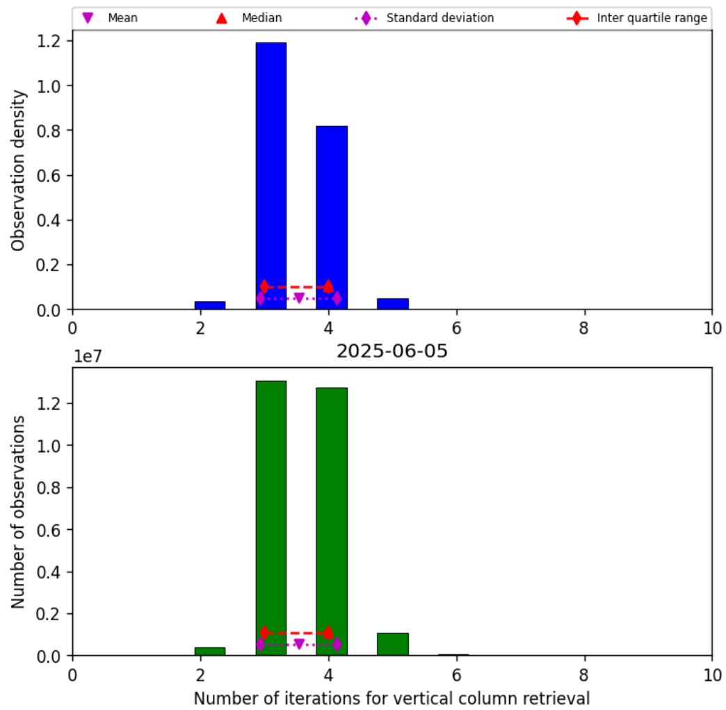
Figure 26: Histogram of “Number of iterations for vertical column retrieval” for 2025-06-04 to 2025-06-06
