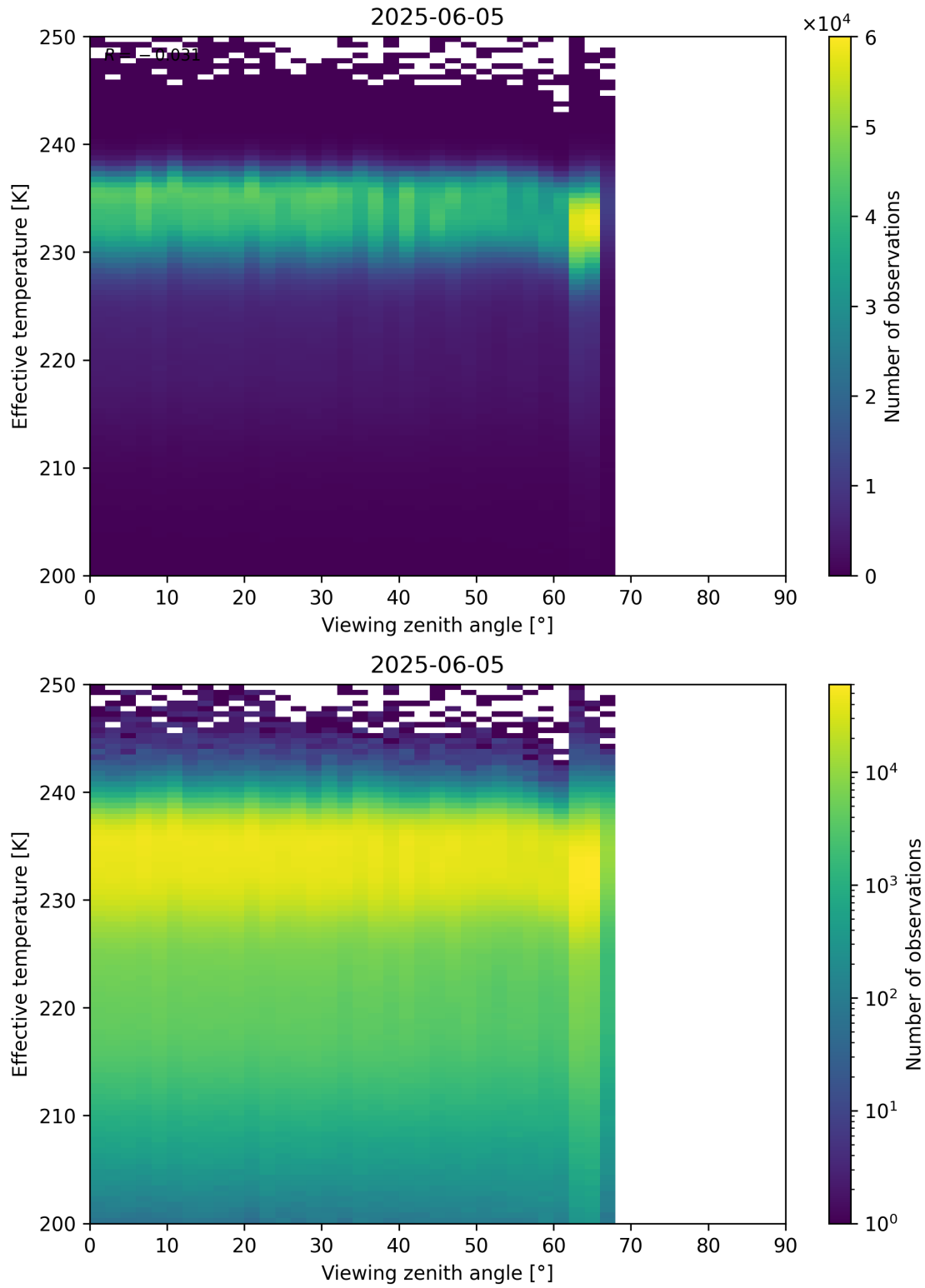
Figure 50: Scatter density plot of “Viewing zenith angle” against “Effective temperature” for 2025-06-04 to 2025-06-06.
