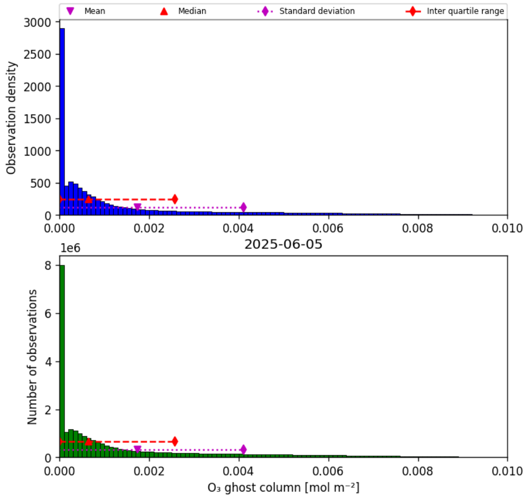
Figure 25: Histogram of “O 3 ghost column” for 2025-06-04 to 2025-06-06
