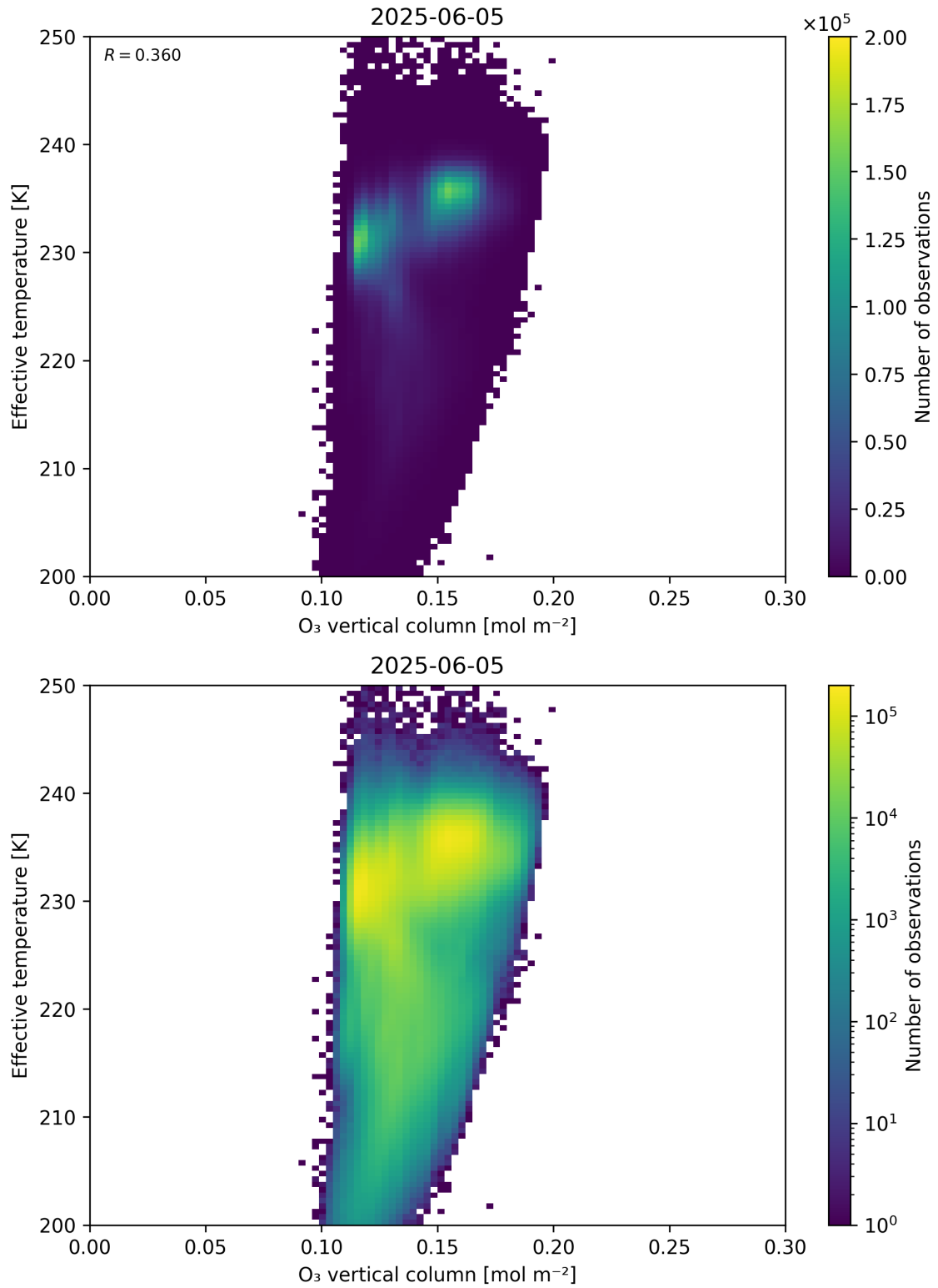
Figure 39: Scatter density plot of “O 3 vertical column” against “Effective temperature” for 2025-06-04 to 2025-06-06.
