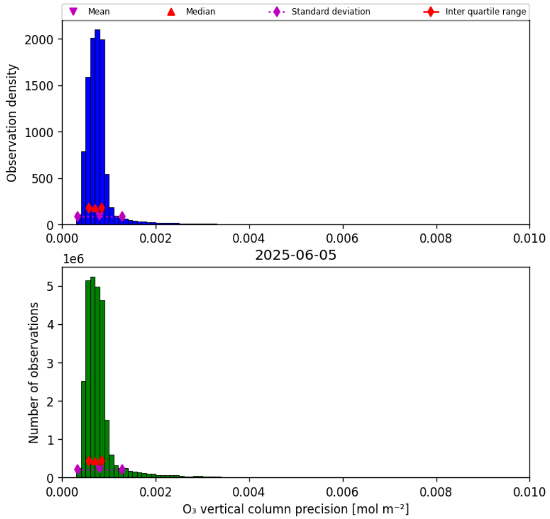
Figure 22: Histogram of “O 3 vertical column precision” for 2025-06-04 to 2025-06-06
