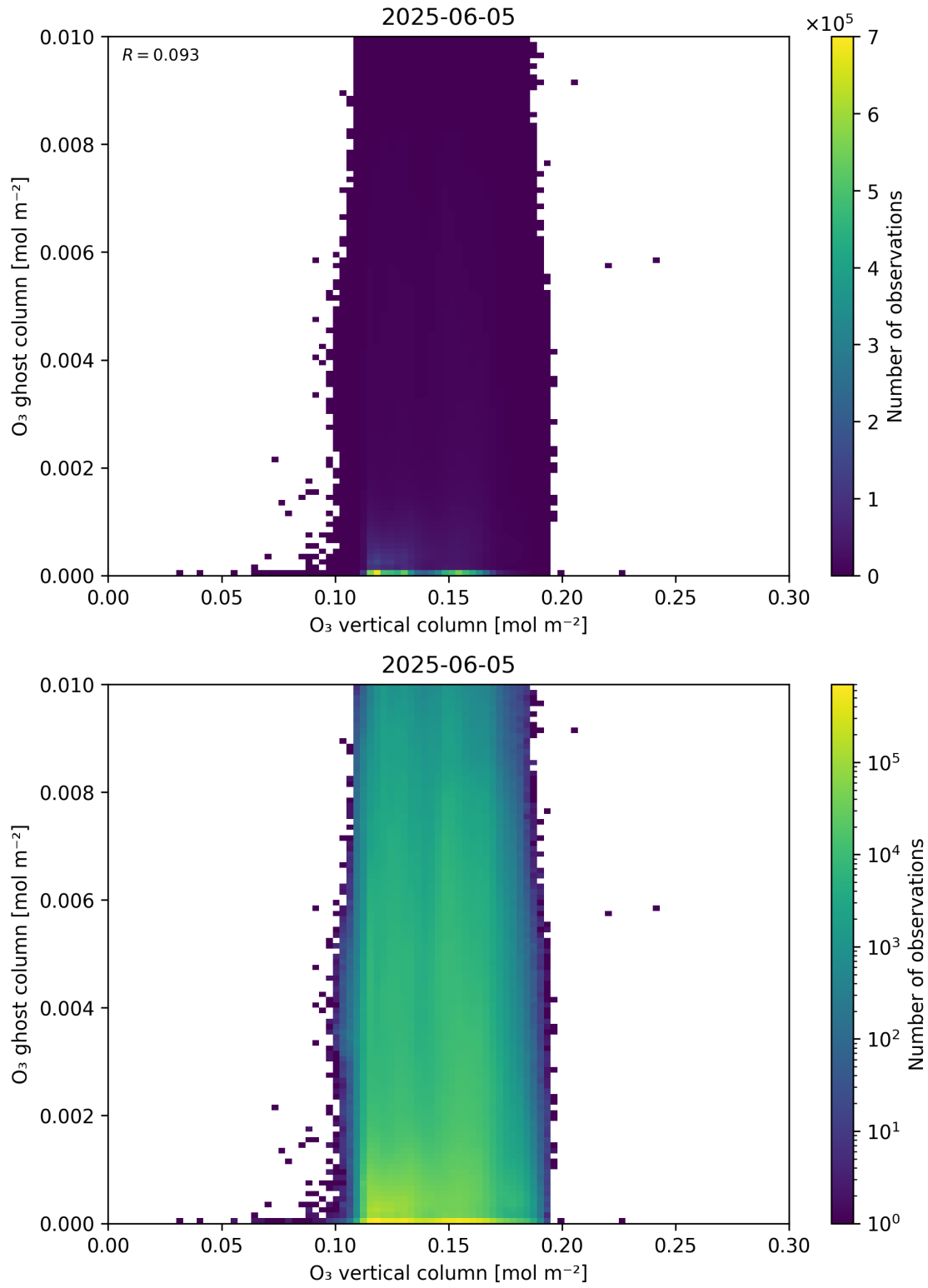
Figure 40: Scatter density plot of “O 3 vertical column” against “O 3 ghost column” for 2025-06-04 to 2025-06-06.
