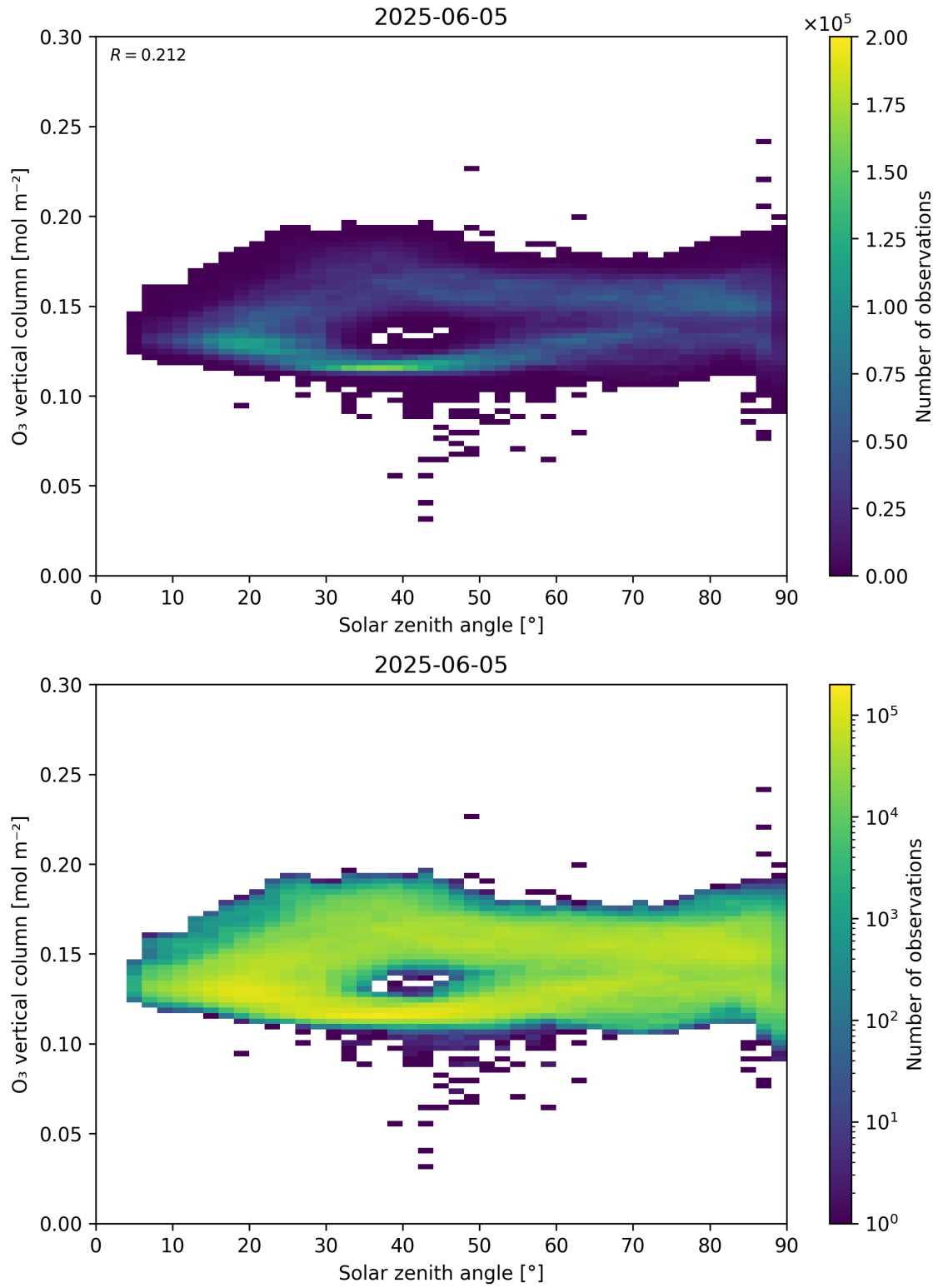
Figure 47: Scatter density plot of “Solar zenith angle” against “O 3 vertical column” for 2025-06-04 to 2025-06-06.
