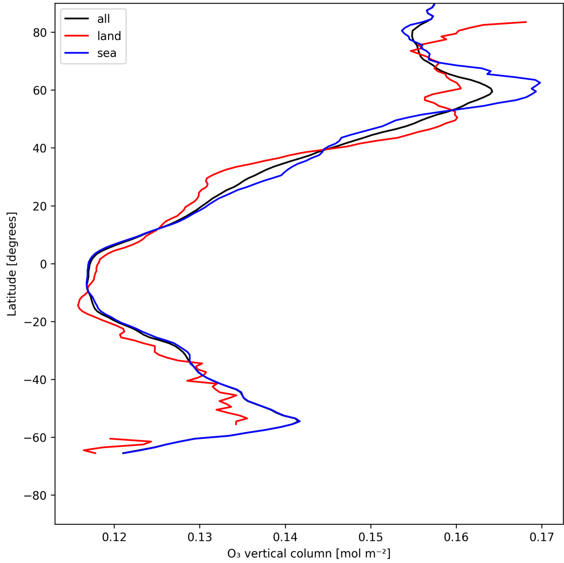
Figure 14: Zonal average of “O 3 vertical column” for 2025-06-04 to 2025-06-06.
