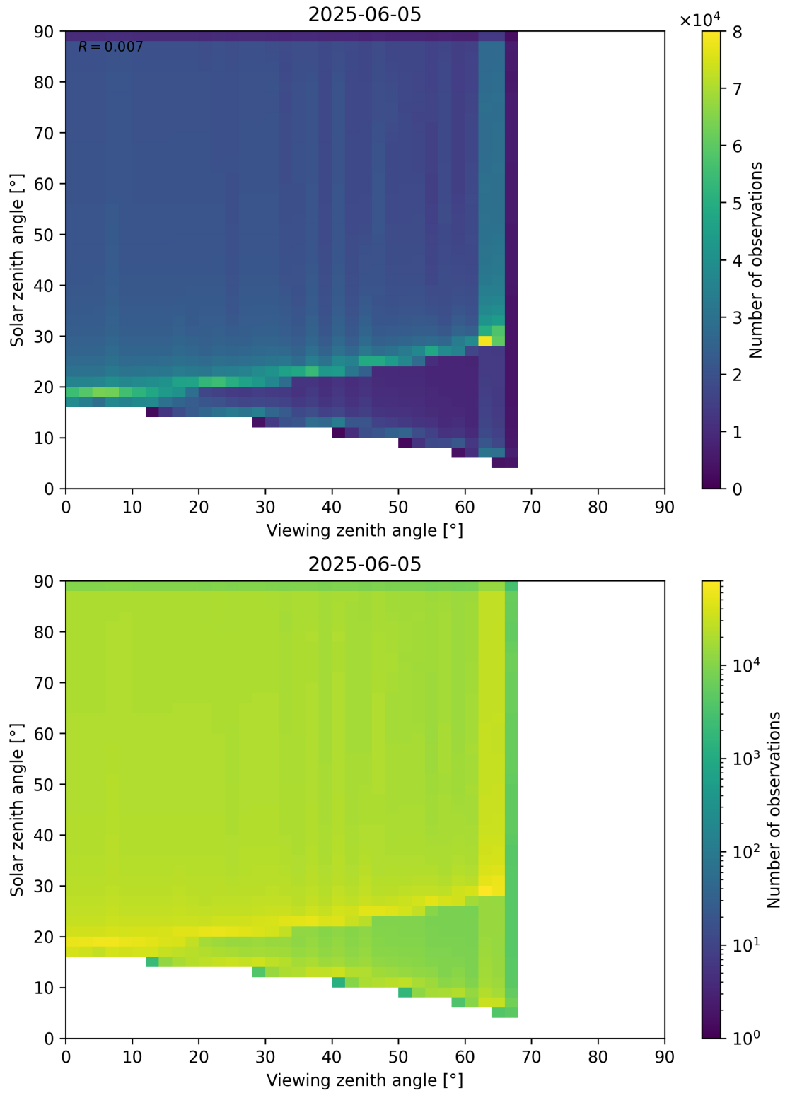
Figure 54: Scatter density plot of “Viewing zenith angle” against “Solar zenith angle” for 2025-06-04 to 2025-06-06.
