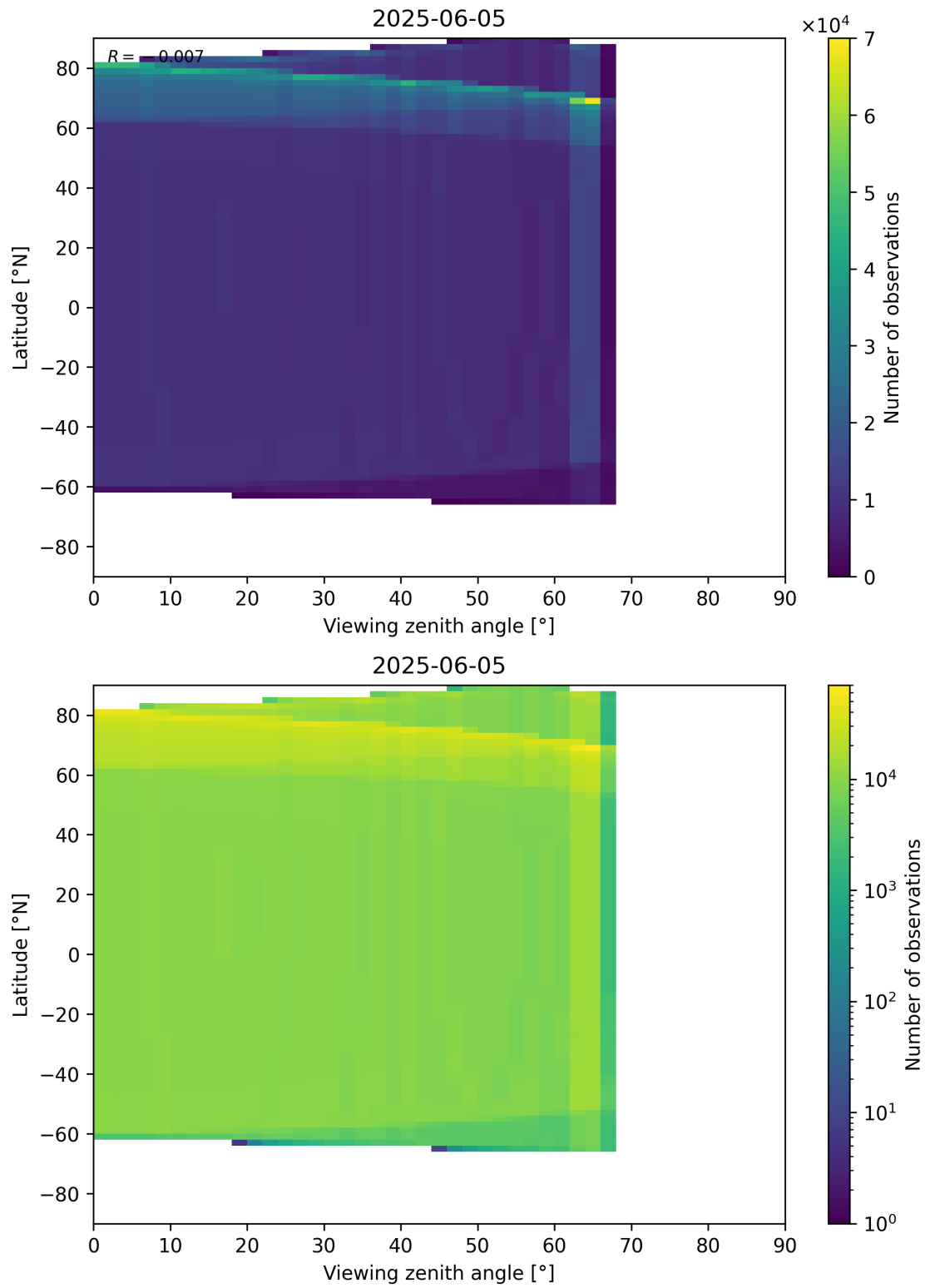
Figure 49: Scatter density plot of “Viewing zenith angle” against “Latitude” for 2025-06-04 to 2025-06-06.
