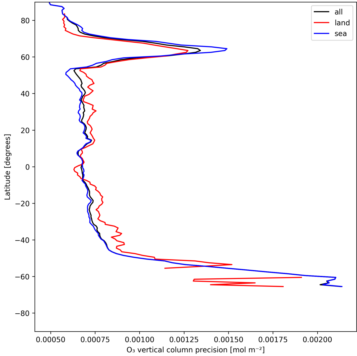
Figure 15: Zonal average of “O 3 vertical column precision” for 2025-06-04 to 2025-06-06.
