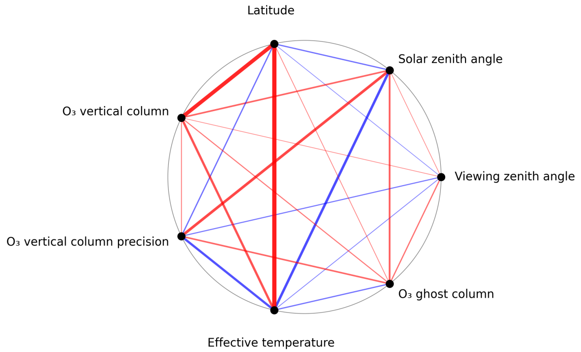
Figure 1: Map of correlation graph for 2025-06-04 to 2025-06-06.
