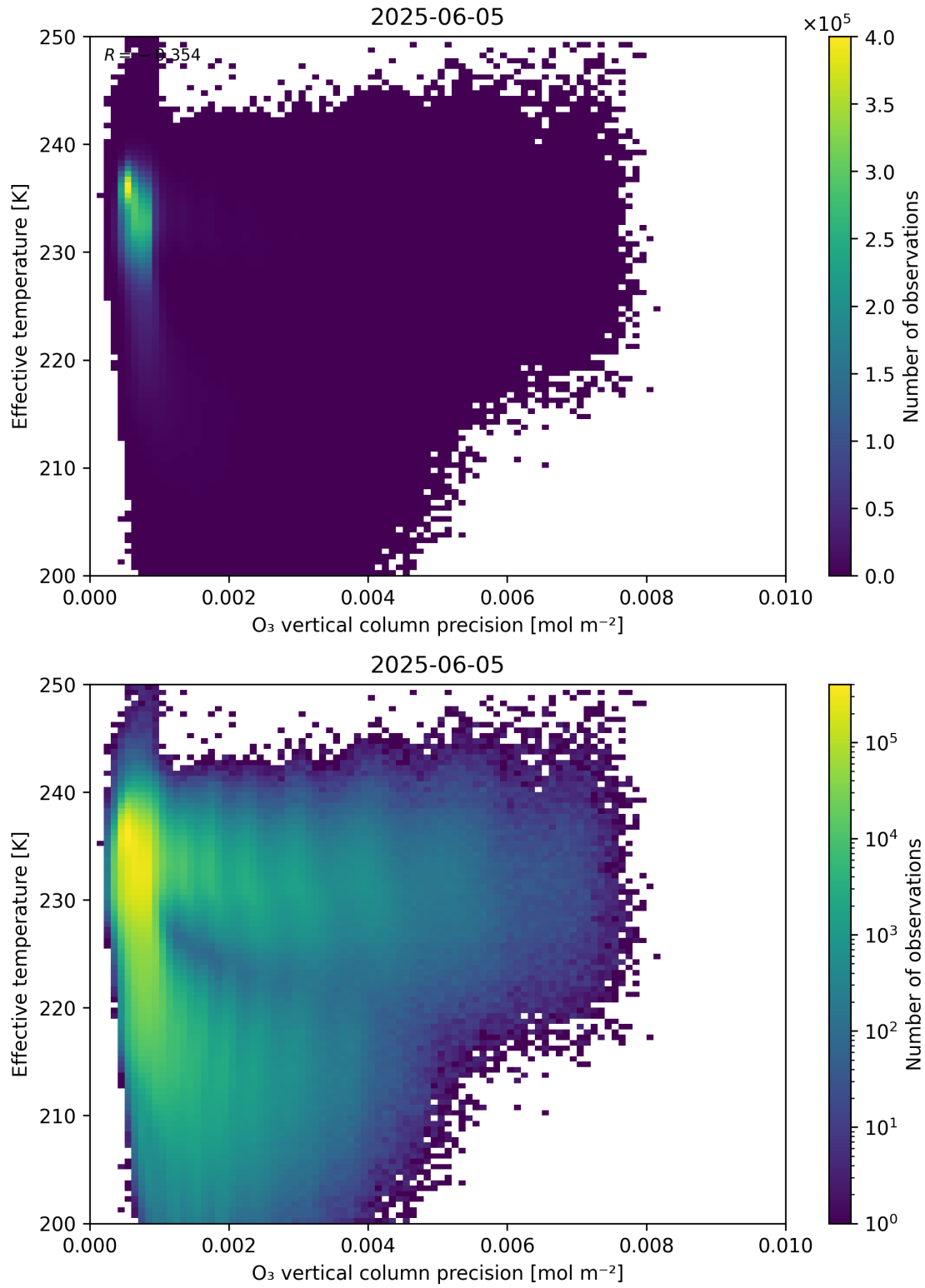
Figure 42: Scatter density plot of “O 3 vertical column precision” against “Effective temperature” for 2025-06-04 to 2025-06-06.
