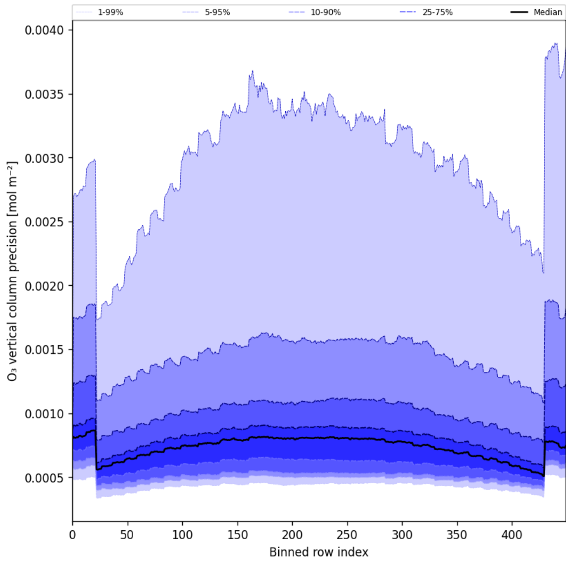
Figure 29: Along track statistics of “O 3 vertical column precision” for 2025-06-07 to 2025-06-09
