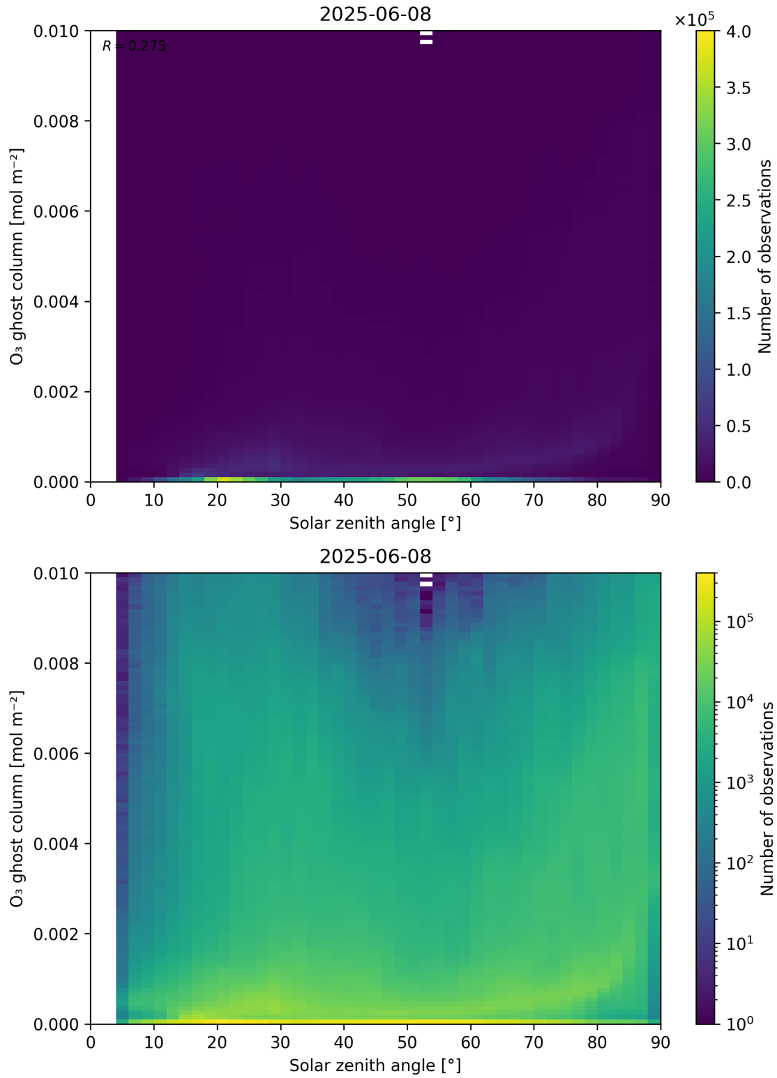
Figure 46: Scatter density plot of “Solar zenith angle” against “O 3 ghost column” for 2025-06-07 to 2025-06-09.
