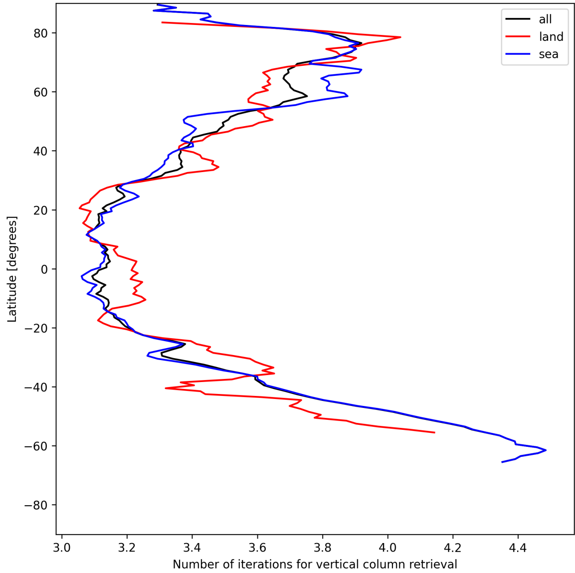
Figure 19: Zonal average of “Number of iterations for vertical column retrieval” for 2025-06-07 to 2025-06-09.
