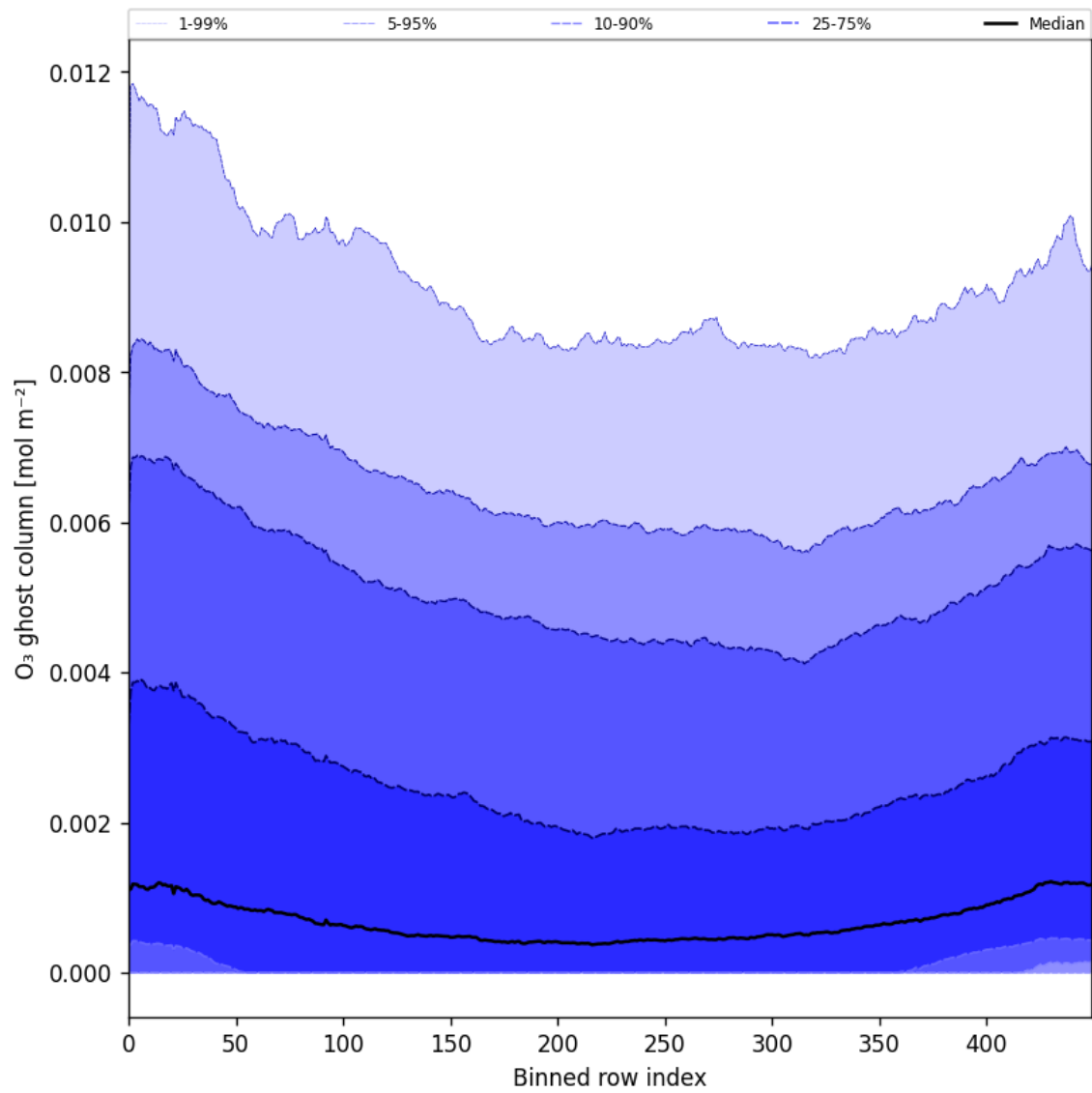
Figure 32: Along track statistics of “O 3 ghost column” for 2025-06-07 to 2025-06-09
