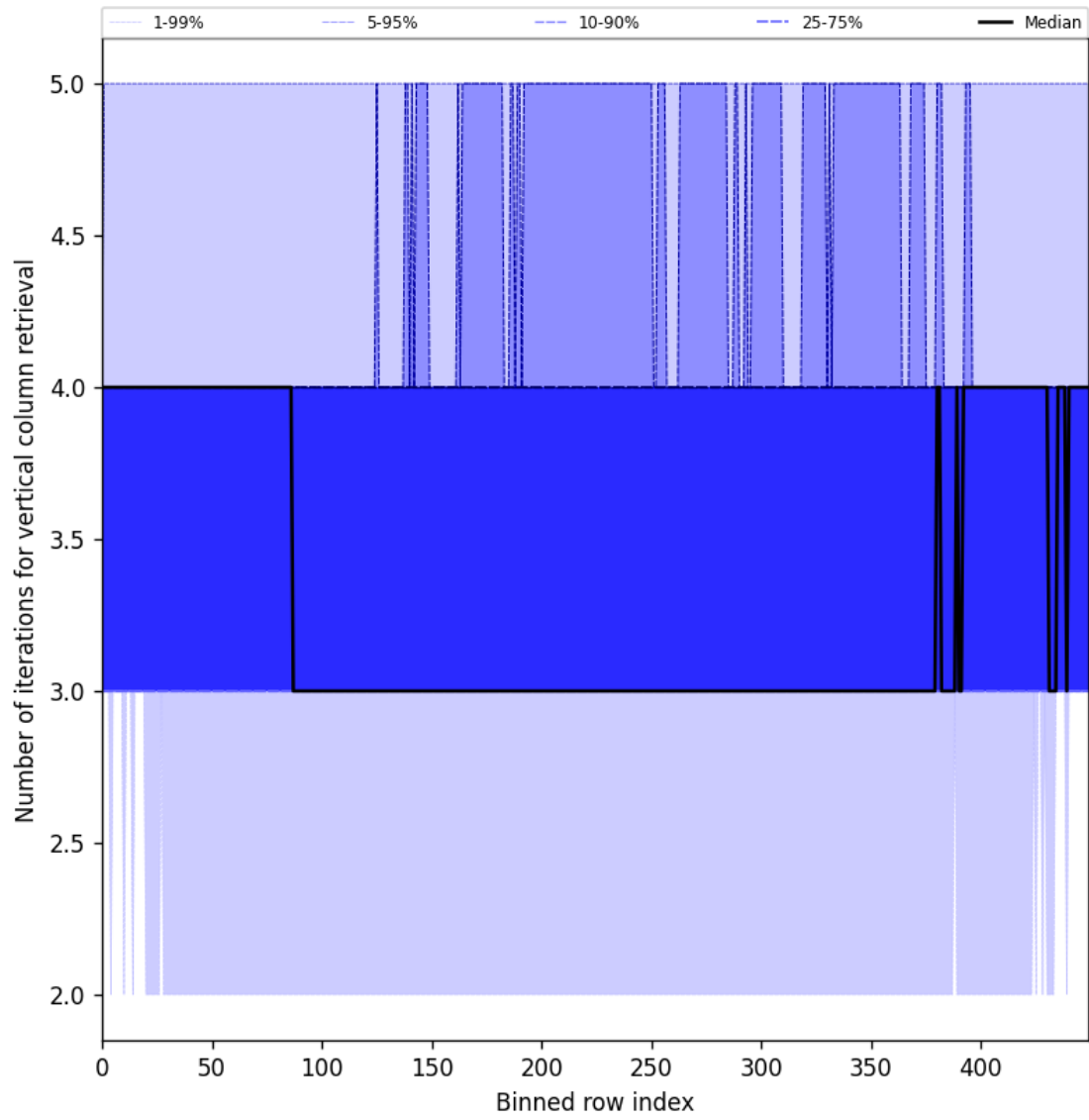
Figure 33: Along track statistics of “Number of iterations for vertical column retrieval” for 2025-06-07 to 2025-06-09
