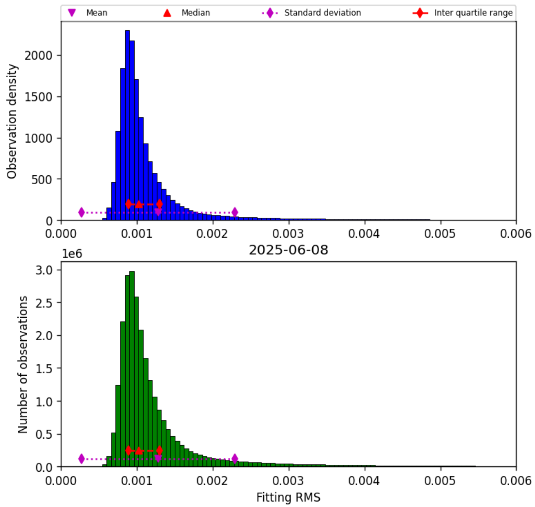
Figure 23: Histogram of “Fitting RMS” for 2025-06-07 to 2025-06-09
