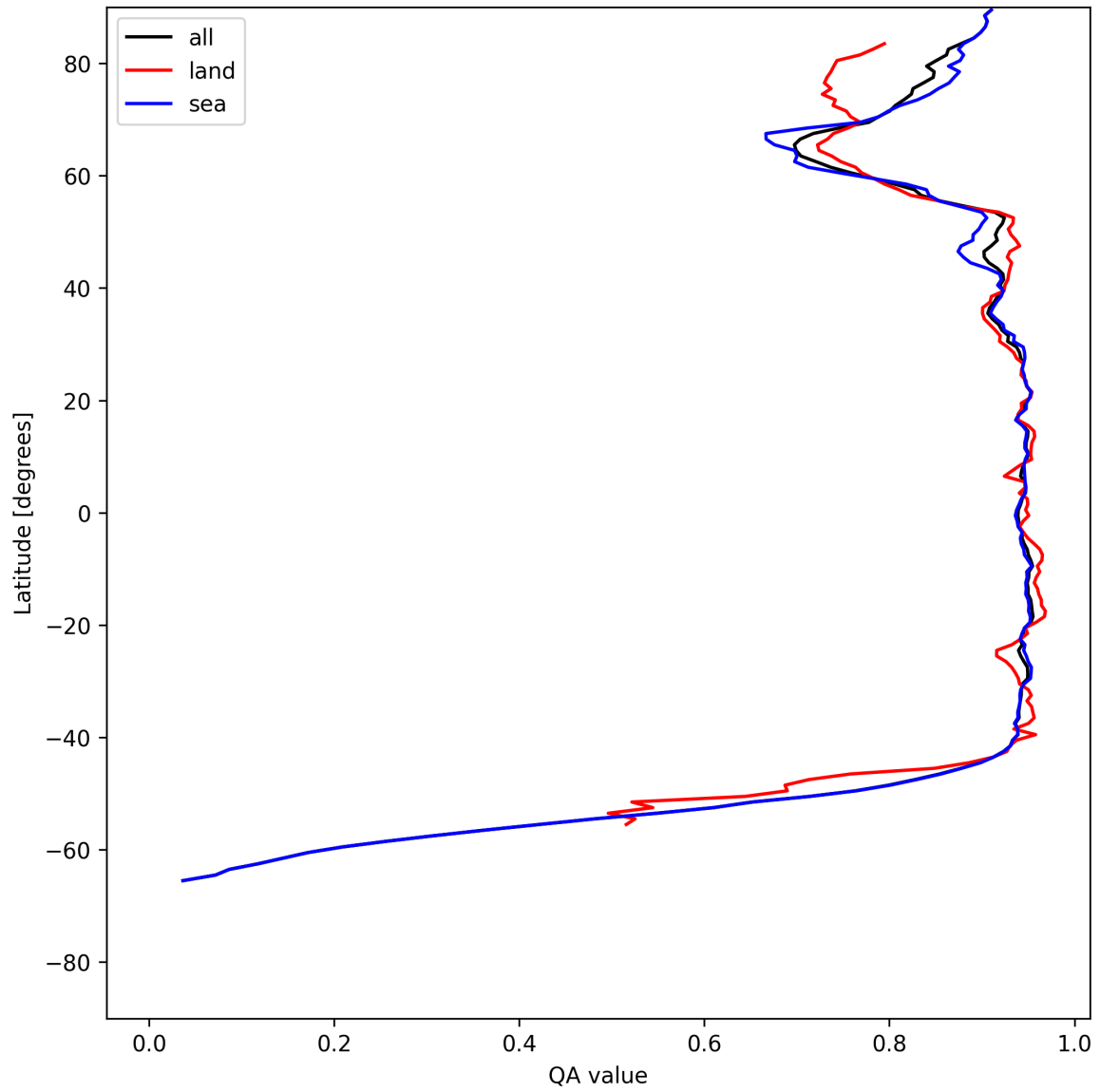
Figure 13: Zonal average of “QA value” for 2025-06-07 to 2025-06-09.
