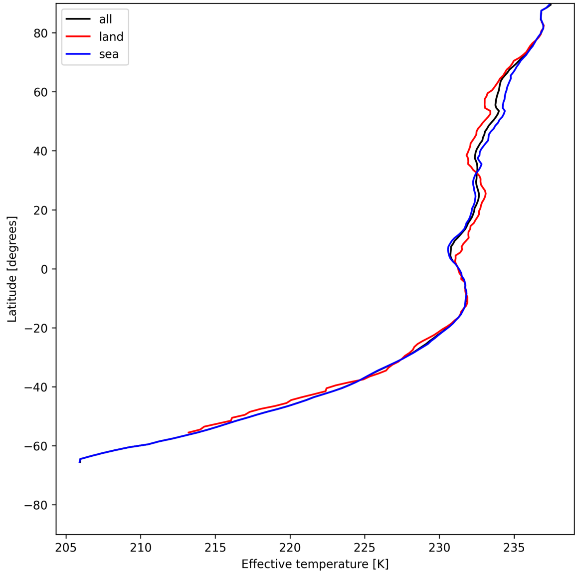
Figure 17: Zonal average of "Effective temperature" for 2025-06-07 to 2025-06-09.
