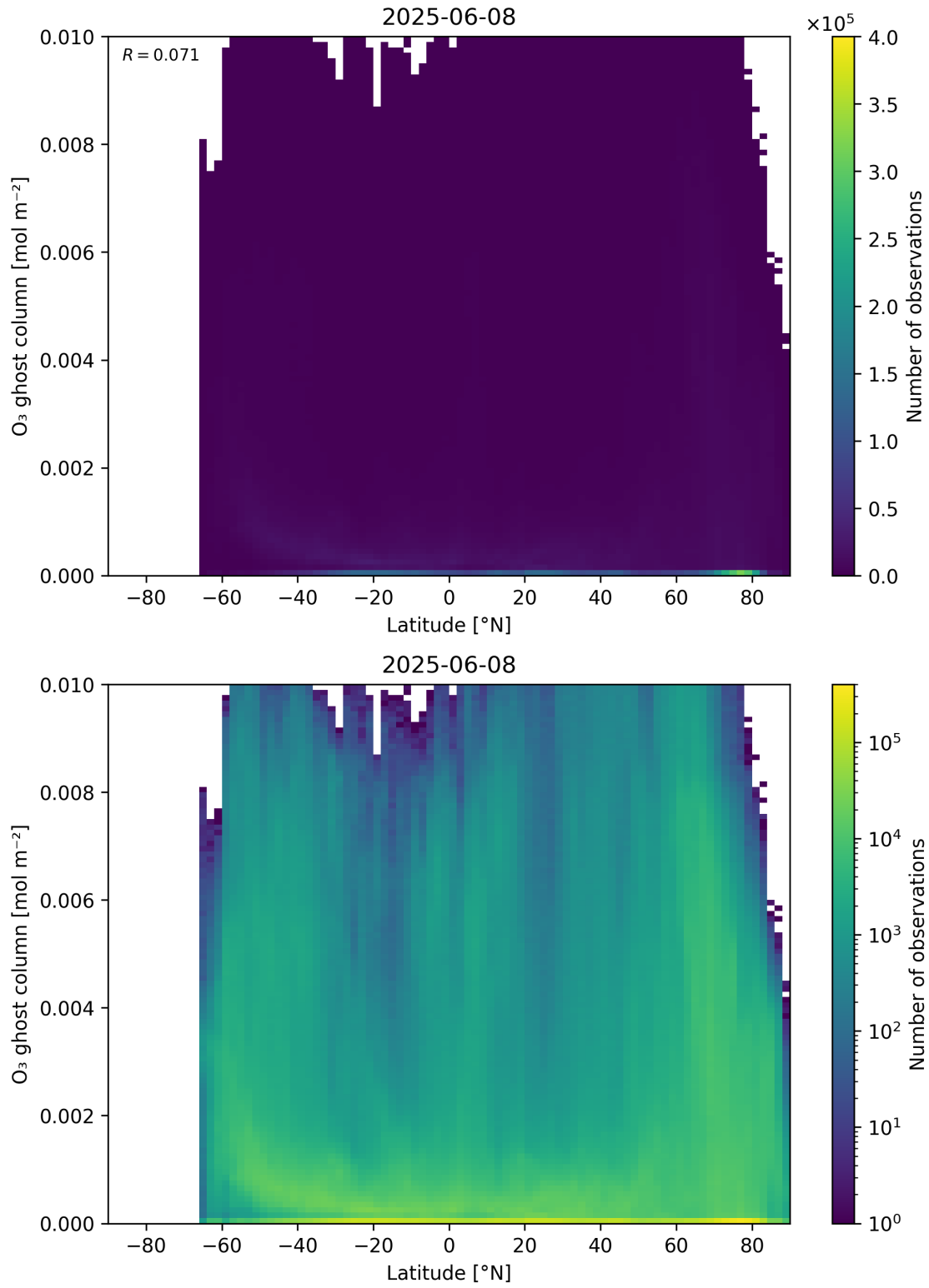
Figure 35: Scatter density plot of “Latitude” against “O 3 ghost column” for 2025-06-07 to 2025-06-09.
