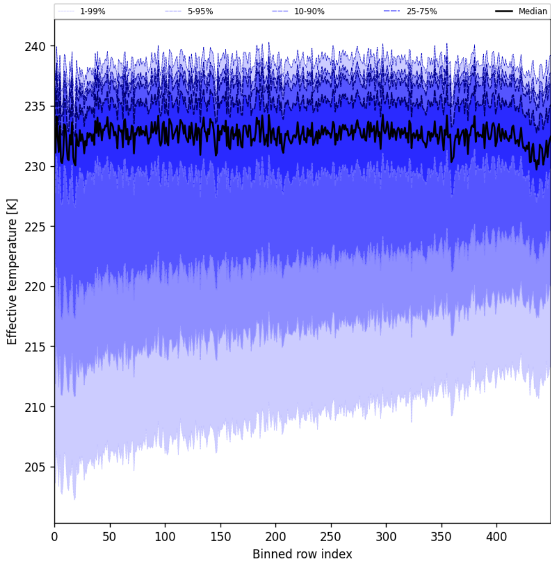
Figure 31: Along track statistics of “Effective temperature” for 2025-06-07 to 2025-06-09
