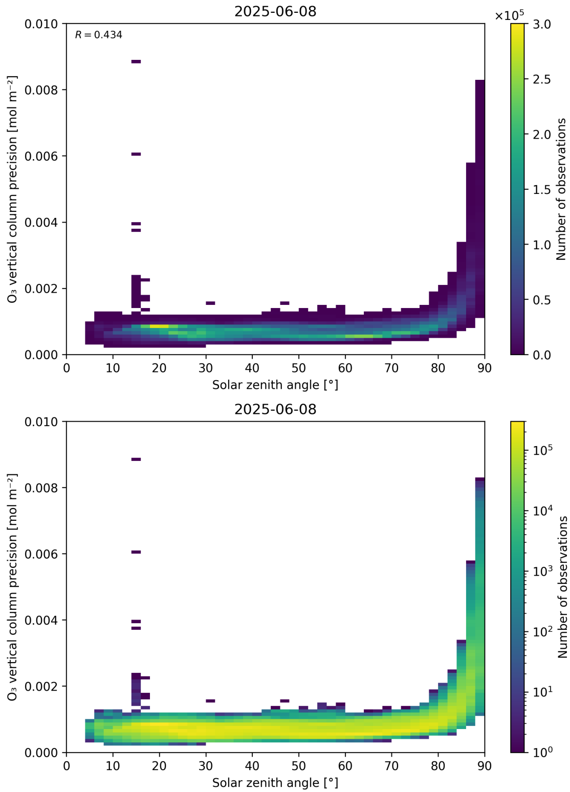
Figure 48: Scatter density plot of “Solar zenith angle” against “O 3 vertical column precision” for 2025-06-07 to 2025-06-09.
