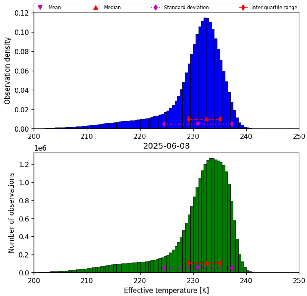
Figure 24: Histogram of “Effective temperature” for 2025-06-07 to 2025-06-09
