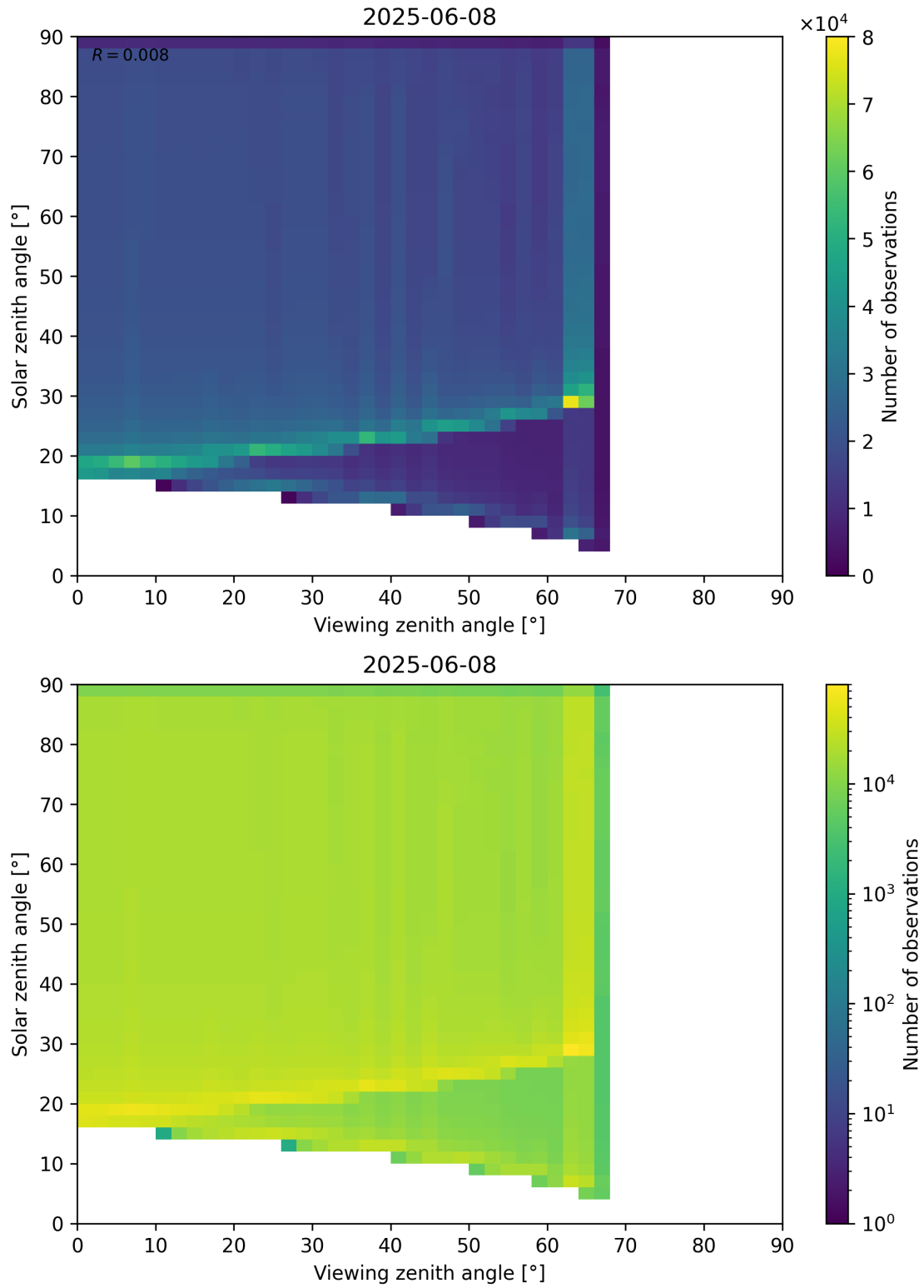
Figure 54: Scatter density plot of “Viewing zenith angle” against “Solar zenith angle” for 2025-06-07 to 2025-06-09.
