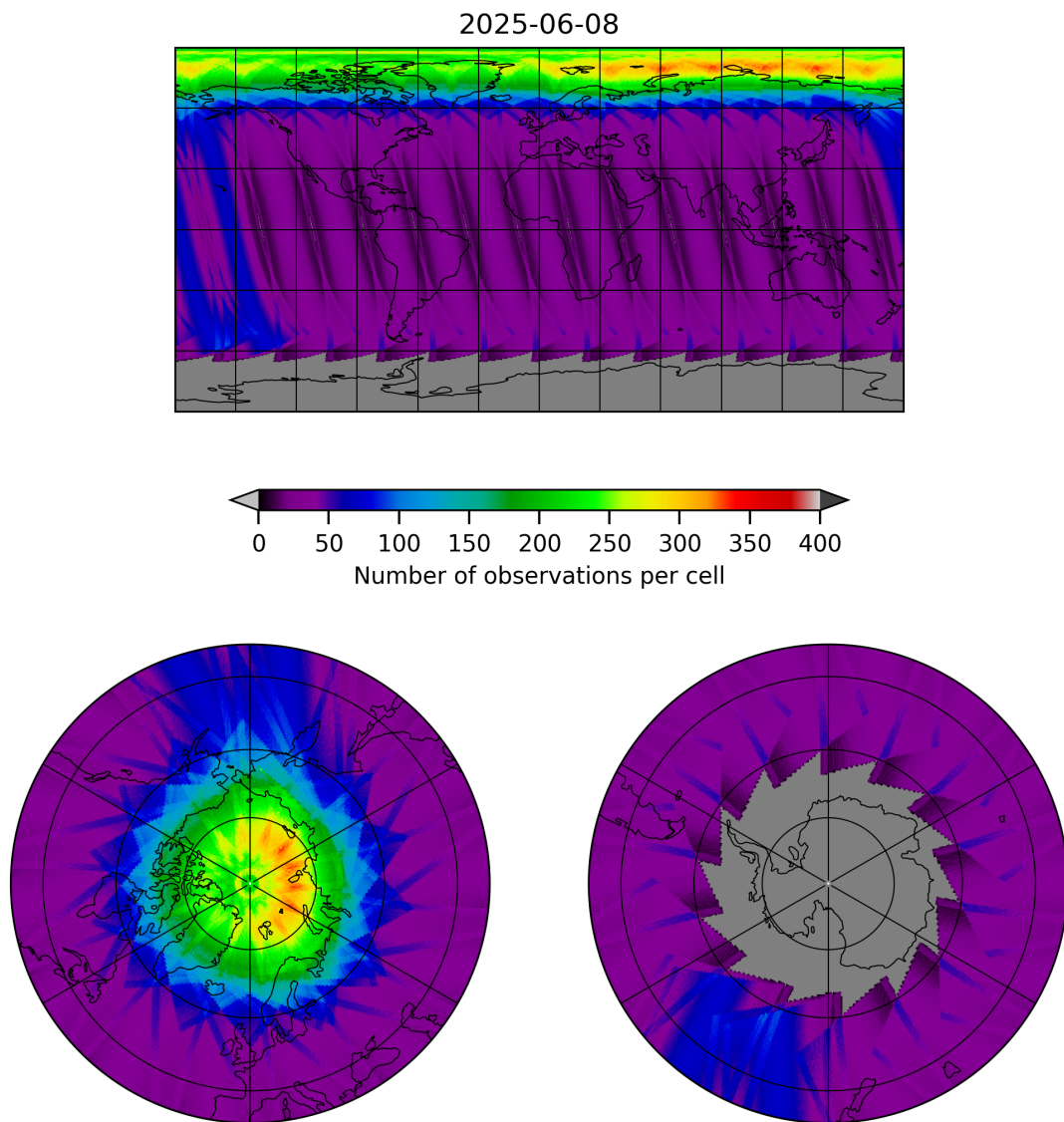
Figure 12: Map of the number of observations for 2025-06-07 to 2025-06-09
