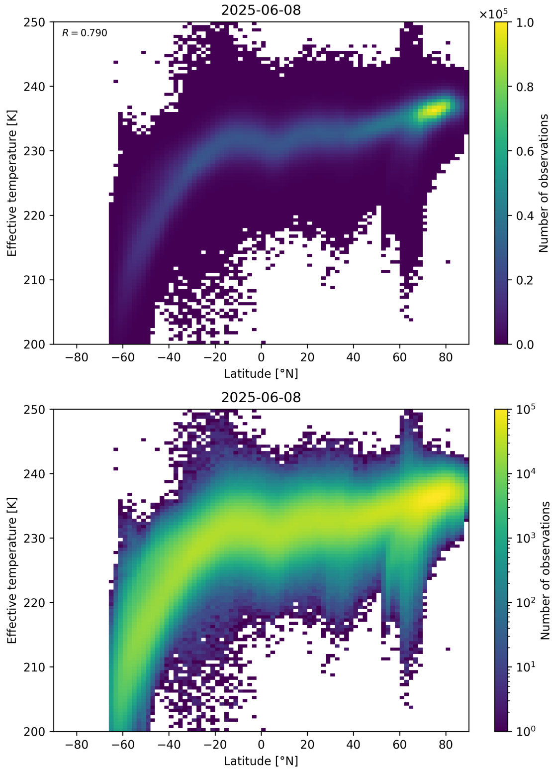
Figure 34: Scatter density plot of “Latitude” against “Effective temperature” for 2025-06-07 to 2025-06-09.
