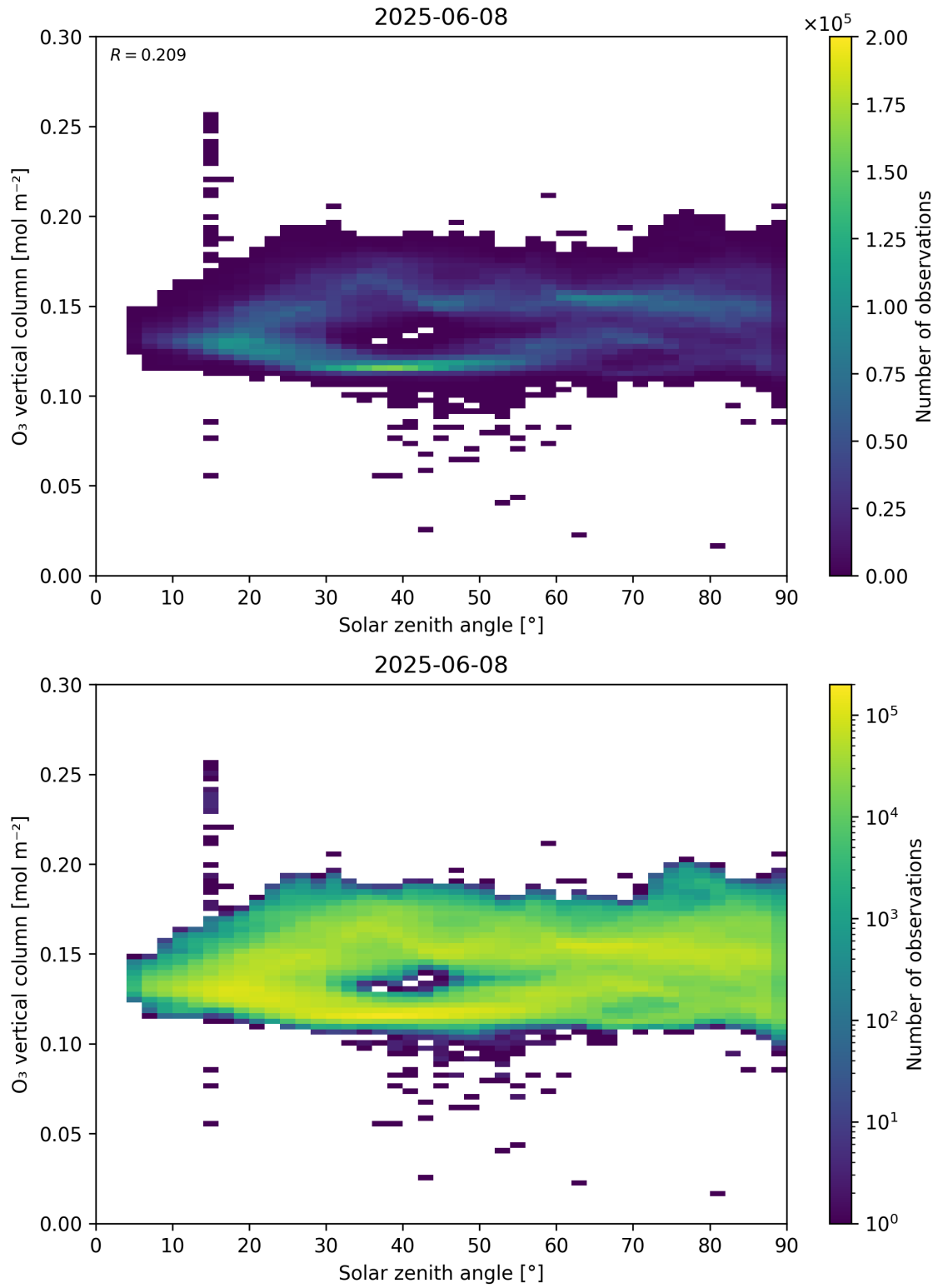
Figure 47: Scatter density plot of “Solar zenith angle” against “O 3 vertical column” for 2025-06-07 to 2025-06-09.
