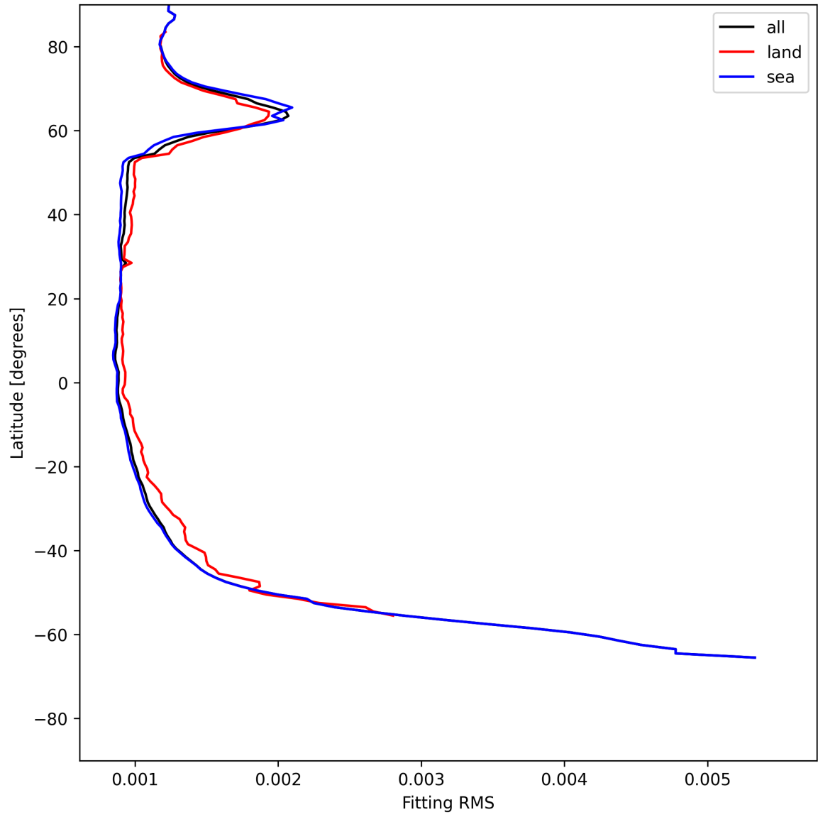
Figure 16: Zonal average of “Fitting RMS” for 2025-06-07 to 2025-06-09.
