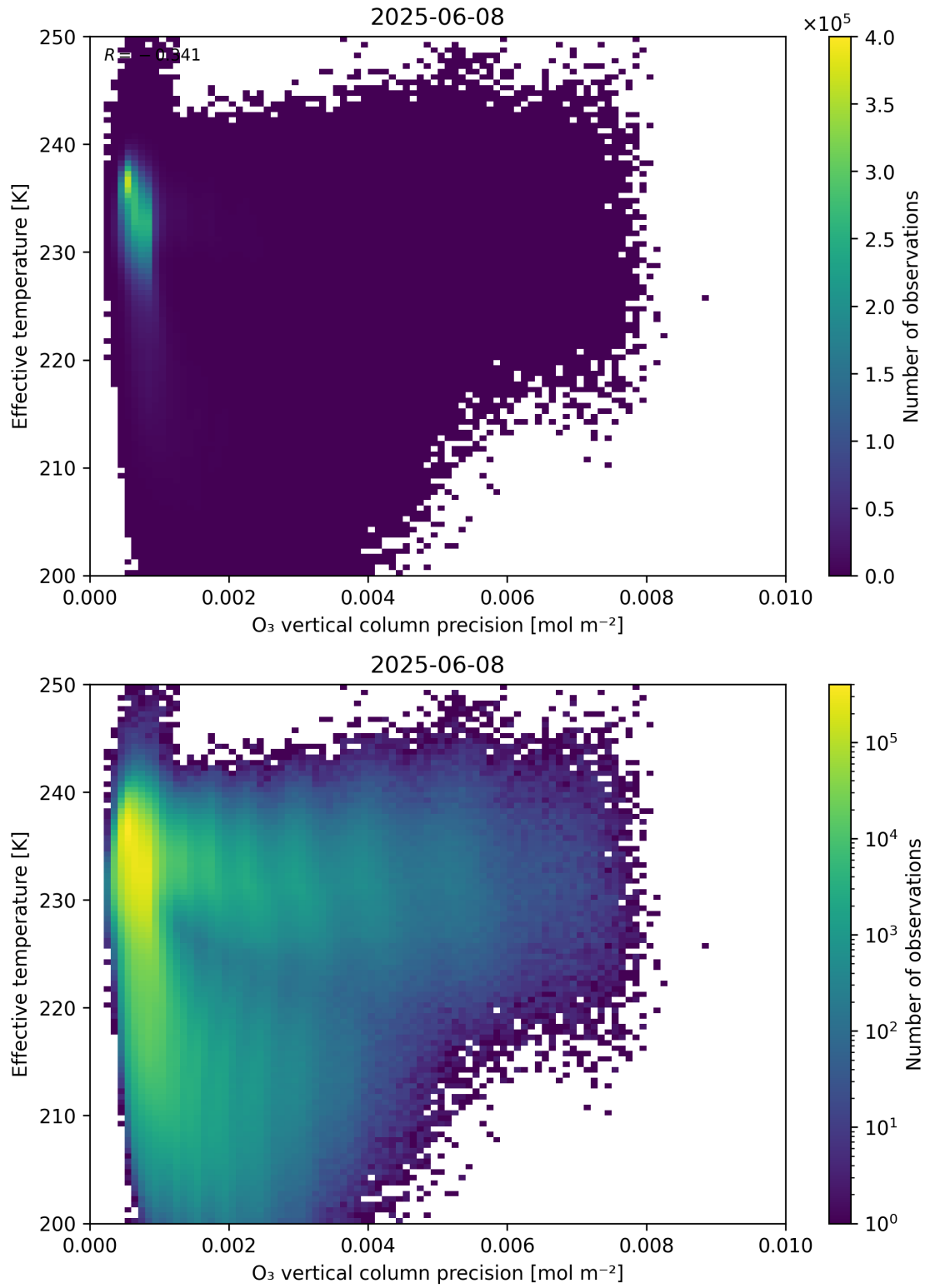
Figure 42: Scatter density plot of “O 3 vertical column precision” against “Effective temperature” for 2025-06-07 to 2025-06-09.
