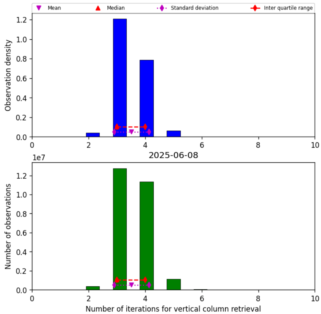
Figure 26: Histogram of “Number of iterations for vertical column retrieval” for 2025-06-07 to 2025-06-09
