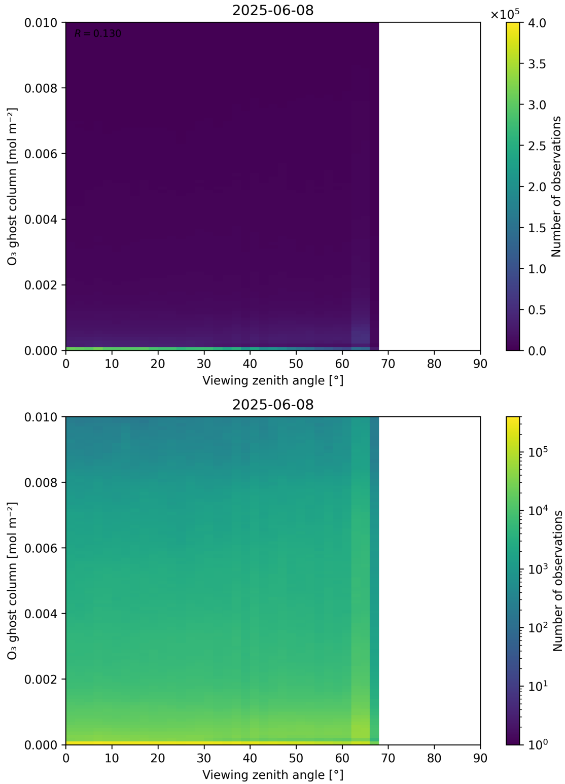
Figure 51: Scatter density plot of “Viewing zenith angle” against “O 3 ghost column” for 2025-06-07 to 2025-06-09.
