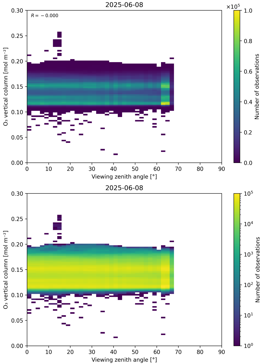
Figure 52: Scatter density plot of “Viewing zenith angle” against “O 3 vertical column” for 2025-06-07 to 2025-06-09.
