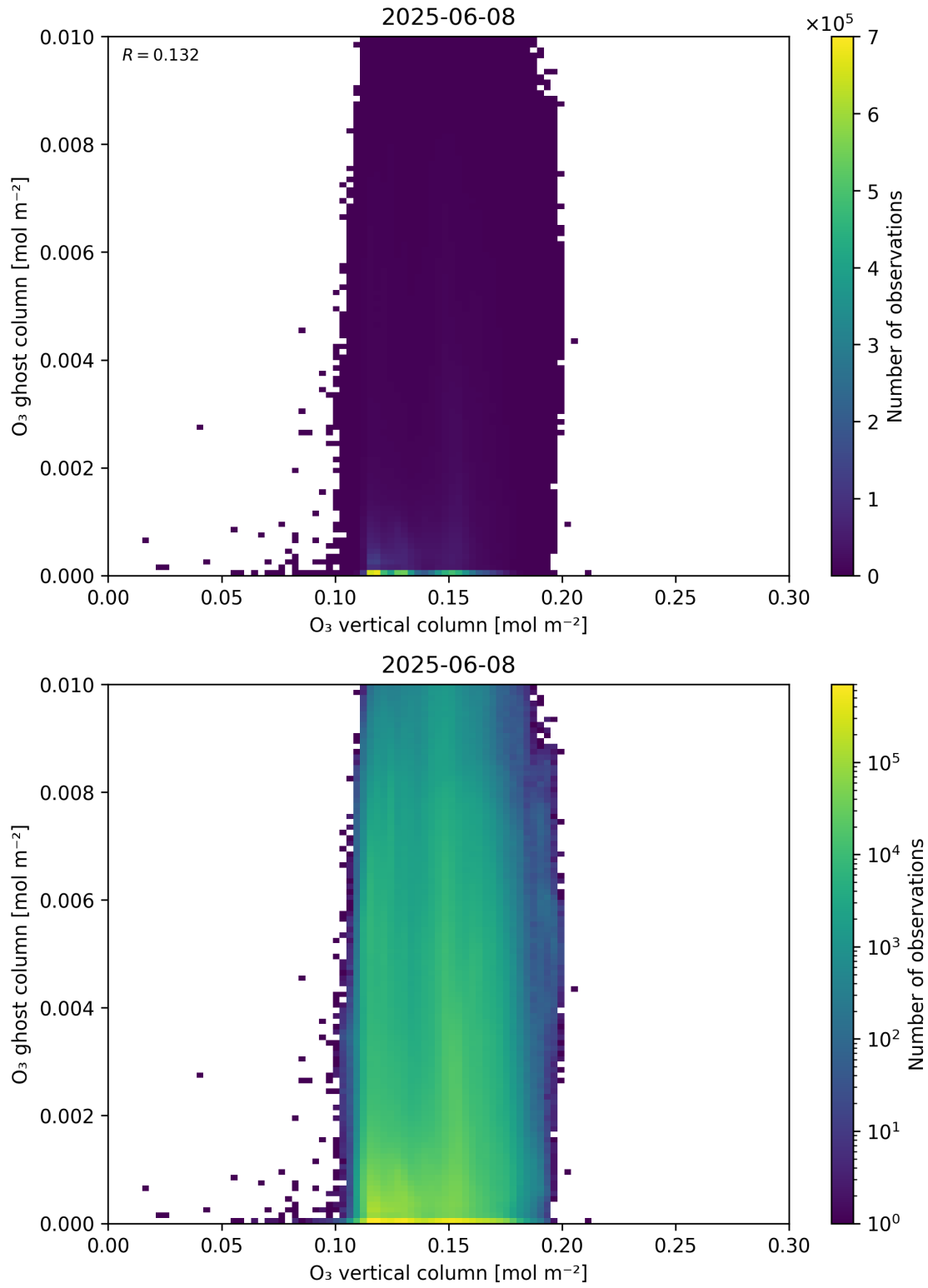
Figure 40: Scatter density plot of “O 3 vertical column” against “O 3 ghost column” for 2025-06-07 to 2025-06-09.
