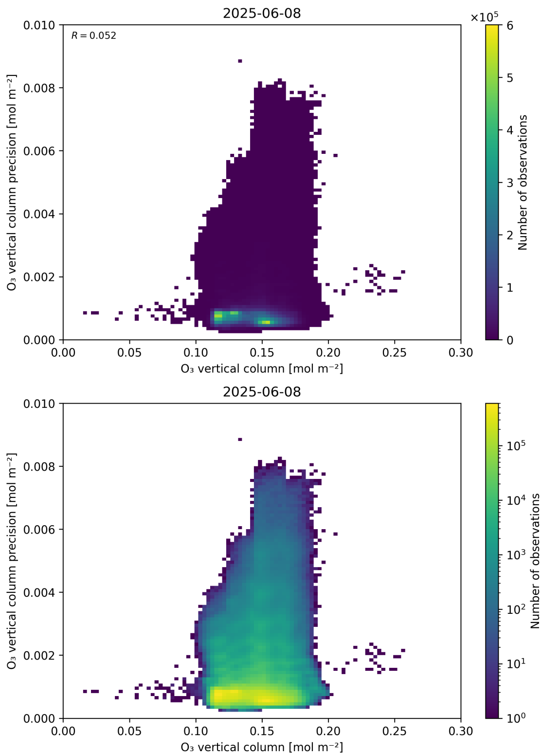
Figure 41: Scatter density plot of “O 3 vertical column” against “O 3 vertical column precision” for 2025-06-07 to 2025-06-09.
