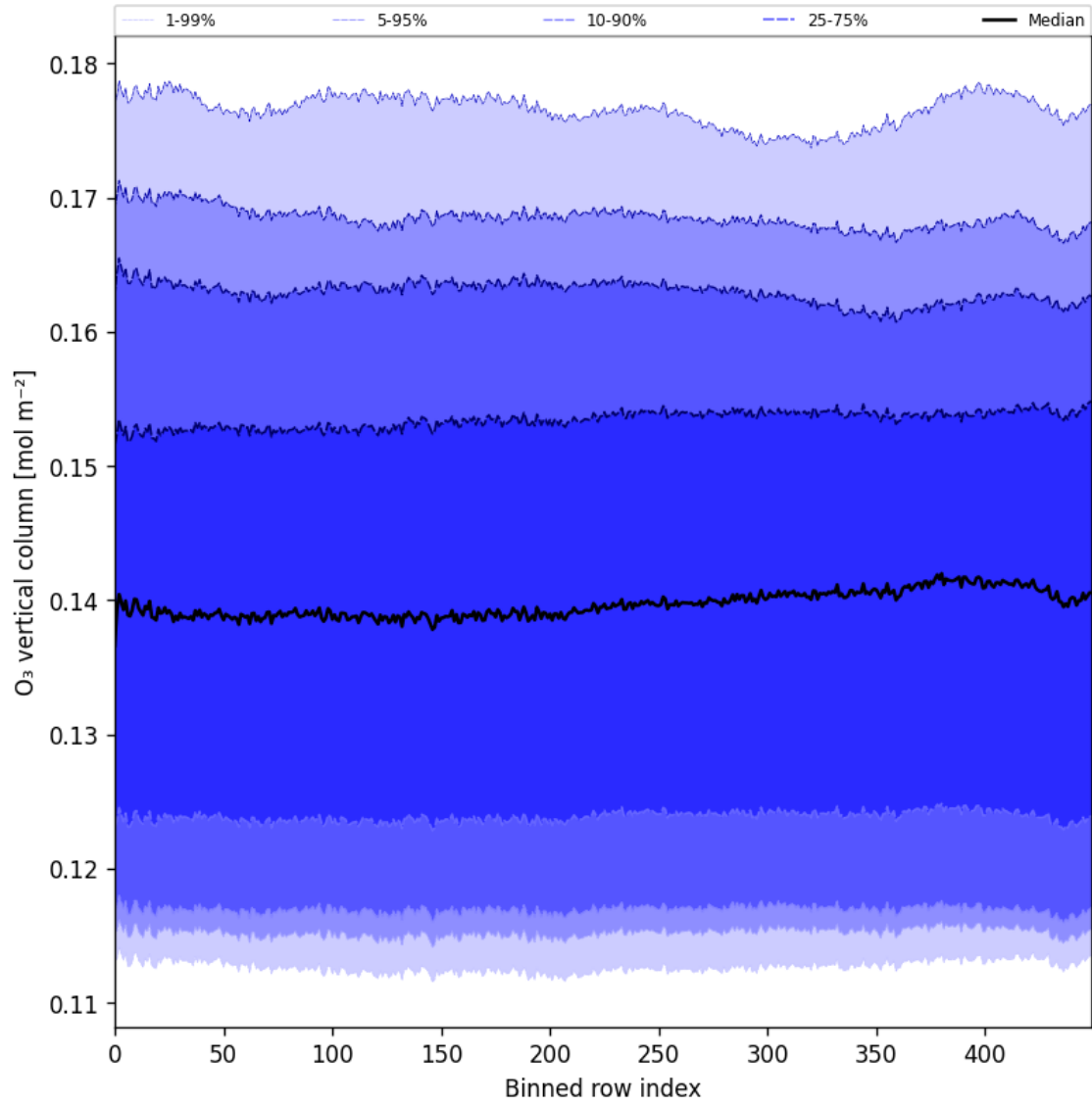
Figure 28: Along track statistics of “O 3 vertical column” for 2025-06-07 to 2025-06-09
