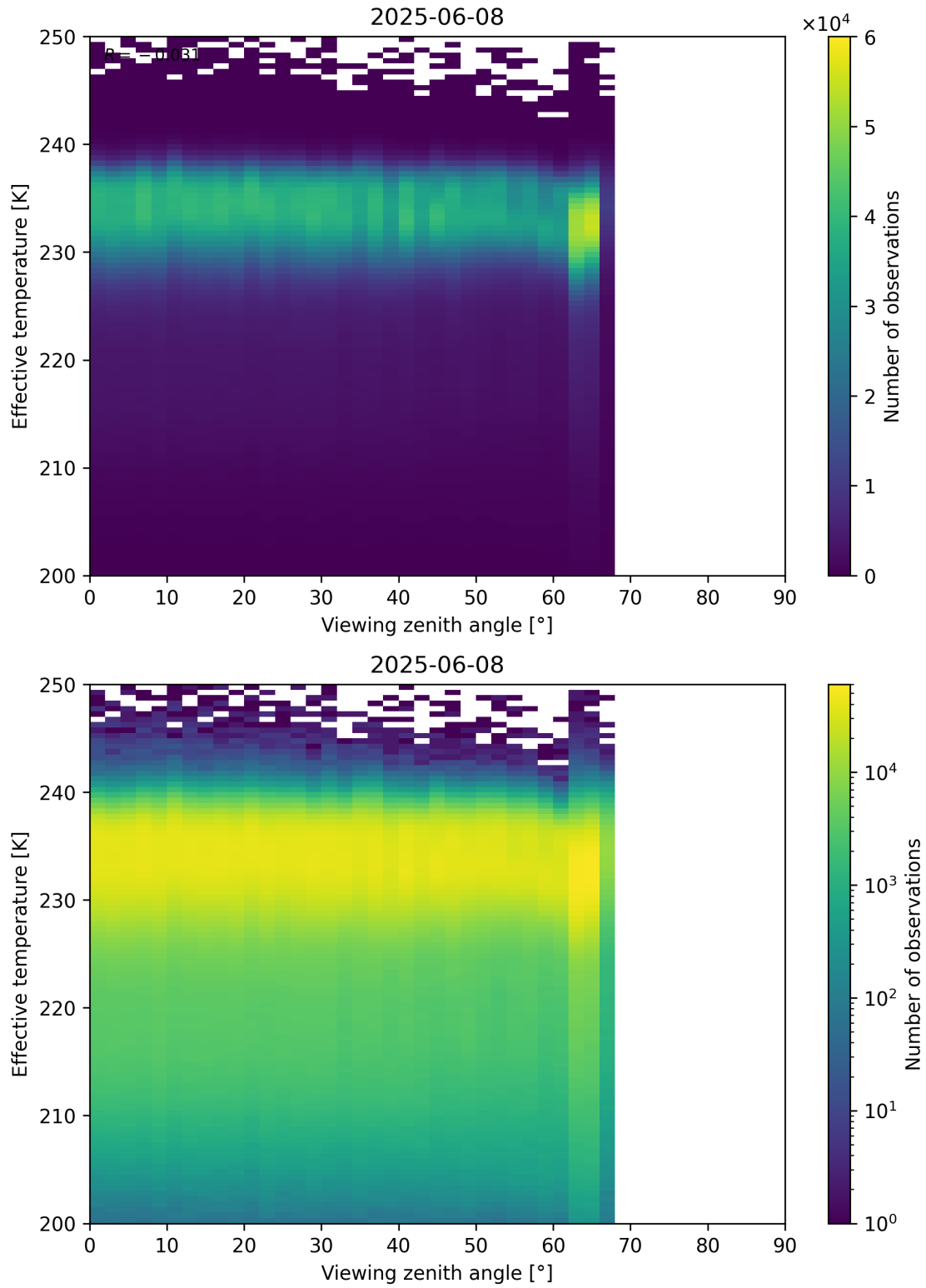
Figure 50: Scatter density plot of “Viewing zenith angle” against “Effective temperature” for 2025-06-07 to 2025-06-09.
