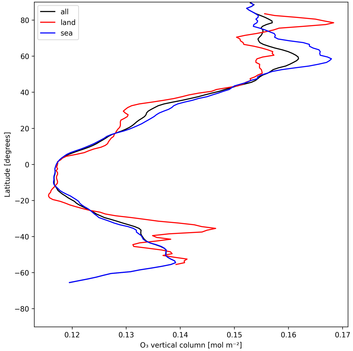
Figure 14: Zonal average of “O 3 vertical column” for 2025-06-07 to 2025-06-09.
