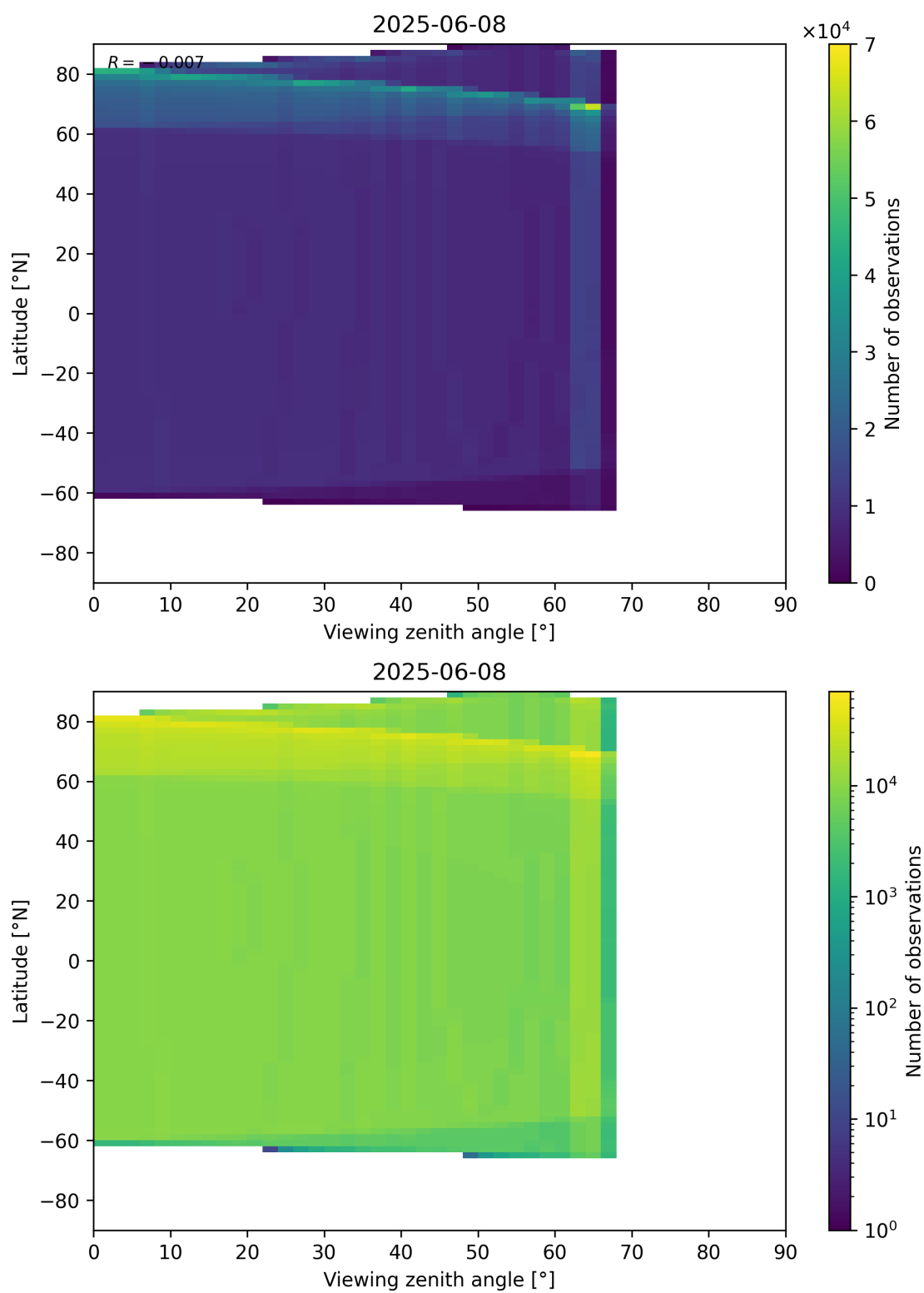
Figure 49: Scatter density plot of “Viewing zenith angle” against “Latitude” for 2025-06-07 to 2025-06-09.
