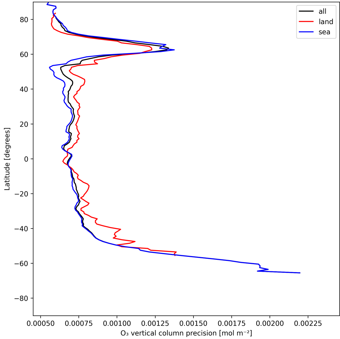
Figure 15: Zonal average of “O 3 vertical column precision” for 2025-06-07 to 2025-06-09.
