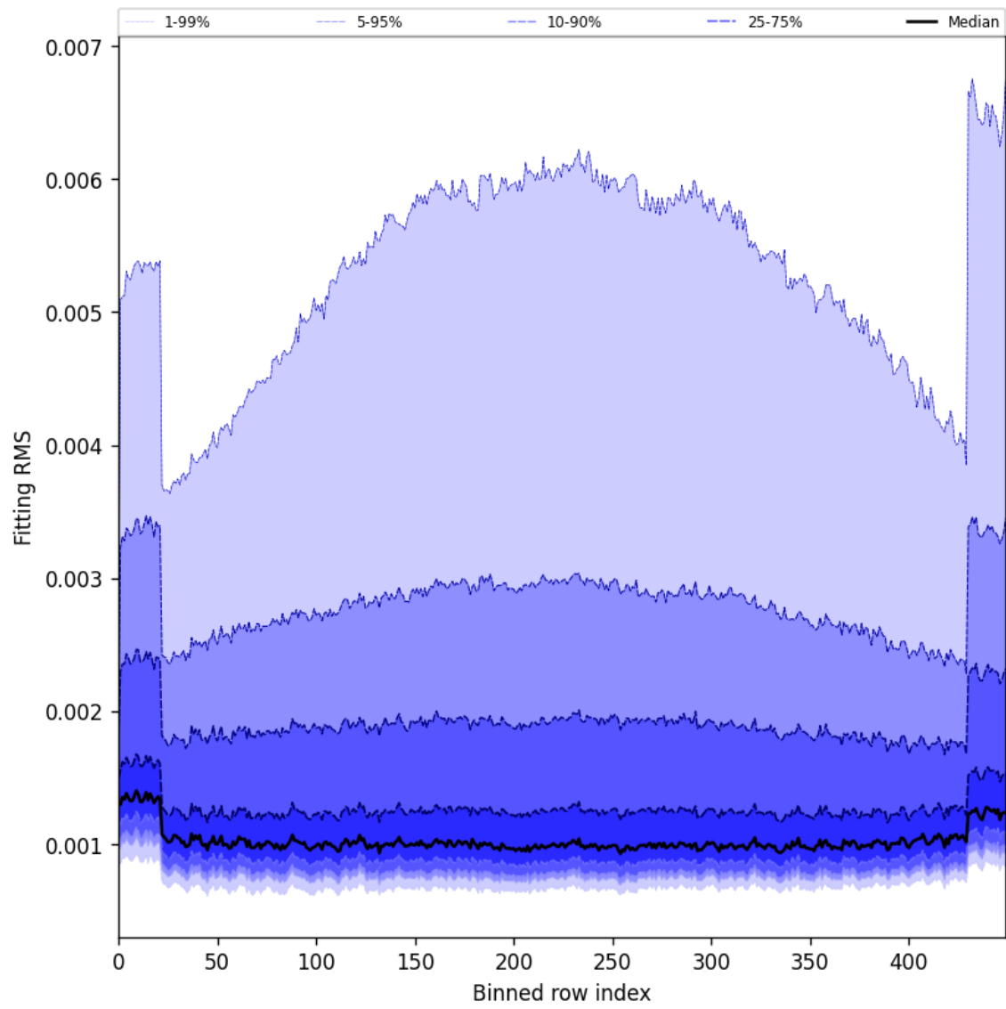
Figure 30: Along track statistics of “Fitting RMS” for 2025-06-07 to 2025-06-09
