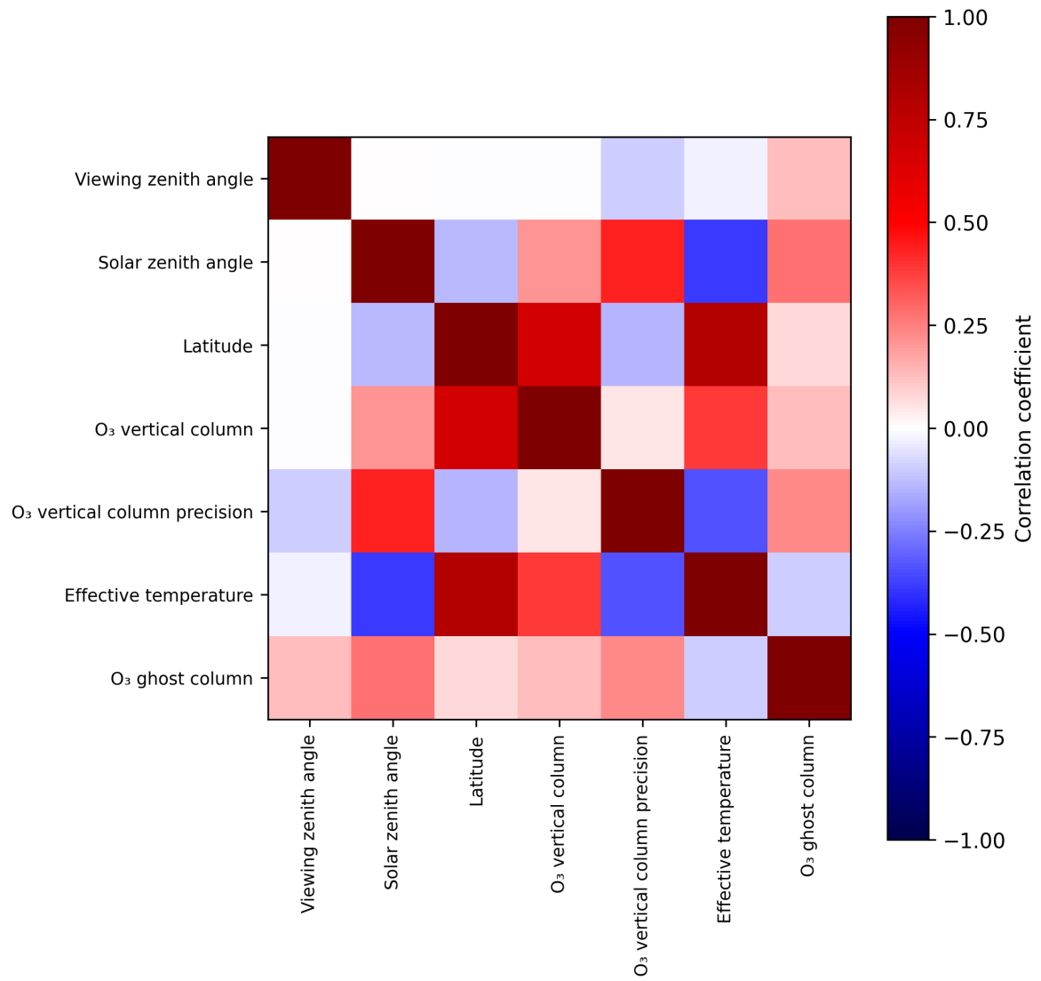
Figure 2: Map of correlation matrix for 2025-06-07 to 2025-06-09.
