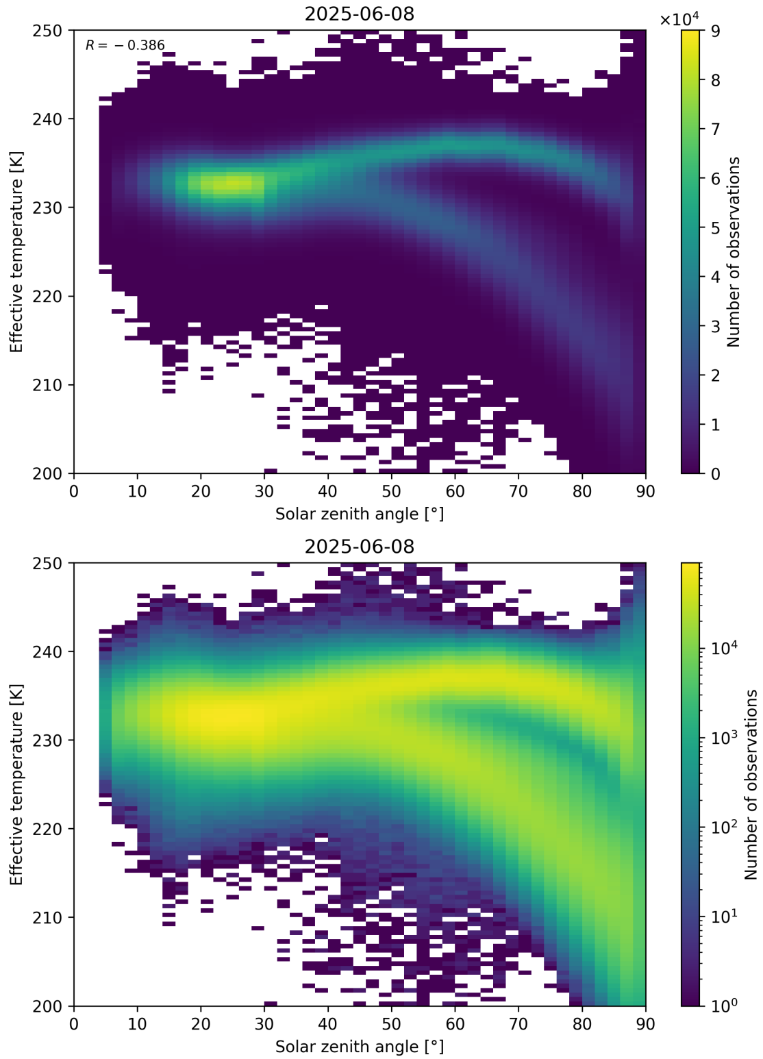
Figure 45: Scatter density plot of “Solar zenith angle” against “Effective temperature” for 2025-06-07 to 2025-06-09.
