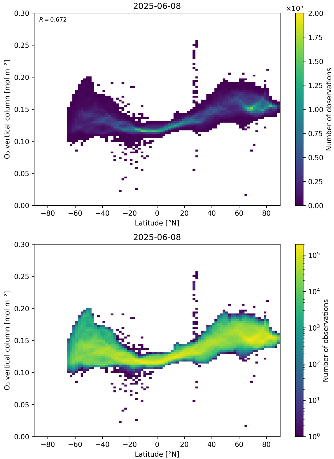
Figure 36: Scatter density plot of “Latitude” against “O 3 vertical column” for 2025-06-07 to 2025-06-09.
