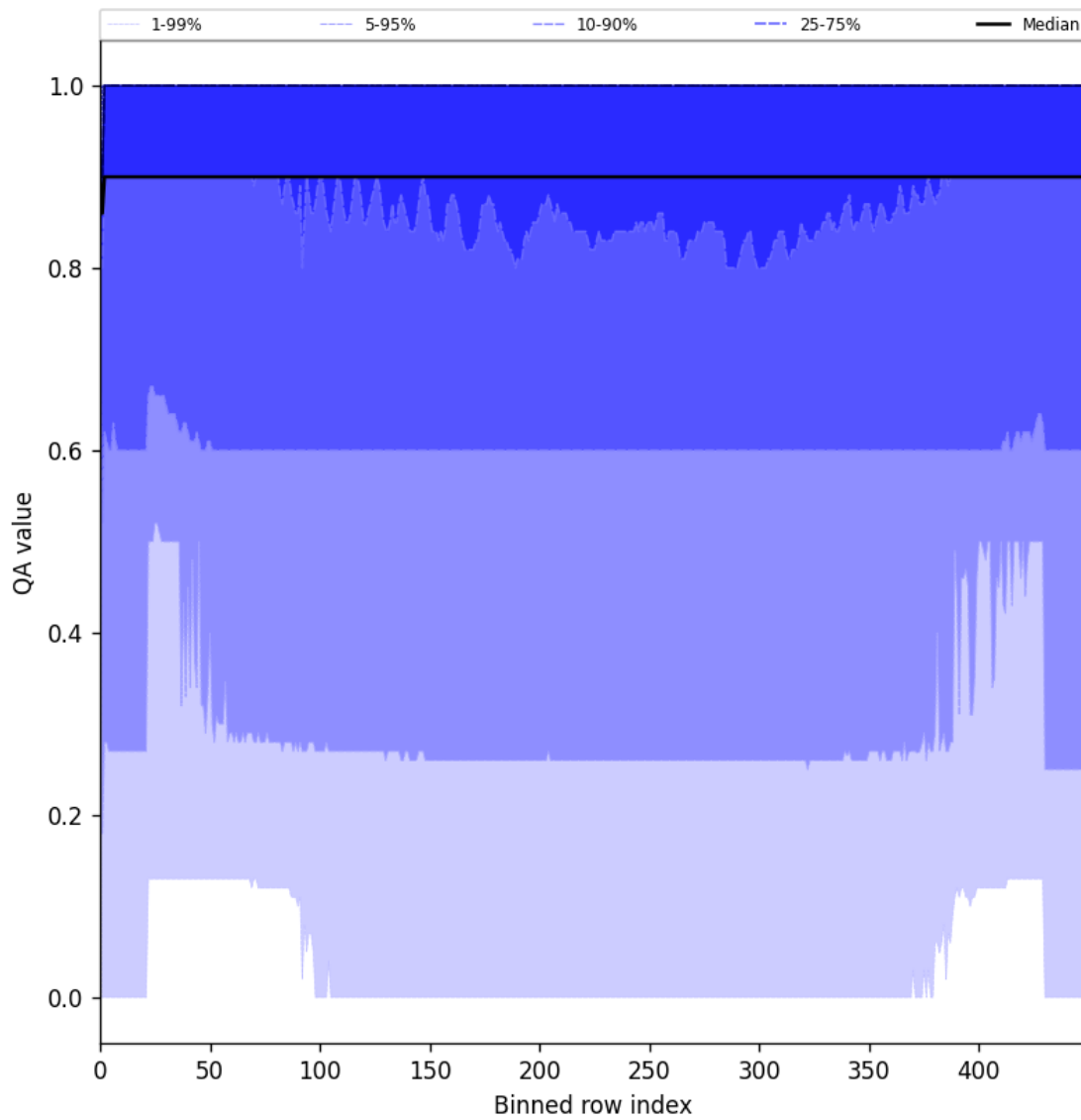
Figure 27: Along track statistics of “QA value” for 2025-06-07 to 2025-06-09
