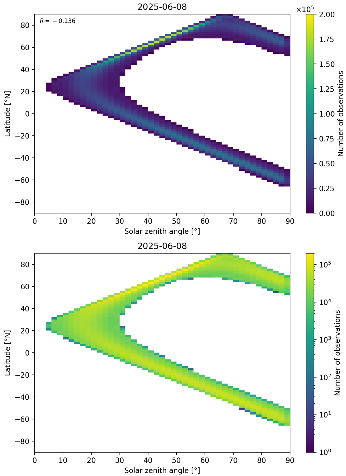
Figure 44: Scatter density plot of “Solar zenith angle” against “Latitude” for 2025-06-07 to 2025-06-09.
