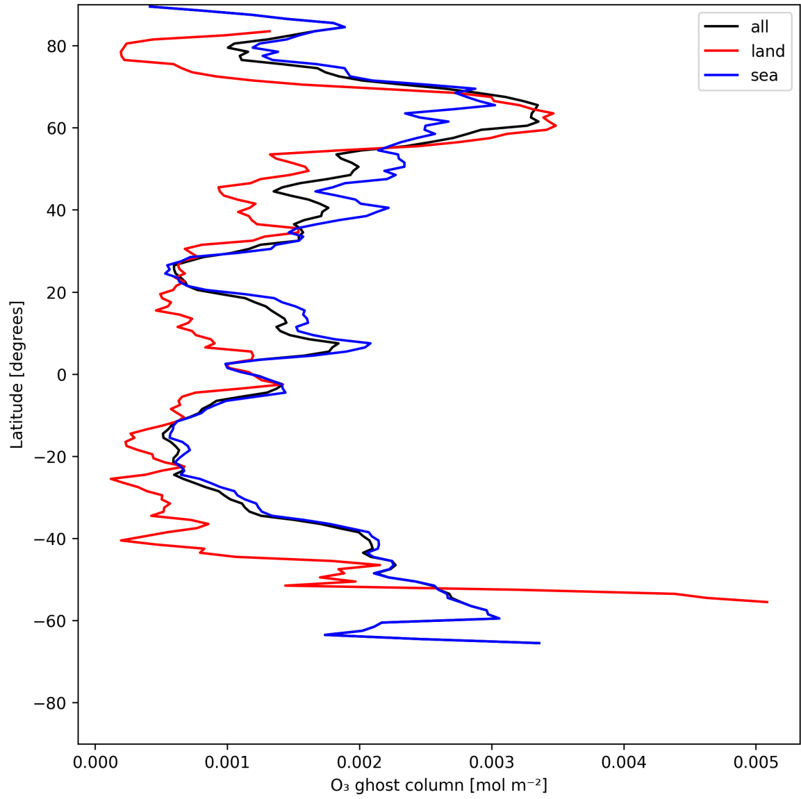
Figure 18: Zonal average of “O 3 ghost column” for 2025-06-07 to 2025-06-09.
