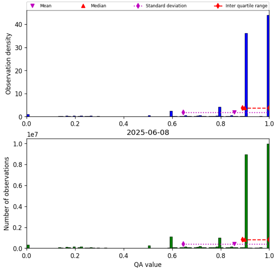
Figure 20: Histogram of “QA value” for 2025-06-07 to 2025-06-09
