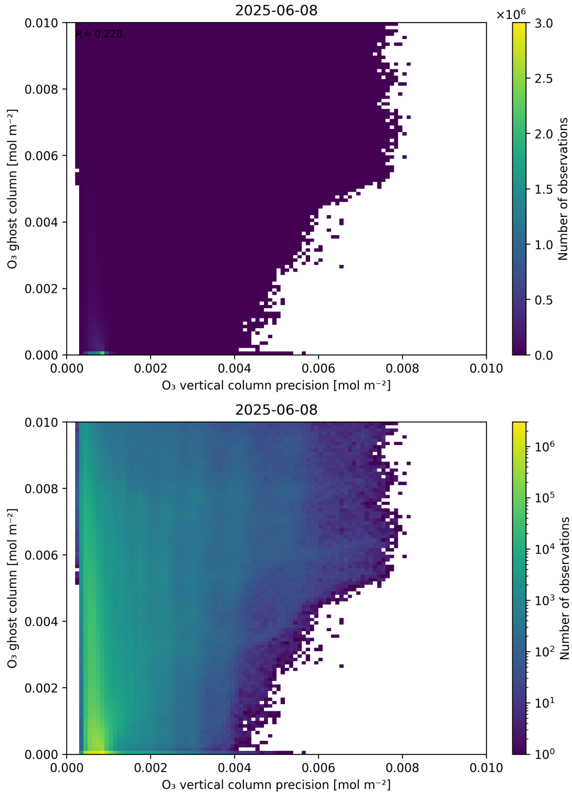
Figure 43: Scatter density plot of “O 3 vertical column precision” against “O 3 ghost column” for 2025-06-07 to 2025-06-09.
