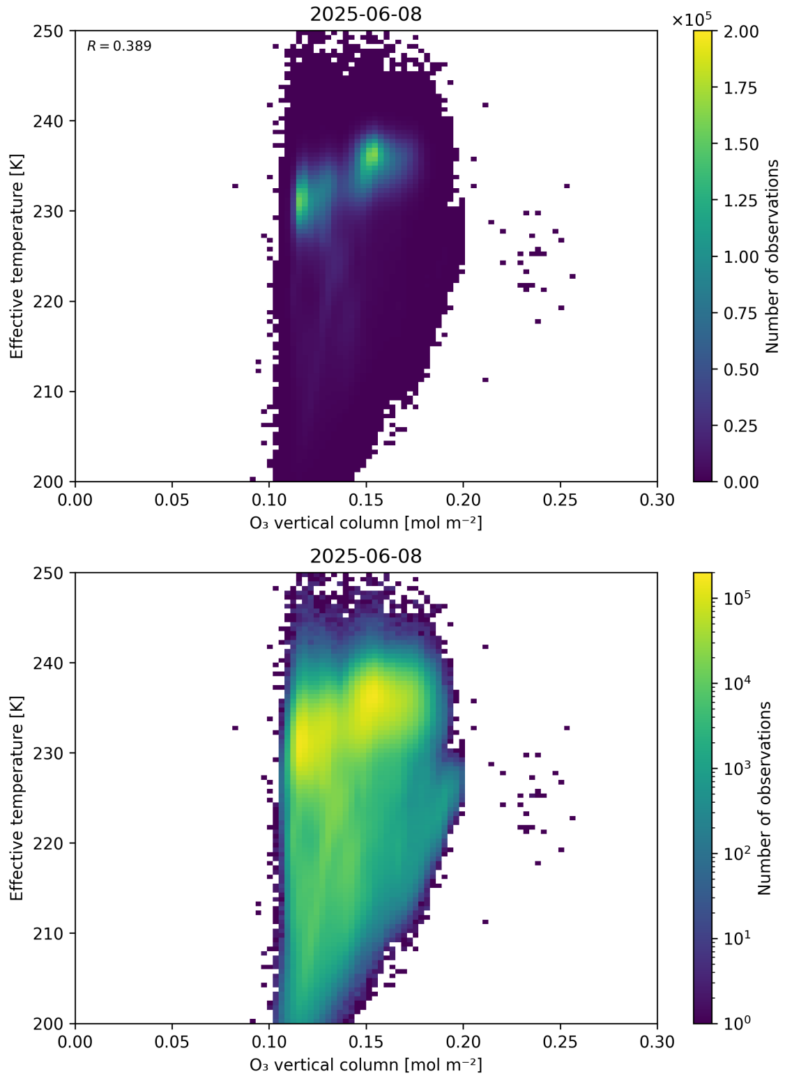
Figure 39: Scatter density plot of “O 3 vertical column” against “Effective temperature” for 2025-06-07 to 2025-06-09.
