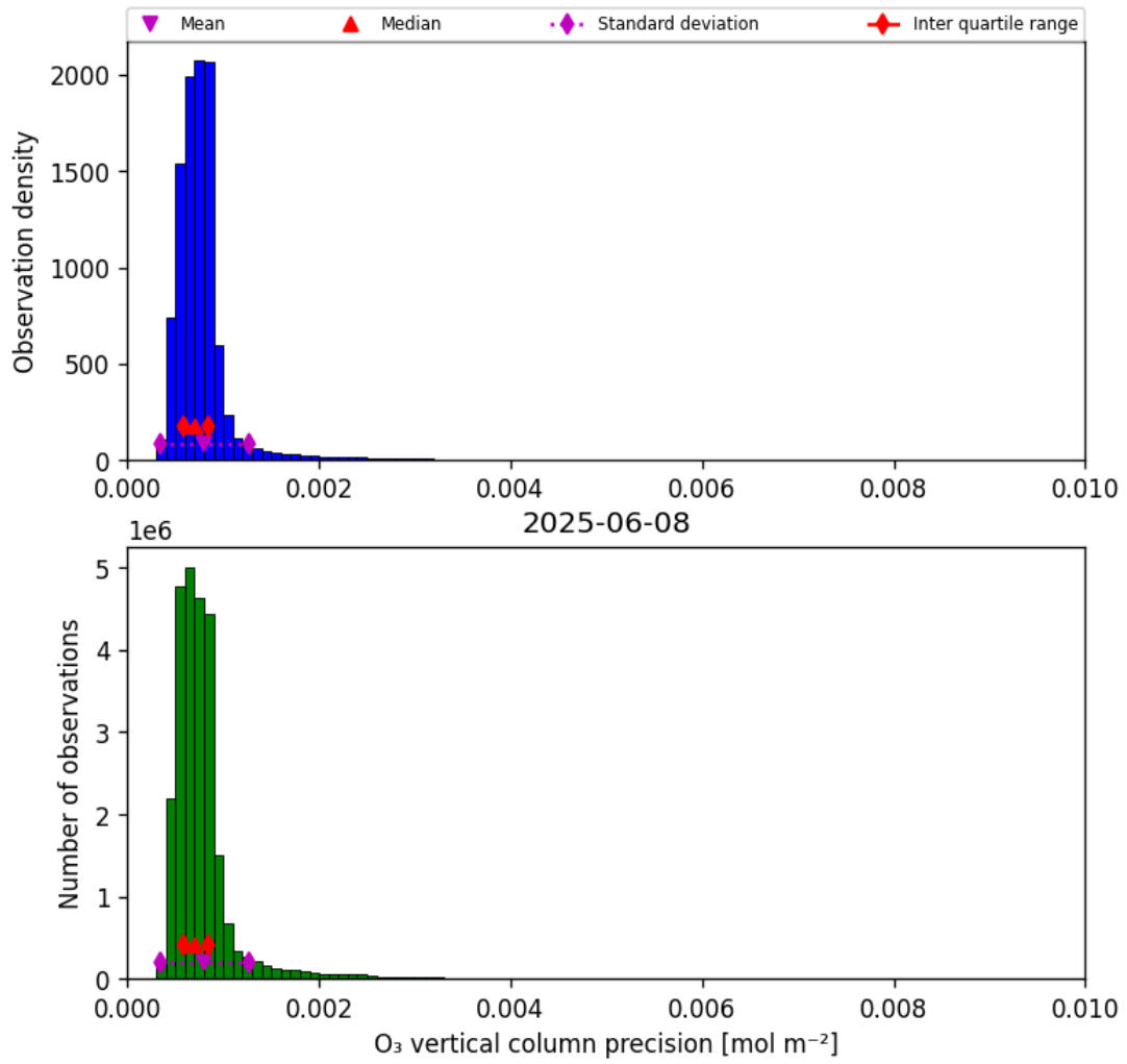
Figure 22: Histogram of “O 3 vertical column precision” for 2025-06-07 to 2025-06-09
