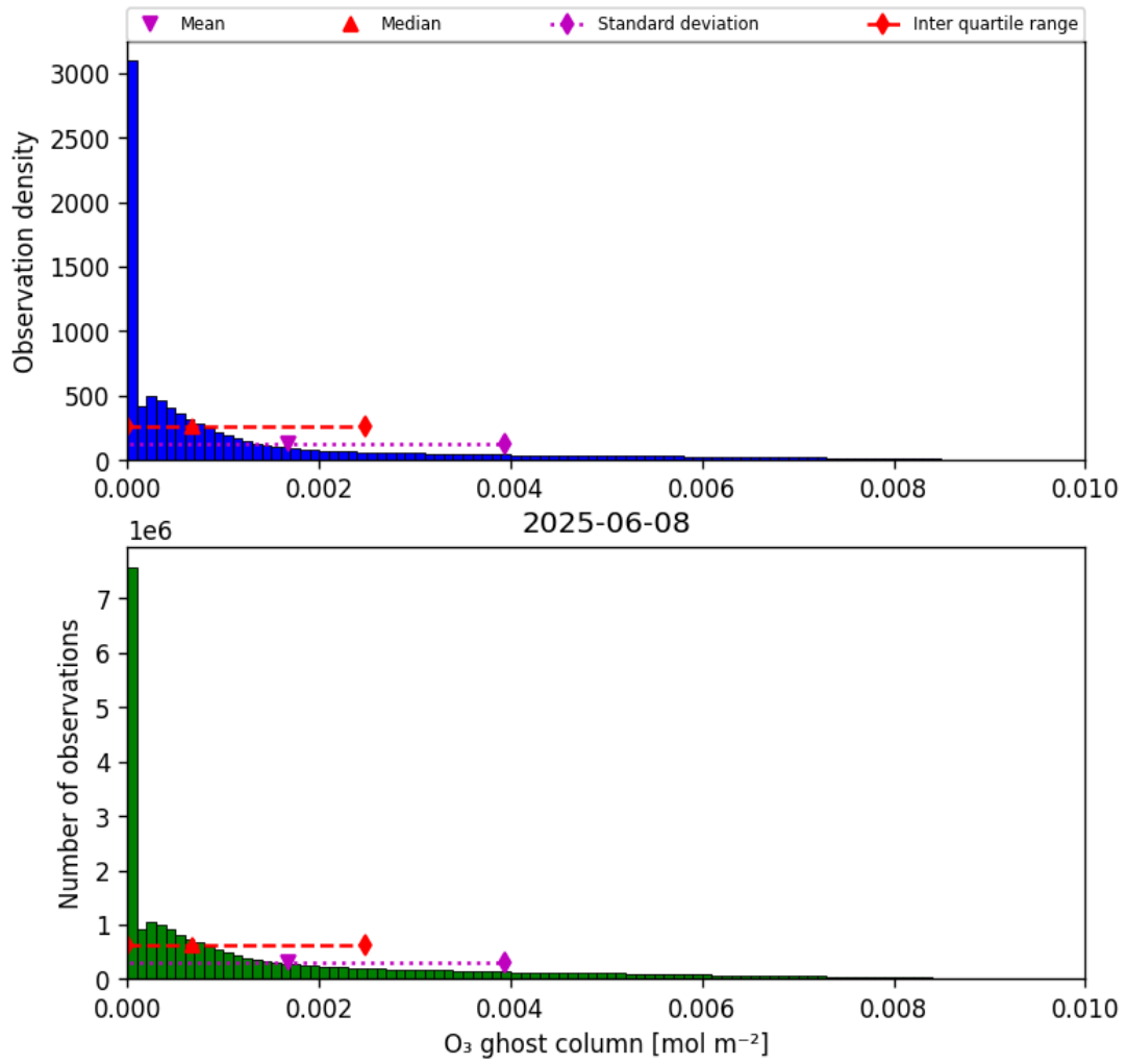
Figure 25: Histogram of “O 3 ghost column” for 2025-06-07 to 2025-06-09
