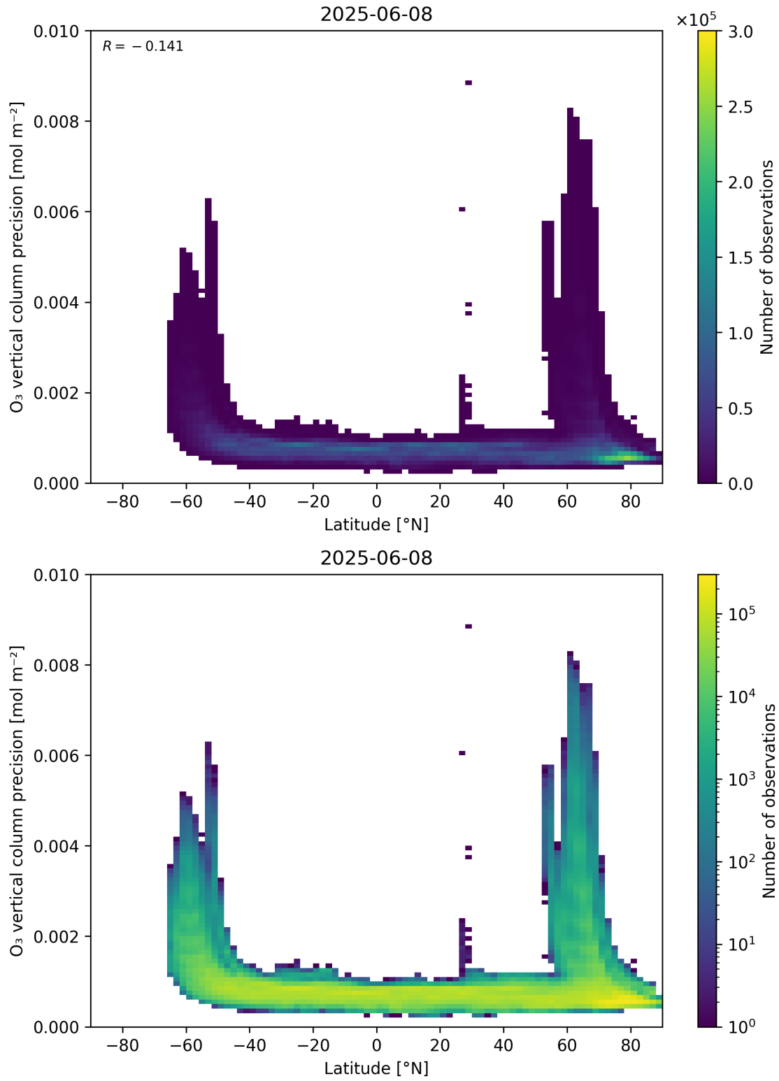
Figure 37: Scatter density plot of “Latitude” against “O 3 vertical column precision” for 2025-06-07 to 2025-06-09.
