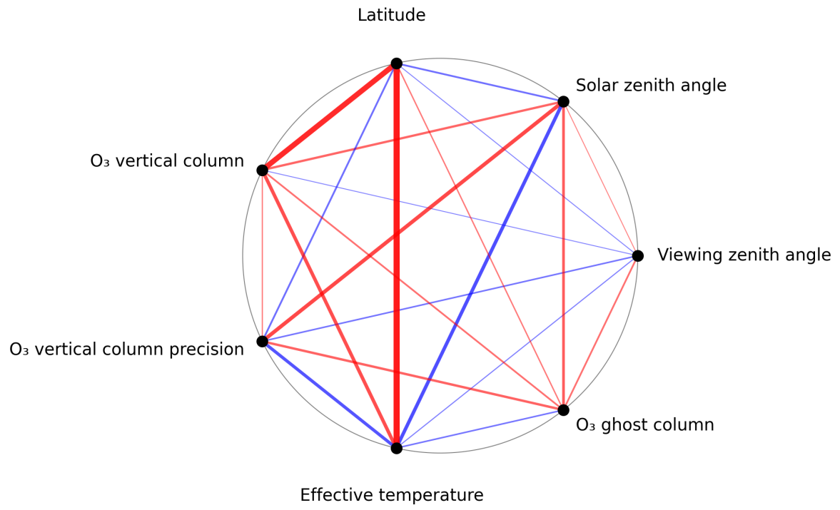
Figure 1: Map of correlation graph for 2025-06-07 to 2025-06-09.
