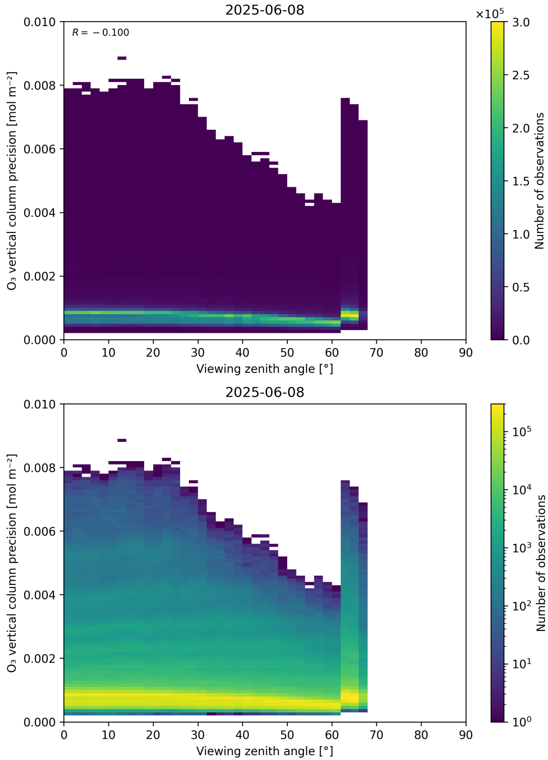
Figure 53: Scatter density plot of “Viewing zenith angle” against “O 3 vertical column precision” for 2025-06-07 to 2025-06-09.
