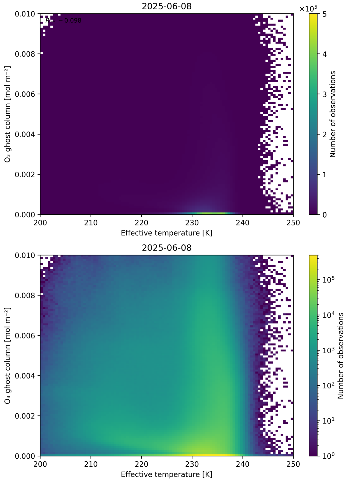
Figure 38: Scatter density plot of “Effective temperature” against “O 3 ghost column” for 2025-06-07 to 2025-06-09.
