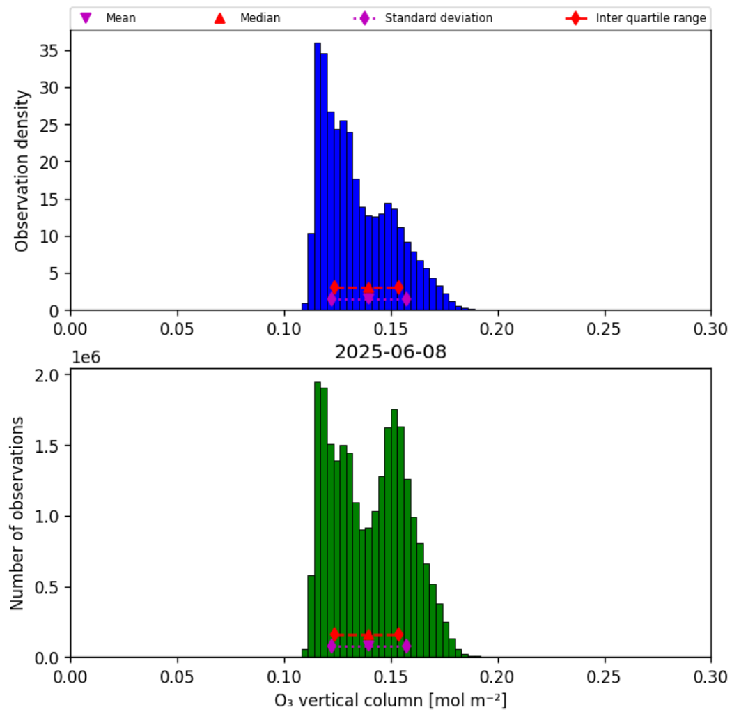
Figure 21: Histogram of “O 3 vertical column” for 2025-06-07 to 2025-06-09
