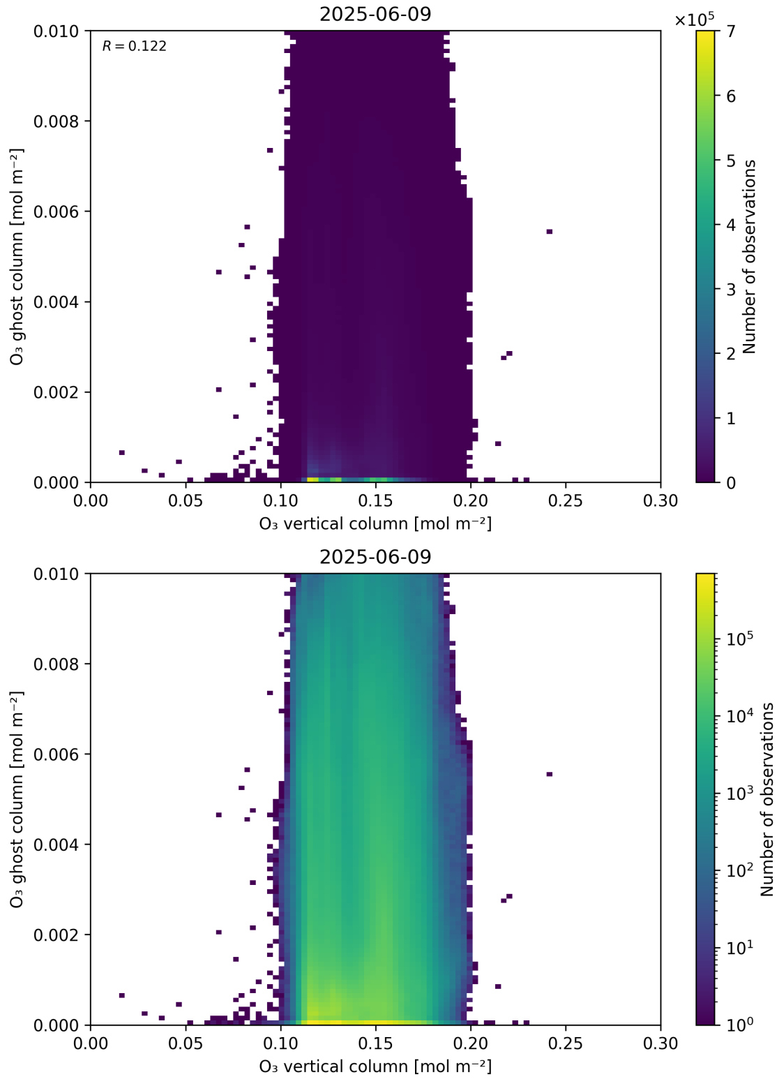
Figure 40: Scatter density plot of “O 3 vertical column” against “O 3 ghost column” for 2025-06-08 to 2025-06-10.
