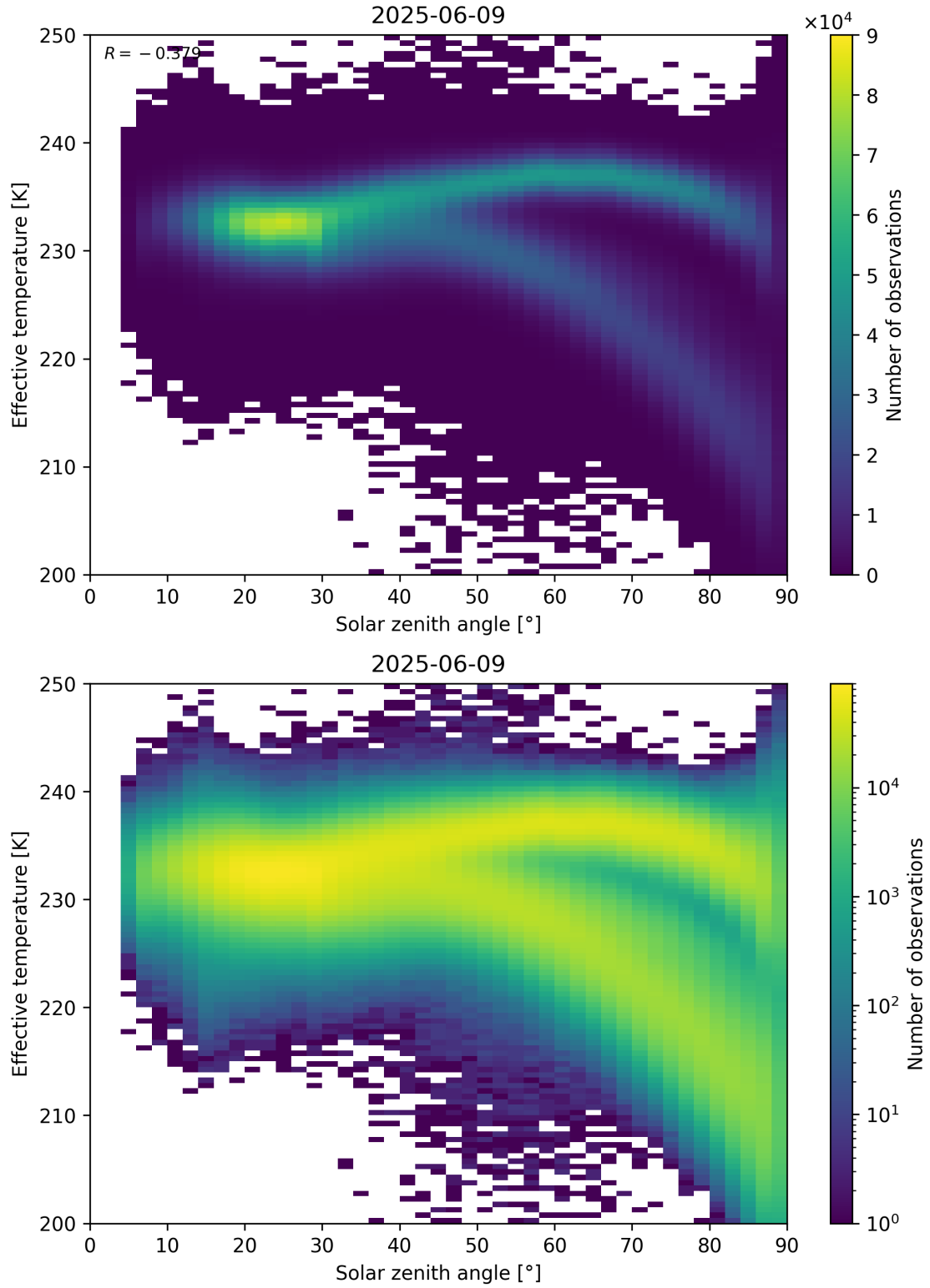
Figure 45: Scatter density plot of “Solar zenith angle” against “Effective temperature” for 2025-06-08 to 2025-06-10.
