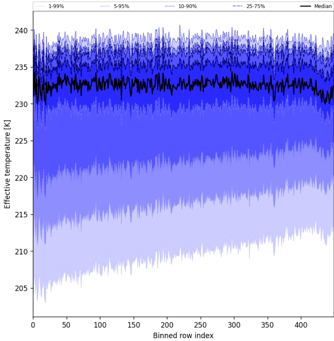
Figure 31: Along track statistics of “Effective temperature” for 2025-06-08 to 2025-06-10
