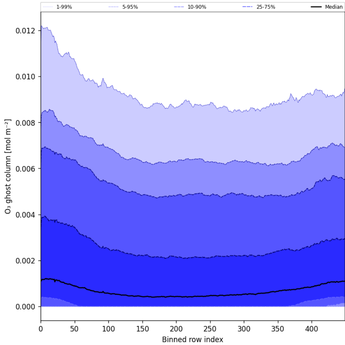
Figure 32: Along track statistics of “O 3 ghost column” for 2025-06-08 to 2025-06-10
