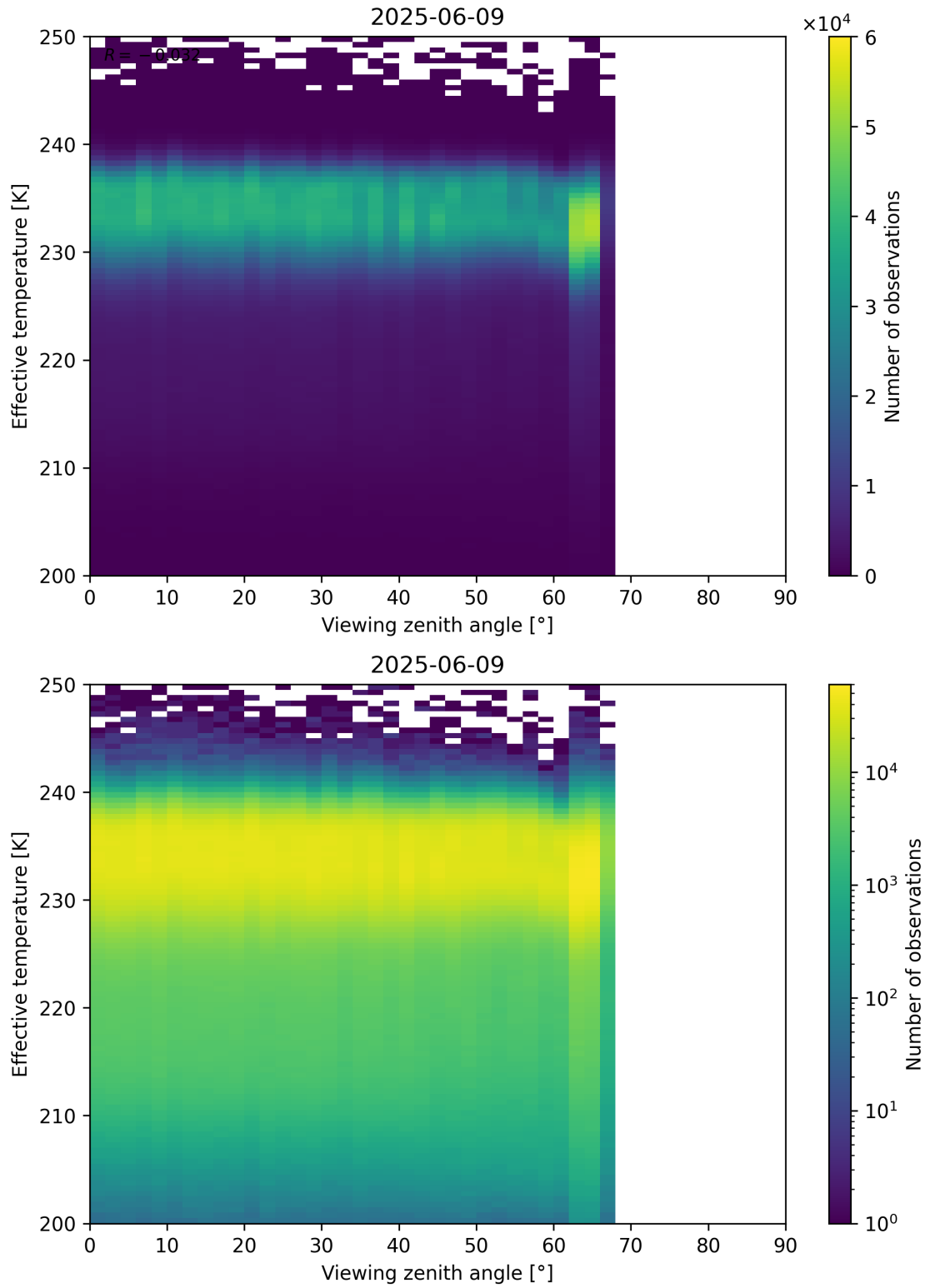
Figure 50: Scatter density plot of “Viewing zenith angle” against “Effective temperature” for 2025-06-08 to 2025-06-10.
