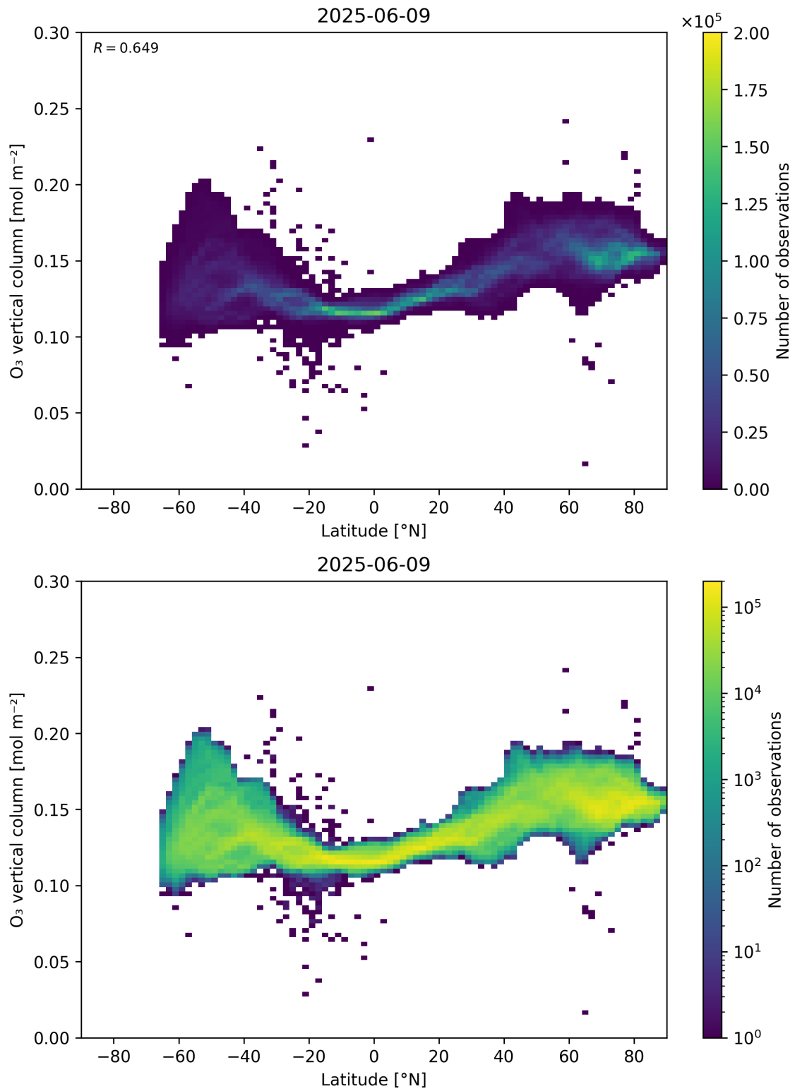
Figure 36: Scatter density plot of “Latitude” against “O 3 vertical column” for 2025-06-08 to 2025-06-10.
