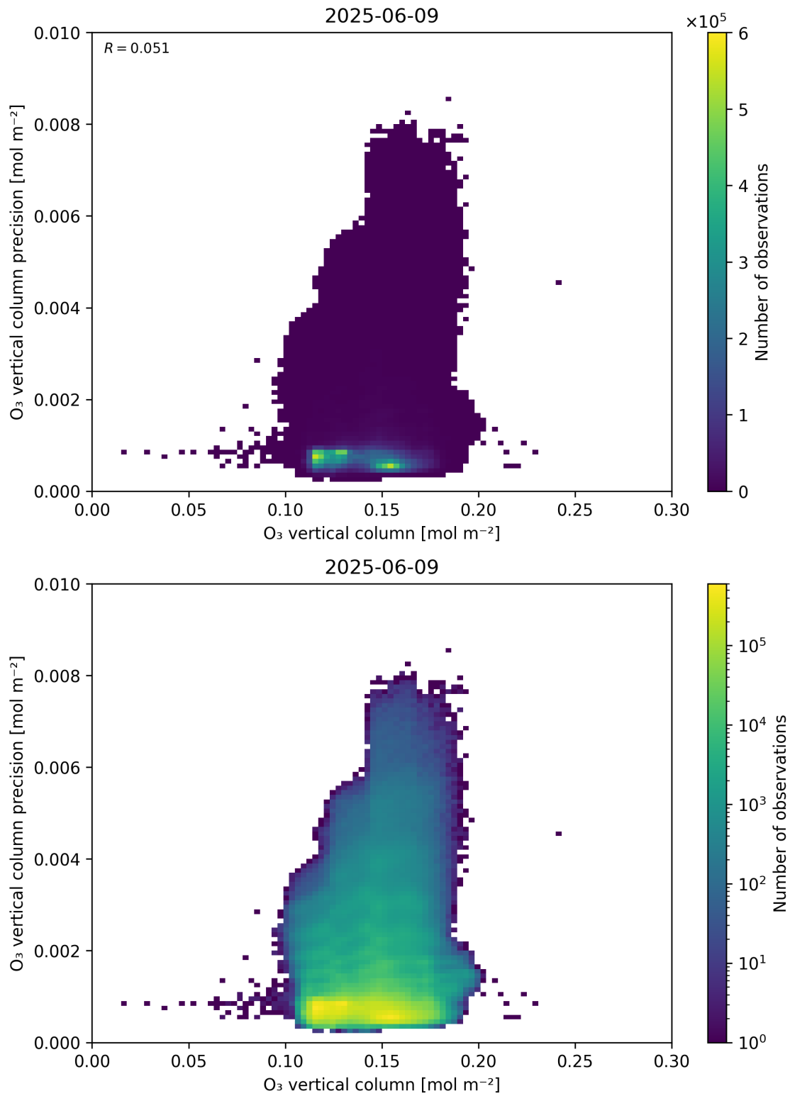
Figure 41: Scatter density plot of “O 3 vertical column” against “O 3 vertical column precision” for 2025-06-08 to 2025-06-10.
