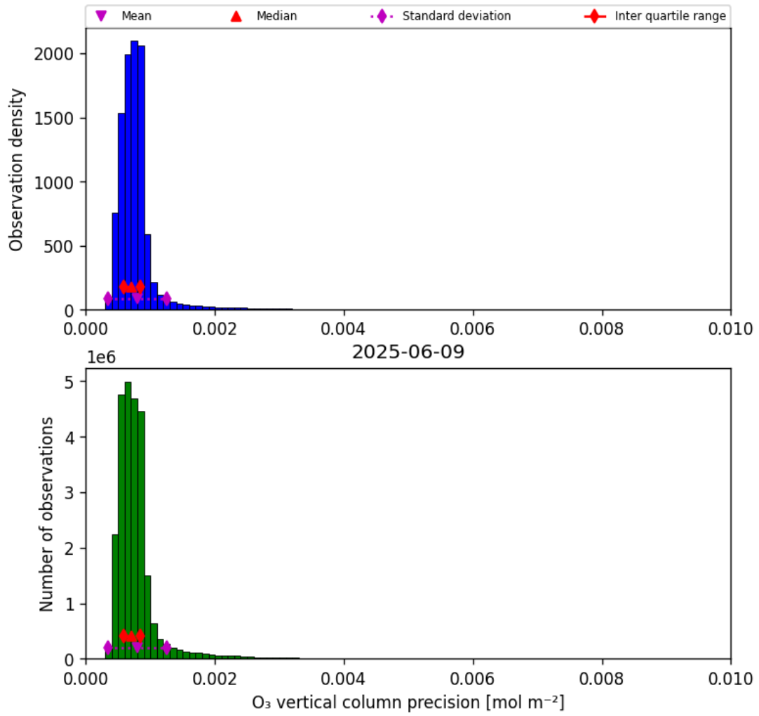
Figure 22: Histogram of “O 3 vertical column precision” for 2025-06-08 to 2025-06-10
