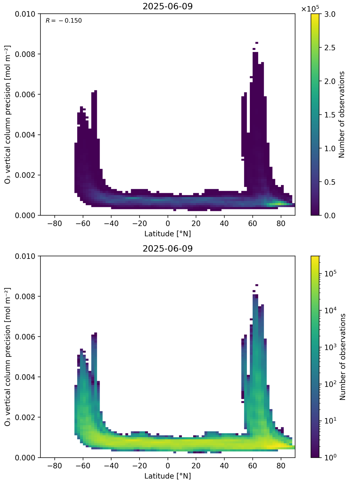
Figure 37: Scatter density plot of “Latitude” against “O 3 vertical column precision” for 2025-06-08 to 2025-06-10.
