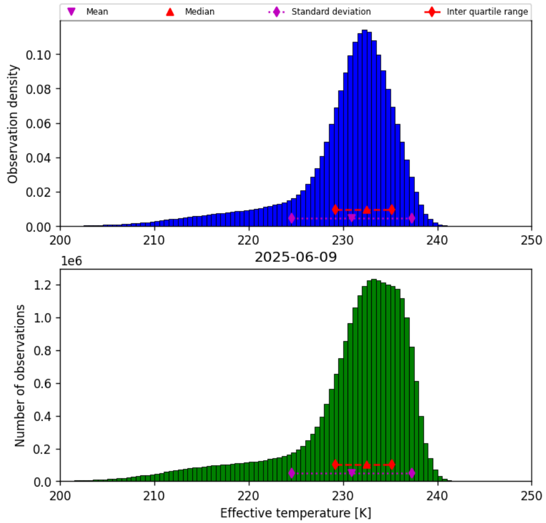
Figure 24: Histogram of “Effective temperature” for 2025-06-08 to 2025-06-10
