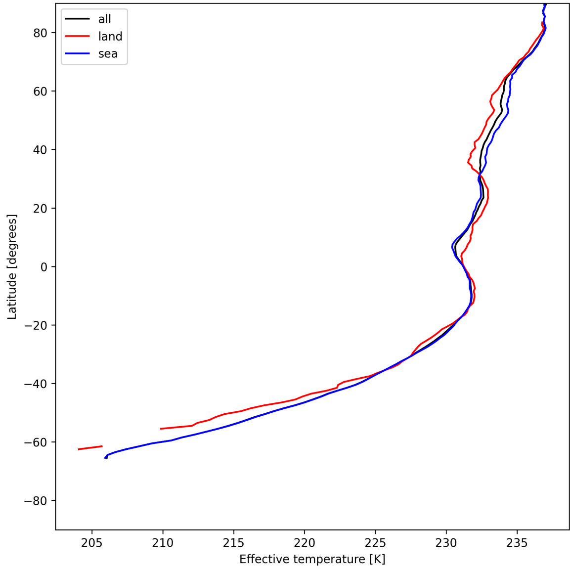
Figure 17: Zonal average of "Effective temperature" for 2025-06-08 to 2025-06-10.
