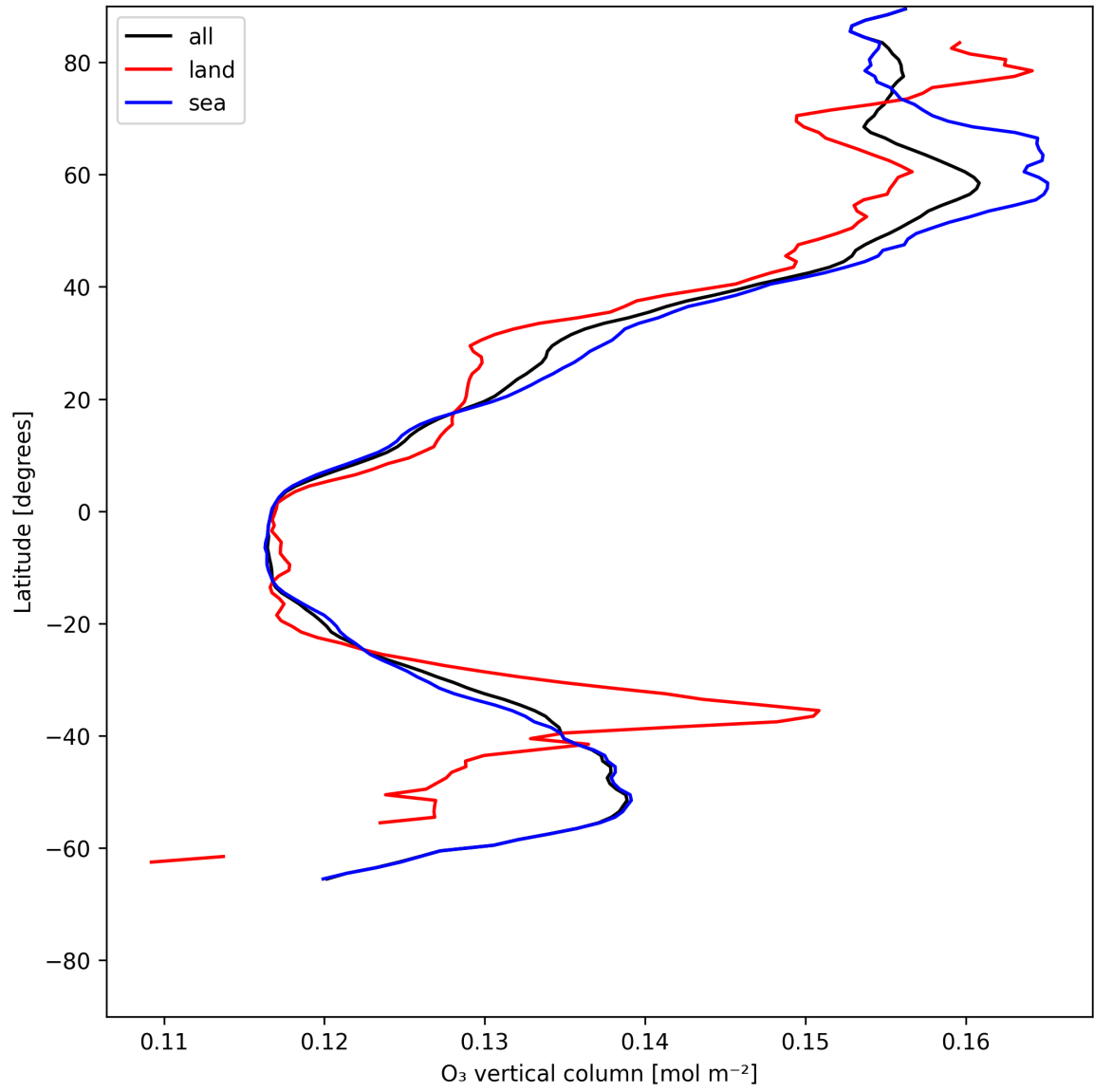
Figure 14: Zonal average of “O 3 vertical column” for 2025-06-08 to 2025-06-10.
