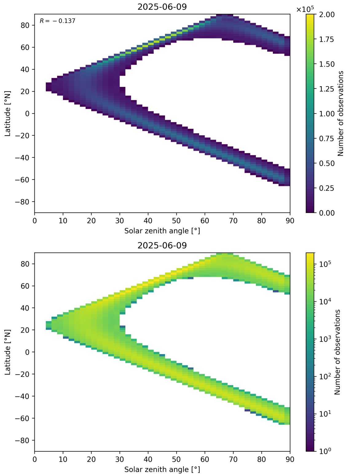
Figure 44: Scatter density plot of “Solar zenith angle” against “Latitude” for 2025-06-08 to 2025-06-10.
