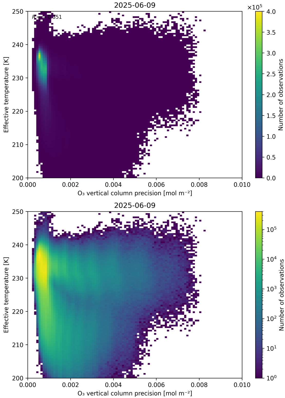
Figure 42: Scatter density plot of “O 3 vertical column precision” against “Effective temperature” for 2025-06-08 to 2025-06-10.
