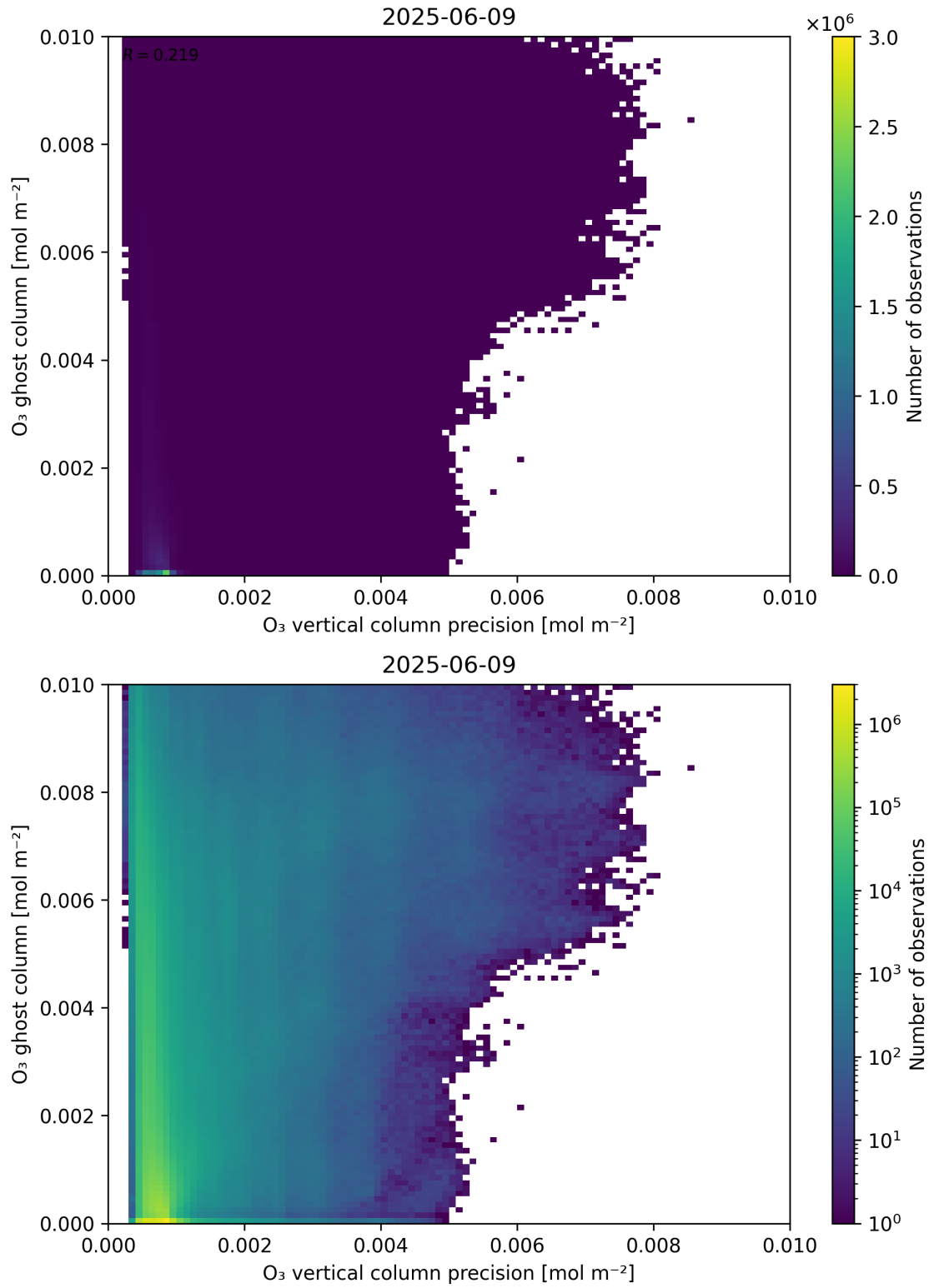
Figure 43: Scatter density plot of “ \text{O}_3 vertical column precision” against “ \text{O}_3 ghost column” for 2025-06-08 to 2025-06-10.
