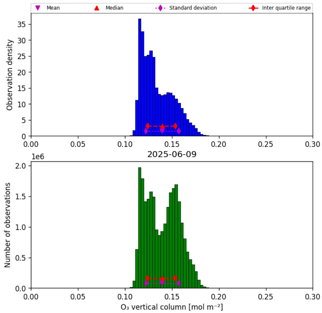
Figure 21: Histogram of “O 3 vertical column” for 2025-06-08 to 2025-06-10
