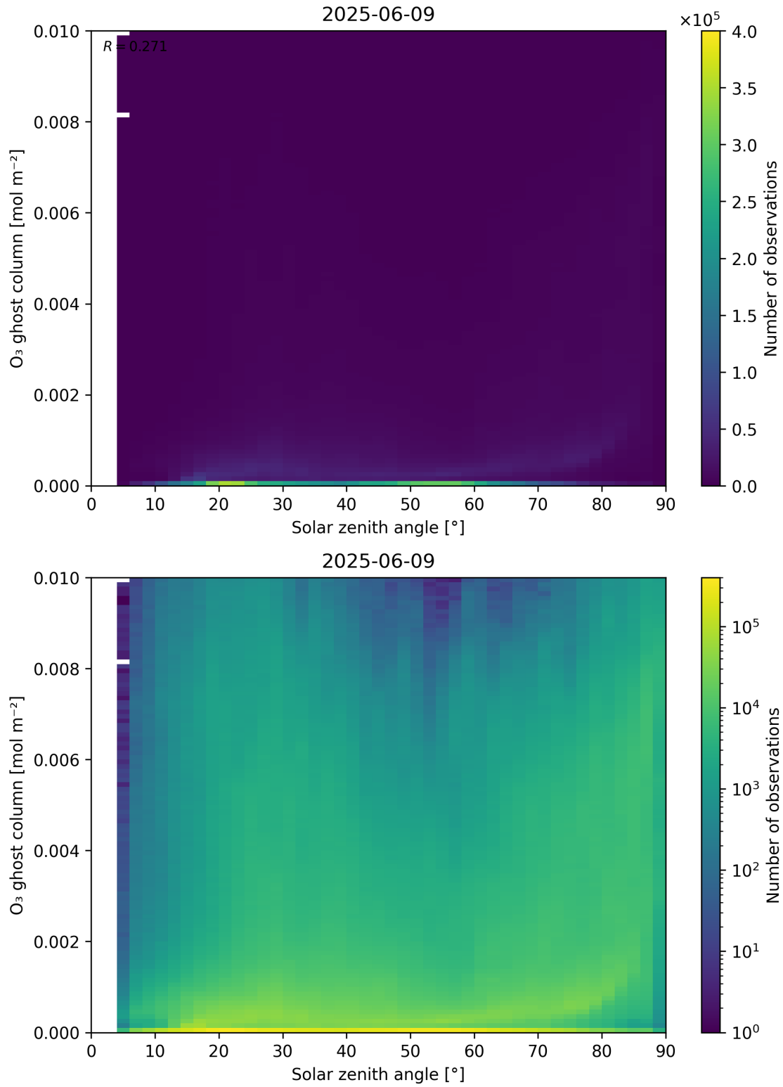
Figure 46: Scatter density plot of “Solar zenith angle” against “O 3 ghost column” for 2025-06-08 to 2025-06-10.
