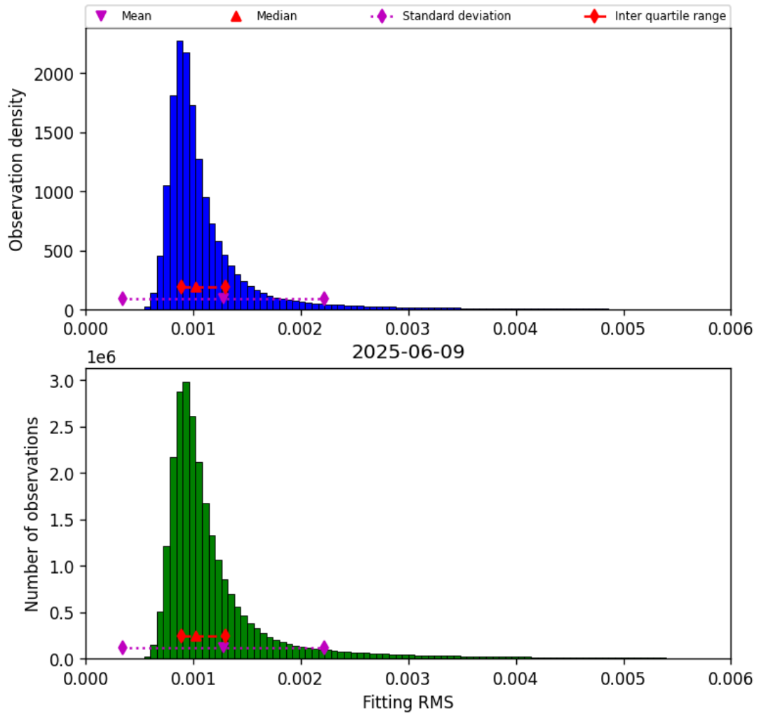
Figure 23: Histogram of “Fitting RMS” for 2025-06-08 to 2025-06-10
