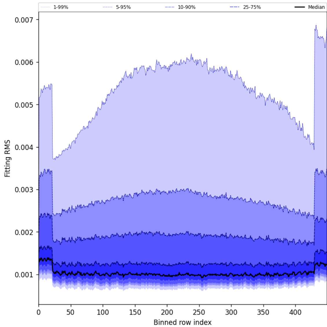
Figure 30: Along track statistics of “Fitting RMS” for 2025-06-08 to 2025-06-10
