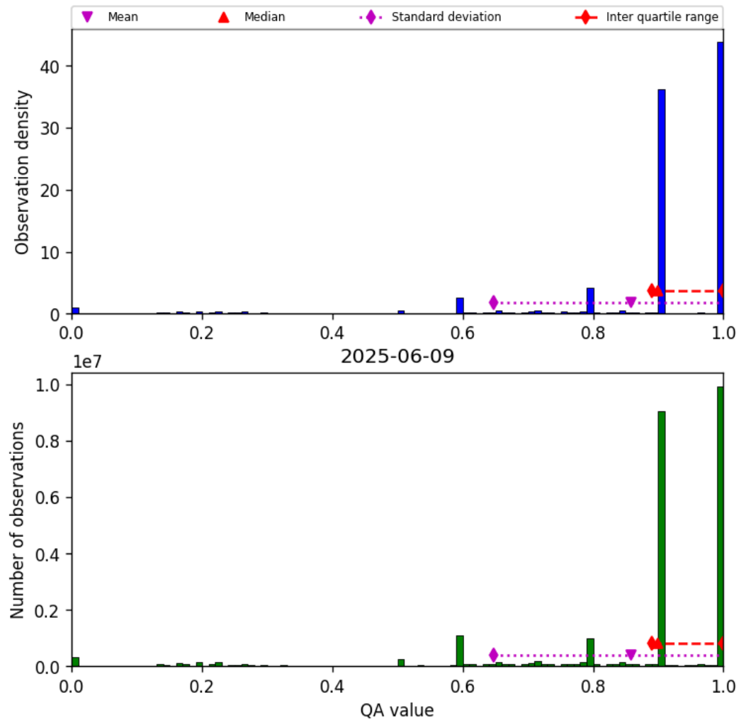
Figure 20: Histogram of “QA value” for 2025-06-08 to 2025-06-10
