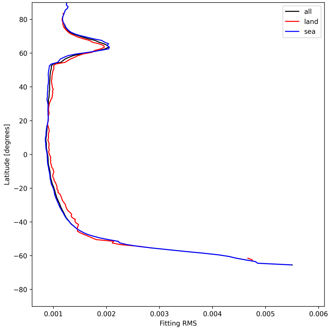
Figure 16: Zonal average of “Fitting RMS” for 2025-06-08 to 2025-06-10.
