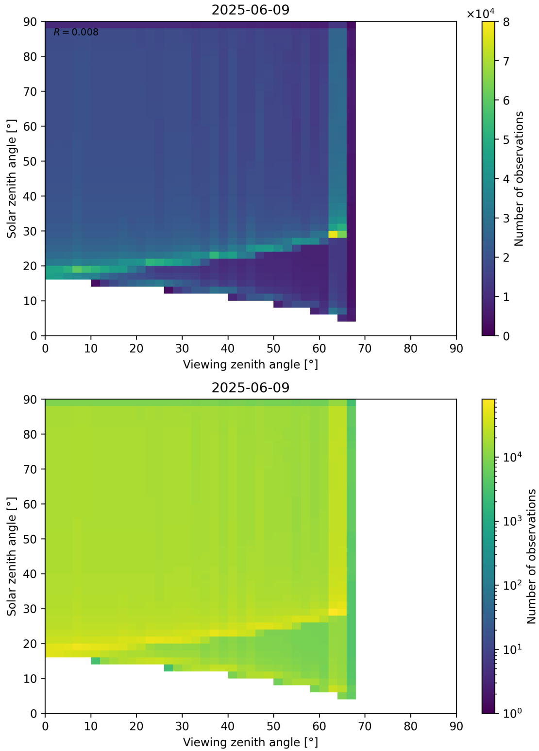
Figure 54: Scatter density plot of “Viewing zenith angle” against “Solar zenith angle” for 2025-06-08 to 2025-06-10.
