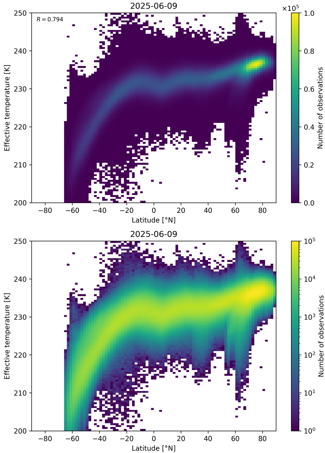
Figure 34: Scatter density plot of “Latitude” against “Effective temperature” for 2025-06-08 to 2025-06-10.
