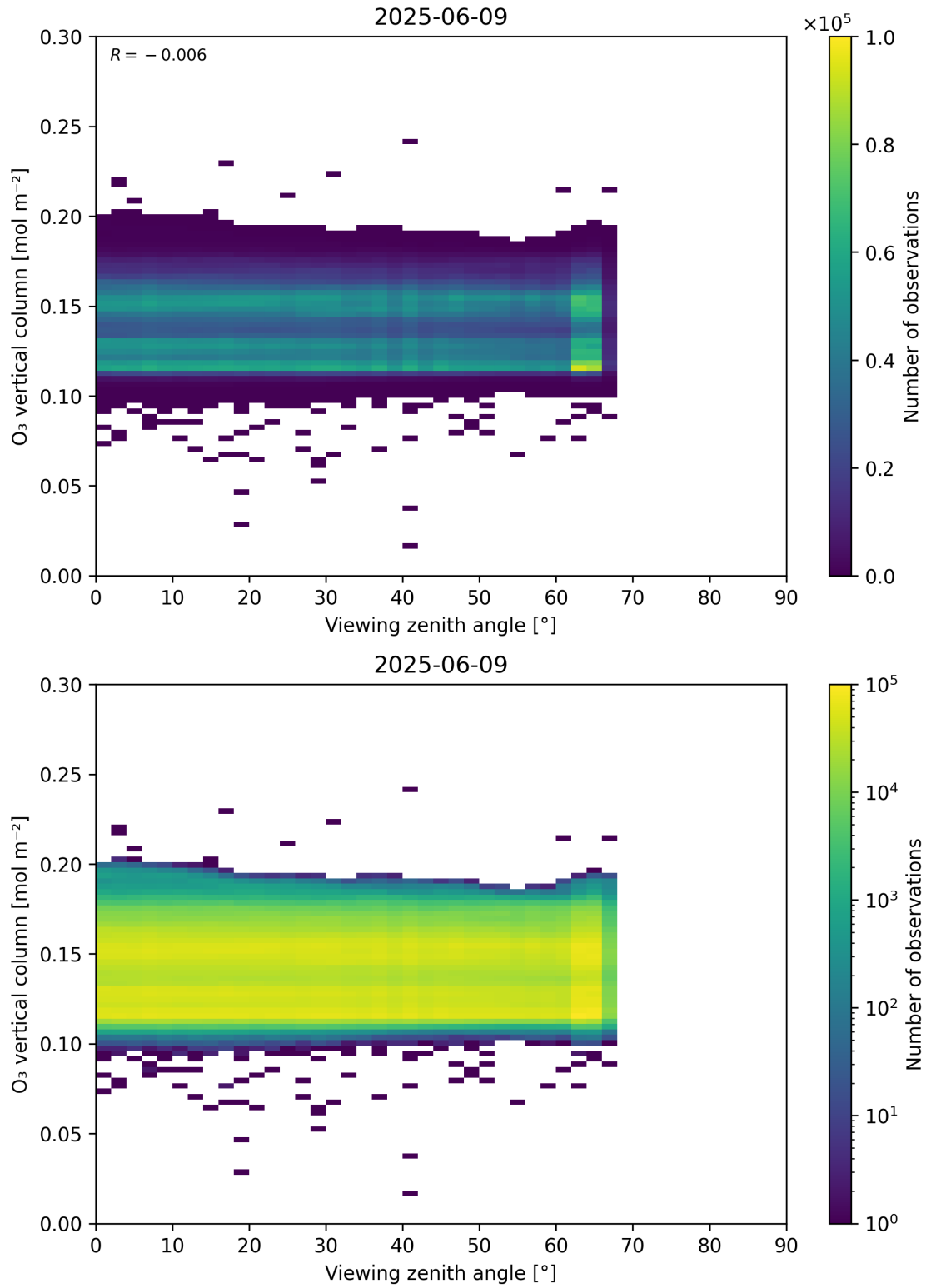
Figure 52: Scatter density plot of “Viewing zenith angle” against “O 3 vertical column” for 2025-06-08 to 2025-06-10.
