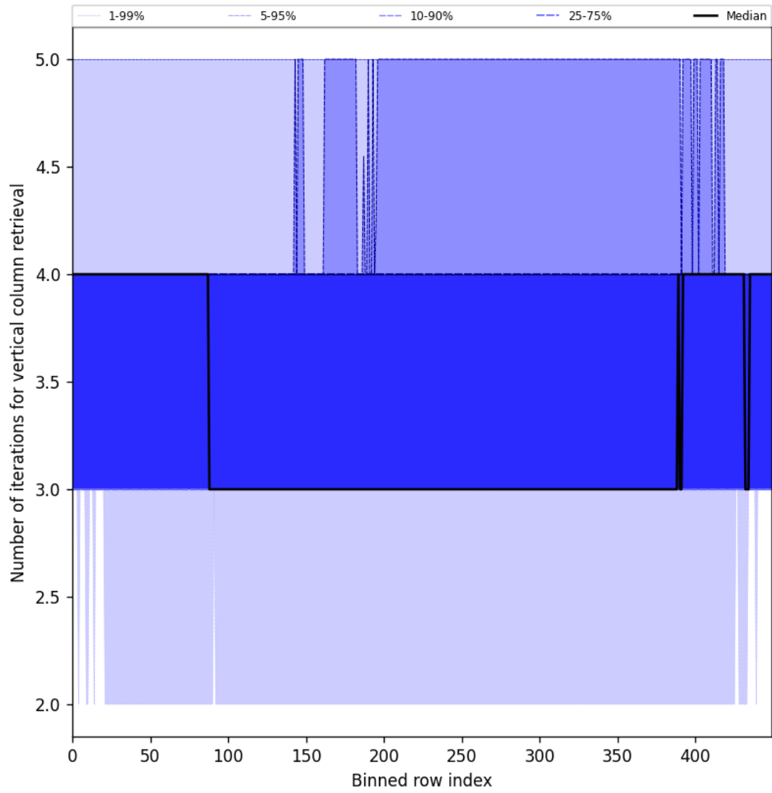
Figure 33: Along track statistics of “Number of iterations for vertical column retrieval” for 2025-06-08 to 2025-06-10
