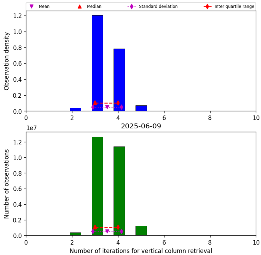
Figure 26: Histogram of “Number of iterations for vertical column retrieval” for 2025-06-08 to 2025-06-10
