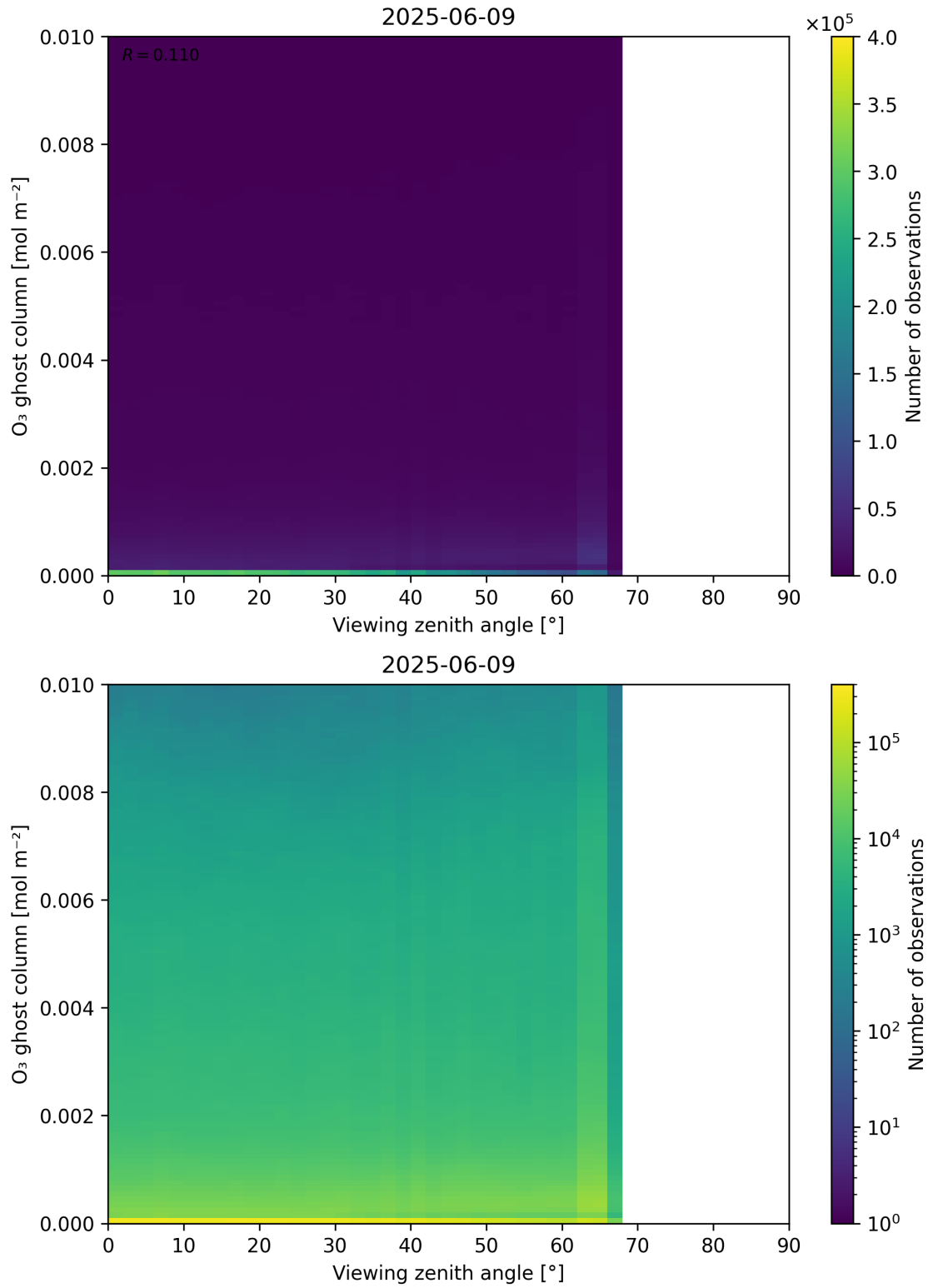
Figure 51: Scatter density plot of “Viewing zenith angle” against “O 3 ghost column” for 2025-06-08 to 2025-06-10.
