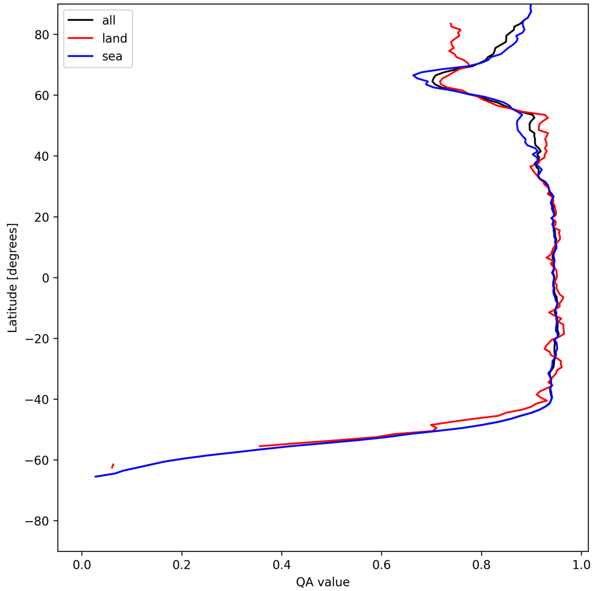
Figure 13: Zonal average of “QA value” for 2025-06-08 to 2025-06-10.
