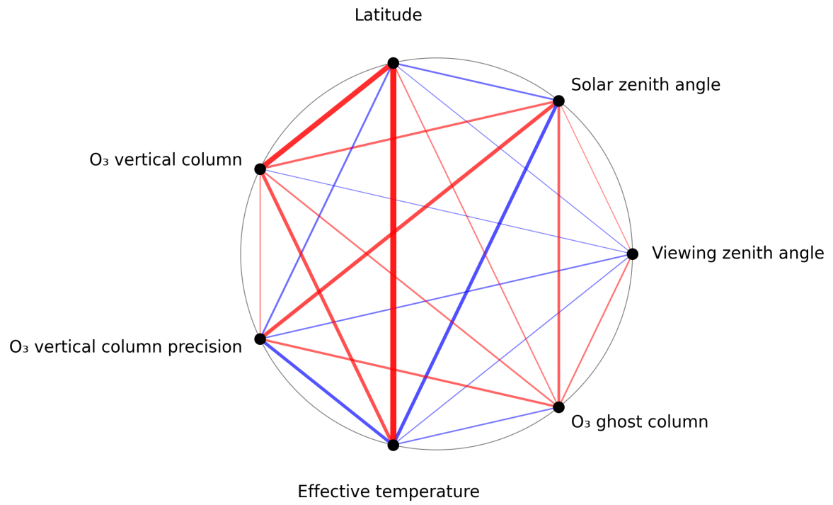
Figure 1: Map of correlation graph for 2025-06-08 to 2025-06-10.
