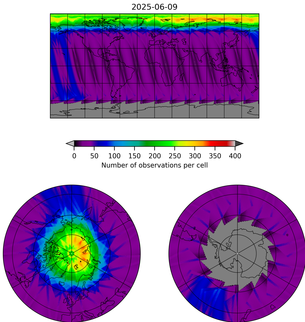
Figure 12: Map of the number of observations for 2025-06-08 to 2025-06-10
