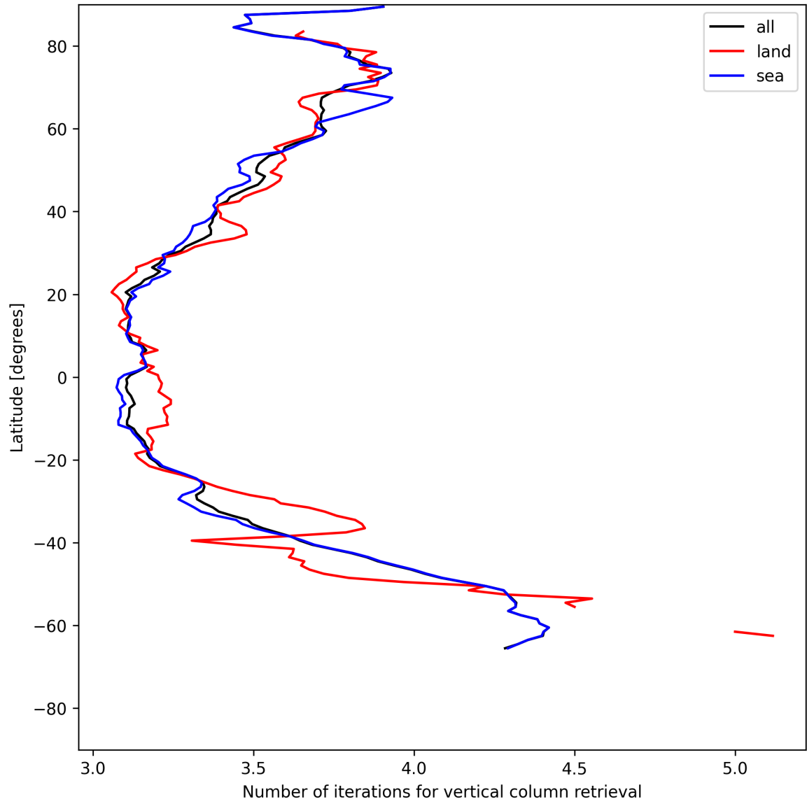
Figure 19: Zonal average of “Number of iterations for vertical column retrieval” for 2025-06-08 to 2025-06-10.
