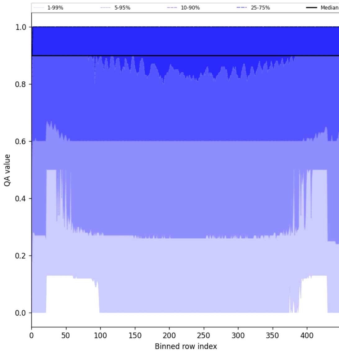
Figure 27: Along track statistics of “QA value” for 2025-06-08 to 2025-06-10
