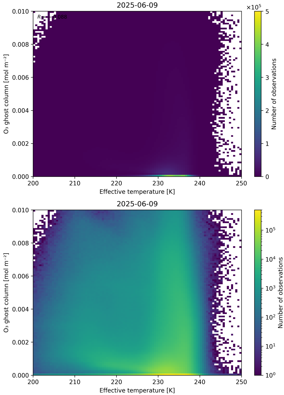
Figure 38: Scatter density plot of “Effective temperature” against “O 3 ghost column” for 2025-06-08 to 2025-06-10.
