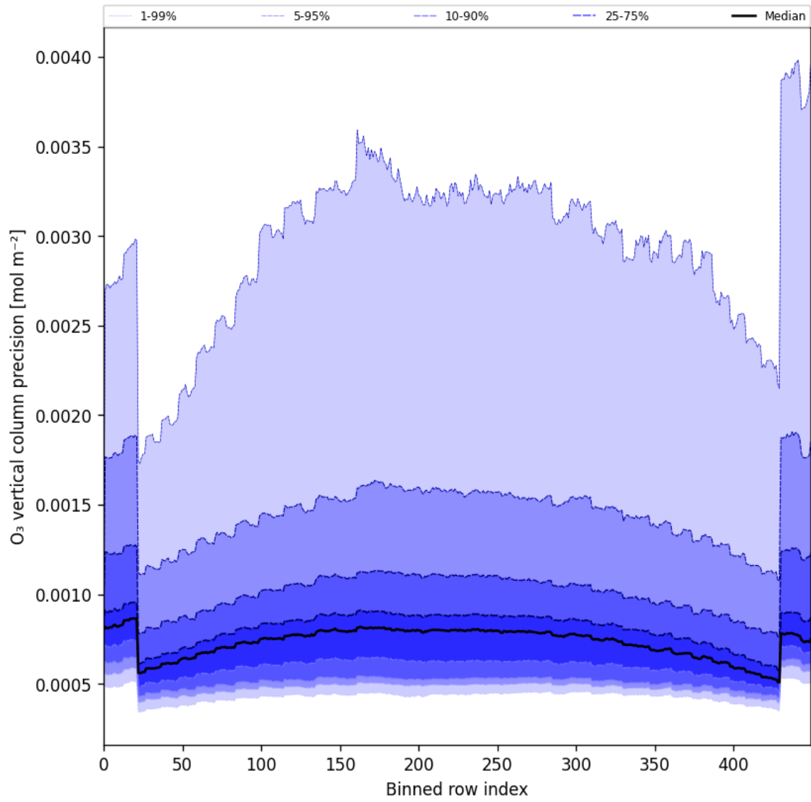
Figure 29: Along track statistics of “O 3 vertical column precision” for 2025-06-08 to 2025-06-10
