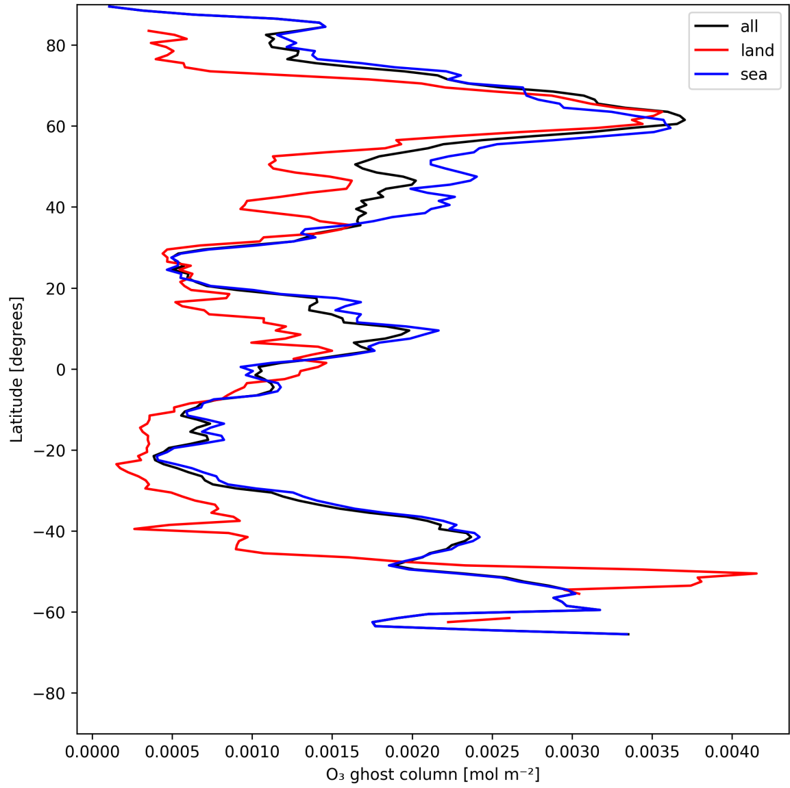
Figure 18: Zonal average of “O 3 ghost column” for 2025-06-08 to 2025-06-10.
