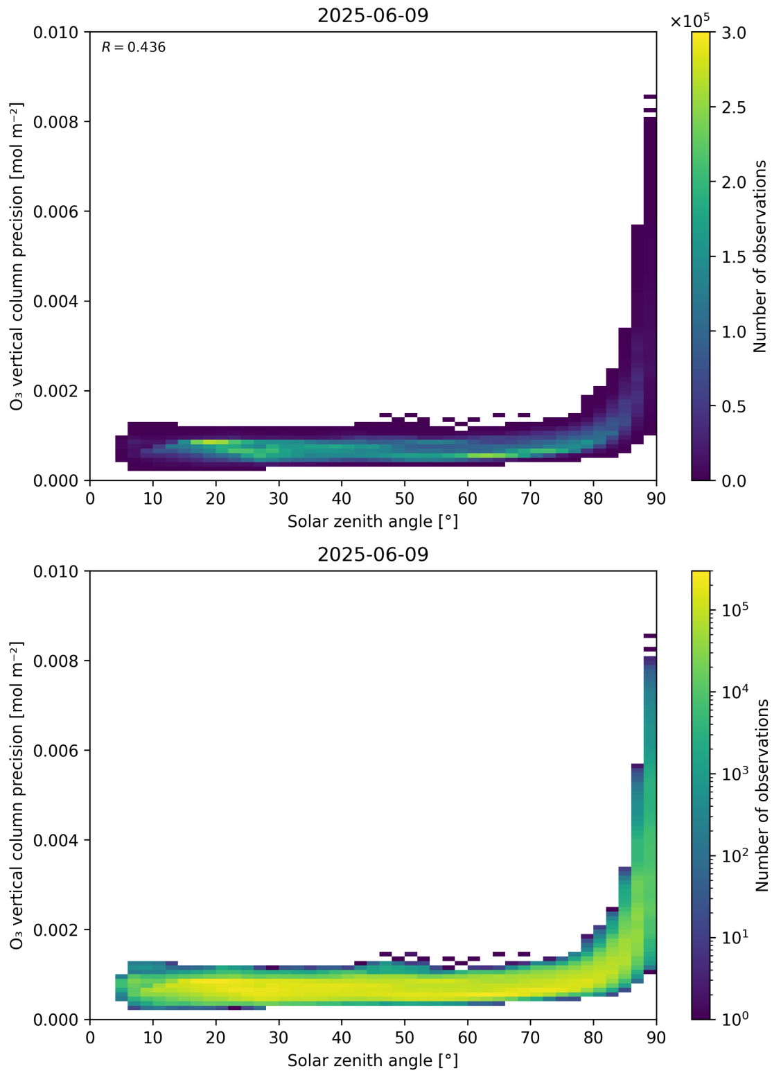
Figure 48: Scatter density plot of “Solar zenith angle” against “O 3 vertical column precision” for 2025-06-08 to 2025-06-10.
