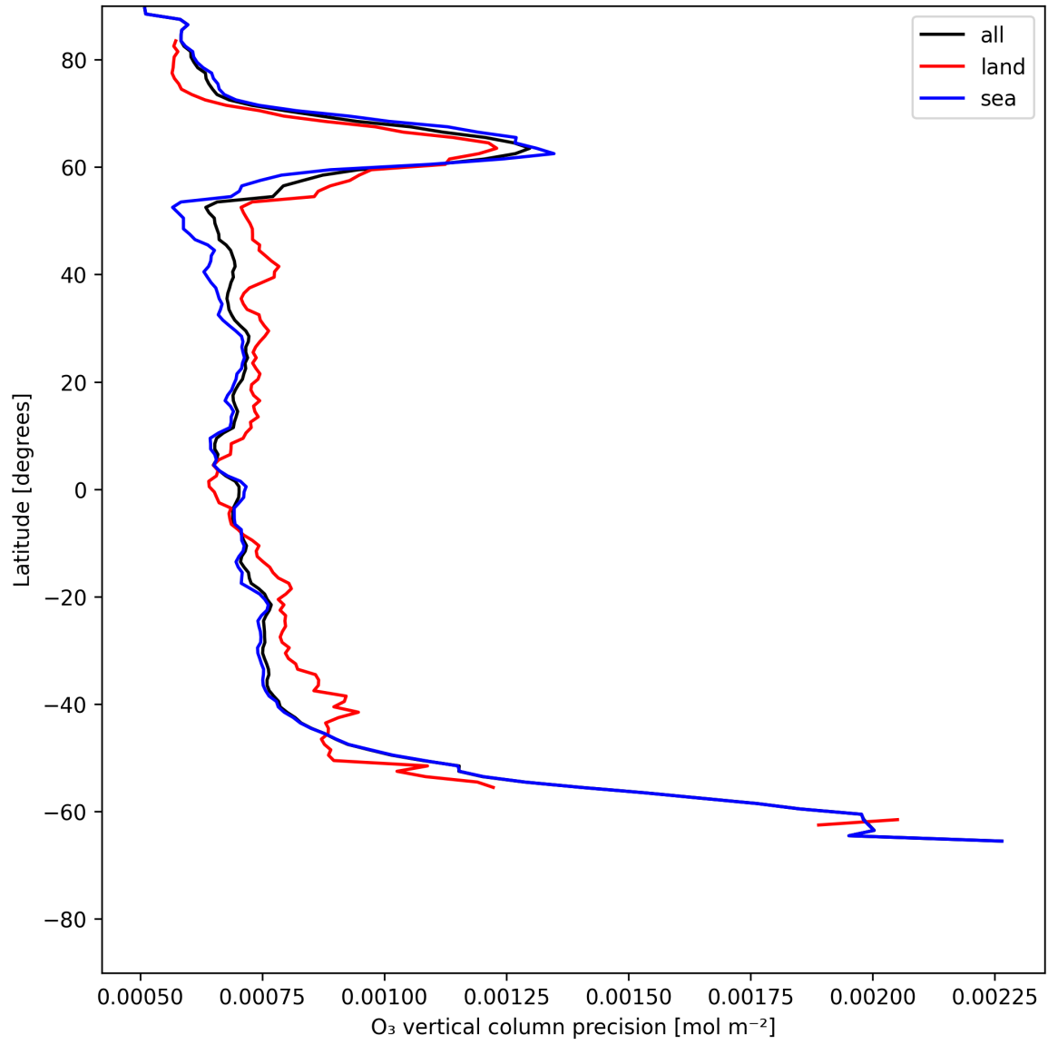
Figure 15: Zonal average of “O 3 vertical column precision” for 2025-06-08 to 2025-06-10.
