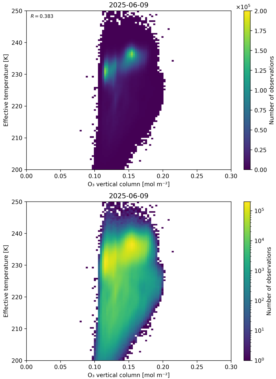
Figure 39: Scatter density plot of “O 3 vertical column” against “Effective temperature” for 2025-06-08 to 2025-06-10.
