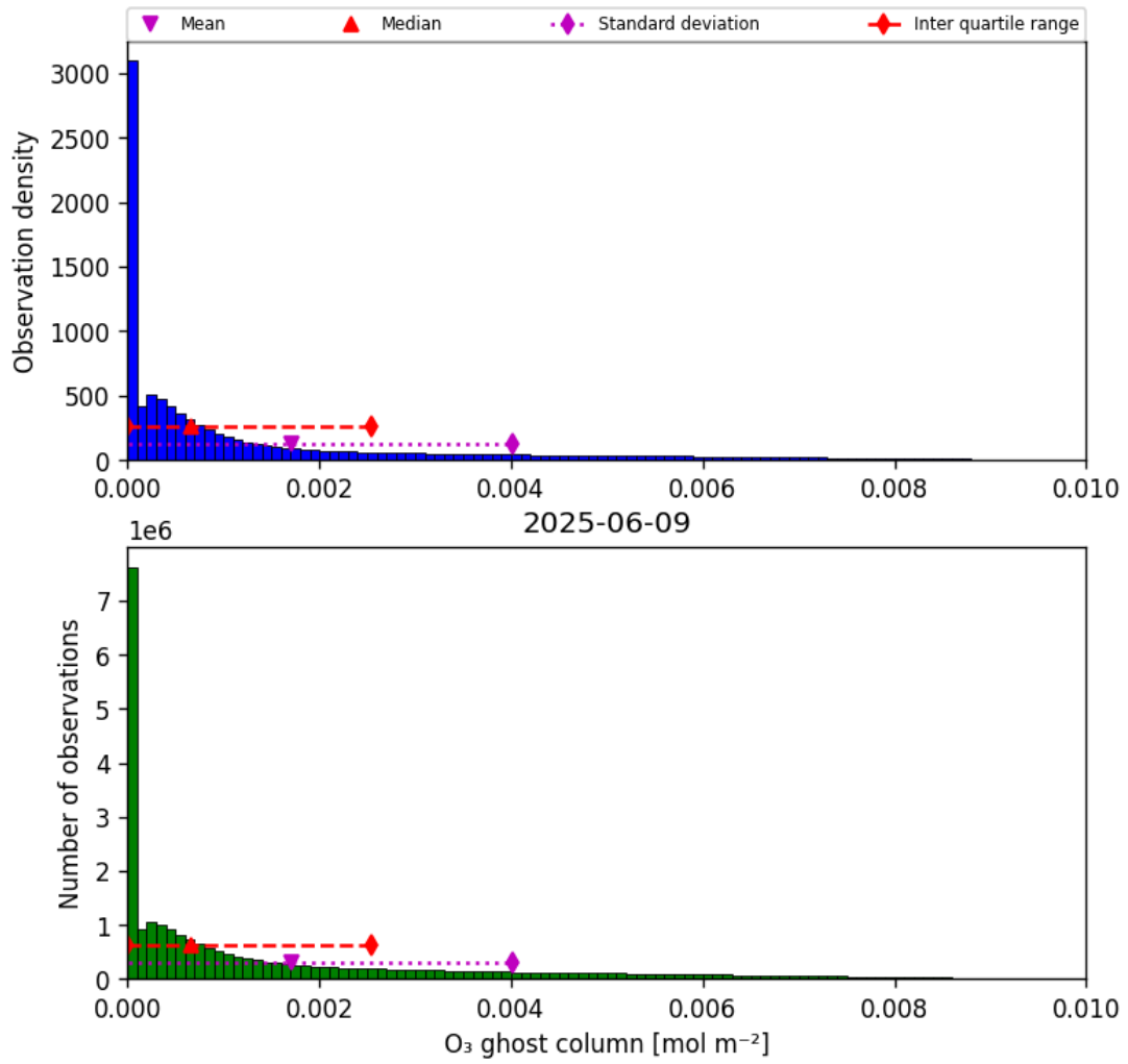
Figure 25: Histogram of “O 3 ghost column” for 2025-06-08 to 2025-06-10
