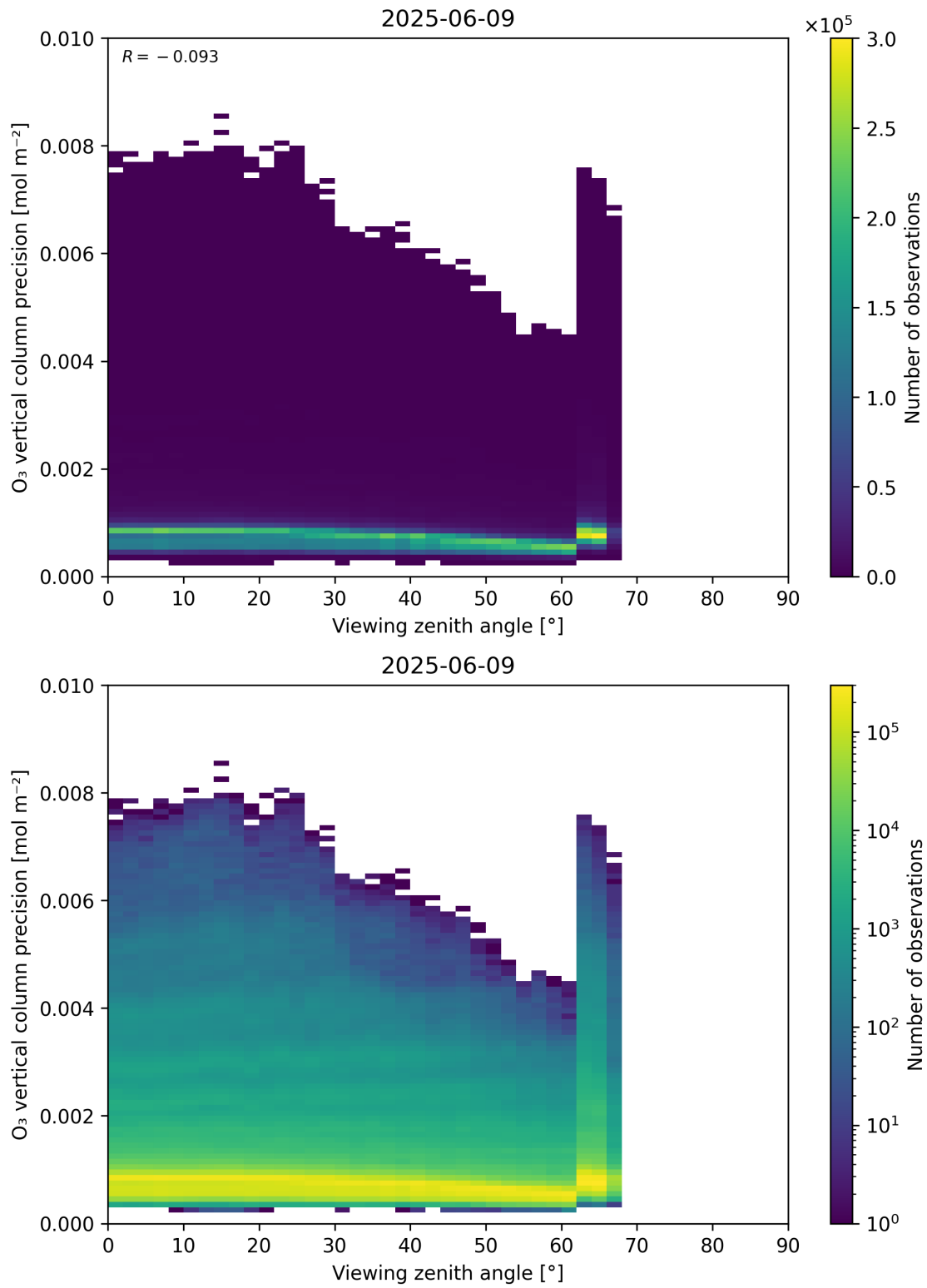
Figure 53: Scatter density plot of “Viewing zenith angle” against “O 3 vertical column precision” for 2025-06-08 to 2025-06-10.
