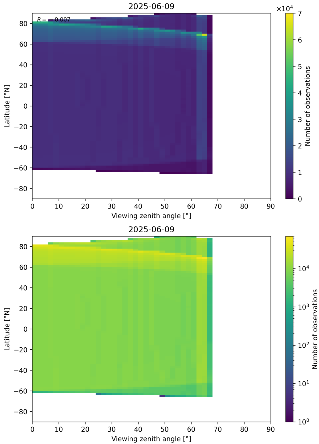
Figure 49: Scatter density plot of “Viewing zenith angle” against “Latitude” for 2025-06-08 to 2025-06-10.
