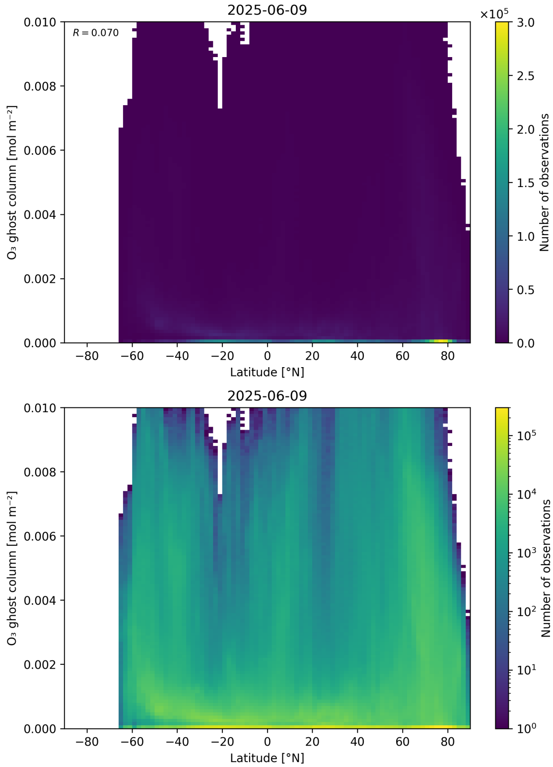
Figure 35: Scatter density plot of “Latitude” against “O 3 ghost column” for 2025-06-08 to 2025-06-10.
