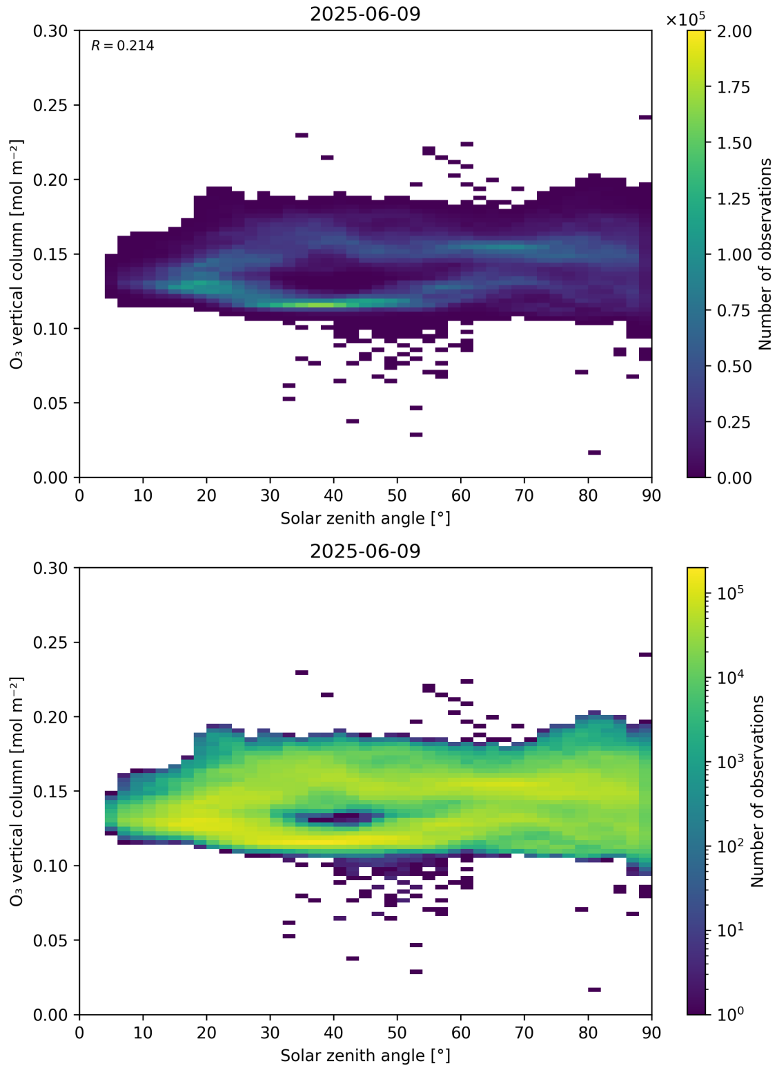
Figure 47: Scatter density plot of “Solar zenith angle” against “O 3 vertical column” for 2025-06-08 to 2025-06-10.
