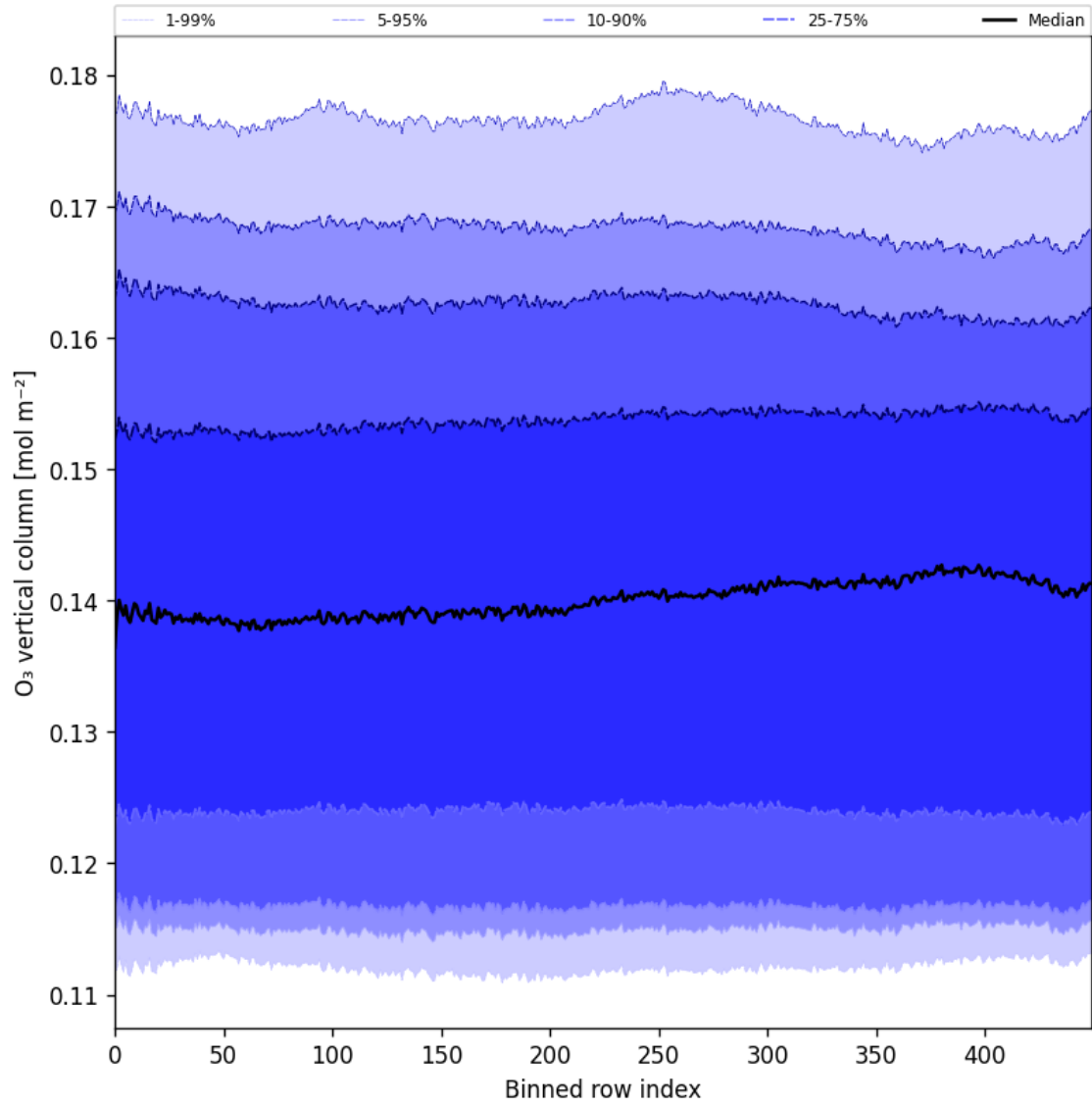
Figure 28: Along track statistics of “O 3 vertical column” for 2025-06-08 to 2025-06-10
