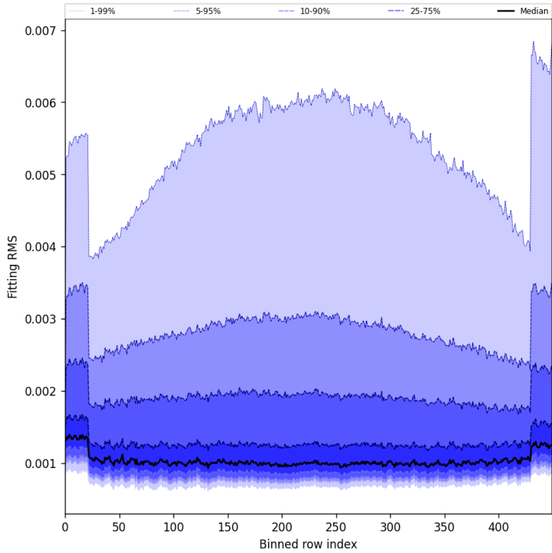
Figure 30: Along track statistics of “Fitting RMS” for 2025-06-11 to 2025-06-12
