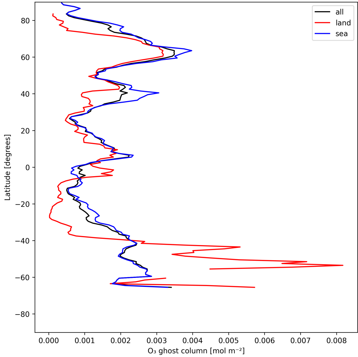
Figure 18: Zonal average of "O 3 ghost column" for 2025-06-11 to 2025-06-12.
