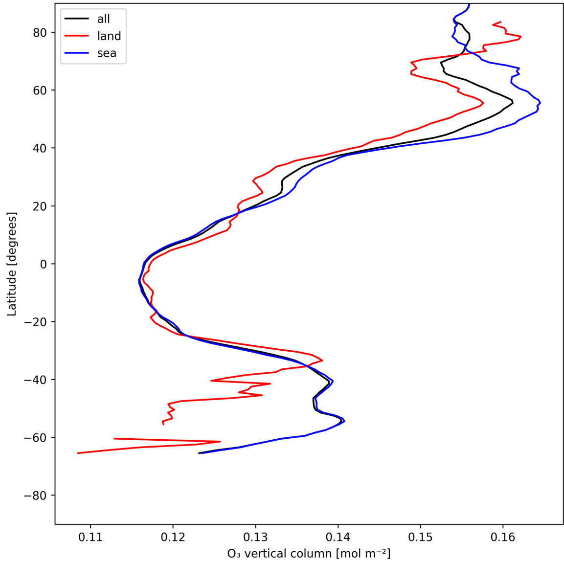
Figure 14: Zonal average of “O 3 vertical column” for 2025-06-11 to 2025-06-12.
