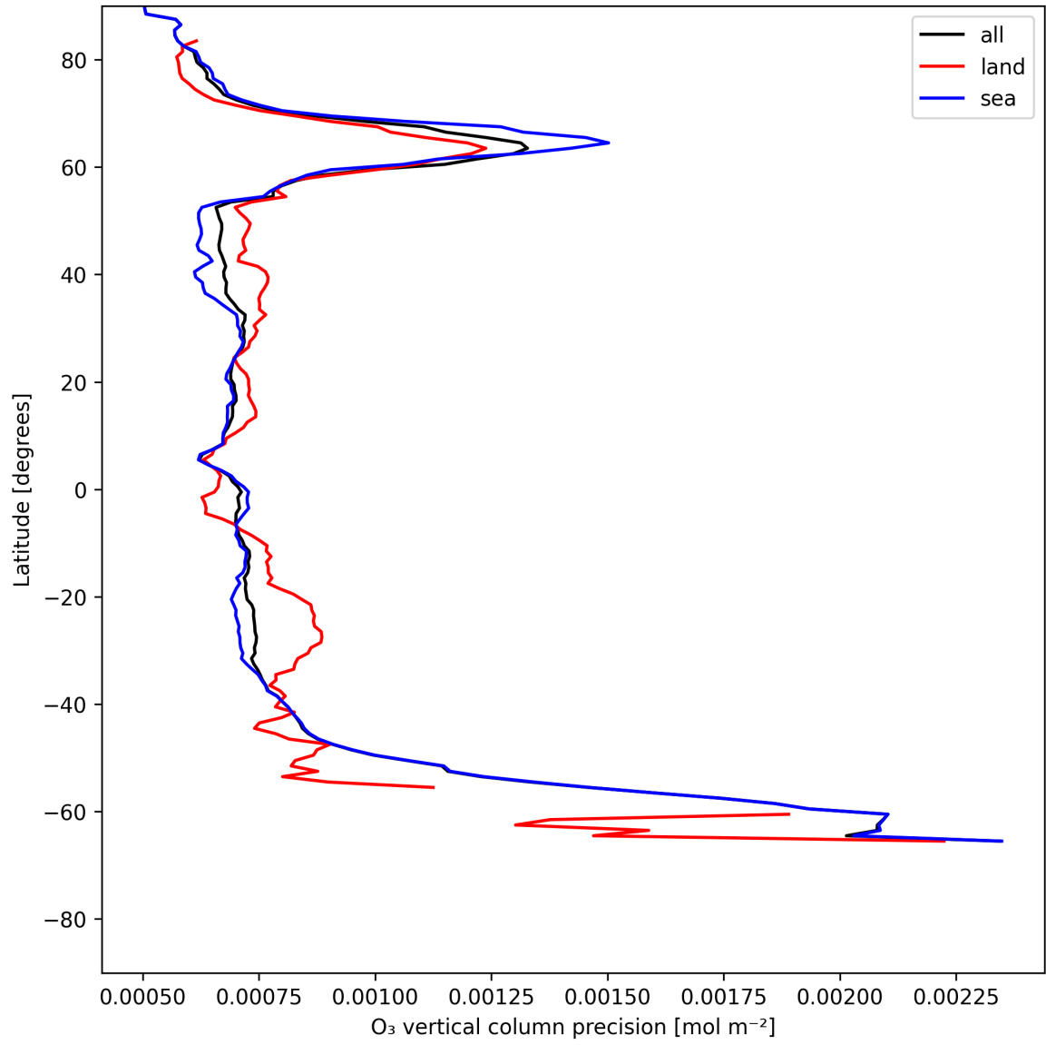
Figure 15: Zonal average of "O 3 vertical column precision" for 2025-06-11 to 2025-06-12.
