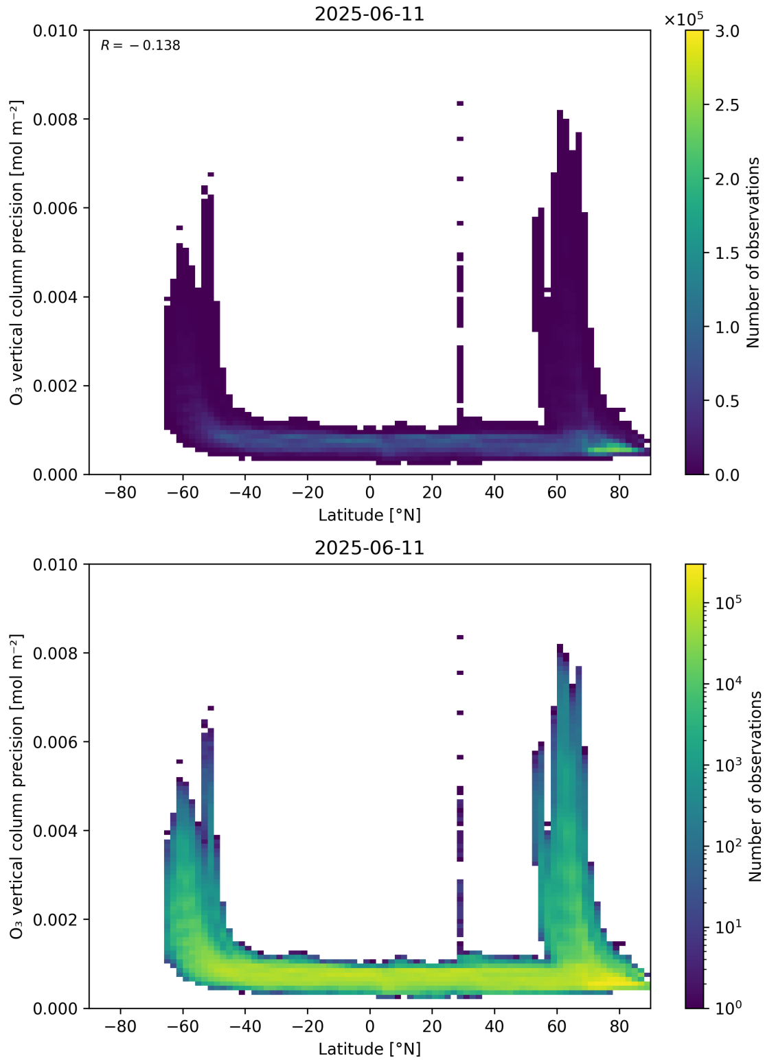
Figure 37: Scatter density plot of “Latitude” against “O 3 vertical column precision” for 2025-06-11 to 2025-06-12.
