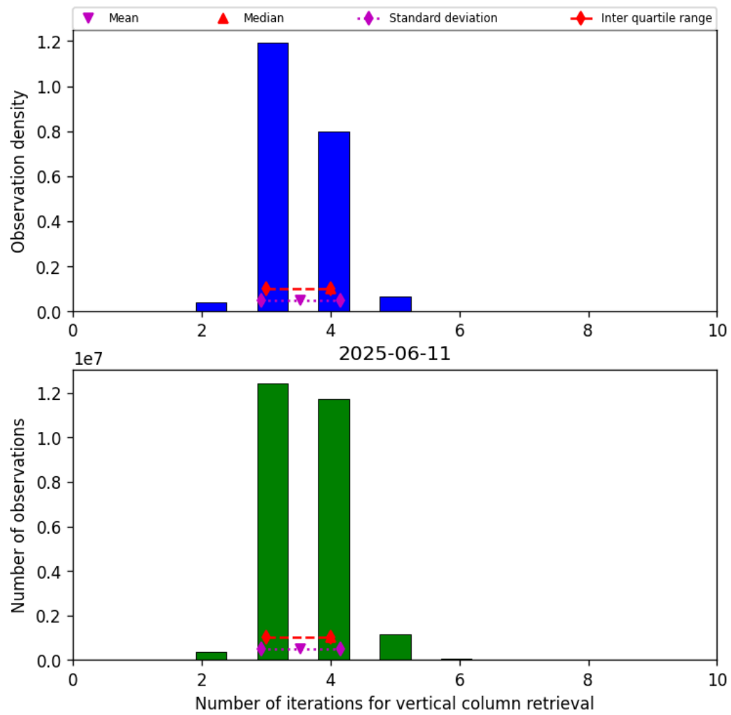
Figure 26: Histogram of “Number of iterations for vertical column retrieval” for 2025-06-11 to 2025-06-12
