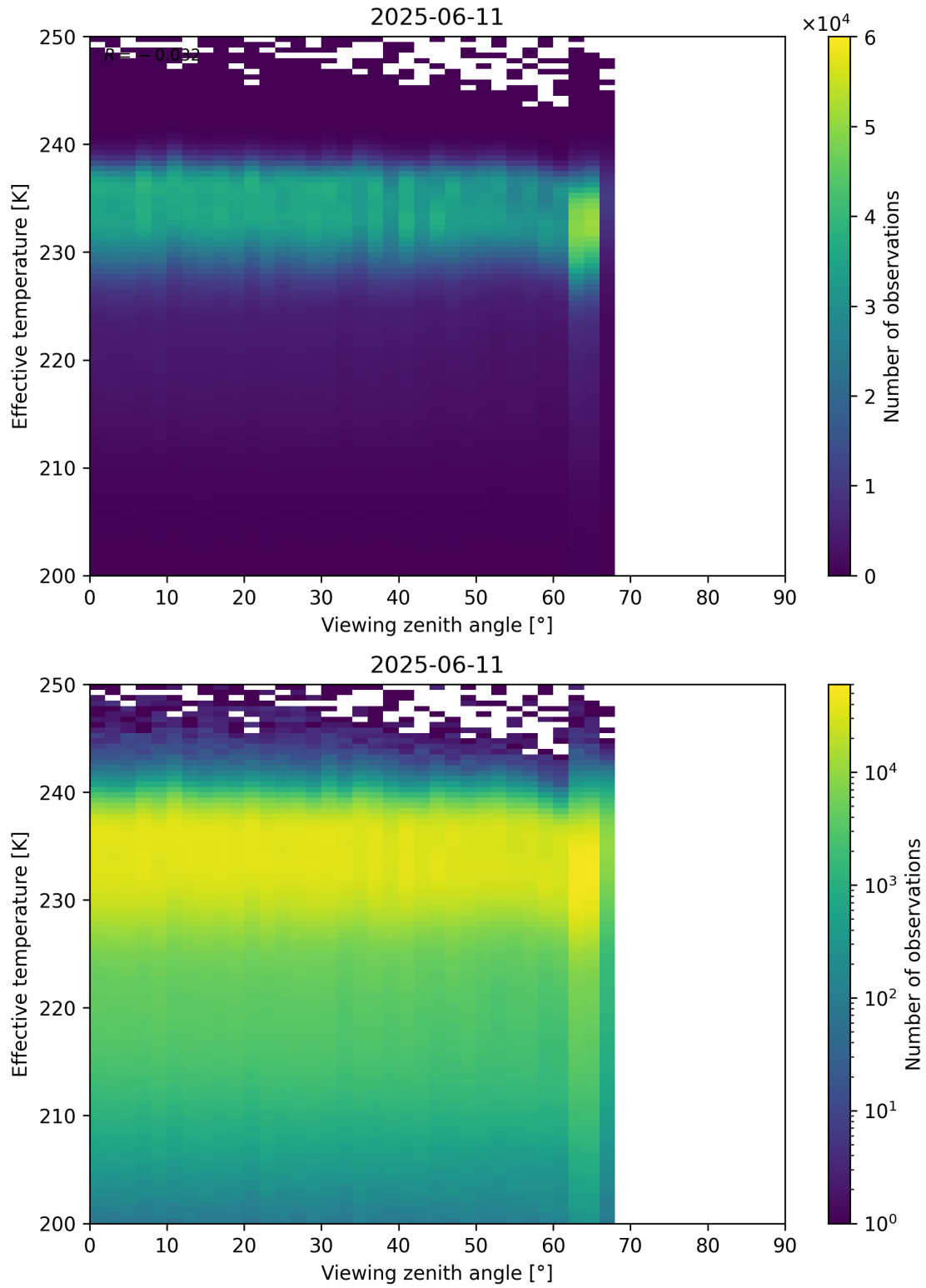
Figure 50: Scatter density plot of “Viewing zenith angle” against “Effective temperature” for 2025-06-11 to 2025-06-12.
