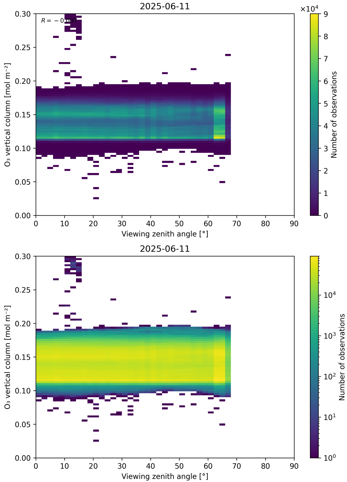
Figure 52: Scatter density plot of “Viewing zenith angle” against “O 3 vertical column” for 2025-06-11 to 2025-06-12.
