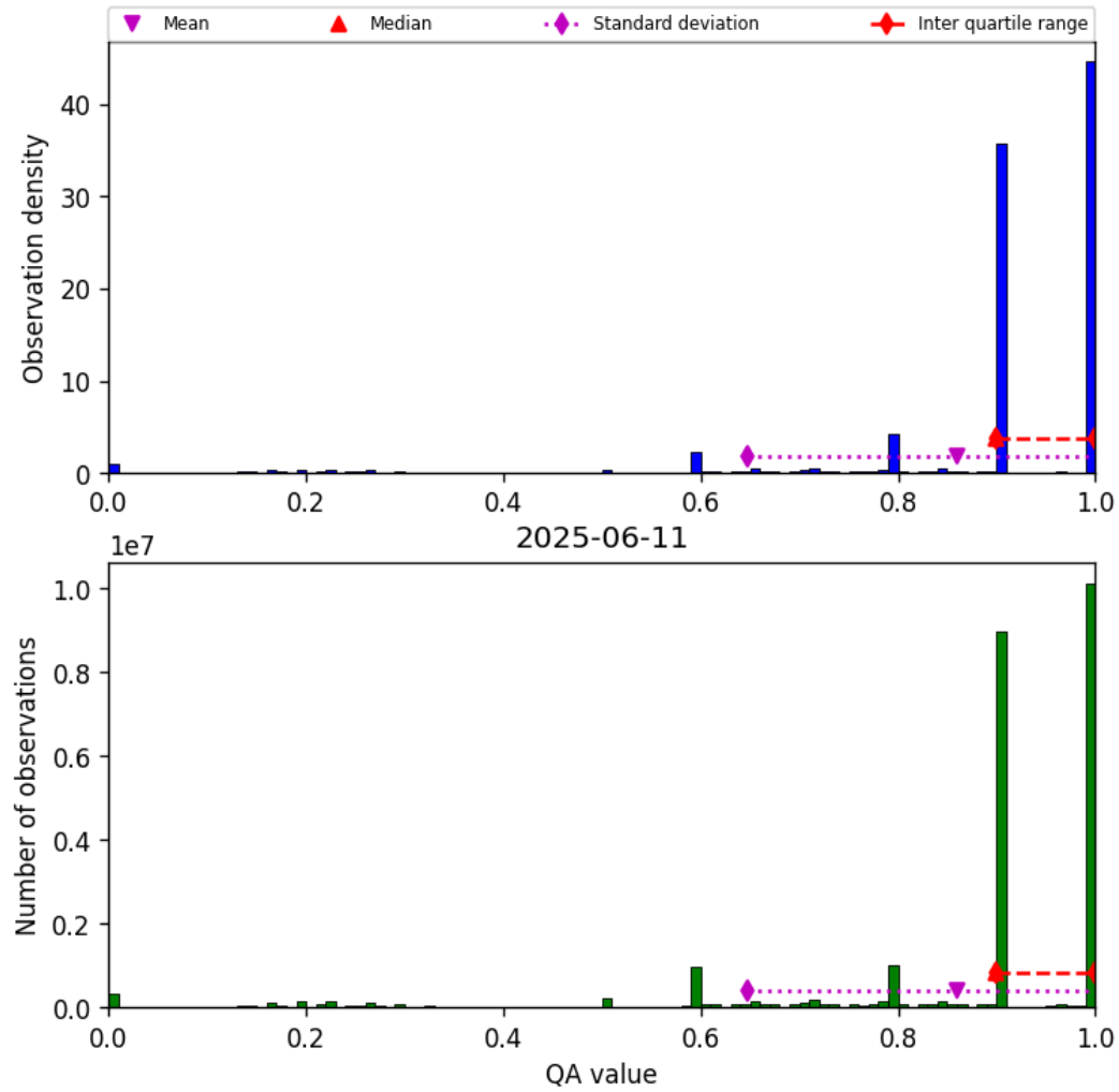
Figure 20: Histogram of “QA value” for 2025-06-11 to 2025-06-12
