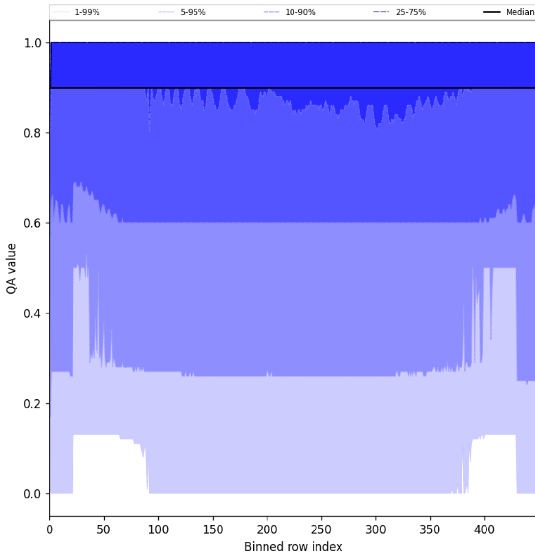
Figure 27: Along track statistics of “QA value” for 2025-06-11 to 2025-06-12
