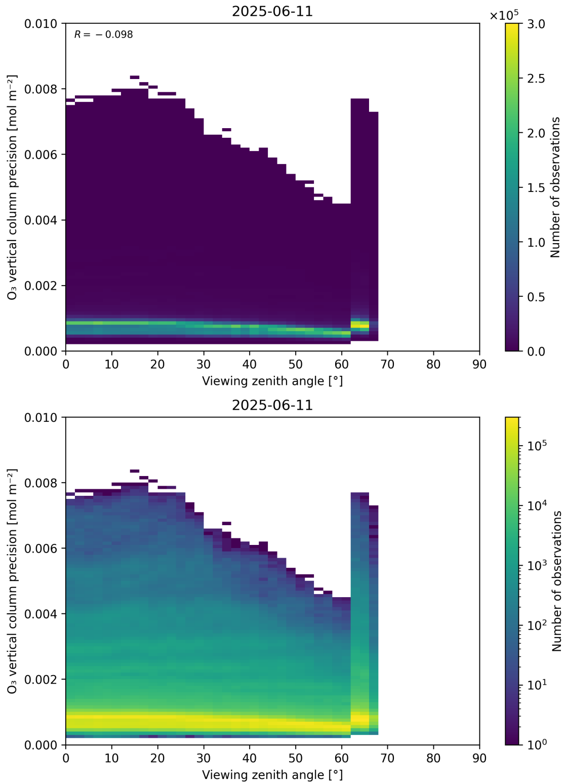
Figure 53: Scatter density plot of “Viewing zenith angle” against “O 3 vertical column precision” for 2025-06-11 to 2025-06-12.
