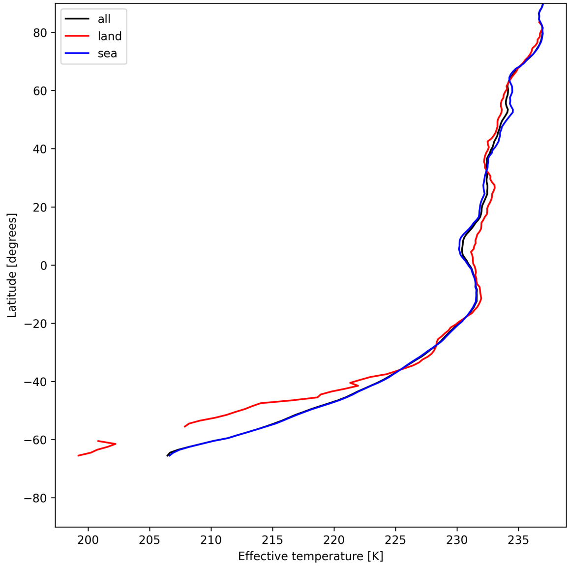
Figure 17: Zonal average of "Effective temperature" for 2025-06-11 to 2025-06-12.
