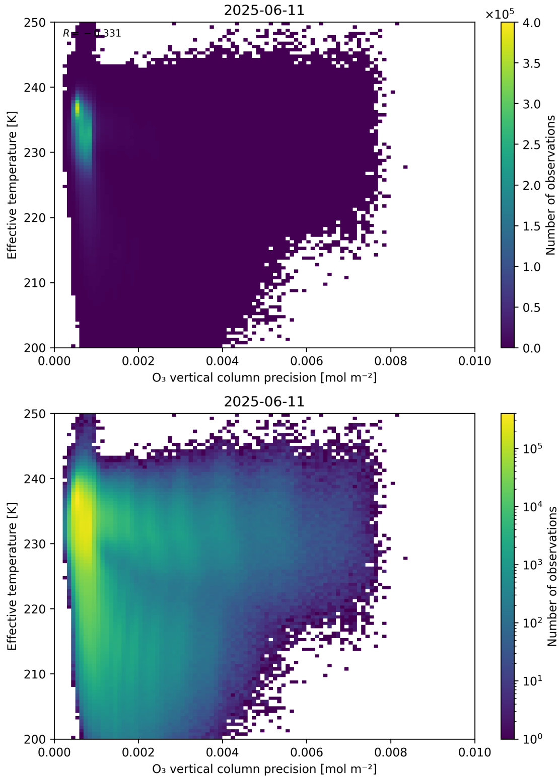
Figure 42: Scatter density plot of “O 3 vertical column precision” against “Effective temperature” for 2025-06-11 to 2025-06-12.
