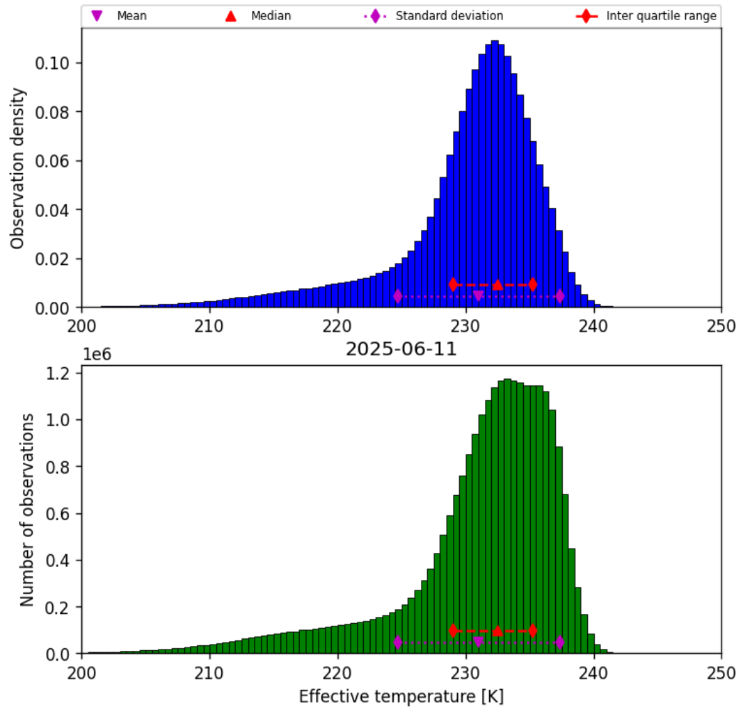
Figure 24: Histogram of “Effective temperature” for 2025-06-11 to 2025-06-12
