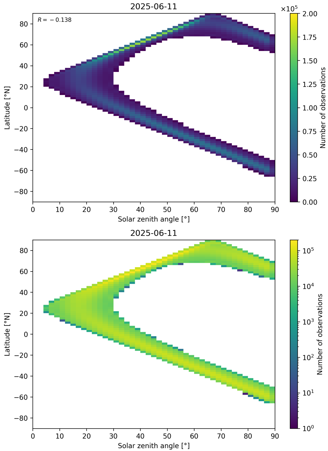
Figure 44: Scatter density plot of “Solar zenith angle” against “Latitude” for 2025-06-11 to 2025-06-12.
