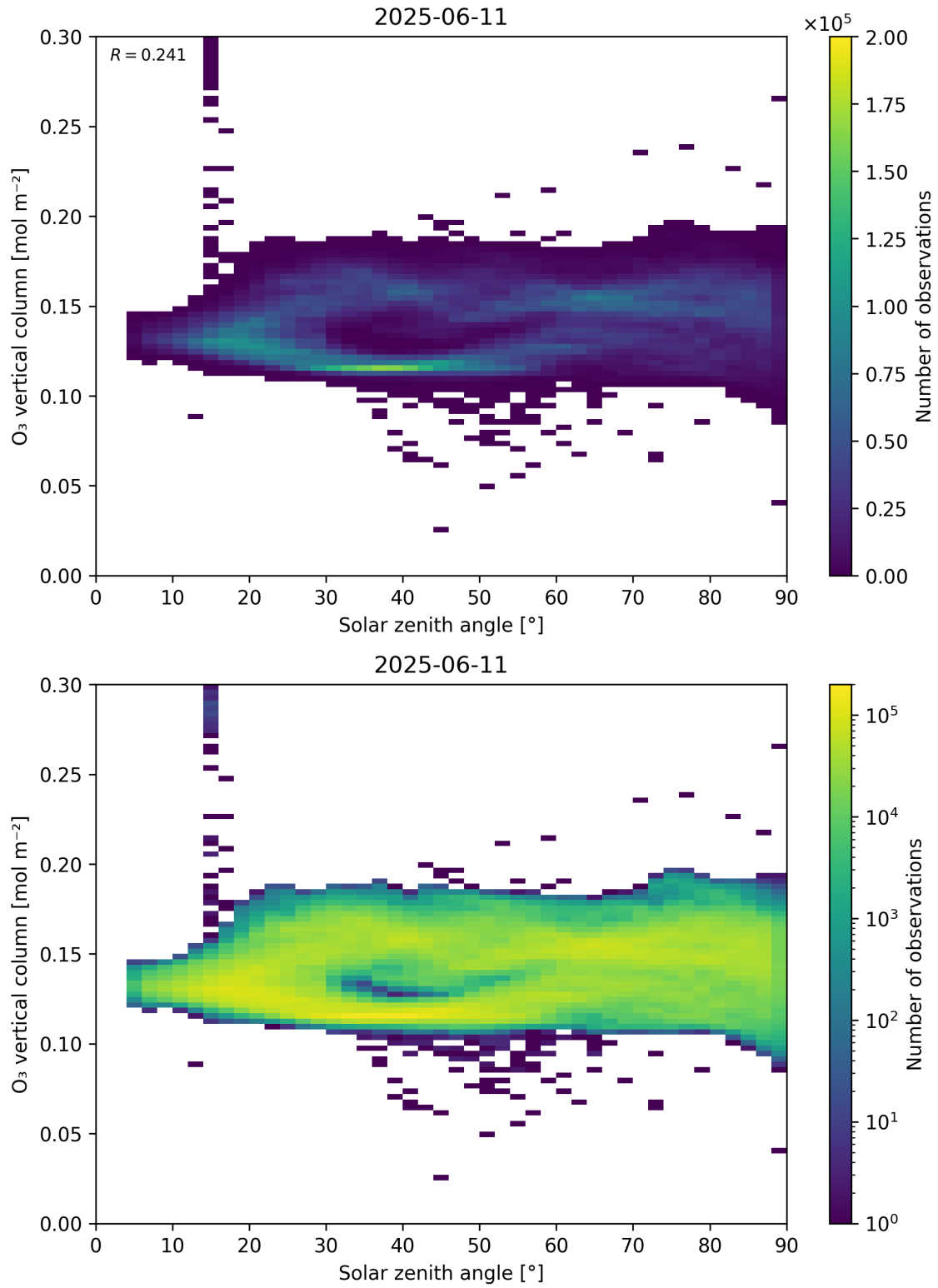
Figure 47: Scatter density plot of “Solar zenith angle” against “O 3 vertical column” for 2025-06-11 to 2025-06-12.
