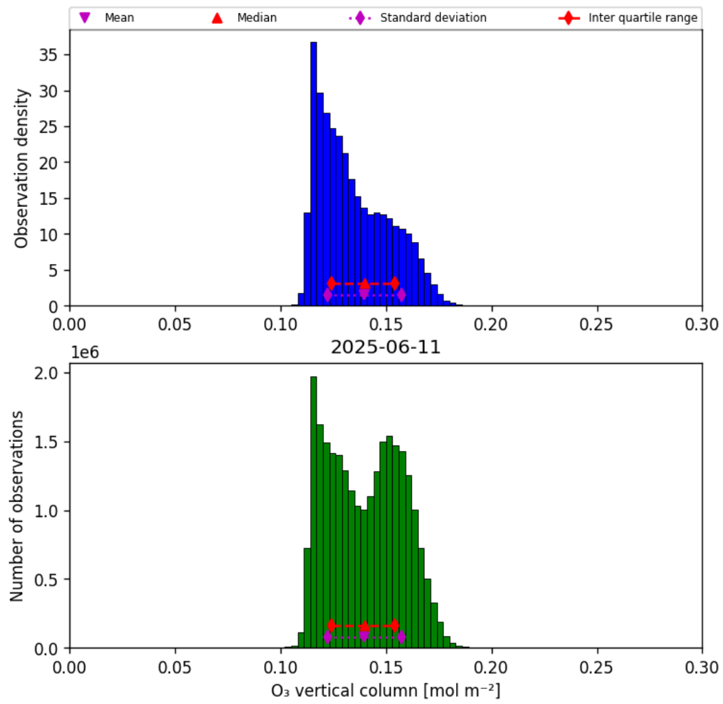
Figure 21: Histogram of “O 3 vertical column” for 2025-06-11 to 2025-06-12
