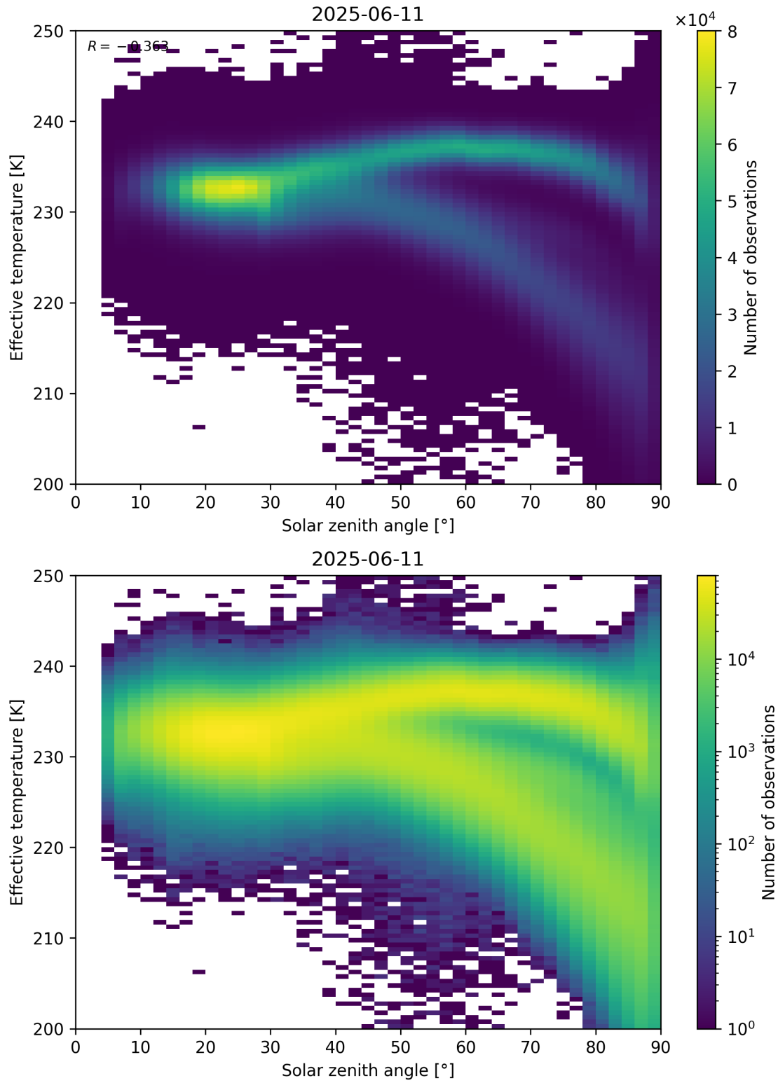
Figure 45: Scatter density plot of “Solar zenith angle” against “Effective temperature” for 2025-06-11 to 2025-06-12.
