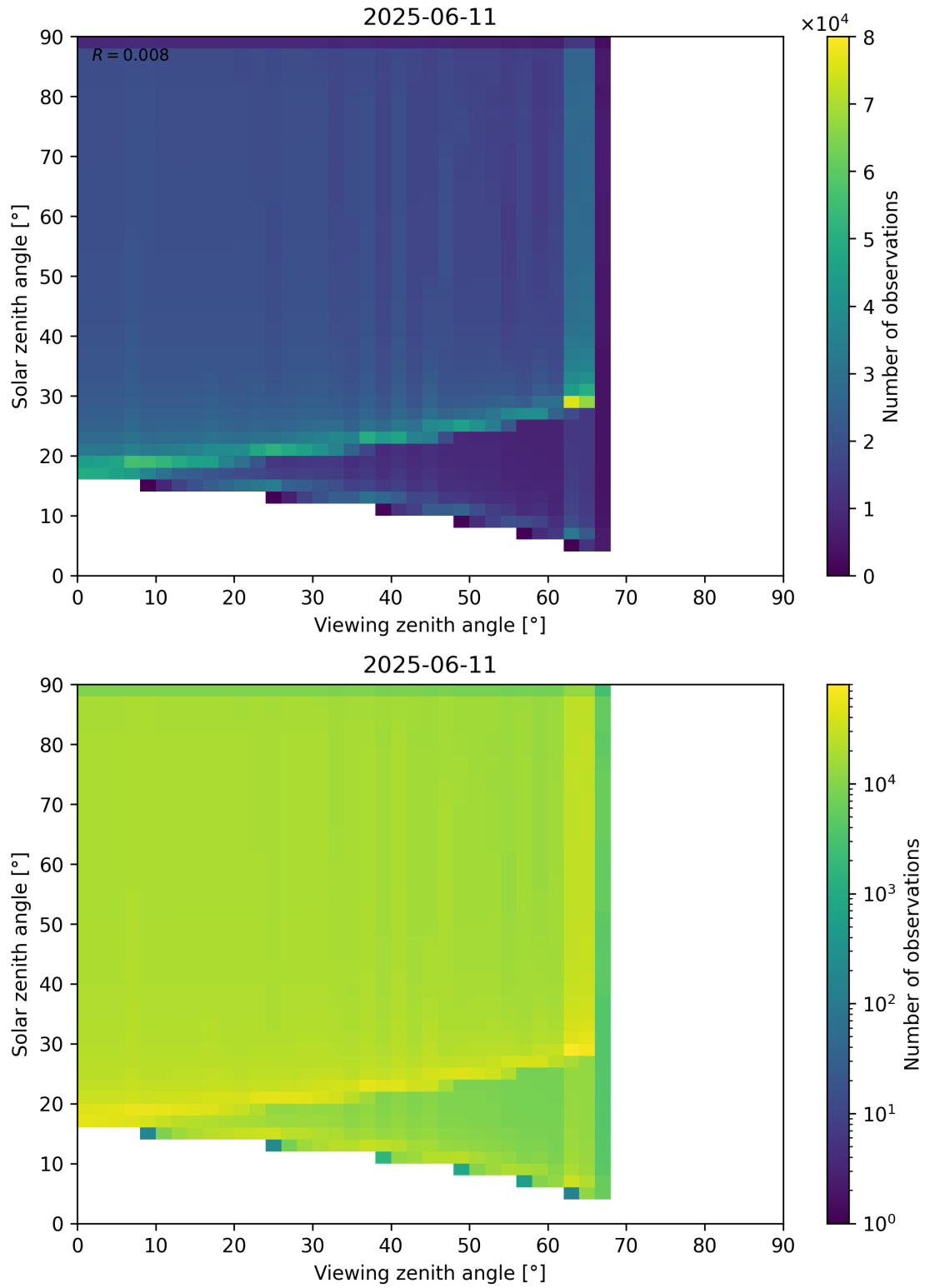
Figure 54: Scatter density plot of “Viewing zenith angle” against “Solar zenith angle” for 2025-06-11 to 2025-06-12.
