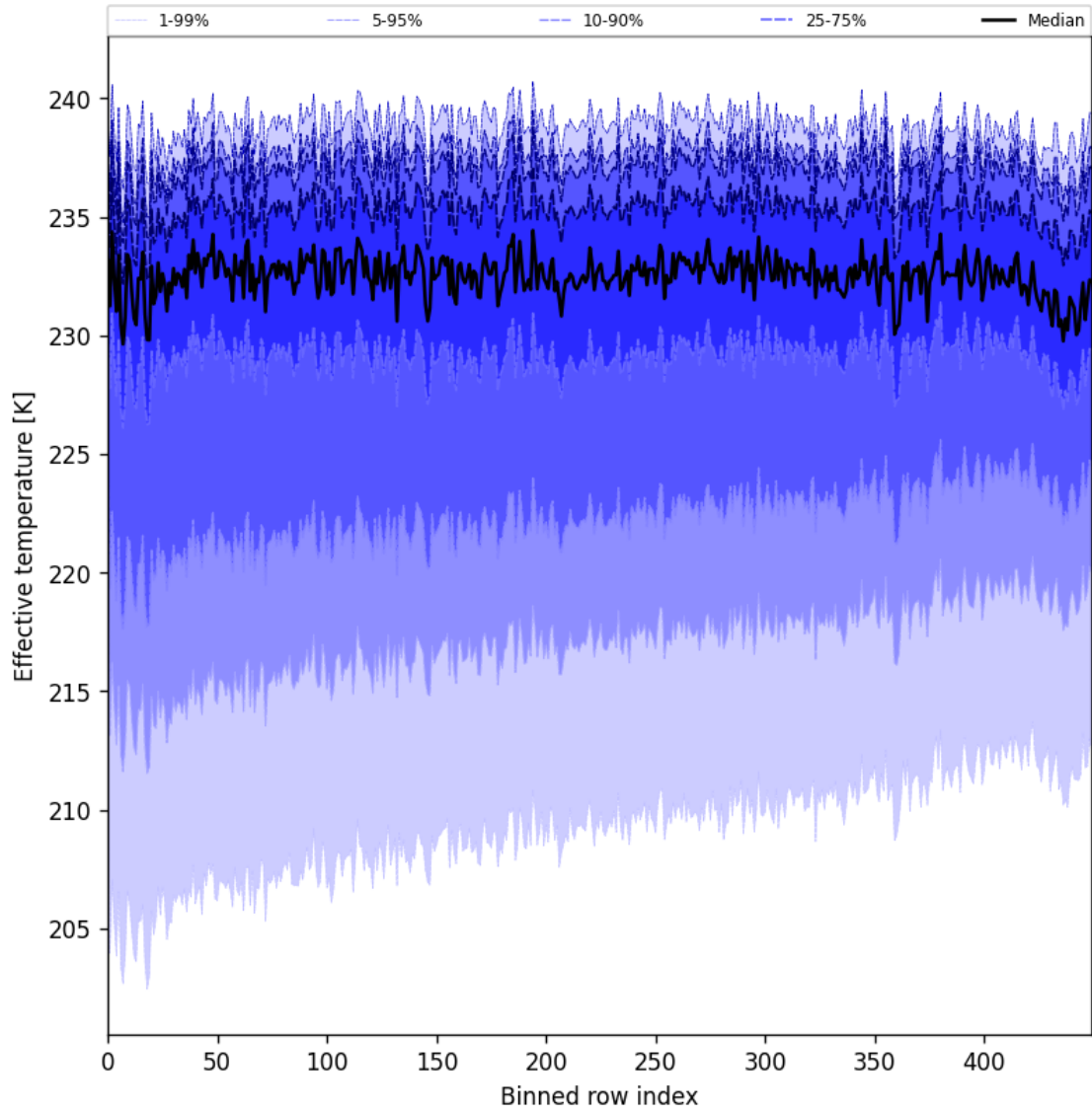
Figure 31: Along track statistics of “Effective temperature” for 2025-06-11 to 2025-06-12
