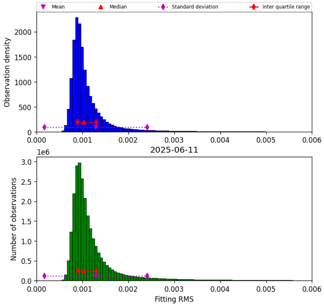
Figure 23: Histogram of “Fitting RMS” for 2025-06-11 to 2025-06-12
