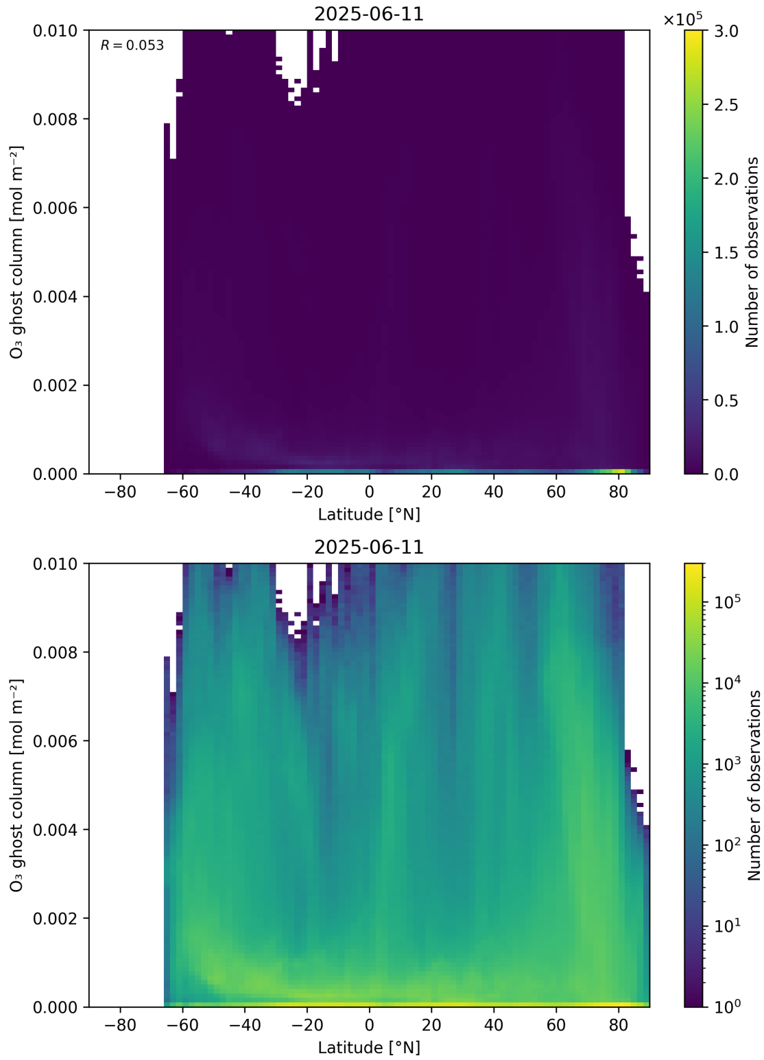
Figure 35: Scatter density plot of “Latitude” against “O 3 ghost column” for 2025-06-11 to 2025-06-12.
