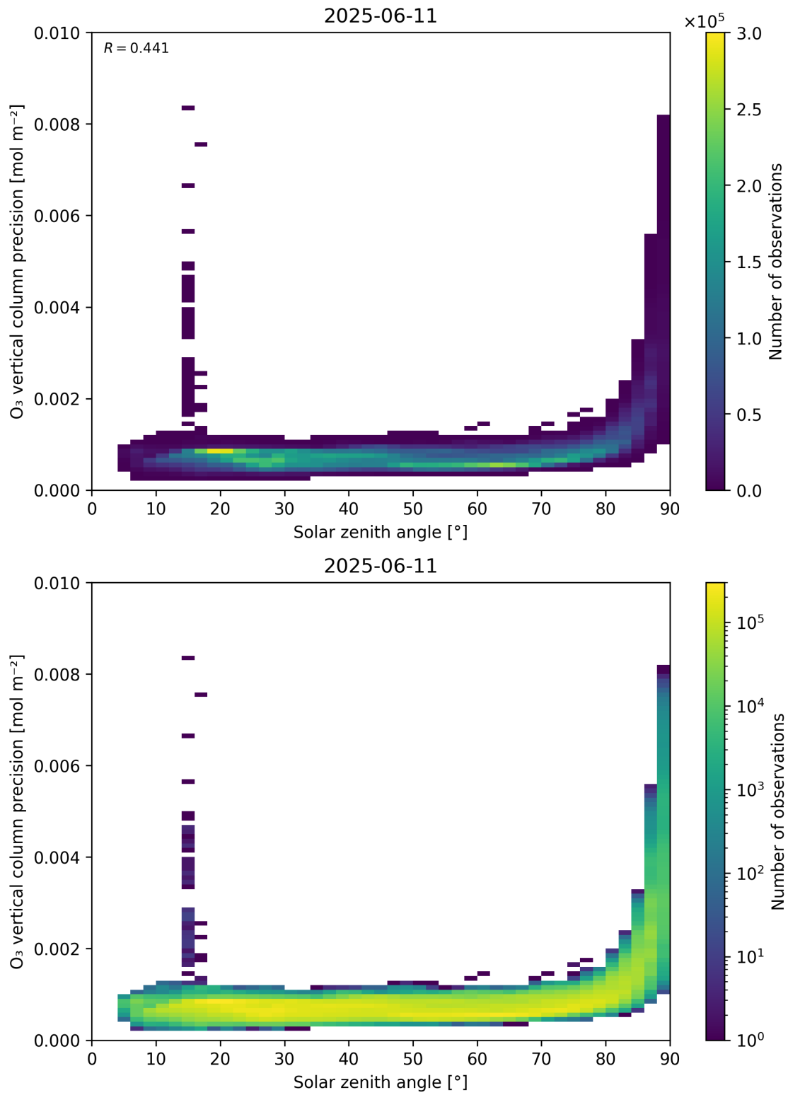
Figure 48: Scatter density plot of “Solar zenith angle” against “O 3 vertical column precision” for 2025-06-11 to 2025-06-12.
