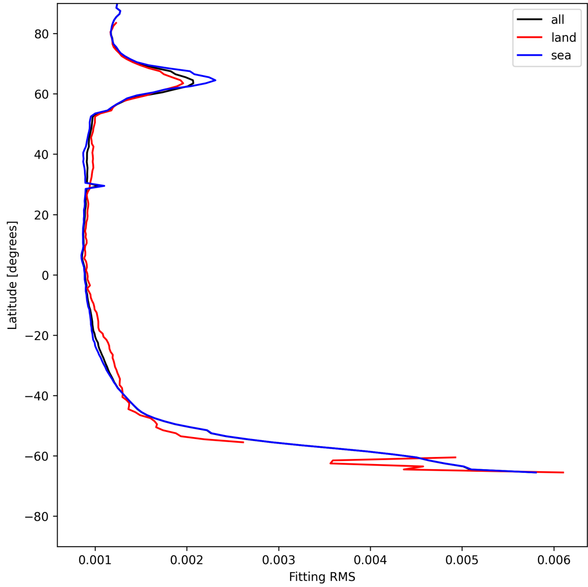
Figure 16: Zonal average of “Fitting RMS” for 2025-06-11 to 2025-06-12.
