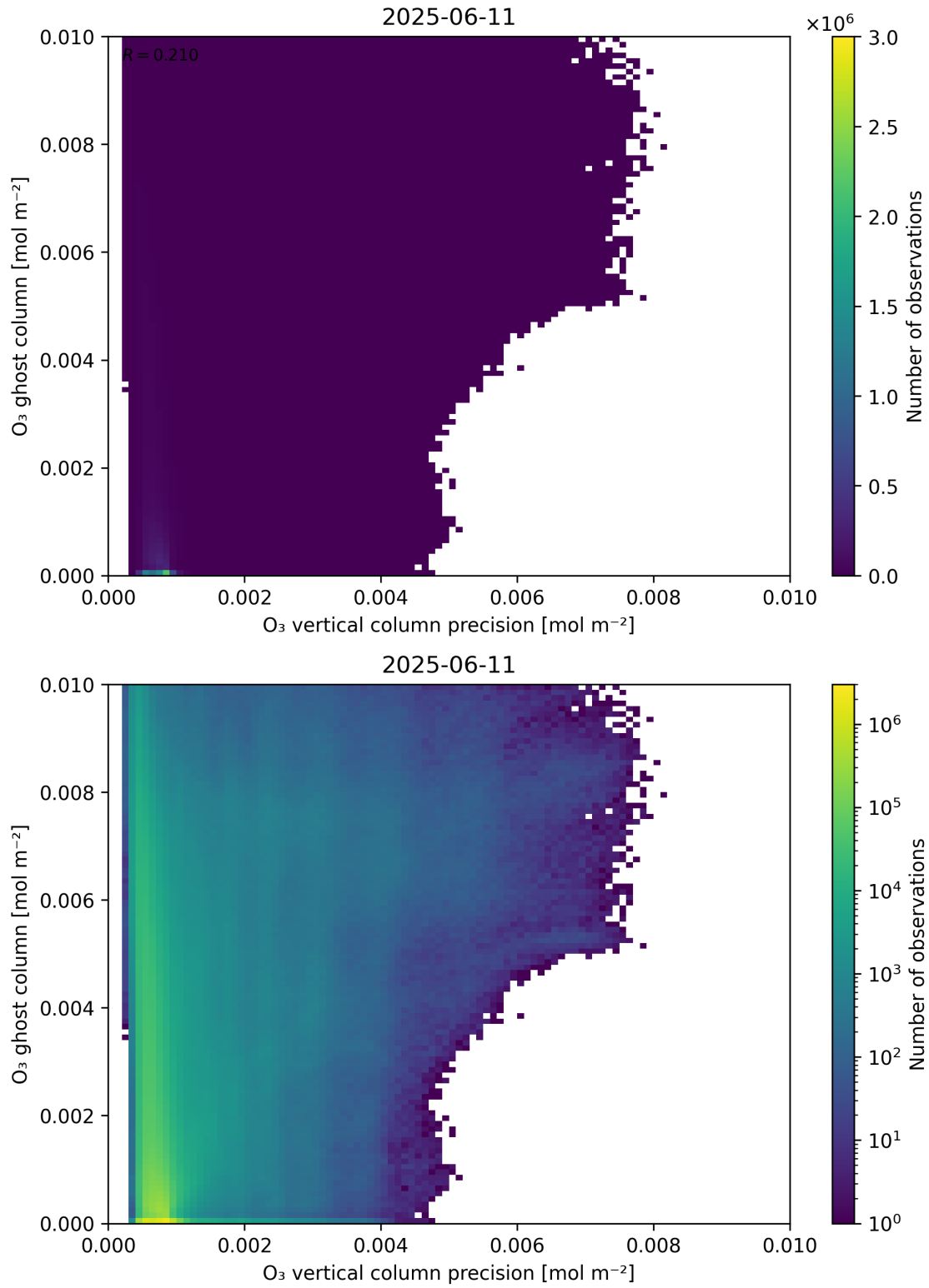
Figure 43: Scatter density plot of “ \text{O}_3 vertical column precision” against “ \text{O}_3 ghost column” for 2025-06-11 to 2025-06-12.
