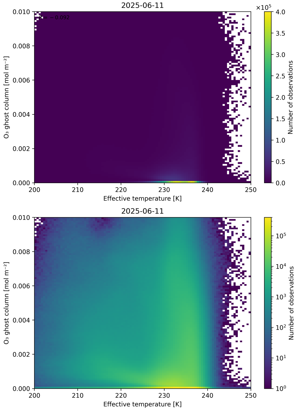
Figure 38: Scatter density plot of “Effective temperature” against “O 3 ghost column” for 2025-06-11 to 2025-06-12.
