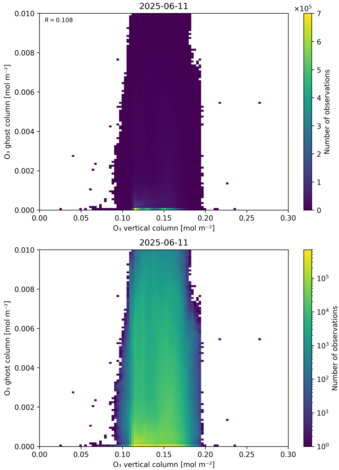
Figure 40: Scatter density plot of “O 3 vertical column” against “O 3 ghost column” for 2025-06-11 to 2025-06-12.
