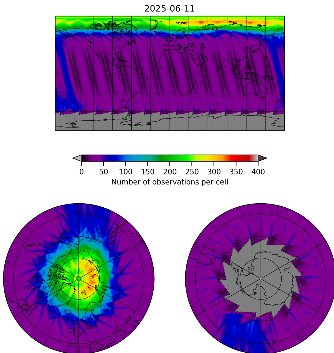
Figure 12: Map of the number of observations for 2025-06-11 to 2025-06-12
