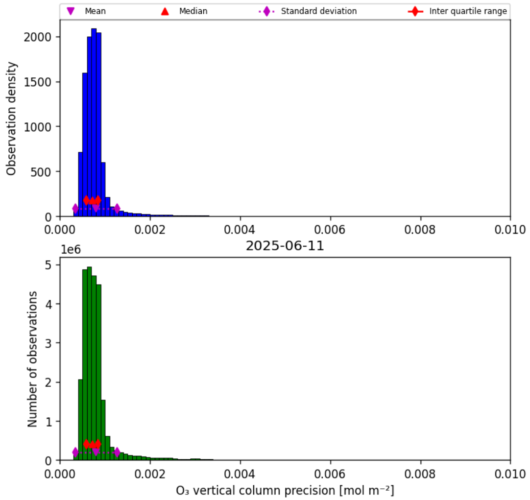
Figure 22: Histogram of “O 3 vertical column precision” for 2025-06-11 to 2025-06-12
