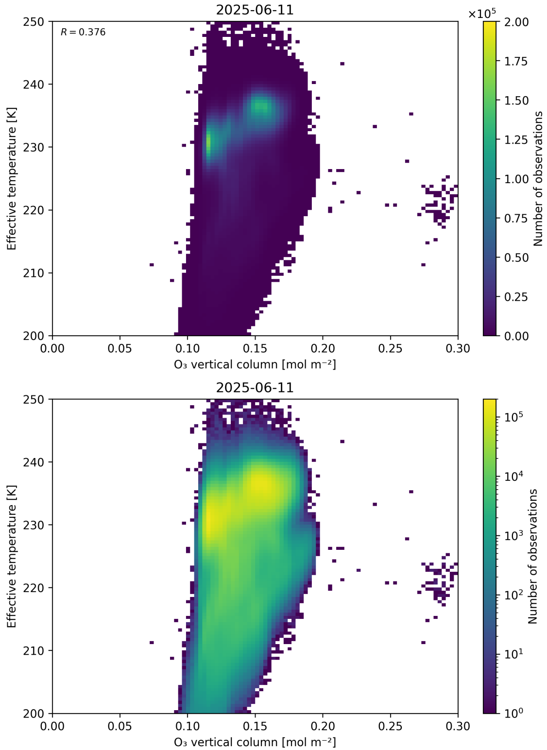
Figure 39: Scatter density plot of “O 3 vertical column” against “Effective temperature” for 2025-06-11 to 2025-06-12.
