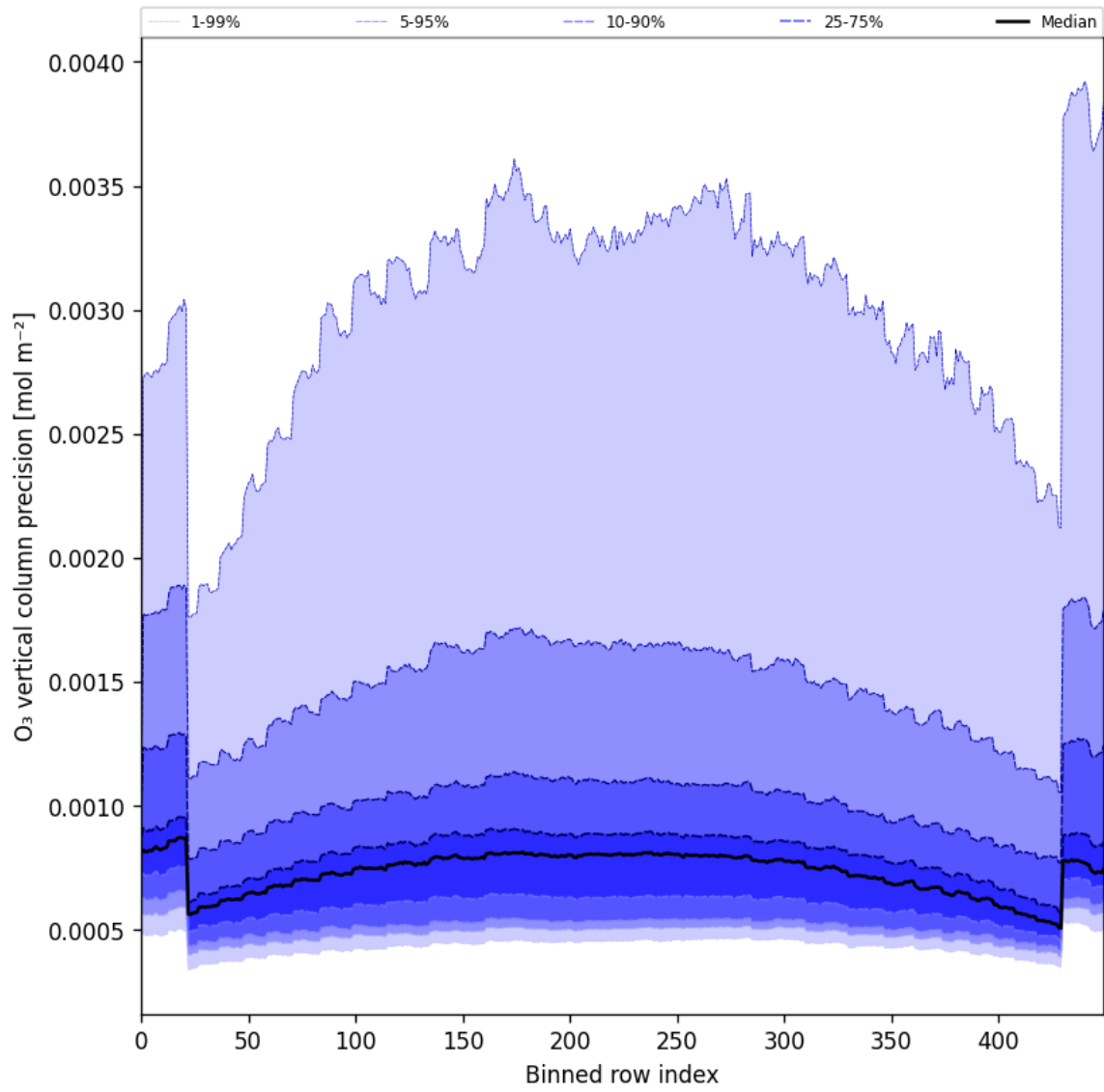
Figure 29: Along track statistics of “O 3 vertical column precision” for 2025-06-11 to 2025-06-12
