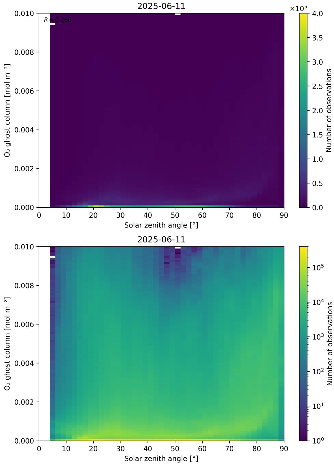
Figure 46: Scatter density plot of “Solar zenith angle” against “O 3 ghost column” for 2025-06-11 to 2025-06-12.
