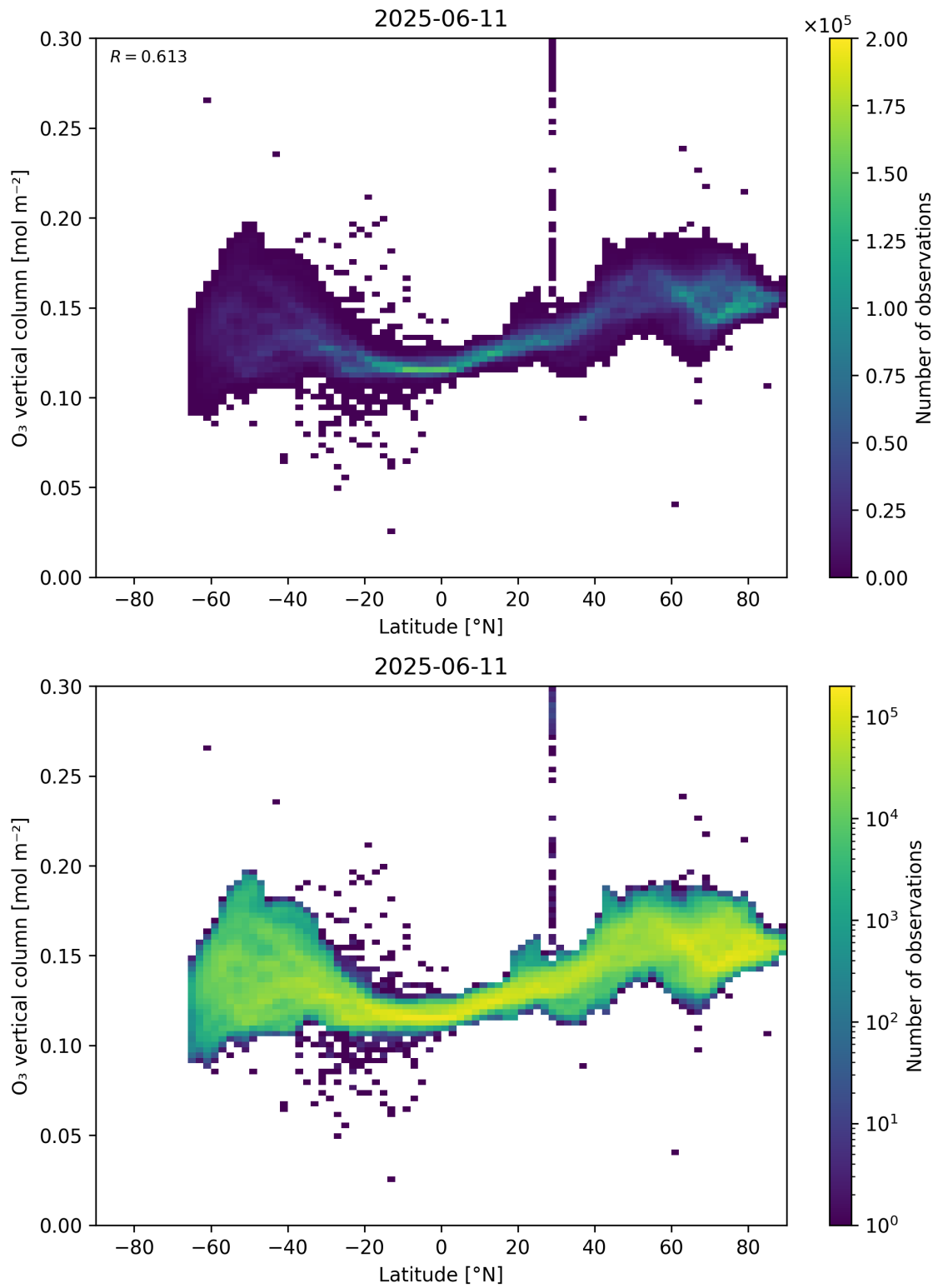
Figure 36: Scatter density plot of “Latitude” against “O 3 vertical column” for 2025-06-11 to 2025-06-12.
