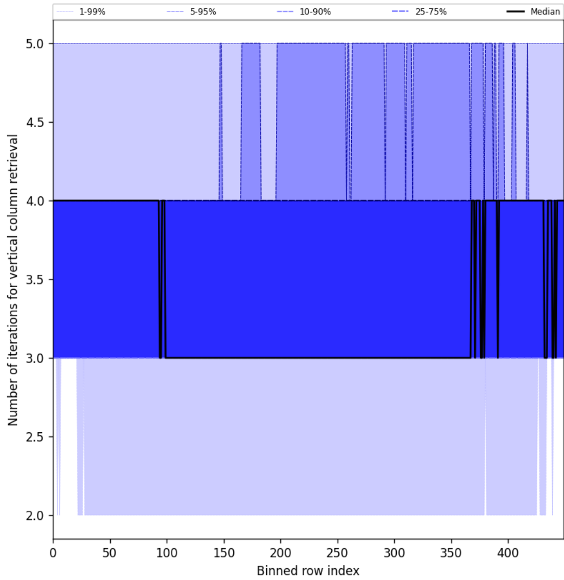
Figure 33: Along track statistics of “Number of iterations for vertical column retrieval” for 2025-06-11 to 2025-06-12
