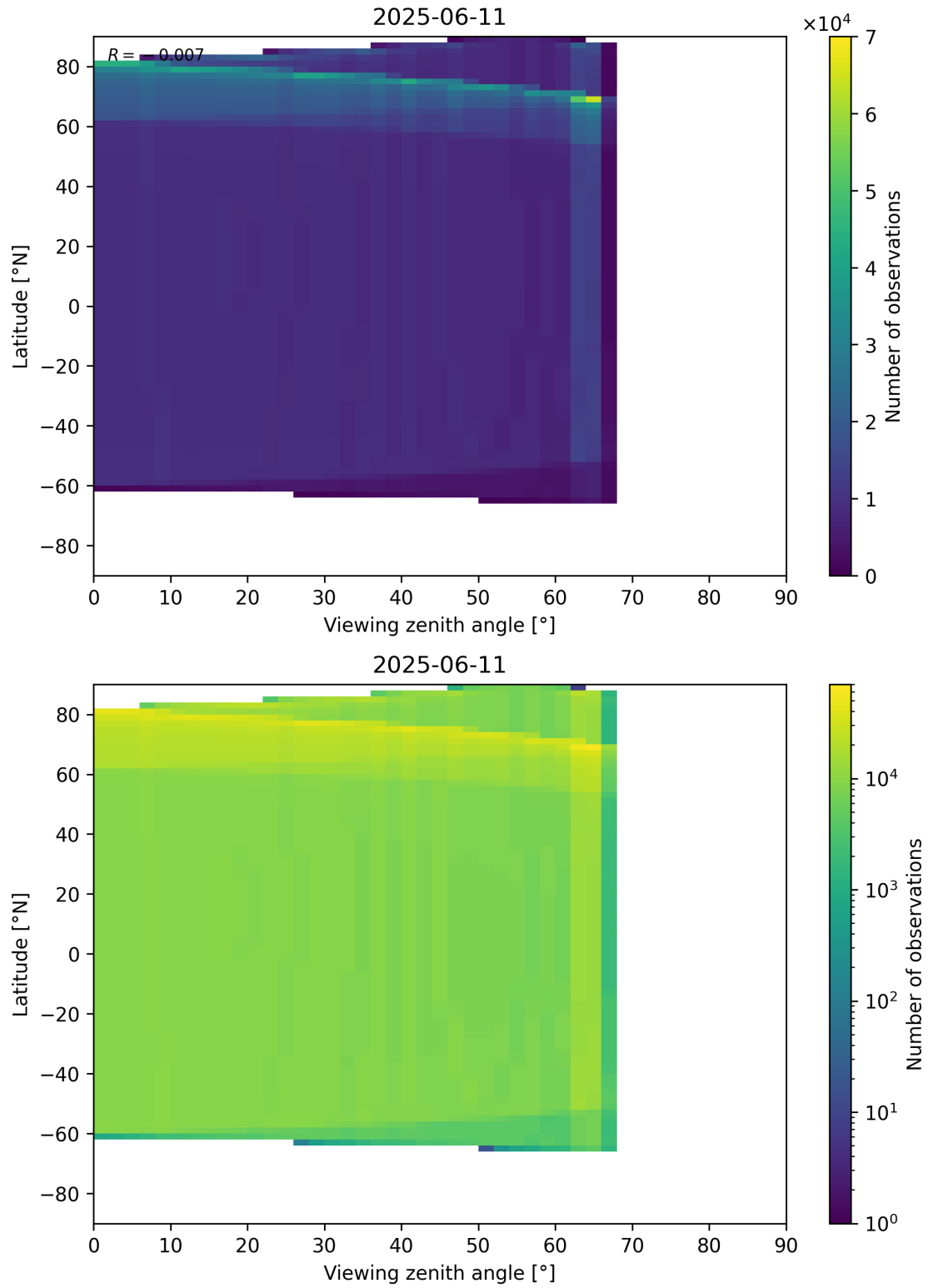
Figure 49: Scatter density plot of “Viewing zenith angle” against “Latitude” for 2025-06-11 to 2025-06-12.
