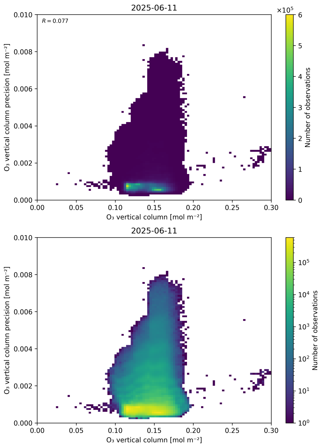
Figure 41: Scatter density plot of “O 3 vertical column” against “O 3 vertical column precision” for 2025-06-11 to 2025-06-12.
