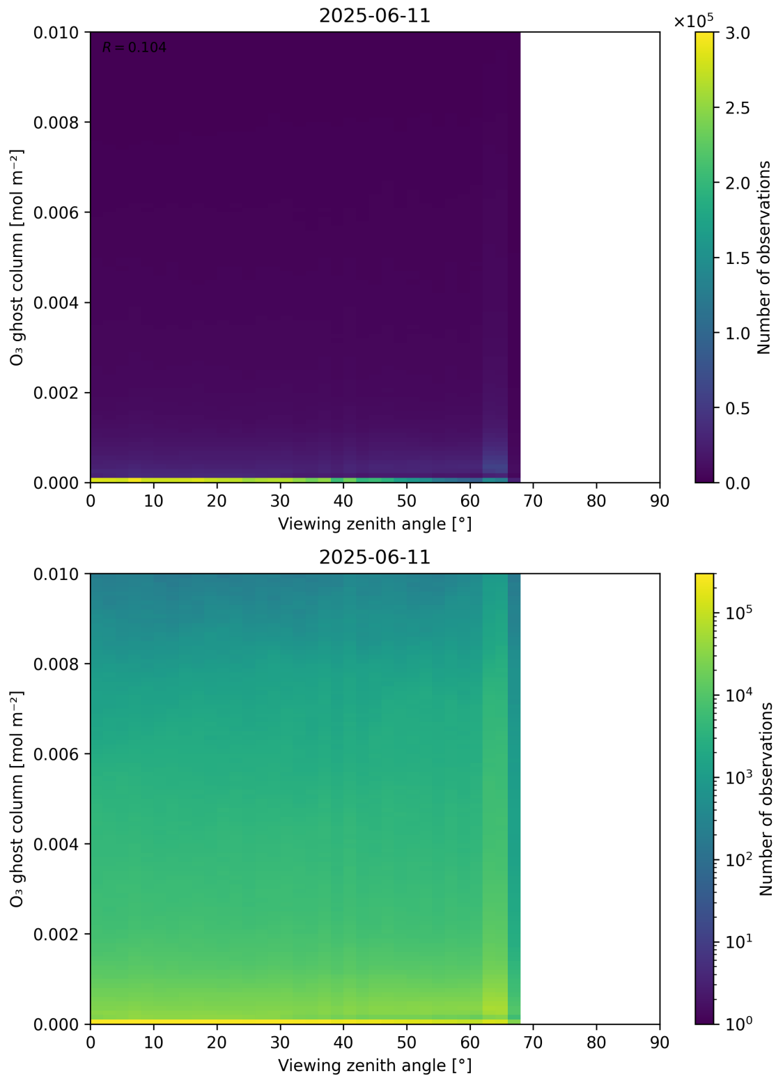
Figure 51: Scatter density plot of “Viewing zenith angle” against “O 3 ghost column” for 2025-06-11 to 2025-06-12.
