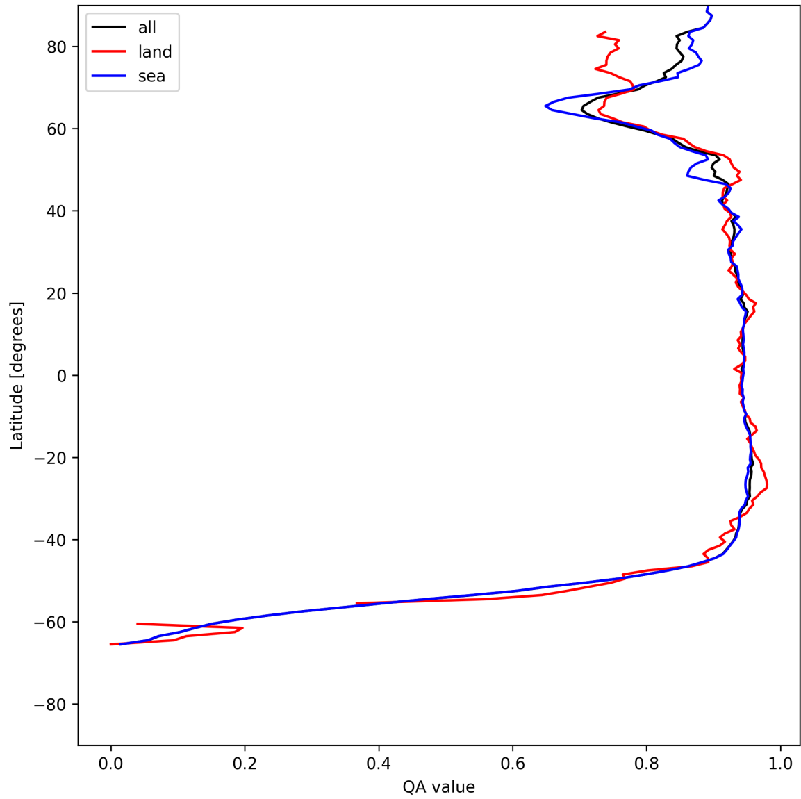
Figure 13: Zonal average of “QA value” for 2025-06-11 to 2025-06-12.
