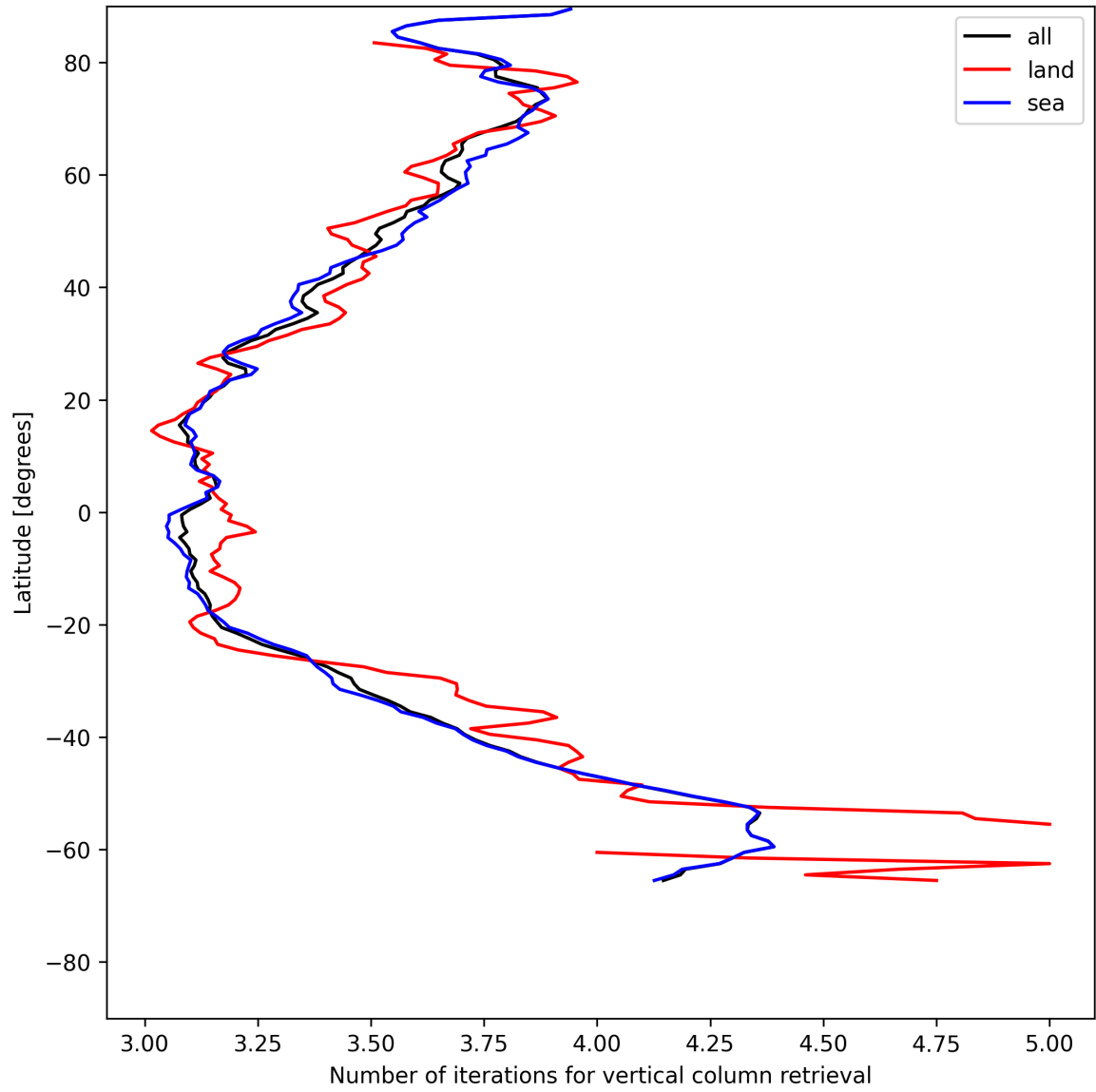
Figure 19: Zonal average of “Number of iterations for vertical column retrieval” for 2025-06-11 to 2025-06-12.
