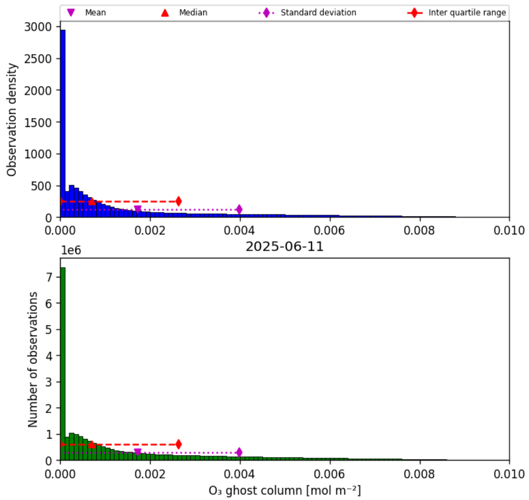
Figure 25: Histogram of “O 3 ghost column” for 2025-06-11 to 2025-06-12
