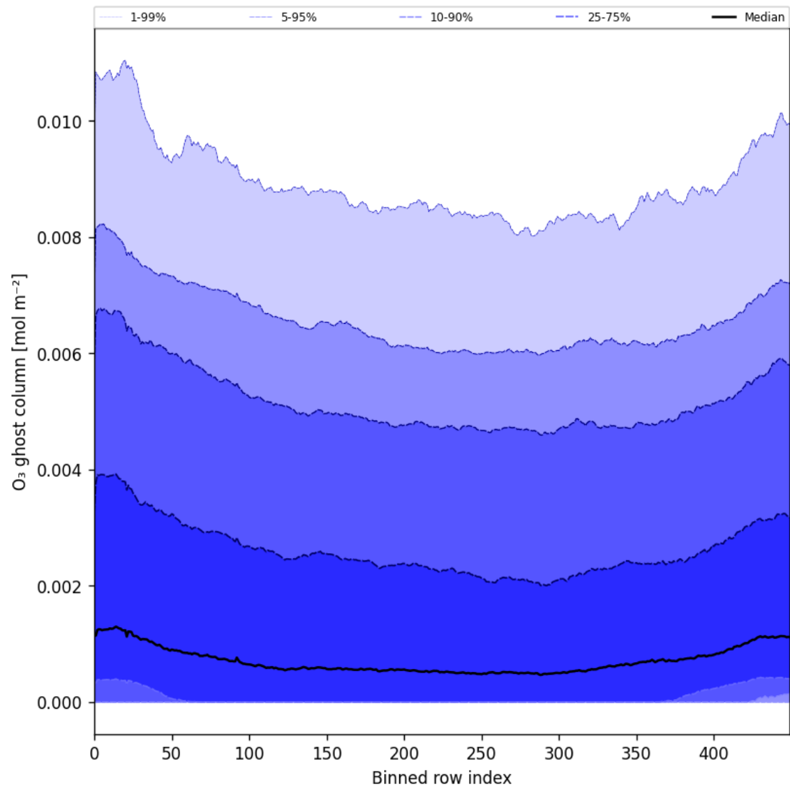
Figure 32: Along track statistics of “O 3 ghost column” for 2025-06-11 to 2025-06-12
