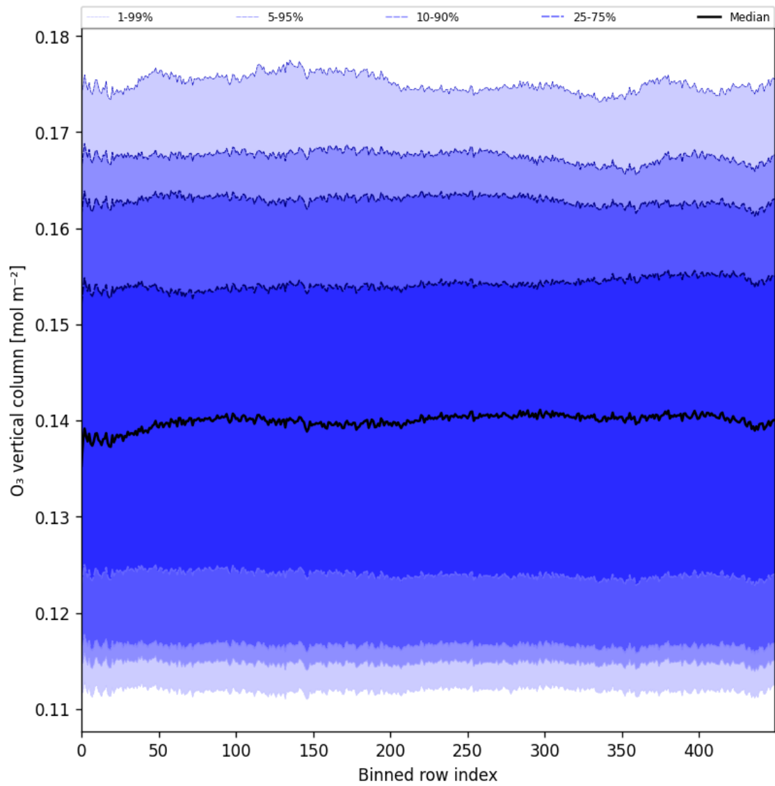
Figure 28: Along track statistics of “O 3 vertical column” for 2025-06-11 to 2025-06-12
