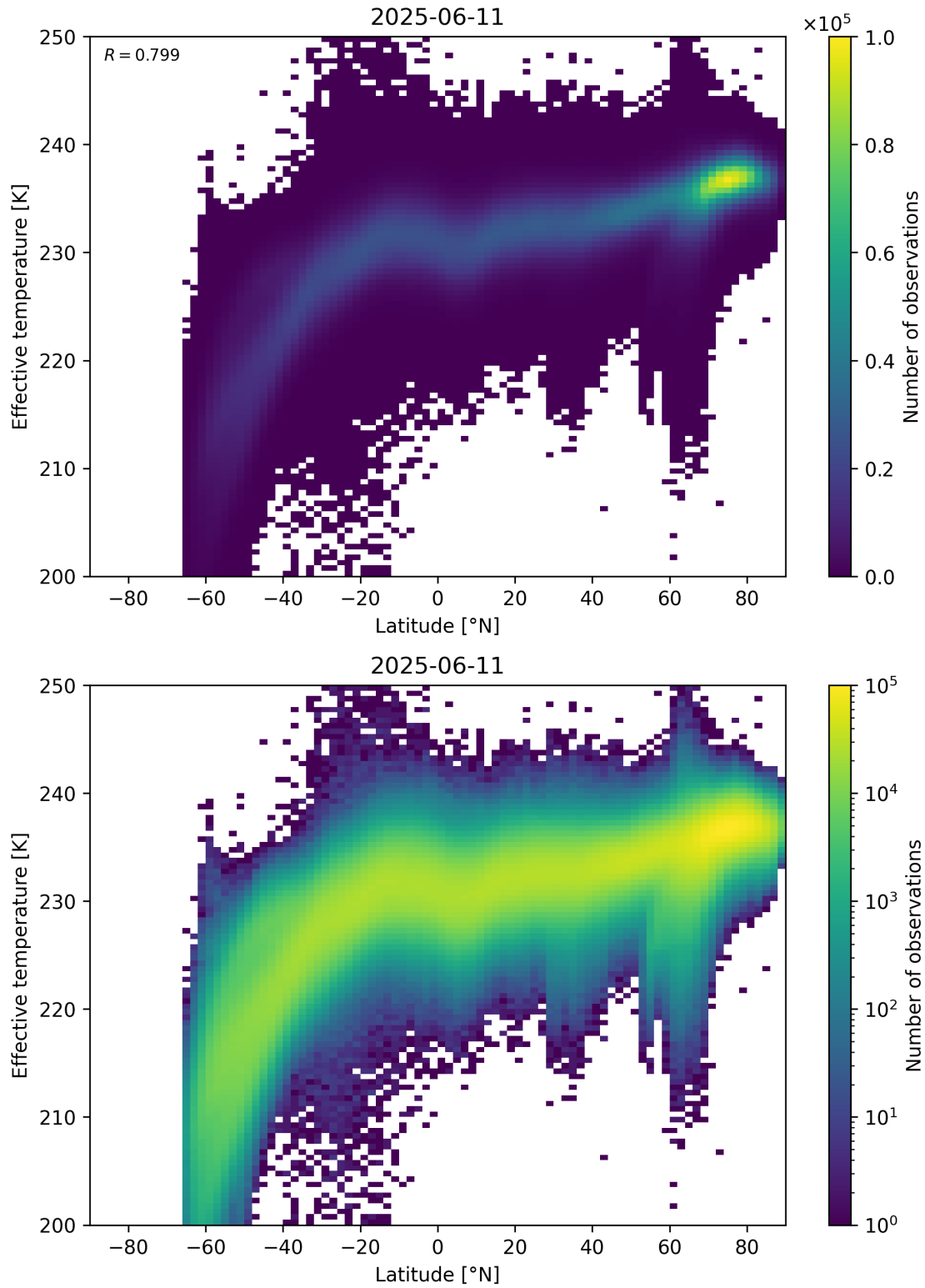
Figure 34: Scatter density plot of “Latitude” against “Effective temperature” for 2025-06-11 to 2025-06-12.
