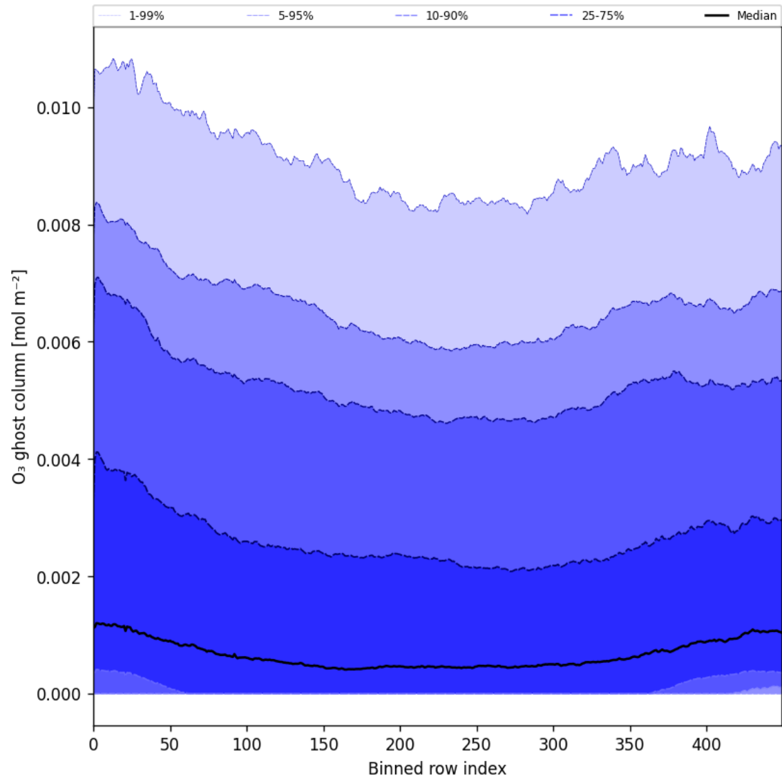
Figure 32: Along track statistics of “O 3 ghost column” for 2025-06-12 to 2025-06-14
