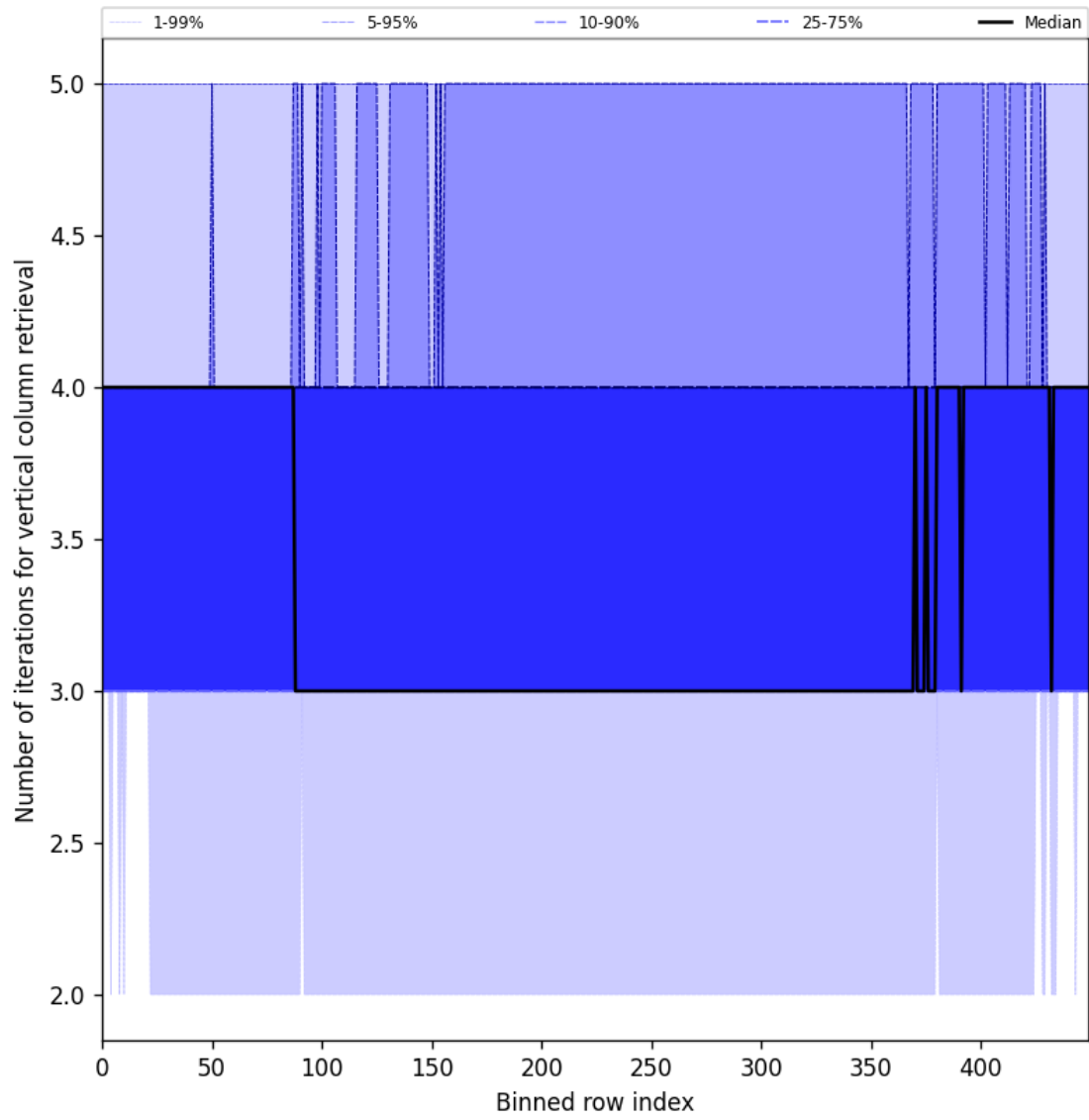
Figure 33: Along track statistics of “Number of iterations for vertical column retrieval” for 2025-06-12 to 2025-06-14
