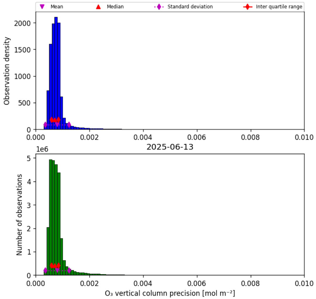
Figure 22: Histogram of “O 3 vertical column precision” for 2025-06-12 to 2025-06-14
