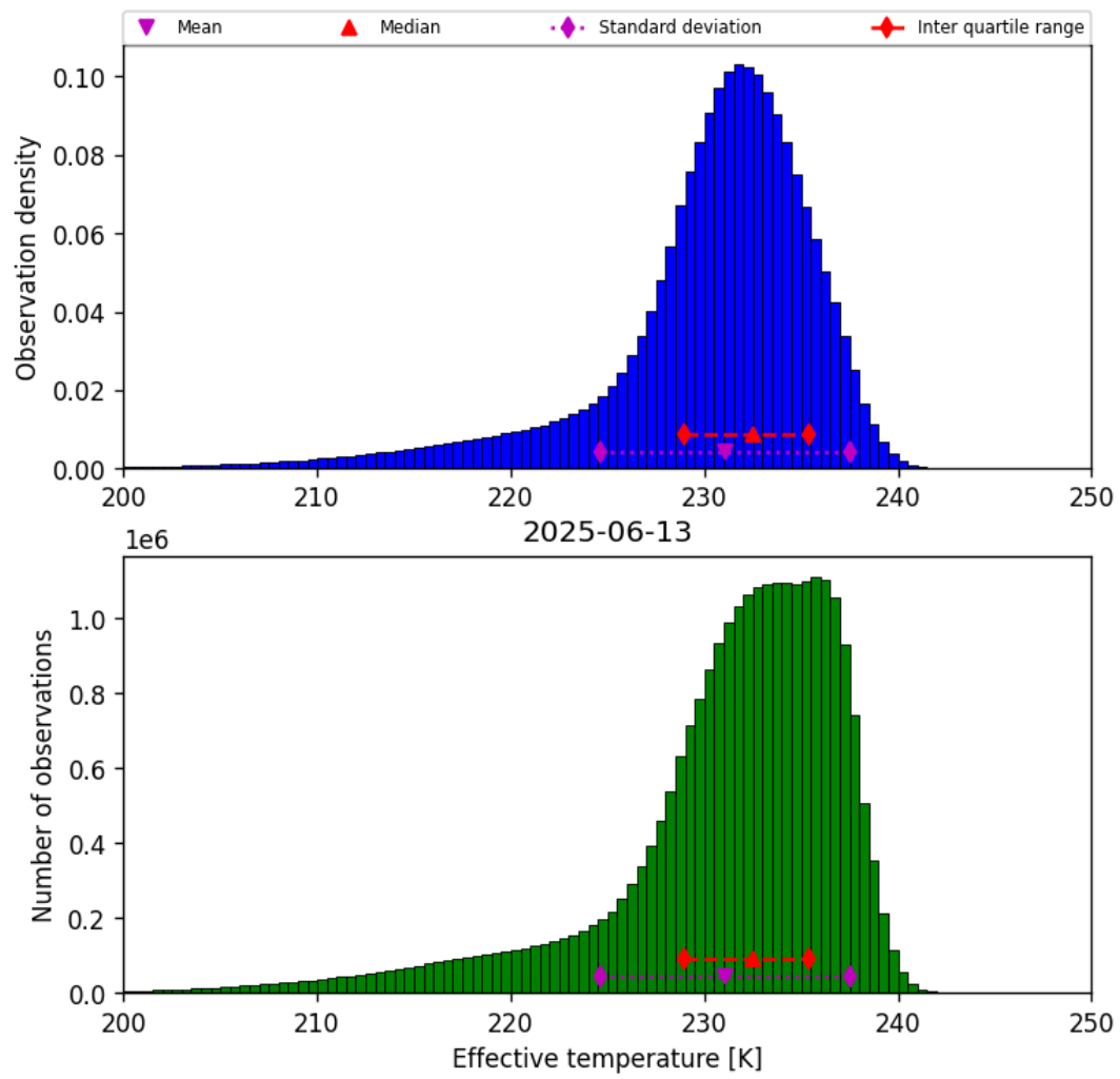
Figure 24: Histogram of “Effective temperature” for 2025-06-12 to 2025-06-14
