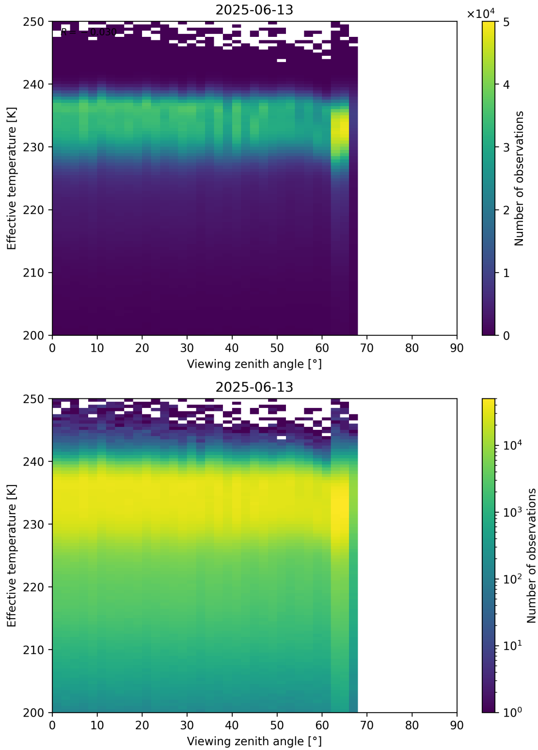
Figure 50: Scatter density plot of “Viewing zenith angle” against “Effective temperature” for 2025-06-12 to 2025-06-14.
