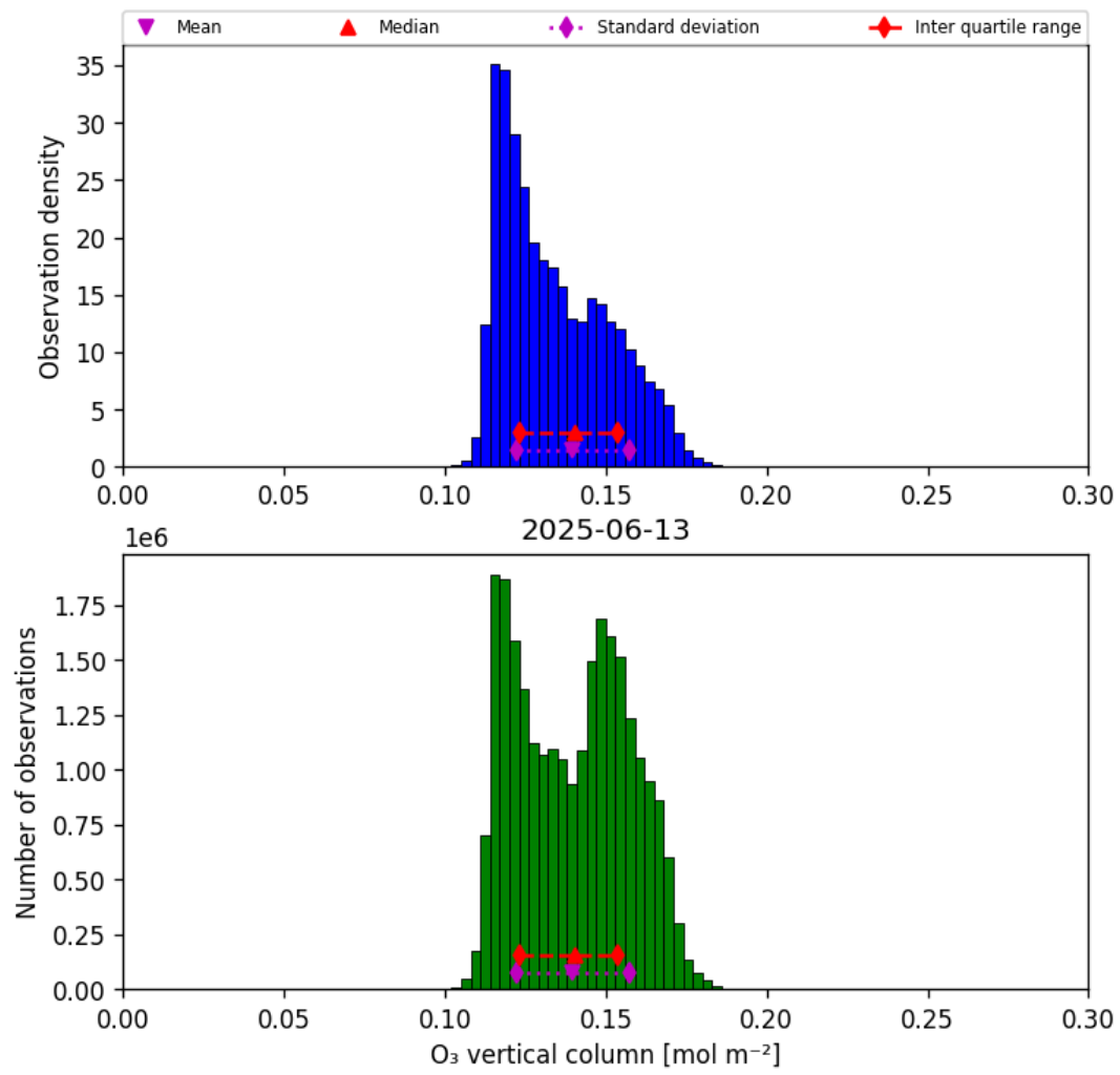
Figure 21: Histogram of “O 3 vertical column” for 2025-06-12 to 2025-06-14
