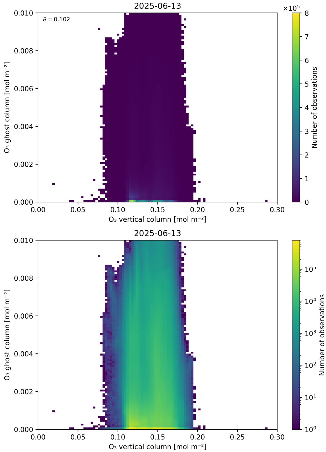
Figure 40: Scatter density plot of “O 3 vertical column” against “O 3 ghost column” for 2025-06-12 to 2025-06-14.
