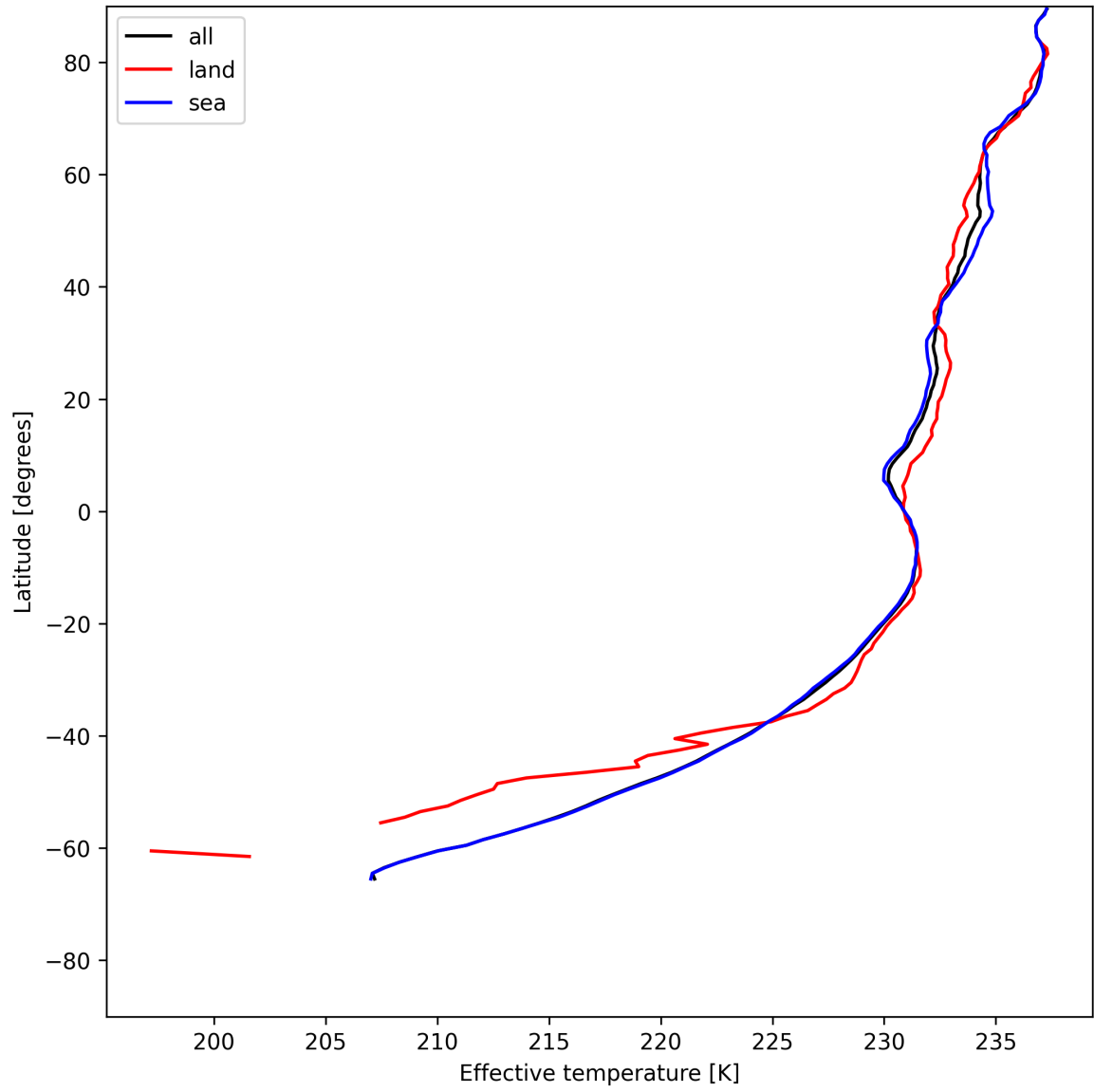
Figure 17: Zonal average of "Effective temperature" for 2025-06-12 to 2025-06-14.
