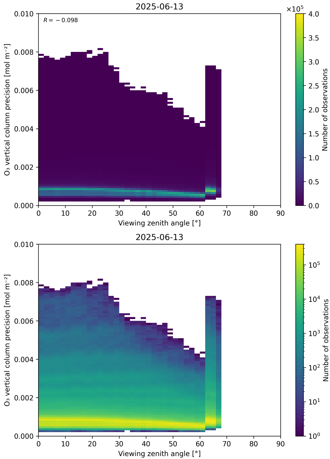
Figure 53: Scatter density plot of “Viewing zenith angle” against “O 3 vertical column precision” for 2025-06-12 to 2025-06-14.
