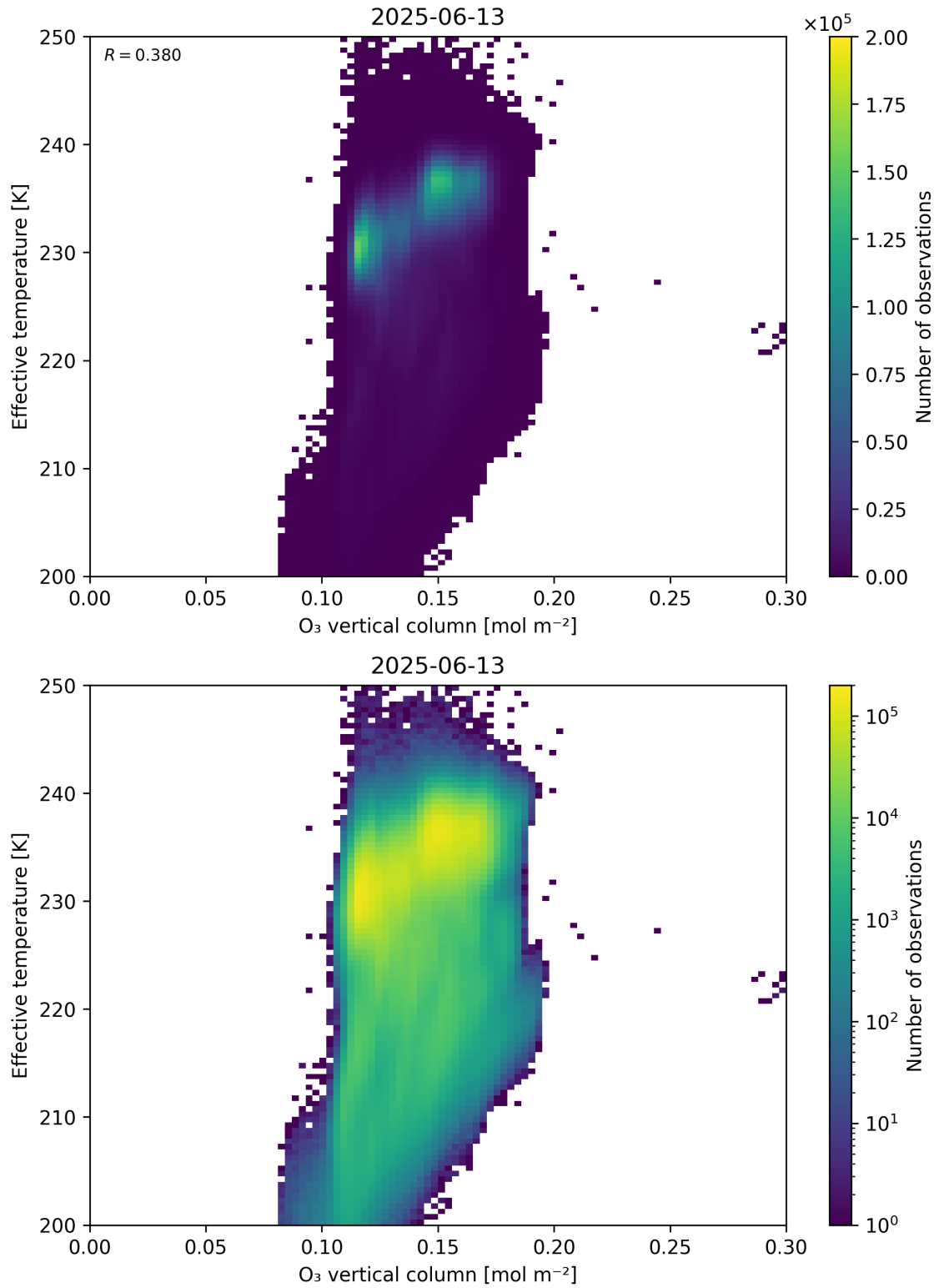
Figure 39: Scatter density plot of “O 3 vertical column” against “Effective temperature” for 2025-06-12 to 2025-06-14.
