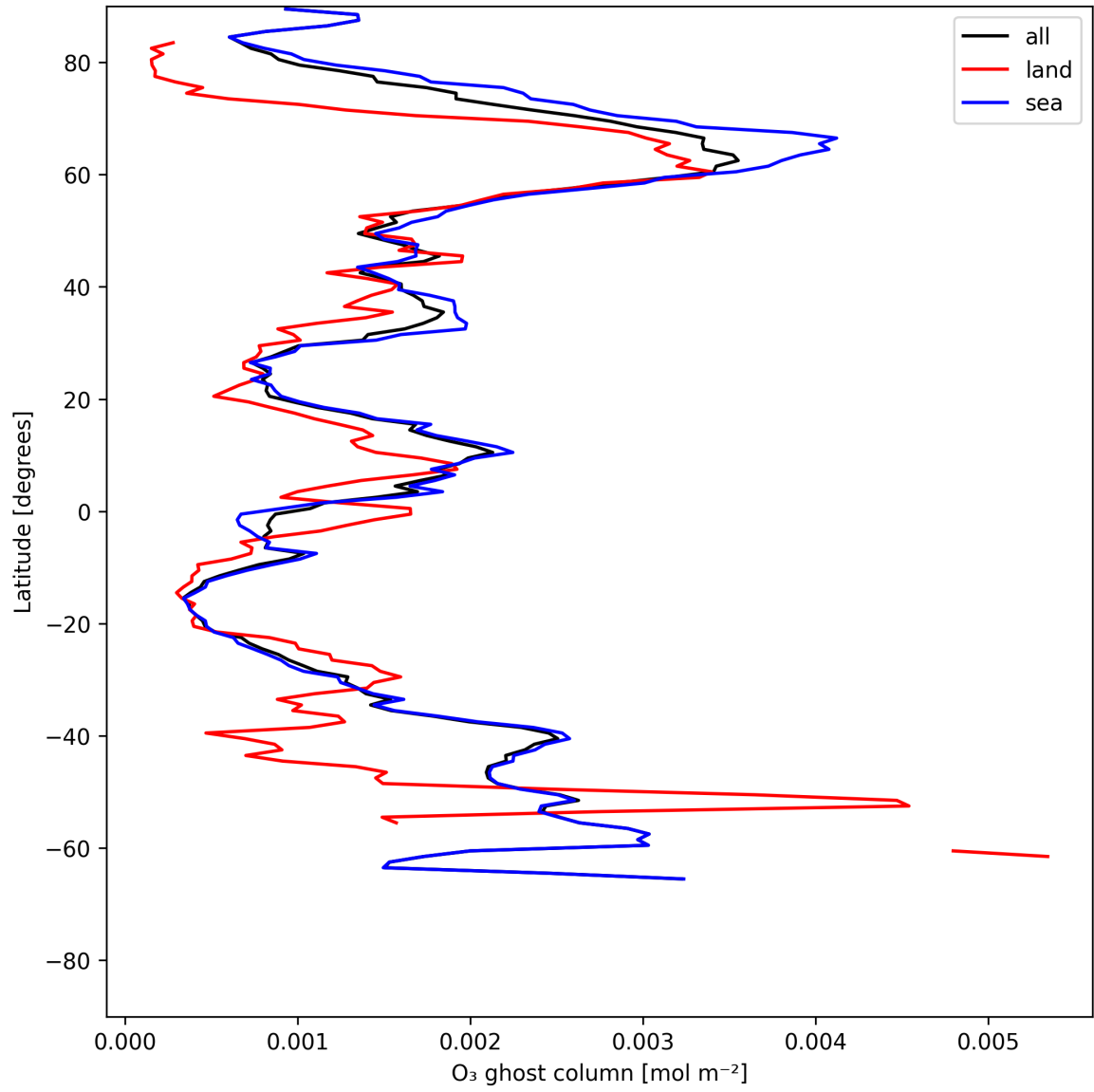
Figure 18: Zonal average of "O 3 ghost column" for 2025-06-12 to 2025-06-14.
