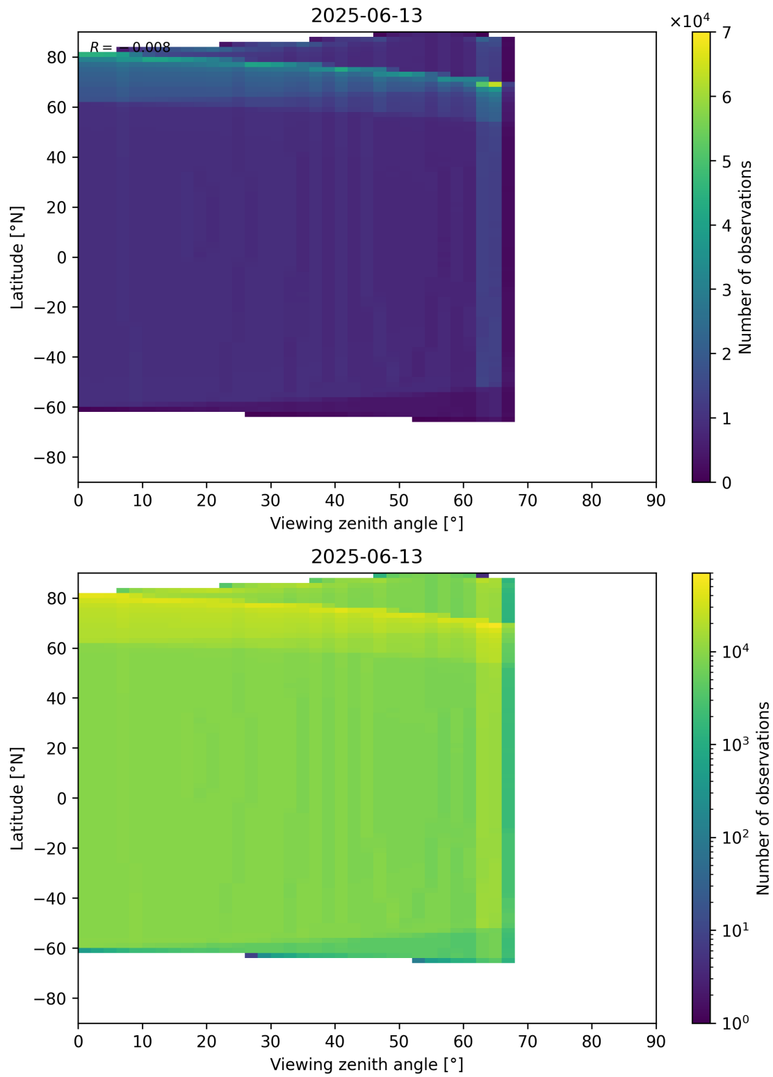
Figure 49: Scatter density plot of “Viewing zenith angle” against “Latitude” for 2025-06-12 to 2025-06-14.
