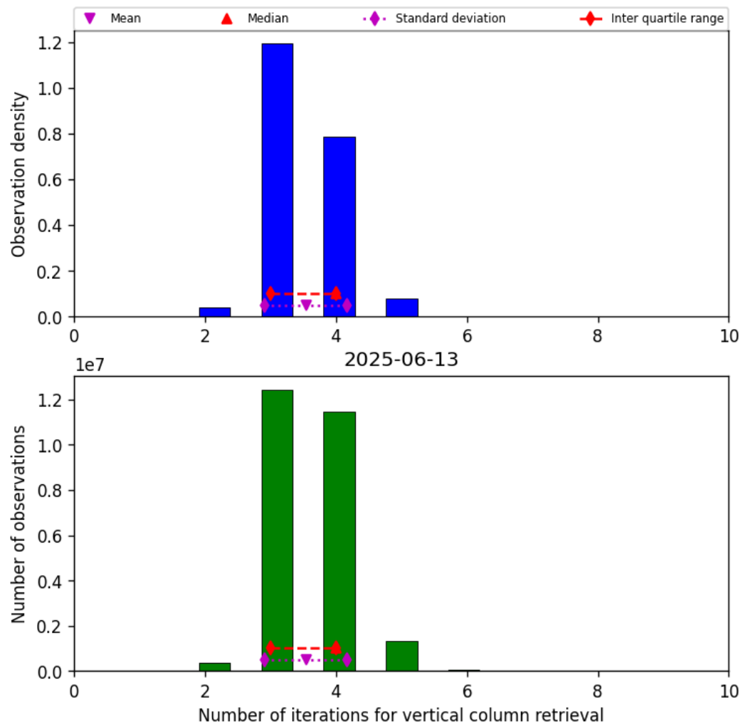
Figure 26: Histogram of “Number of iterations for vertical column retrieval” for 2025-06-12 to 2025-06-14
