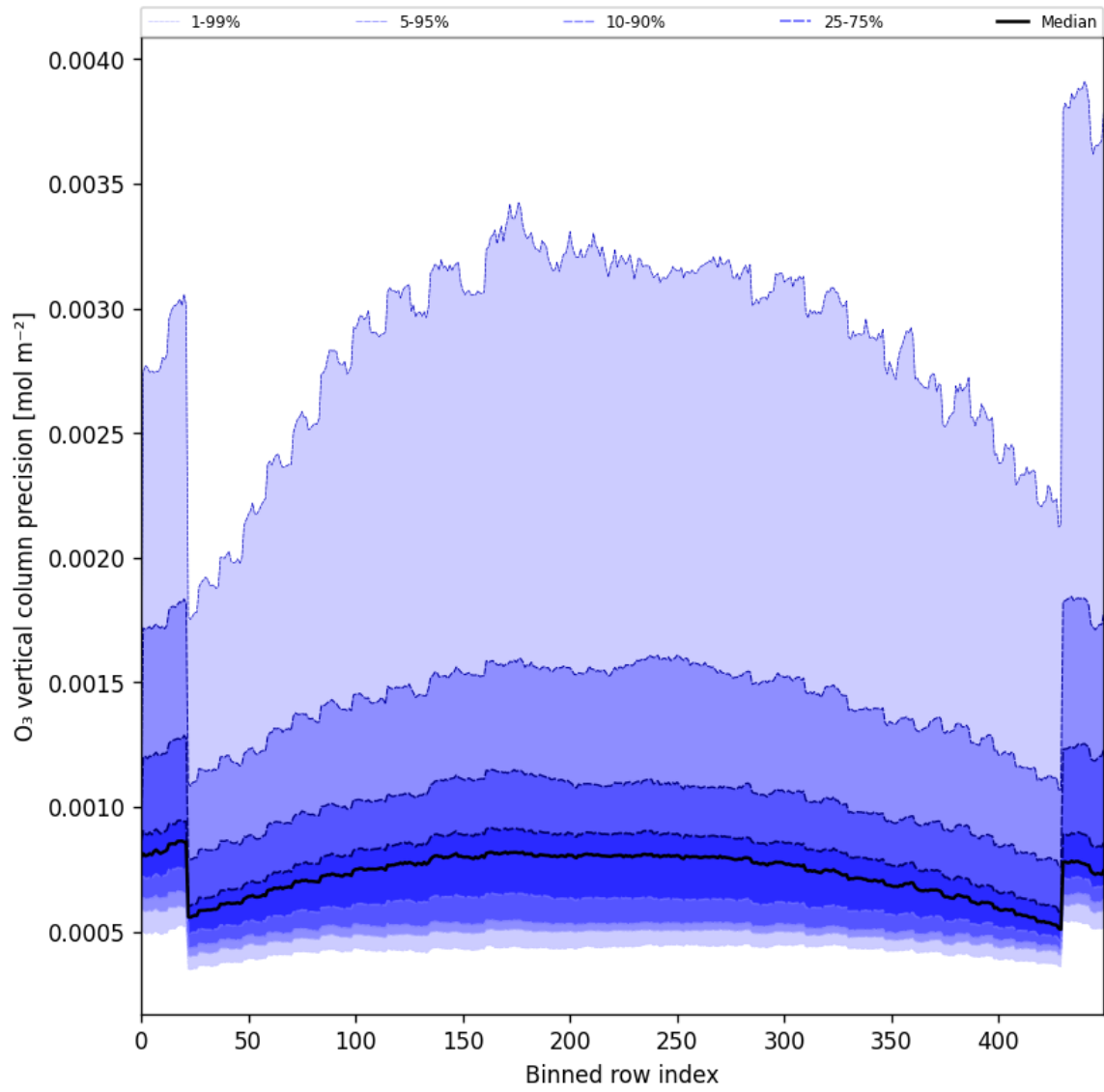
Figure 29: Along track statistics of “O 3 vertical column precision” for 2025-06-12 to 2025-06-14
