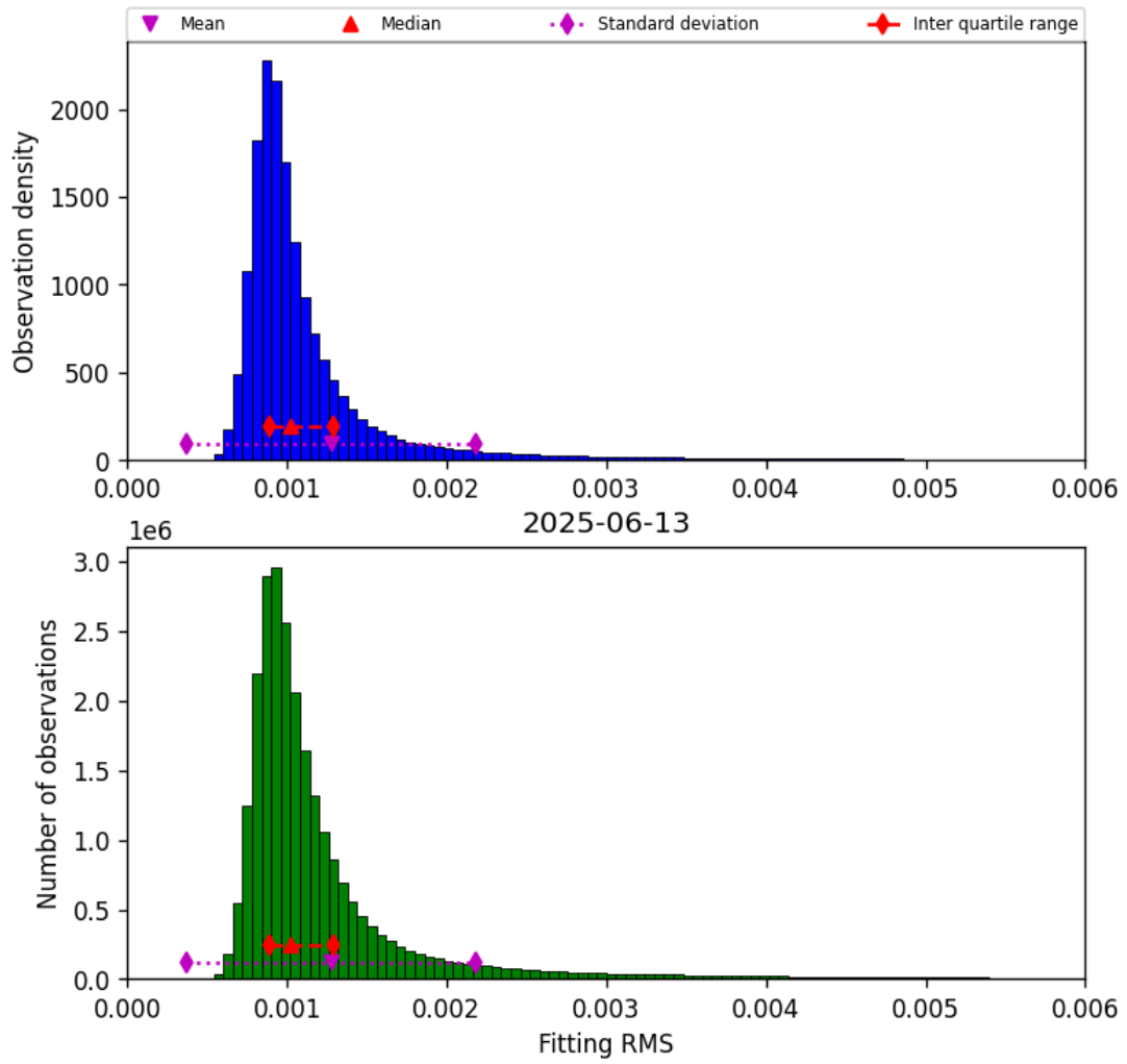
Figure 23: Histogram of “Fitting RMS” for 2025-06-12 to 2025-06-14
