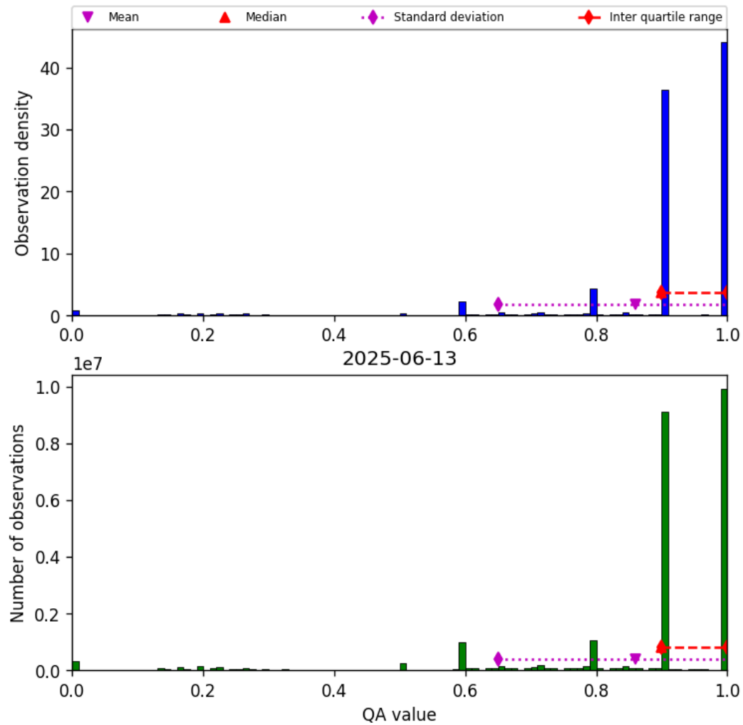
Figure 20: Histogram of “QA value” for 2025-06-12 to 2025-06-14
