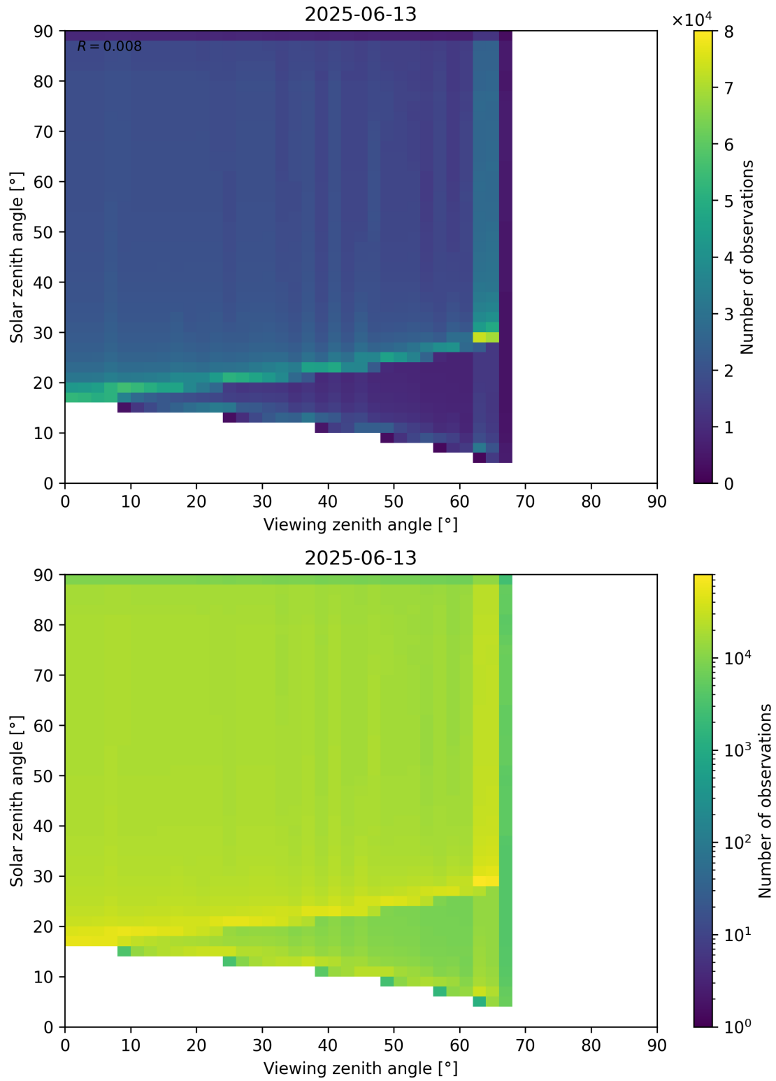
Figure 54: Scatter density plot of “Viewing zenith angle” against “Solar zenith angle” for 2025-06-12 to 2025-06-14.
