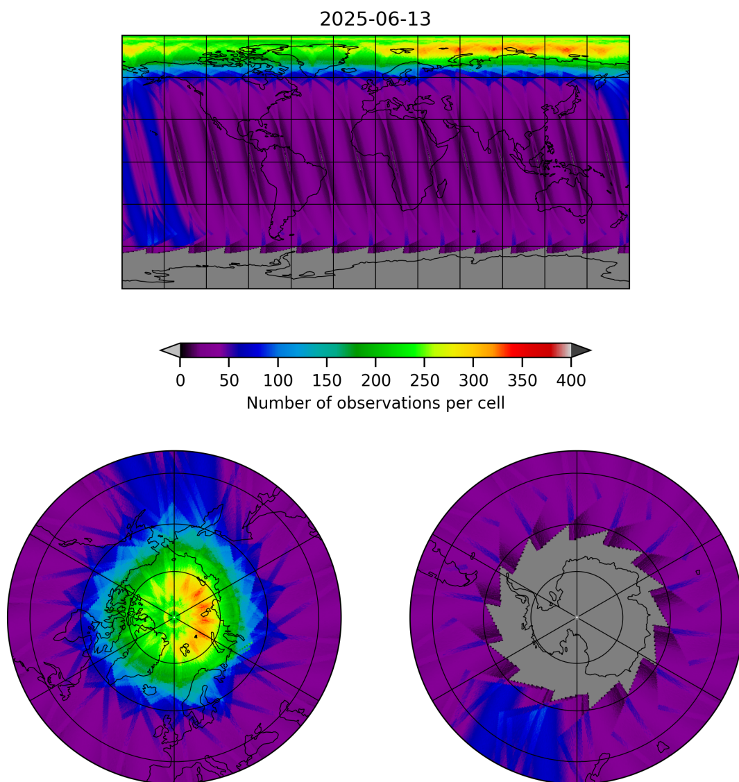
Figure 12: Map of the number of observations for 2025-06-12 to 2025-06-14
