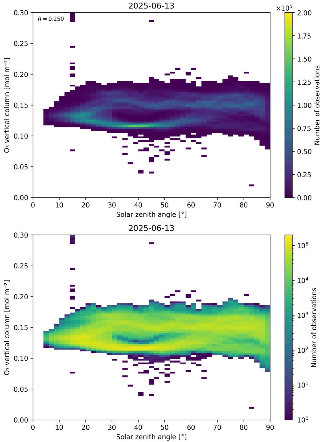
Figure 47: Scatter density plot of “Solar zenith angle” against “O 3 vertical column” for 2025-06-12 to 2025-06-14.
