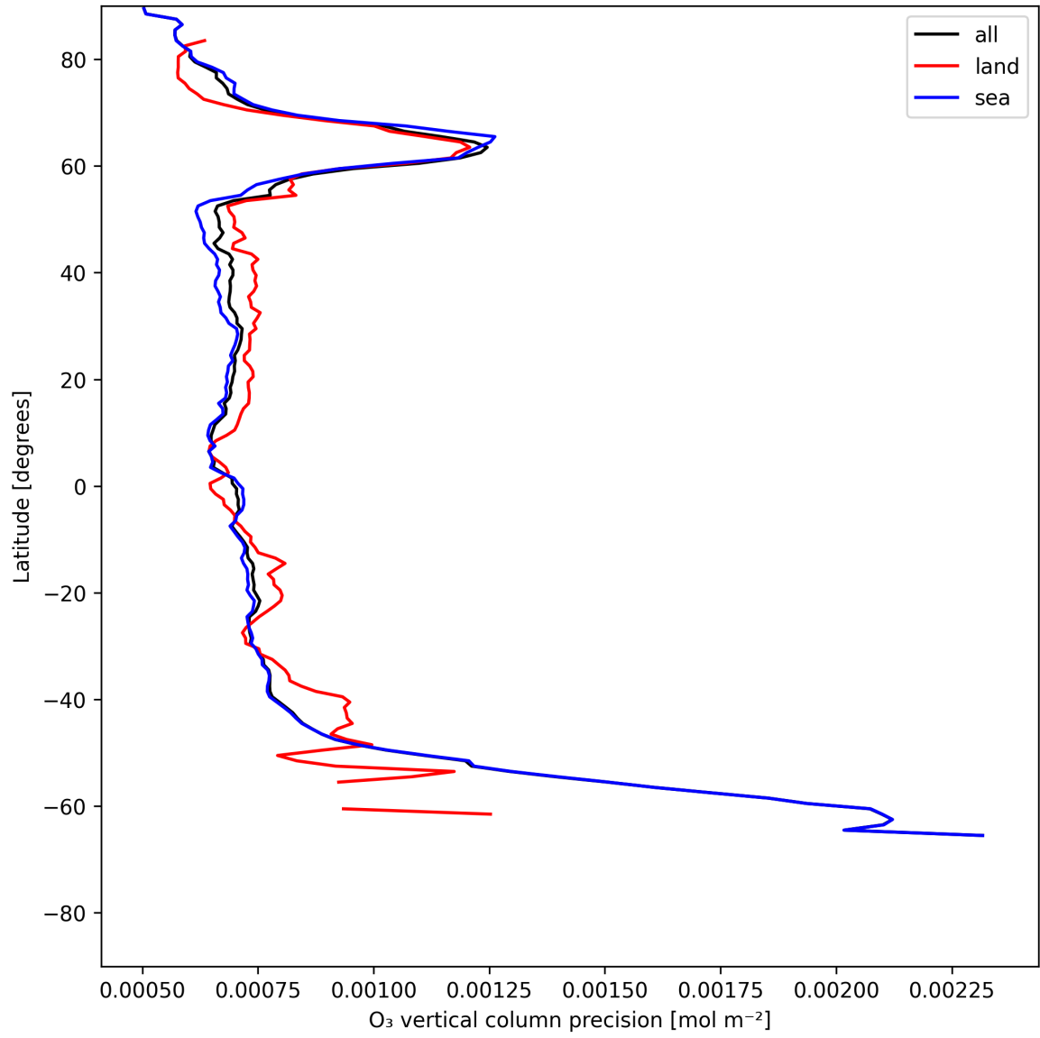
Figure 15: Zonal average of “O 3 vertical column precision” for 2025-06-12 to 2025-06-14.
