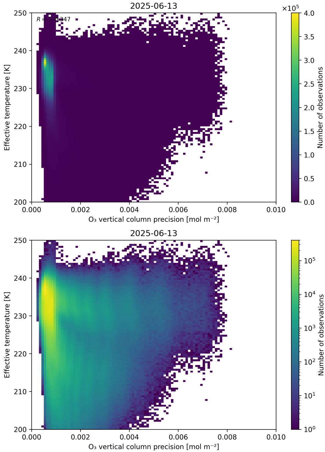
Figure 42: Scatter density plot of “O 3 vertical column precision” against “Effective temperature” for 2025-06-12 to 2025-06-14.
