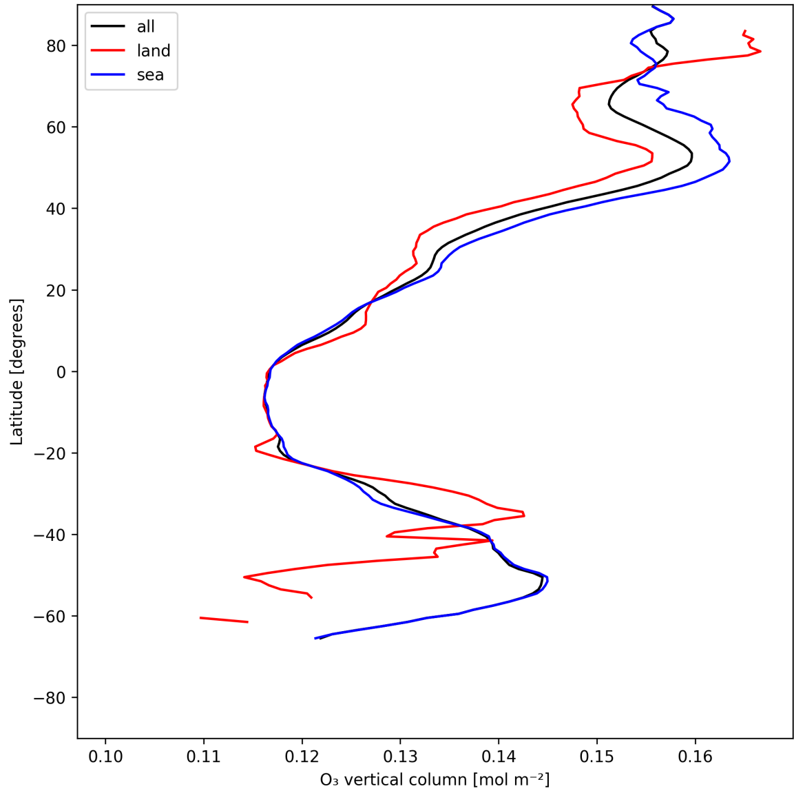
Figure 14: Zonal average of “O 3 vertical column” for 2025-06-12 to 2025-06-14.
