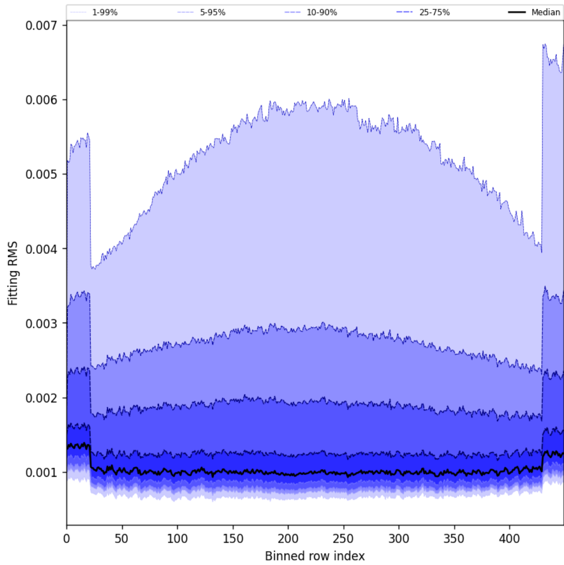
Figure 30: Along track statistics of “Fitting RMS” for 2025-06-12 to 2025-06-14
