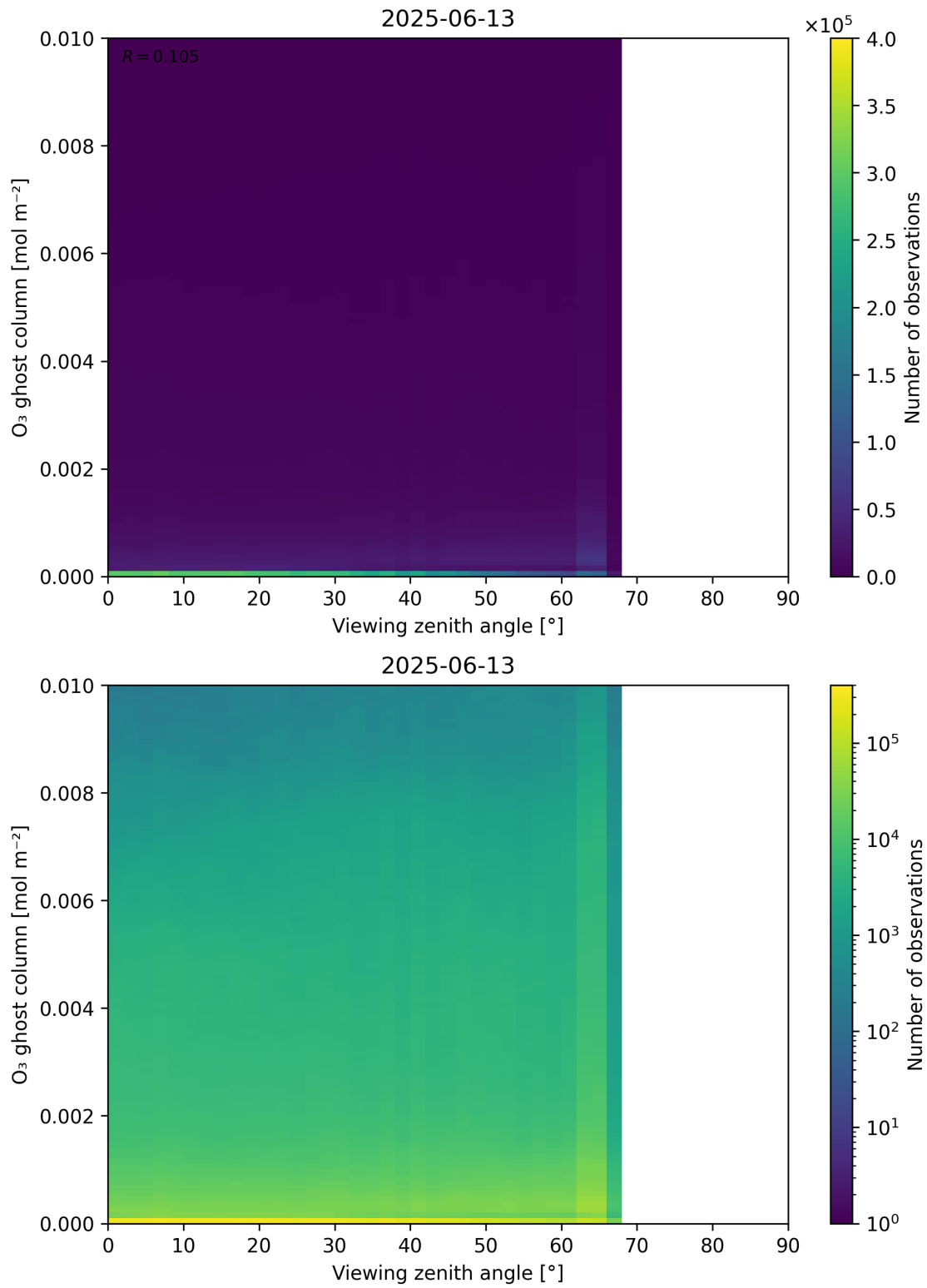
Figure 51: Scatter density plot of “Viewing zenith angle” against “O 3 ghost column” for 2025-06-12 to 2025-06-14.
