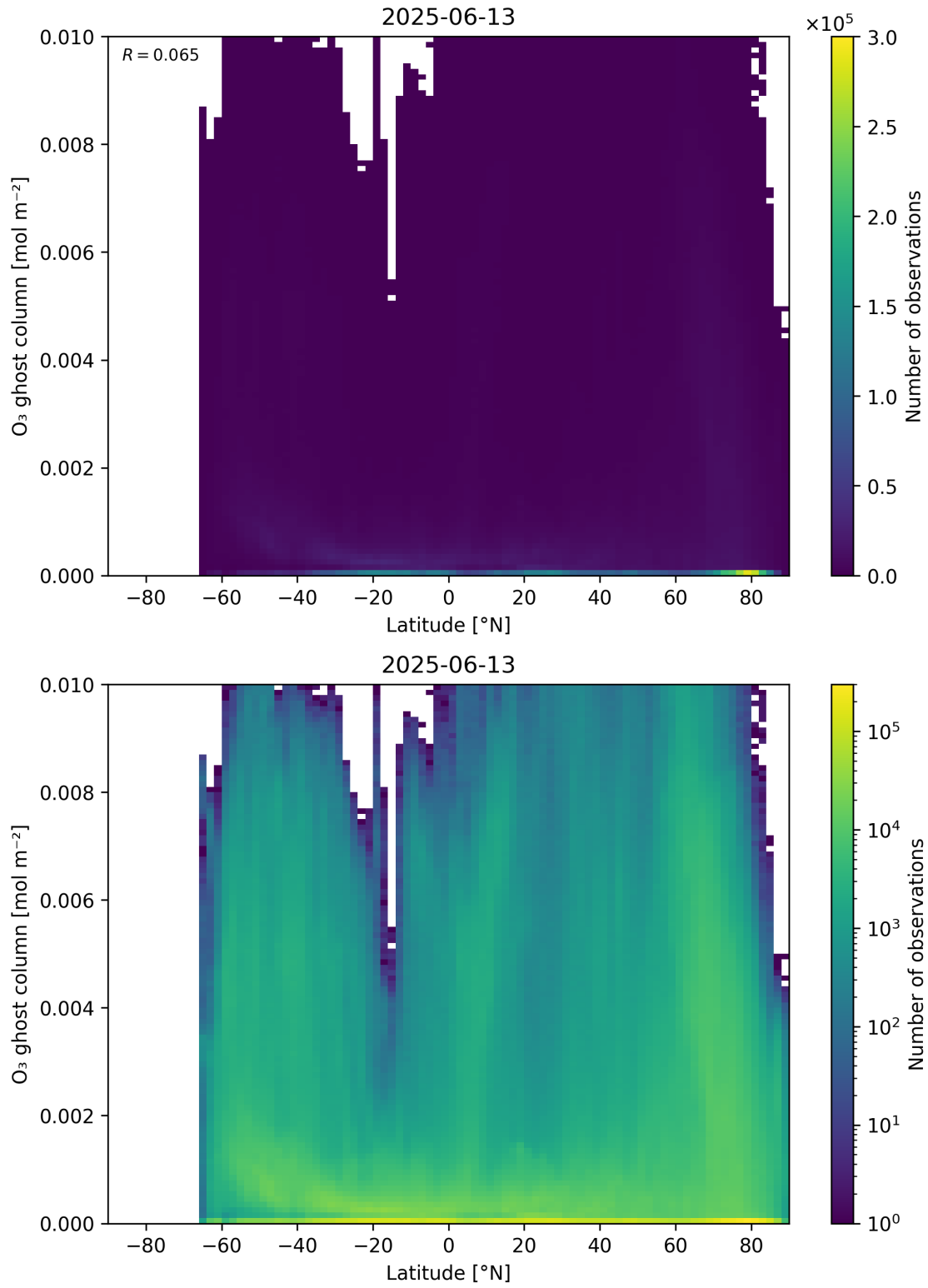
Figure 35: Scatter density plot of “Latitude” against “O 3 ghost column” for 2025-06-12 to 2025-06-14.
