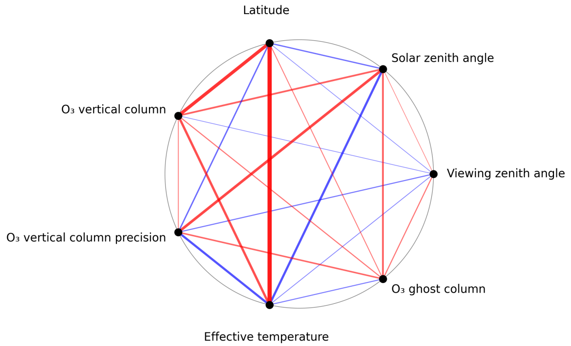
Figure 1: Map of correlation graph for 2025-06-12 to 2025-06-14.
