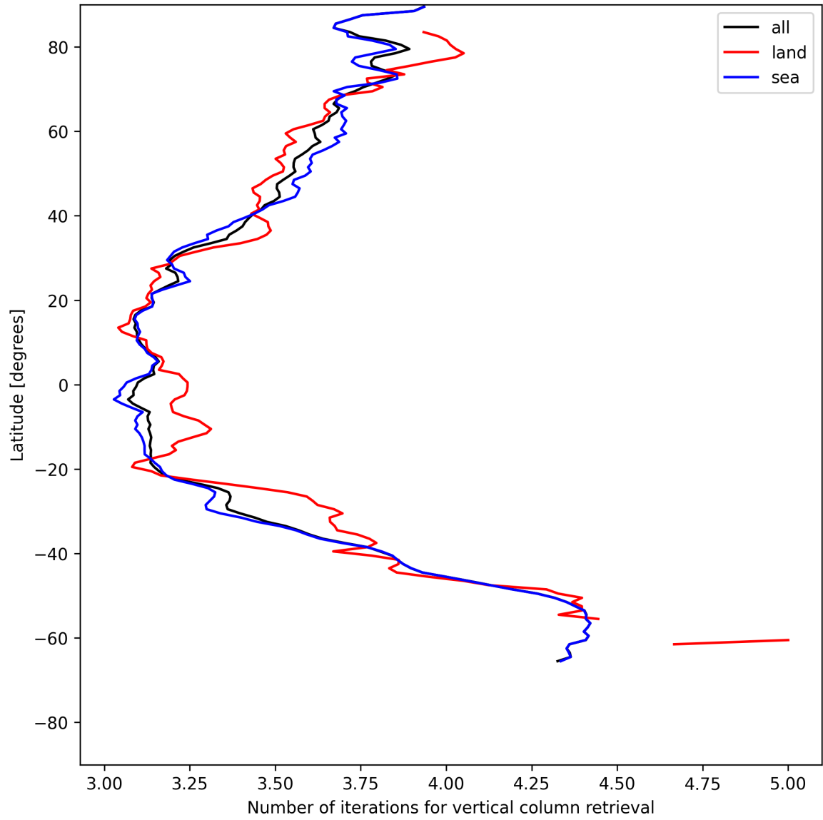
Figure 19: Zonal average of “Number of iterations for vertical column retrieval” for 2025-06-12 to 2025-06-14.
