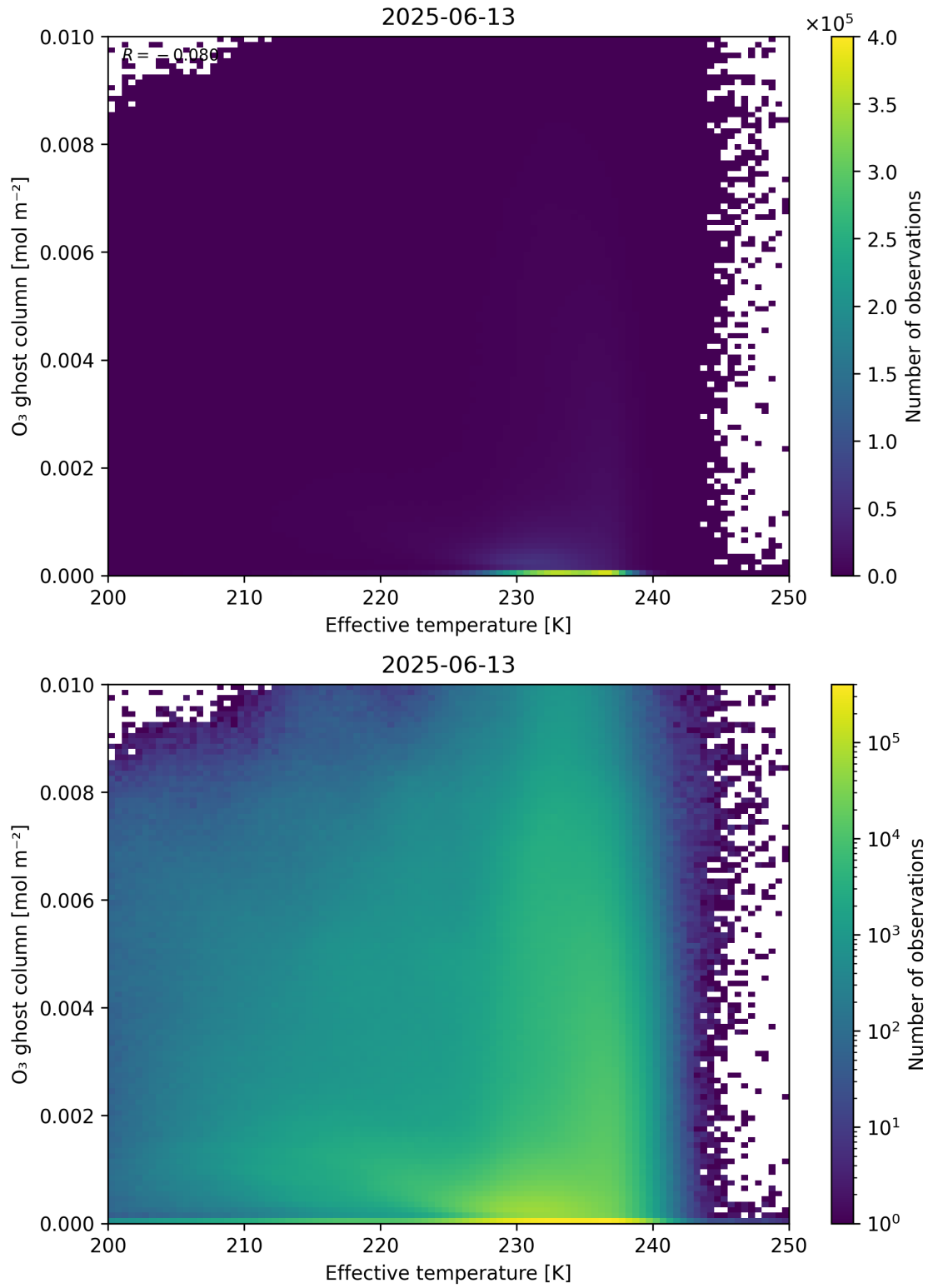
Figure 38: Scatter density plot of “Effective temperature” against “O 3 ghost column” for 2025-06-12 to 2025-06-14.
