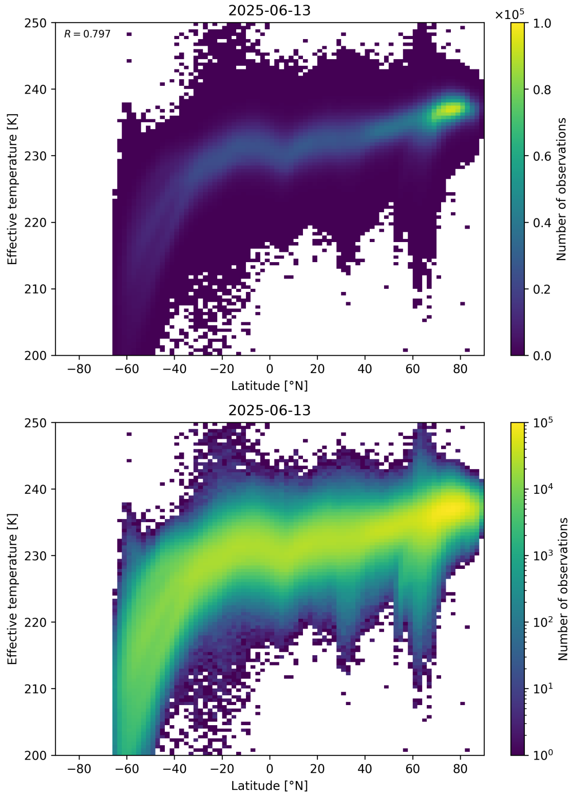
Figure 34: Scatter density plot of “Latitude” against “Effective temperature” for 2025-06-12 to 2025-06-14.
