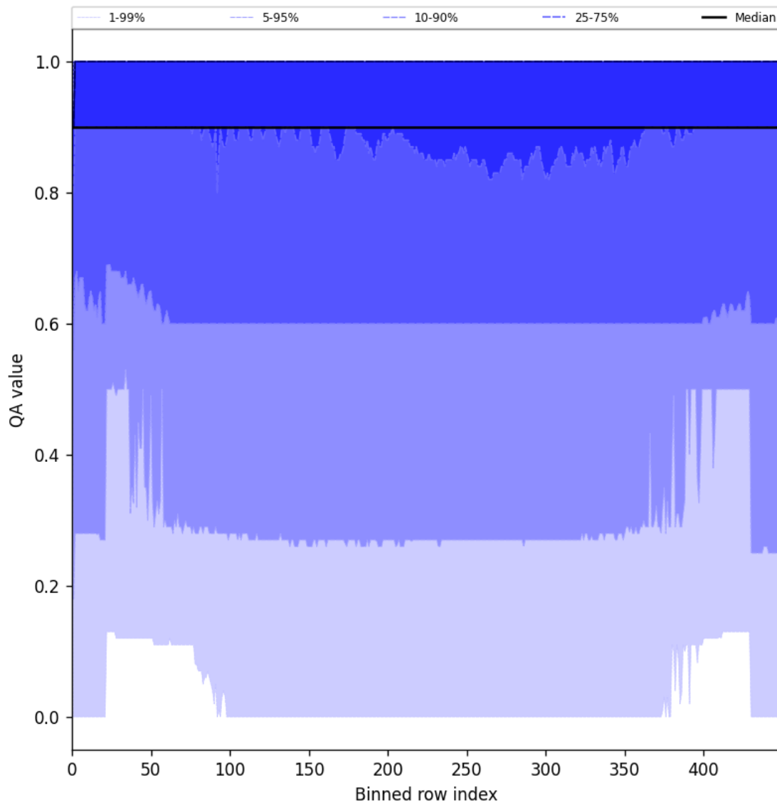
Figure 27: Along track statistics of “QA value” for 2025-06-12 to 2025-06-14
