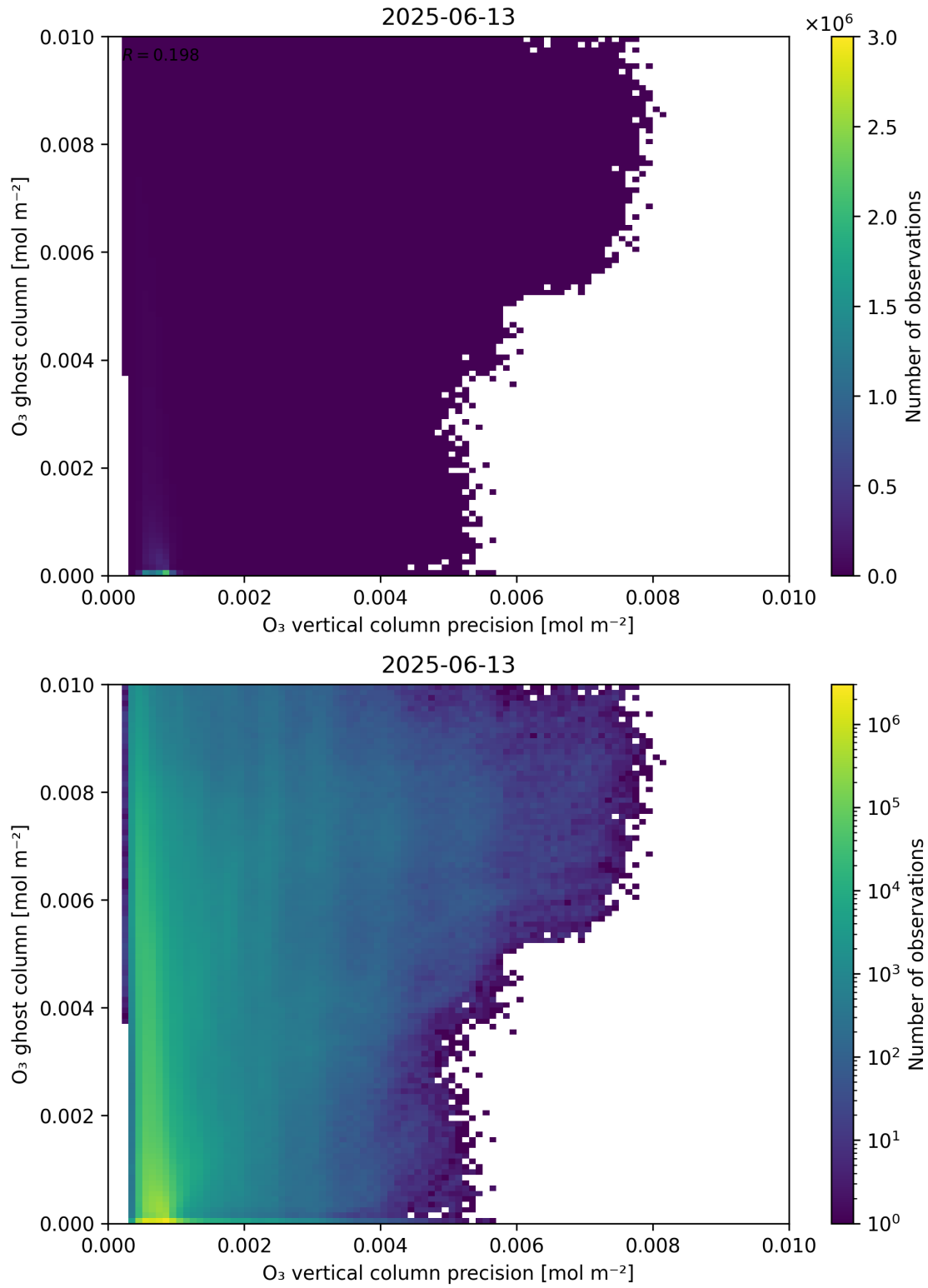
Figure 43: Scatter density plot of “ \text{O}_3 vertical column precision” against “ \text{O}_3 ghost column” for 2025-06-12 to 2025-06-14.
