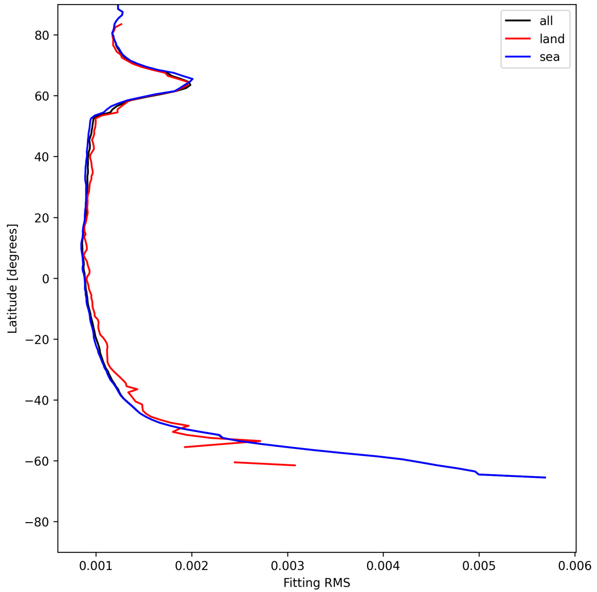
Figure 16: Zonal average of “Fitting RMS” for 2025-06-12 to 2025-06-14.
