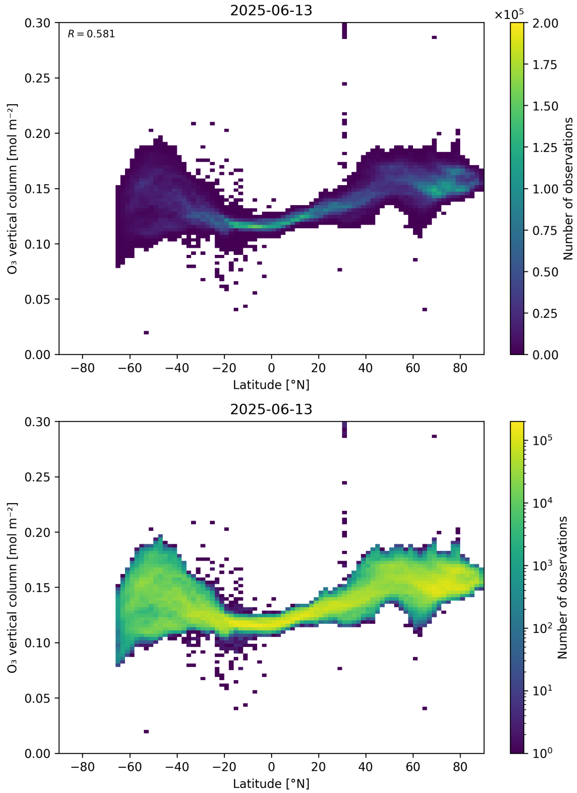
Figure 36: Scatter density plot of “Latitude” against “O 3 vertical column” for 2025-06-12 to 2025-06-14.
