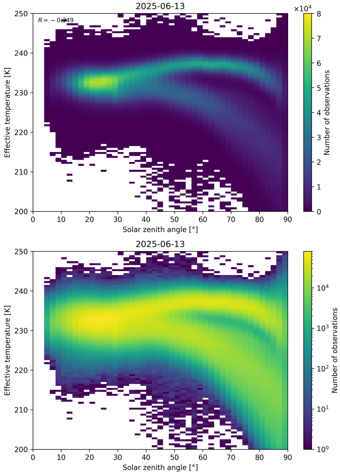
Figure 45: Scatter density plot of “Solar zenith angle” against “Effective temperature” for 2025-06-12 to 2025-06-14.
