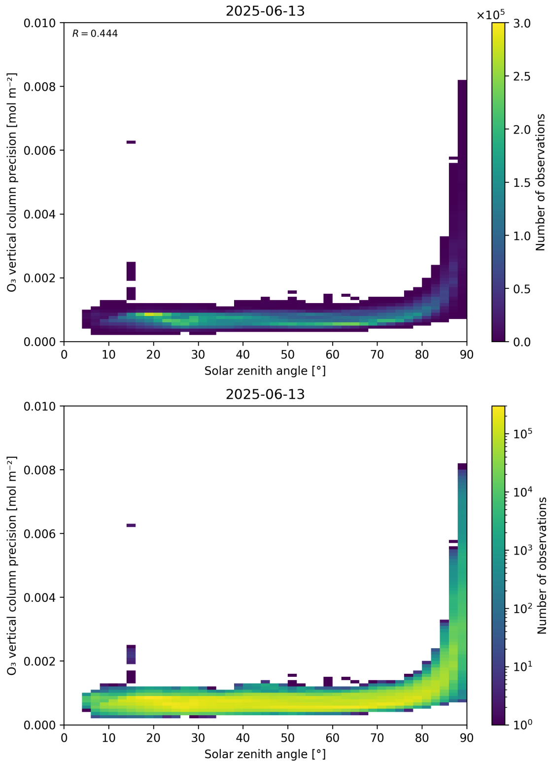
Figure 48: Scatter density plot of “Solar zenith angle” against “O 3 vertical column precision” for 2025-06-12 to 2025-06-14.
