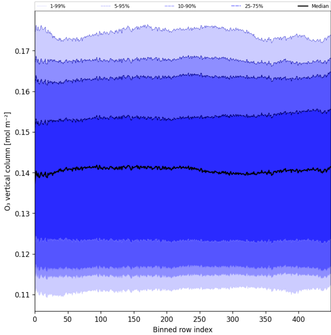
Figure 28: Along track statistics of “O 3 vertical column” for 2025-06-12 to 2025-06-14
