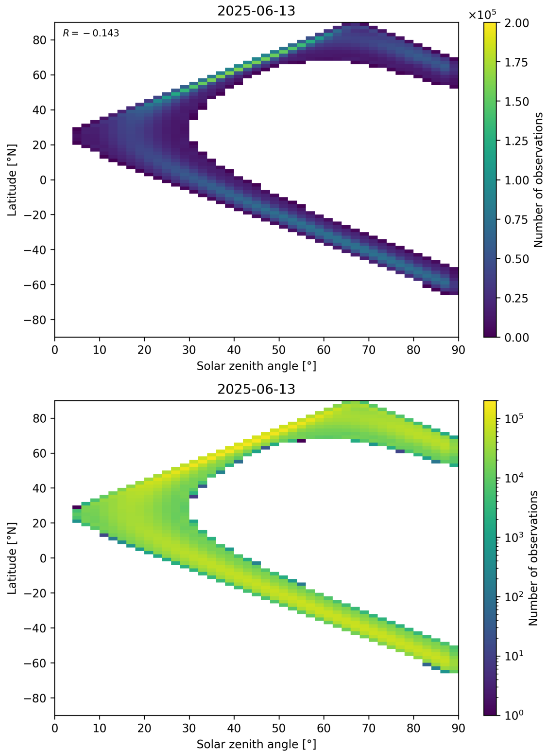
Figure 44: Scatter density plot of “Solar zenith angle” against “Latitude” for 2025-06-12 to 2025-06-14.
