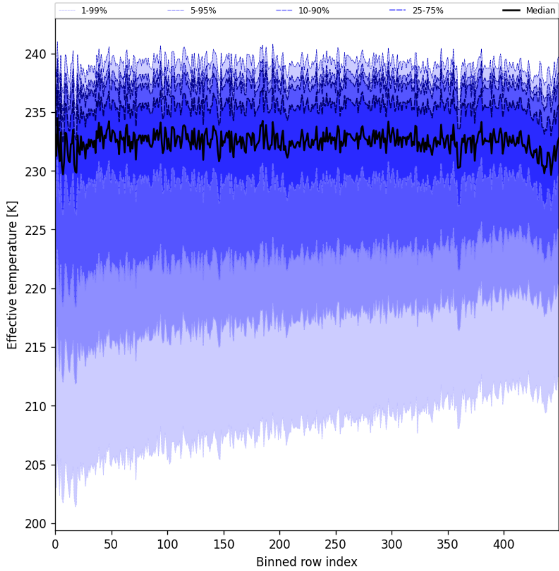
Figure 31: Along track statistics of “Effective temperature” for 2025-06-12 to 2025-06-14
