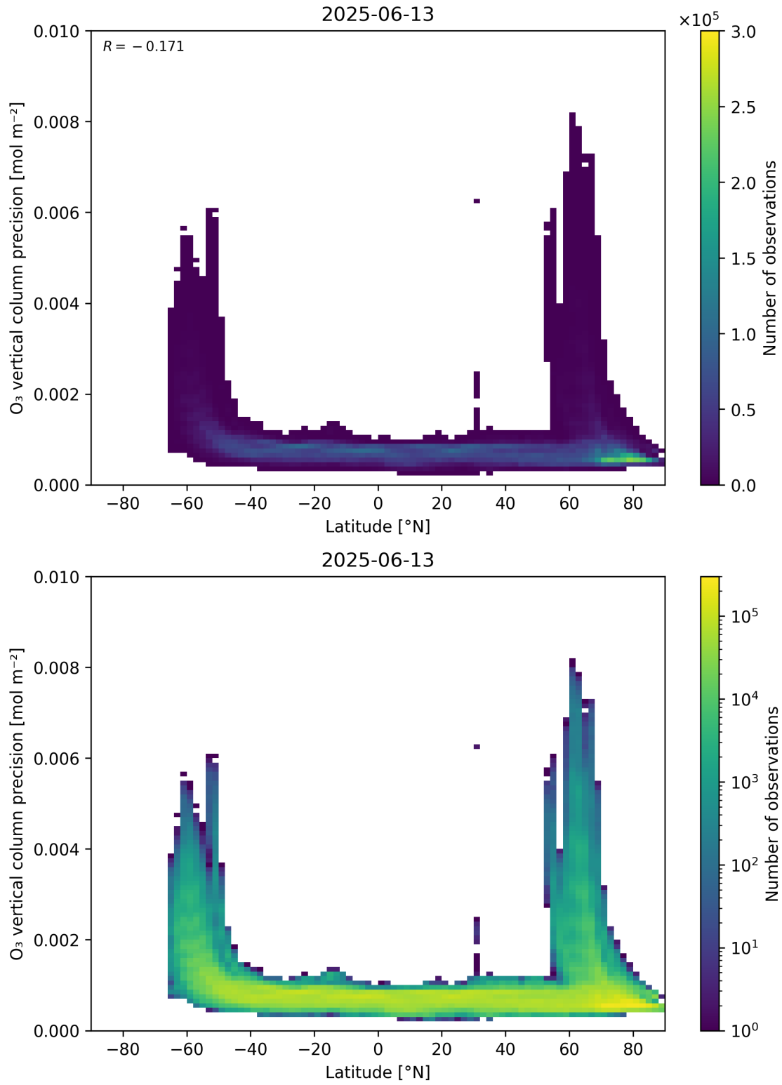
Figure 37: Scatter density plot of “Latitude” against “O 3 vertical column precision” for 2025-06-12 to 2025-06-14.
