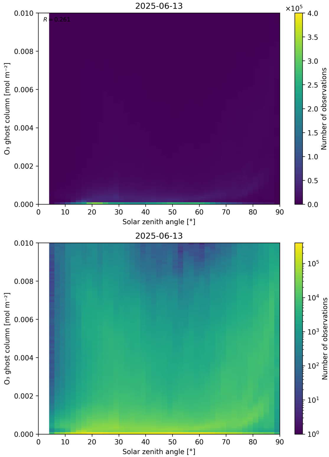
Figure 46: Scatter density plot of “Solar zenith angle” against “O 3 ghost column” for 2025-06-12 to 2025-06-14.
