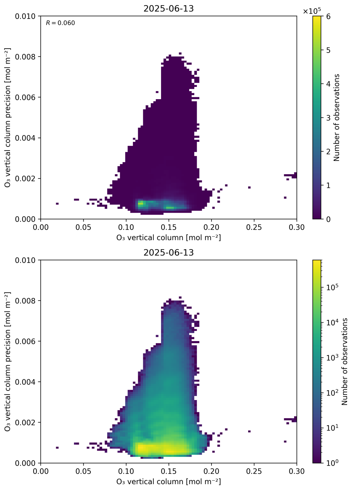
Figure 41: Scatter density plot of “O 3 vertical column” against “O 3 vertical column precision” for 2025-06-12 to 2025-06-14.
