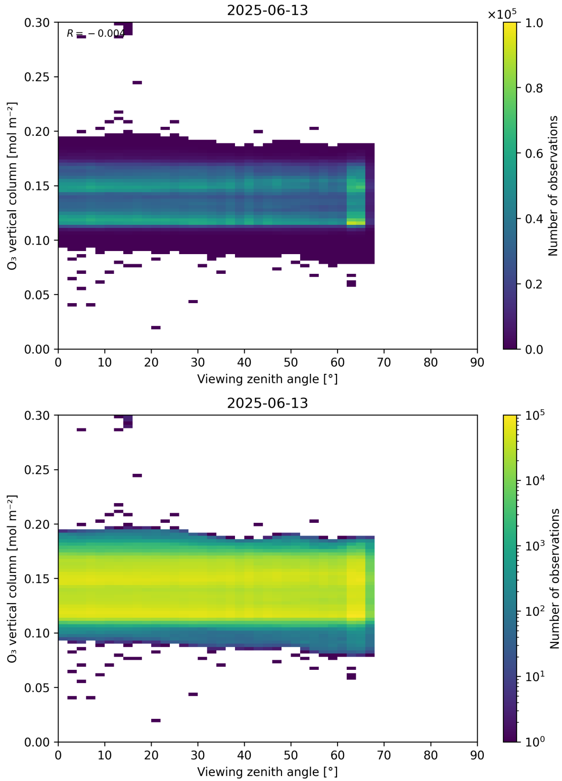
Figure 52: Scatter density plot of “Viewing zenith angle” against “O 3 vertical column” for 2025-06-12 to 2025-06-14.
