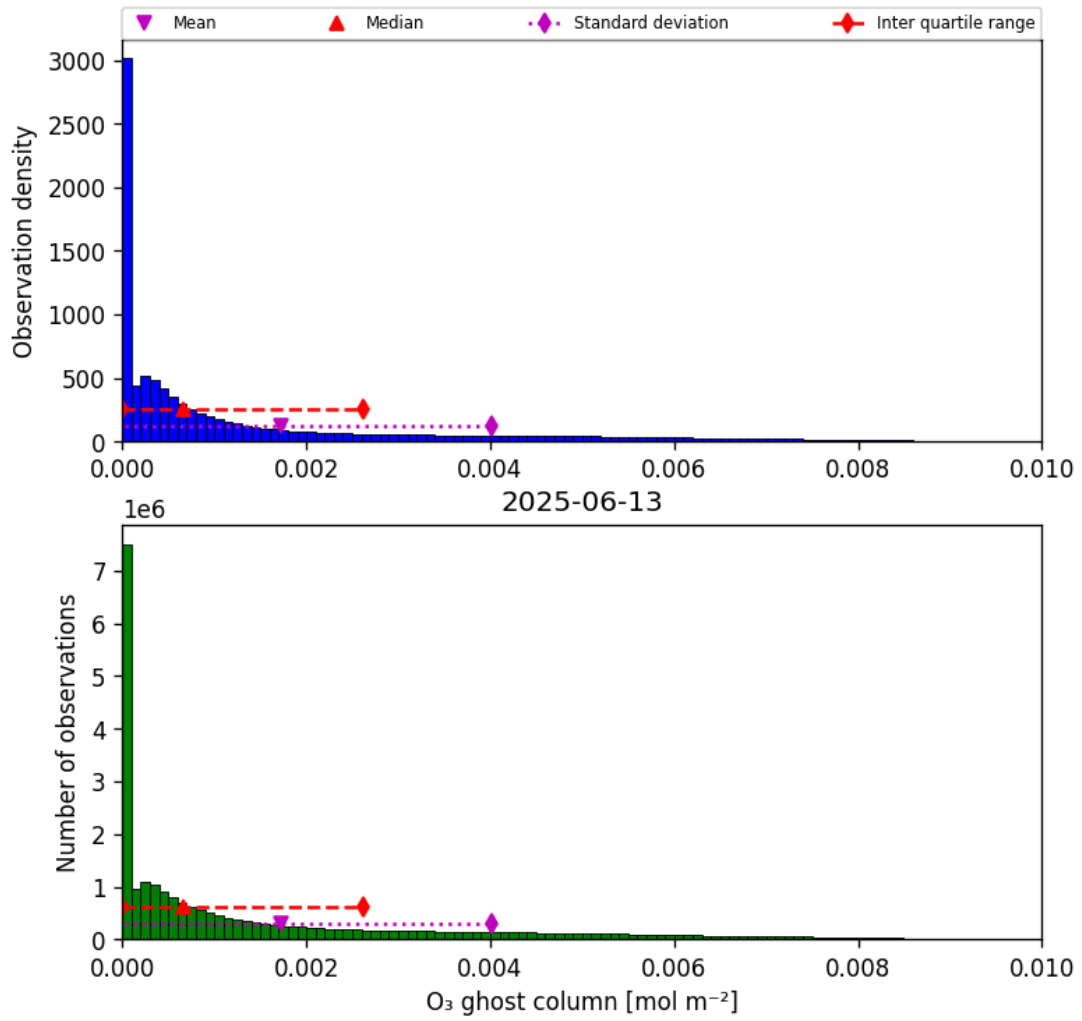
Figure 25: Histogram of “O 3 ghost column” for 2025-06-12 to 2025-06-14
