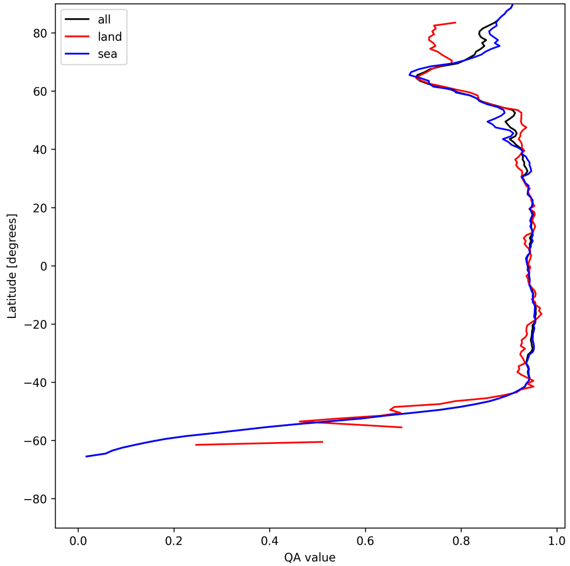
Figure 13: Zonal average of “QA value” for 2025-06-12 to 2025-06-14.
