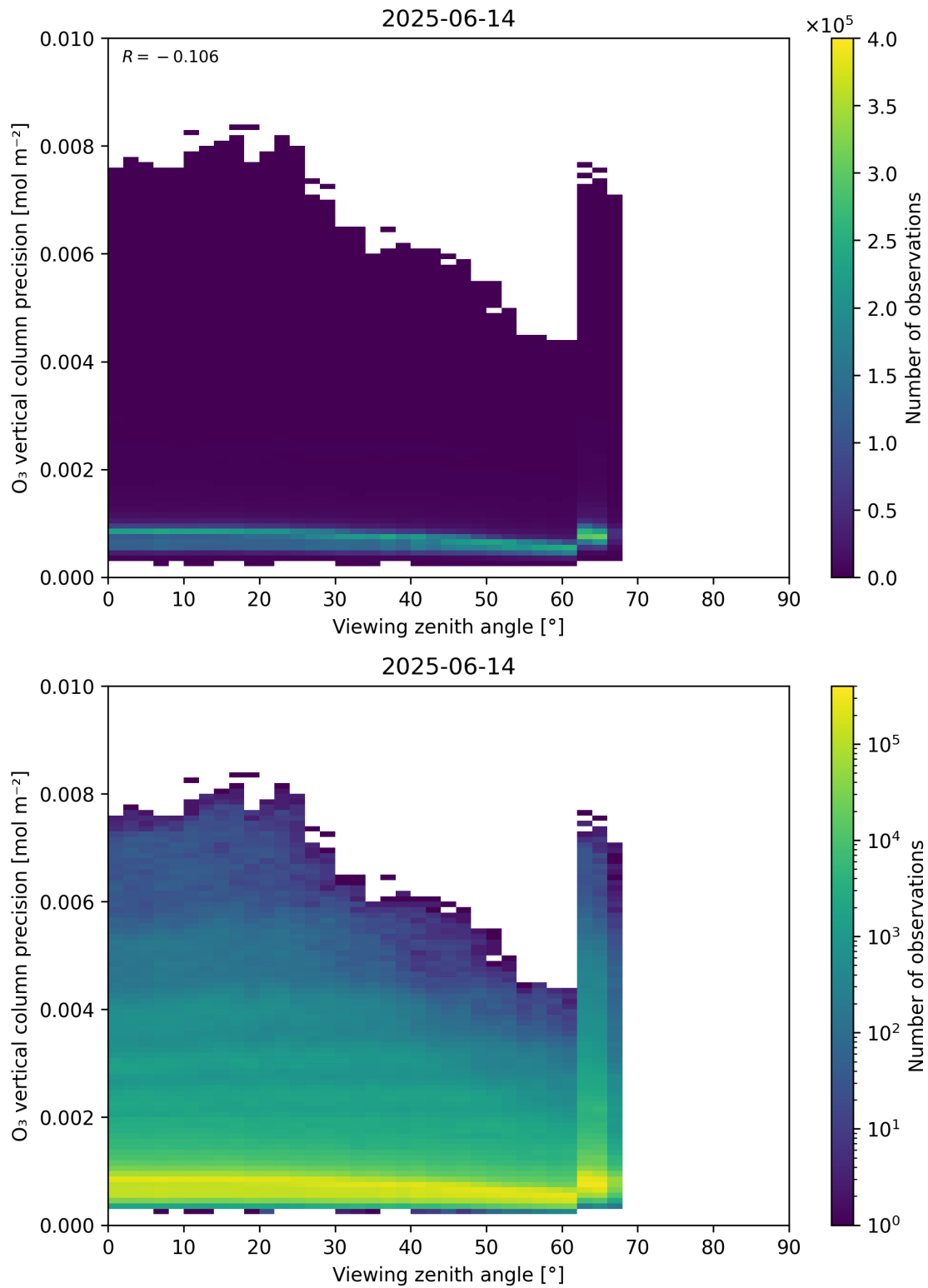
Figure 53: Scatter density plot of “Viewing zenith angle” against “O 3 vertical column precision” for 2025-06-13 to 2025-06-15.
