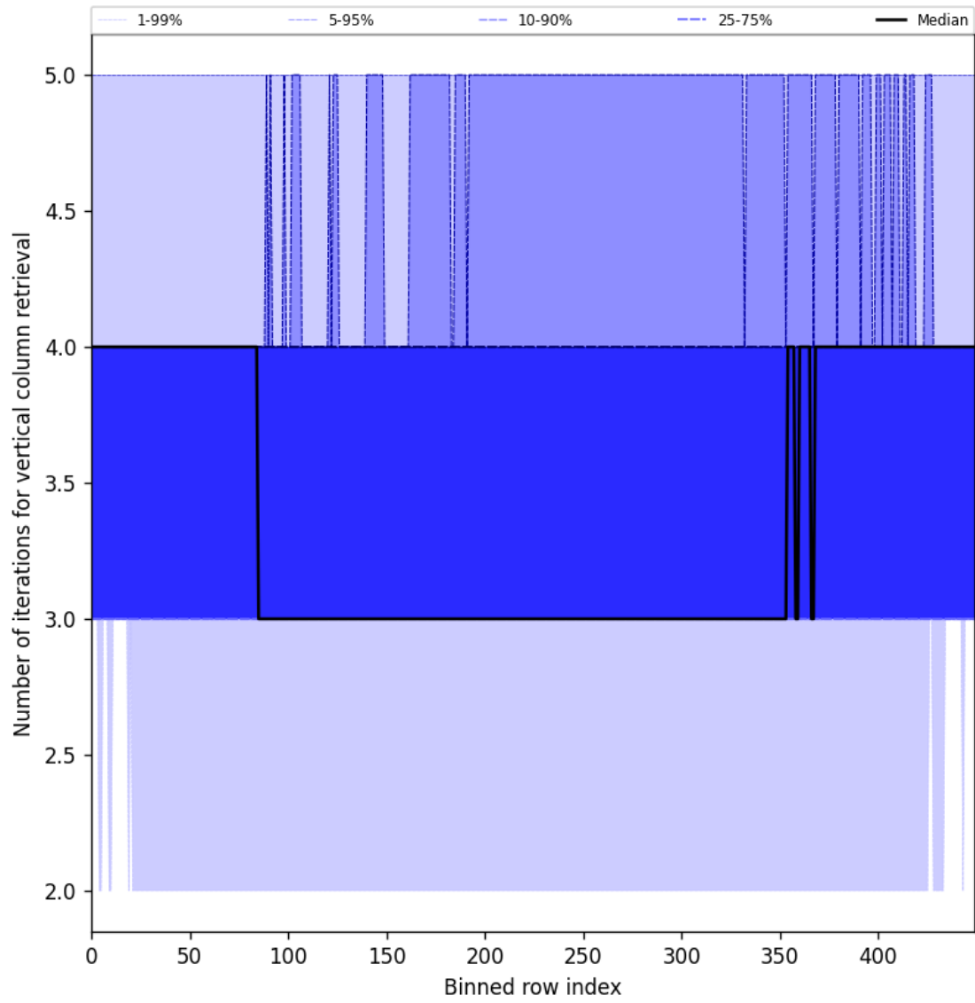
Figure 33: Along track statistics of “Number of iterations for vertical column retrieval” for 2025-06-13 to 2025-06-15
