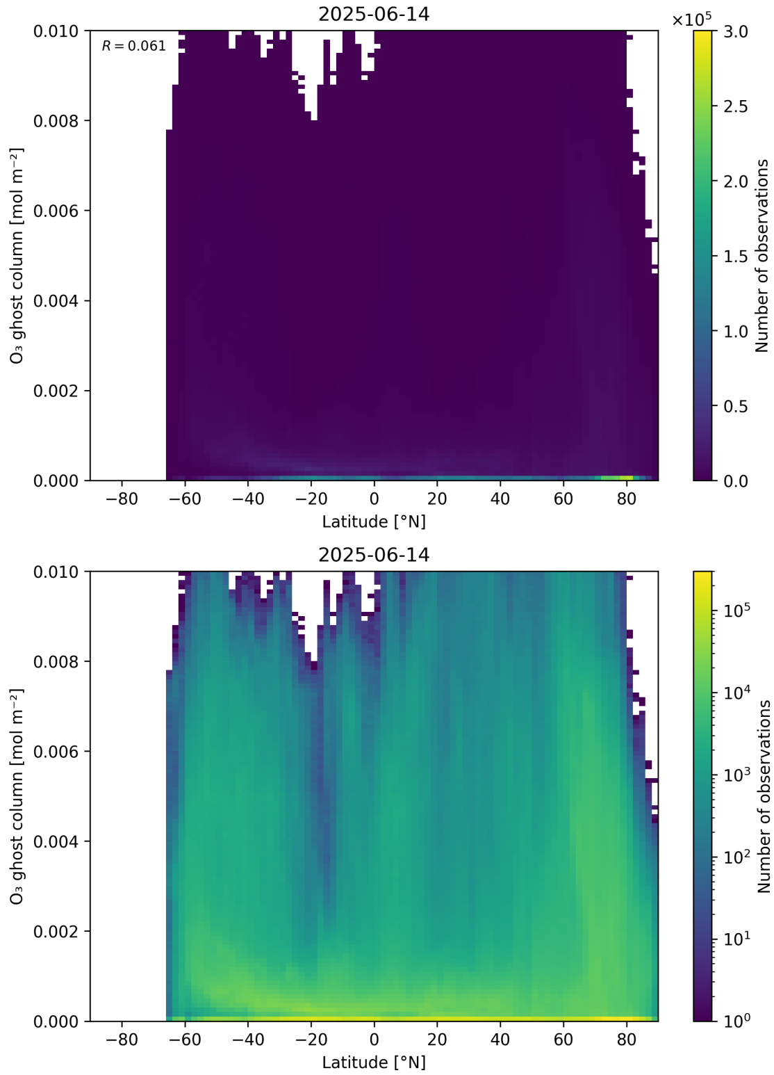
Figure 35: Scatter density plot of “Latitude” against “O 3 ghost column” for 2025-06-13 to 2025-06-15.
