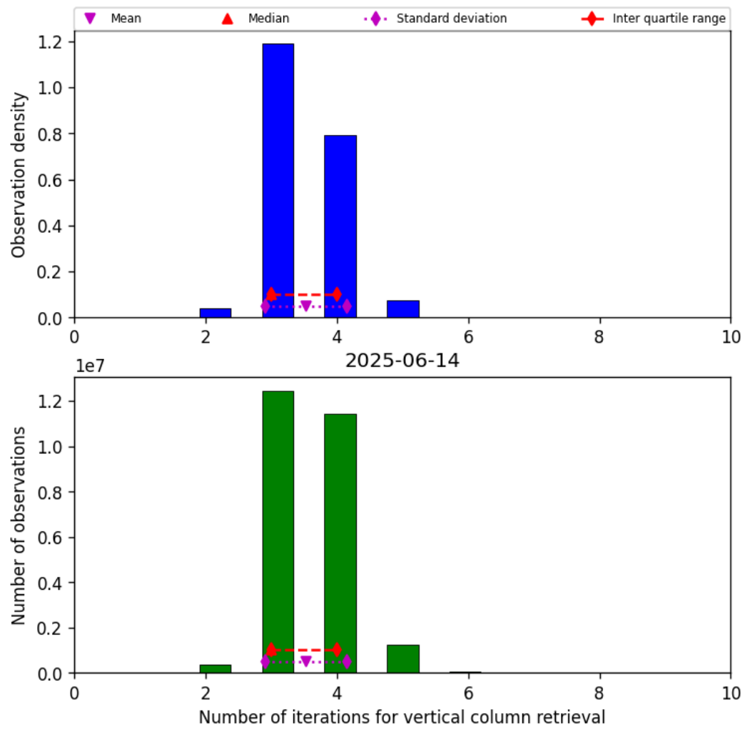
Figure 26: Histogram of “Number of iterations for vertical column retrieval” for 2025-06-13 to 2025-06-15
