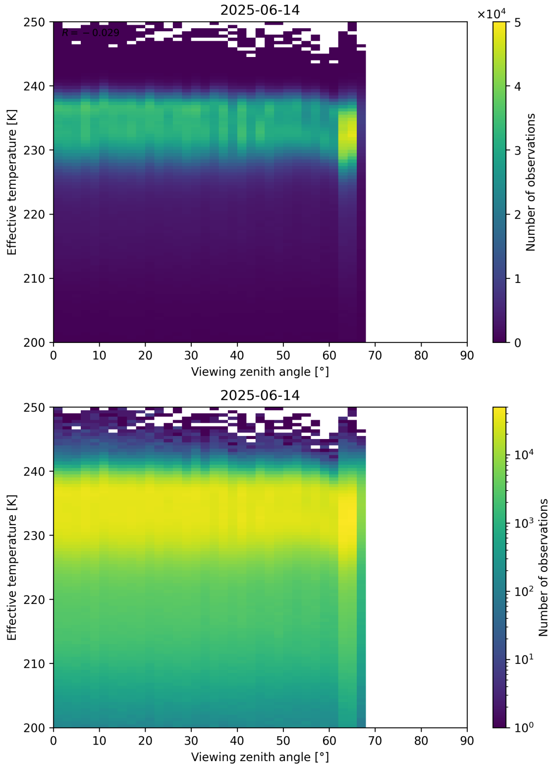
Figure 50: Scatter density plot of “Viewing zenith angle” against “Effective temperature” for 2025-06-13 to 2025-06-15.
