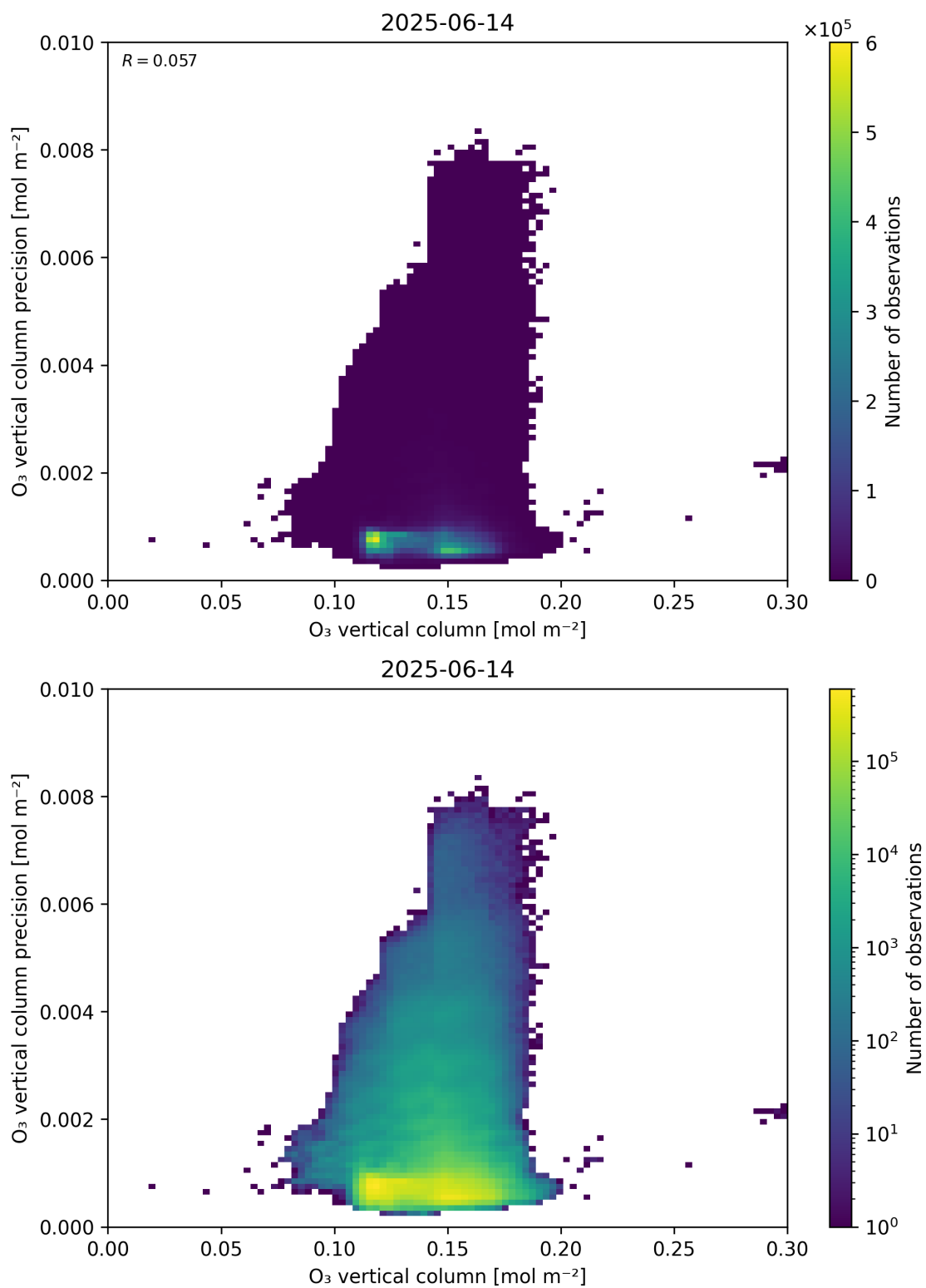
Figure 41: Scatter density plot of “O 3 vertical column” against “O 3 vertical column precision” for 2025-06-13 to 2025-06-15.
