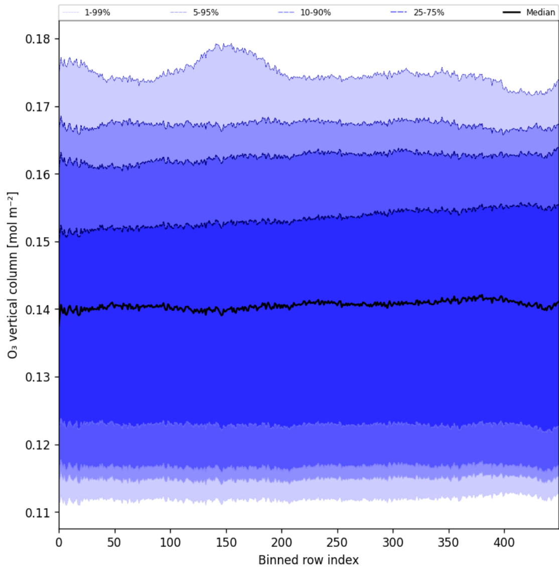
Figure 28: Along track statistics of “O 3 vertical column” for 2025-06-13 to 2025-06-15
