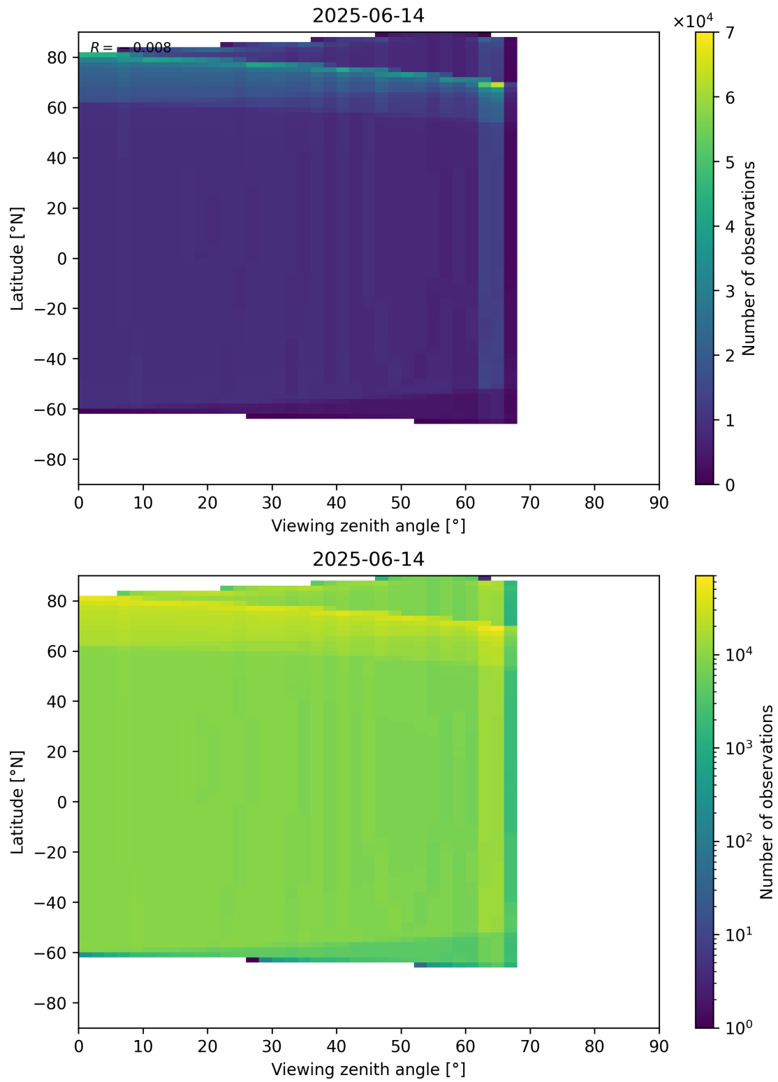
Figure 49: Scatter density plot of “Viewing zenith angle” against “Latitude” for 2025-06-13 to 2025-06-15.
