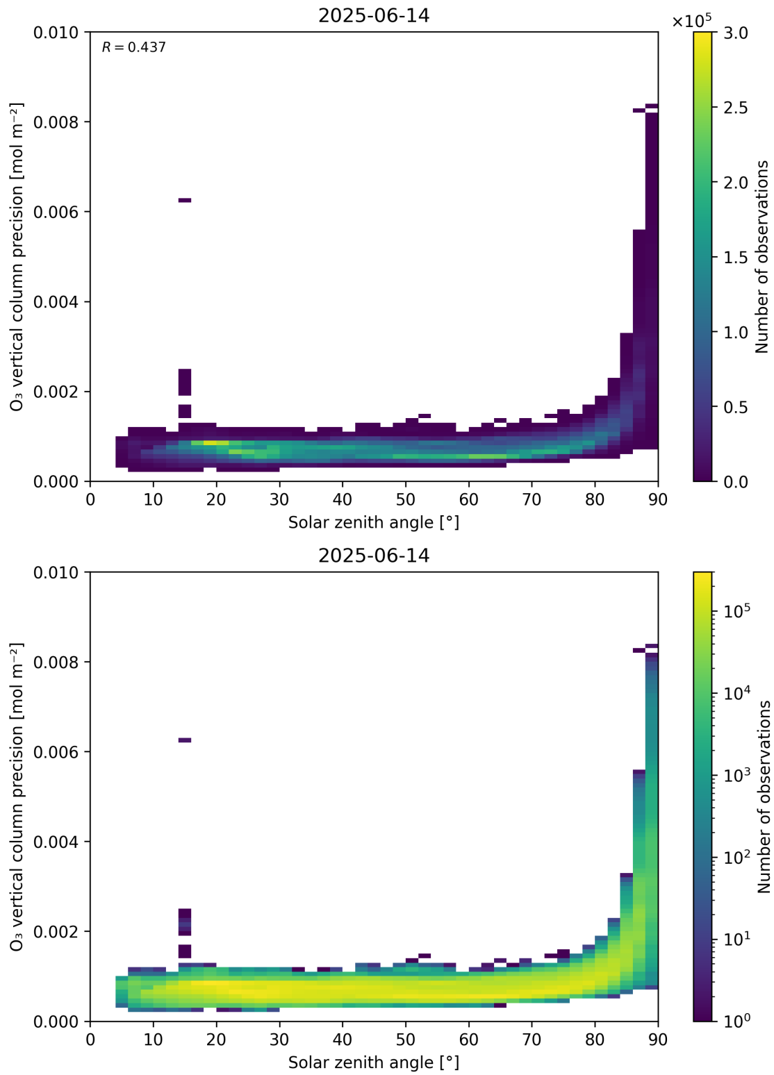
Figure 48: Scatter density plot of “Solar zenith angle” against “O 3 vertical column precision” for 2025-06-13 to 2025-06-15.
