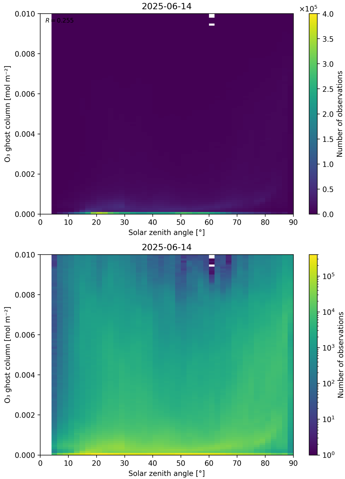
Figure 46: Scatter density plot of “Solar zenith angle” against “O 3 ghost column” for 2025-06-13 to 2025-06-15.
