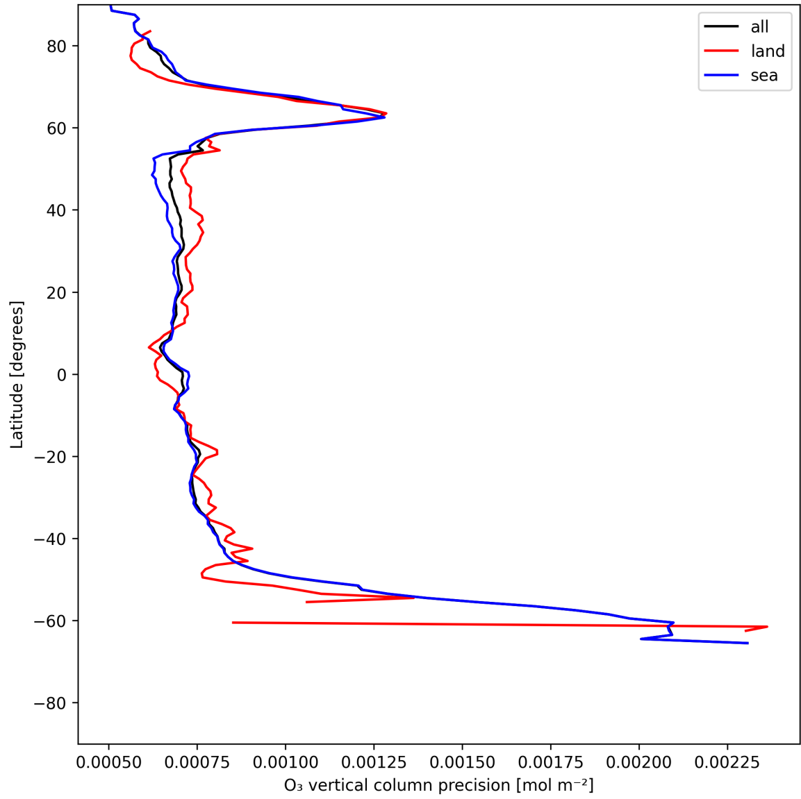
Figure 15: Zonal average of “O 3 vertical column precision” for 2025-06-13 to 2025-06-15.
