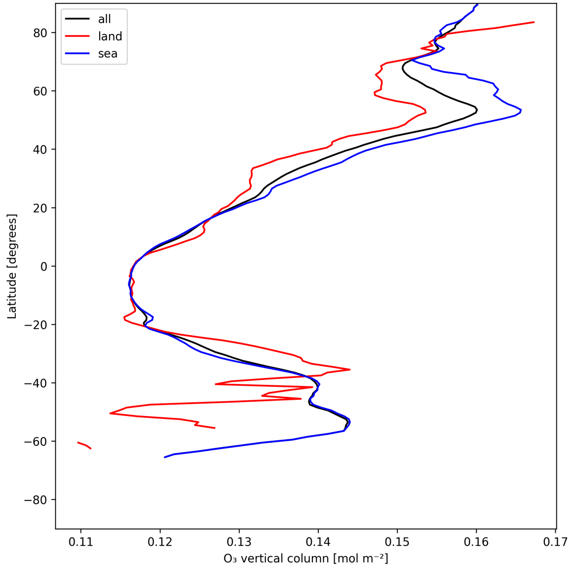
Figure 14: Zonal average of “O 3 vertical column” for 2025-06-13 to 2025-06-15.
