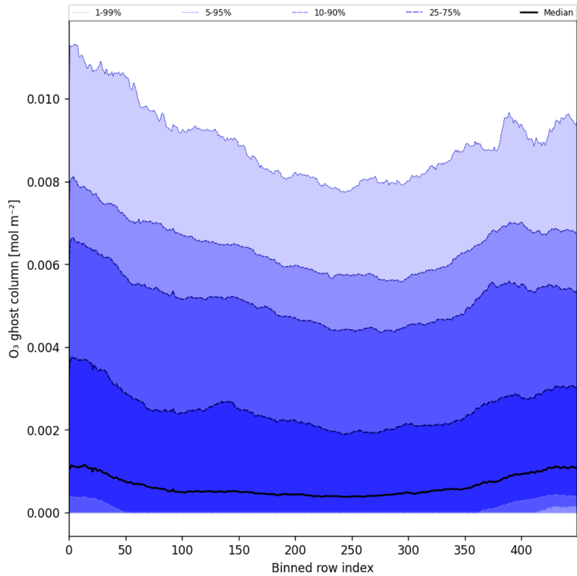
Figure 32: Along track statistics of “O 3 ghost column” for 2025-06-13 to 2025-06-15
