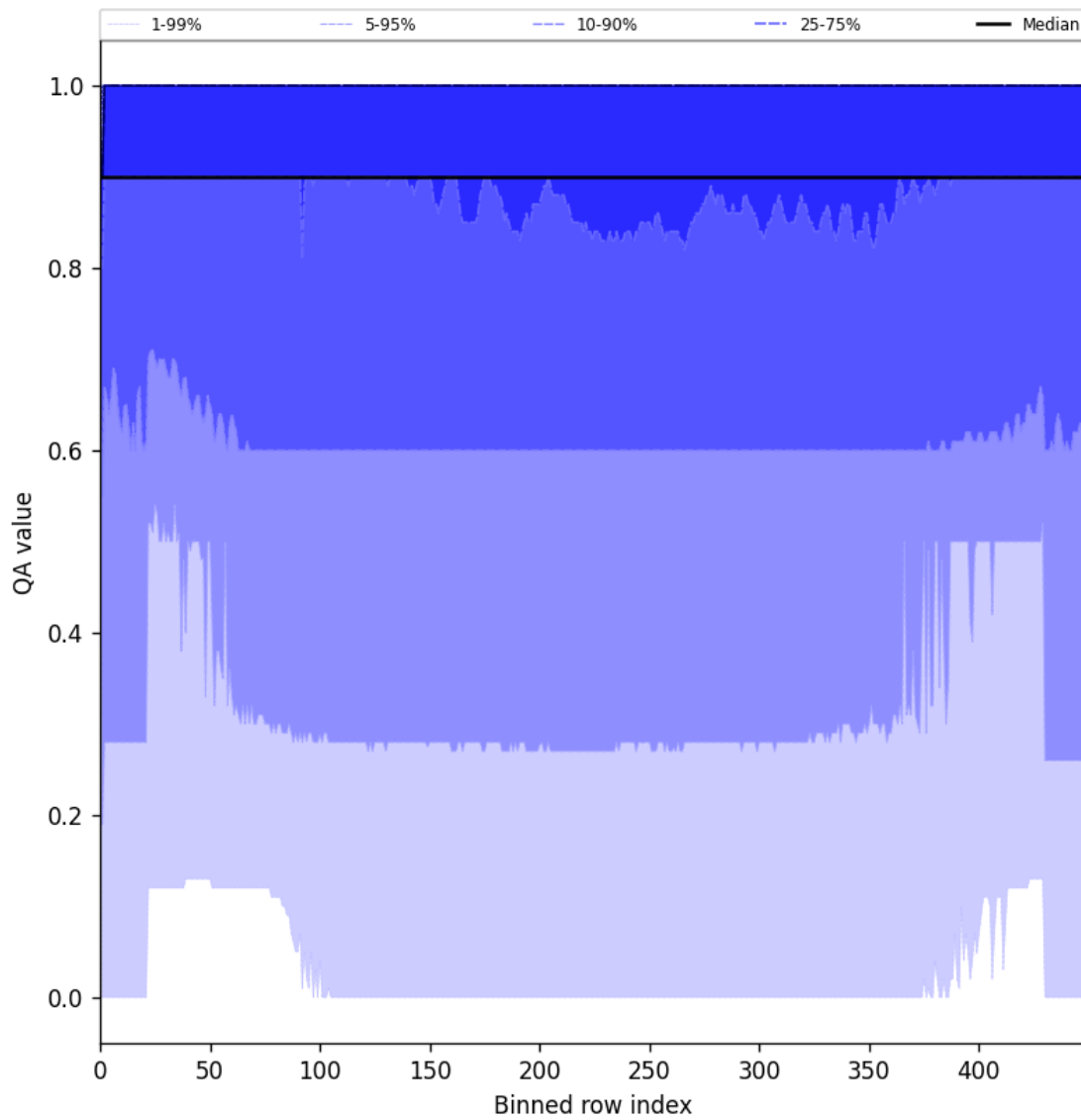
Figure 27: Along track statistics of “QA value” for 2025-06-13 to 2025-06-15
