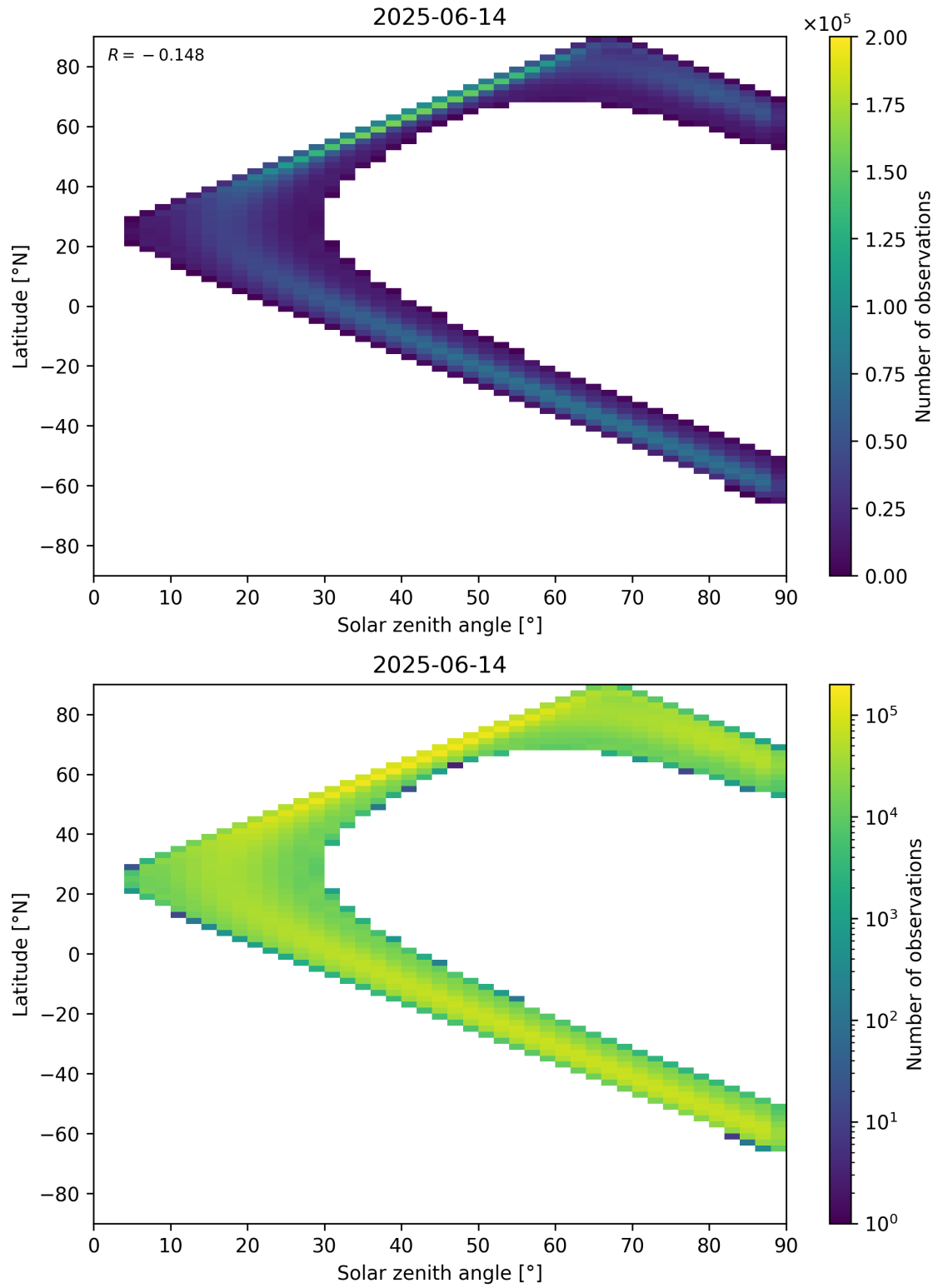
Figure 44: Scatter density plot of “Solar zenith angle” against “Latitude” for 2025-06-13 to 2025-06-15.
