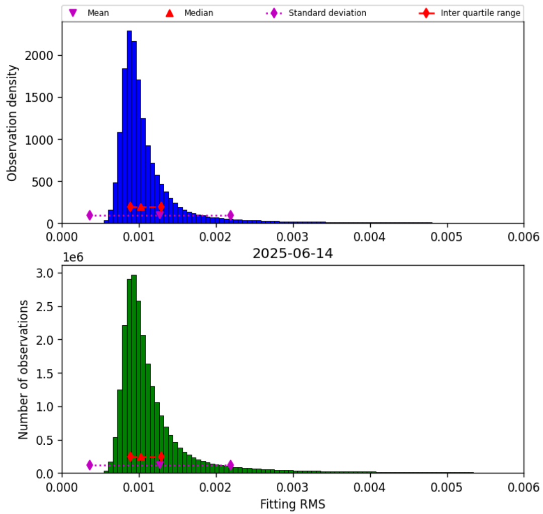
Figure 23: Histogram of “Fitting RMS” for 2025-06-13 to 2025-06-15
