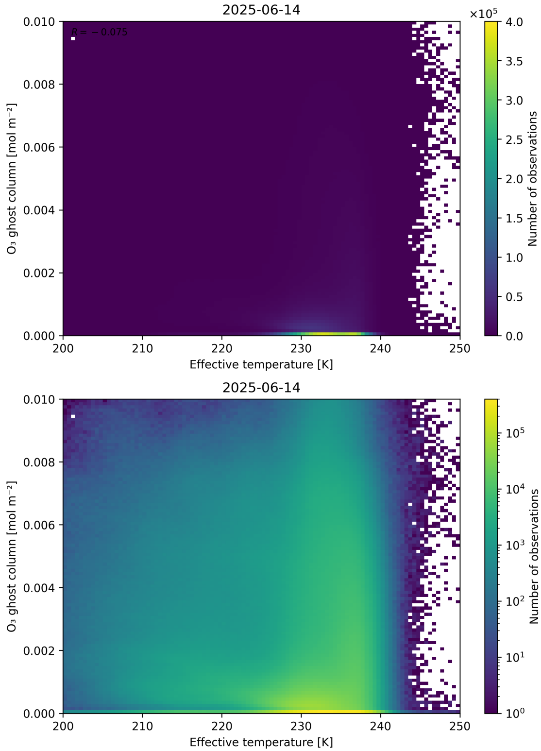
Figure 38: Scatter density plot of “Effective temperature” against “O 3 ghost column” for 2025-06-13 to 2025-06-15.
