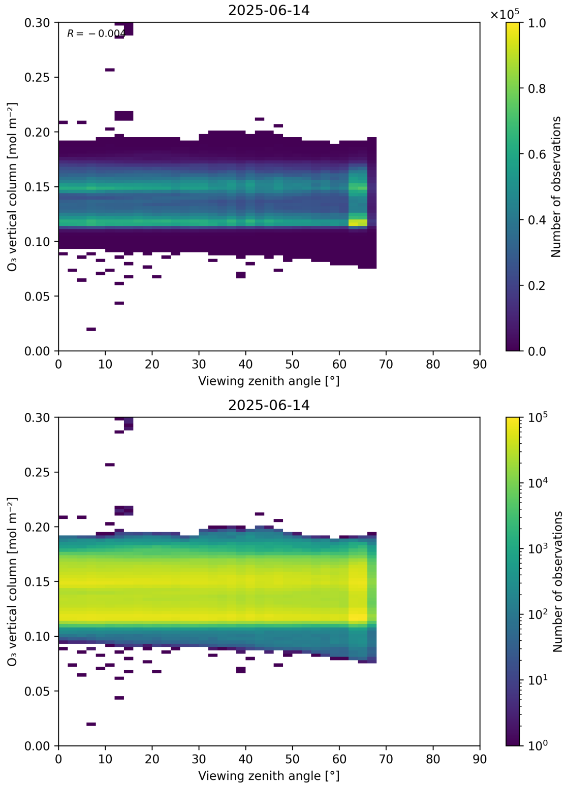
Figure 52: Scatter density plot of “Viewing zenith angle” against “O 3 vertical column” for 2025-06-13 to 2025-06-15.
