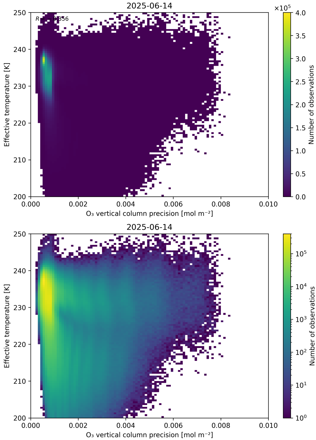
Figure 42: Scatter density plot of “O 3 vertical column precision” against “Effective temperature” for 2025-06-13 to 2025-06-15.
