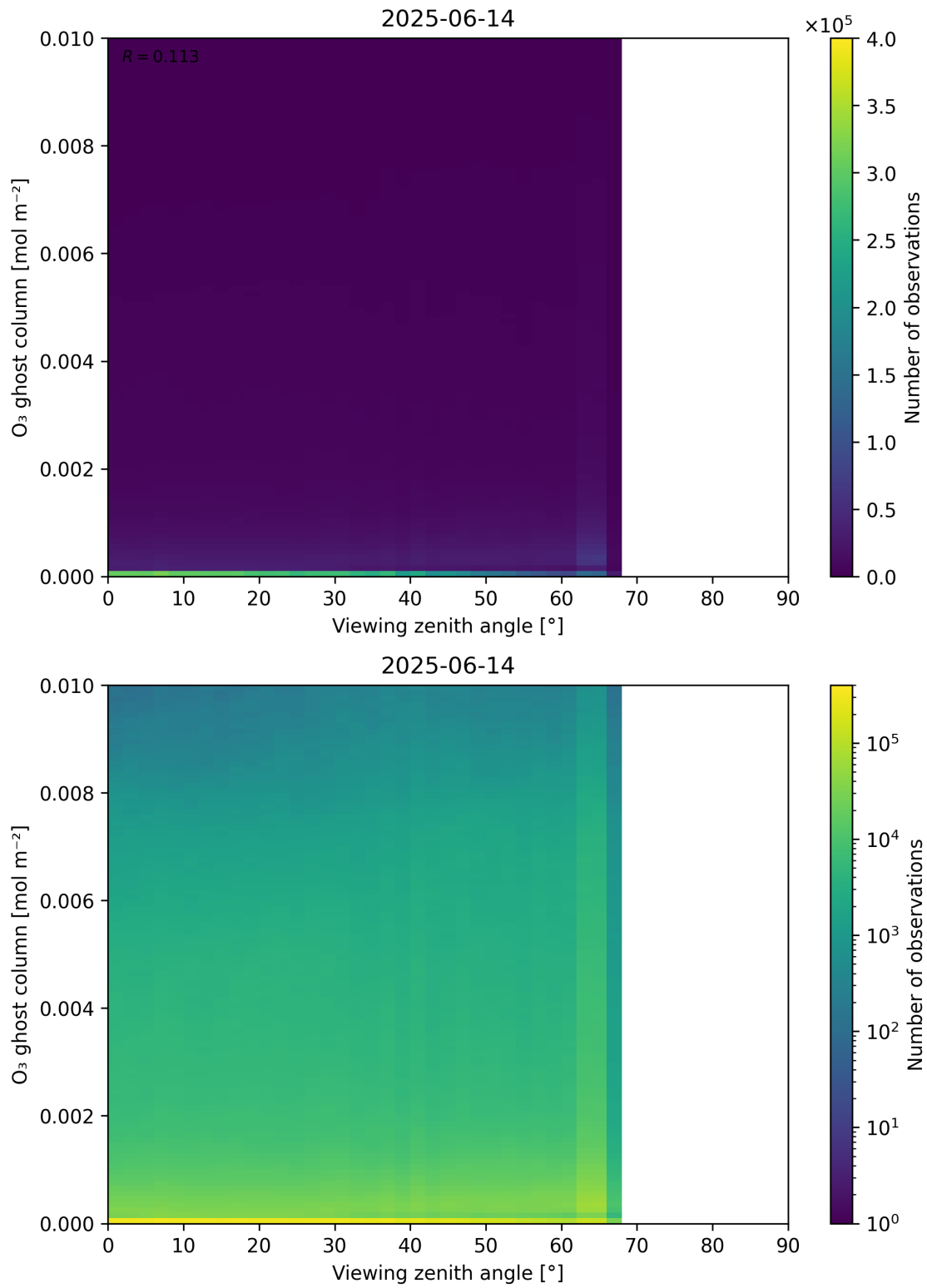
Figure 51: Scatter density plot of “Viewing zenith angle” against “O 3 ghost column” for 2025-06-13 to 2025-06-15.
