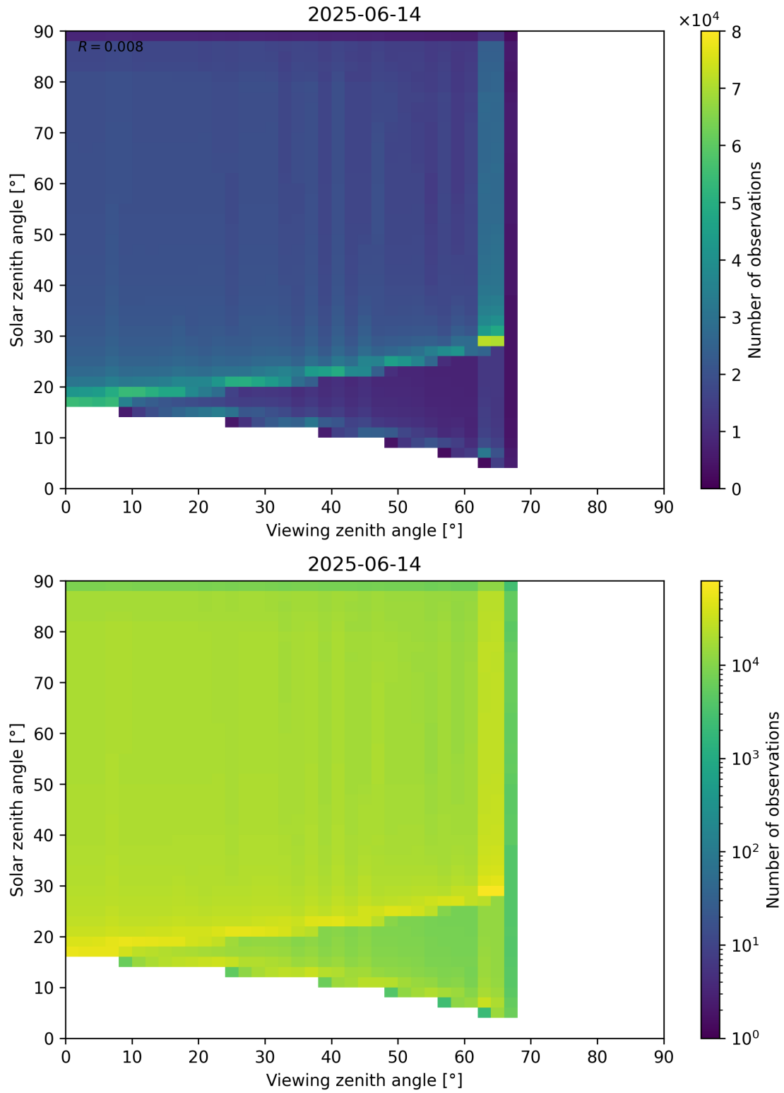
Figure 54: Scatter density plot of “Viewing zenith angle” against “Solar zenith angle” for 2025-06-13 to 2025-06-15.
