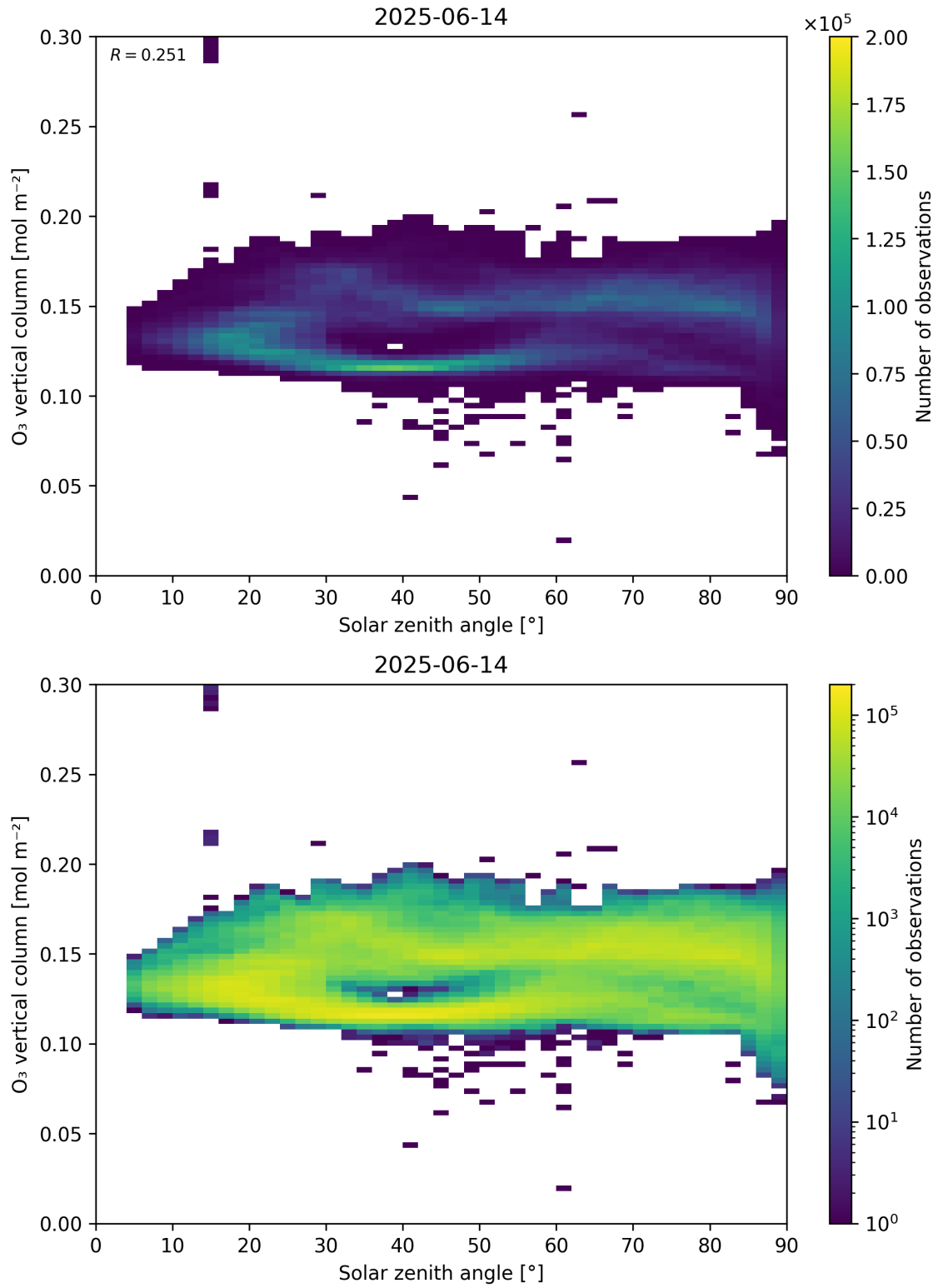
Figure 47: Scatter density plot of “Solar zenith angle” against “O 3 vertical column” for 2025-06-13 to 2025-06-15.
