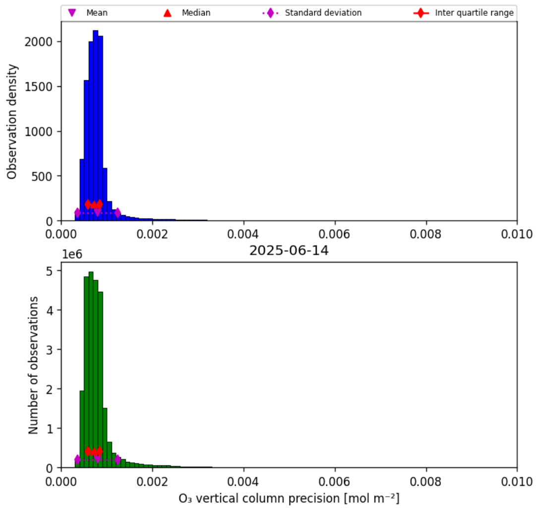
Figure 22: Histogram of “O 3 vertical column precision” for 2025-06-13 to 2025-06-15
