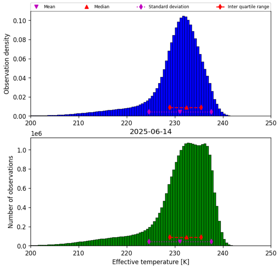
Figure 24: Histogram of “Effective temperature” for 2025-06-13 to 2025-06-15
