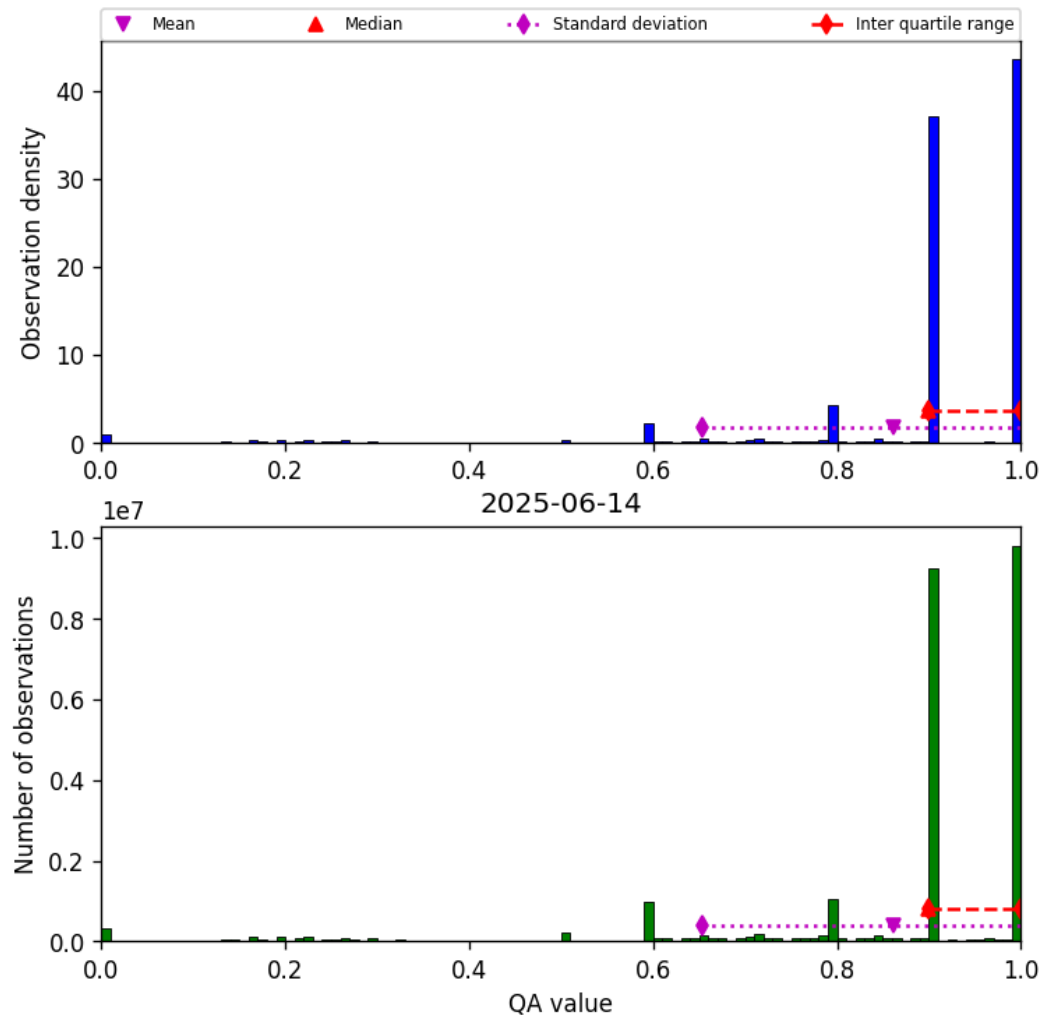
Figure 20: Histogram of “QA value” for 2025-06-13 to 2025-06-15
