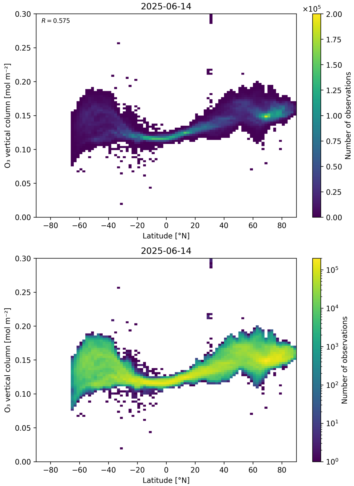
Figure 36: Scatter density plot of “Latitude” against “O 3 vertical column” for 2025-06-13 to 2025-06-15.
