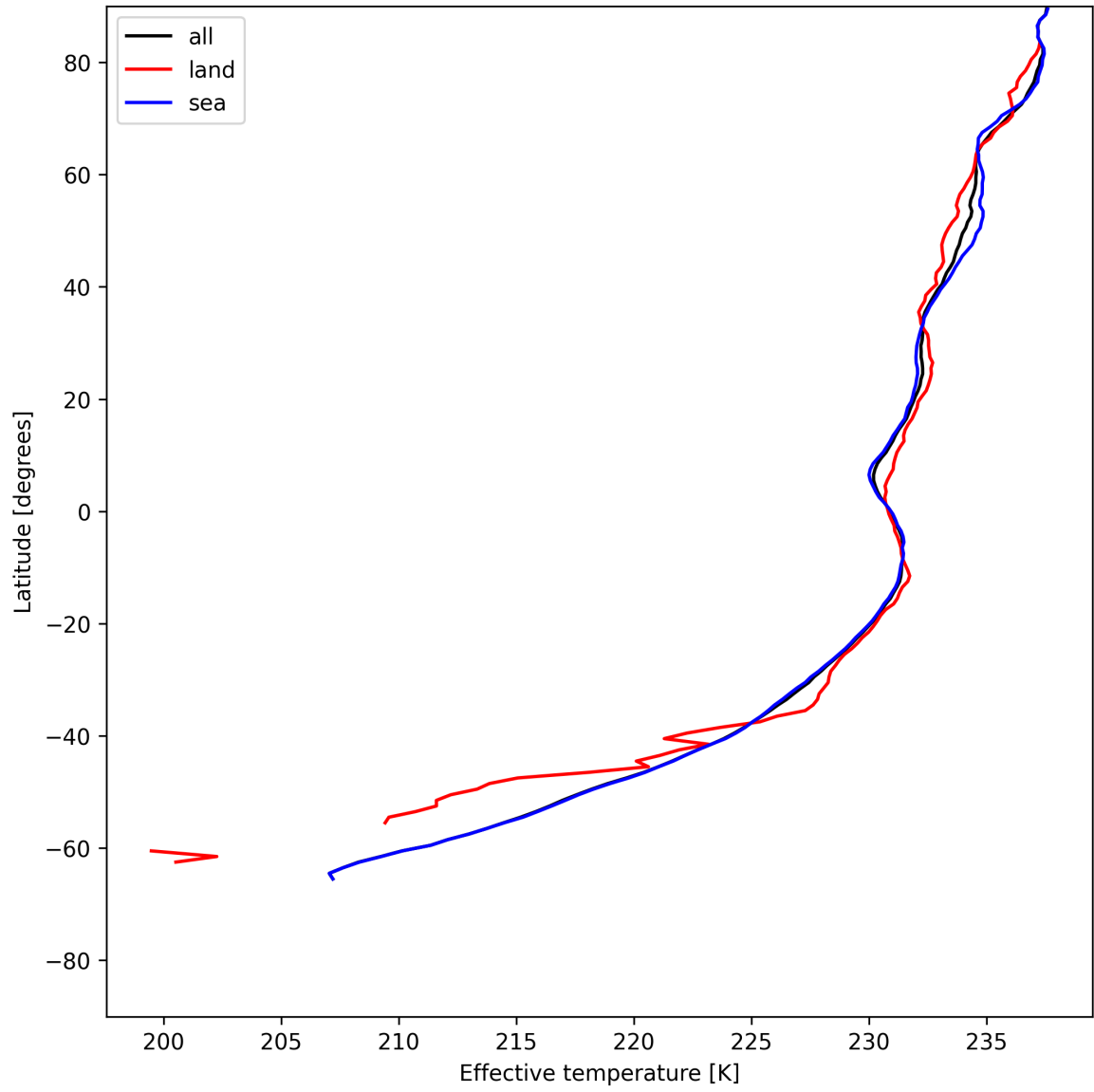
Figure 17: Zonal average of "Effective temperature" for 2025-06-13 to 2025-06-15.
