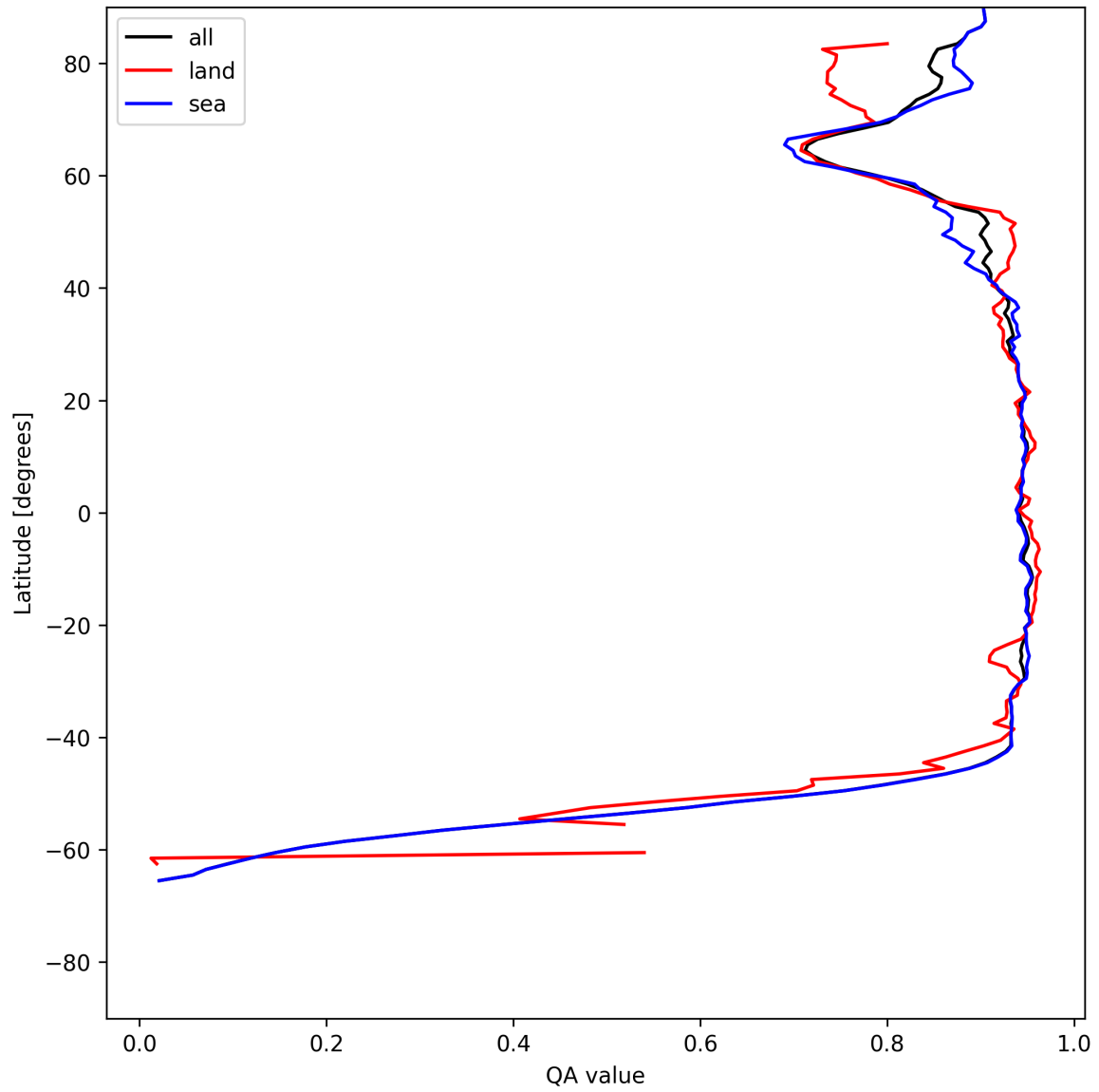
Figure 13: Zonal average of “QA value” for 2025-06-13 to 2025-06-15.
