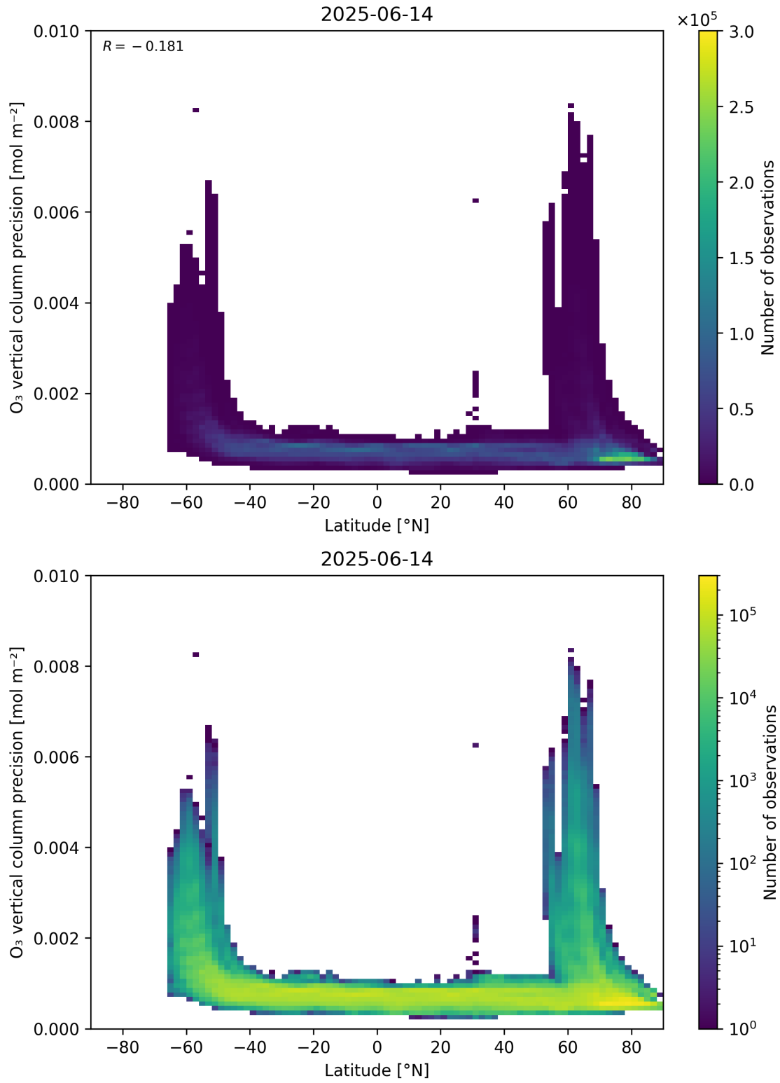
Figure 37: Scatter density plot of “Latitude” against “O 3 vertical column precision” for 2025-06-13 to 2025-06-15.
