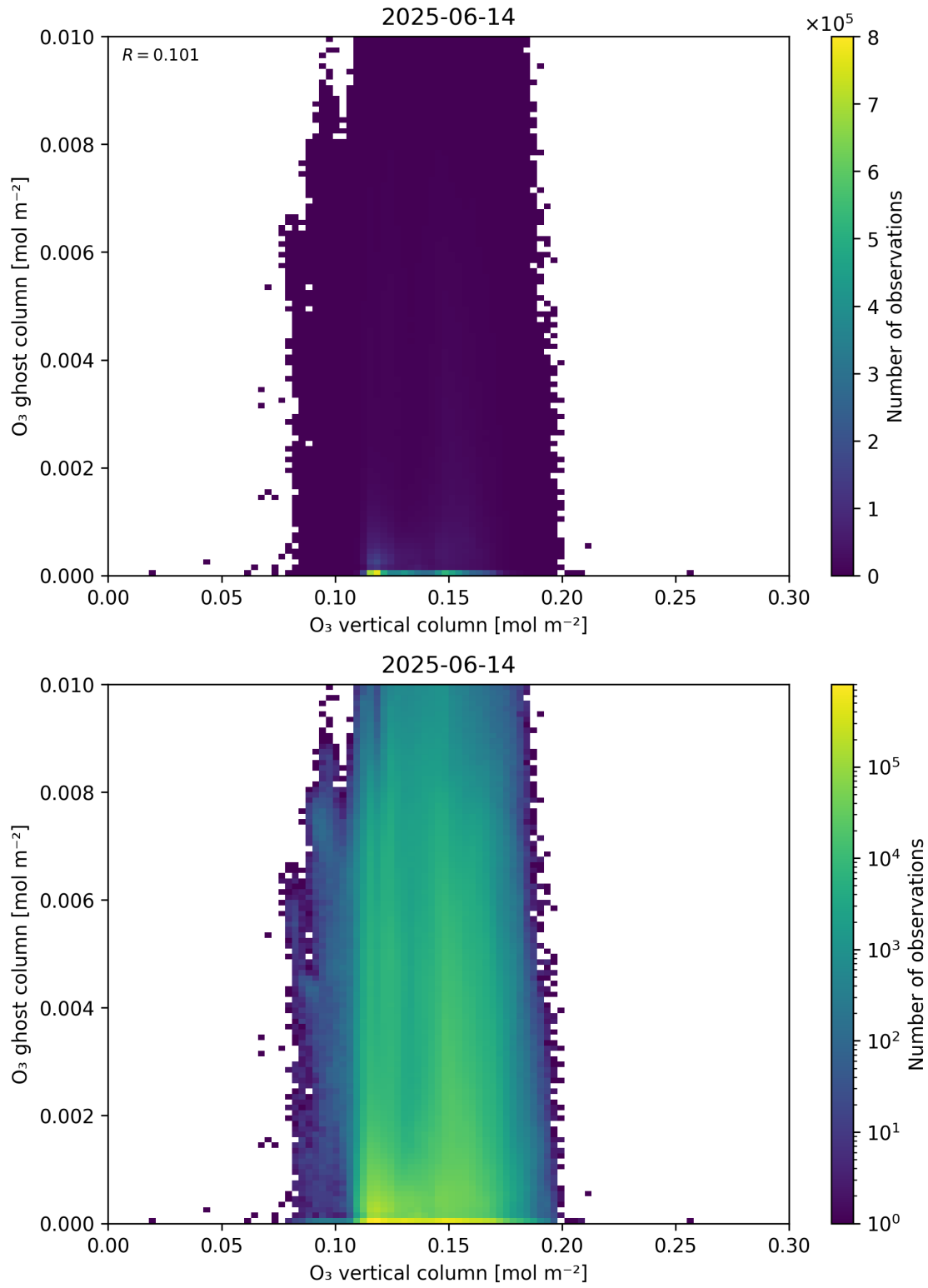
Figure 40: Scatter density plot of “O 3 vertical column” against “O 3 ghost column” for 2025-06-13 to 2025-06-15.
