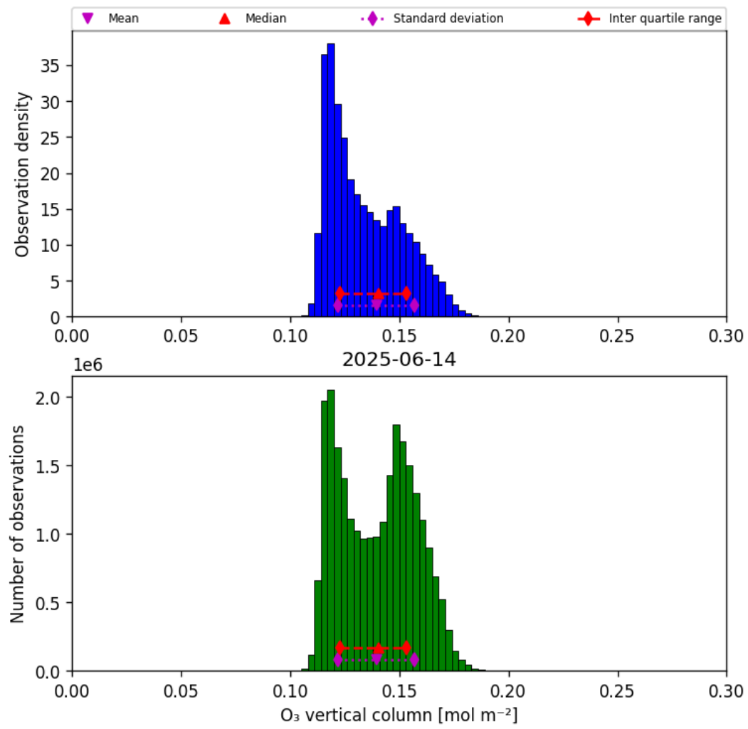
Figure 21: Histogram of “O 3 vertical column” for 2025-06-13 to 2025-06-15
