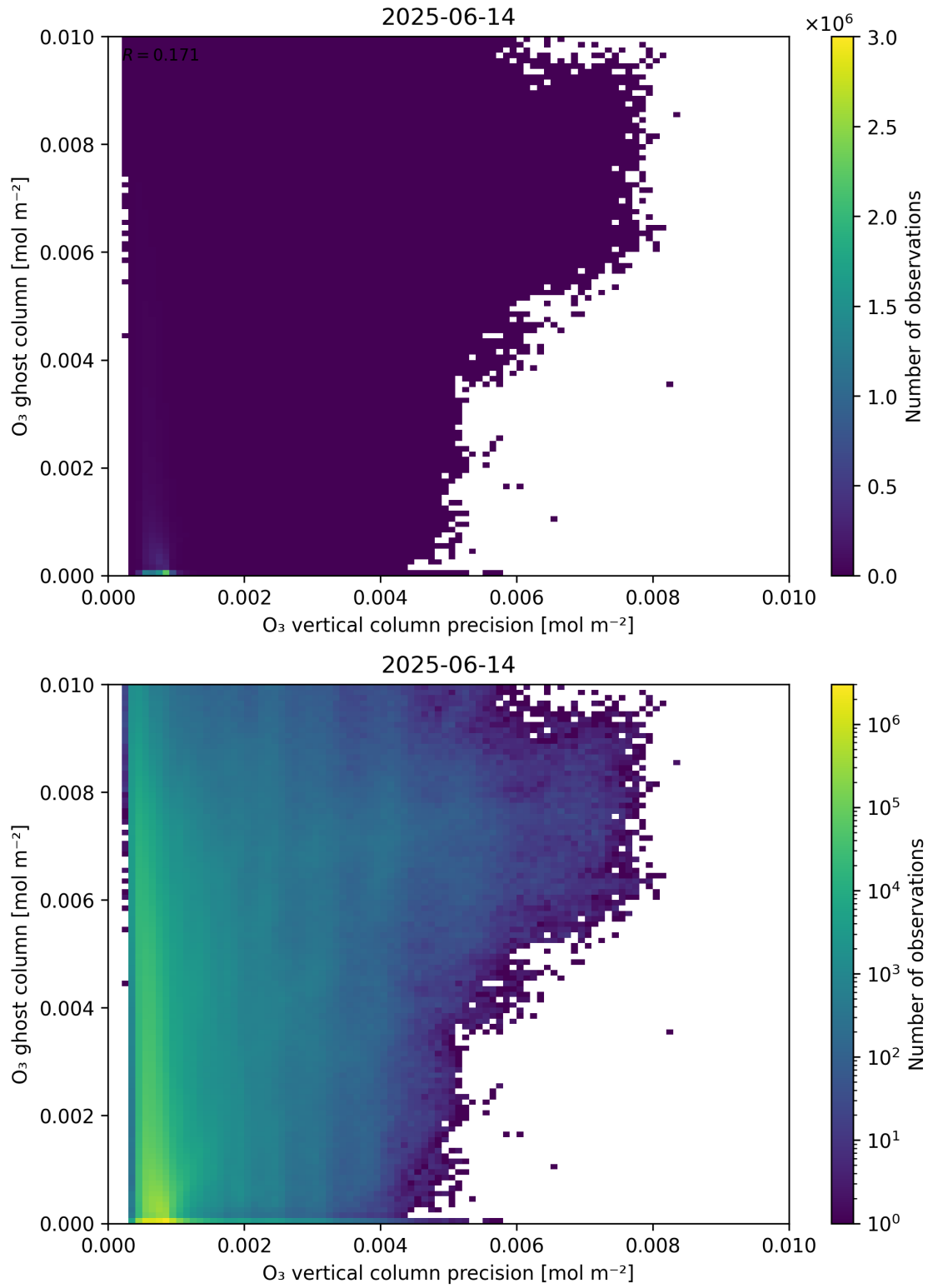
Figure 43: Scatter density plot of “ \text{O}_3 vertical column precision” against “ \text{O}_3 ghost column” for 2025-06-13 to 2025-06-15.
