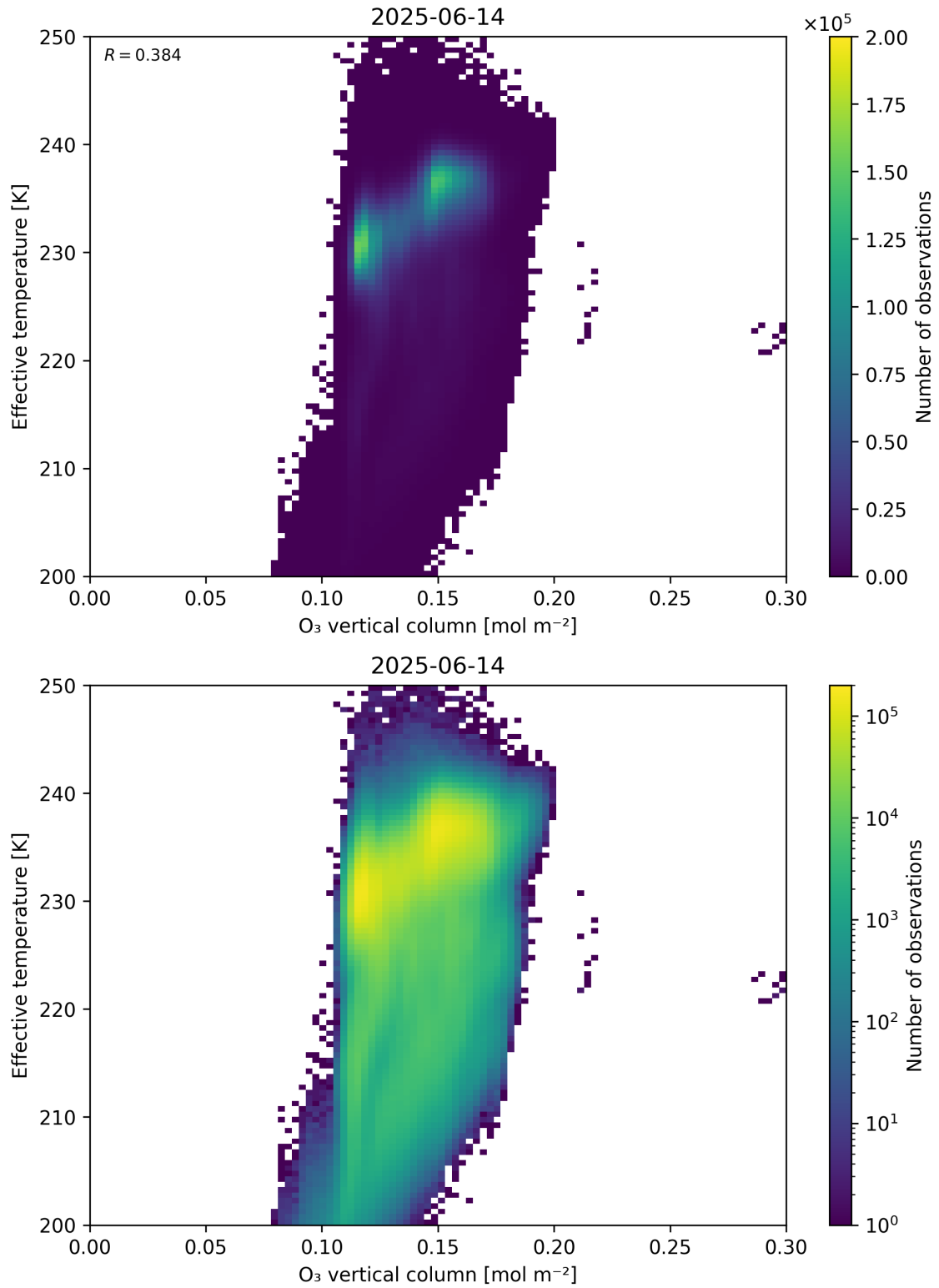
Figure 39: Scatter density plot of “O 3 vertical column” against “Effective temperature” for 2025-06-13 to 2025-06-15.
