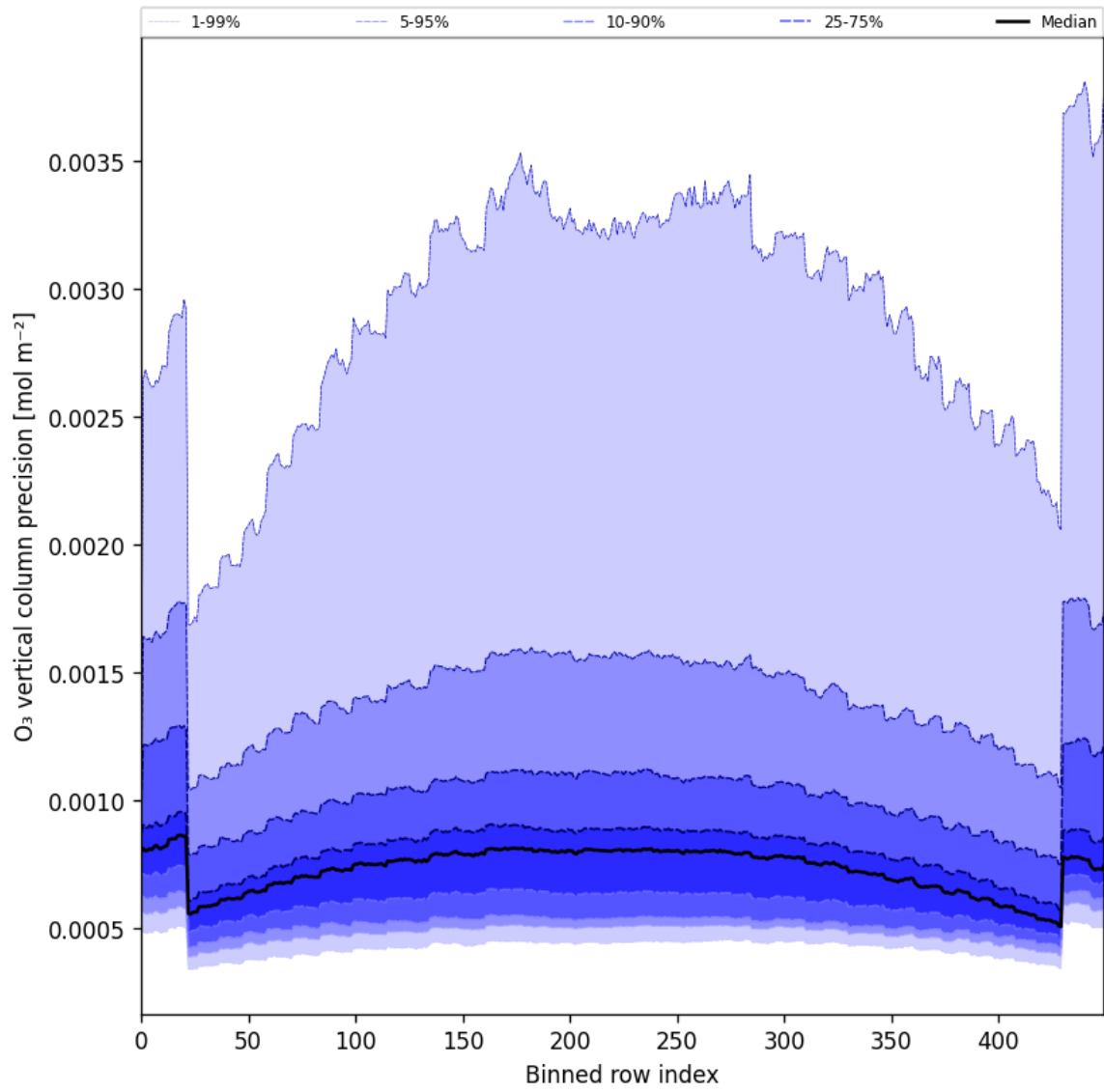
Figure 29: Along track statistics of “O 3 vertical column precision” for 2025-06-13 to 2025-06-15
