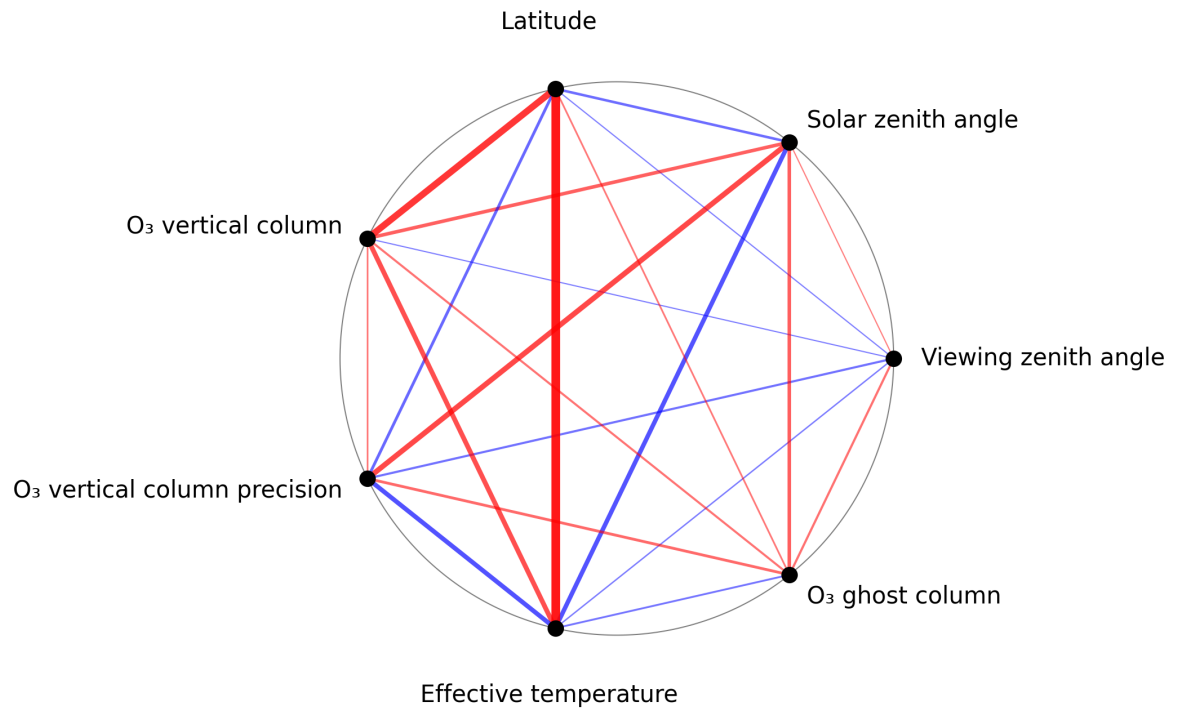
Figure 1: Map of correlation graph for 2025-06-13 to 2025-06-15.
