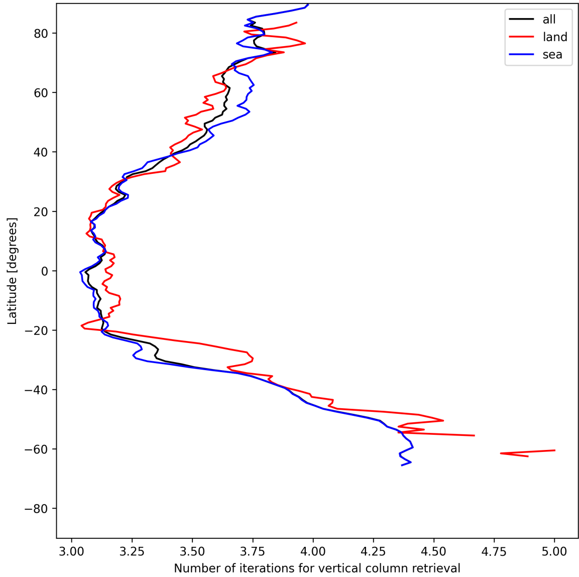
Figure 19: Zonal average of “Number of iterations for vertical column retrieval” for 2025-06-13 to 2025-06-15.
