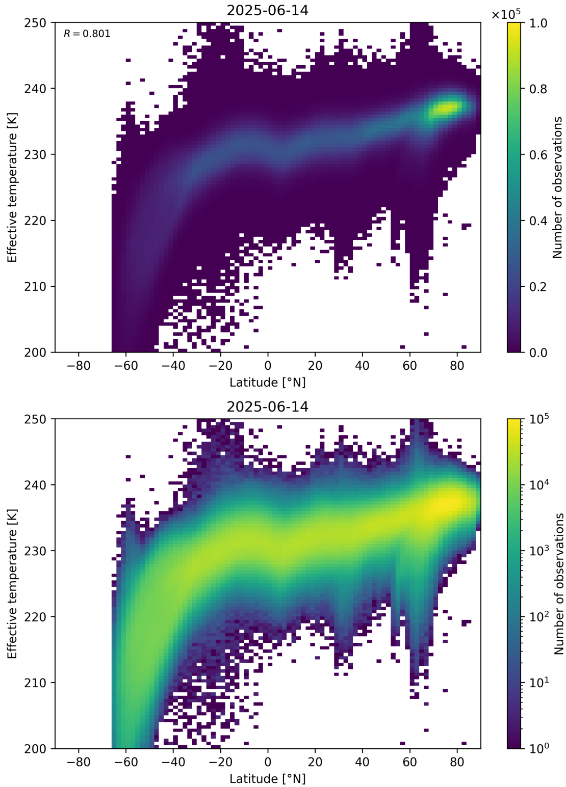
Figure 34: Scatter density plot of “Latitude” against “Effective temperature” for 2025-06-13 to 2025-06-15.
