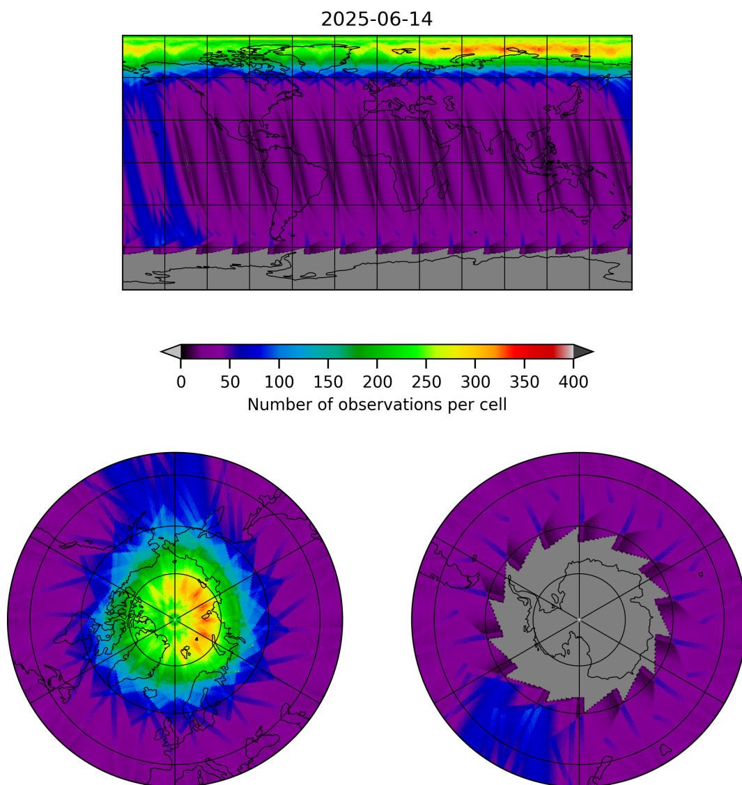
Figure 12: Map of the number of observations for 2025-06-13 to 2025-06-15
