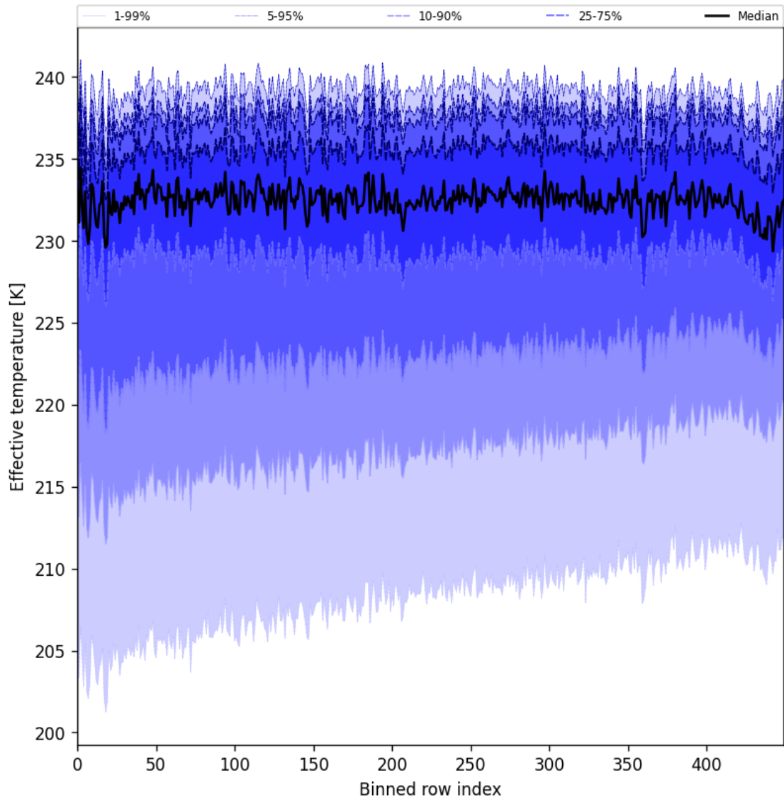
Figure 31: Along track statistics of “Effective temperature” for 2025-06-13 to 2025-06-15
