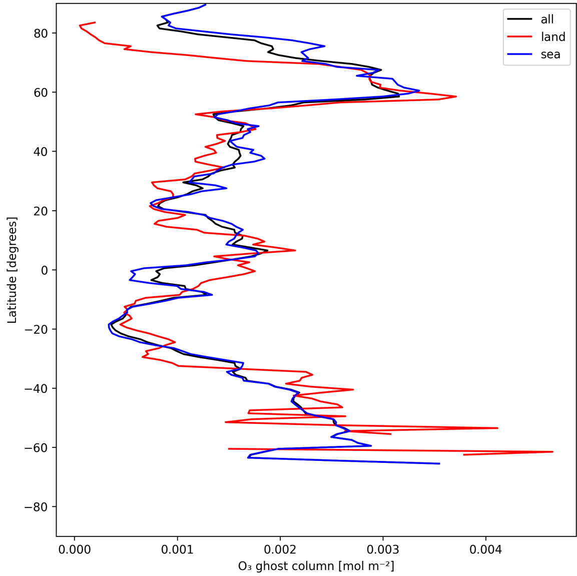
Figure 18: Zonal average of "O 3 ghost column" for 2025-06-13 to 2025-06-15.
