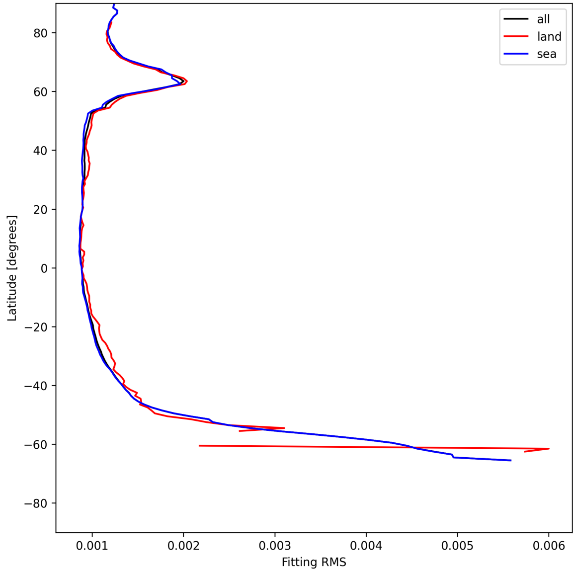
Figure 16: Zonal average of “Fitting RMS” for 2025-06-13 to 2025-06-15.
