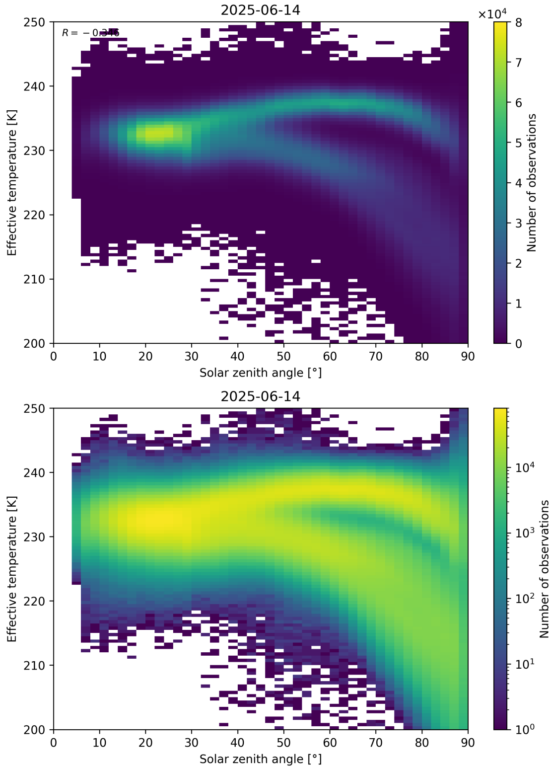
Figure 45: Scatter density plot of “Solar zenith angle” against “Effective temperature” for 2025-06-13 to 2025-06-15.
