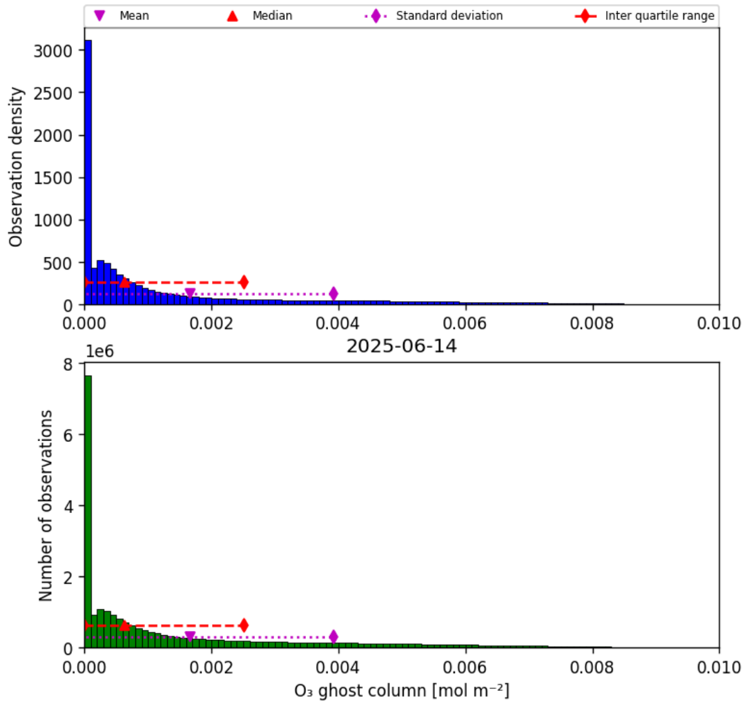
Figure 25: Histogram of “O 3 ghost column” for 2025-06-13 to 2025-06-15
