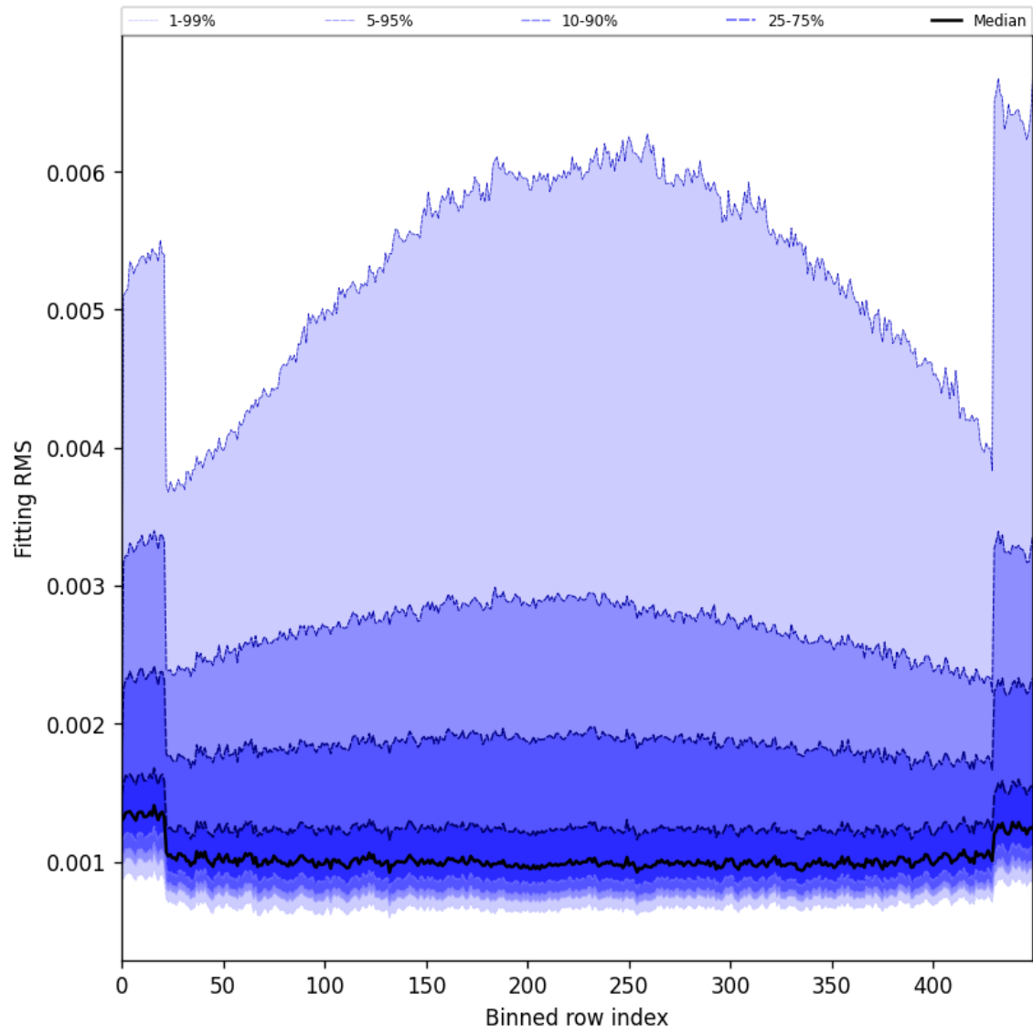
Figure 30: Along track statistics of “Fitting RMS” for 2025-06-13 to 2025-06-15
