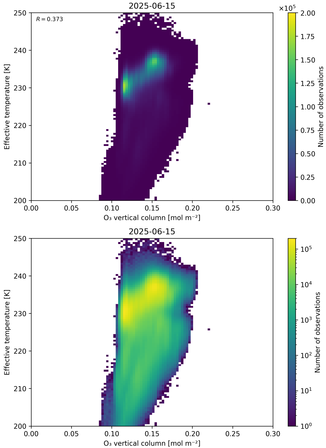
Figure 39: Scatter density plot of “O 3 vertical column” against “Effective temperature” for 2025-06-14 to 2025-06-16.
