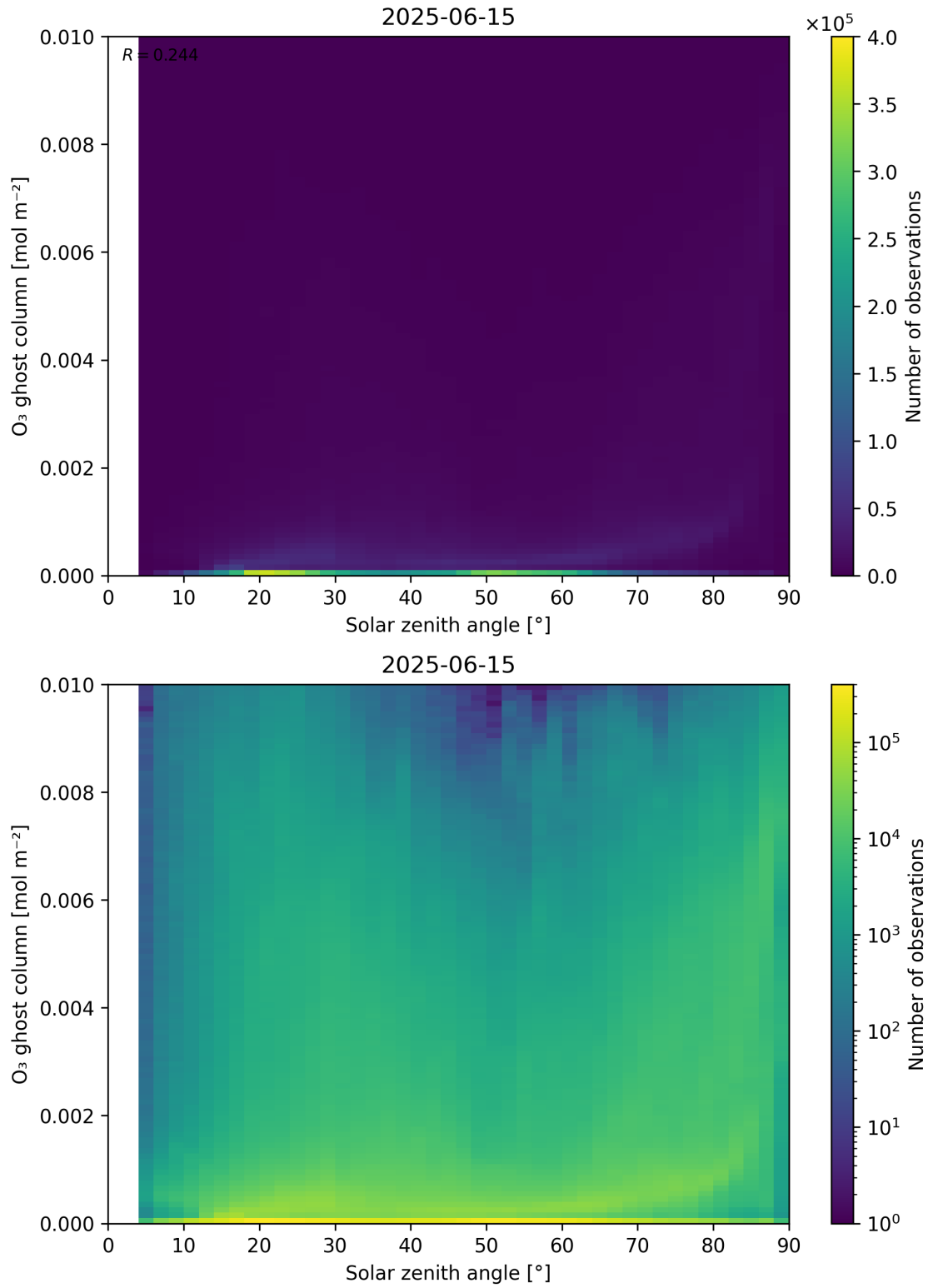
Figure 46: Scatter density plot of “Solar zenith angle” against “O 3 ghost column” for 2025-06-14 to 2025-06-16.
