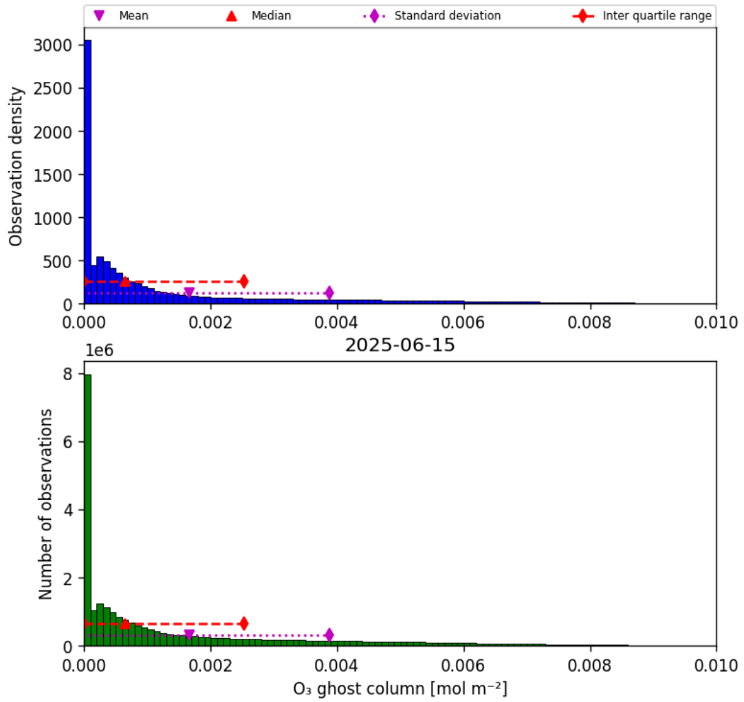
Figure 25: Histogram of “O 3 ghost column” for 2025-06-14 to 2025-06-16
