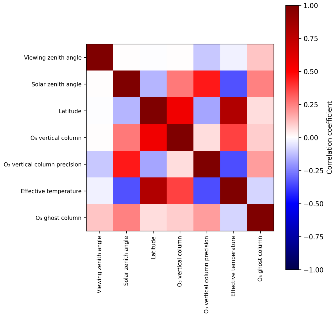
Figure 2: Map of correlation matrix for 2025-06-14 to 2025-06-16.
