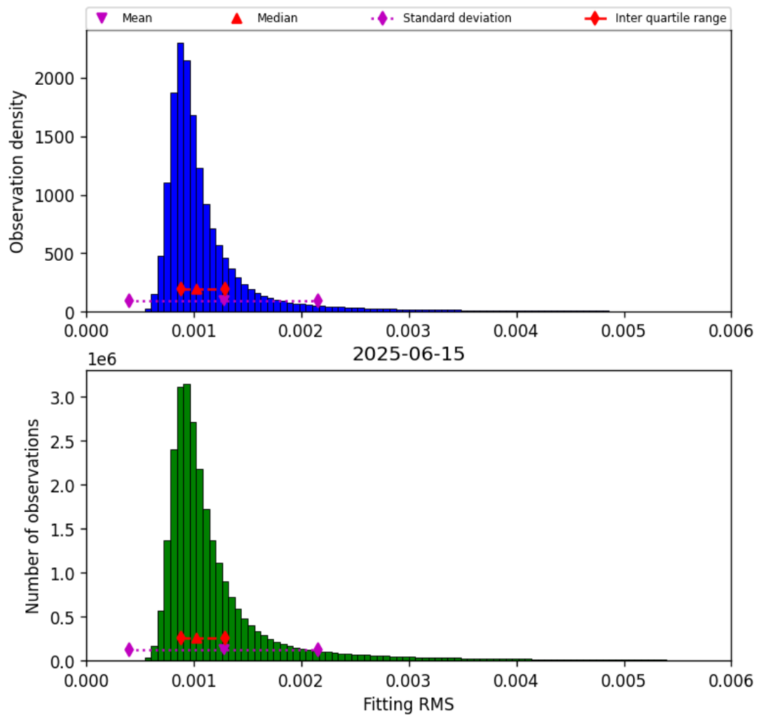
Figure 23: Histogram of “Fitting RMS” for 2025-06-14 to 2025-06-16
