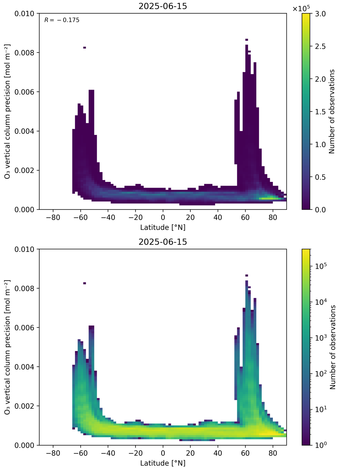
Figure 37: Scatter density plot of “Latitude” against “O 3 vertical column precision” for 2025-06-14 to 2025-06-16.
