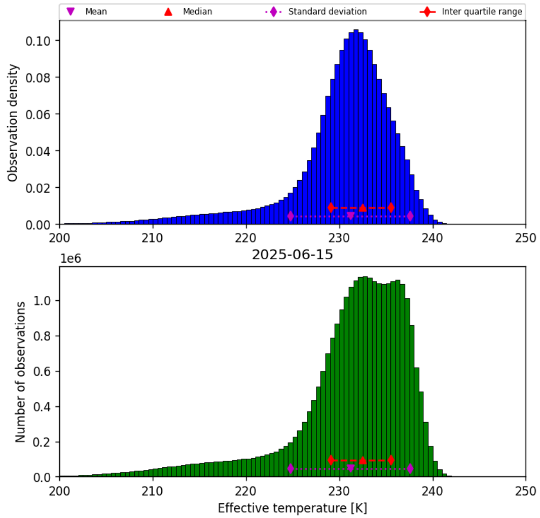
Figure 24: Histogram of “Effective temperature” for 2025-06-14 to 2025-06-16
