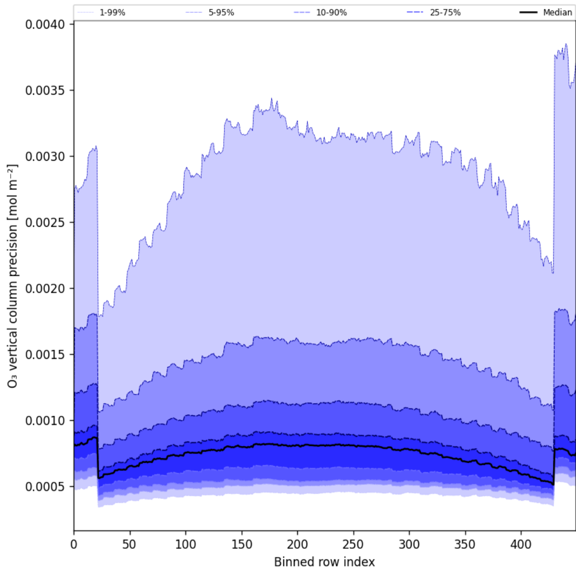
Figure 29: Along track statistics of “O 3 vertical column precision” for 2025-06-14 to 2025-06-16
