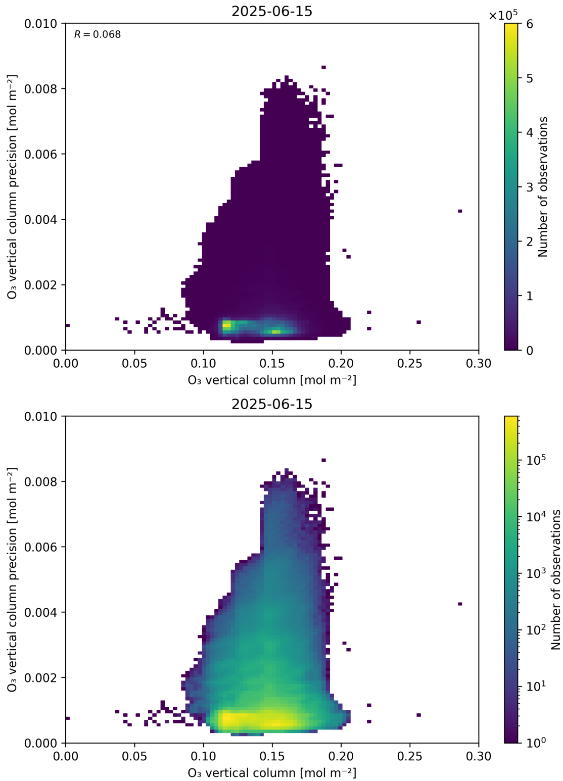
Figure 41: Scatter density plot of “O 3 vertical column” against “O 3 vertical column precision” for 2025-06-14 to 2025-06-16.
