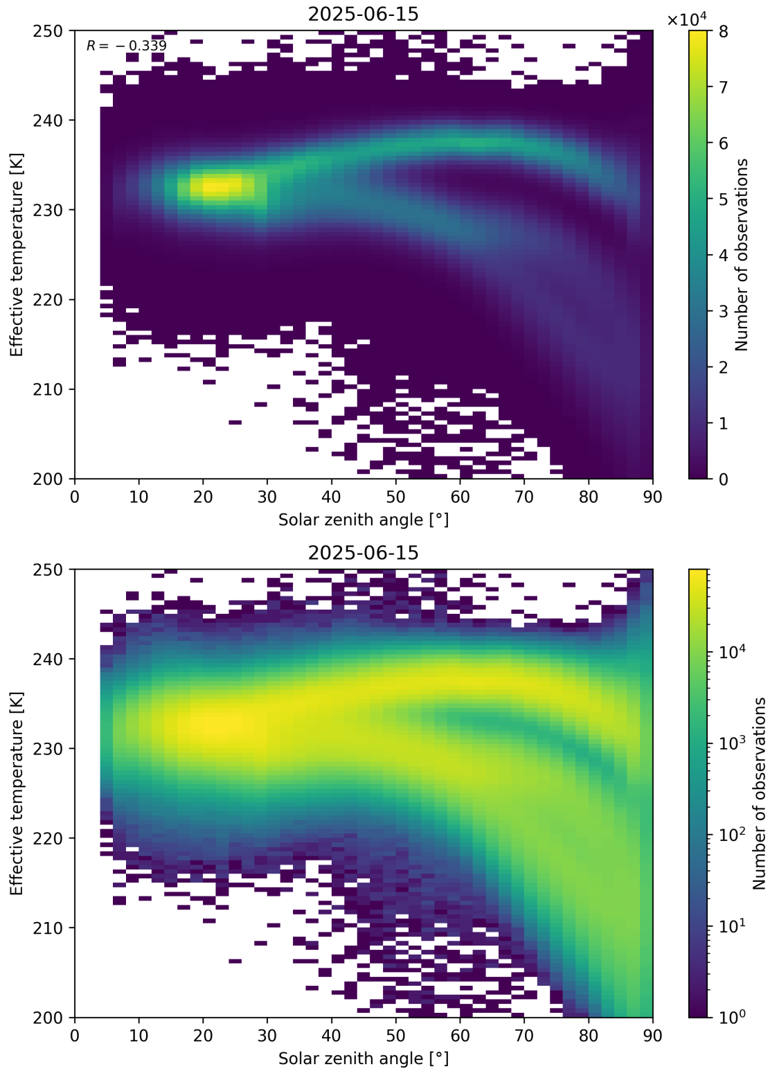
Figure 45: Scatter density plot of “Solar zenith angle” against “Effective temperature” for 2025-06-14 to 2025-06-16.
