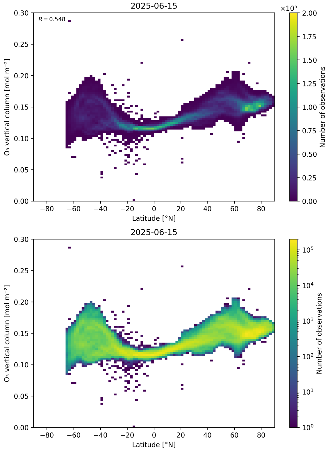
Figure 36: Scatter density plot of “Latitude” against “O 3 vertical column” for 2025-06-14 to 2025-06-16.
