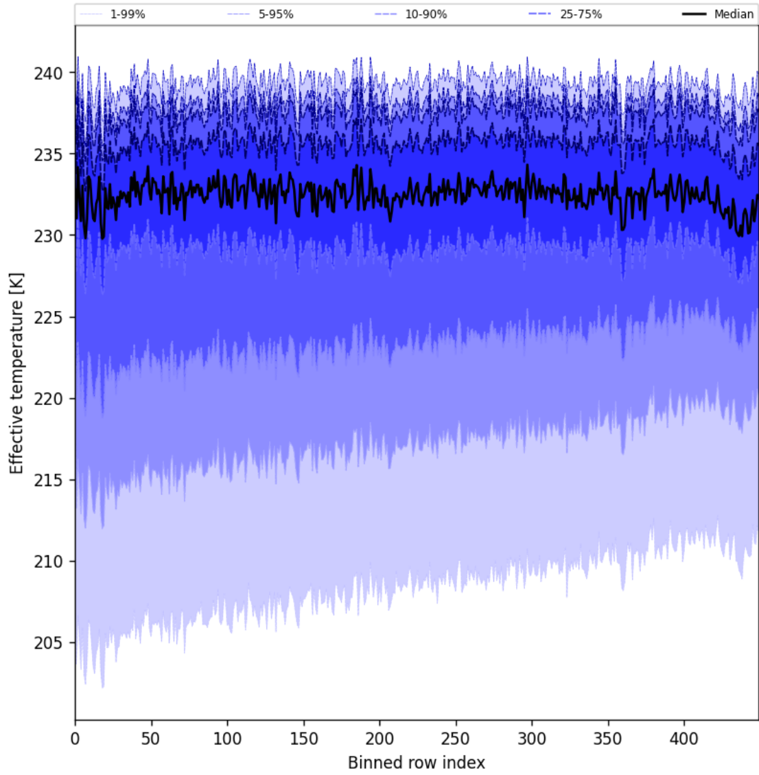
Figure 31: Along track statistics of “Effective temperature” for 2025-06-14 to 2025-06-16
