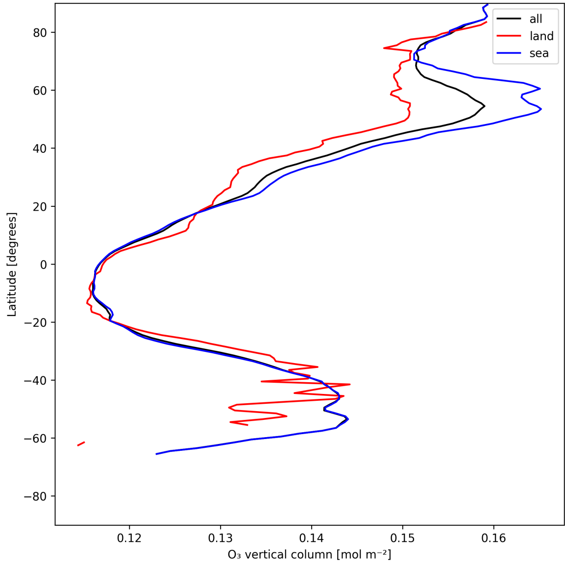
Figure 14: Zonal average of “O 3 vertical column” for 2025-06-14 to 2025-06-16.
