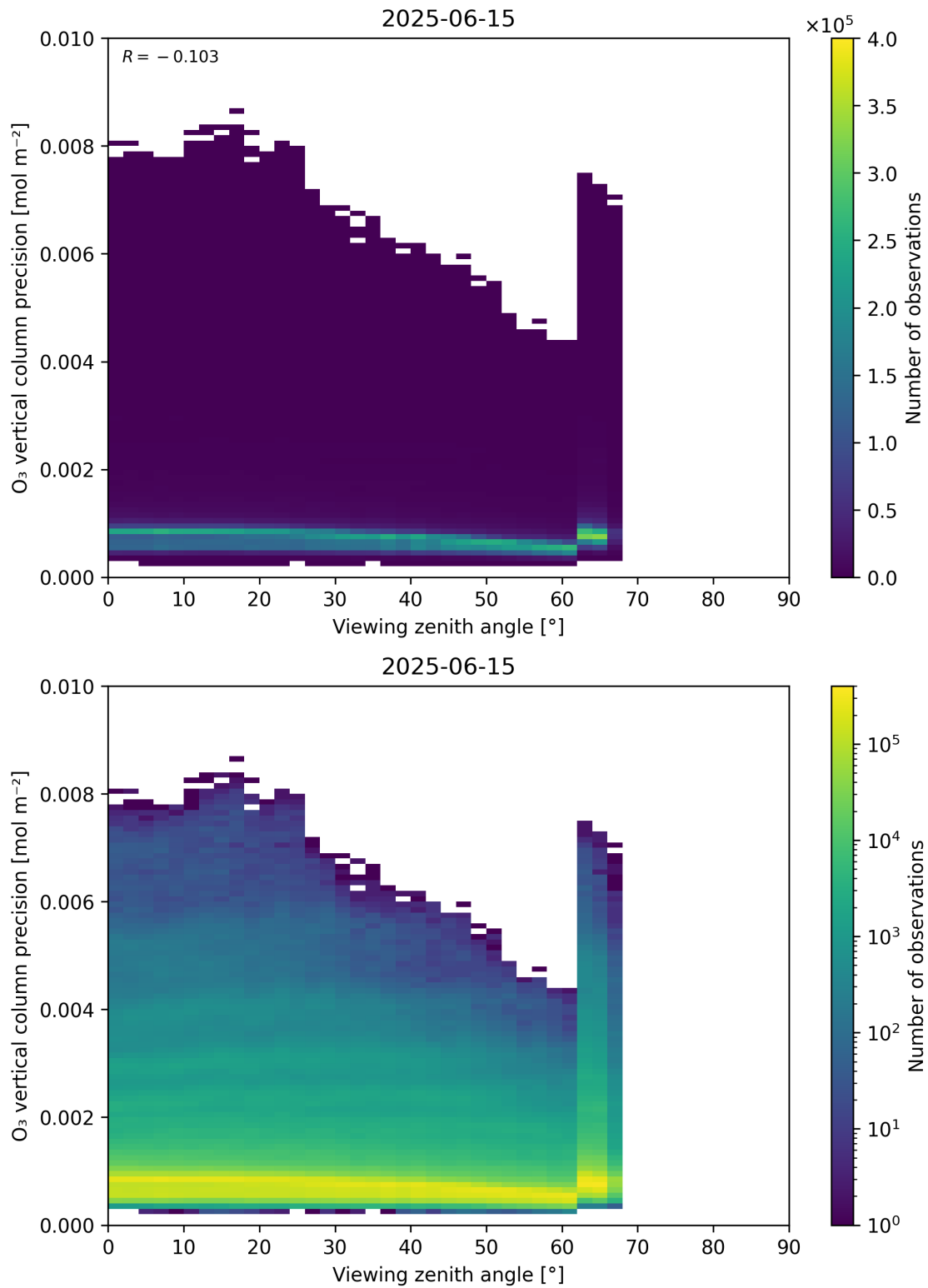
Figure 53: Scatter density plot of “Viewing zenith angle” against “O 3 vertical column precision” for 2025-06-14 to 2025-06-16.
