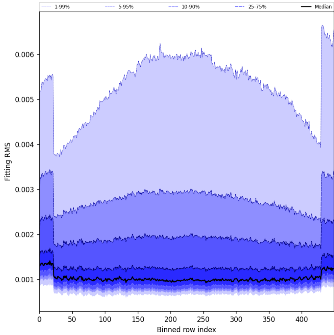
Figure 30: Along track statistics of “Fitting RMS” for 2025-06-14 to 2025-06-16
