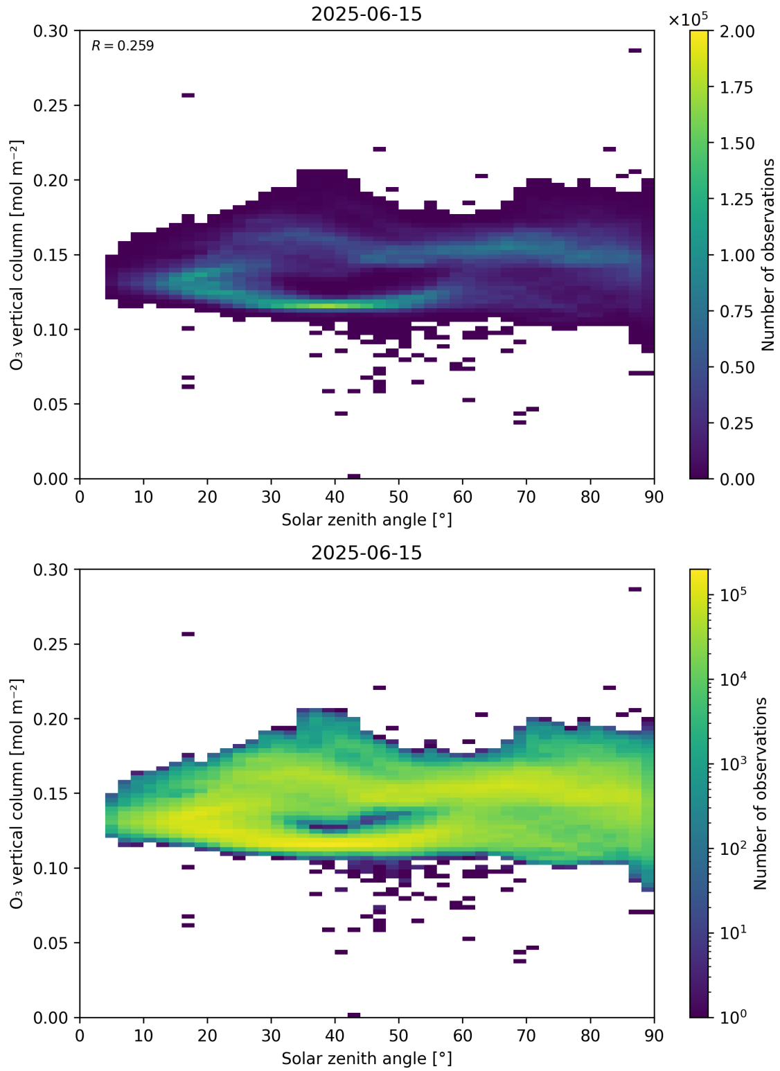
Figure 47: Scatter density plot of “Solar zenith angle” against “O 3 vertical column” for 2025-06-14 to 2025-06-16.
