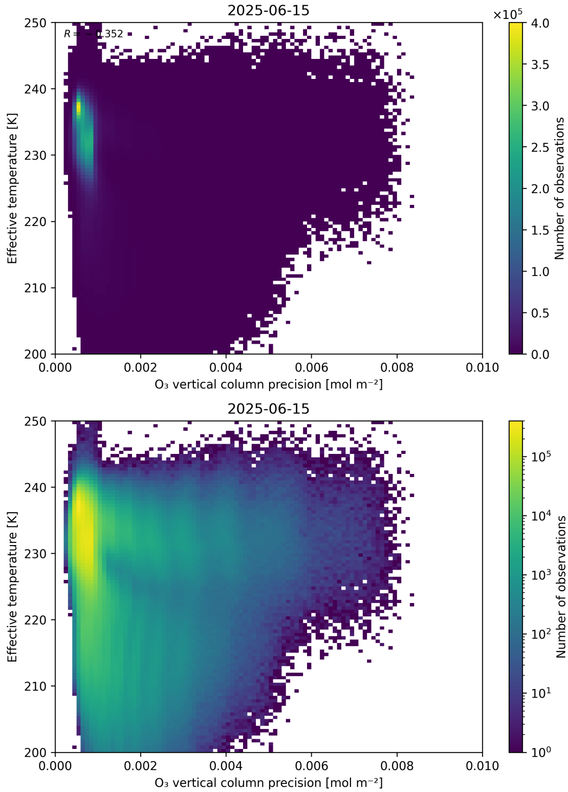
Figure 42: Scatter density plot of “O 3 vertical column precision” against “Effective temperature” for 2025-06-14 to 2025-06-16.
