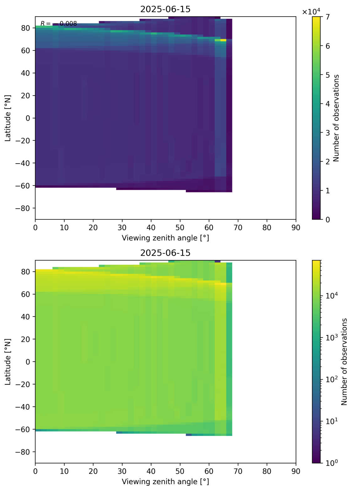
Figure 49: Scatter density plot of “Viewing zenith angle” against “Latitude” for 2025-06-14 to 2025-06-16.
