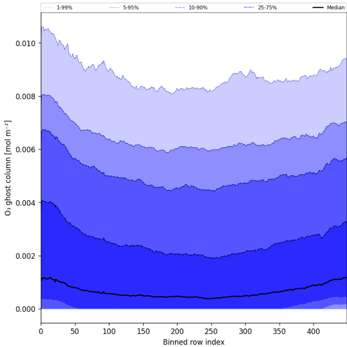
Figure 32: Along track statistics of “O 3 ghost column” for 2025-06-14 to 2025-06-16
