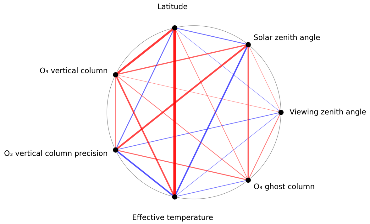
Figure 1: Map of correlation graph for 2025-06-14 to 2025-06-16.
