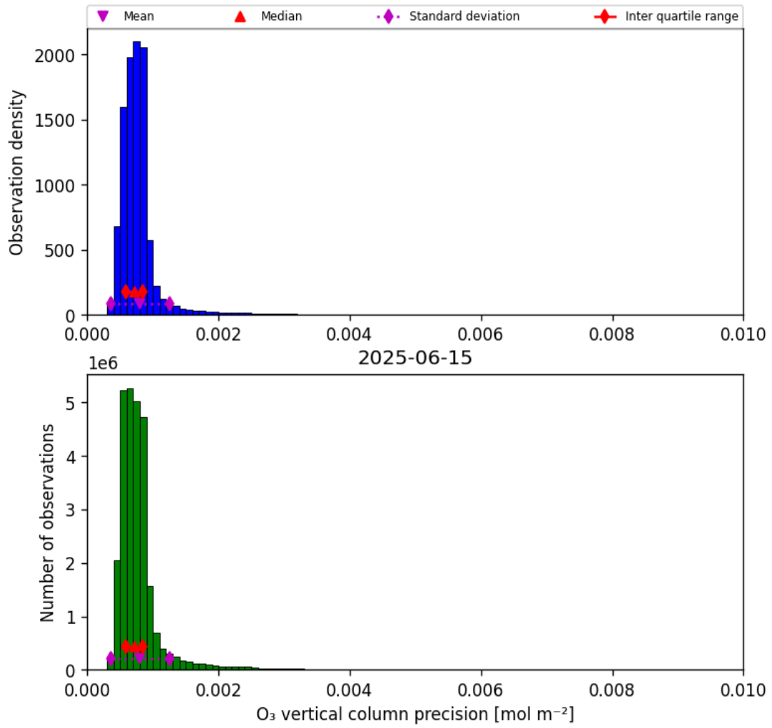
Figure 22: Histogram of “O 3 vertical column precision” for 2025-06-14 to 2025-06-16
