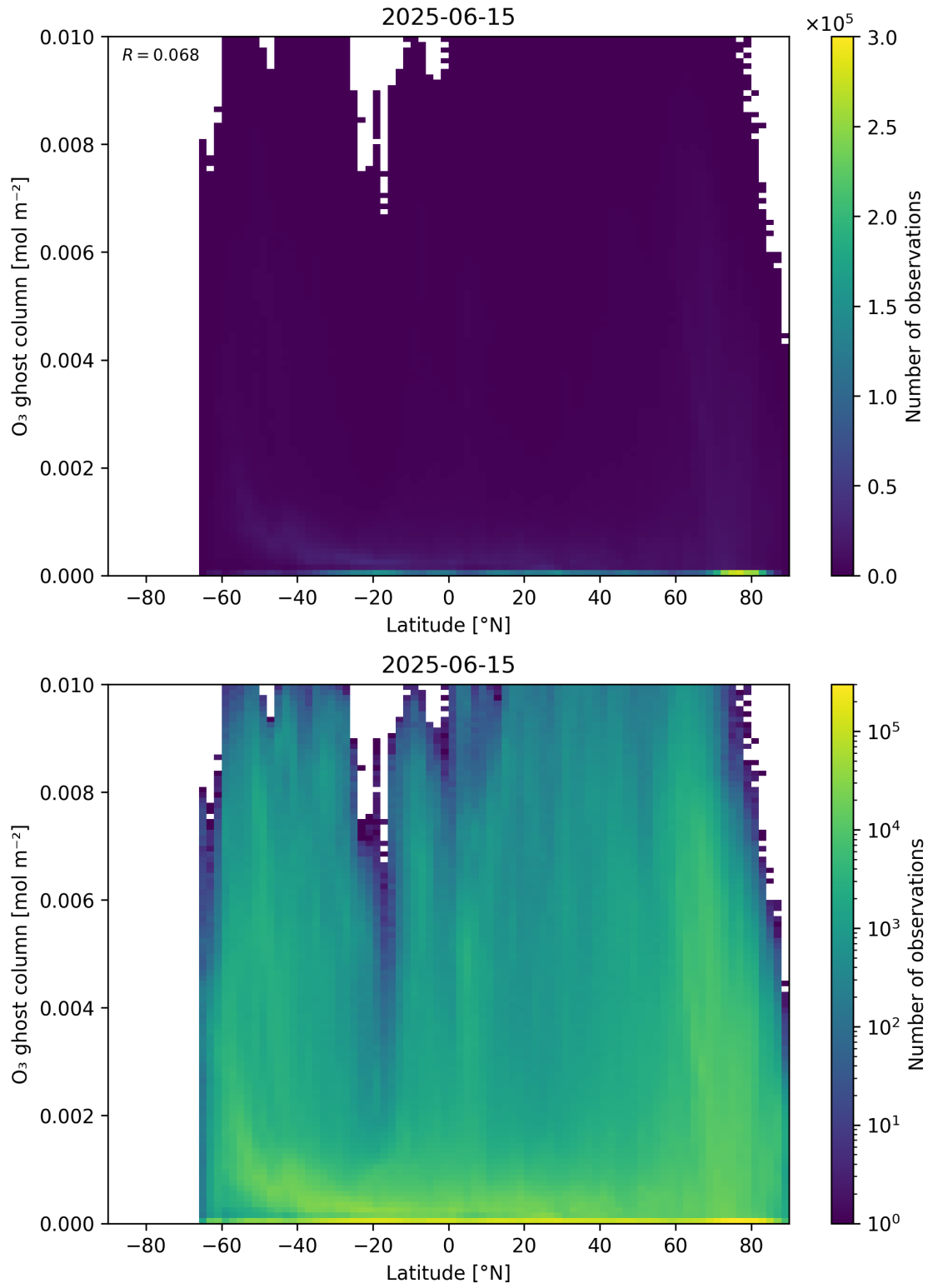
Figure 35: Scatter density plot of “Latitude” against “O 3 ghost column” for 2025-06-14 to 2025-06-16.
