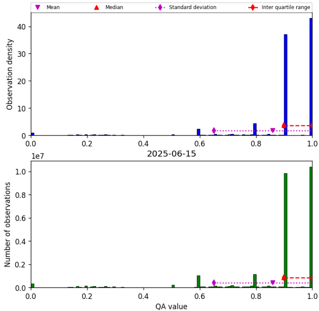
Figure 20: Histogram of “QA value” for 2025-06-14 to 2025-06-16
