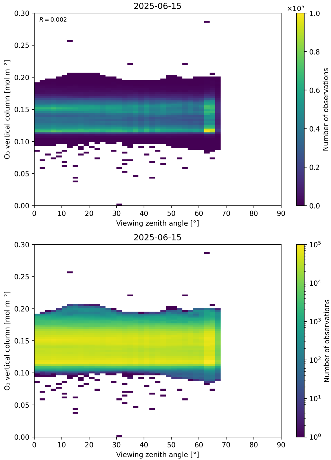
Figure 52: Scatter density plot of “Viewing zenith angle” against “O 3 vertical column” for 2025-06-14 to 2025-06-16.
