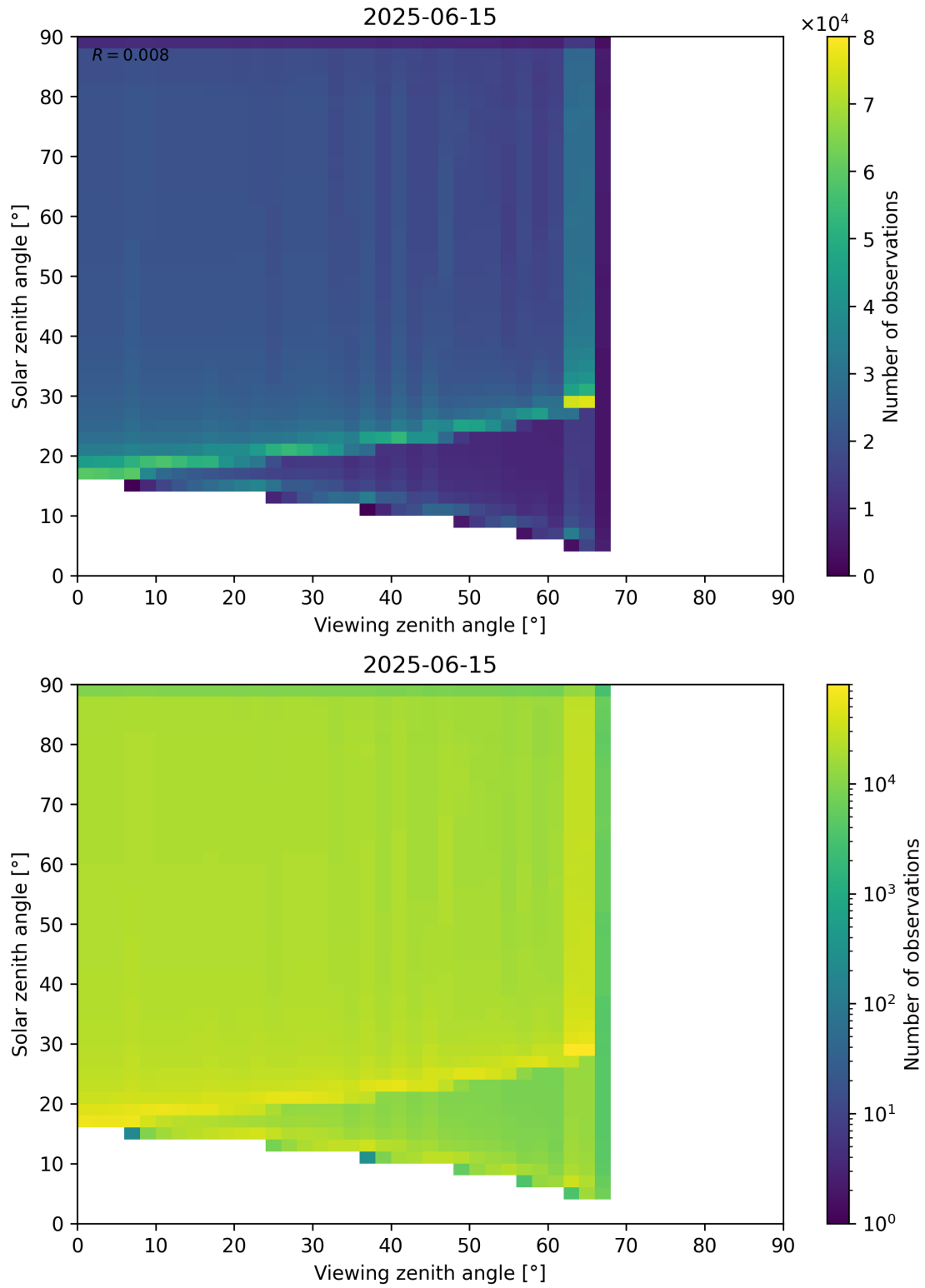
Figure 54: Scatter density plot of “Viewing zenith angle” against “Solar zenith angle” for 2025-06-14 to 2025-06-16.
