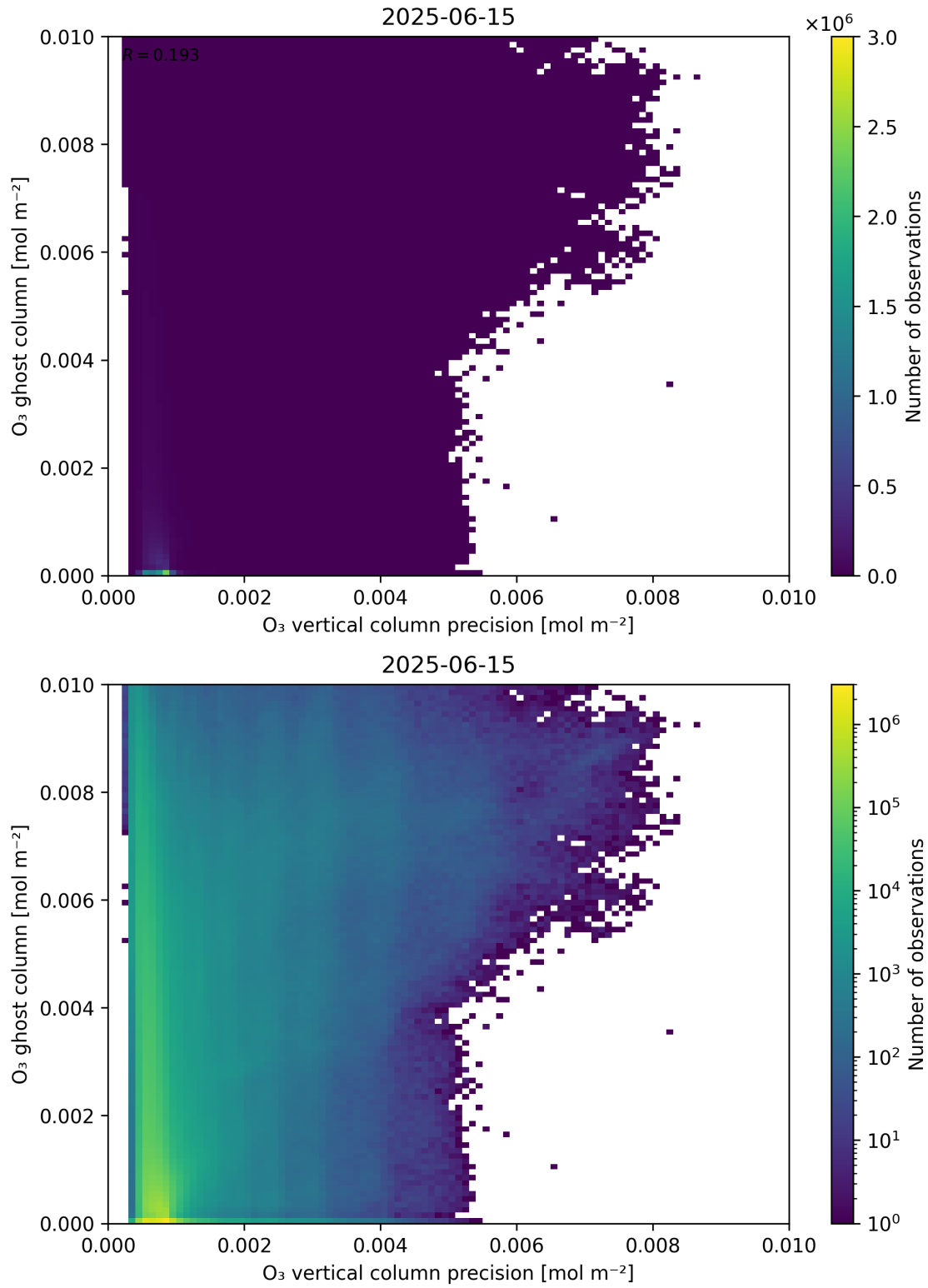
Figure 43: Scatter density plot of “O 3 vertical column precision” against “O 3 ghost column” for 2025-06-14 to 2025-06-16.
