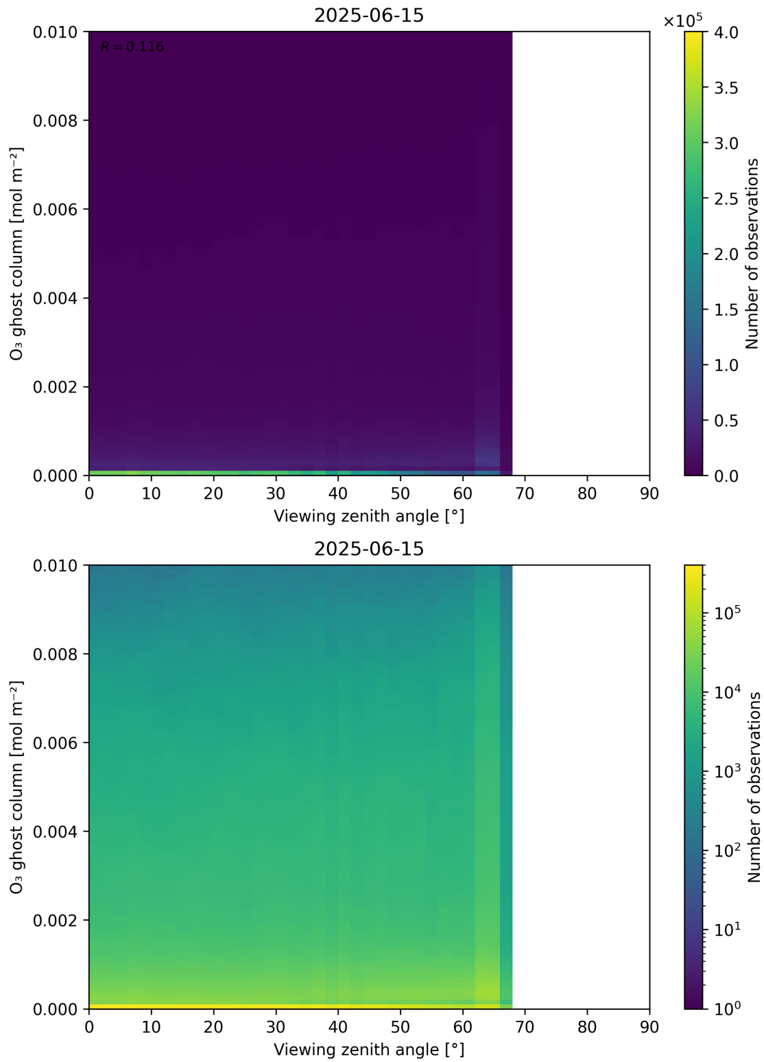
Figure 51: Scatter density plot of “Viewing zenith angle” against “O 3 ghost column” for 2025-06-14 to 2025-06-16.
