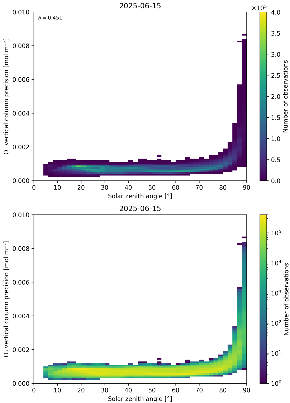
Figure 48: Scatter density plot of “Solar zenith angle” against “O 3 vertical column precision” for 2025-06-14 to 2025-06-16.
