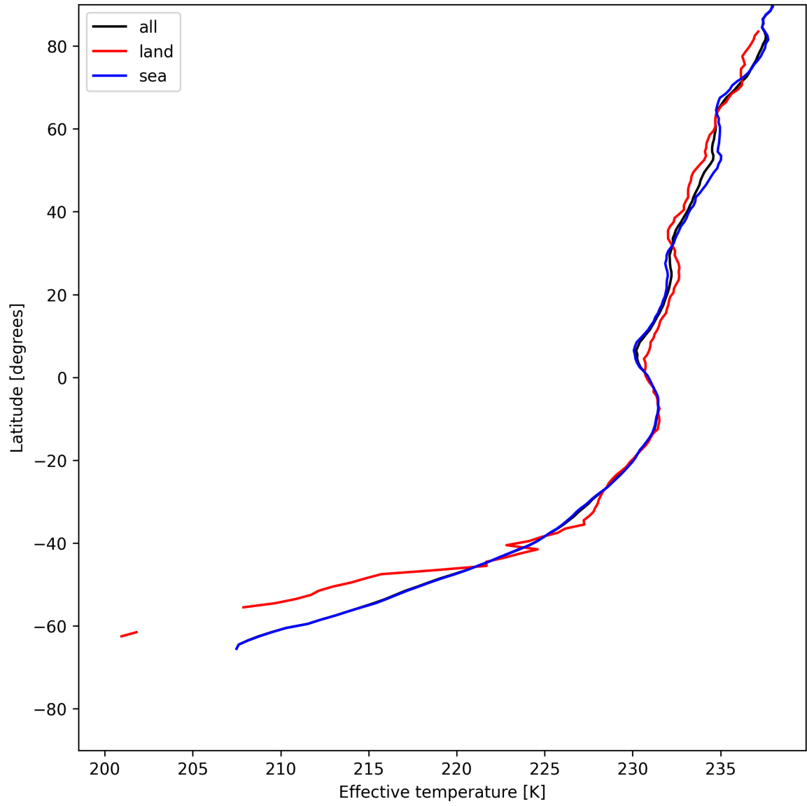
Figure 17: Zonal average of “Effective temperature” for 2025-06-14 to 2025-06-16.
