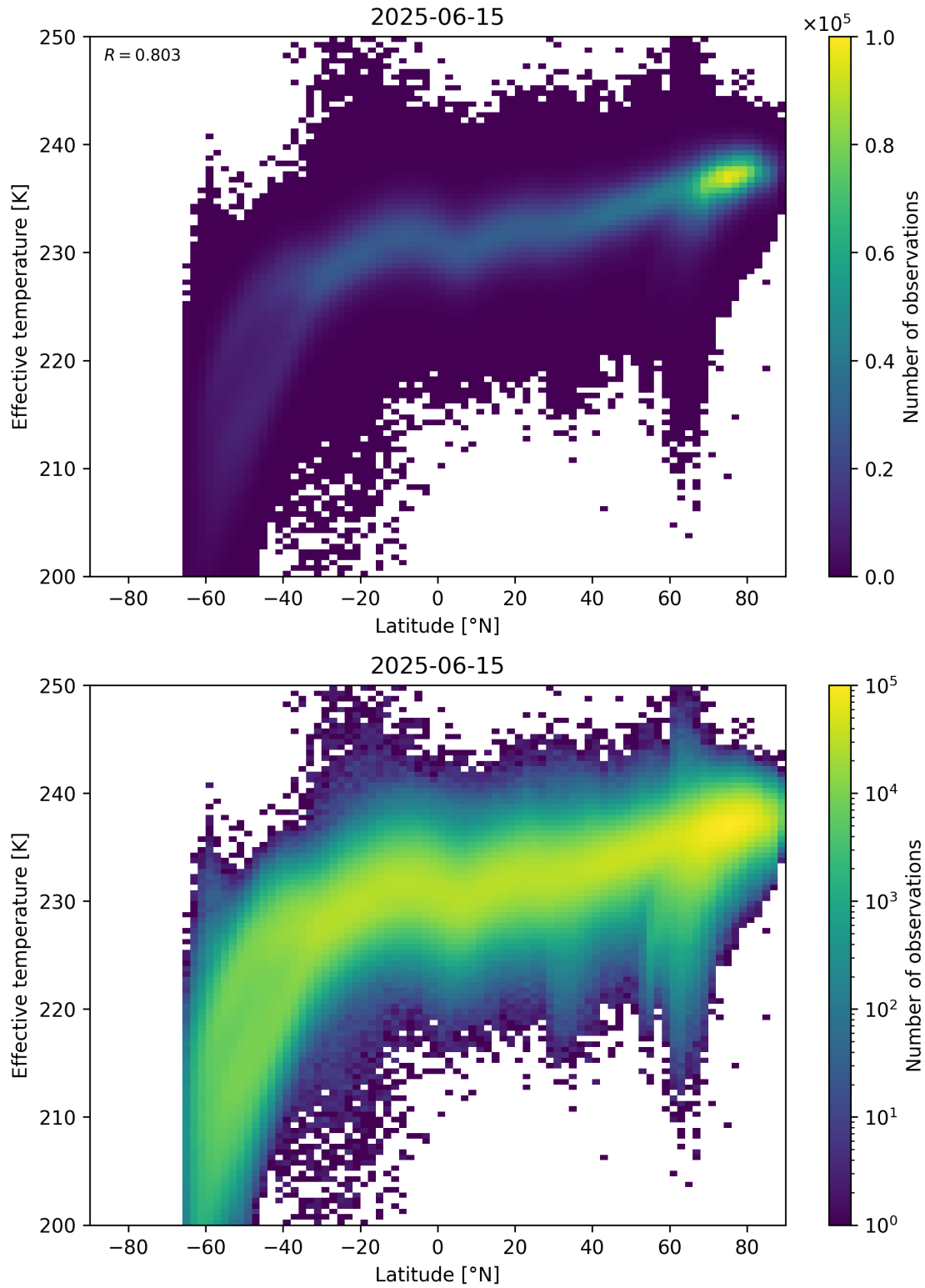
Figure 34: Scatter density plot of “Latitude” against “Effective temperature” for 2025-06-14 to 2025-06-16.
