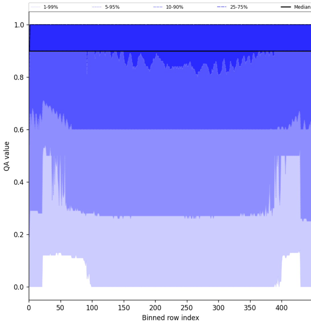
Figure 27: Along track statistics of “QA value” for 2025-06-14 to 2025-06-16
