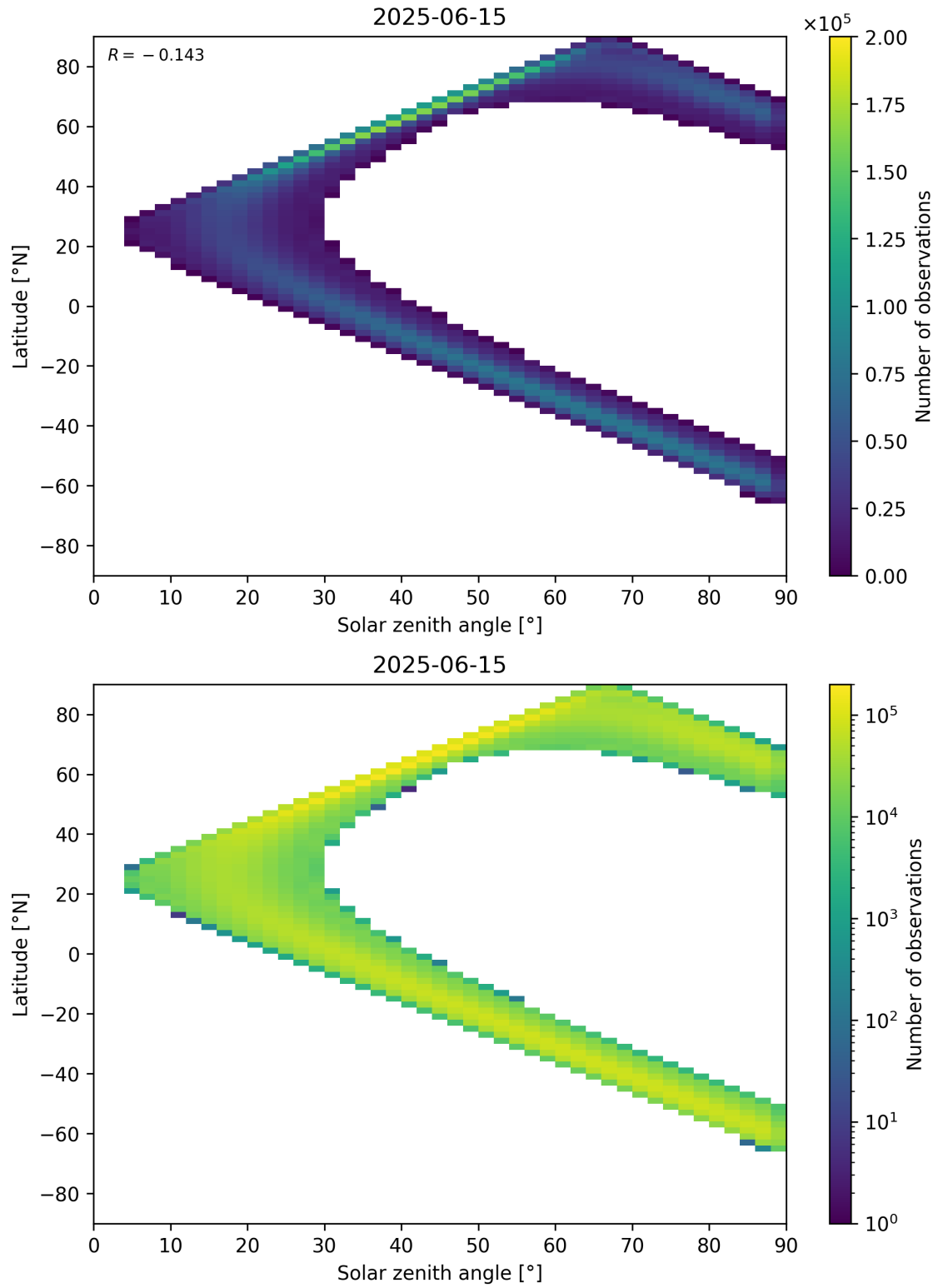
Figure 44: Scatter density plot of “Solar zenith angle” against “Latitude” for 2025-06-14 to 2025-06-16.
