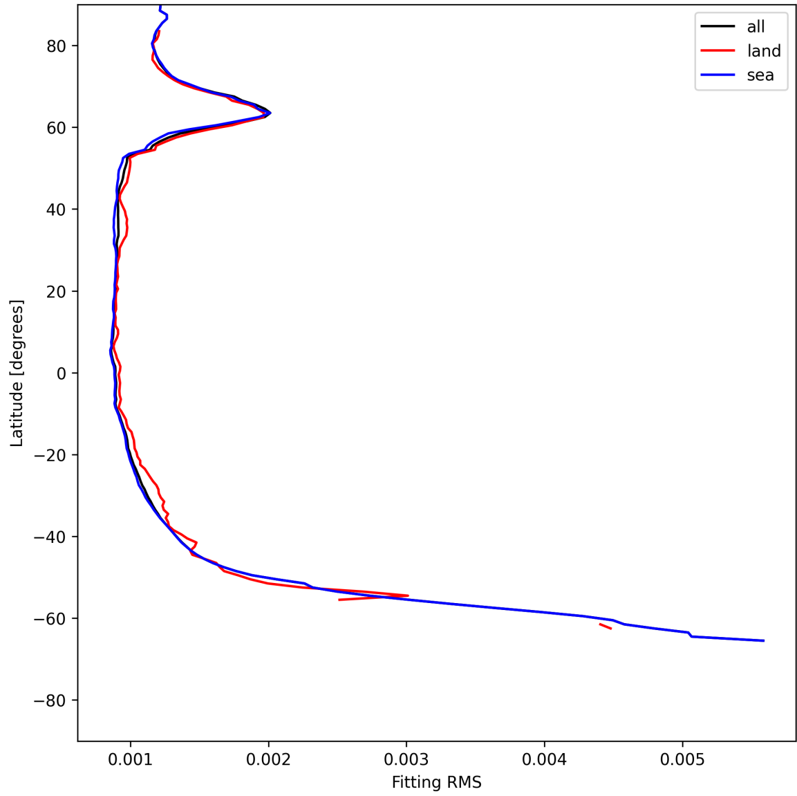
Figure 16: Zonal average of “Fitting RMS” for 2025-06-14 to 2025-06-16.
