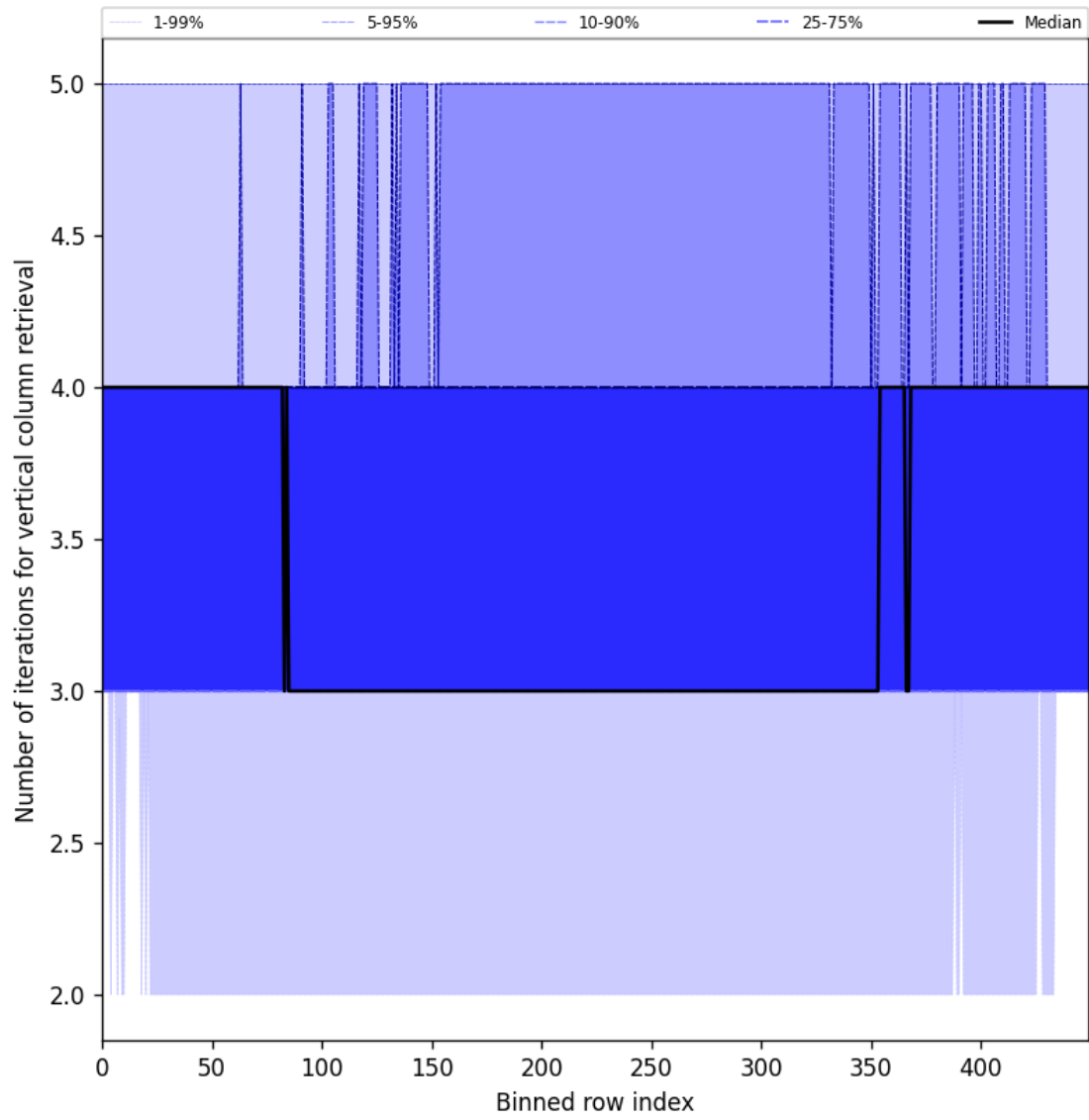
Figure 33: Along track statistics of “Number of iterations for vertical column retrieval” for 2025-06-14 to 2025-06-16
