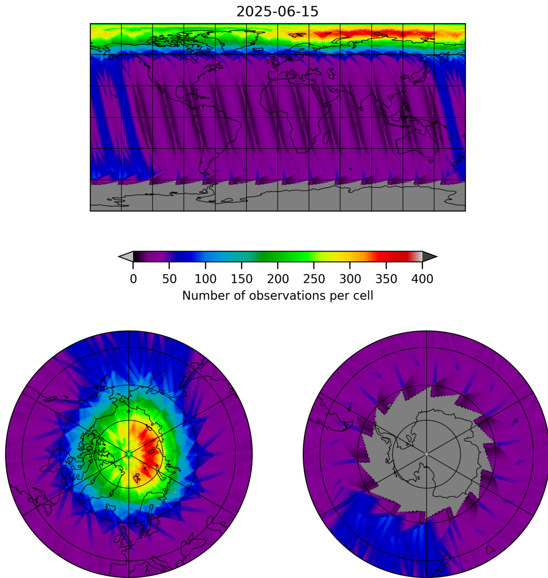
Figure 12: Map of the number of observations for 2025-06-14 to 2025-06-16
