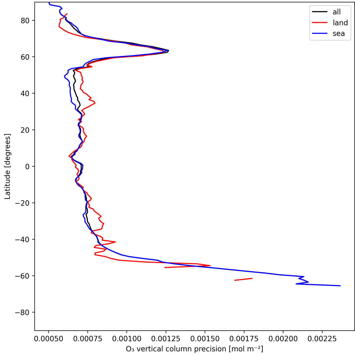
Figure 15: Zonal average of “O 3 vertical column precision” for 2025-06-14 to 2025-06-16.
