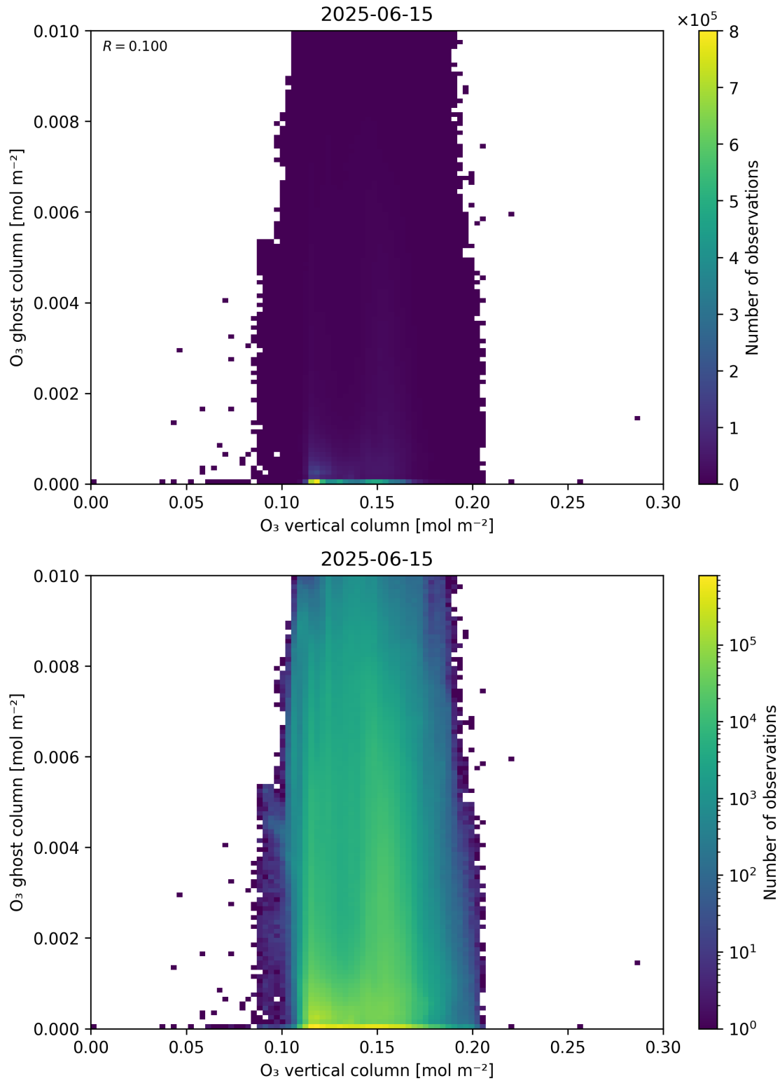
Figure 40: Scatter density plot of “O 3 vertical column” against “O 3 ghost column” for 2025-06-14 to 2025-06-16.
