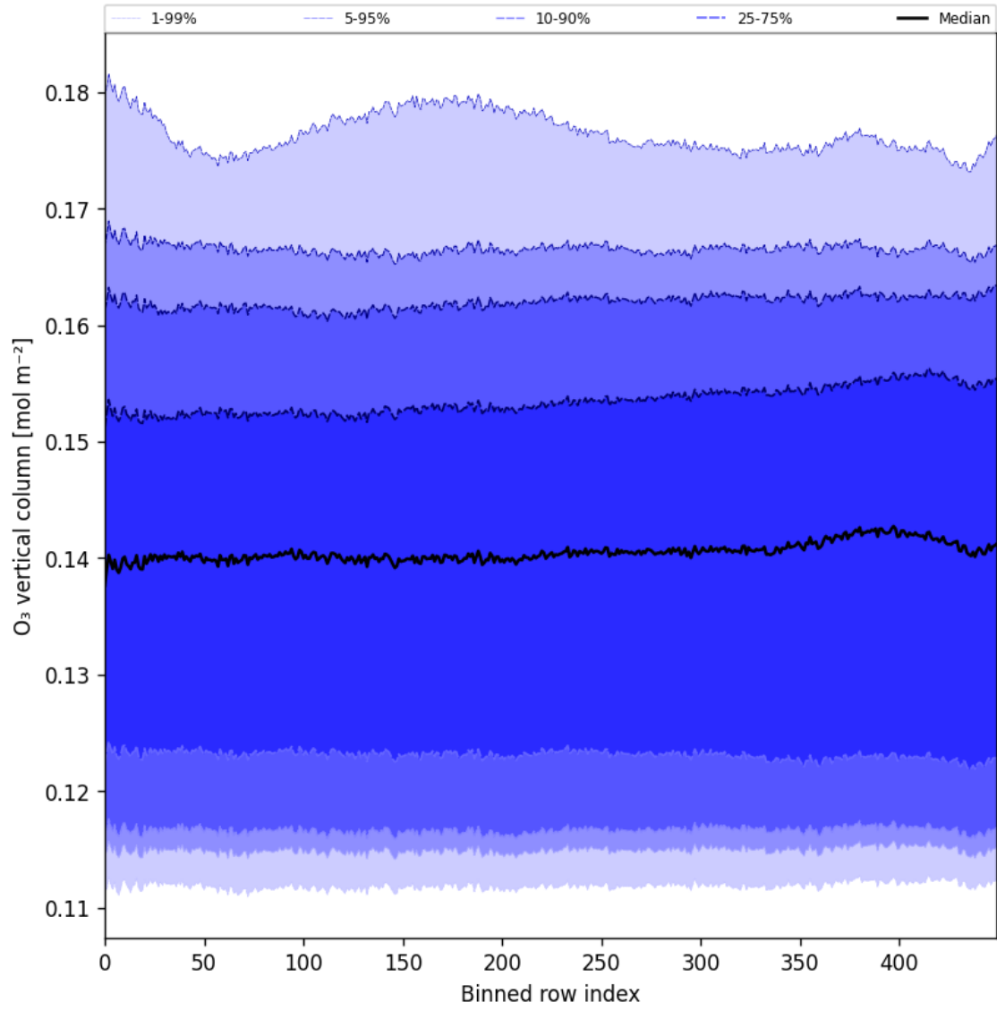
Figure 28: Along track statistics of “O 3 vertical column” for 2025-06-14 to 2025-06-16
