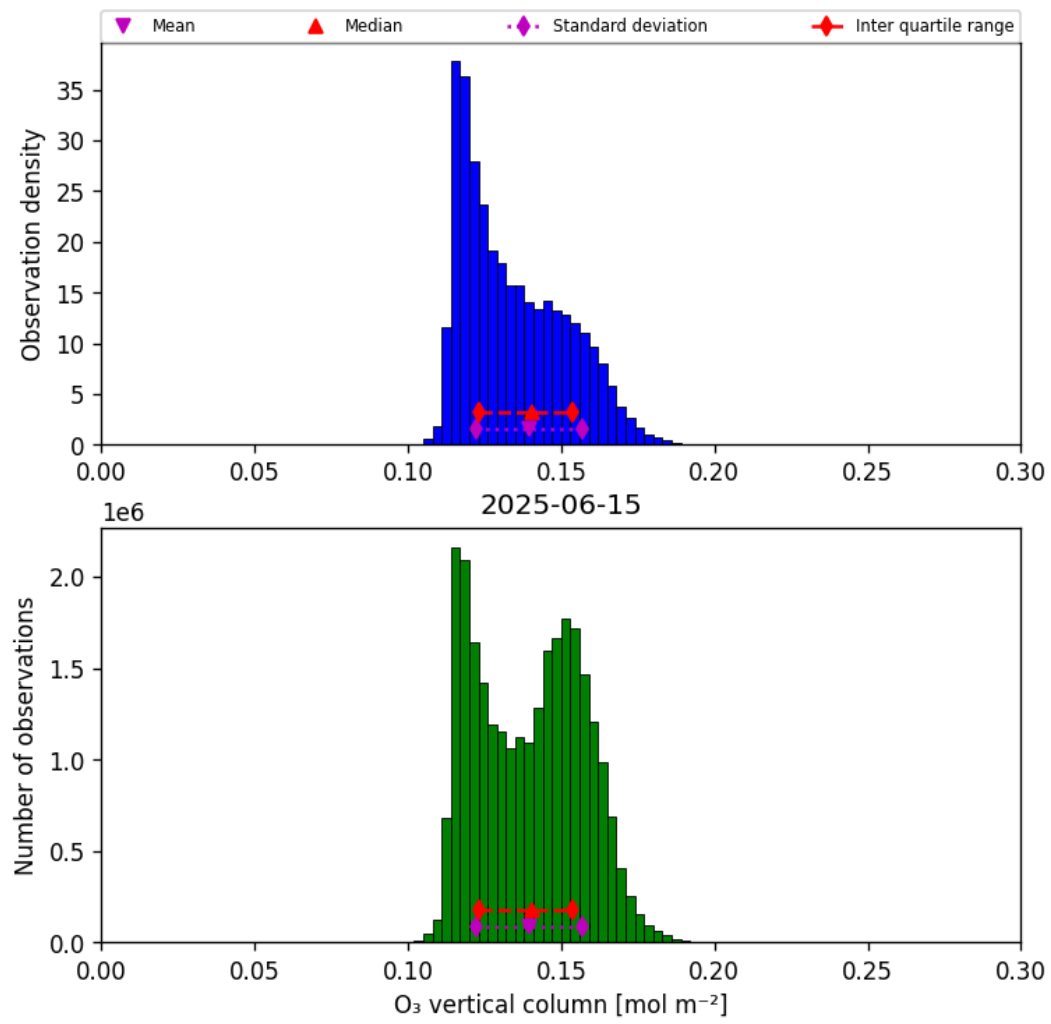
Figure 21: Histogram of “O 3 vertical column” for 2025-06-14 to 2025-06-16
