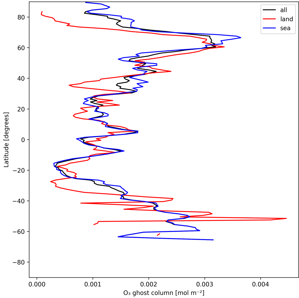
Figure 18: Zonal average of "O 3 ghost column" for 2025-06-14 to 2025-06-16.
