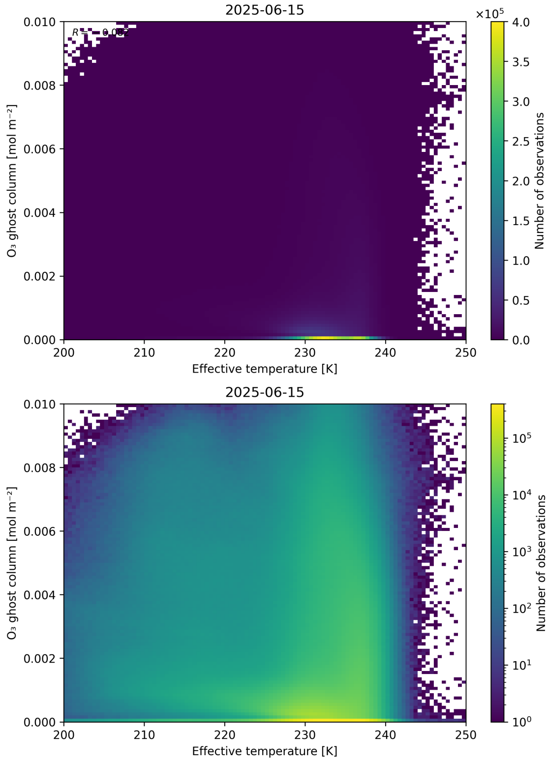
Figure 38: Scatter density plot of “Effective temperature” against “O 3 ghost column” for 2025-06-14 to 2025-06-16.
