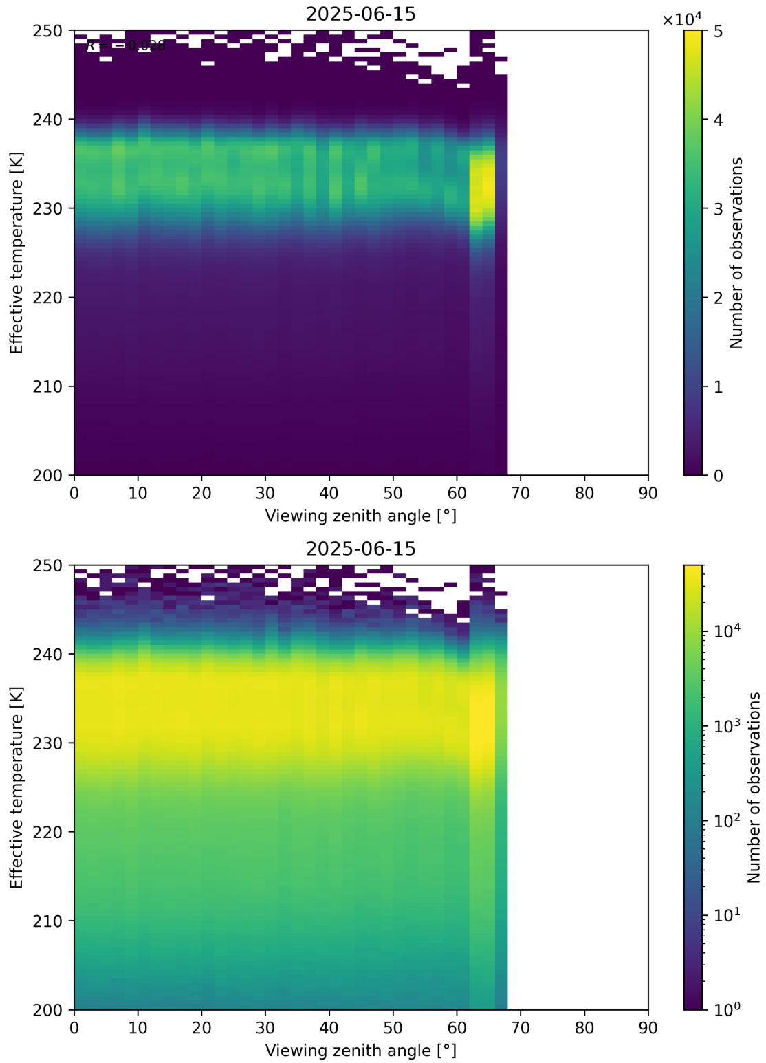
Figure 50: Scatter density plot of “Viewing zenith angle” against “Effective temperature” for 2025-06-14 to 2025-06-16.
