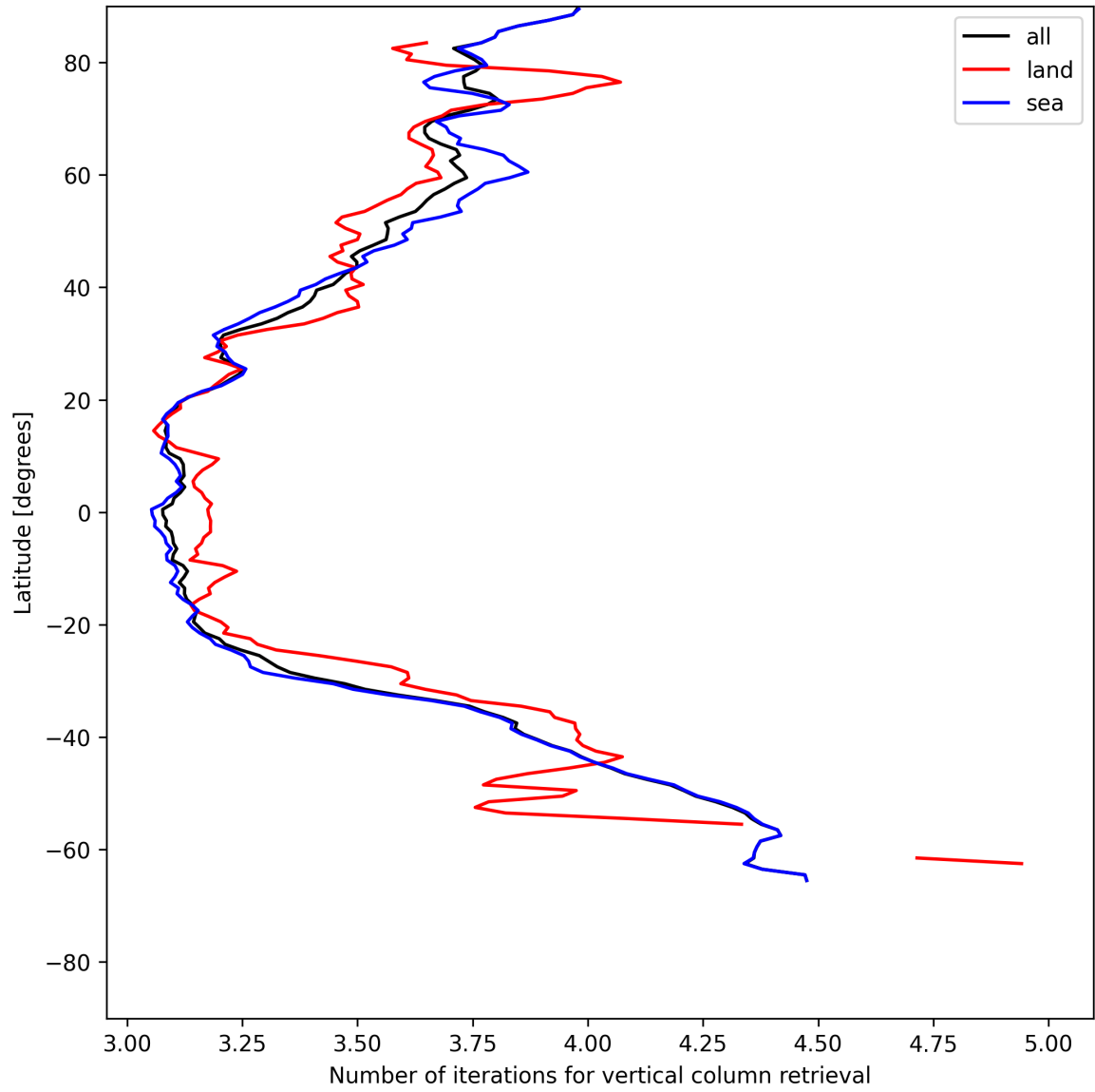
Figure 19: Zonal average of “Number of iterations for vertical column retrieval” for 2025-06-14 to 2025-06-16.
