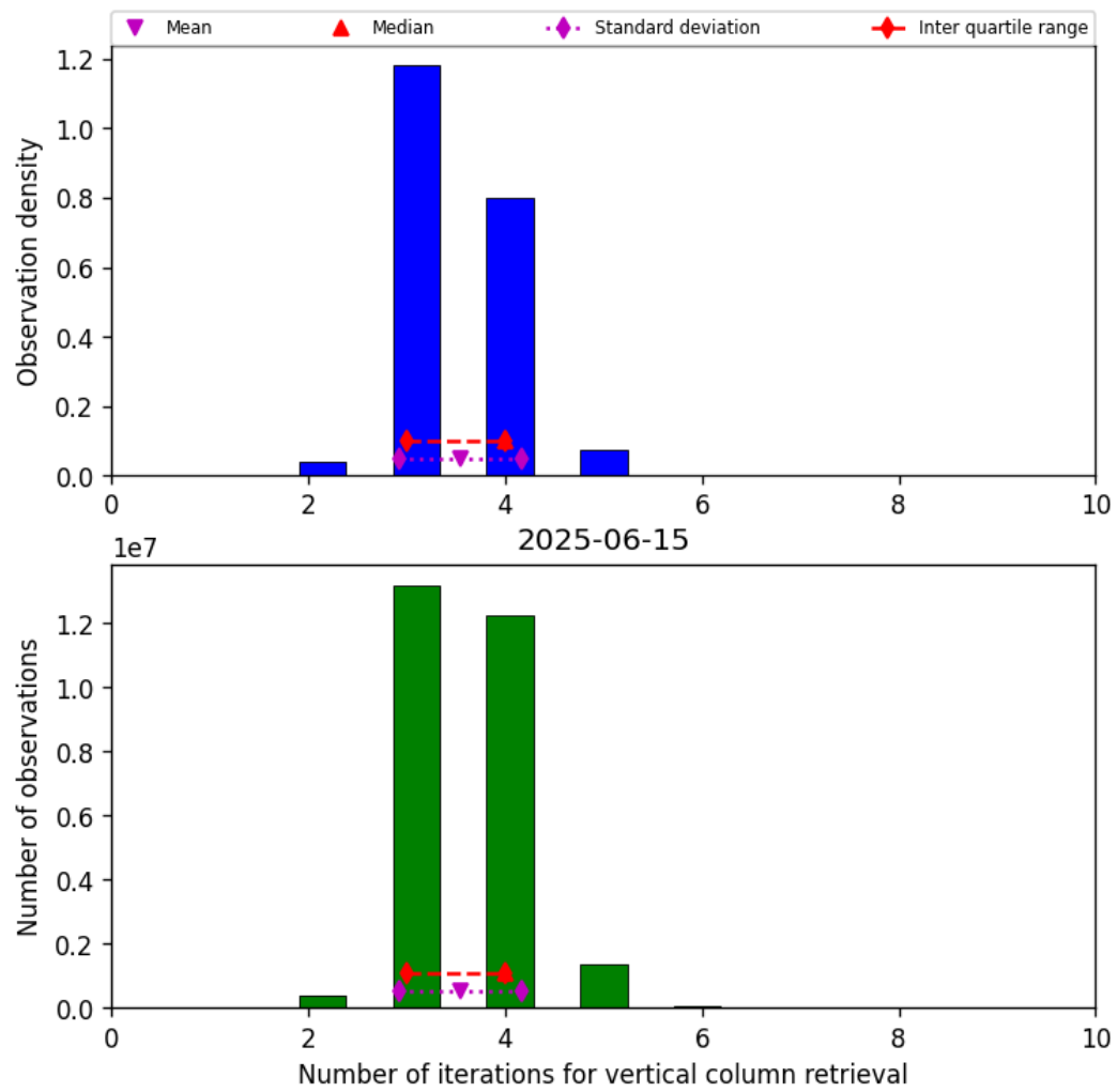
Figure 26: Histogram of “Number of iterations for vertical column retrieval” for 2025-06-14 to 2025-06-16
