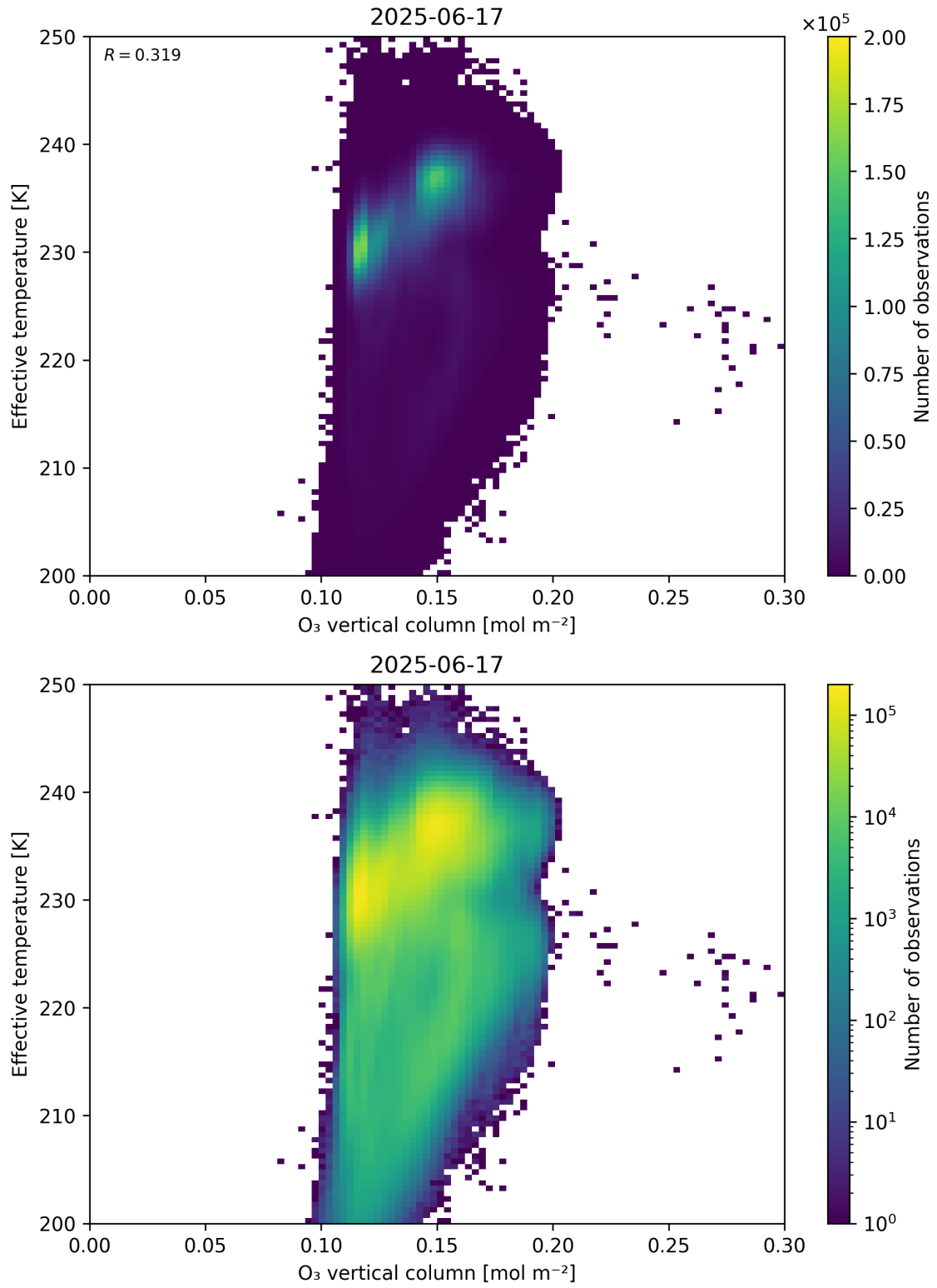
Figure 39: Scatter density plot of “O 3 vertical column” against “Effective temperature” for 2025-06-17 to 2025-06-18.
