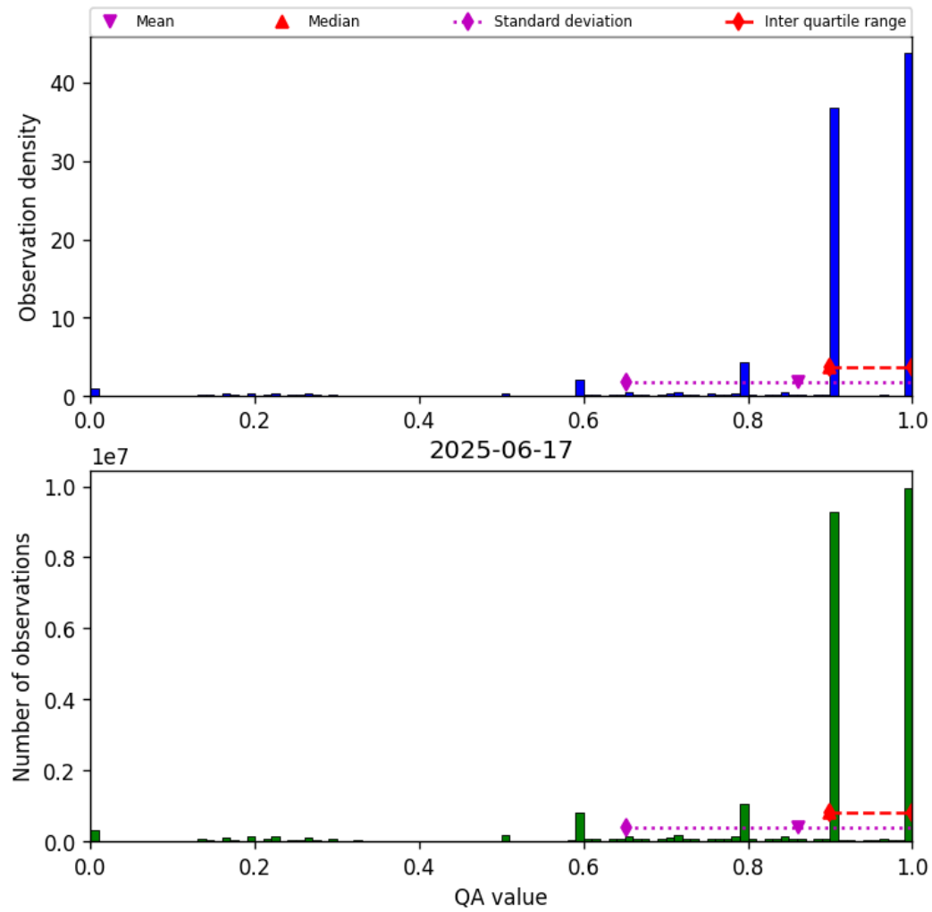
Figure 20: Histogram of “QA value” for 2025-06-17 to 2025-06-18
