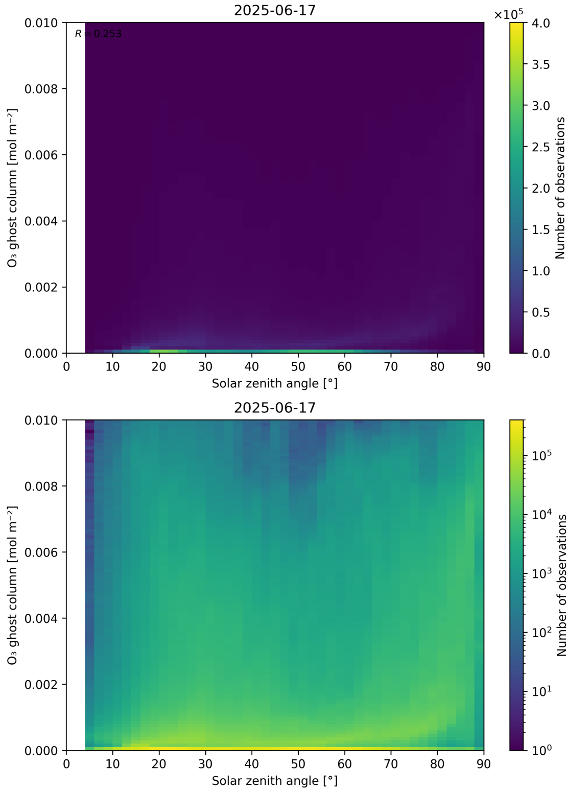
Figure 46: Scatter density plot of “Solar zenith angle” against “O 3 ghost column” for 2025-06-17 to 2025-06-18.
