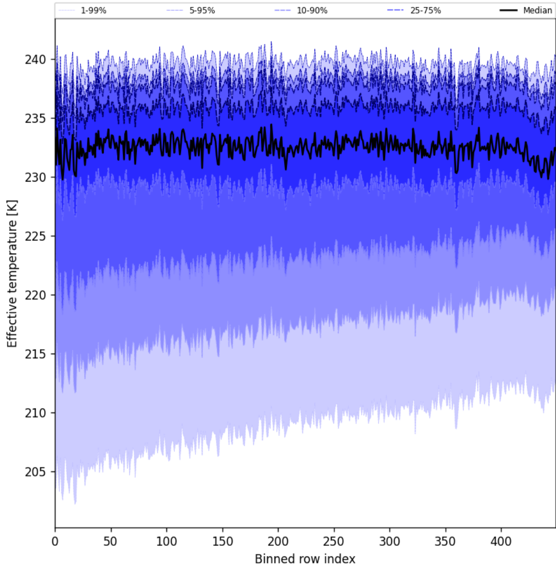
Figure 31: Along track statistics of “Effective temperature” for 2025-06-17 to 2025-06-18
