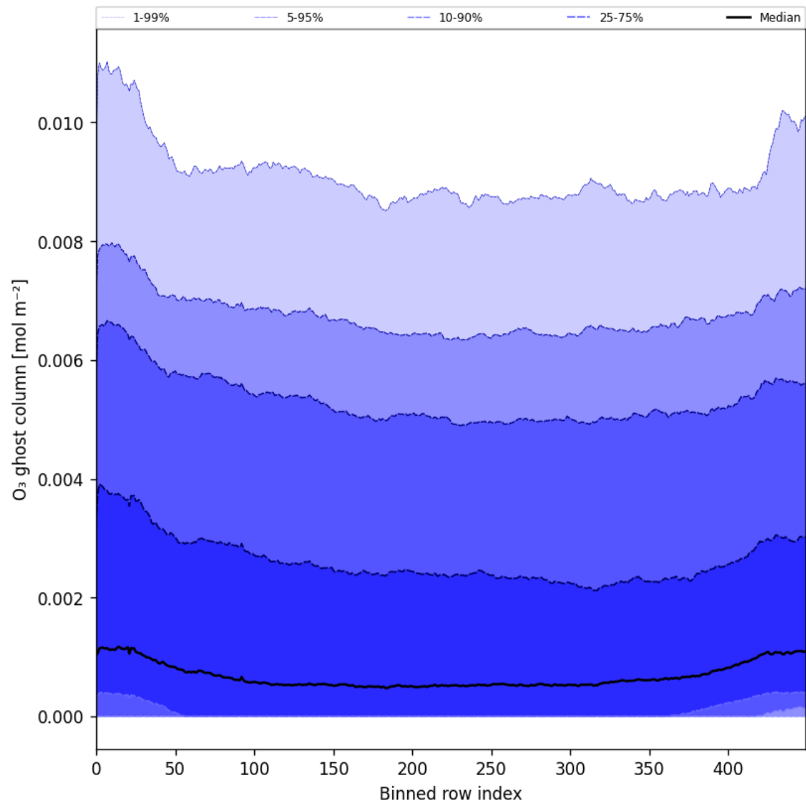
Figure 32: Along track statistics of “O 3 ghost column” for 2025-06-17 to 2025-06-18
