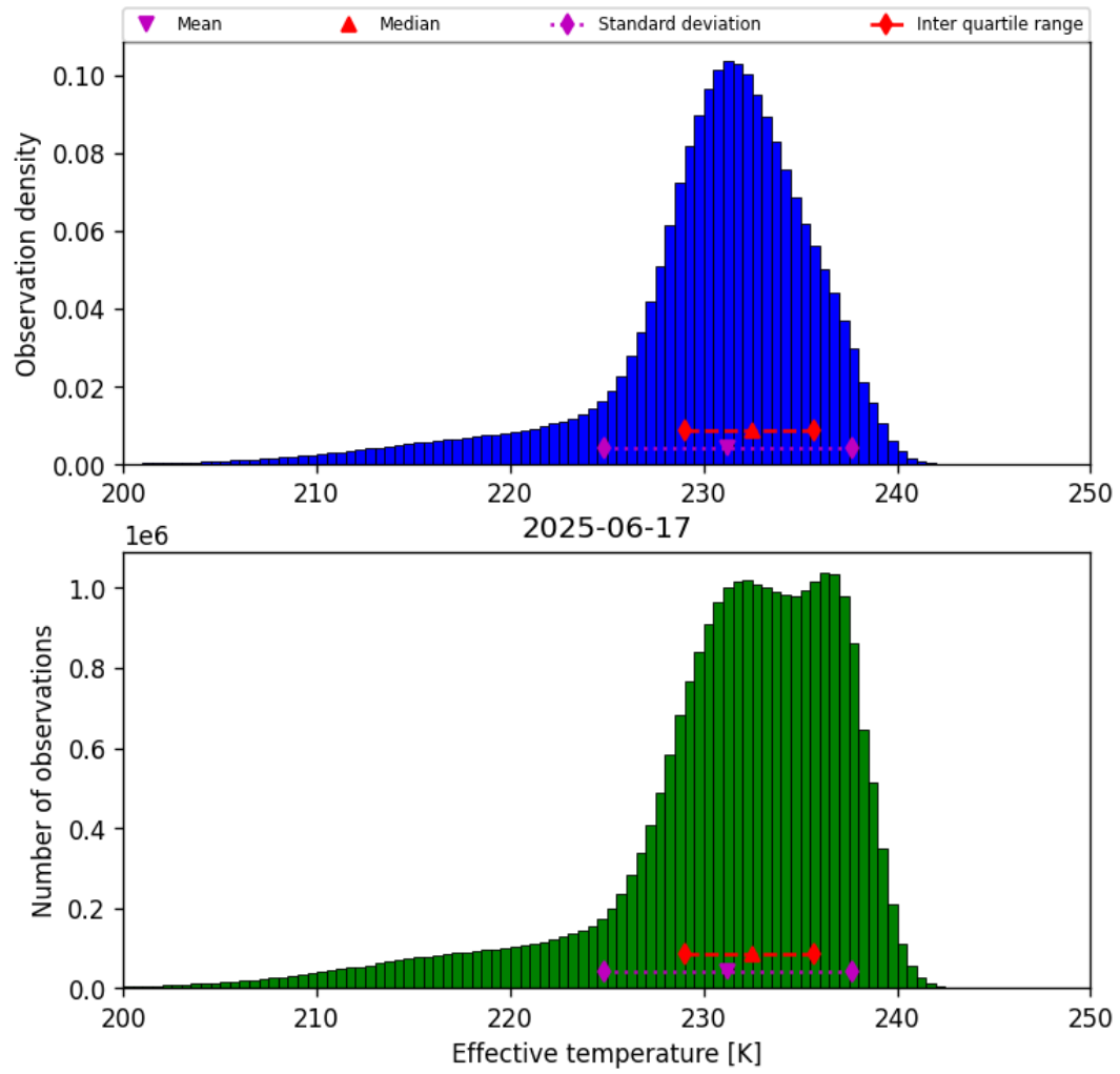
Figure 24: Histogram of “Effective temperature” for 2025-06-17 to 2025-06-18
