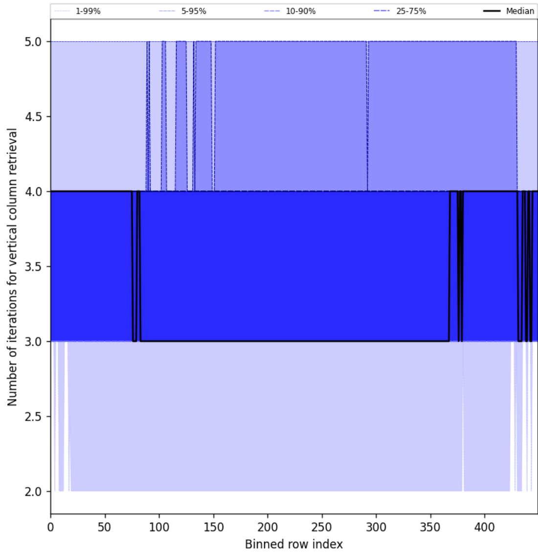
Figure 33: Along track statistics of “Number of iterations for vertical column retrieval” for 2025-06-17 to 2025-06-18
