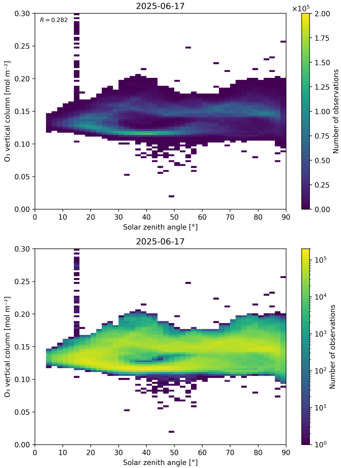
Figure 47: Scatter density plot of “Solar zenith angle” against “O 3 vertical column” for 2025-06-17 to 2025-06-18.
