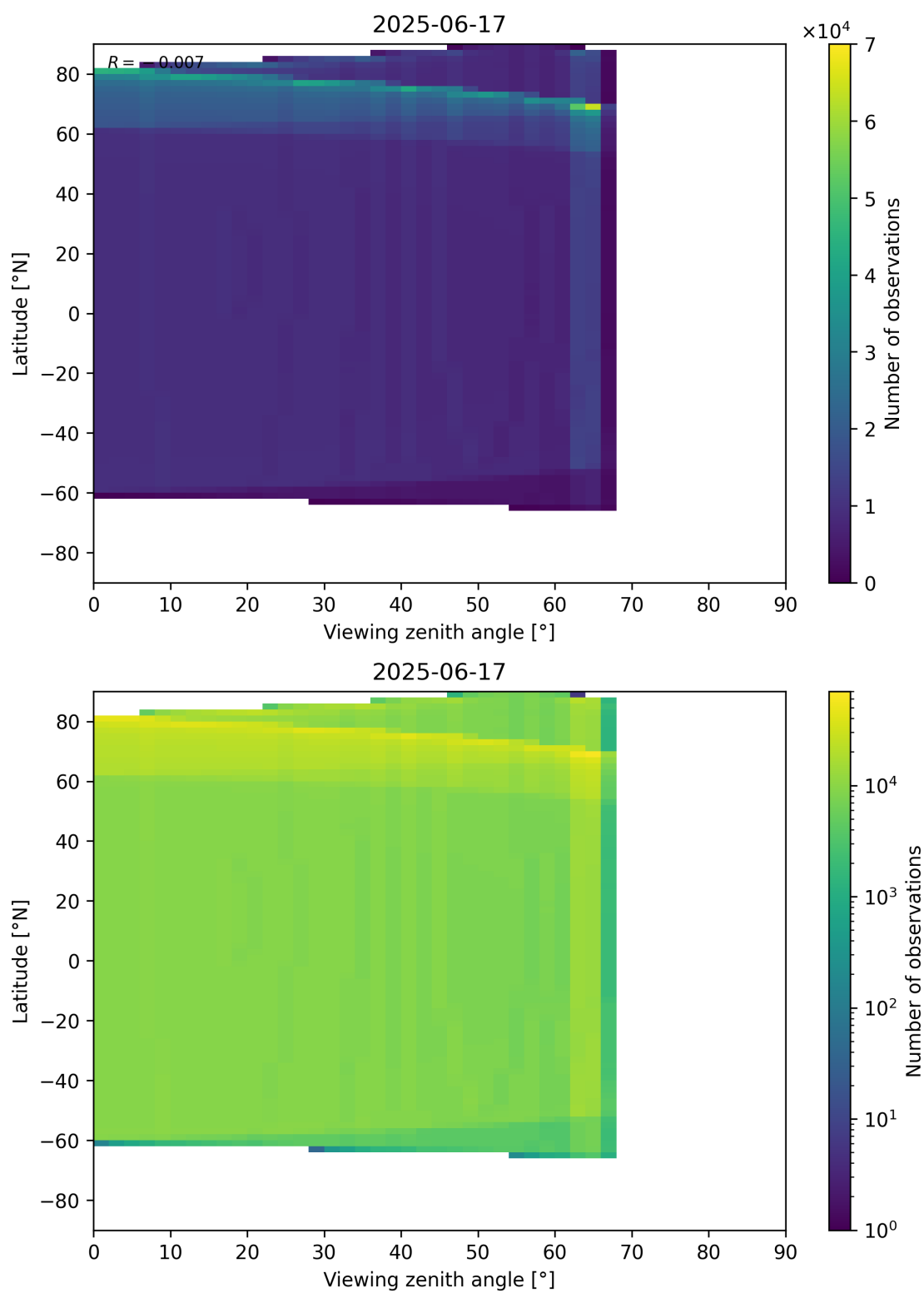
Figure 49: Scatter density plot of “Viewing zenith angle” against “Latitude” for 2025-06-17 to 2025-06-18.
