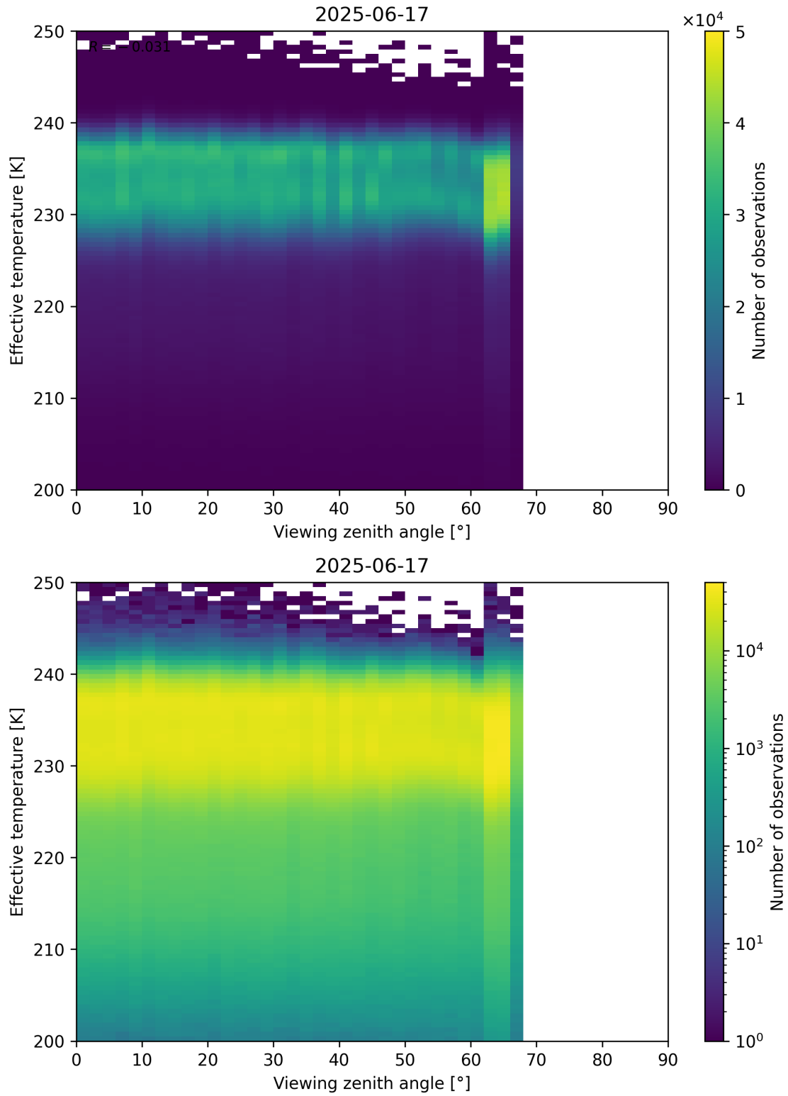
Figure 50: Scatter density plot of “Viewing zenith angle” against “Effective temperature” for 2025-06-17 to 2025-06-18.
