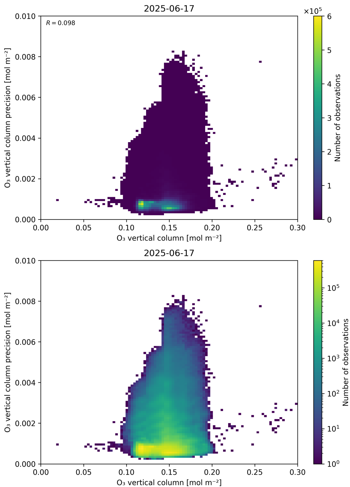
Figure 41: Scatter density plot of “O 3 vertical column” against “O 3 vertical column precision” for 2025-06-17 to 2025-06-18.
