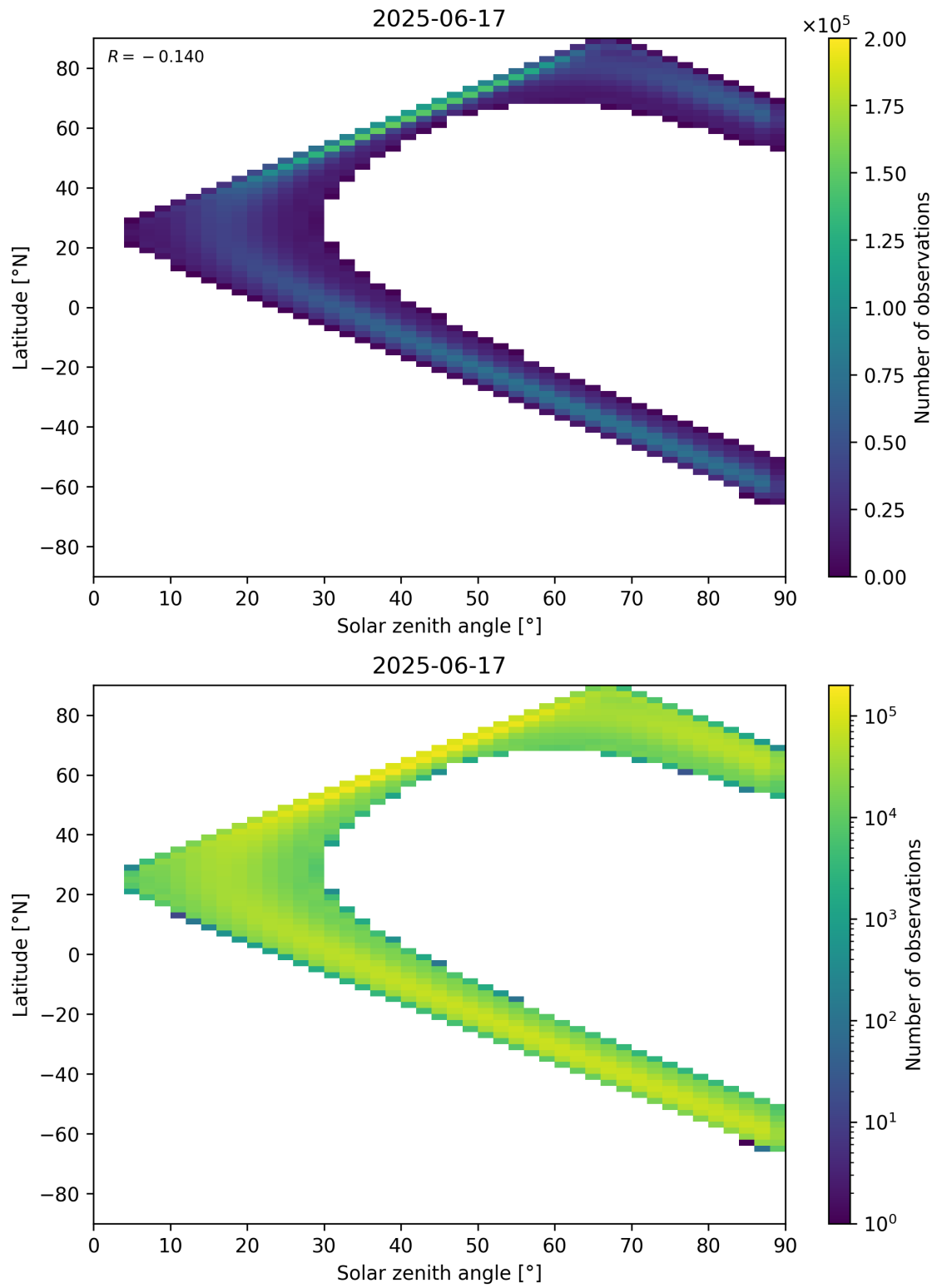
Figure 44: Scatter density plot of “Solar zenith angle” against “Latitude” for 2025-06-17 to 2025-06-18.
