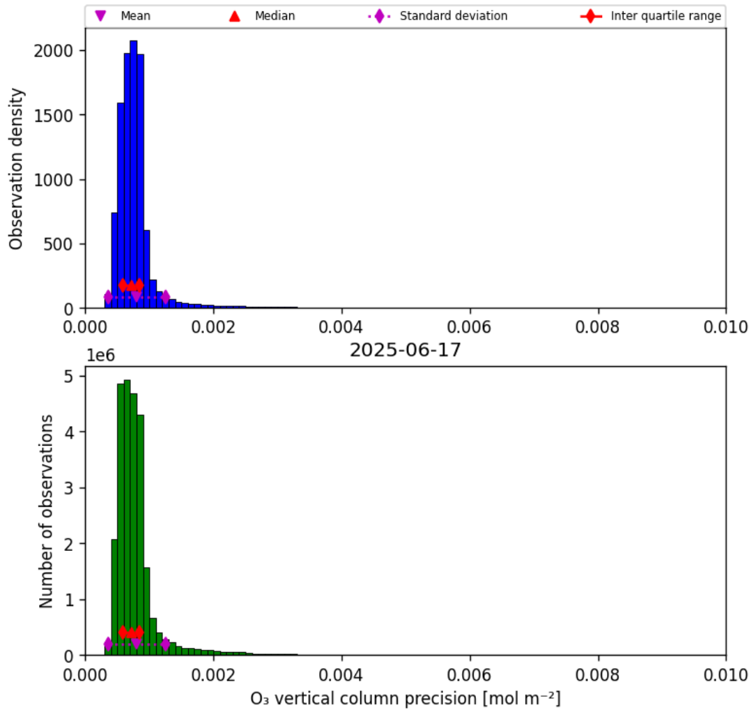
Figure 22: Histogram of “O 3 vertical column precision” for 2025-06-17 to 2025-06-18
