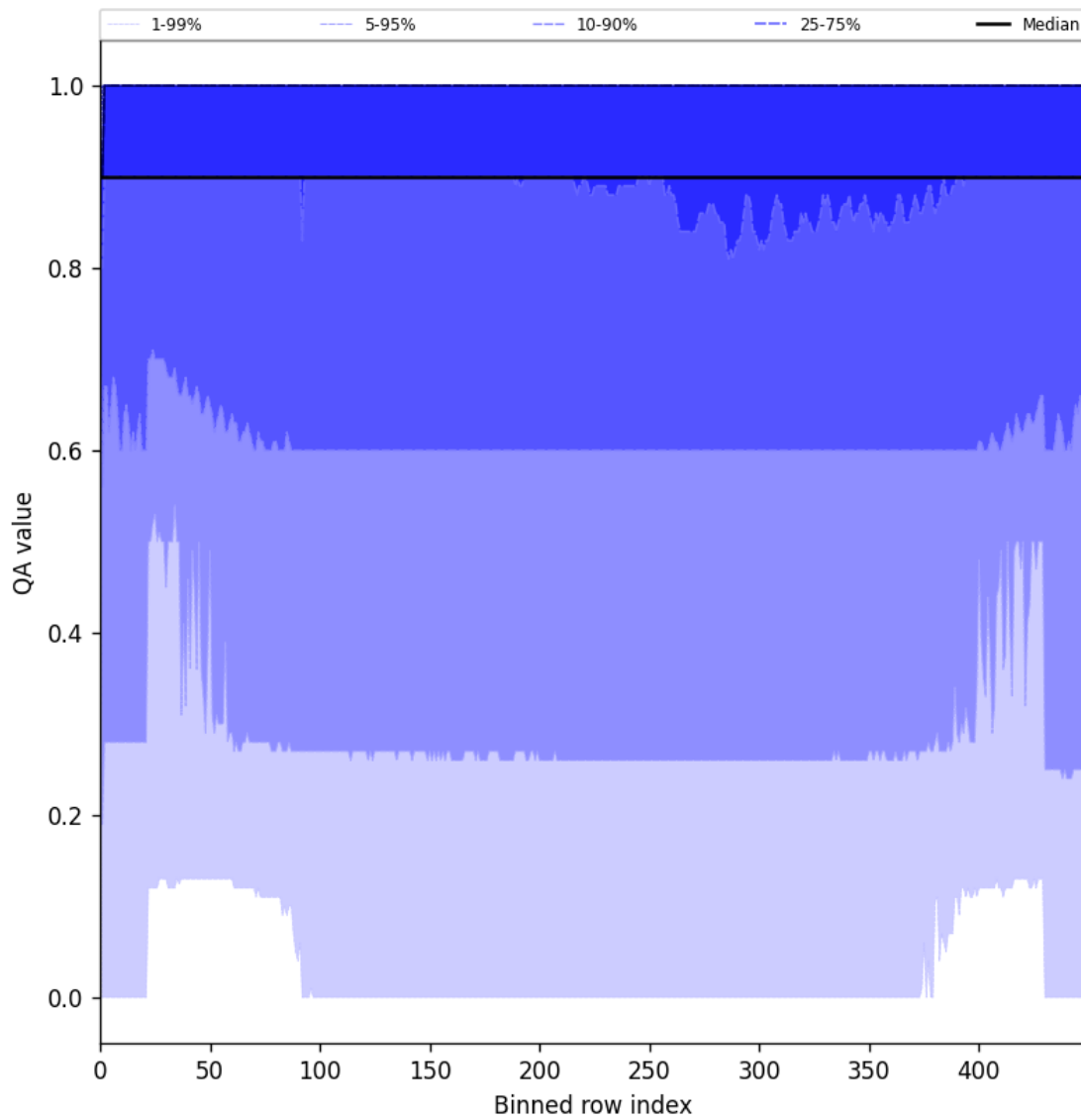
Figure 27: Along track statistics of “QA value” for 2025-06-17 to 2025-06-18
