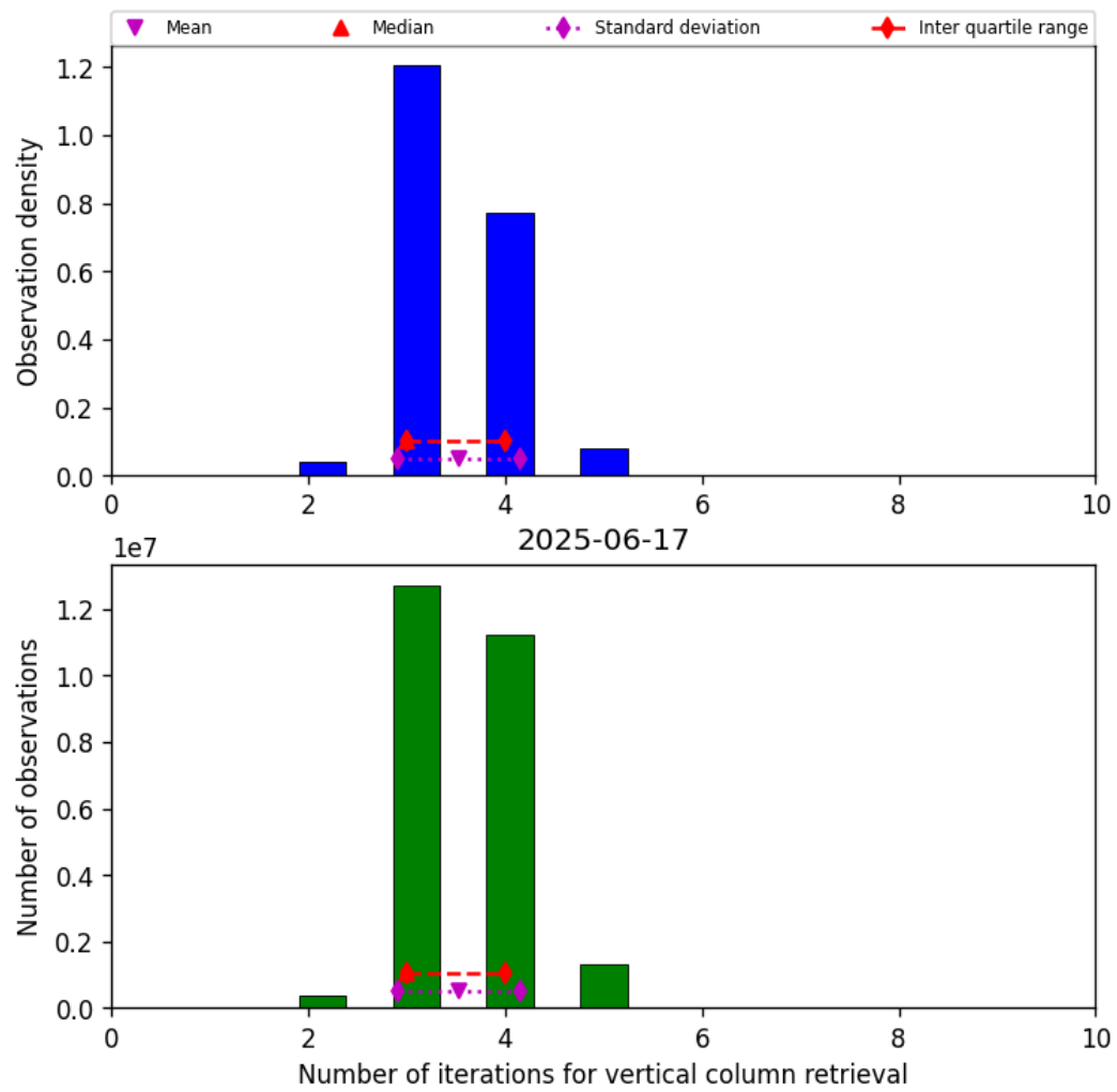
Figure 26: Histogram of “Number of iterations for vertical column retrieval” for 2025-06-17 to 2025-06-18
