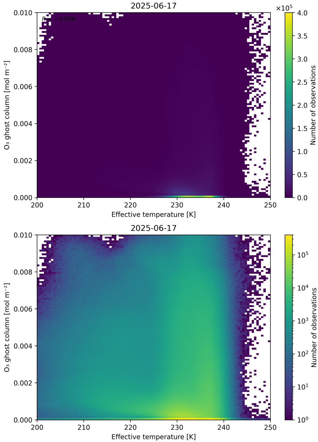
Figure 38: Scatter density plot of “Effective temperature” against “O 3 ghost column” for 2025-06-17 to 2025-06-18.
