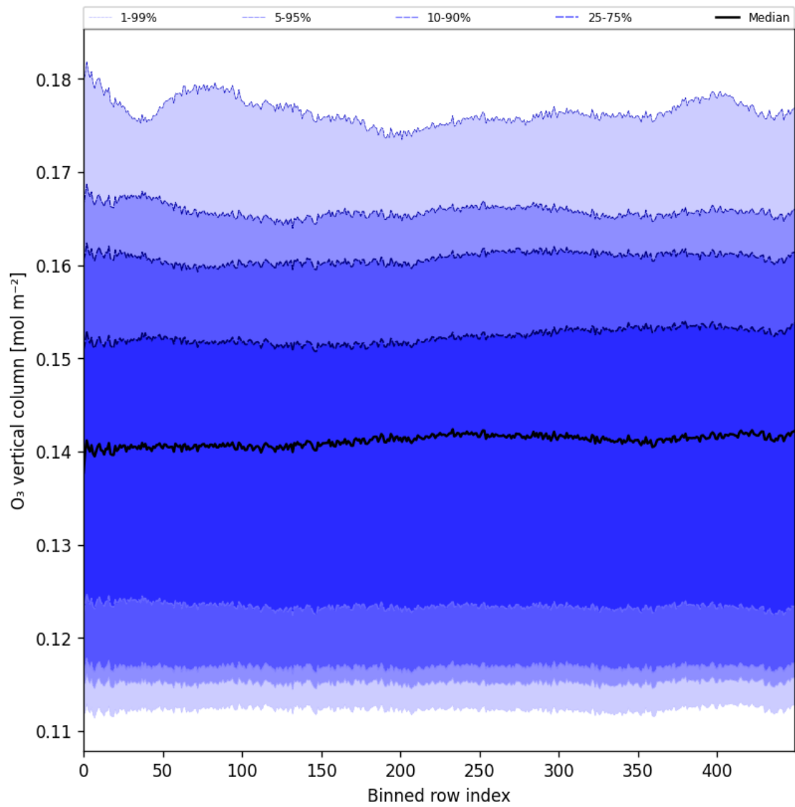
Figure 28: Along track statistics of “ O_3 vertical column” for 2025-06-17 to 2025-06-18
