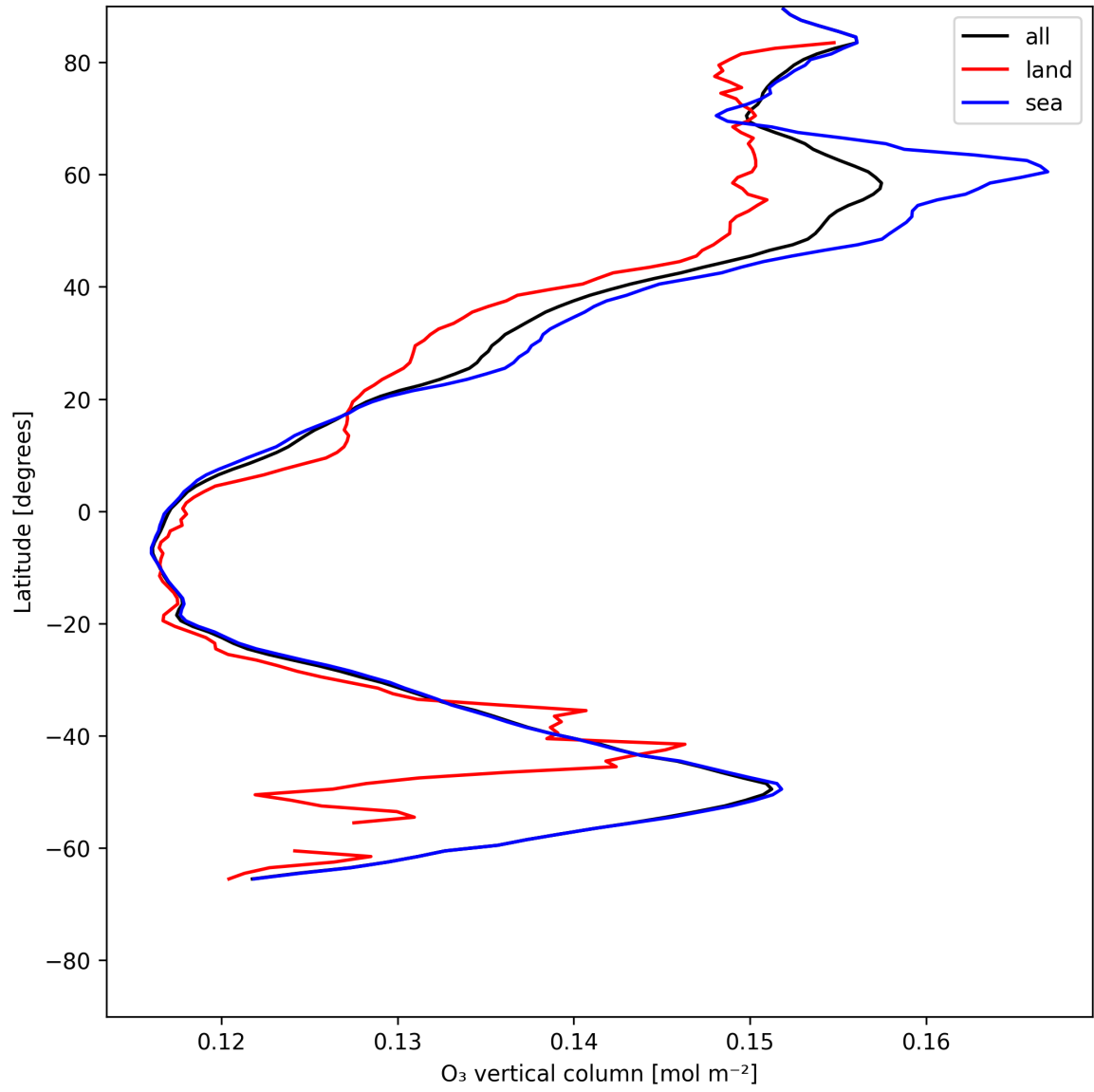
Figure 14: Zonal average of “O 3 vertical column” for 2025-06-17 to 2025-06-18.
