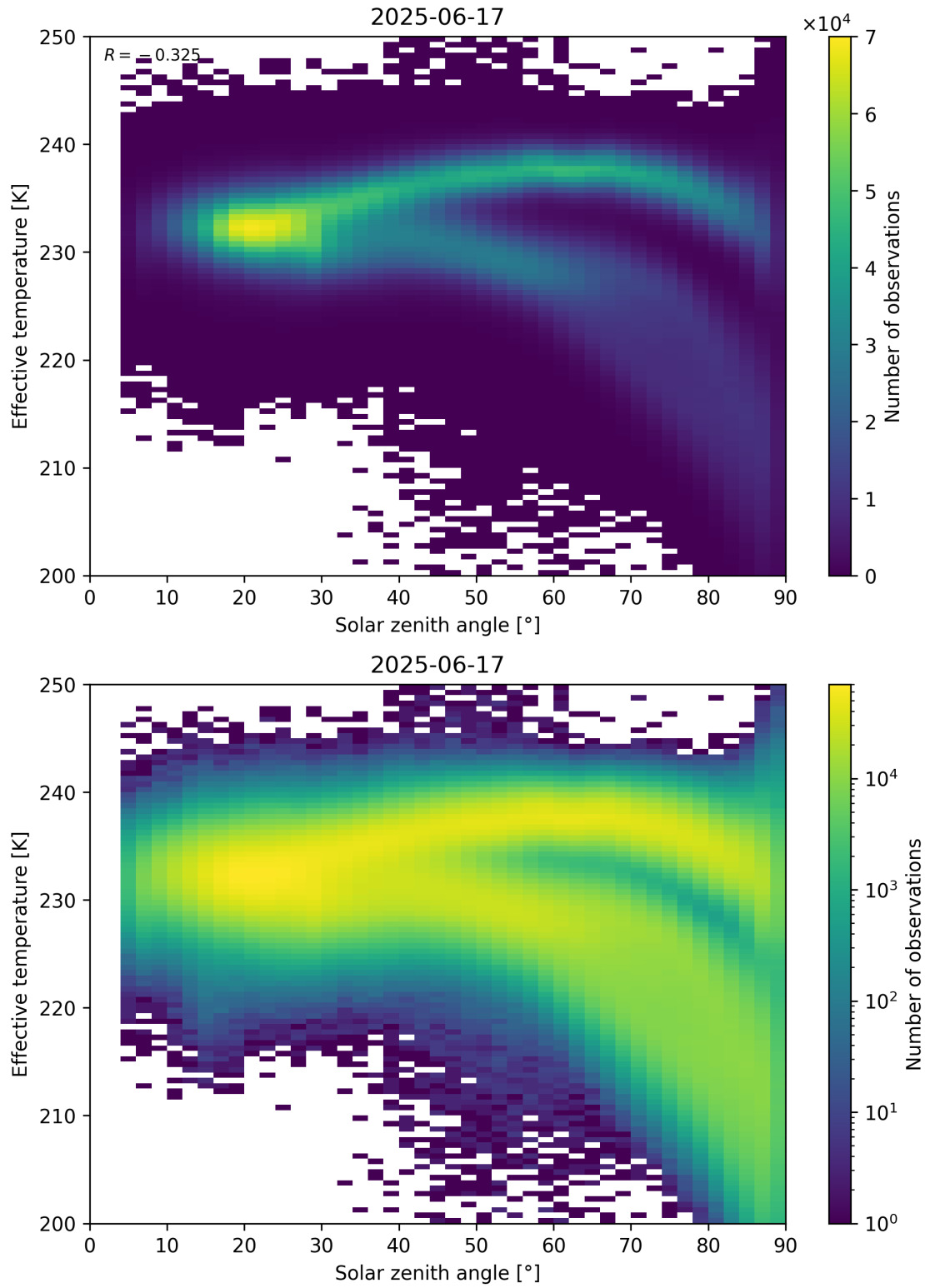
Figure 45: Scatter density plot of “Solar zenith angle” against “Effective temperature” for 2025-06-17 to 2025-06-18.
