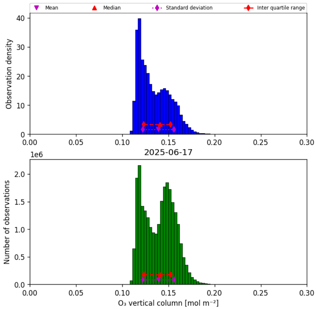
Figure 21: Histogram of “O 3 vertical column” for 2025-06-17 to 2025-06-18
