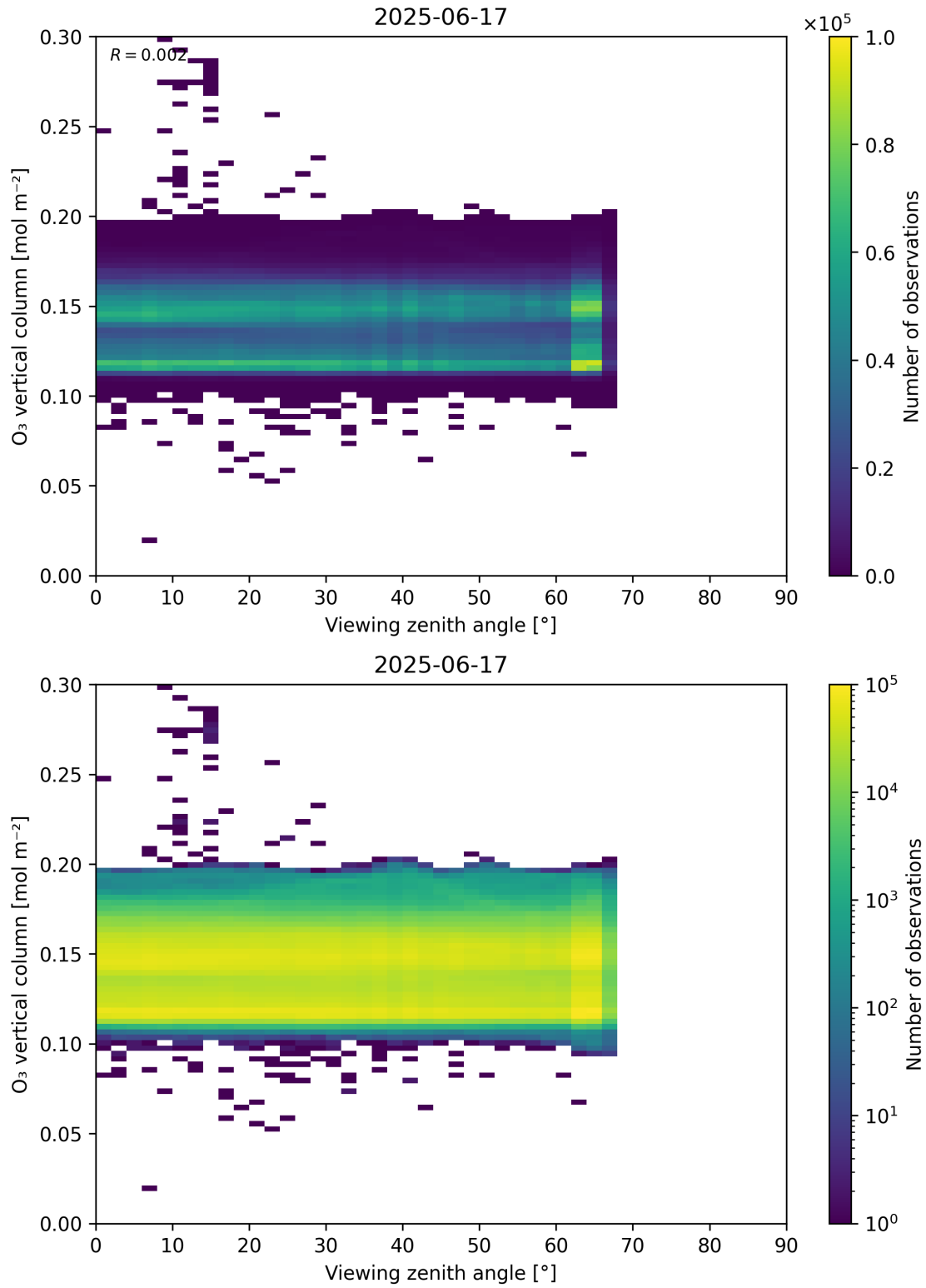
Figure 52: Scatter density plot of “Viewing zenith angle” against “O 3 vertical column” for 2025-06-17 to 2025-06-18.
