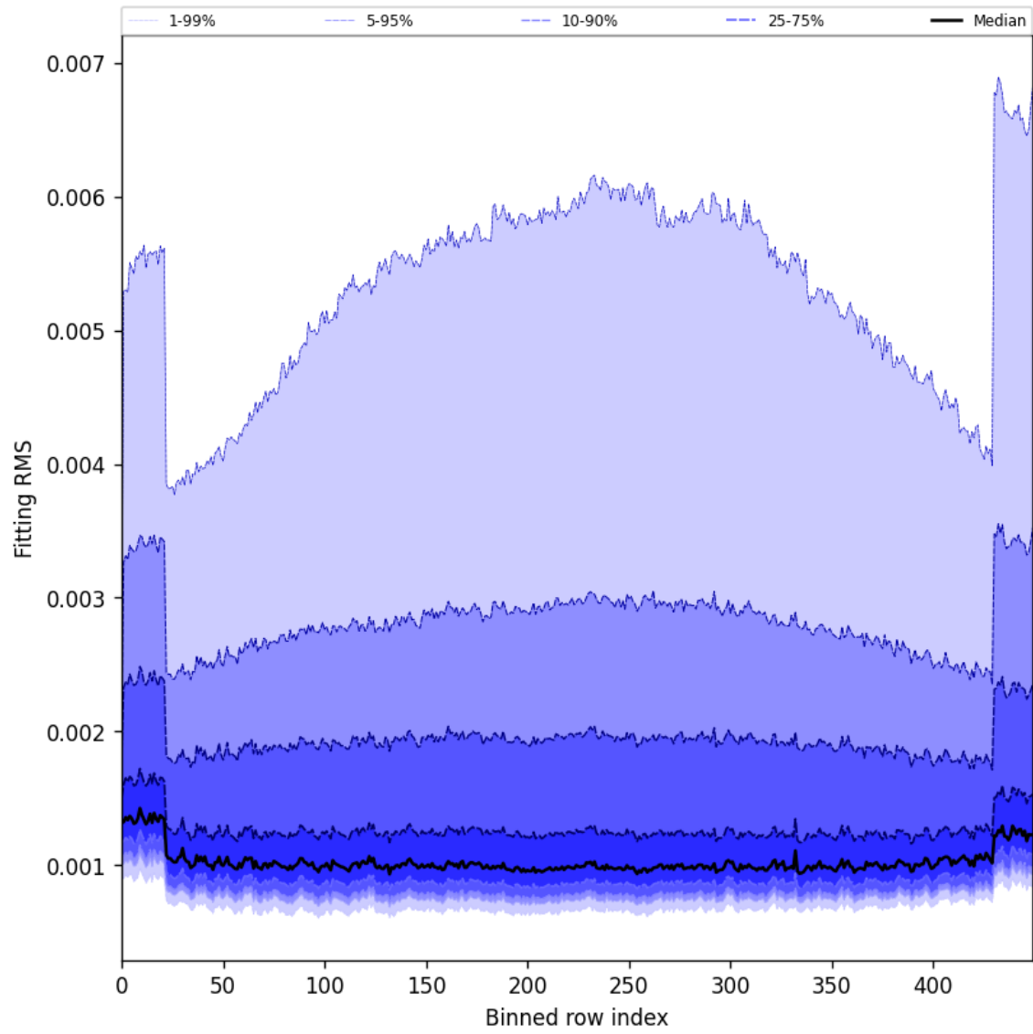
Figure 30: Along track statistics of “Fitting RMS” for 2025-06-17 to 2025-06-18
