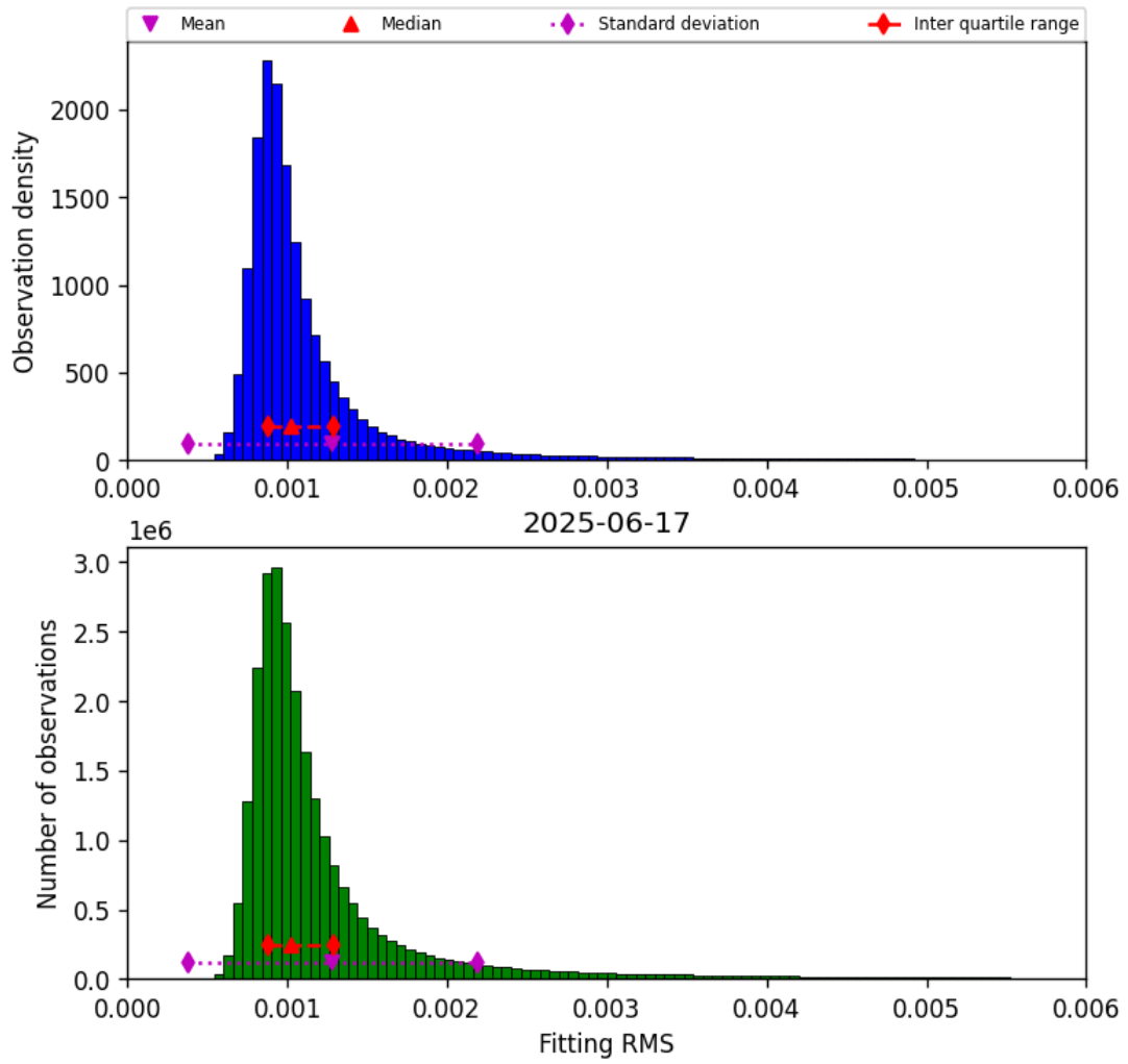
Figure 23: Histogram of “Fitting RMS” for 2025-06-17 to 2025-06-18
