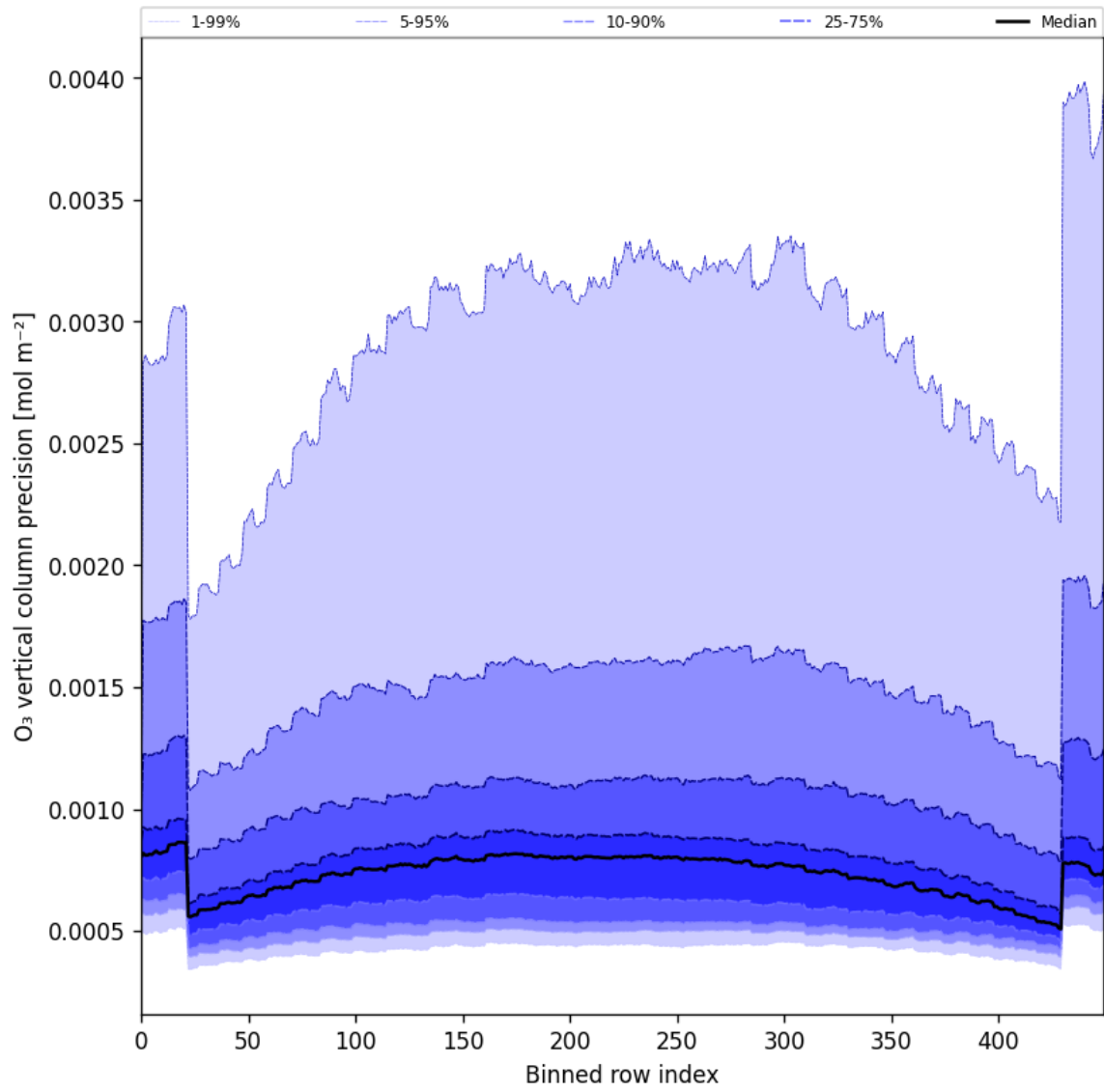
Figure 29: Along track statistics of “O 3 vertical column precision” for 2025-06-17 to 2025-06-18
