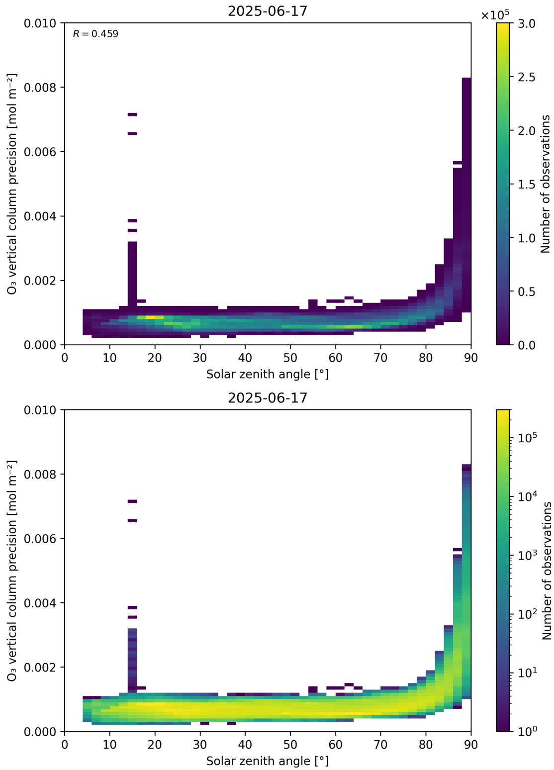
Figure 48: Scatter density plot of “Solar zenith angle” against “O 3 vertical column precision” for 2025-06-17 to 2025-06-18.
