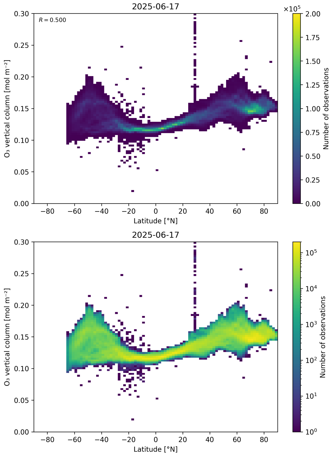
Figure 36: Scatter density plot of “Latitude” against “O 3 vertical column” for 2025-06-17 to 2025-06-18.
