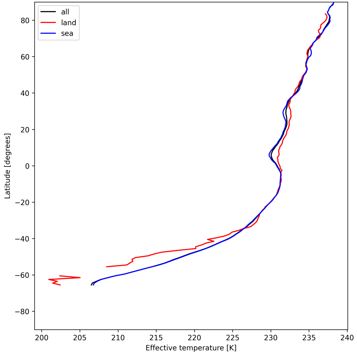
Figure 17: Zonal average of "Effective temperature" for 2025-06-17 to 2025-06-18.
