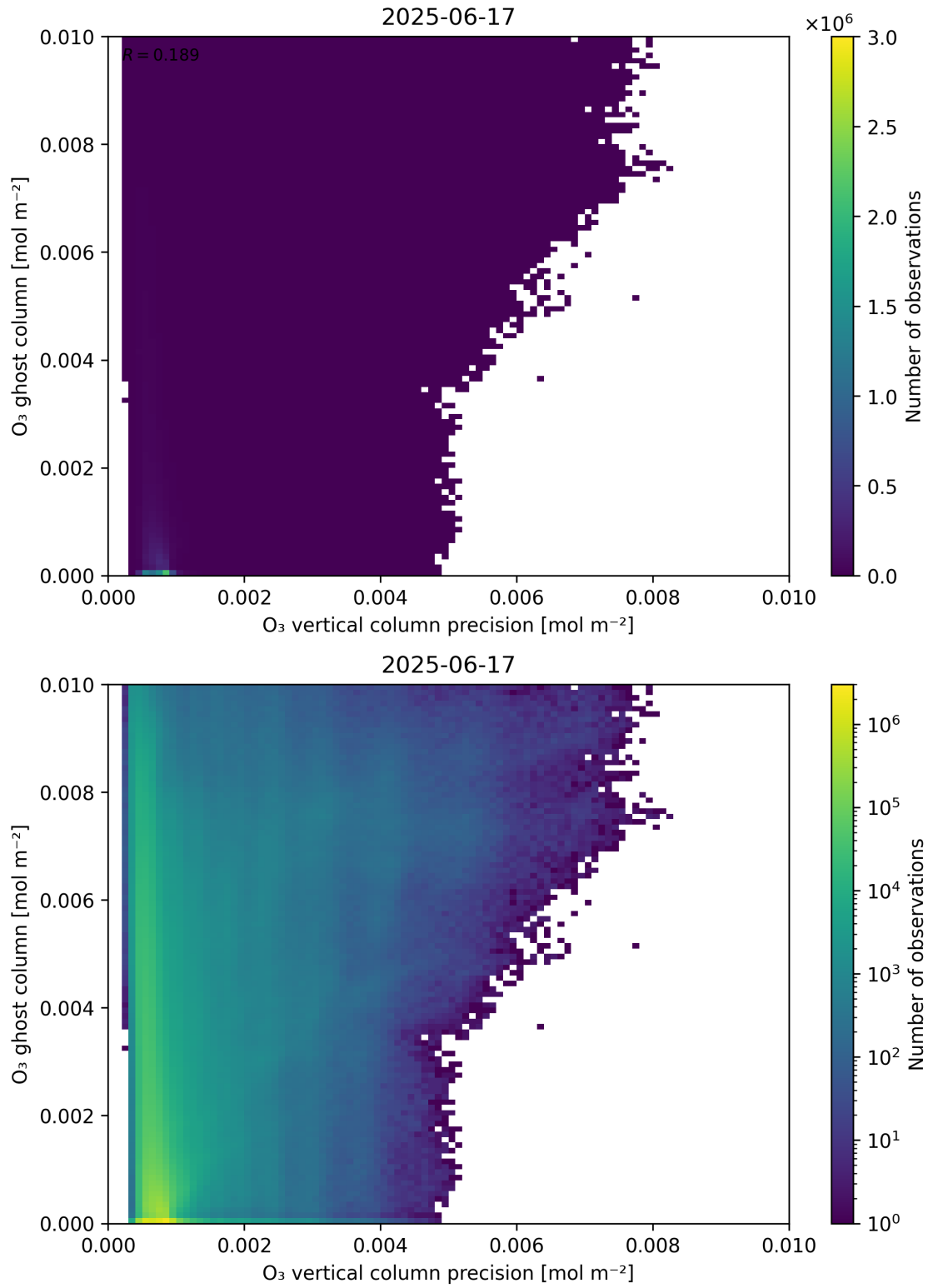
Figure 43: Scatter density plot of “ O_3 vertical column precision” against “ O_3 ghost column” for 2025-06-17 to 2025-06-18.
