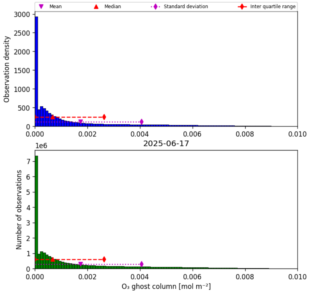
Figure 25: Histogram of “O 3 ghost column” for 2025-06-17 to 2025-06-18
