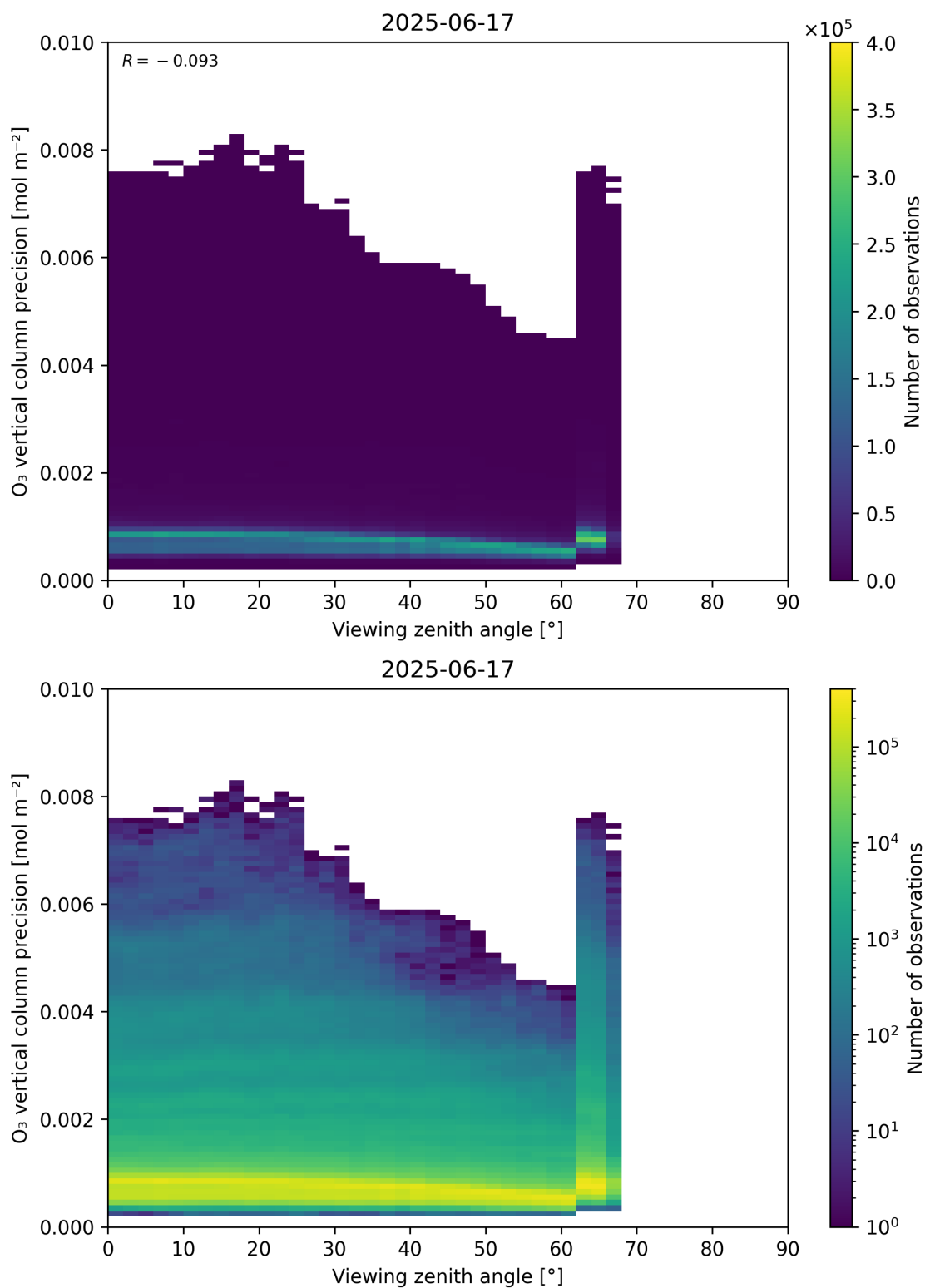
Figure 53: Scatter density plot of “Viewing zenith angle” against “O 3 vertical column precision” for 2025-06-17 to 2025-06-18.
