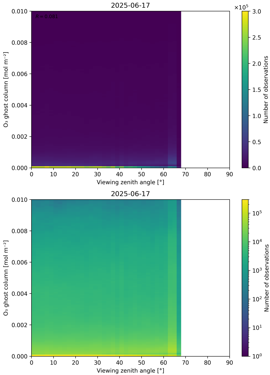
Figure 51: Scatter density plot of “Viewing zenith angle” against “O 3 ghost column” for 2025-06-17 to 2025-06-18.
