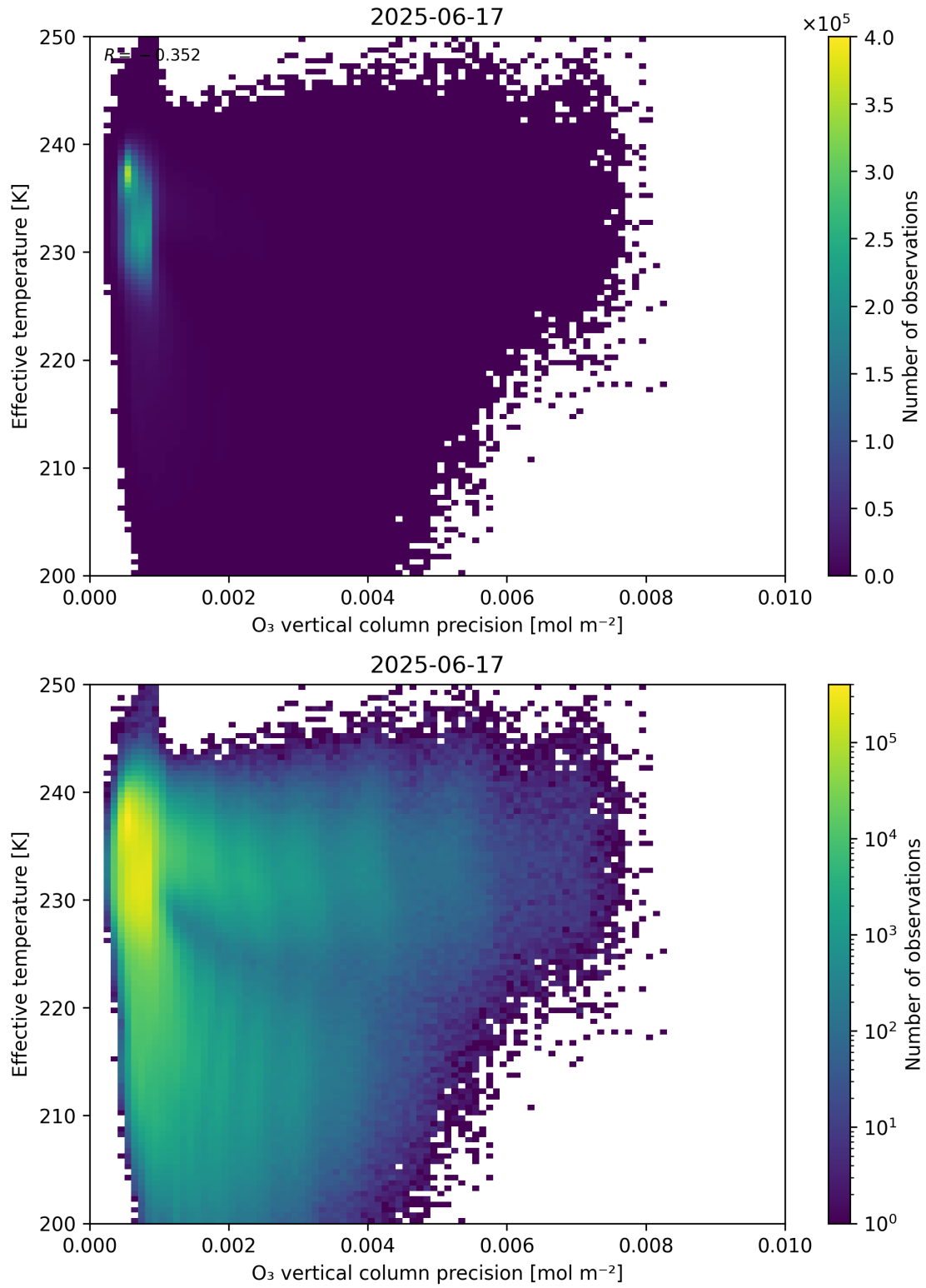
Figure 42: Scatter density plot of “O 3 vertical column precision” against “Effective temperature” for 2025-06-17 to 2025-06-18.
