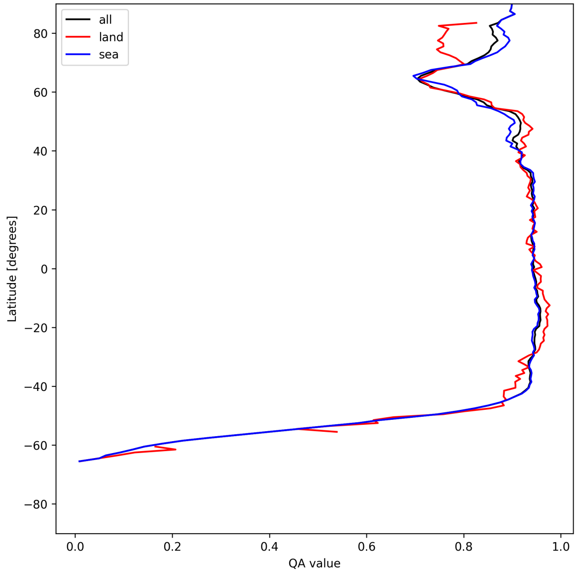
Figure 13: Zonal average of “QA value” for 2025-06-17 to 2025-06-18.
