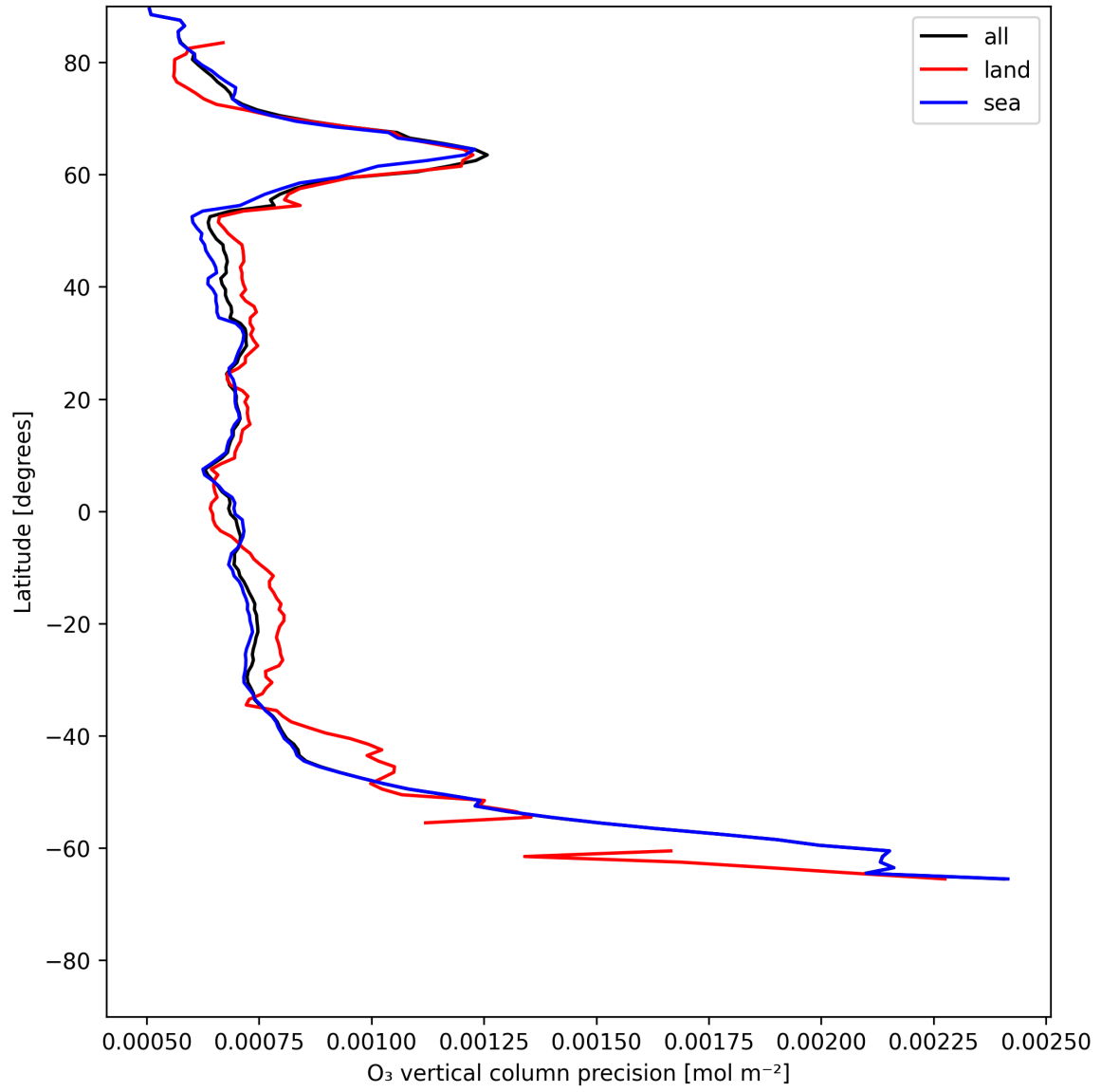
Figure 15: Zonal average of "O 3 vertical column precision" for 2025-06-17 to 2025-06-18.
