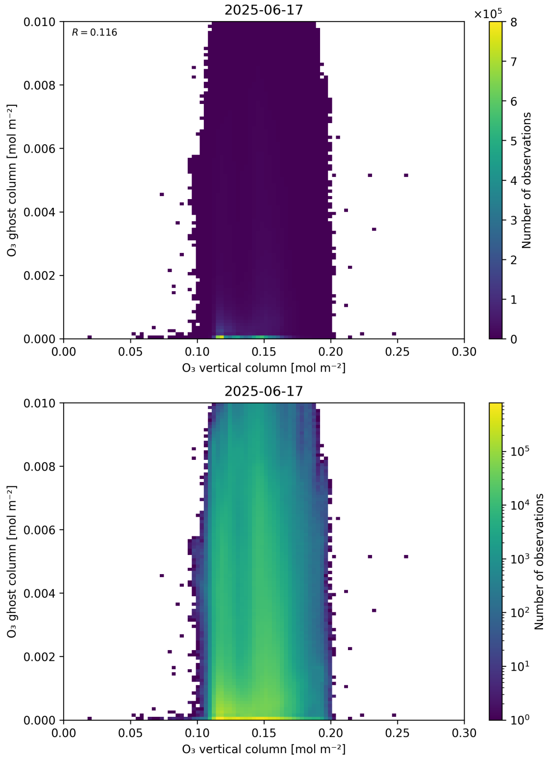
Figure 40: Scatter density plot of “O 3 vertical column” against “O 3 ghost column” for 2025-06-17 to 2025-06-18.
