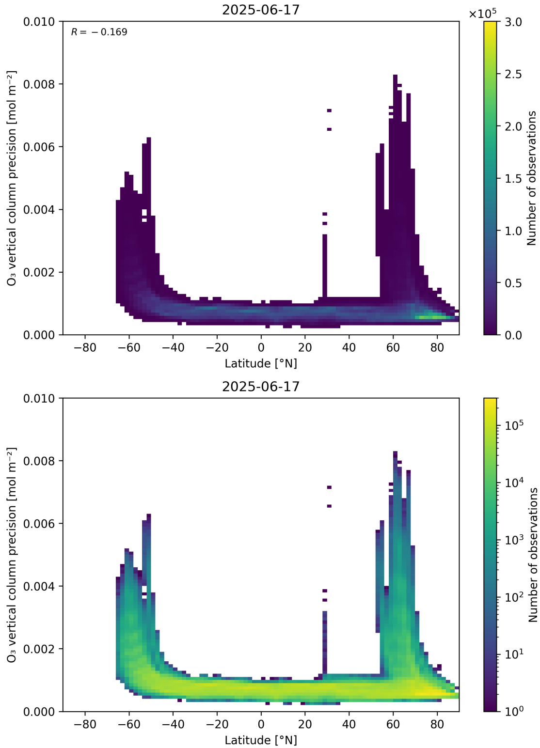
Figure 37: Scatter density plot of “Latitude” against “O 3 vertical column precision” for 2025-06-17 to 2025-06-18.
