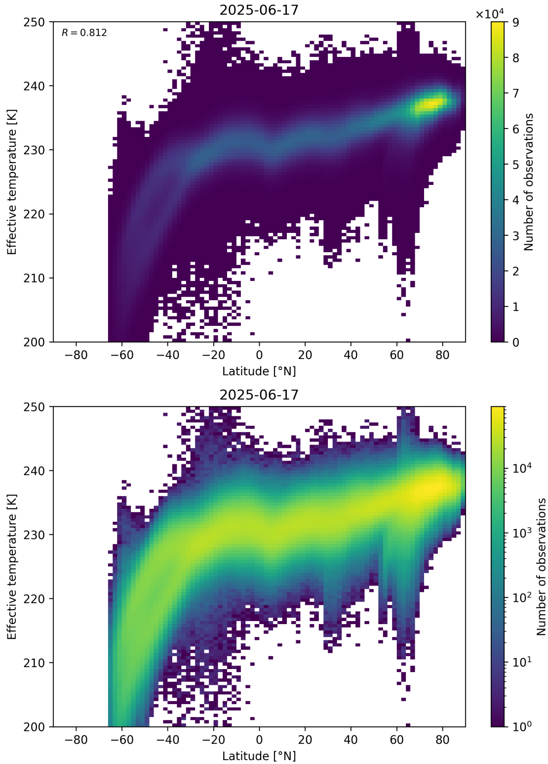
Figure 34: Scatter density plot of “Latitude” against “Effective temperature” for 2025-06-17 to 2025-06-18.
