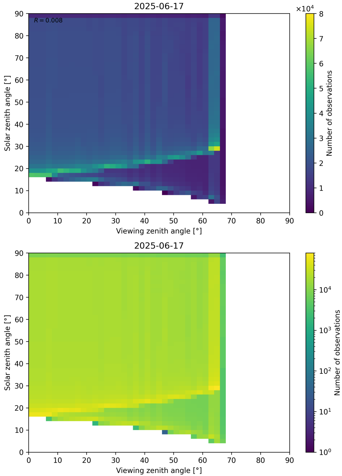
Figure 54: Scatter density plot of “Viewing zenith angle” against “Solar zenith angle” for 2025-06-17 to 2025-06-18.
