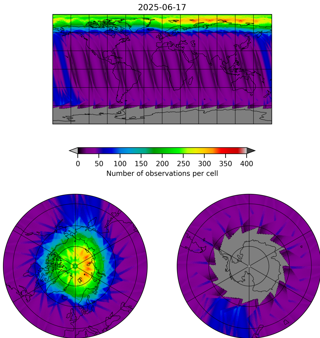
Figure 12: Map of the number of observations for 2025-06-17 to 2025-06-18
