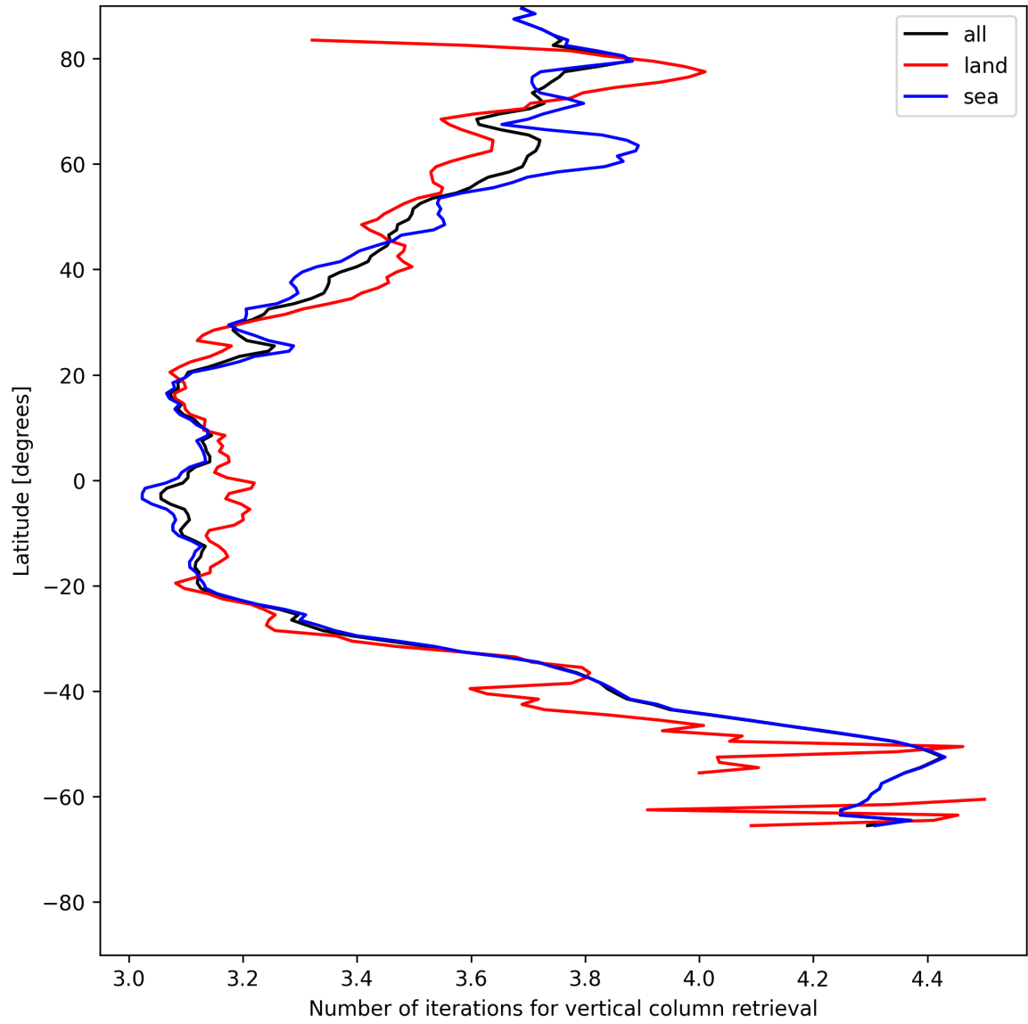
Figure 19: Zonal average of “Number of iterations for vertical column retrieval” for 2025-06-17 to 2025-06-18.
