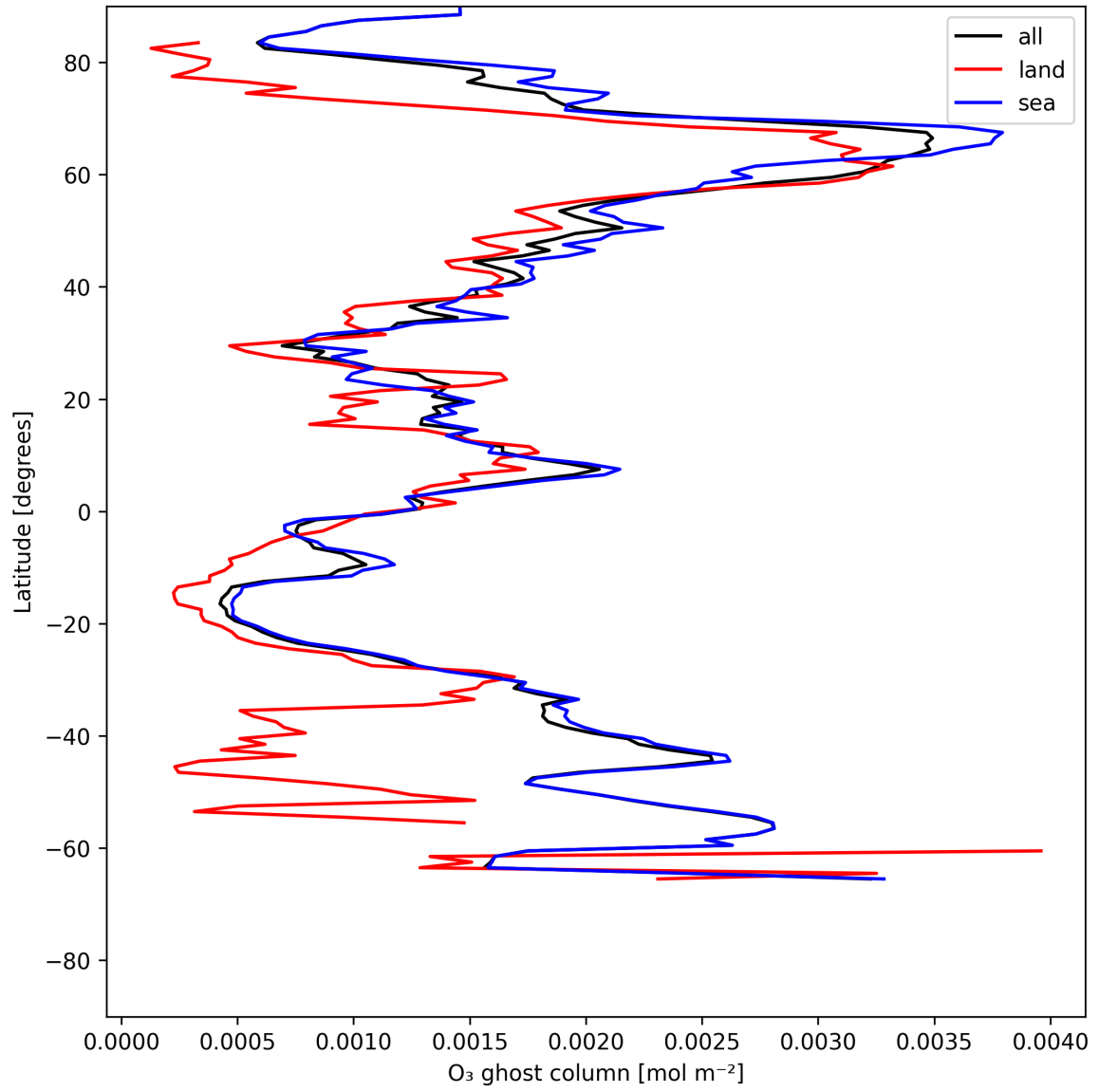
Figure 18: Zonal average of “O 3 ghost column” for 2025-06-17 to 2025-06-18.
