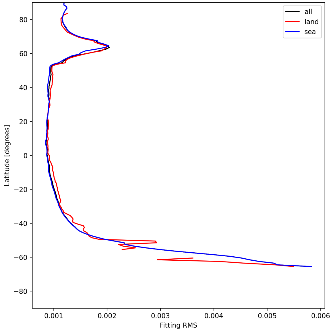
Figure 16: Zonal average of “Fitting RMS” for 2025-06-17 to 2025-06-18.
