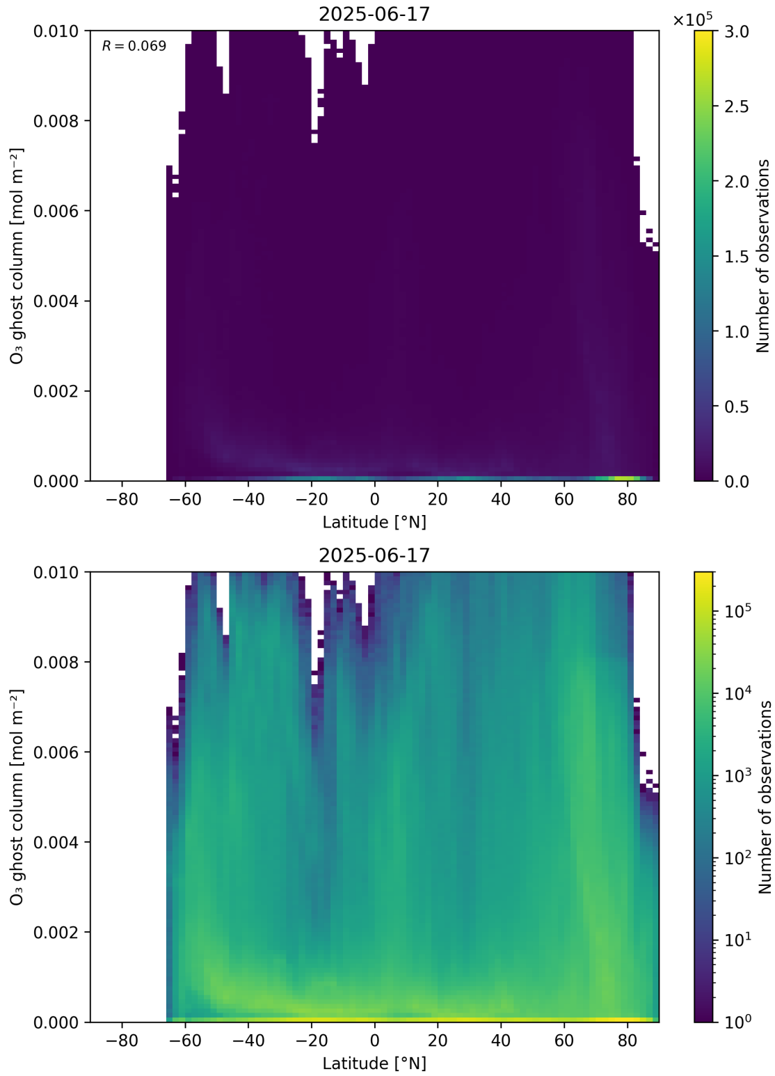
Figure 35: Scatter density plot of “Latitude” against “O 3 ghost column” for 2025-06-17 to 2025-06-18.
