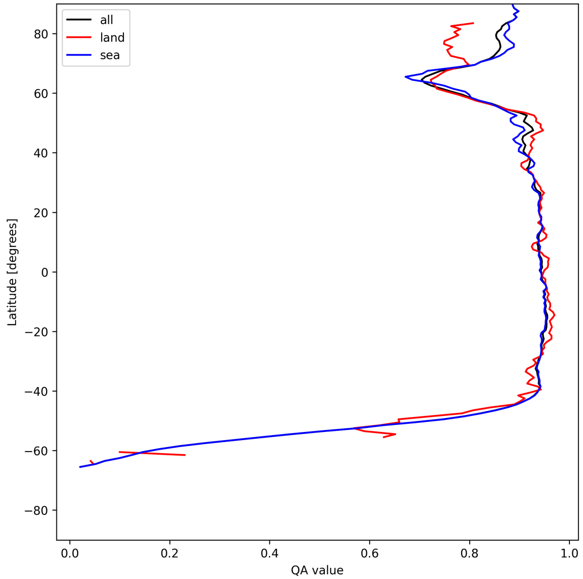
Figure 13: Zonal average of “QA value” for 2025-06-17 to 2025-06-19.
