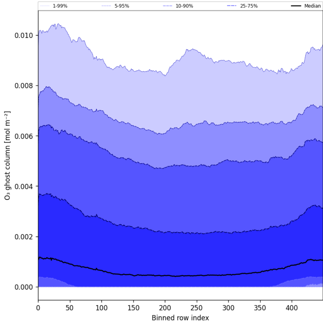
Figure 32: Along track statistics of “O 3 ghost column” for 2025-06-17 to 2025-06-19
