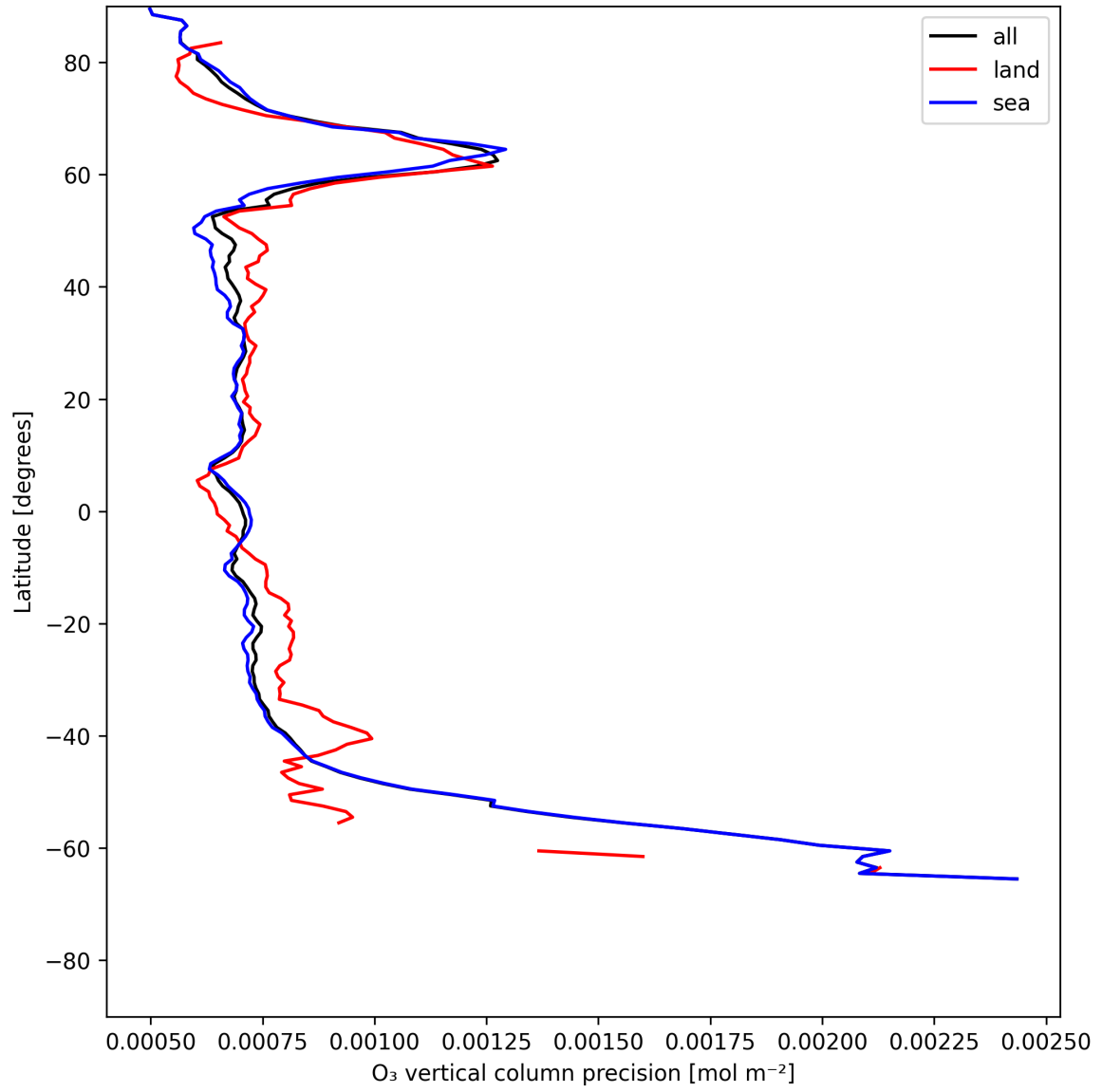
Figure 15: Zonal average of "O 3 vertical column precision" for 2025-06-17 to 2025-06-19.
