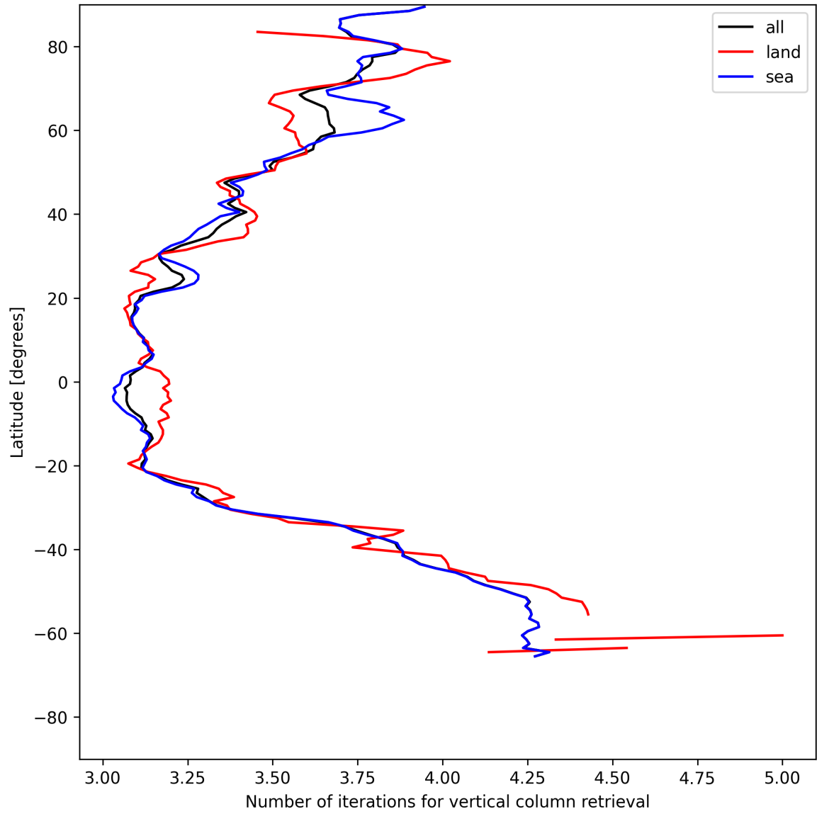
Figure 19: Zonal average of “Number of iterations for vertical column retrieval” for 2025-06-17 to 2025-06-19.
