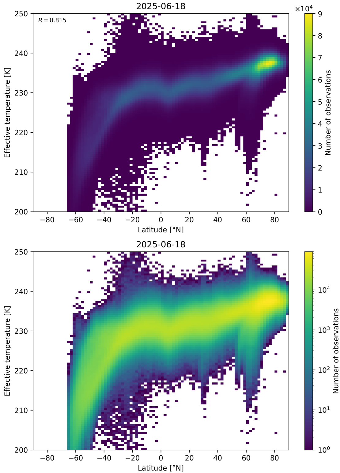
Figure 34: Scatter density plot of “Latitude” against “Effective temperature” for 2025-06-17 to 2025-06-19.
