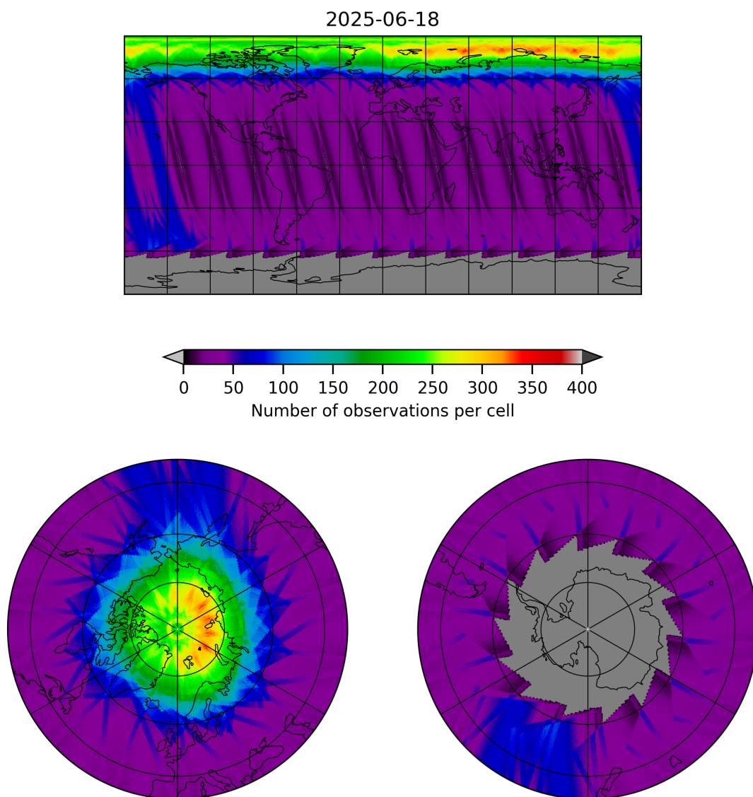
Figure 12: Map of the number of observations for 2025-06-17 to 2025-06-19
