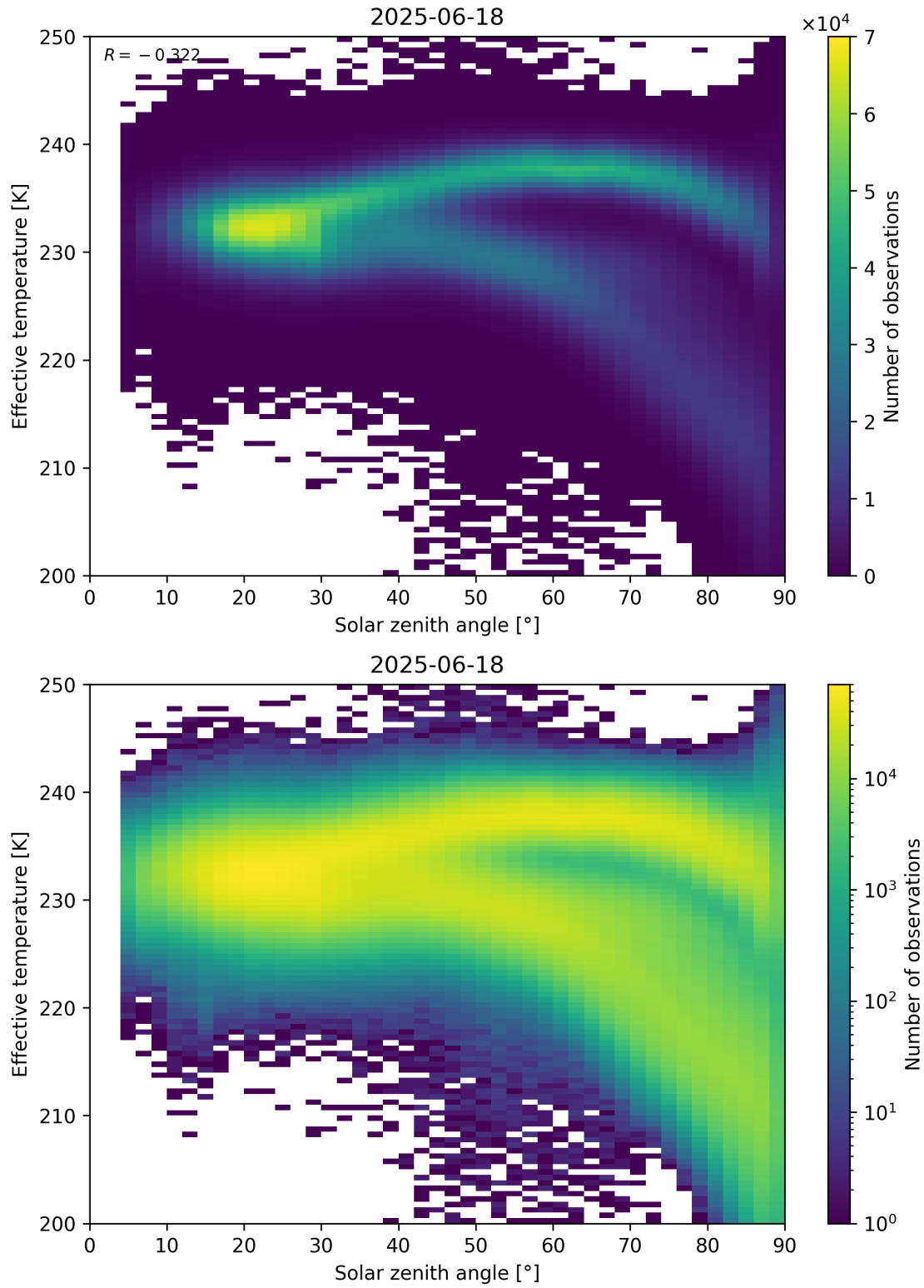
Figure 45: Scatter density plot of “Solar zenith angle” against “Effective temperature” for 2025-06-17 to 2025-06-19.
