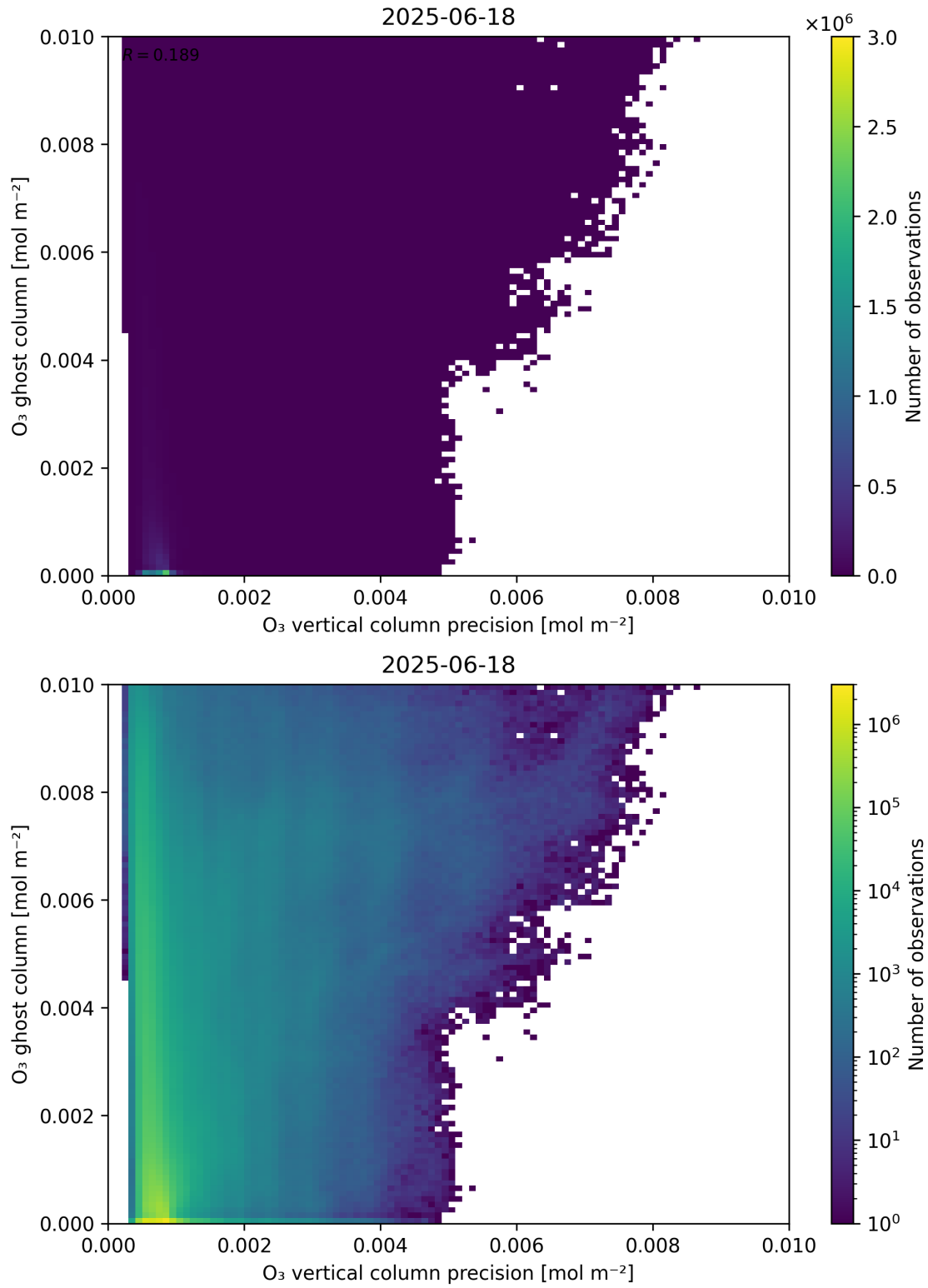
Figure 43: Scatter density plot of “ \text{O}_3 vertical column precision” against “ \text{O}_3 ghost column” for 2025-06-17 to 2025-06-19.
