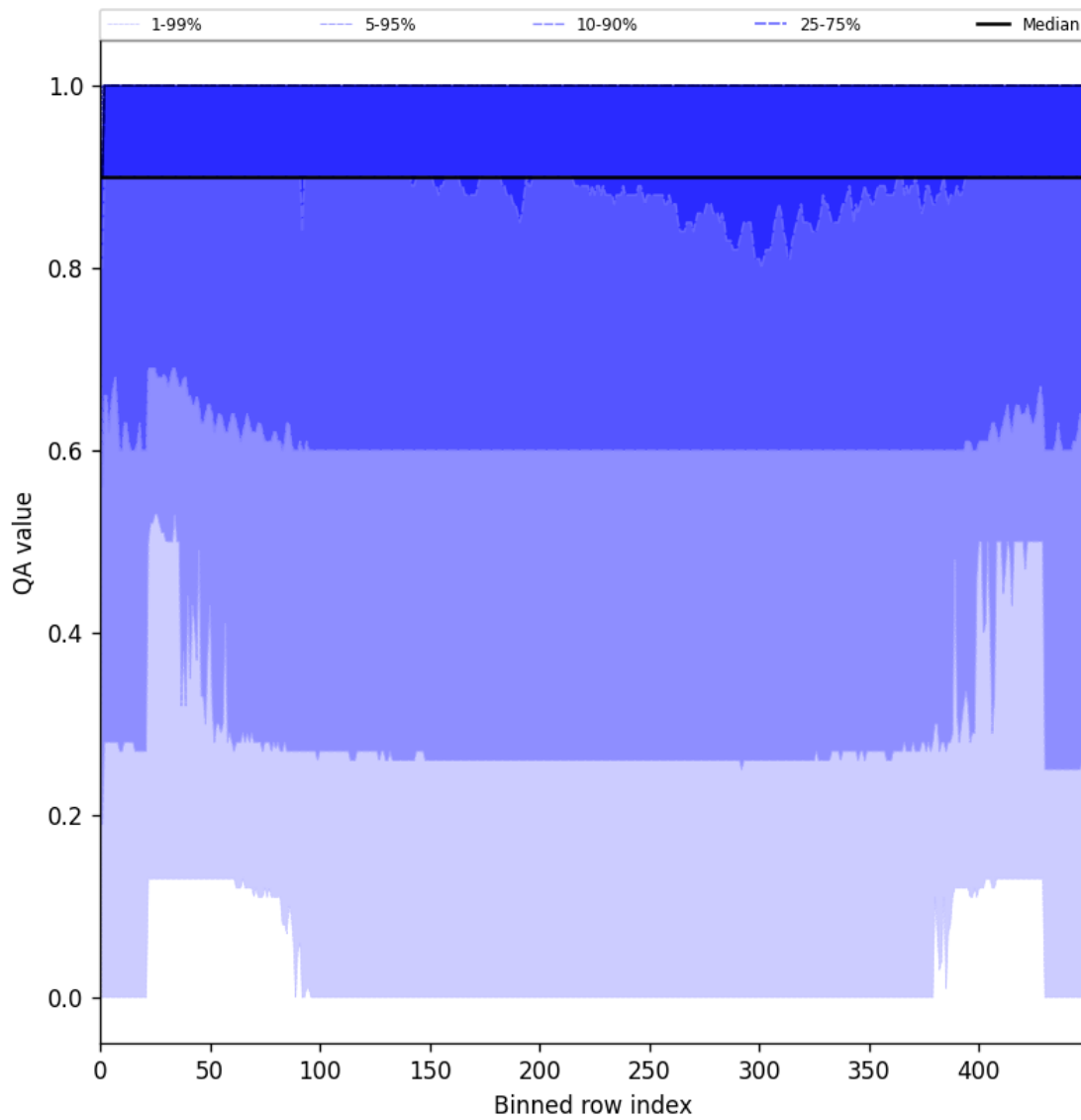
Figure 27: Along track statistics of “QA value” for 2025-06-17 to 2025-06-19
