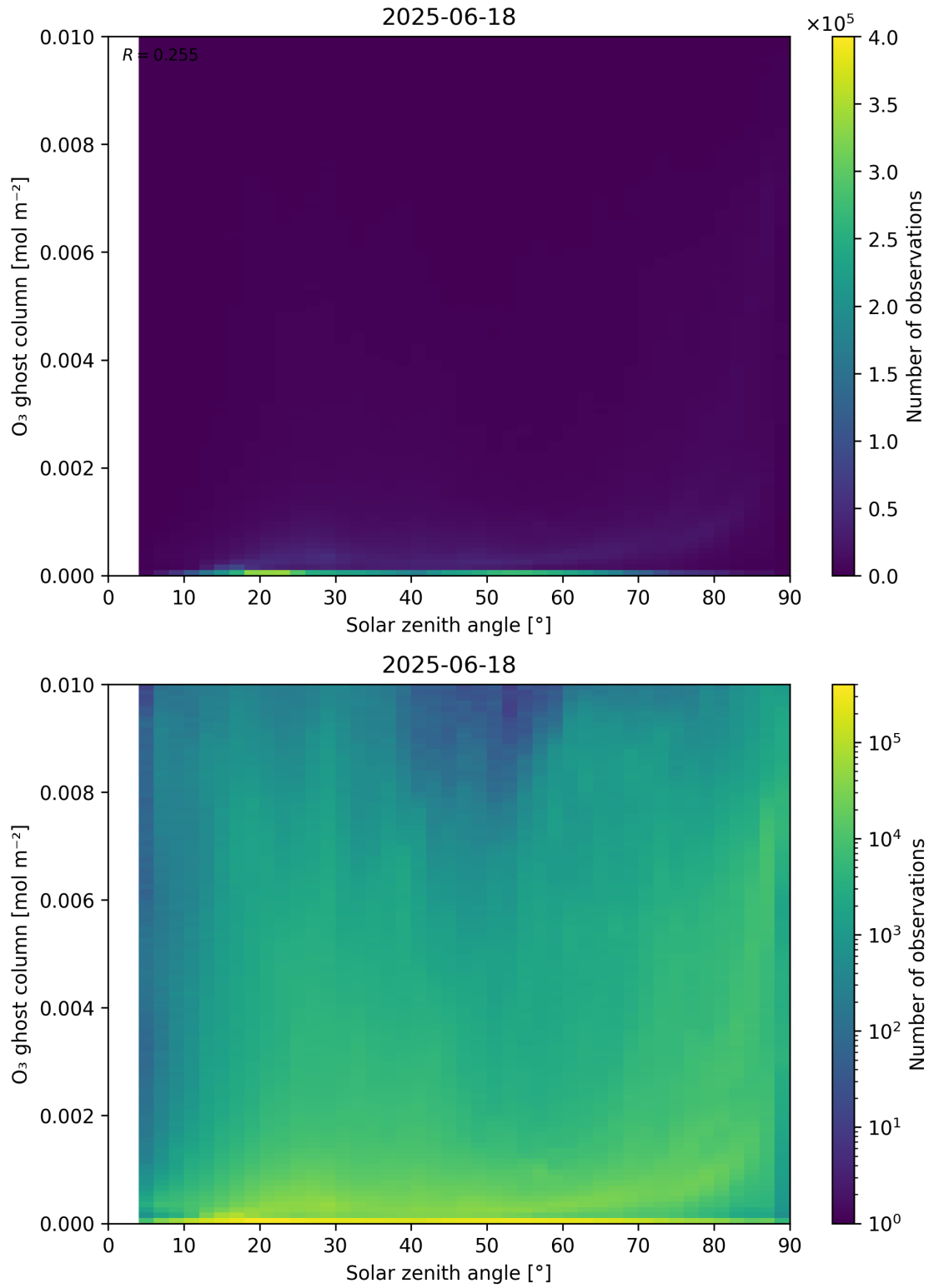
Figure 46: Scatter density plot of “Solar zenith angle” against “O 3 ghost column” for 2025-06-17 to 2025-06-19.
