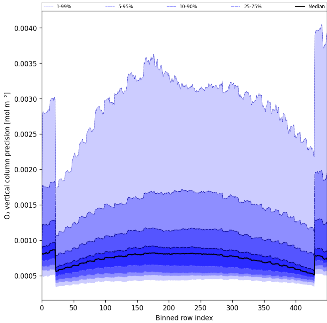
Figure 29: Along track statistics of “O 3 vertical column precision” for 2025-06-17 to 2025-06-19
