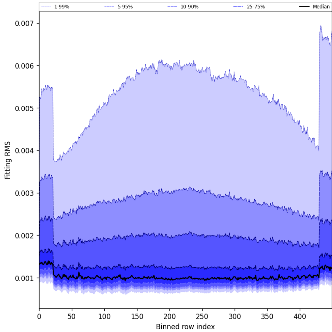
Figure 30: Along track statistics of “Fitting RMS” for 2025-06-17 to 2025-06-19
