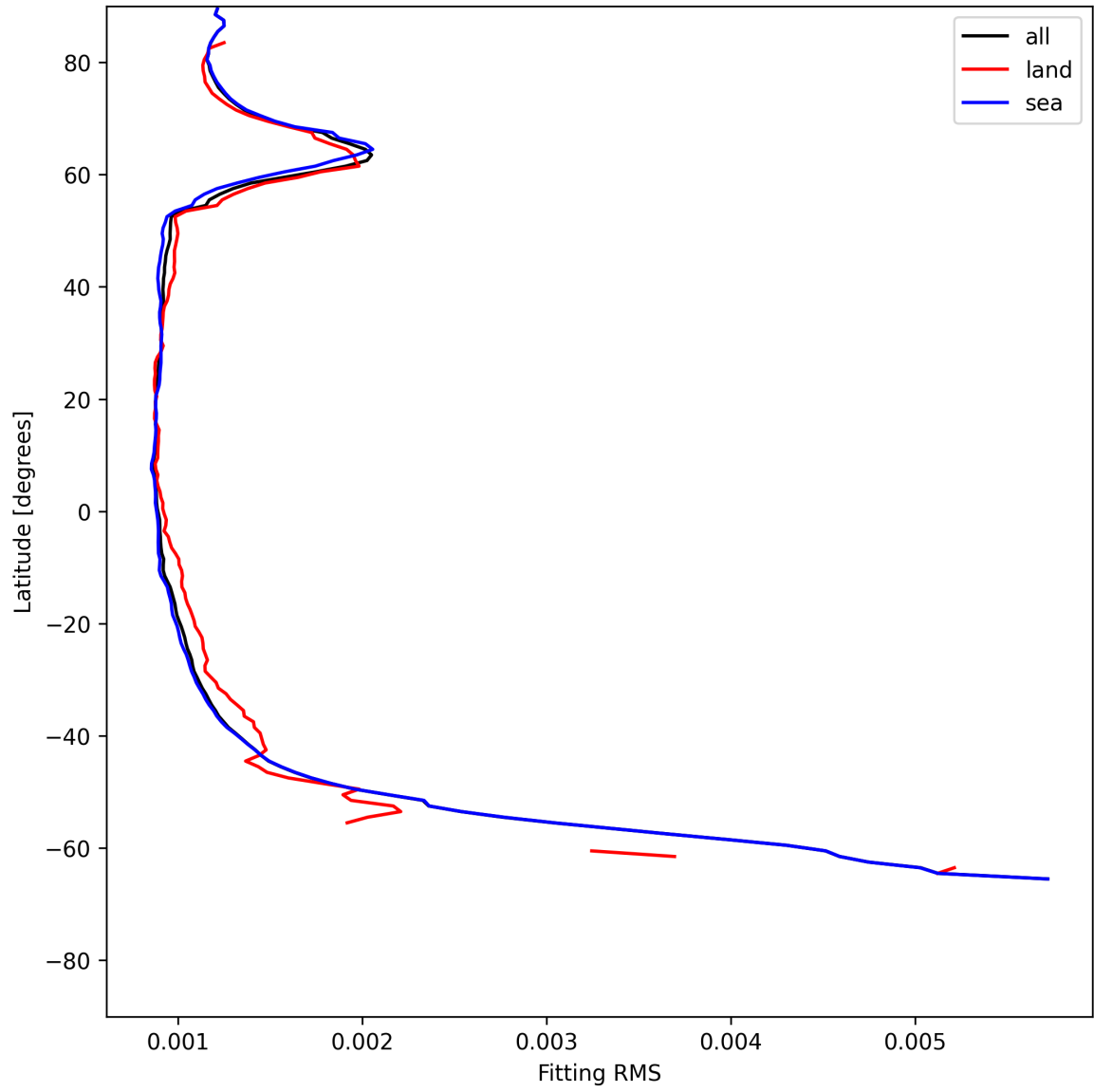
Figure 16: Zonal average of “Fitting RMS” for 2025-06-17 to 2025-06-19.
