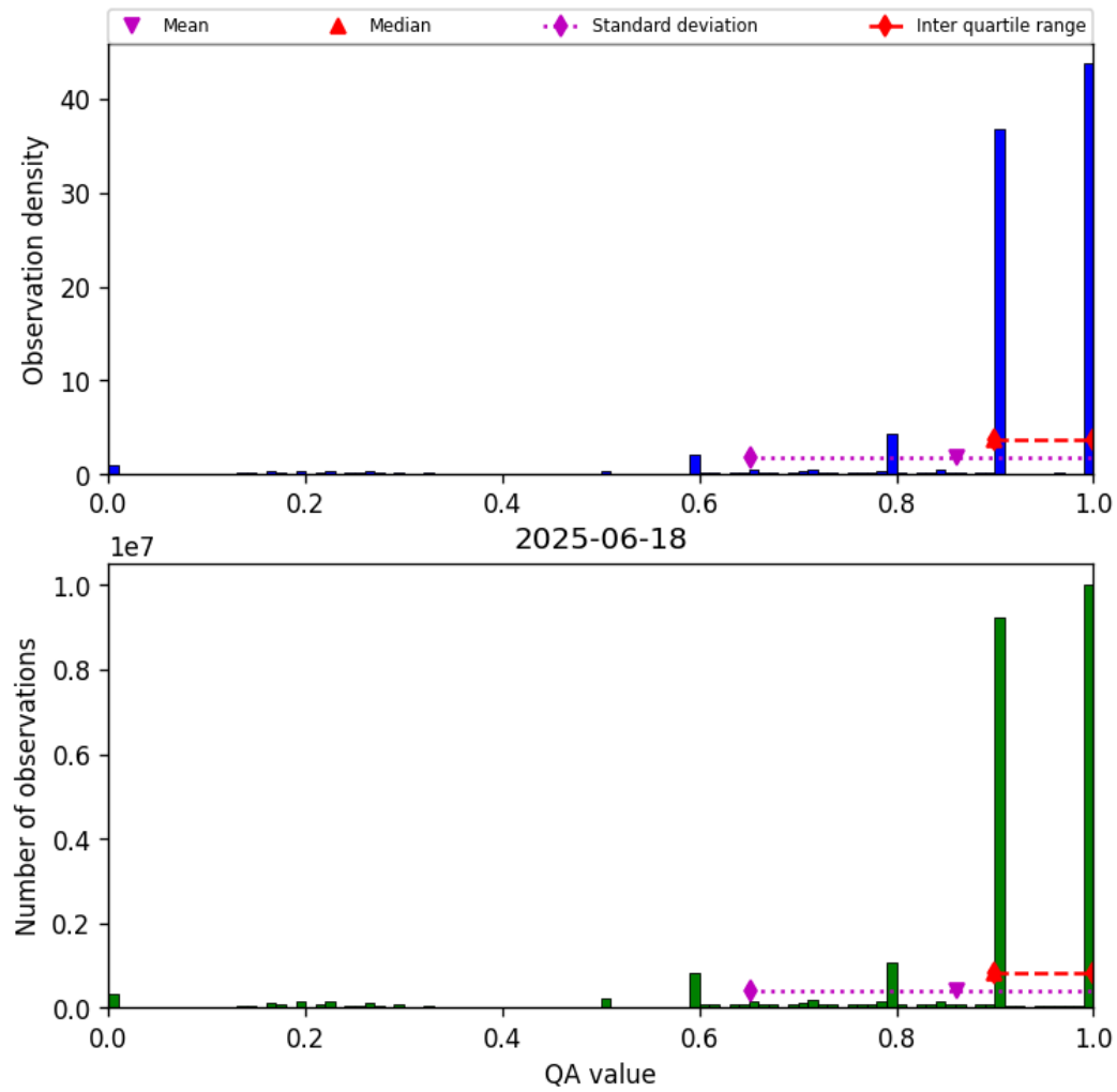
Figure 20: Histogram of “QA value” for 2025-06-17 to 2025-06-19
