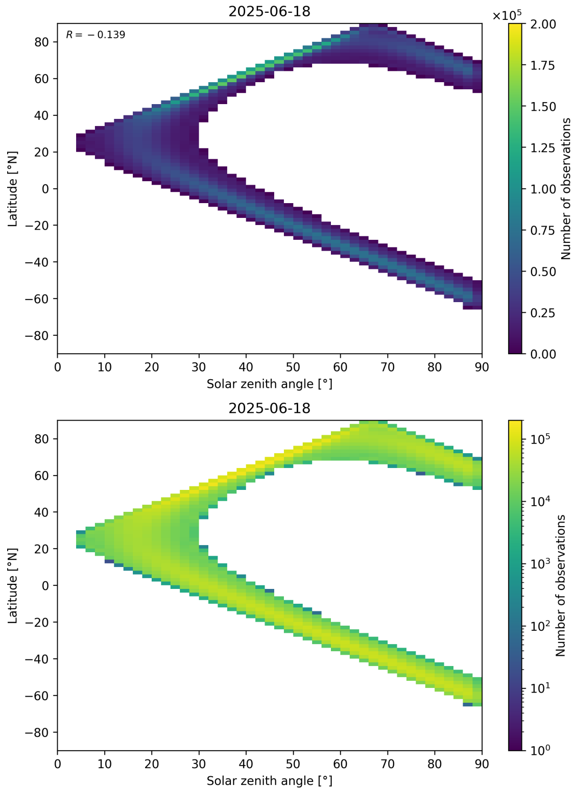
Figure 44: Scatter density plot of “Solar zenith angle” against “Latitude” for 2025-06-17 to 2025-06-19.
