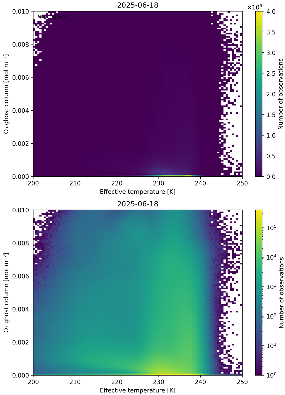
Figure 38: Scatter density plot of “Effective temperature” against “O 3 ghost column” for 2025-06-17 to 2025-06-19.
