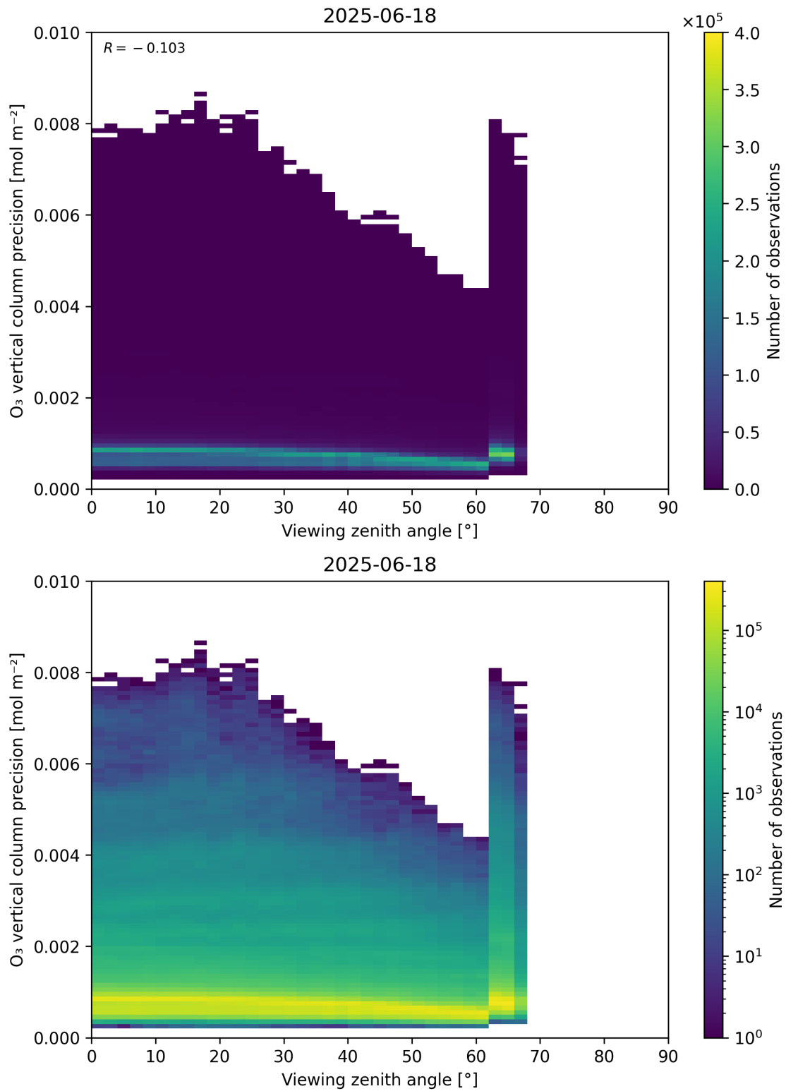
Figure 53: Scatter density plot of “Viewing zenith angle” against “O 3 vertical column precision” for 2025-06-17 to 2025-06-19.
