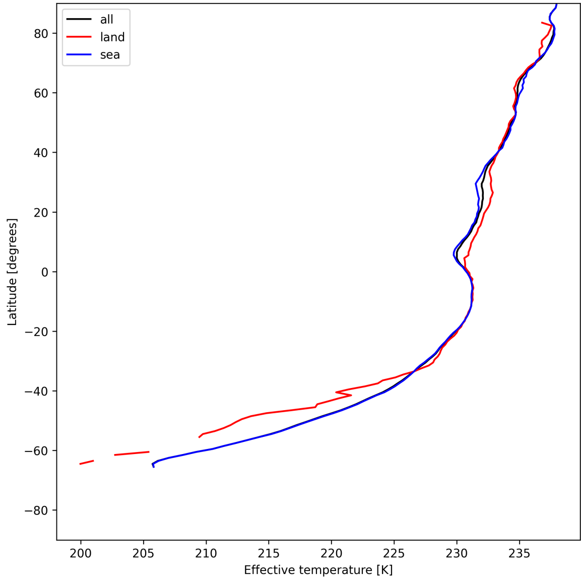
Figure 17: Zonal average of "Effective temperature" for 2025-06-17 to 2025-06-19.
