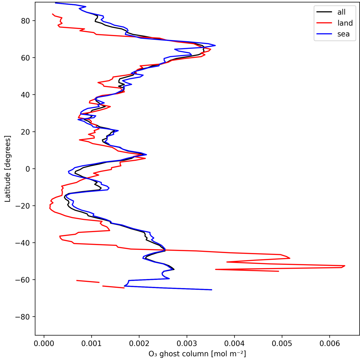
Figure 18: Zonal average of "O 3 ghost column" for 2025-06-17 to 2025-06-19.
