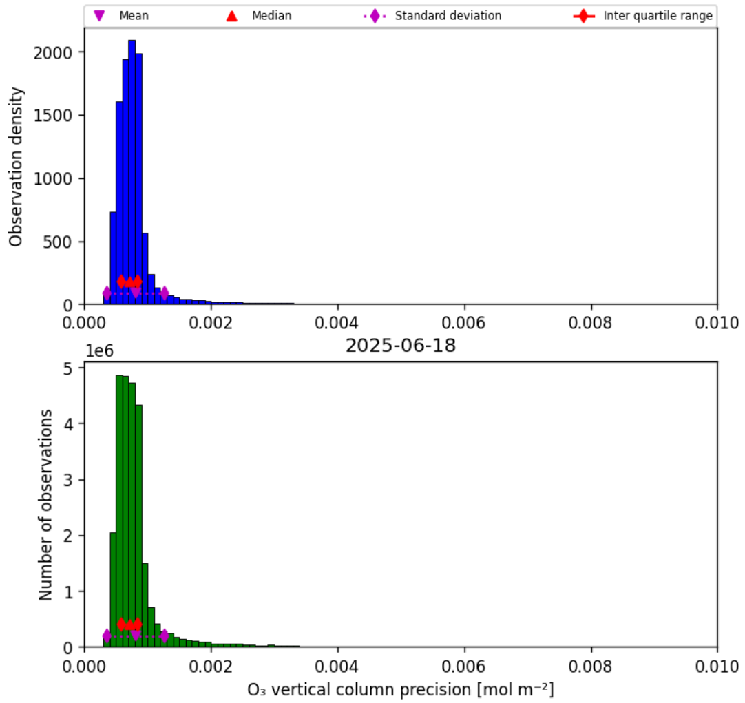
Figure 22: Histogram of "O 3 vertical column precision" for 2025-06-17 to 2025-06-19
