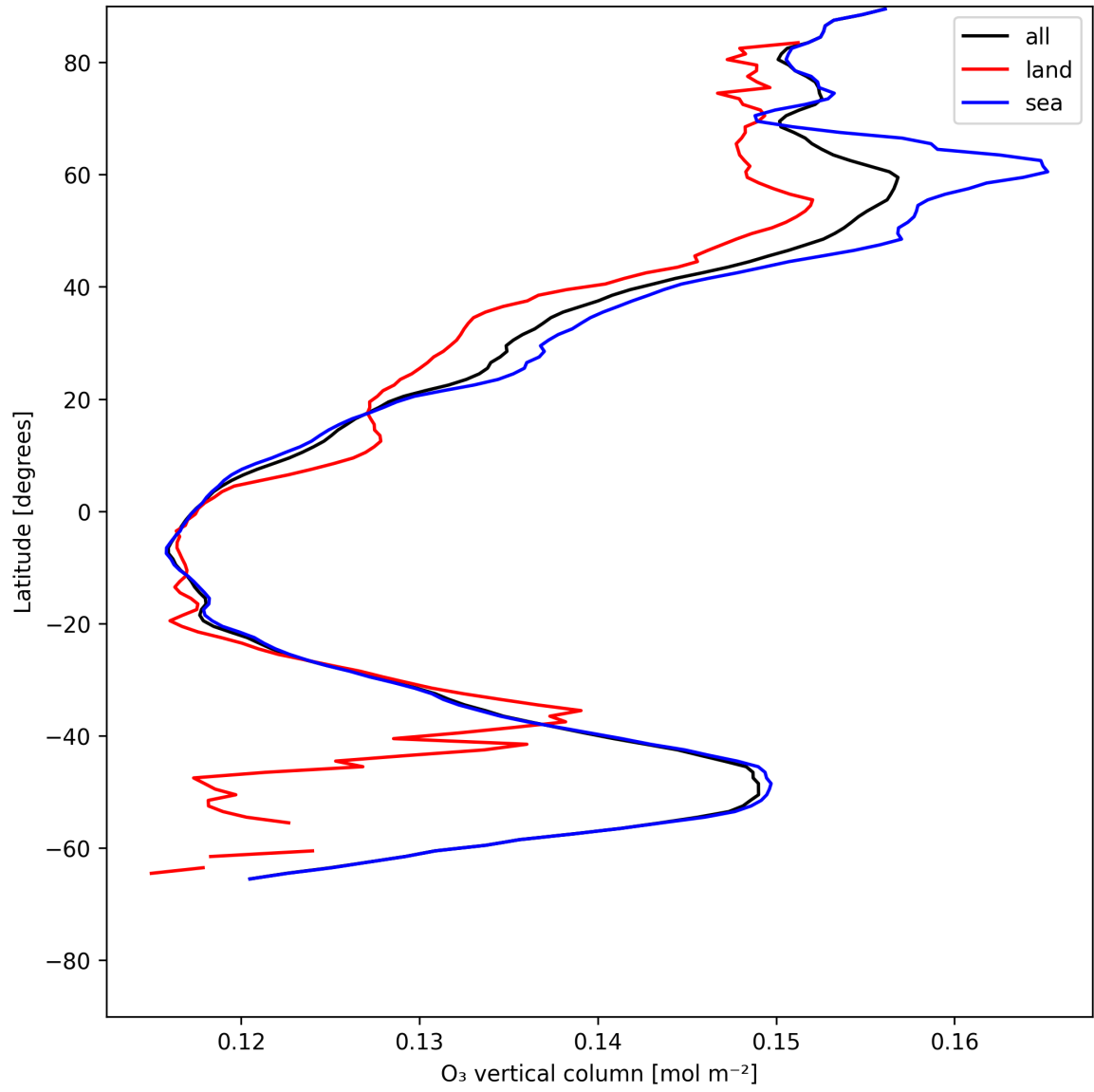
Figure 14: Zonal average of “O 3 vertical column” for 2025-06-17 to 2025-06-19.
