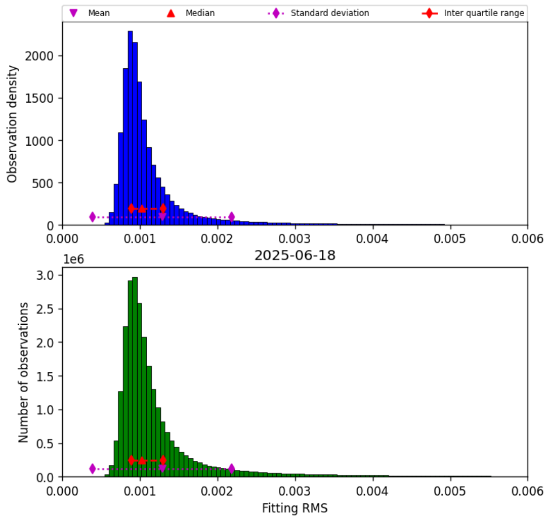
Figure 23: Histogram of “Fitting RMS” for 2025-06-17 to 2025-06-19
