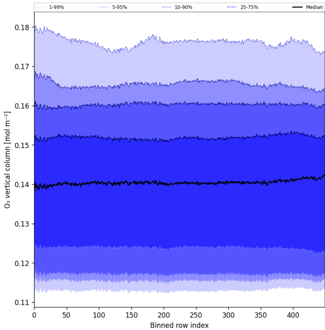
Figure 28: Along track statistics of “O 3 vertical column” for 2025-06-17 to 2025-06-19
