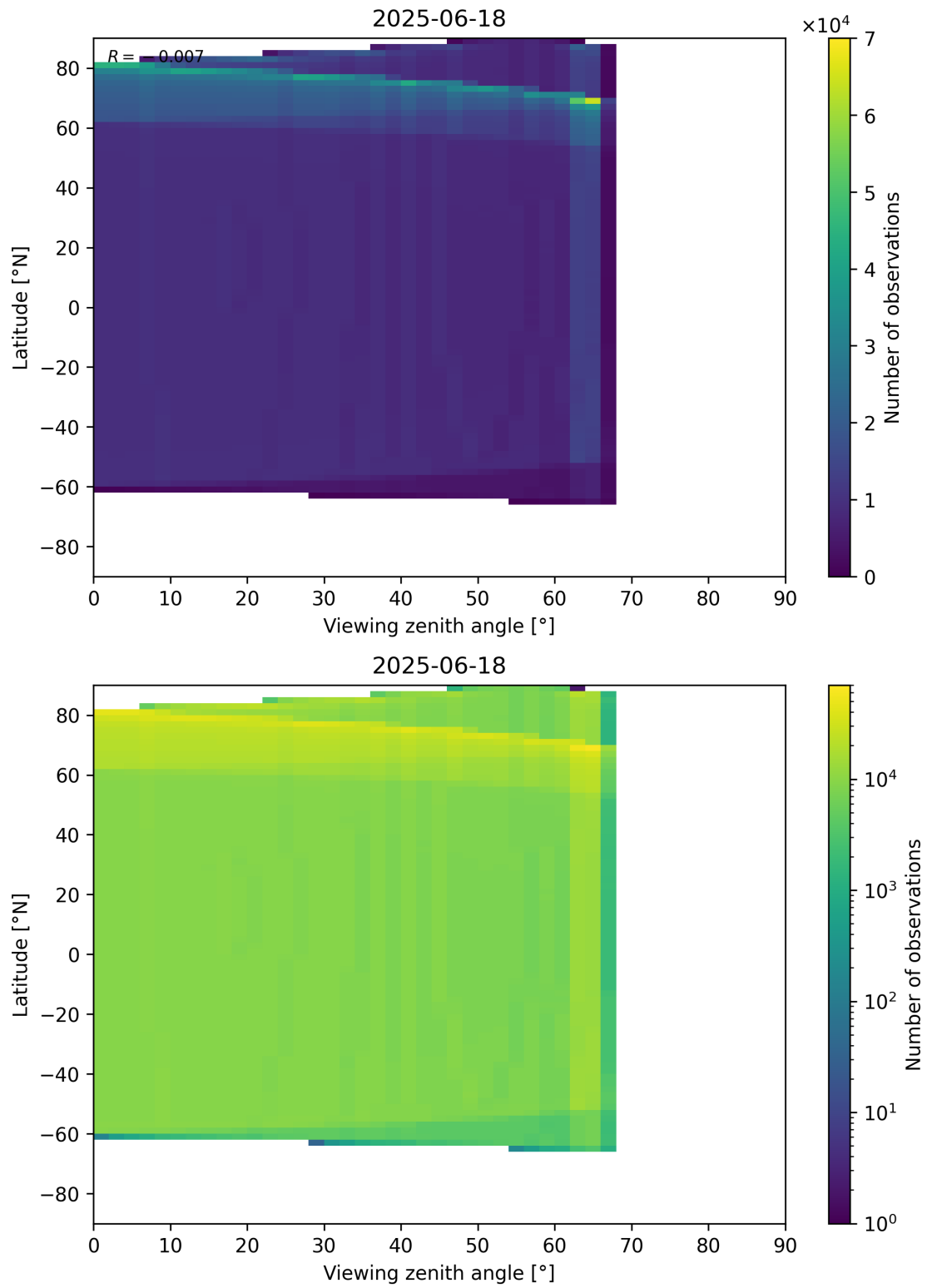
Figure 49: Scatter density plot of “Viewing zenith angle” against “Latitude” for 2025-06-17 to 2025-06-19.
