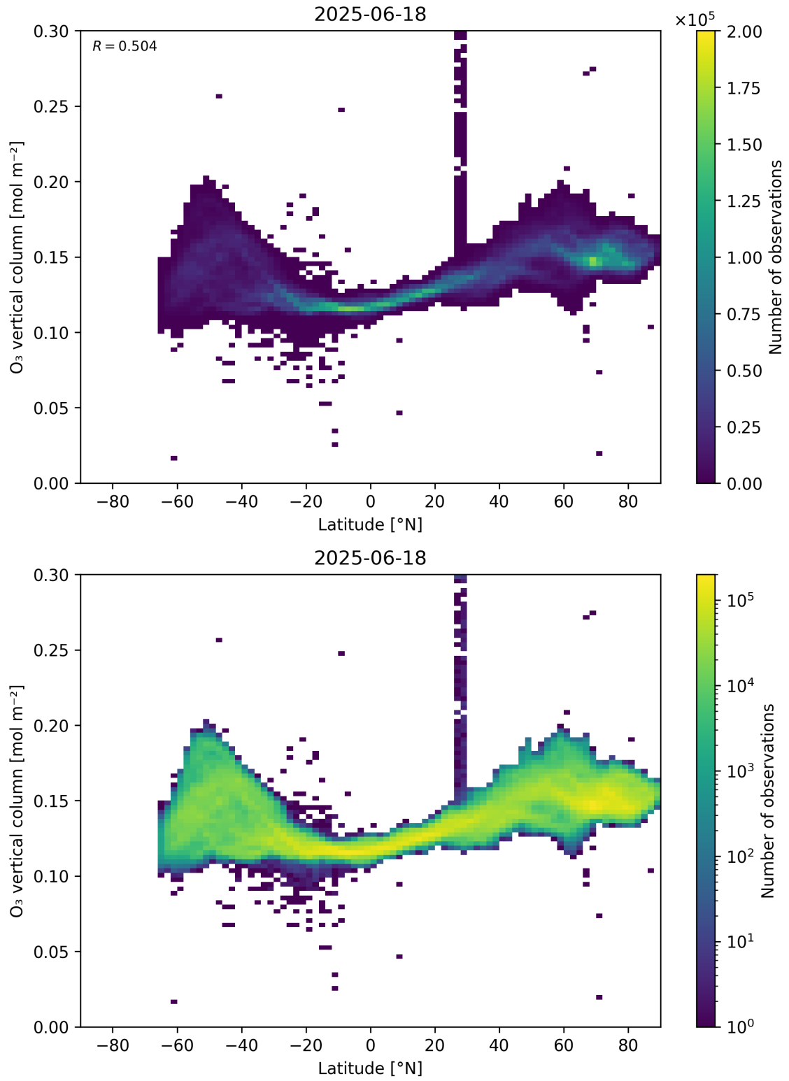
Figure 36: Scatter density plot of “Latitude” against “O 3 vertical column” for 2025-06-17 to 2025-06-19.
