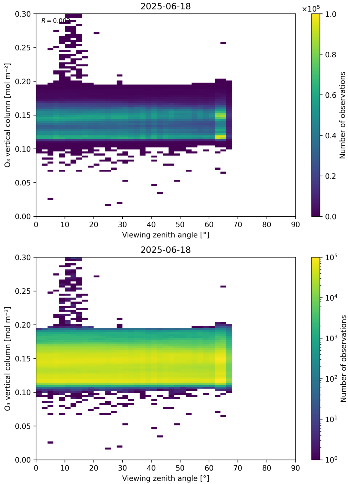
Figure 52: Scatter density plot of “Viewing zenith angle” against “O 3 vertical column” for 2025-06-17 to 2025-06-19.
