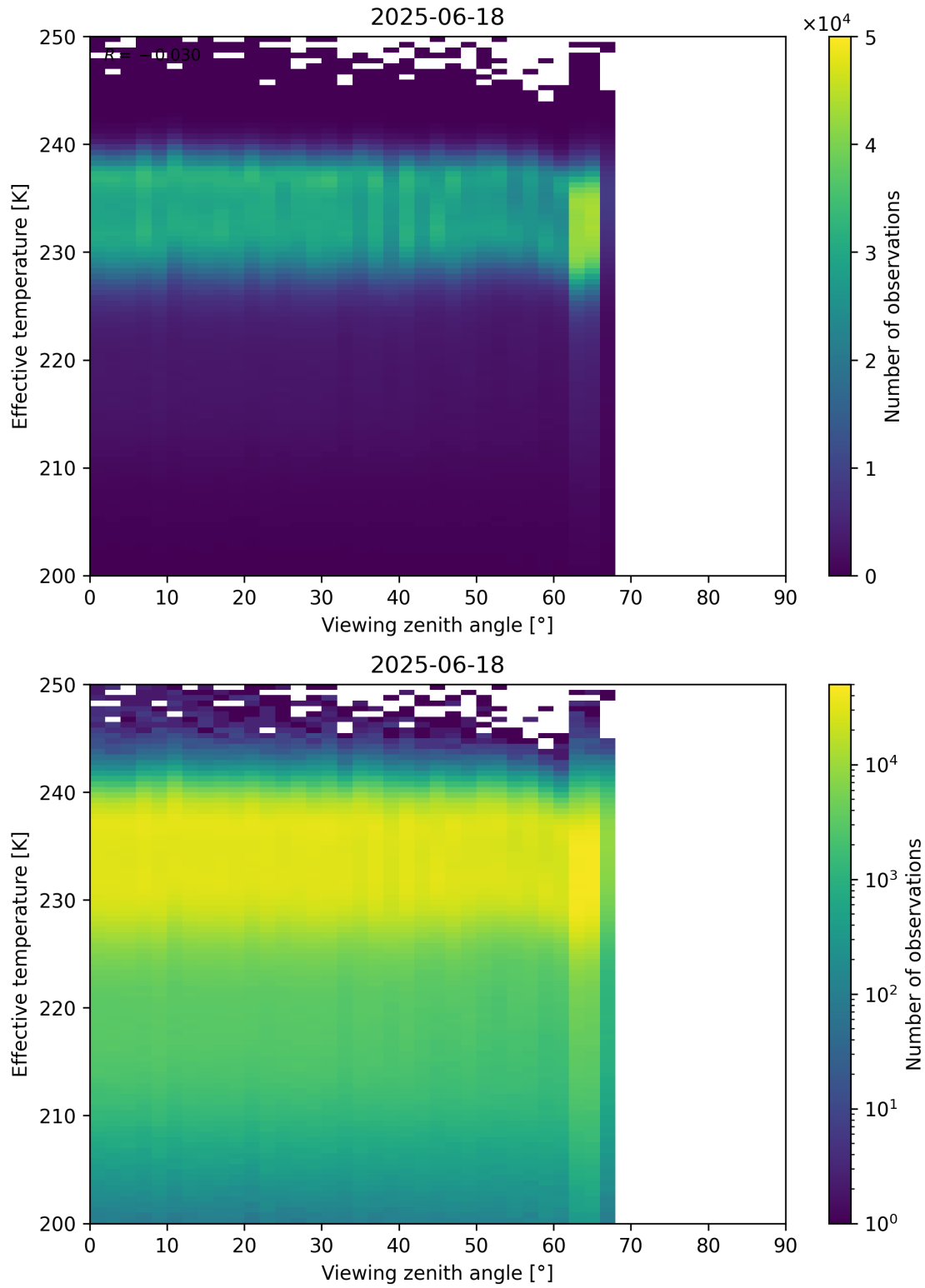
Figure 50: Scatter density plot of “Viewing zenith angle” against “Effective temperature” for 2025-06-17 to 2025-06-19.
