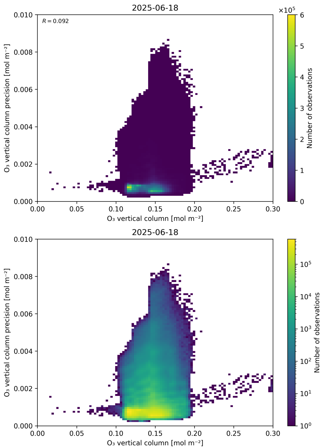
Figure 41: Scatter density plot of “O 3 vertical column” against “O 3 vertical column precision” for 2025-06-17 to 2025-06-19.
