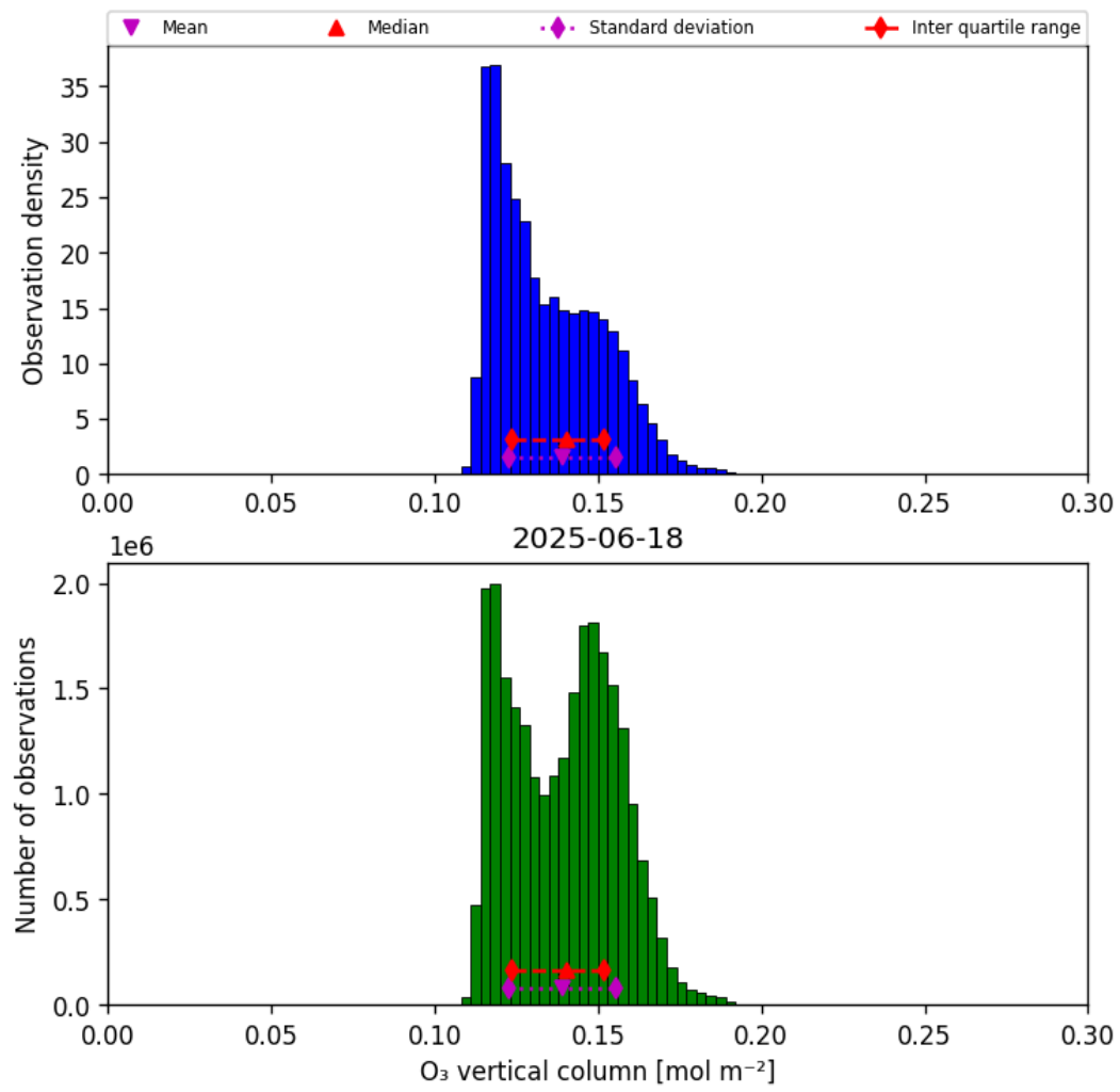
Figure 21: Histogram of “O 3 vertical column” for 2025-06-17 to 2025-06-19
