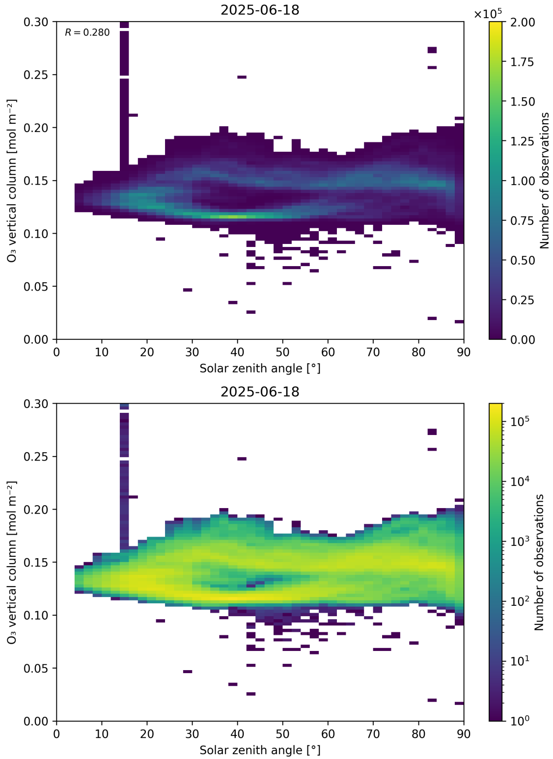
Figure 47: Scatter density plot of “Solar zenith angle” against “O 3 vertical column” for 2025-06-17 to 2025-06-19.
