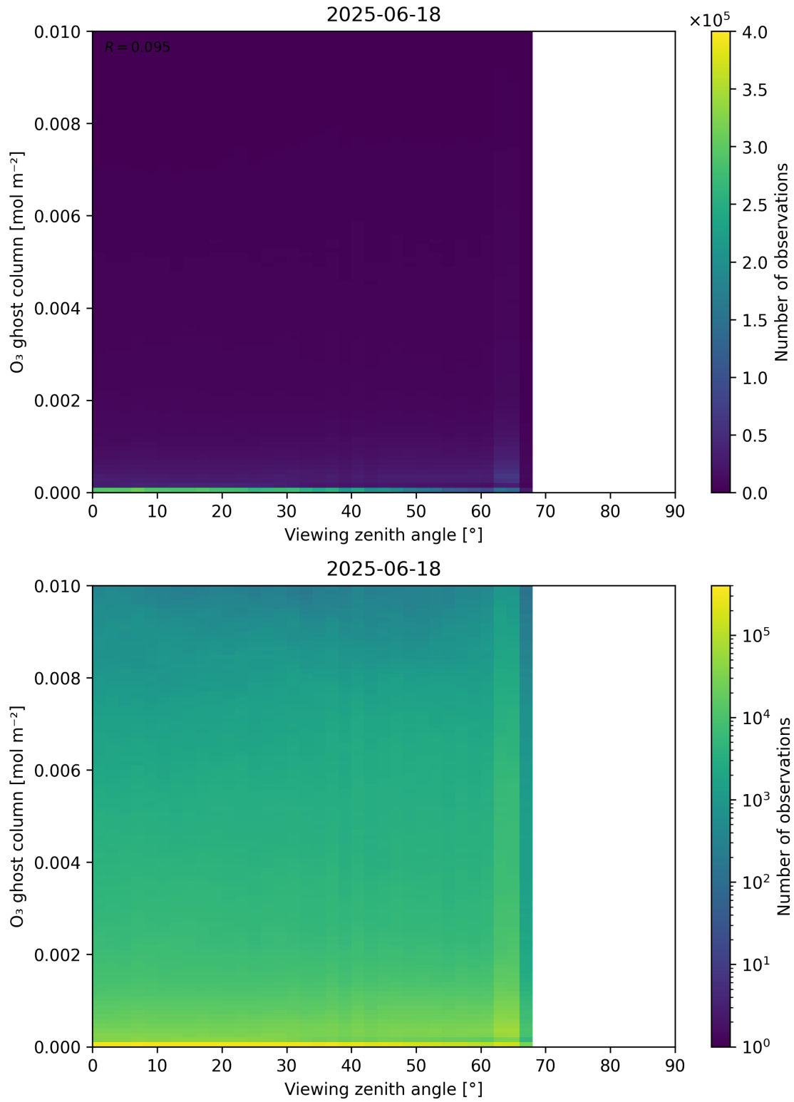
Figure 51: Scatter density plot of “Viewing zenith angle” against “O 3 ghost column” for 2025-06-17 to 2025-06-19.
