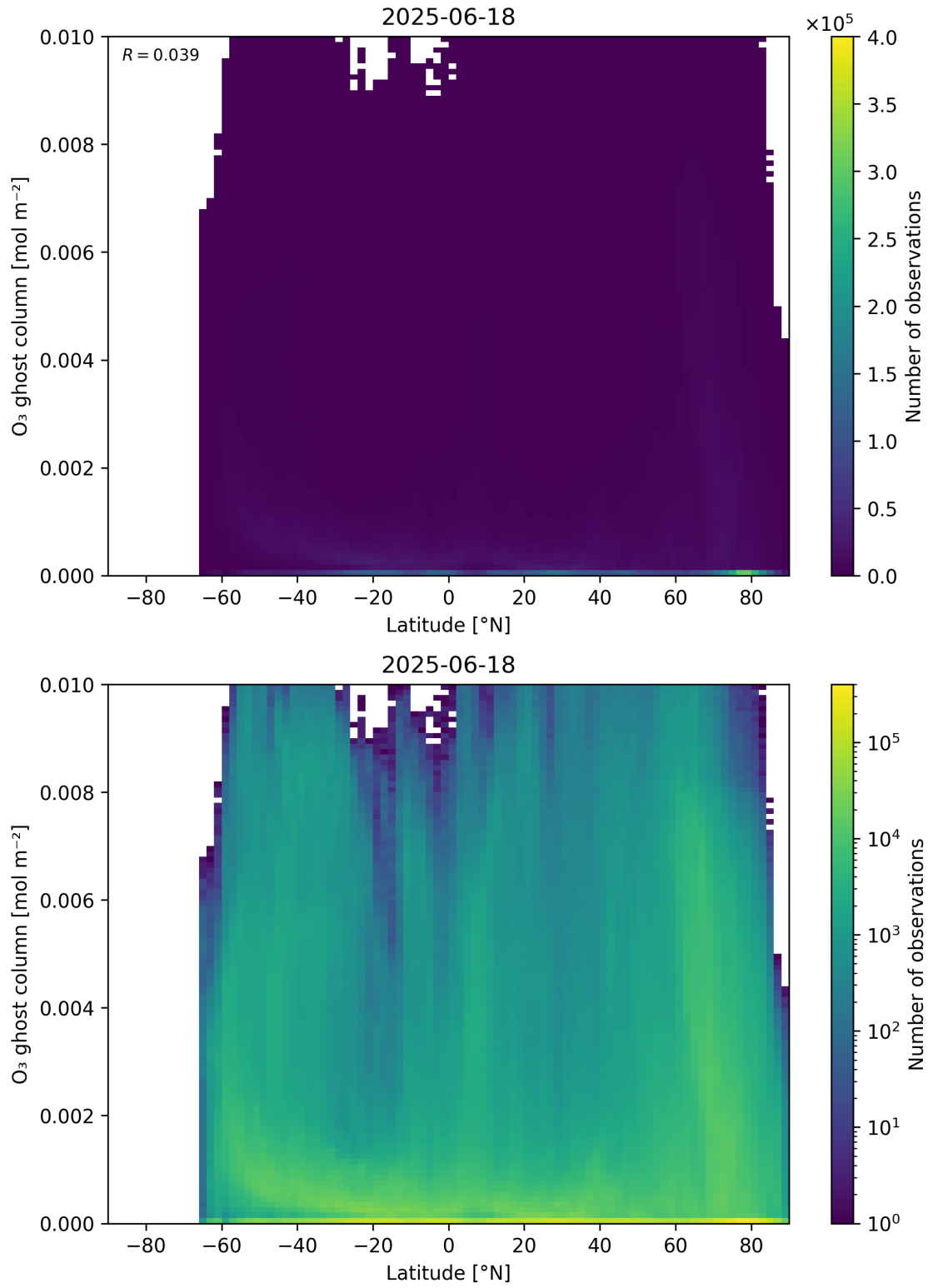
Figure 35: Scatter density plot of “Latitude” against “O 3 ghost column” for 2025-06-17 to 2025-06-19.
