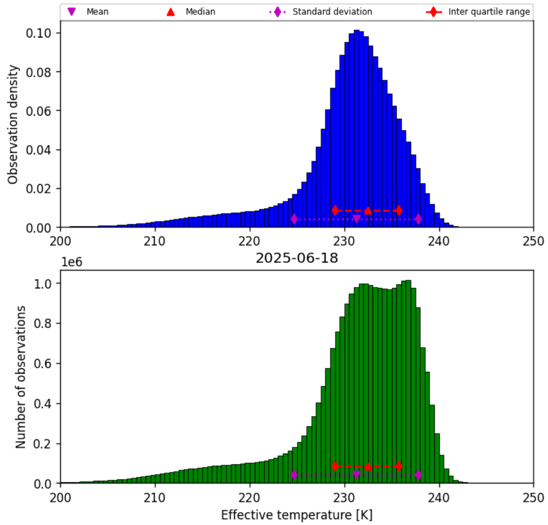
Figure 24: Histogram of “Effective temperature” for 2025-06-17 to 2025-06-19
