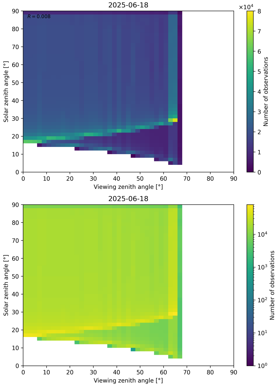
Figure 54: Scatter density plot of “Viewing zenith angle” against “Solar zenith angle” for 2025-06-17 to 2025-06-19.
