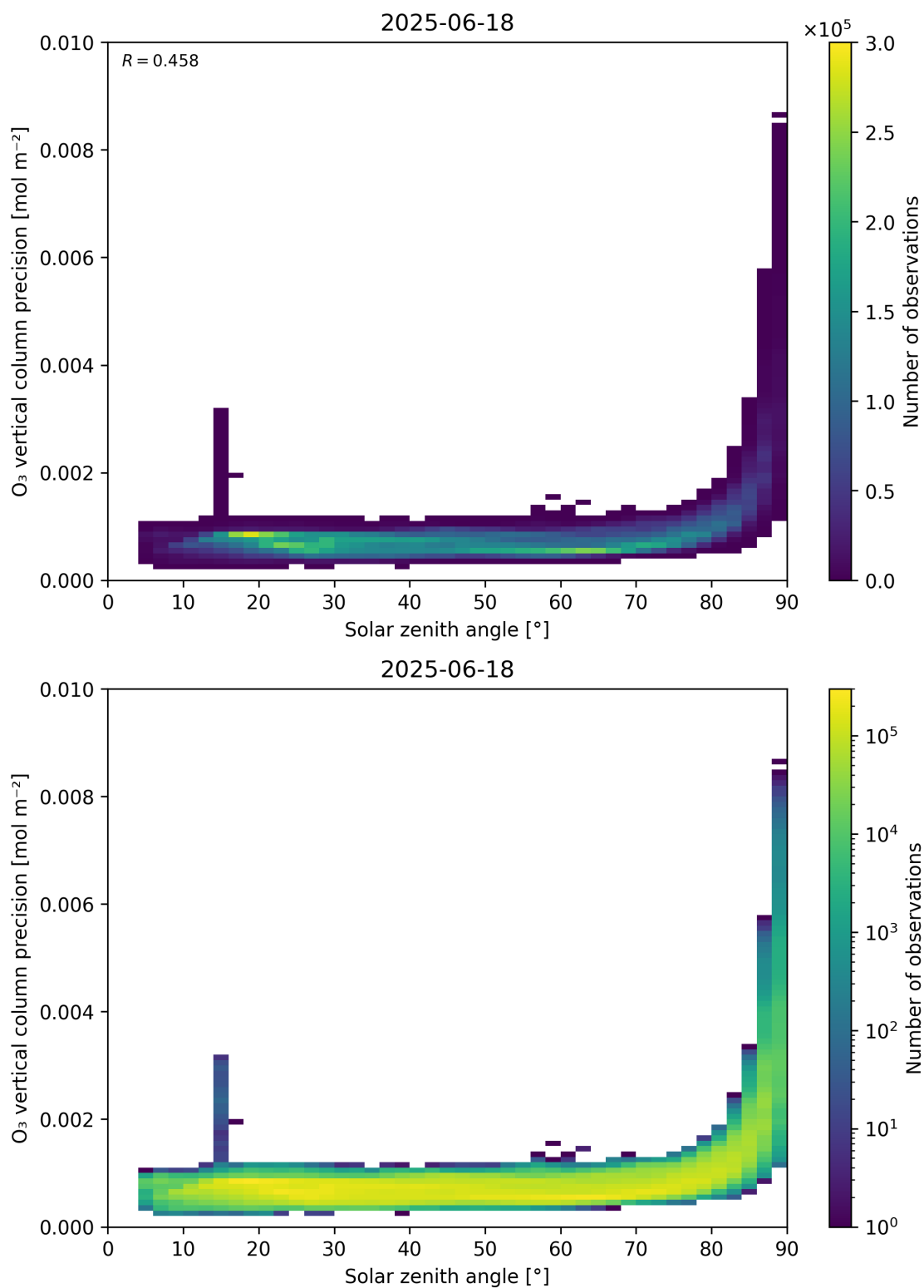
Figure 48: Scatter density plot of “Solar zenith angle” against “O 3 vertical column precision” for 2025-06-17 to 2025-06-19.
