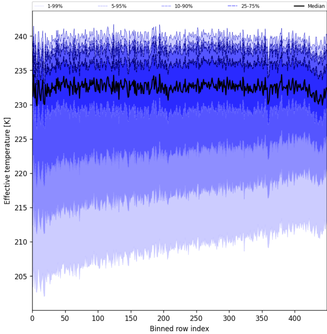
Figure 31: Along track statistics of “Effective temperature” for 2025-06-17 to 2025-06-19
