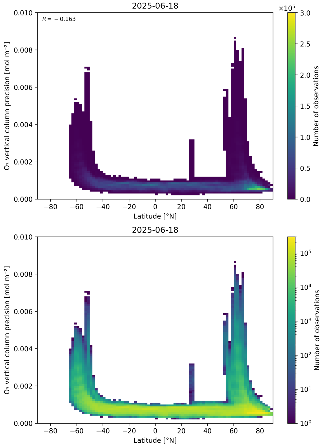
Figure 37: Scatter density plot of “Latitude” against “O 3 vertical column precision” for 2025-06-17 to 2025-06-19.
