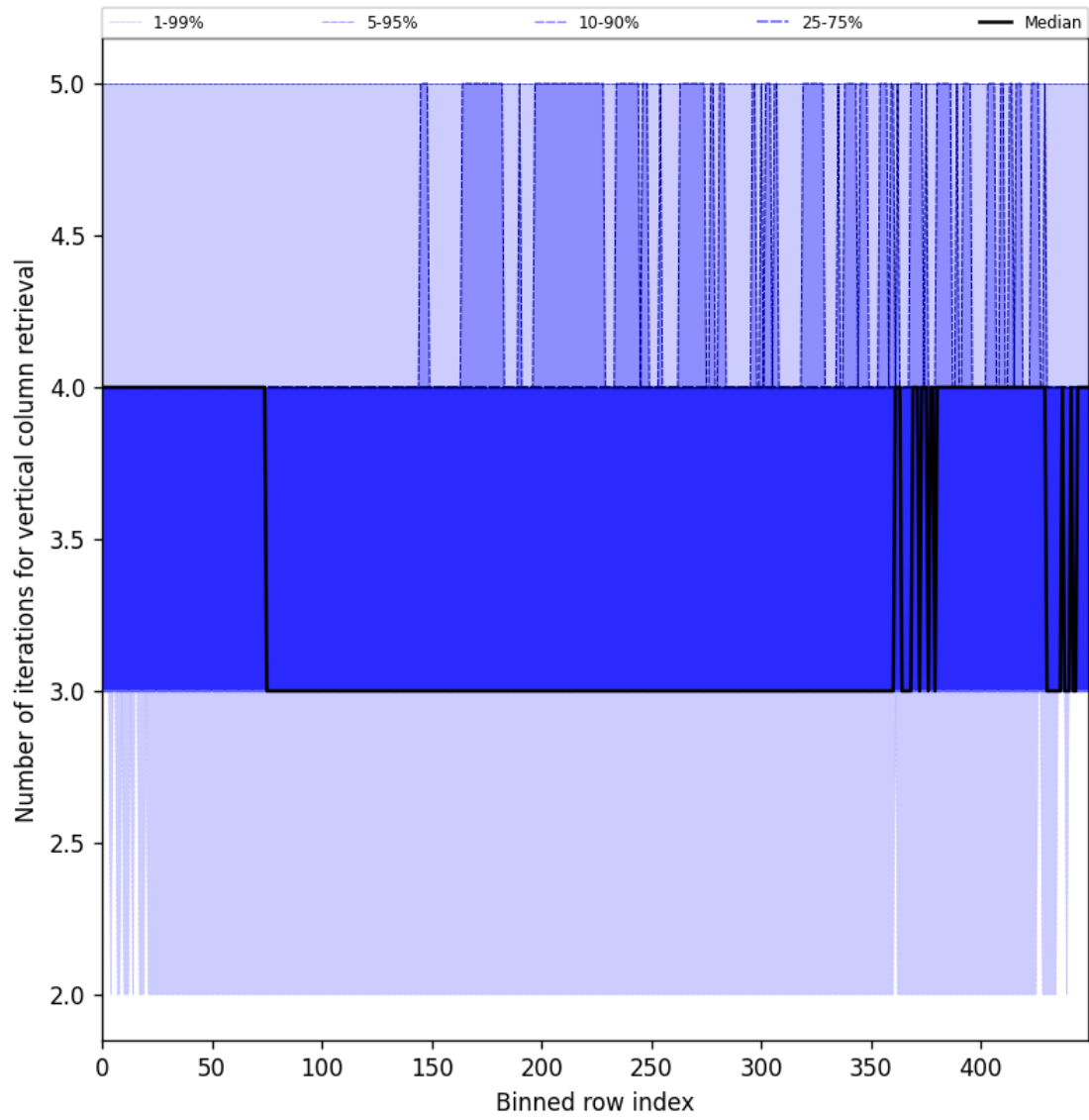
Figure 33: Along track statistics of “Number of iterations for vertical column retrieval” for 2025-06-17 to 2025-06-19
