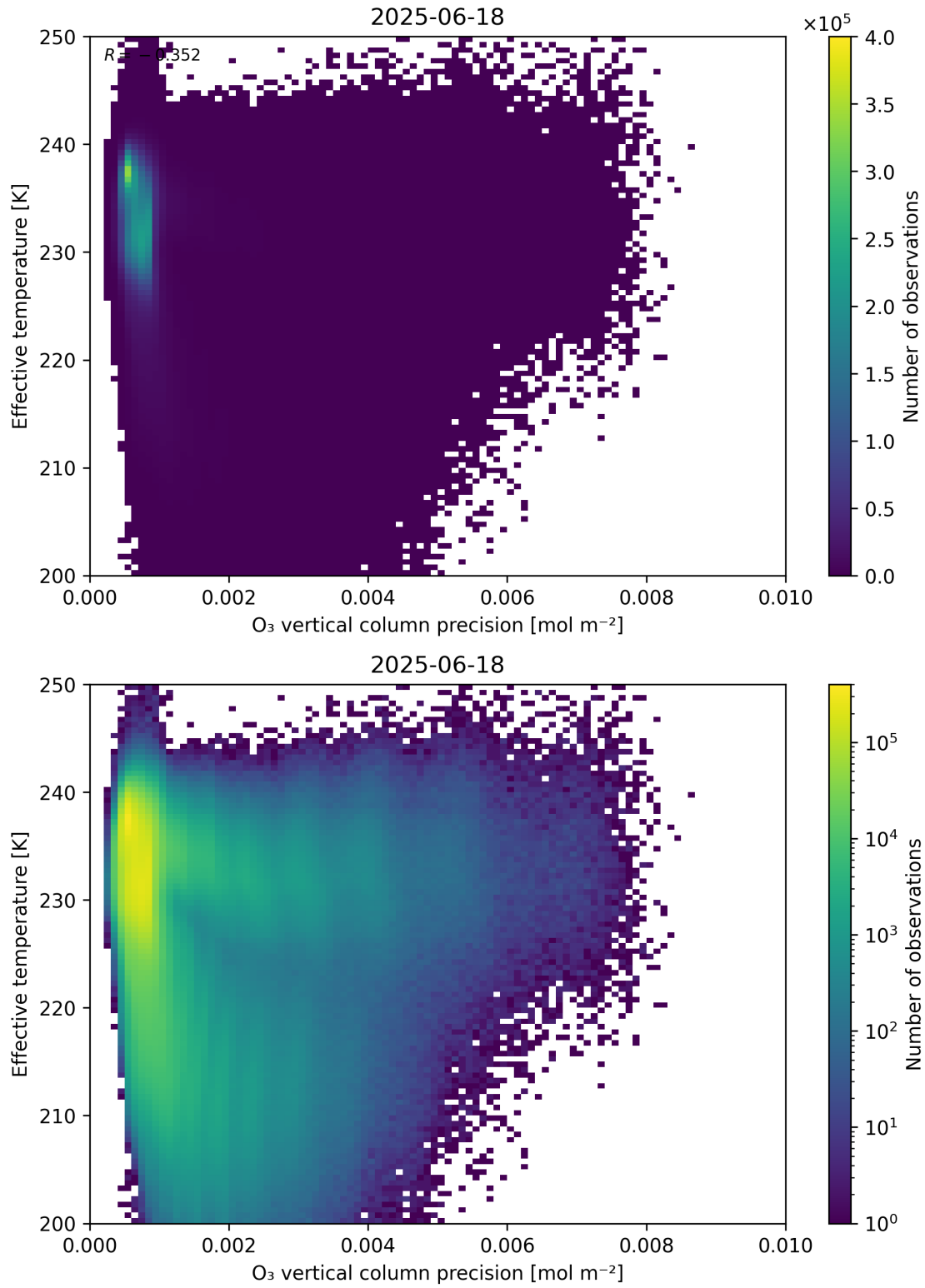
Figure 42: Scatter density plot of “O 3 vertical column precision” against “Effective temperature” for 2025-06-17 to 2025-06-19.
