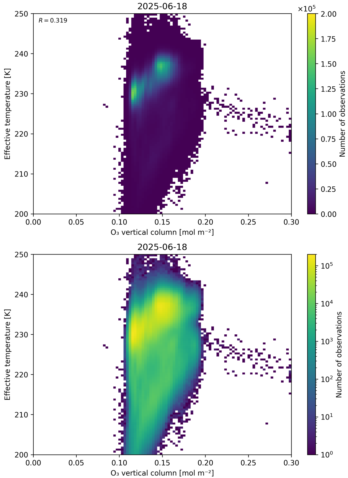
Figure 39: Scatter density plot of “O 3 vertical column” against “Effective temperature” for 2025-06-17 to 2025-06-19.
