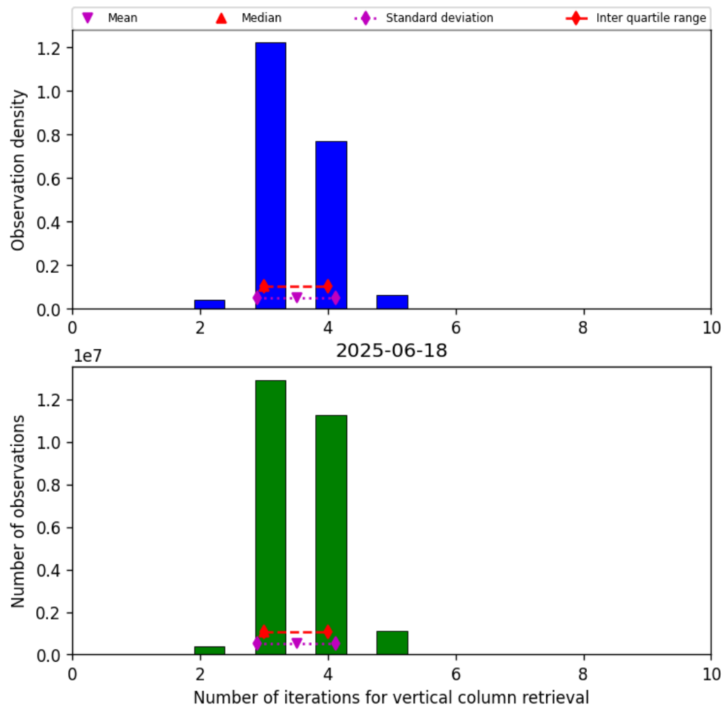
Figure 26: Histogram of “Number of iterations for vertical column retrieval” for 2025-06-17 to 2025-06-19
