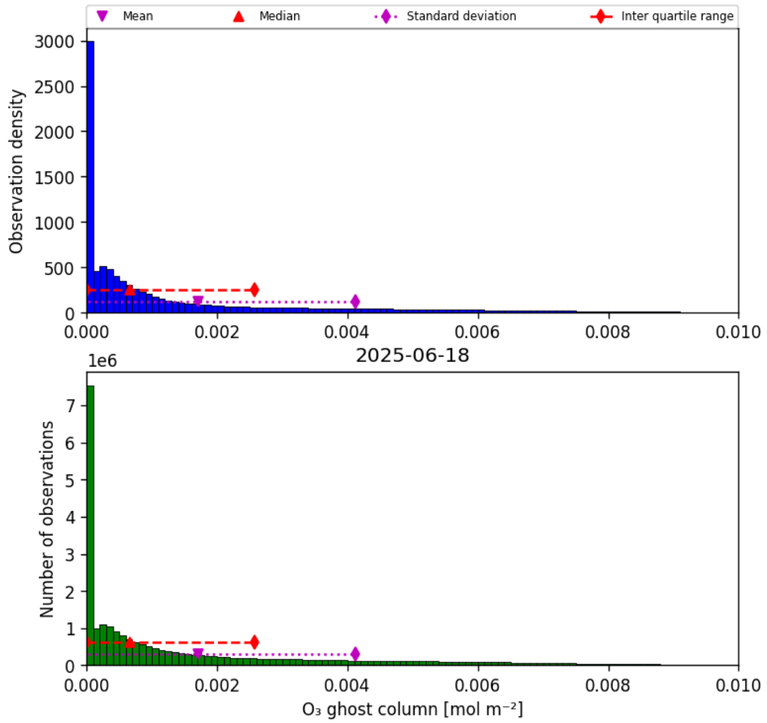
Figure 25: Histogram of “O 3 ghost column” for 2025-06-17 to 2025-06-19
