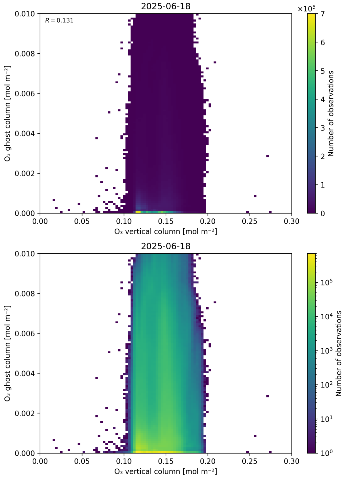
Figure 40: Scatter density plot of “O 3 vertical column” against “O 3 ghost column” for 2025-06-17 to 2025-06-19.
