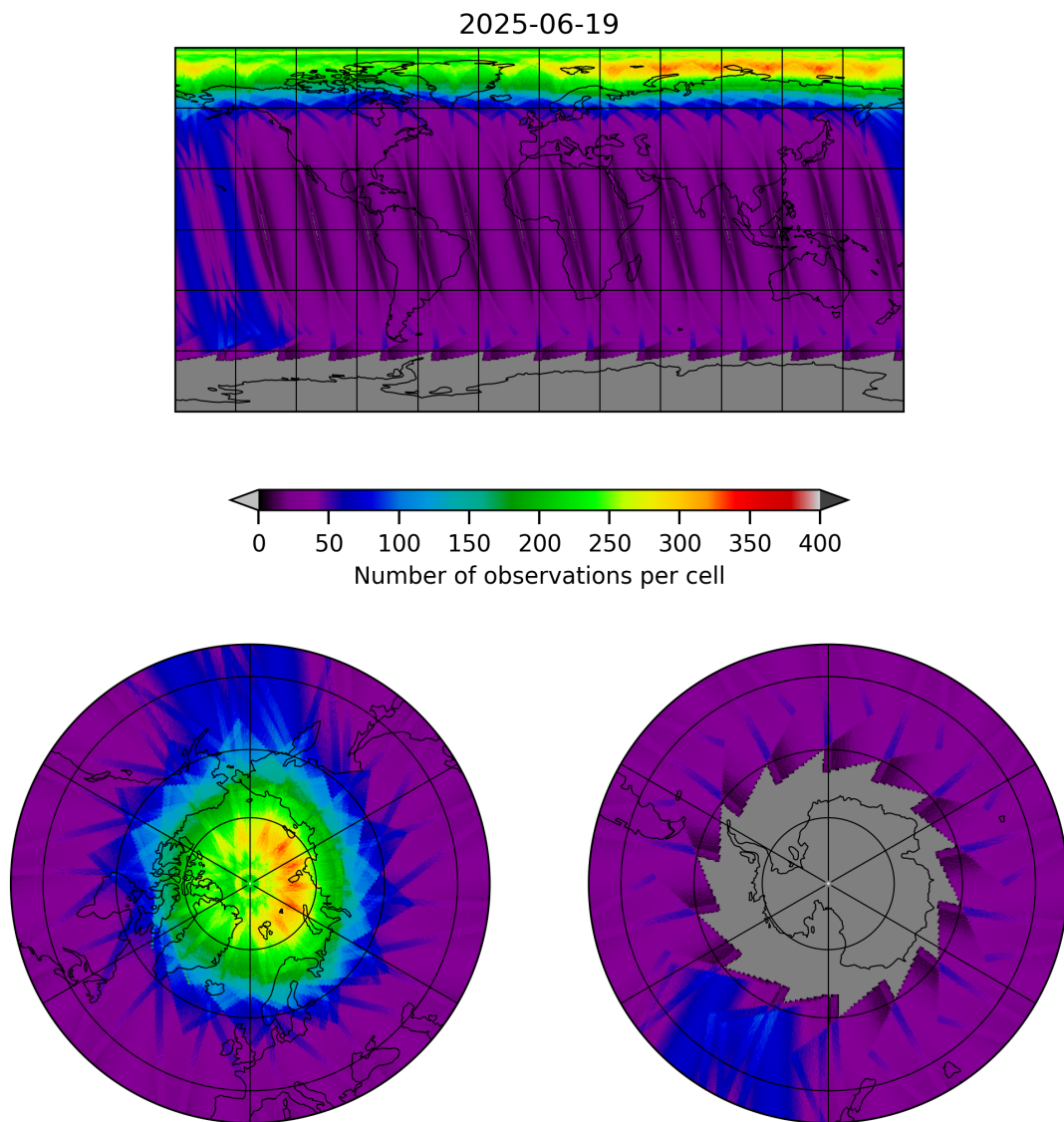
Figure 12: Map of the number of observations for 2025-06-18 to 2025-06-20
