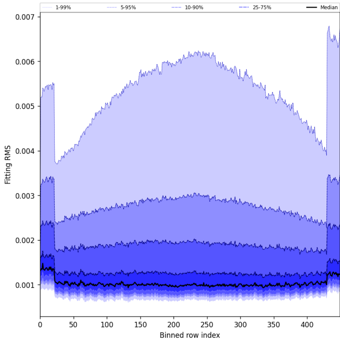
Figure 30: Along track statistics of “Fitting RMS” for 2025-06-18 to 2025-06-20
