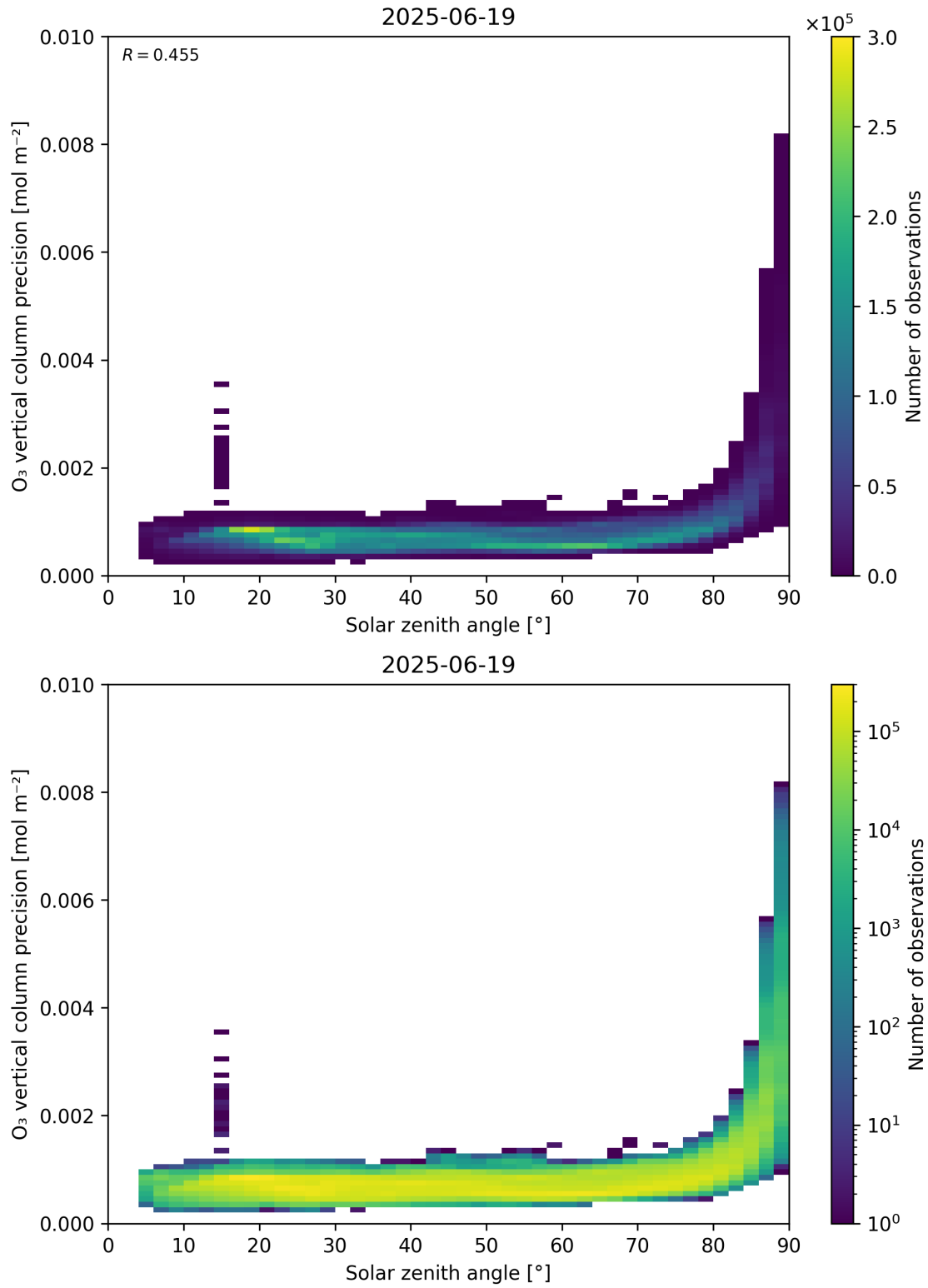
Figure 48: Scatter density plot of “Solar zenith angle” against “O 3 vertical column precision” for 2025-06-18 to 2025-06-20.
