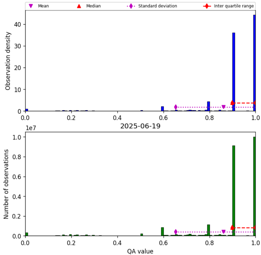
Figure 20: Histogram of “QA value” for 2025-06-18 to 2025-06-20
