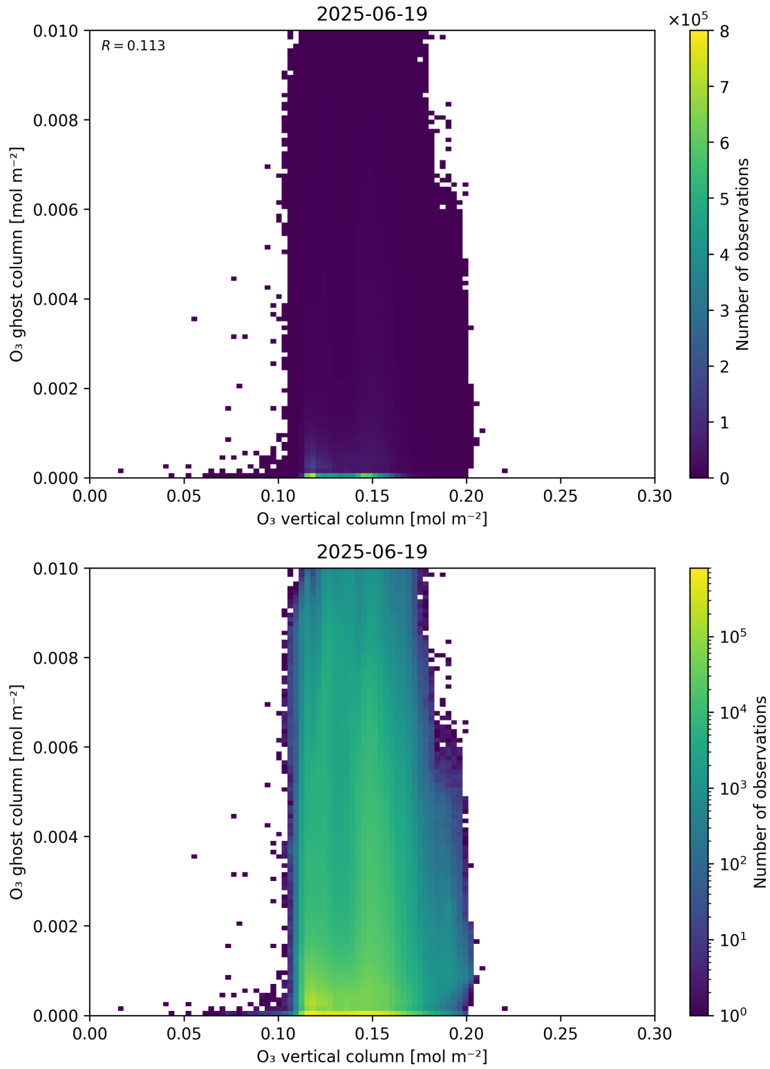
Figure 40: Scatter density plot of “O 3 vertical column” against “O 3 ghost column” for 2025-06-18 to 2025-06-20.
