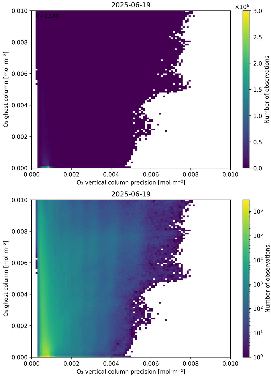
Figure 43: Scatter density plot of “ O_3 vertical column precision” against “ O_3 ghost column” for 2025-06-18 to 2025-06-20.
