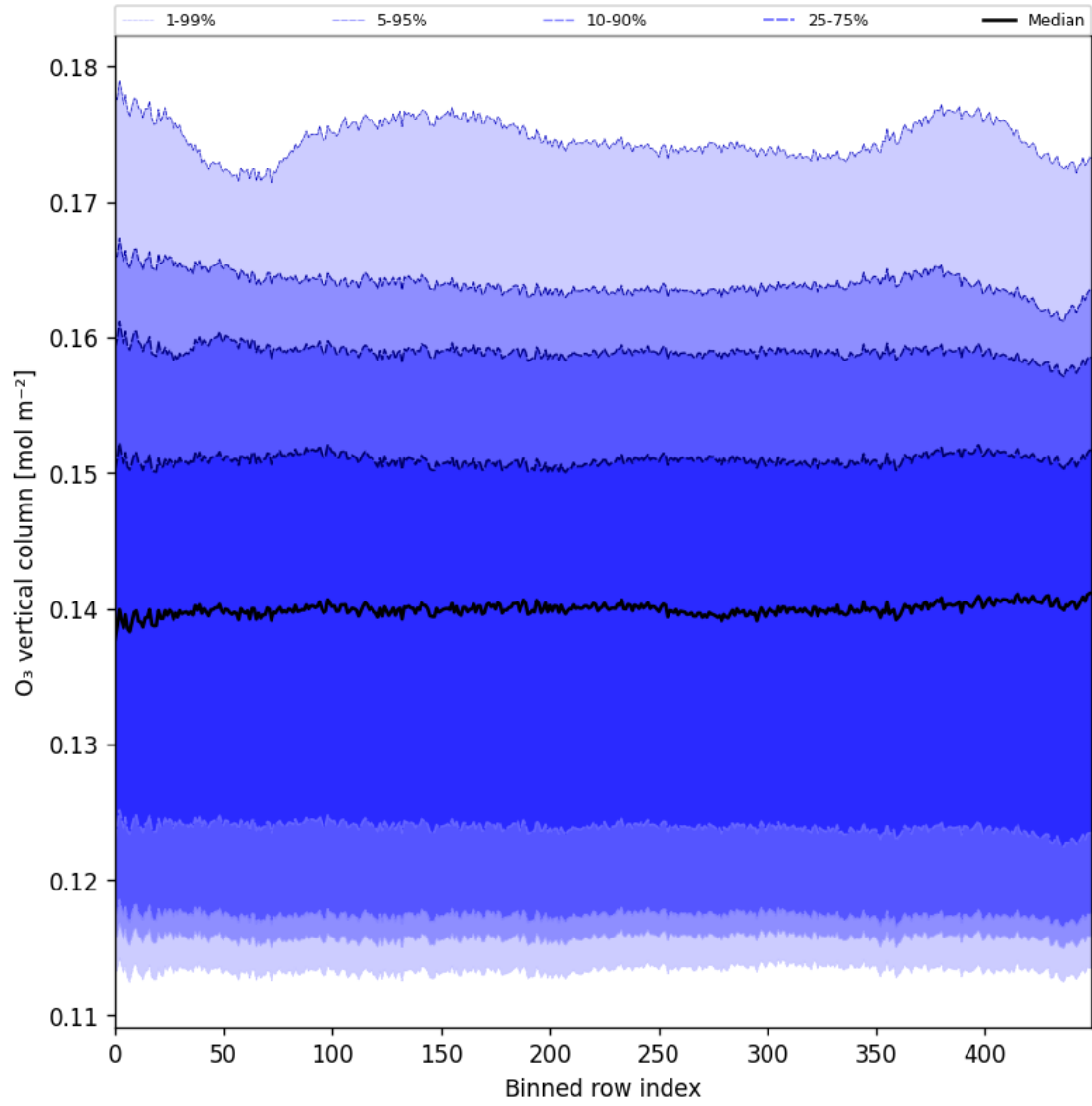
Figure 28: Along track statistics of “O 3 vertical column” for 2025-06-18 to 2025-06-20
