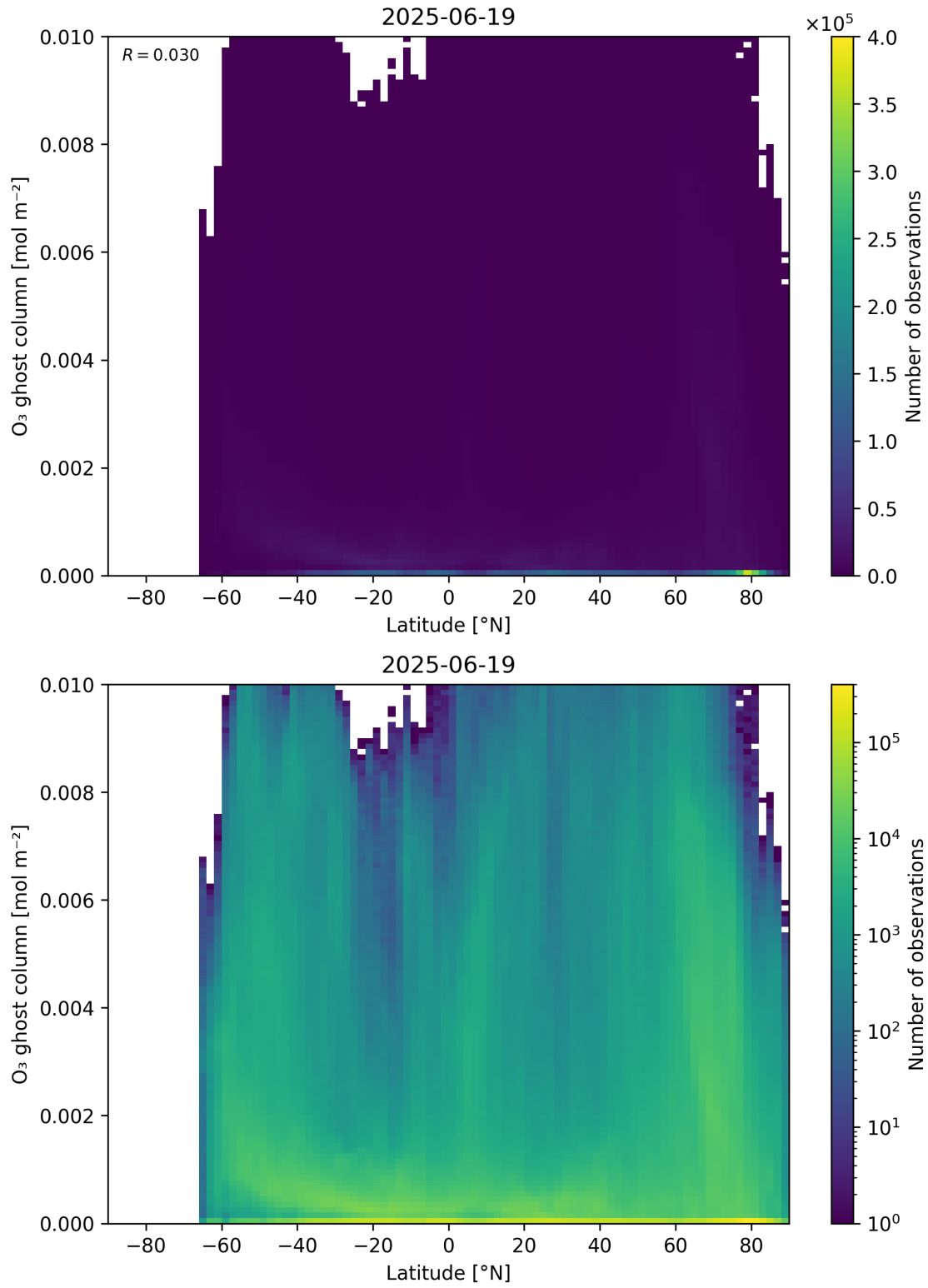
Figure 35: Scatter density plot of “Latitude” against “O 3 ghost column” for 2025-06-18 to 2025-06-20.
