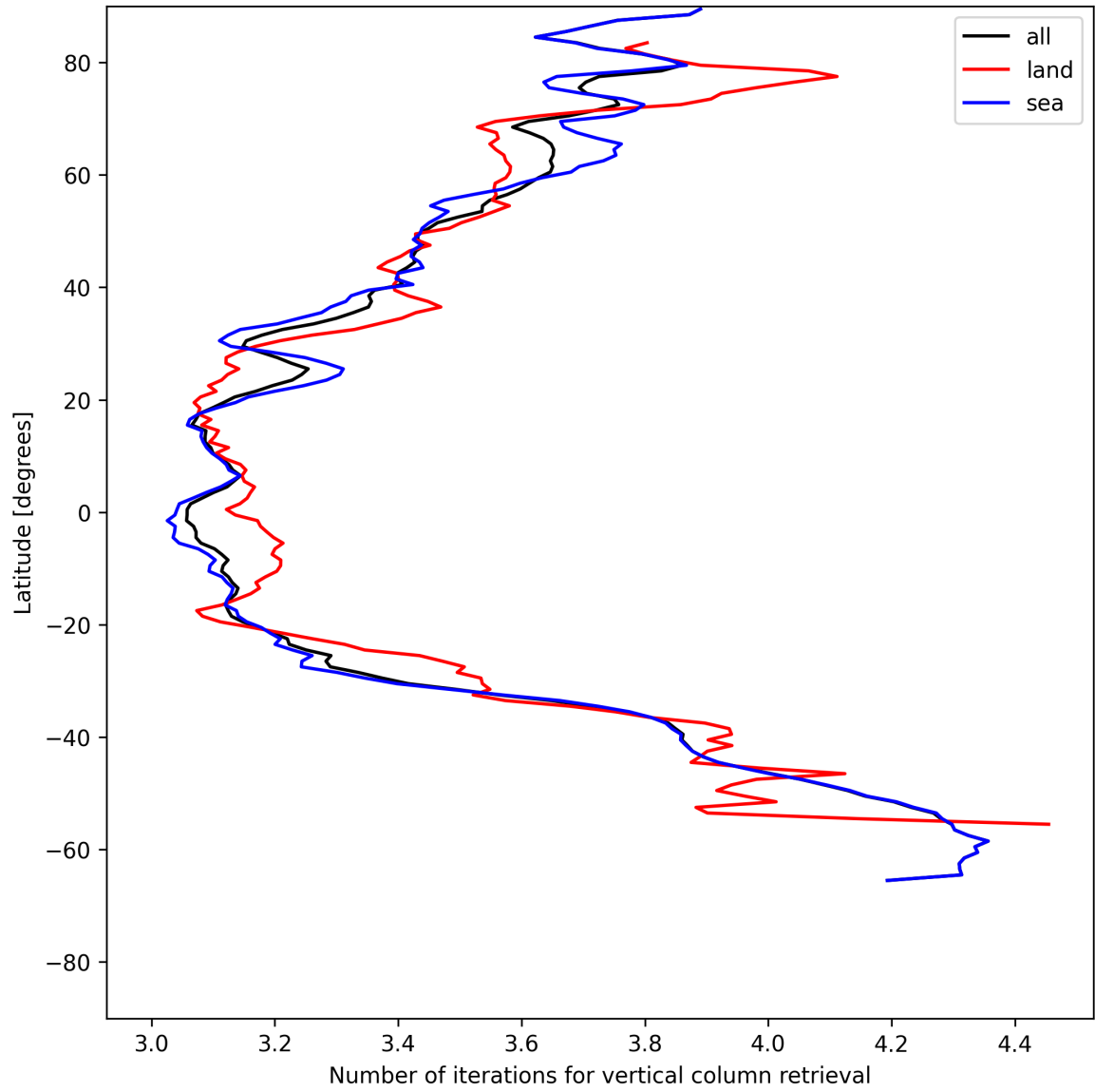
Figure 19: Zonal average of “Number of iterations for vertical column retrieval” for 2025-06-18 to 2025-06-20.
