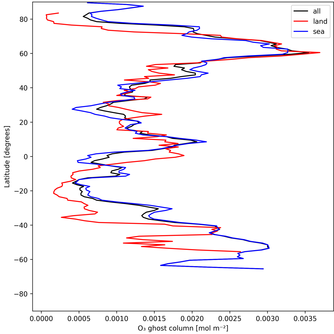
Figure 18: Zonal average of “O 3 ghost column” for 2025-06-18 to 2025-06-20.
