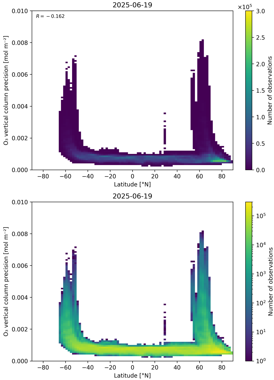
Figure 37: Scatter density plot of “Latitude” against “O 3 vertical column precision” for 2025-06-18 to 2025-06-20.
