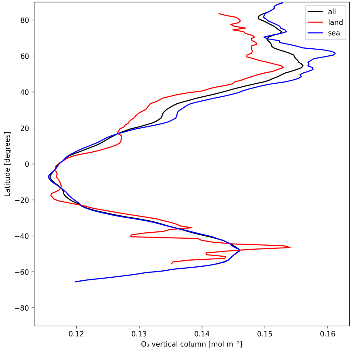
Figure 14: Zonal average of “O 3 vertical column” for 2025-06-18 to 2025-06-20.
