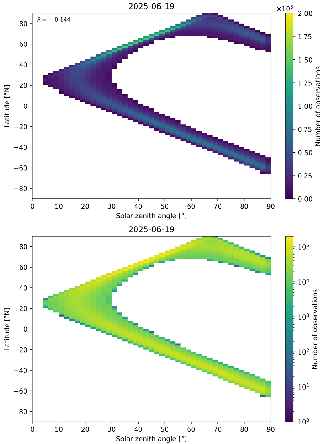
Figure 44: Scatter density plot of “Solar zenith angle” against “Latitude” for 2025-06-18 to 2025-06-20.
