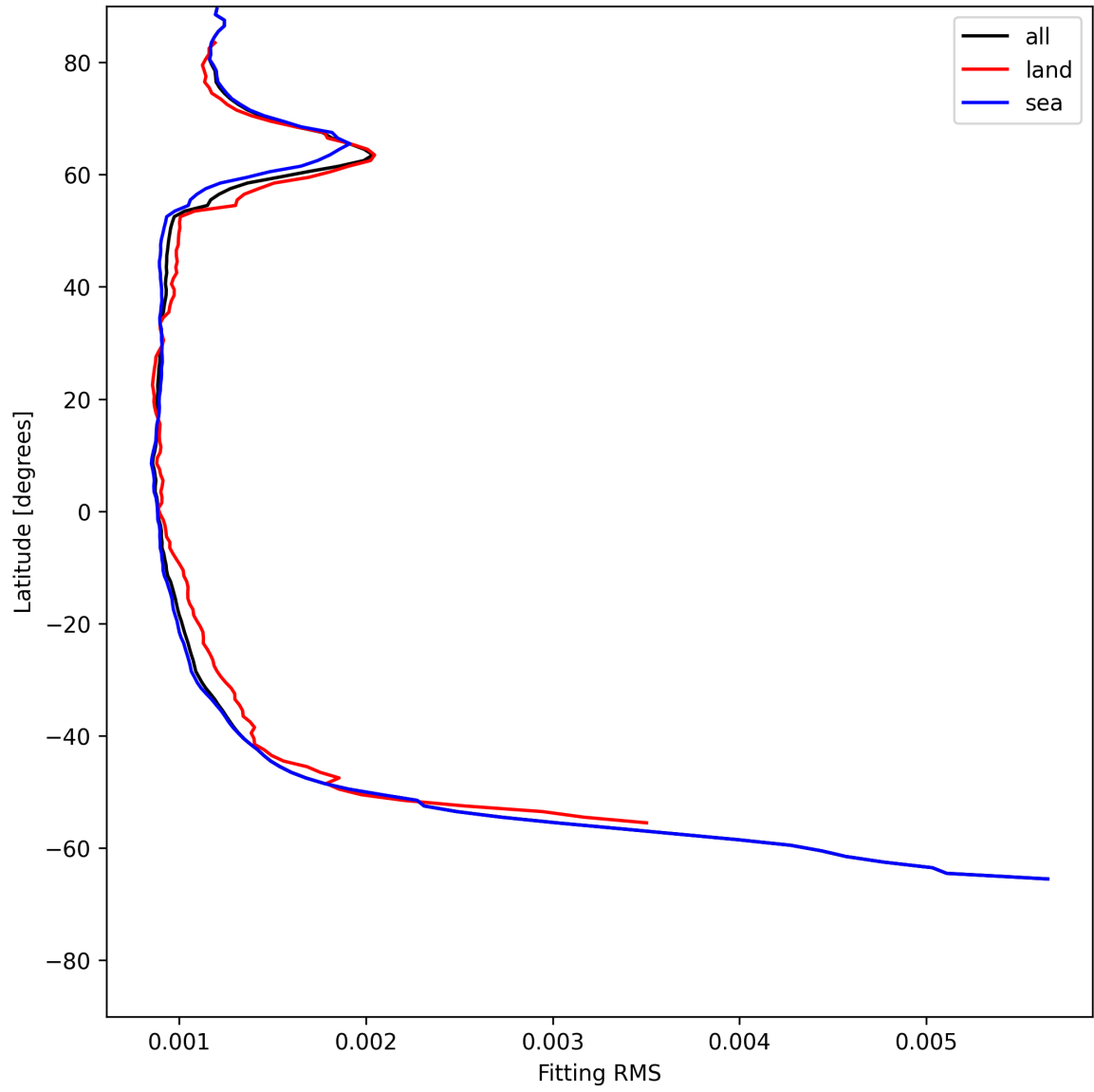
Figure 16: Zonal average of “Fitting RMS” for 2025-06-18 to 2025-06-20.
