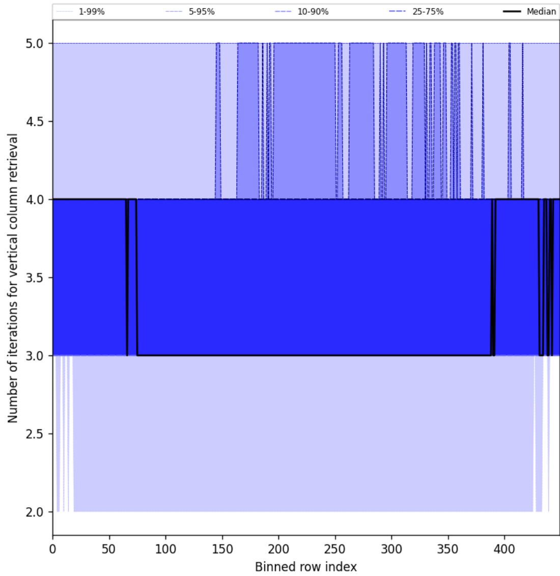
Figure 33: Along track statistics of “Number of iterations for vertical column retrieval” for 2025-06-18 to 2025-06-20
