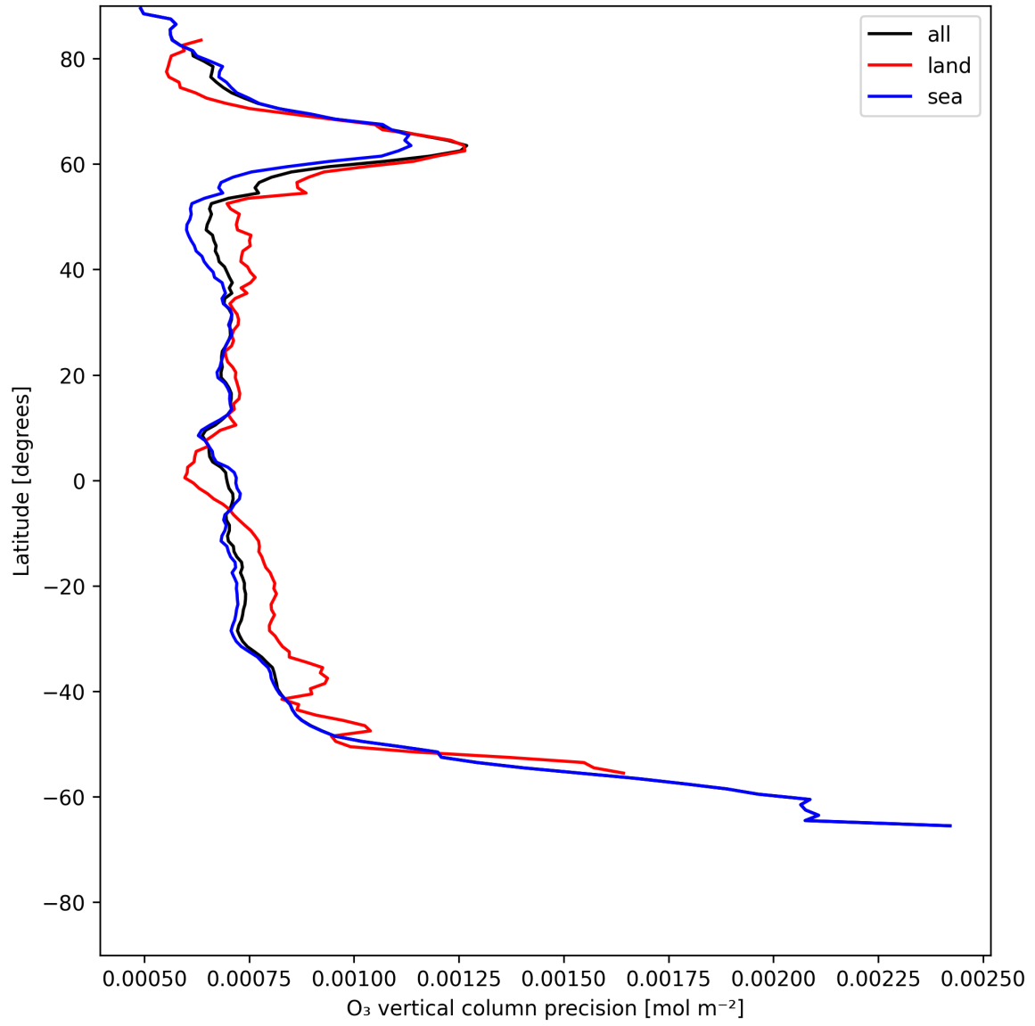
Figure 15: Zonal average of “O 3 vertical column precision” for 2025-06-18 to 2025-06-20.
