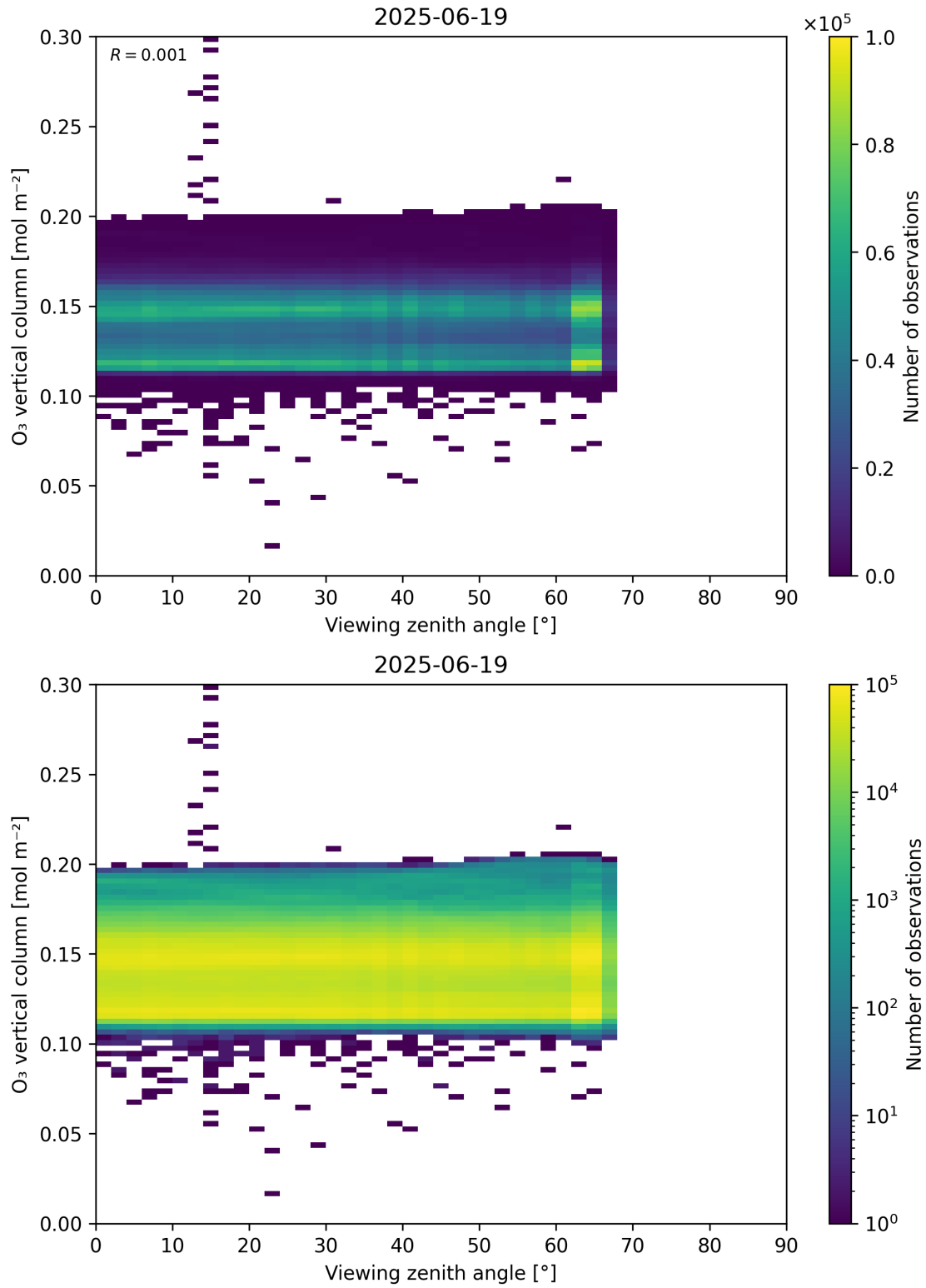
Figure 52: Scatter density plot of “Viewing zenith angle” against “O 3 vertical column” for 2025-06-18 to 2025-06-20.
