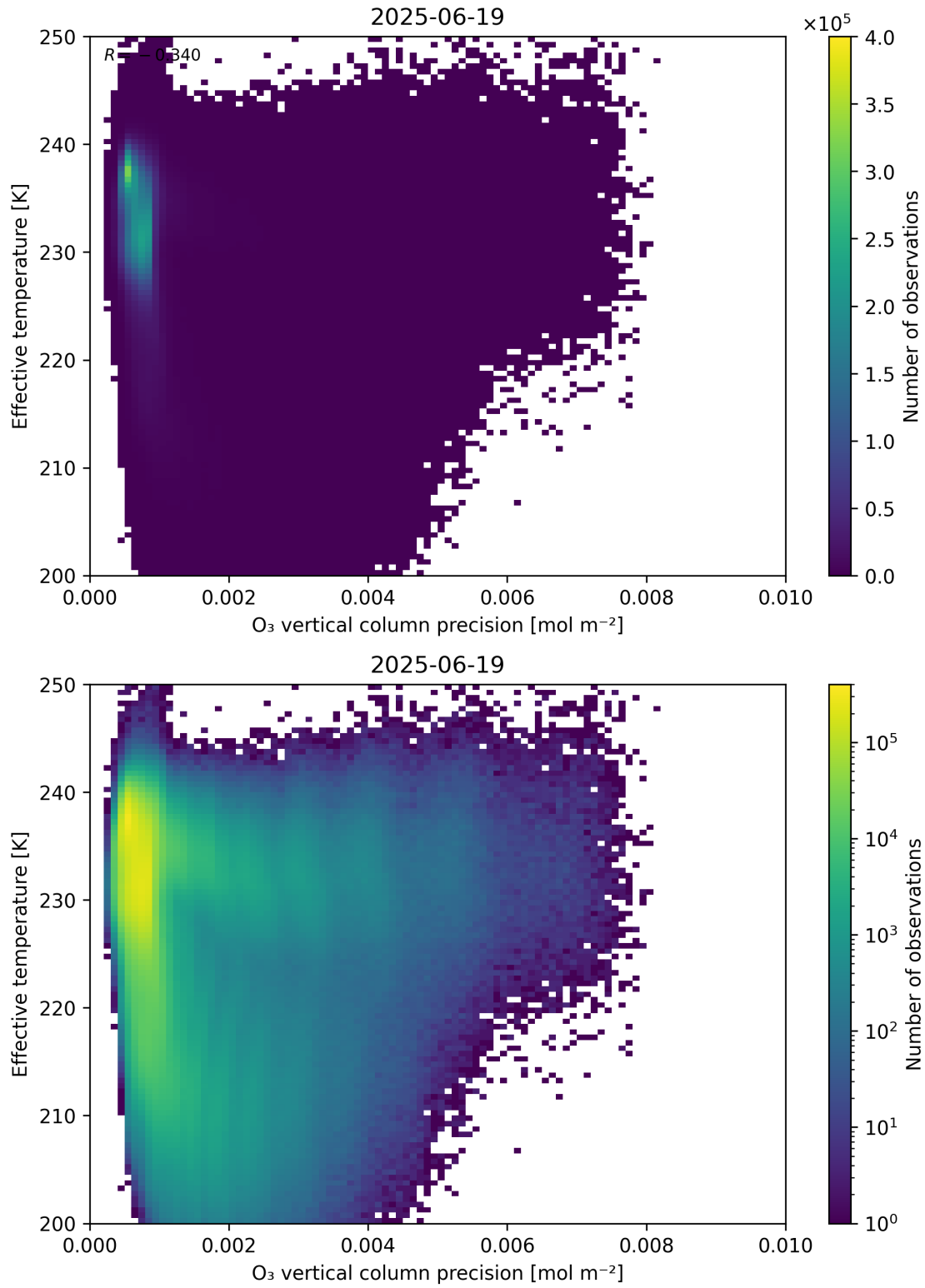
Figure 42: Scatter density plot of “O 3 vertical column precision” against “Effective temperature” for 2025-06-18 to 2025-06-20.
