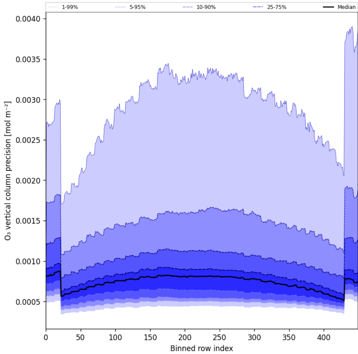
Figure 29: Along track statistics of “O 3 vertical column precision” for 2025-06-18 to 2025-06-20
