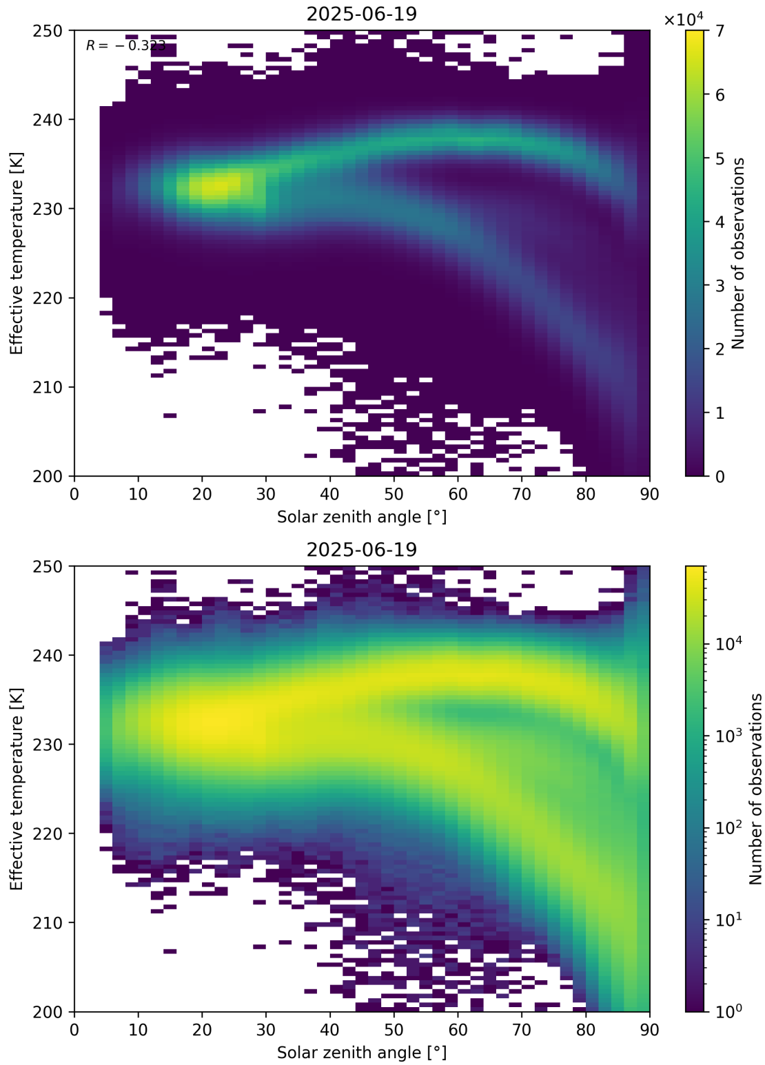
Figure 45: Scatter density plot of “Solar zenith angle” against “Effective temperature” for 2025-06-18 to 2025-06-20.
