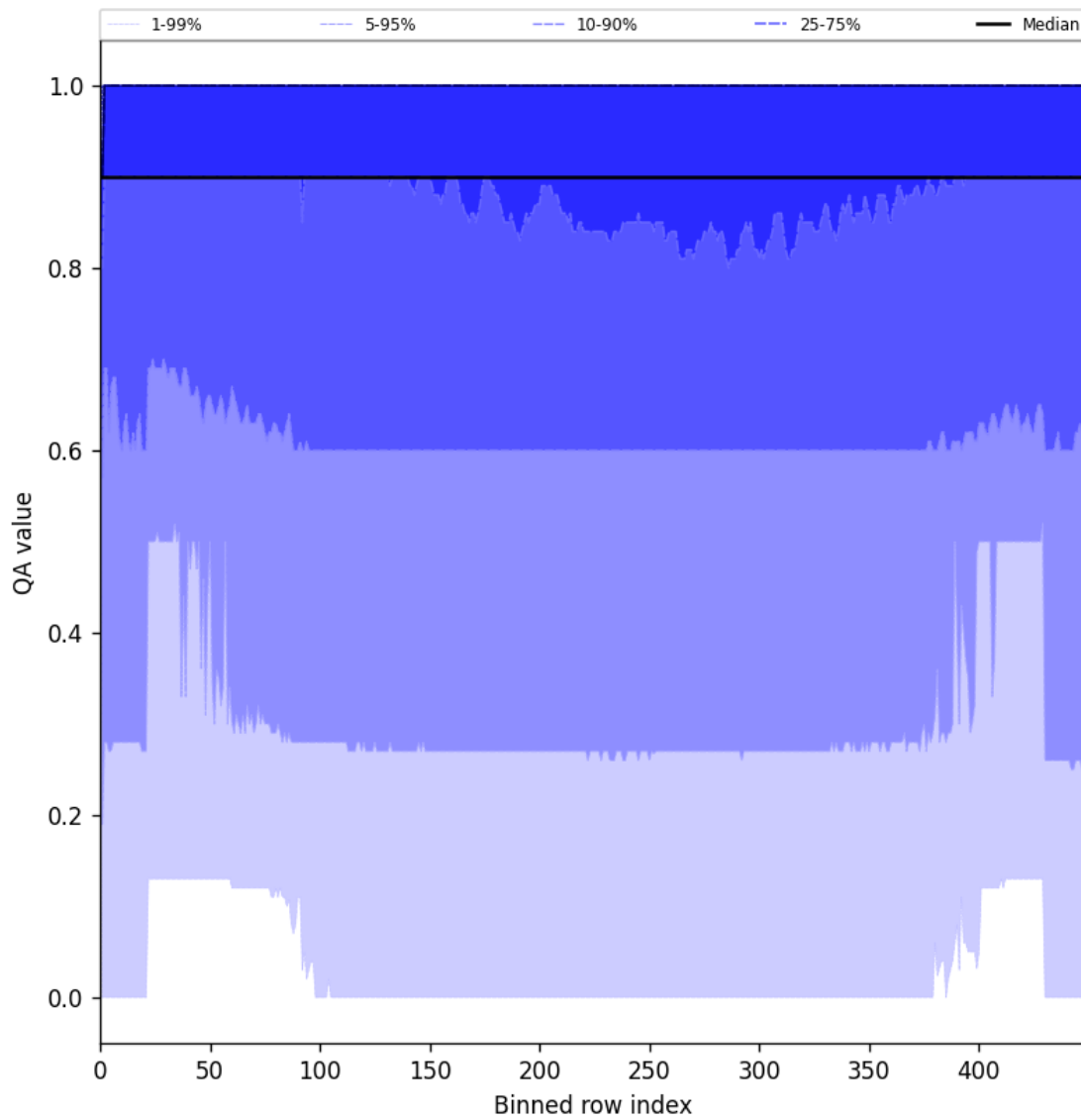
Figure 27: Along track statistics of “QA value” for 2025-06-18 to 2025-06-20
