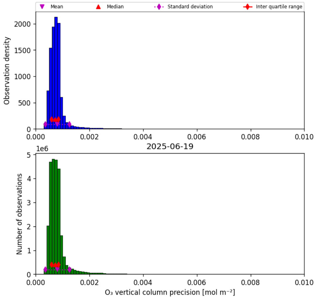
Figure 22: Histogram of “O 3 vertical column precision” for 2025-06-18 to 2025-06-20
