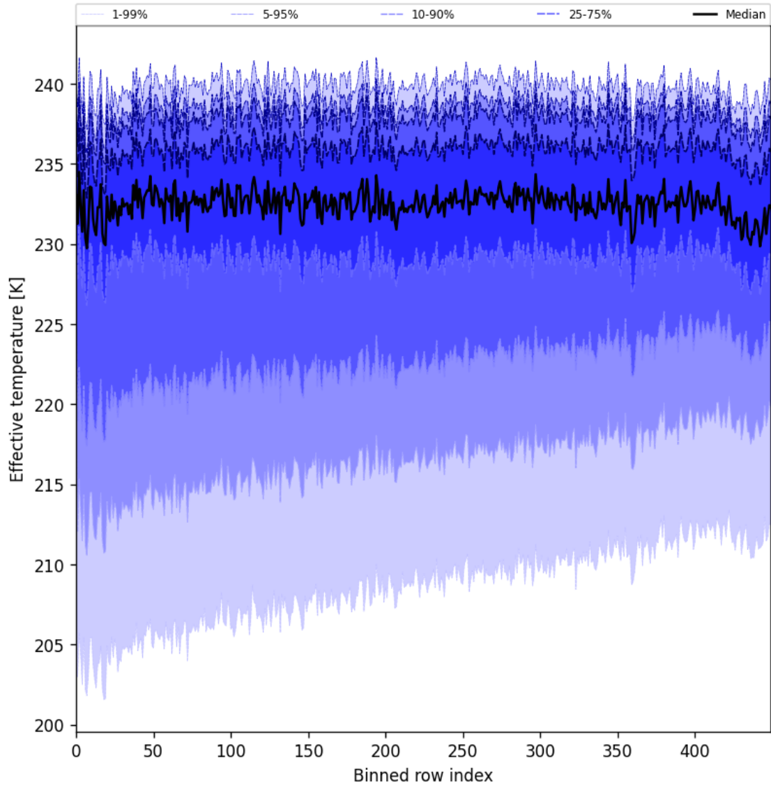
Figure 31: Along track statistics of “Effective temperature” for 2025-06-18 to 2025-06-20
