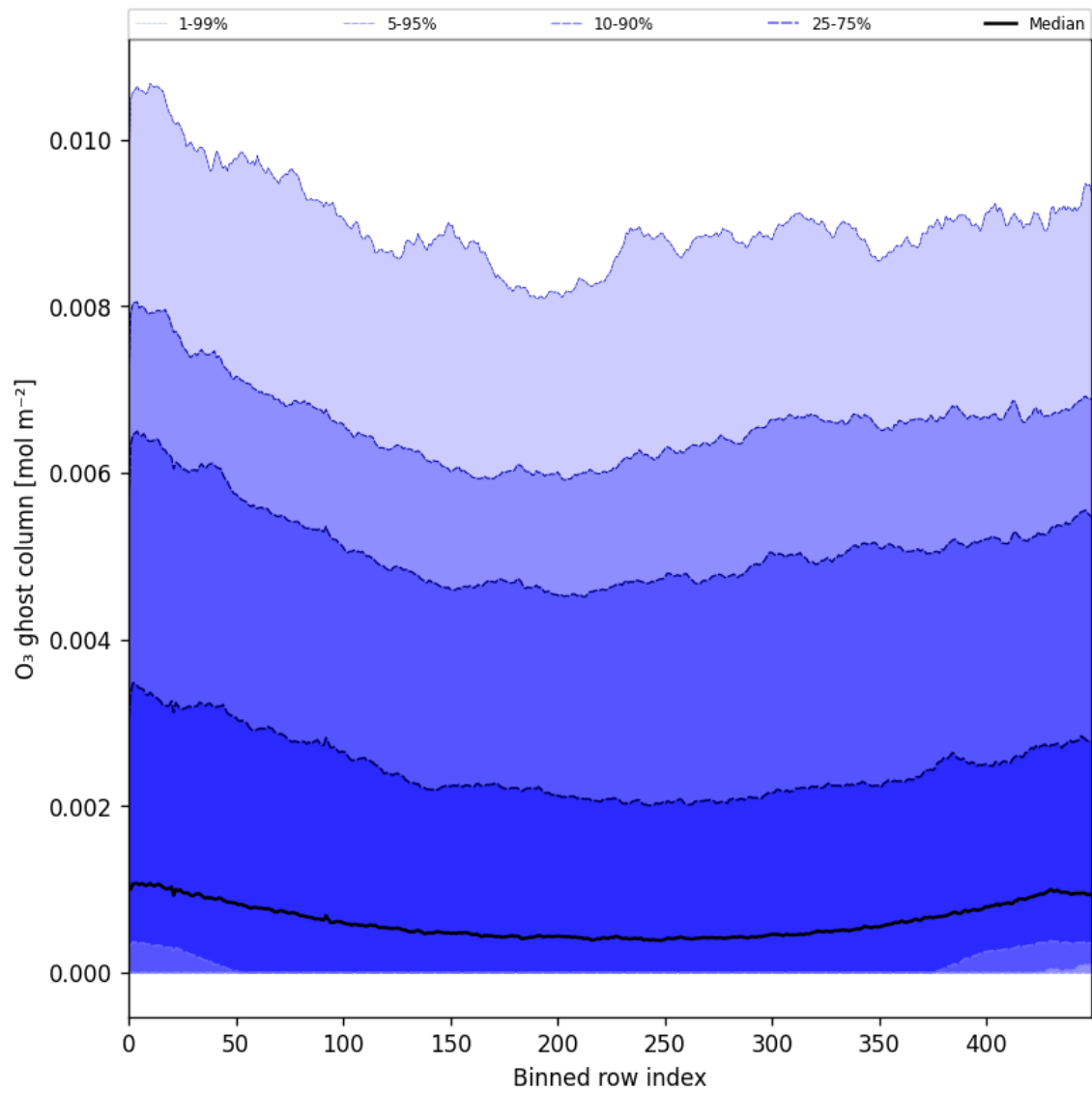
Figure 32: Along track statistics of “O 3 ghost column” for 2025-06-18 to 2025-06-20
