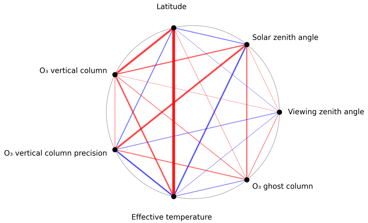
Figure 1: Map of correlation graph for 2025-06-18 to 2025-06-20.
