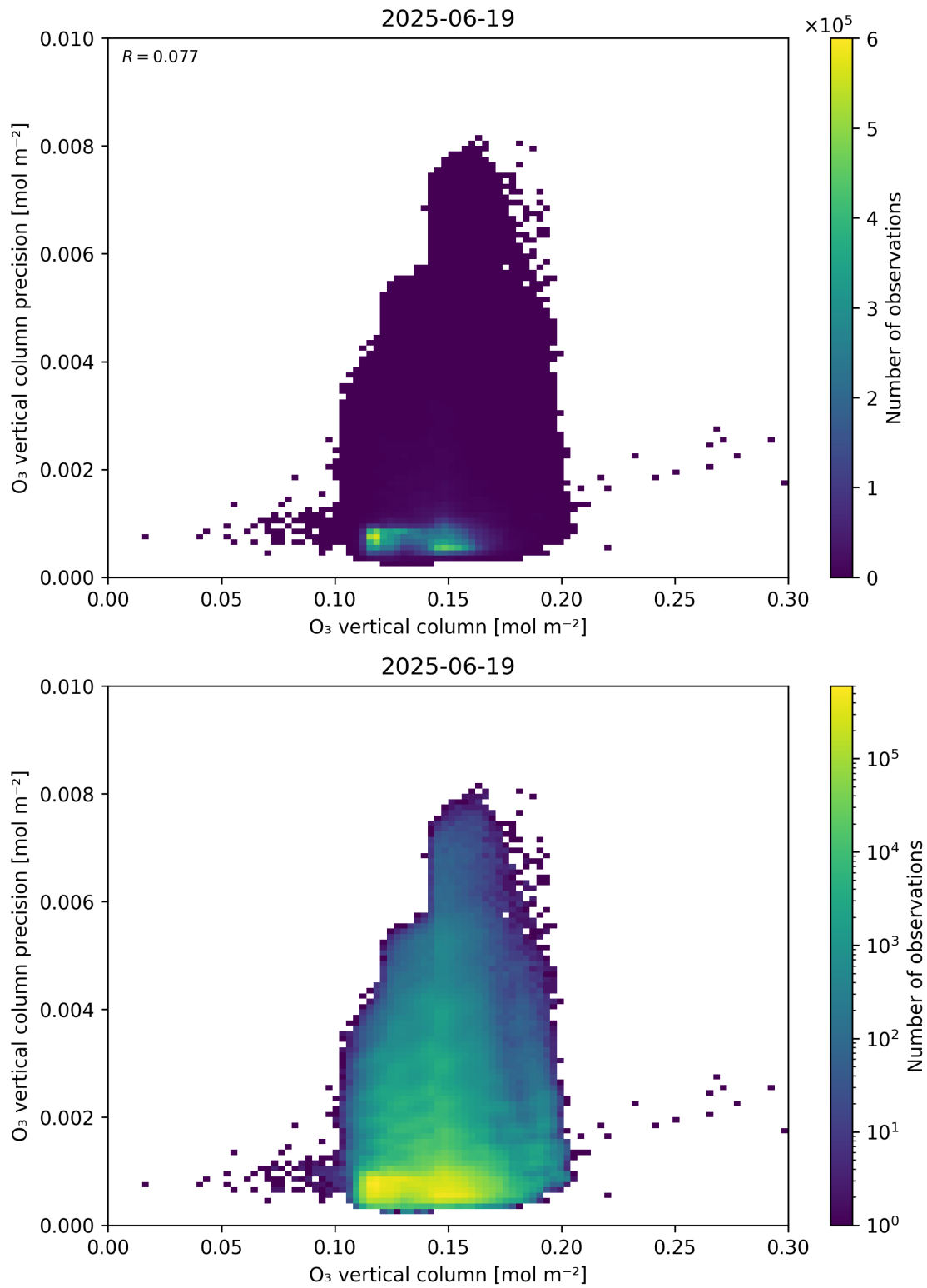
Figure 41: Scatter density plot of “O 3 vertical column” against “O 3 vertical column precision” for 2025-06-18 to 2025-06-20.
