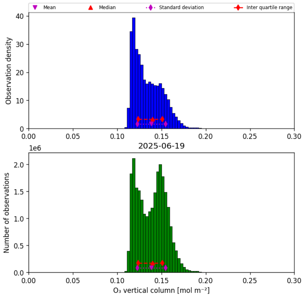
Figure 21: Histogram of “O 3 vertical column” for 2025-06-18 to 2025-06-20
