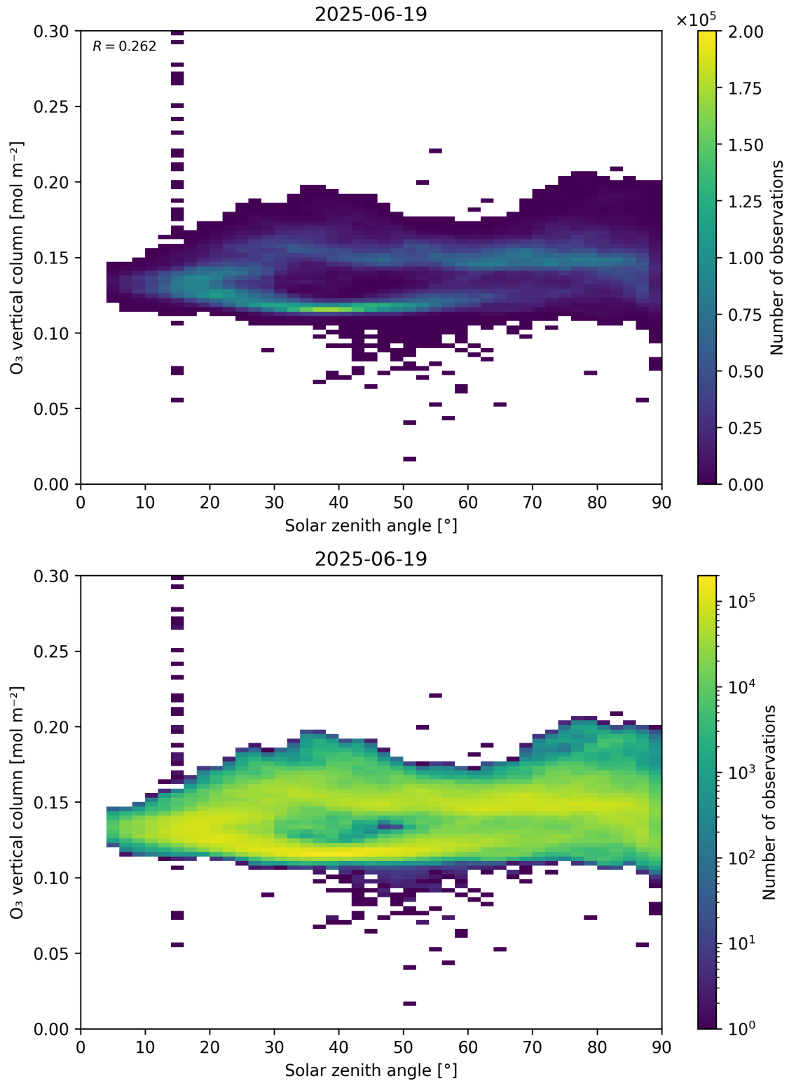
Figure 47: Scatter density plot of “Solar zenith angle” against “O 3 vertical column” for 2025-06-18 to 2025-06-20.
