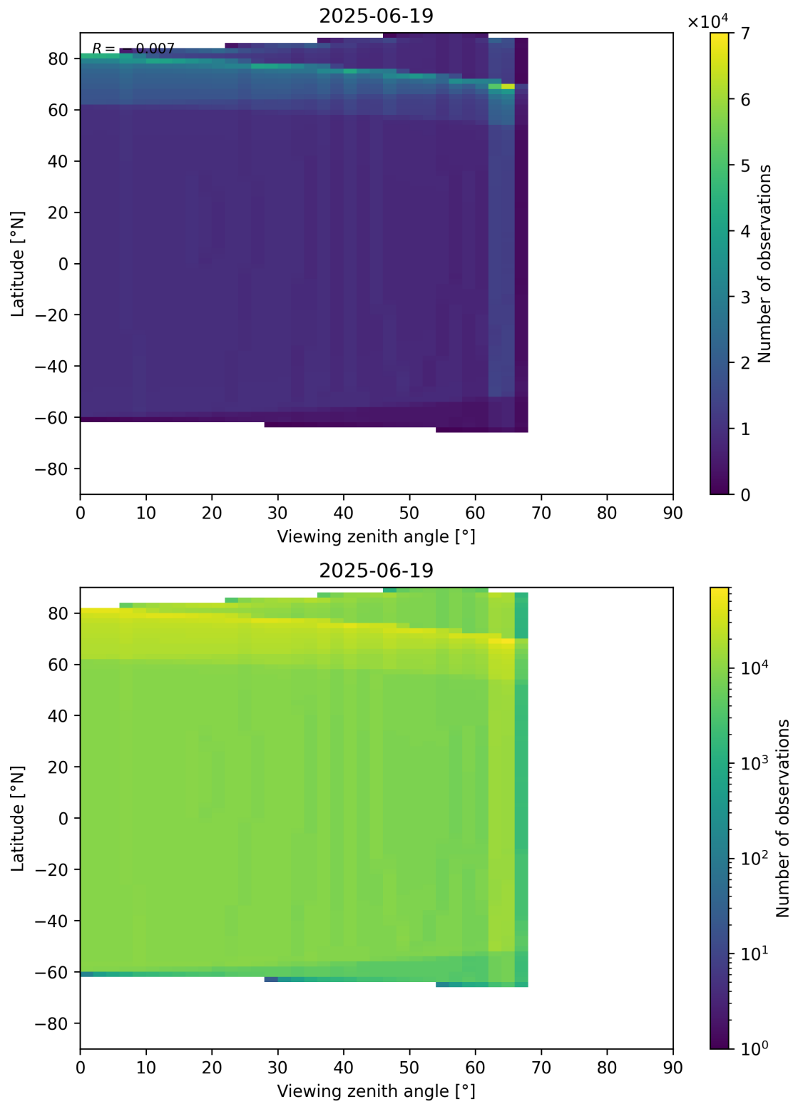
Figure 49: Scatter density plot of “Viewing zenith angle” against “Latitude” for 2025-06-18 to 2025-06-20.
