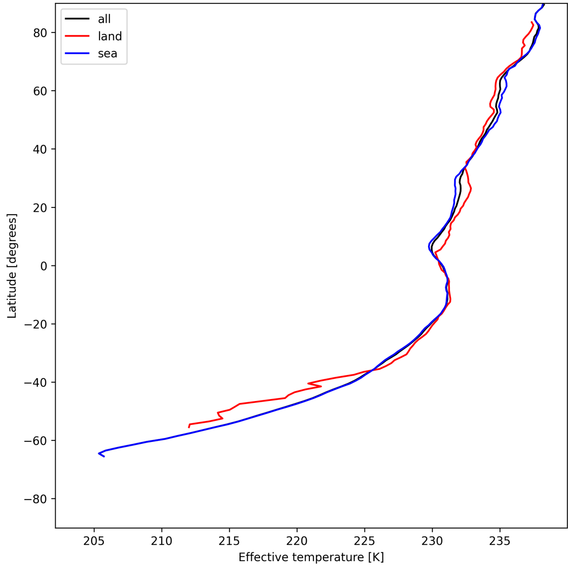
Figure 17: Zonal average of "Effective temperature" for 2025-06-18 to 2025-06-20.
