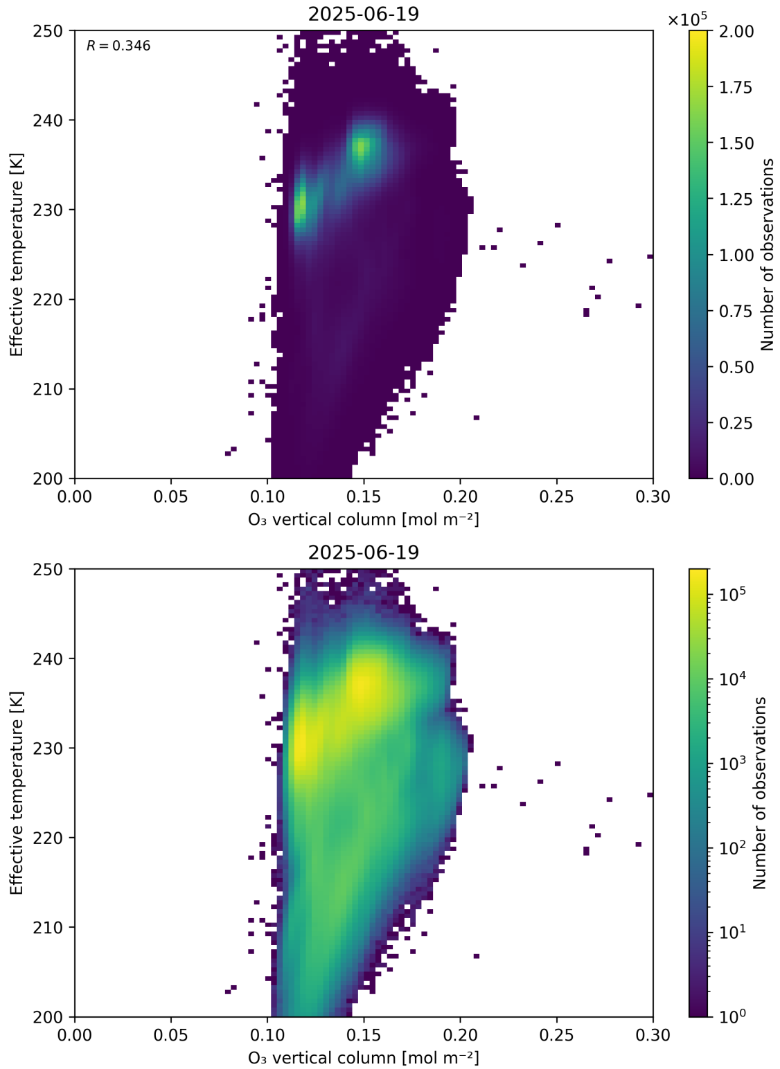
Figure 39: Scatter density plot of “O 3 vertical column” against “Effective temperature” for 2025-06-18 to 2025-06-20.
