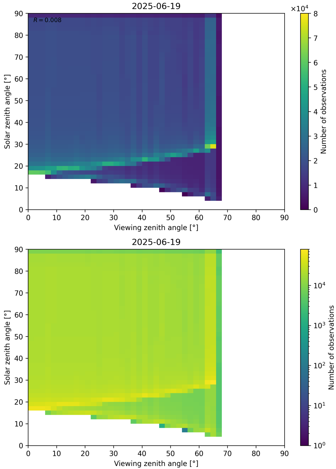
Figure 54: Scatter density plot of “Viewing zenith angle” against “Solar zenith angle” for 2025-06-18 to 2025-06-20.
