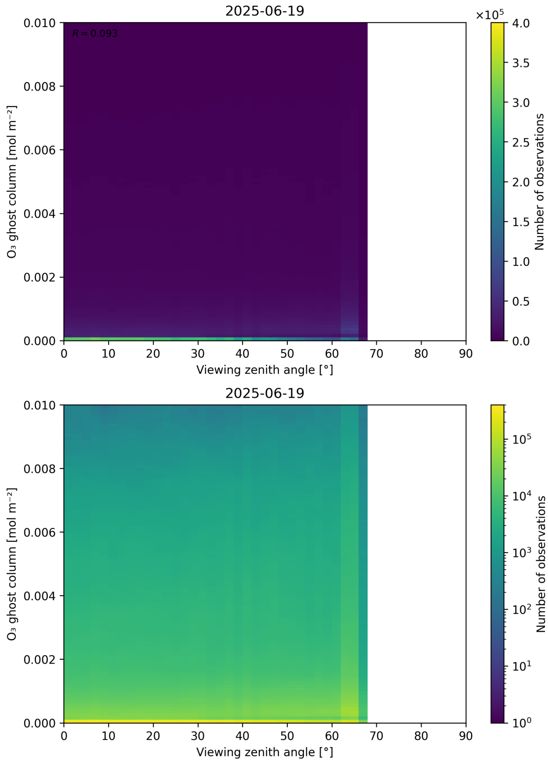
Figure 51: Scatter density plot of “Viewing zenith angle” against “O 3 ghost column” for 2025-06-18 to 2025-06-20.
