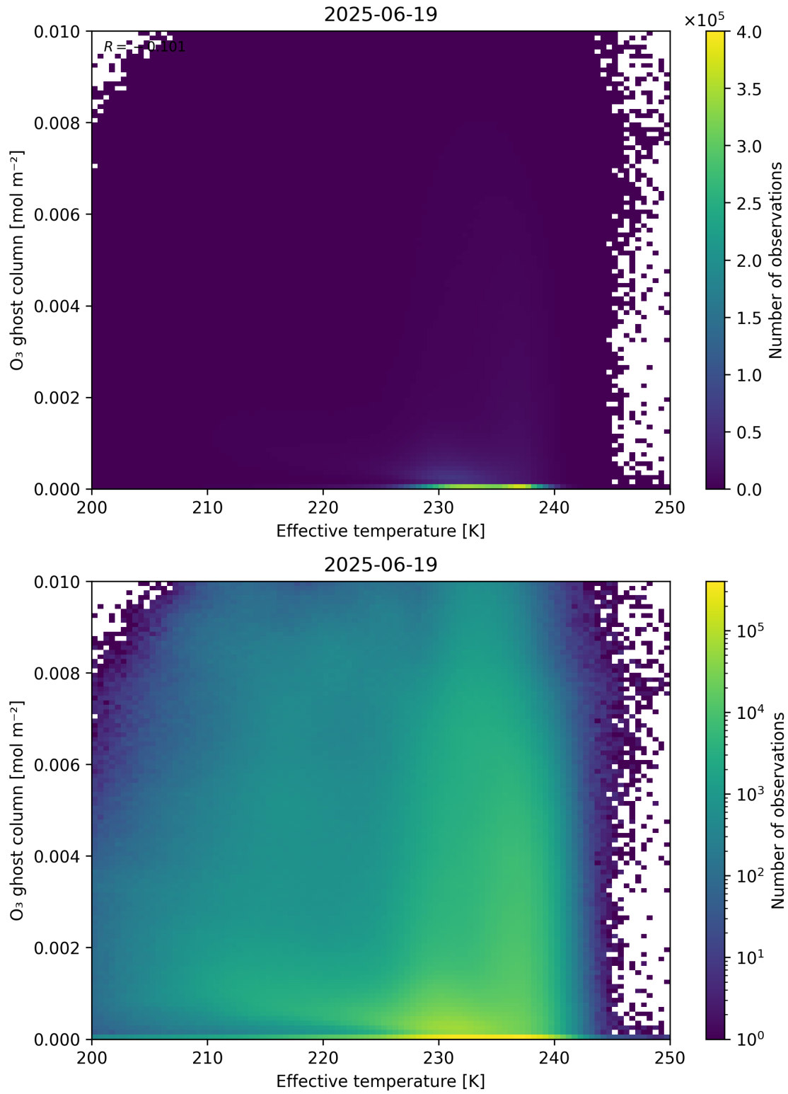
Figure 38: Scatter density plot of “Effective temperature” against “O 3 ghost column” for 2025-06-18 to 2025-06-20.
