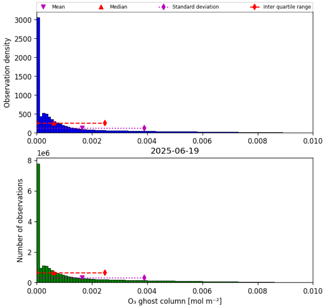
Figure 25: Histogram of “O 3 ghost column” for 2025-06-18 to 2025-06-20
