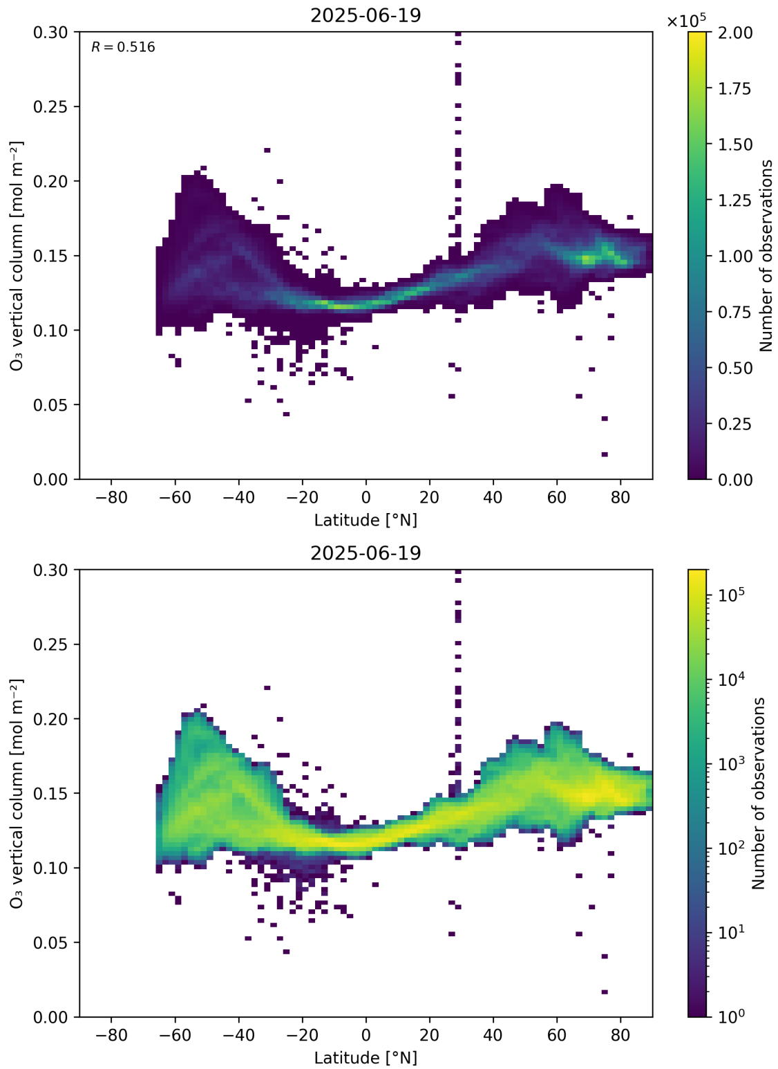
Figure 36: Scatter density plot of “Latitude” against “O 3 vertical column” for 2025-06-18 to 2025-06-20.
