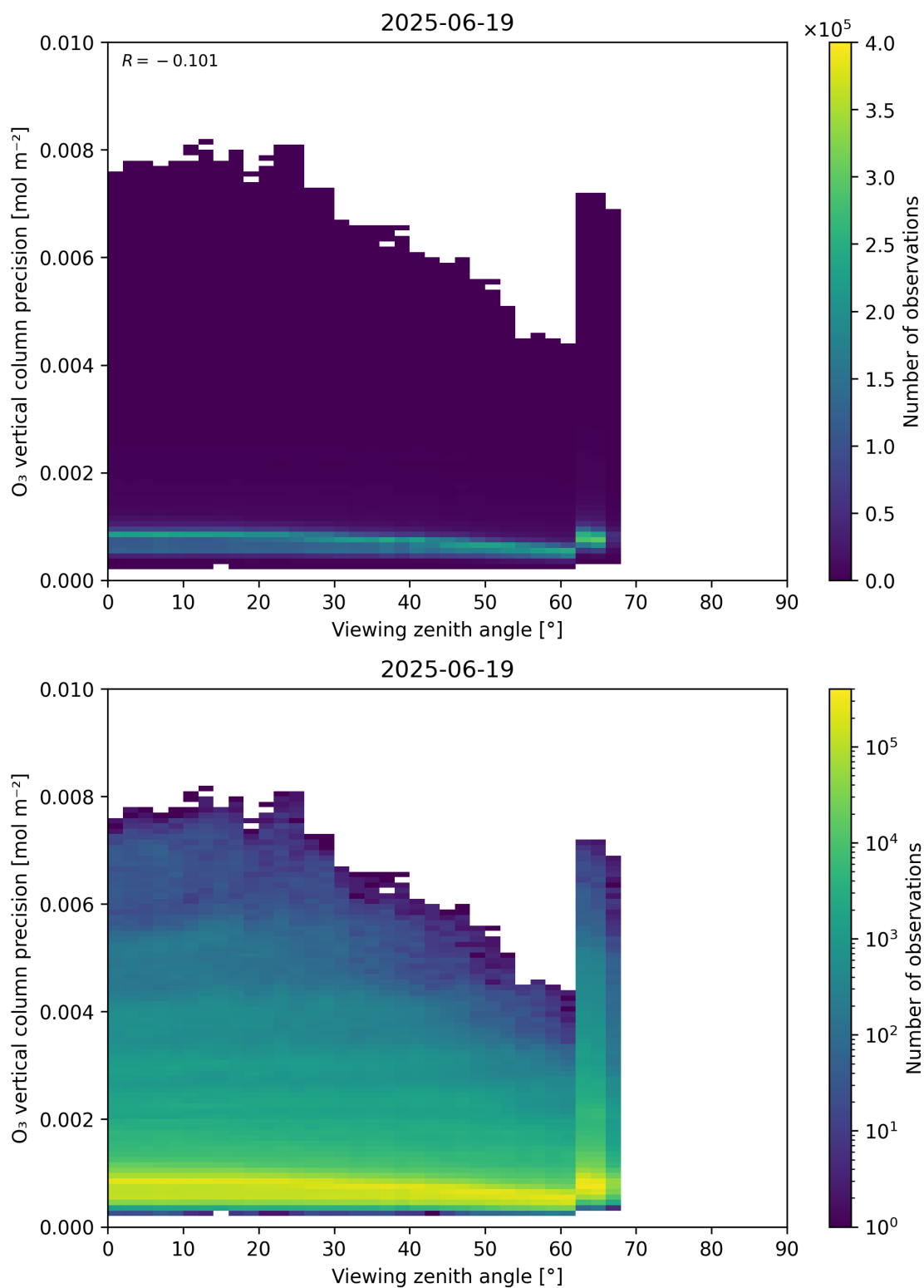
Figure 53: Scatter density plot of “Viewing zenith angle” against “O 3 vertical column precision” for 2025-06-18 to 2025-06-20.
