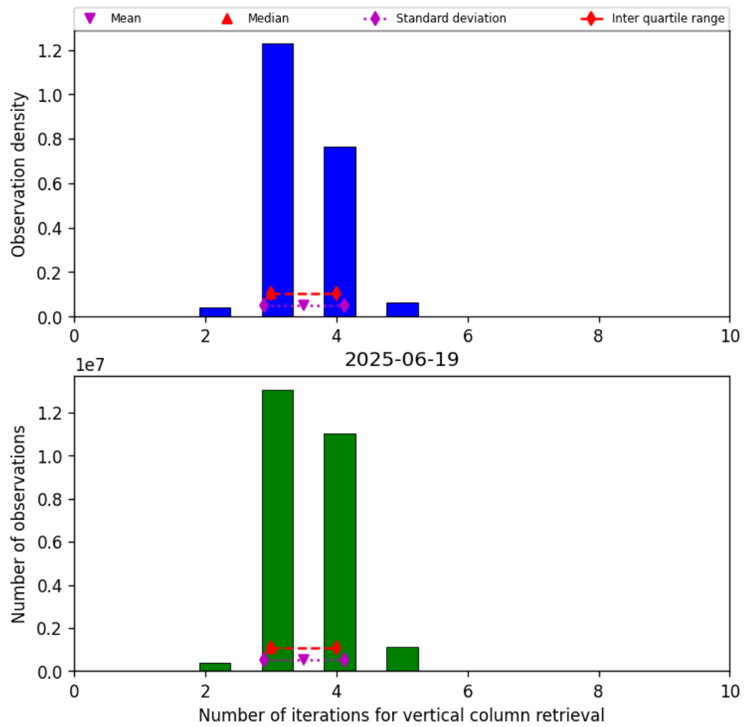
Figure 26: Histogram of “Number of iterations for vertical column retrieval” for 2025-06-18 to 2025-06-20
