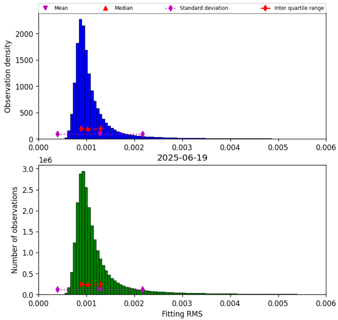
Figure 23: Histogram of “Fitting RMS” for 2025-06-18 to 2025-06-20
