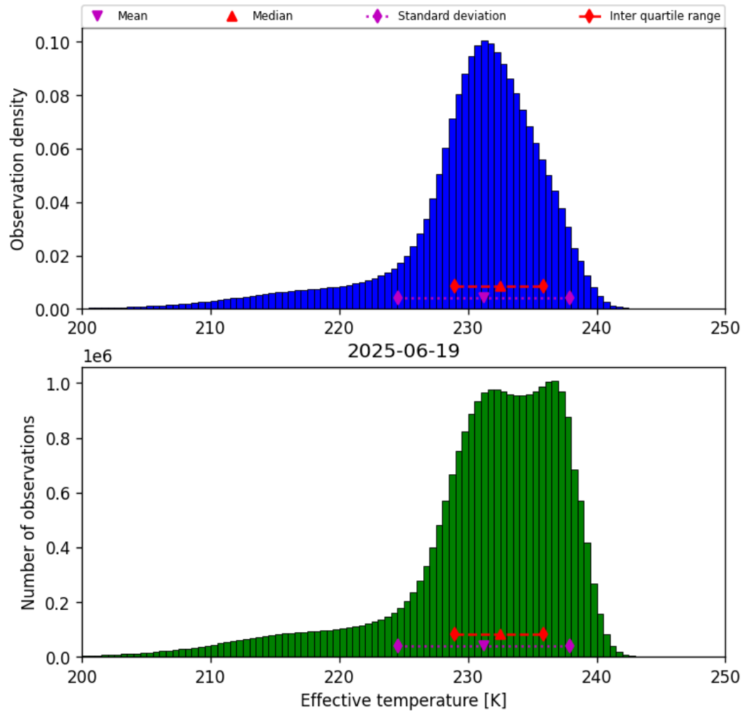
Figure 24: Histogram of “Effective temperature” for 2025-06-18 to 2025-06-20
