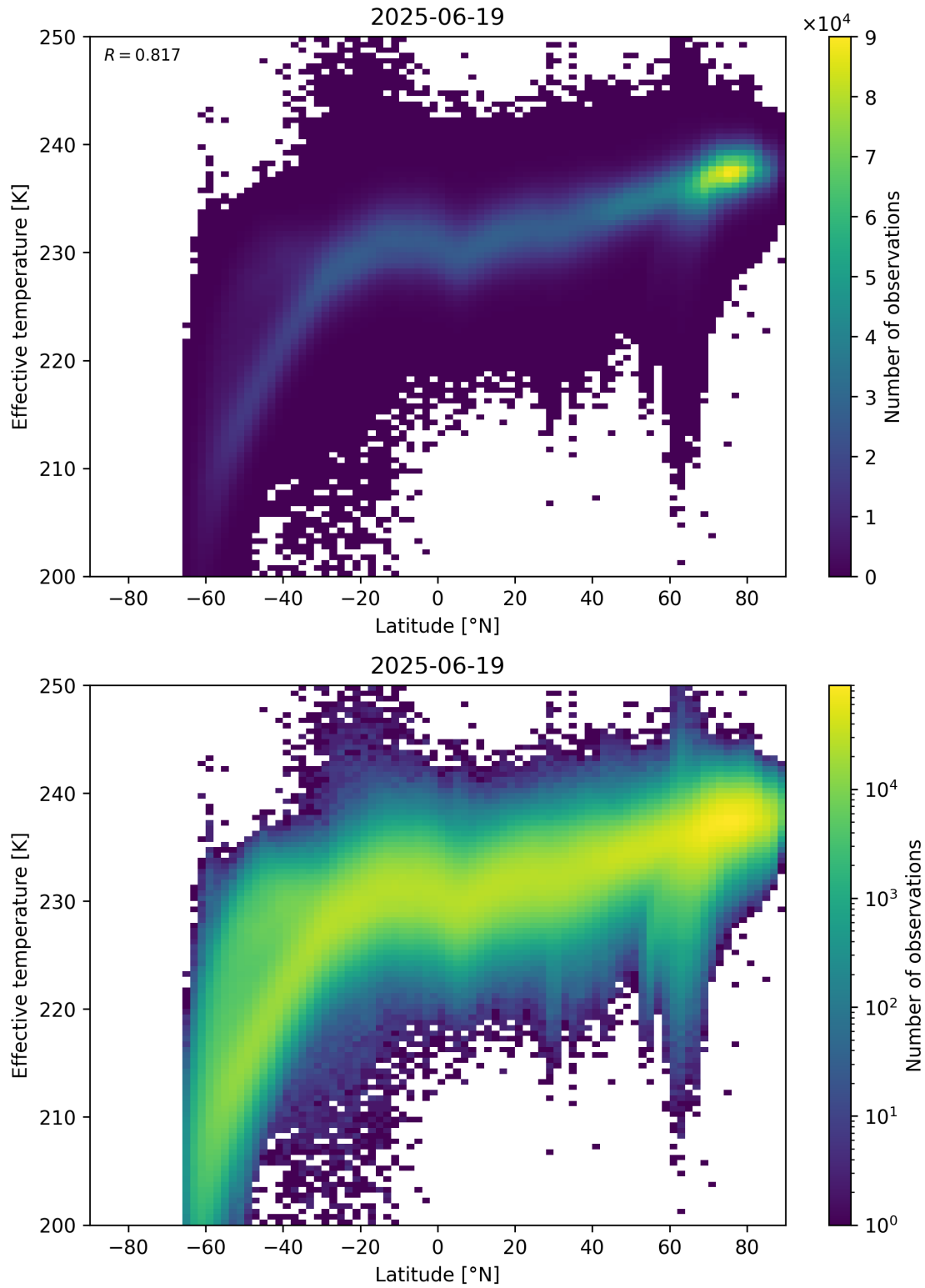
Figure 34: Scatter density plot of “Latitude” against “Effective temperature” for 2025-06-18 to 2025-06-20.
