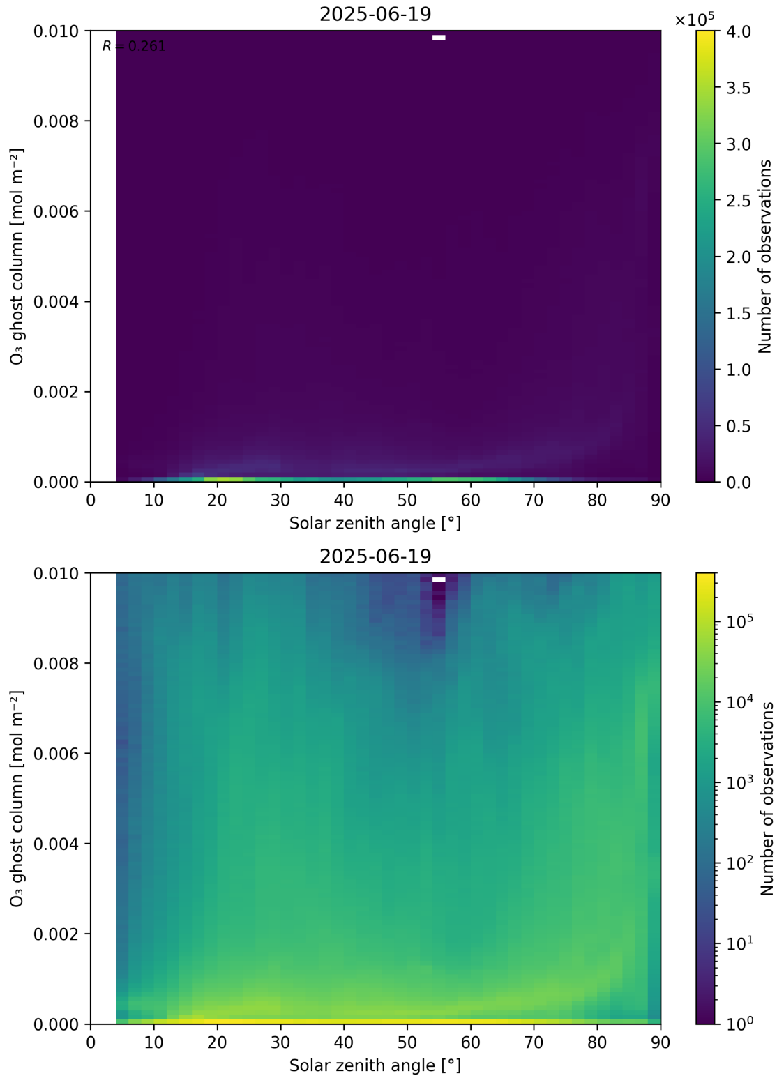
Figure 46: Scatter density plot of “Solar zenith angle” against “O 3 ghost column” for 2025-06-18 to 2025-06-20.
