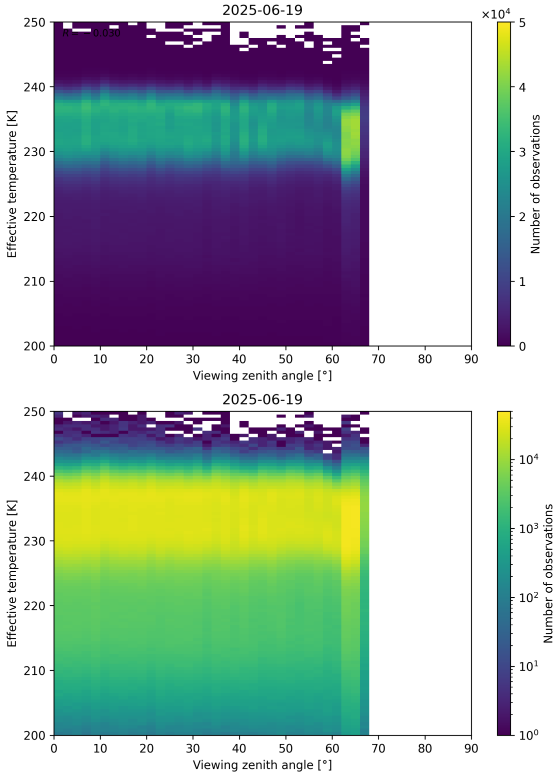
Figure 50: Scatter density plot of “Viewing zenith angle” against “Effective temperature” for 2025-06-18 to 2025-06-20.
