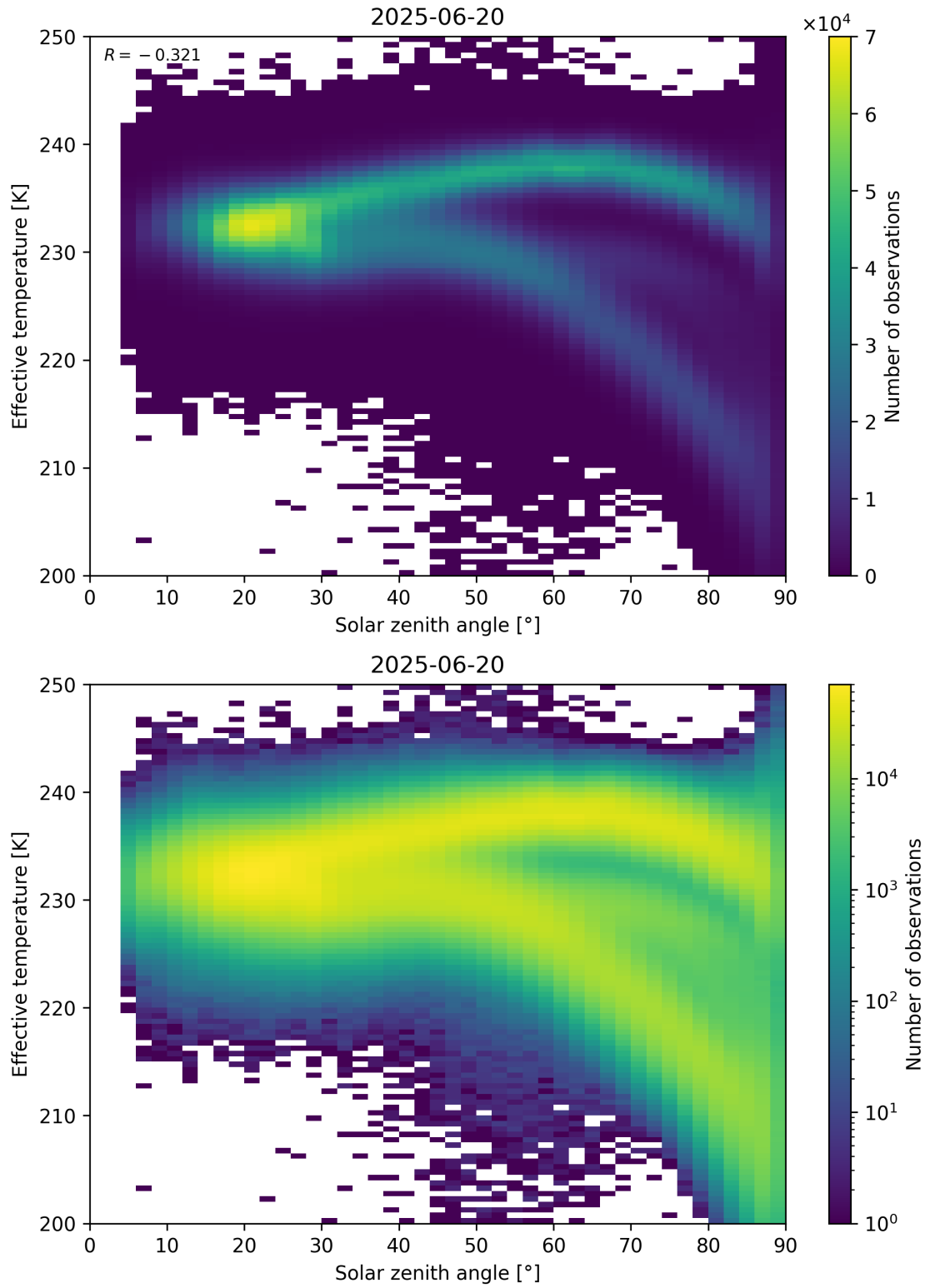
Figure 45: Scatter density plot of “Solar zenith angle” against “Effective temperature” for 2025-06-19 to 2025-06-21.
