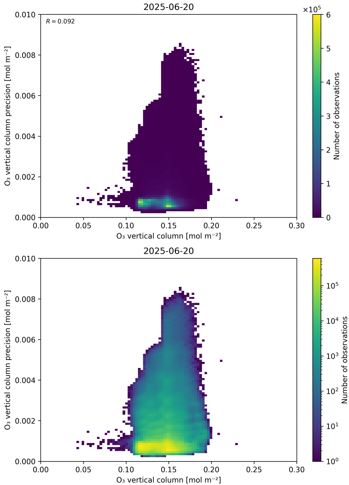
Figure 41: Scatter density plot of “O 3 vertical column” against “O 3 vertical column precision” for 2025-06-19 to 2025-06-21.
