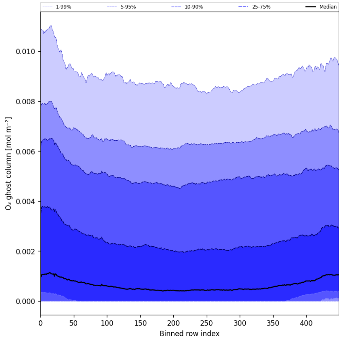
Figure 32: Along track statistics of “O 3 ghost column” for 2025-06-19 to 2025-06-21
