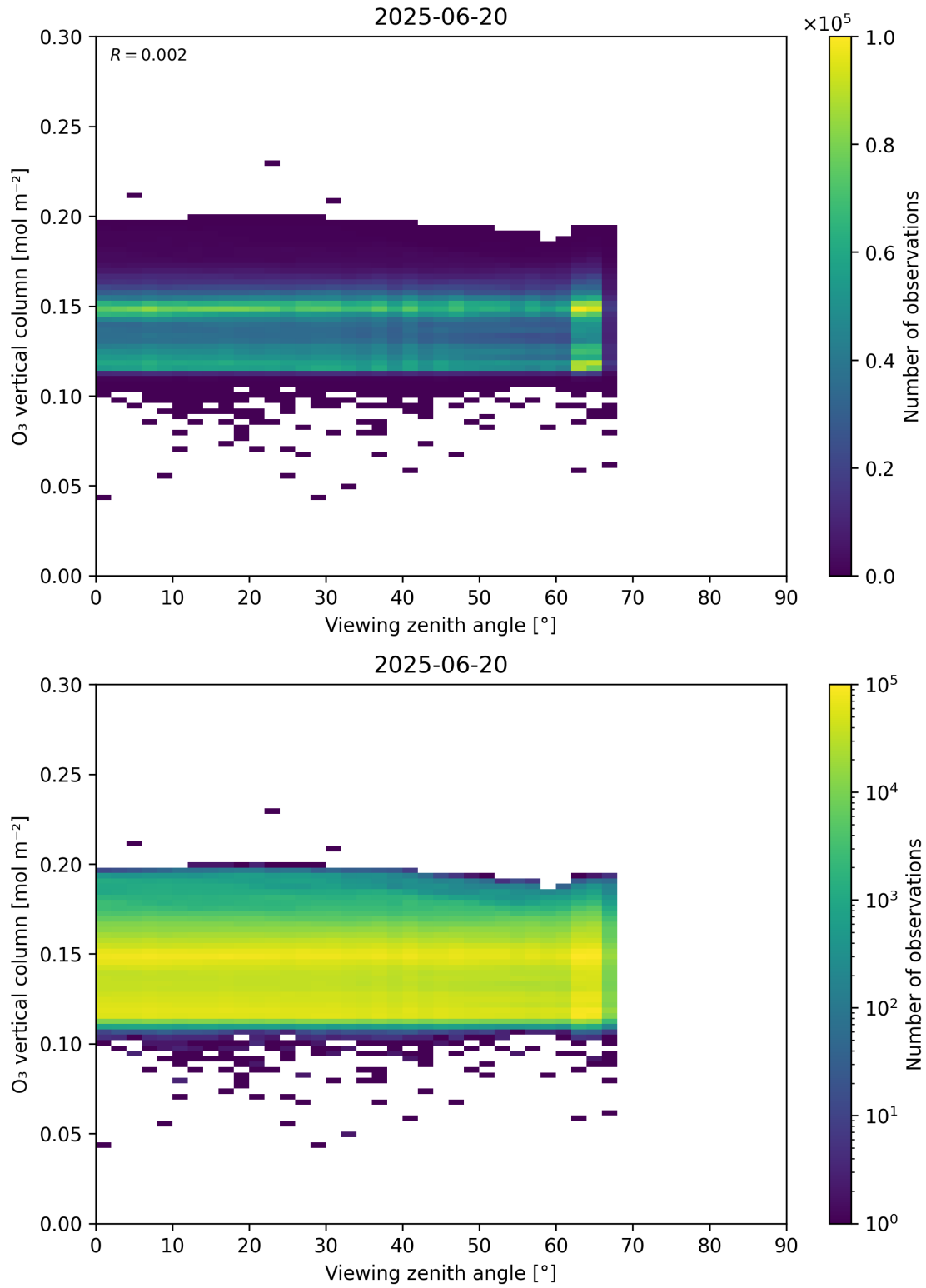
Figure 52: Scatter density plot of “Viewing zenith angle” against “O 3 vertical column” for 2025-06-19 to 2025-06-21.
