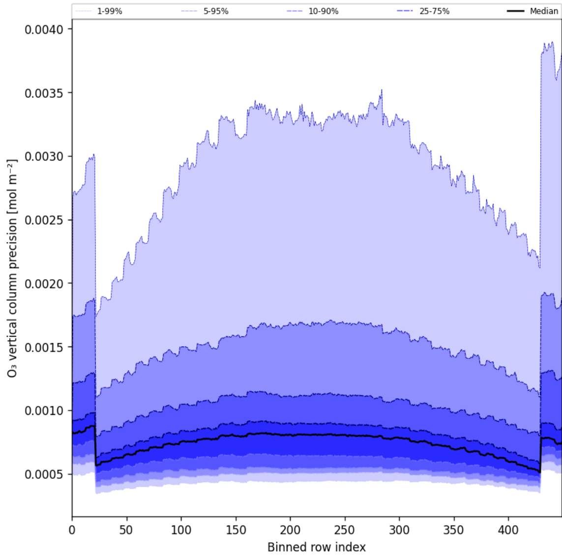
Figure 29: Along track statistics of “O 3 vertical column precision” for 2025-06-19 to 2025-06-21
