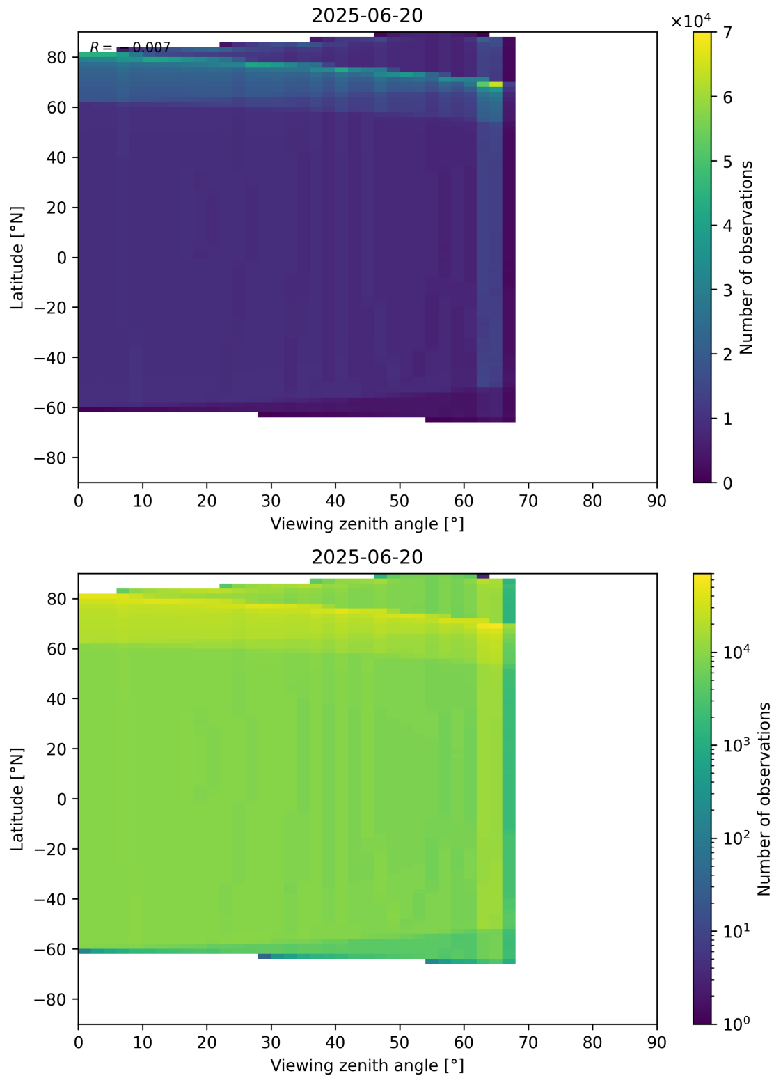
Figure 49: Scatter density plot of “Viewing zenith angle” against “Latitude” for 2025-06-19 to 2025-06-21.
