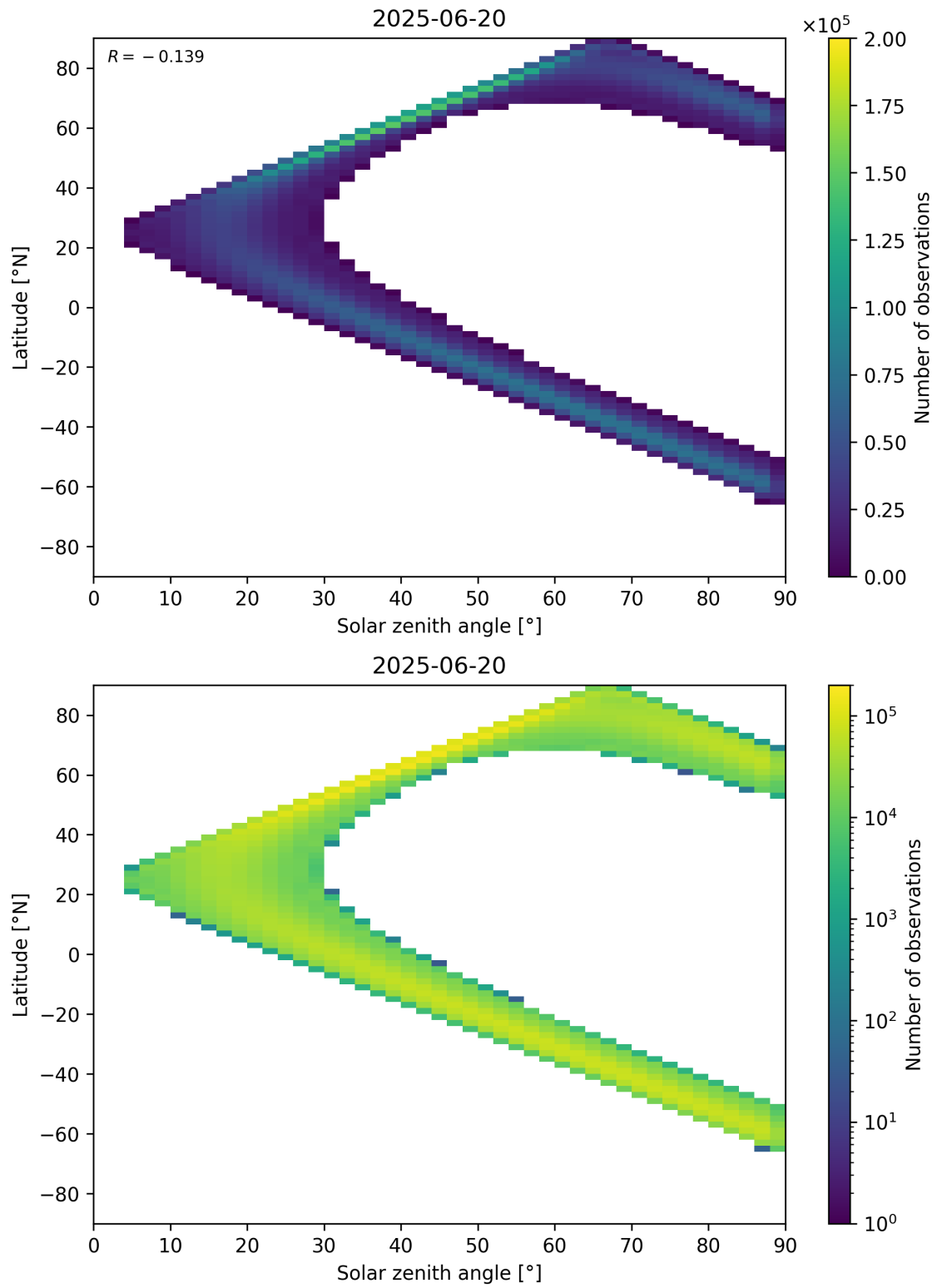
Figure 44: Scatter density plot of “Solar zenith angle” against “Latitude” for 2025-06-19 to 2025-06-21.
