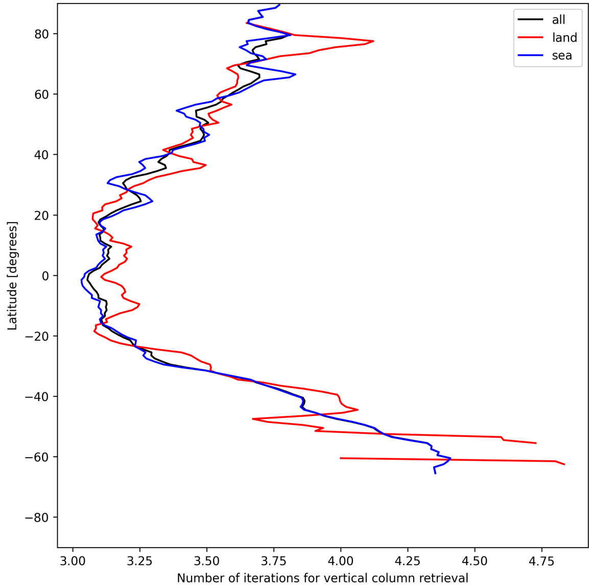
Figure 19: Zonal average of “Number of iterations for vertical column retrieval” for 2025-06-19 to 2025-06-21.
