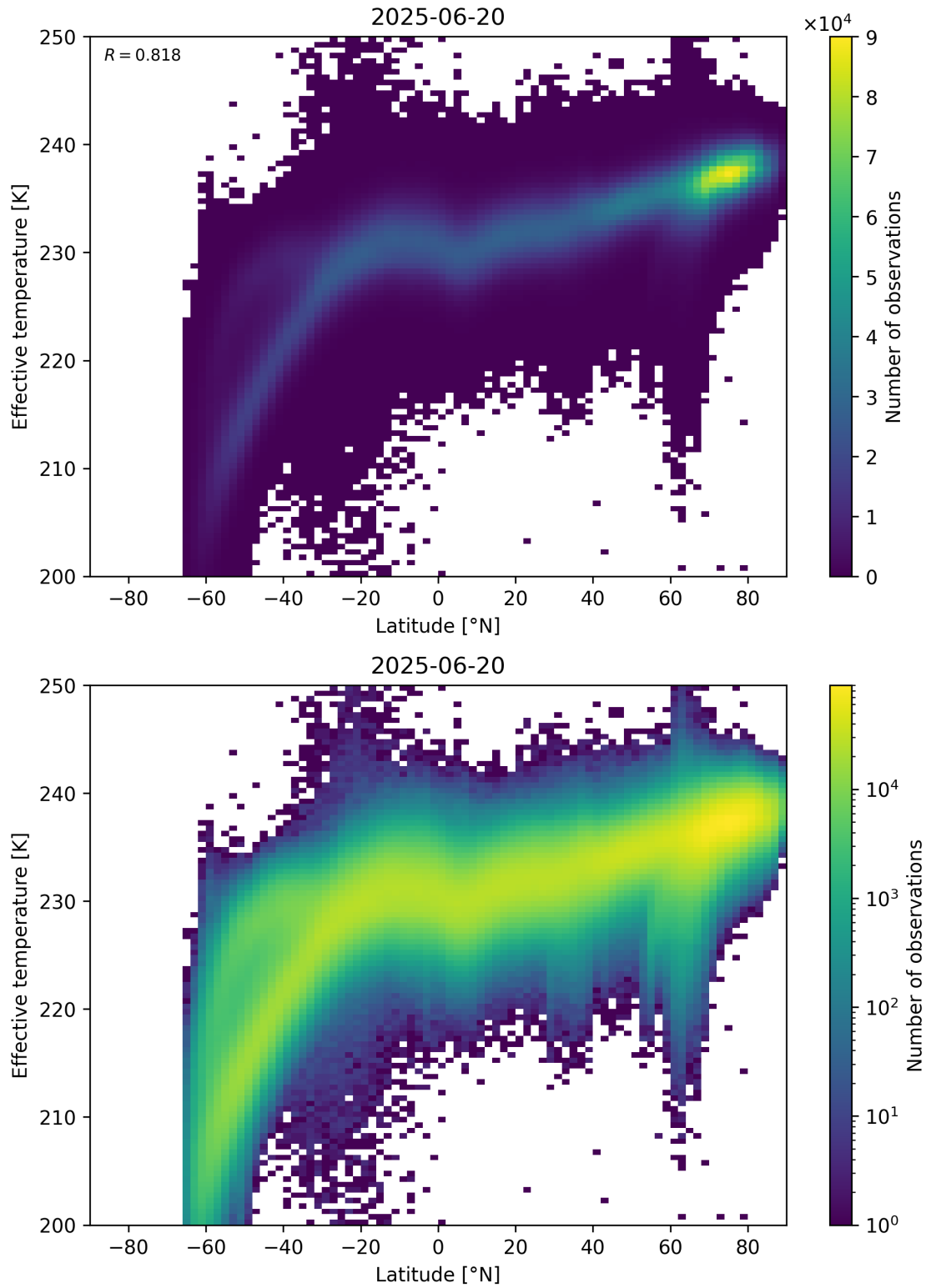
Figure 34: Scatter density plot of “Latitude” against “Effective temperature” for 2025-06-19 to 2025-06-21.
