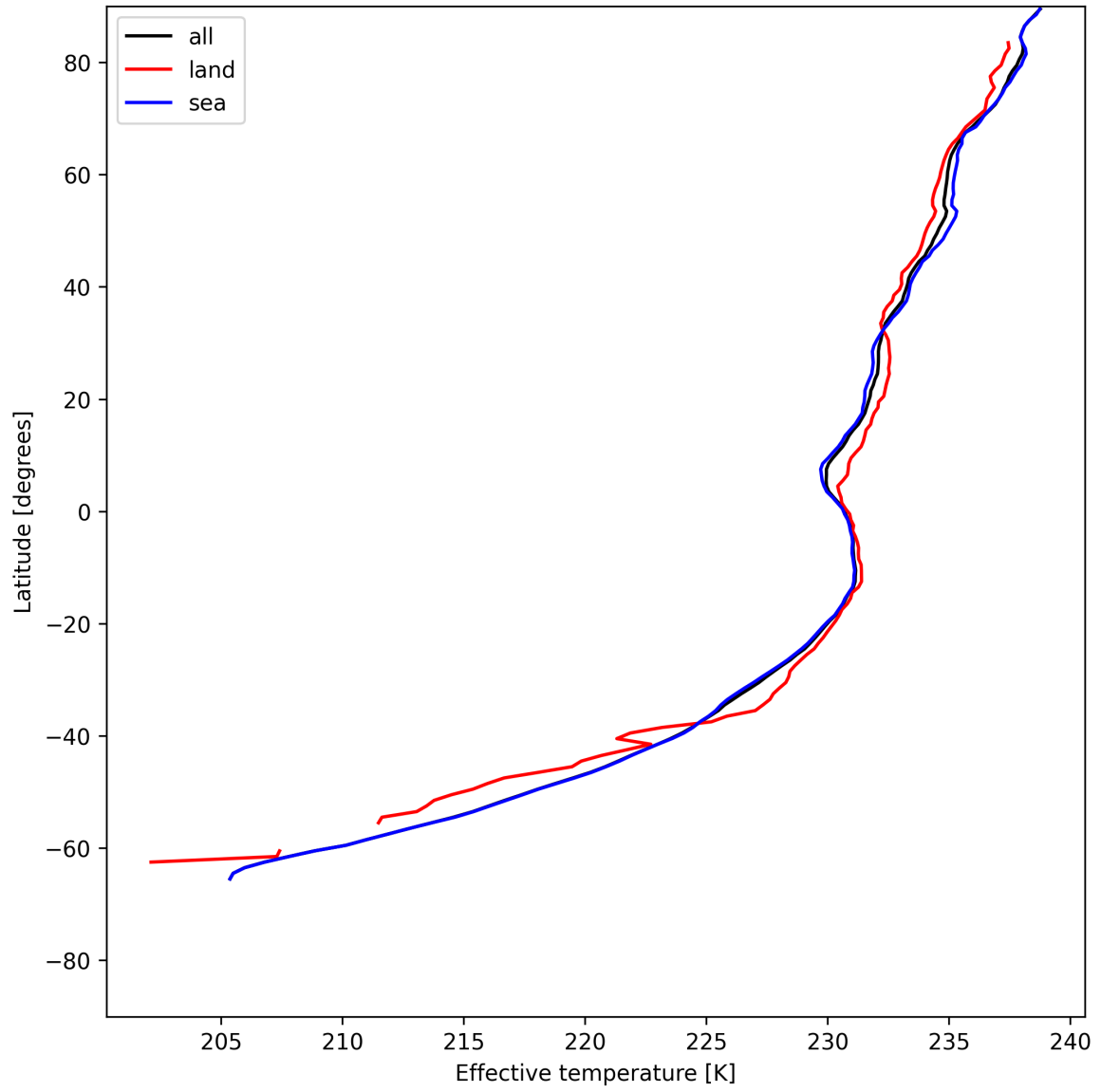
Figure 17: Zonal average of “Effective temperature” for 2025-06-19 to 2025-06-21.
