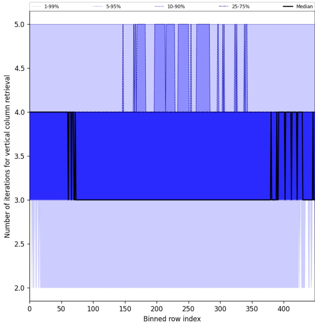
Figure 33: Along track statistics of “Number of iterations for vertical column retrieval” for 2025-06-19 to 2025-06-21
