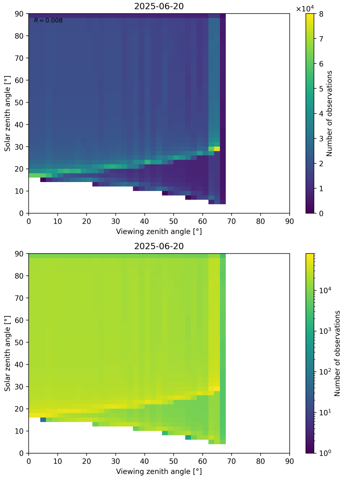
Figure 54: Scatter density plot of “Viewing zenith angle” against “Solar zenith angle” for 2025-06-19 to 2025-06-21.
