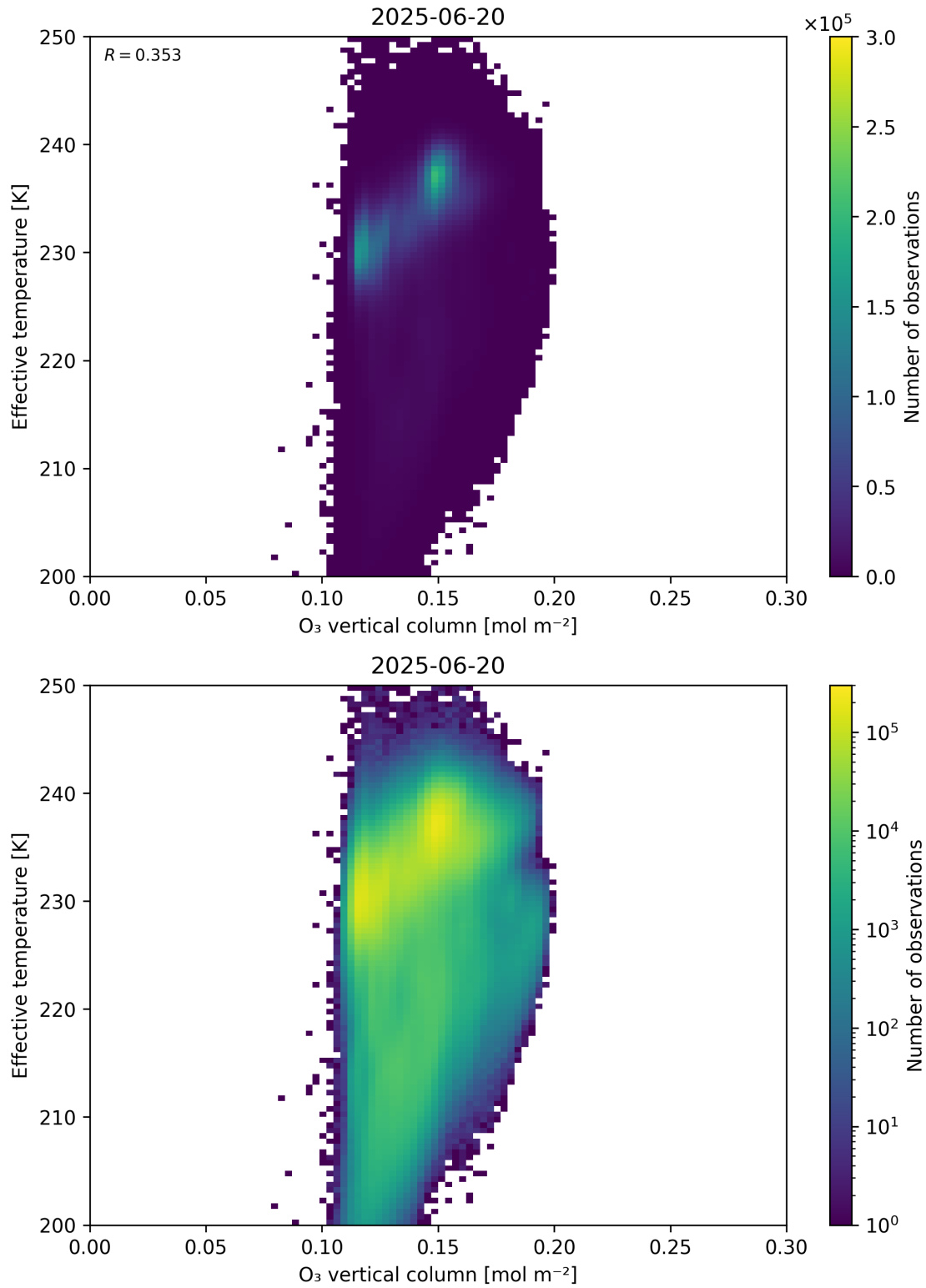
Figure 39: Scatter density plot of “O 3 vertical column” against “Effective temperature” for 2025-06-19 to 2025-06-21.
