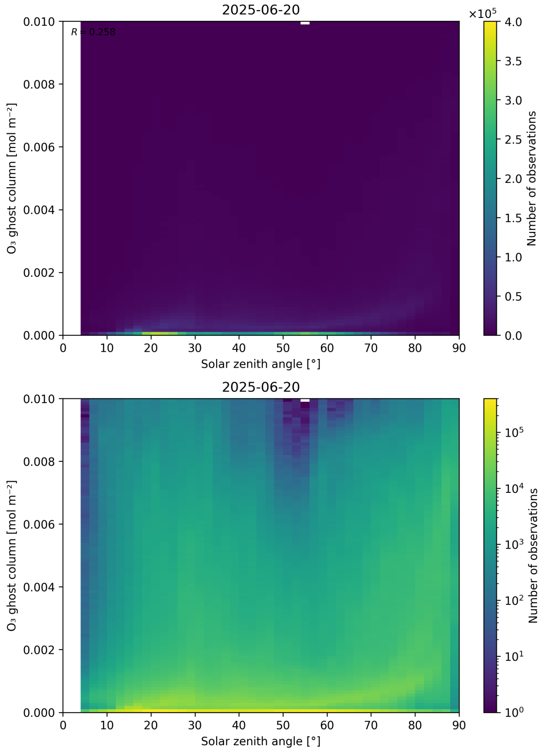
Figure 46: Scatter density plot of “Solar zenith angle” against “O 3 ghost column” for 2025-06-19 to 2025-06-21.
