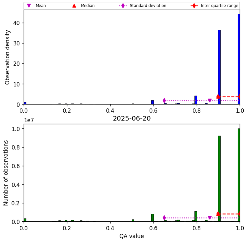
Figure 20: Histogram of “QA value” for 2025-06-19 to 2025-06-21
