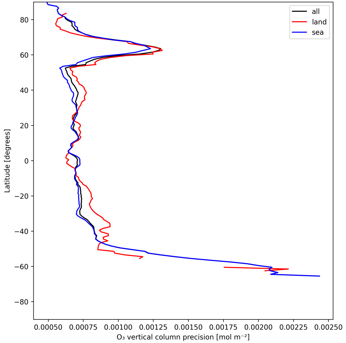
Figure 15: Zonal average of “O 3 vertical column precision” for 2025-06-19 to 2025-06-21.
