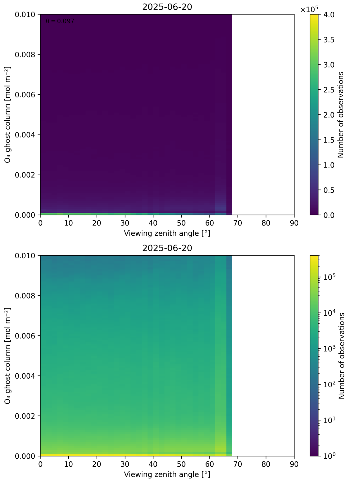
Figure 51: Scatter density plot of “Viewing zenith angle” against “O 3 ghost column” for 2025-06-19 to 2025-06-21.
