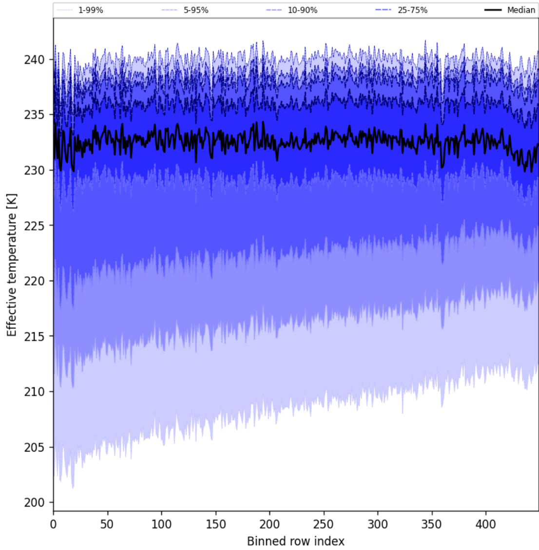
Figure 31: Along track statistics of “Effective temperature” for 2025-06-19 to 2025-06-21
