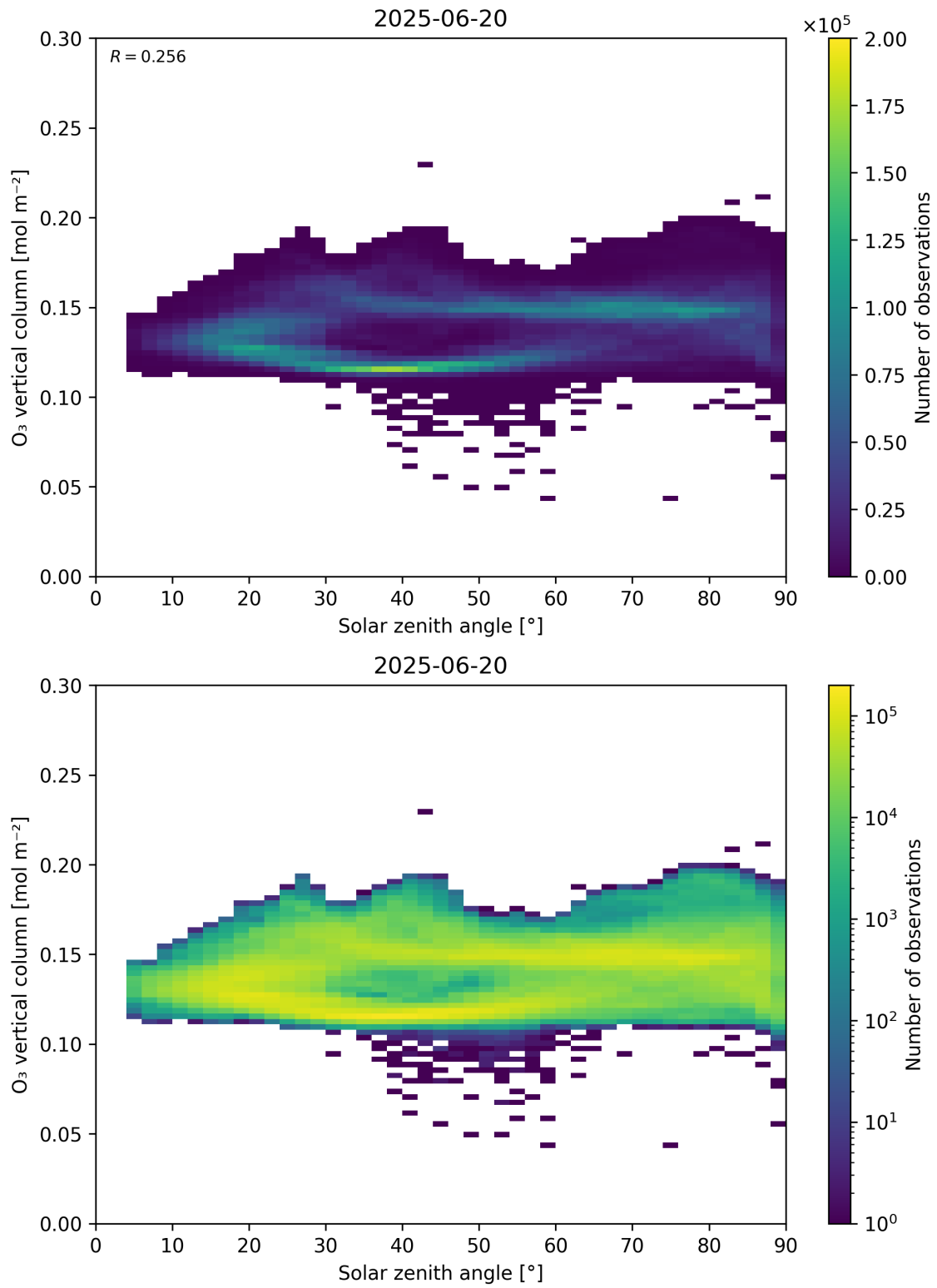
Figure 47: Scatter density plot of “Solar zenith angle” against “O 3 vertical column” for 2025-06-19 to 2025-06-21.
