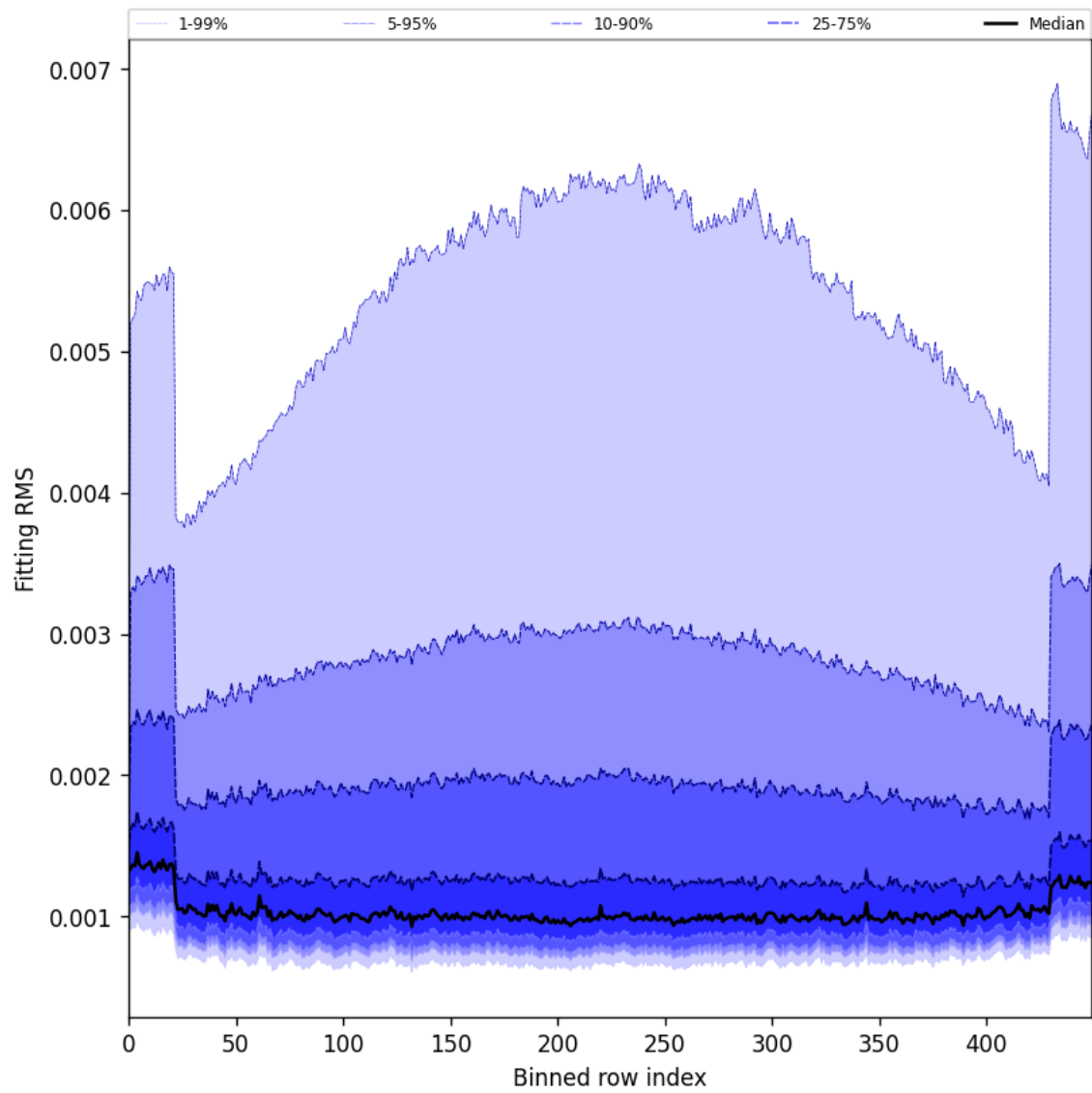
Figure 30: Along track statistics of “Fitting RMS” for 2025-06-19 to 2025-06-21
