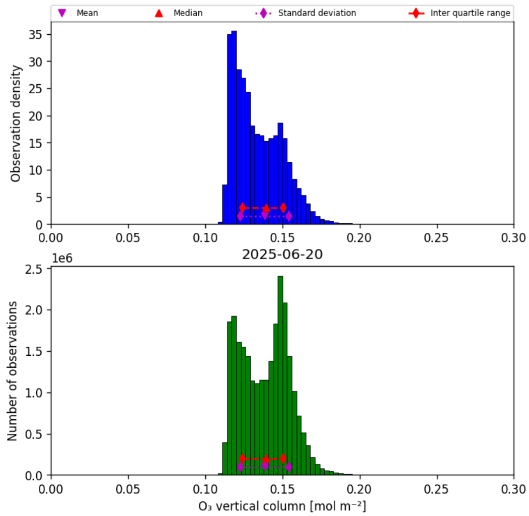
Figure 21: Histogram of “O 3 vertical column” for 2025-06-19 to 2025-06-21
