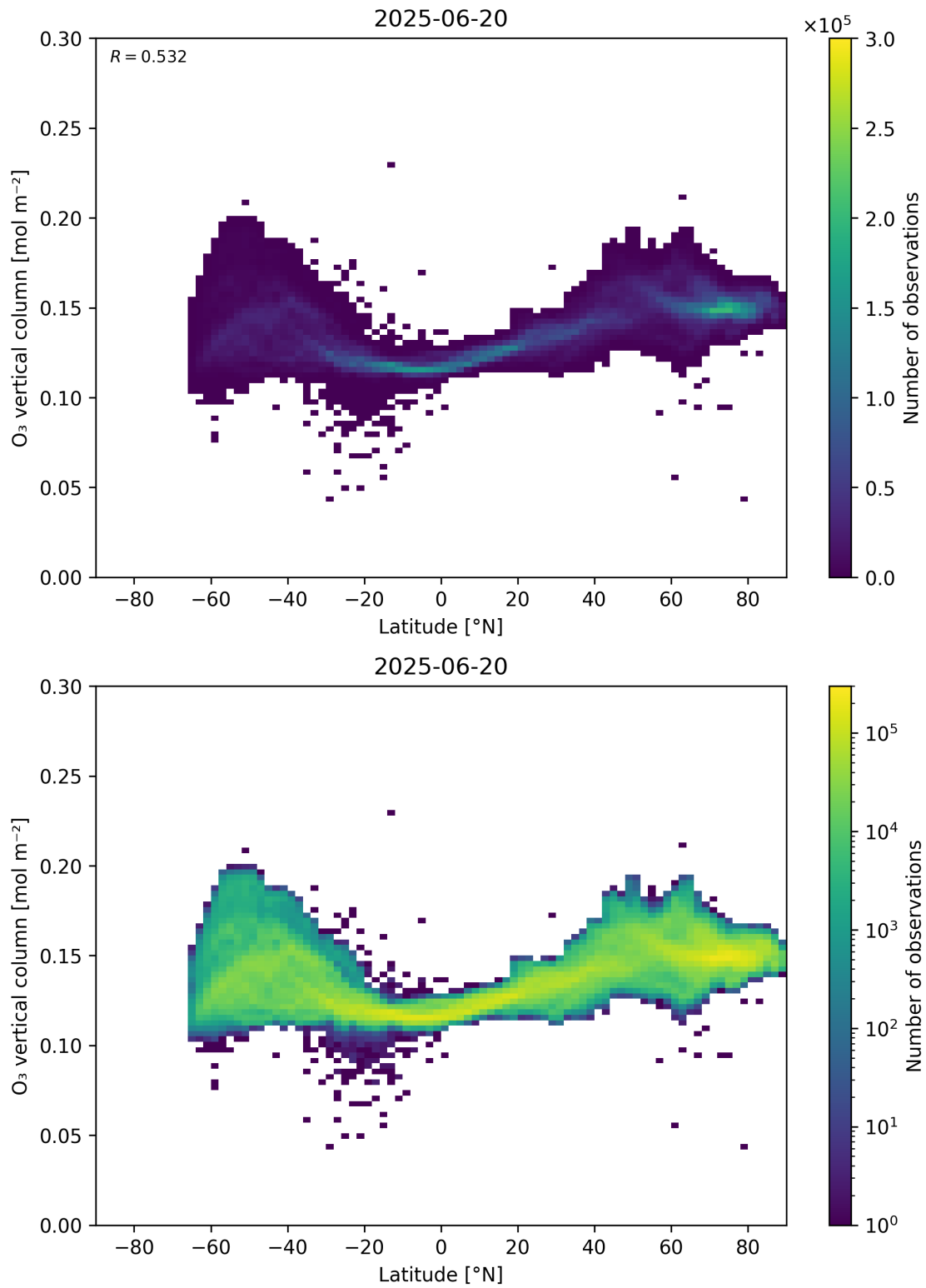
Figure 36: Scatter density plot of “Latitude” against “O 3 vertical column” for 2025-06-19 to 2025-06-21.
