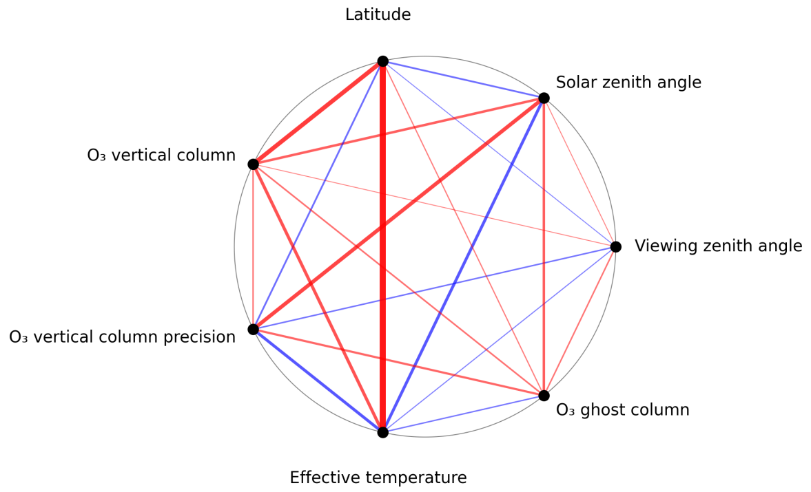
Figure 1: Map of correlation graph for 2025-06-19 to 2025-06-21.
