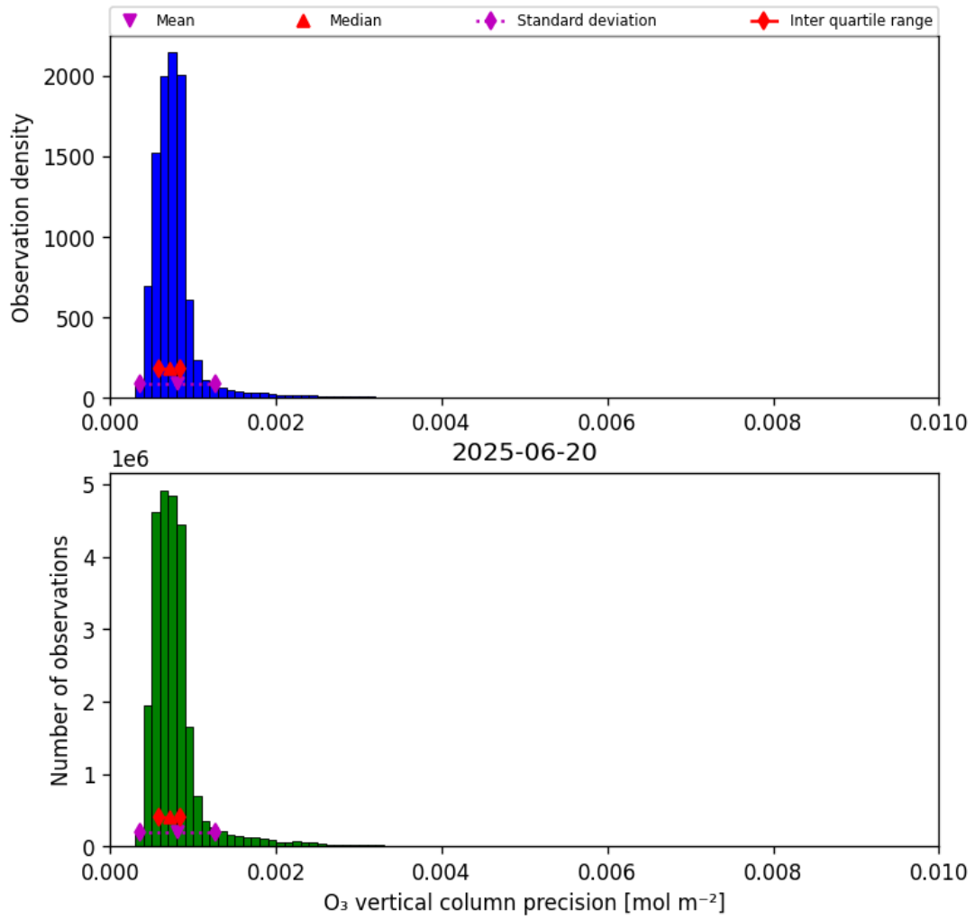
Figure 22: Histogram of “O 3 vertical column precision” for 2025-06-19 to 2025-06-21
