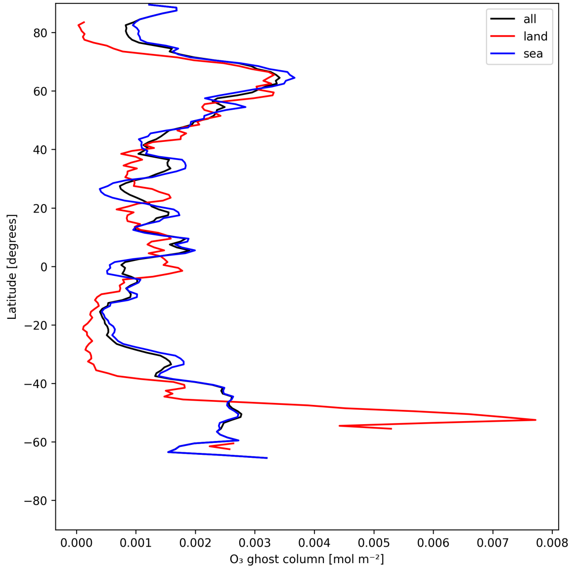
Figure 18: Zonal average of "O 3 ghost column" for 2025-06-19 to 2025-06-21.
