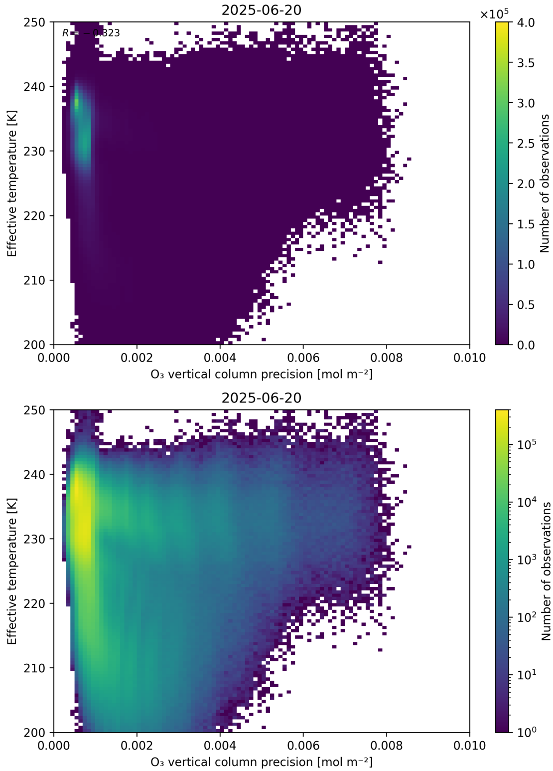
Figure 42: Scatter density plot of “O 3 vertical column precision” against “Effective temperature” for 2025-06-19 to 2025-06-21.
