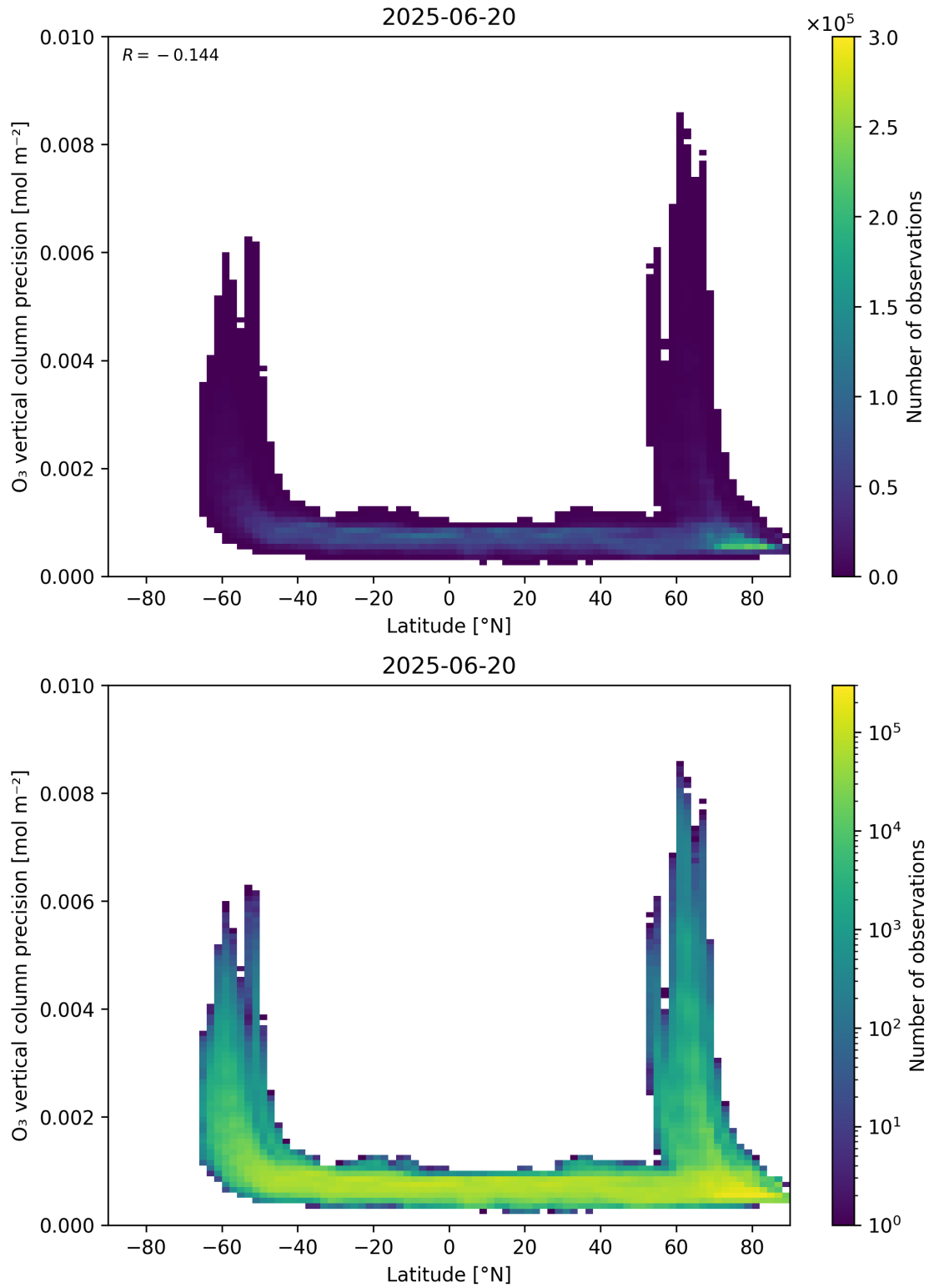
Figure 37: Scatter density plot of “Latitude” against “O 3 vertical column precision” for 2025-06-19 to 2025-06-21.
