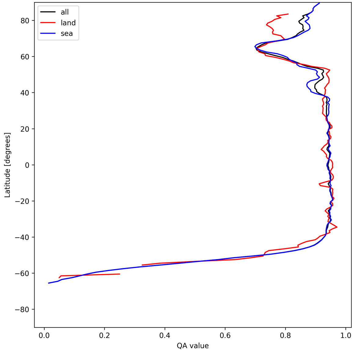
Figure 13: Zonal average of “QA value” for 2025-06-19 to 2025-06-21.
