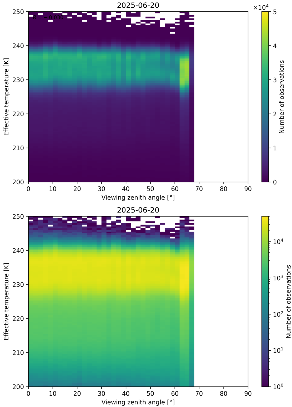
Figure 50: Scatter density plot of “Viewing zenith angle” against “Effective temperature” for 2025-06-19 to 2025-06-21.
