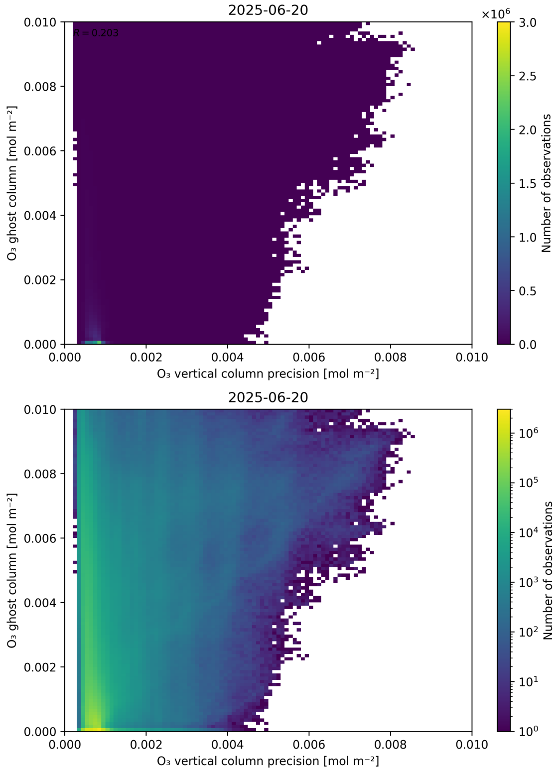
Figure 43: Scatter density plot of “ \text{O}_3 vertical column precision” against “ \text{O}_3 ghost column” for 2025-06-19 to 2025-06-21.
