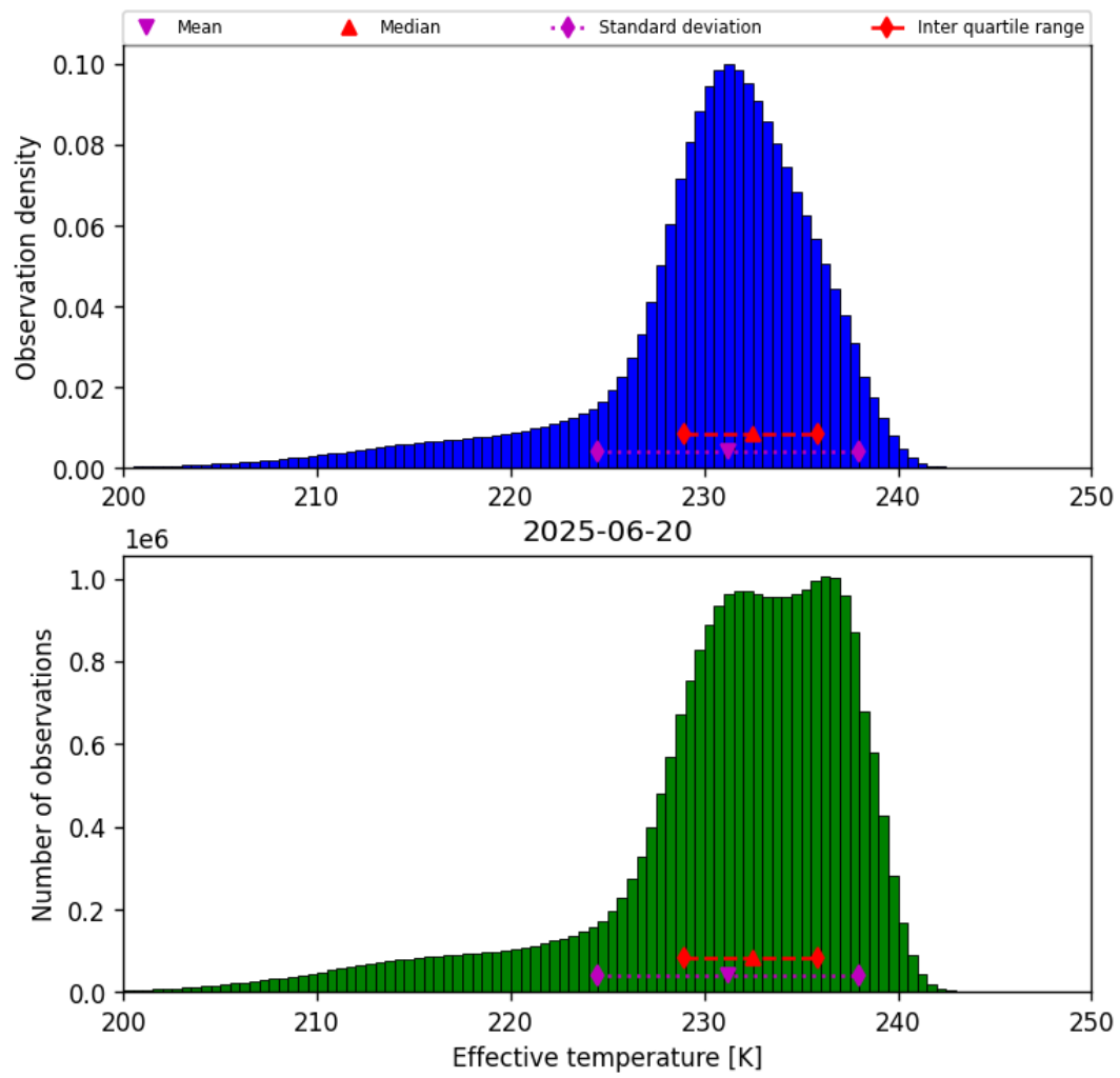
Figure 24: Histogram of “Effective temperature” for 2025-06-19 to 2025-06-21
