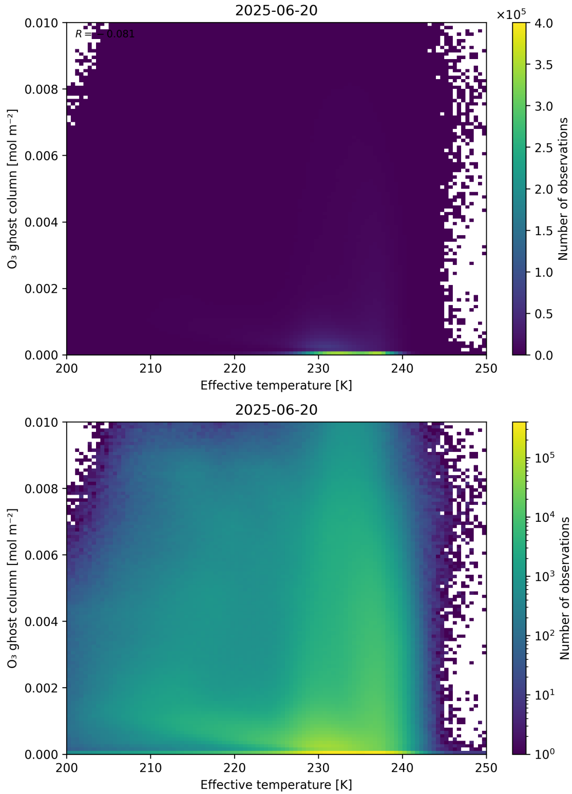
Figure 38: Scatter density plot of “Effective temperature” against “O 3 ghost column” for 2025-06-19 to 2025-06-21.
