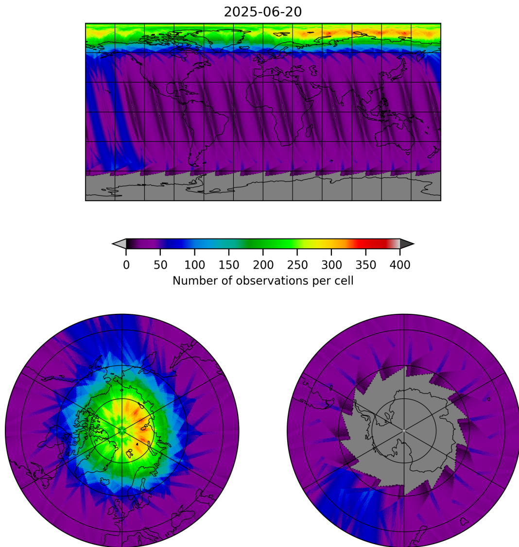
Figure 12: Map of the number of observations for 2025-06-19 to 2025-06-21
