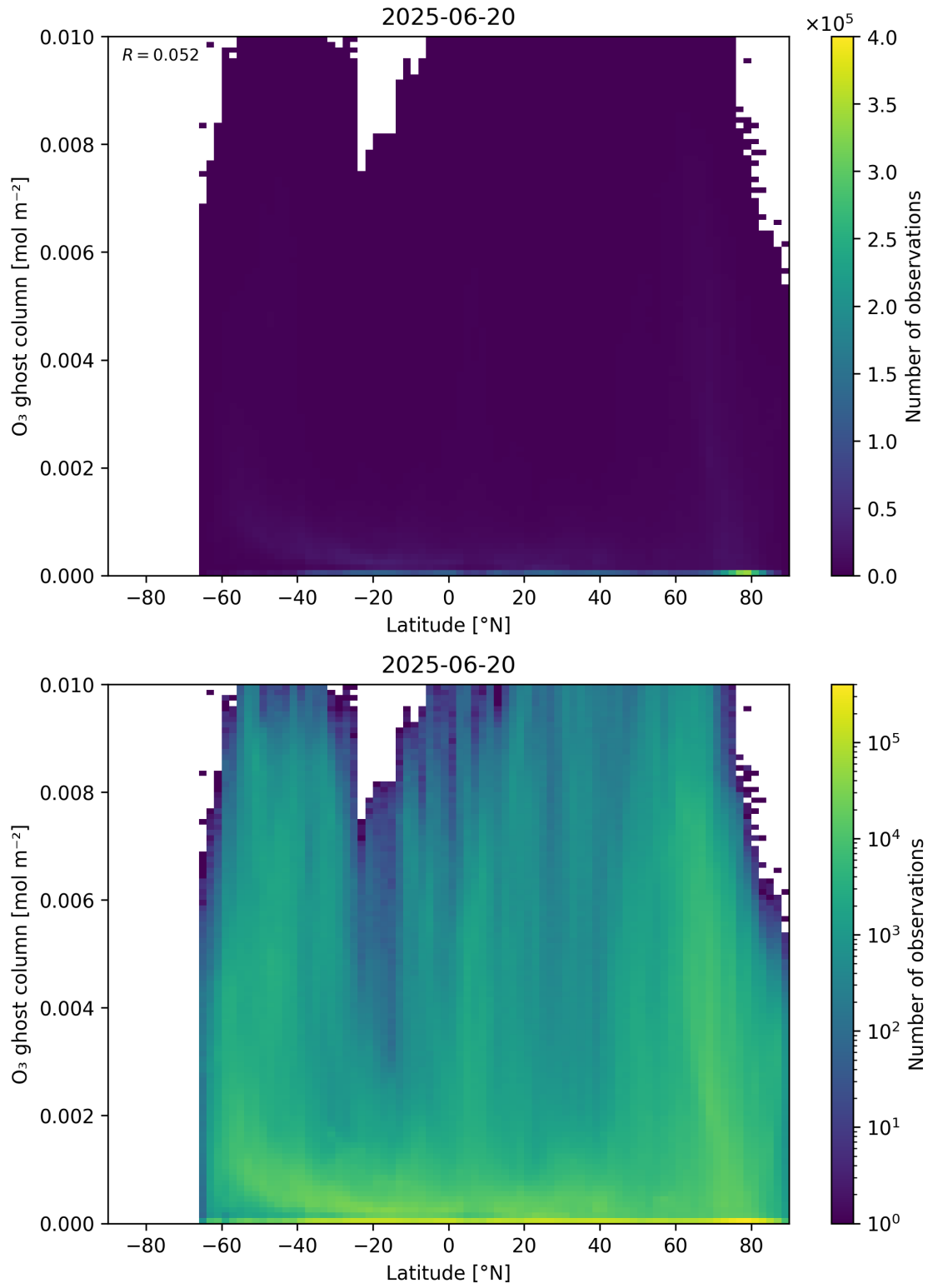
Figure 35: Scatter density plot of “Latitude” against “O 3 ghost column” for 2025-06-19 to 2025-06-21.
