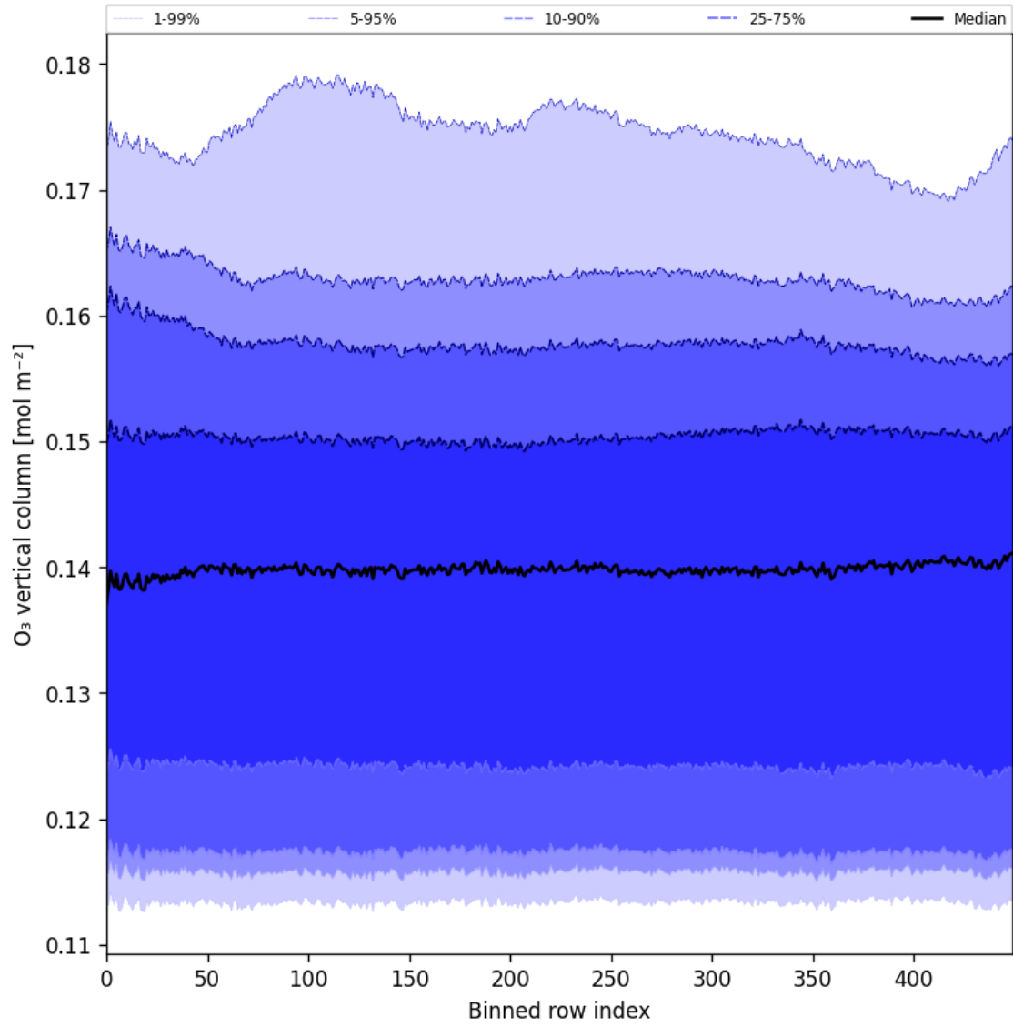
Figure 28: Along track statistics of “O 3 vertical column” for 2025-06-19 to 2025-06-21
