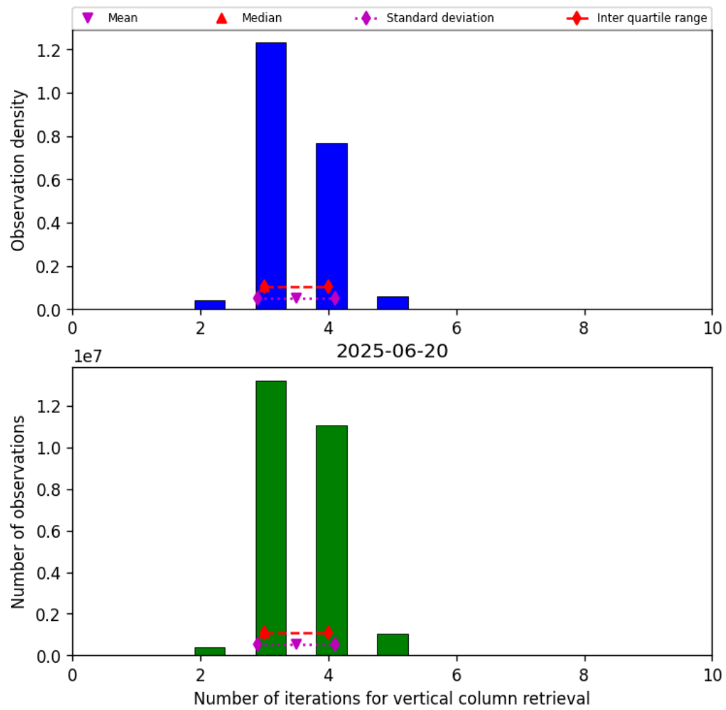
Figure 26: Histogram of “Number of iterations for vertical column retrieval” for 2025-06-19 to 2025-06-21
