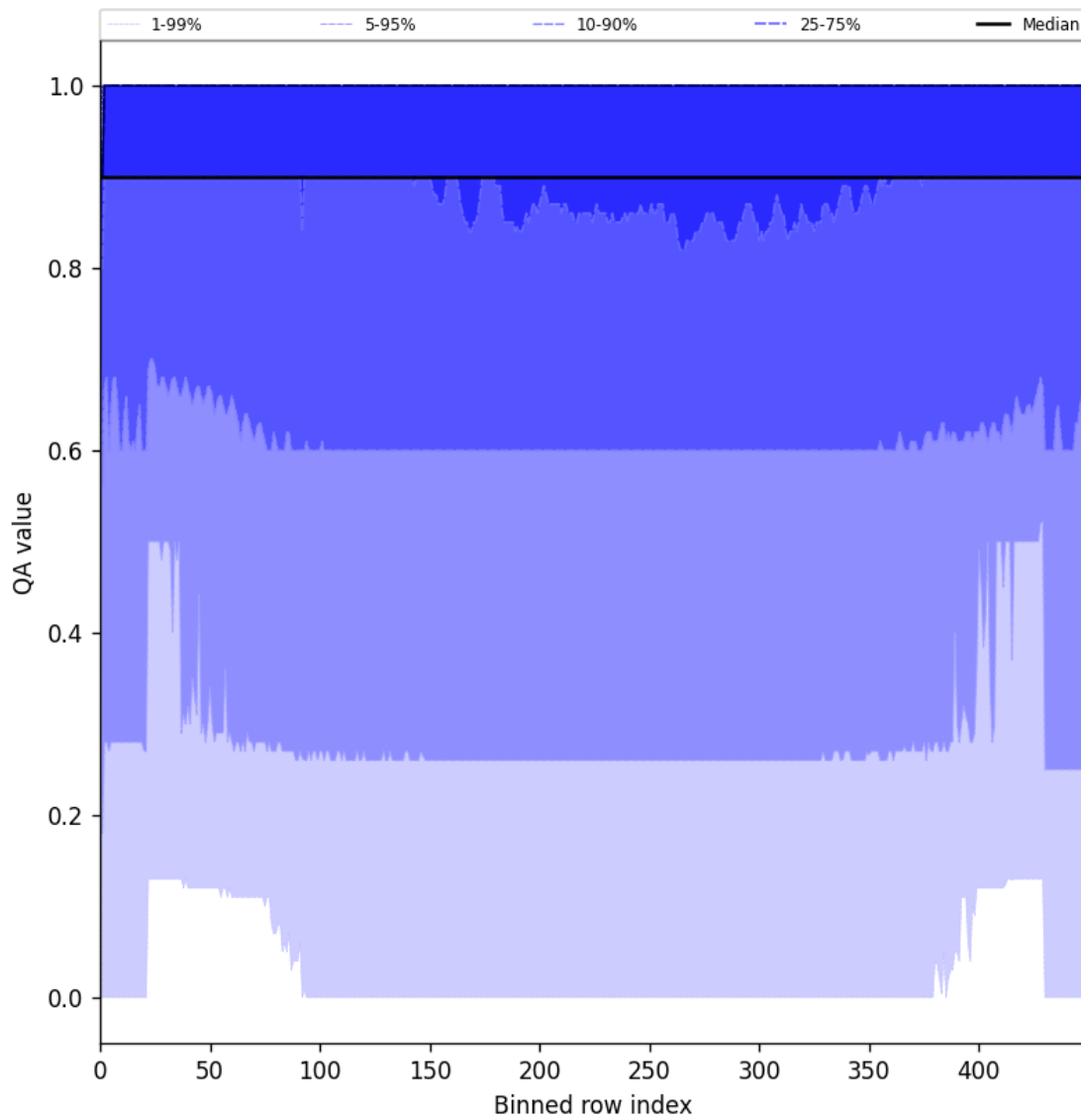
Figure 27: Along track statistics of “QA value” for 2025-06-19 to 2025-06-21
