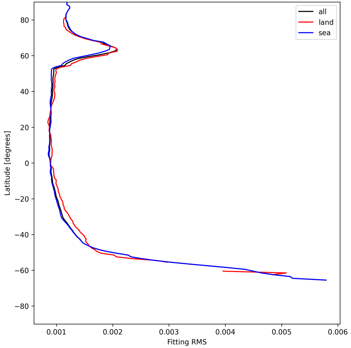
Figure 16: Zonal average of “Fitting RMS” for 2025-06-19 to 2025-06-21.
