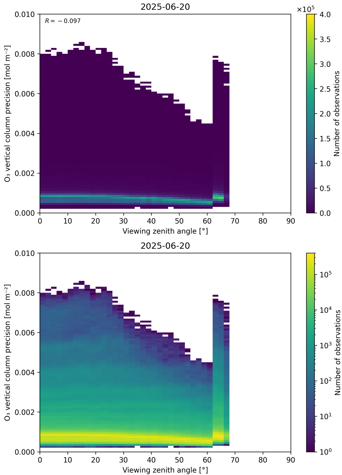
Figure 53: Scatter density plot of “Viewing zenith angle” against “O 3 vertical column precision” for 2025-06-19 to 2025-06-21.
