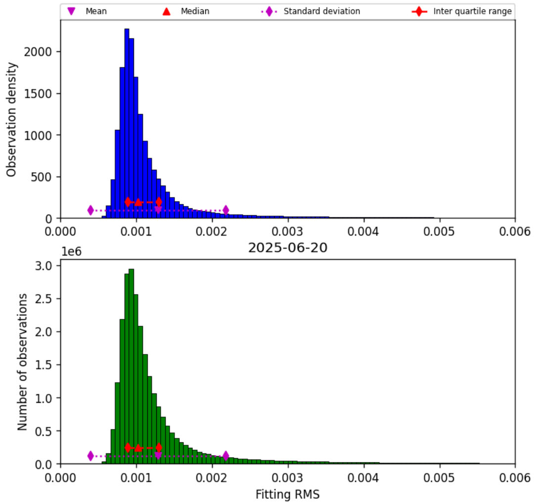
Figure 23: Histogram of “Fitting RMS” for 2025-06-19 to 2025-06-21
