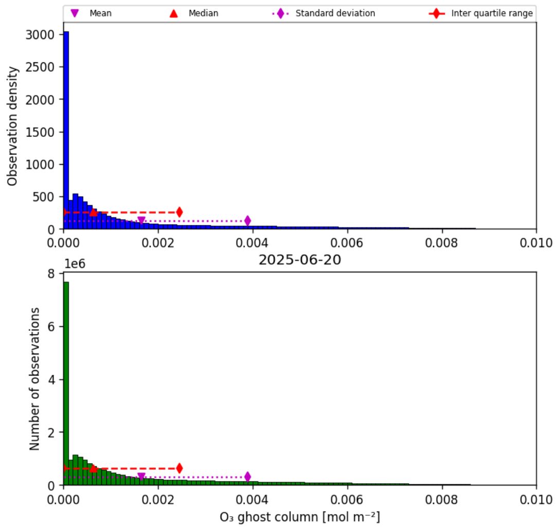
Figure 25: Histogram of “O 3 ghost column” for 2025-06-19 to 2025-06-21
