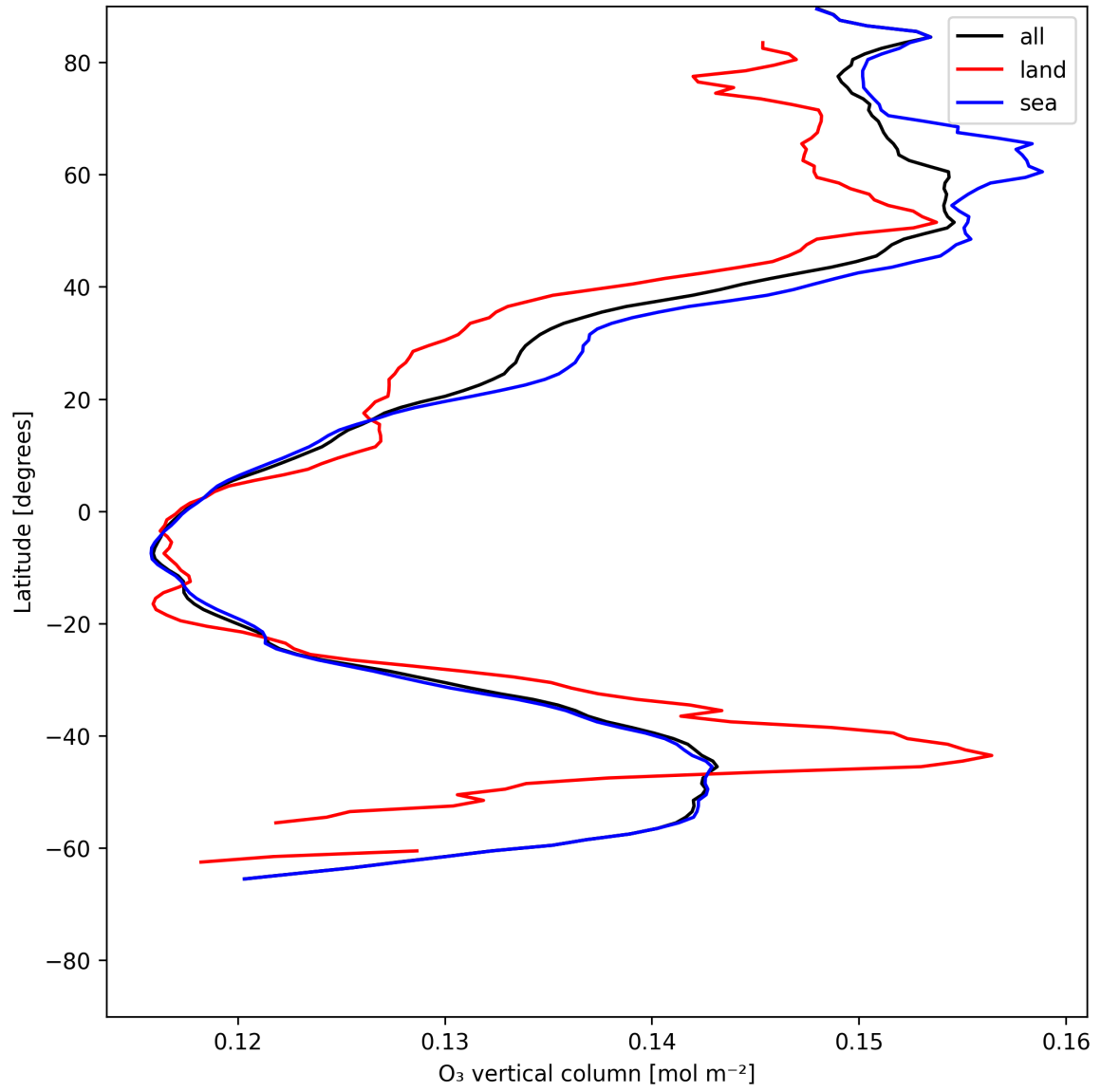
Figure 14: Zonal average of “O 3 vertical column” for 2025-06-19 to 2025-06-21.
