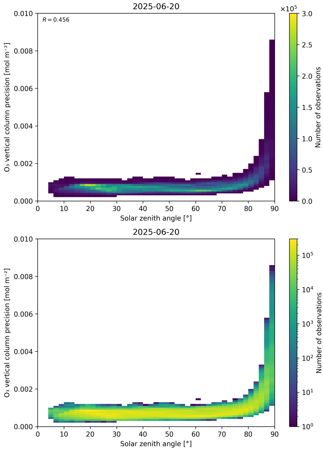
Figure 48: Scatter density plot of “Solar zenith angle” against “O 3 vertical column precision” for 2025-06-19 to 2025-06-21.
