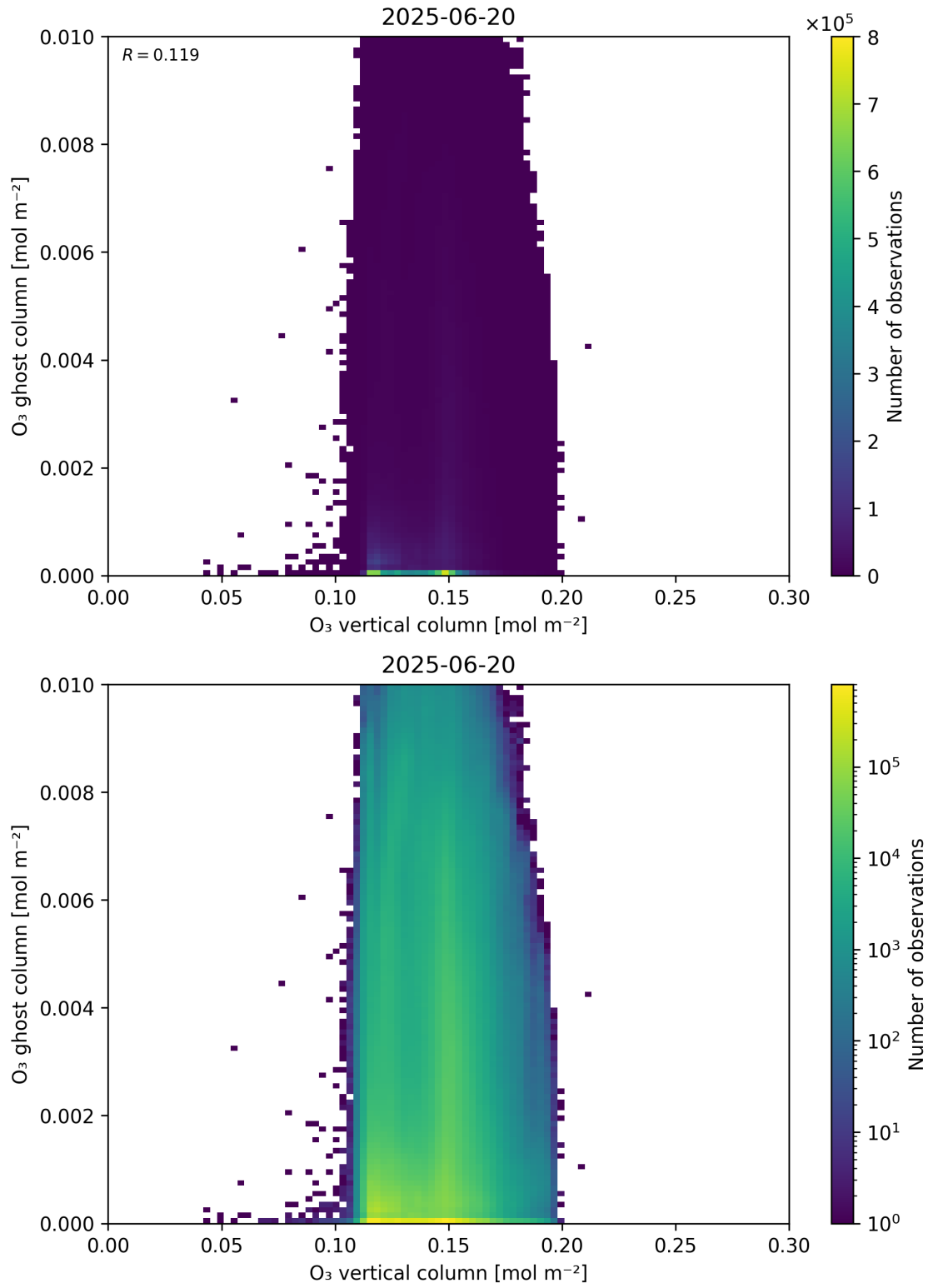
Figure 40: Scatter density plot of “O 3 vertical column” against “O 3 ghost column” for 2025-06-19 to 2025-06-21.
