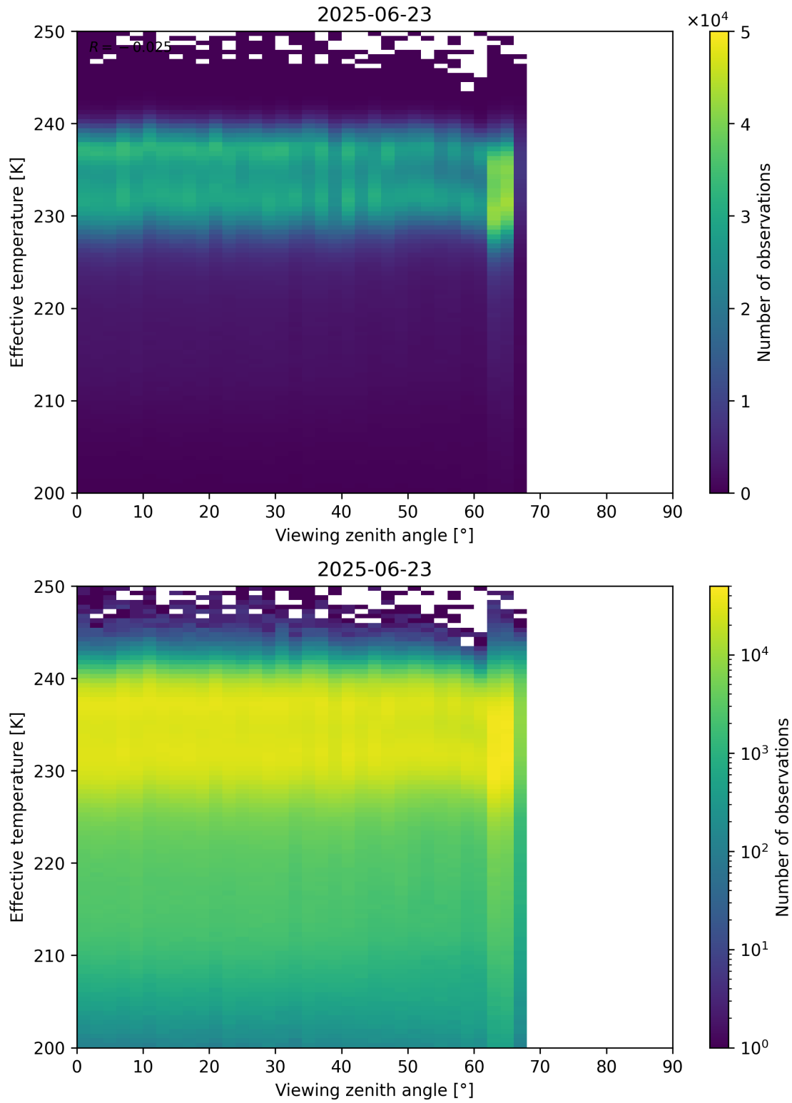
Figure 50: Scatter density plot of “Viewing zenith angle” against “Effective temperature” for 2025-06-22 to 2025-06-24.
