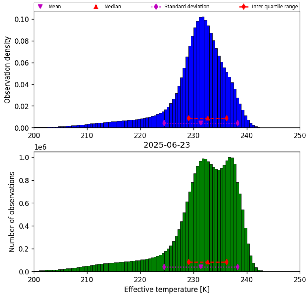
Figure 24: Histogram of “Effective temperature” for 2025-06-22 to 2025-06-24
