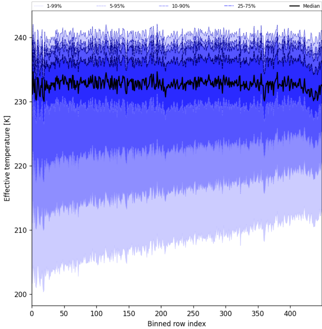
Figure 31: Along track statistics of “Effective temperature” for 2025-06-22 to 2025-06-24
