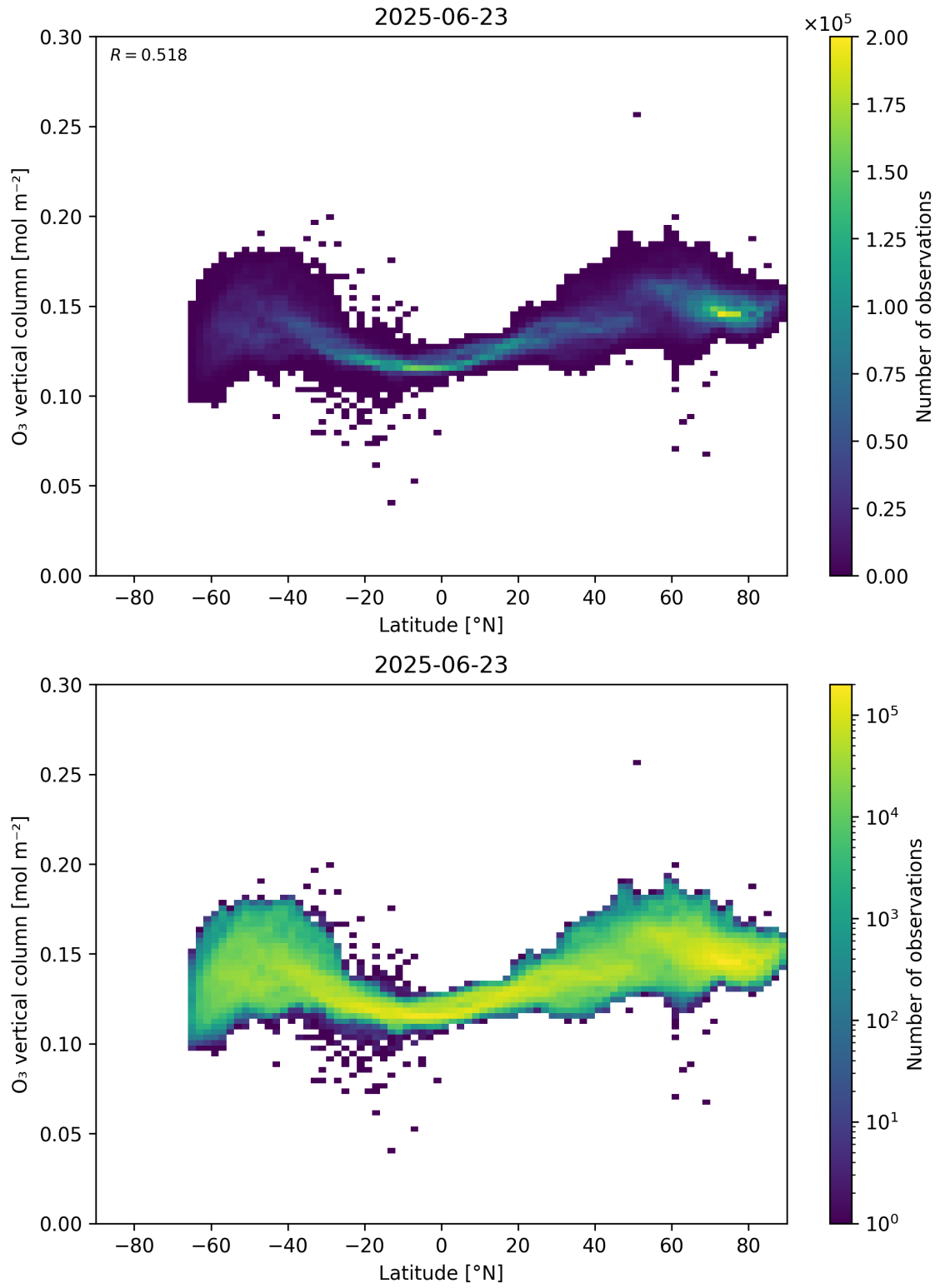
Figure 36: Scatter density plot of “Latitude” against “O 3 vertical column” for 2025-06-22 to 2025-06-24.
