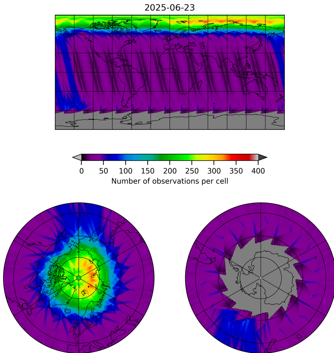
Figure 12: Map of the number of observations for 2025-06-22 to 2025-06-24
