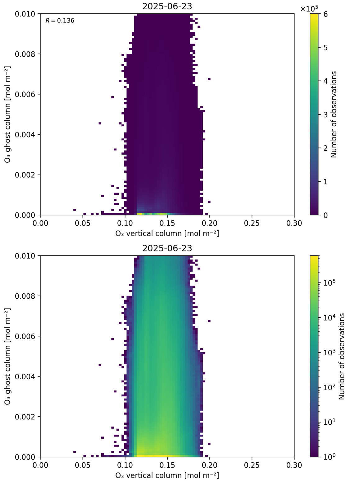
Figure 40: Scatter density plot of “O 3 vertical column” against “O 3 ghost column” for 2025-06-22 to 2025-06-24.
