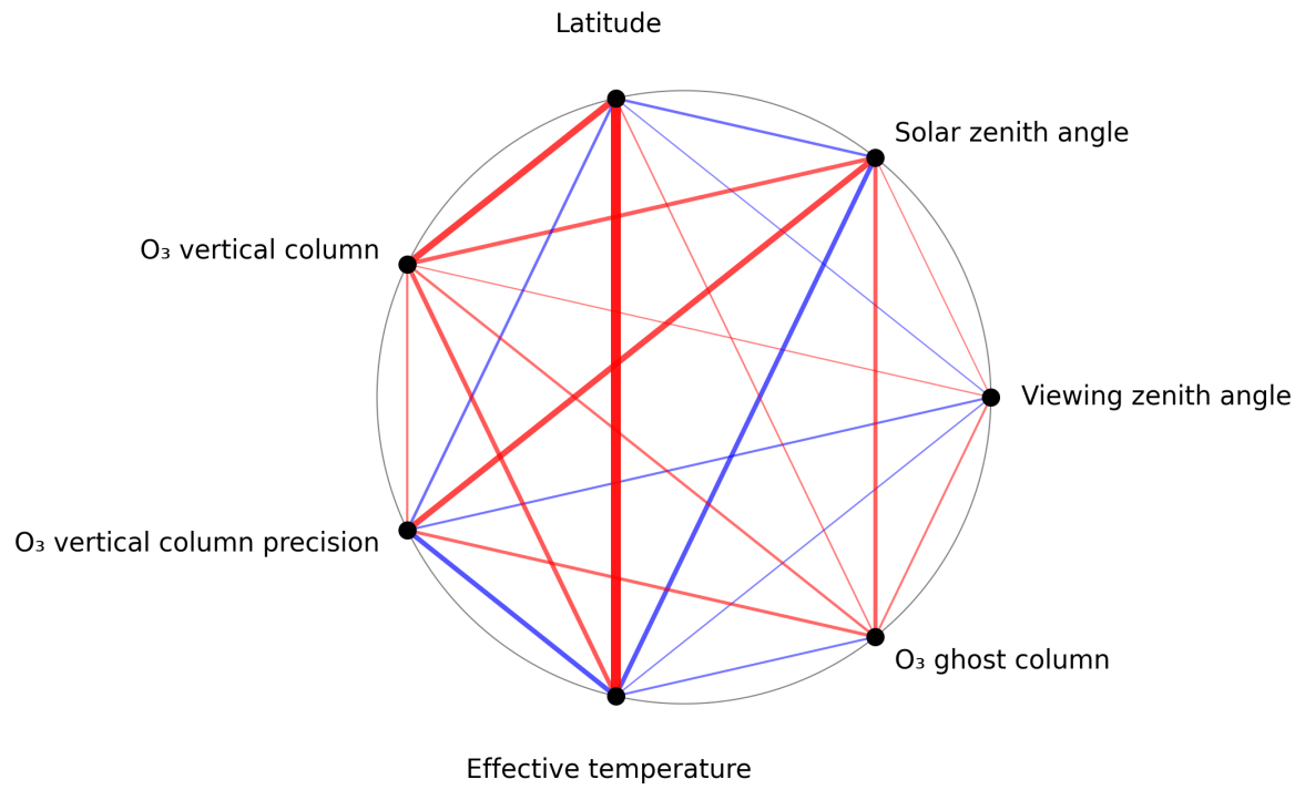
Figure 1: Map of correlation graph for 2025-06-22 to 2025-06-24.
