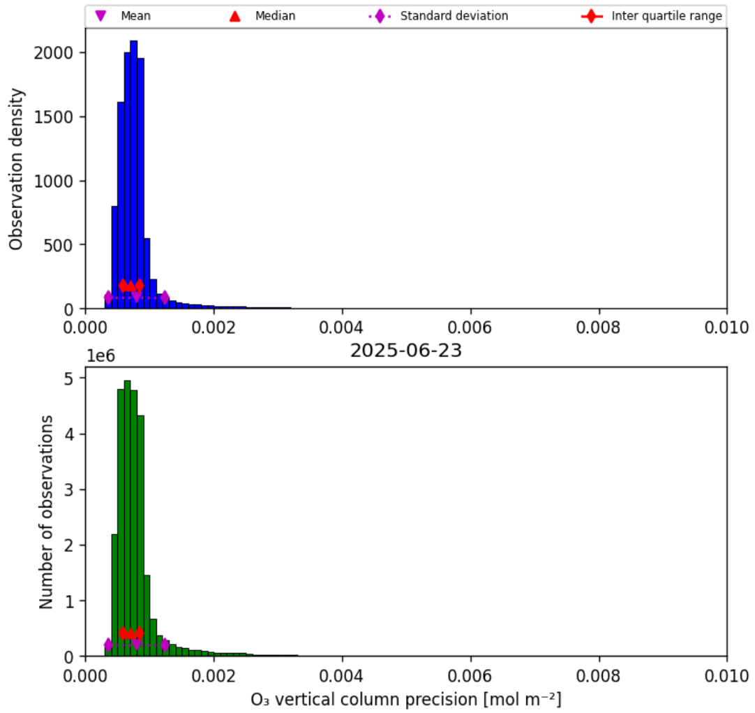
Figure 22: Histogram of “O 3 vertical column precision” for 2025-06-22 to 2025-06-24
