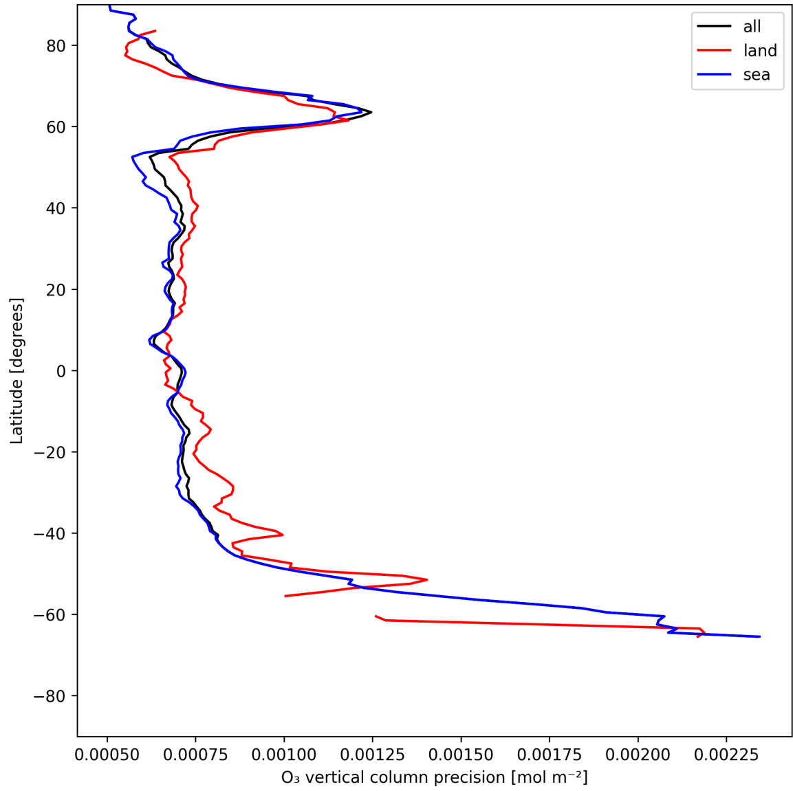
Figure 15: Zonal average of “O 3 vertical column precision” for 2025-06-22 to 2025-06-24.
