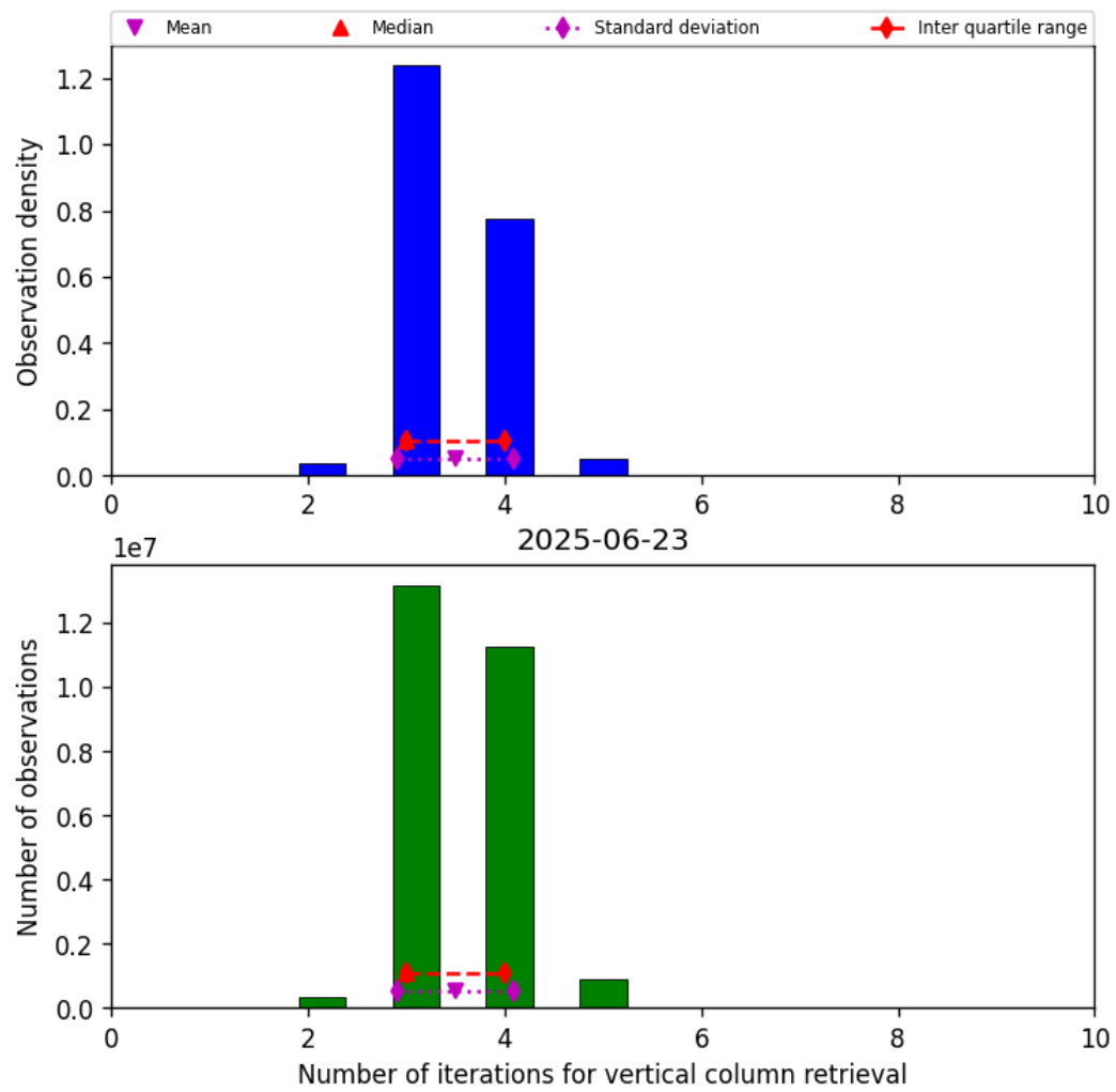
Figure 26: Histogram of “Number of iterations for vertical column retrieval” for 2025-06-22 to 2025-06-24
