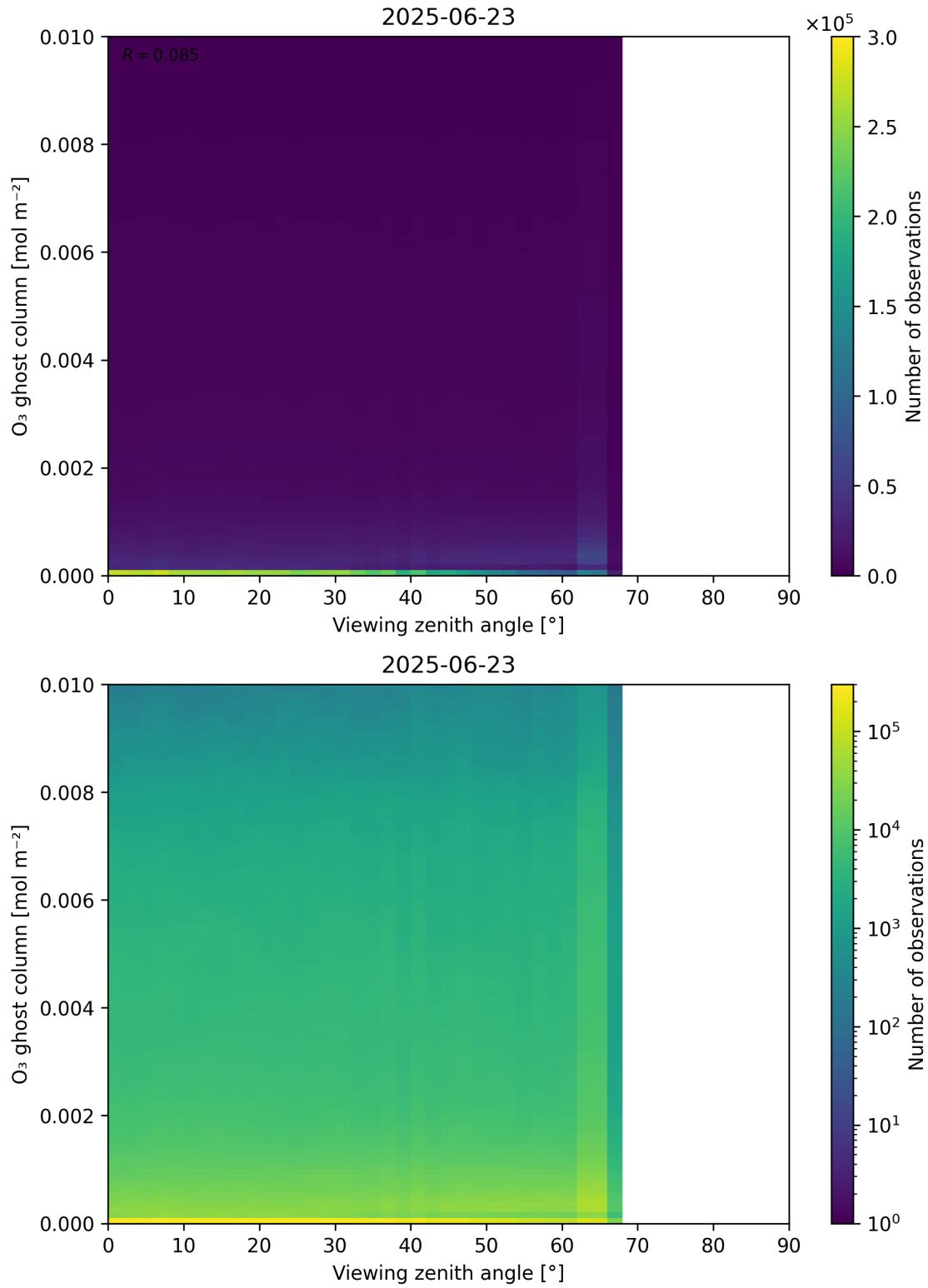
Figure 51: Scatter density plot of “Viewing zenith angle” against “O 3 ghost column” for 2025-06-22 to 2025-06-24.
