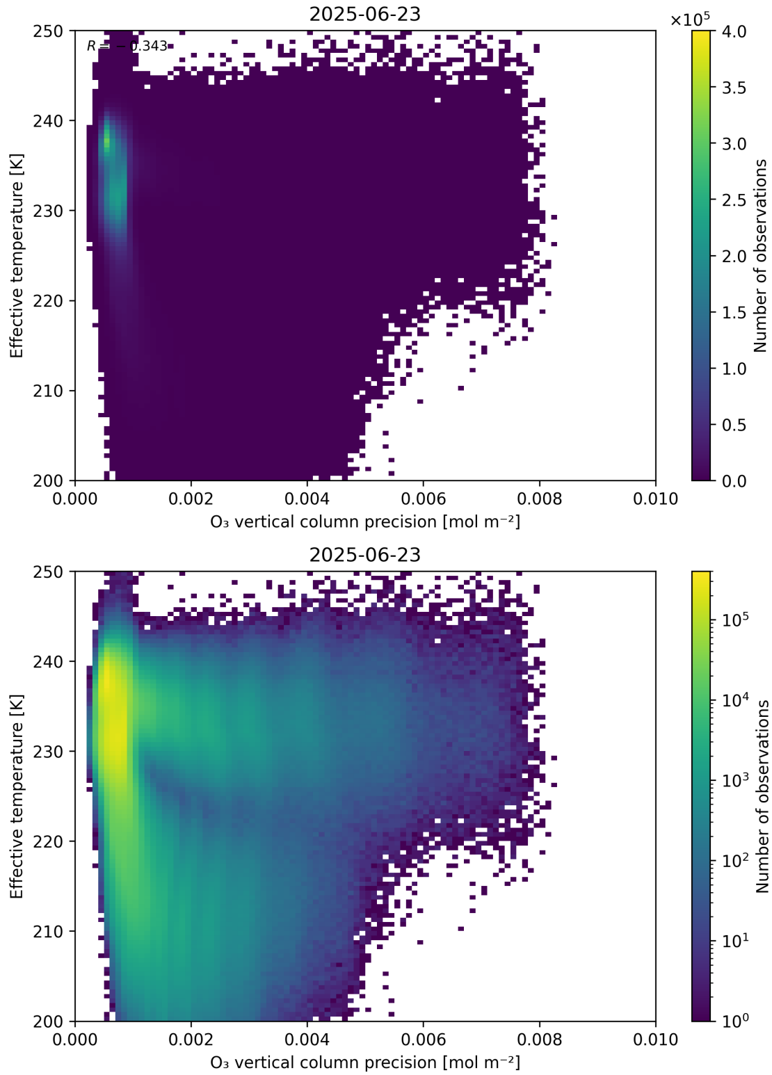
Figure 42: Scatter density plot of “O 3 vertical column precision” against “Effective temperature” for 2025-06-22 to 2025-06-24.
