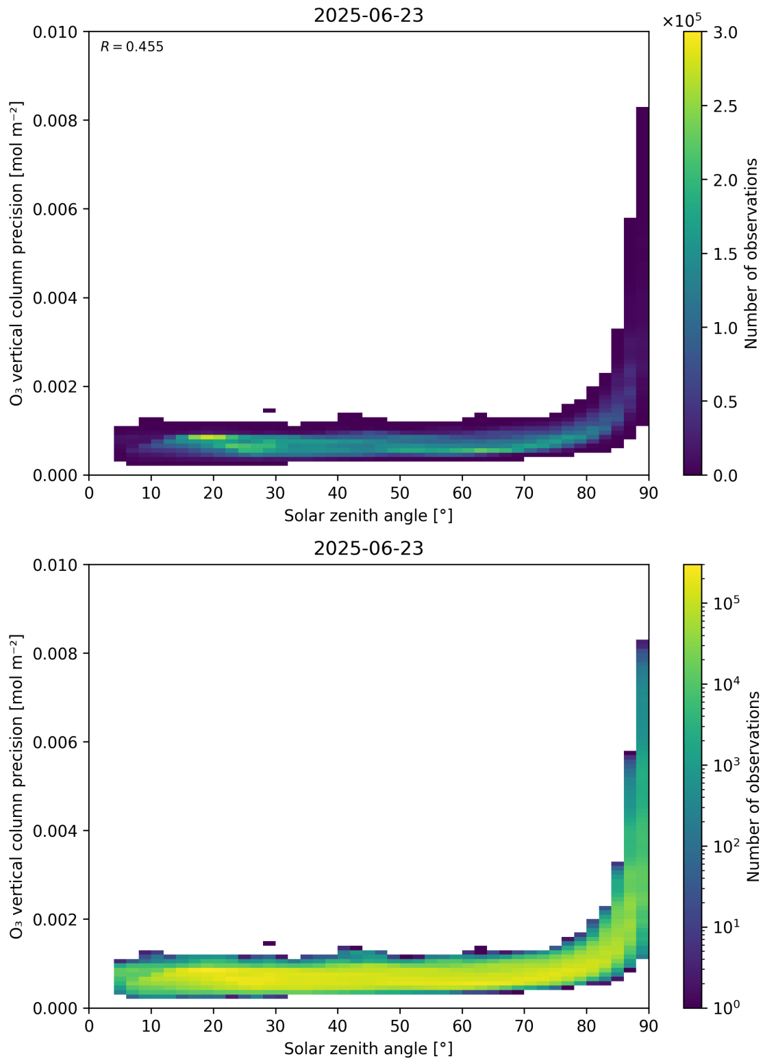
Figure 48: Scatter density plot of “Solar zenith angle” against “O 3 vertical column precision” for 2025-06-22 to 2025-06-24.
