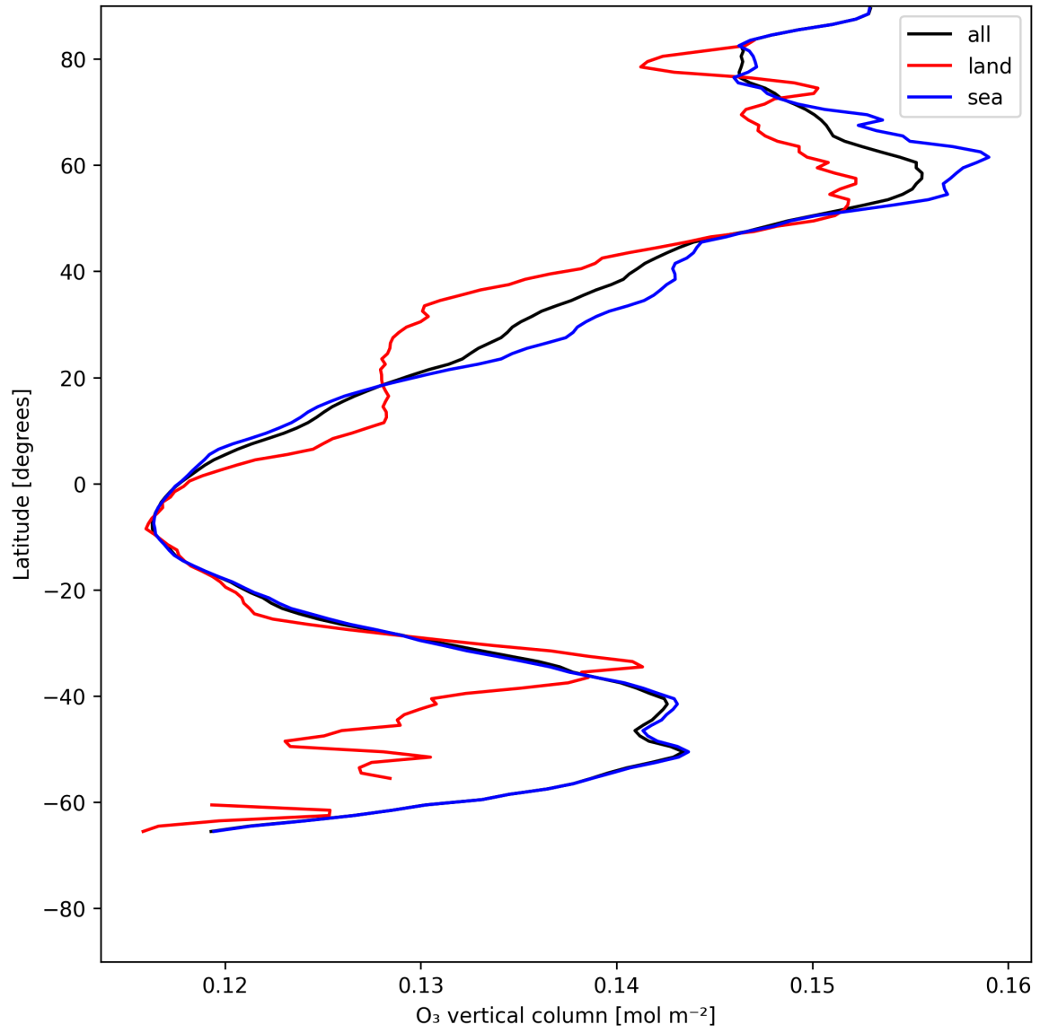
Figure 14: Zonal average of “O 3 vertical column” for 2025-06-22 to 2025-06-24.
