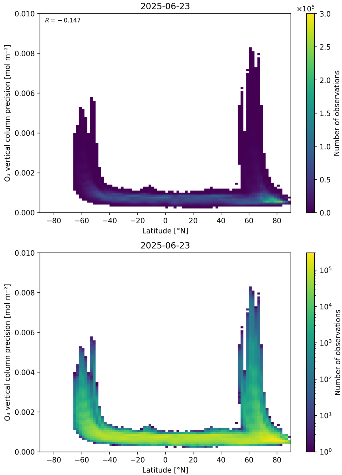
Figure 37: Scatter density plot of “Latitude” against “O 3 vertical column precision” for 2025-06-22 to 2025-06-24.
