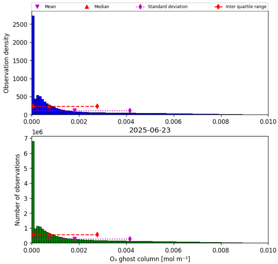
Figure 25: Histogram of “O 3 ghost column” for 2025-06-22 to 2025-06-24
