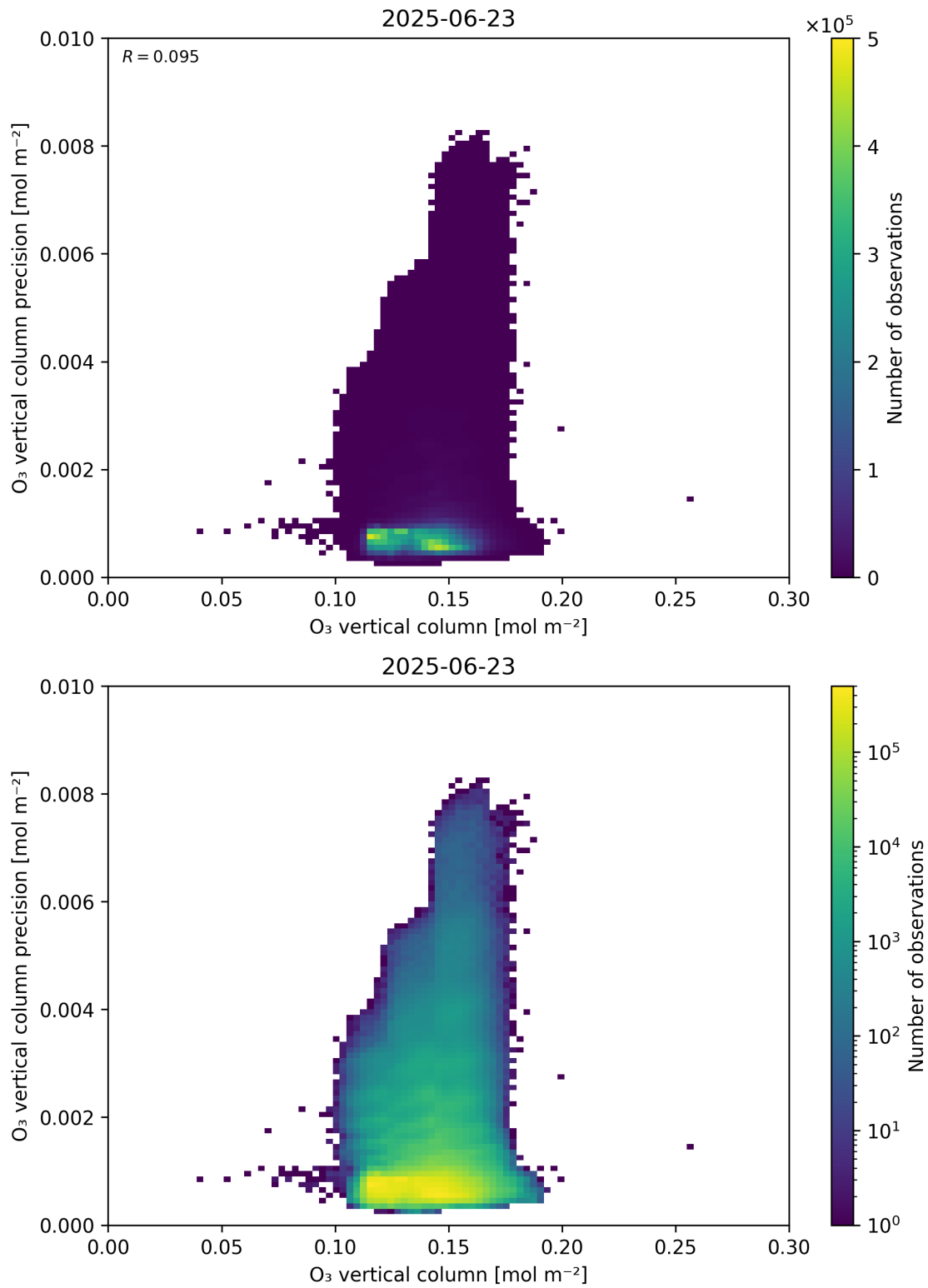
Figure 41: Scatter density plot of “O 3 vertical column” against “O 3 vertical column precision” for 2025-06-22 to 2025-06-24.
