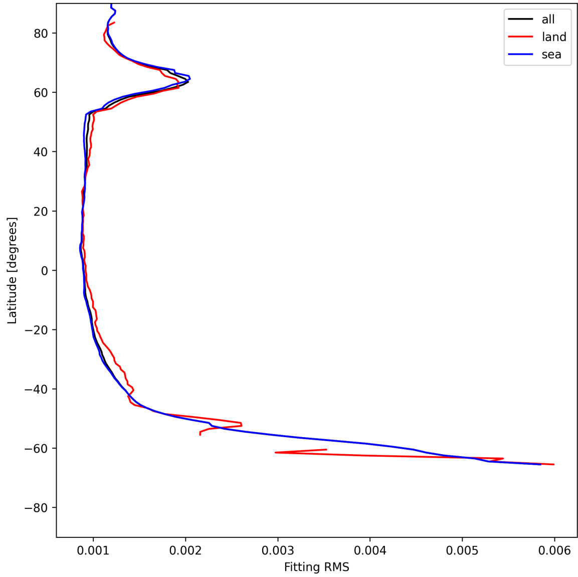
Figure 16: Zonal average of “Fitting RMS” for 2025-06-22 to 2025-06-24.
