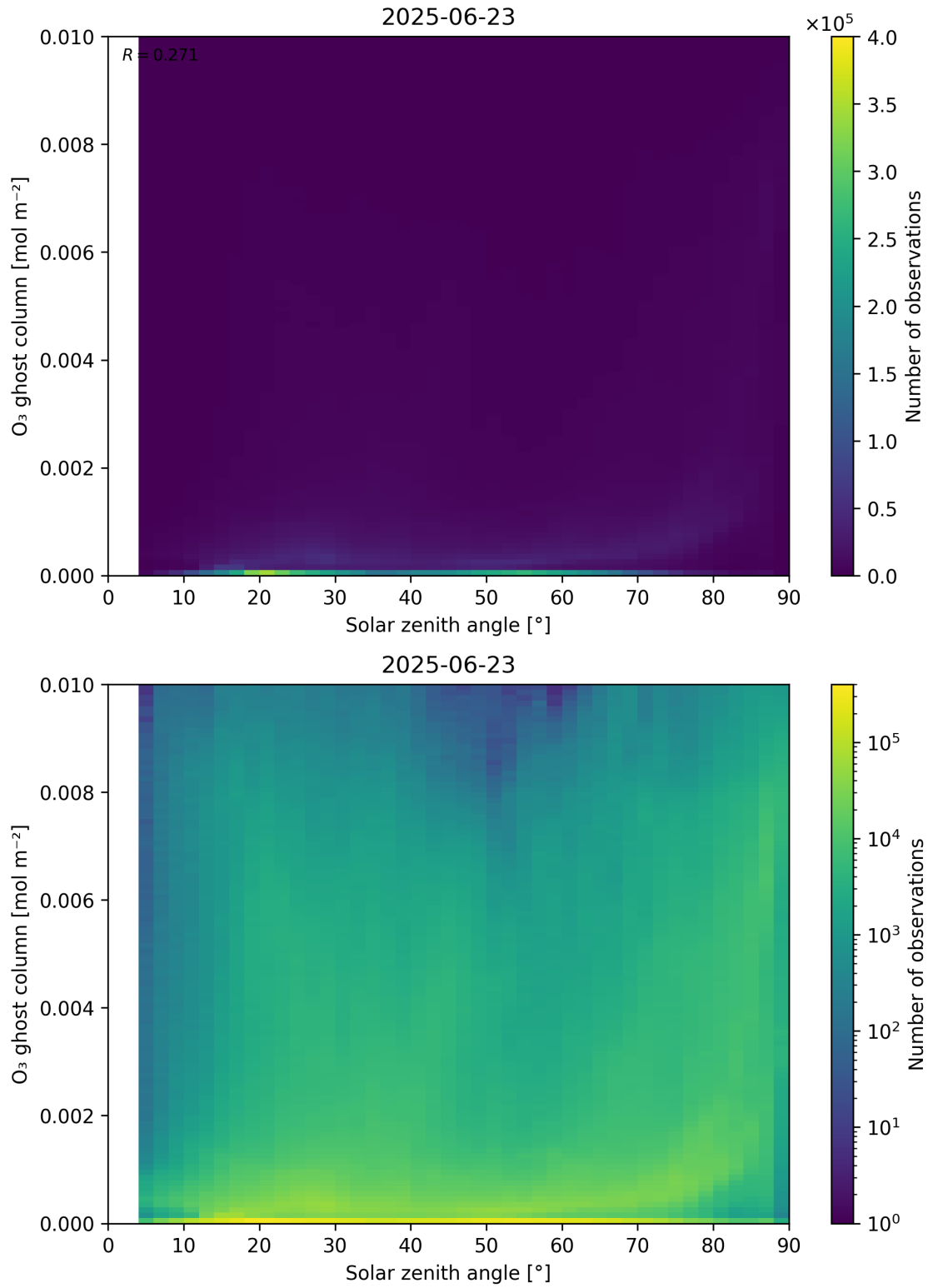
Figure 46: Scatter density plot of “Solar zenith angle” against “O 3 ghost column” for 2025-06-22 to 2025-06-24.
