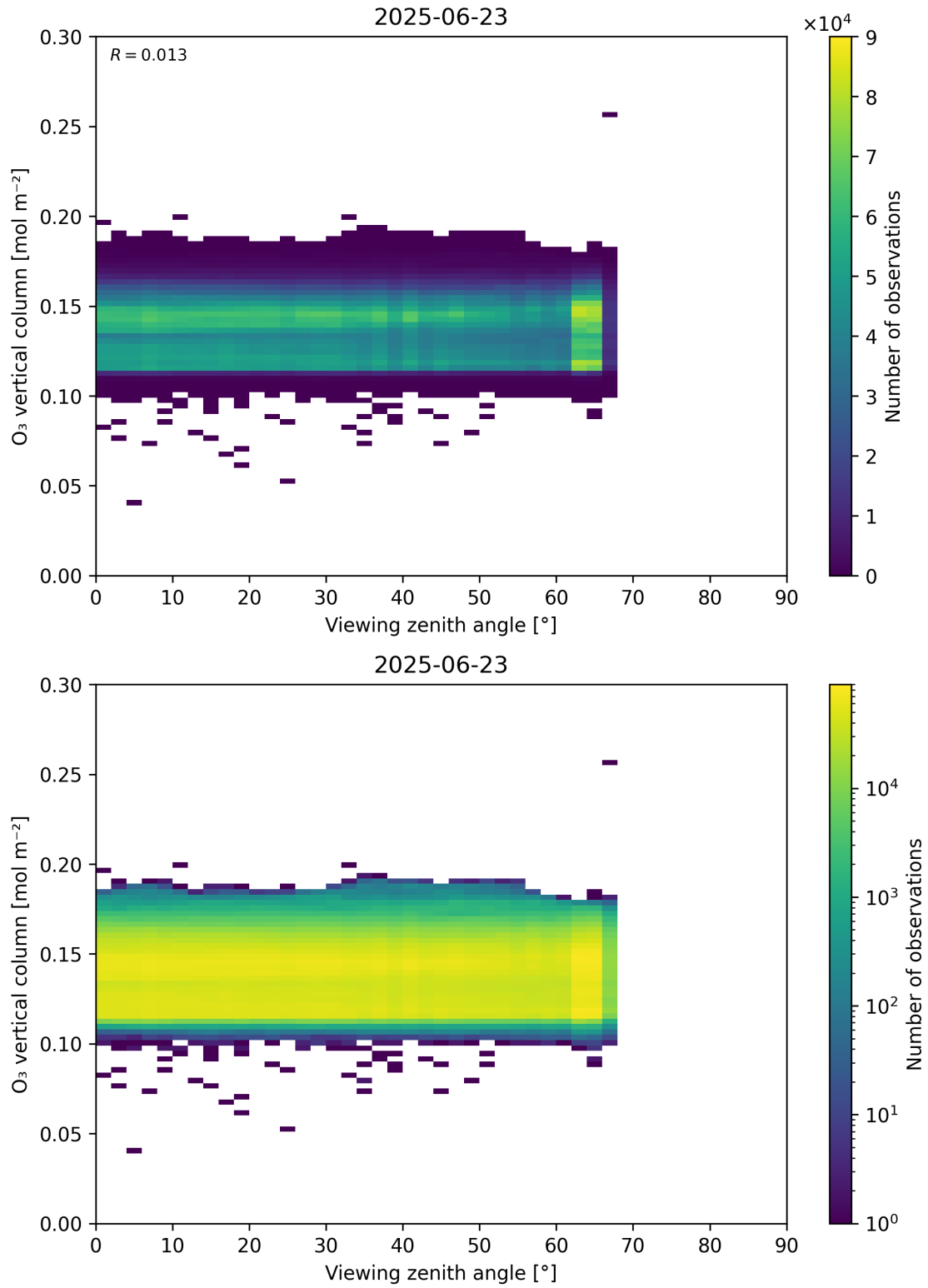
Figure 52: Scatter density plot of “Viewing zenith angle” against “O 3 vertical column” for 2025-06-22 to 2025-06-24.
