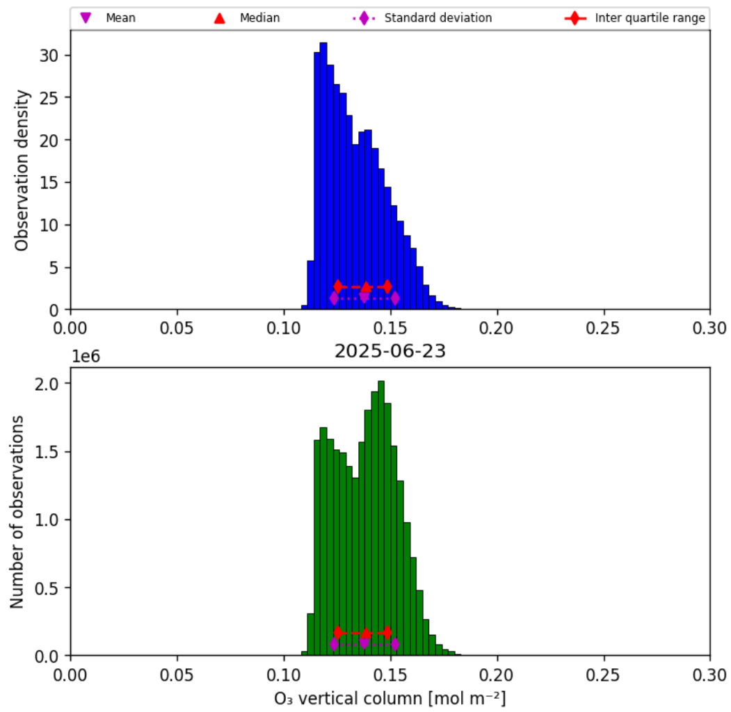
Figure 21: Histogram of “O 3 vertical column” for 2025-06-22 to 2025-06-24
