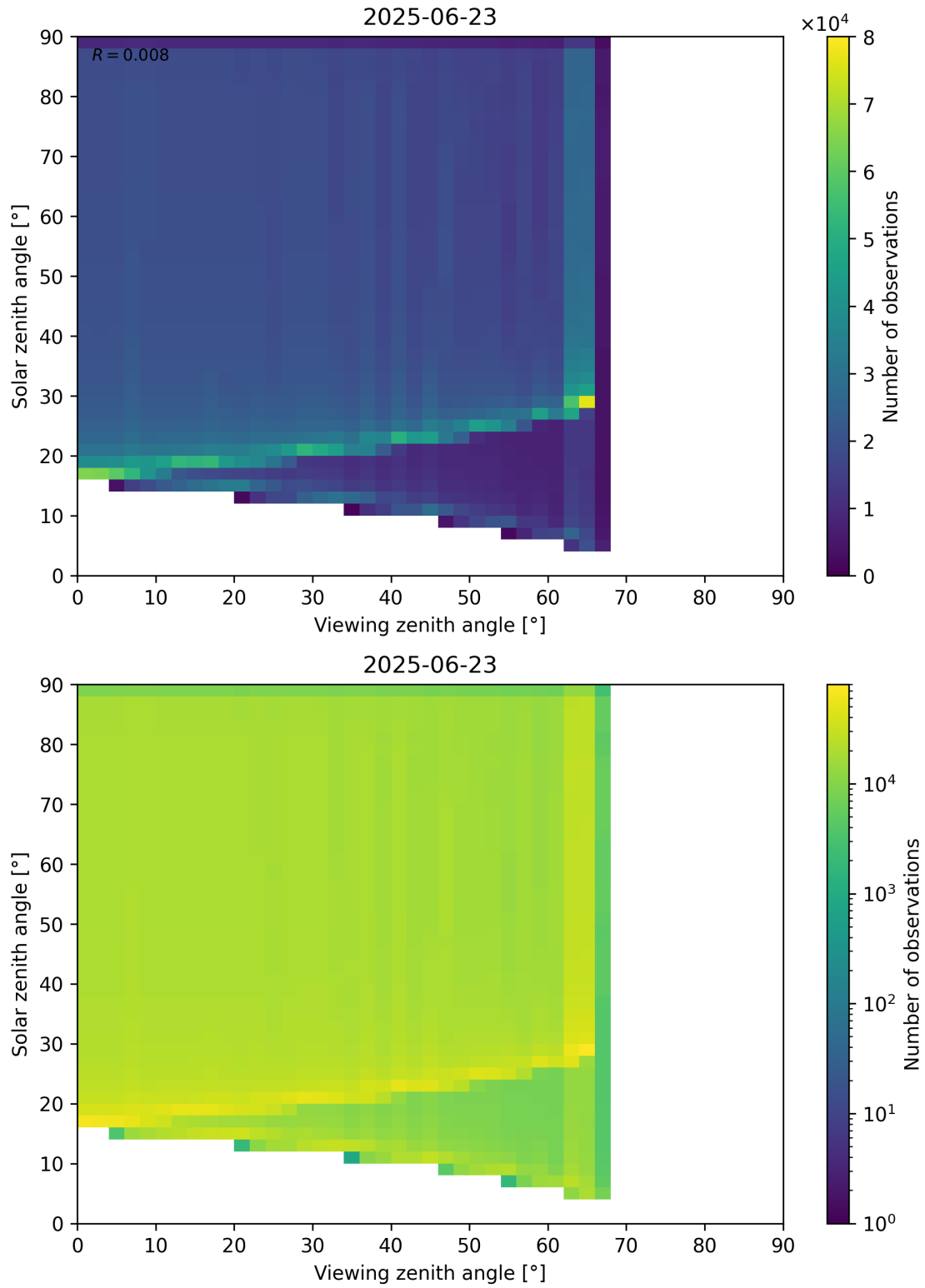
Figure 54: Scatter density plot of “Viewing zenith angle” against “Solar zenith angle” for 2025-06-22 to 2025-06-24.
