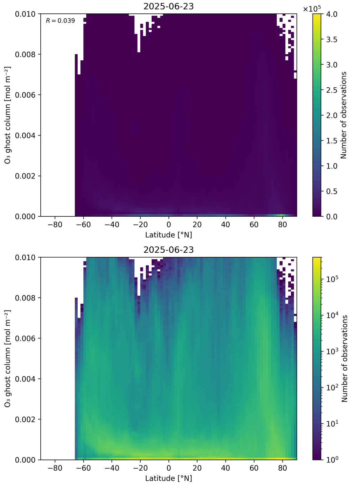
Figure 35: Scatter density plot of “Latitude” against “O 3 ghost column” for 2025-06-22 to 2025-06-24.
