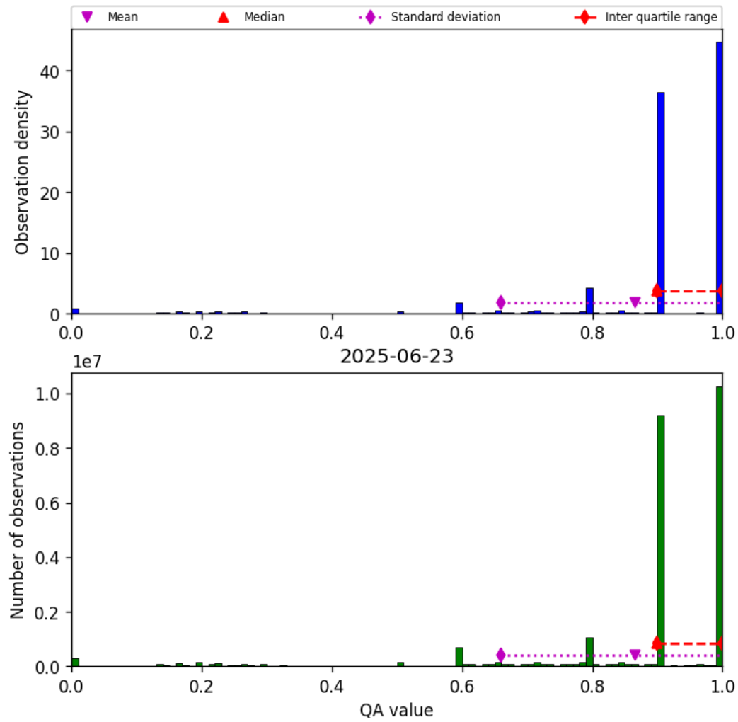
Figure 20: Histogram of “QA value” for 2025-06-22 to 2025-06-24
