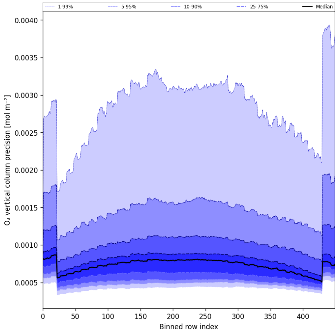
Figure 29: Along track statistics of “O 3 vertical column precision” for 2025-06-22 to 2025-06-24
