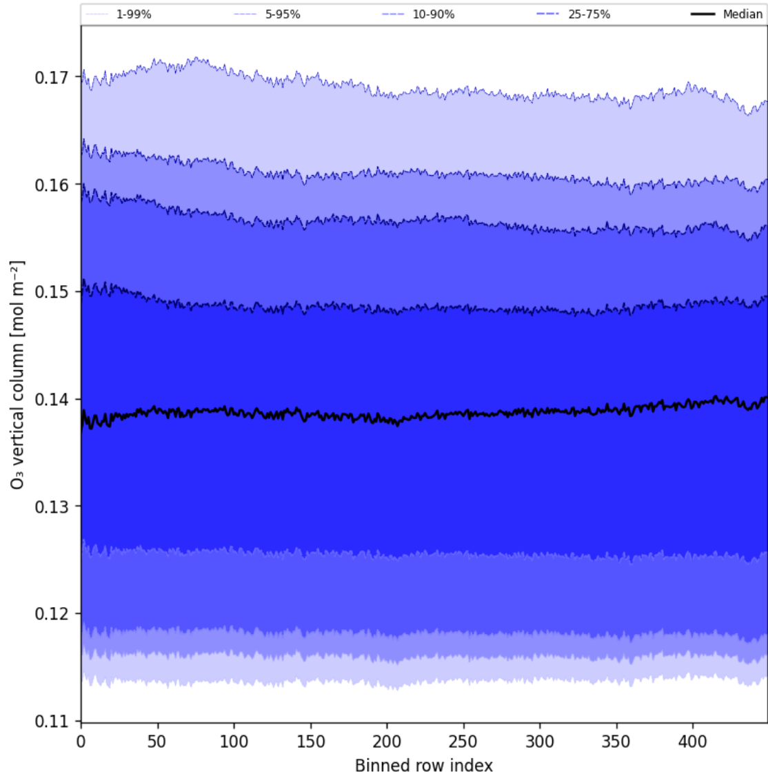
Figure 28: Along track statistics of “O 3 vertical column” for 2025-06-22 to 2025-06-24
