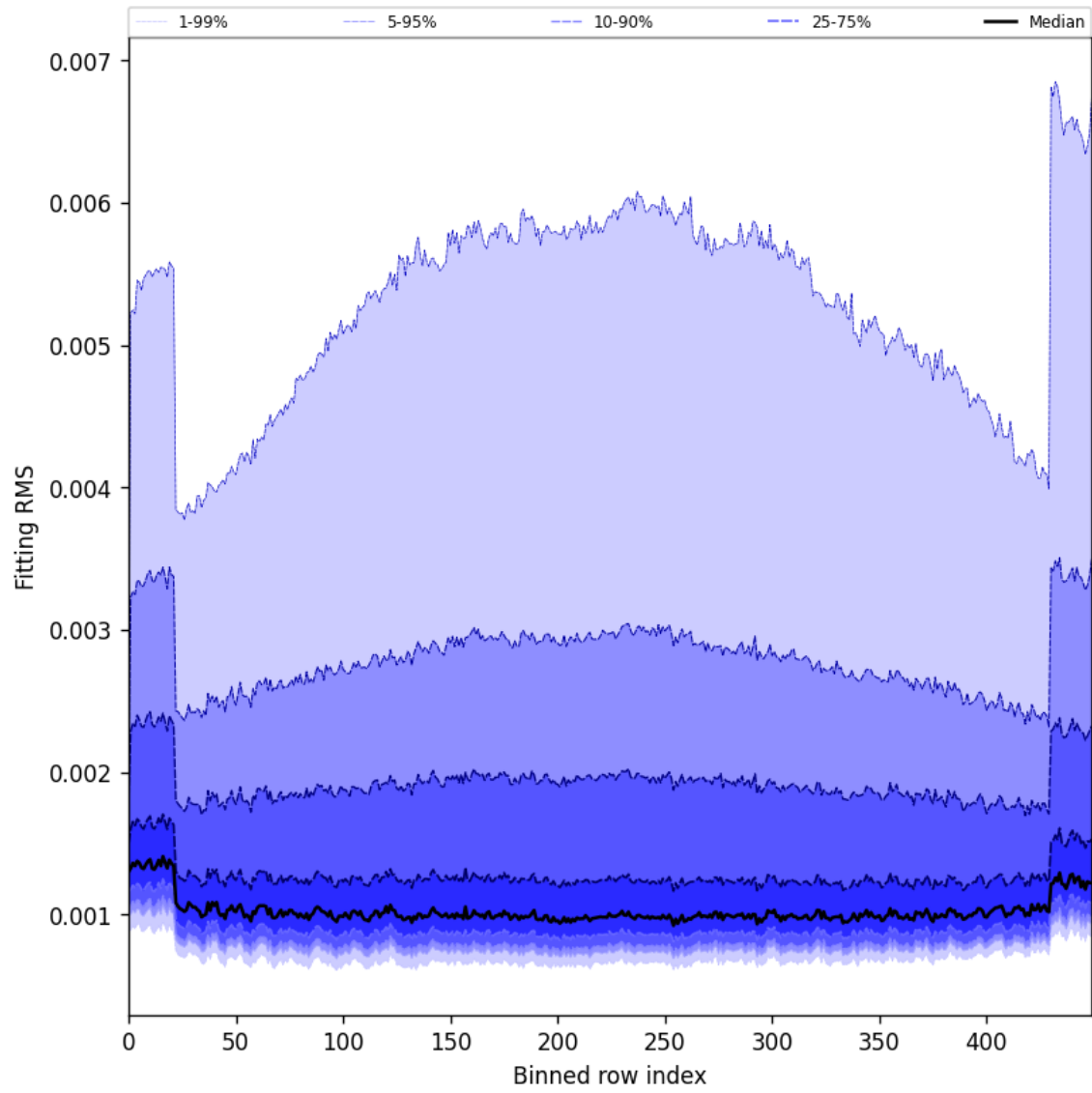
Figure 30: Along track statistics of “Fitting RMS” for 2025-06-22 to 2025-06-24
