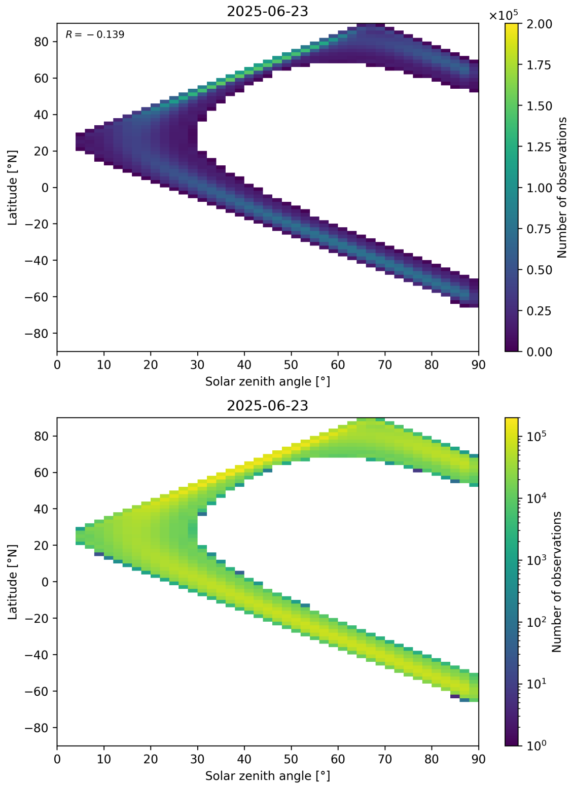
Figure 44: Scatter density plot of “Solar zenith angle” against “Latitude” for 2025-06-22 to 2025-06-24.
