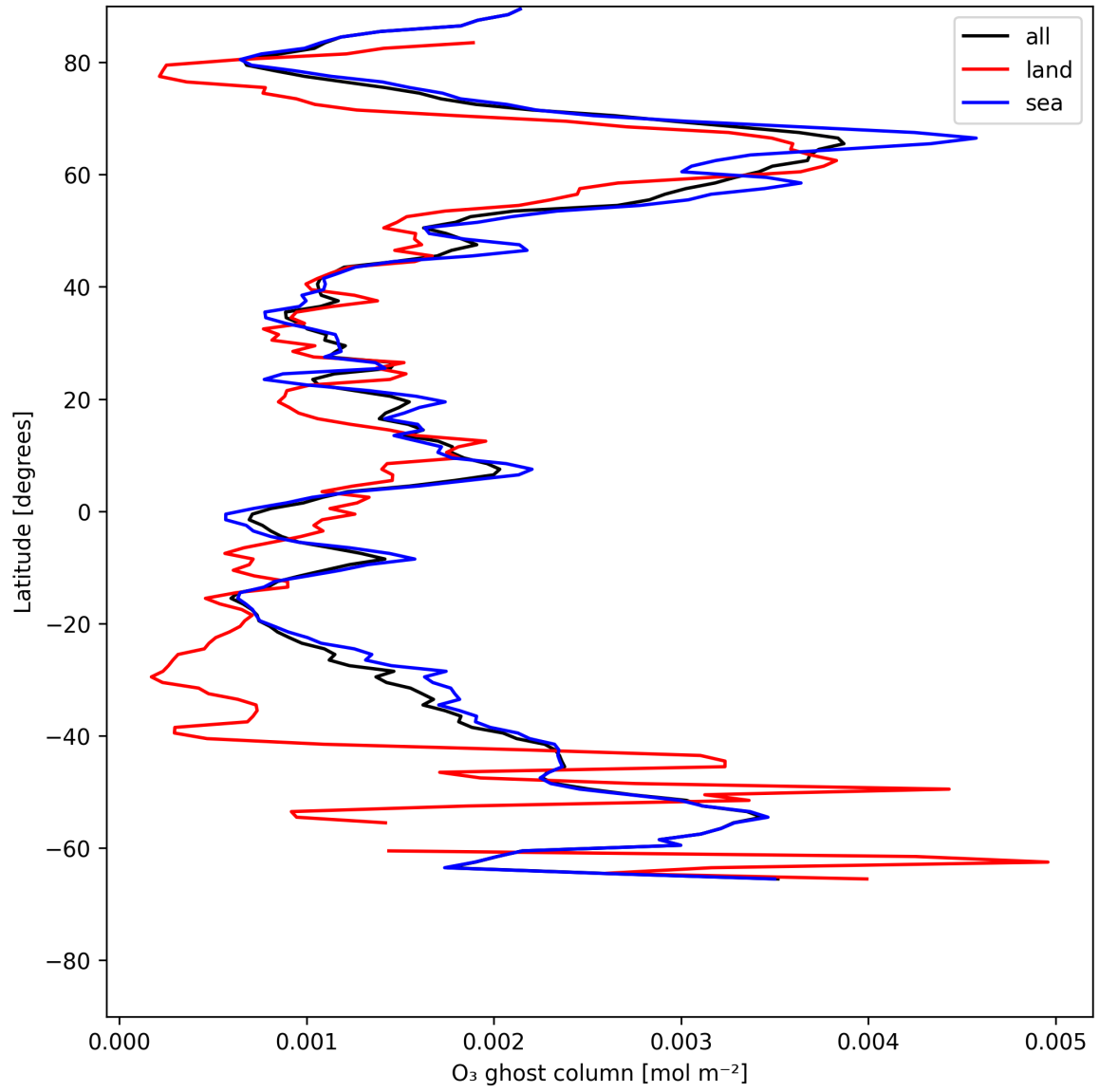
Figure 18: Zonal average of "O 3 ghost column" for 2025-06-22 to 2025-06-24.
