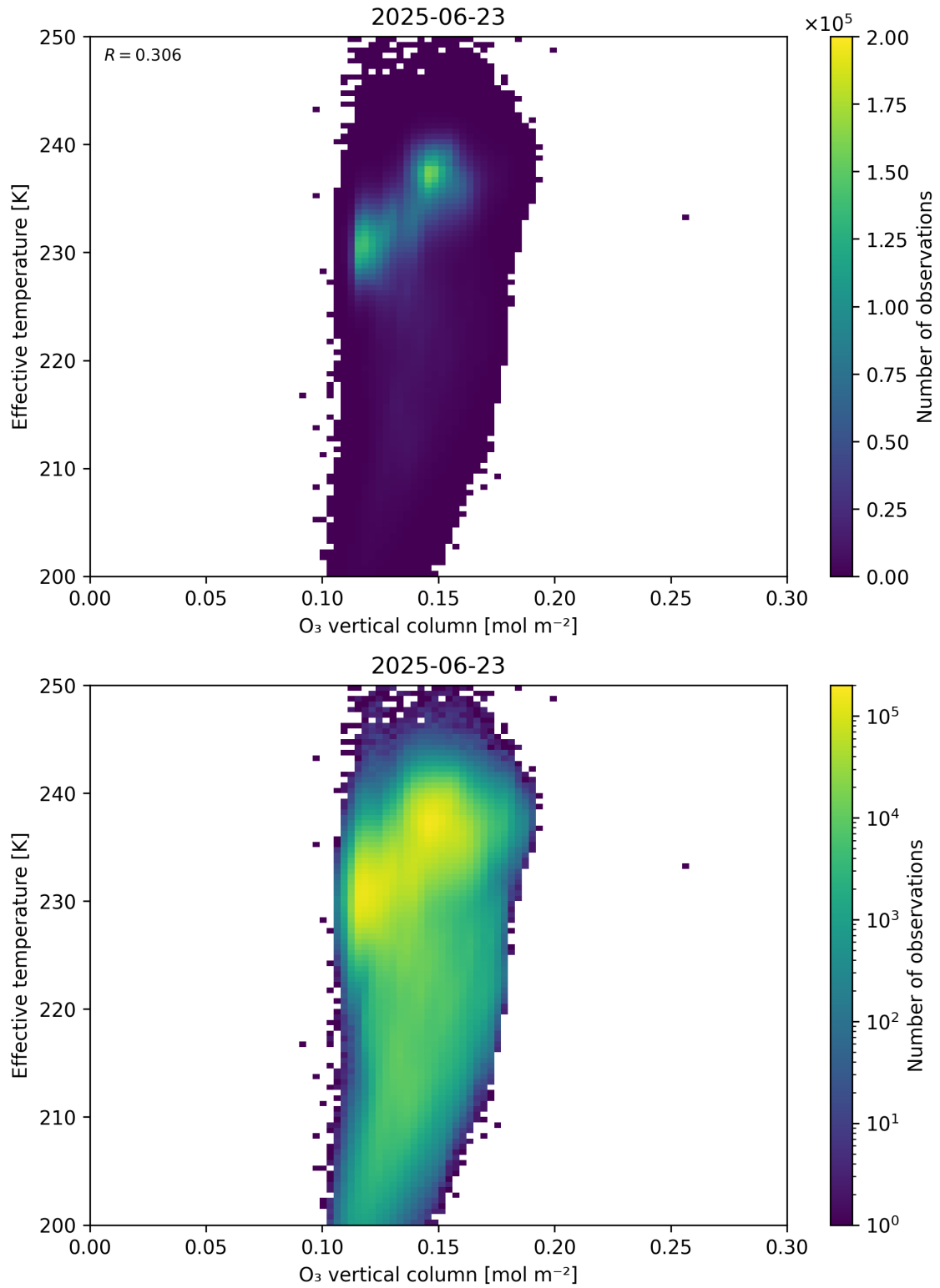
Figure 39: Scatter density plot of “O 3 vertical column” against “Effective temperature” for 2025-06-22 to 2025-06-24.
