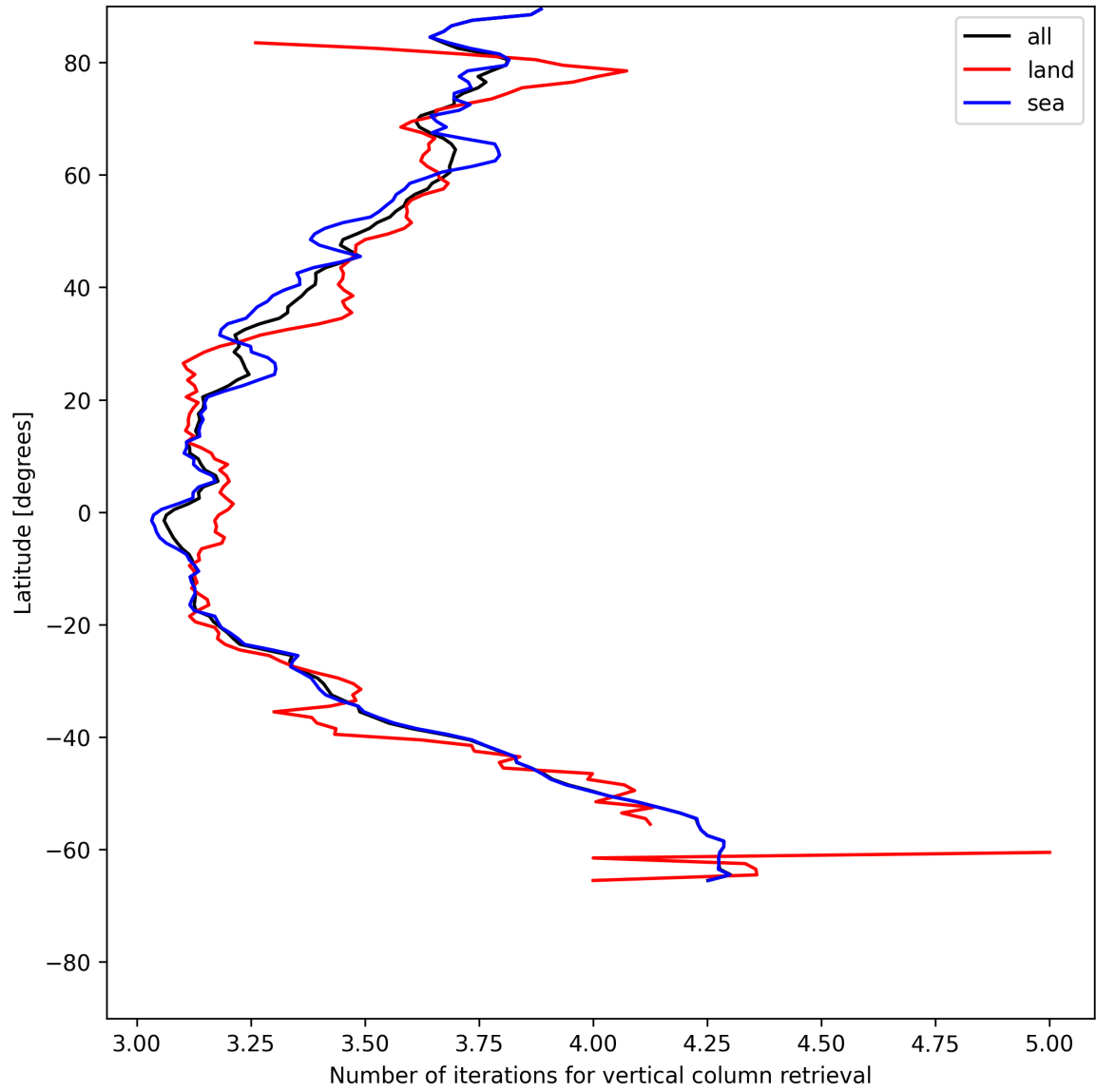
Figure 19: Zonal average of “Number of iterations for vertical column retrieval” for 2025-06-22 to 2025-06-24.
