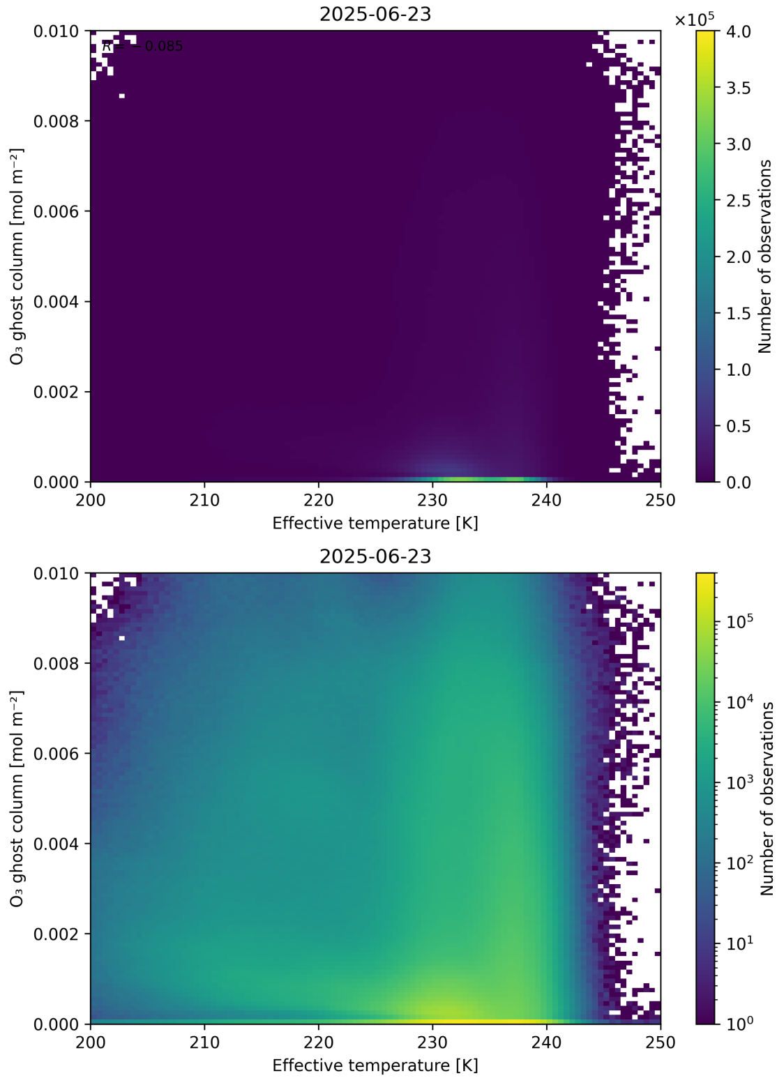
Figure 38: Scatter density plot of “Effective temperature” against “O 3 ghost column” for 2025-06-22 to 2025-06-24.
