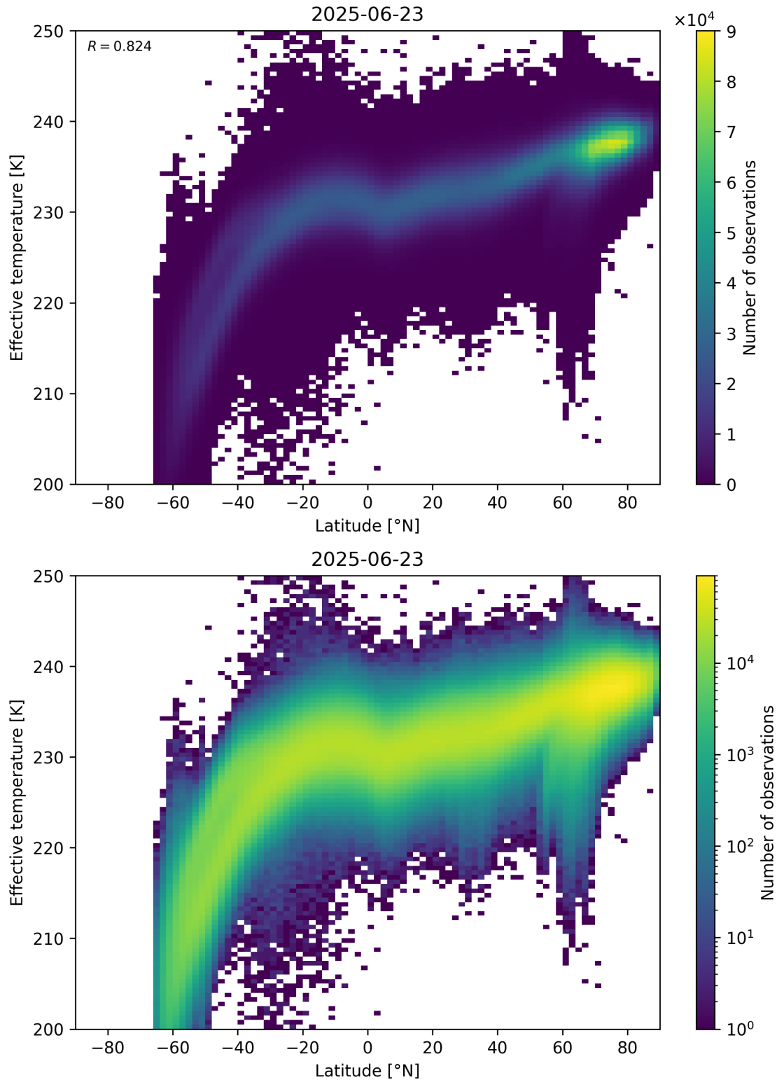
Figure 34: Scatter density plot of “Latitude” against “Effective temperature” for 2025-06-22 to 2025-06-24.
