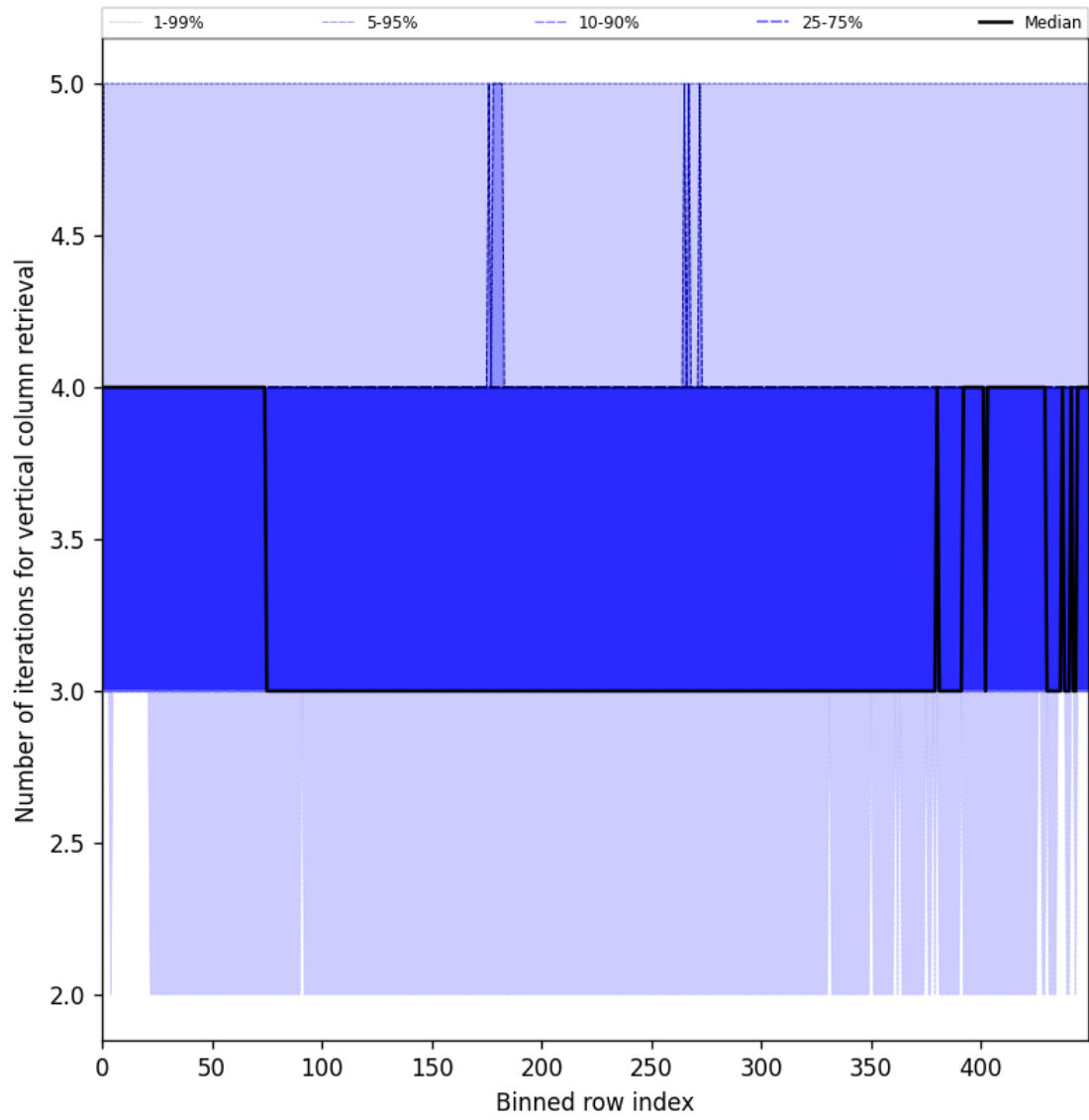
Figure 33: Along track statistics of “Number of iterations for vertical column retrieval” for 2025-06-22 to 2025-06-24
