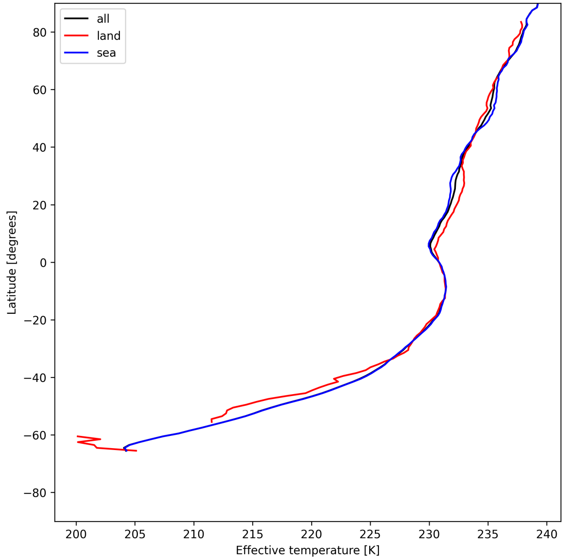
Figure 17: Zonal average of "Effective temperature" for 2025-06-22 to 2025-06-24.
