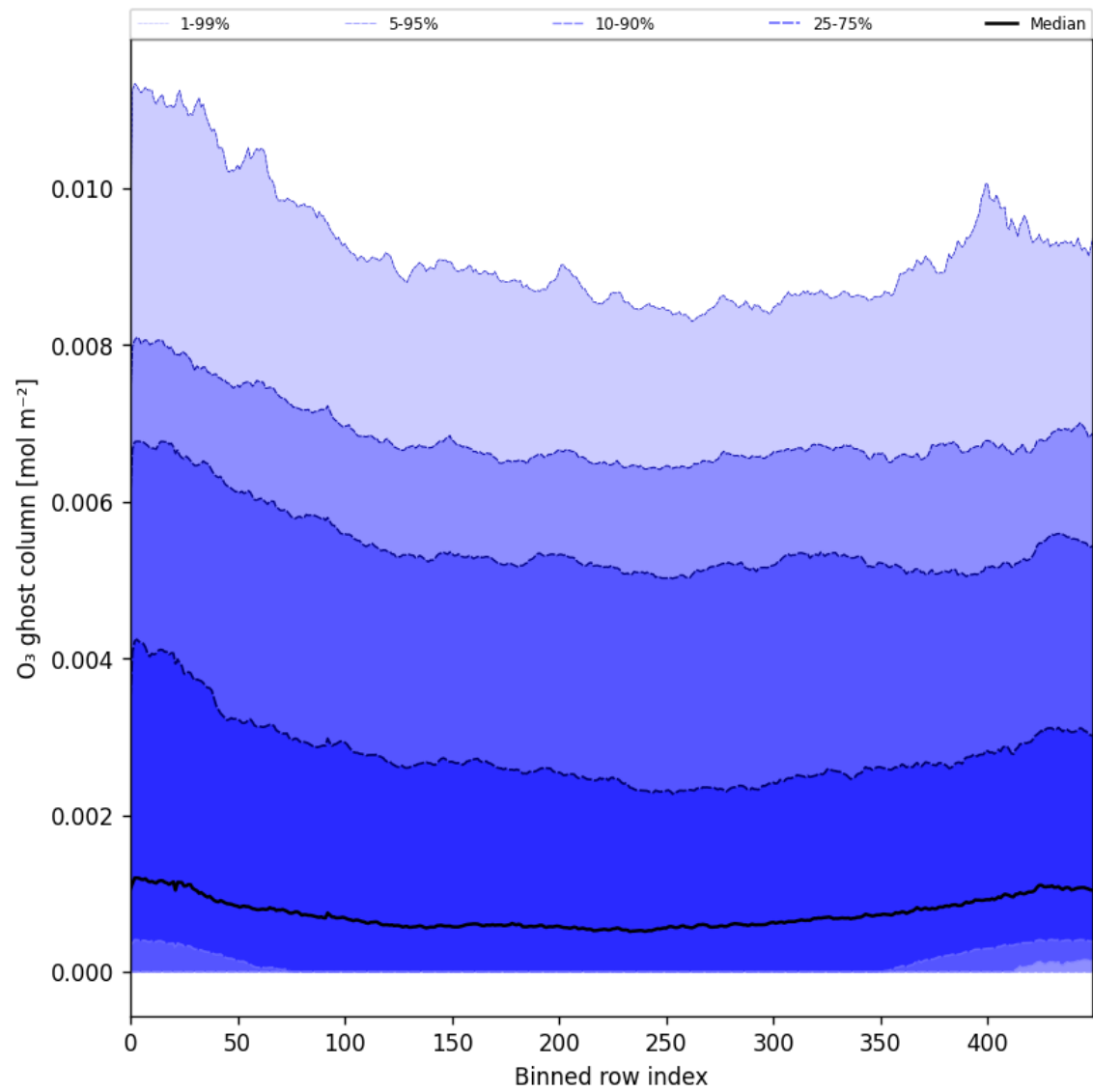
Figure 32: Along track statistics of “O 3 ghost column” for 2025-06-22 to 2025-06-24
