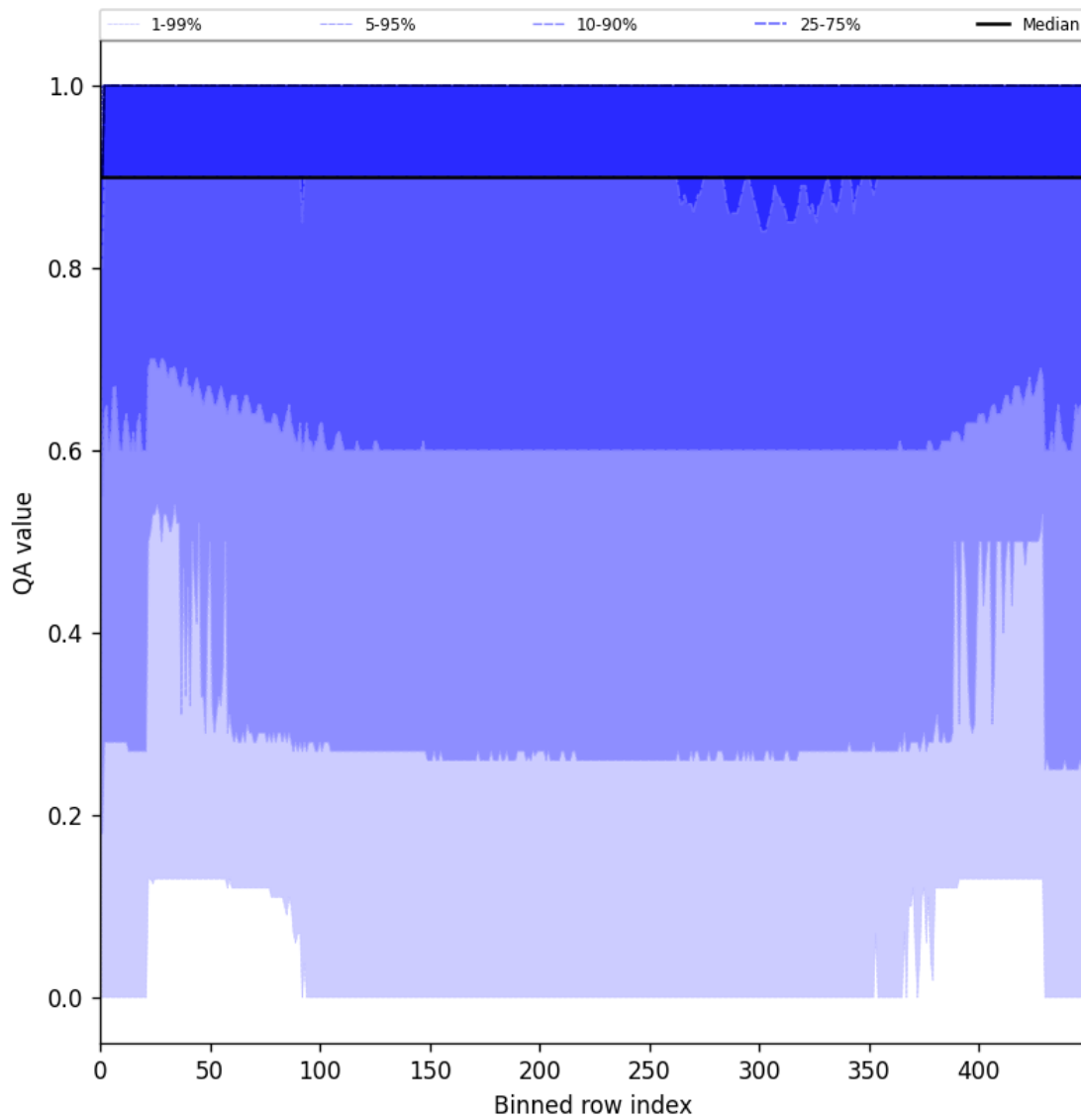
Figure 27: Along track statistics of “QA value” for 2025-06-22 to 2025-06-24
