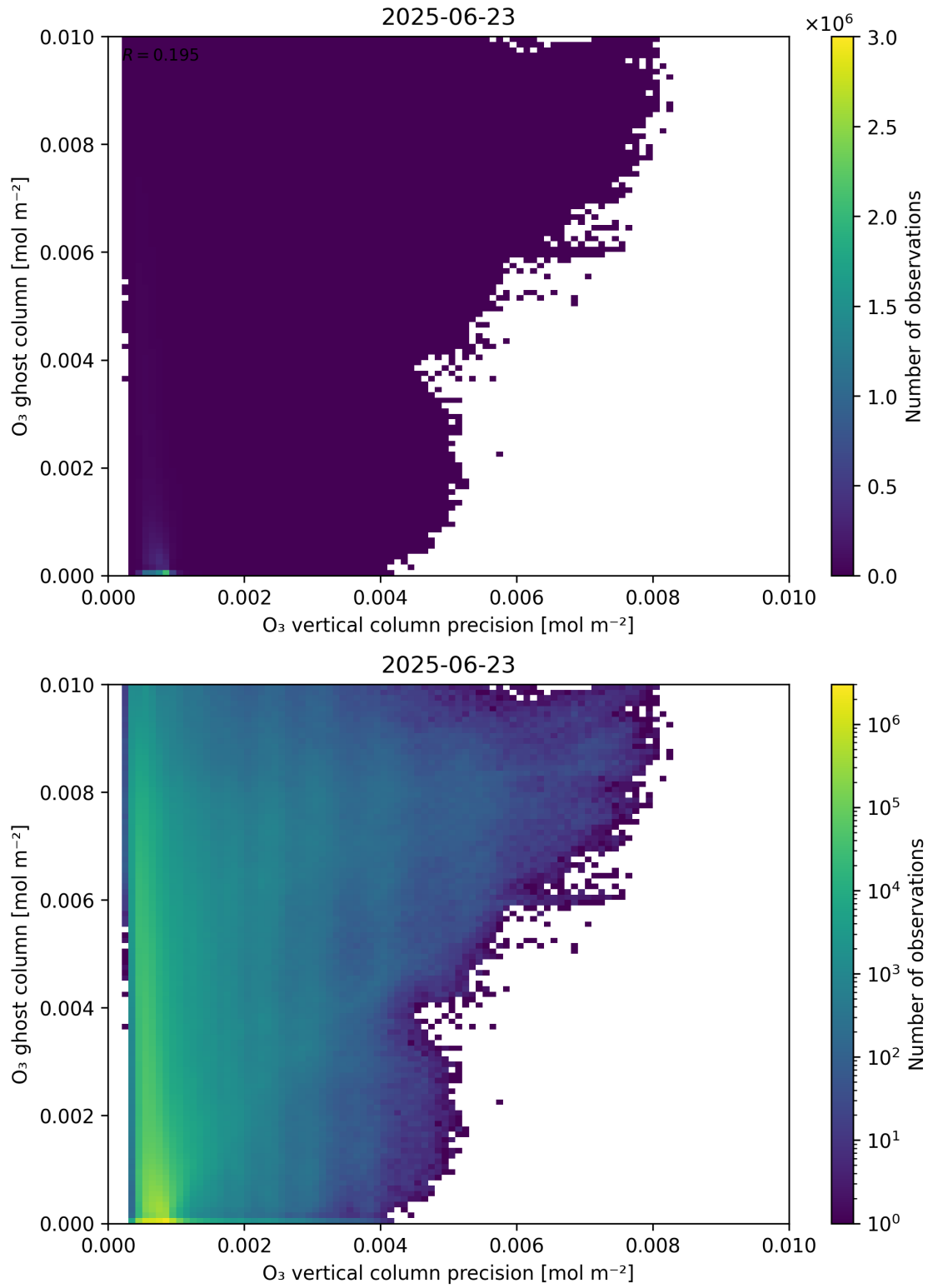
Figure 43: Scatter density plot of “ O_3 vertical column precision” against “ O_3 ghost column” for 2025-06-22 to 2025-06-24.
