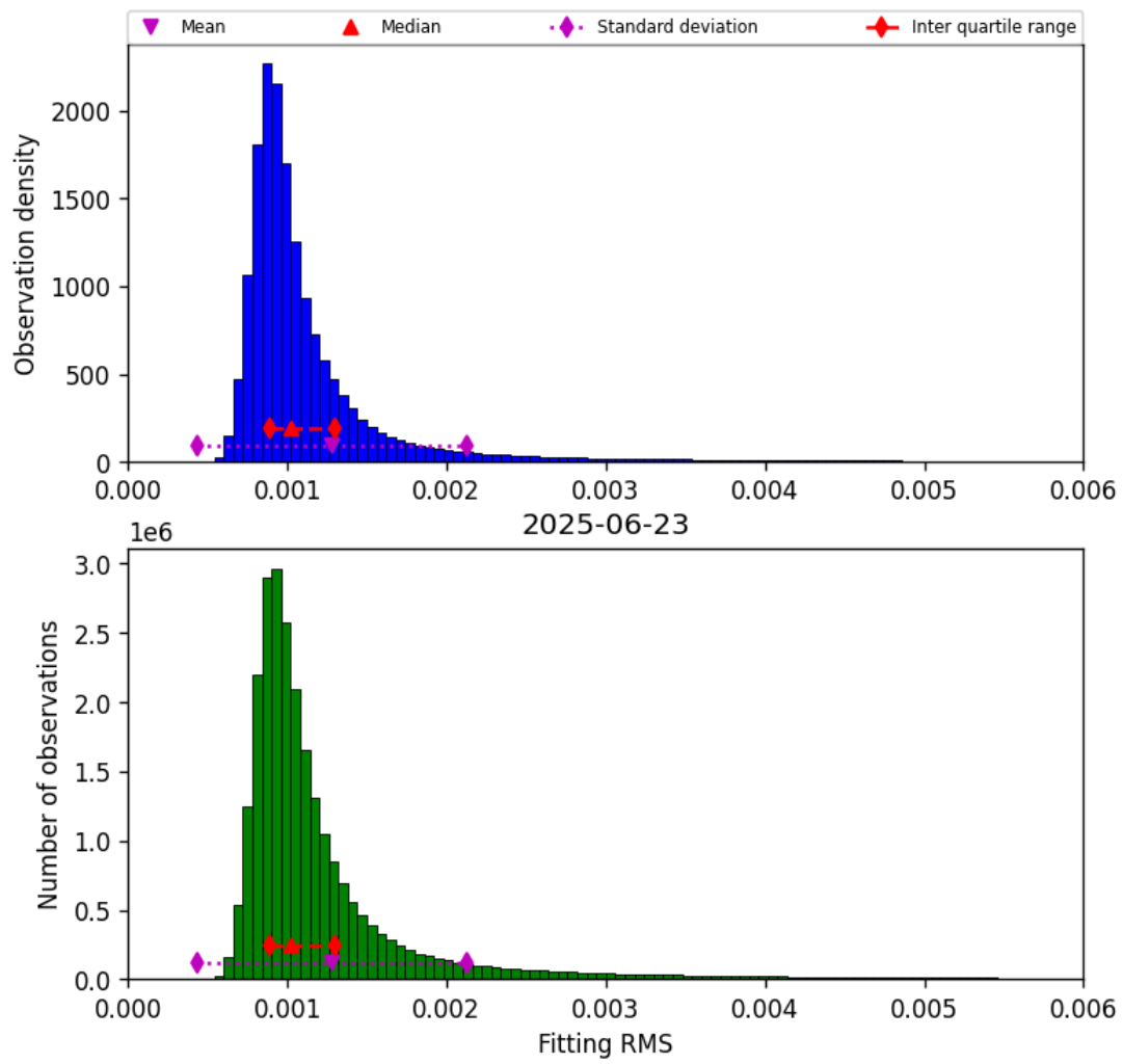
Figure 23: Histogram of “Fitting RMS” for 2025-06-22 to 2025-06-24
