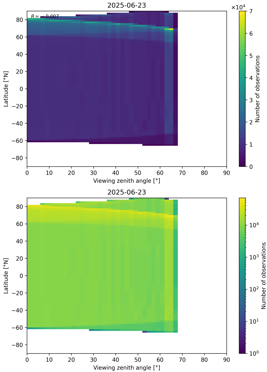
Figure 49: Scatter density plot of “Viewing zenith angle” against “Latitude” for 2025-06-22 to 2025-06-24.
