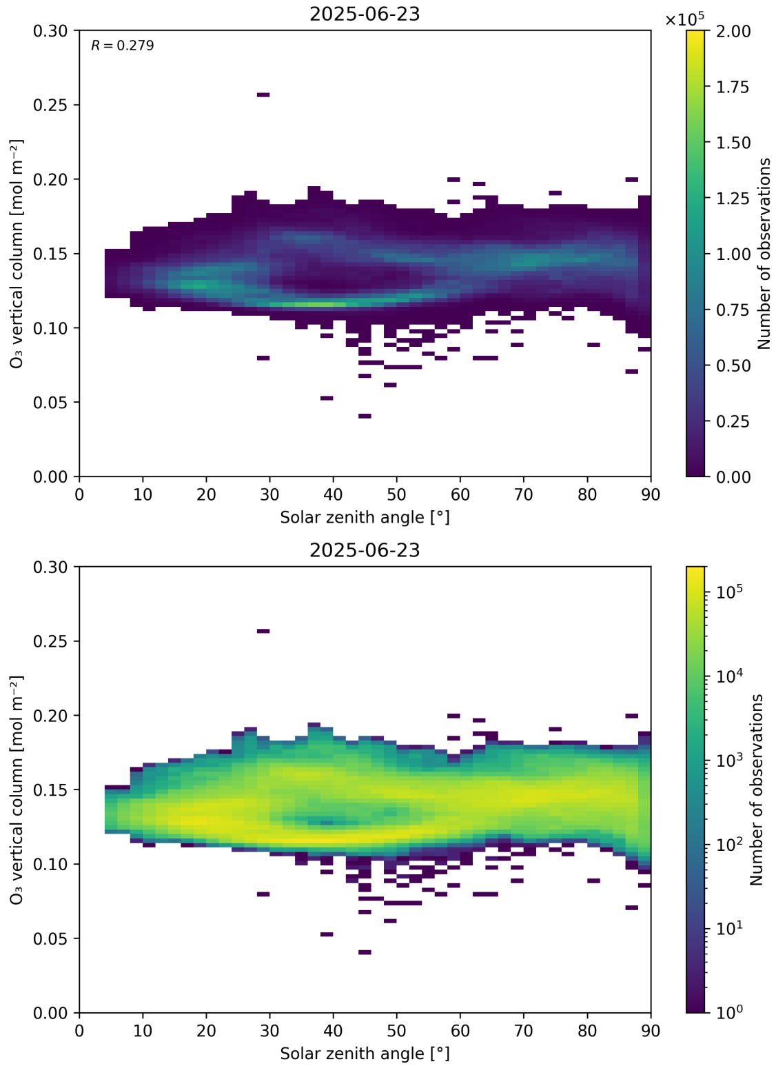
Figure 47: Scatter density plot of “Solar zenith angle” against “O 3 vertical column” for 2025-06-22 to 2025-06-24.
