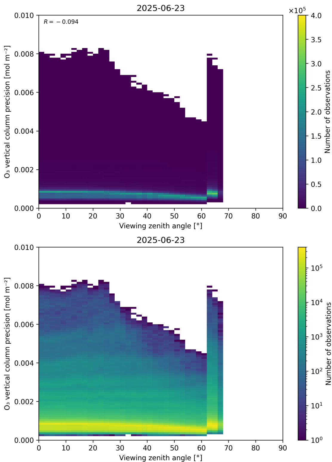
Figure 53: Scatter density plot of “Viewing zenith angle” against “O 3 vertical column precision” for 2025-06-22 to 2025-06-24.
