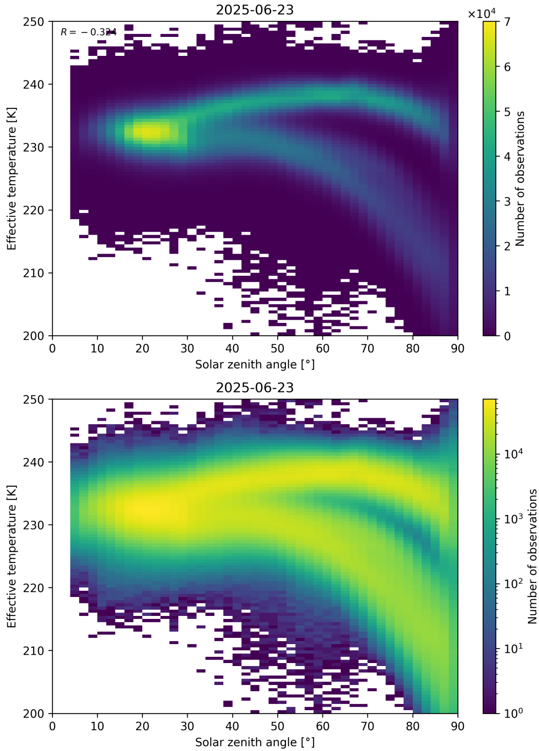
Figure 45: Scatter density plot of “Solar zenith angle” against “Effective temperature” for 2025-06-22 to 2025-06-24.
