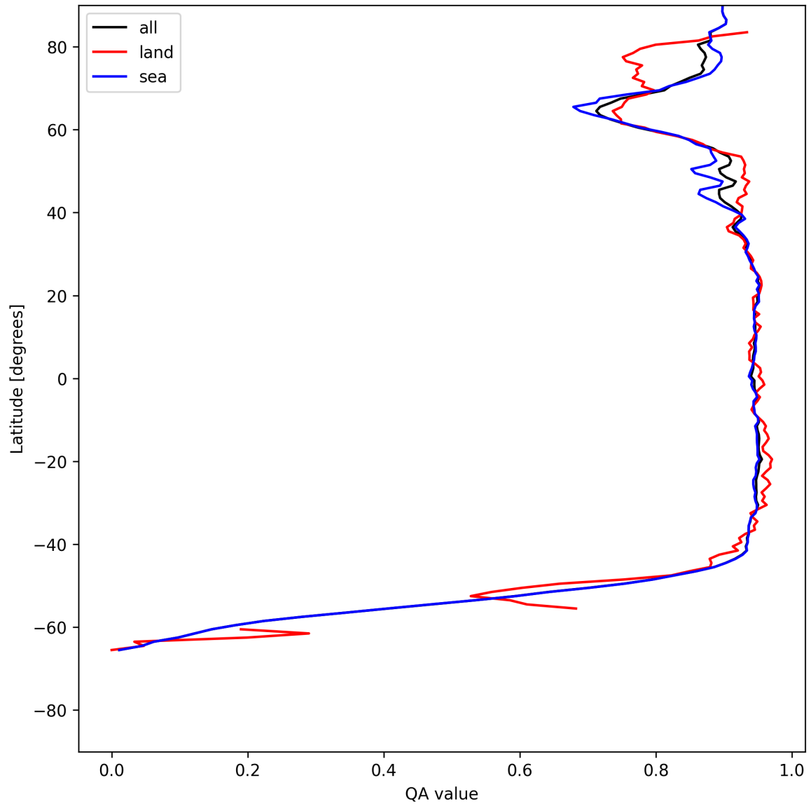
Figure 13: Zonal average of “QA value” for 2025-06-22 to 2025-06-24.
