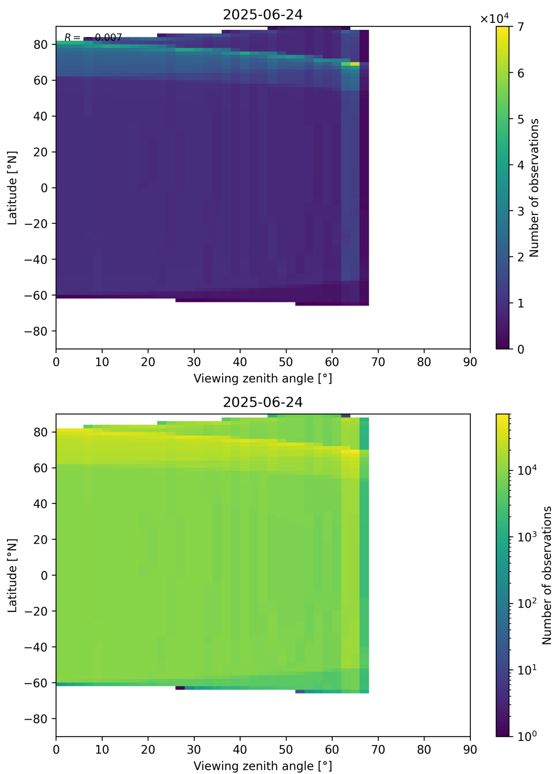
Figure 49: Scatter density plot of “Viewing zenith angle” against “Latitude” for 2025-06-23 to 2025-06-25.
