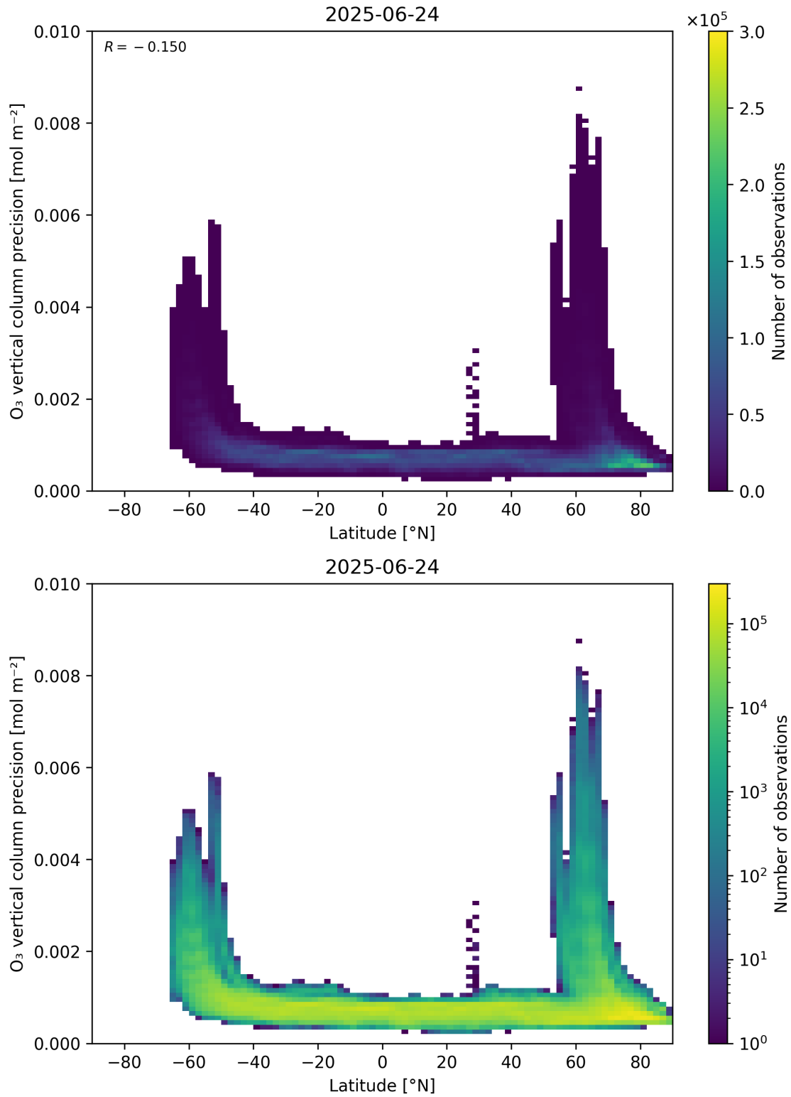
Figure 37: Scatter density plot of “Latitude” against “O 3 vertical column precision” for 2025-06-23 to 2025-06-25.
