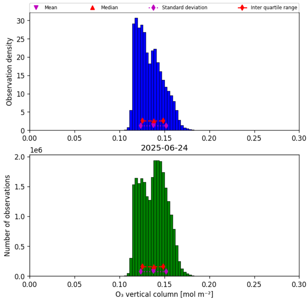
Figure 21: Histogram of “O 3 vertical column” for 2025-06-23 to 2025-06-25
