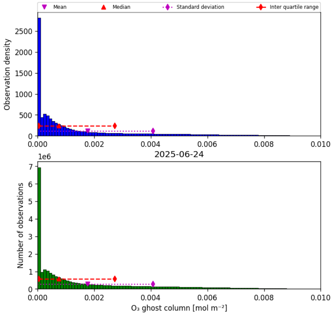
Figure 25: Histogram of “O 3 ghost column” for 2025-06-23 to 2025-06-25
