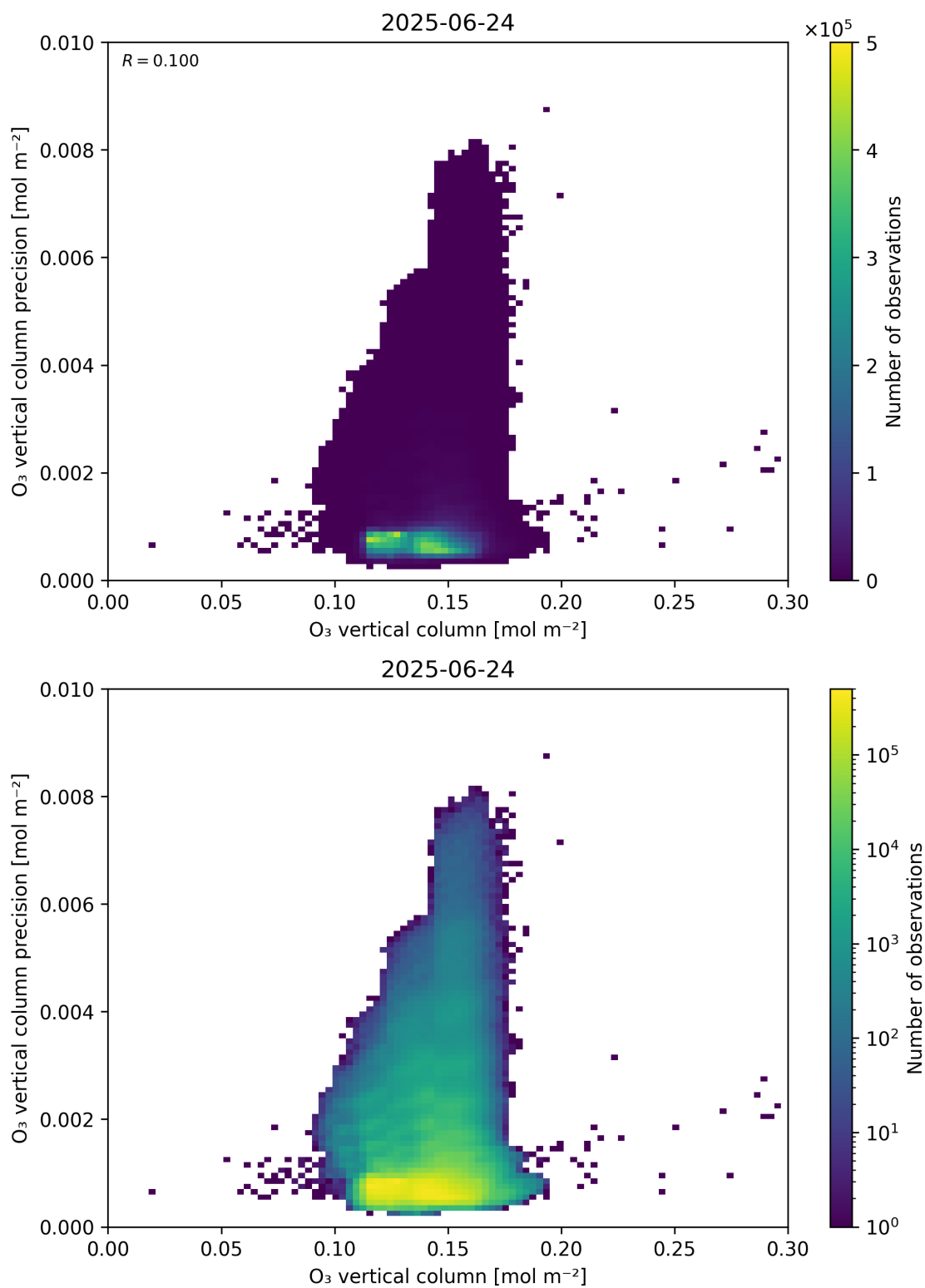
Figure 41: Scatter density plot of “O 3 vertical column” against “O 3 vertical column precision” for 2025-06-23 to 2025-06-25.
