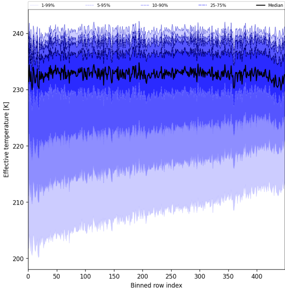
Figure 31: Along track statistics of “Effective temperature” for 2025-06-23 to 2025-06-25
