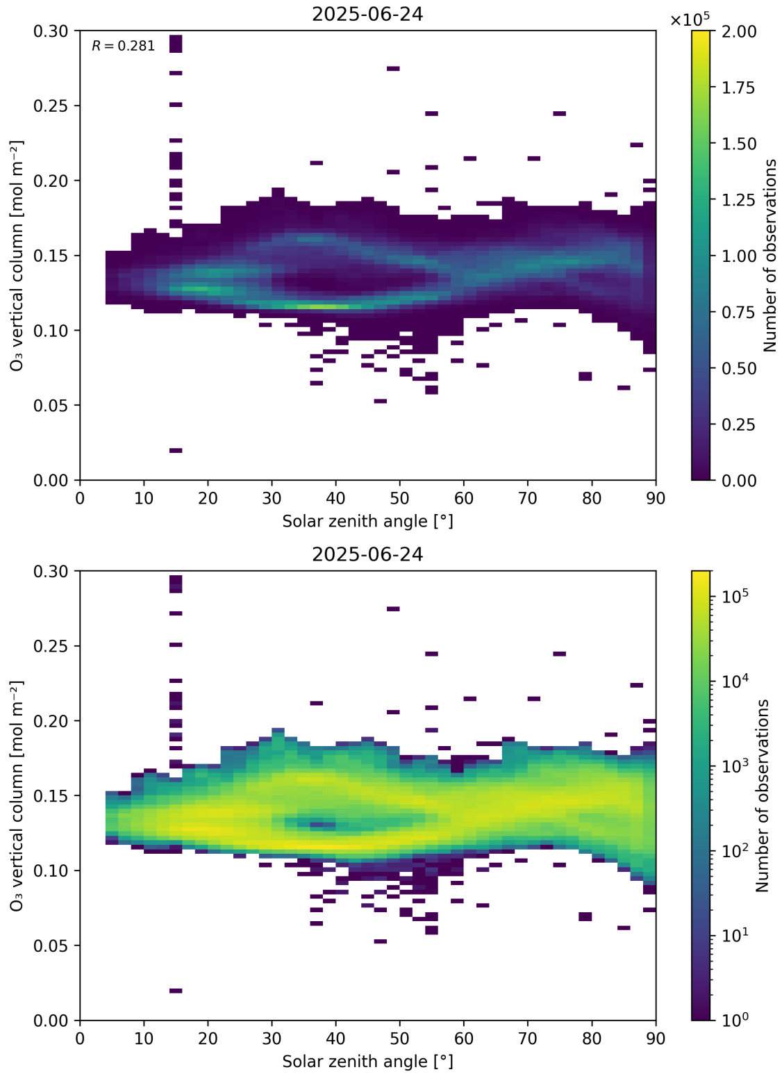
Figure 47: Scatter density plot of “Solar zenith angle” against “O 3 vertical column” for 2025-06-23 to 2025-06-25.
