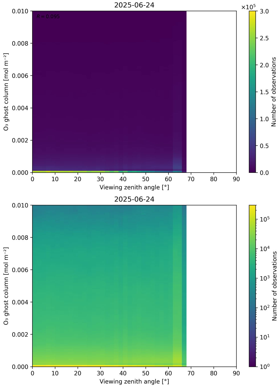
Figure 51: Scatter density plot of “Viewing zenith angle” against “O 3 ghost column” for 2025-06-23 to 2025-06-25.
