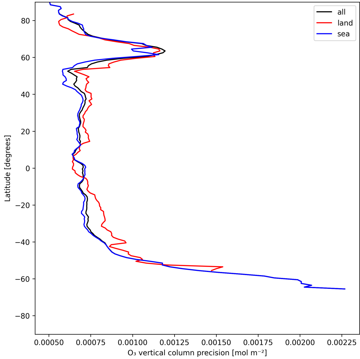
Figure 15: Zonal average of “O 3 vertical column precision” for 2025-06-23 to 2025-06-25.
