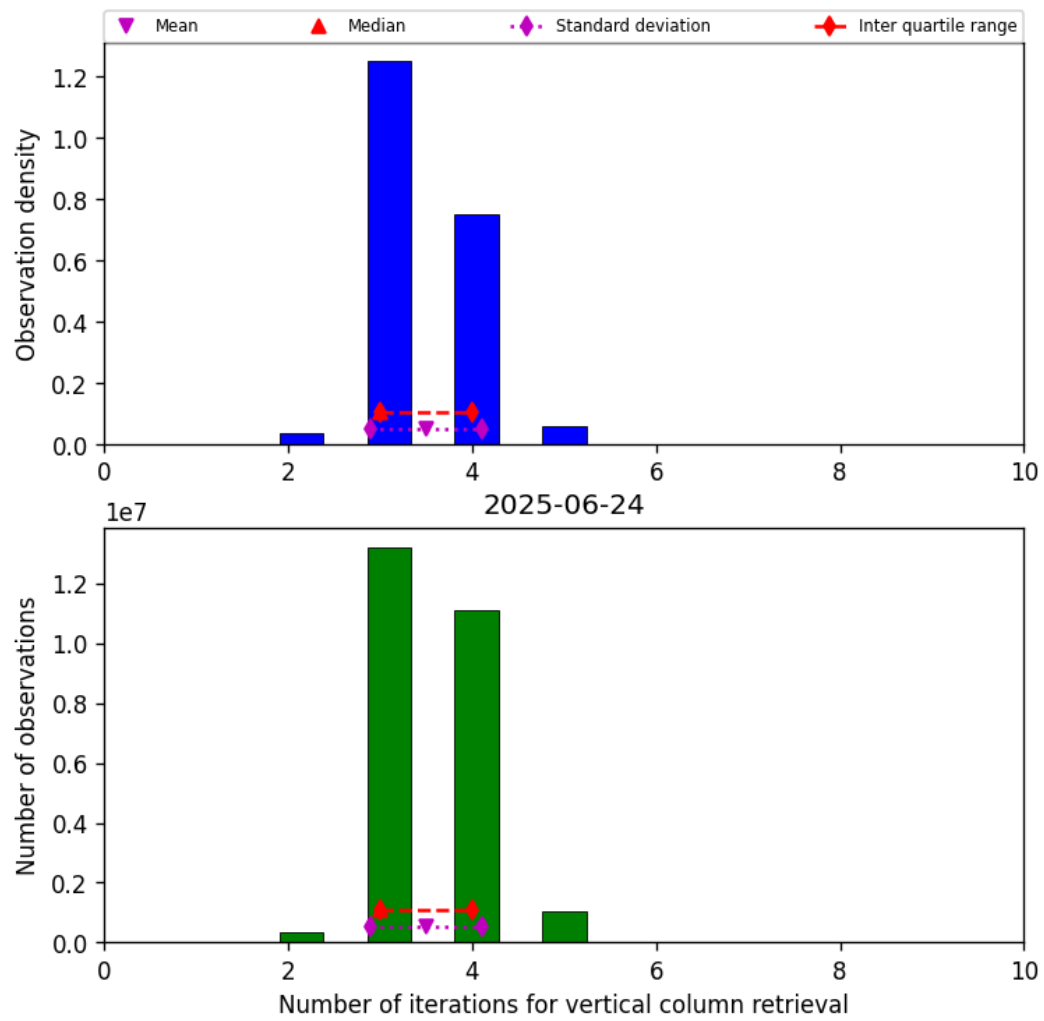
Figure 26: Histogram of “Number of iterations for vertical column retrieval” for 2025-06-23 to 2025-06-25
