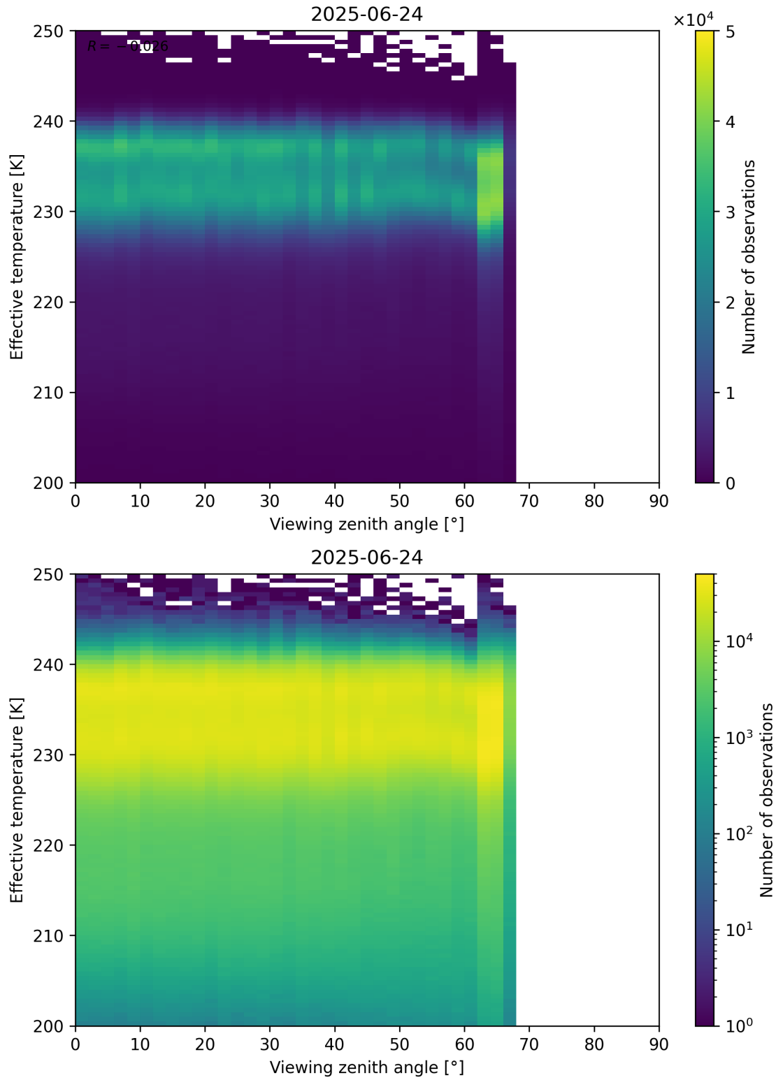
Figure 50: Scatter density plot of “Viewing zenith angle” against “Effective temperature” for 2025-06-23 to 2025-06-25.
