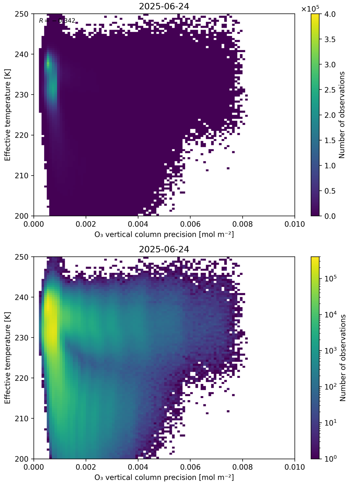
Figure 42: Scatter density plot of “O 3 vertical column precision” against “Effective temperature” for 2025-06-23 to 2025-06-25.
