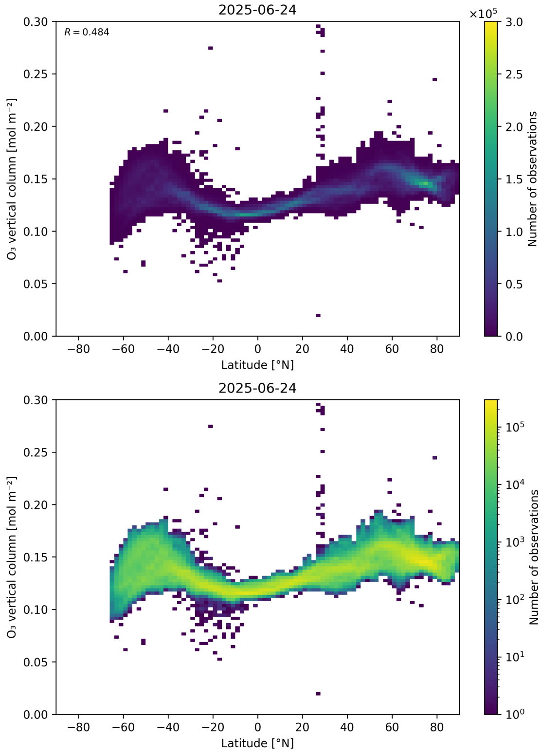
Figure 36: Scatter density plot of “Latitude” against “O 3 vertical column” for 2025-06-23 to 2025-06-25.
