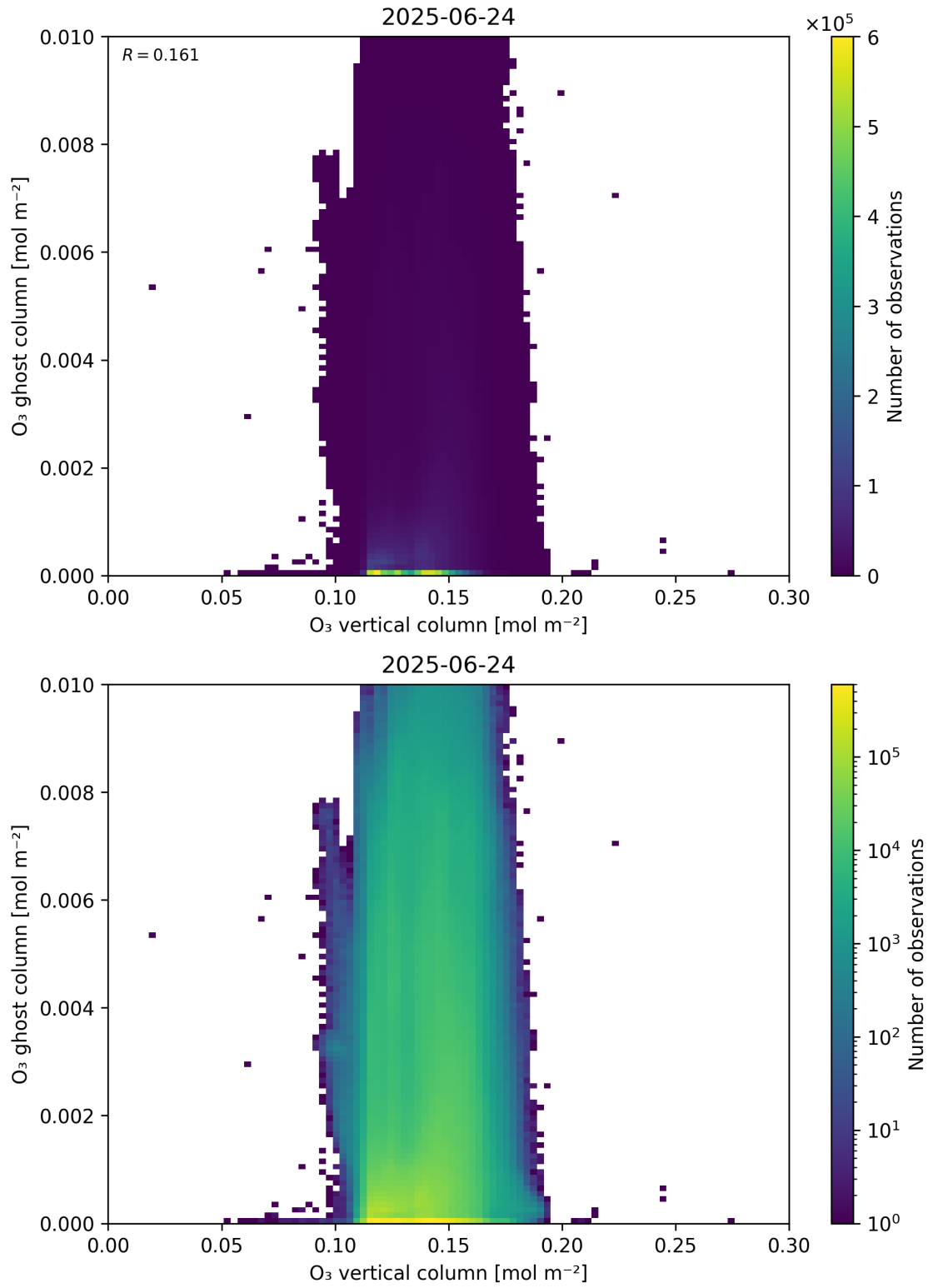
Figure 40: Scatter density plot of “O 3 vertical column” against “O 3 ghost column” for 2025-06-23 to 2025-06-25.
