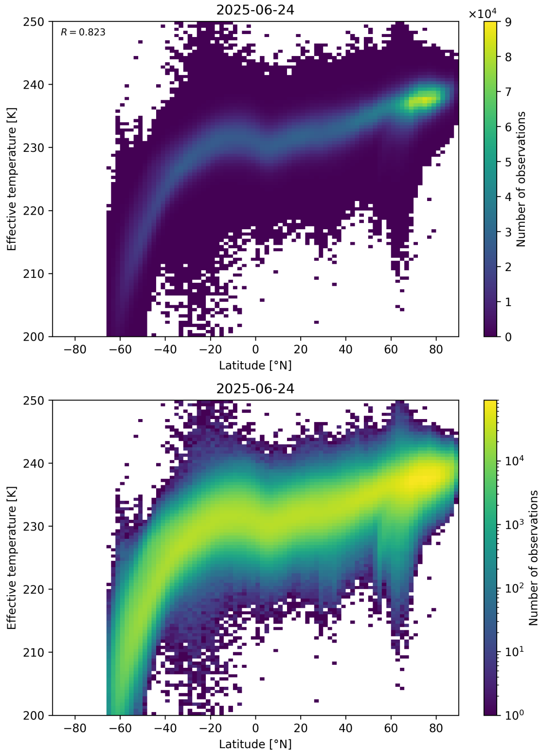
Figure 34: Scatter density plot of “Latitude” against “Effective temperature” for 2025-06-23 to 2025-06-25.
