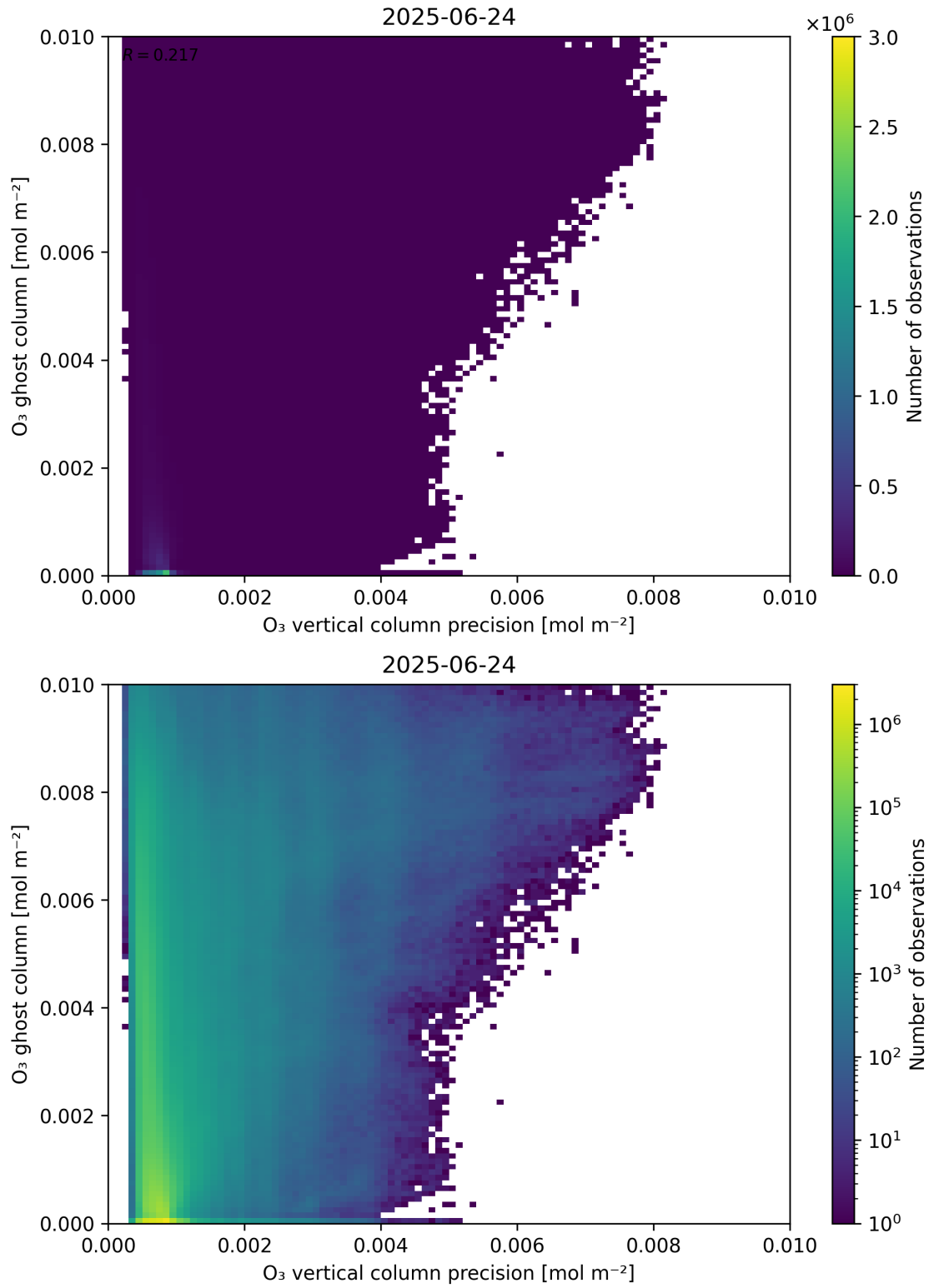
Figure 43: Scatter density plot of “ O_3 vertical column precision” against “ O_3 ghost column” for 2025-06-23 to 2025-06-25.
