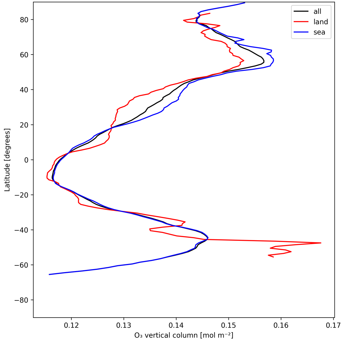
Figure 14: Zonal average of “O 3 vertical column” for 2025-06-23 to 2025-06-25.
