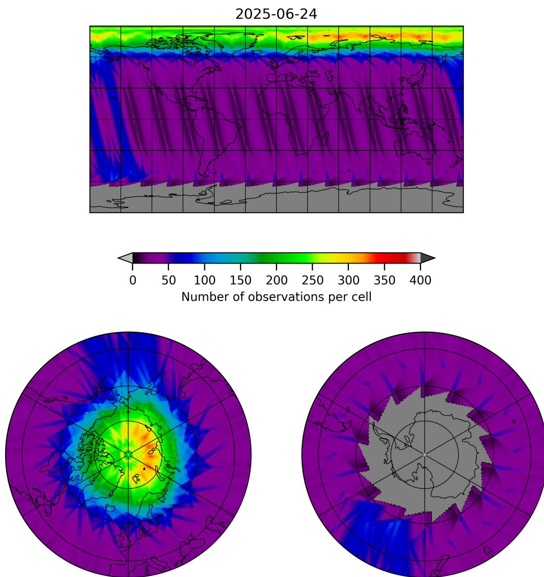
Figure 12: Map of the number of observations for 2025-06-23 to 2025-06-25
