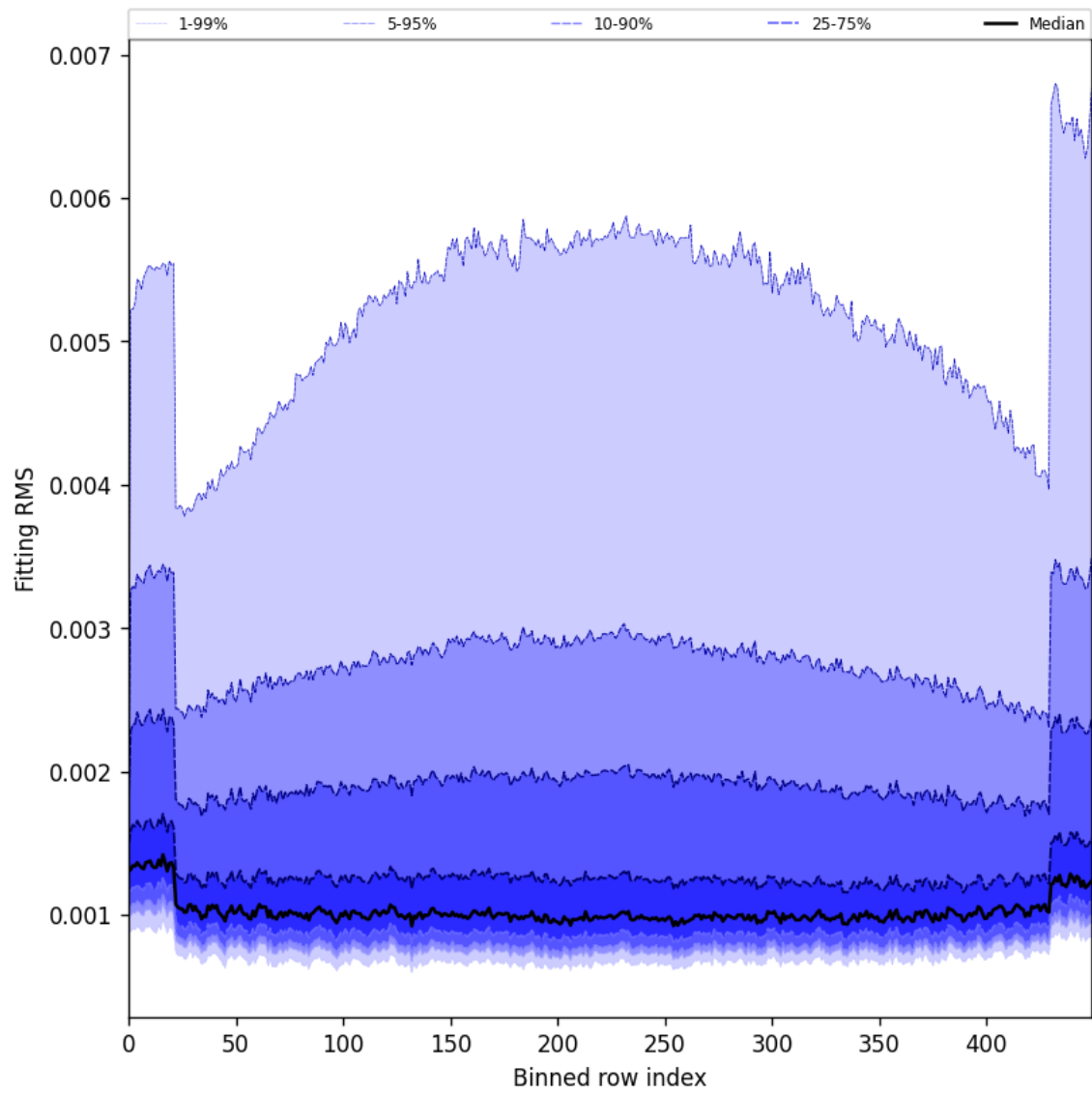
Figure 30: Along track statistics of “Fitting RMS” for 2025-06-23 to 2025-06-25
