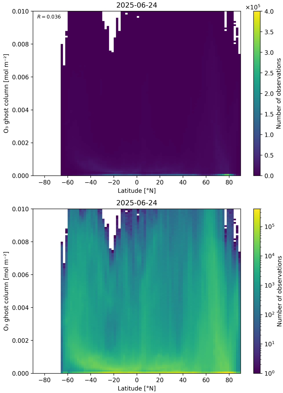
Figure 35: Scatter density plot of “Latitude” against “O 3 ghost column” for 2025-06-23 to 2025-06-25.
