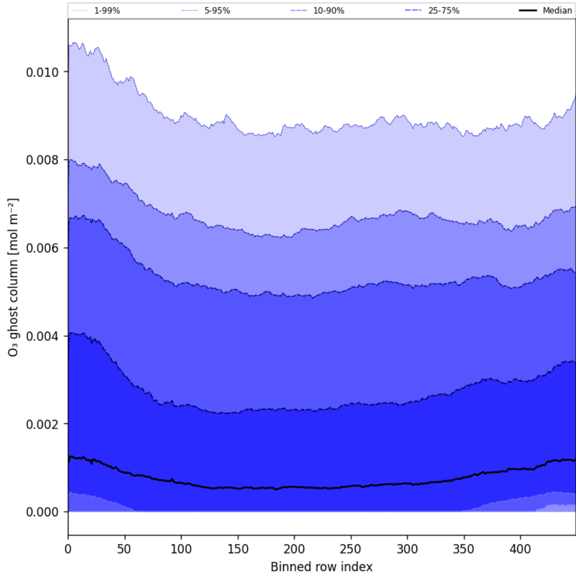
Figure 32: Along track statistics of “O 3 ghost column” for 2025-06-23 to 2025-06-25
