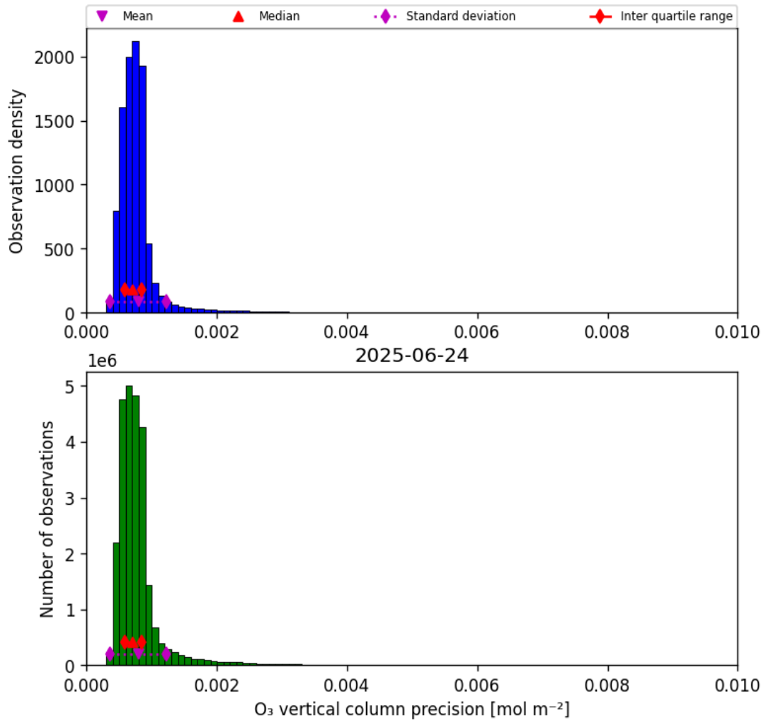
Figure 22: Histogram of “O 3 vertical column precision” for 2025-06-23 to 2025-06-25
