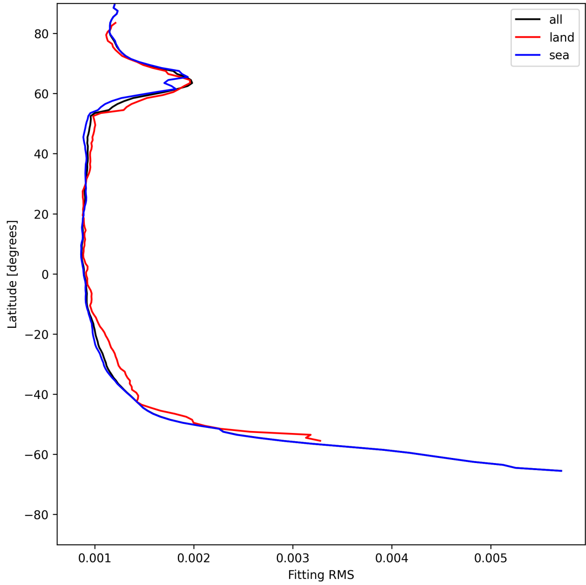
Figure 16: Zonal average of “Fitting RMS” for 2025-06-23 to 2025-06-25.
