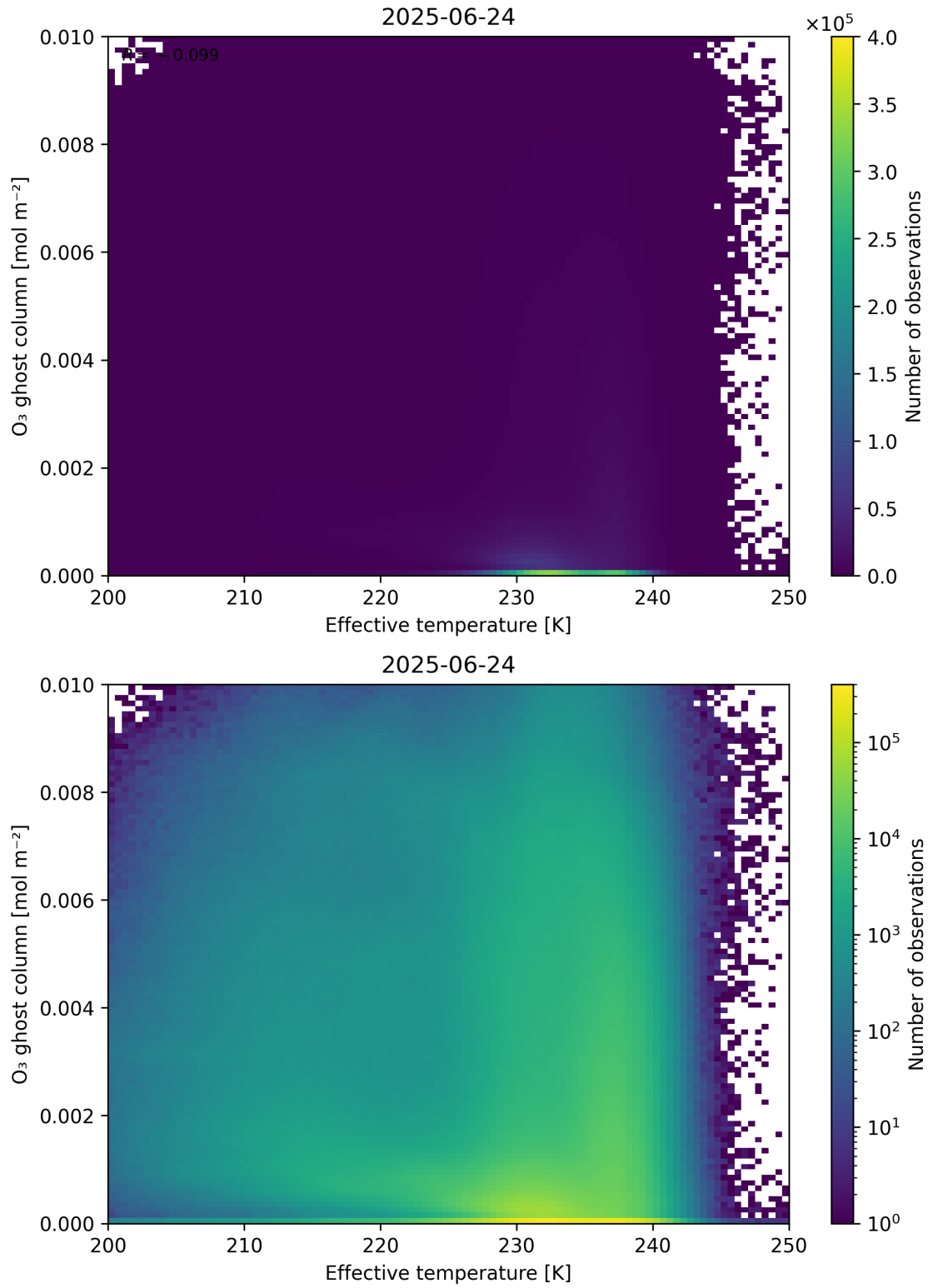
Figure 38: Scatter density plot of “Effective temperature” against “O 3 ghost column” for 2025-06-23 to 2025-06-25.
