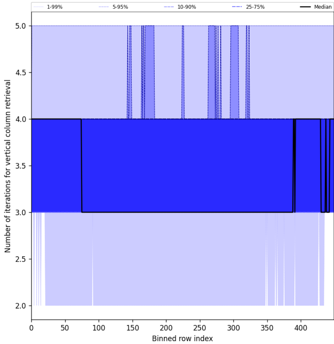
Figure 33: Along track statistics of “Number of iterations for vertical column retrieval” for 2025-06-23 to 2025-06-25
