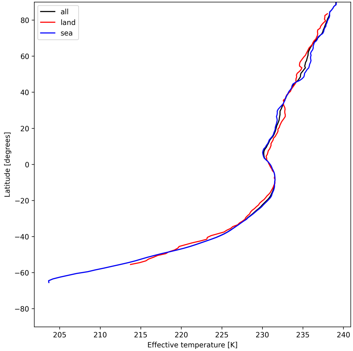
Figure 17: Zonal average of "Effective temperature" for 2025-06-23 to 2025-06-25.
