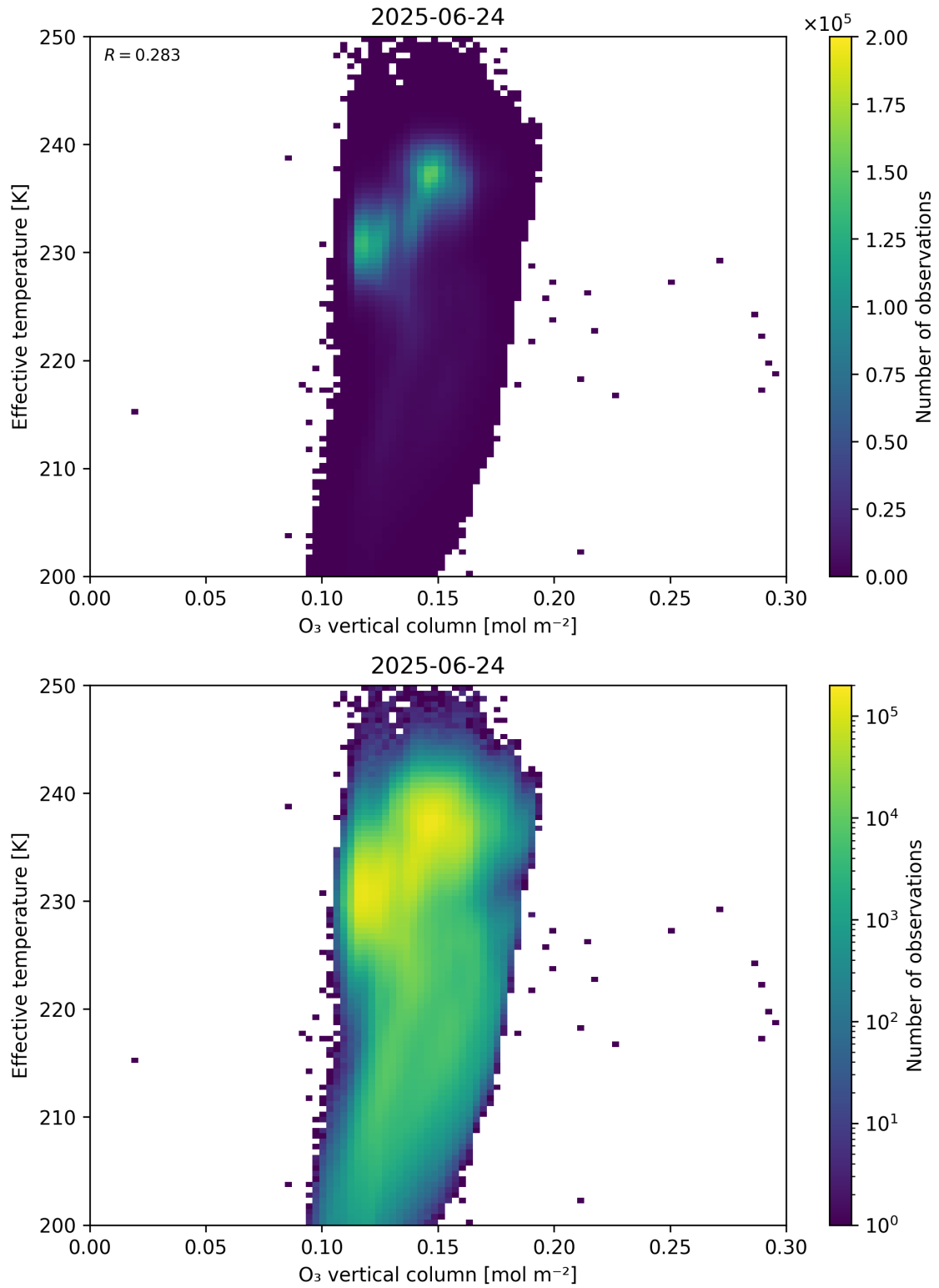
Figure 39: Scatter density plot of “O 3 vertical column” against “Effective temperature” for 2025-06-23 to 2025-06-25.
