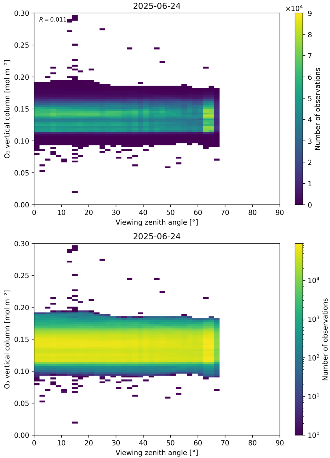
Figure 52: Scatter density plot of “Viewing zenith angle” against “O 3 vertical column” for 2025-06-23 to 2025-06-25.
