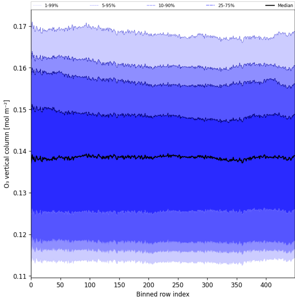
Figure 28: Along track statistics of “O 3 vertical column” for 2025-06-23 to 2025-06-25
