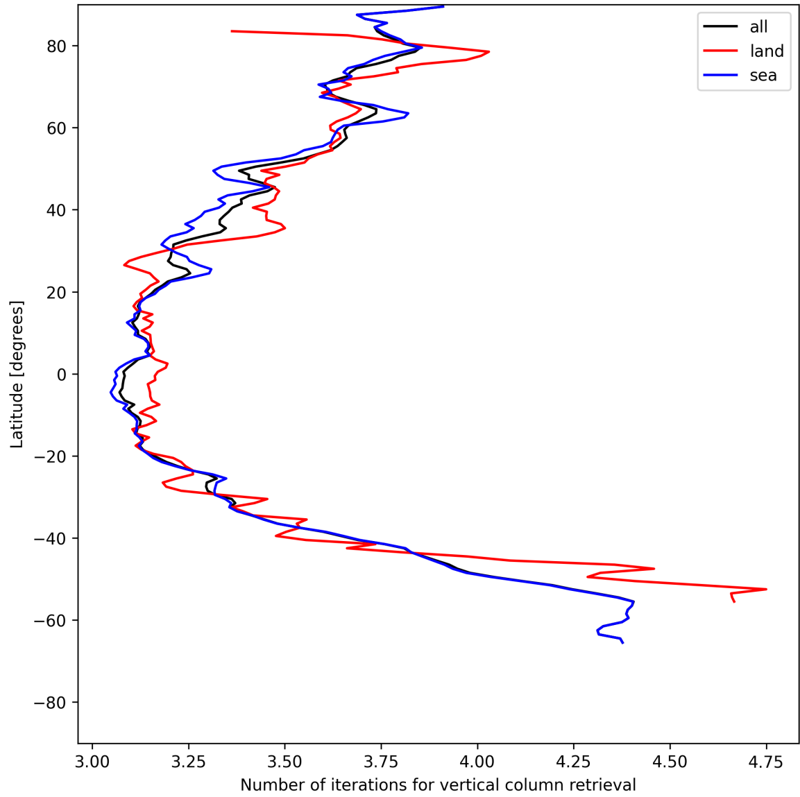
Figure 19: Zonal average of “Number of iterations for vertical column retrieval” for 2025-06-23 to 2025-06-25.
