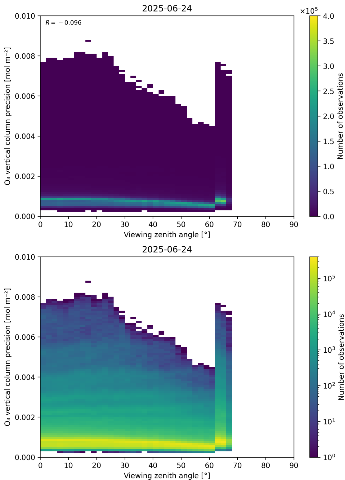
Figure 53: Scatter density plot of “Viewing zenith angle” against “O 3 vertical column precision” for 2025-06-23 to 2025-06-25.
