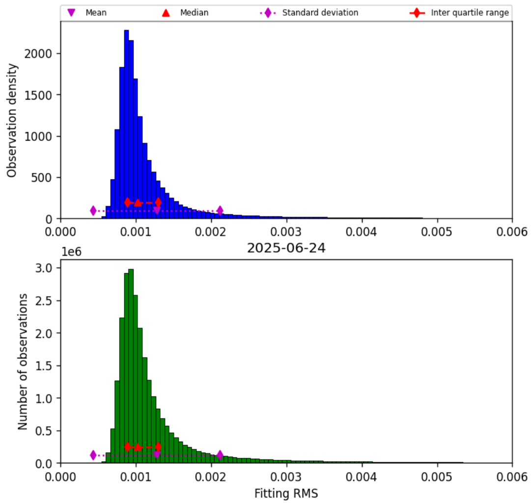
Figure 23: Histogram of “Fitting RMS” for 2025-06-23 to 2025-06-25
