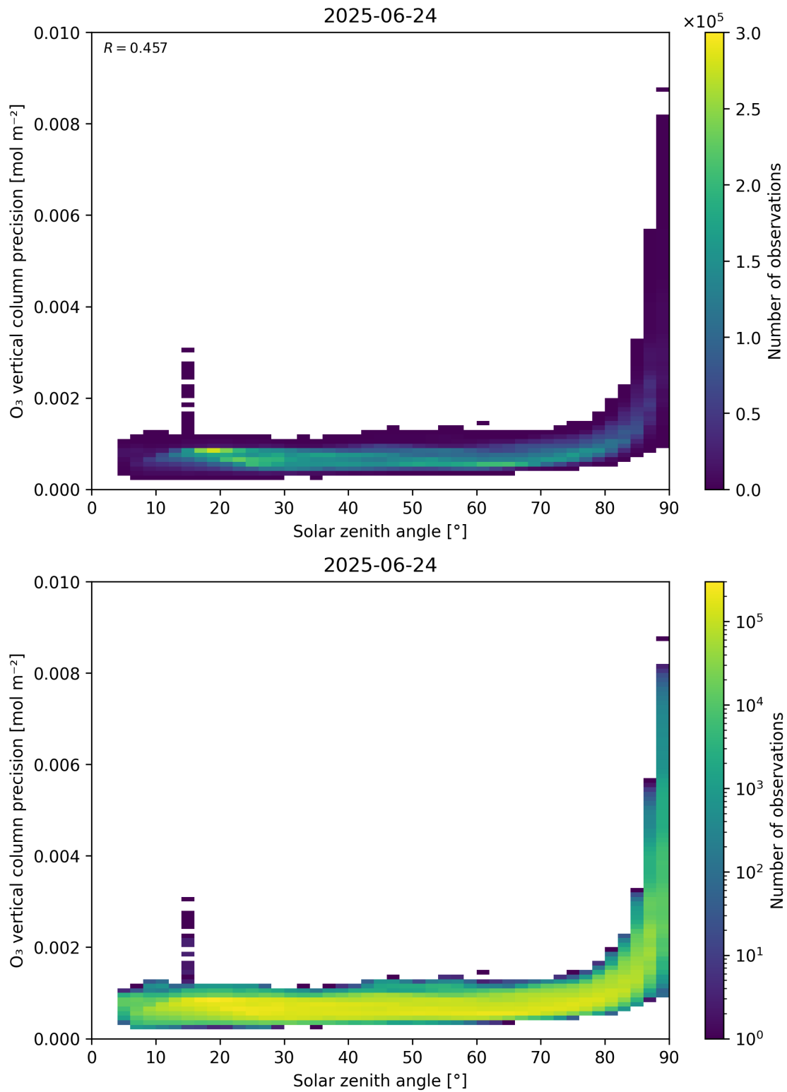
Figure 48: Scatter density plot of “Solar zenith angle” against “O 3 vertical column precision” for 2025-06-23 to 2025-06-25.
