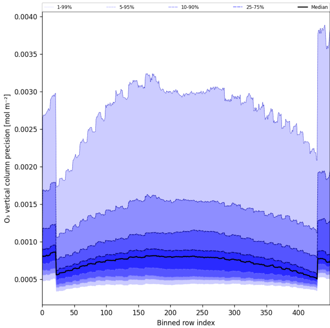
Figure 29: Along track statistics of “O 3 vertical column precision” for 2025-06-23 to 2025-06-25
