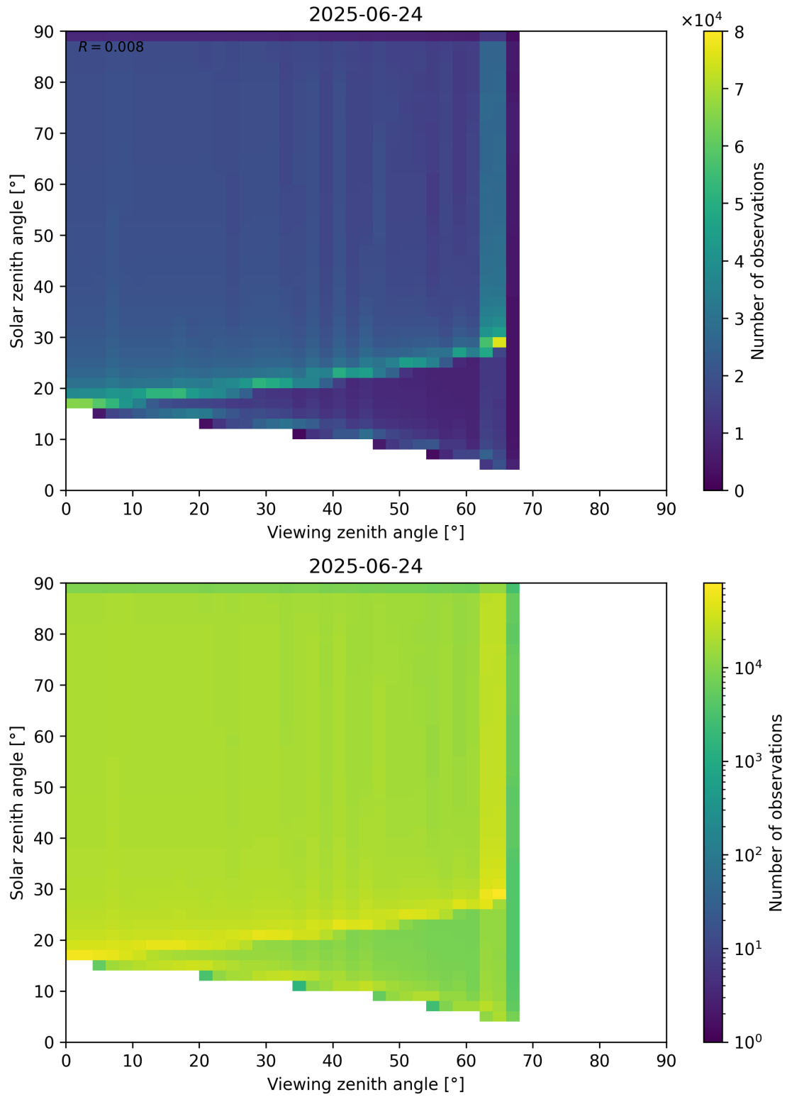
Figure 54: Scatter density plot of “Viewing zenith angle” against “Solar zenith angle” for 2025-06-23 to 2025-06-25.
