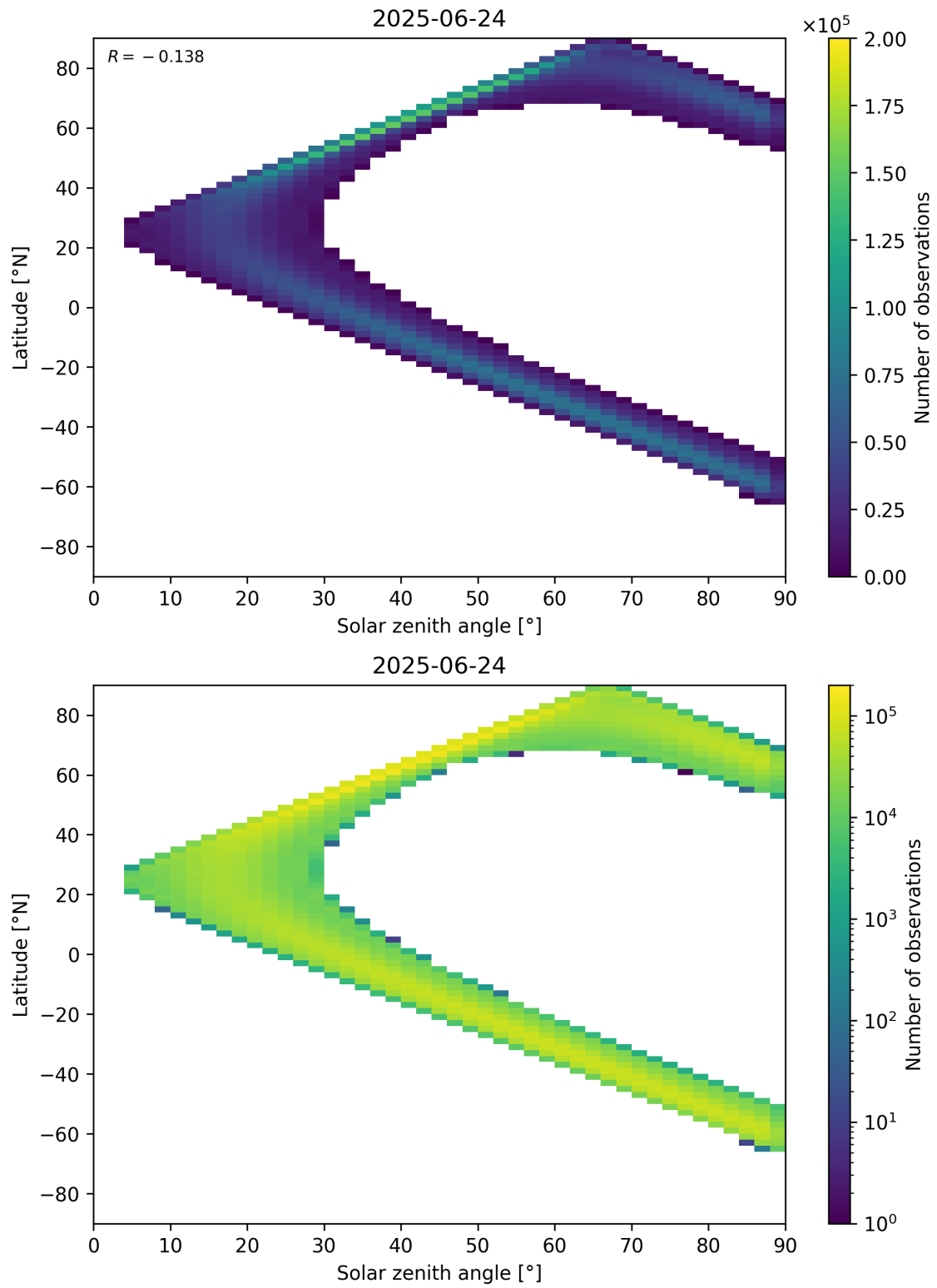
Figure 44: Scatter density plot of “Solar zenith angle” against “Latitude” for 2025-06-23 to 2025-06-25.
