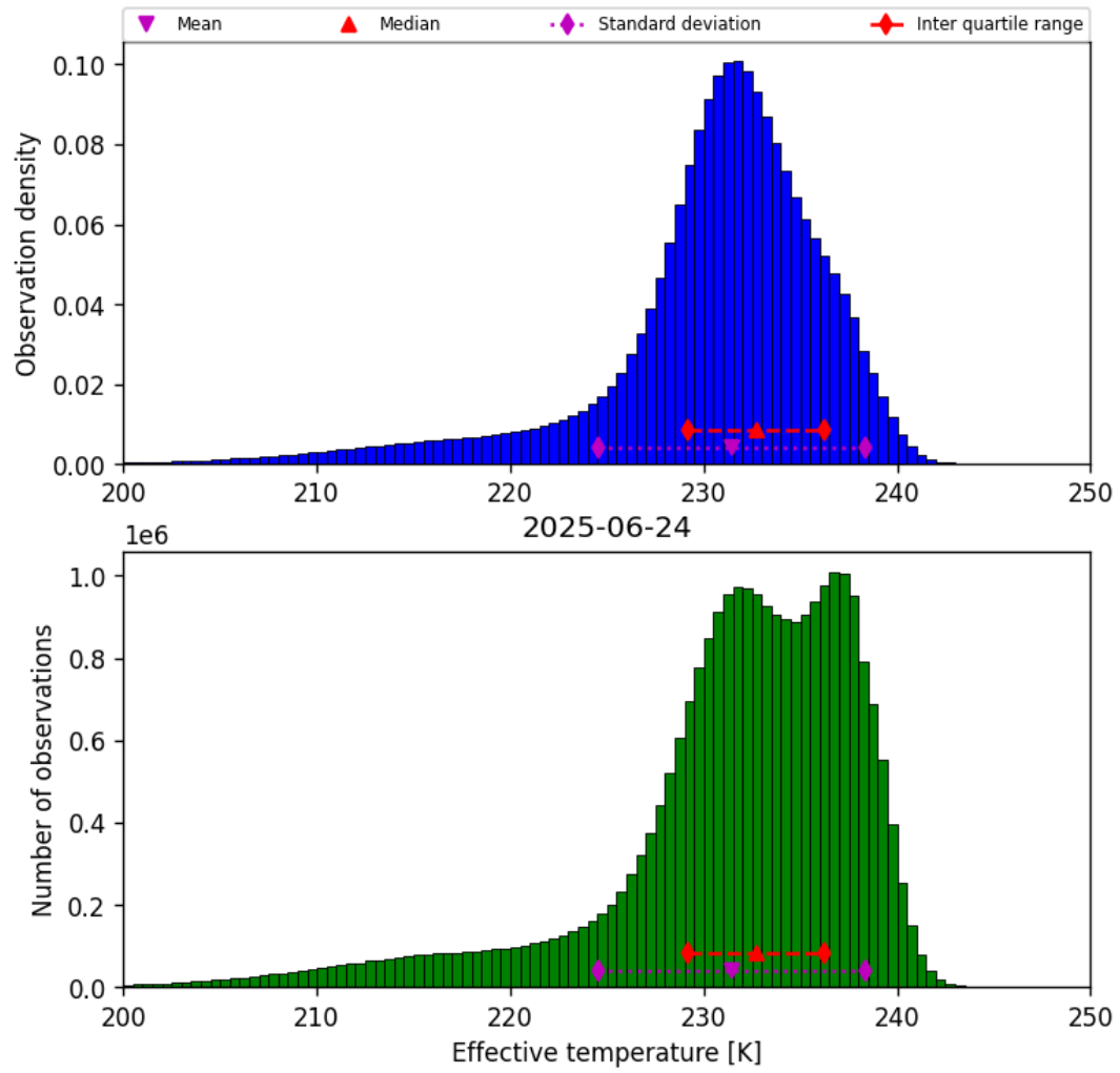
Figure 24: Histogram of “Effective temperature” for 2025-06-23 to 2025-06-25
