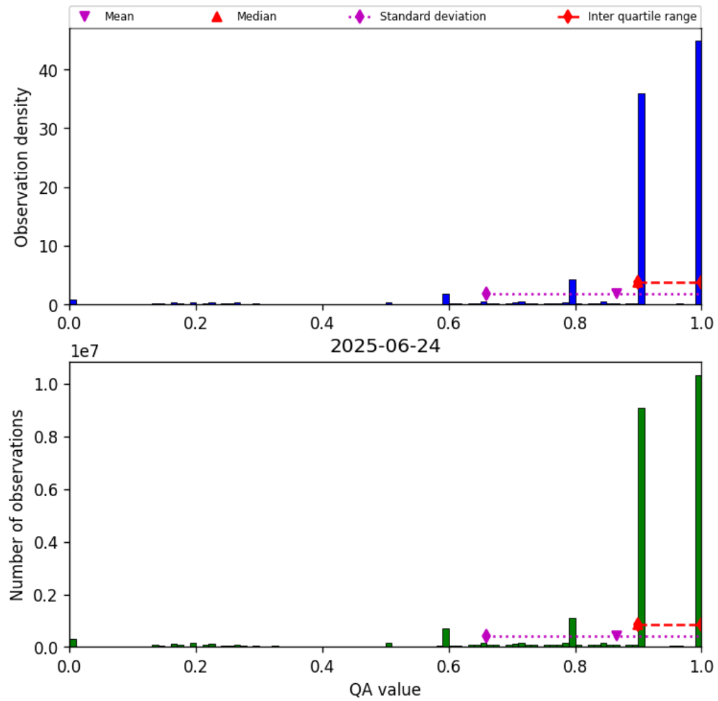
Figure 20: Histogram of “QA value” for 2025-06-23 to 2025-06-25
