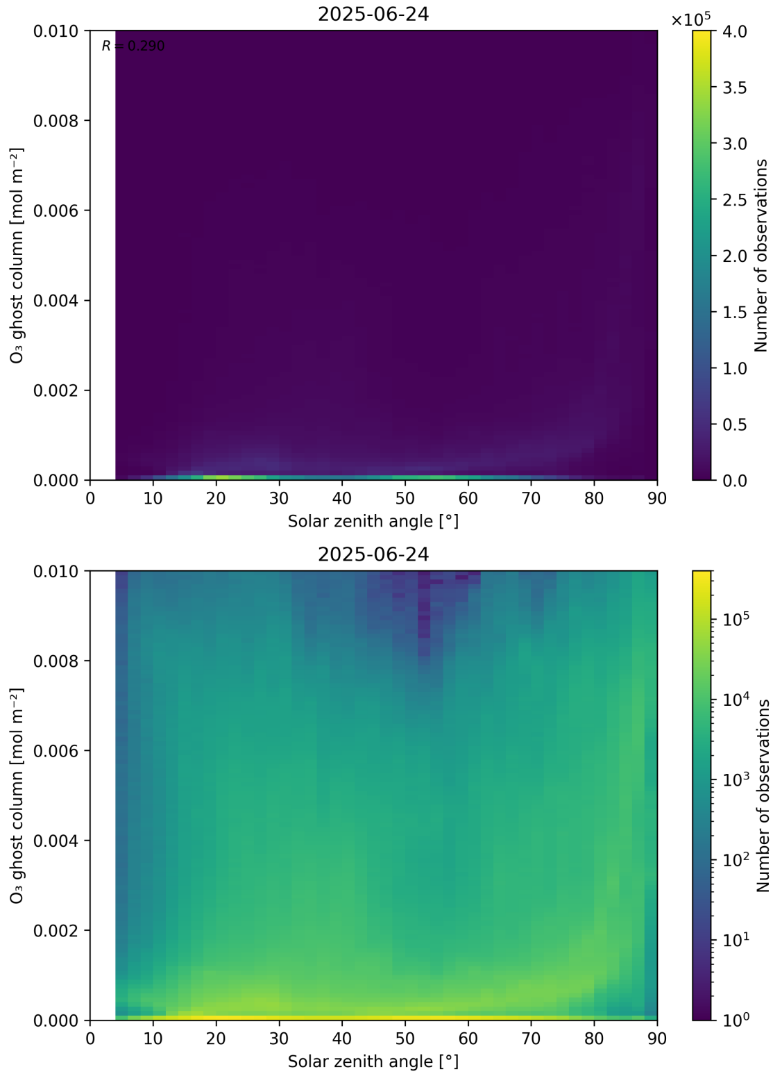
Figure 46: Scatter density plot of “Solar zenith angle” against “O 3 ghost column” for 2025-06-23 to 2025-06-25.
