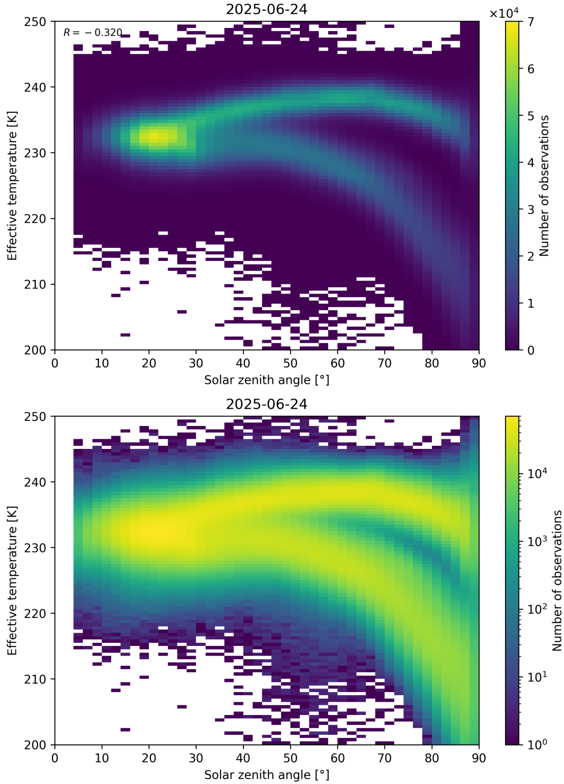
Figure 45: Scatter density plot of “Solar zenith angle” against “Effective temperature” for 2025-06-23 to 2025-06-25.
