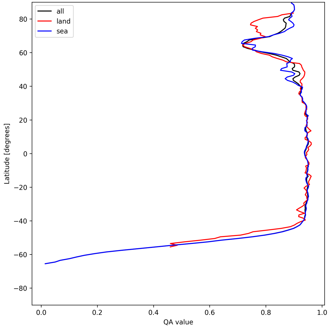
Figure 13: Zonal average of “QA value” for 2025-06-23 to 2025-06-25.
