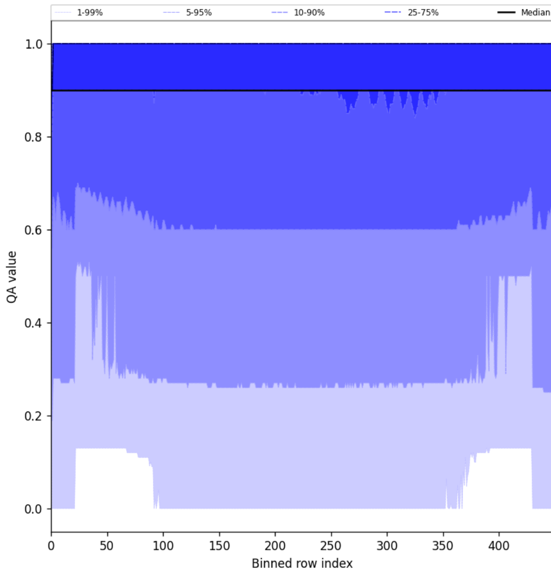
Figure 27: Along track statistics of “QA value” for 2025-06-23 to 2025-06-25
