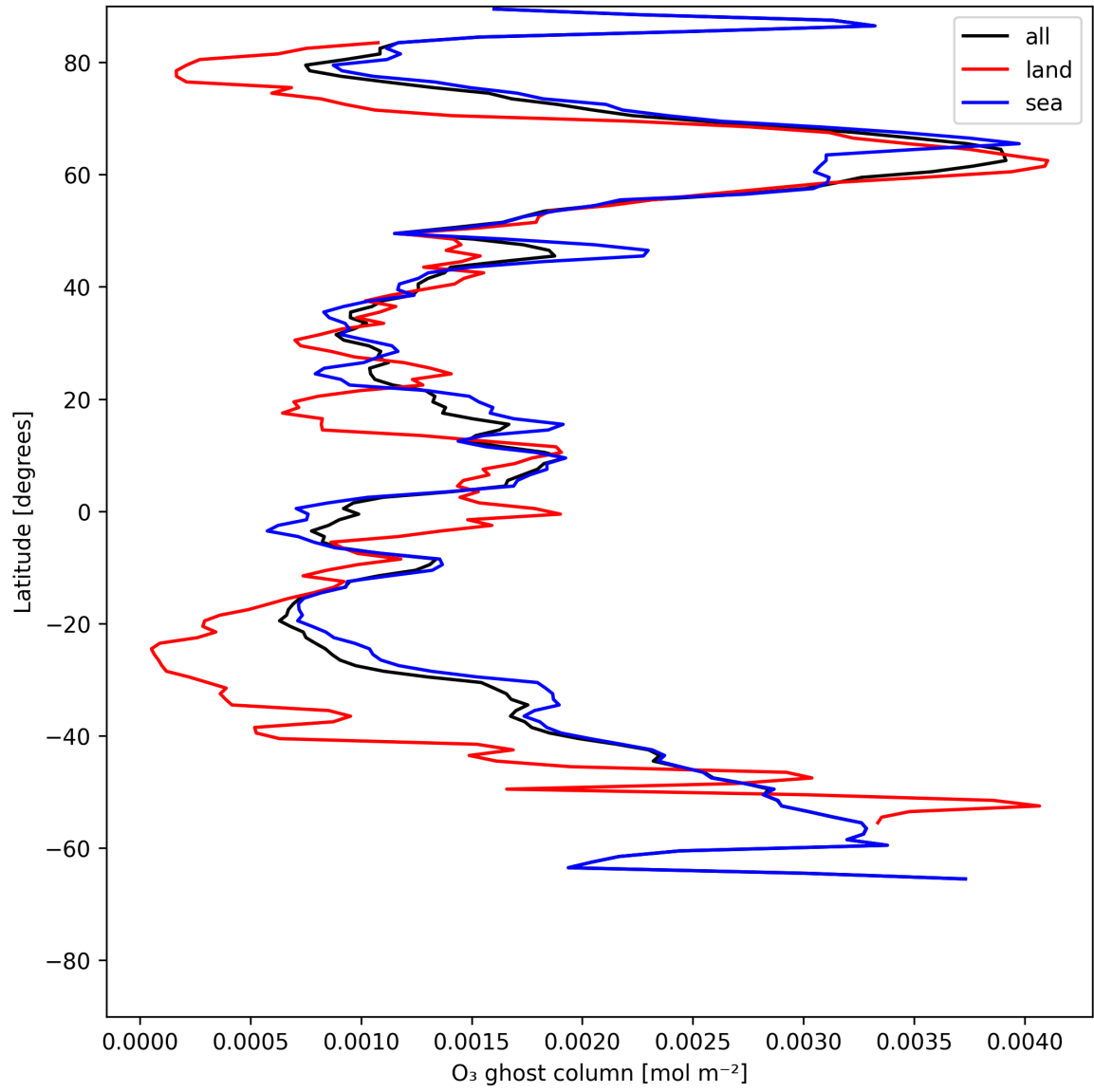
Figure 18: Zonal average of "O 3 ghost column" for 2025-06-23 to 2025-06-25.
