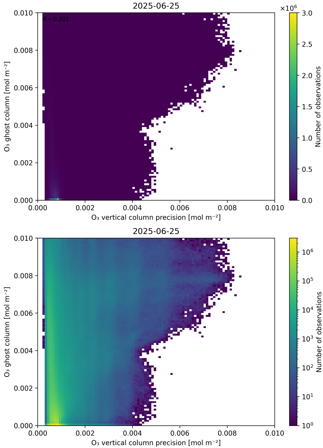
Figure 43: Scatter density plot of “O 3 vertical column precision” against “O 3 ghost column” for 2025-06-24 to 2025-06-26.
