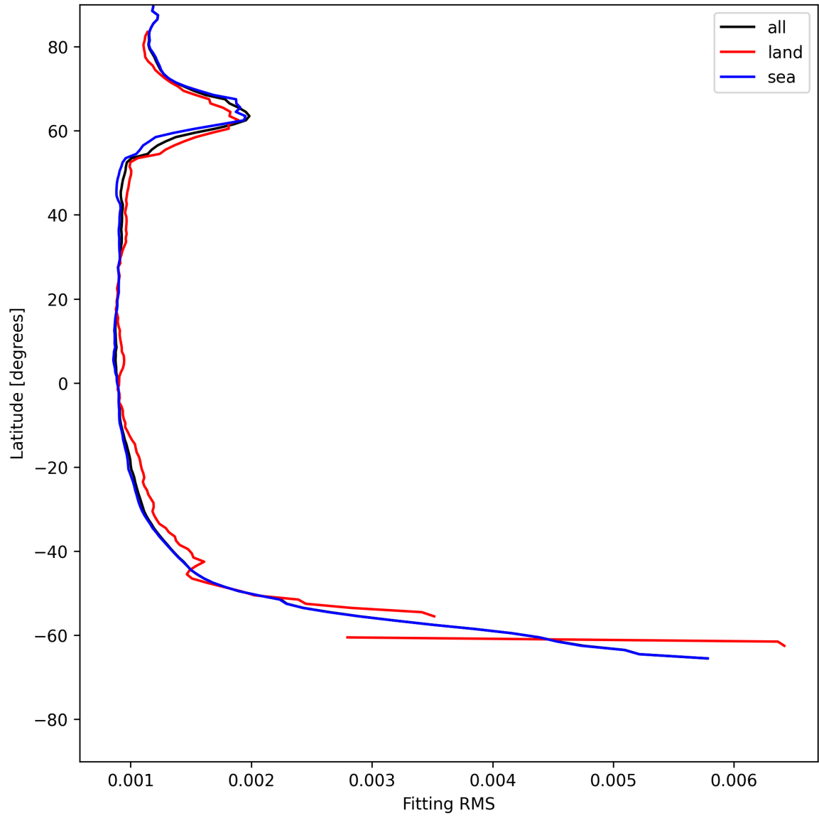
Figure 16: Zonal average of “Fitting RMS” for 2025-06-24 to 2025-06-26.
