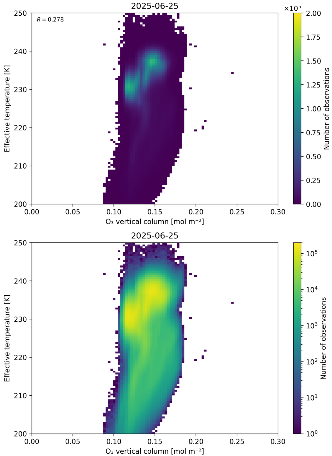
Figure 39: Scatter density plot of “O 3 vertical column” against “Effective temperature” for 2025-06-24 to 2025-06-26.
