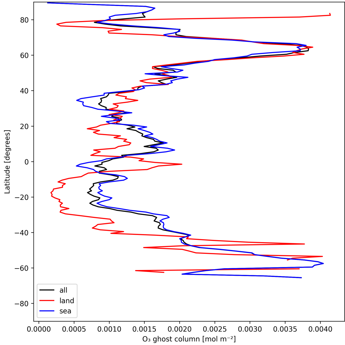
Figure 18: Zonal average of “O 3 ghost column” for 2025-06-24 to 2025-06-26.
