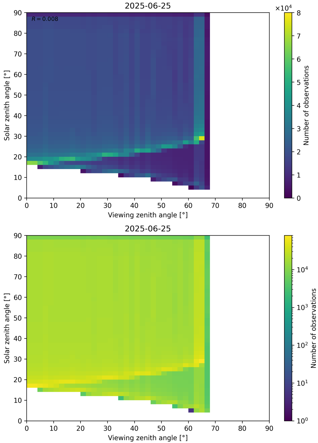
Figure 54: Scatter density plot of “Viewing zenith angle” against “Solar zenith angle” for 2025-06-24 to 2025-06-26.
