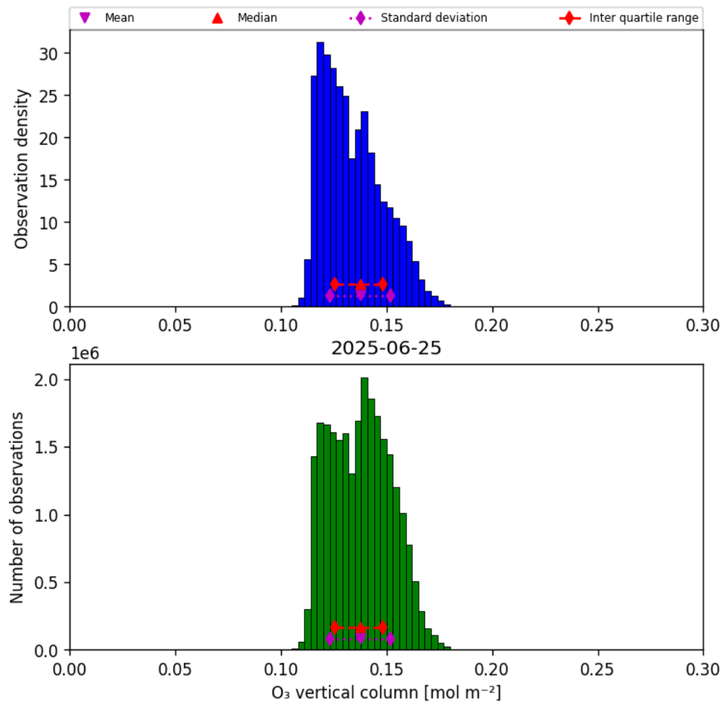
Figure 21: Histogram of “O 3 vertical column” for 2025-06-24 to 2025-06-26
