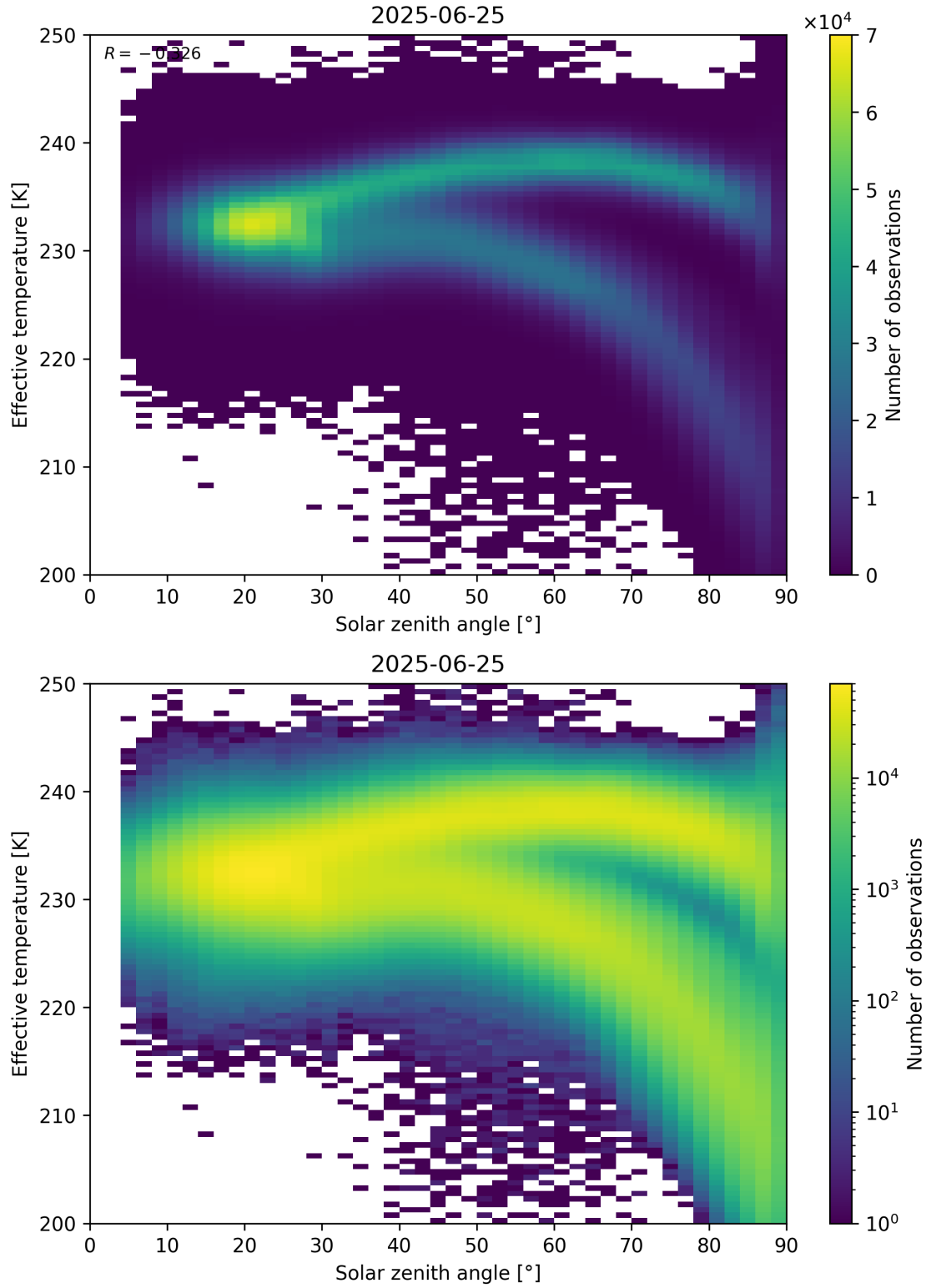
Figure 45: Scatter density plot of “Solar zenith angle” against “Effective temperature” for 2025-06-24 to 2025-06-26.
