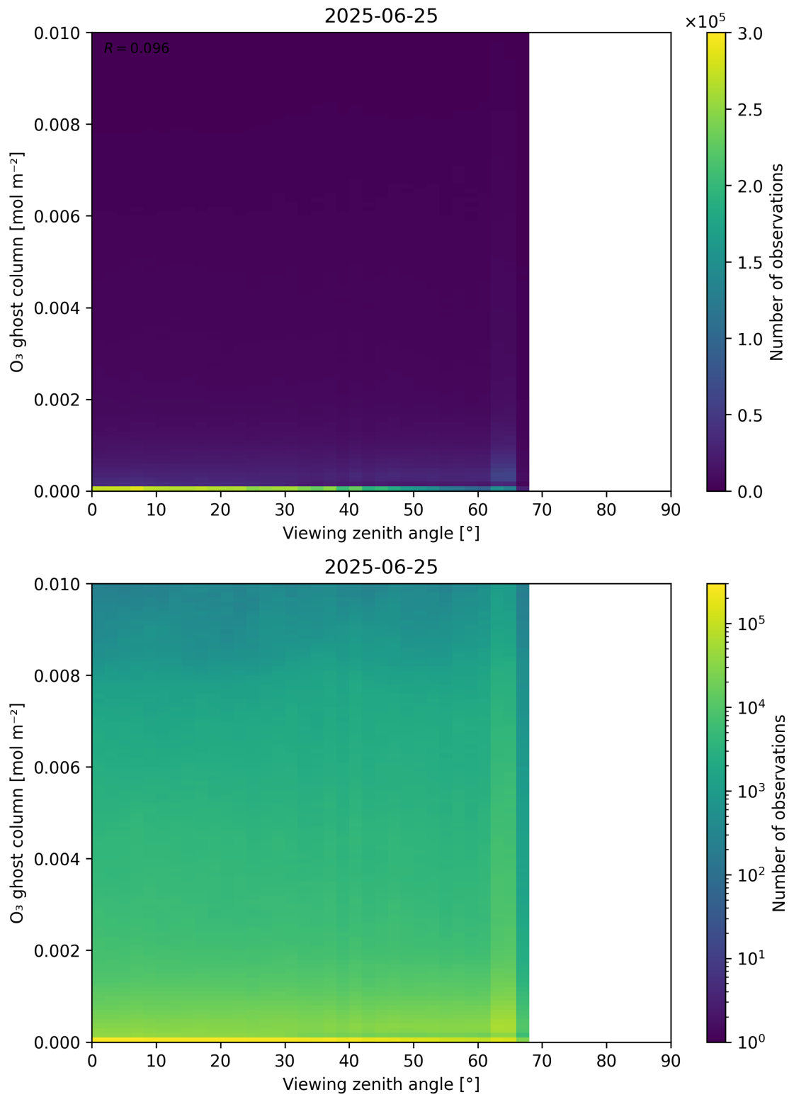
Figure 51: Scatter density plot of “Viewing zenith angle” against “O 3 ghost column” for 2025-06-24 to 2025-06-26.
