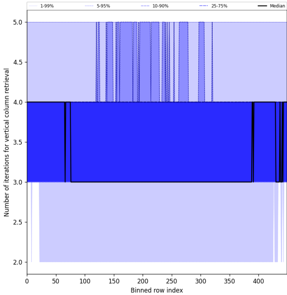
Figure 33: Along track statistics of “Number of iterations for vertical column retrieval” for 2025-06-24 to 2025-06-26
