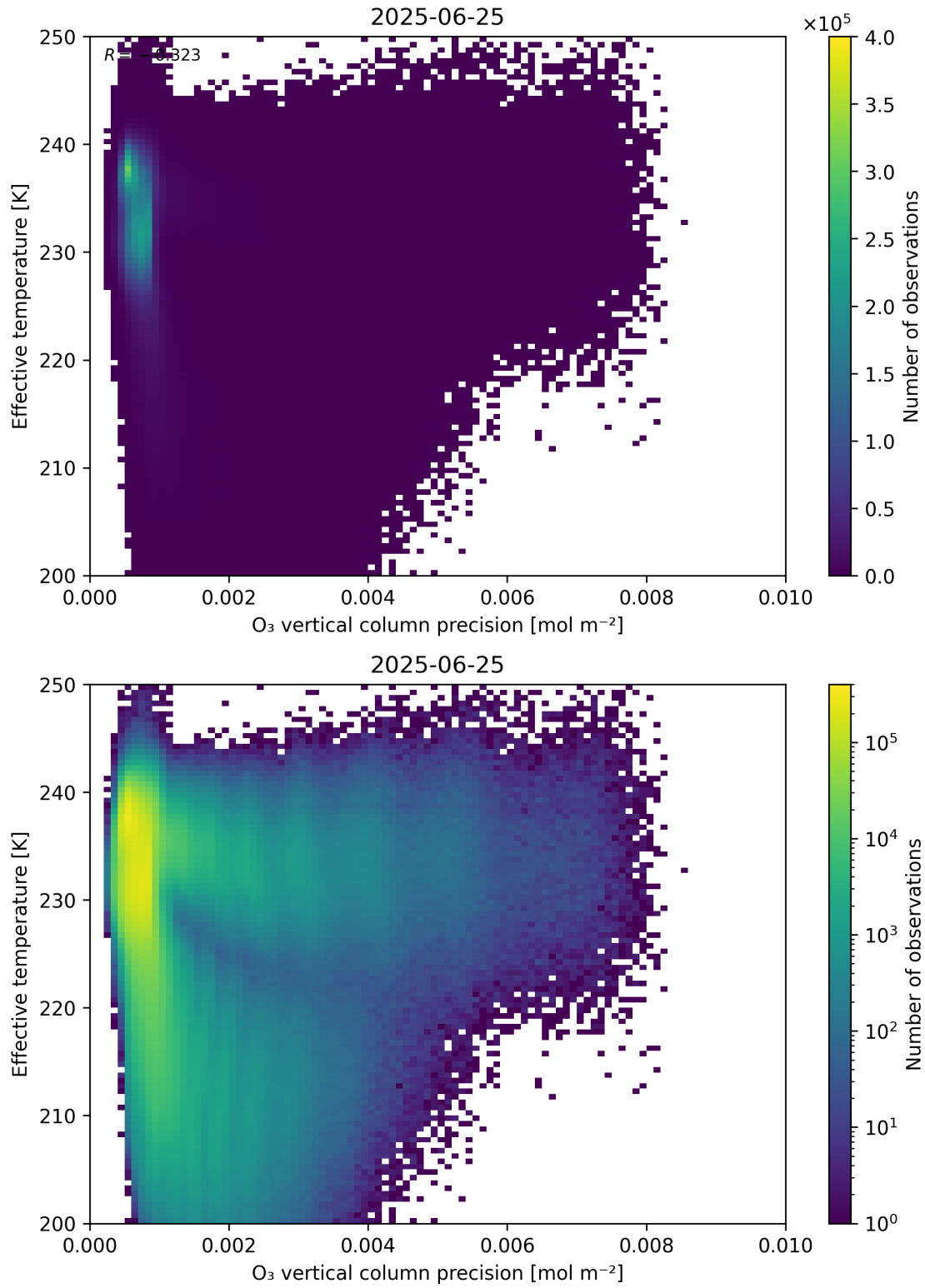
Figure 42: Scatter density plot of “O 3 vertical column precision” against “Effective temperature” for 2025-06-24 to 2025-06-26.
