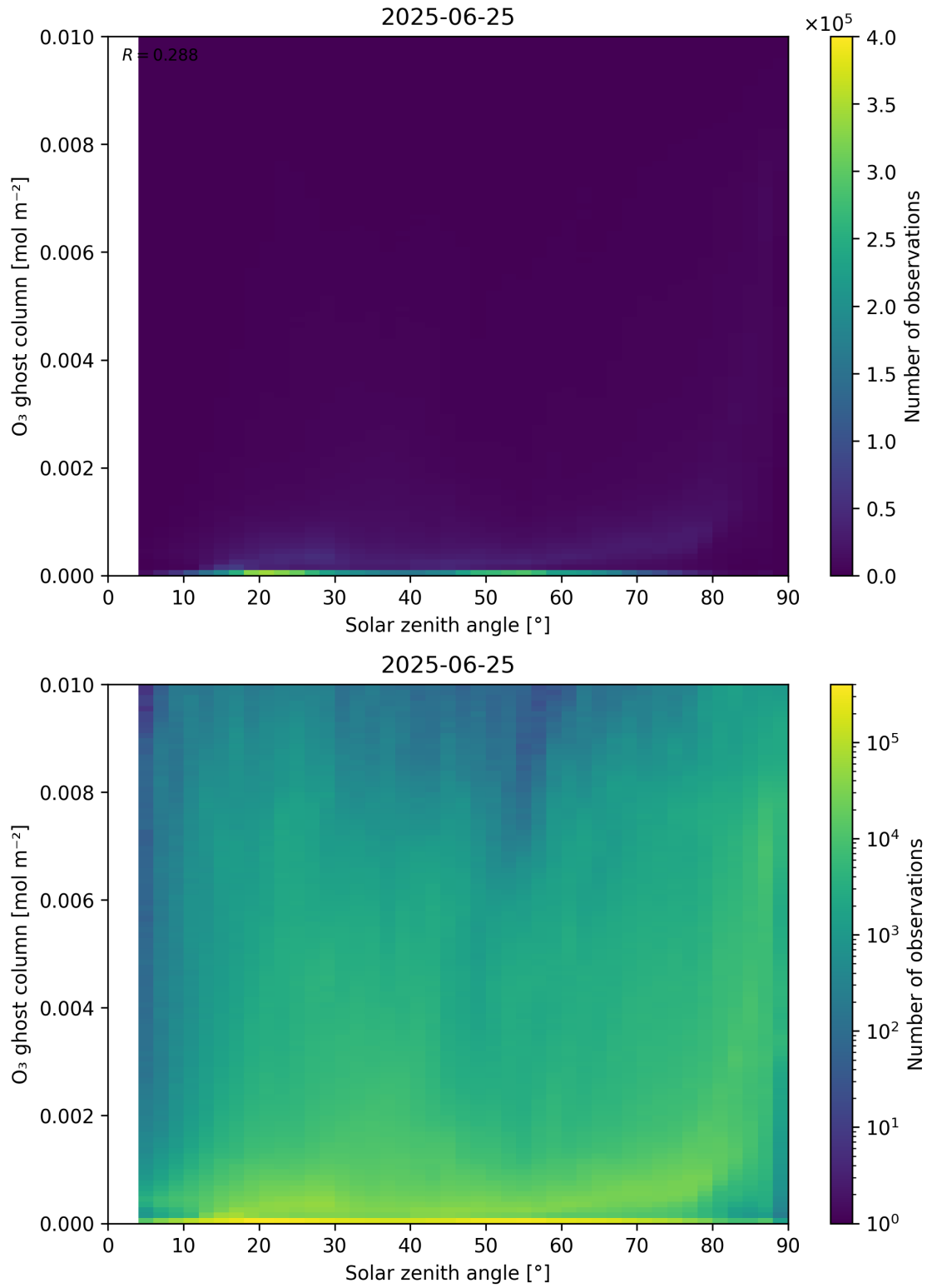
Figure 46: Scatter density plot of “Solar zenith angle” against “O 3 ghost column” for 2025-06-24 to 2025-06-26.
