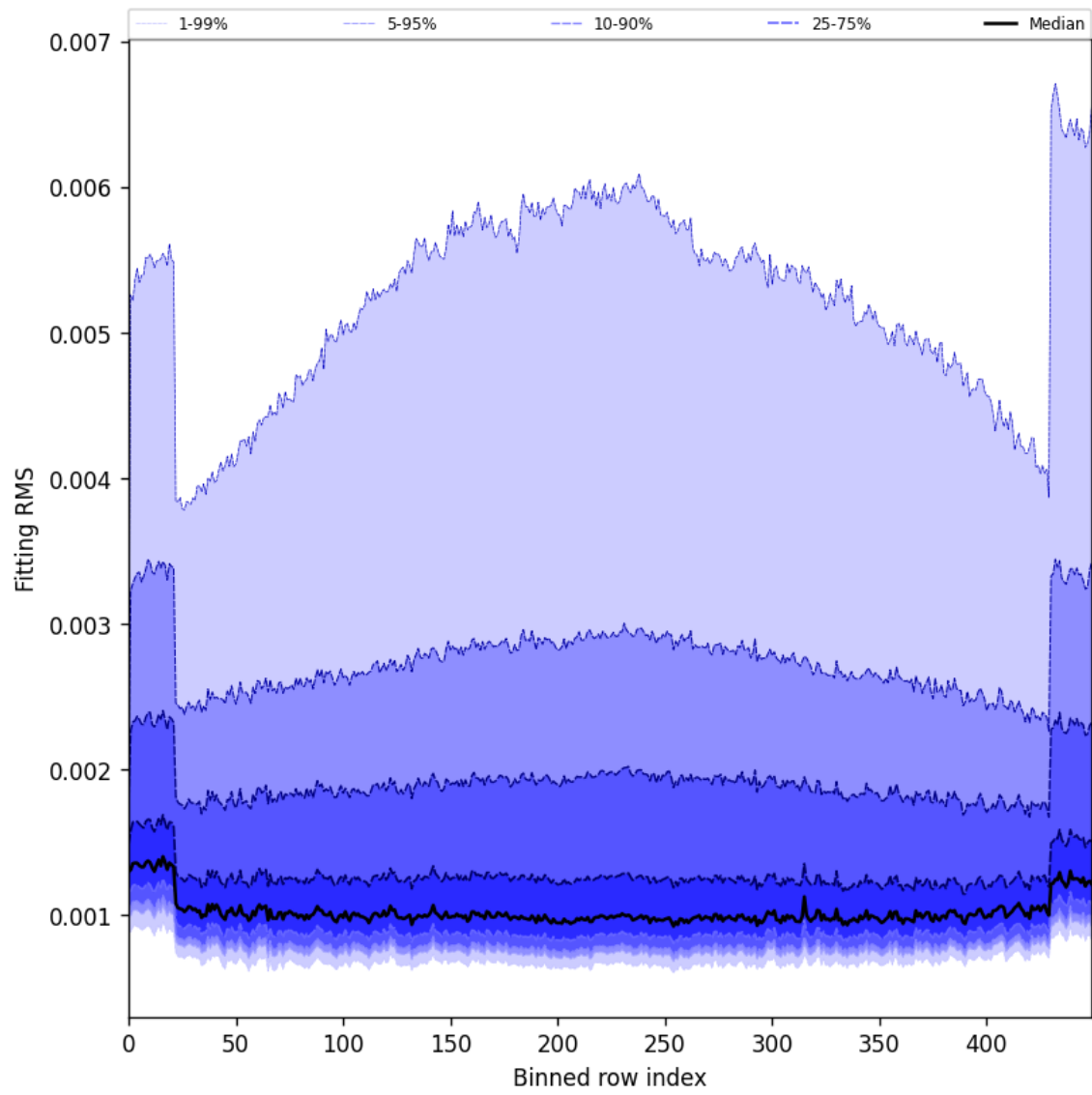
Figure 30: Along track statistics of “Fitting RMS” for 2025-06-24 to 2025-06-26
