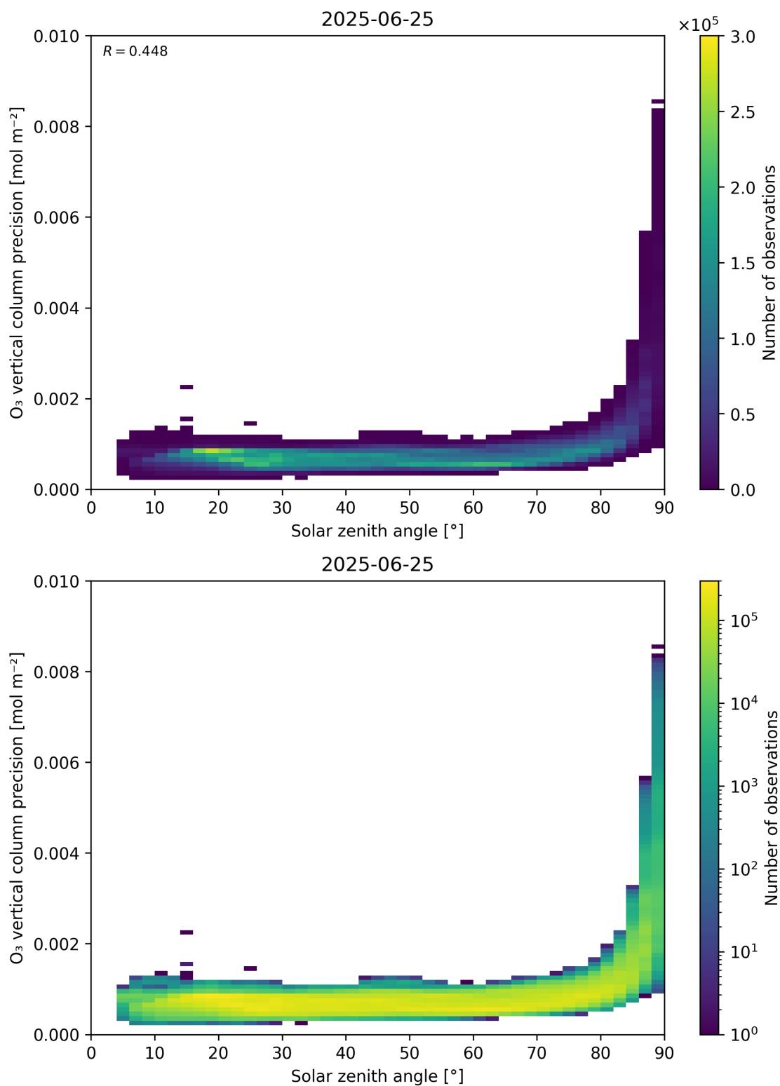
Figure 48: Scatter density plot of “Solar zenith angle” against “O 3 vertical column precision” for 2025-06-24 to 2025-06-26.
