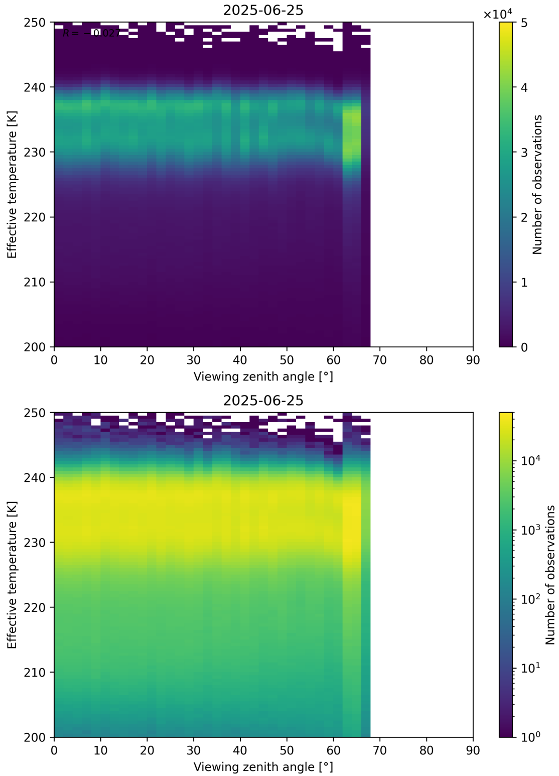
Figure 50: Scatter density plot of “Viewing zenith angle” against “Effective temperature” for 2025-06-24 to 2025-06-26.
