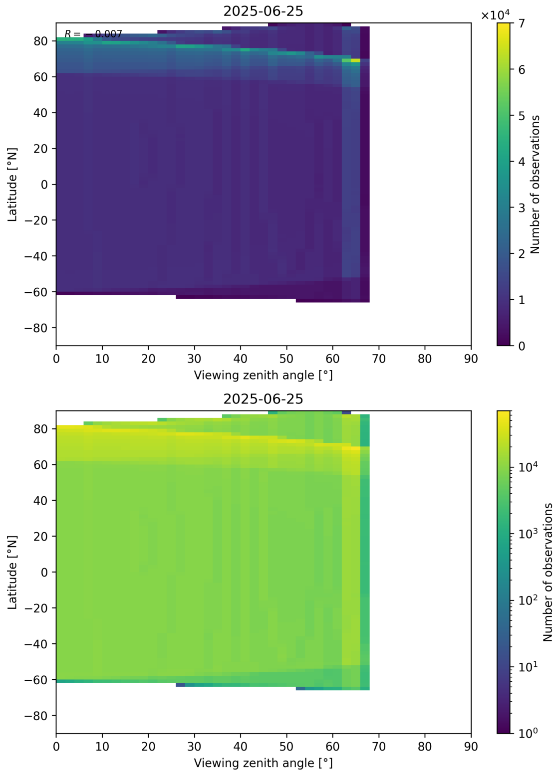
Figure 49: Scatter density plot of “Viewing zenith angle” against “Latitude” for 2025-06-24 to 2025-06-26.
