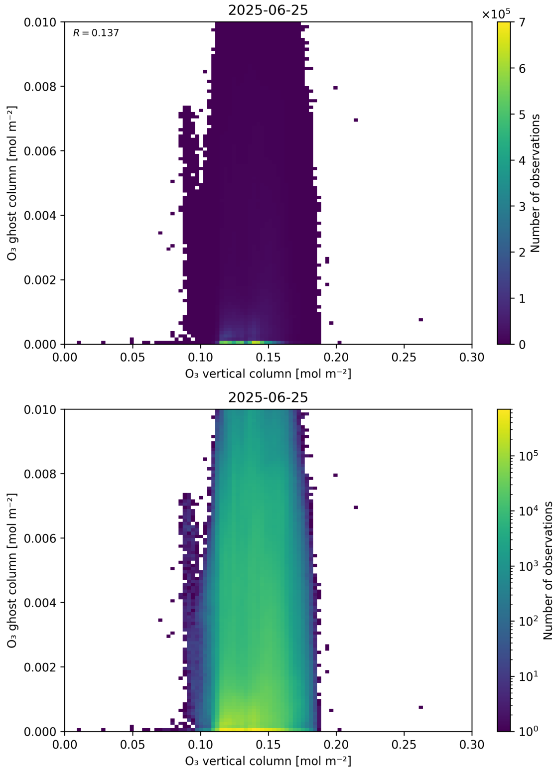
Figure 40: Scatter density plot of “O 3 vertical column” against “O 3 ghost column” for 2025-06-24 to 2025-06-26.
