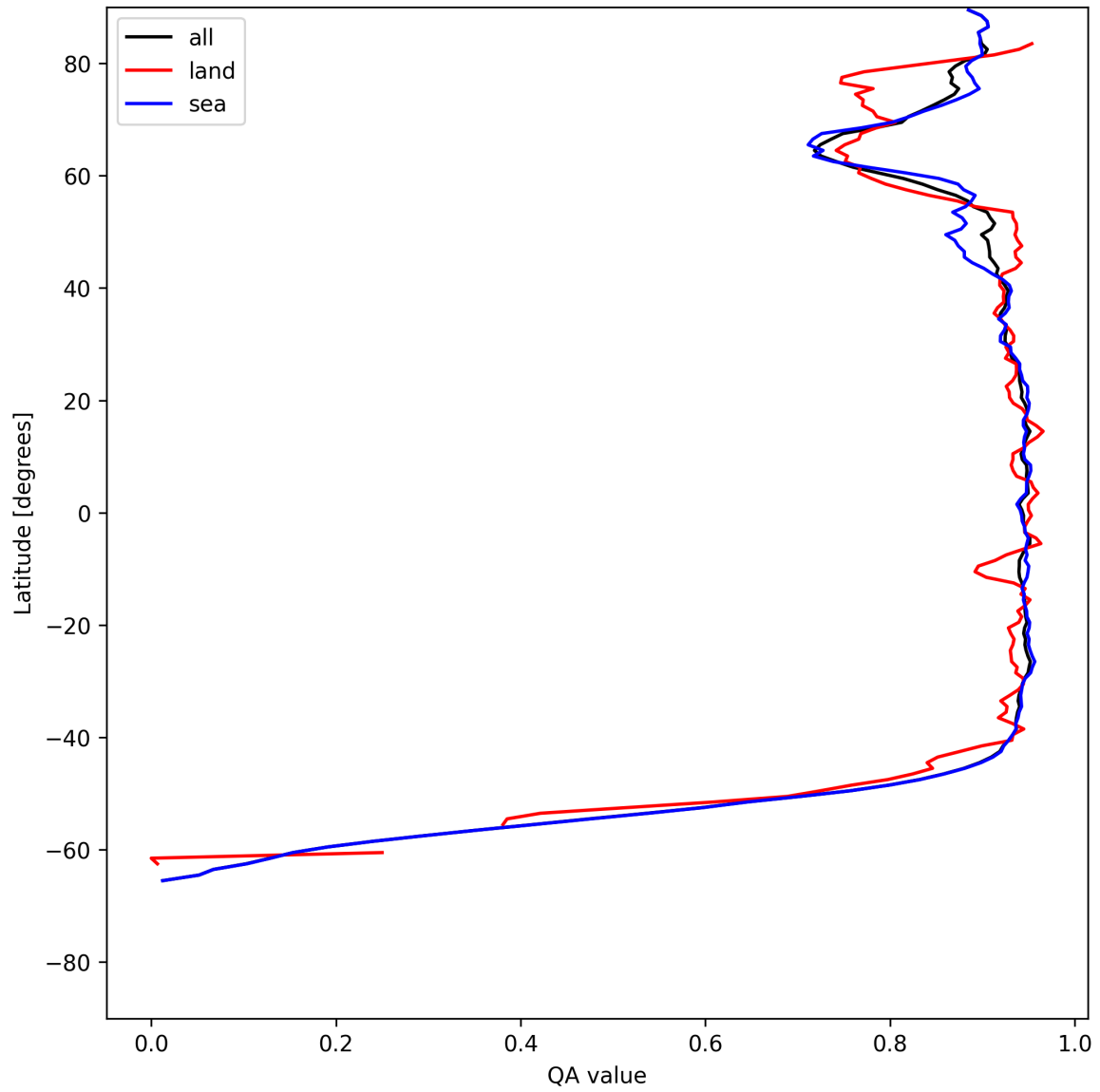
Figure 13: Zonal average of “QA value” for 2025-06-24 to 2025-06-26.
