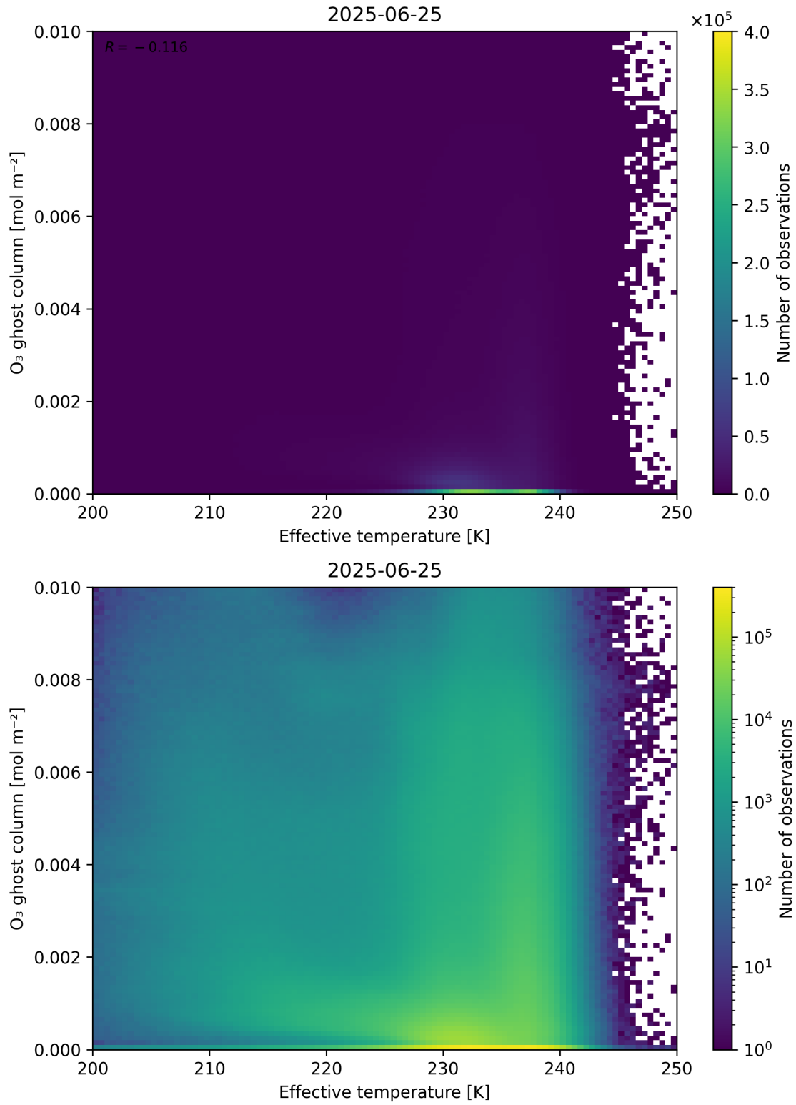
Figure 38: Scatter density plot of “Effective temperature” against “O 3 ghost column” for 2025-06-24 to 2025-06-26.
