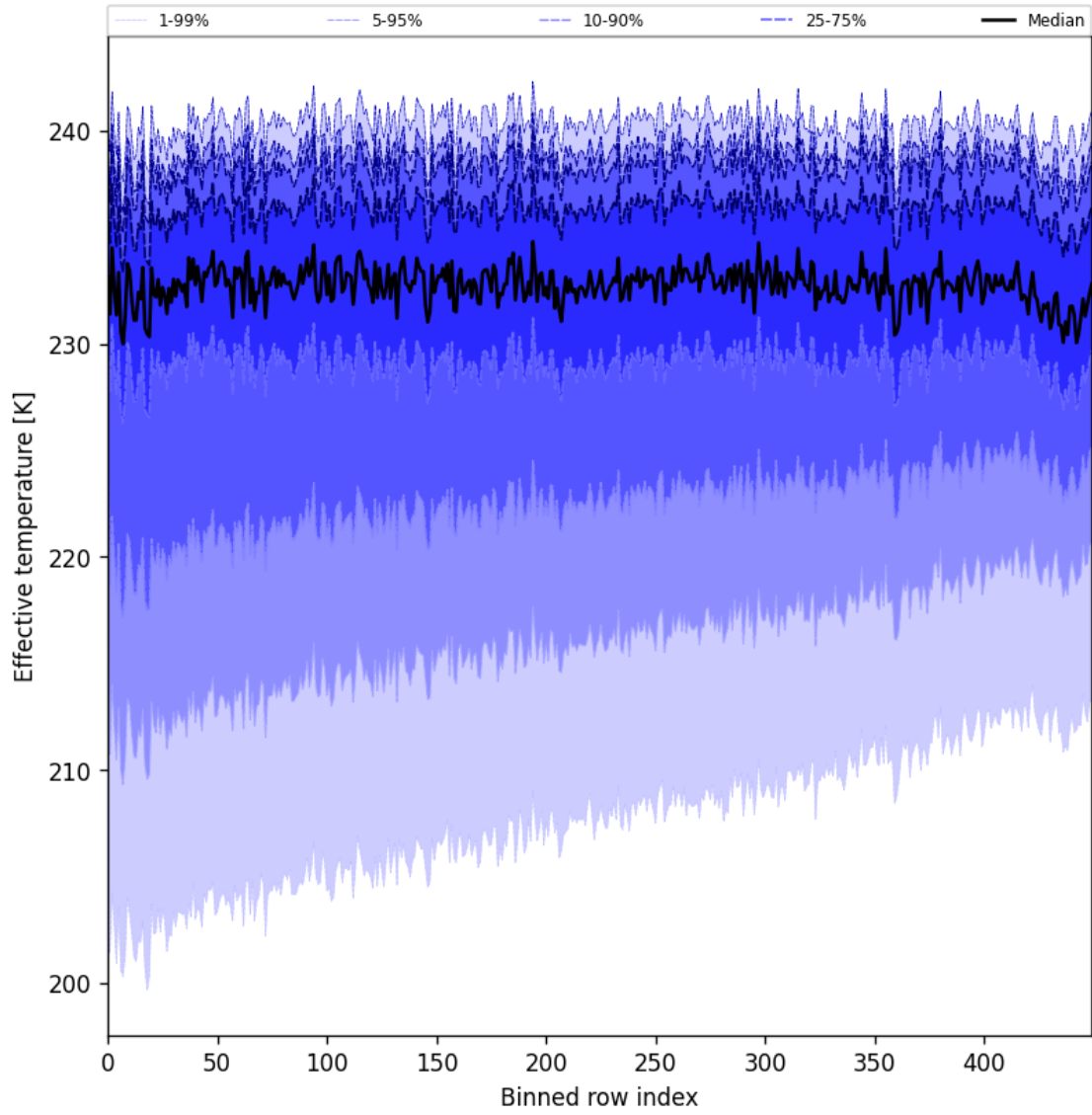
Figure 31: Along track statistics of “Effective temperature” for 2025-06-24 to 2025-06-26
