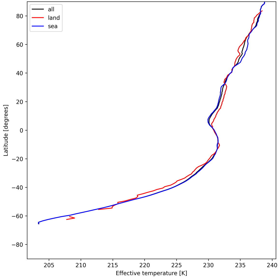
Figure 17: Zonal average of "Effective temperature" for 2025-06-24 to 2025-06-26.
