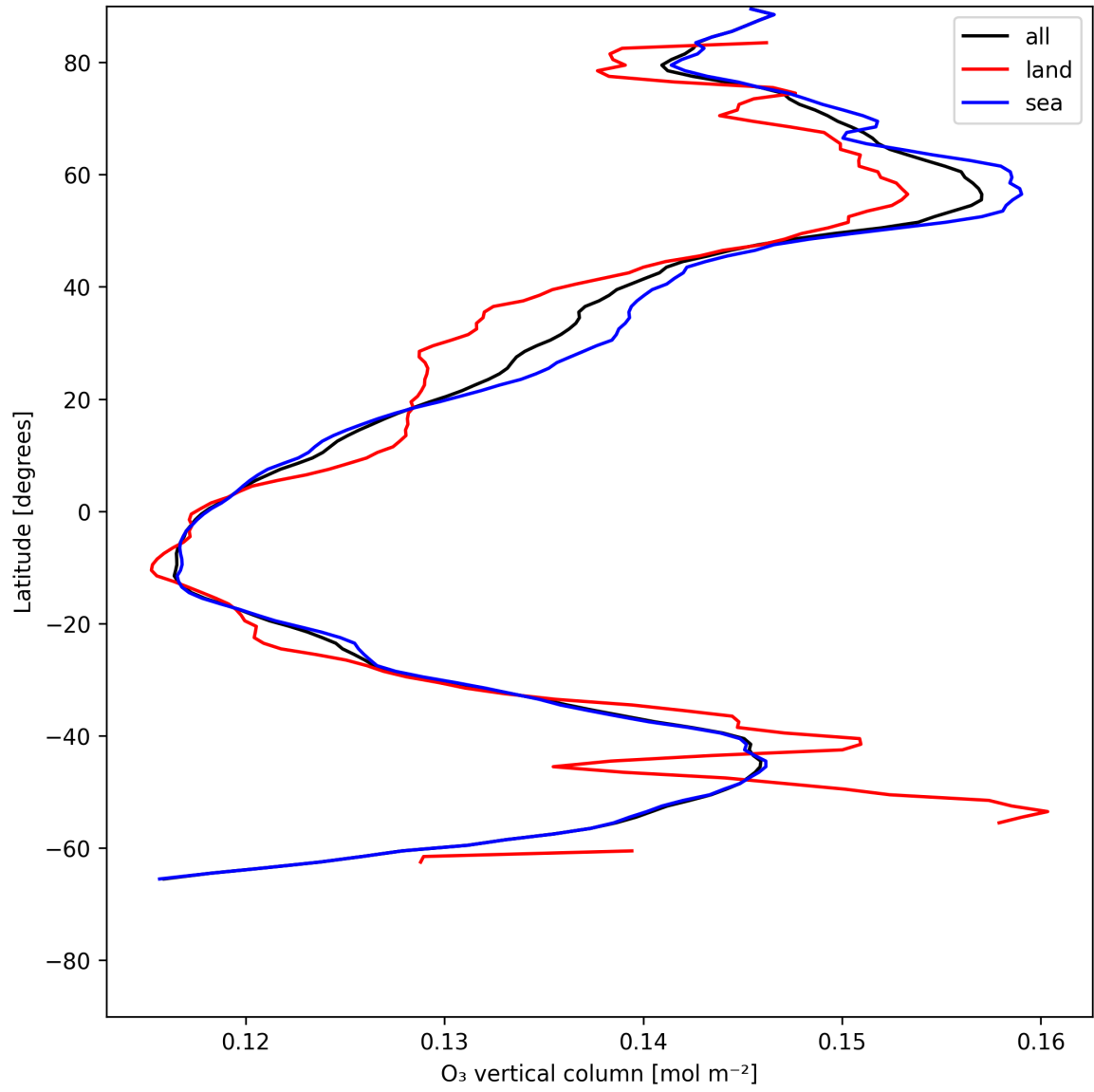
Figure 14: Zonal average of “O 3 vertical column” for 2025-06-24 to 2025-06-26.
