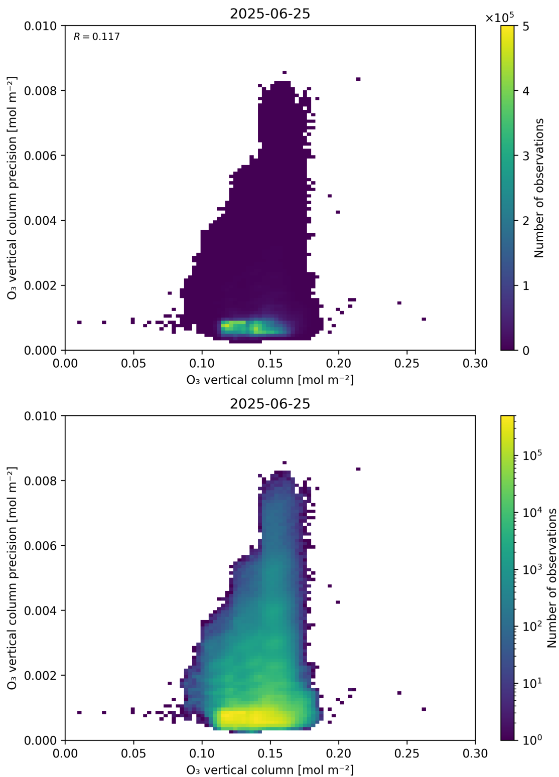
Figure 41: Scatter density plot of “O 3 vertical column” against “O 3 vertical column precision” for 2025-06-24 to 2025-06-26.
