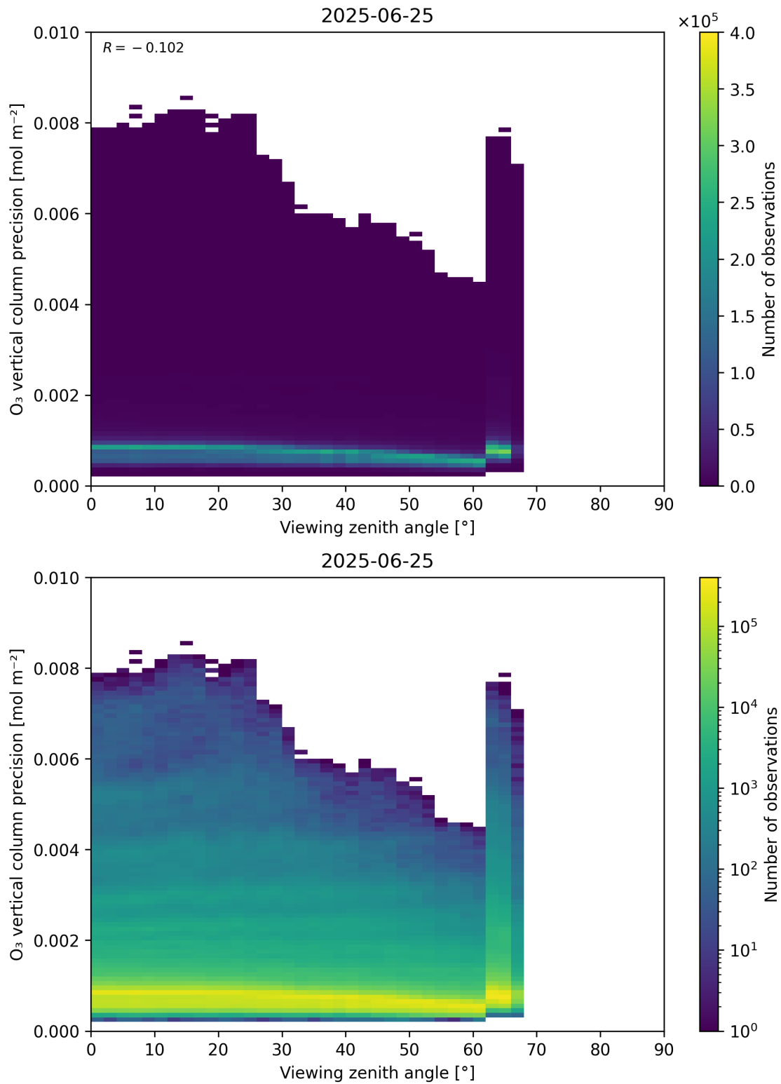
Figure 53: Scatter density plot of “Viewing zenith angle” against “O 3 vertical column precision” for 2025-06-24 to 2025-06-26.
