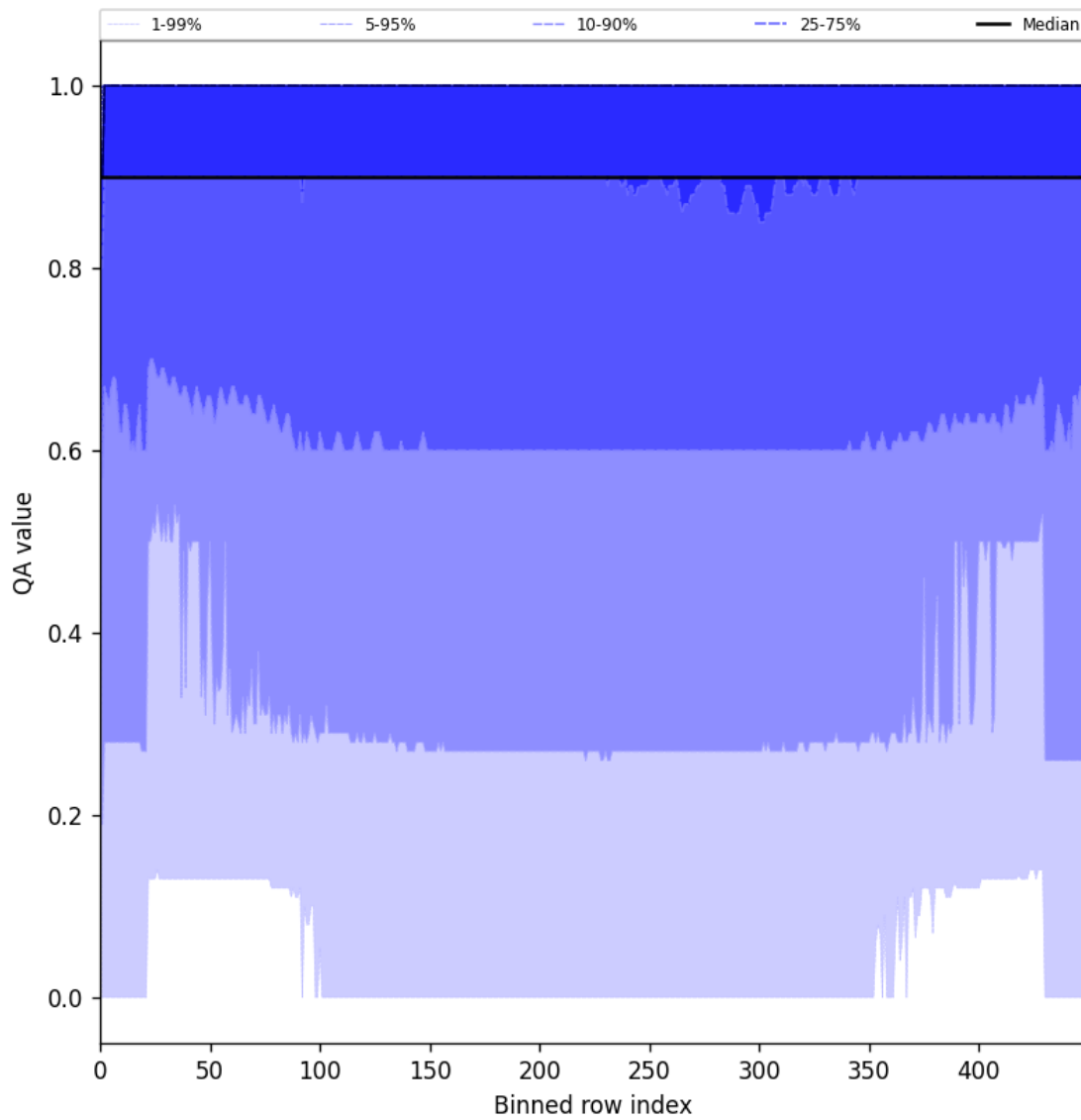
Figure 27: Along track statistics of “QA value” for 2025-06-24 to 2025-06-26
