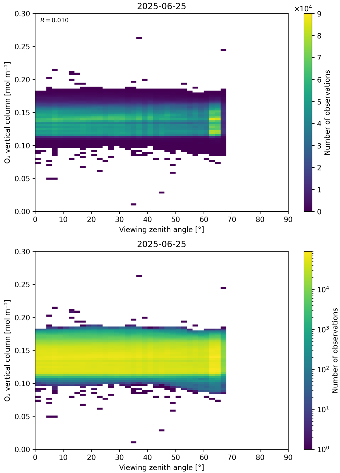
Figure 52: Scatter density plot of “Viewing zenith angle” against “O 3 vertical column” for 2025-06-24 to 2025-06-26.
