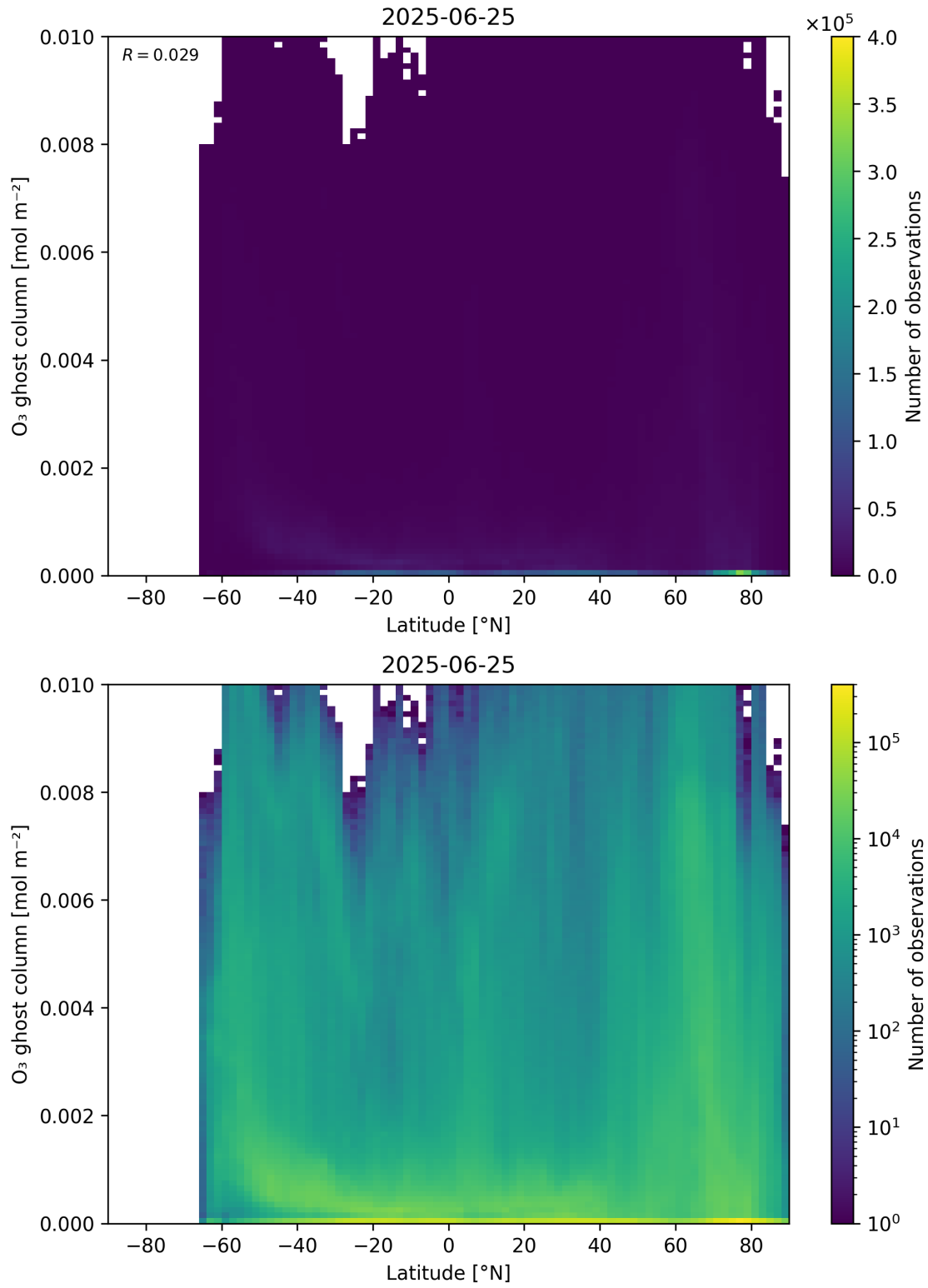
Figure 35: Scatter density plot of “Latitude” against “O 3 ghost column” for 2025-06-24 to 2025-06-26.
