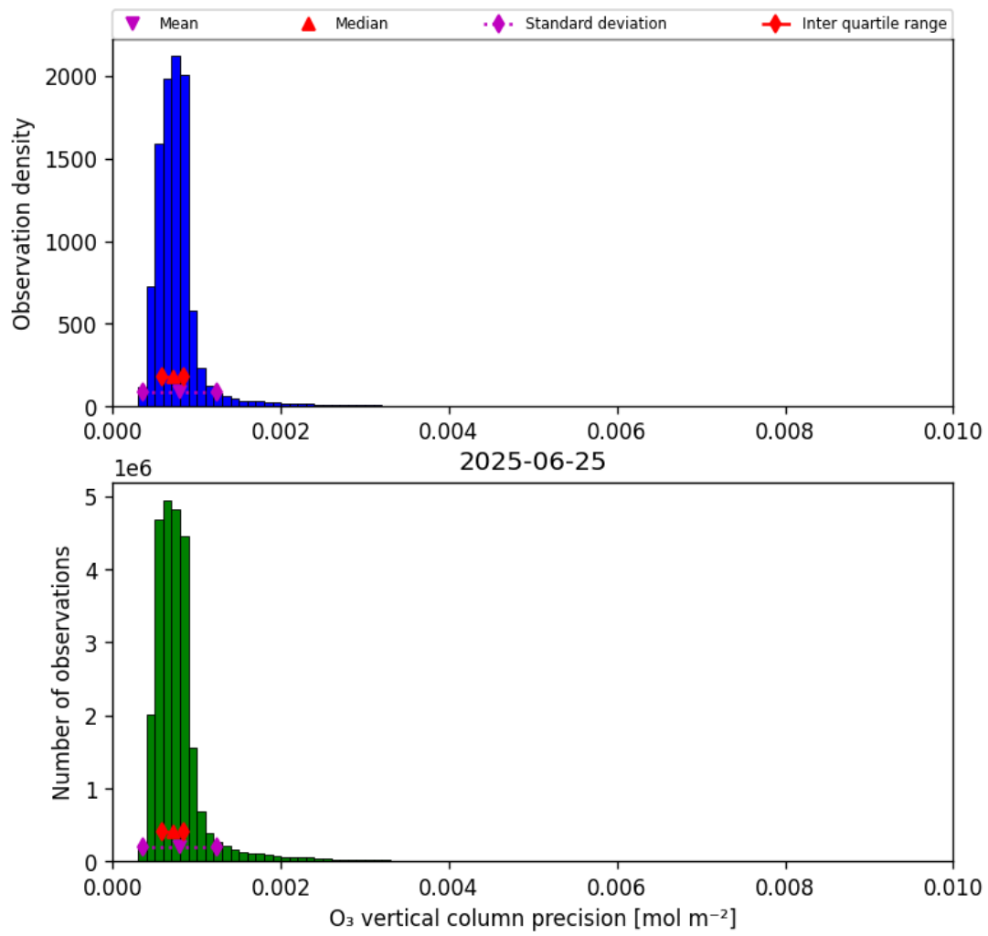
Figure 22: Histogram of “O 3 vertical column precision” for 2025-06-24 to 2025-06-26
