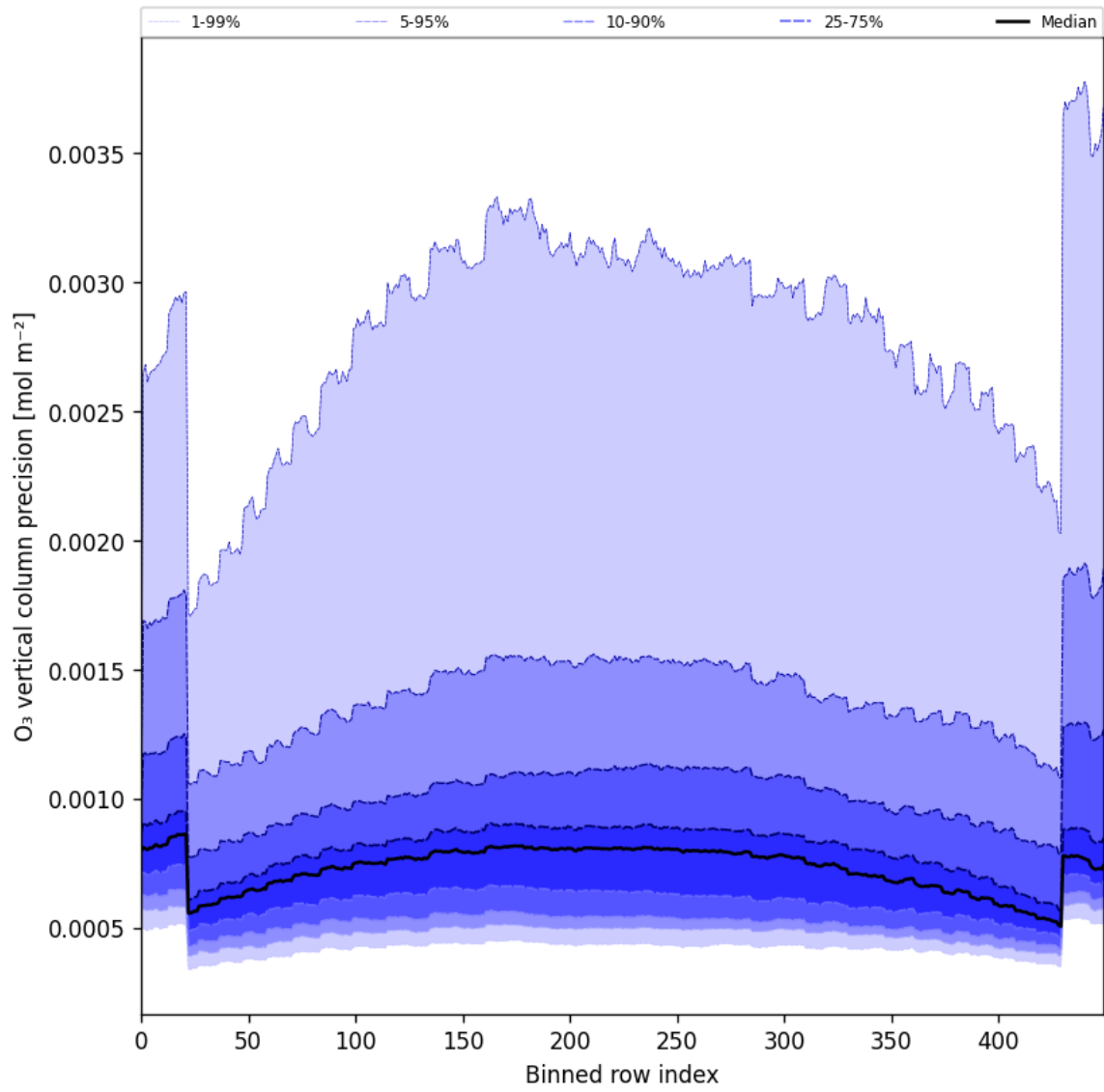
Figure 29: Along track statistics of “O 3 vertical column precision” for 2025-06-24 to 2025-06-26
