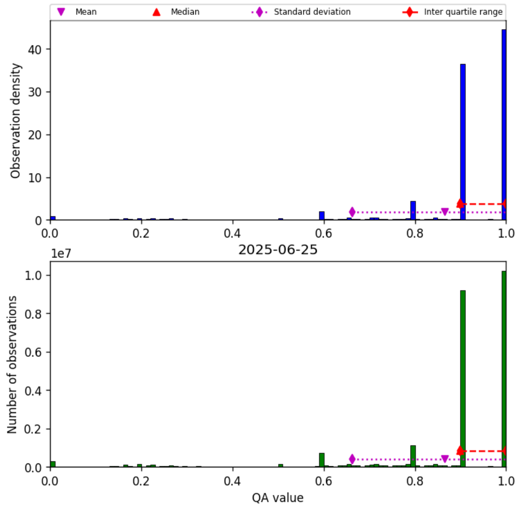
Figure 20: Histogram of “QA value” for 2025-06-24 to 2025-06-26
