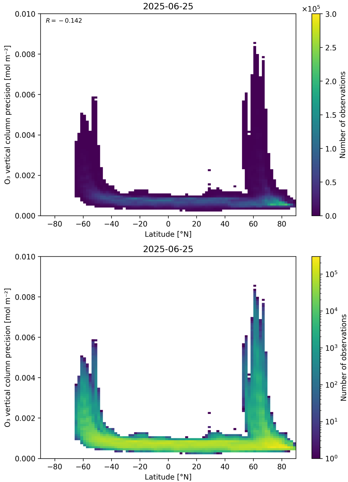
Figure 37: Scatter density plot of “Latitude” against “O 3 vertical column precision” for 2025-06-24 to 2025-06-26.
