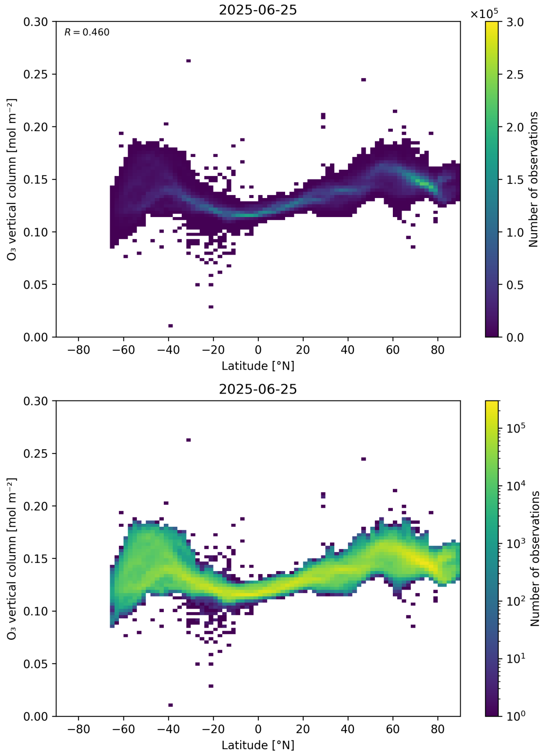
Figure 36: Scatter density plot of “Latitude” against “O 3 vertical column” for 2025-06-24 to 2025-06-26.
