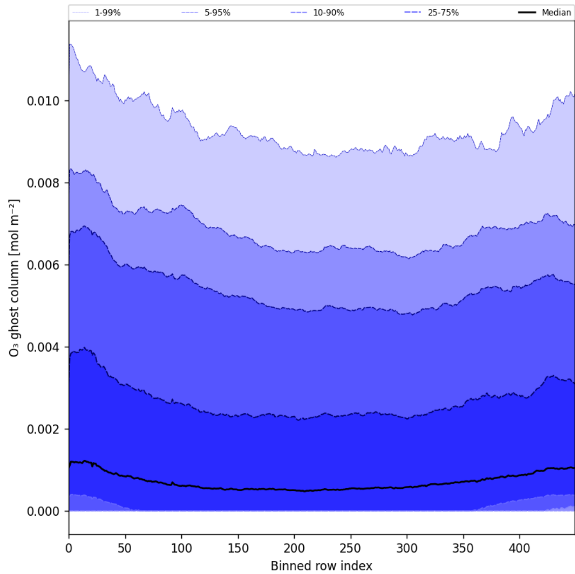
Figure 32: Along track statistics of “O 3 ghost column” for 2025-06-24 to 2025-06-26
