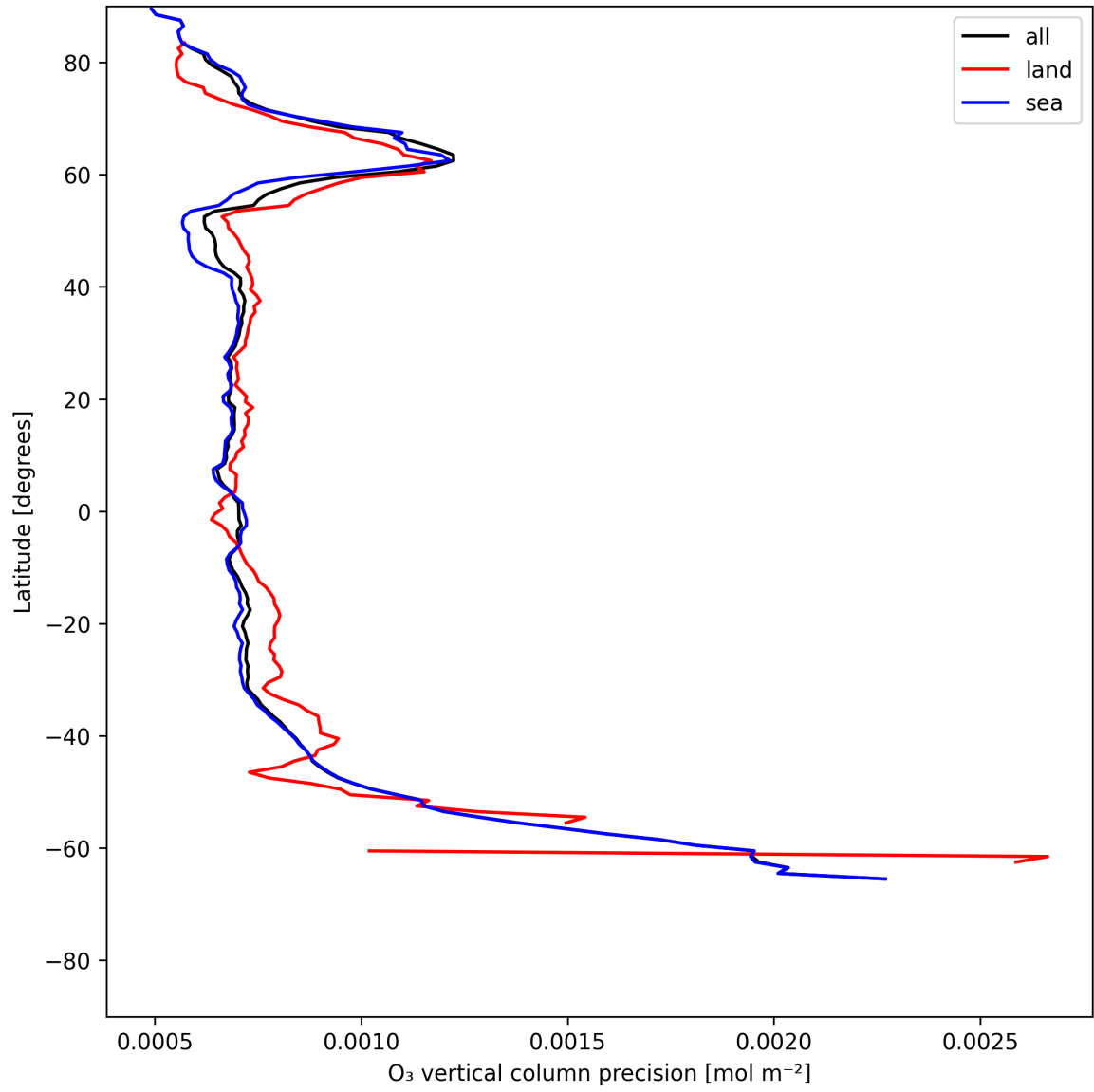
Figure 15: Zonal average of “O 3 vertical column precision” for 2025-06-24 to 2025-06-26.
