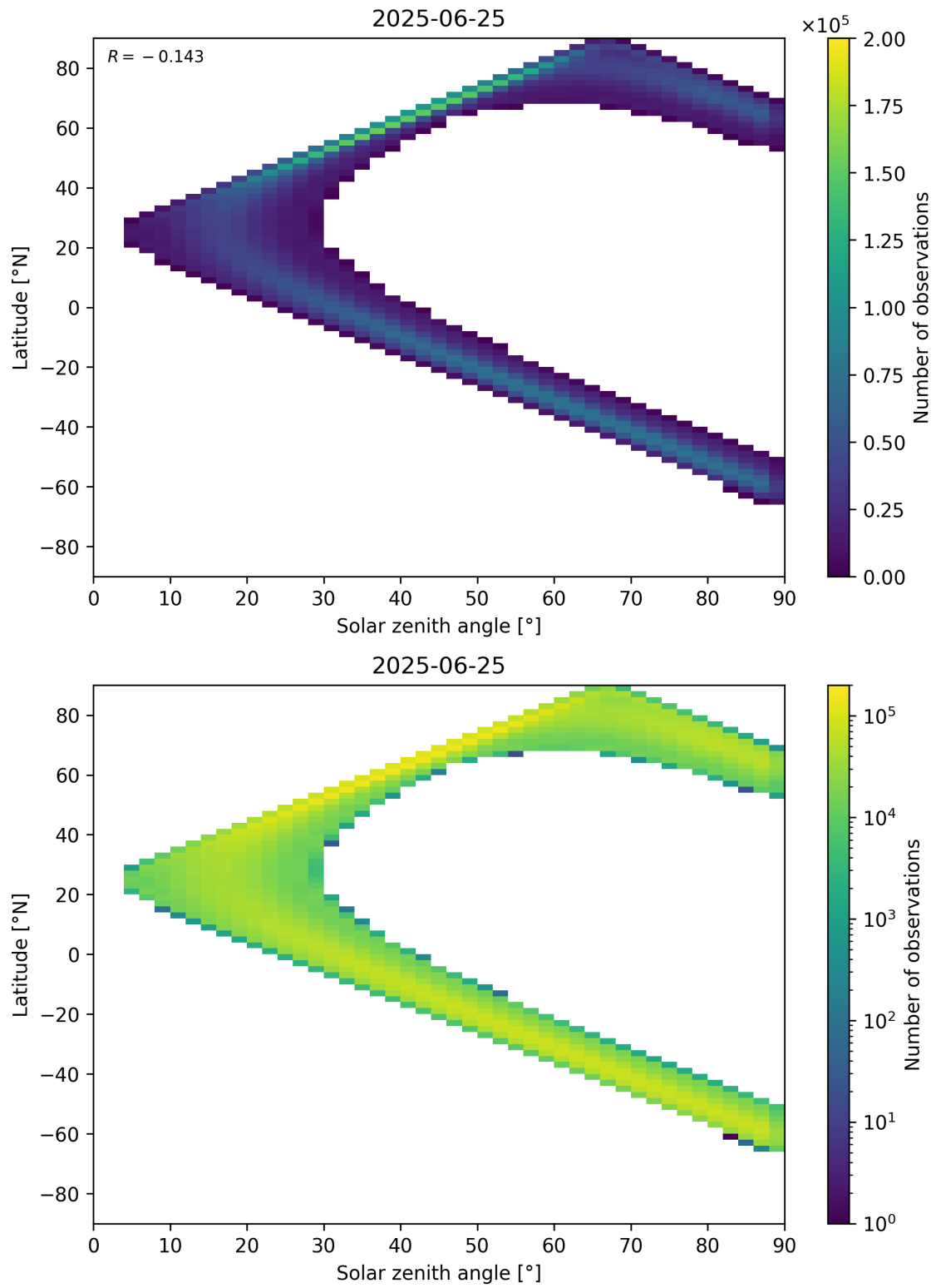
Figure 44: Scatter density plot of “Solar zenith angle” against “Latitude” for 2025-06-24 to 2025-06-26.
