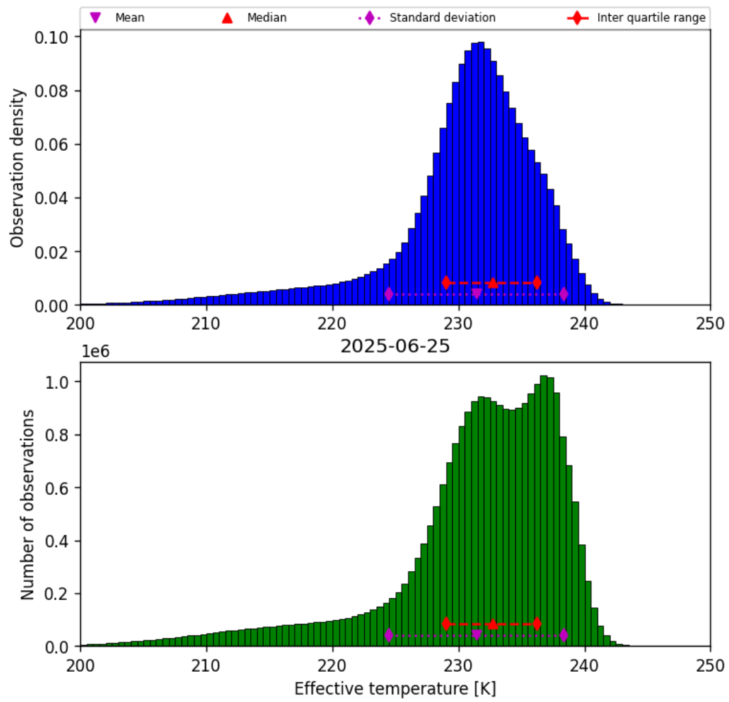
Figure 24: Histogram of “Effective temperature” for 2025-06-24 to 2025-06-26
