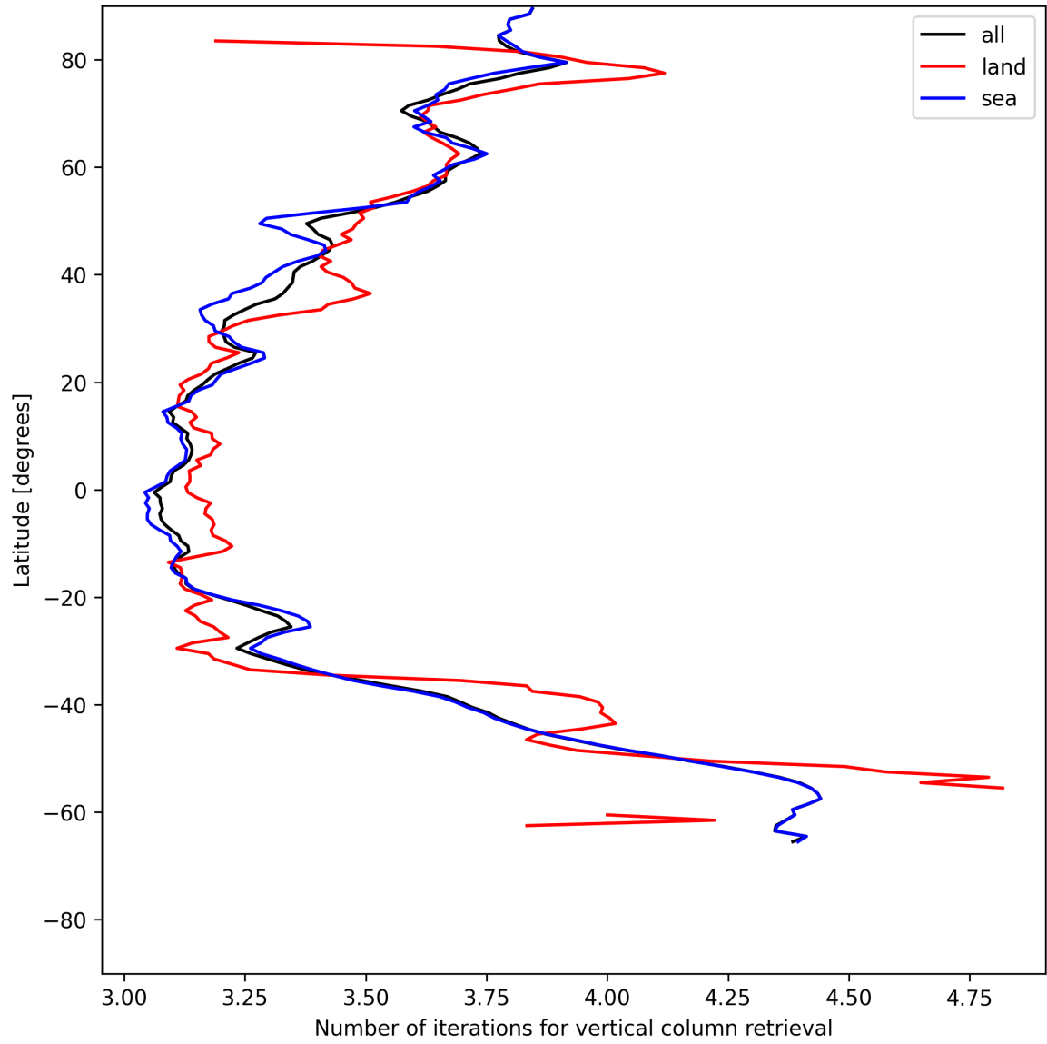
Figure 19: Zonal average of “Number of iterations for vertical column retrieval” for 2025-06-24 to 2025-06-26.
