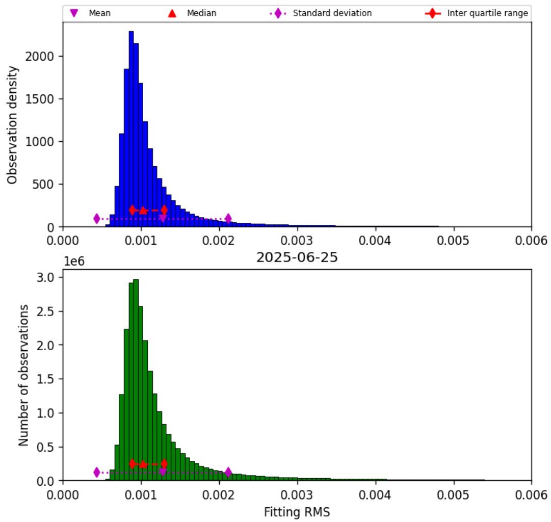
Figure 23: Histogram of “Fitting RMS” for 2025-06-24 to 2025-06-26
