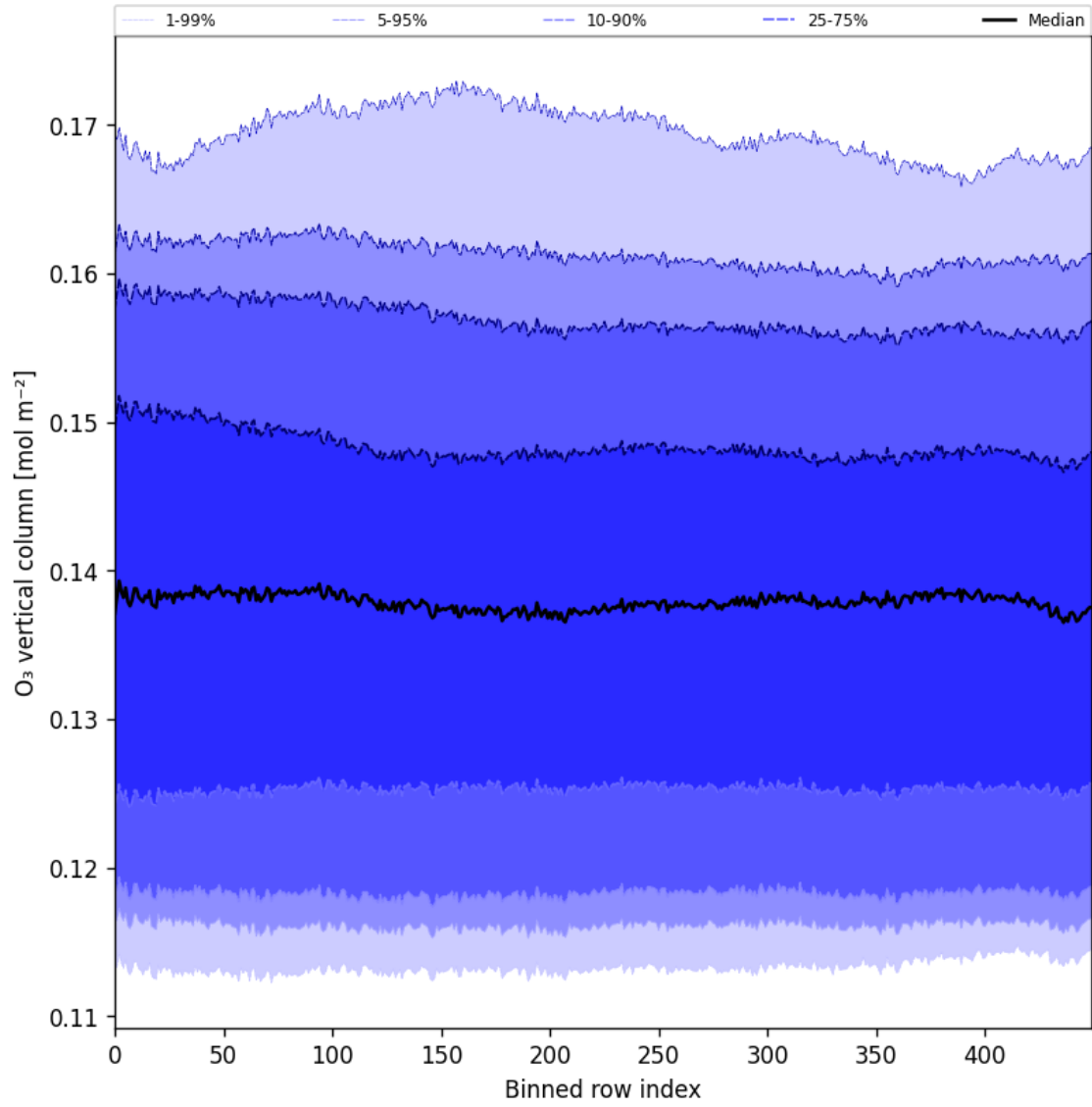
Figure 28: Along track statistics of “O 3 vertical column” for 2025-06-24 to 2025-06-26
