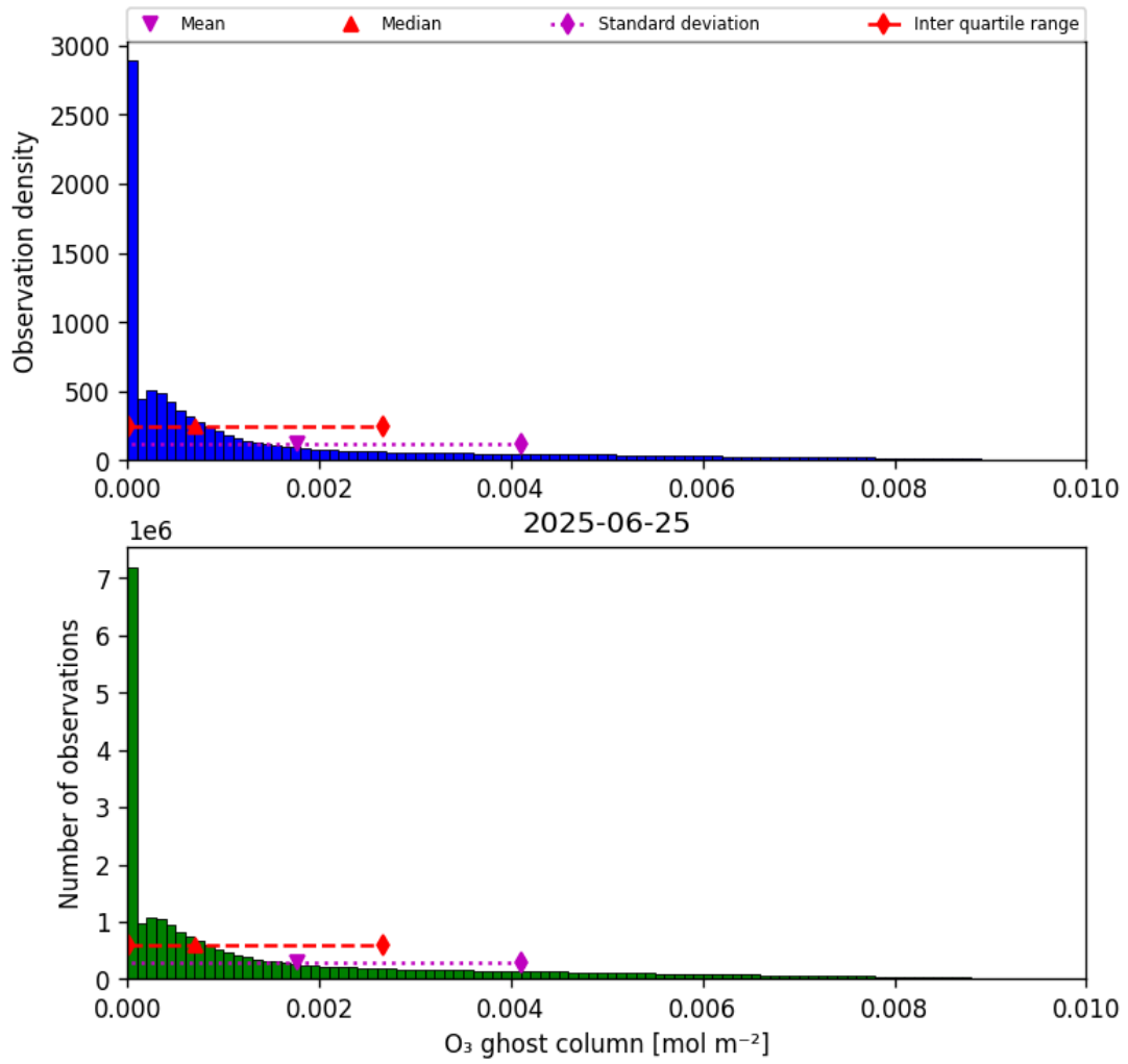
Figure 25: Histogram of “O 3 ghost column” for 2025-06-24 to 2025-06-26
