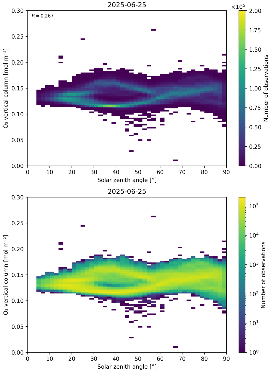
Figure 47: Scatter density plot of “Solar zenith angle” against “O 3 vertical column” for 2025-06-24 to 2025-06-26.
