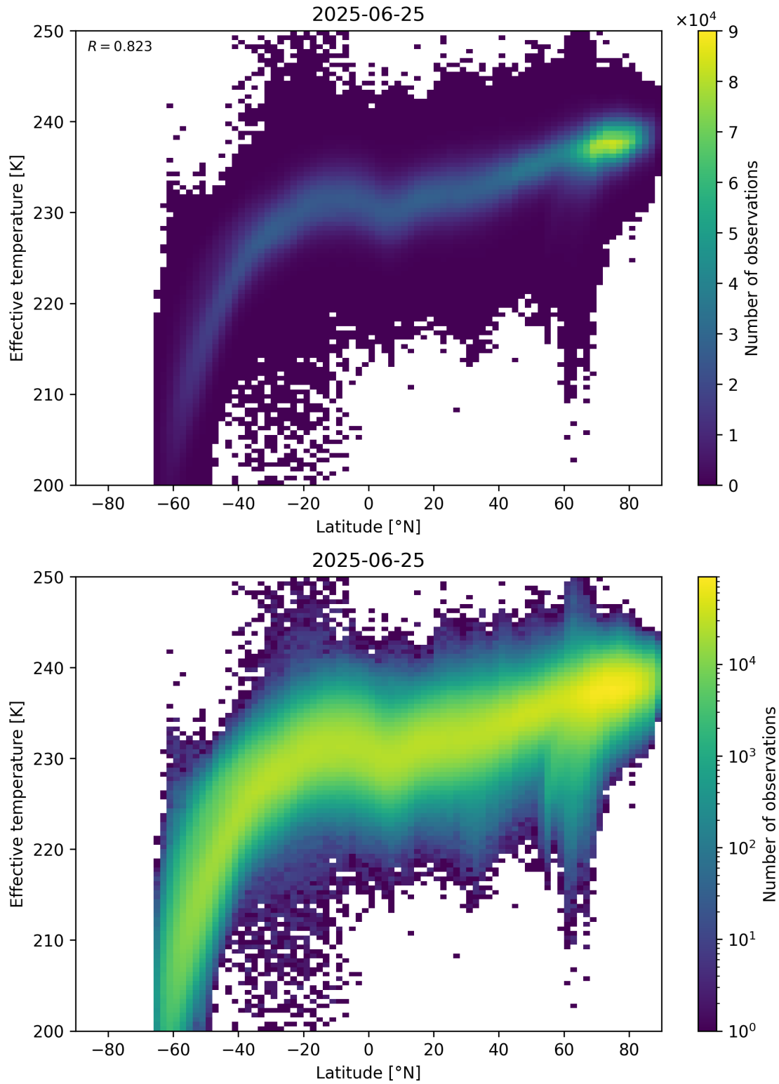
Figure 34: Scatter density plot of “Latitude” against “Effective temperature” for 2025-06-24 to 2025-06-26.
