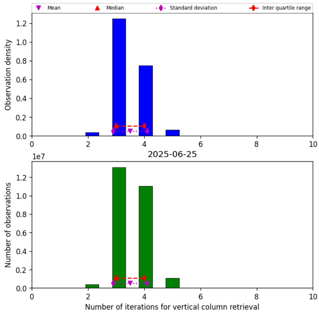
Figure 26: Histogram of “Number of iterations for vertical column retrieval” for 2025-06-24 to 2025-06-26
