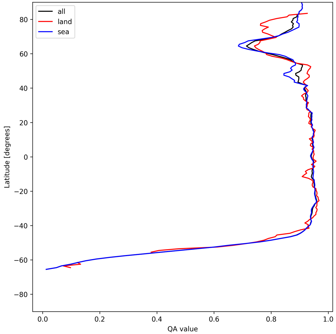
Figure 13: Zonal average of “QA value” for 2025-06-25 to 2025-06-27.
