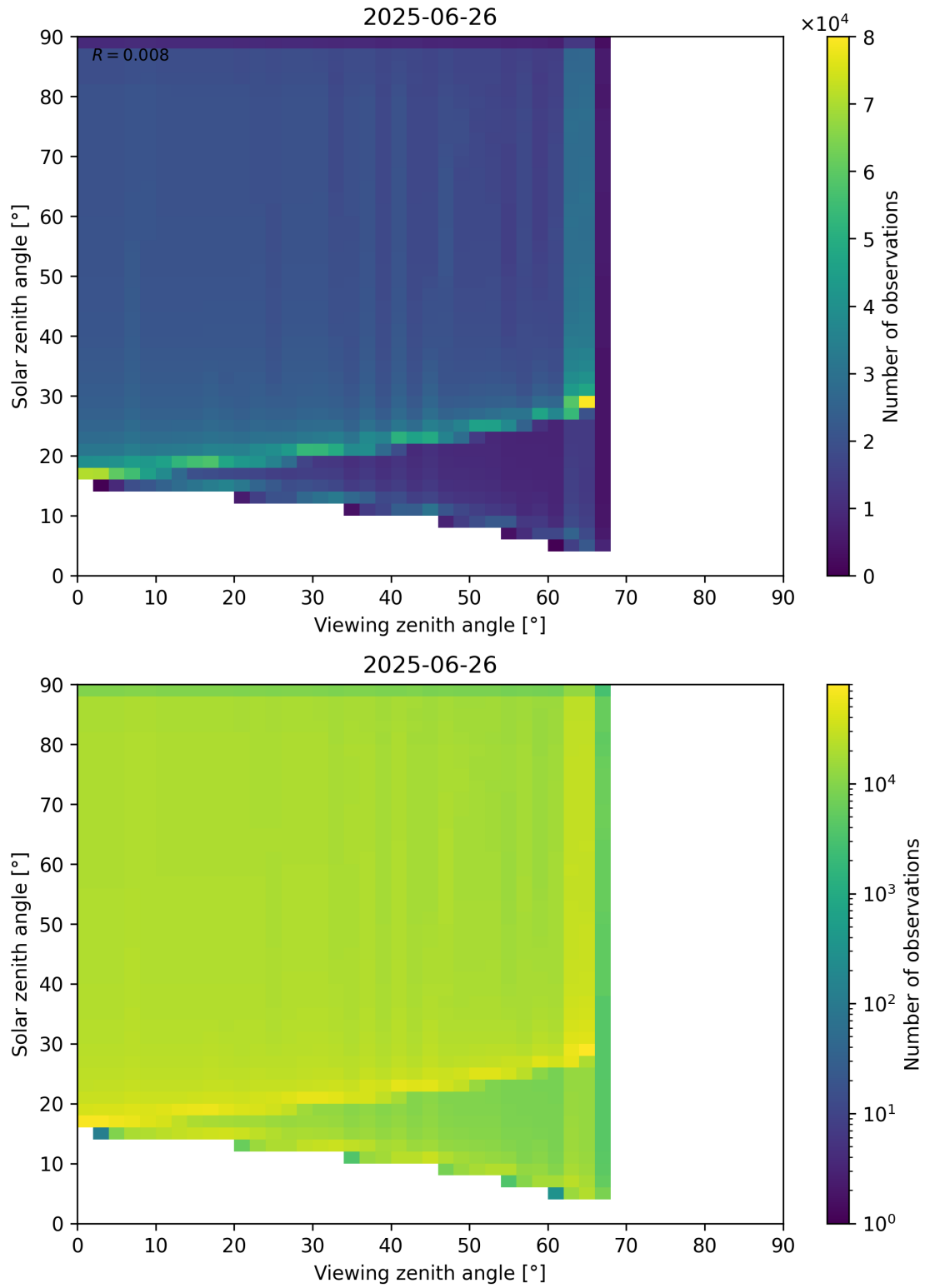
Figure 54: Scatter density plot of “Viewing zenith angle” against “Solar zenith angle” for 2025-06-25 to 2025-06-27.
