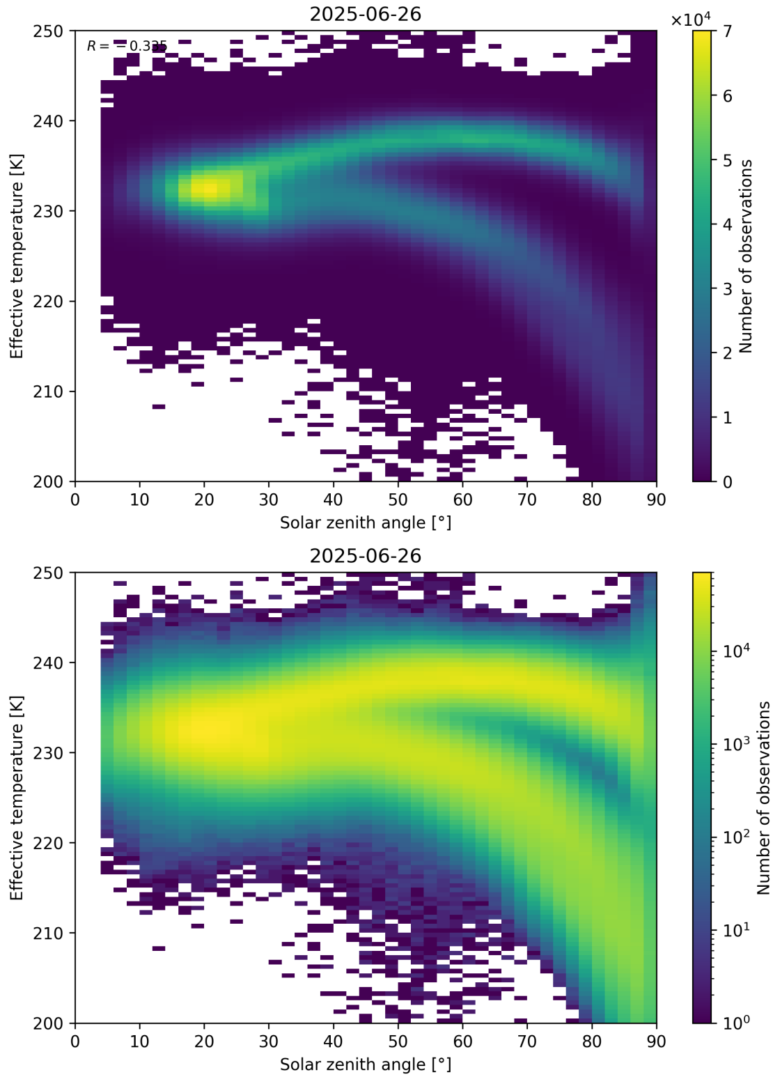
Figure 45: Scatter density plot of “Solar zenith angle” against “Effective temperature” for 2025-06-25 to 2025-06-27.
