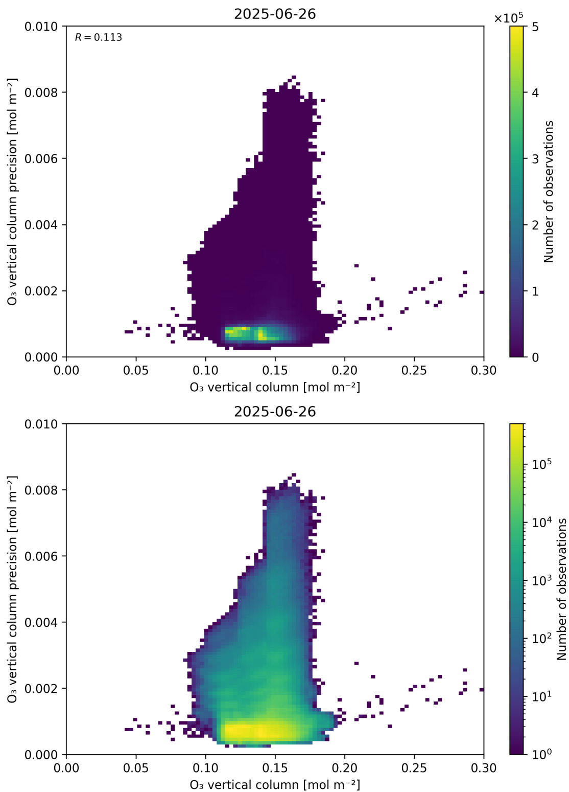
Figure 41: Scatter density plot of “O 3 vertical column” against “O 3 vertical column precision” for 2025-06-25 to 2025-06-27.
