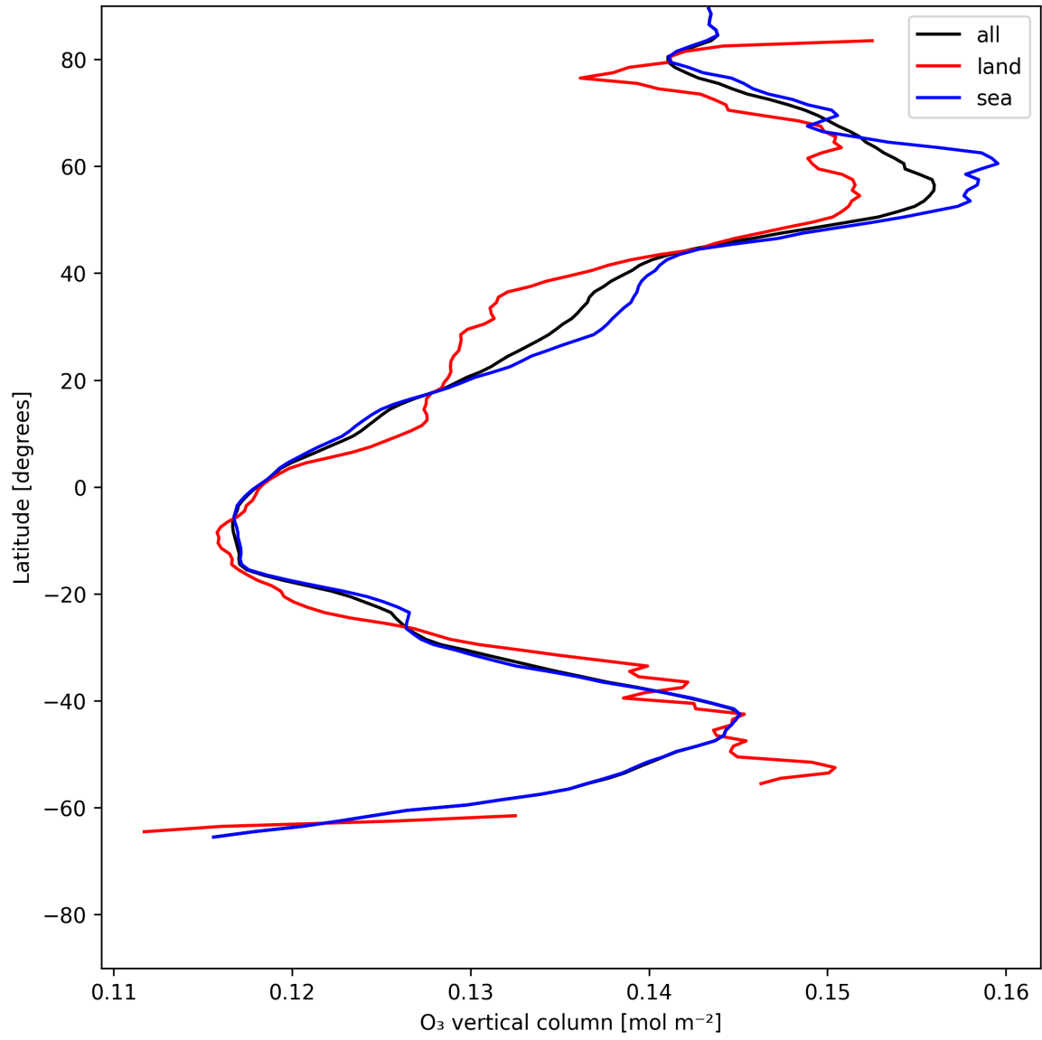
Figure 14: Zonal average of “O 3 vertical column” for 2025-06-25 to 2025-06-27.
