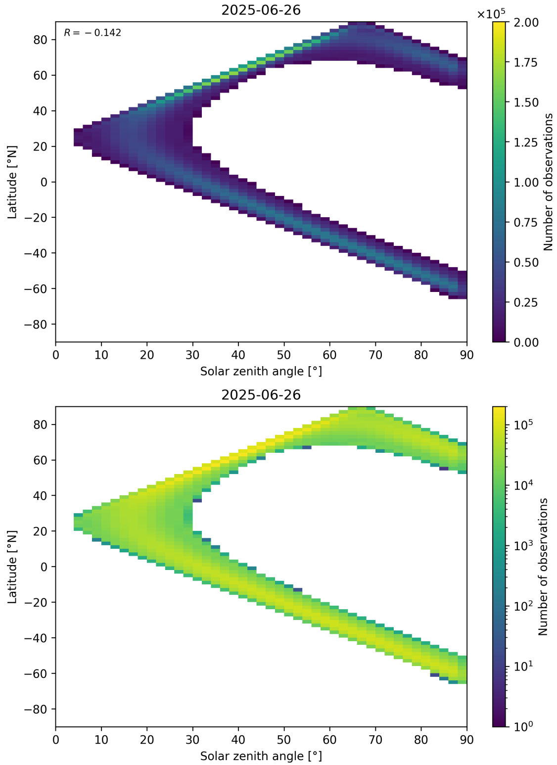
Figure 44: Scatter density plot of “Solar zenith angle” against “Latitude” for 2025-06-25 to 2025-06-27.
