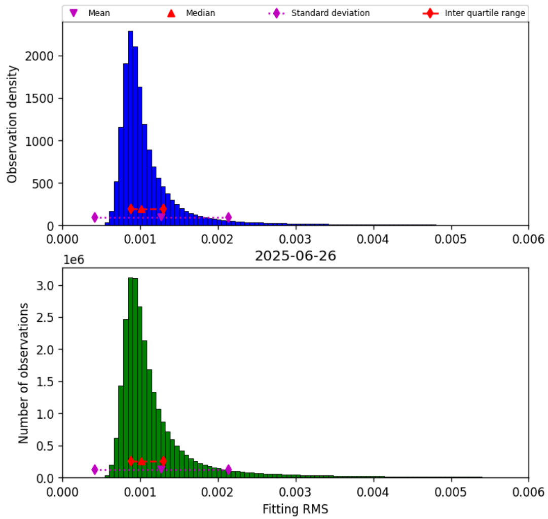
Figure 23: Histogram of “Fitting RMS” for 2025-06-25 to 2025-06-27
