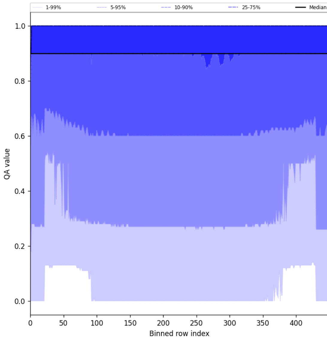
Figure 27: Along track statistics of “QA value” for 2025-06-25 to 2025-06-27
