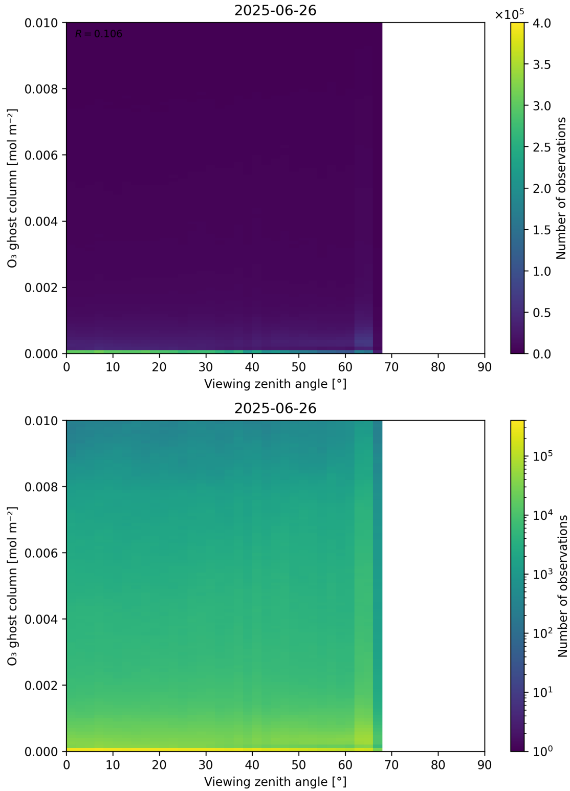
Figure 51: Scatter density plot of “Viewing zenith angle” against “O 3 ghost column” for 2025-06-25 to 2025-06-27.
