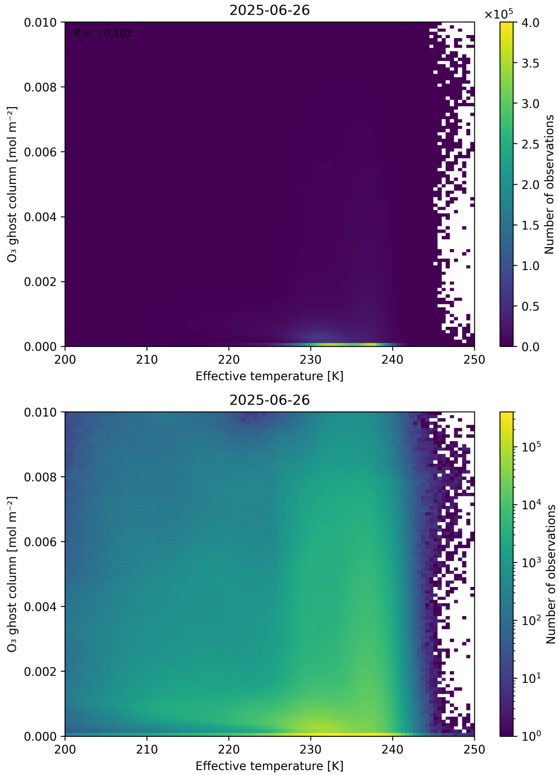
Figure 38: Scatter density plot of “Effective temperature” against “O 3 ghost column” for 2025-06-25 to 2025-06-27.
