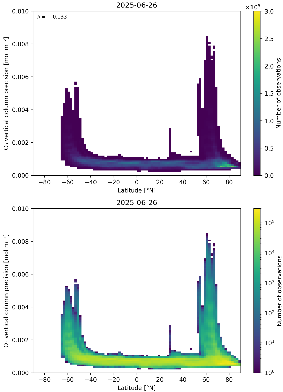
Figure 37: Scatter density plot of “Latitude” against “O 3 vertical column precision” for 2025-06-25 to 2025-06-27.
