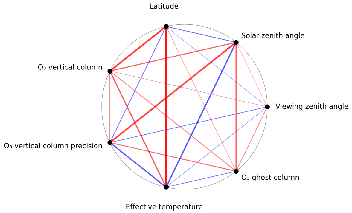
Figure 1: Map of correlation graph for 2025-06-25 to 2025-06-27.
