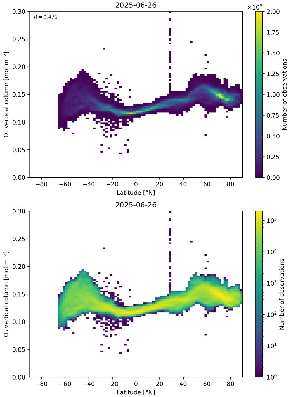
Figure 36: Scatter density plot of “Latitude” against “O 3 vertical column” for 2025-06-25 to 2025-06-27.
