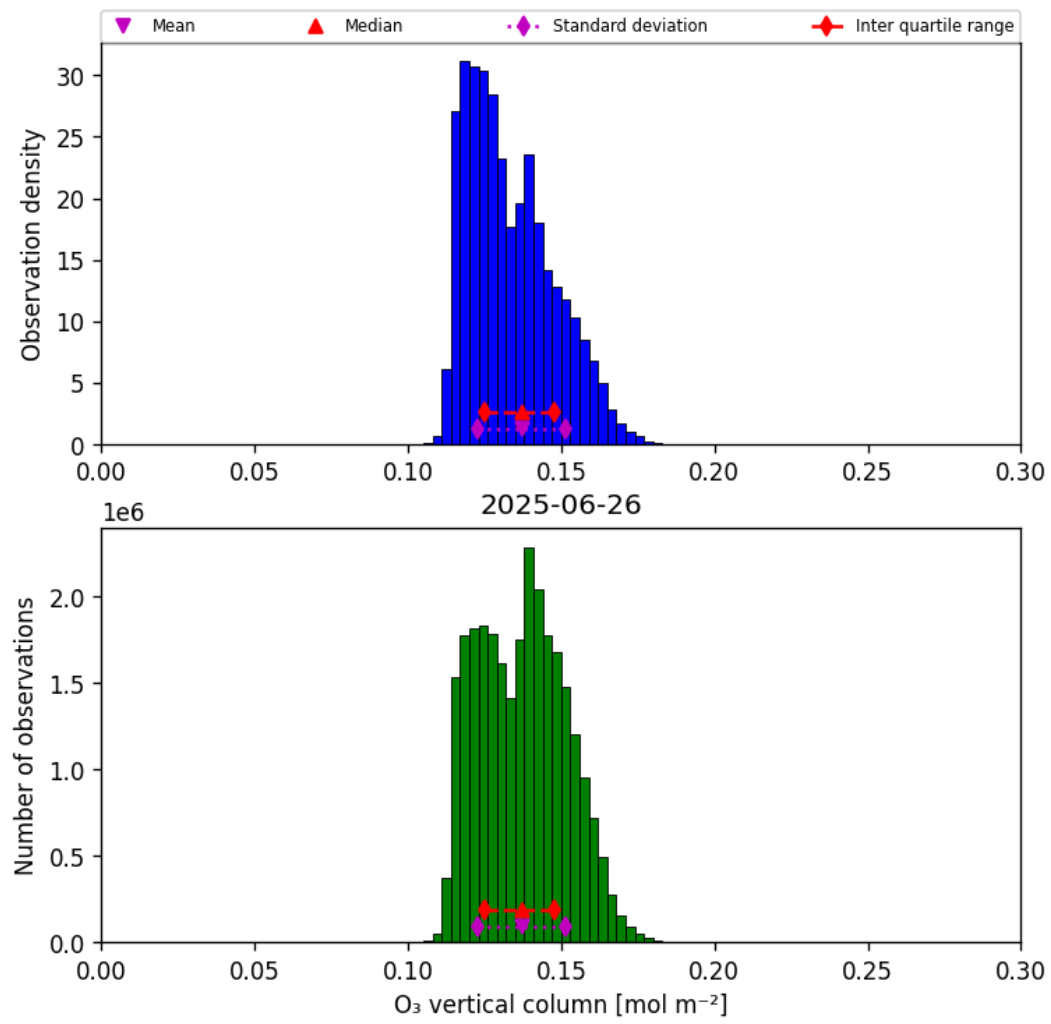
Figure 21: Histogram of “O 3 vertical column” for 2025-06-25 to 2025-06-27
