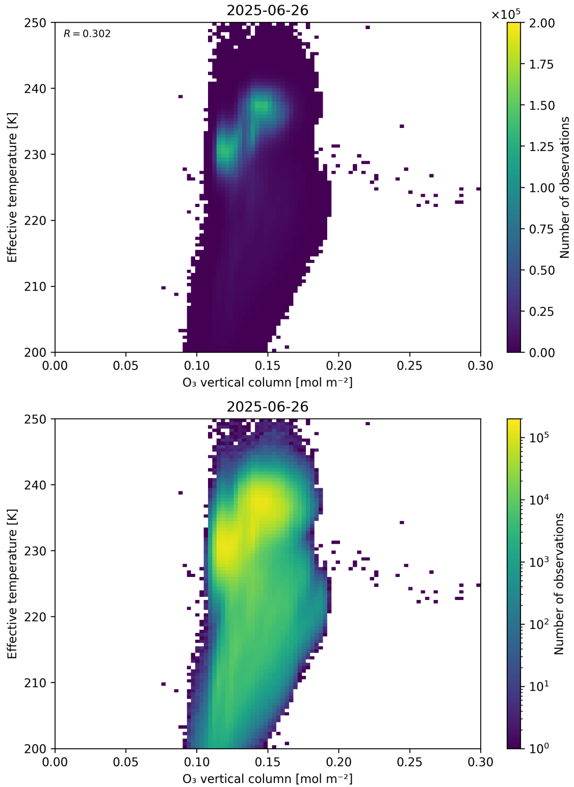
Figure 39: Scatter density plot of “O 3 vertical column” against “Effective temperature” for 2025-06-25 to 2025-06-27.
