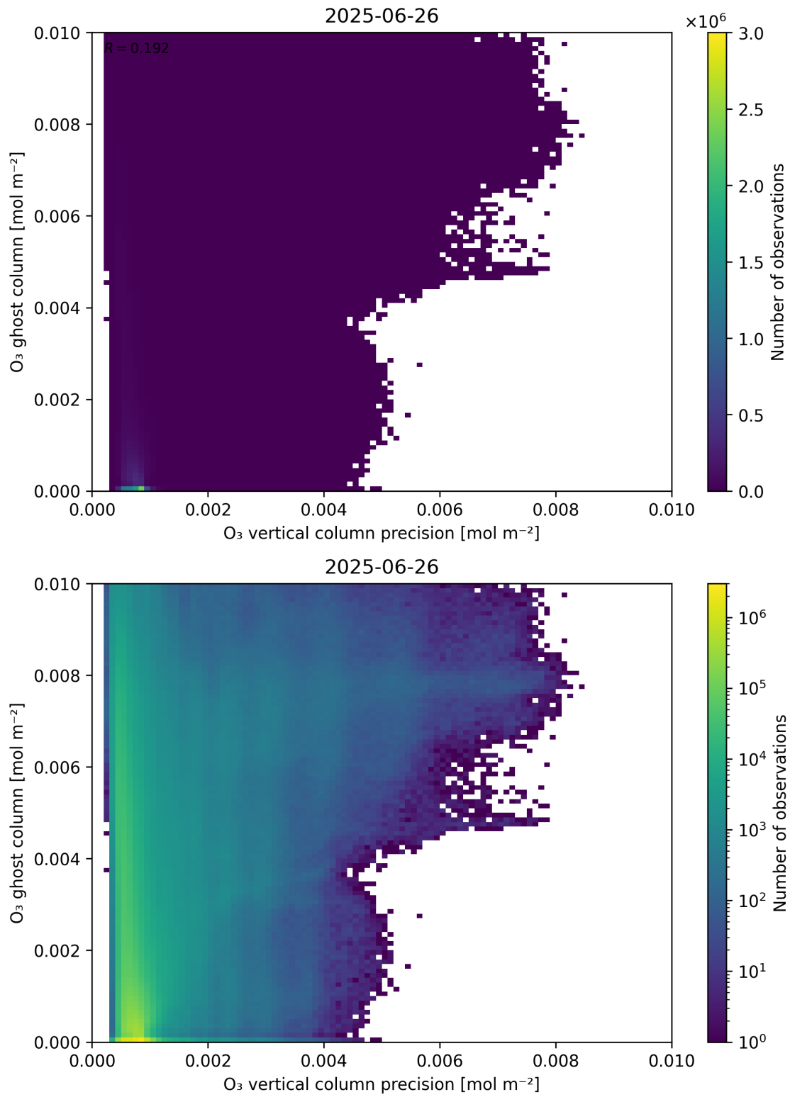
Figure 43: Scatter density plot of “ \text{O}_3 vertical column precision” against “ \text{O}_3 ghost column” for 2025-06-25 to 2025-06-27.
