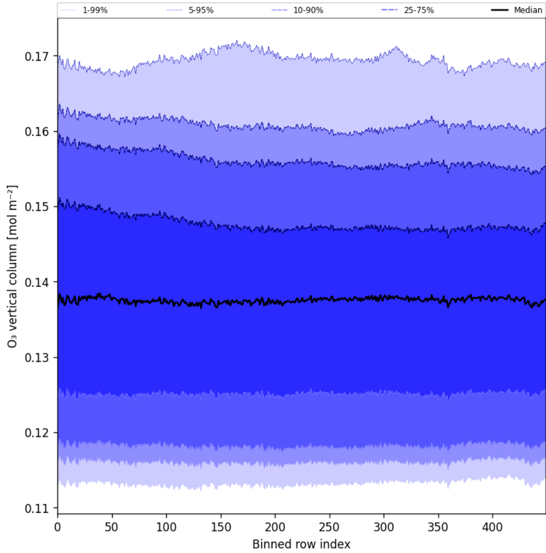
Figure 28: Along track statistics of “O 3 vertical column” for 2025-06-25 to 2025-06-27
