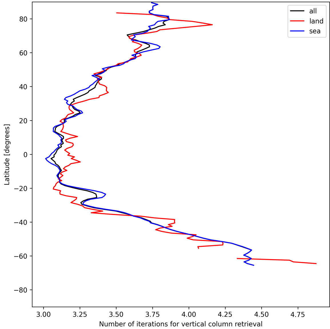
Figure 19: Zonal average of “Number of iterations for vertical column retrieval” for 2025-06-25 to 2025-06-27.
