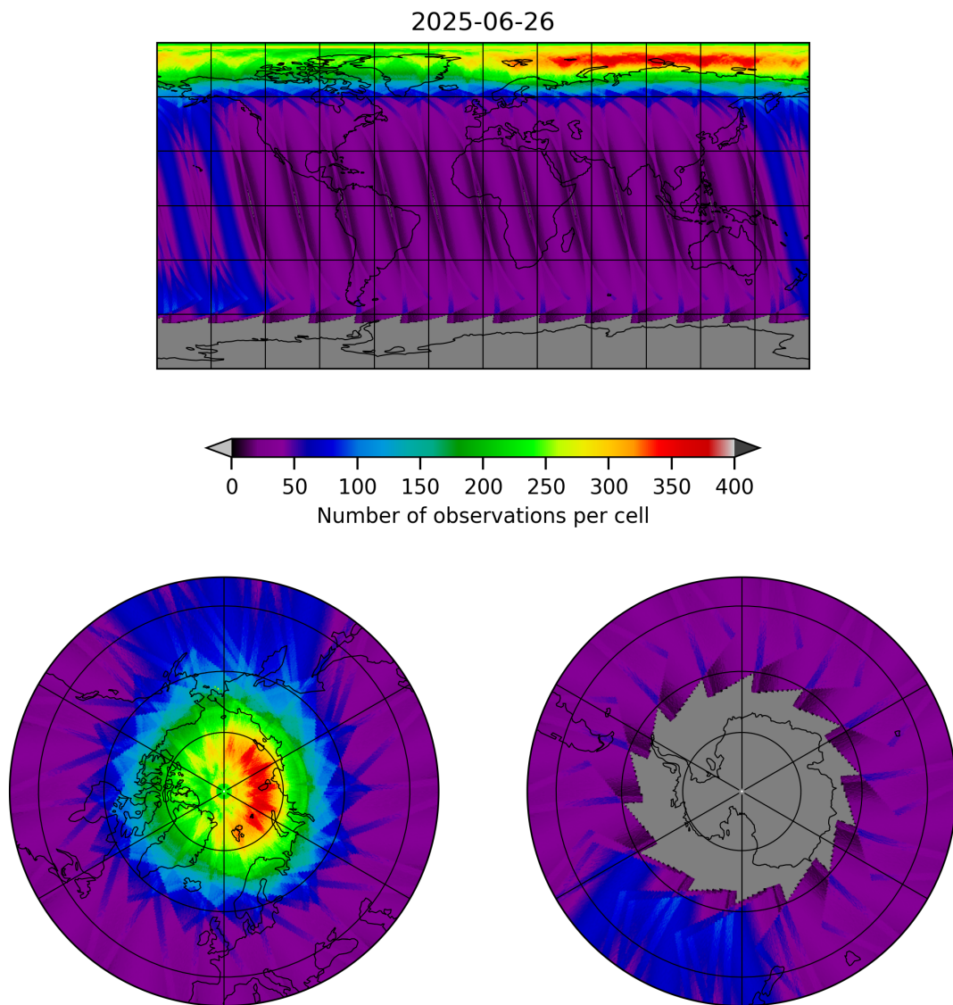
Figure 12: Map of the number of observations for 2025-06-25 to 2025-06-27
