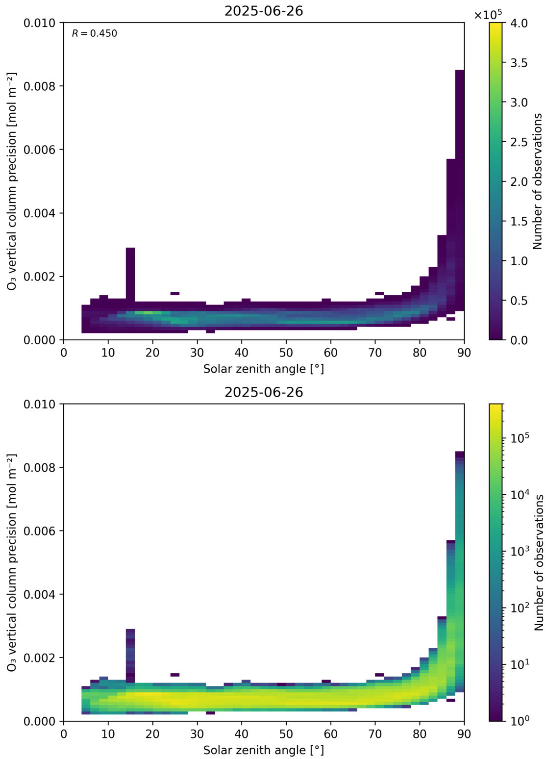
Figure 48: Scatter density plot of “Solar zenith angle” against “O 3 vertical column precision” for 2025-06-25 to 2025-06-27.
