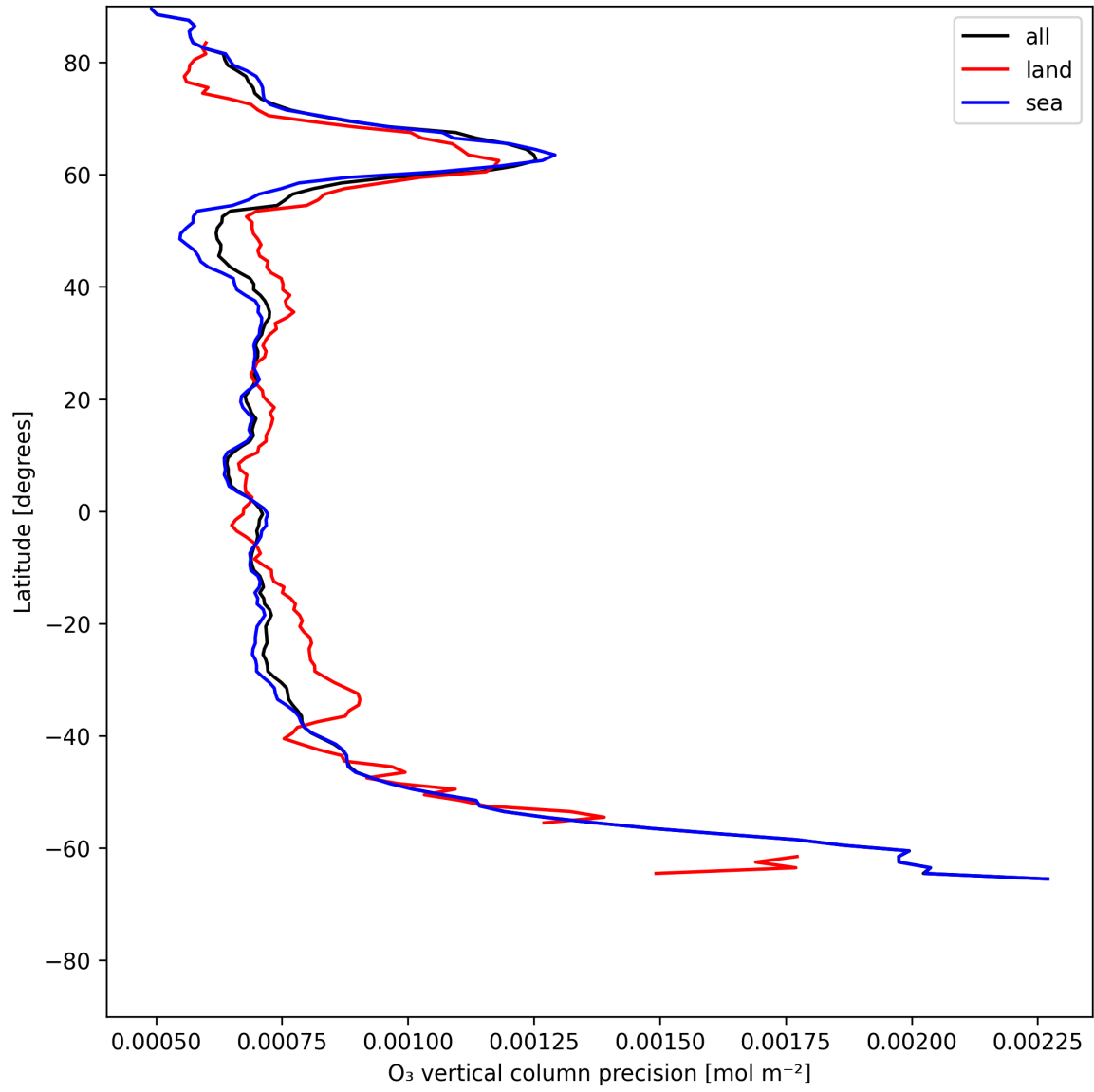
Figure 15: Zonal average of “O 3 vertical column precision” for 2025-06-25 to 2025-06-27.
