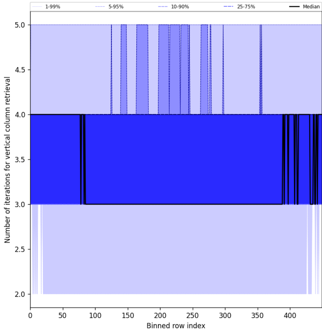
Figure 33: Along track statistics of “Number of iterations for vertical column retrieval” for 2025-06-25 to 2025-06-27
