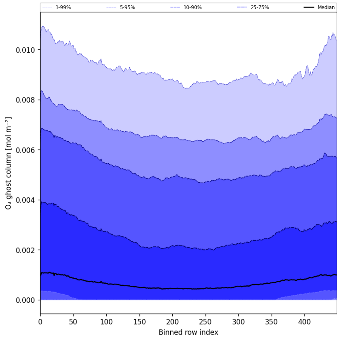
Figure 32: Along track statistics of “O 3 ghost column” for 2025-06-25 to 2025-06-27
