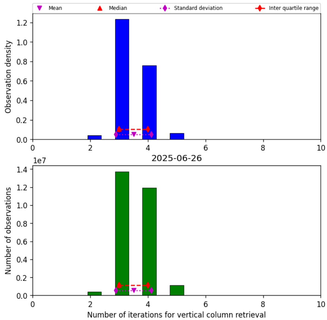
Figure 26: Histogram of “Number of iterations for vertical column retrieval” for 2025-06-25 to 2025-06-27
