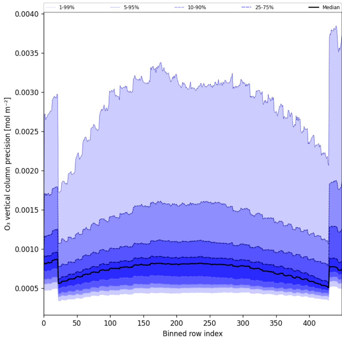
Figure 29: Along track statistics of “O 3 vertical column precision” for 2025-06-25 to 2025-06-27
