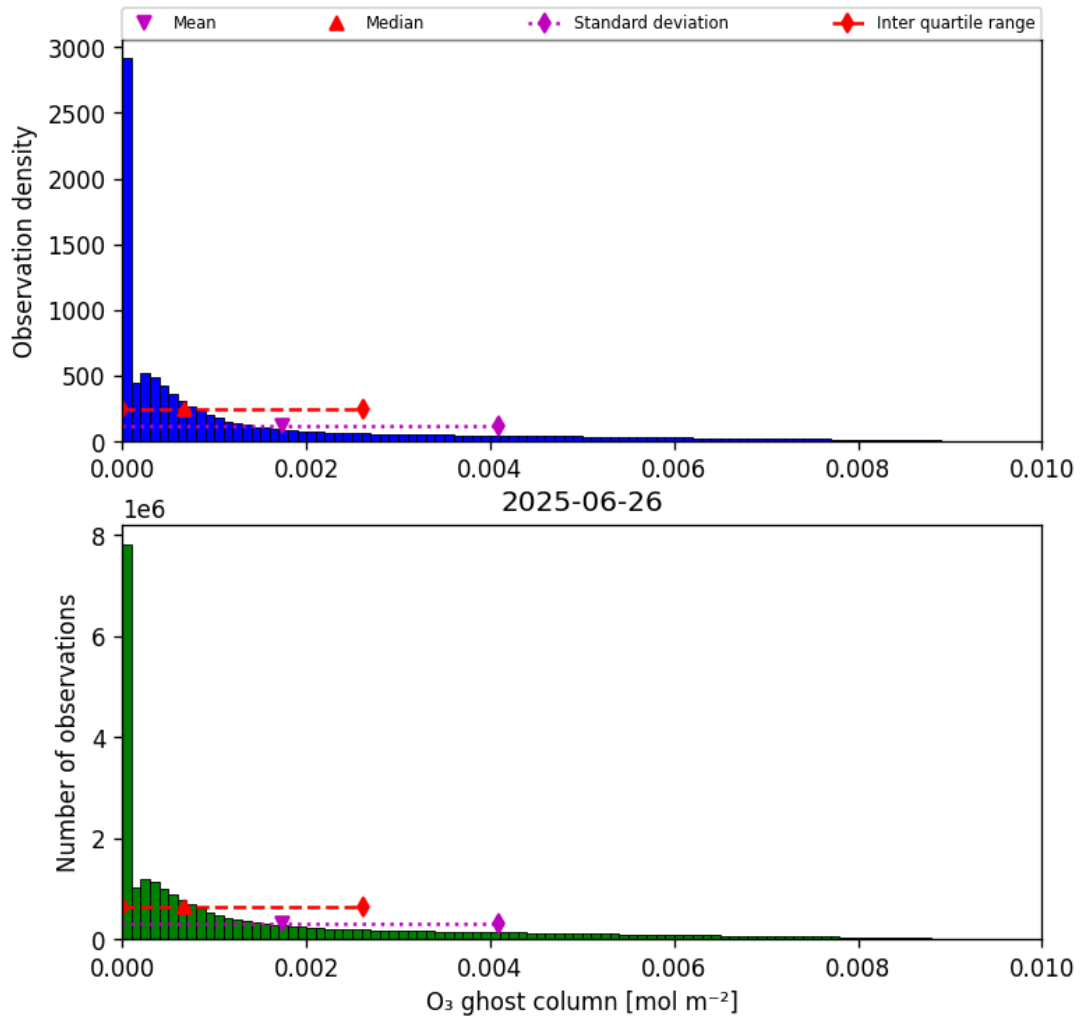
Figure 25: Histogram of “O 3 ghost column” for 2025-06-25 to 2025-06-27
