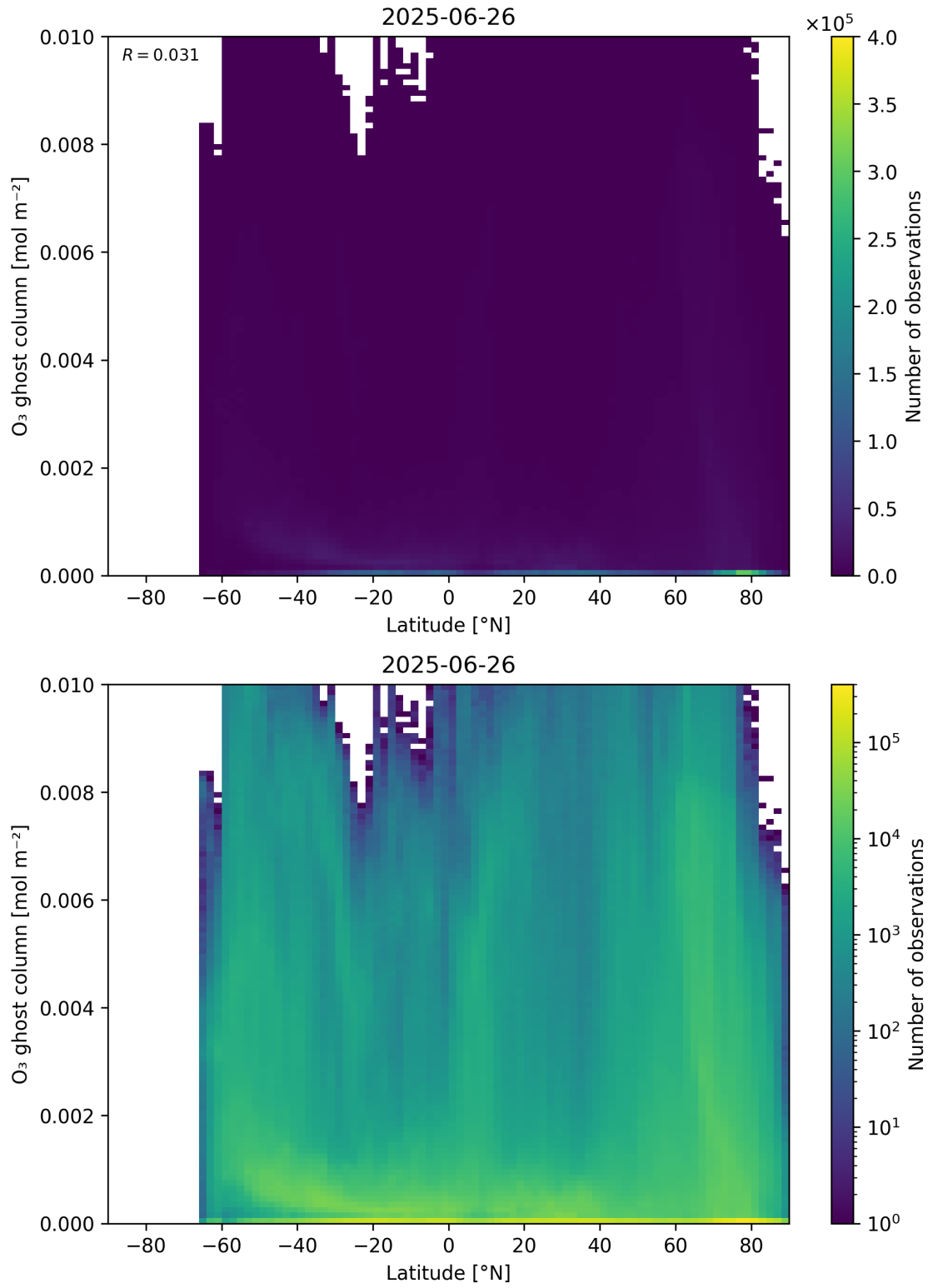
Figure 35: Scatter density plot of “Latitude” against “O 3 ghost column” for 2025-06-25 to 2025-06-27.
