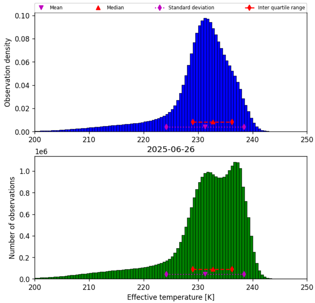
Figure 24: Histogram of “Effective temperature” for 2025-06-25 to 2025-06-27
