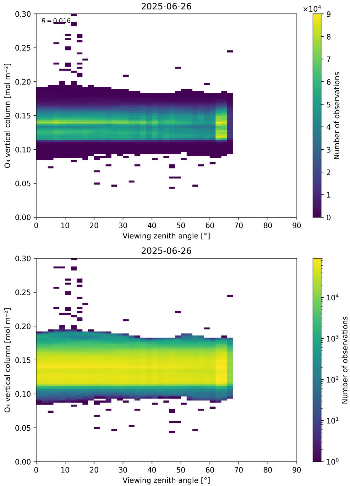
Figure 52: Scatter density plot of “Viewing zenith angle” against “O 3 vertical column” for 2025-06-25 to 2025-06-27.
