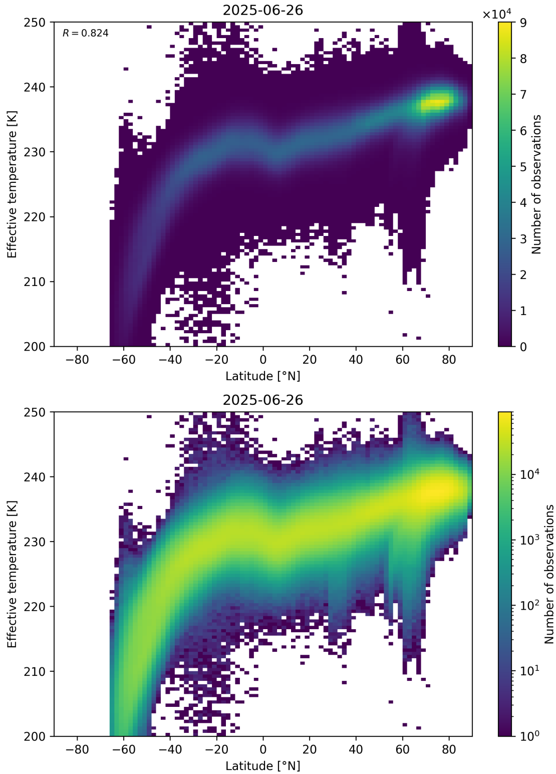
Figure 34: Scatter density plot of “Latitude” against “Effective temperature” for 2025-06-25 to 2025-06-27.
