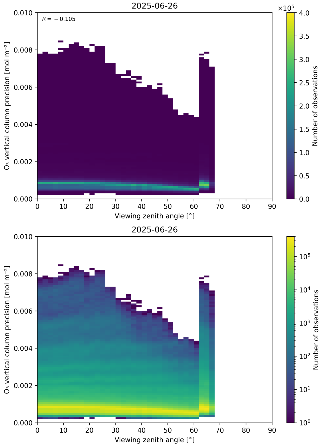
Figure 53: Scatter density plot of “Viewing zenith angle” against “O 3 vertical column precision” for 2025-06-25 to 2025-06-27.
