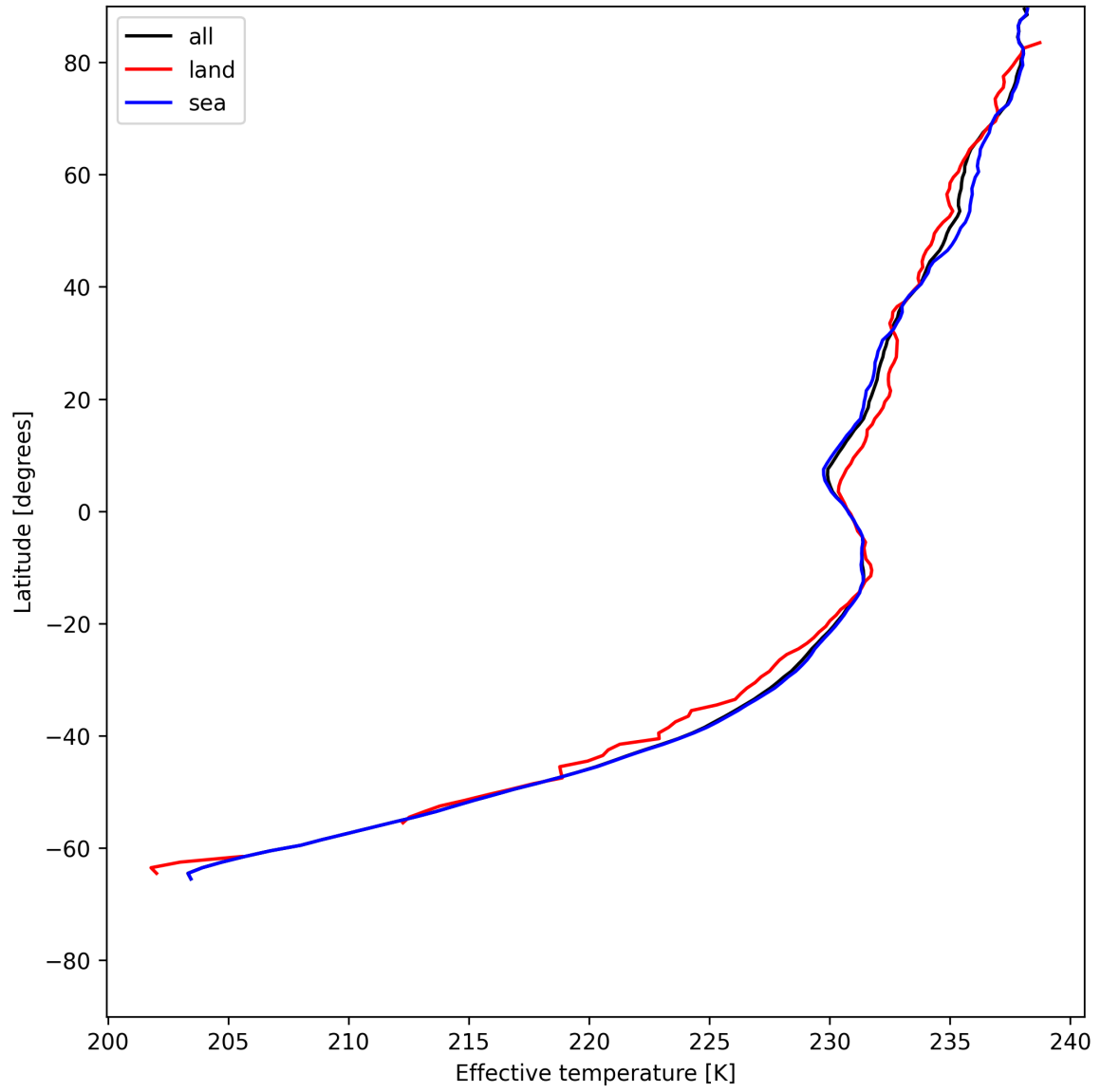
Figure 17: Zonal average of "Effective temperature" for 2025-06-25 to 2025-06-27.
