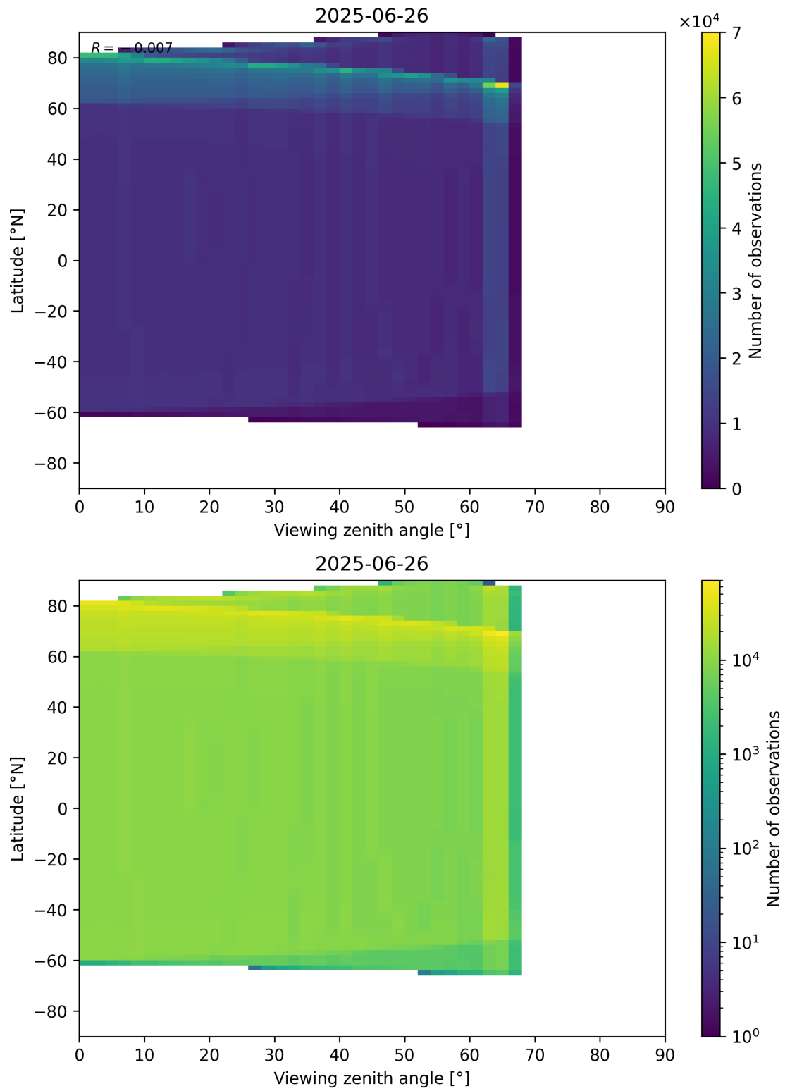
Figure 49: Scatter density plot of “Viewing zenith angle” against “Latitude” for 2025-06-25 to 2025-06-27.
