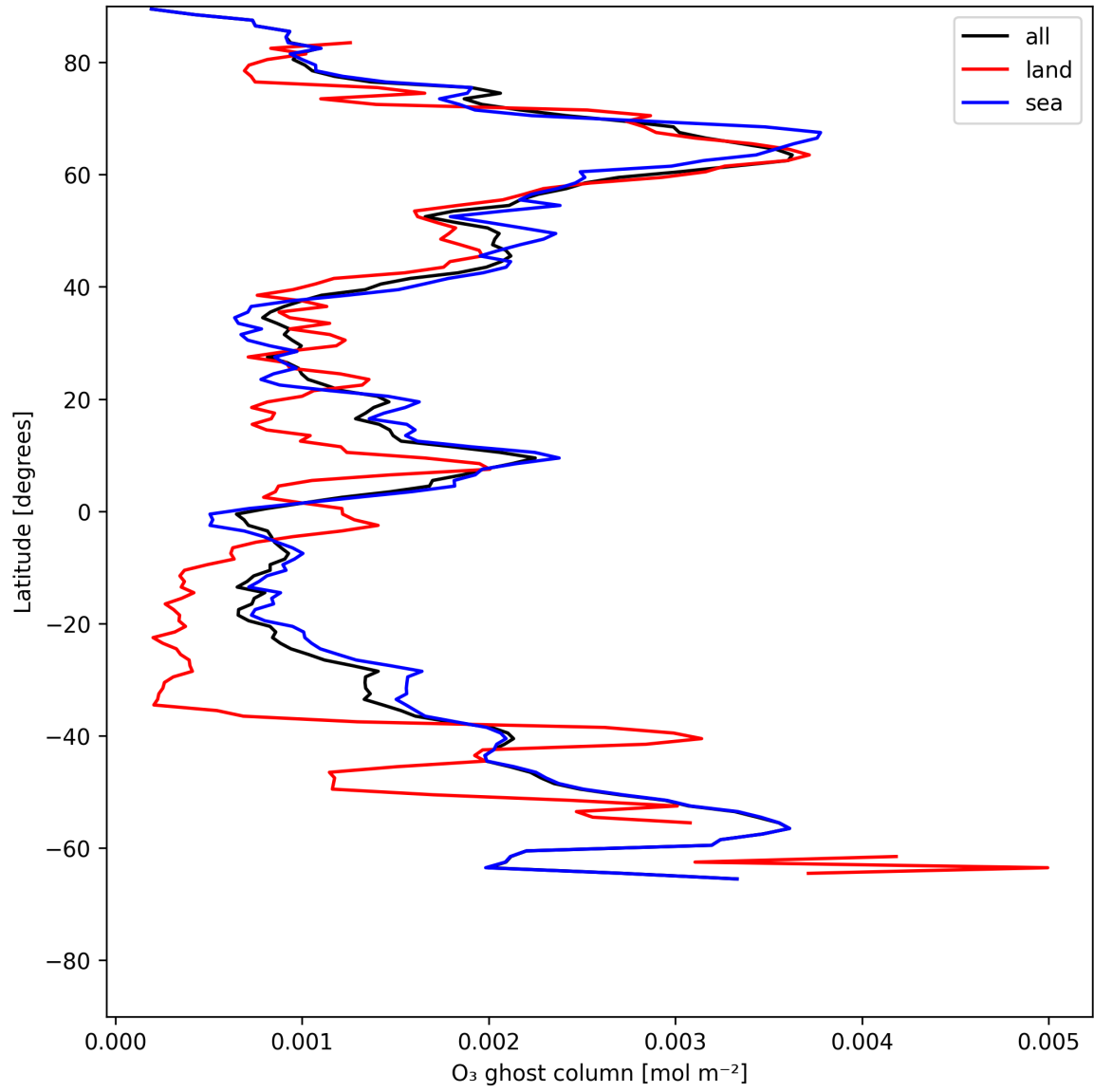
Figure 18: Zonal average of “O 3 ghost column” for 2025-06-25 to 2025-06-27.
