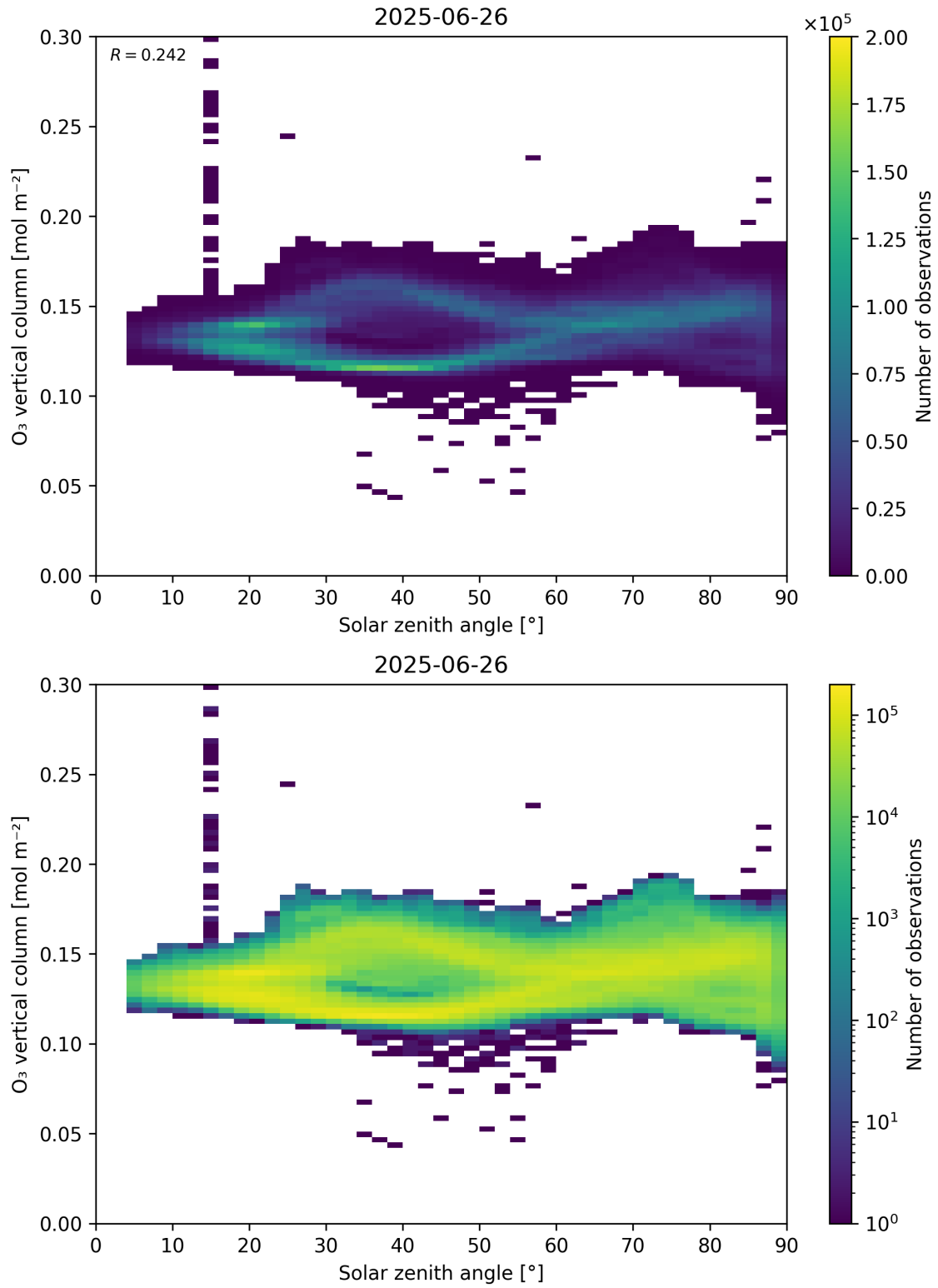
Figure 47: Scatter density plot of “Solar zenith angle” against “O 3 vertical column” for 2025-06-25 to 2025-06-27.
