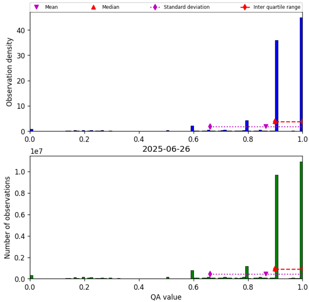
Figure 20: Histogram of “QA value” for 2025-06-25 to 2025-06-27
