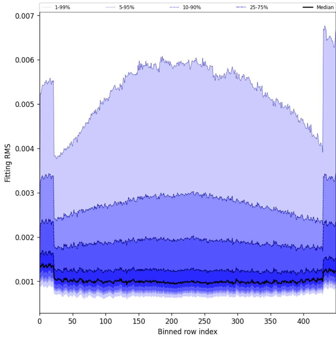
Figure 30: Along track statistics of “Fitting RMS” for 2025-06-25 to 2025-06-27
