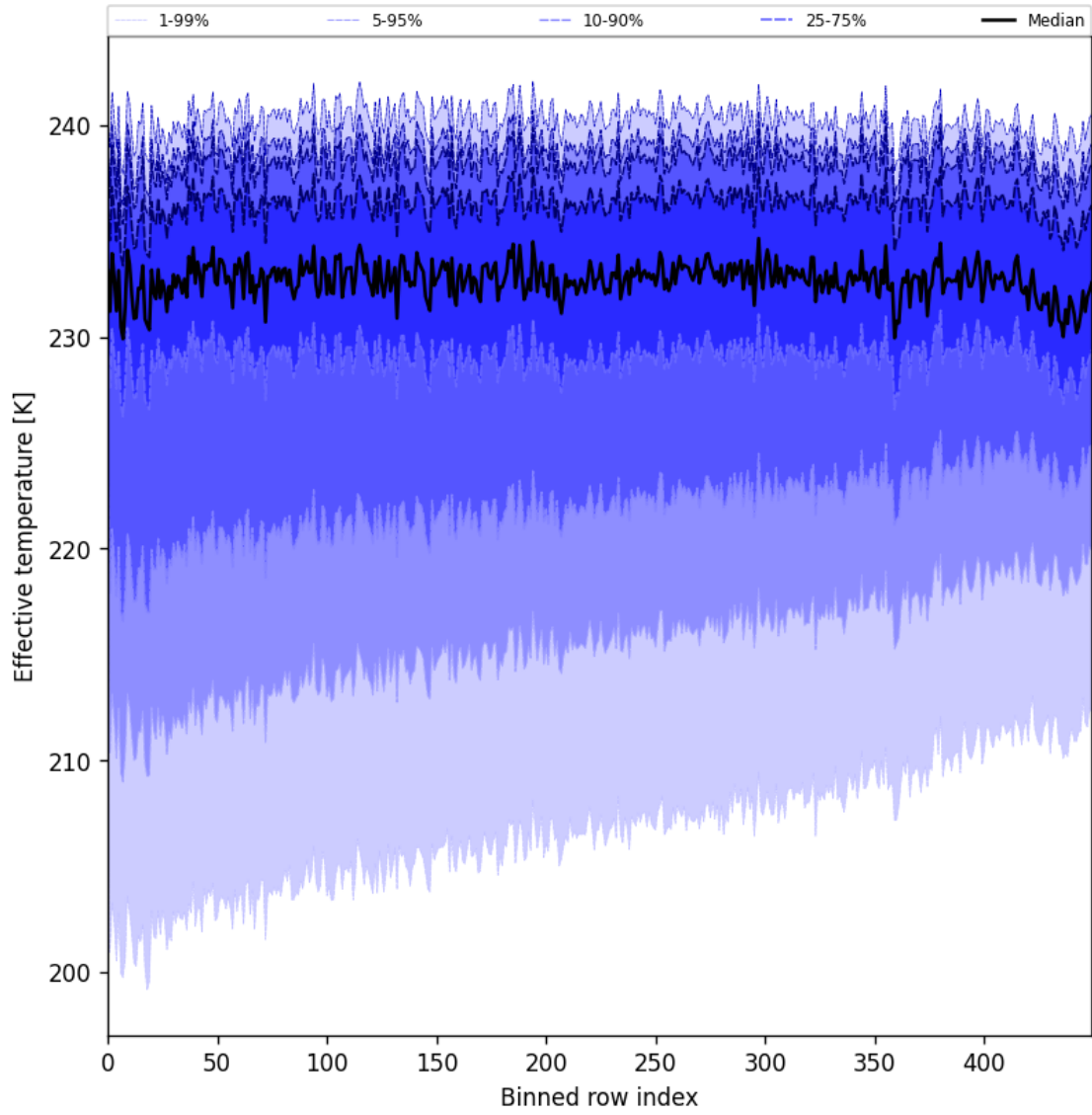
Figure 31: Along track statistics of “Effective temperature” for 2025-06-25 to 2025-06-27
