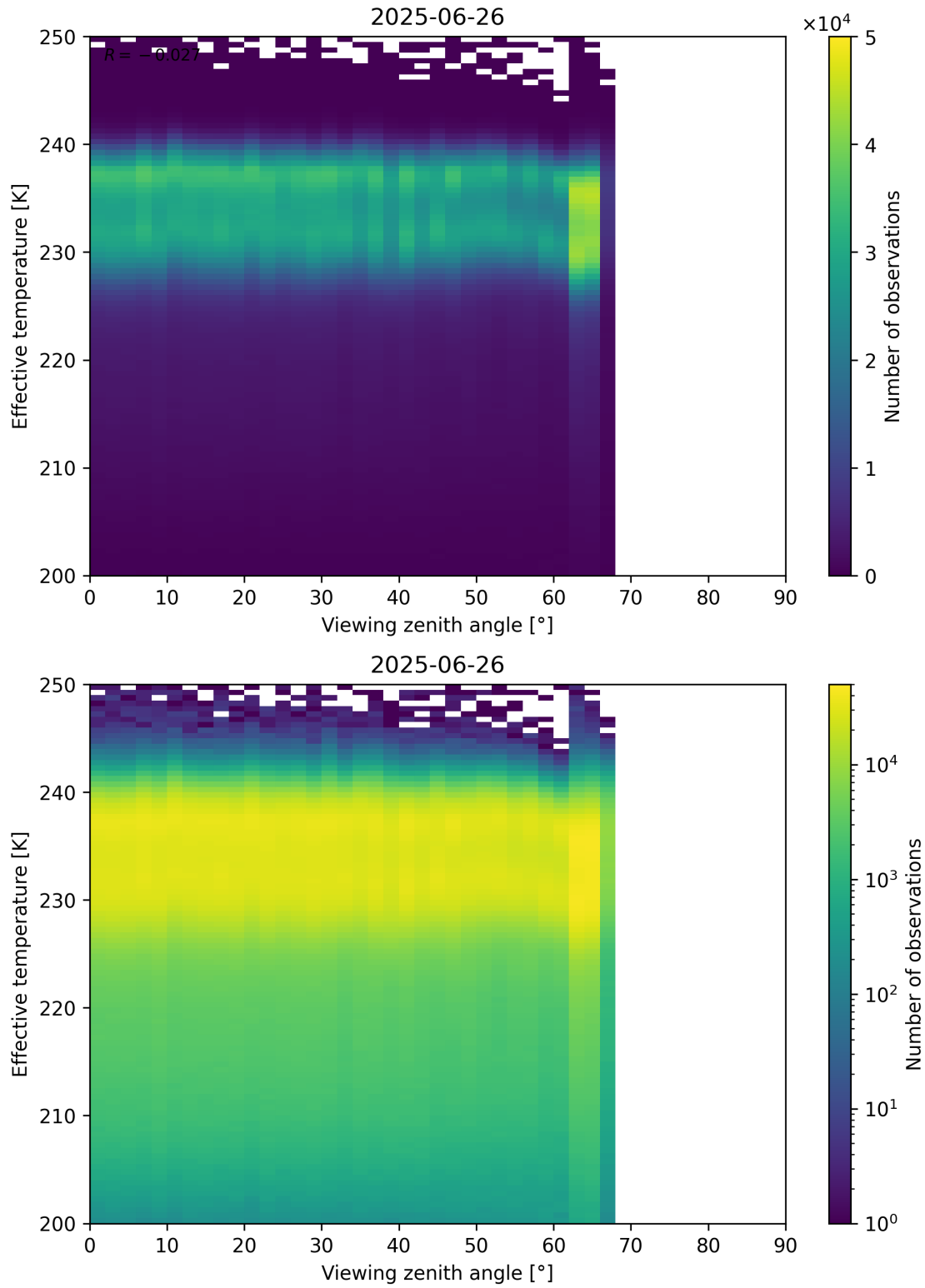
Figure 50: Scatter density plot of “Viewing zenith angle” against “Effective temperature” for 2025-06-25 to 2025-06-27.
