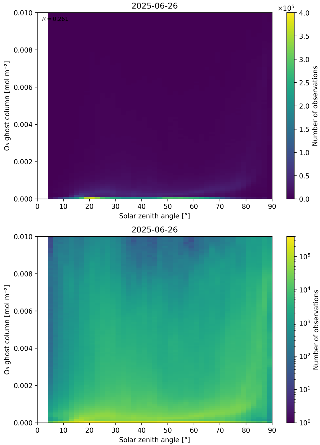
Figure 46: Scatter density plot of “Solar zenith angle” against “O 3 ghost column” for 2025-06-25 to 2025-06-27.
