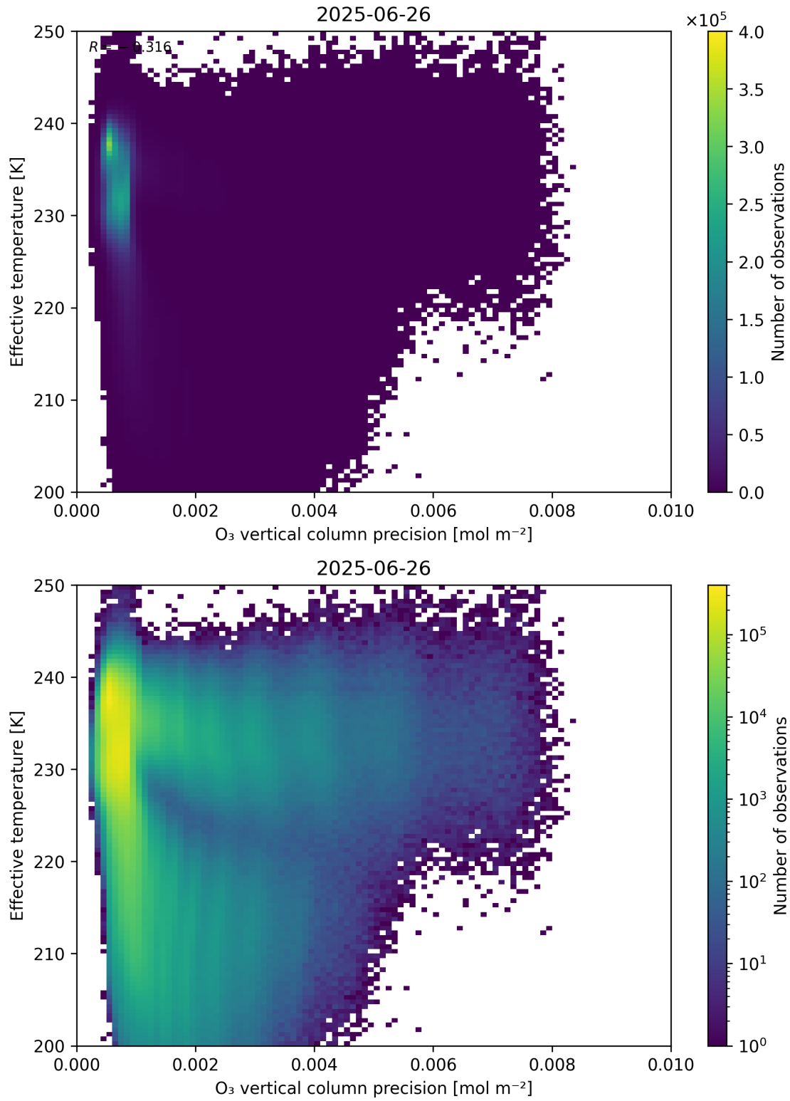
Figure 42: Scatter density plot of “O 3 vertical column precision” against “Effective temperature” for 2025-06-25 to 2025-06-27.
