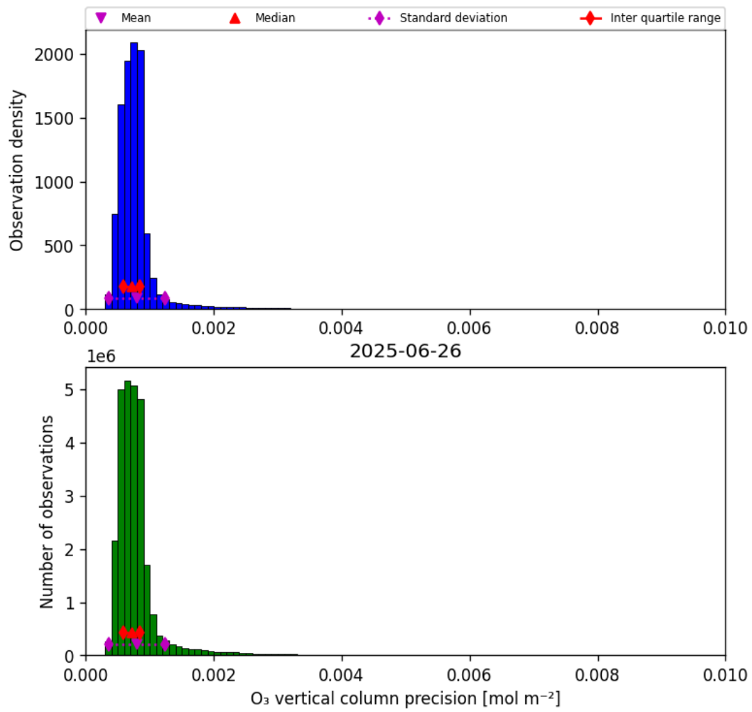
Figure 22: Histogram of “O 3 vertical column precision” for 2025-06-25 to 2025-06-27
