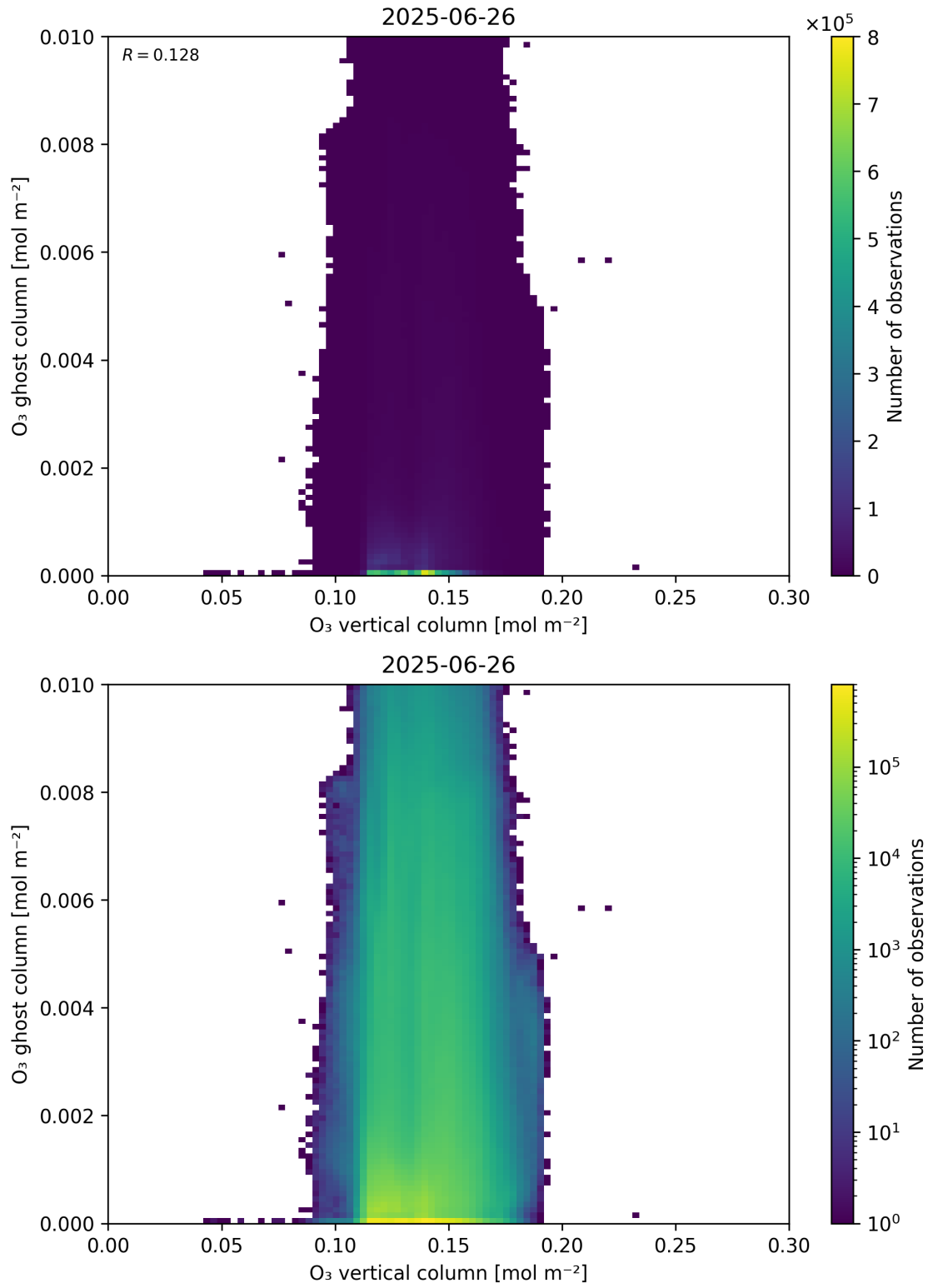
Figure 40: Scatter density plot of “O 3 vertical column” against “O 3 ghost column” for 2025-06-25 to 2025-06-27.
