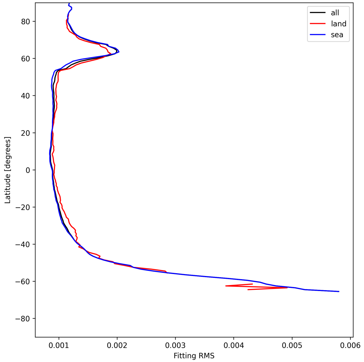
Figure 16: Zonal average of “Fitting RMS” for 2025-06-25 to 2025-06-27.
