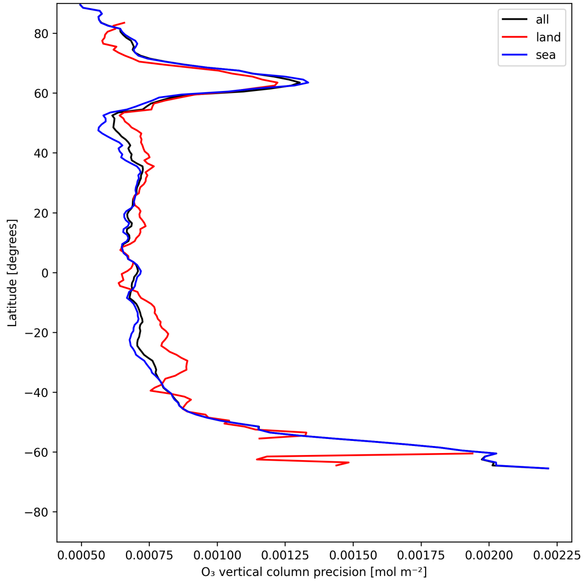
Figure 15: Zonal average of "O 3 vertical column precision" for 2025-06-27 to 2025-06-28.
