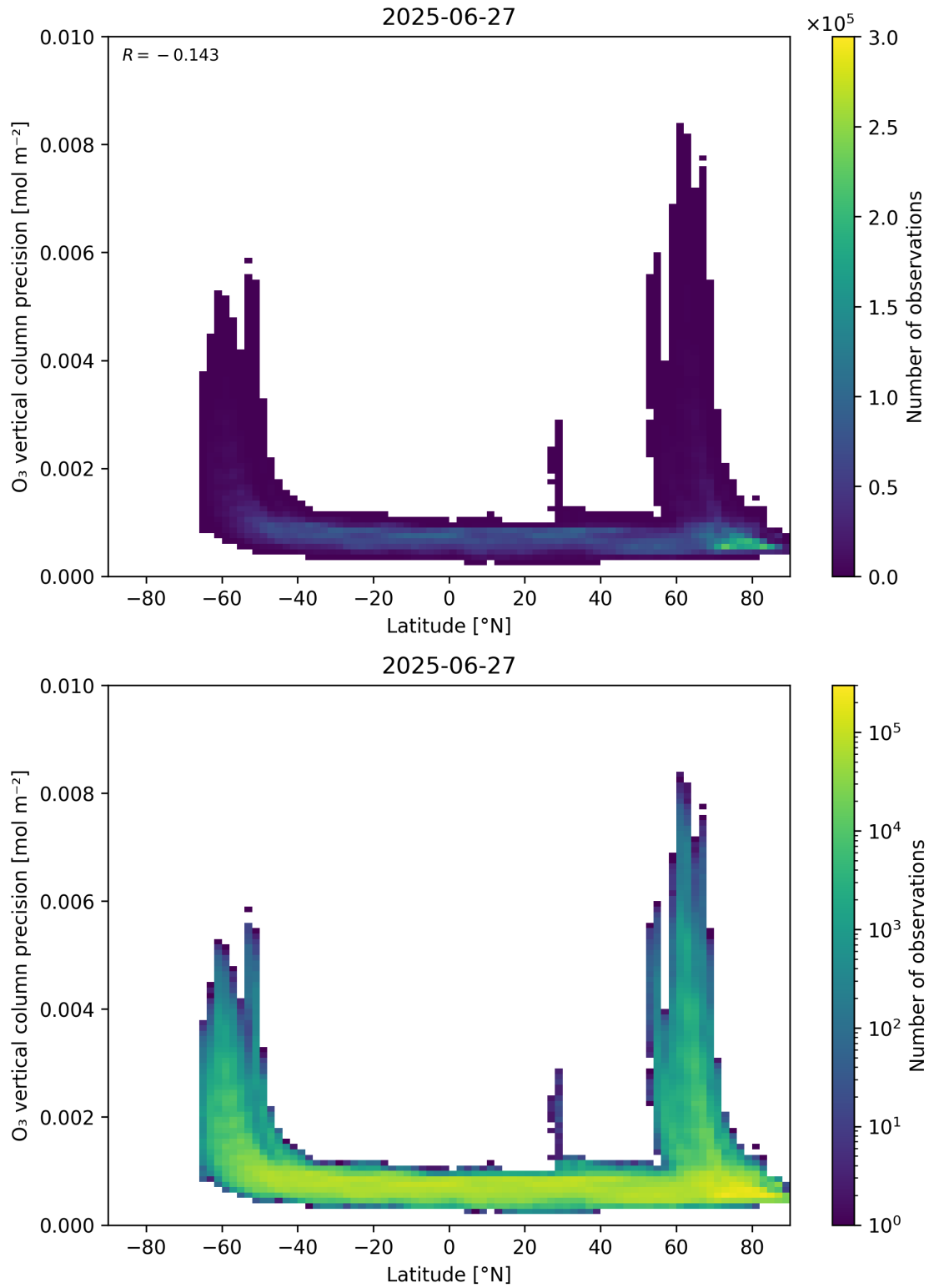
Figure 37: Scatter density plot of “Latitude” against “O 3 vertical column precision” for 2025-06-27 to 2025-06-28.
