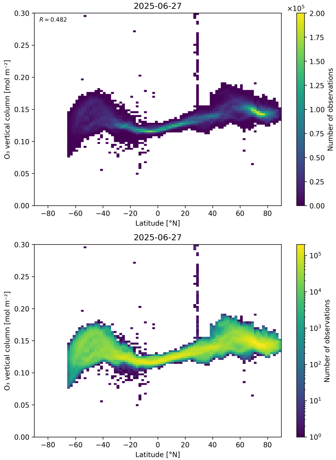
Figure 36: Scatter density plot of “Latitude” against “O 3 vertical column” for 2025-06-27 to 2025-06-28.
