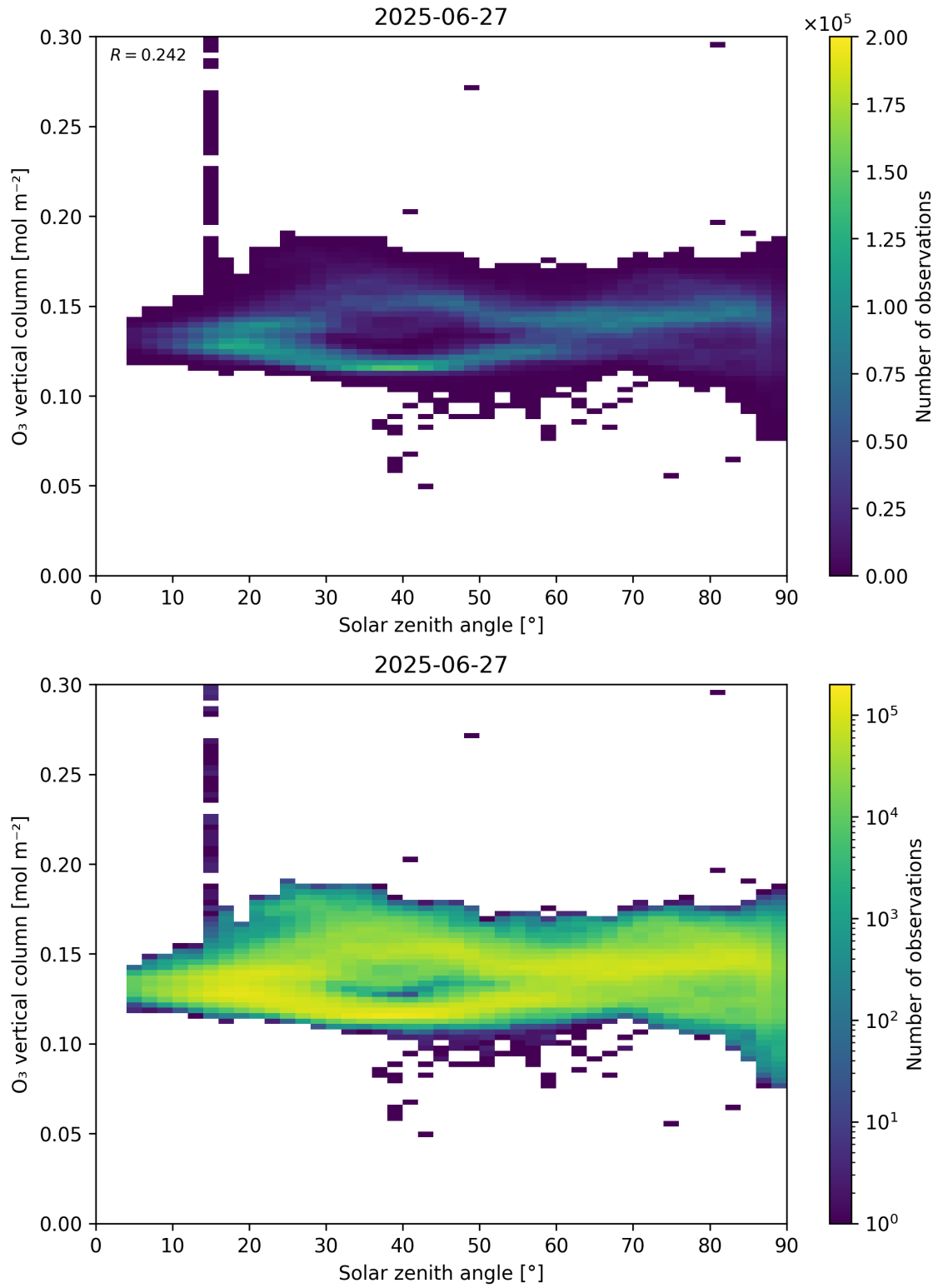
Figure 47: Scatter density plot of “Solar zenith angle” against “O 3 vertical column” for 2025-06-27 to 2025-06-28.
