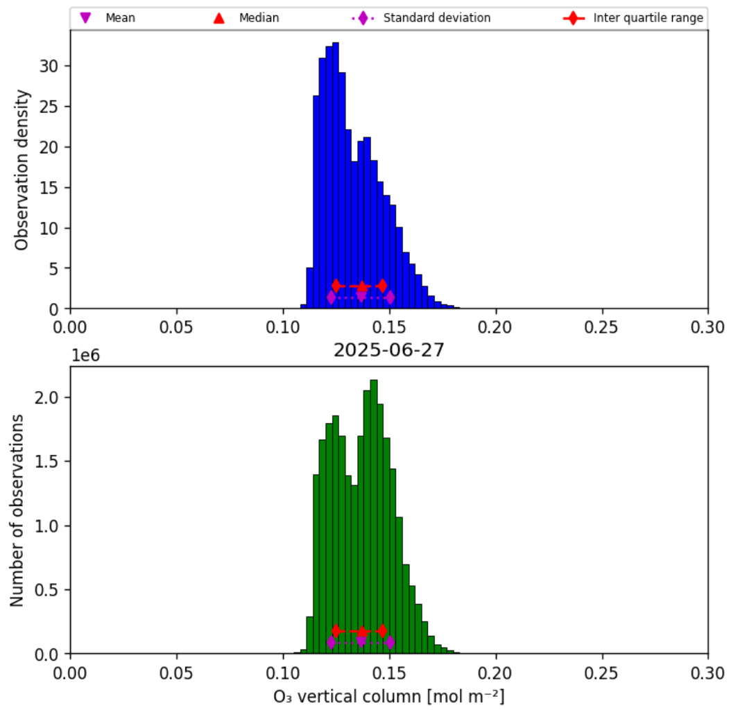
Figure 21: Histogram of “O 3 vertical column” for 2025-06-27 to 2025-06-28
