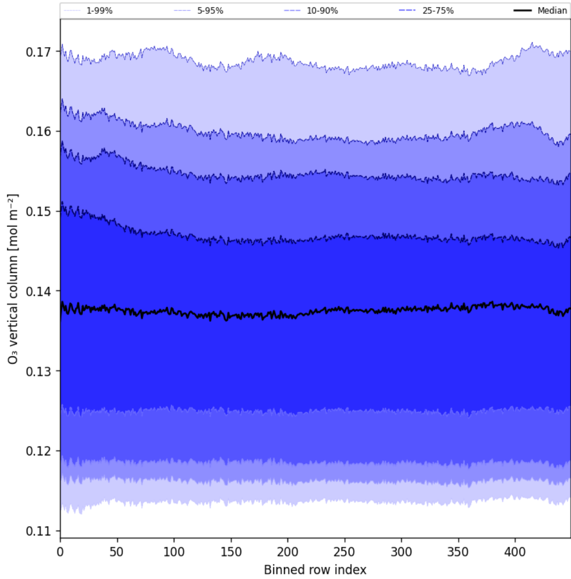
Figure 28: Along track statistics of “O 3 vertical column” for 2025-06-27 to 2025-06-28
