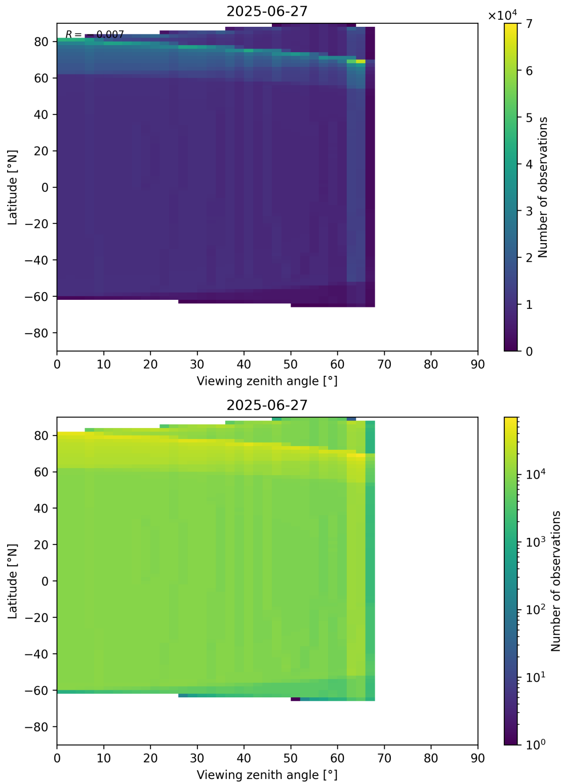
Figure 49: Scatter density plot of “Viewing zenith angle” against “Latitude” for 2025-06-27 to 2025-06-28.
