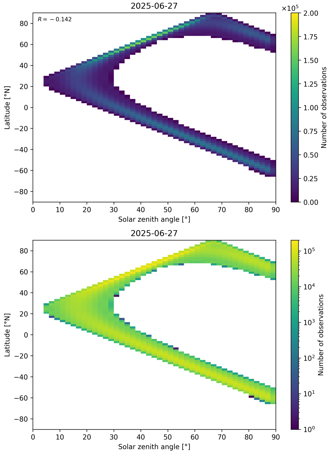
Figure 44: Scatter density plot of “Solar zenith angle” against “Latitude” for 2025-06-27 to 2025-06-28.
