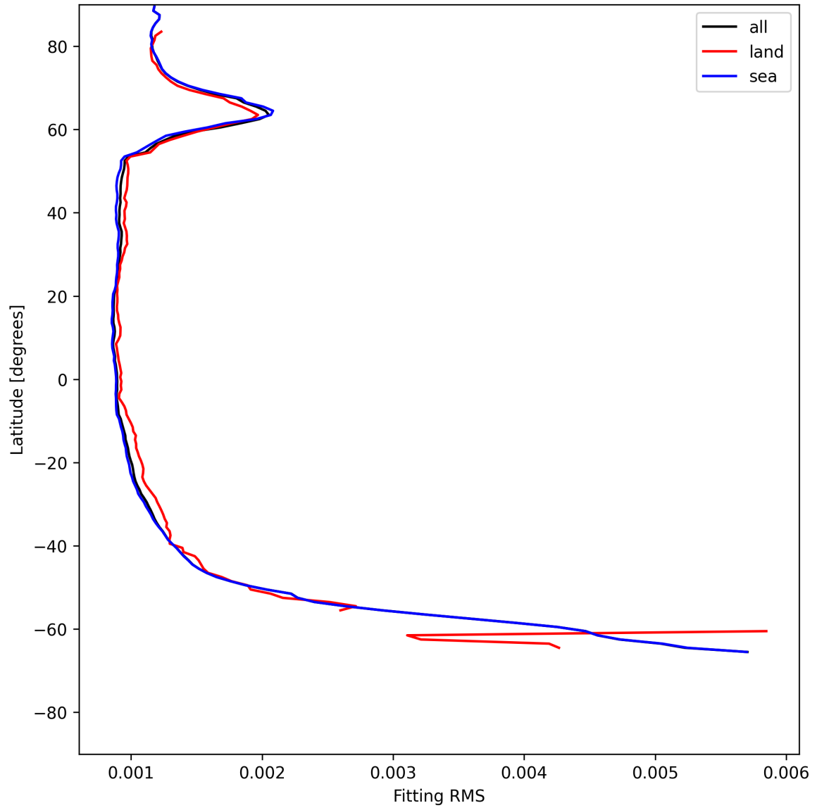
Figure 16: Zonal average of “Fitting RMS” for 2025-06-27 to 2025-06-28.
