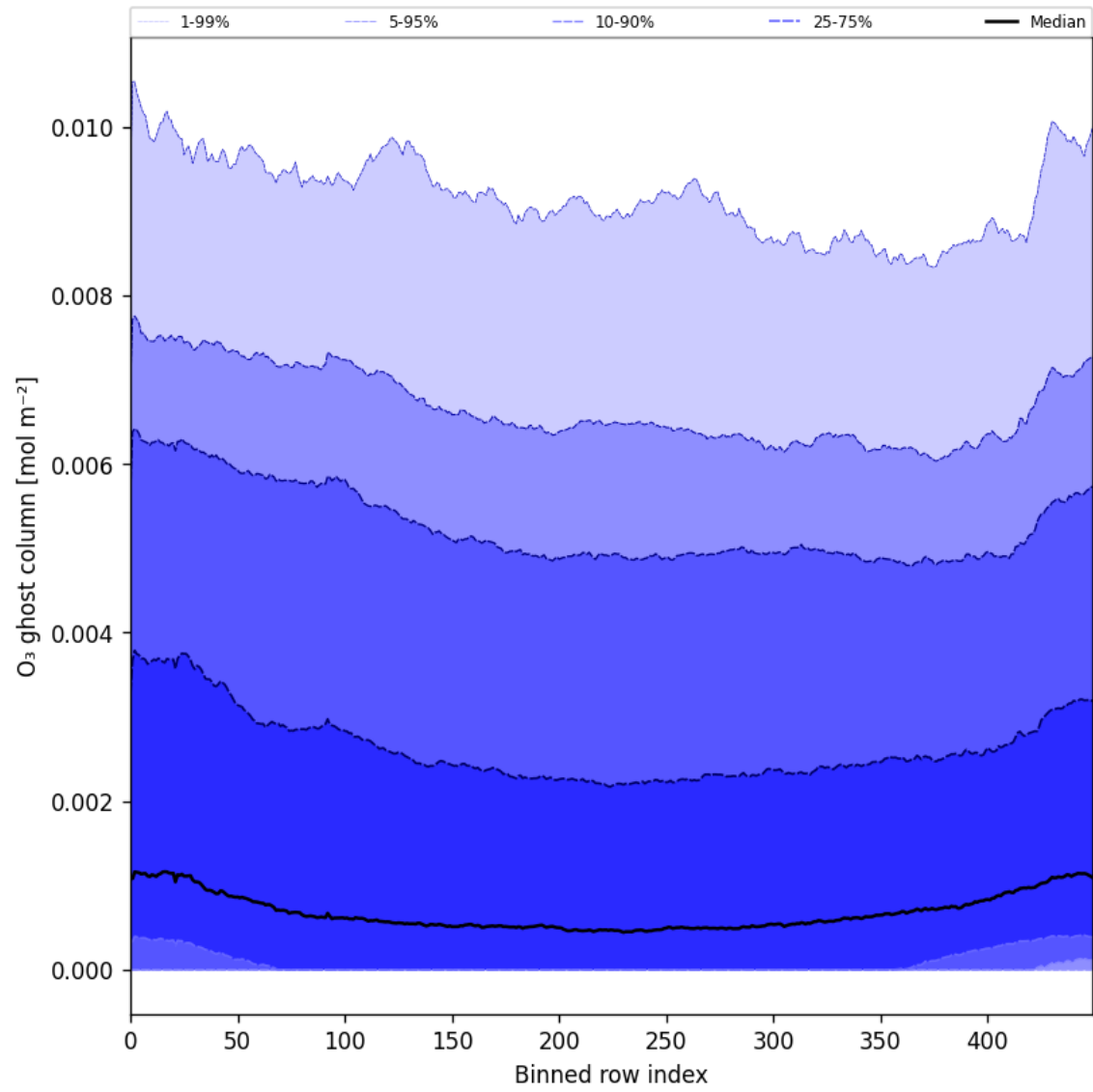
Figure 32: Along track statistics of “O 3 ghost column” for 2025-06-27 to 2025-06-28
