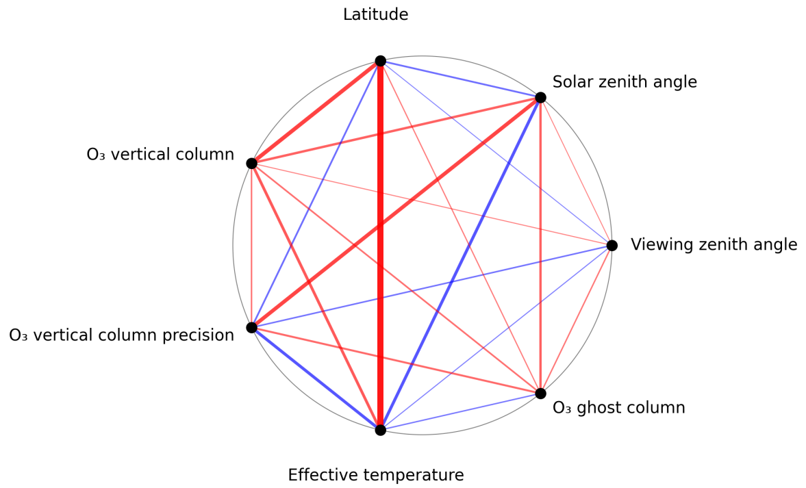
Figure 1: Map of correlation graph for 2025-06-27 to 2025-06-28.
