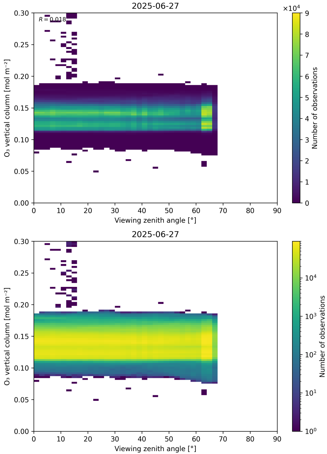
Figure 52: Scatter density plot of “Viewing zenith angle” against “O 3 vertical column” for 2025-06-27 to 2025-06-28.
