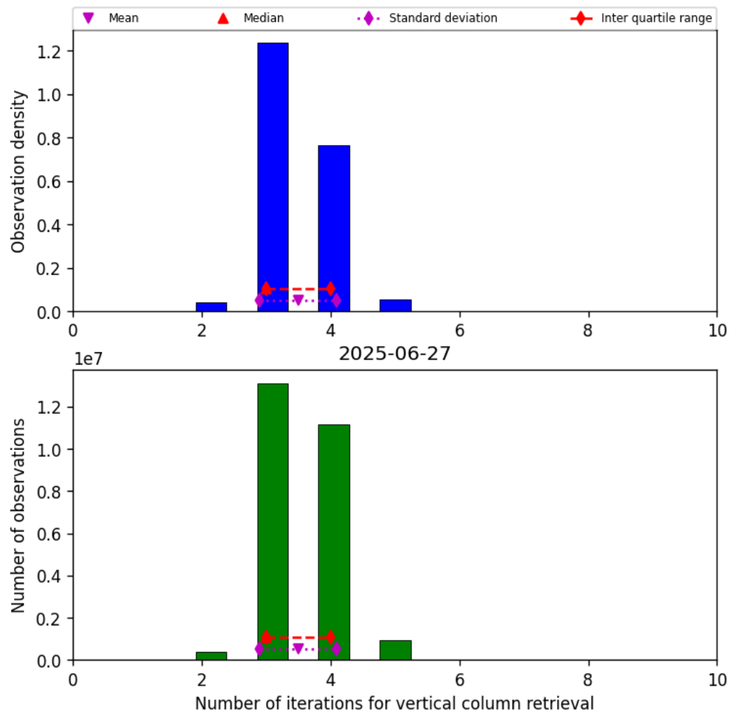
Figure 26: Histogram of “Number of iterations for vertical column retrieval” for 2025-06-27 to 2025-06-28
