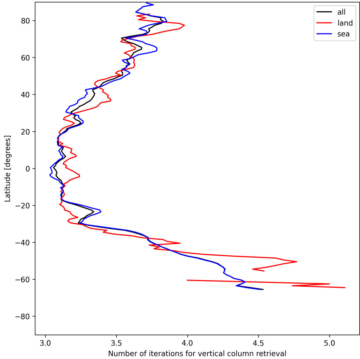
Figure 19: Zonal average of “Number of iterations for vertical column retrieval” for 2025-06-27 to 2025-06-28.
