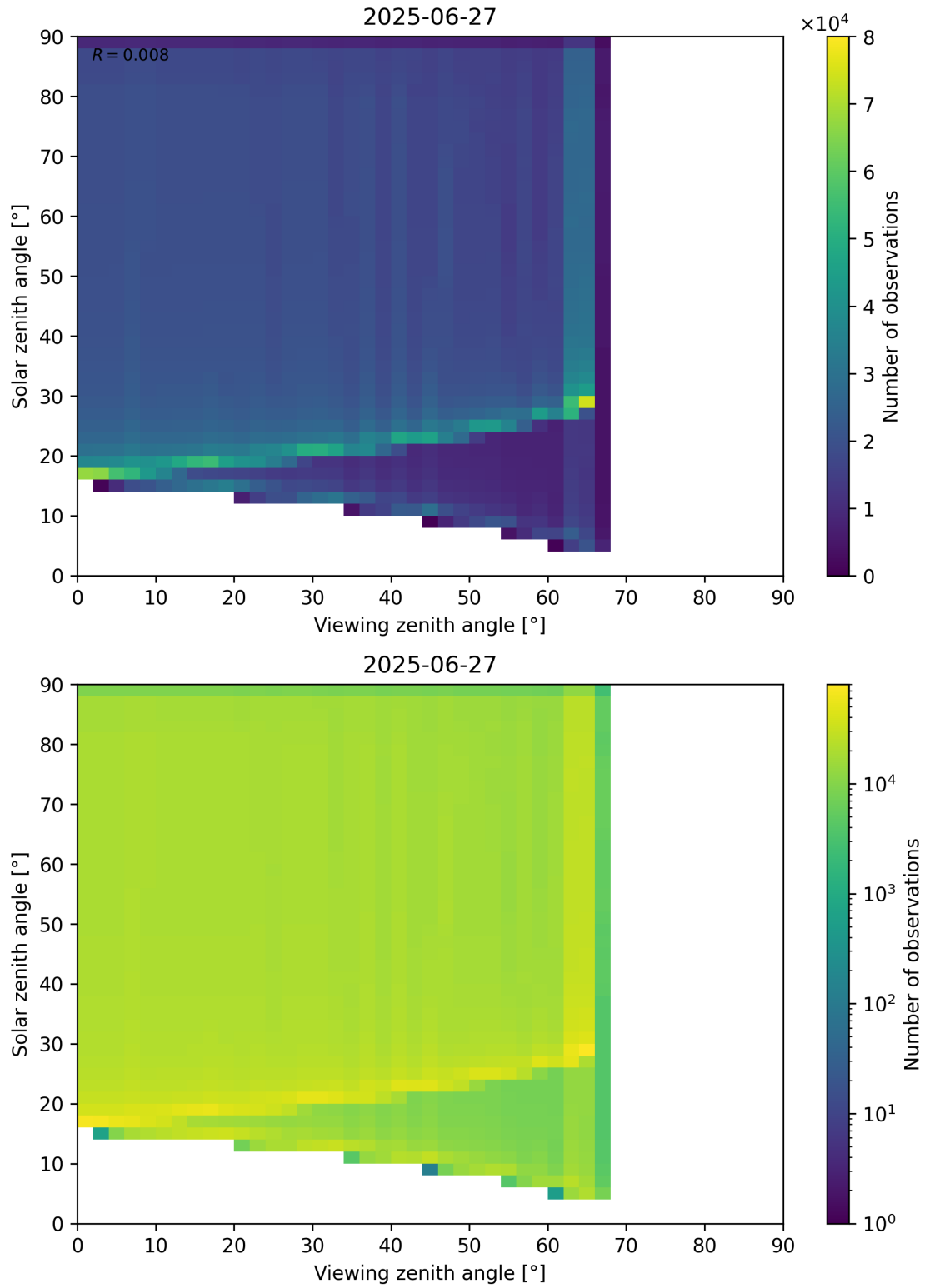
Figure 54: Scatter density plot of “Viewing zenith angle” against “Solar zenith angle” for 2025-06-27 to 2025-06-28.
