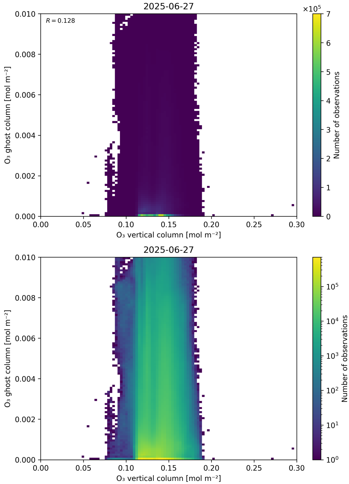
Figure 40: Scatter density plot of “O 3 vertical column” against “O 3 ghost column” for 2025-06-27 to 2025-06-28.
