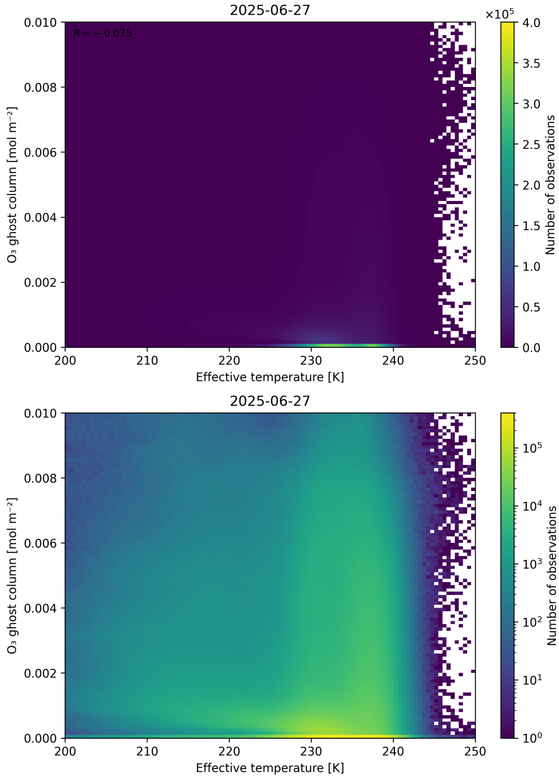
Figure 38: Scatter density plot of “Effective temperature” against “O 3 ghost column” for 2025-06-27 to 2025-06-28.
