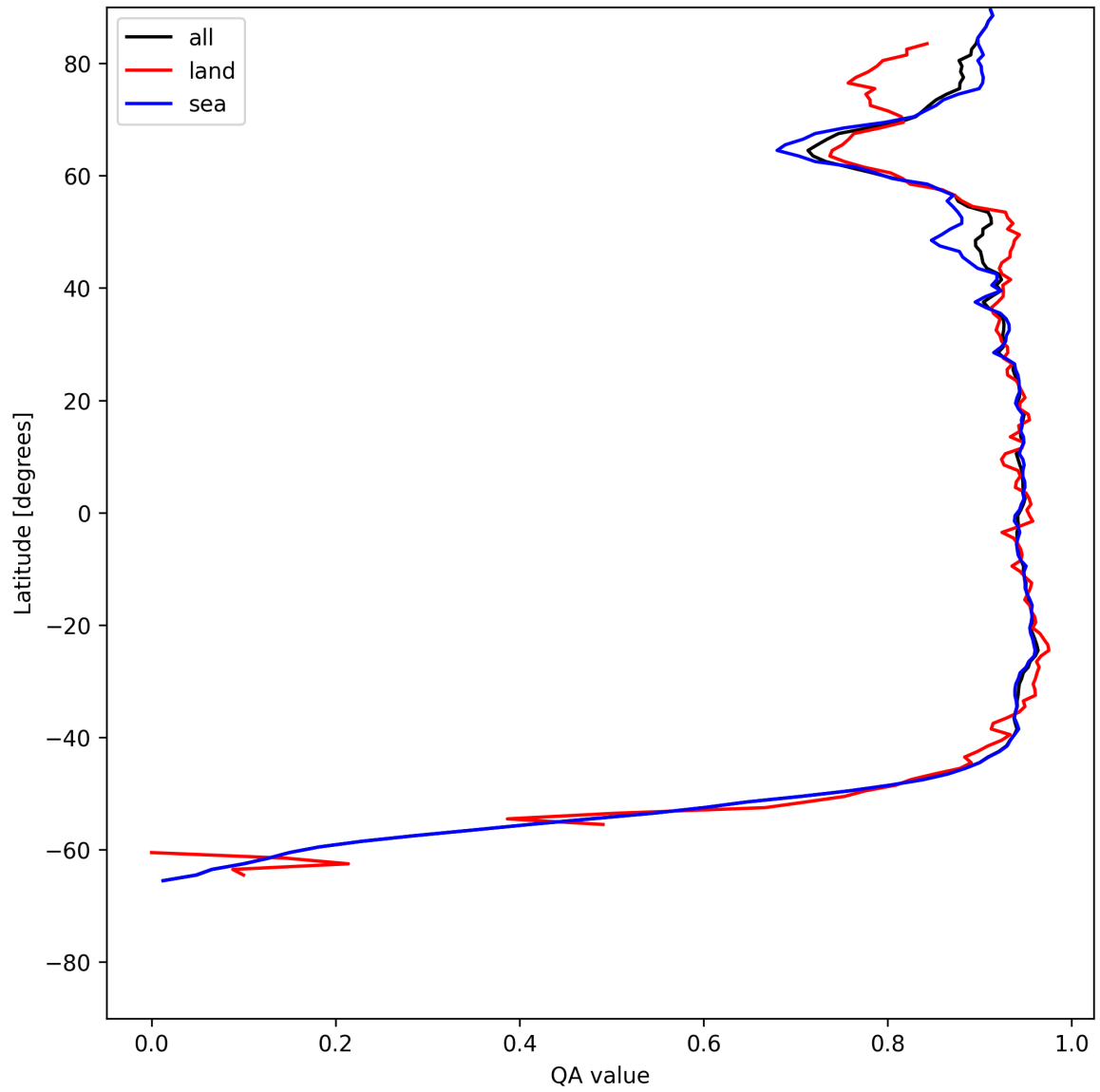
Figure 13: Zonal average of “QA value” for 2025-06-27 to 2025-06-28.
