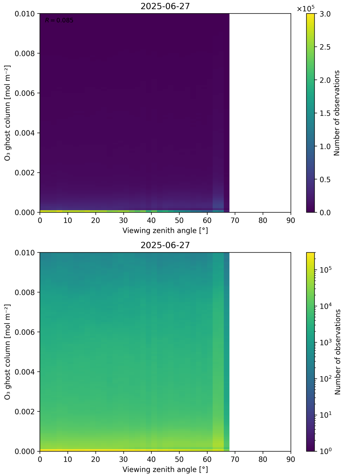
Figure 51: Scatter density plot of “Viewing zenith angle” against “O 3 ghost column” for 2025-06-27 to 2025-06-28.
