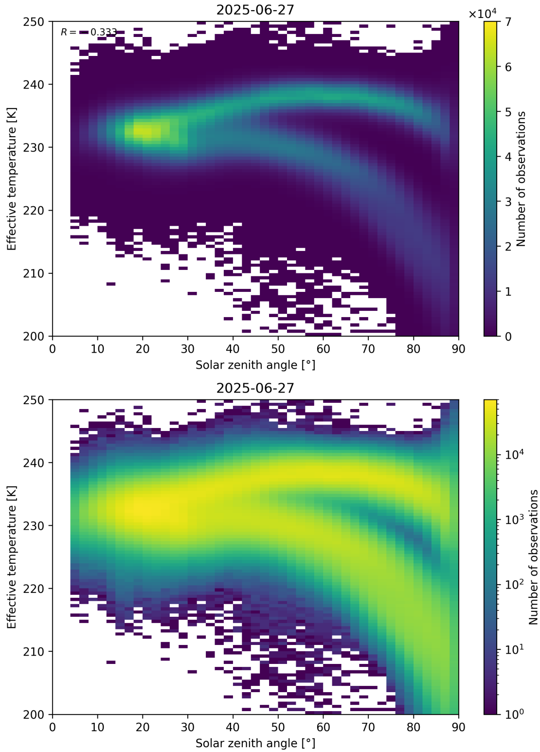
Figure 45: Scatter density plot of “Solar zenith angle” against “Effective temperature” for 2025-06-27 to 2025-06-28.
