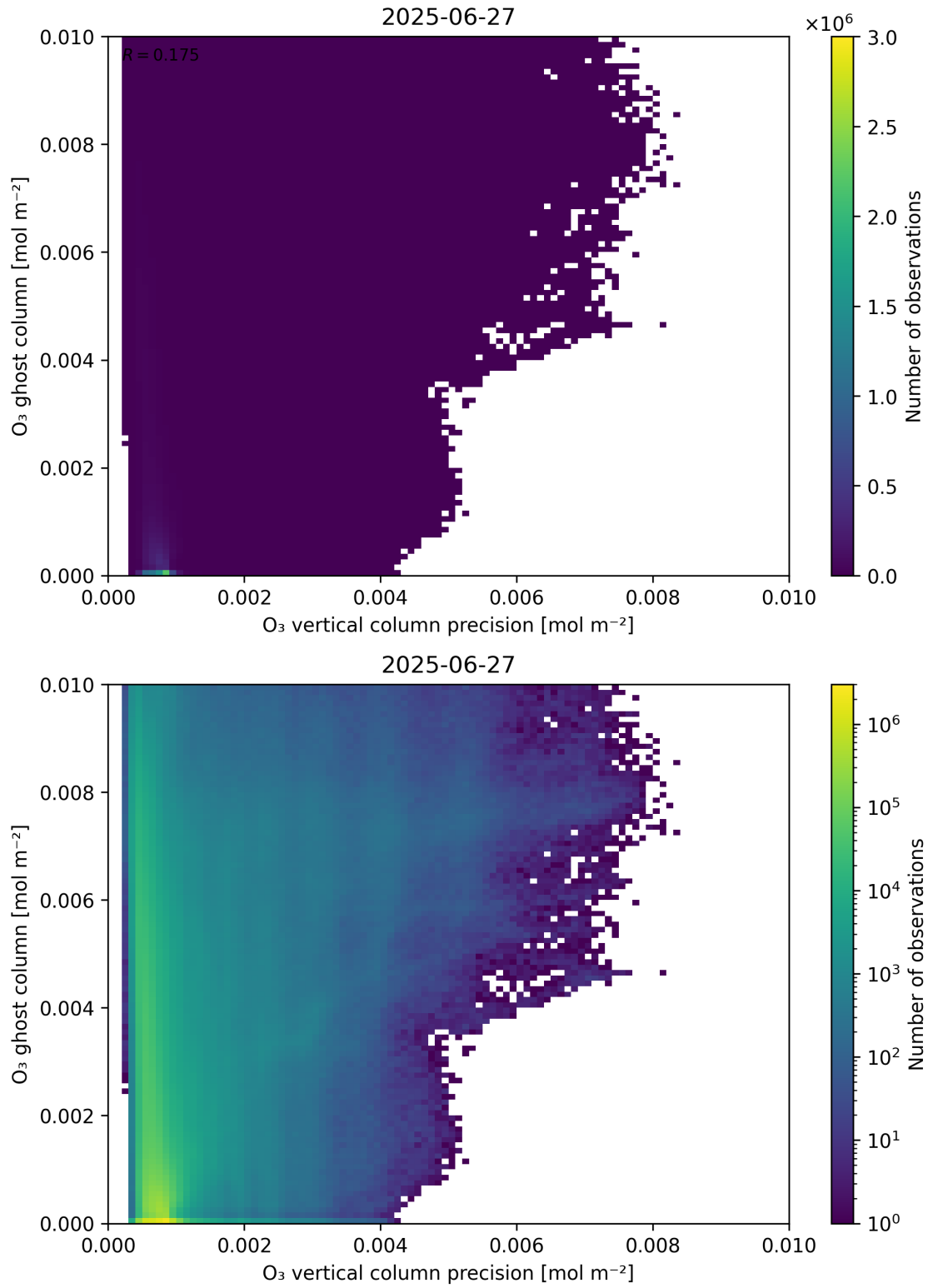
Figure 43: Scatter density plot of “ \text{O}_3 vertical column precision” against “ \text{O}_3 ghost column” for 2025-06-27 to 2025-06-28.
