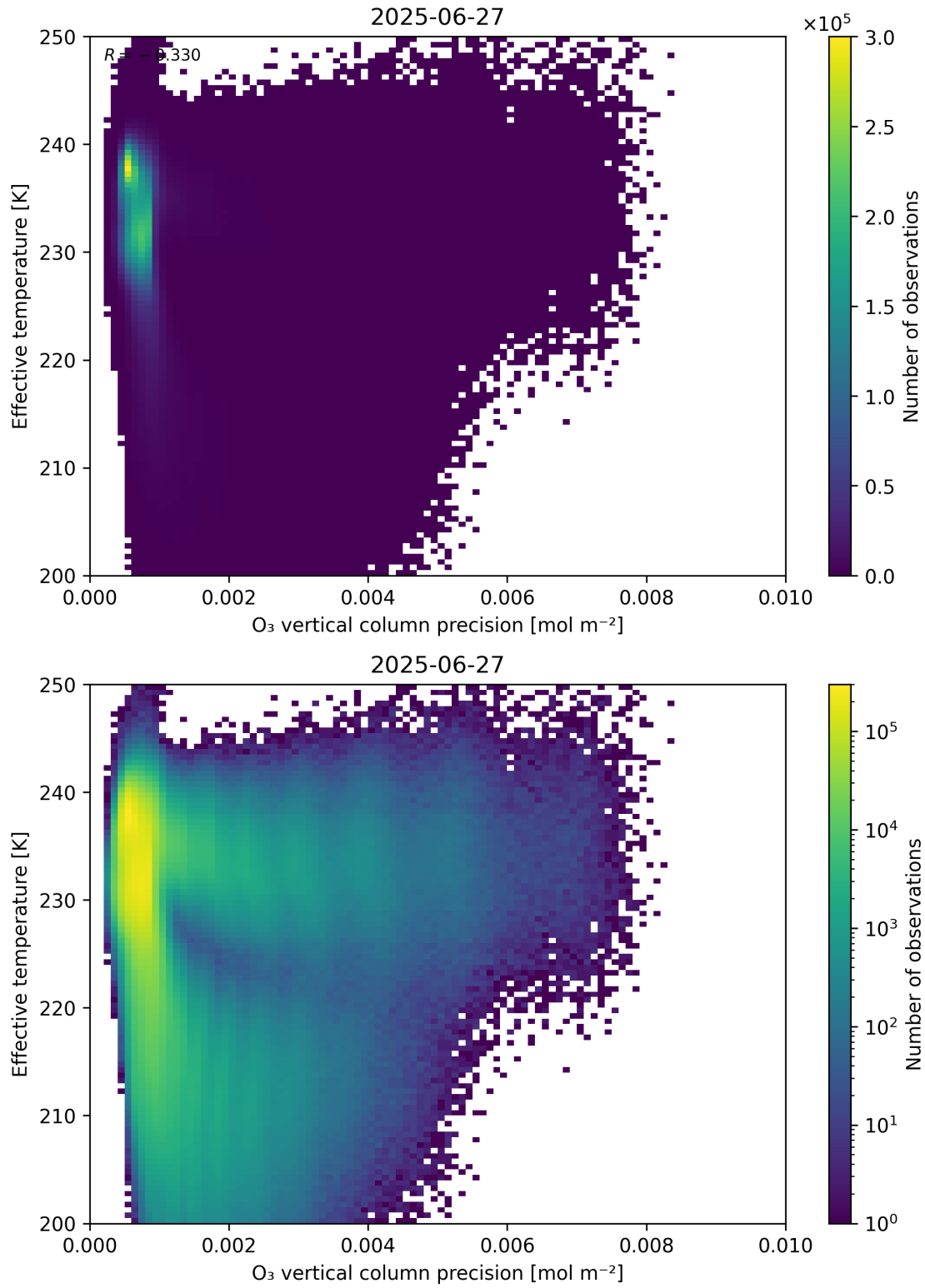
Figure 42: Scatter density plot of “ O_3 vertical column precision” against “Effective temperature” for 2025-06-27 to 2025-06-28.
