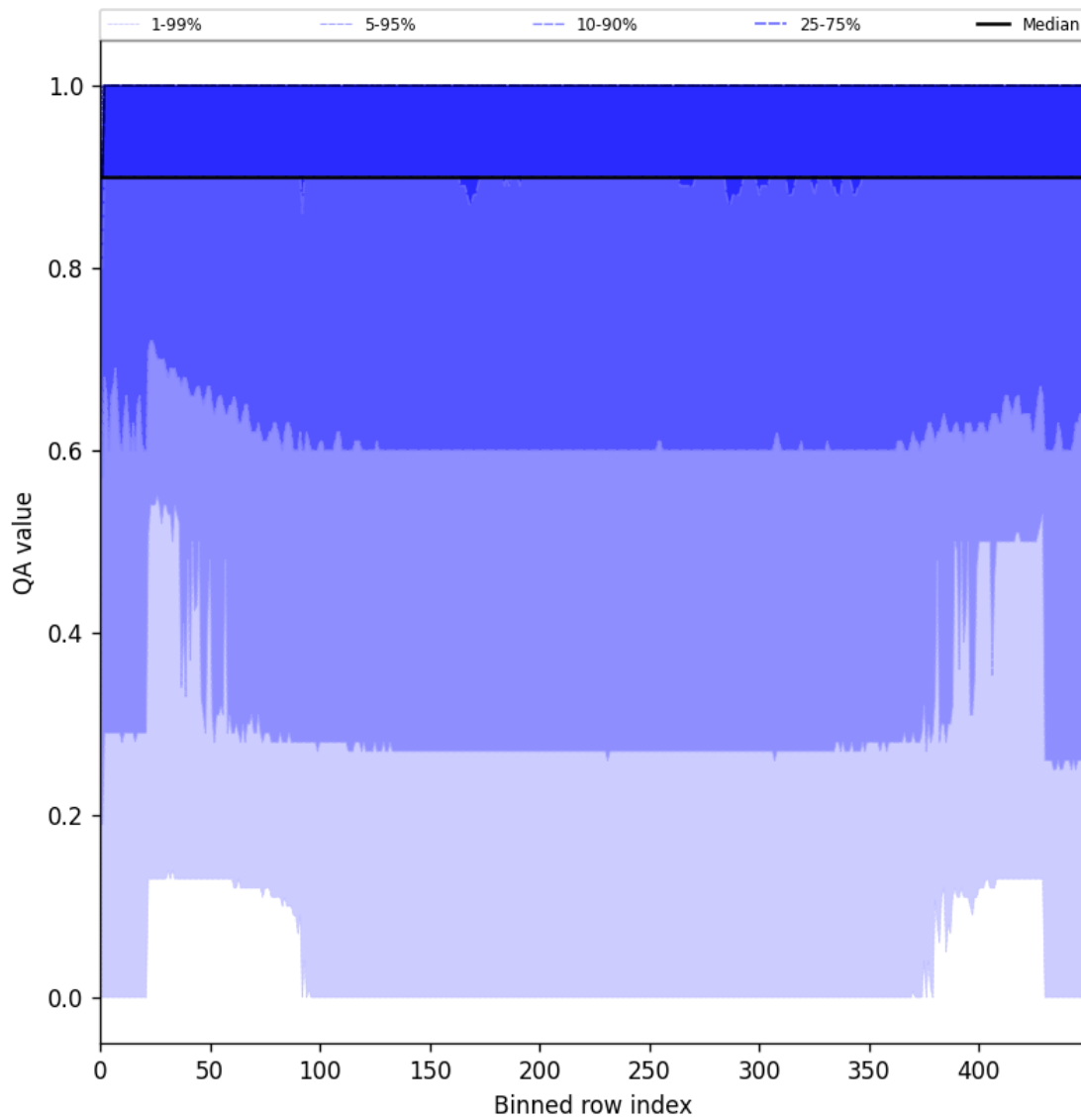
Figure 27: Along track statistics of “QA value” for 2025-06-27 to 2025-06-28
