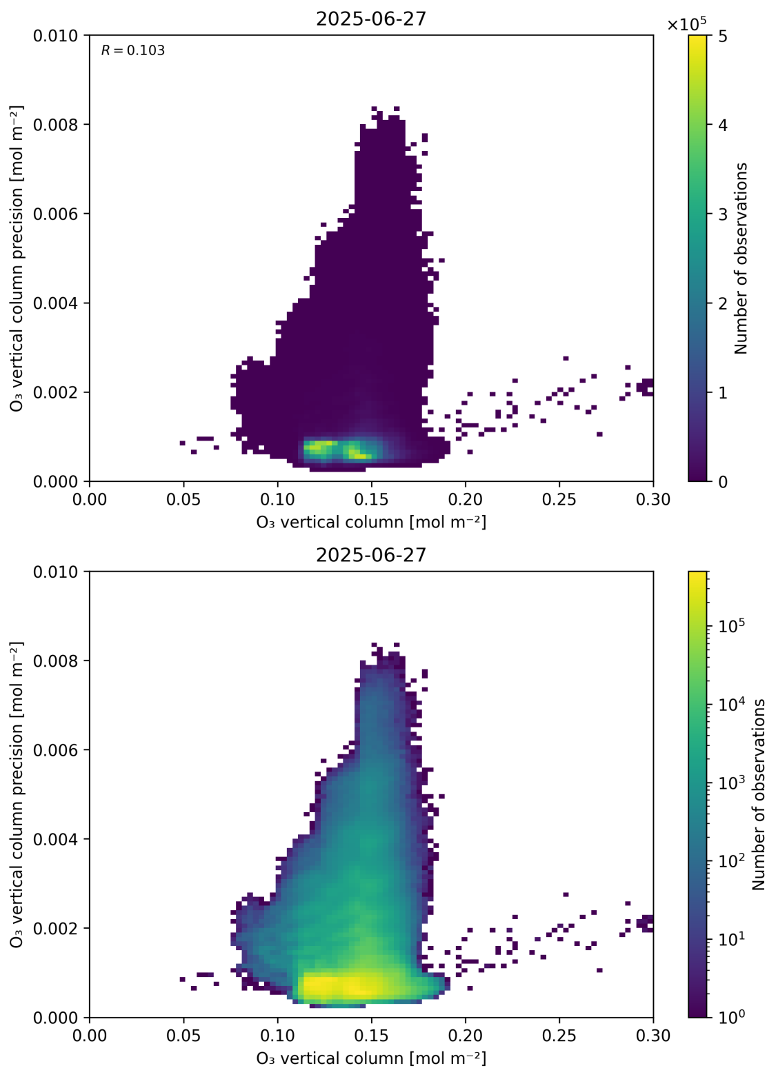
Figure 41: Scatter density plot of “O 3 vertical column” against “O 3 vertical column precision” for 2025-06-27 to 2025-06-28.
