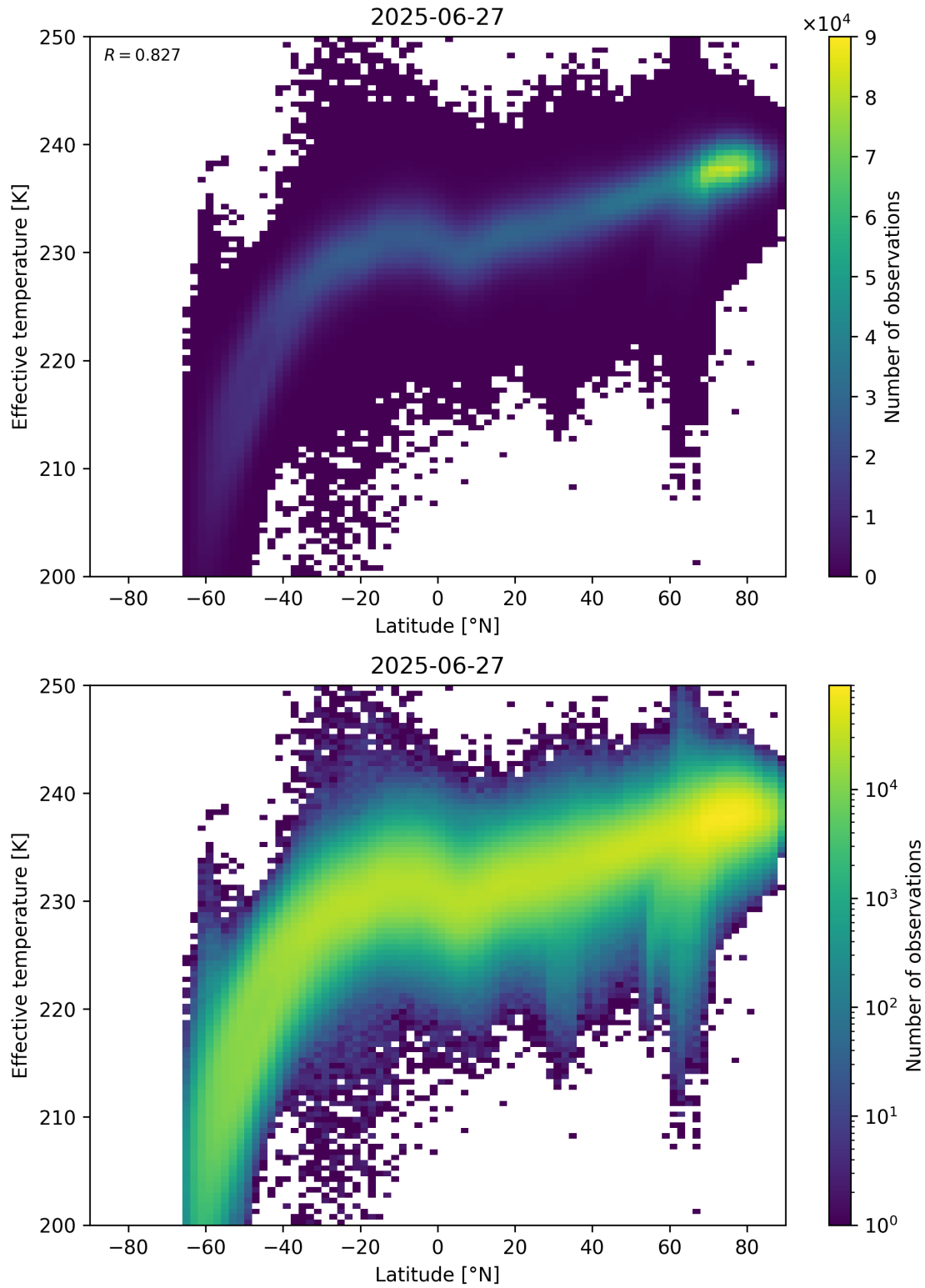
Figure 34: Scatter density plot of “Latitude” against “Effective temperature” for 2025-06-27 to 2025-06-28.
