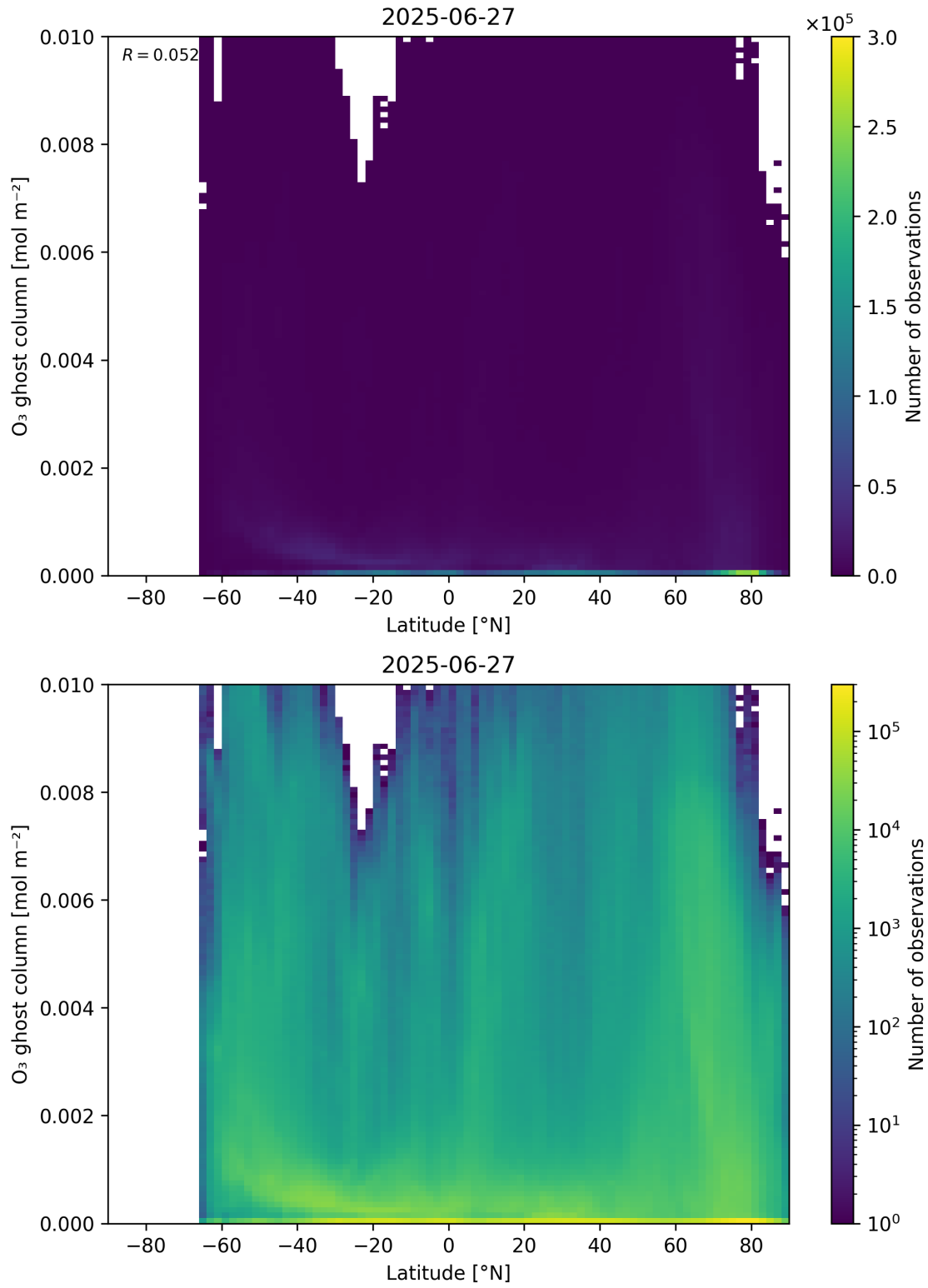
Figure 35: Scatter density plot of “Latitude” against “O 3 ghost column” for 2025-06-27 to 2025-06-28.
