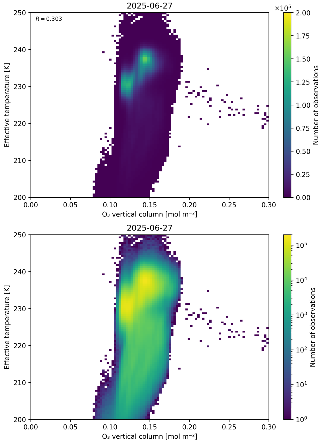
Figure 39: Scatter density plot of “O 3 vertical column” against “Effective temperature” for 2025-06-27 to 2025-06-28.
