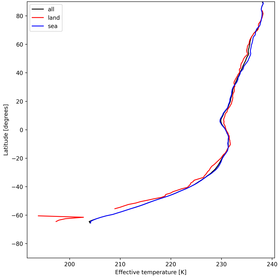
Figure 17: Zonal average of "Effective temperature" for 2025-06-27 to 2025-06-28.
