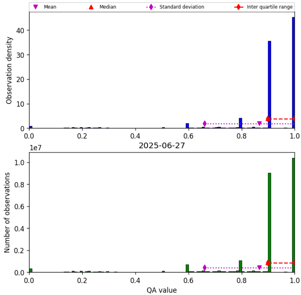
Figure 20: Histogram of “QA value” for 2025-06-27 to 2025-06-28
