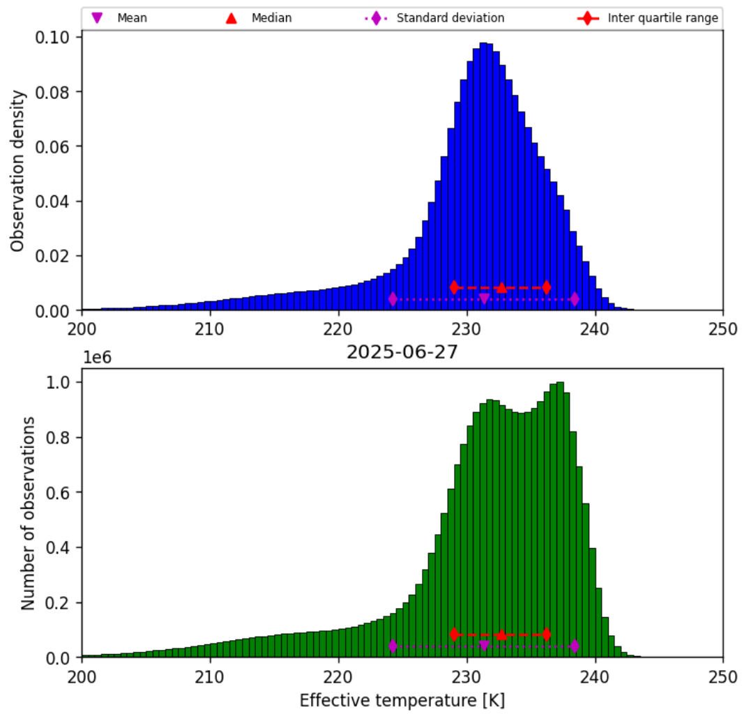
Figure 24: Histogram of “Effective temperature” for 2025-06-27 to 2025-06-28
