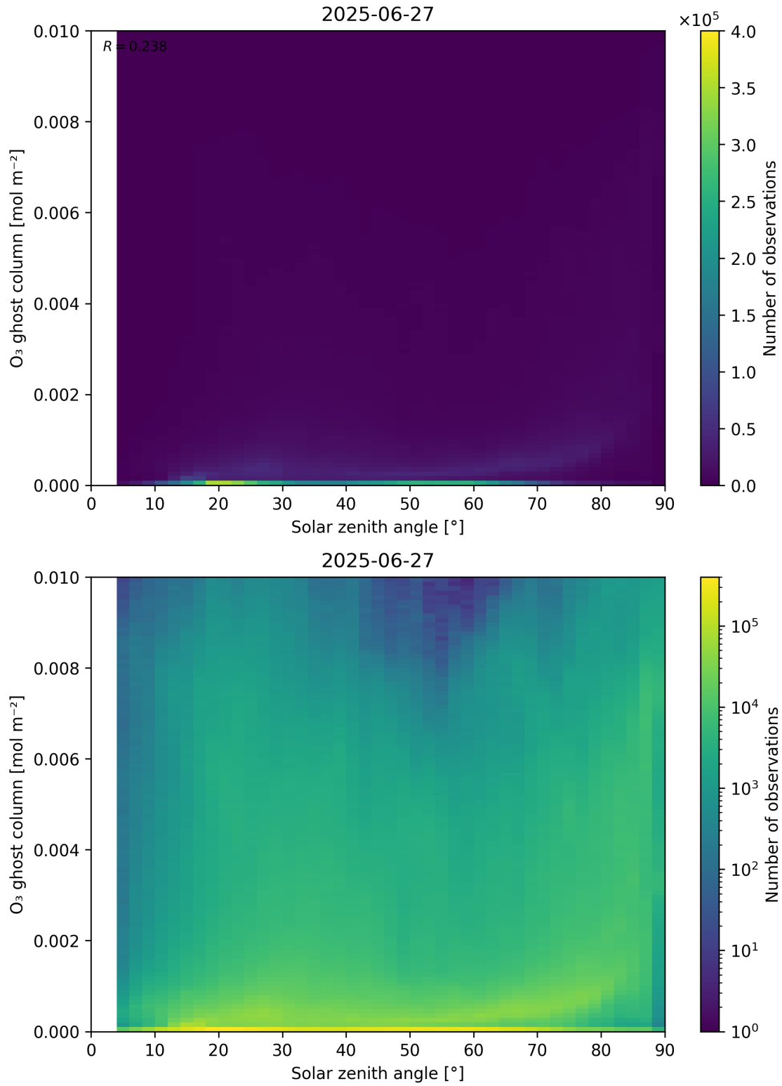
Figure 46: Scatter density plot of “Solar zenith angle” against “O 3 ghost column” for 2025-06-27 to 2025-06-28.
