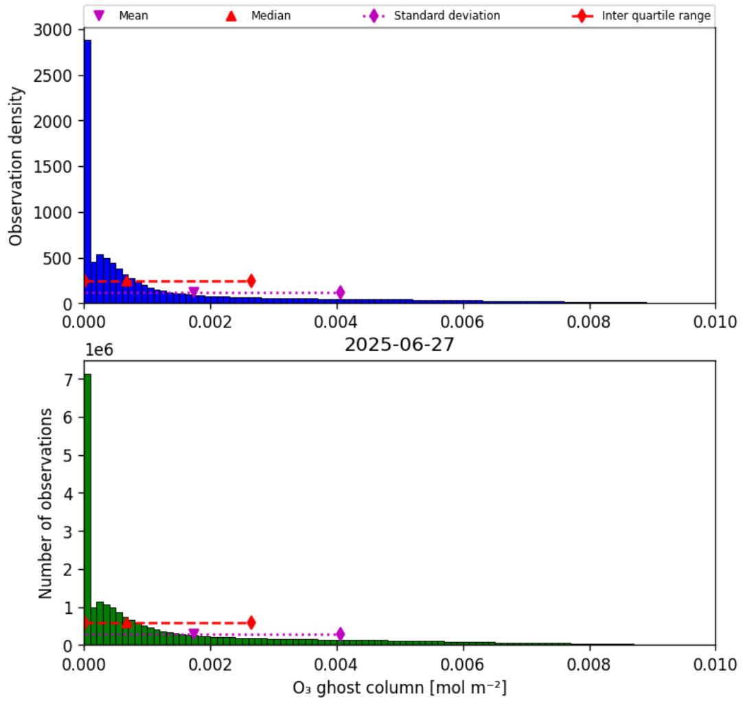
Figure 25: Histogram of “O 3 ghost column” for 2025-06-27 to 2025-06-28
