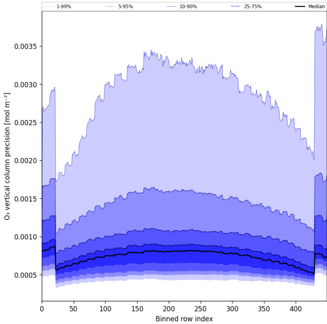
Figure 29: Along track statistics of “O 3 vertical column precision” for 2025-06-27 to 2025-06-28
