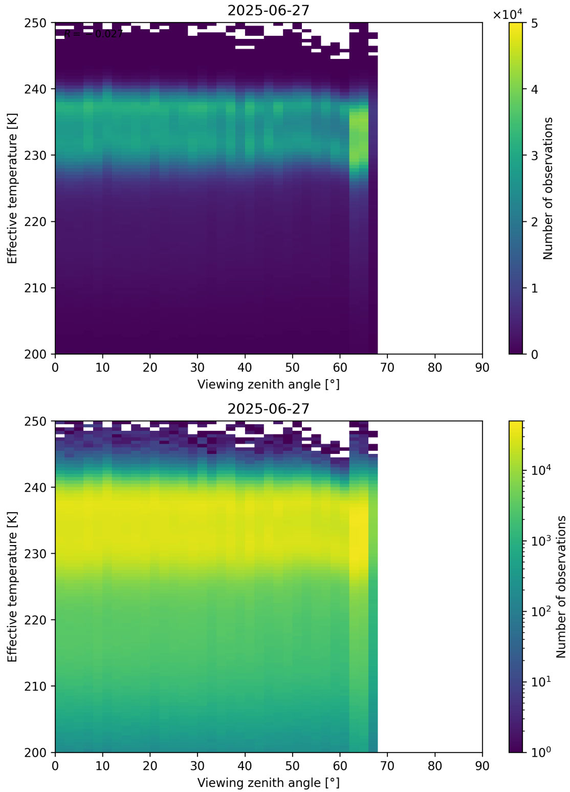
Figure 50: Scatter density plot of “Viewing zenith angle” against “Effective temperature” for 2025-06-27 to 2025-06-28.
