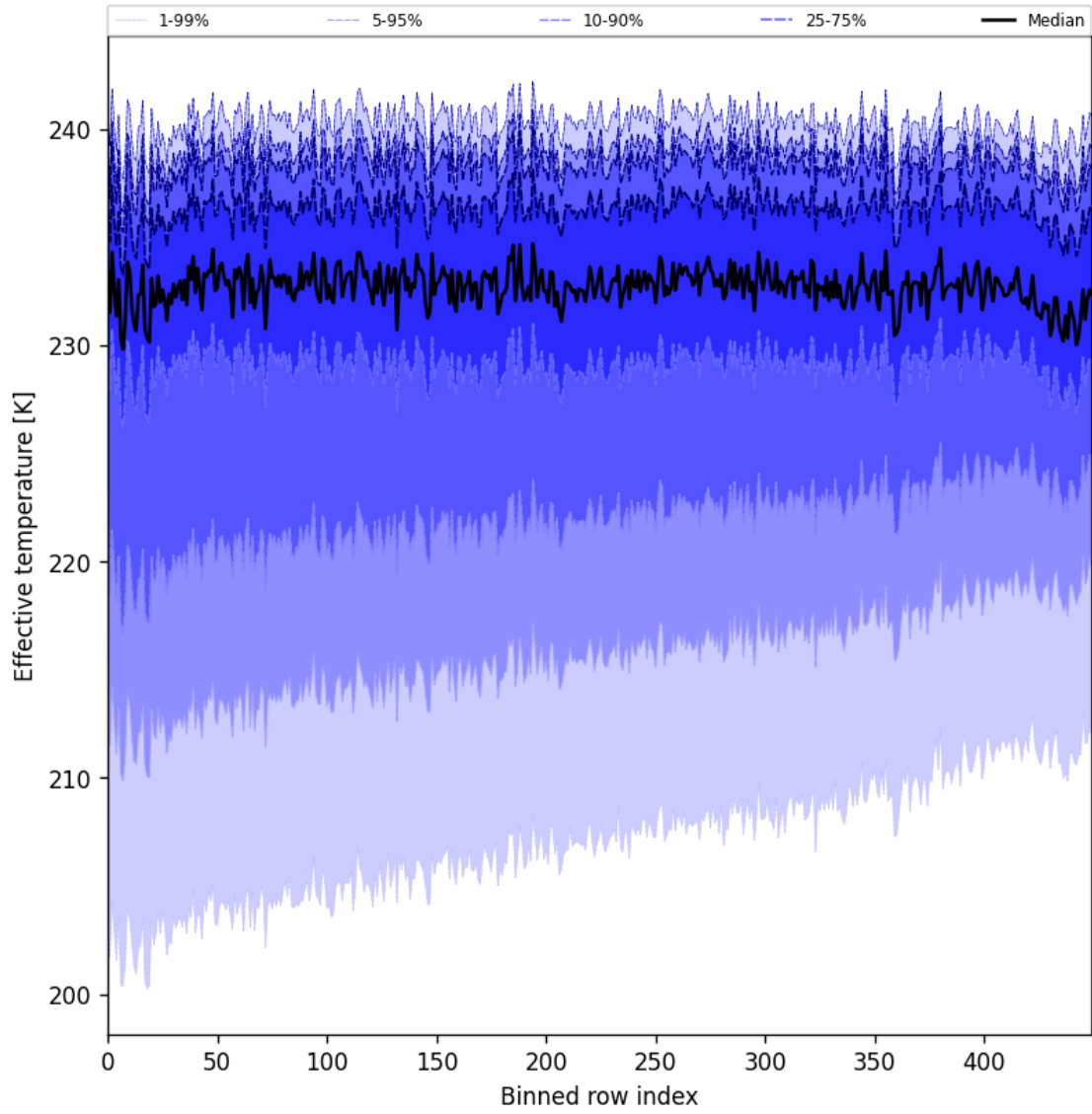
Figure 31: Along track statistics of “Effective temperature” for 2025-06-27 to 2025-06-28
