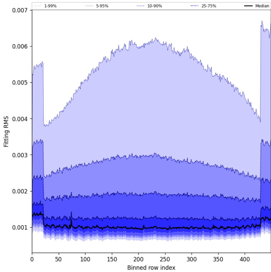
Figure 30: Along track statistics of “Fitting RMS” for 2025-06-27 to 2025-06-28
