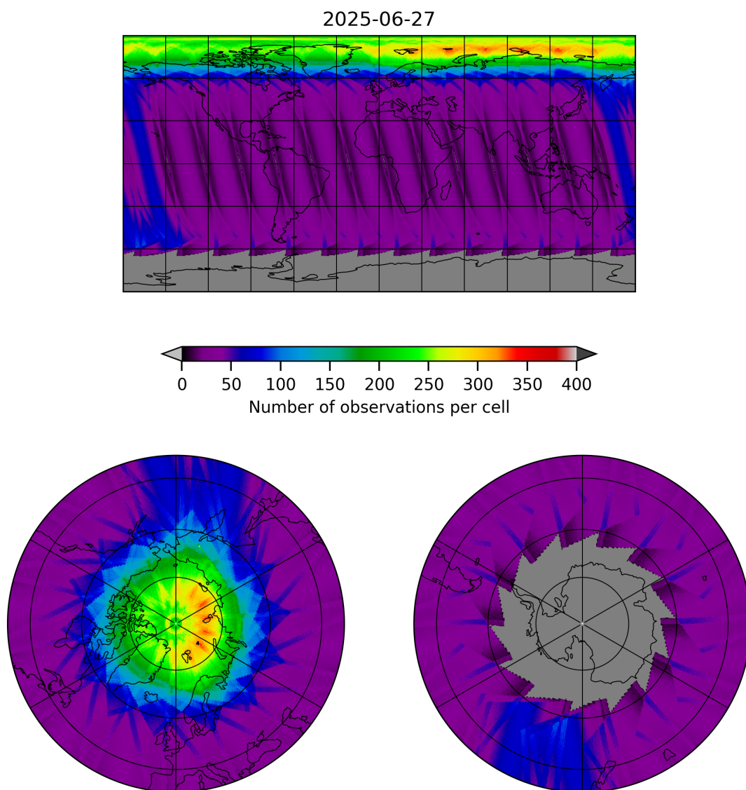
Figure 12: Map of the number of observations for 2025-06-27 to 2025-06-28
