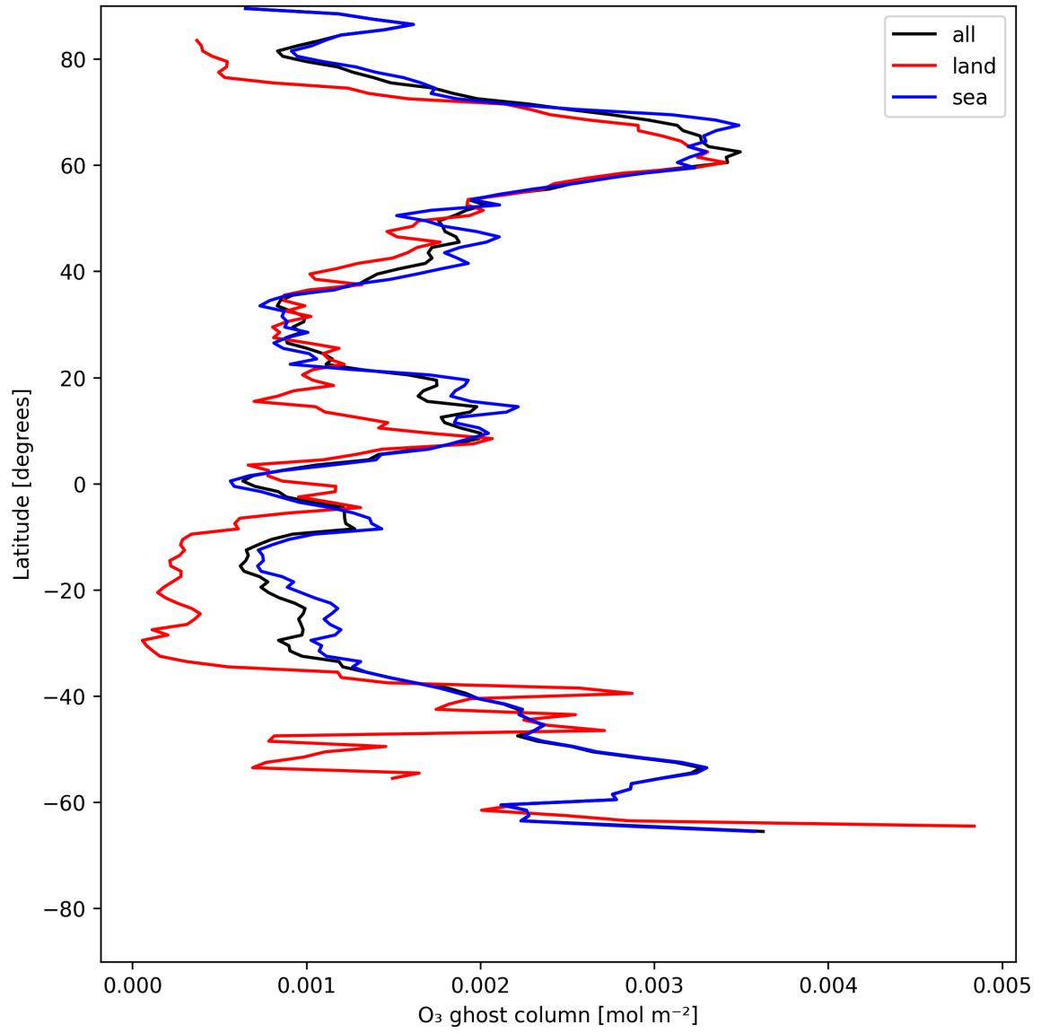
Figure 18: Zonal average of "O 3 ghost column" for 2025-06-27 to 2025-06-28.
