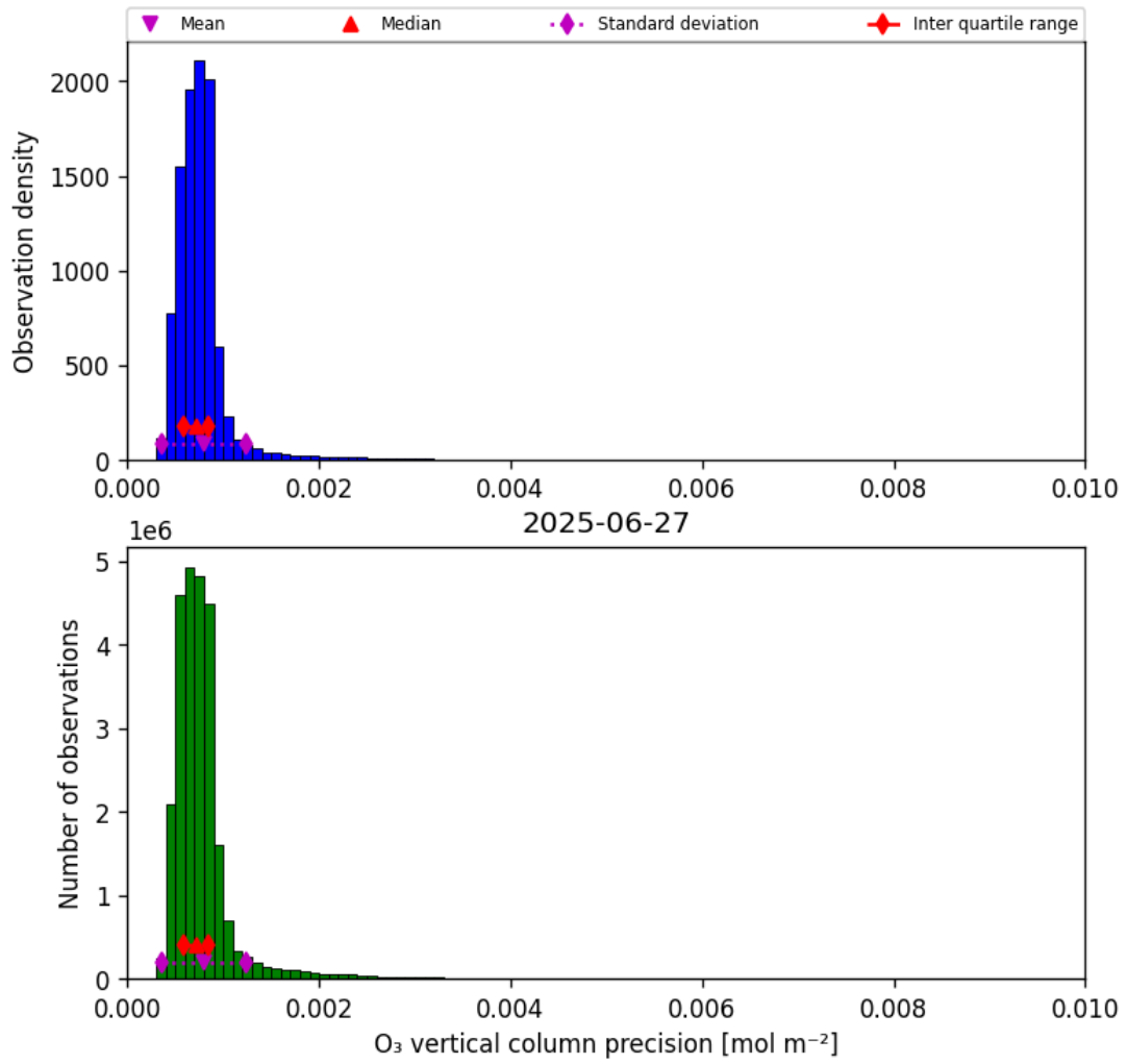
Figure 22: Histogram of “O 3 vertical column precision” for 2025-06-27 to 2025-06-28
