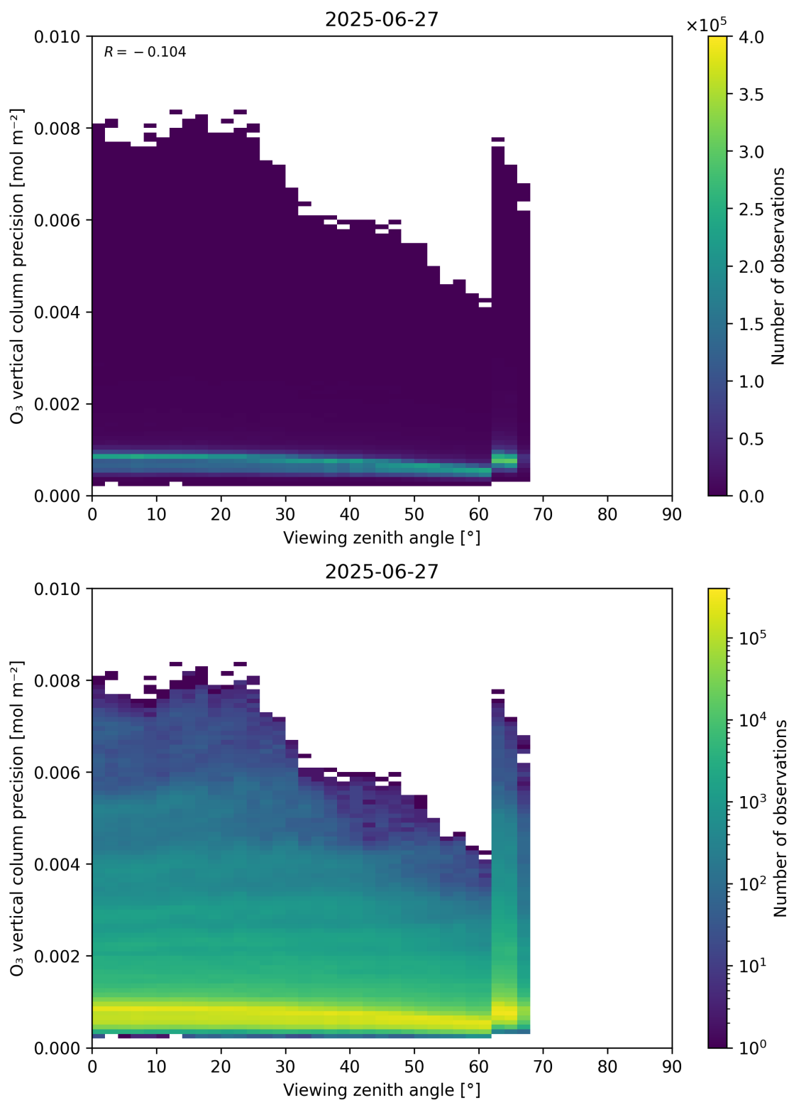
Figure 53: Scatter density plot of “Viewing zenith angle” against “O 3 vertical column precision” for 2025-06-27 to 2025-06-28.
