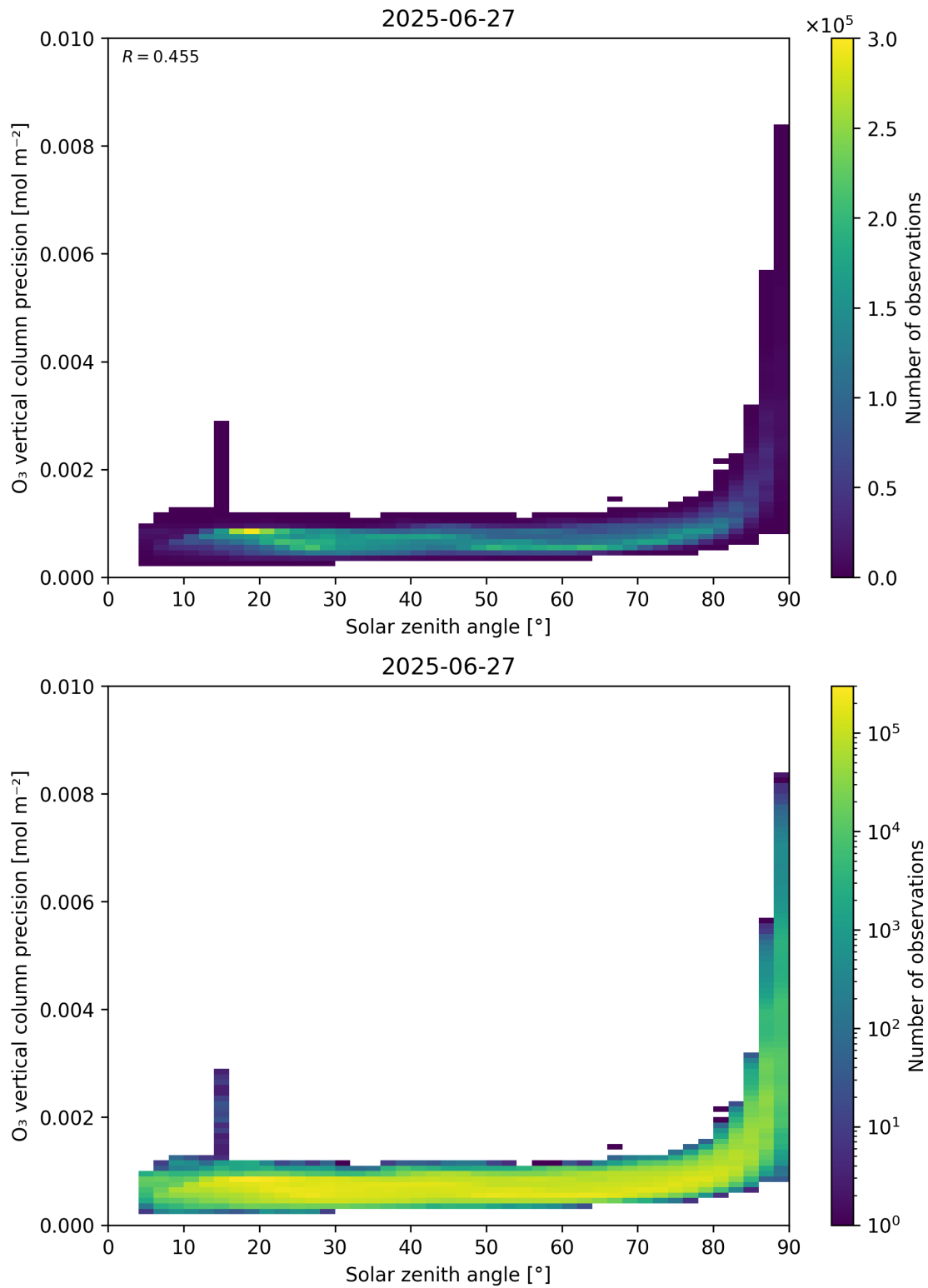
Figure 48: Scatter density plot of “Solar zenith angle” against “O 3 vertical column precision” for 2025-06-27 to 2025-06-28.
