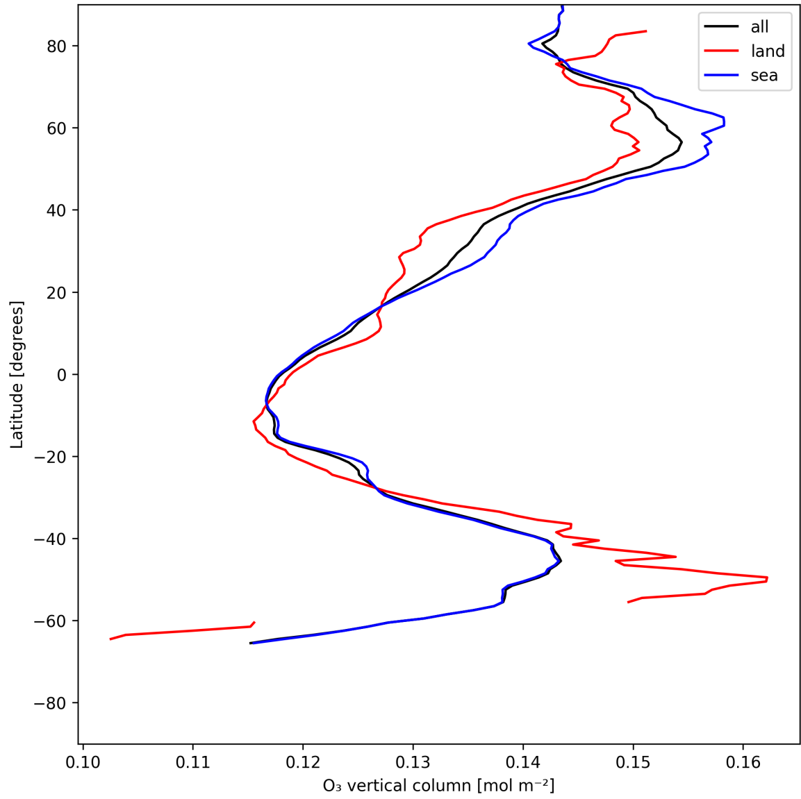
Figure 14: Zonal average of “O 3 vertical column” for 2025-06-27 to 2025-06-28.
