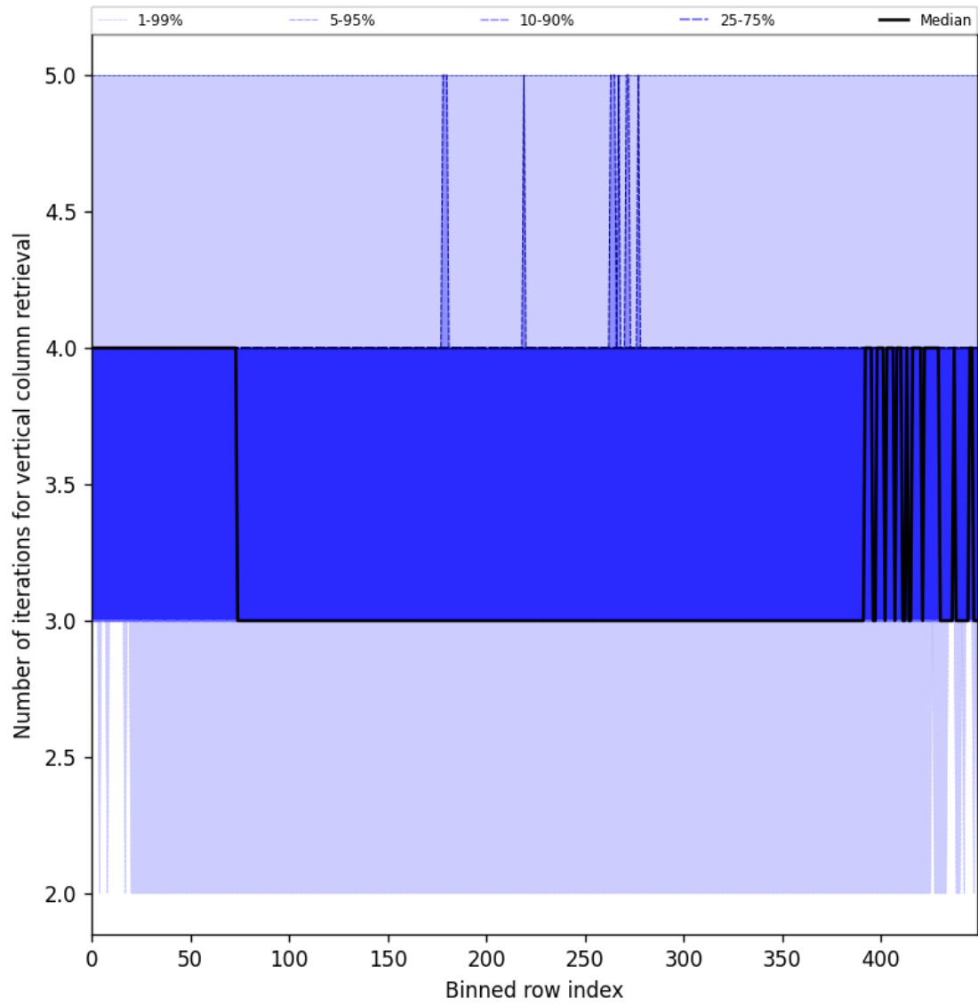
Figure 33: Along track statistics of “Number of iterations for vertical column retrieval” for 2025-06-27 to 2025-06-28
