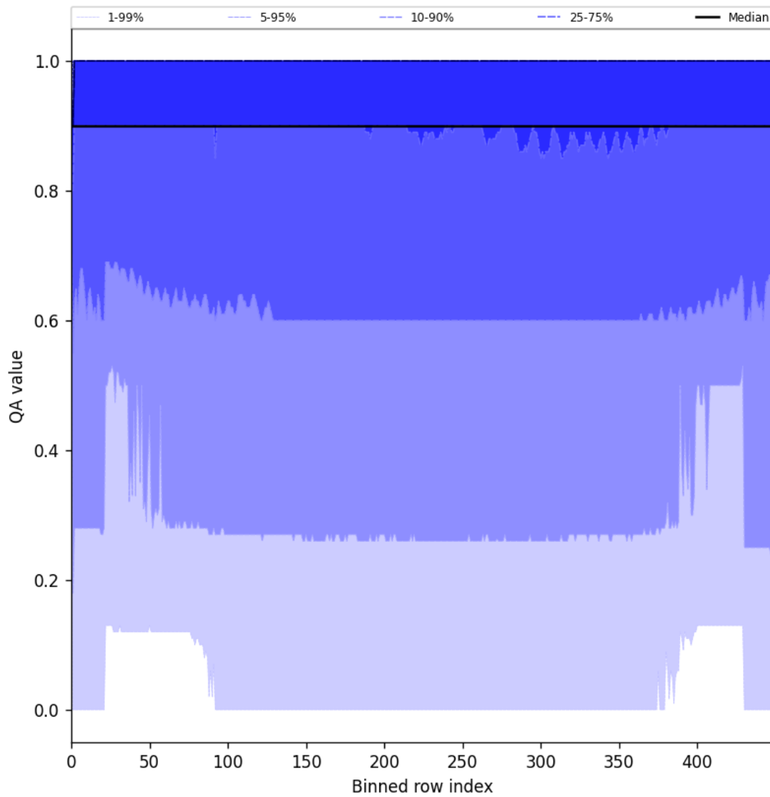
Figure 27: Along track statistics of “QA value” for 2025-06-27 to 2025-06-29
