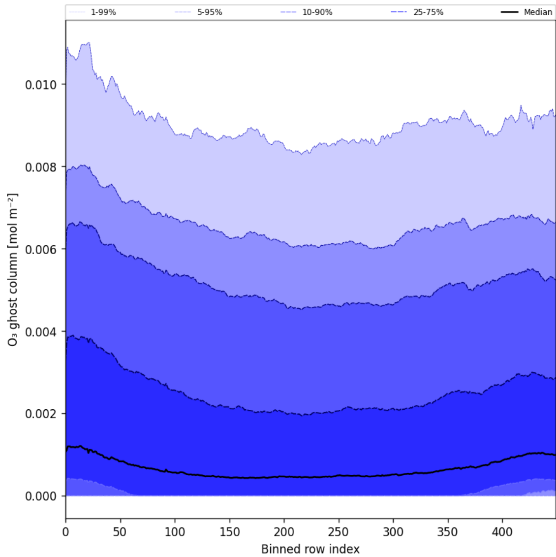
Figure 32: Along track statistics of “O 3 ghost column” for 2025-06-27 to 2025-06-29
