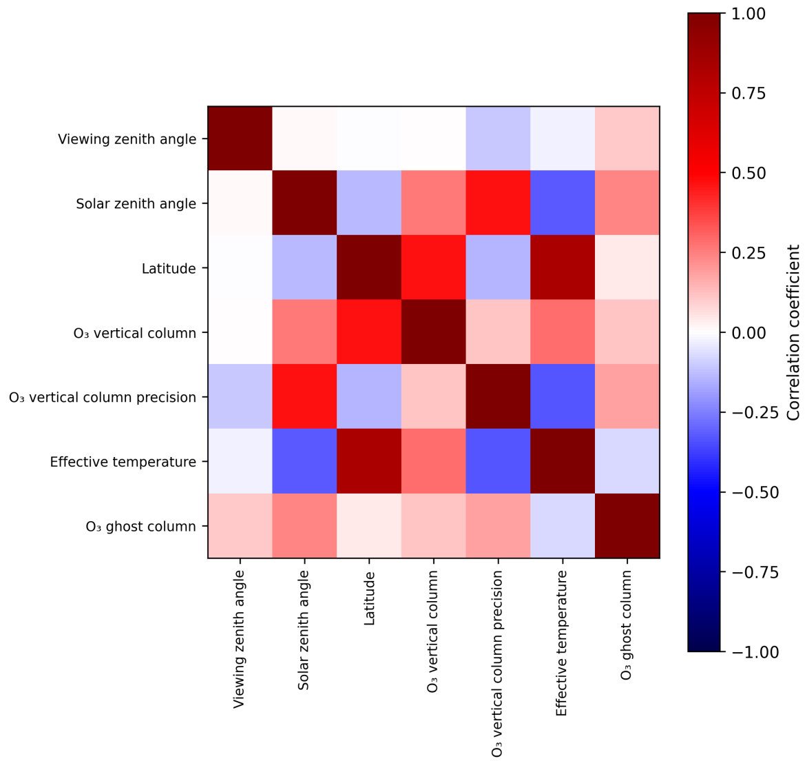
Figure 2: Map of correlation matrix for 2025-06-27 to 2025-06-29.
