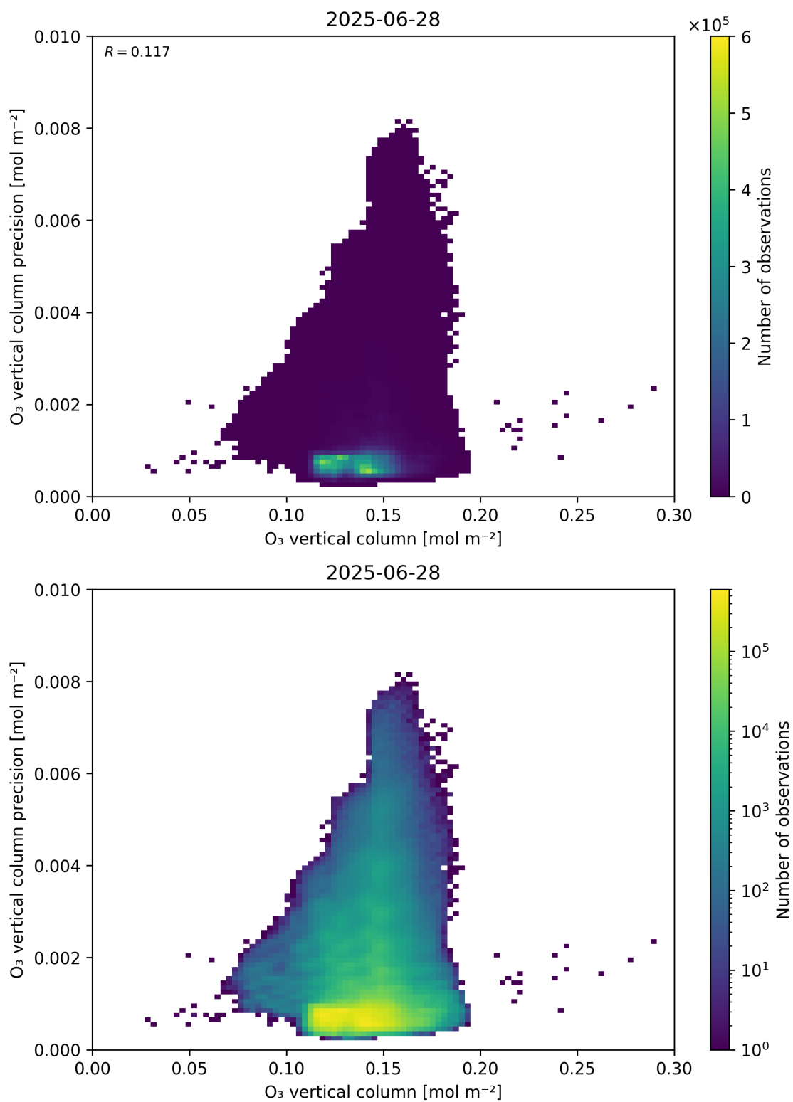
Figure 41: Scatter density plot of “O 3 vertical column” against “O 3 vertical column precision” for 2025-06-27 to 2025-06-29.
