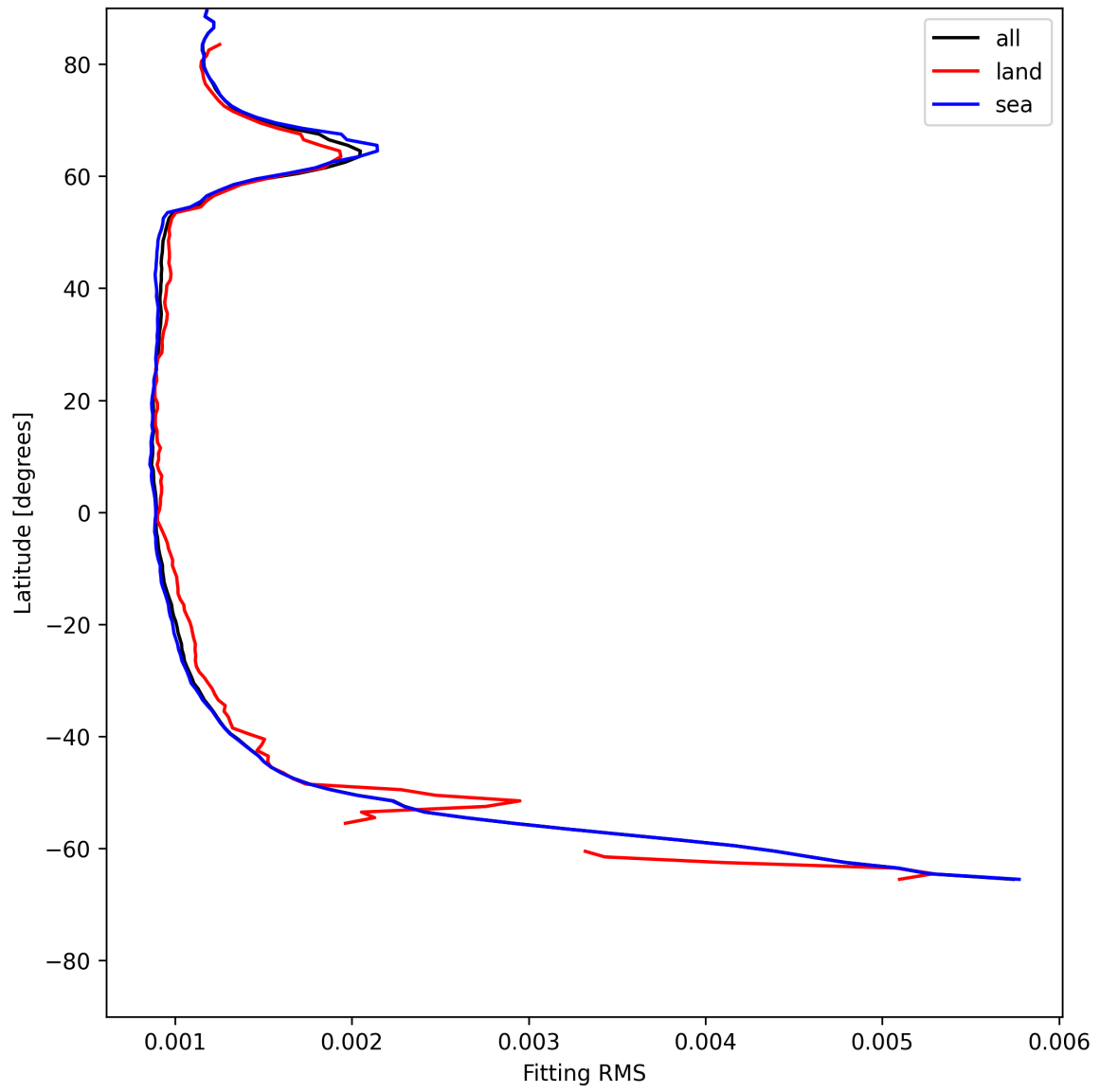
Figure 16: Zonal average of “Fitting RMS” for 2025-06-27 to 2025-06-29.
