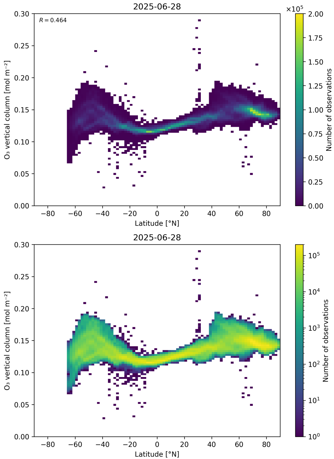
Figure 36: Scatter density plot of “Latitude” against “O 3 vertical column” for 2025-06-27 to 2025-06-29.
