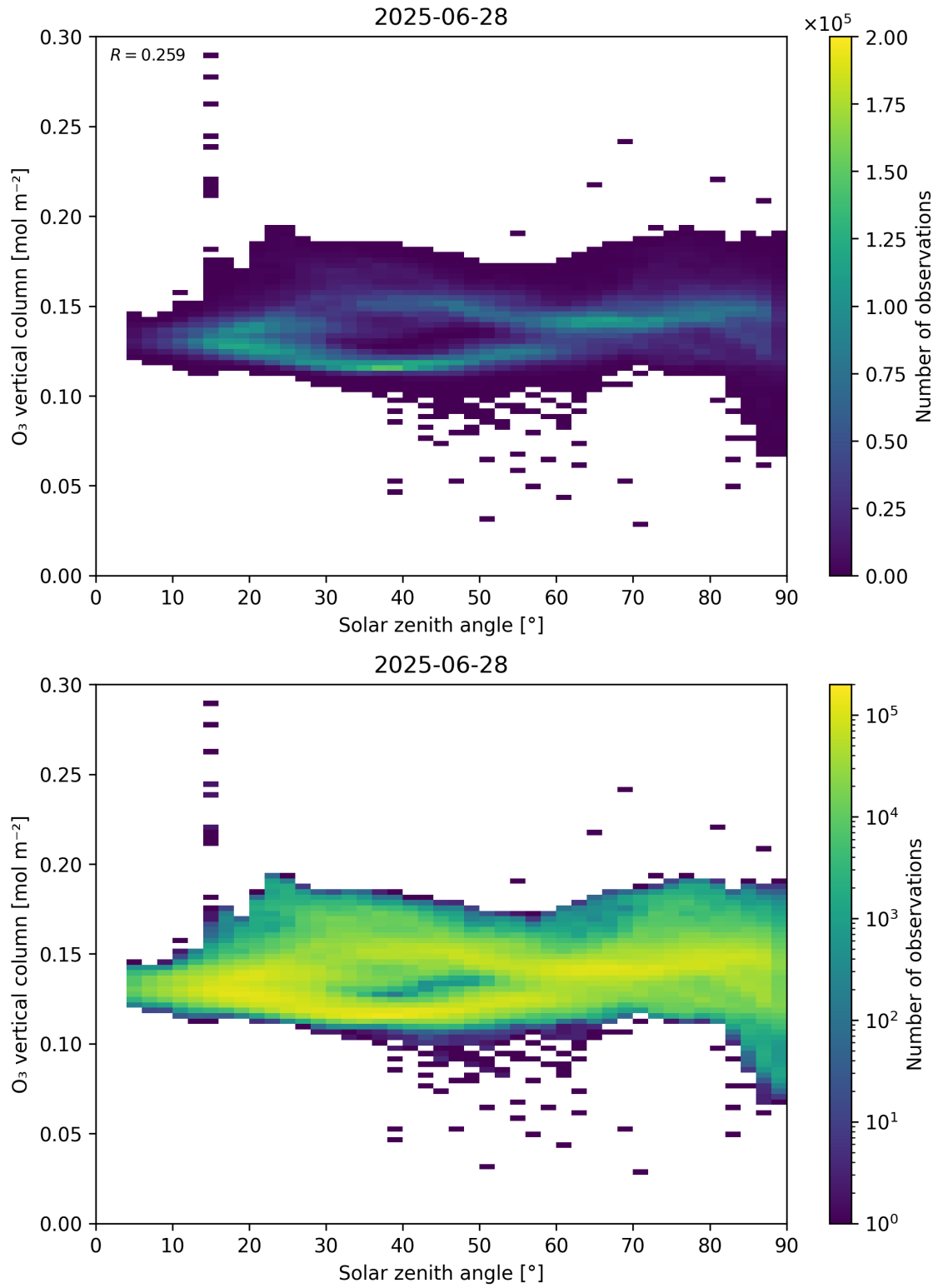
Figure 47: Scatter density plot of “Solar zenith angle” against “O 3 vertical column” for 2025-06-27 to 2025-06-29.
