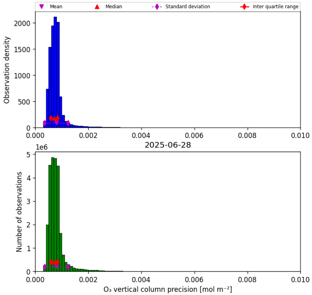
Figure 22: Histogram of “O 3 vertical column precision” for 2025-06-27 to 2025-06-29
