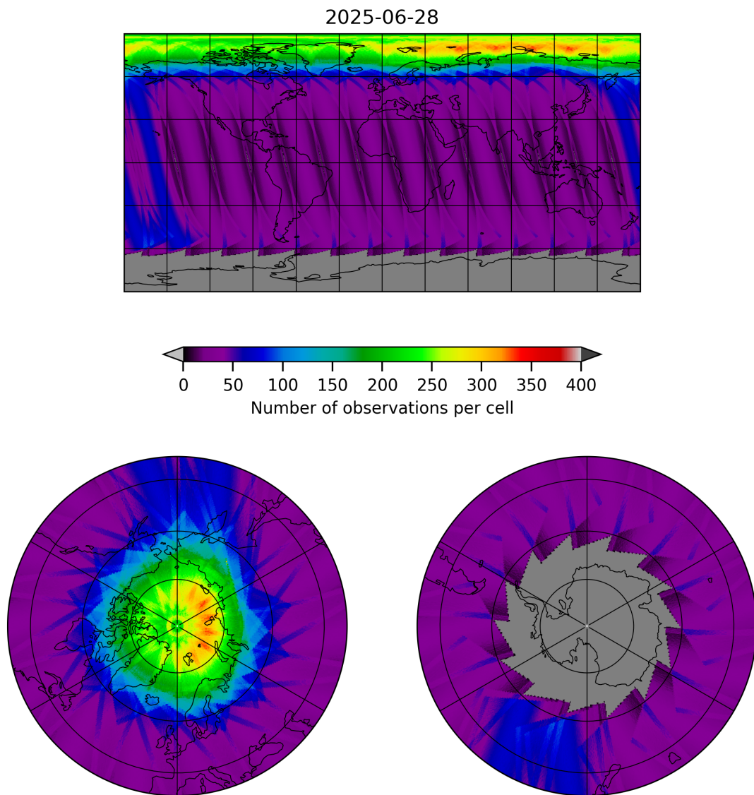
Figure 12: Map of the number of observations for 2025-06-27 to 2025-06-29
