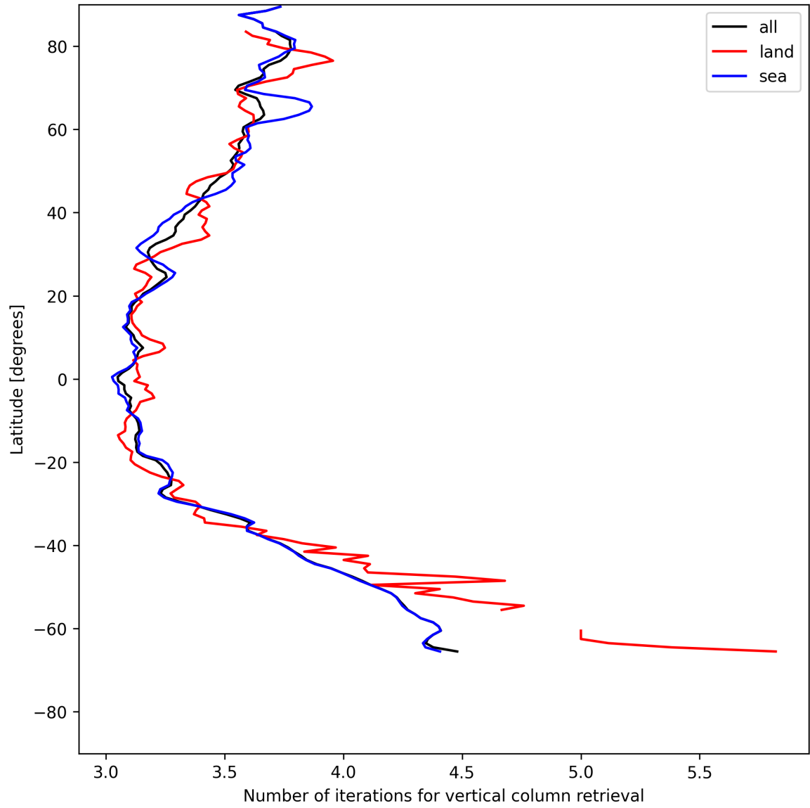
Figure 19: Zonal average of “Number of iterations for vertical column retrieval” for 2025-06-27 to 2025-06-29.
