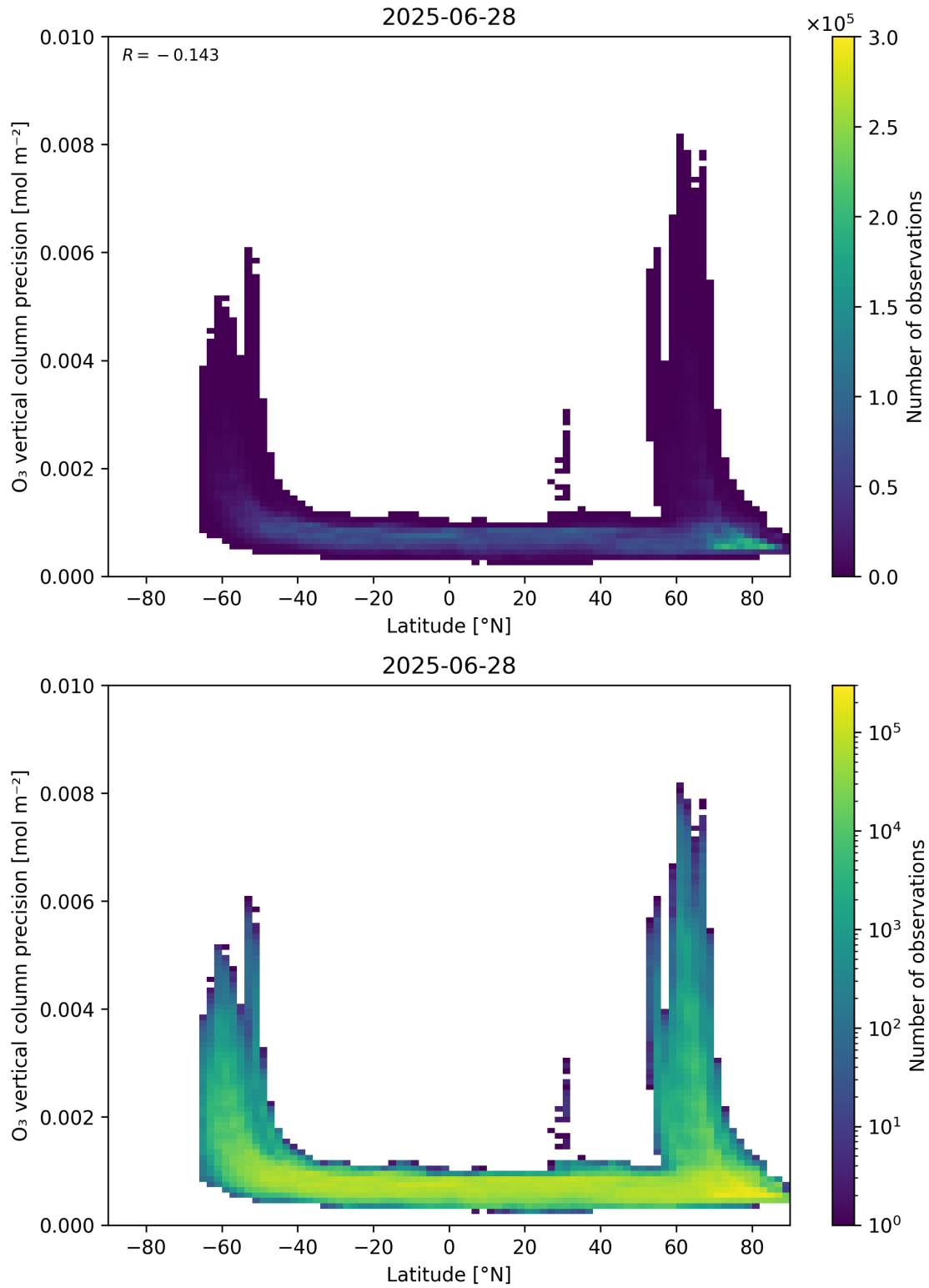
Figure 37: Scatter density plot of “Latitude” against “O 3 vertical column precision” for 2025-06-27 to 2025-06-29.
