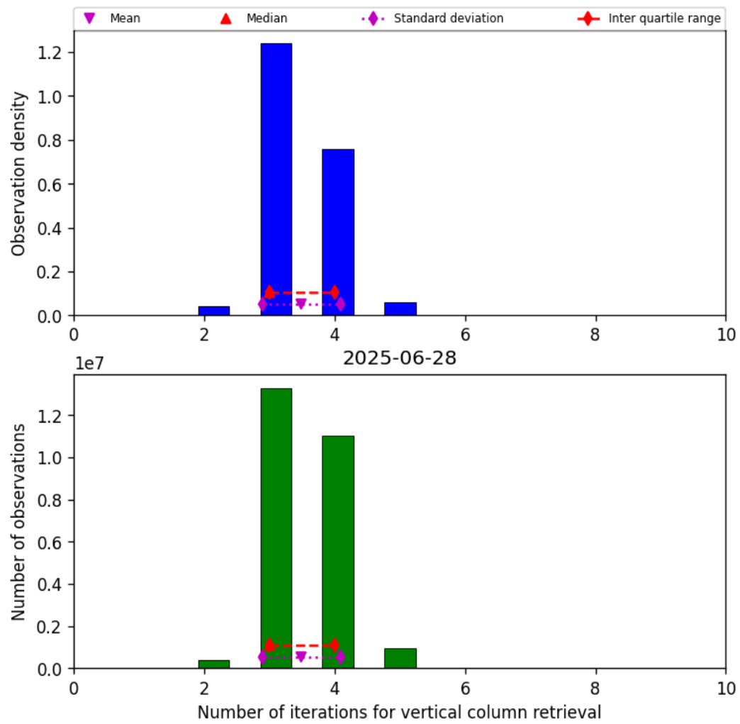
Figure 26: Histogram of “Number of iterations for vertical column retrieval” for 2025-06-27 to 2025-06-29
