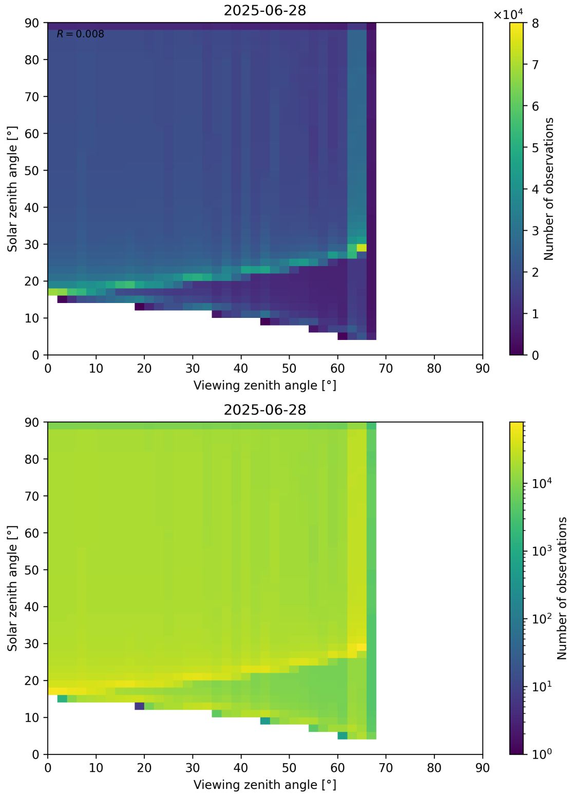
Figure 54: Scatter density plot of “Viewing zenith angle” against “Solar zenith angle” for 2025-06-27 to 2025-06-29.
