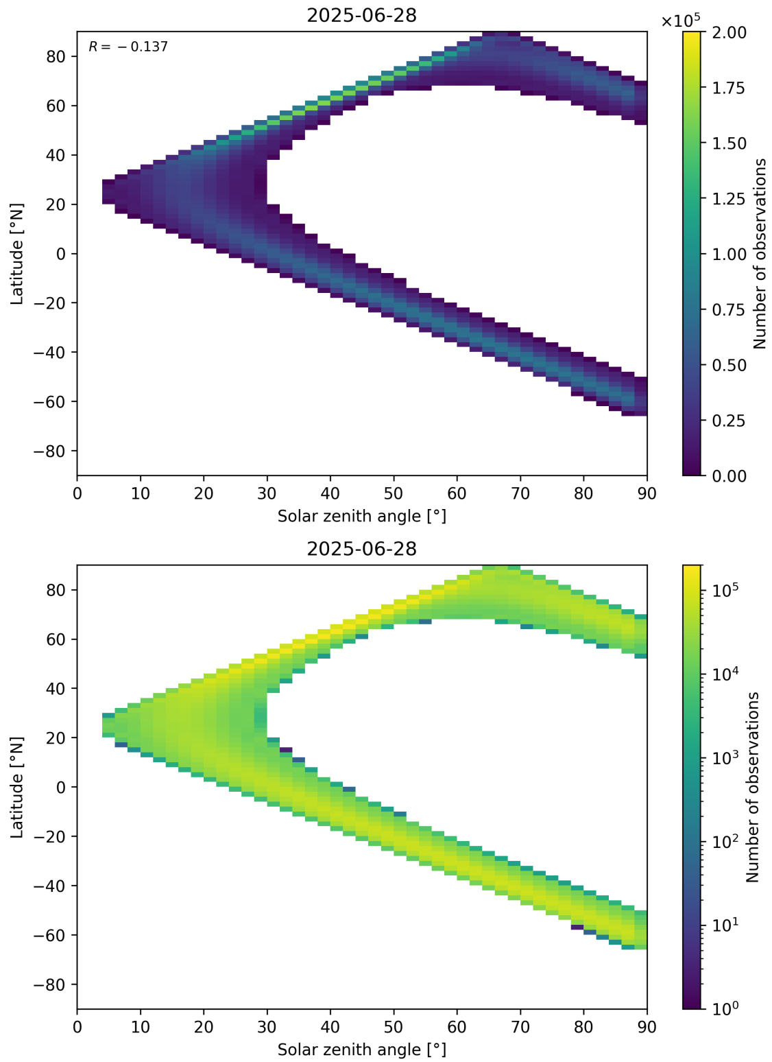
Figure 44: Scatter density plot of “Solar zenith angle” against “Latitude” for 2025-06-27 to 2025-06-29.
