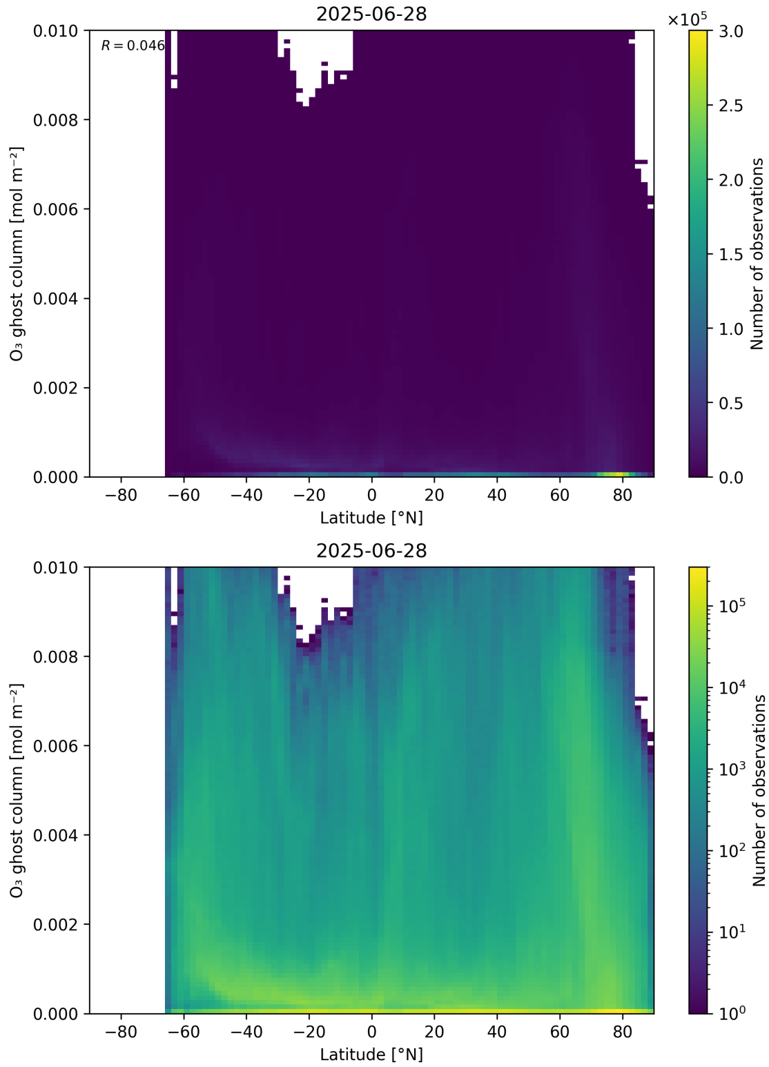
Figure 35: Scatter density plot of “Latitude” against “O 3 ghost column” for 2025-06-27 to 2025-06-29.
