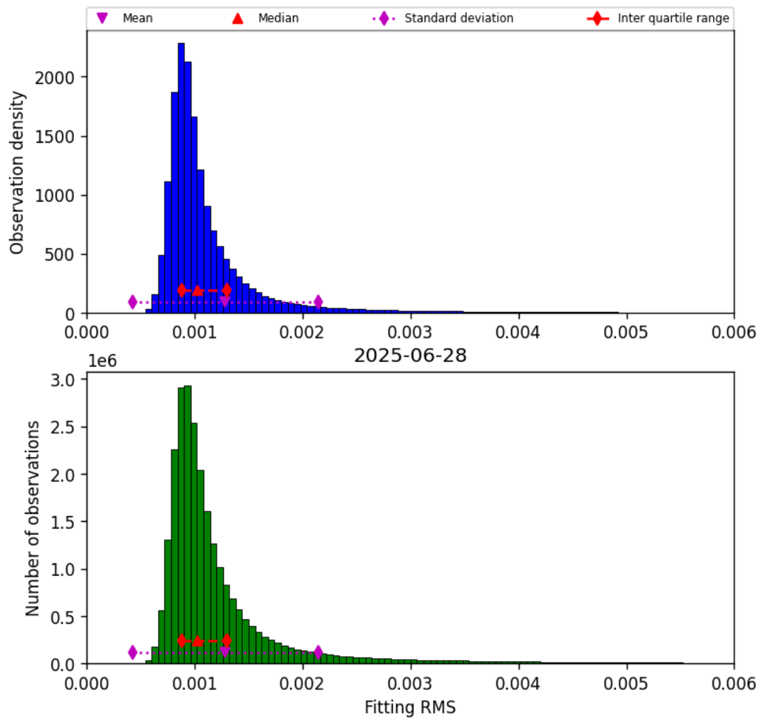
Figure 23: Histogram of “Fitting RMS” for 2025-06-27 to 2025-06-29
