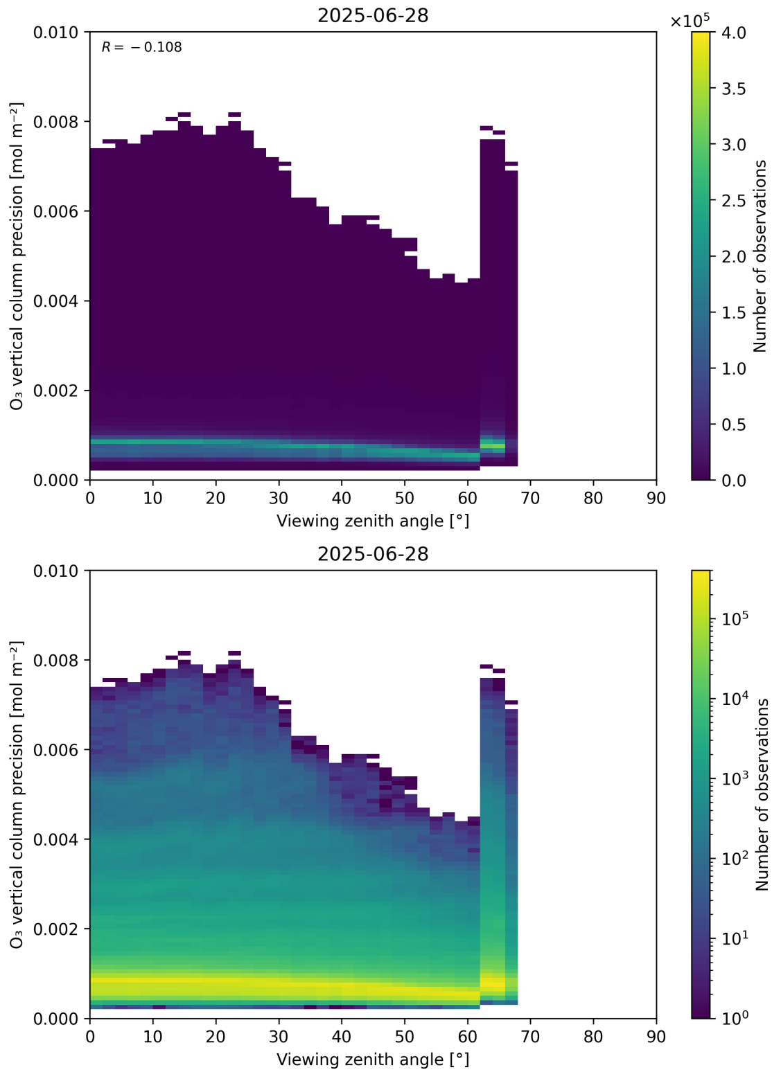
Figure 53: Scatter density plot of “Viewing zenith angle” against “O 3 vertical column precision” for 2025-06-27 to 2025-06-29.
