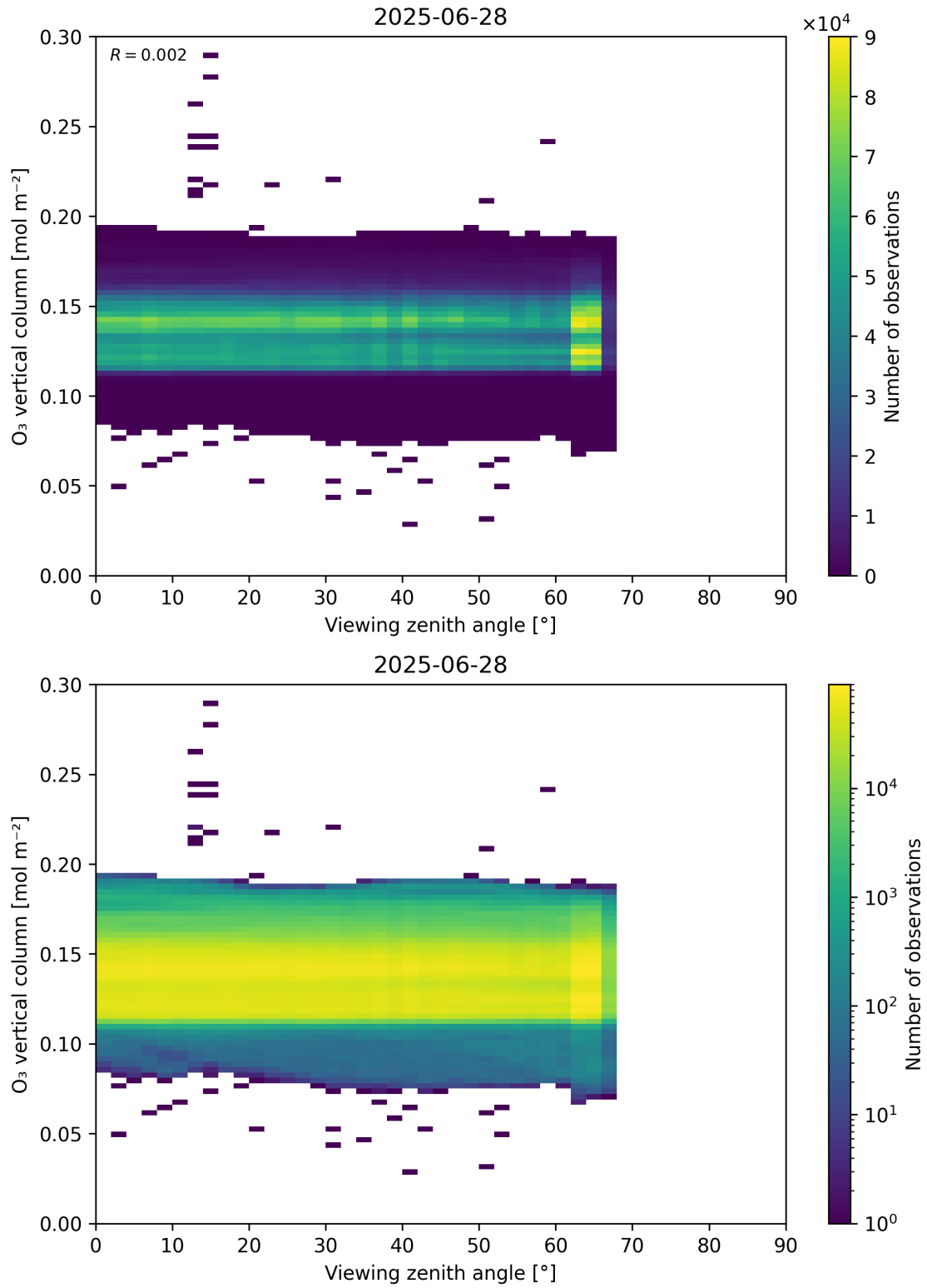
Figure 52: Scatter density plot of “Viewing zenith angle” against “O 3 vertical column” for 2025-06-27 to 2025-06-29.
