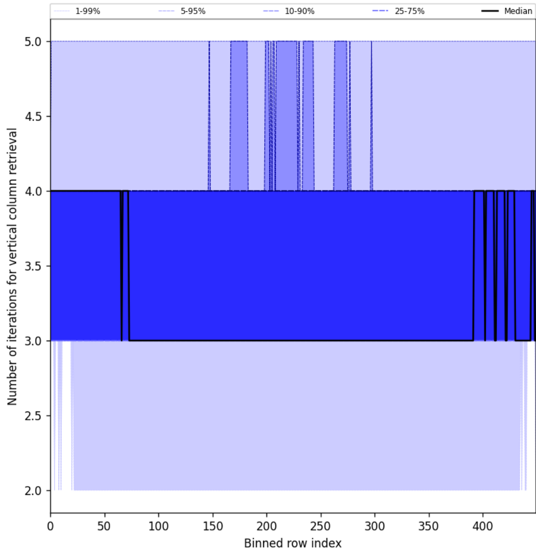
Figure 33: Along track statistics of “Number of iterations for vertical column retrieval” for 2025-06-27 to 2025-06-29
