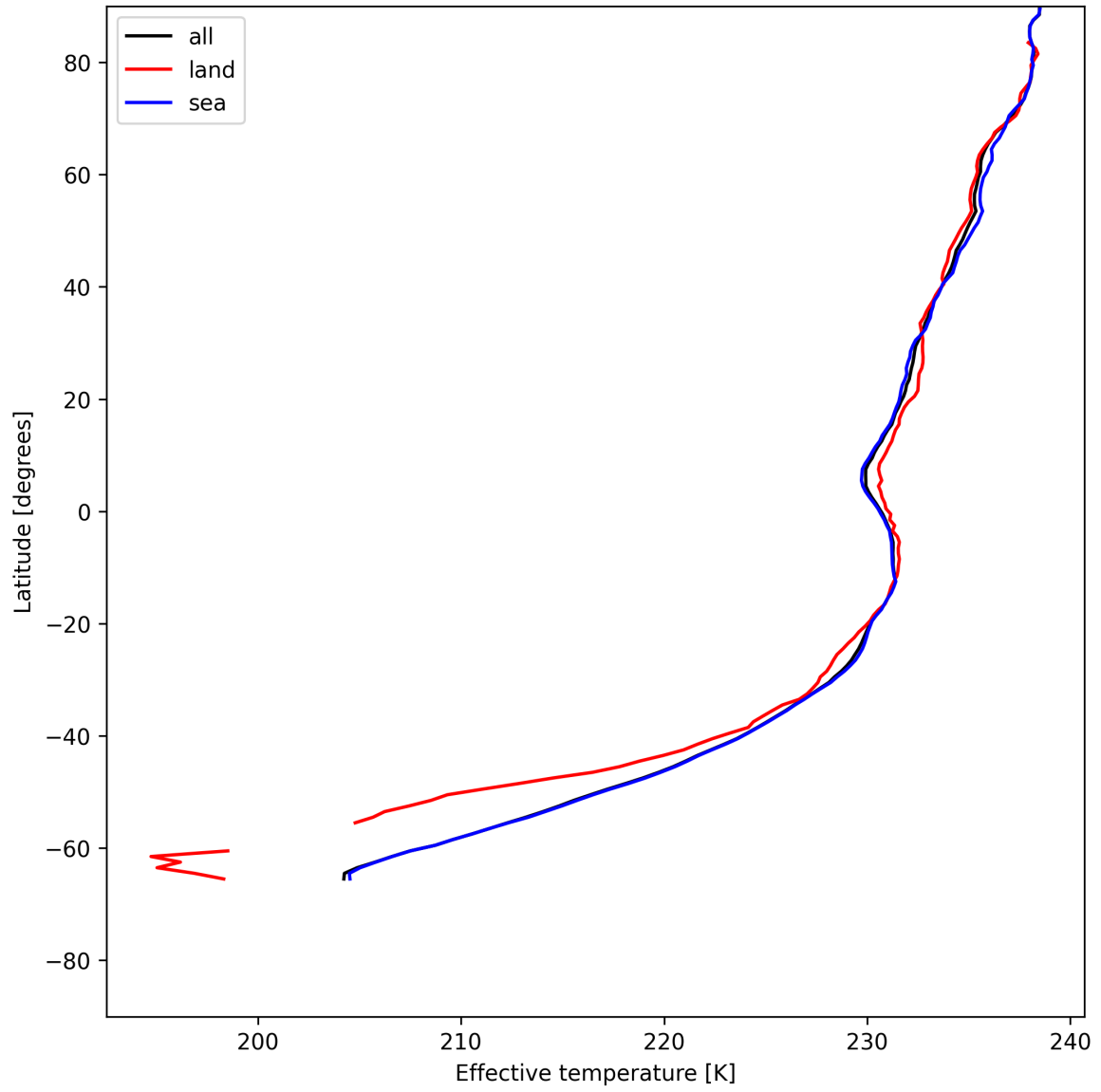
Figure 17: Zonal average of "Effective temperature" for 2025-06-27 to 2025-06-29.
