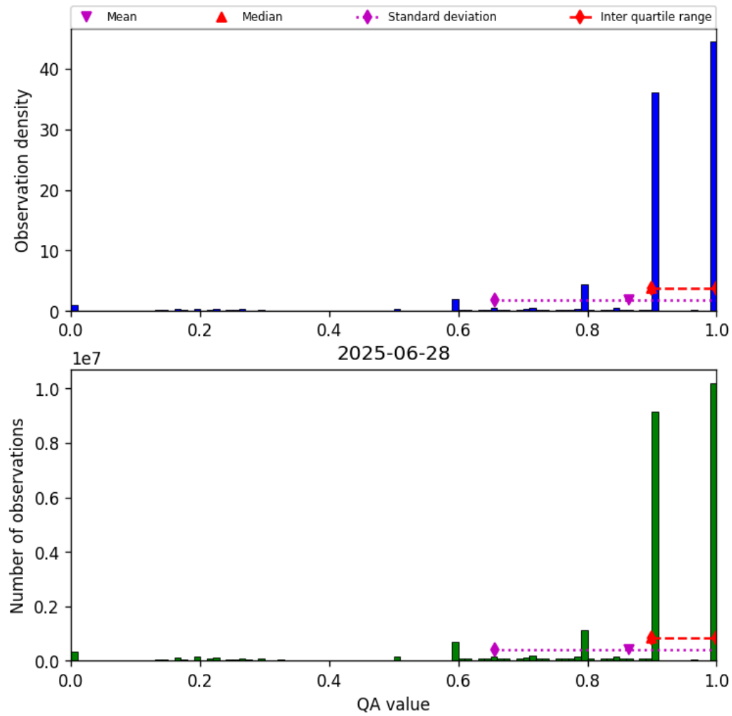
Figure 20: Histogram of “QA value” for 2025-06-27 to 2025-06-29
