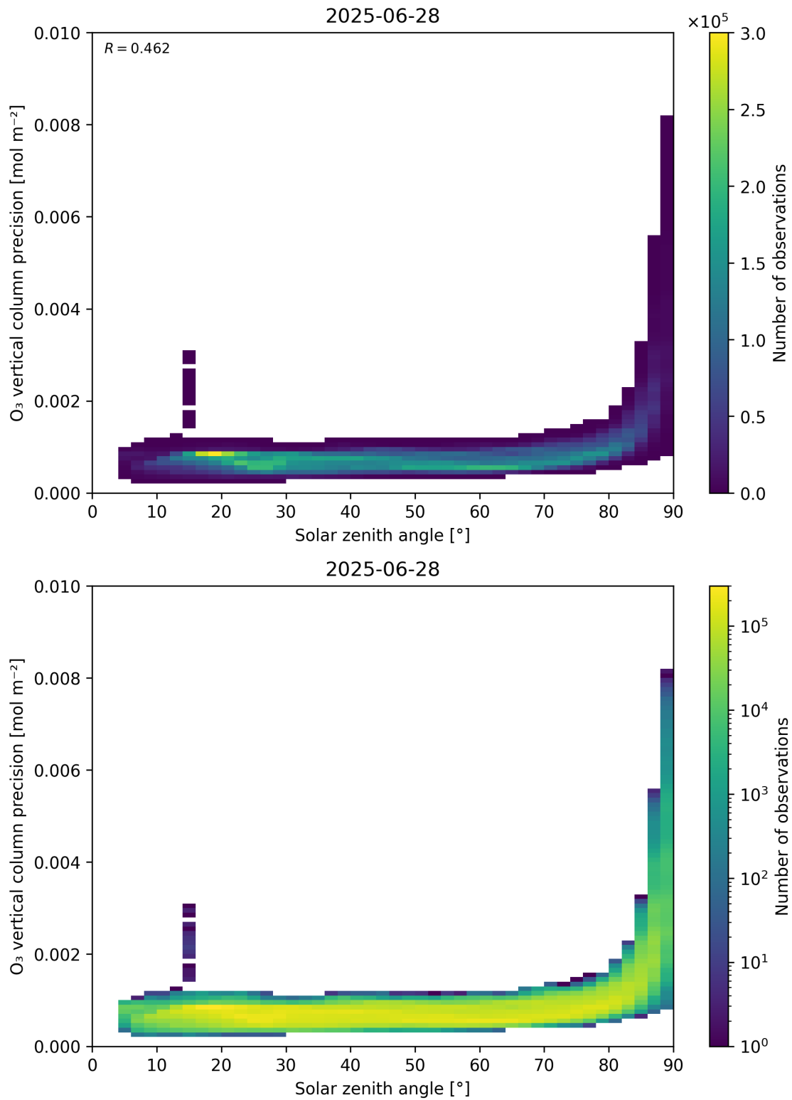
Figure 48: Scatter density plot of “Solar zenith angle” against “O 3 vertical column precision” for 2025-06-27 to 2025-06-29.
