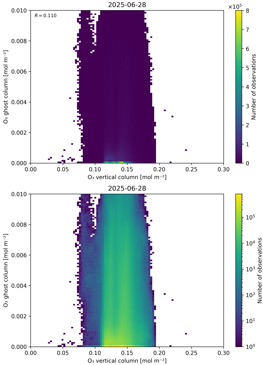
Figure 40: Scatter density plot of “O 3 vertical column” against “O 3 ghost column” for 2025-06-27 to 2025-06-29.
