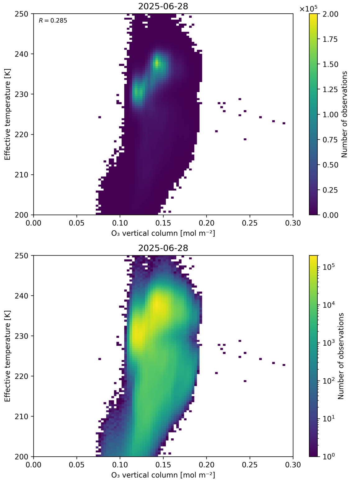
Figure 39: Scatter density plot of “O 3 vertical column” against “Effective temperature” for 2025-06-27 to 2025-06-29.
