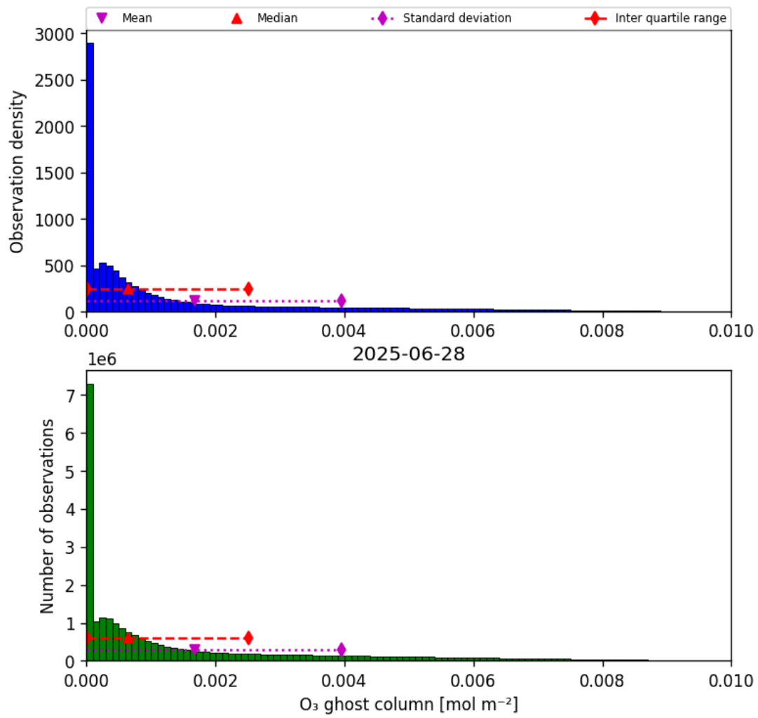
Figure 25: Histogram of “O 3 ghost column” for 2025-06-27 to 2025-06-29
