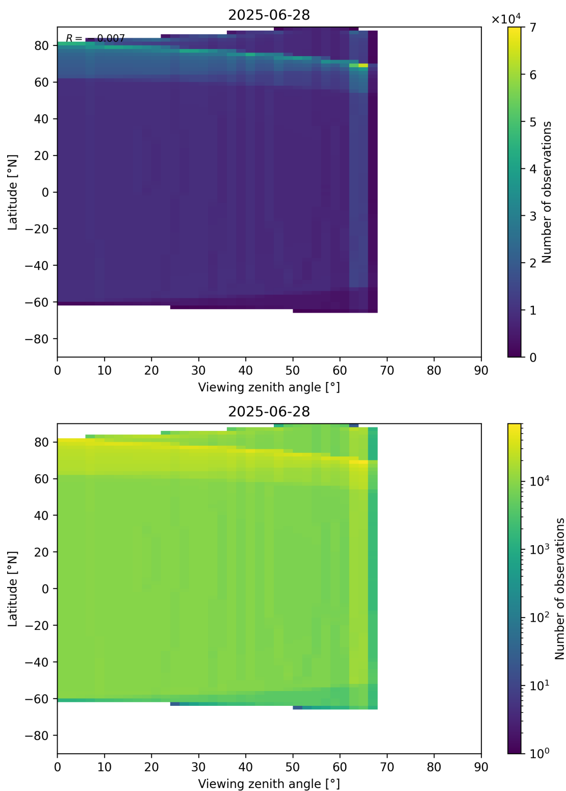
Figure 49: Scatter density plot of “Viewing zenith angle” against “Latitude” for 2025-06-27 to 2025-06-29.
