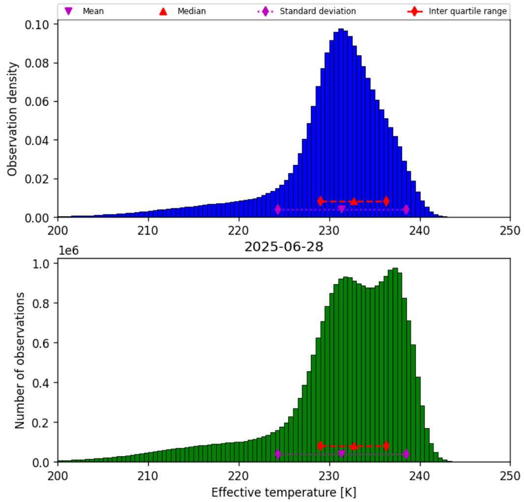
Figure 24: Histogram of “Effective temperature” for 2025-06-27 to 2025-06-29
