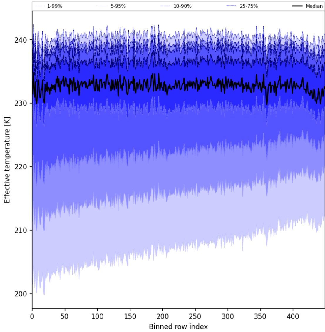
Figure 31: Along track statistics of “Effective temperature” for 2025-06-27 to 2025-06-29
