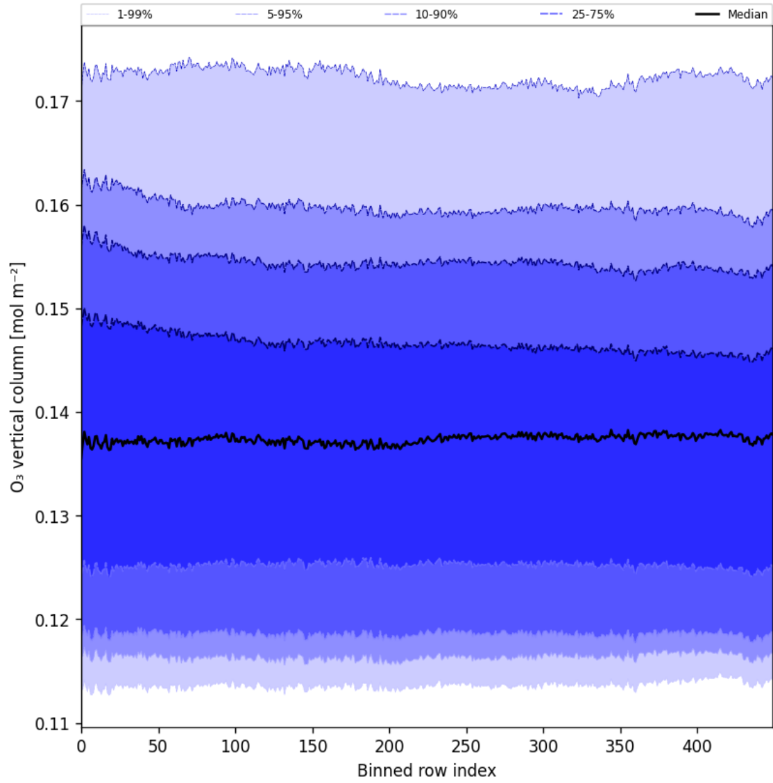
Figure 28: Along track statistics of “O 3 vertical column” for 2025-06-27 to 2025-06-29
