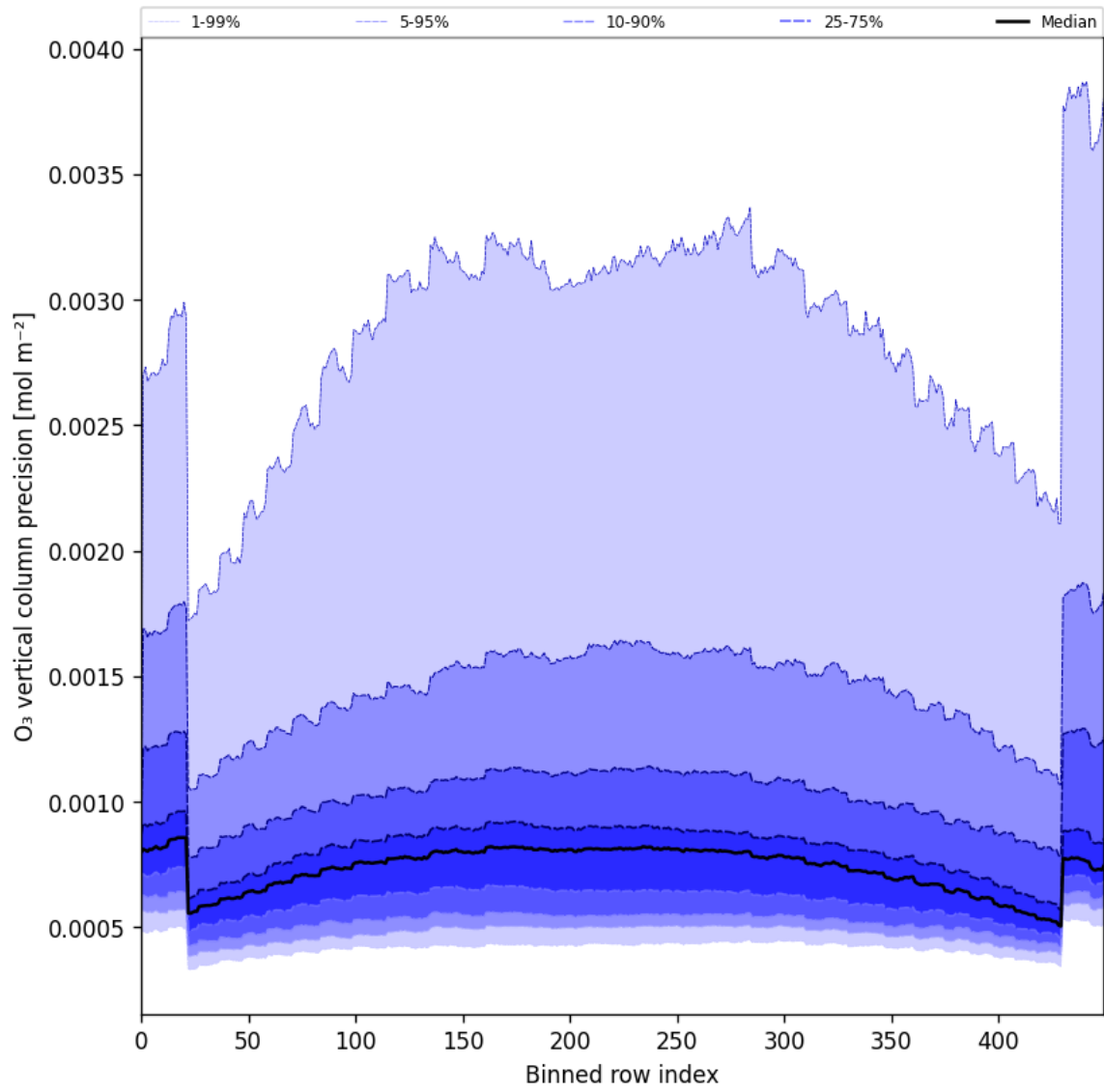
Figure 29: Along track statistics of “O 3 vertical column precision” for 2025-06-27 to 2025-06-29
