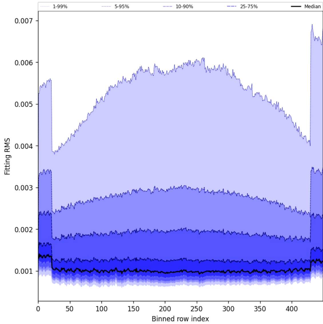
Figure 30: Along track statistics of “Fitting RMS” for 2025-06-27 to 2025-06-29
