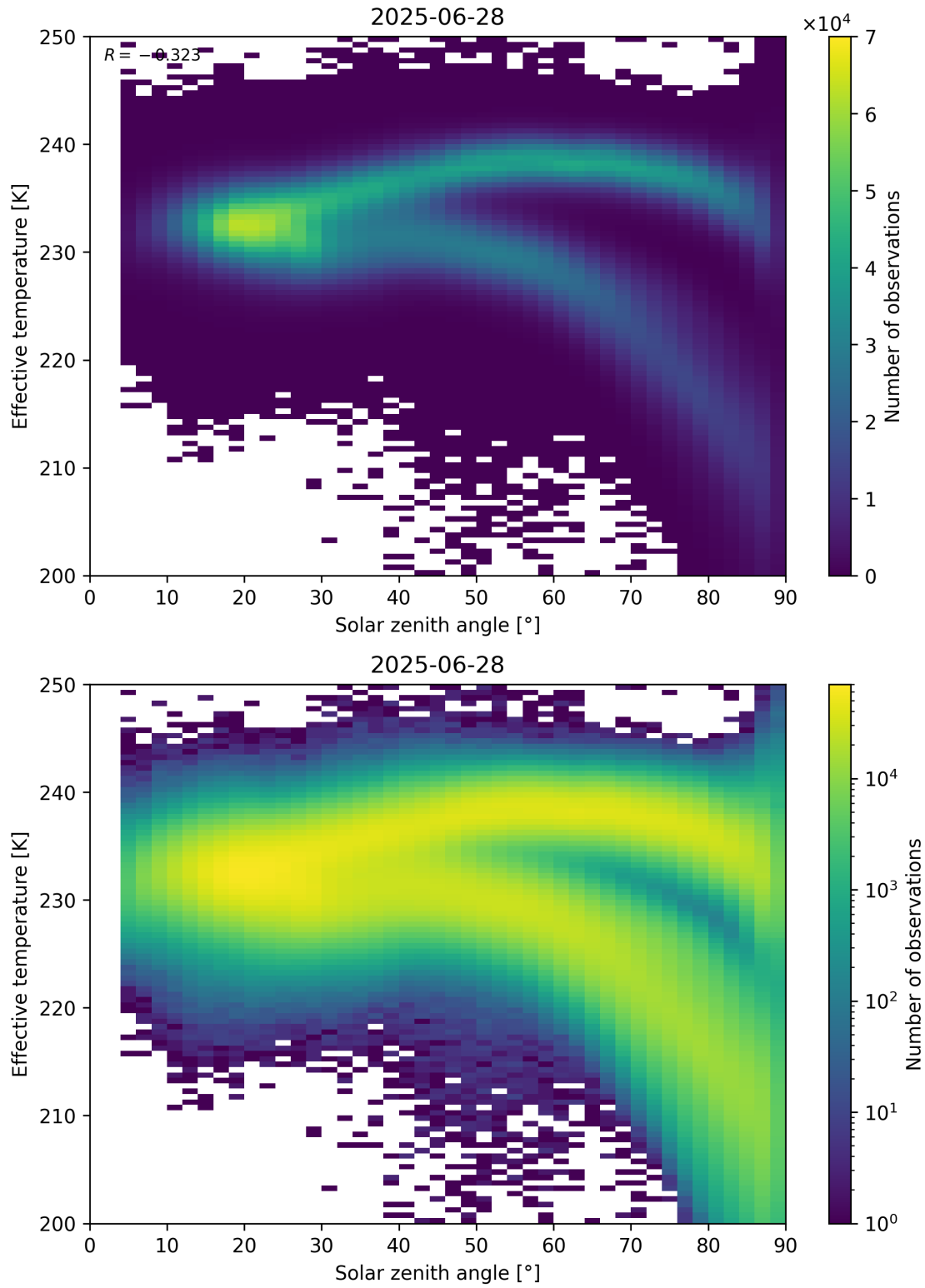
Figure 45: Scatter density plot of “Solar zenith angle” against “Effective temperature” for 2025-06-27 to 2025-06-29.
