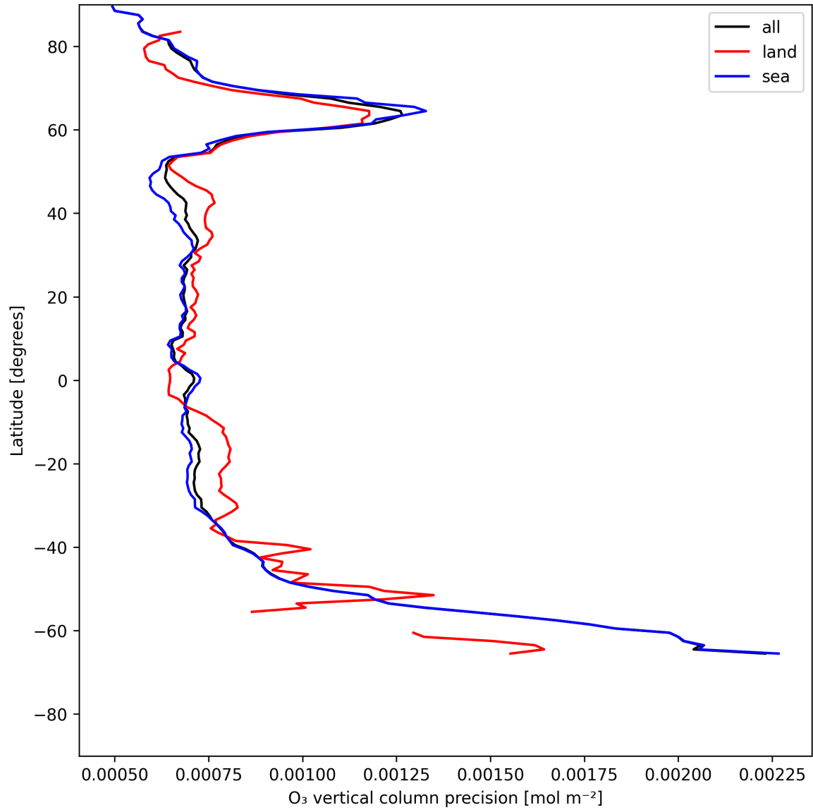
Figure 15: Zonal average of “O 3 vertical column precision” for 2025-06-27 to 2025-06-29.
