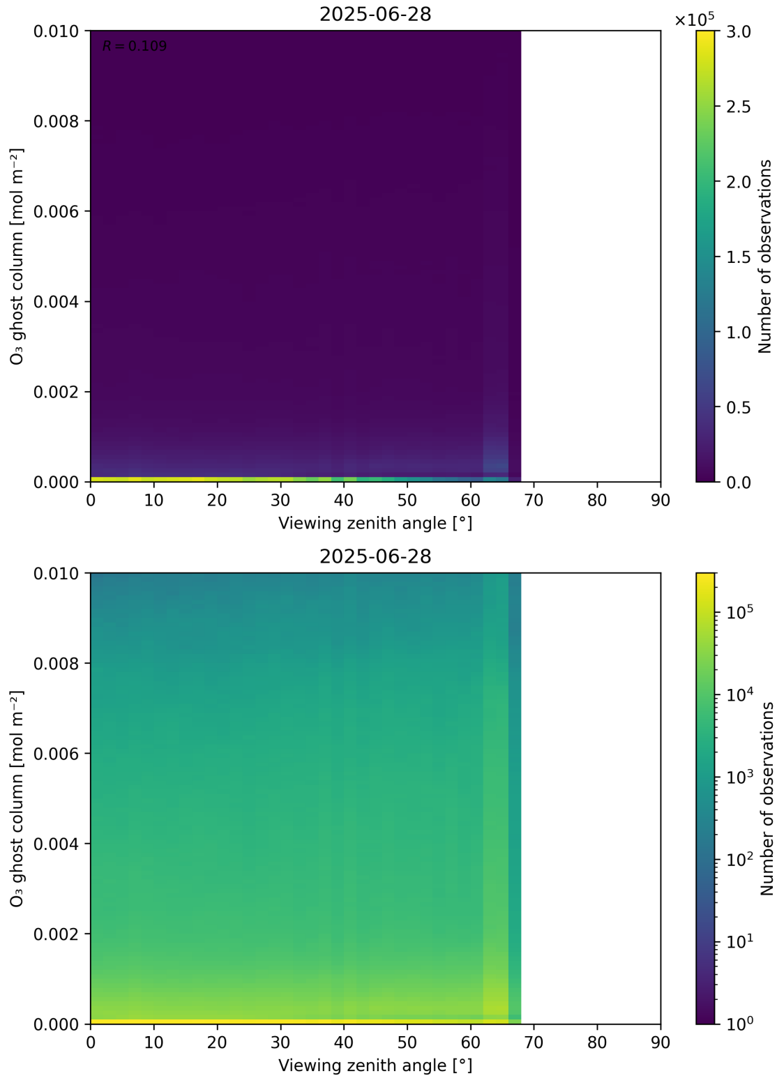
Figure 51: Scatter density plot of “Viewing zenith angle” against “O 3 ghost column” for 2025-06-27 to 2025-06-29.
