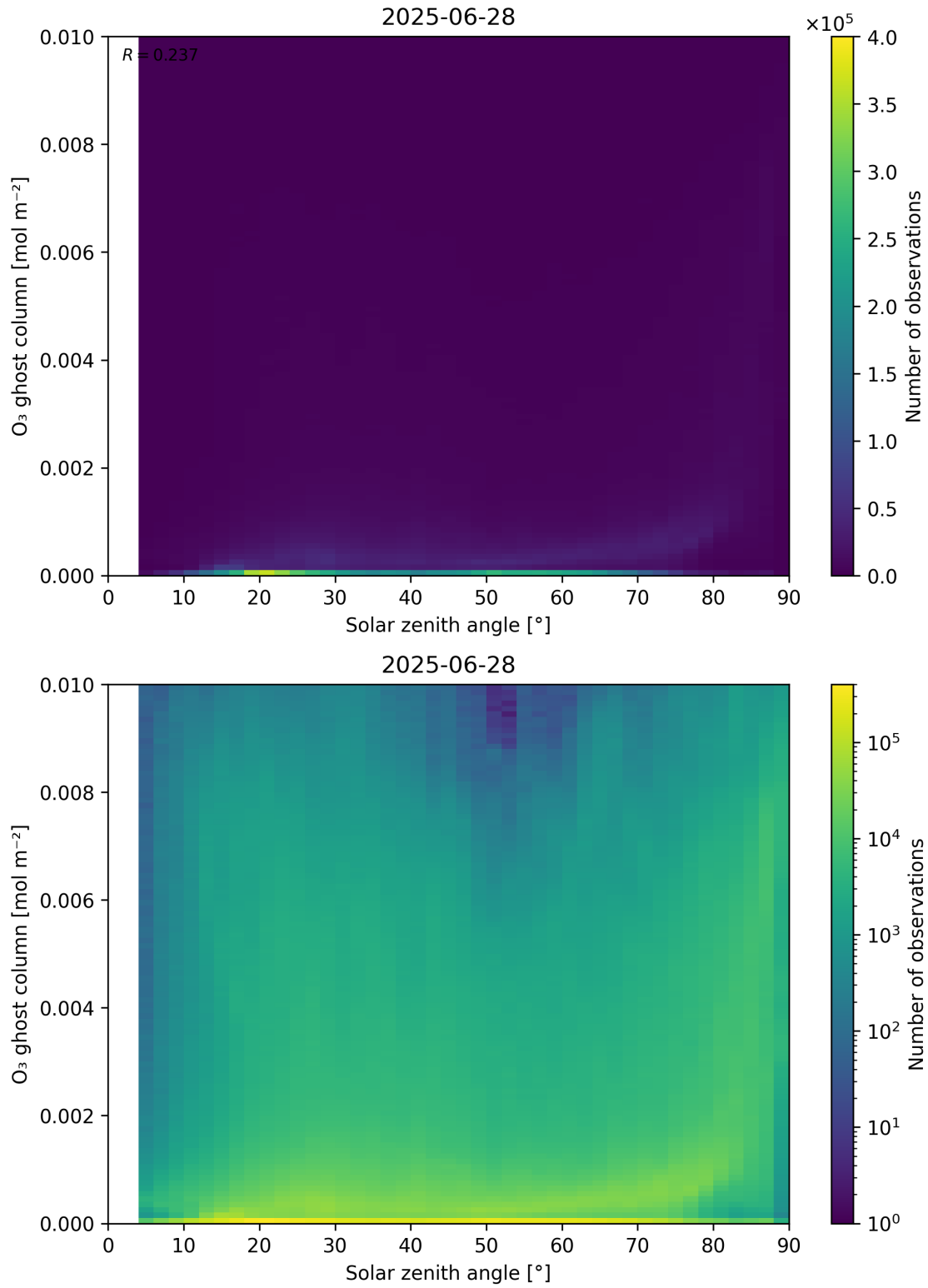
Figure 46: Scatter density plot of “Solar zenith angle” against “O 3 ghost column” for 2025-06-27 to 2025-06-29.
