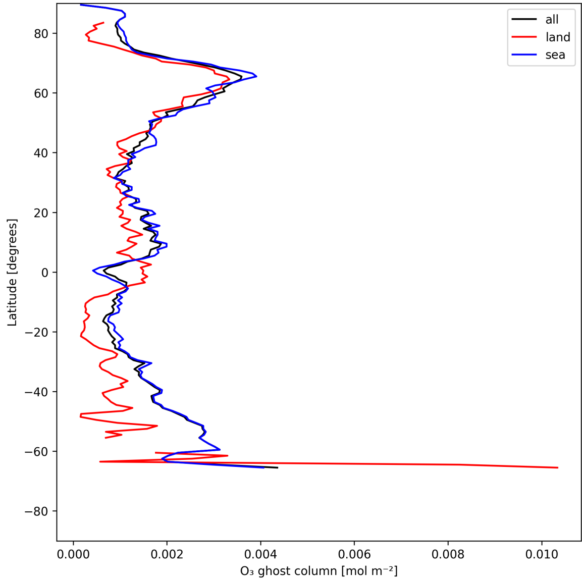
Figure 18: Zonal average of “O 3 ghost column” for 2025-06-27 to 2025-06-29.
