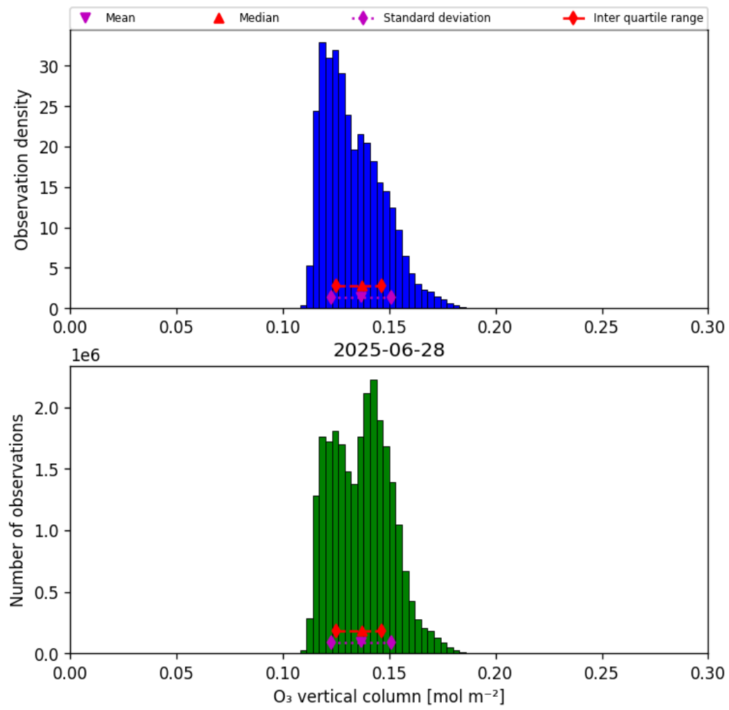
Figure 21: Histogram of “O 3 vertical column” for 2025-06-27 to 2025-06-29
