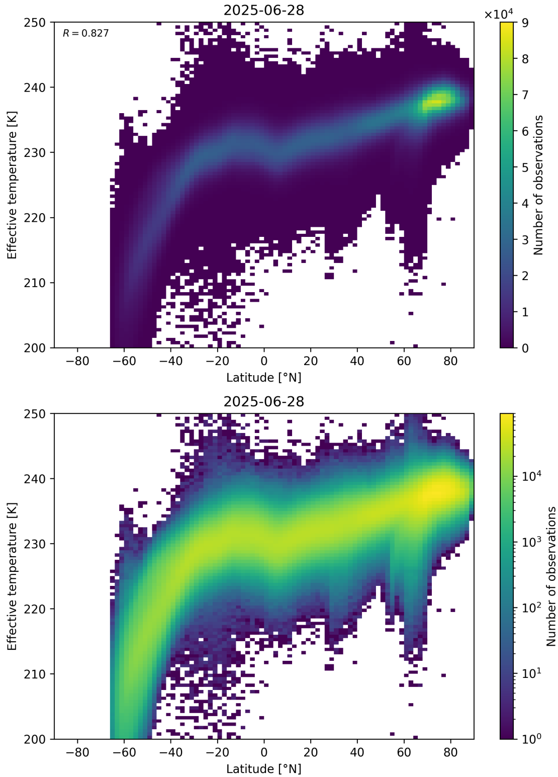
Figure 34: Scatter density plot of “Latitude” against “Effective temperature” for 2025-06-27 to 2025-06-29.
