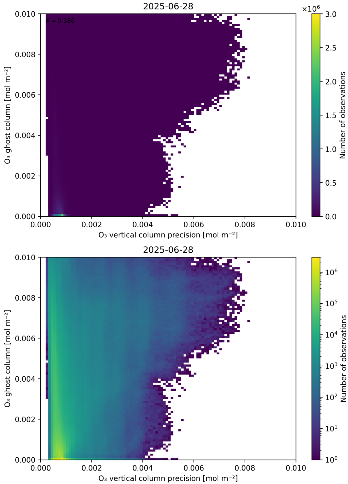
Figure 43: Scatter density plot of “ \text{O}_3 vertical column precision” against “ \text{O}_3 ghost column” for 2025-06-27 to 2025-06-29.
