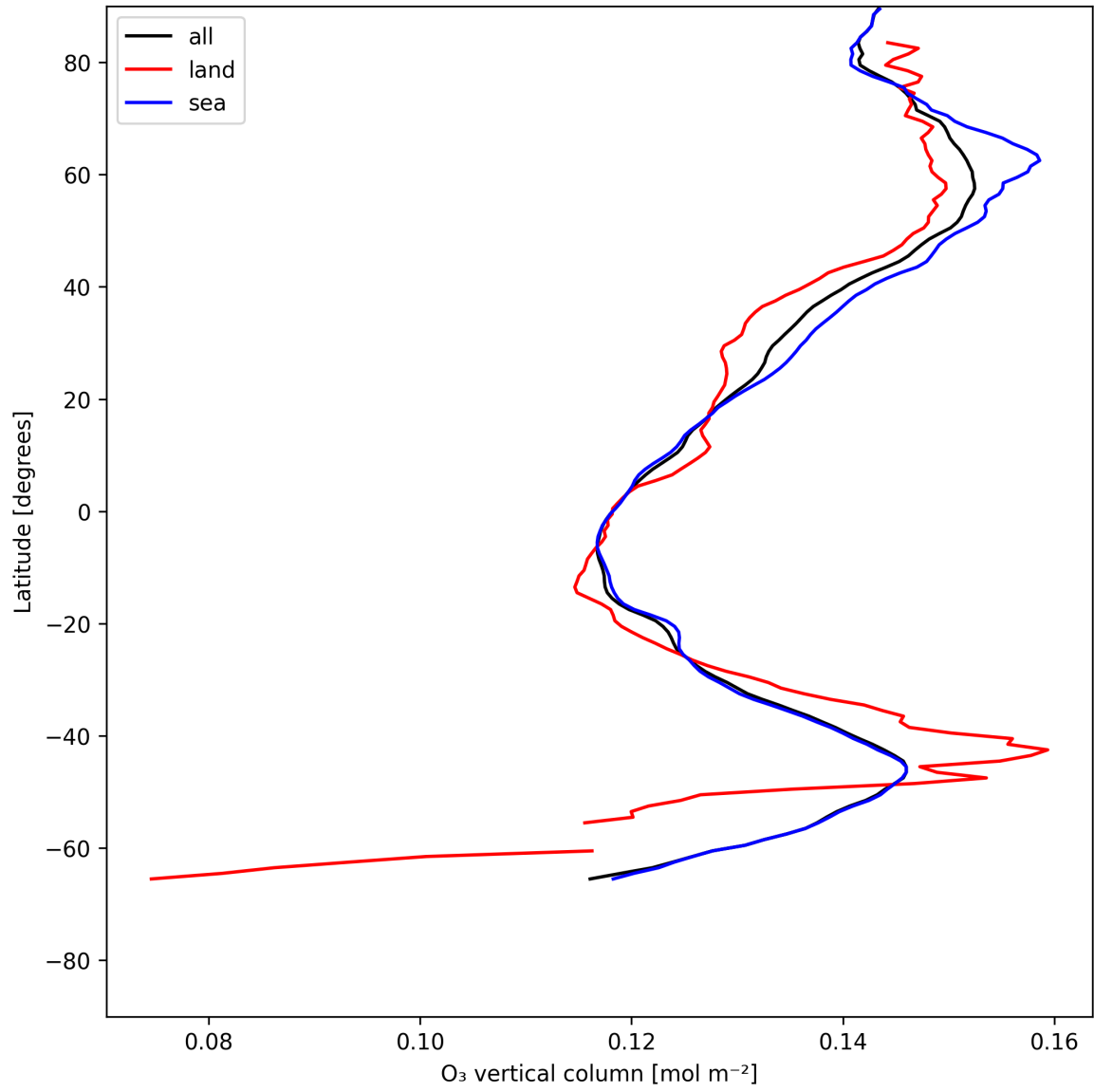
Figure 14: Zonal average of “O 3 vertical column” for 2025-06-27 to 2025-06-29.
