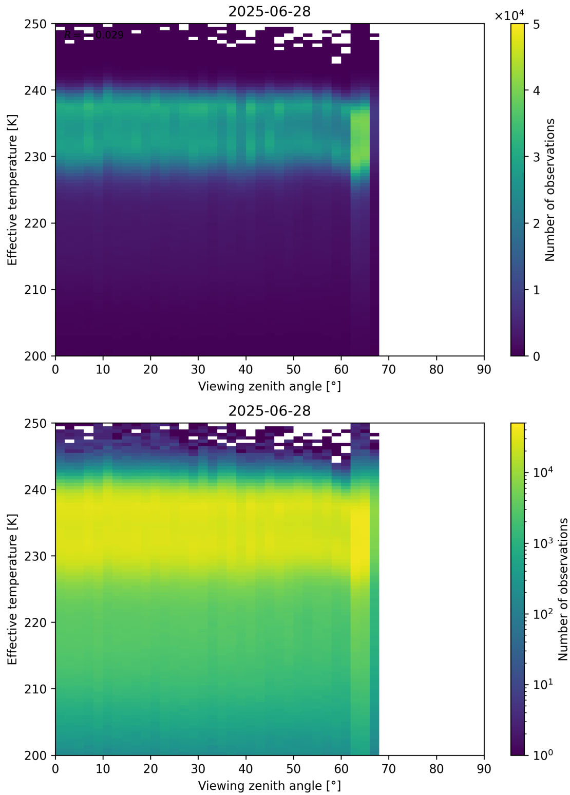
Figure 50: Scatter density plot of “Viewing zenith angle” against “Effective temperature” for 2025-06-27 to 2025-06-29.
