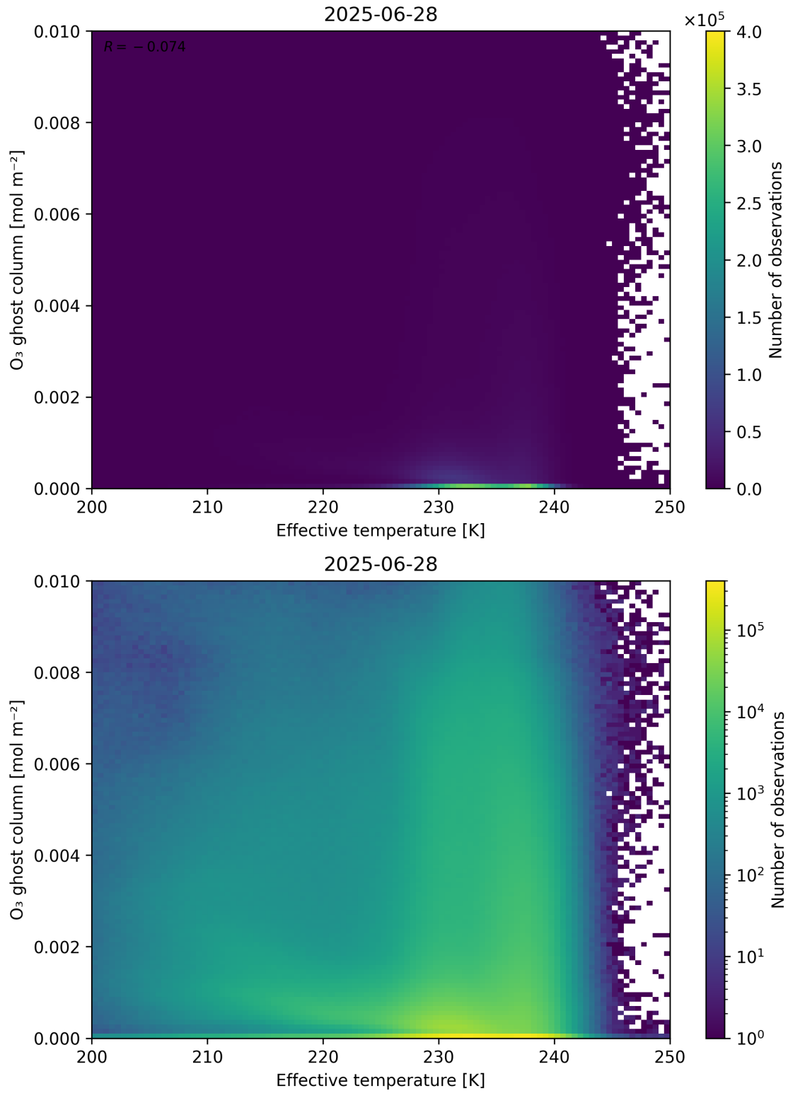
Figure 38: Scatter density plot of “Effective temperature” against “O 3 ghost column” for 2025-06-27 to 2025-06-29.
