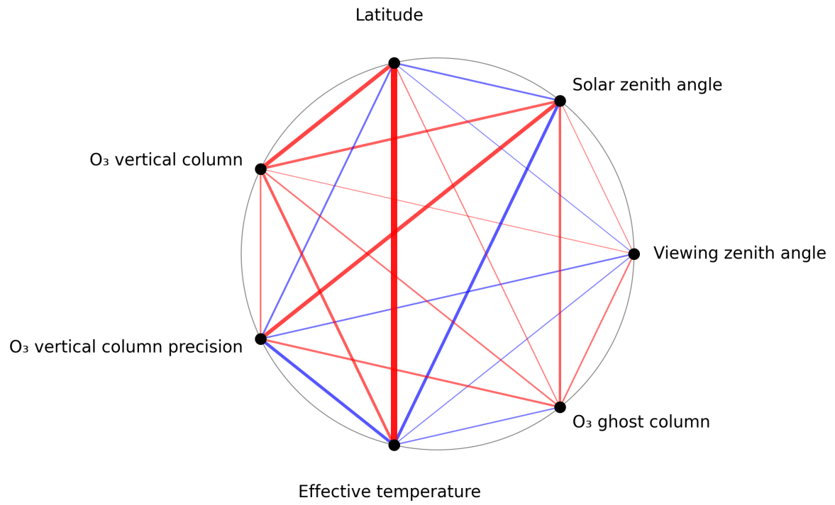
Figure 1: Map of correlation graph for 2025-06-27 to 2025-06-29.
