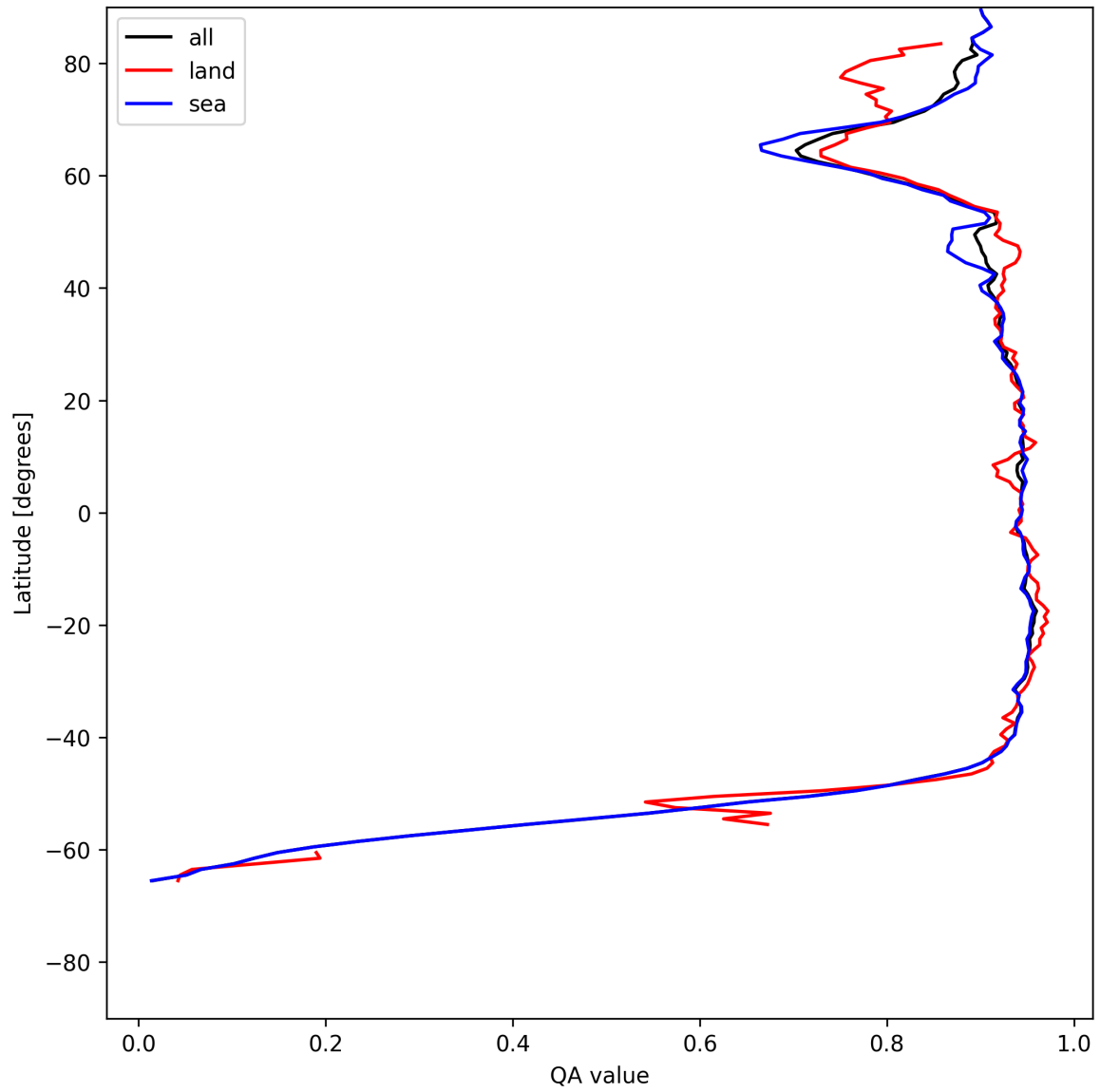
Figure 13: Zonal average of “QA value” for 2025-06-27 to 2025-06-29.
