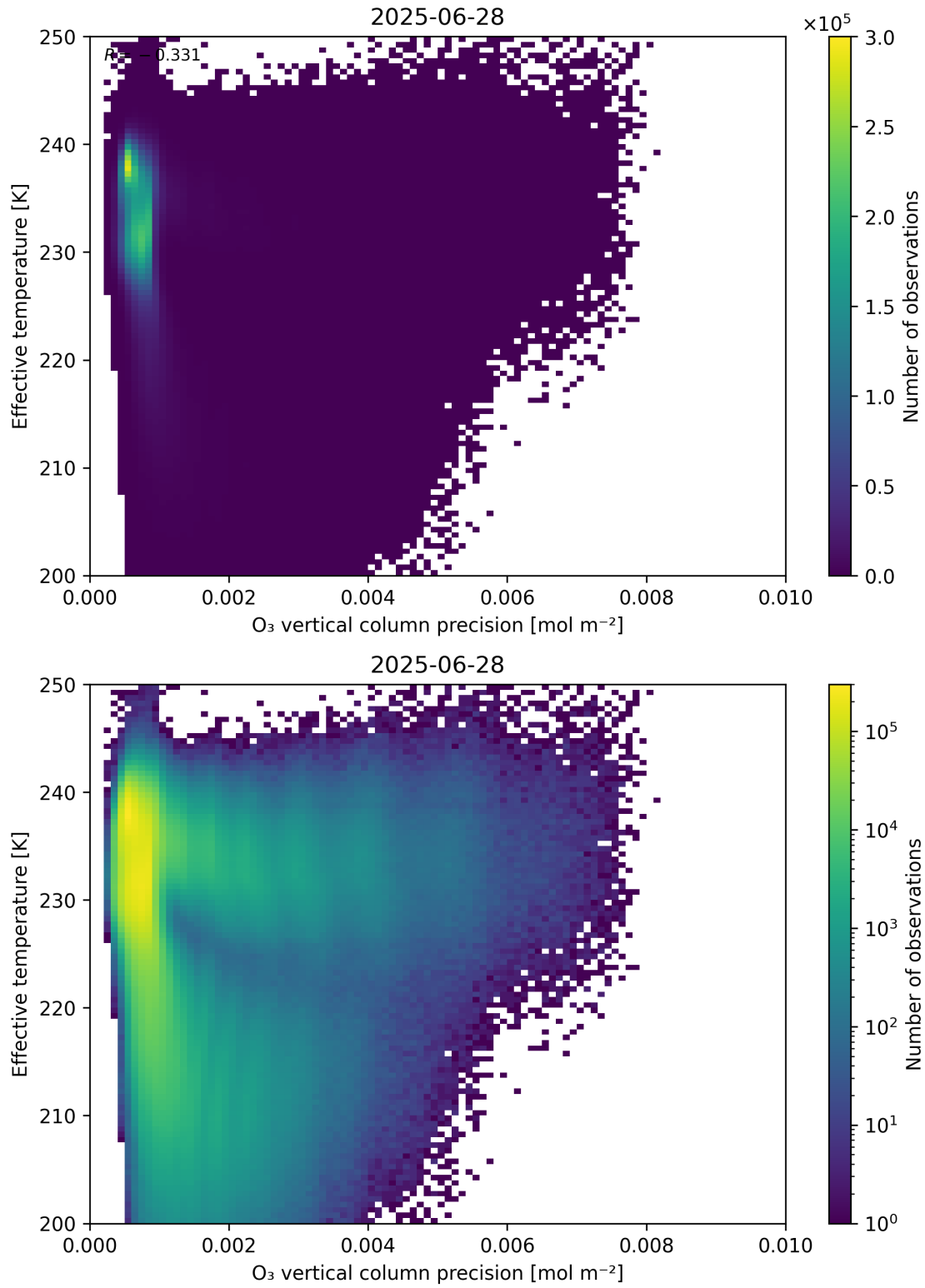
Figure 42: Scatter density plot of “O 3 vertical column precision” against “Effective temperature” for 2025-06-27 to 2025-06-29.
