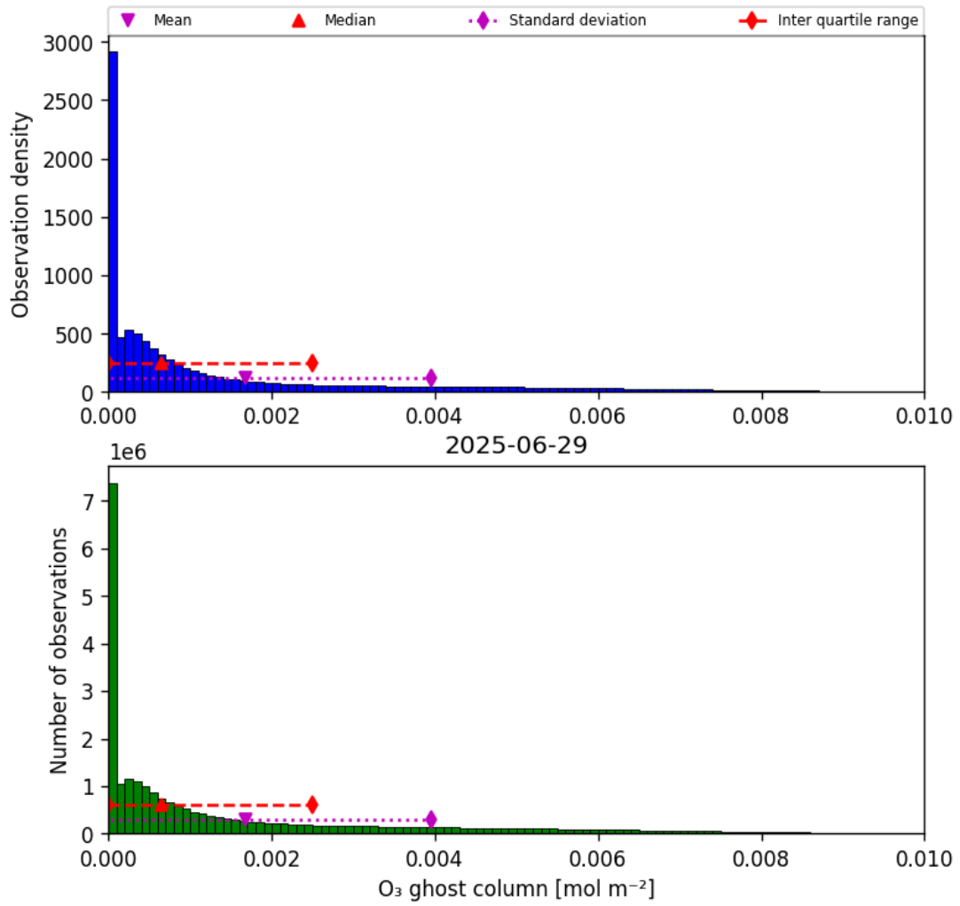
Figure 25: Histogram of “O 3 ghost column” for 2025-06-28 to 2025-06-30
