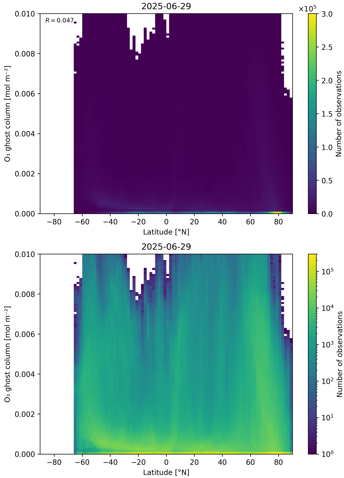
Figure 35: Scatter density plot of “Latitude” against “O 3 ghost column” for 2025-06-28 to 2025-06-30.
