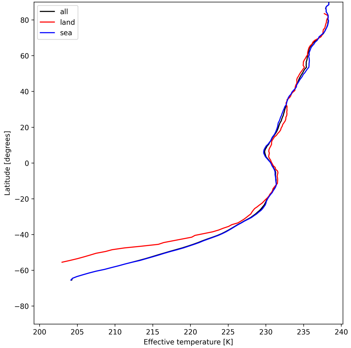
Figure 17: Zonal average of “Effective temperature” for 2025-06-28 to 2025-06-30.
