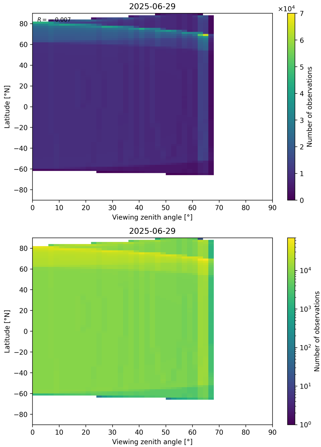
Figure 49: Scatter density plot of “Viewing zenith angle” against “Latitude” for 2025-06-28 to 2025-06-30.
