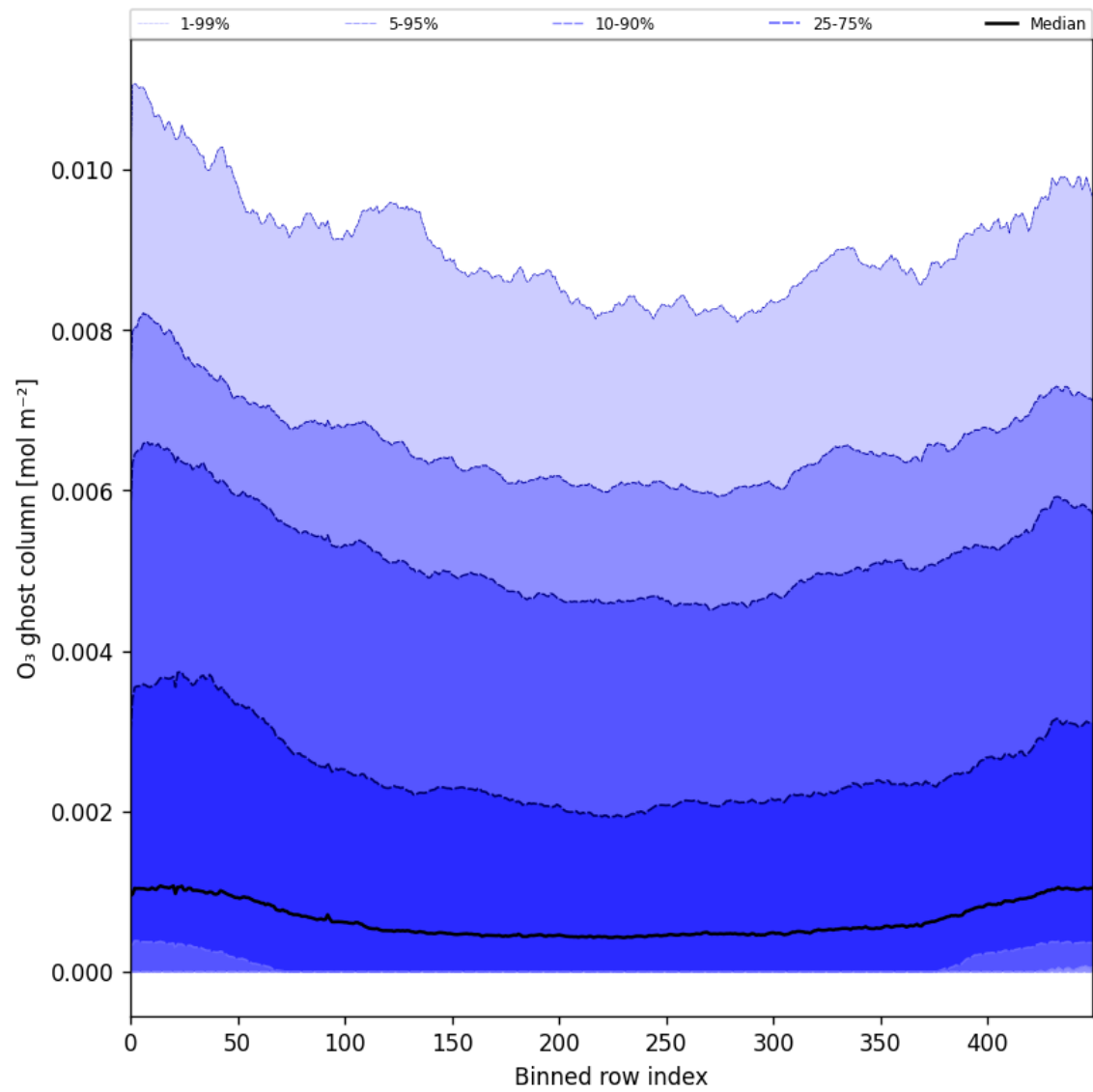
Figure 32: Along track statistics of “O 3 ghost column” for 2025-06-28 to 2025-06-30
