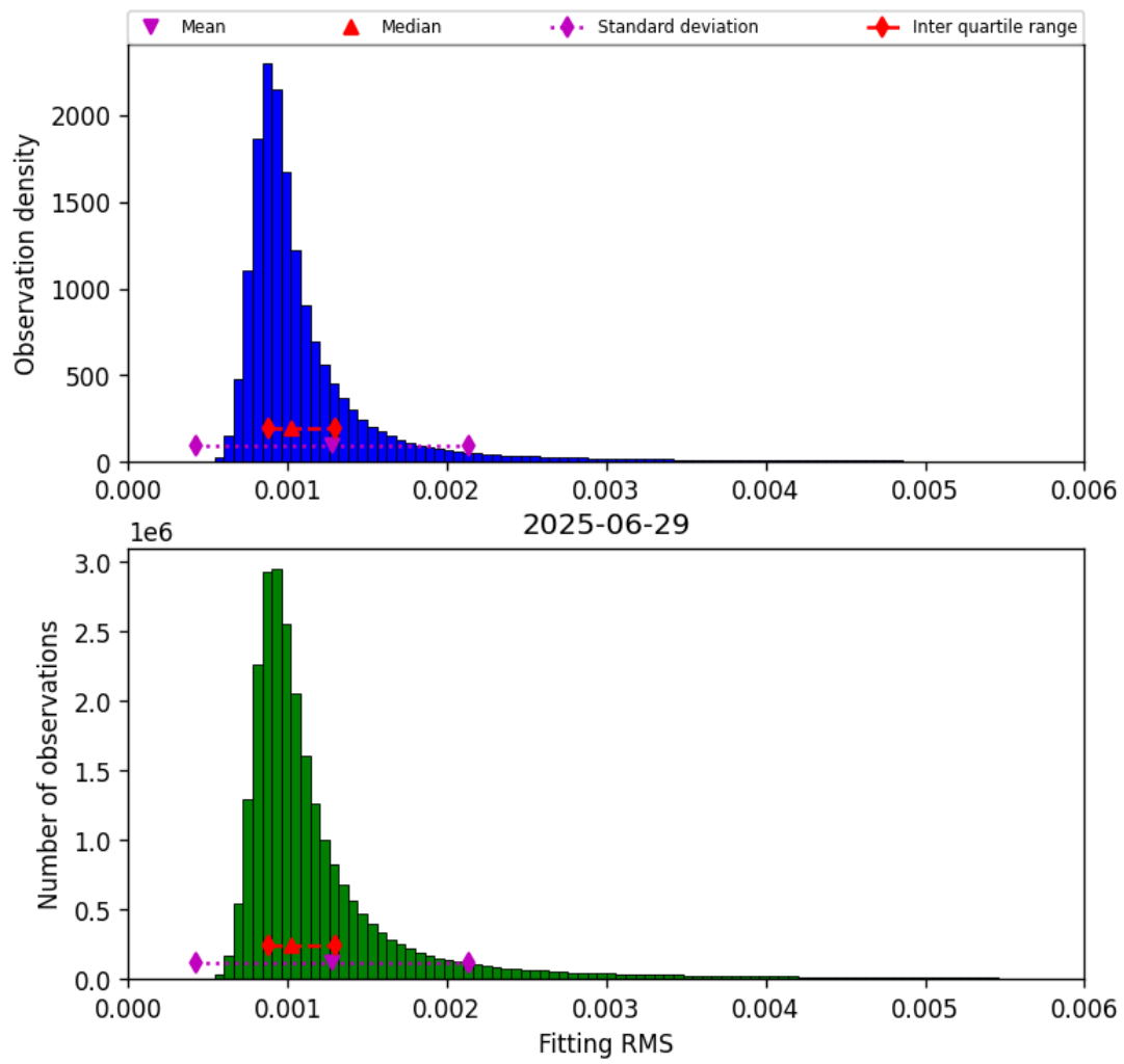
Figure 23: Histogram of “Fitting RMS” for 2025-06-28 to 2025-06-30
