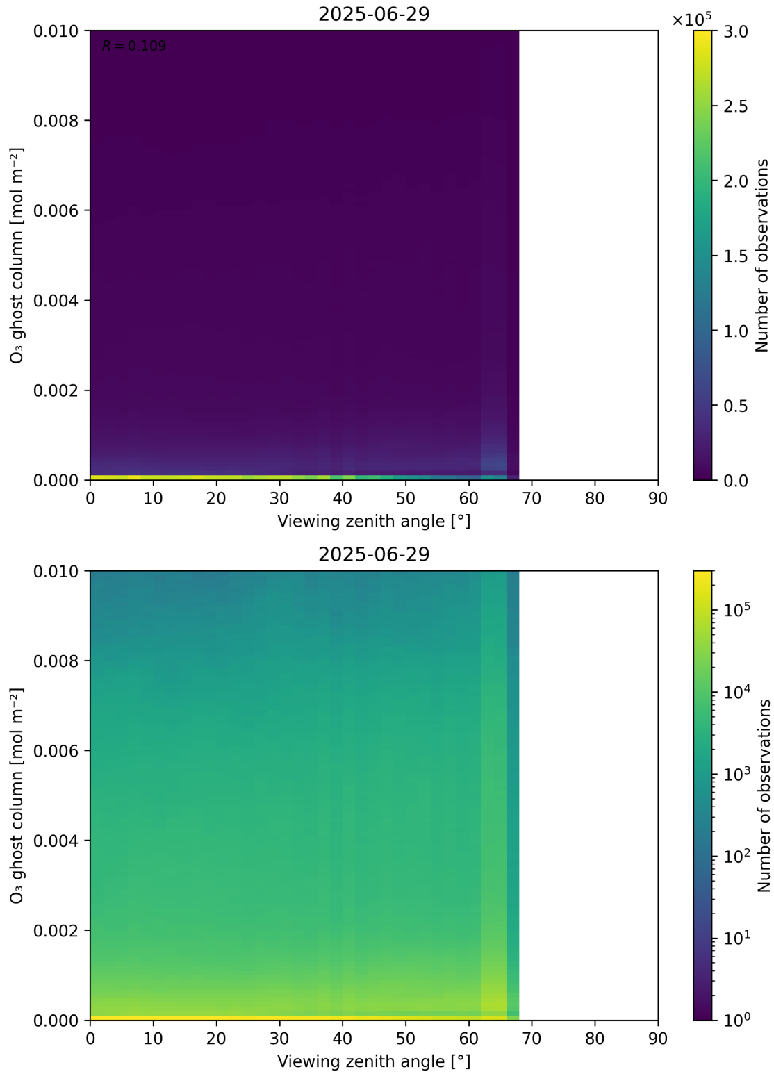
Figure 51: Scatter density plot of “Viewing zenith angle” against “O 3 ghost column” for 2025-06-28 to 2025-06-30.
