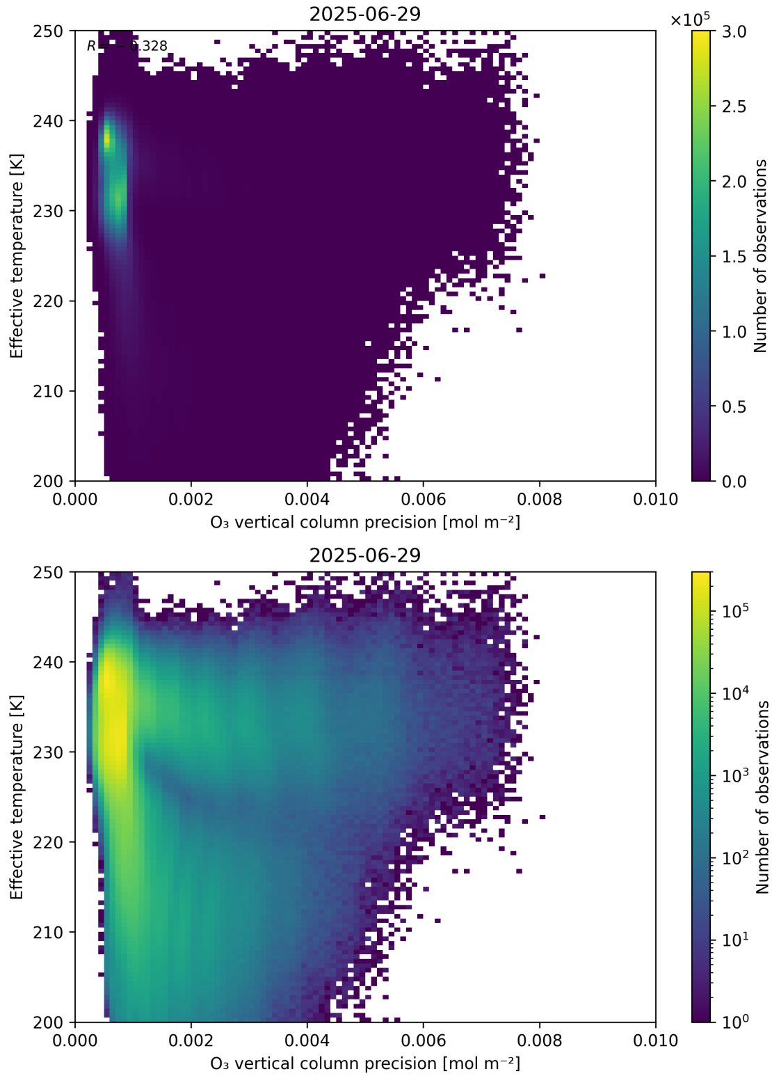
Figure 42: Scatter density plot of “ O_3 vertical column precision” against “Effective temperature” for 2025-06-28 to 2025-06-30.
