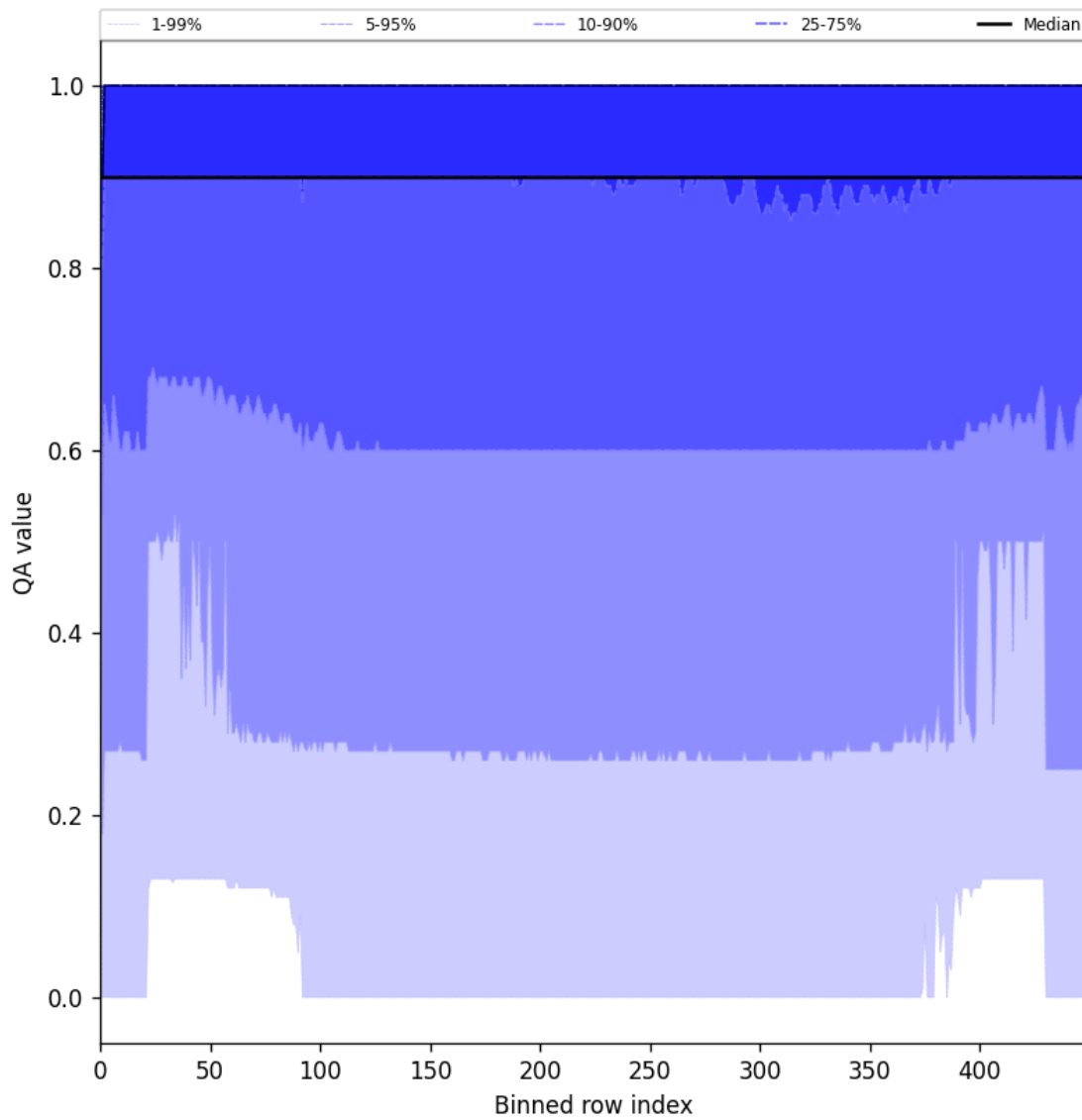
Figure 27: Along track statistics of “QA value” for 2025-06-28 to 2025-06-30
