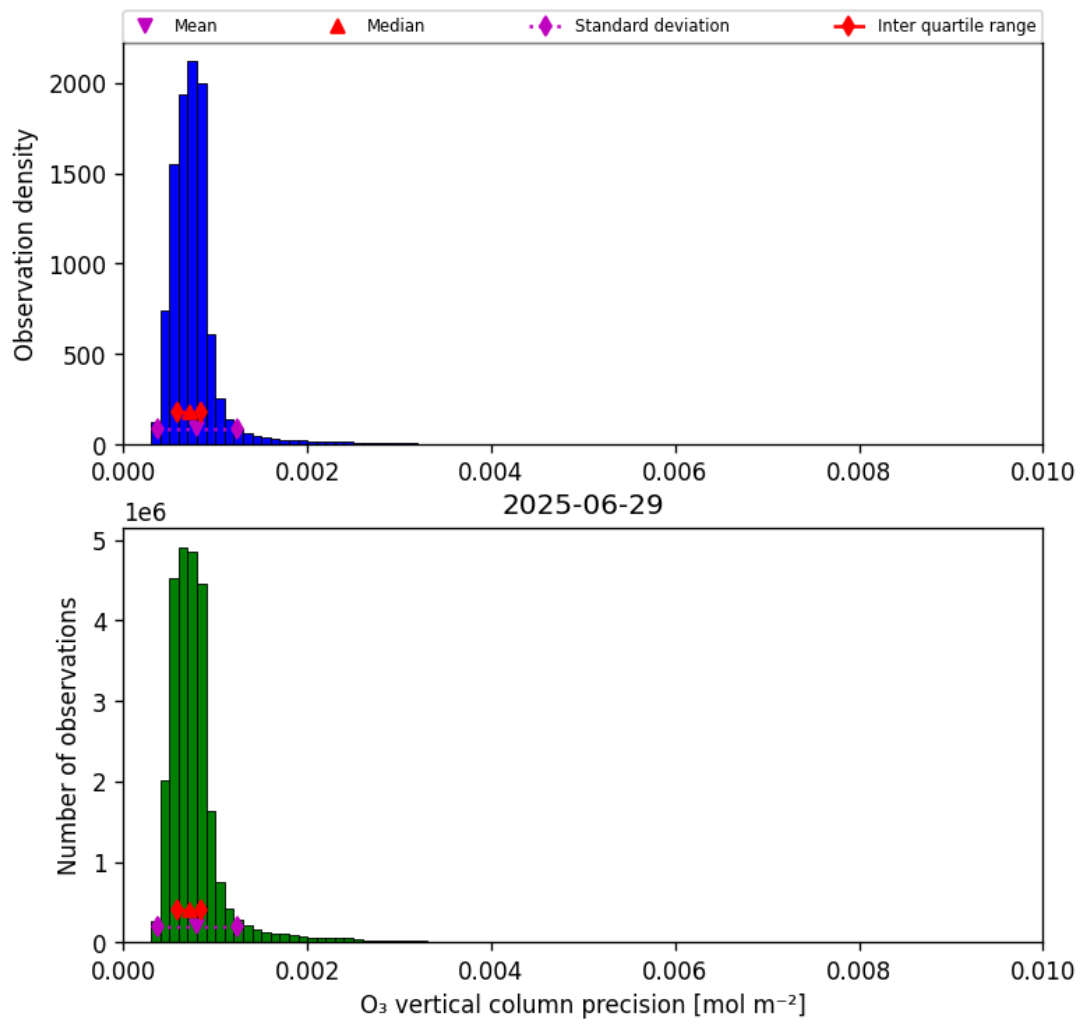
Figure 22: Histogram of “O 3 vertical column precision” for 2025-06-28 to 2025-06-30
