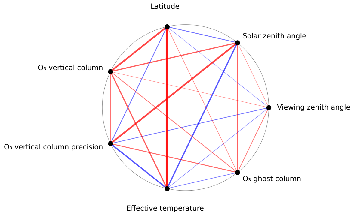
Figure 1: Map of correlation graph for 2025-06-28 to 2025-06-30.
