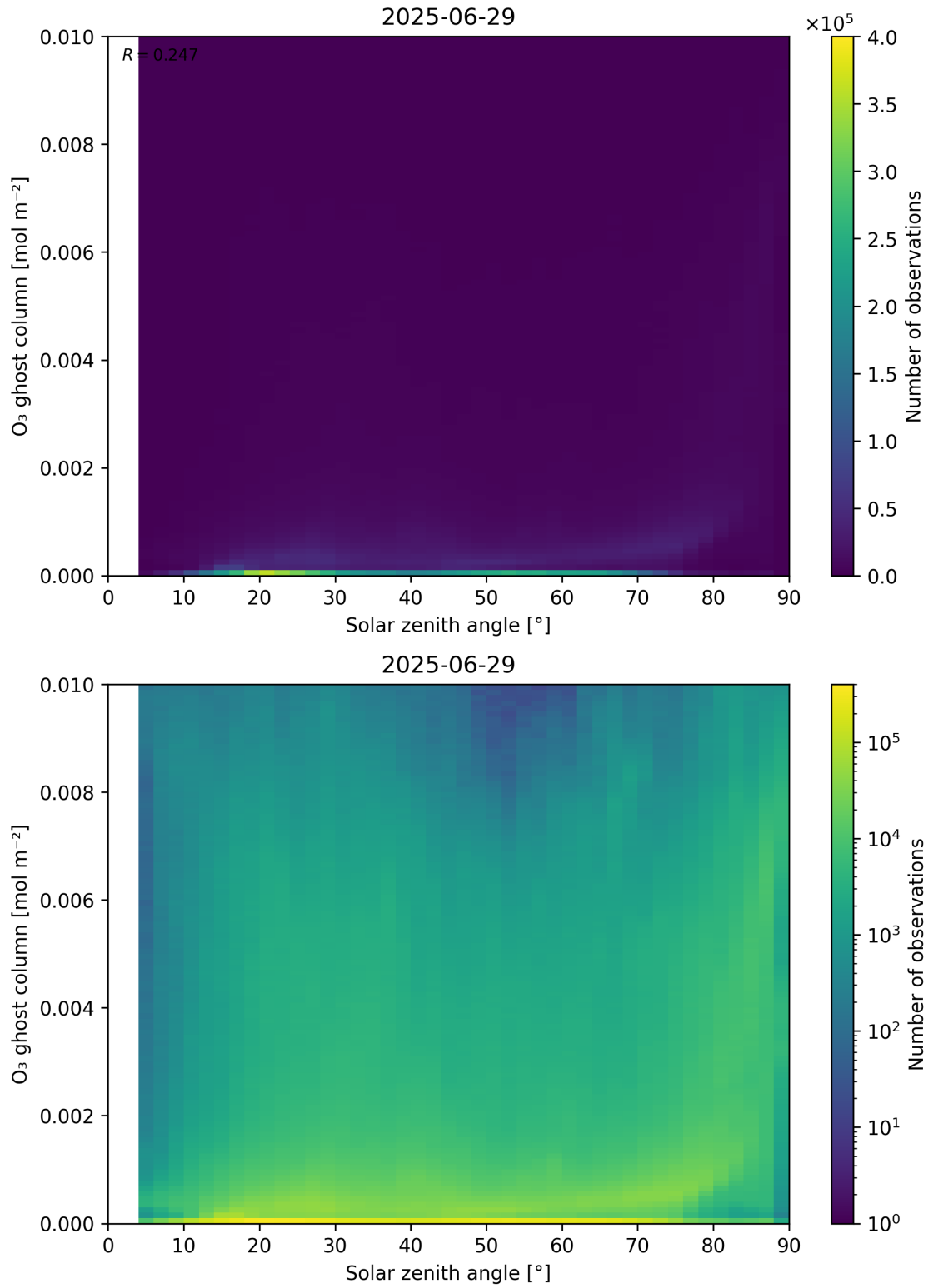
Figure 46: Scatter density plot of “Solar zenith angle” against “O 3 ghost column” for 2025-06-28 to 2025-06-30.
