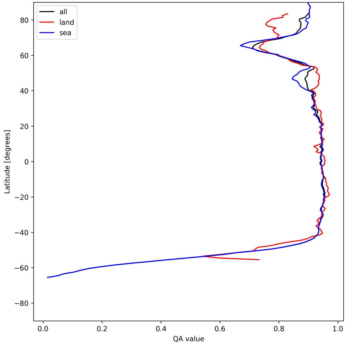
Figure 13: Zonal average of “QA value” for 2025-06-28 to 2025-06-30.
