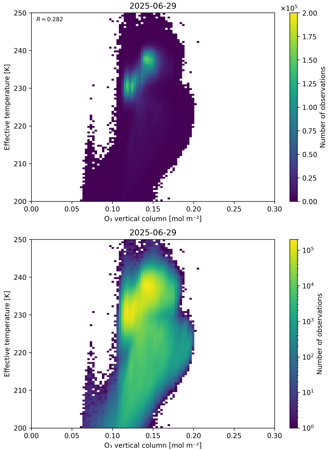
Figure 39: Scatter density plot of “O 3 vertical column” against “Effective temperature” for 2025-06-28 to 2025-06-30.
