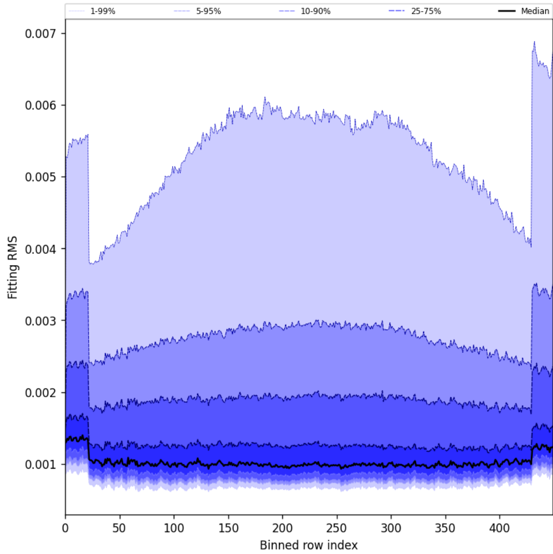
Figure 30: Along track statistics of “Fitting RMS” for 2025-06-28 to 2025-06-30
