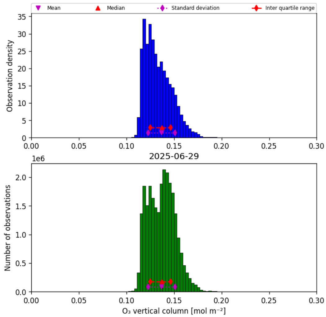
Figure 21: Histogram of “O 3 vertical column” for 2025-06-28 to 2025-06-30
