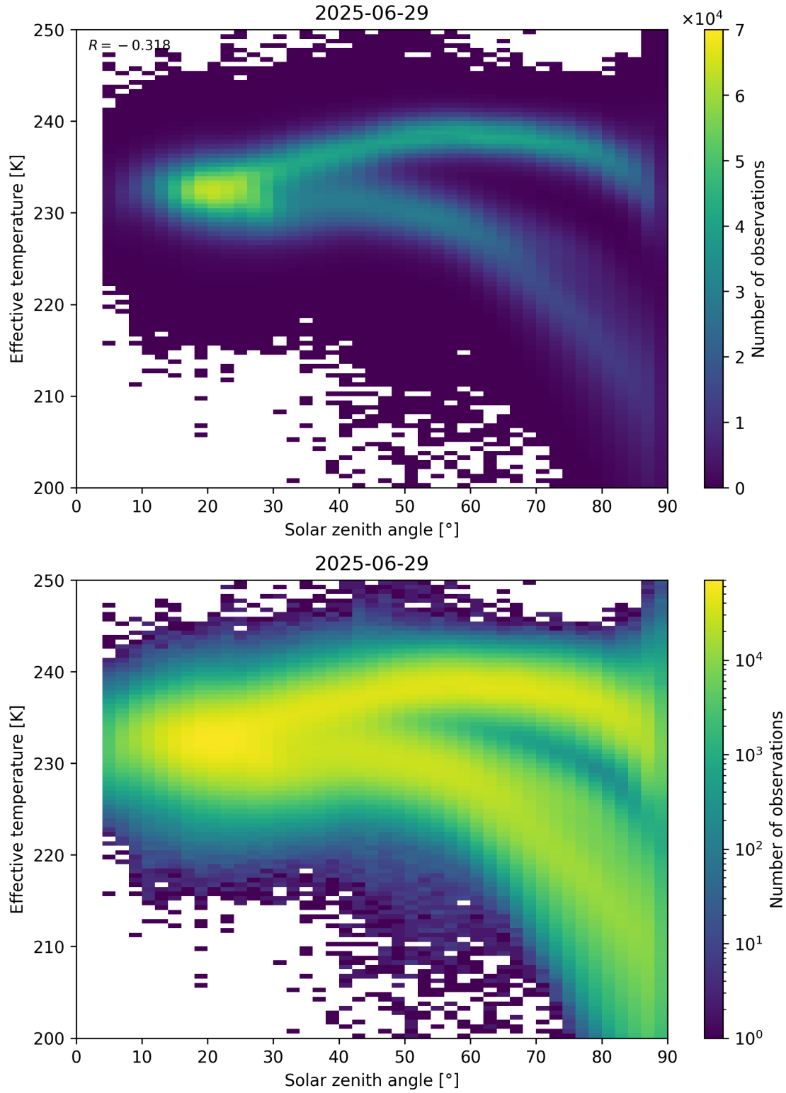
Figure 45: Scatter density plot of “Solar zenith angle” against “Effective temperature” for 2025-06-28 to 2025-06-30.
