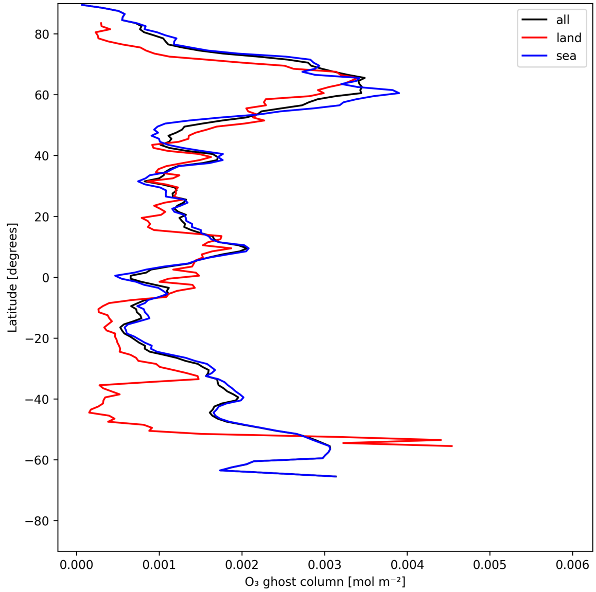
Figure 18: Zonal average of “O 3 ghost column” for 2025-06-28 to 2025-06-30.
