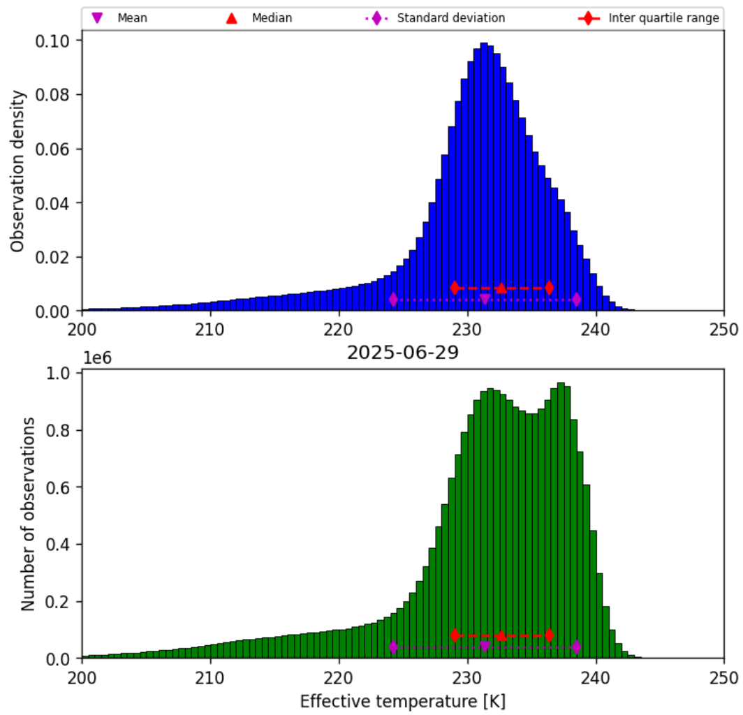
Figure 24: Histogram of “Effective temperature” for 2025-06-28 to 2025-06-30
