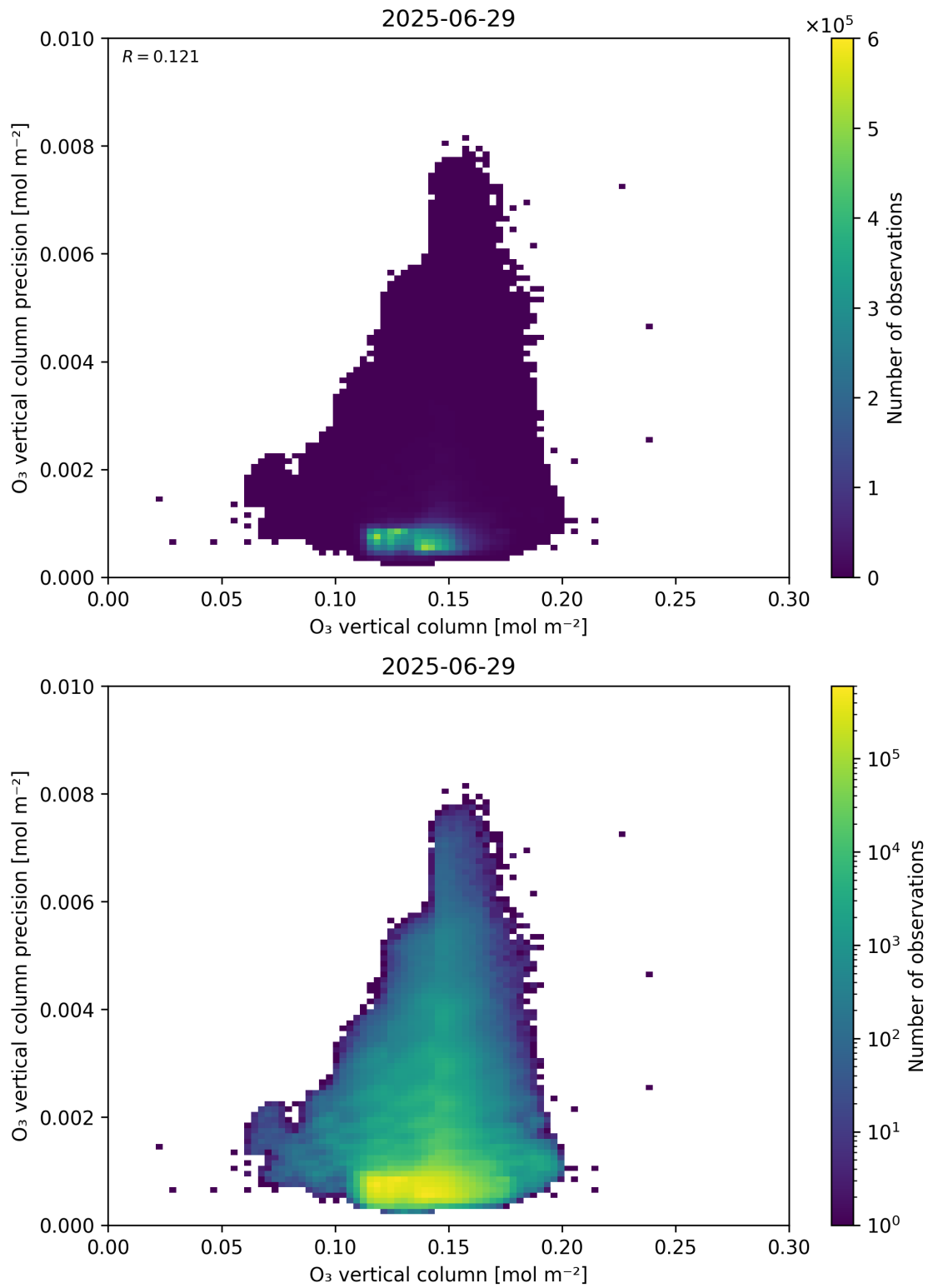
Figure 41: Scatter density plot of “O 3 vertical column” against “O 3 vertical column precision” for 2025-06-28 to 2025-06-30.
