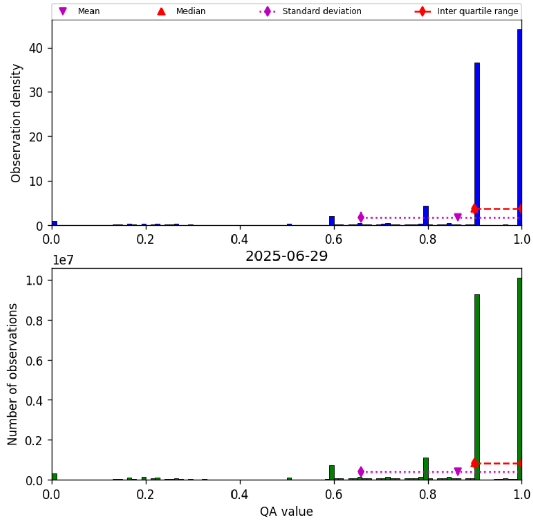
Figure 20: Histogram of “QA value” for 2025-06-28 to 2025-06-30
