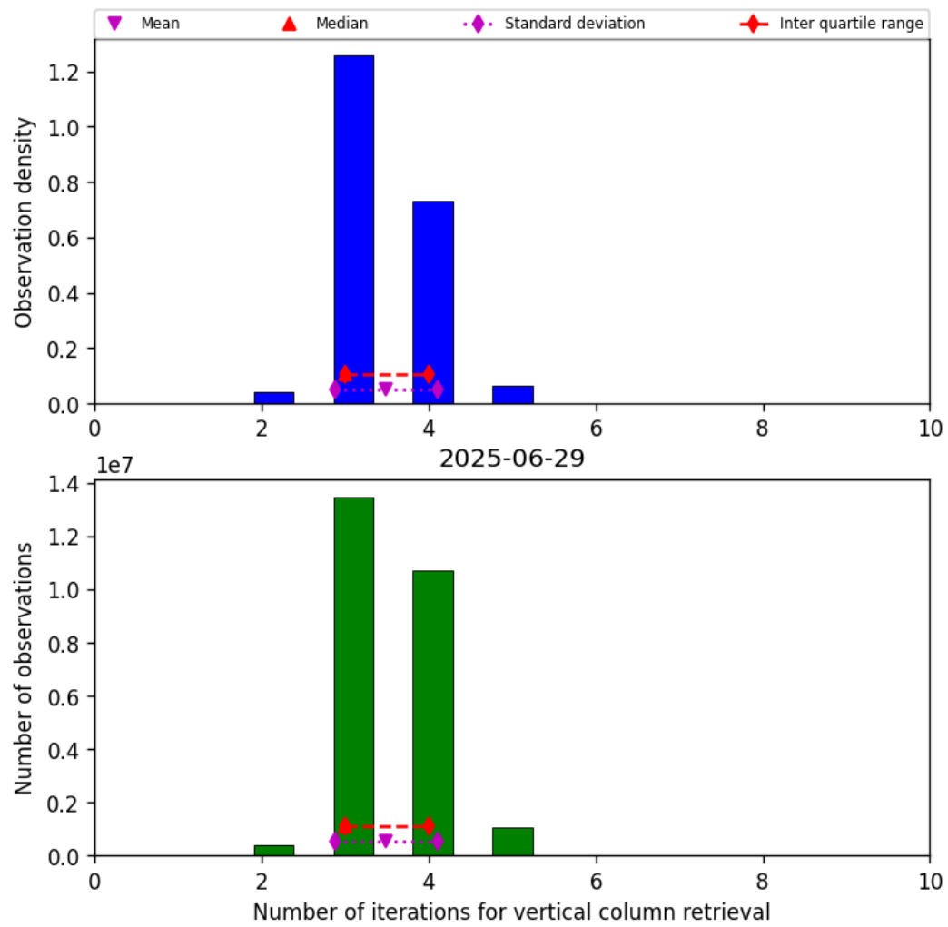
Figure 26: Histogram of “Number of iterations for vertical column retrieval” for 2025-06-28 to 2025-06-30
