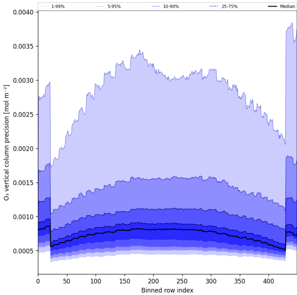
Figure 29: Along track statistics of “O 3 vertical column precision” for 2025-06-28 to 2025-06-30
