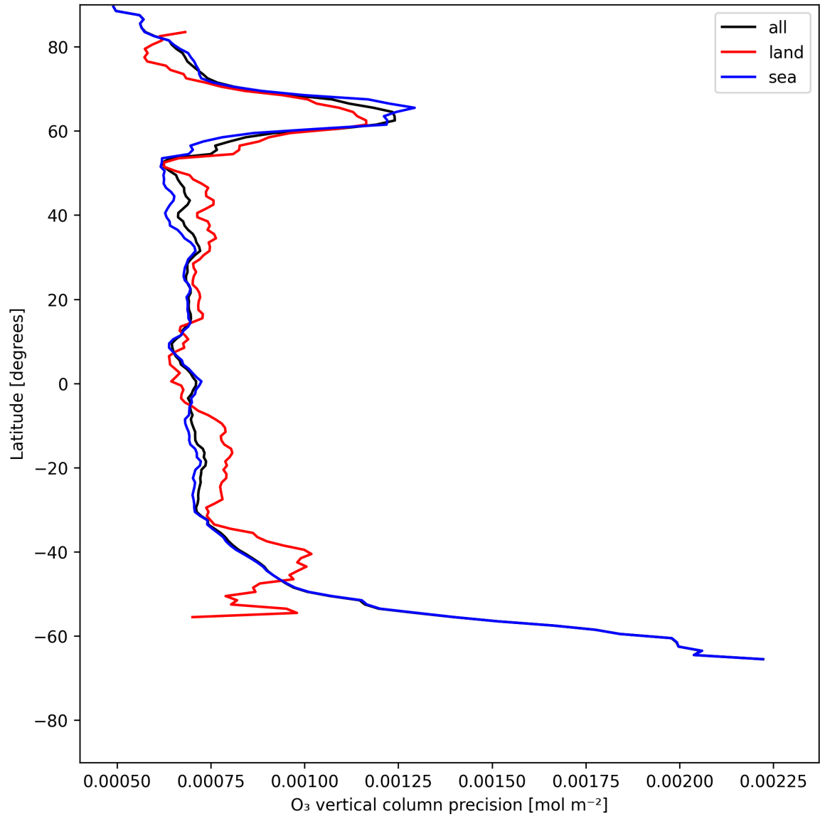
Figure 15: Zonal average of “O 3 vertical column precision” for 2025-06-28 to 2025-06-30.
