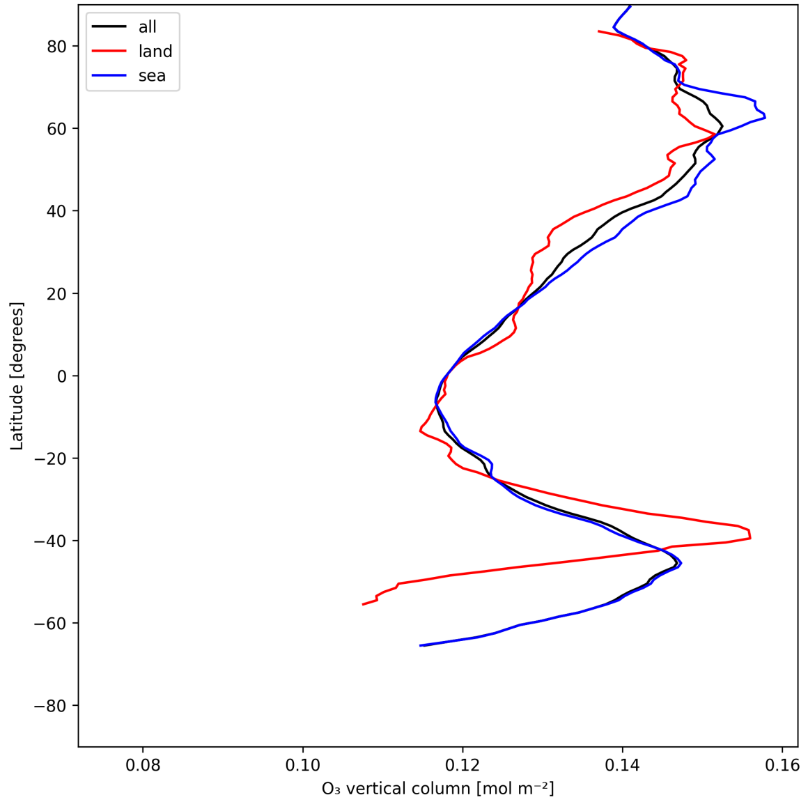
Figure 14: Zonal average of “O 3 vertical column” for 2025-06-28 to 2025-06-30.
