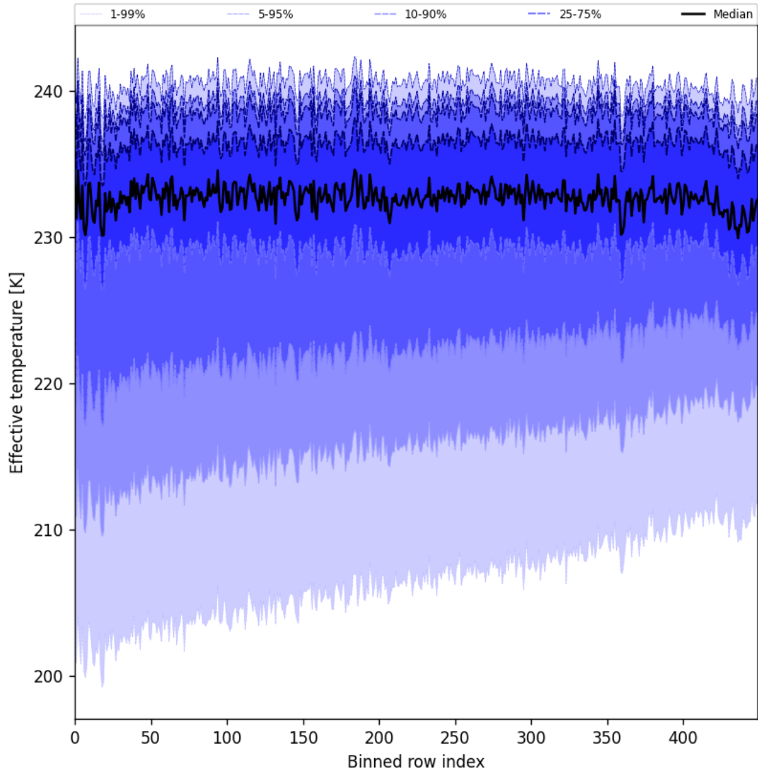
Figure 31: Along track statistics of “Effective temperature” for 2025-06-28 to 2025-06-30
