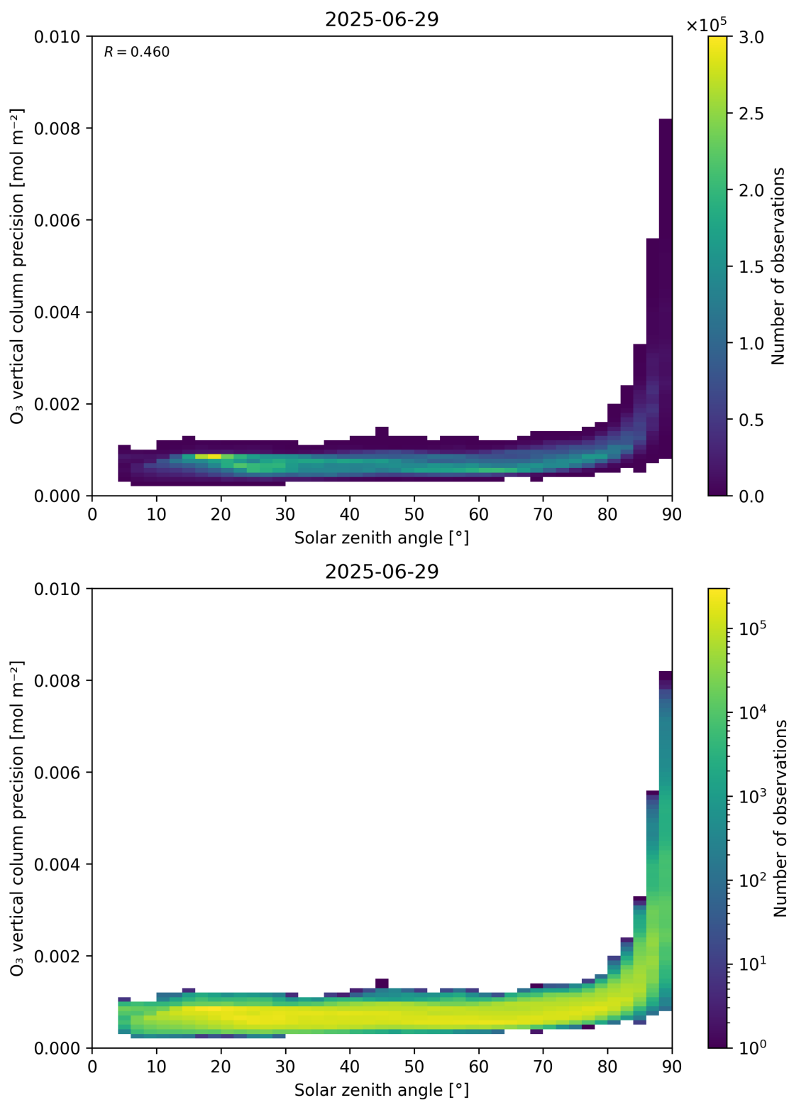
Figure 48: Scatter density plot of “Solar zenith angle” against “O 3 vertical column precision” for 2025-06-28 to 2025-06-30.
