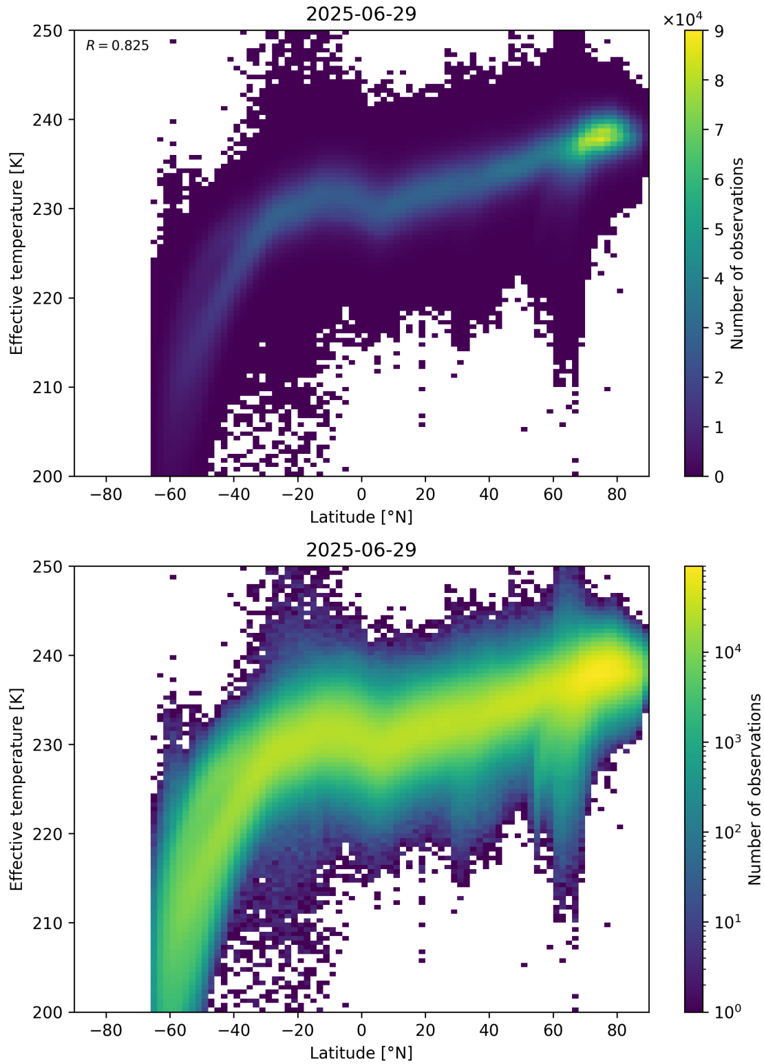
Figure 34: Scatter density plot of “Latitude” against “Effective temperature” for 2025-06-28 to 2025-06-30.
