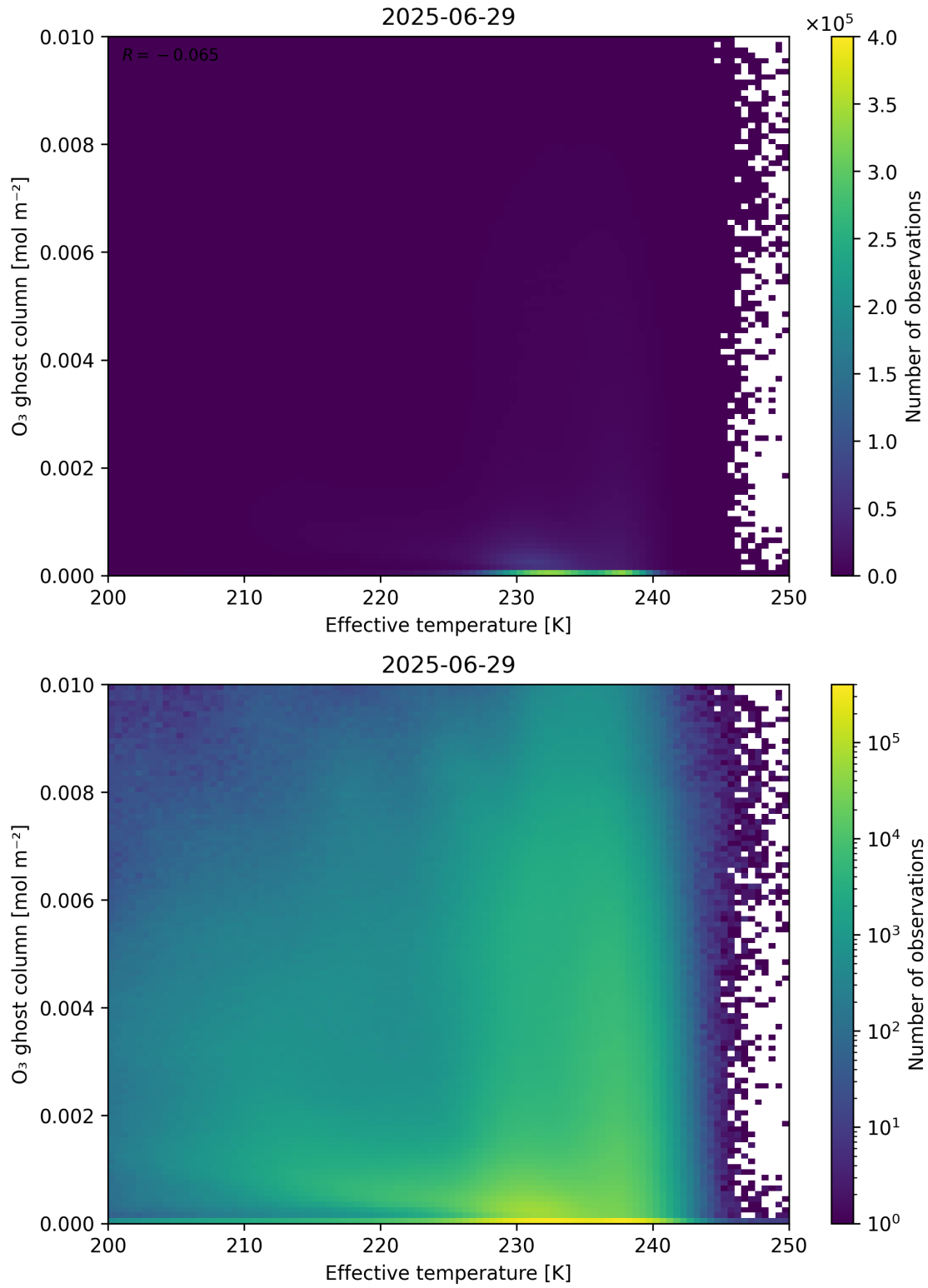
Figure 38: Scatter density plot of “Effective temperature” against “O 3 ghost column” for 2025-06-28 to 2025-06-30.
