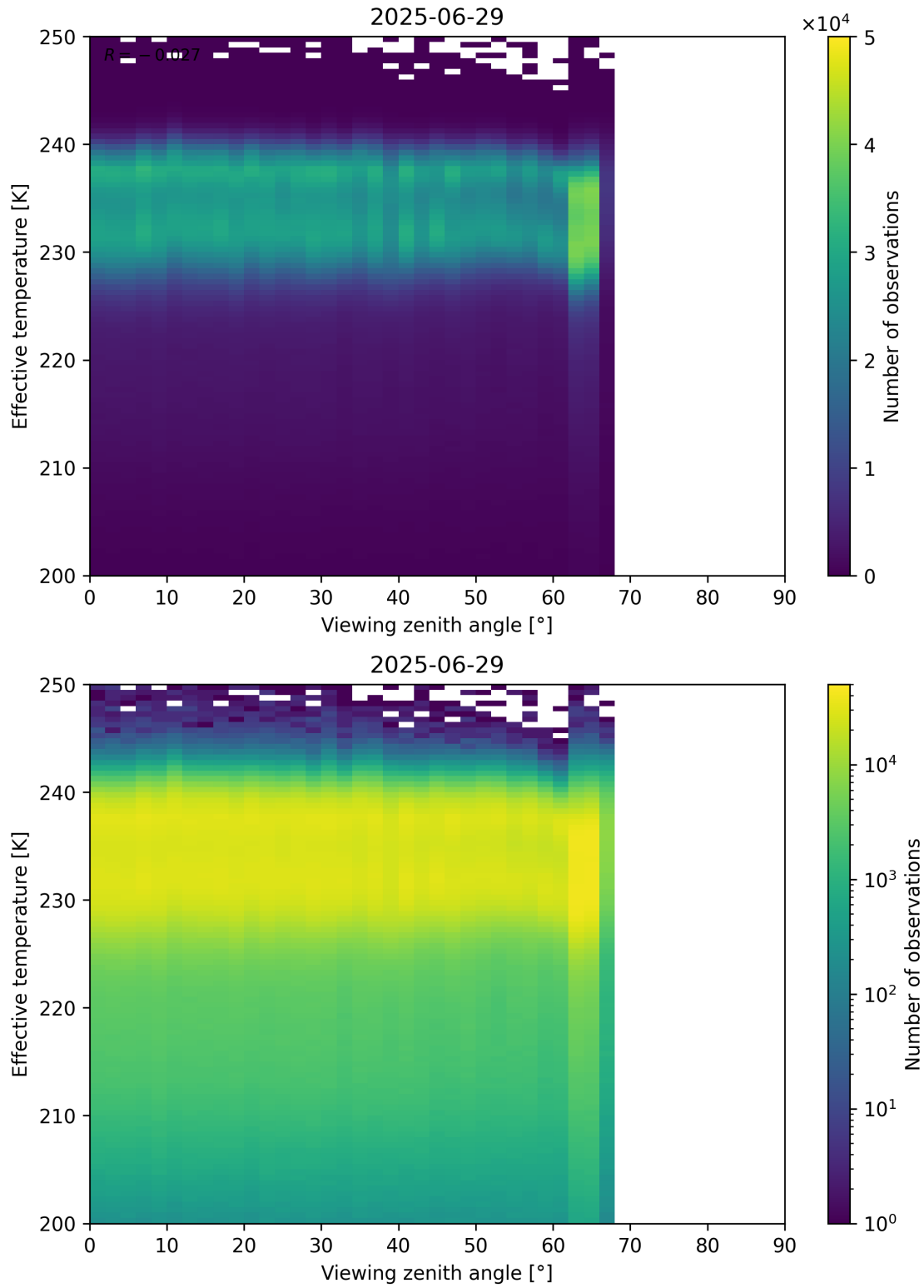
Figure 50: Scatter density plot of “Viewing zenith angle” against “Effective temperature” for 2025-06-28 to 2025-06-30.
