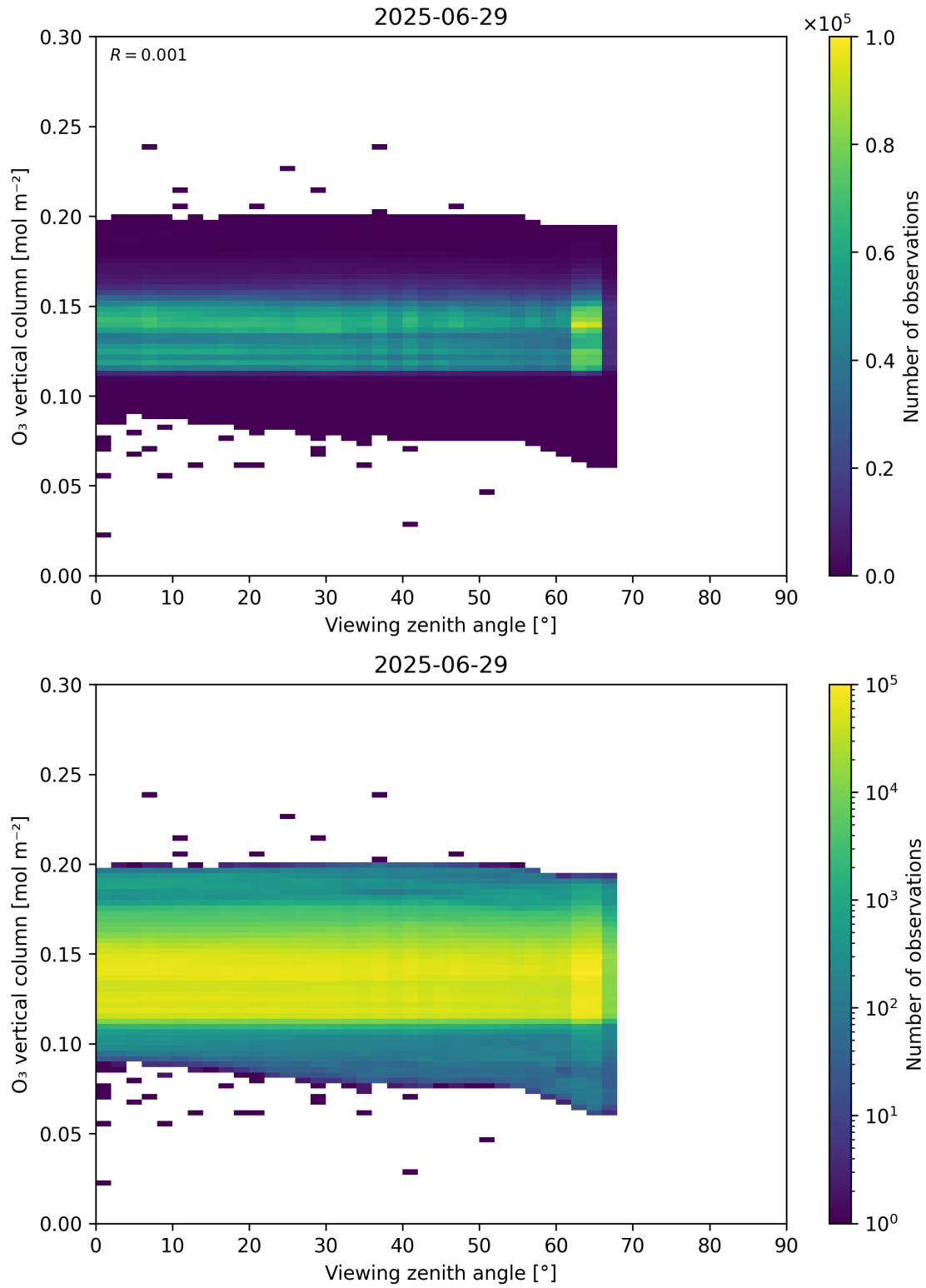
Figure 52: Scatter density plot of “Viewing zenith angle” against “O 3 vertical column” for 2025-06-28 to 2025-06-30.
