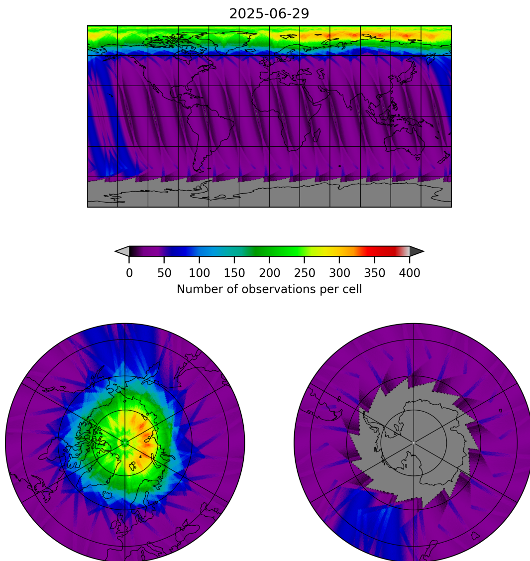
Figure 12: Map of the number of observations for 2025-06-28 to 2025-06-30
