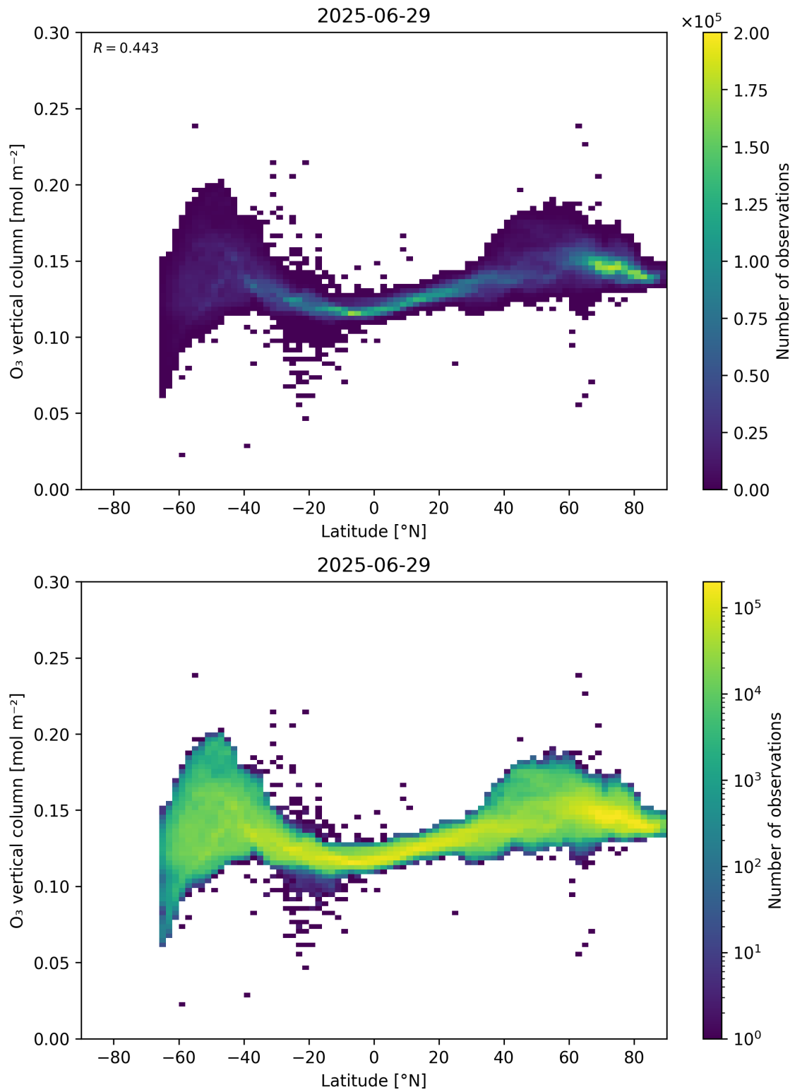
Figure 36: Scatter density plot of “Latitude” against “O 3 vertical column” for 2025-06-28 to 2025-06-30.
