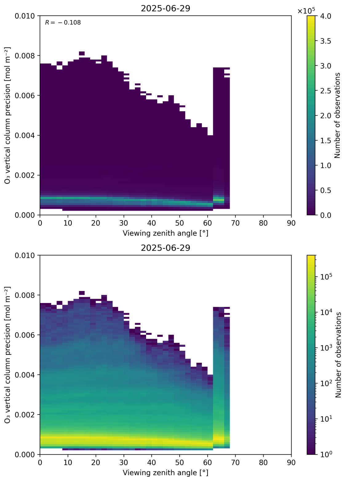
Figure 53: Scatter density plot of “Viewing zenith angle” against “O 3 vertical column precision” for 2025-06-28 to 2025-06-30.
