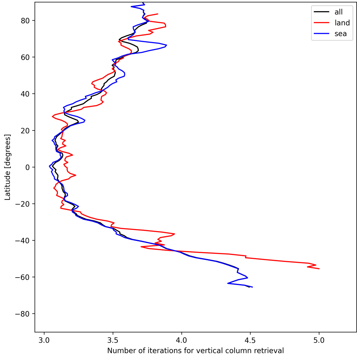
Figure 19: Zonal average of “Number of iterations for vertical column retrieval” for 2025-06-28 to 2025-06-30.
