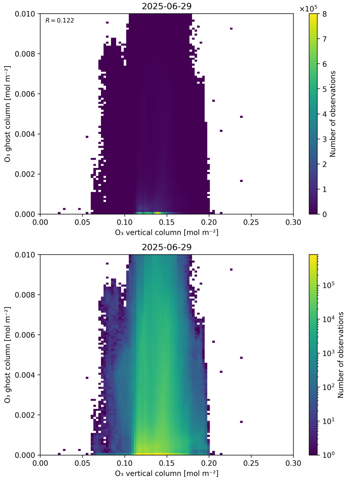
Figure 40: Scatter density plot of “O 3 vertical column” against “O 3 ghost column” for 2025-06-28 to 2025-06-30.
