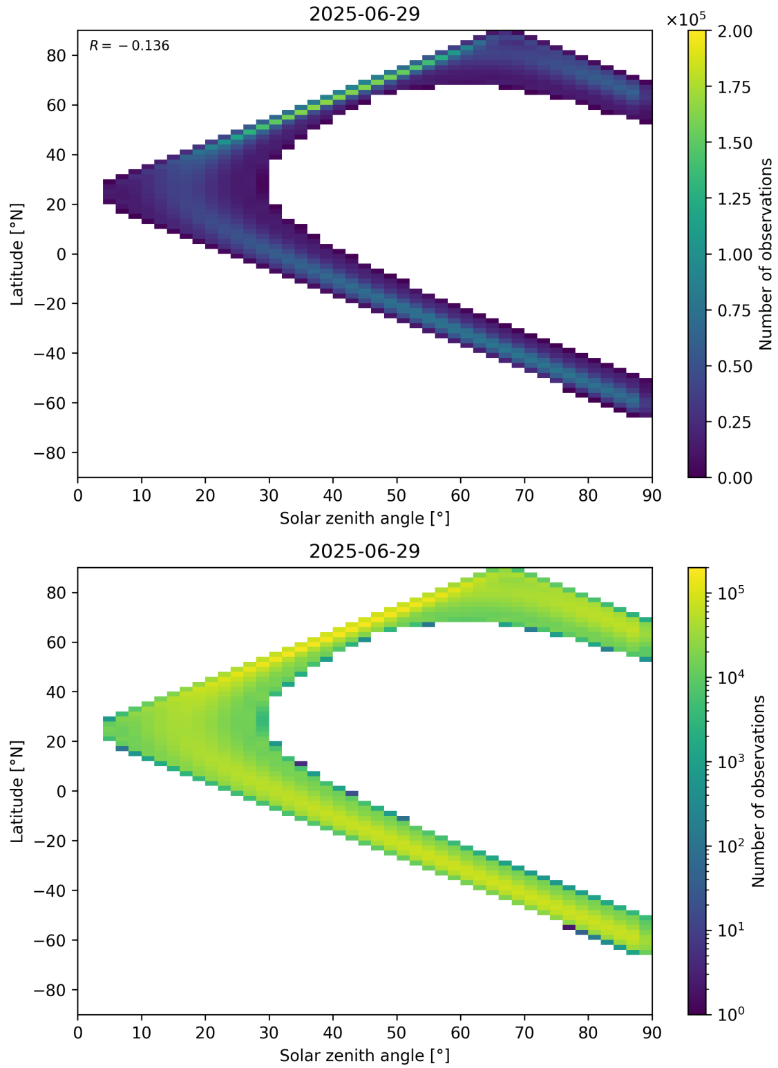
Figure 44: Scatter density plot of “Solar zenith angle” against “Latitude” for 2025-06-28 to 2025-06-30.
