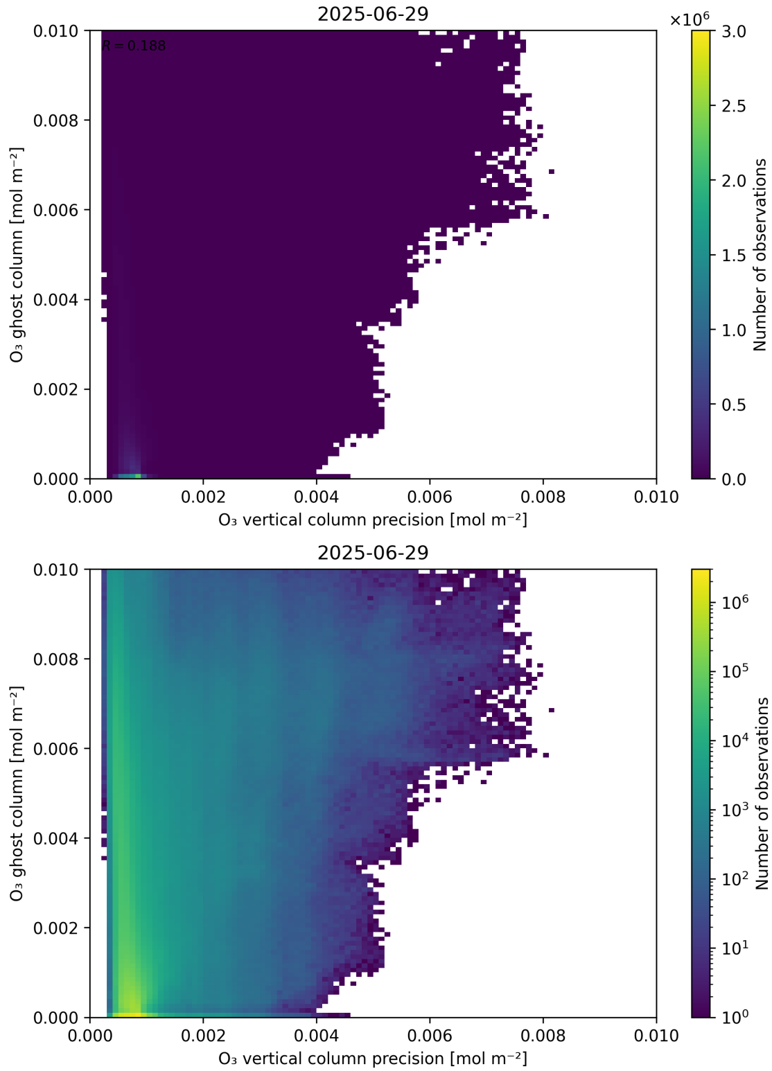
Figure 43: Scatter density plot of “ \text{O}_3 vertical column precision” against “ \text{O}_3 ghost column” for 2025-06-28 to 2025-06-30.
