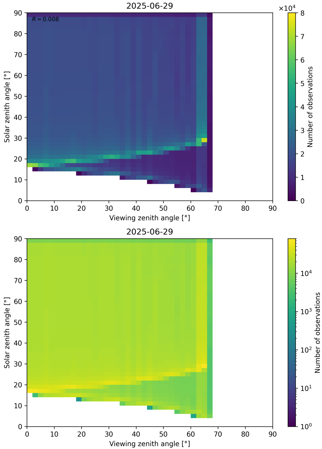
Figure 54: Scatter density plot of “Viewing zenith angle” against “Solar zenith angle” for 2025-06-28 to 2025-06-30.
