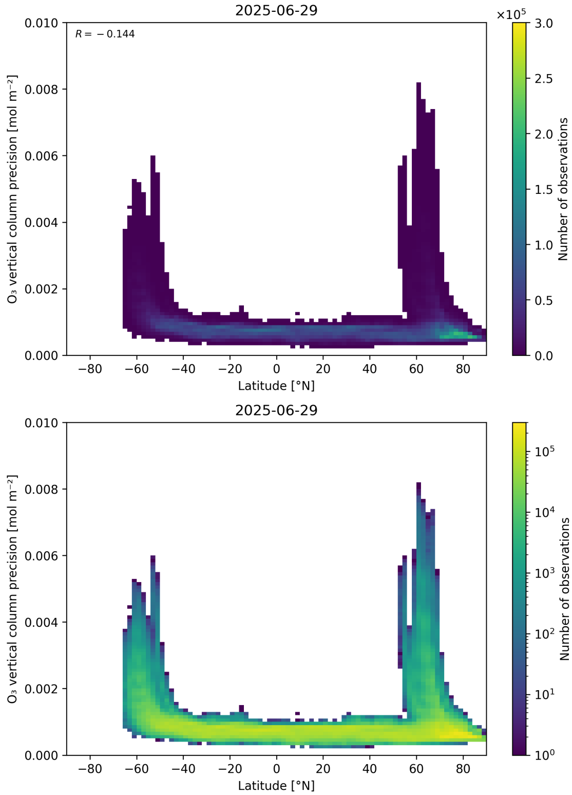
Figure 37: Scatter density plot of “Latitude” against “O 3 vertical column precision” for 2025-06-28 to 2025-06-30.
