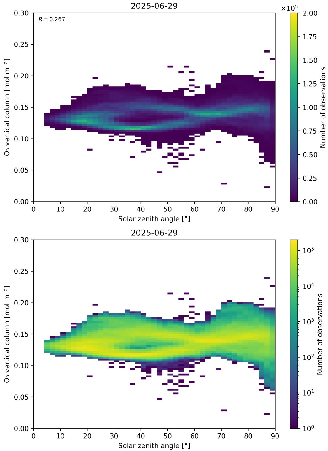
Figure 47: Scatter density plot of “Solar zenith angle” against “O 3 vertical column” for 2025-06-28 to 2025-06-30.
