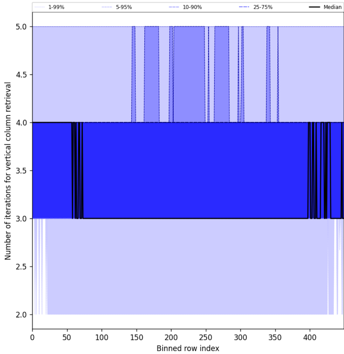
Figure 33: Along track statistics of “Number of iterations for vertical column retrieval” for 2025-06-28 to 2025-06-30
