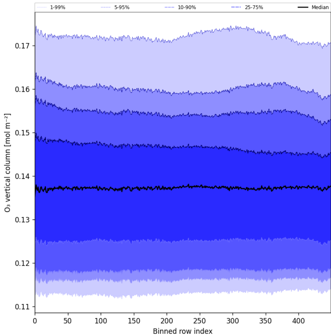
Figure 28: Along track statistics of “O 3 vertical column” for 2025-06-28 to 2025-06-30
