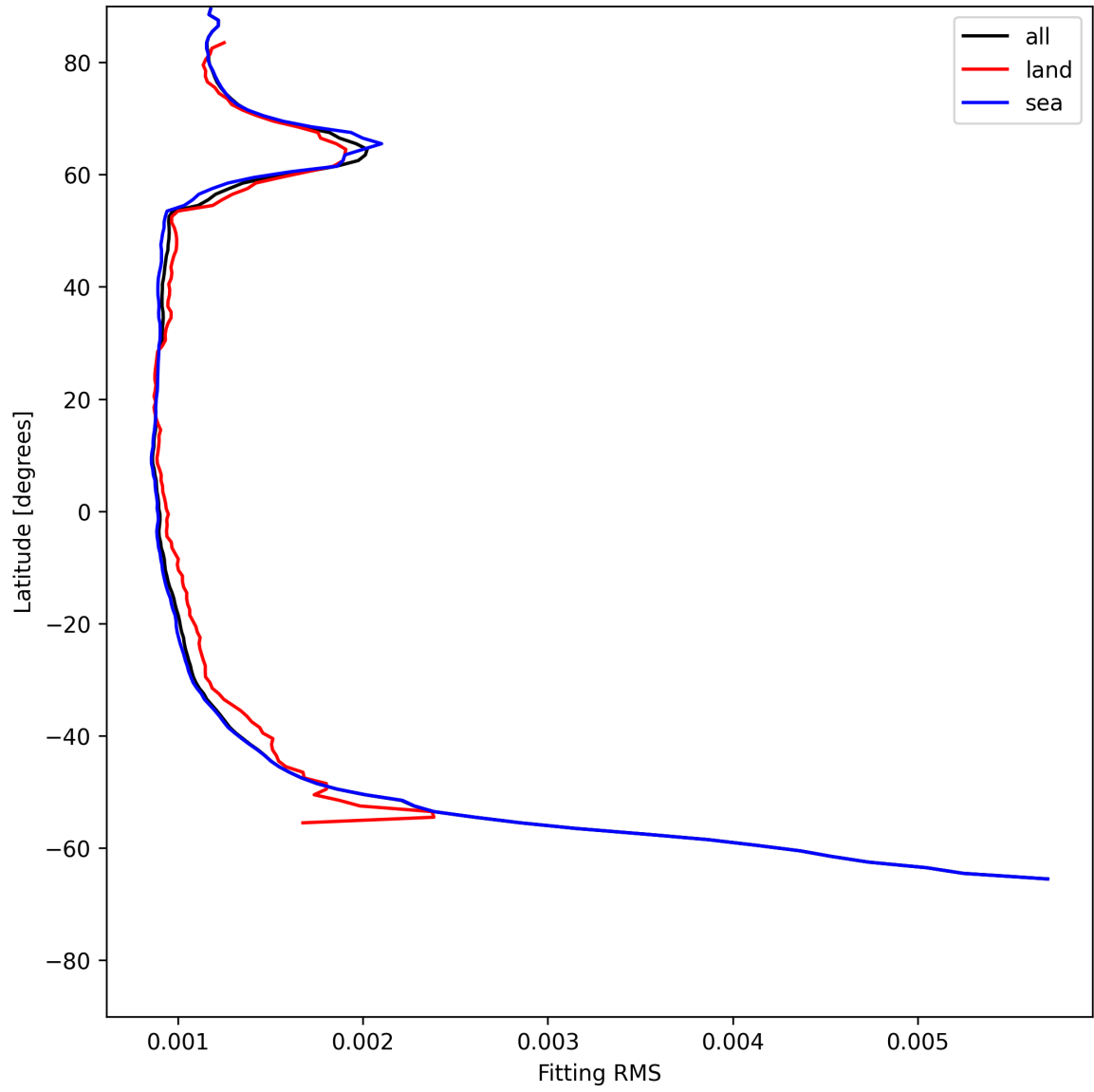
Figure 16: Zonal average of “Fitting RMS” for 2025-06-28 to 2025-06-30.
