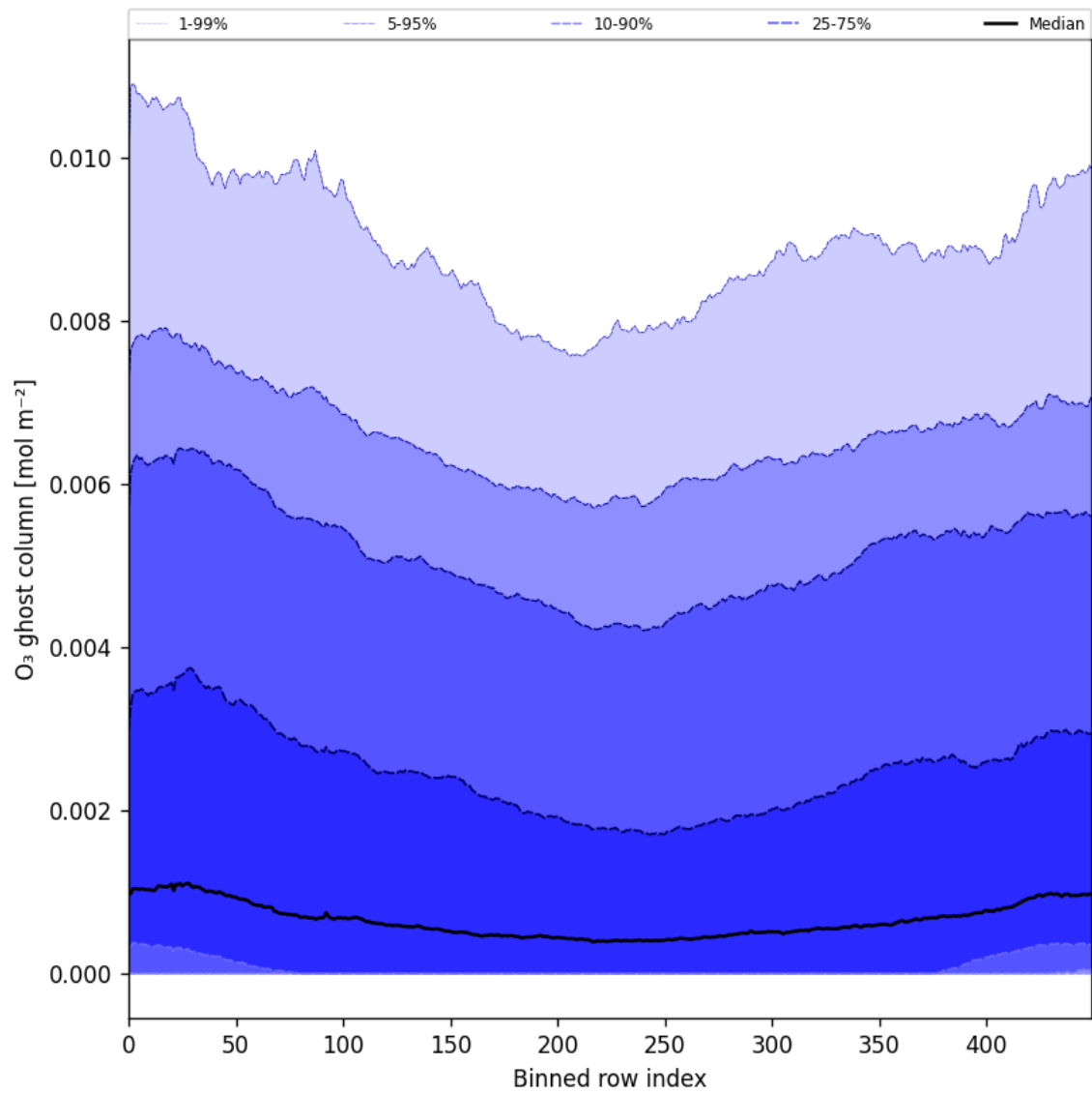
Figure 32: Along track statistics of “O 3 ghost column” for 2025-06-29 to 2025-07-01
