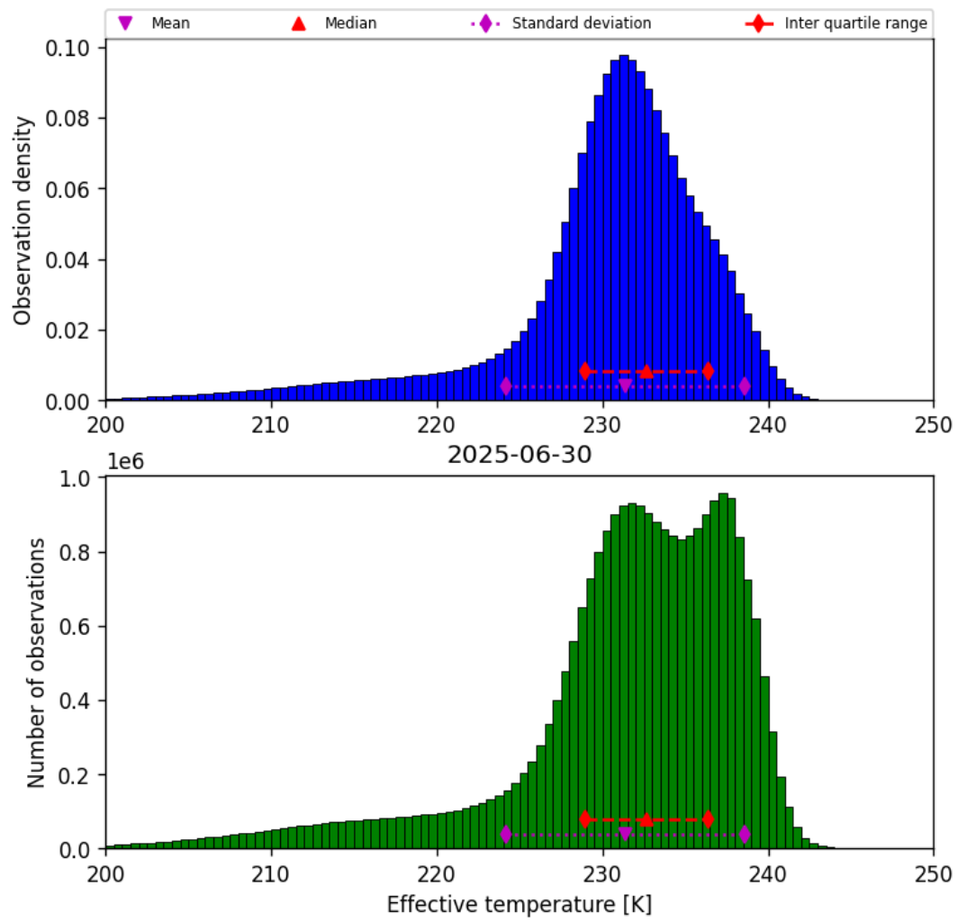
Figure 24: Histogram of “Effective temperature” for 2025-06-29 to 2025-07-01
