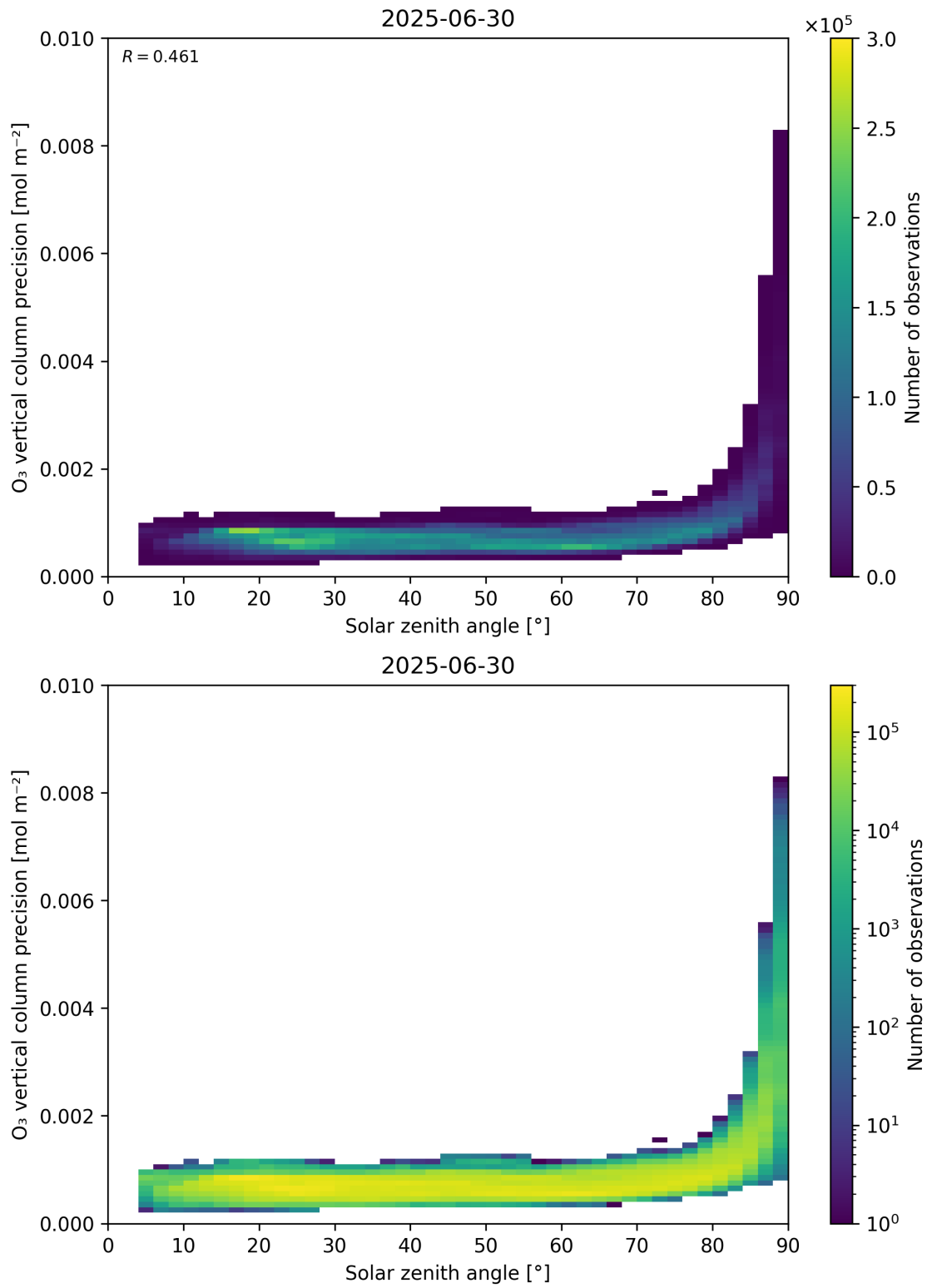
Figure 48: Scatter density plot of “Solar zenith angle” against “O 3 vertical column precision” for 2025-06-29 to 2025-07-01.
