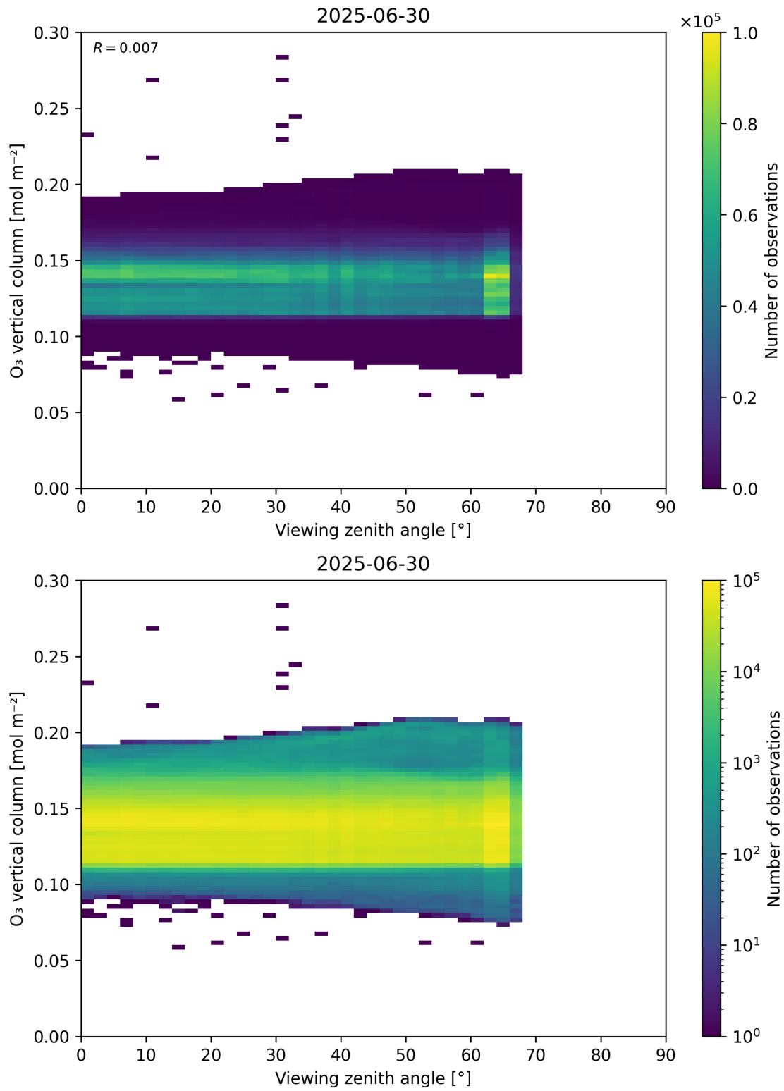
Figure 52: Scatter density plot of “Viewing zenith angle” against “O 3 vertical column” for 2025-06-29 to 2025-07-01.
