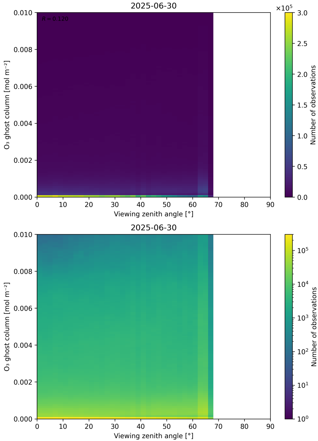
Figure 51: Scatter density plot of “Viewing zenith angle” against “O 3 ghost column” for 2025-06-29 to 2025-07-01.
