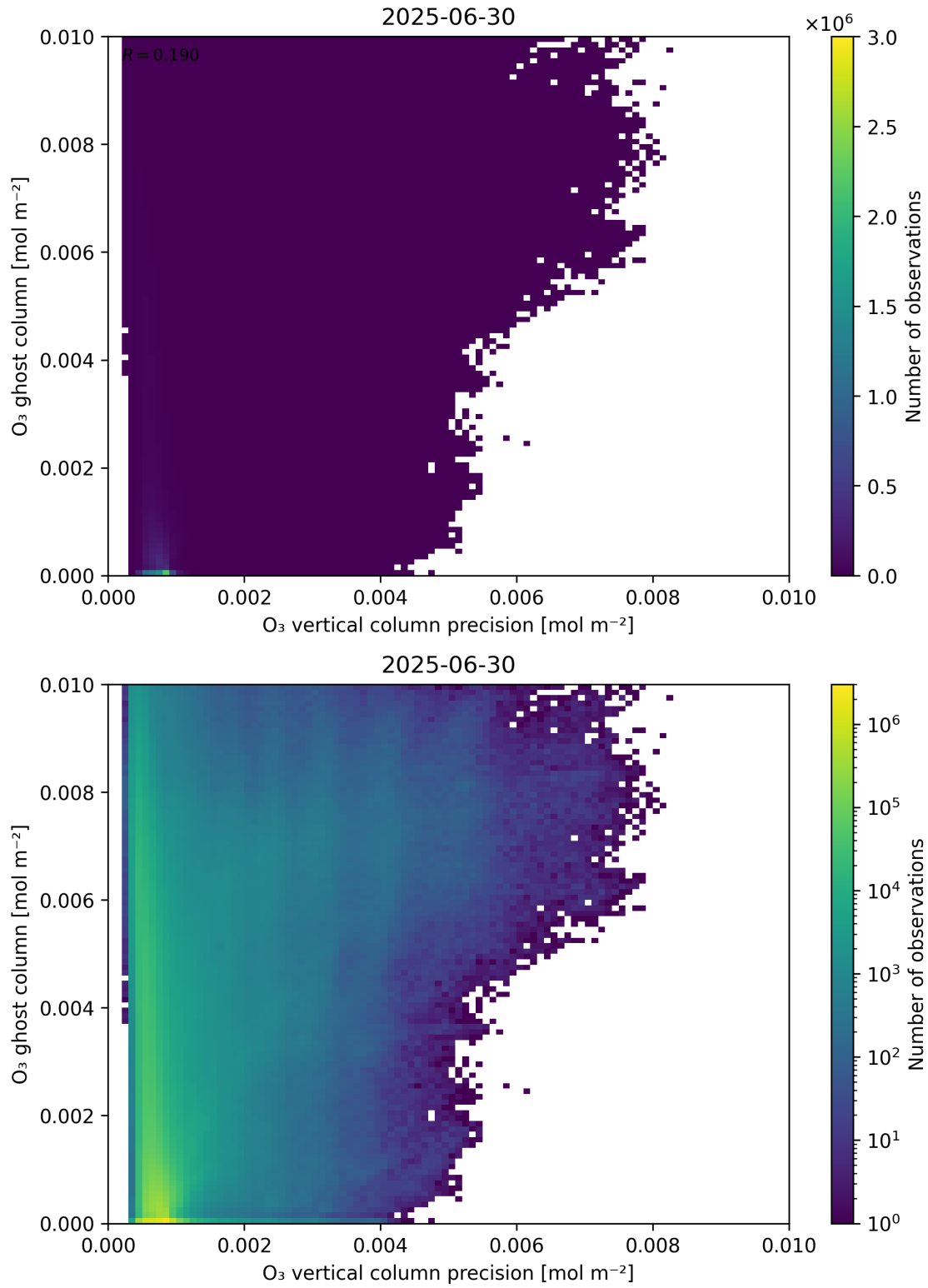
Figure 43: Scatter density plot of “ \text{O}_3 vertical column precision” against “ \text{O}_3 ghost column” for 2025-06-29 to 2025-07-01.
