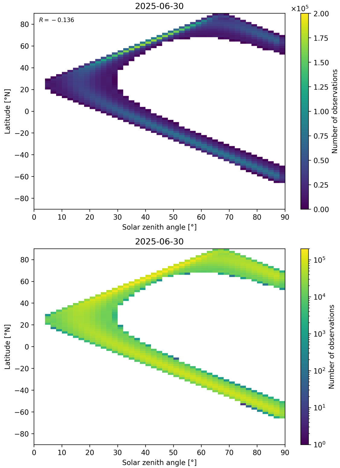
Figure 44: Scatter density plot of “Solar zenith angle” against “Latitude” for 2025-06-29 to 2025-07-01.
