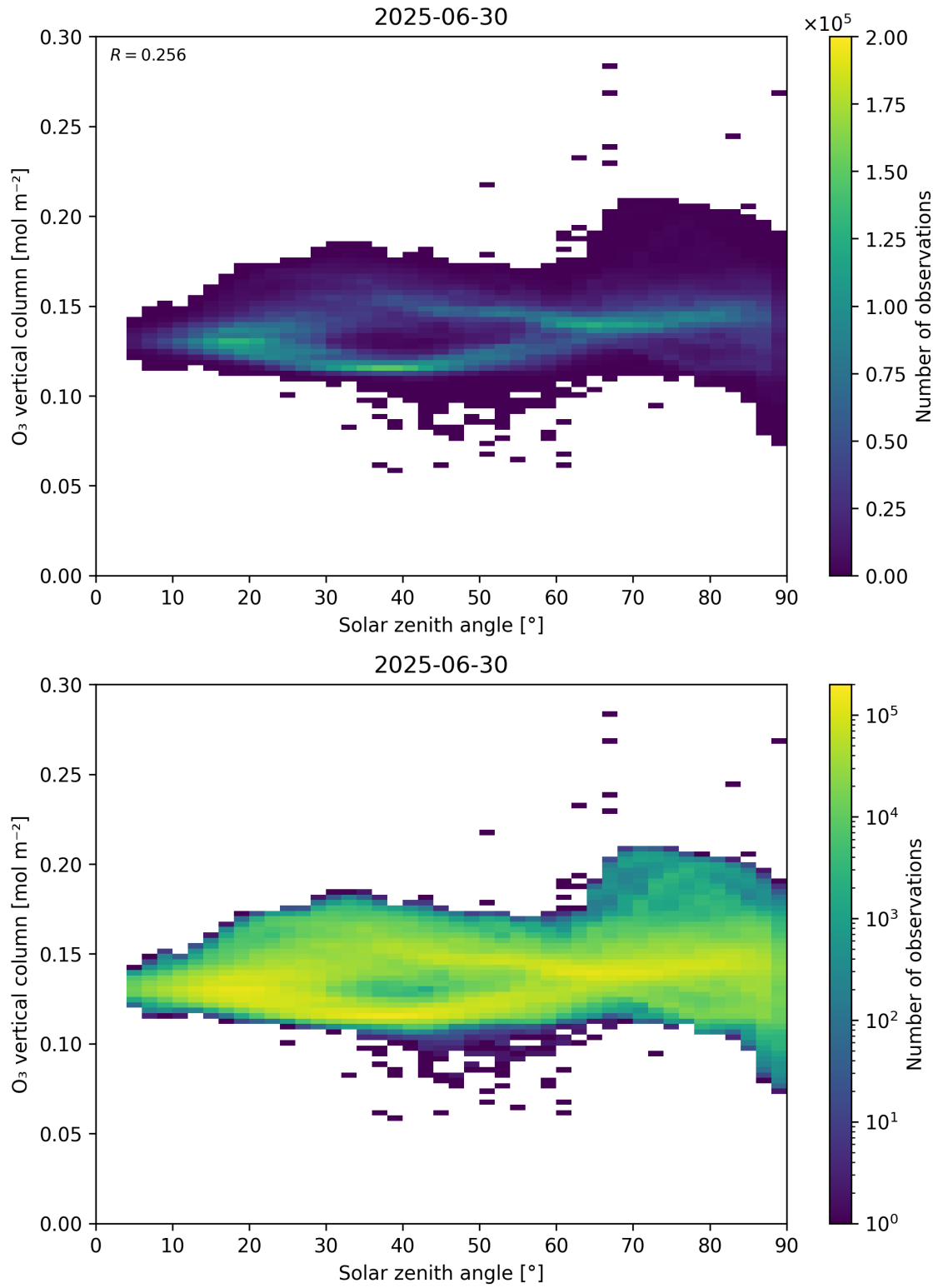
Figure 47: Scatter density plot of “Solar zenith angle” against “O 3 vertical column” for 2025-06-29 to 2025-07-01.
