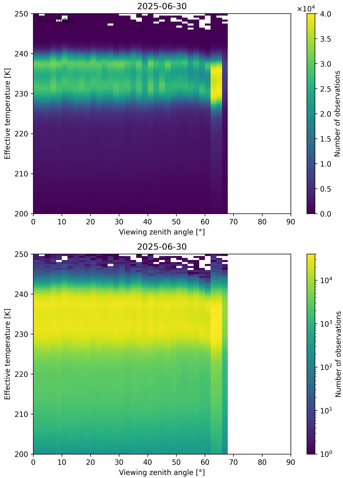
Figure 50: Scatter density plot of “Viewing zenith angle” against “Effective temperature” for 2025-06-29 to 2025-07-01.
