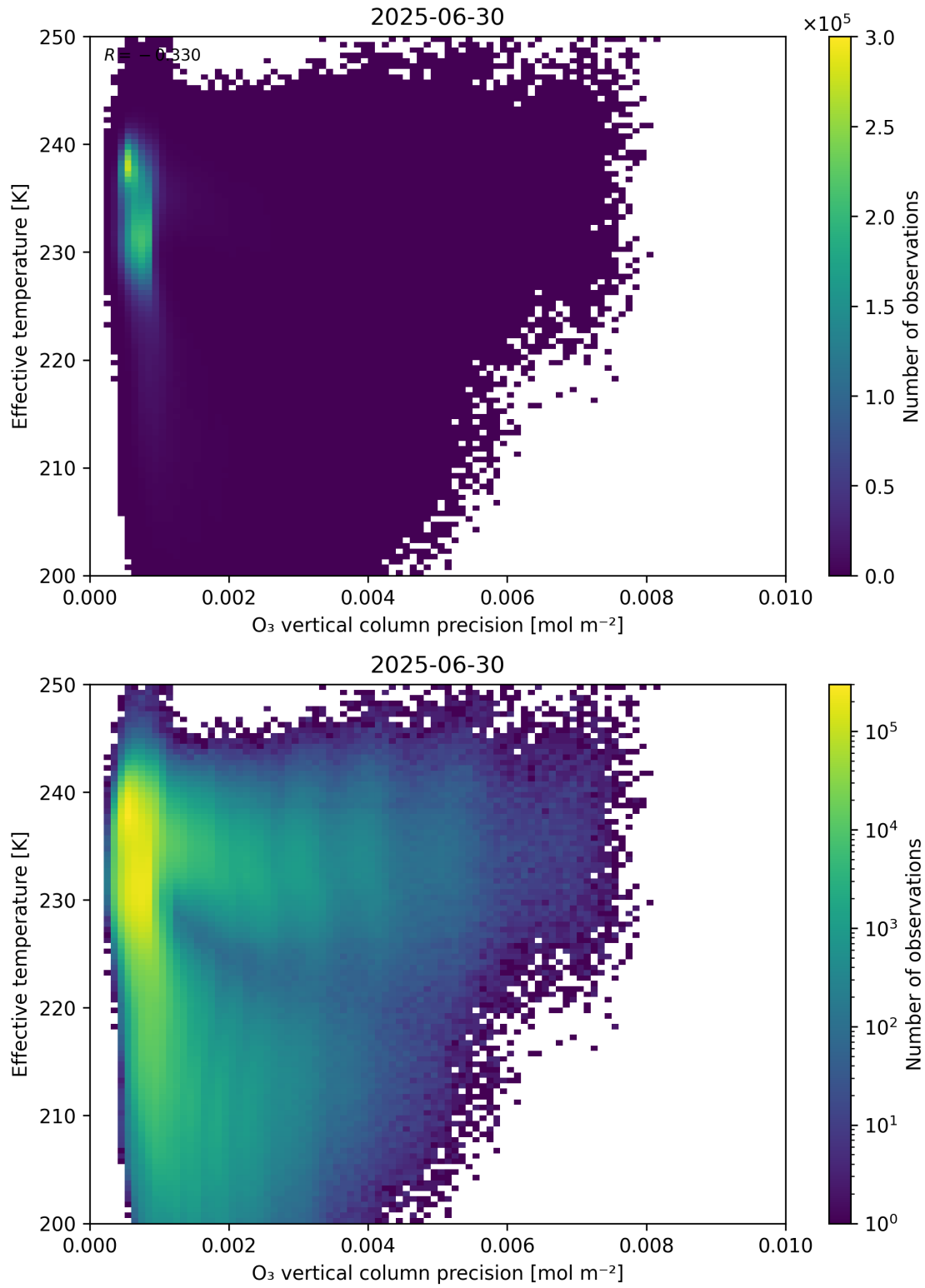
Figure 42: Scatter density plot of “O 3 vertical column precision” against “Effective temperature” for 2025-06-29 to 2025-07-01.
