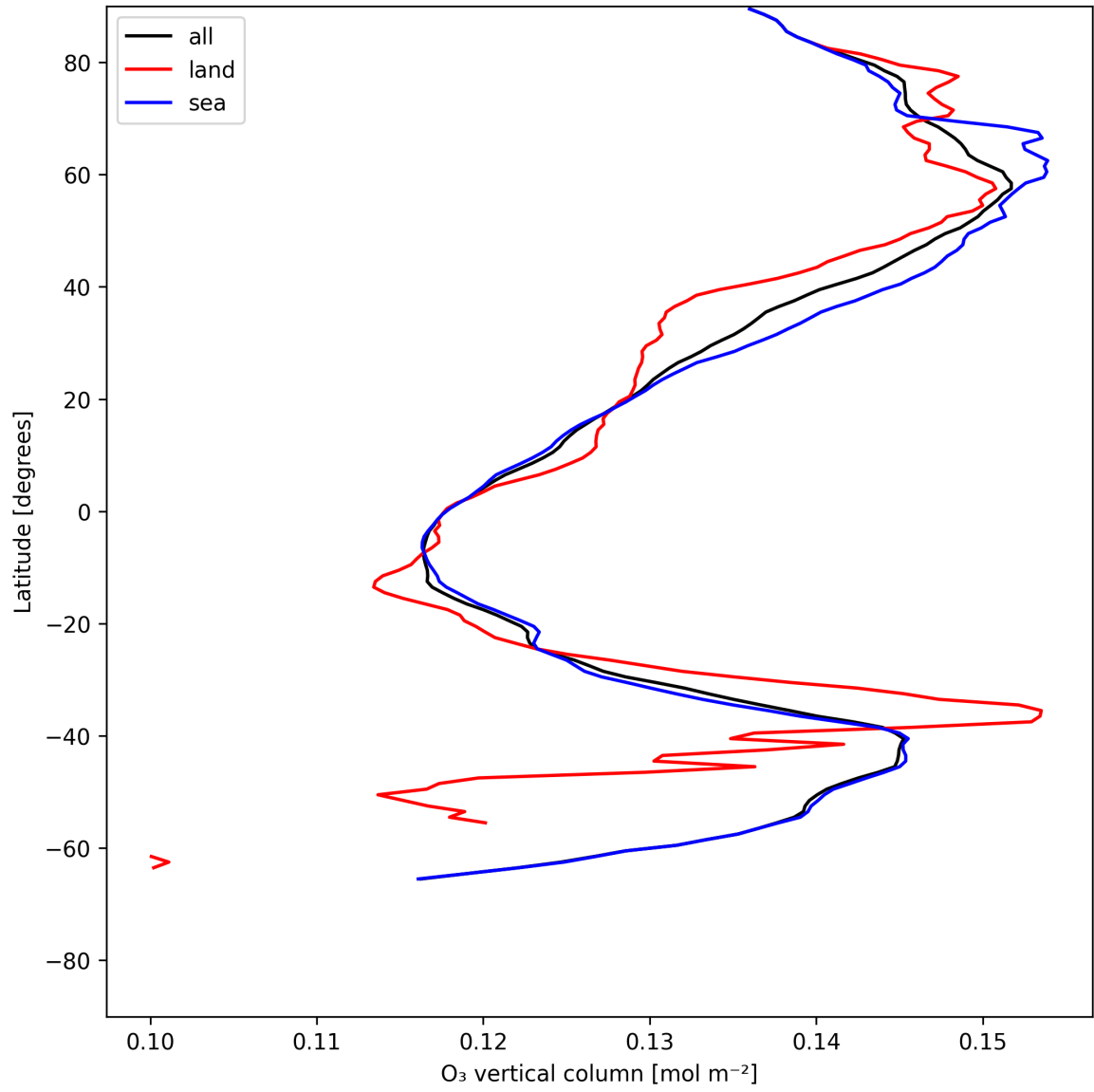
Figure 14: Zonal average of “O 3 vertical column” for 2025-06-29 to 2025-07-01.
