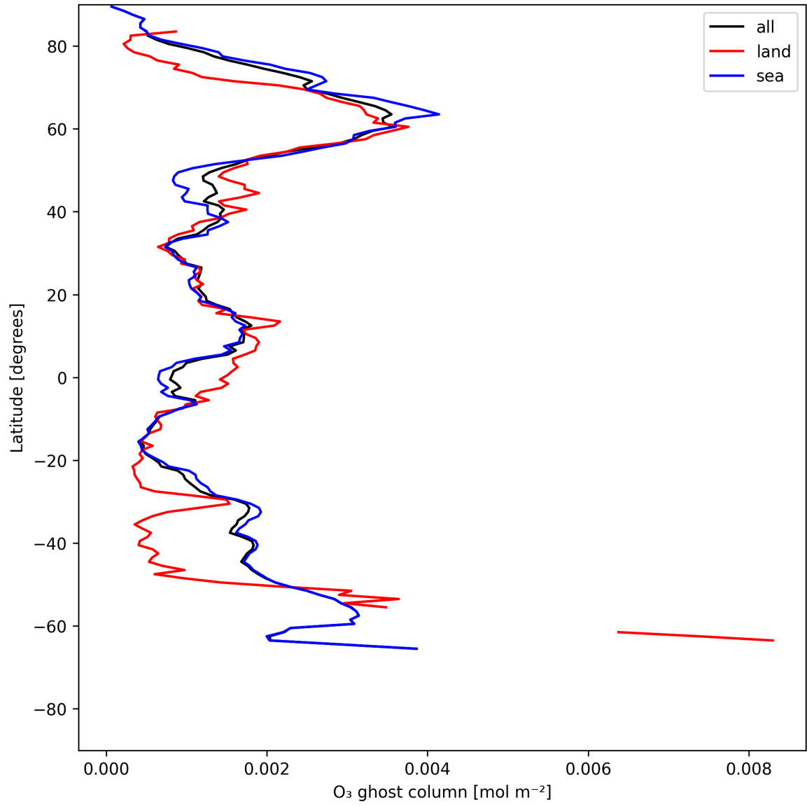
Figure 18: Zonal average of “O 3 ghost column” for 2025-06-29 to 2025-07-01.
