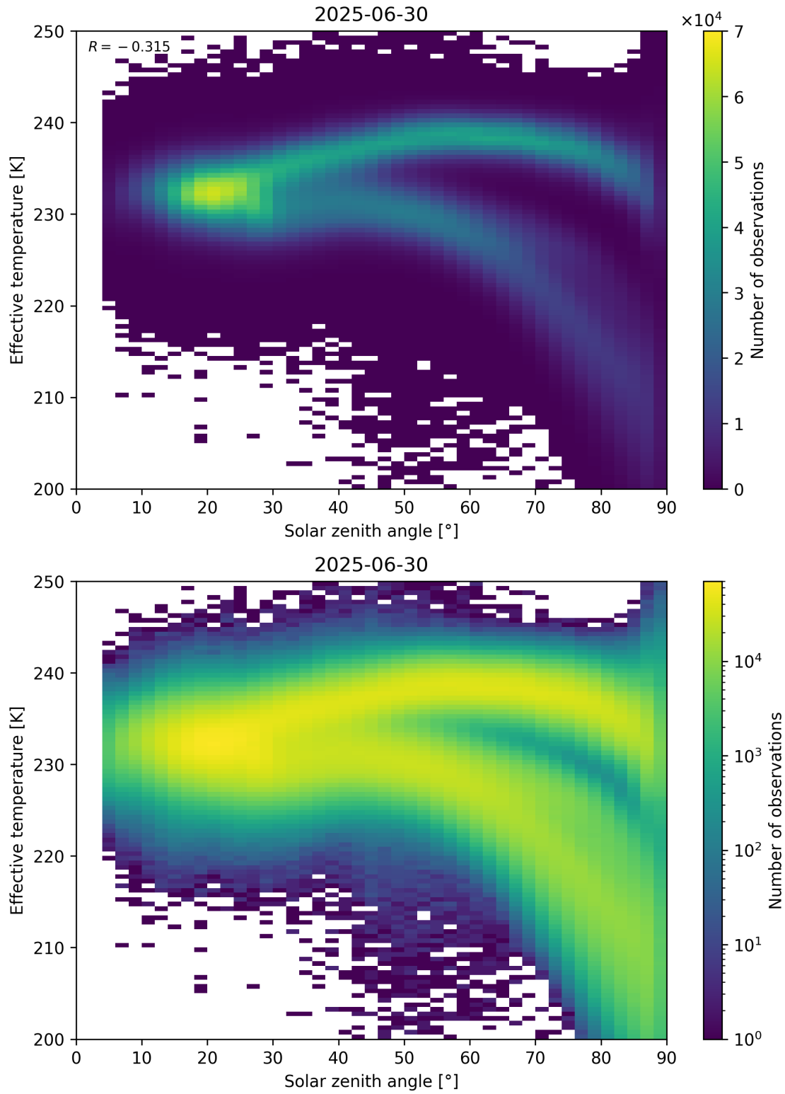
Figure 45: Scatter density plot of “Solar zenith angle” against “Effective temperature” for 2025-06-29 to 2025-07-01.
