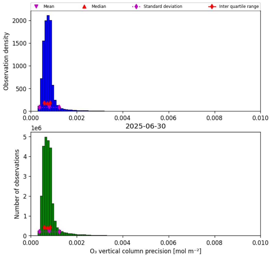
Figure 22: Histogram of “O 3 vertical column precision” for 2025-06-29 to 2025-07-01
