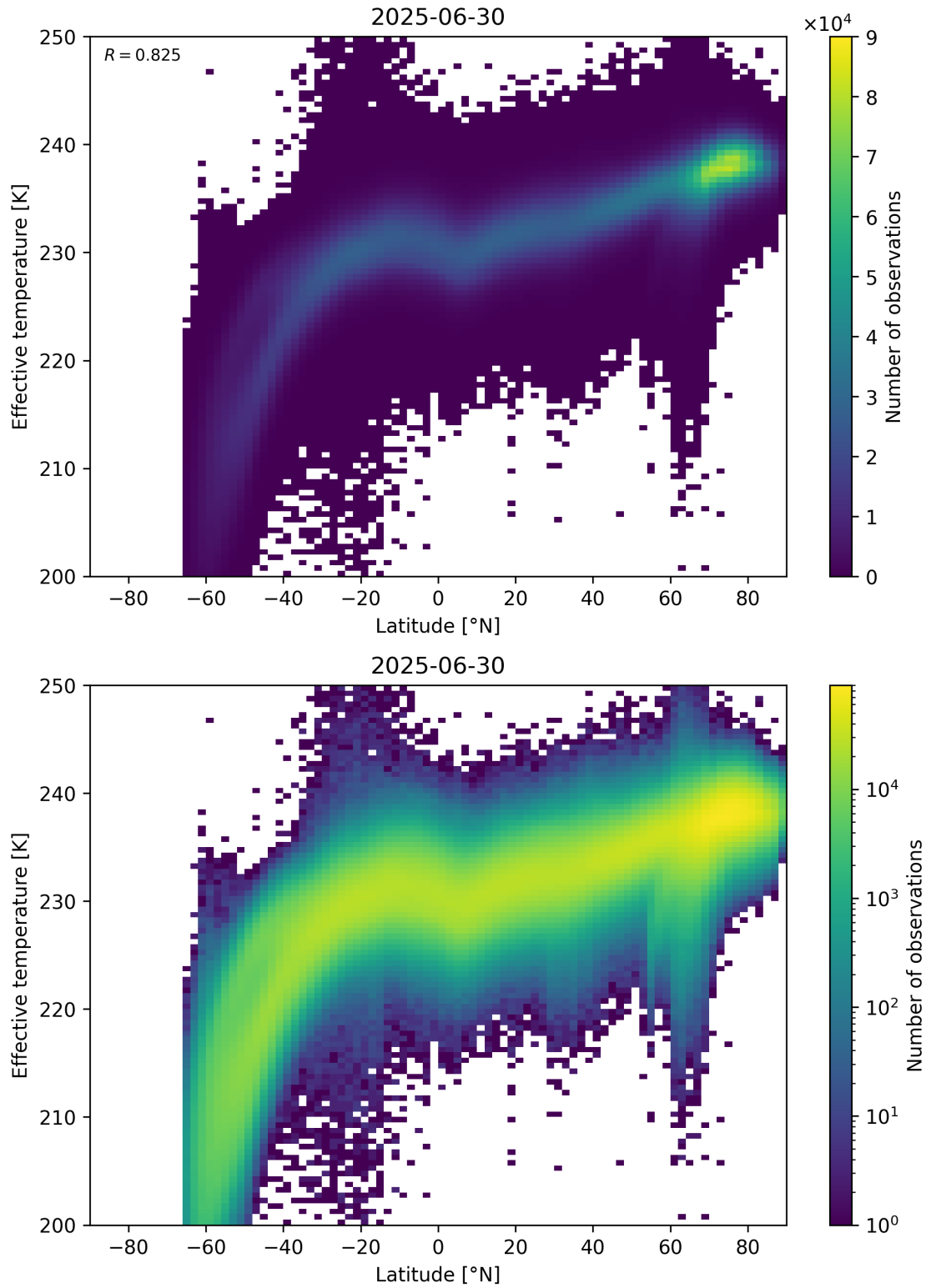
Figure 34: Scatter density plot of “Latitude” against “Effective temperature” for 2025-06-29 to 2025-07-01.
