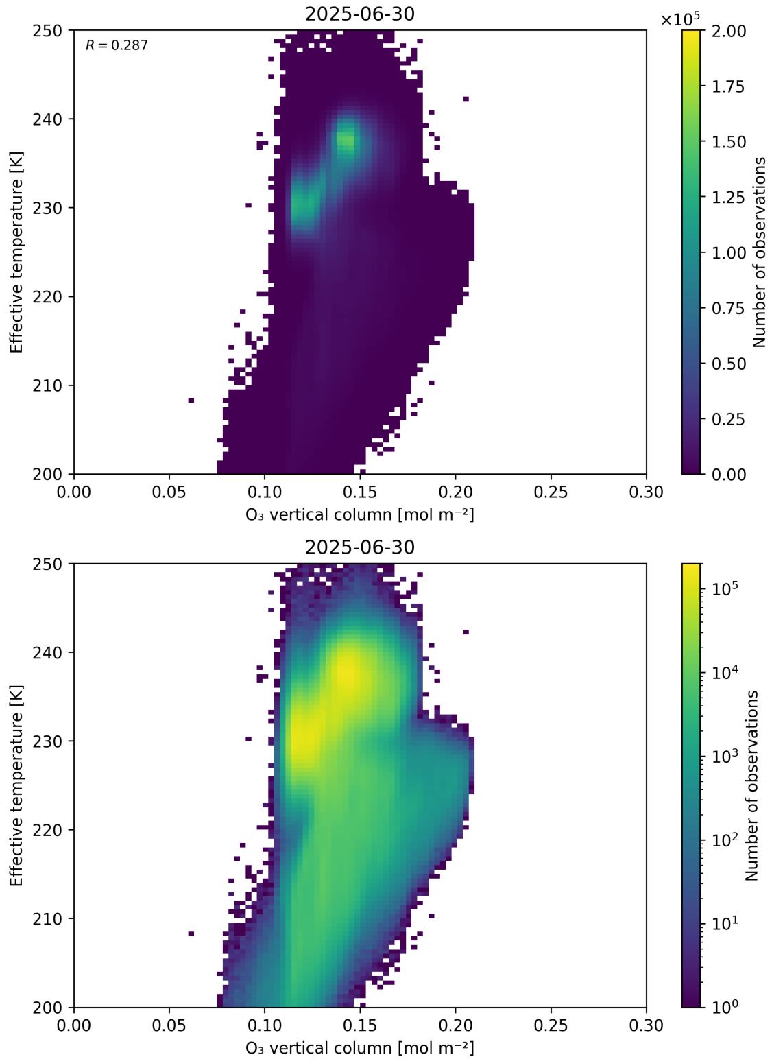
Figure 39: Scatter density plot of “O 3 vertical column” against “Effective temperature” for 2025-06-29 to 2025-07-01.
