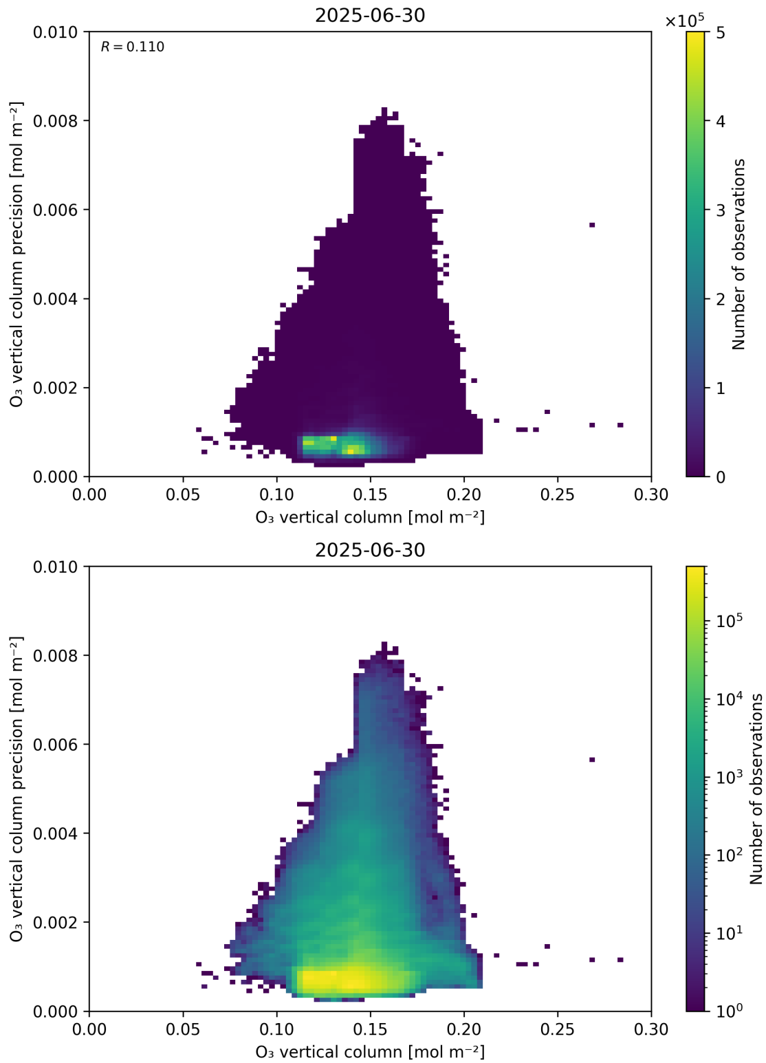
Figure 41: Scatter density plot of “O 3 vertical column” against “O 3 vertical column precision” for 2025-06-29 to 2025-07-01.
