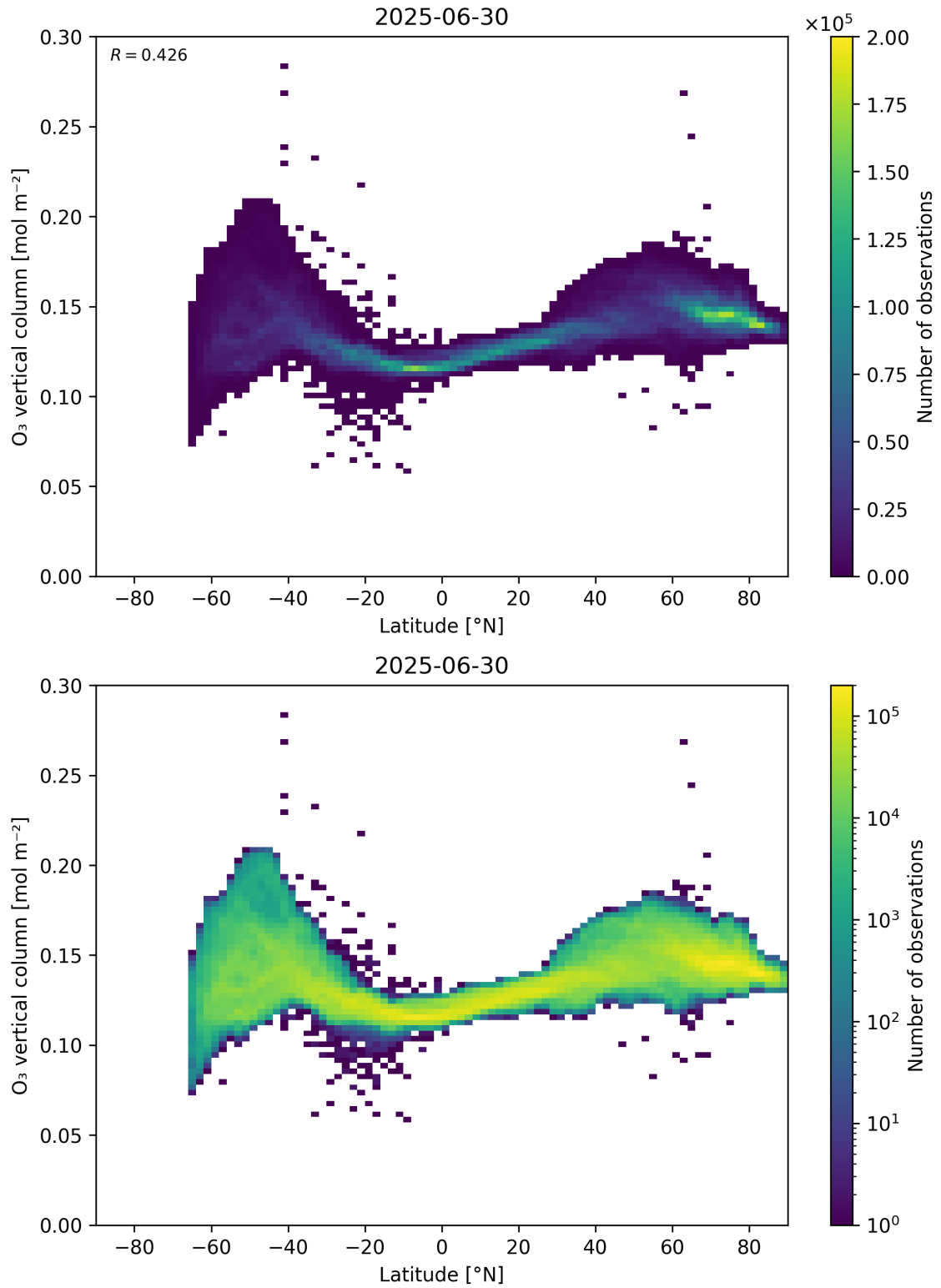
Figure 36: Scatter density plot of “Latitude” against “O 3 vertical column” for 2025-06-29 to 2025-07-01.
