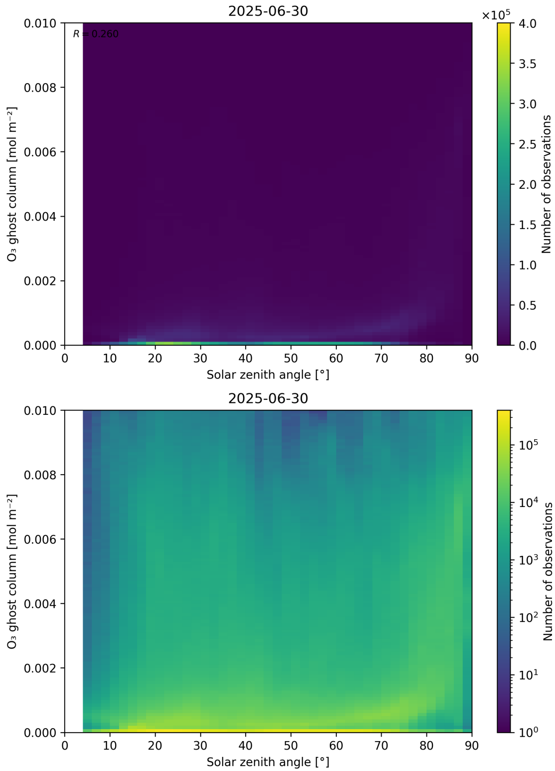
Figure 46: Scatter density plot of “Solar zenith angle” against “O 3 ghost column” for 2025-06-29 to 2025-07-01.
