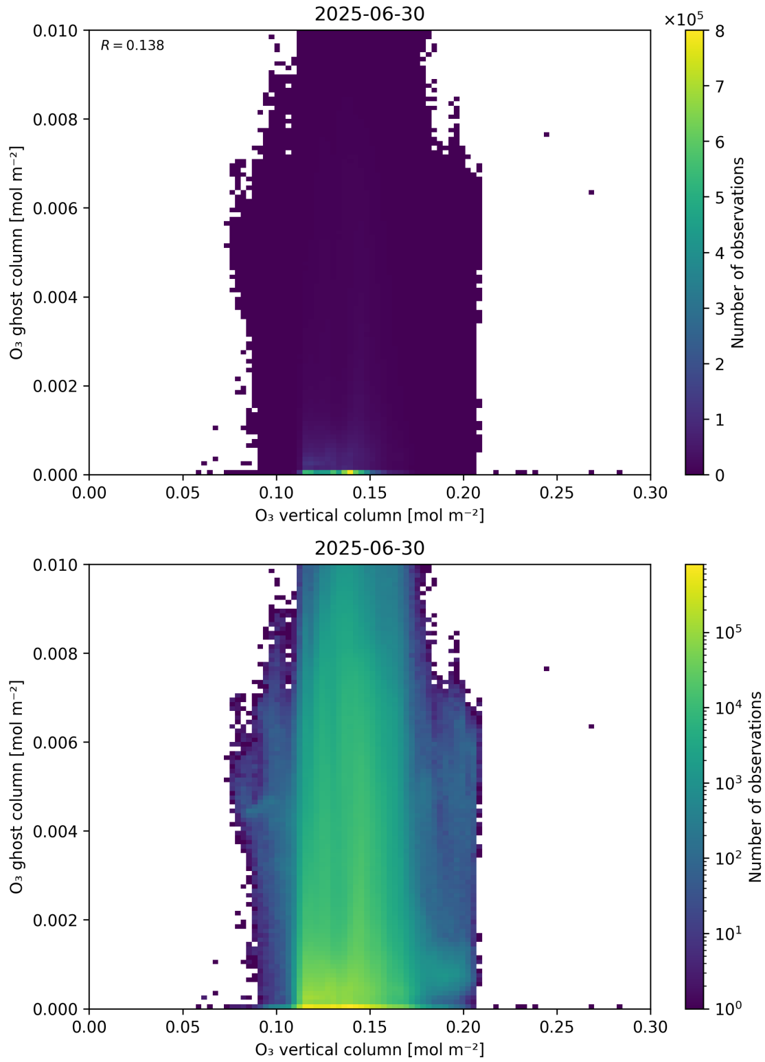
Figure 40: Scatter density plot of “O 3 vertical column” against “O 3 ghost column” for 2025-06-29 to 2025-07-01.
