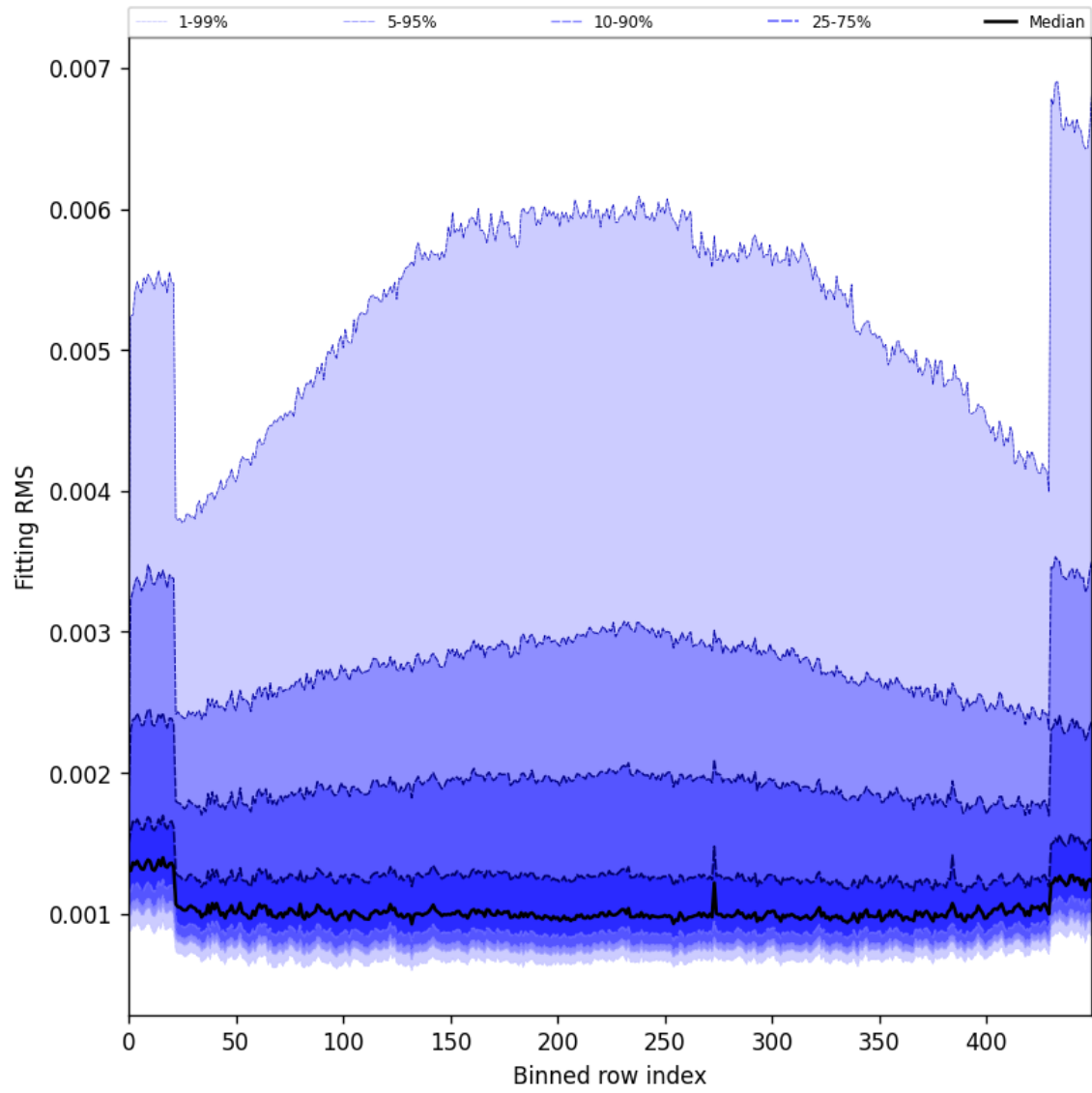
Figure 30: Along track statistics of “Fitting RMS” for 2025-06-29 to 2025-07-01
