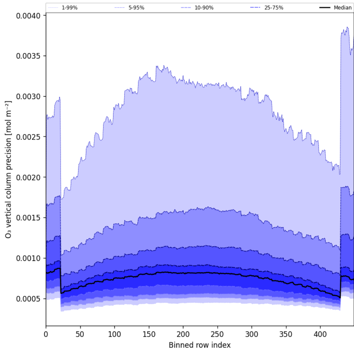
Figure 29: Along track statistics of “O 3 vertical column precision” for 2025-06-29 to 2025-07-01
