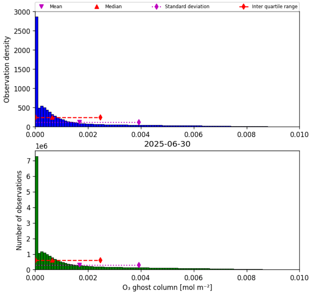
Figure 25: Histogram of “O 3 ghost column” for 2025-06-29 to 2025-07-01
