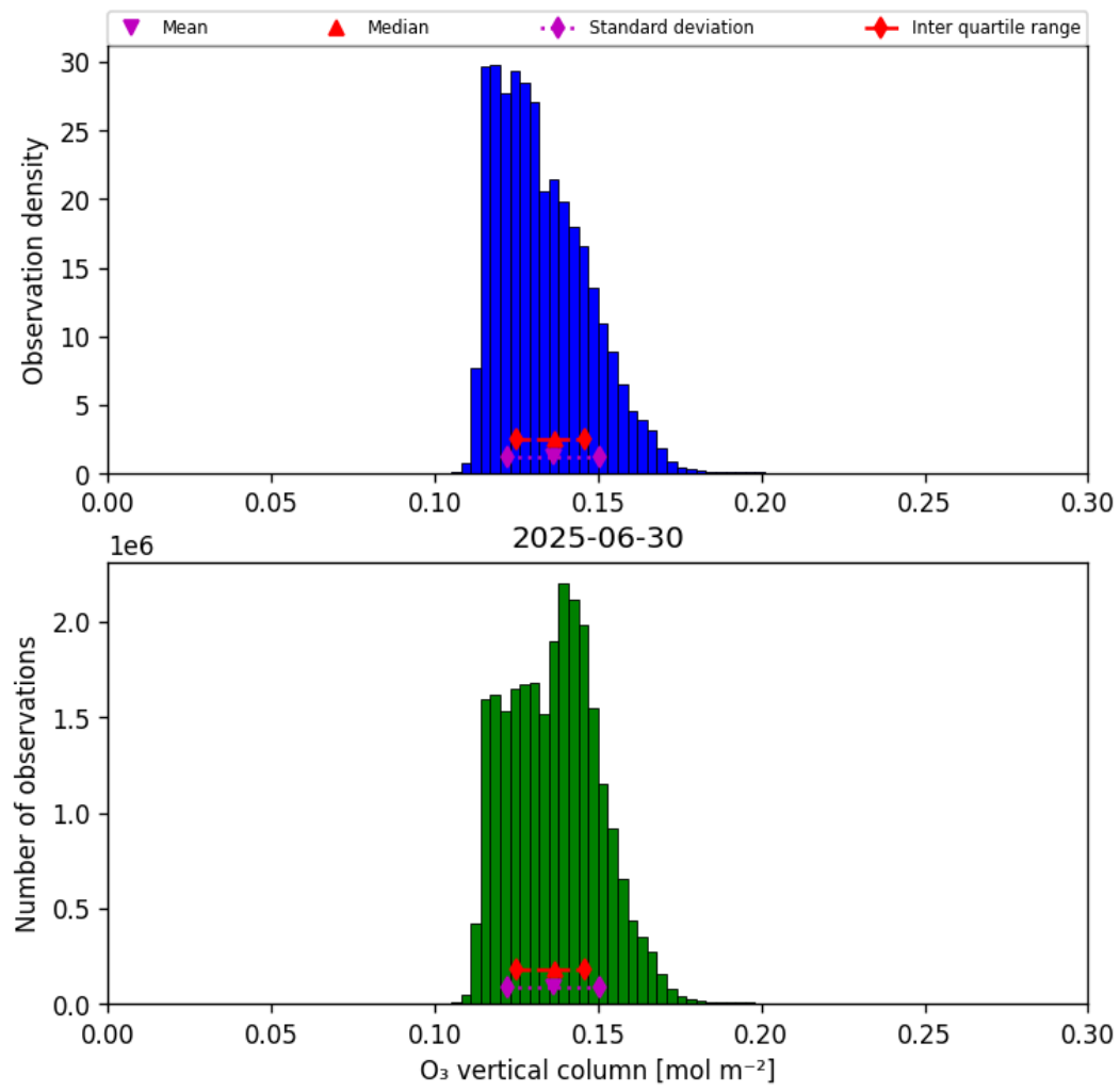
Figure 21: Histogram of “O 3 vertical column” for 2025-06-29 to 2025-07-01
