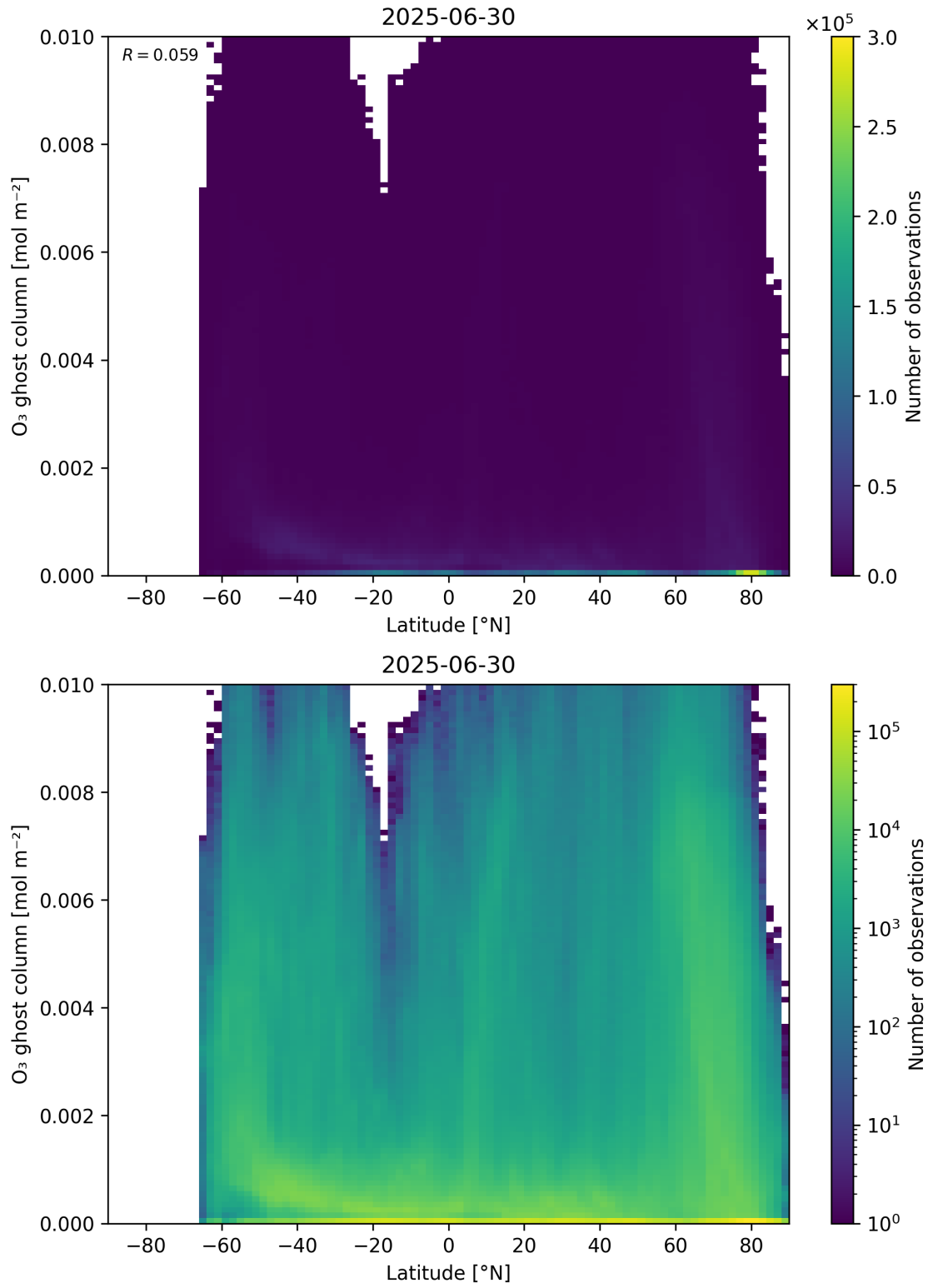
Figure 35: Scatter density plot of “Latitude” against “O 3 ghost column” for 2025-06-29 to 2025-07-01.
