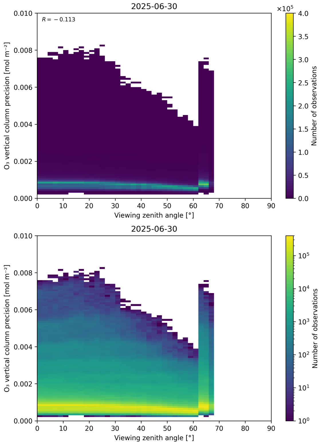
Figure 53: Scatter density plot of “Viewing zenith angle” against “O 3 vertical column precision” for 2025-06-29 to 2025-07-01.
