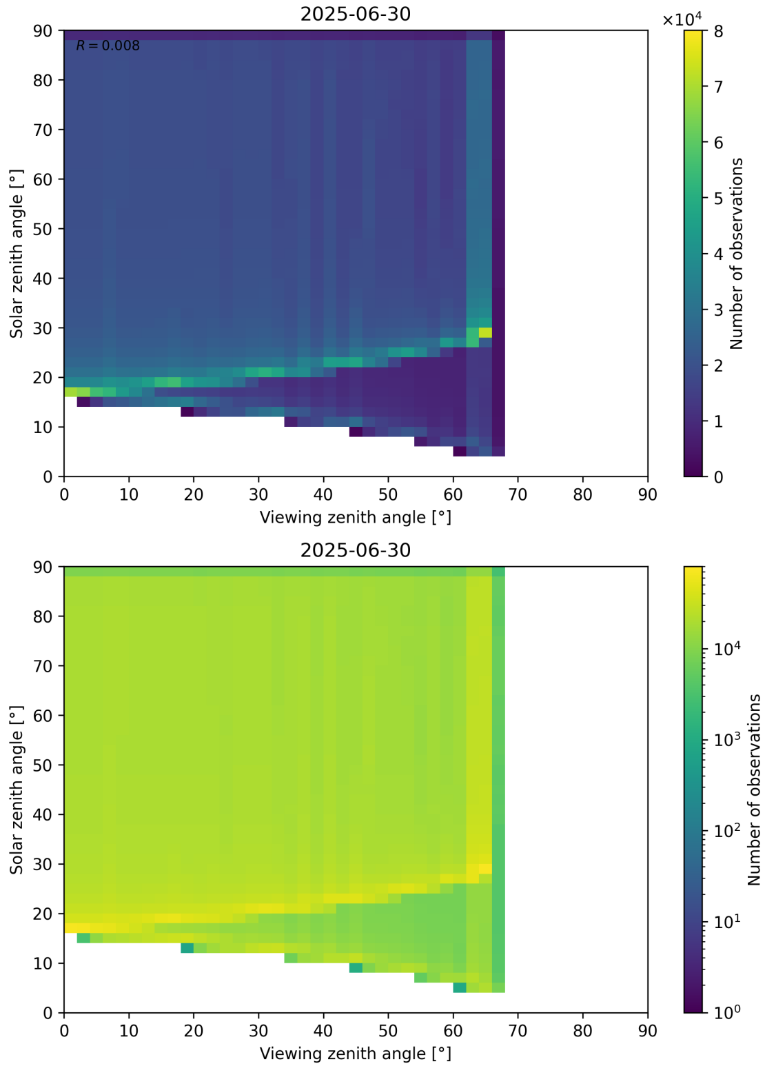
Figure 54: Scatter density plot of “Viewing zenith angle” against “Solar zenith angle” for 2025-06-29 to 2025-07-01.
