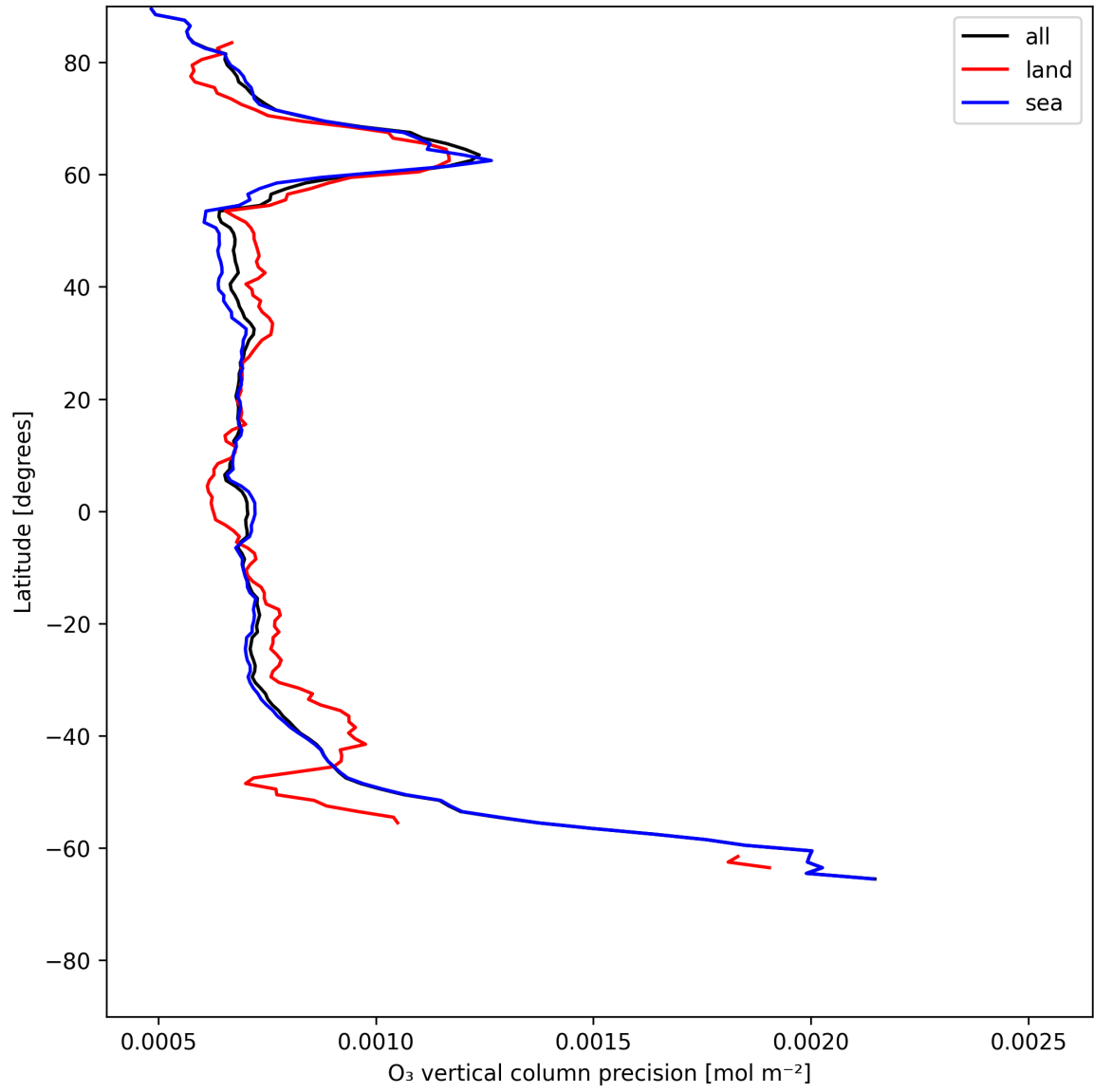
Figure 15: Zonal average of “O 3 vertical column precision” for 2025-06-29 to 2025-07-01.
