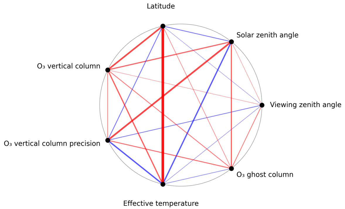
Figure 1: Map of correlation graph for 2025-06-29 to 2025-07-01.
