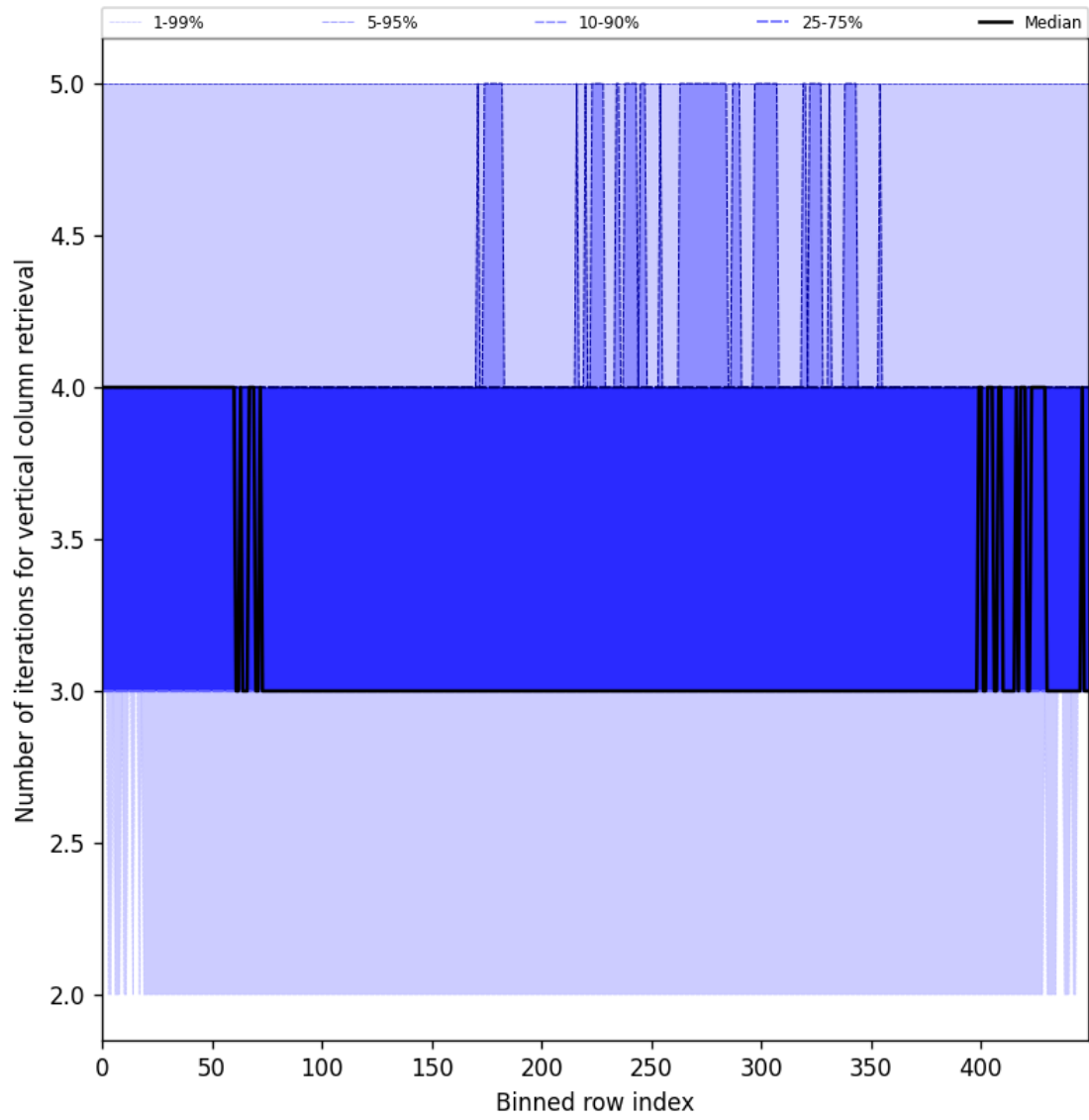
Figure 33: Along track statistics of “Number of iterations for vertical column retrieval” for 2025-06-29 to 2025-07-01
