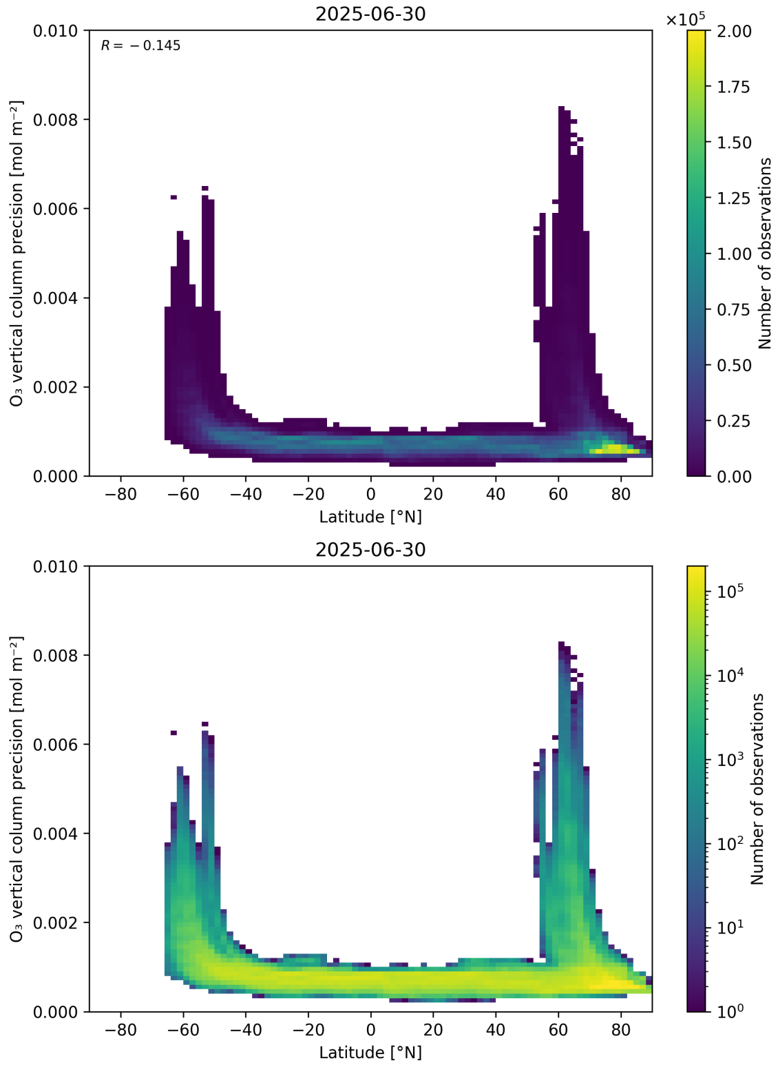
Figure 37: Scatter density plot of “Latitude” against “O 3 vertical column precision” for 2025-06-29 to 2025-07-01.
