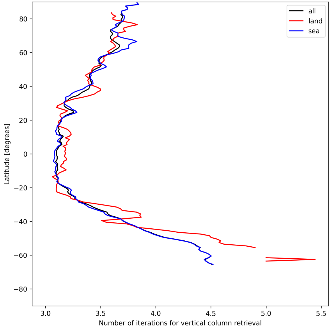
Figure 19: Zonal average of “Number of iterations for vertical column retrieval” for 2025-06-29 to 2025-07-01.
