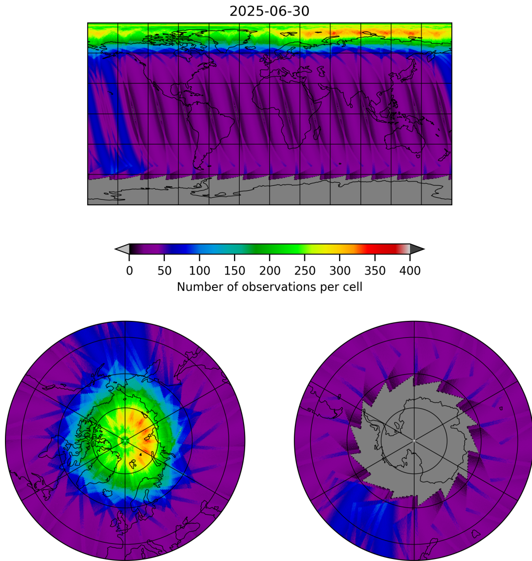
Figure 12: Map of the number of observations for 2025-06-29 to 2025-07-01
