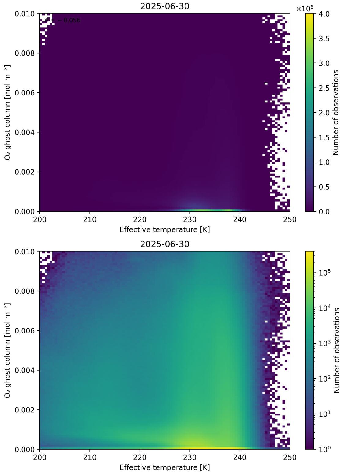
Figure 38: Scatter density plot of “Effective temperature” against “O 3 ghost column” for 2025-06-29 to 2025-07-01.
