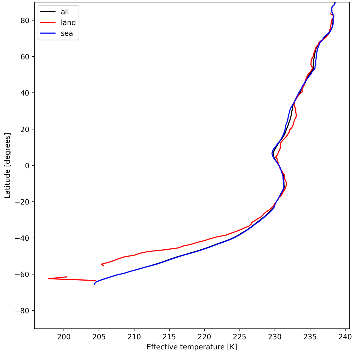
Figure 17: Zonal average of "Effective temperature" for 2025-06-29 to 2025-07-01.
