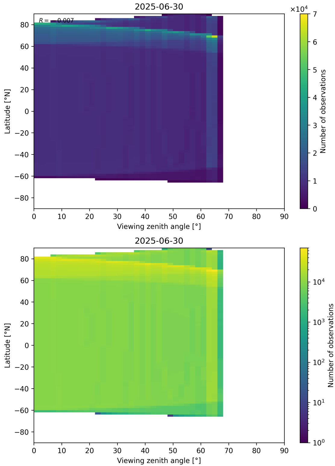
Figure 49: Scatter density plot of “Viewing zenith angle” against “Latitude” for 2025-06-29 to 2025-07-01.
