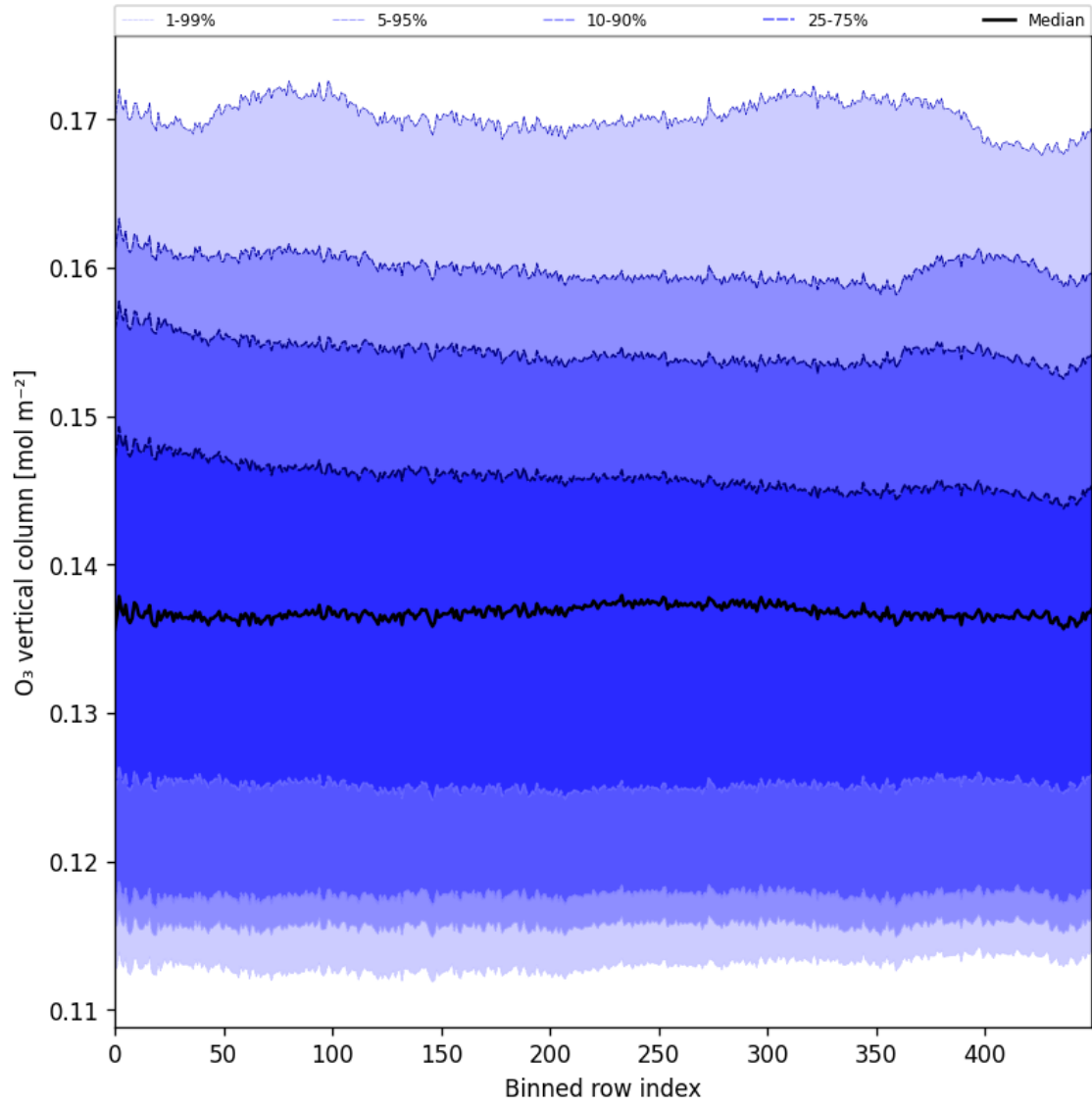
Figure 28: Along track statistics of “O 3 vertical column” for 2025-06-29 to 2025-07-01
