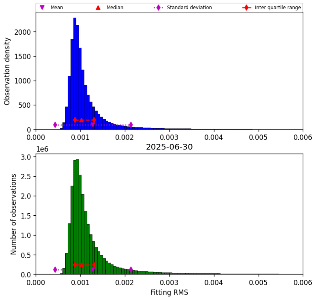
Figure 23: Histogram of “Fitting RMS” for 2025-06-29 to 2025-07-01
