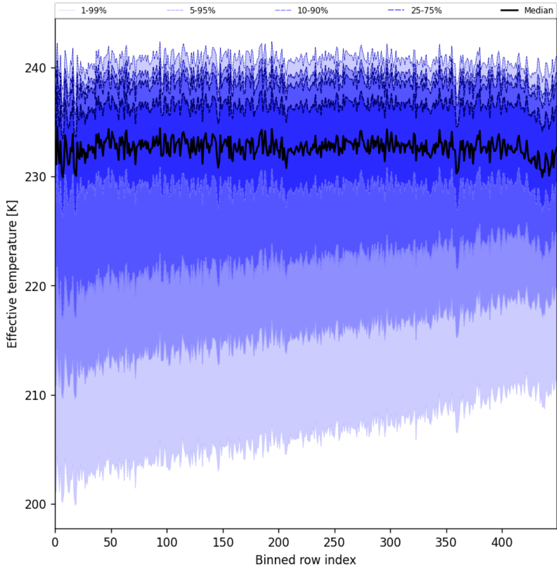
Figure 31: Along track statistics of “Effective temperature” for 2025-06-29 to 2025-07-01
