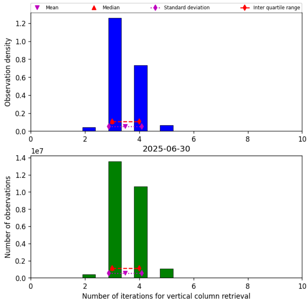
Figure 26: Histogram of “Number of iterations for vertical column retrieval” for 2025-06-29 to 2025-07-01
