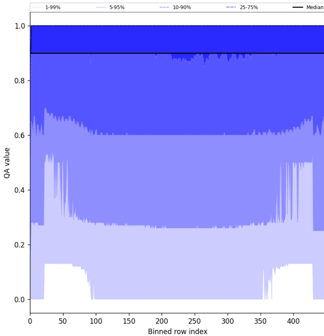
Figure 27: Along track statistics of “QA value” for 2025-06-29 to 2025-07-01
