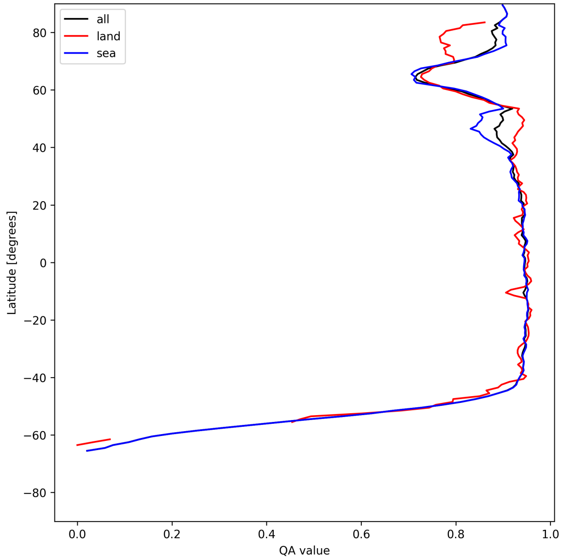
Figure 13: Zonal average of “QA value” for 2025-06-29 to 2025-07-01.
