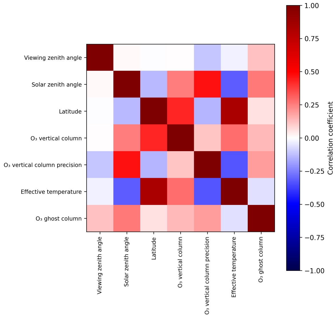
Figure 2: Map of correlation matrix for 2025-06-29 to 2025-07-01.
