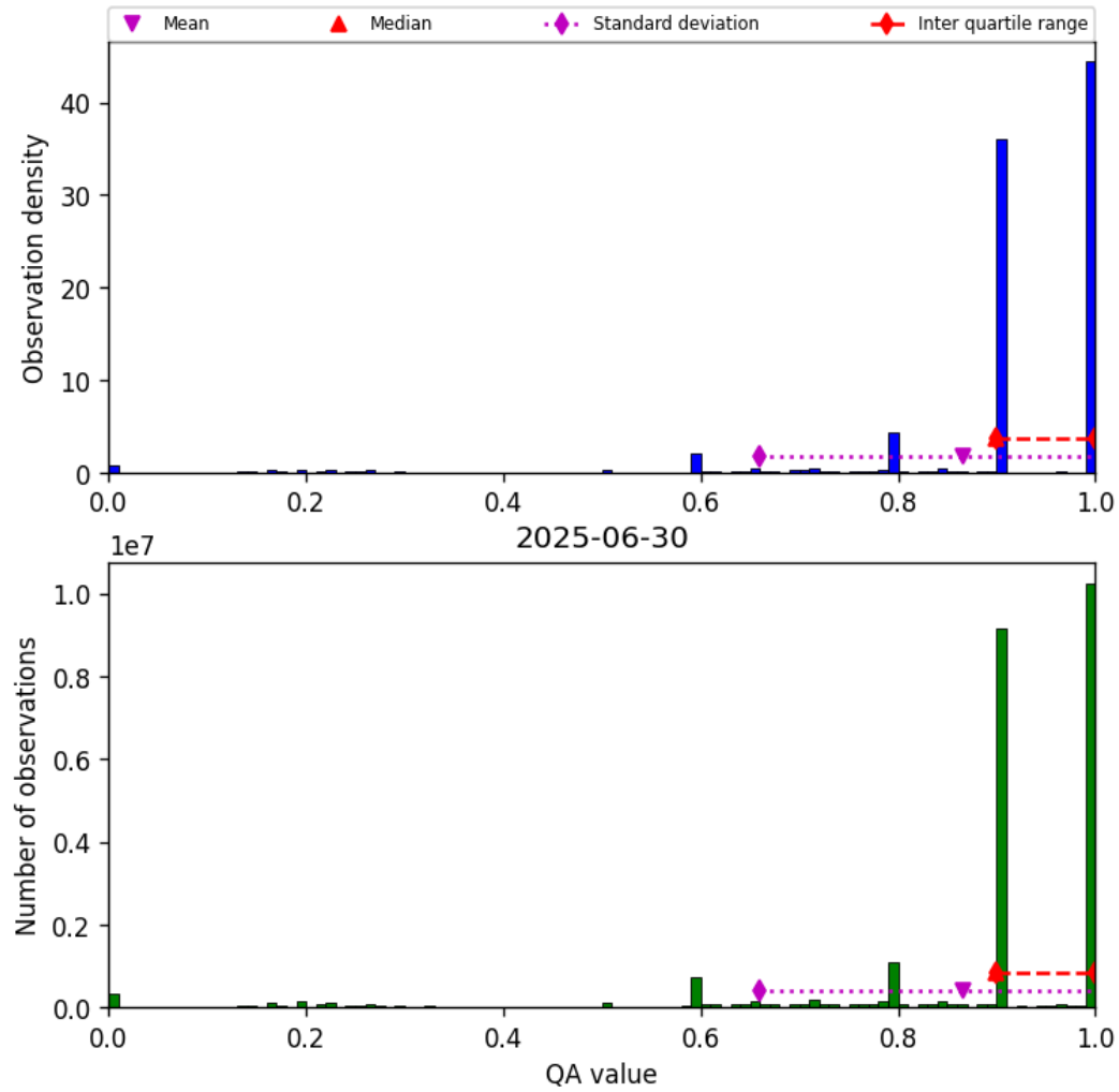
Figure 20: Histogram of “QA value” for 2025-06-29 to 2025-07-01
