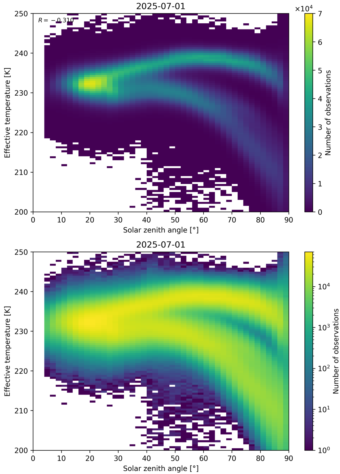
Figure 45: Scatter density plot of “Solar zenith angle” against “Effective temperature” for 2025-06-30 to 2025-07-02.
