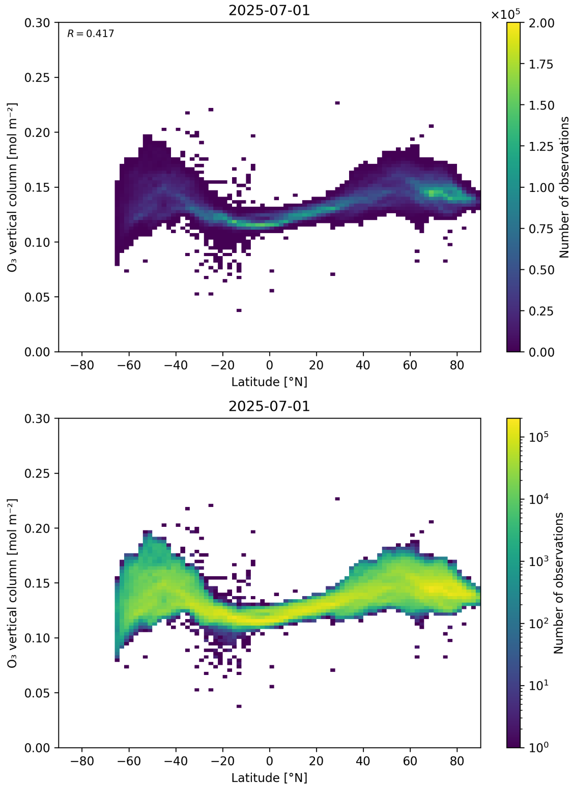
Figure 36: Scatter density plot of “Latitude” against “O 3 vertical column” for 2025-06-30 to 2025-07-02.
