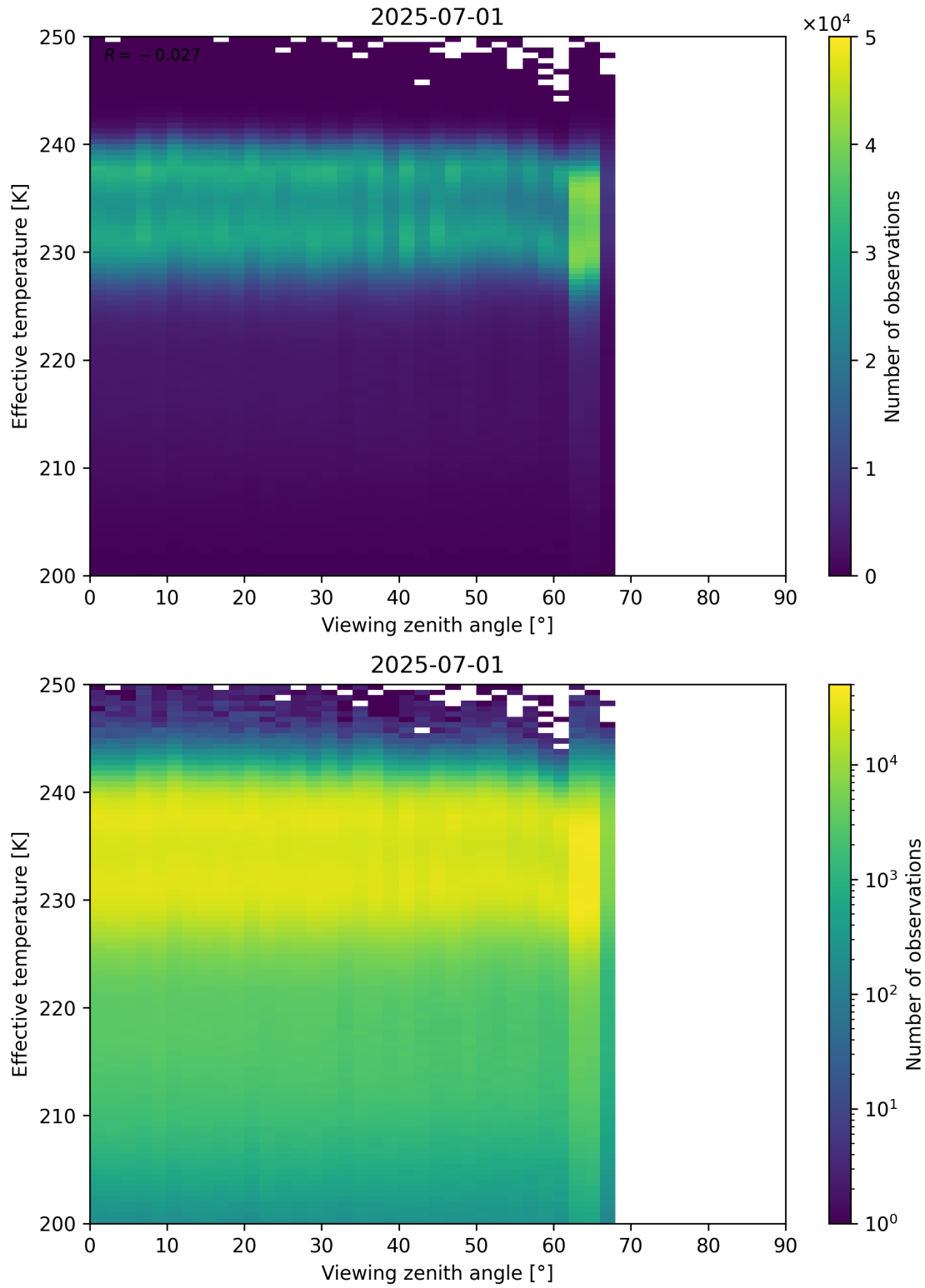
Figure 50: Scatter density plot of “Viewing zenith angle” against “Effective temperature” for 2025-06-30 to 2025-07-02.
