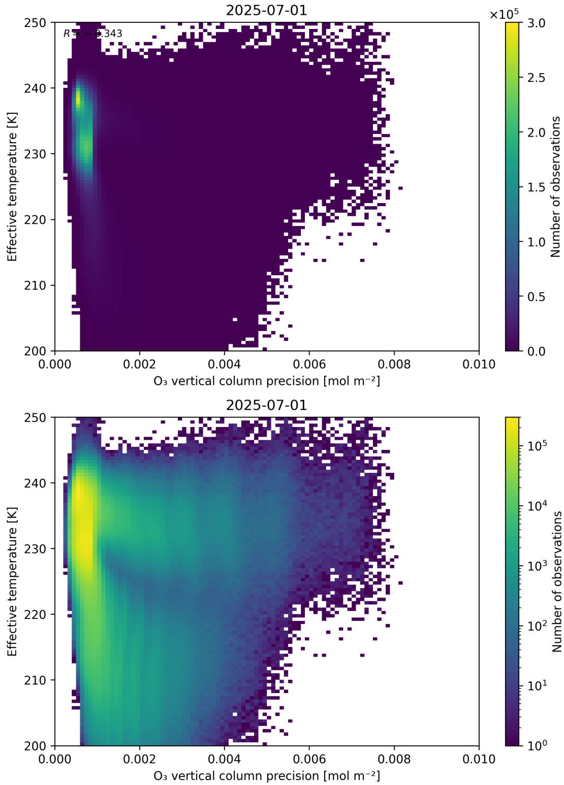
Figure 42: Scatter density plot of “O 3 vertical column precision” against “Effective temperature” for 2025-06-30 to 2025-07-02.
