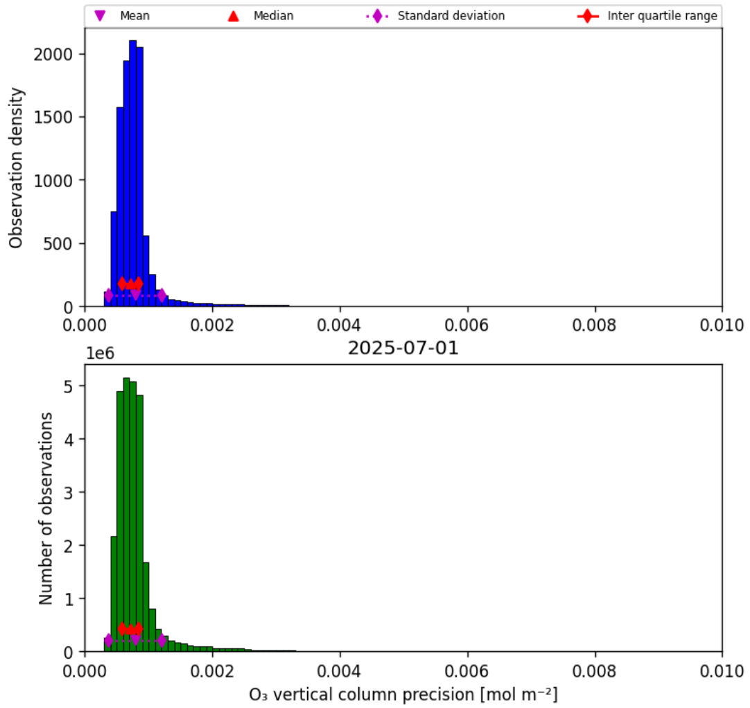
Figure 22: Histogram of “O 3 vertical column precision” for 2025-06-30 to 2025-07-02
