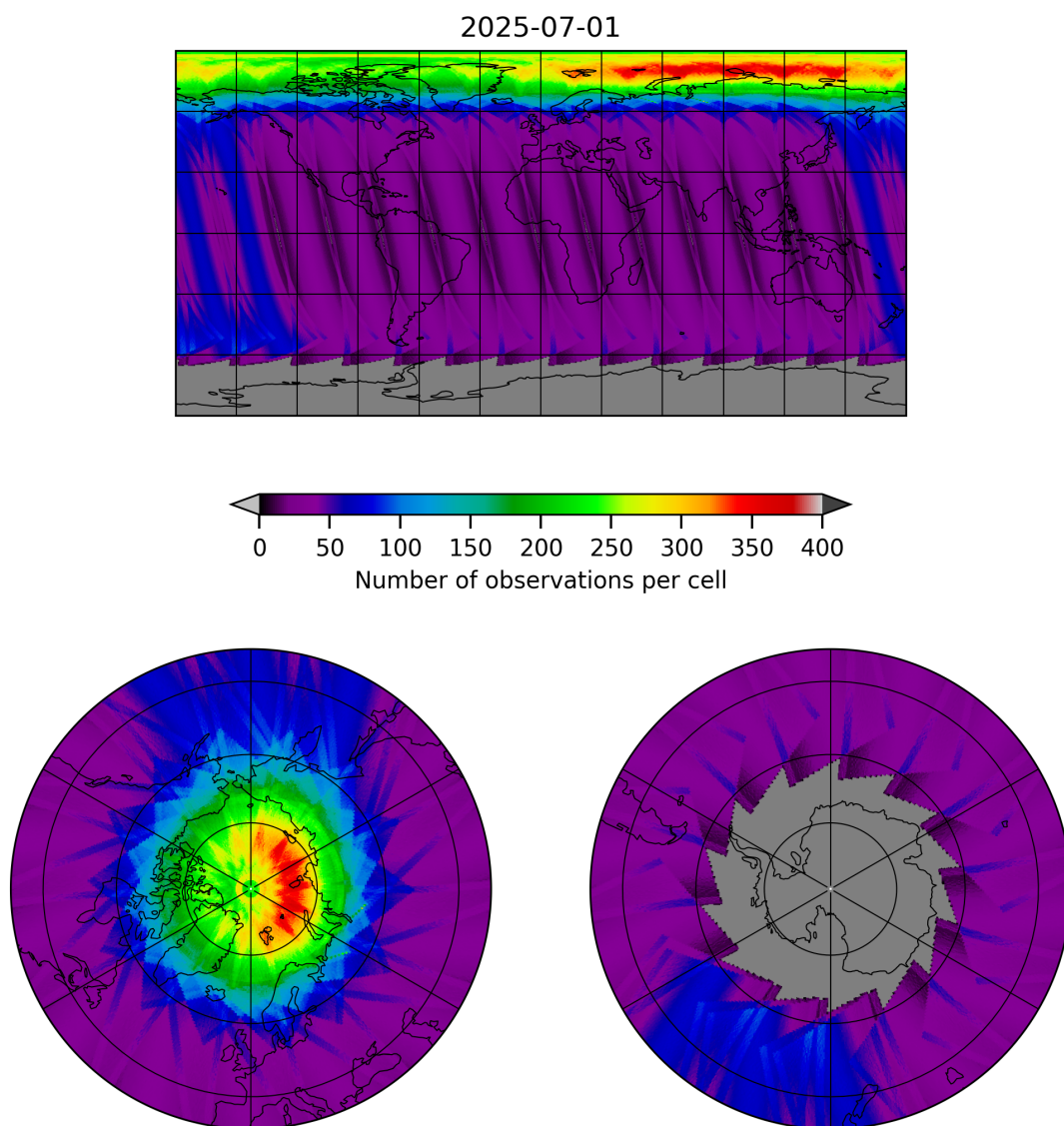
Figure 12: Map of the number of observations for 2025-06-30 to 2025-07-02
