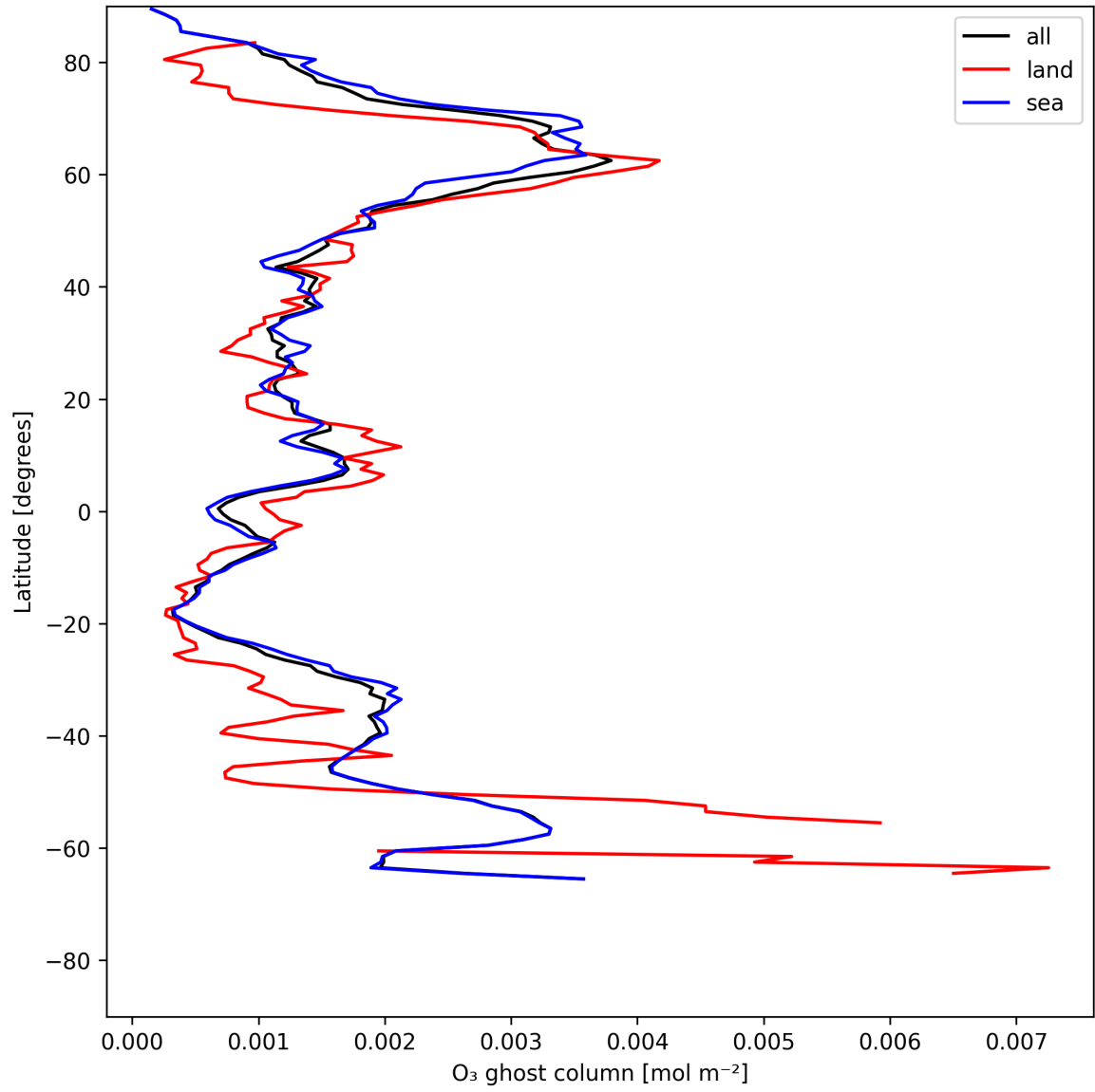
Figure 18: Zonal average of “O 3 ghost column” for 2025-06-30 to 2025-07-02.
