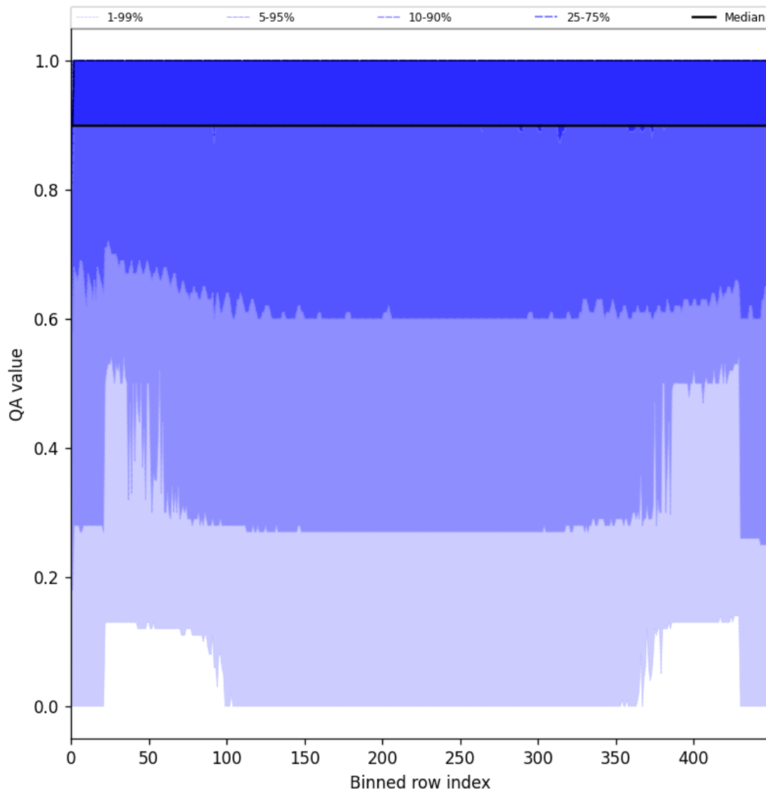
Figure 27: Along track statistics of “QA value” for 2025-06-30 to 2025-07-02
