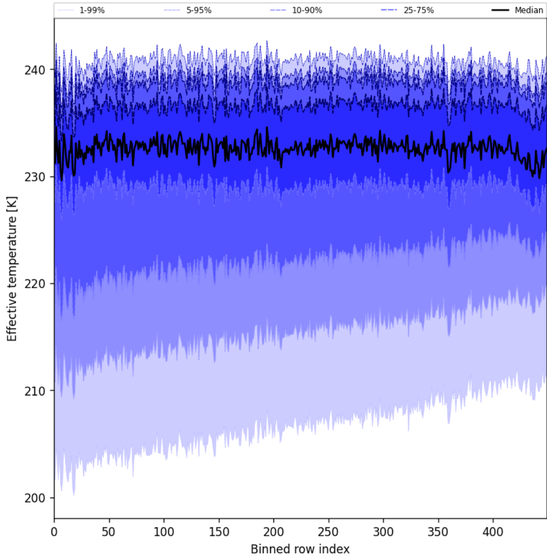
Figure 31: Along track statistics of “Effective temperature” for 2025-06-30 to 2025-07-02
