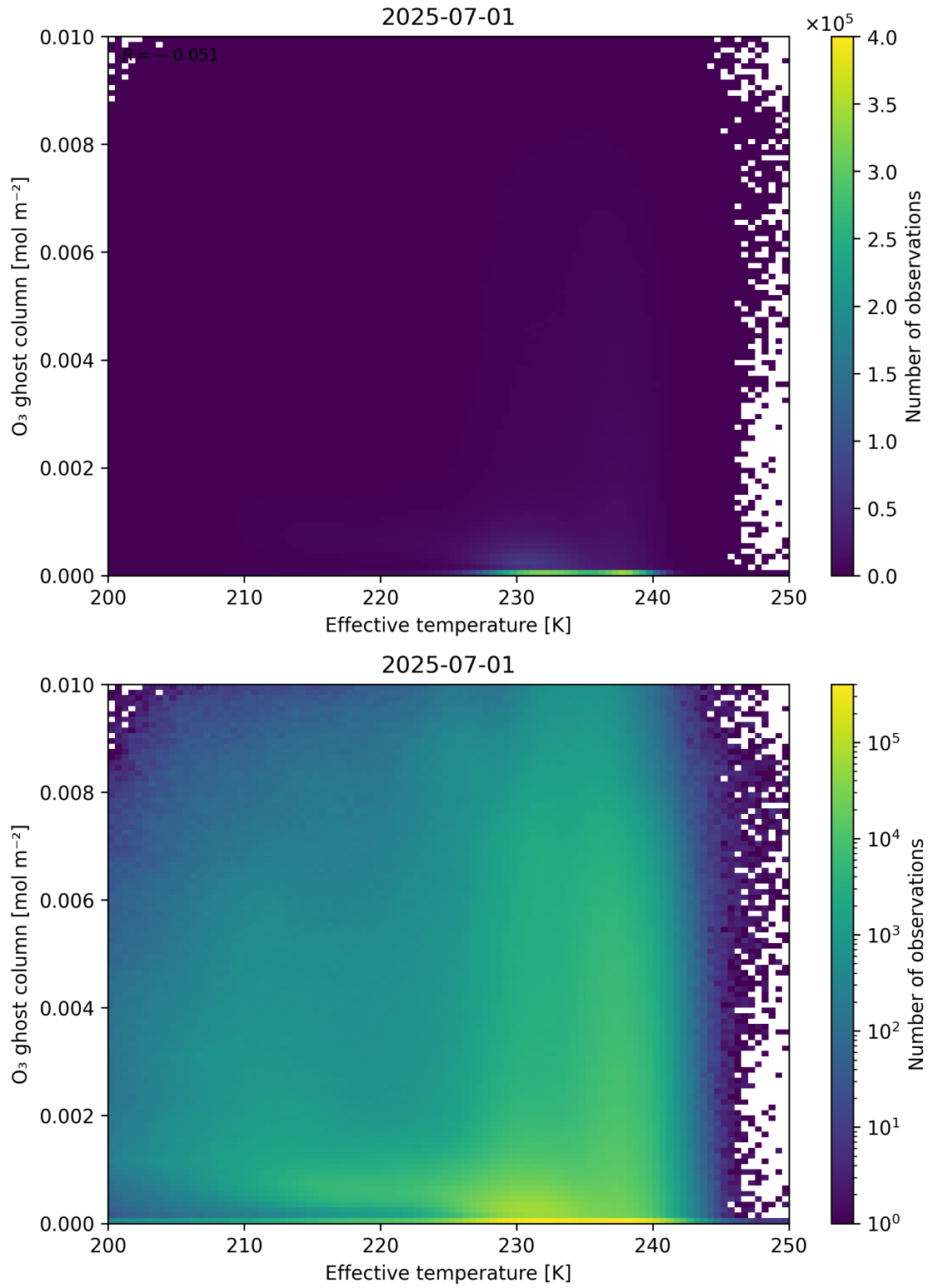
Figure 38: Scatter density plot of “Effective temperature” against “O 3 ghost column” for 2025-06-30 to 2025-07-02.
