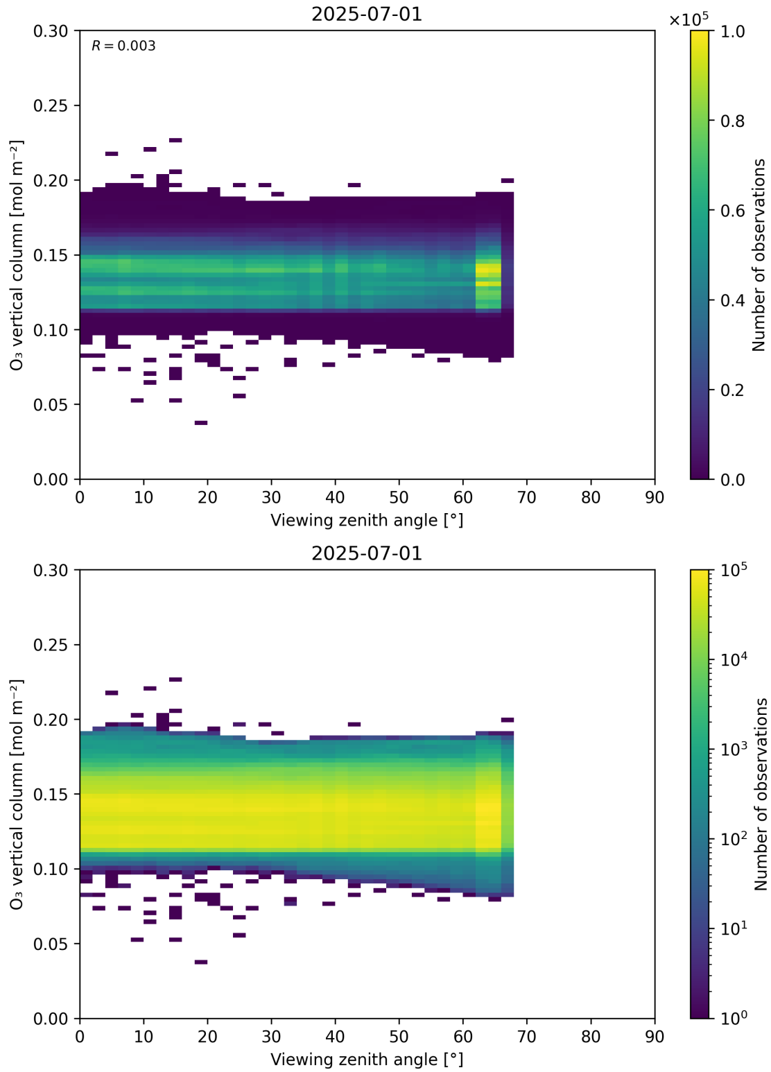
Figure 52: Scatter density plot of “Viewing zenith angle” against “O 3 vertical column” for 2025-06-30 to 2025-07-02.
