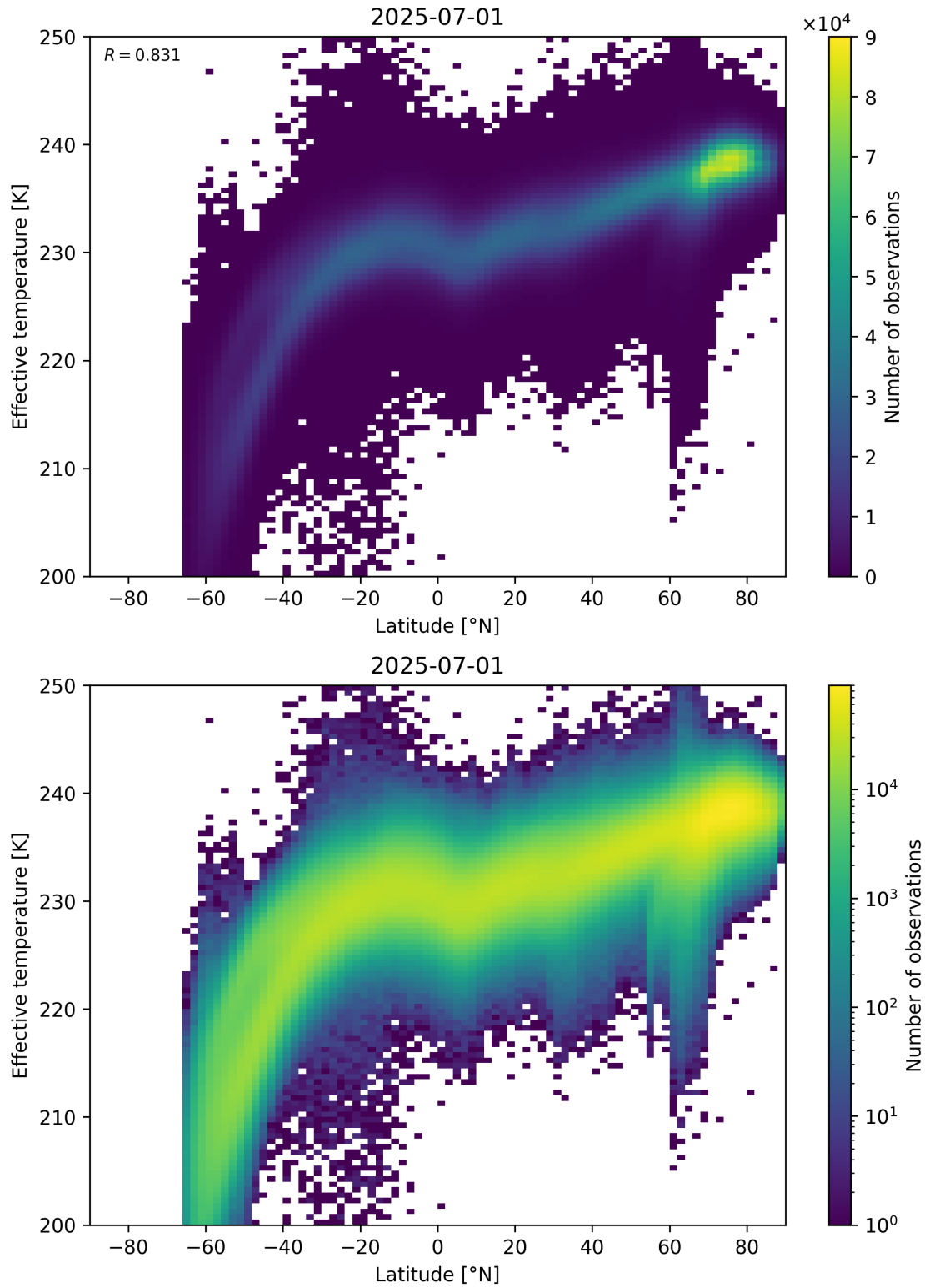
Figure 34: Scatter density plot of “Latitude” against “Effective temperature” for 2025-06-30 to 2025-07-02.
