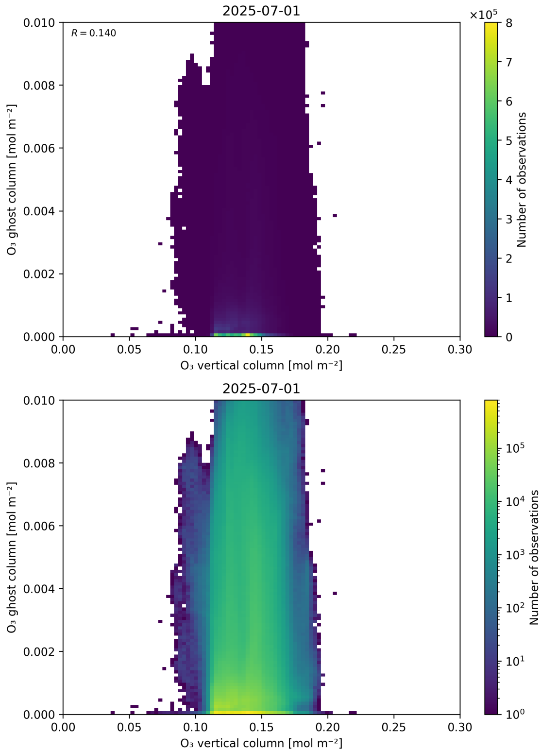
Figure 40: Scatter density plot of “O 3 vertical column” against “O 3 ghost column” for 2025-06-30 to 2025-07-02.
