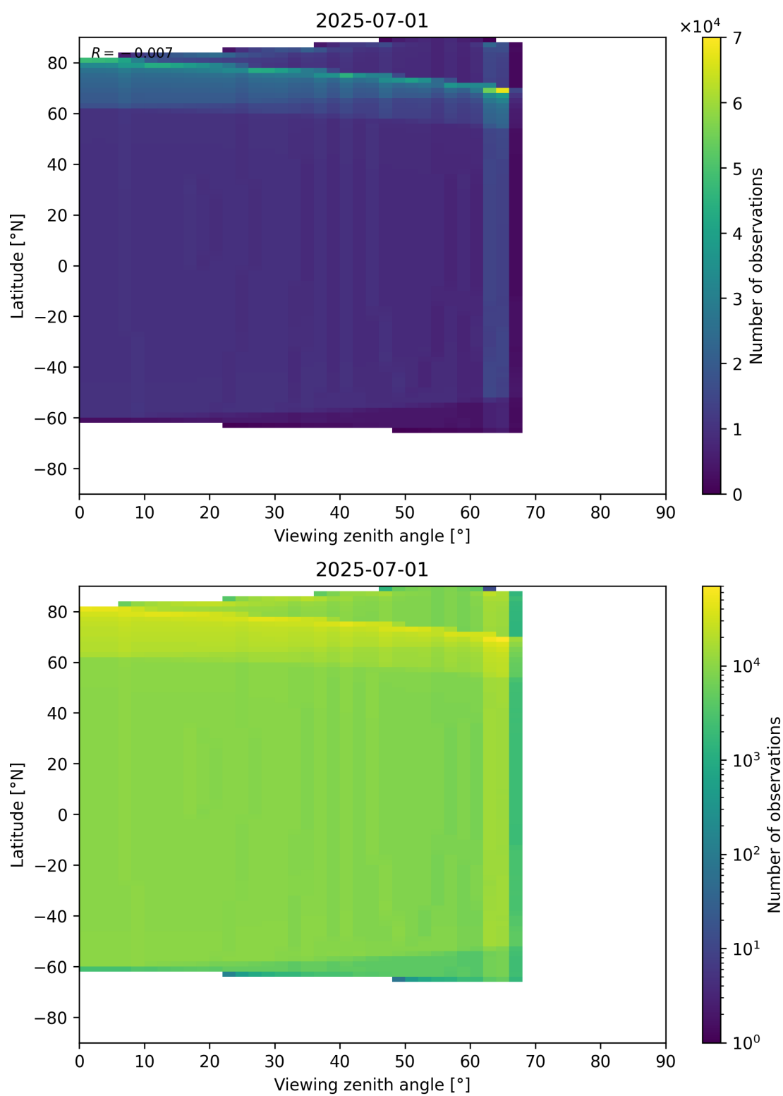
Figure 49: Scatter density plot of “Viewing zenith angle” against “Latitude” for 2025-06-30 to 2025-07-02.
