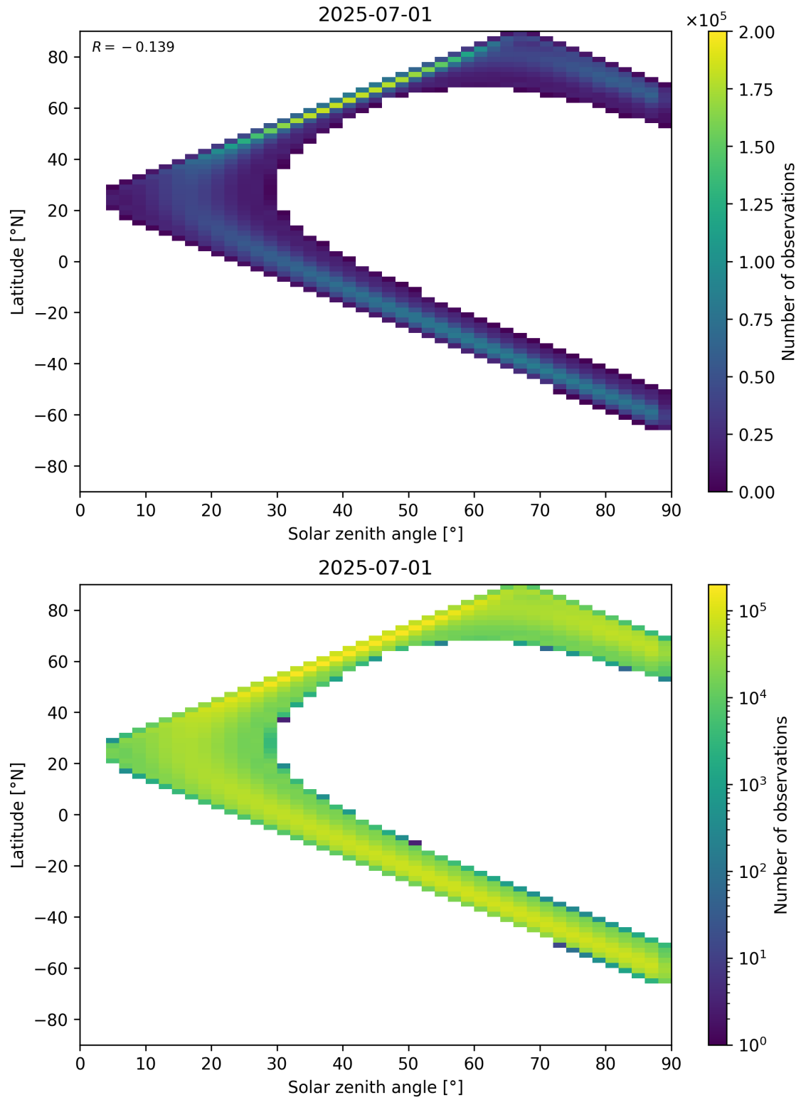
Figure 44: Scatter density plot of “Solar zenith angle” against “Latitude” for 2025-06-30 to 2025-07-02.
