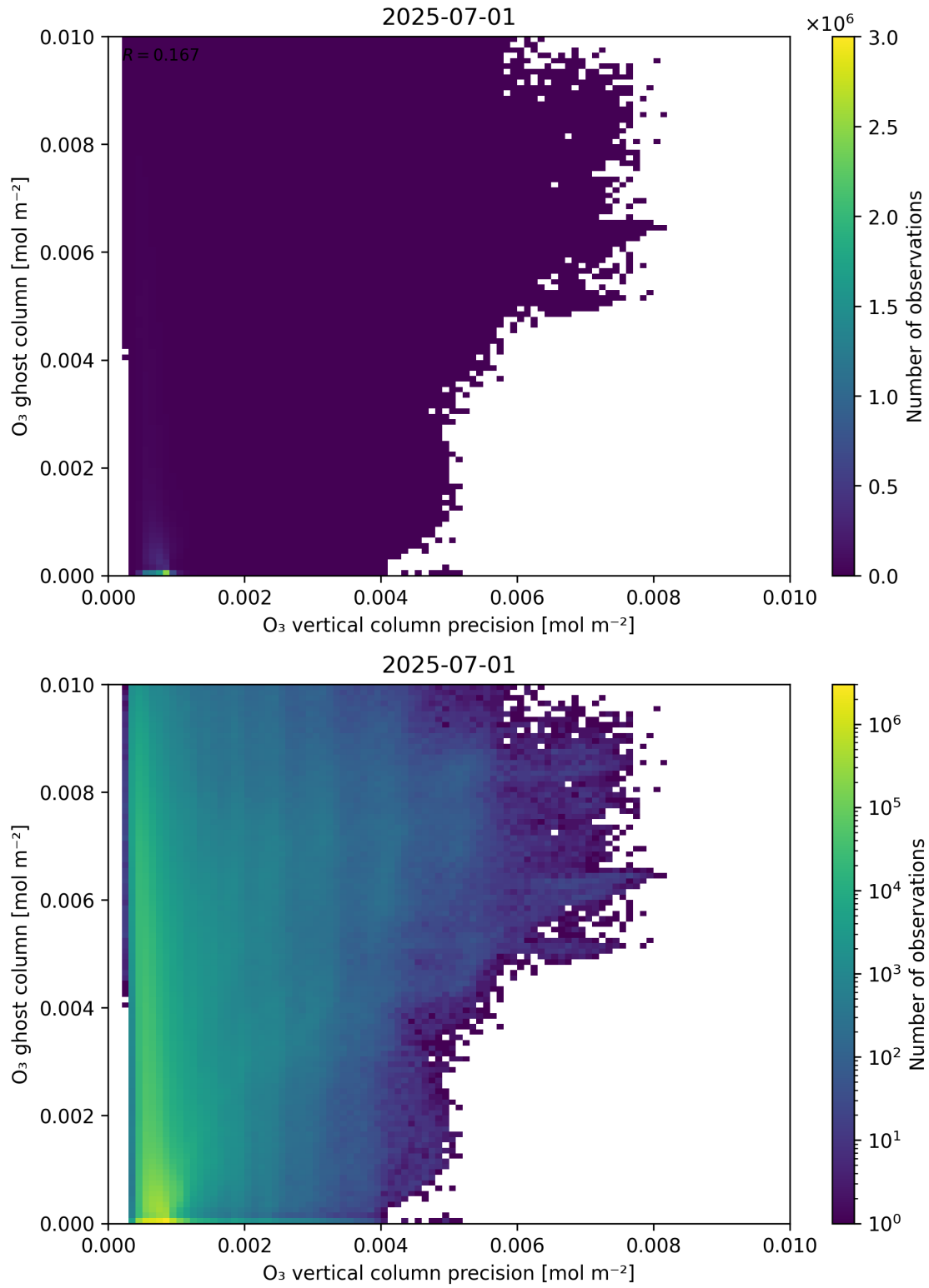
Figure 43: Scatter density plot of “ \text{O}_3 vertical column precision” against “ \text{O}_3 ghost column” for 2025-06-30 to 2025-07-02.
