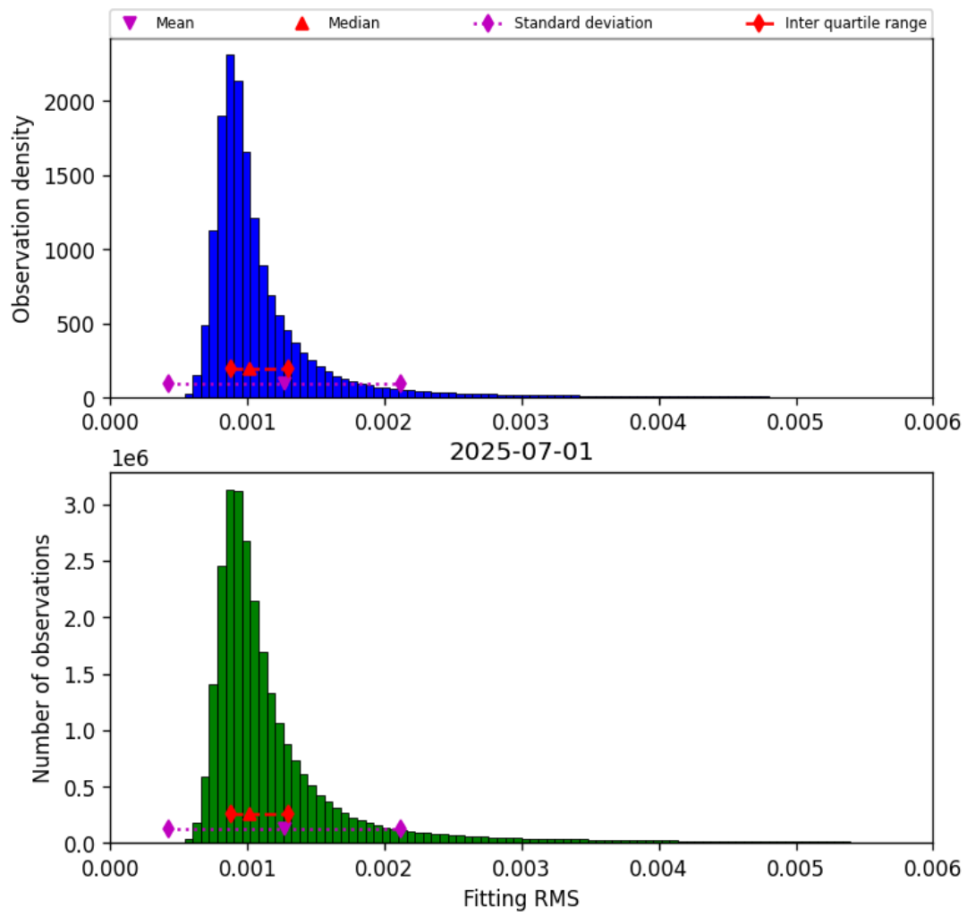
Figure 23: Histogram of “Fitting RMS” for 2025-06-30 to 2025-07-02
