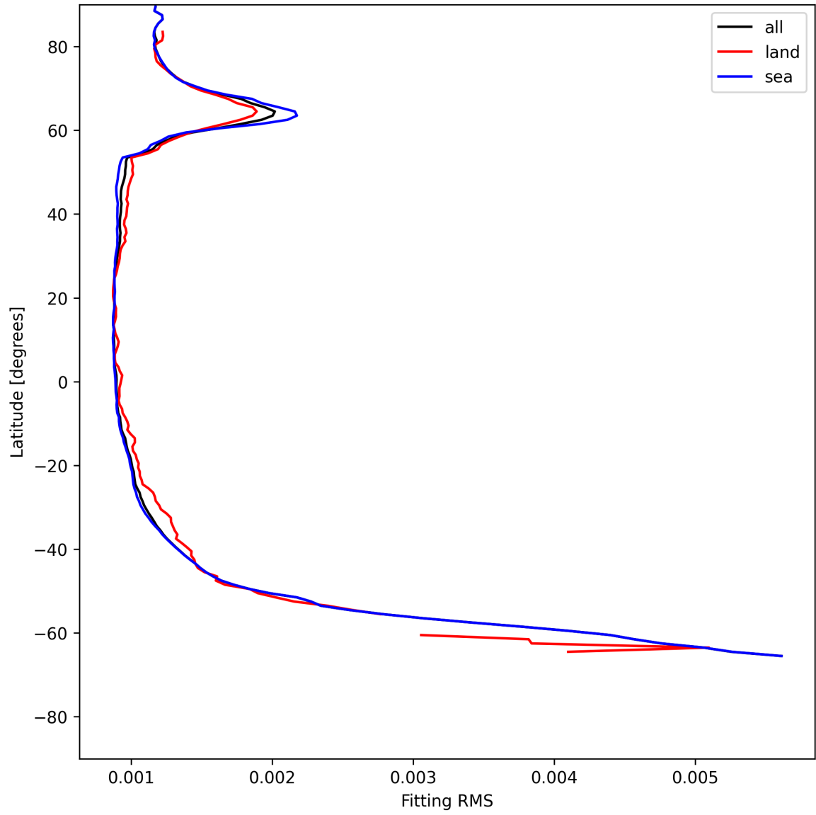
Figure 16: Zonal average of “Fitting RMS” for 2025-06-30 to 2025-07-02.
