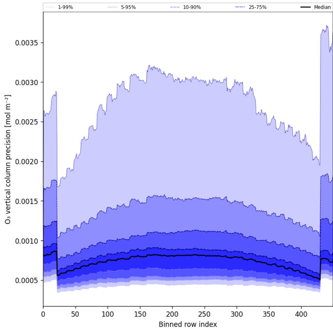
Figure 29: Along track statistics of “O 3 vertical column precision” for 2025-06-30 to 2025-07-02
