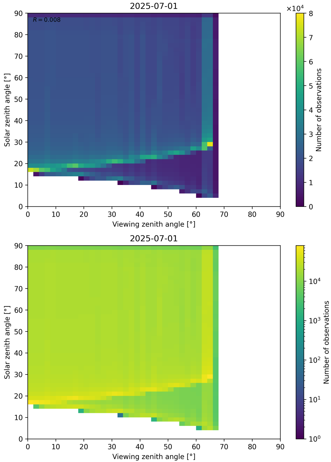
Figure 54: Scatter density plot of “Viewing zenith angle” against “Solar zenith angle” for 2025-06-30 to 2025-07-02.
