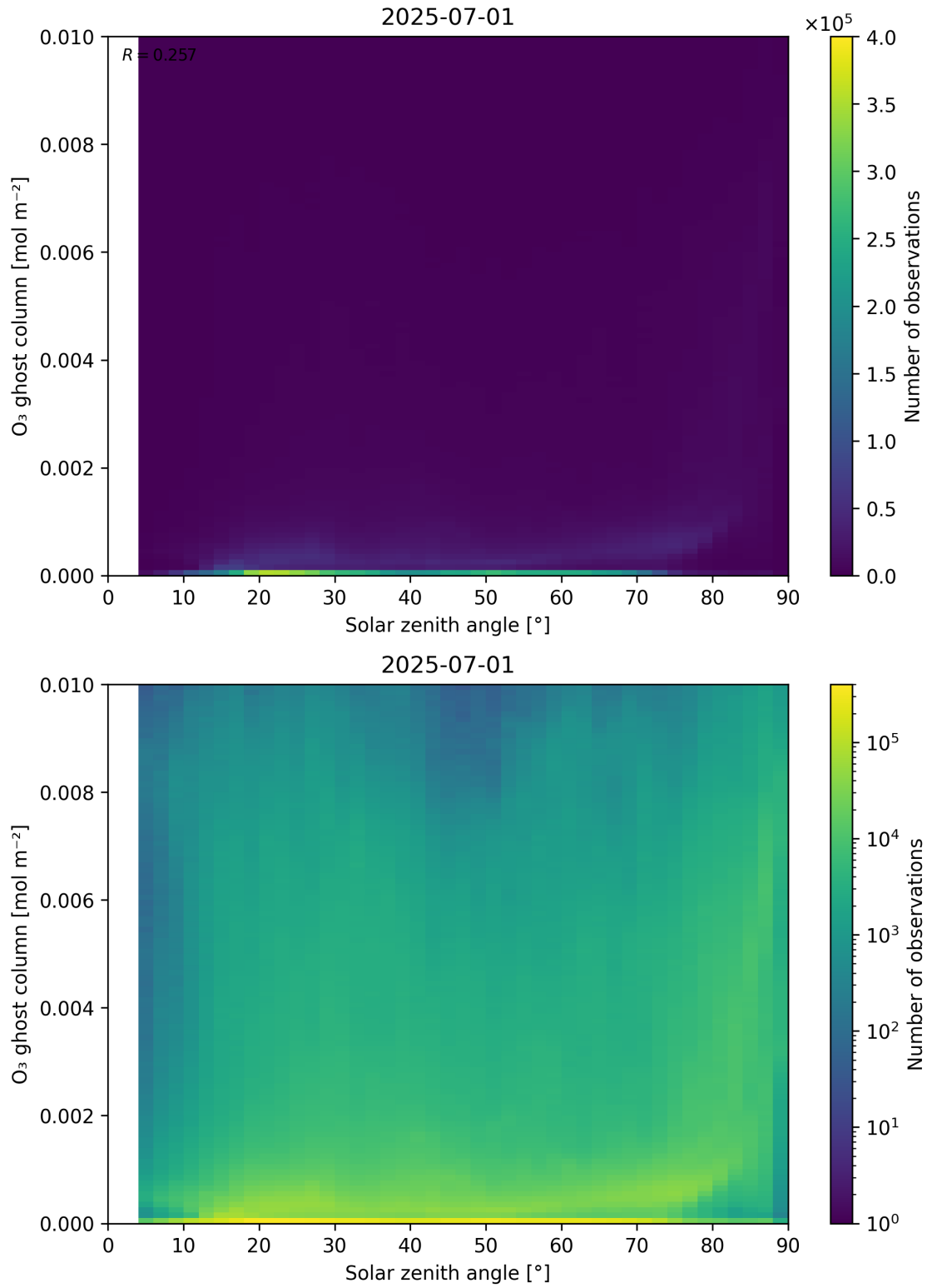
Figure 46: Scatter density plot of “Solar zenith angle” against “O 3 ghost column” for 2025-06-30 to 2025-07-02.
