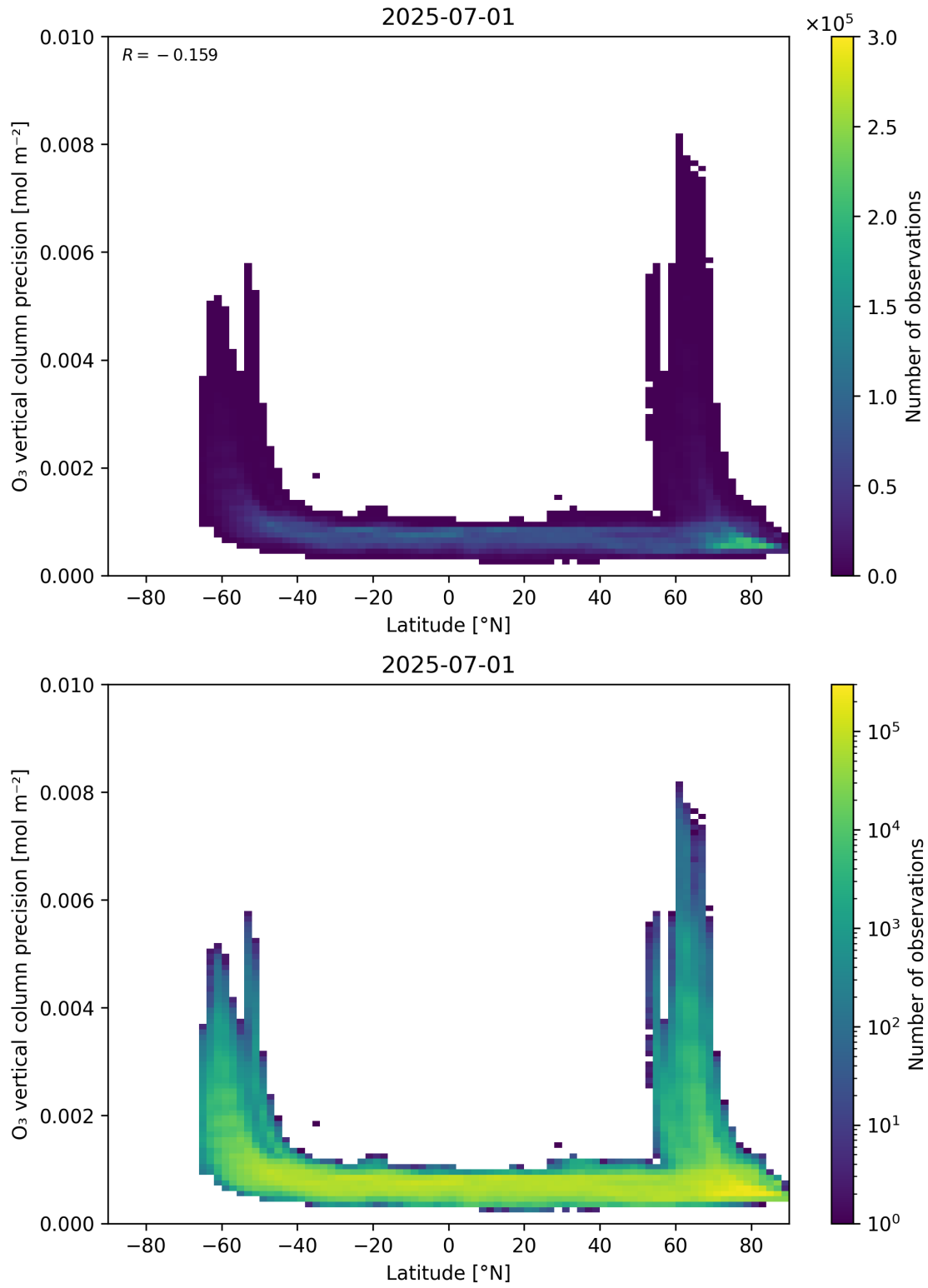
Figure 37: Scatter density plot of “Latitude” against “O 3 vertical column precision” for 2025-06-30 to 2025-07-02.
