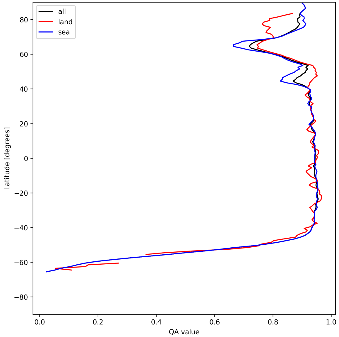
Figure 13: Zonal average of “QA value” for 2025-06-30 to 2025-07-02.
