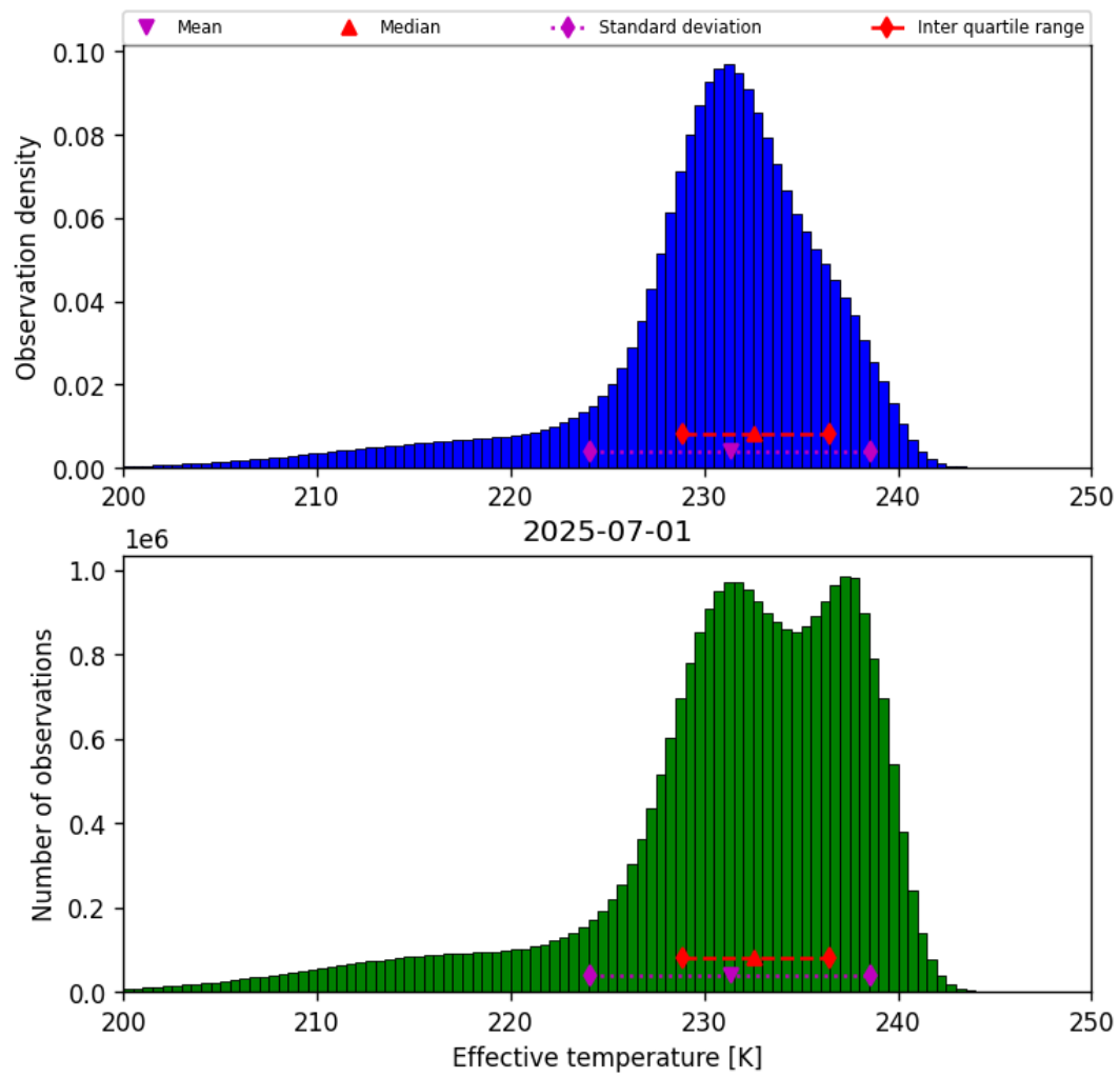
Figure 24: Histogram of “Effective temperature” for 2025-06-30 to 2025-07-02
