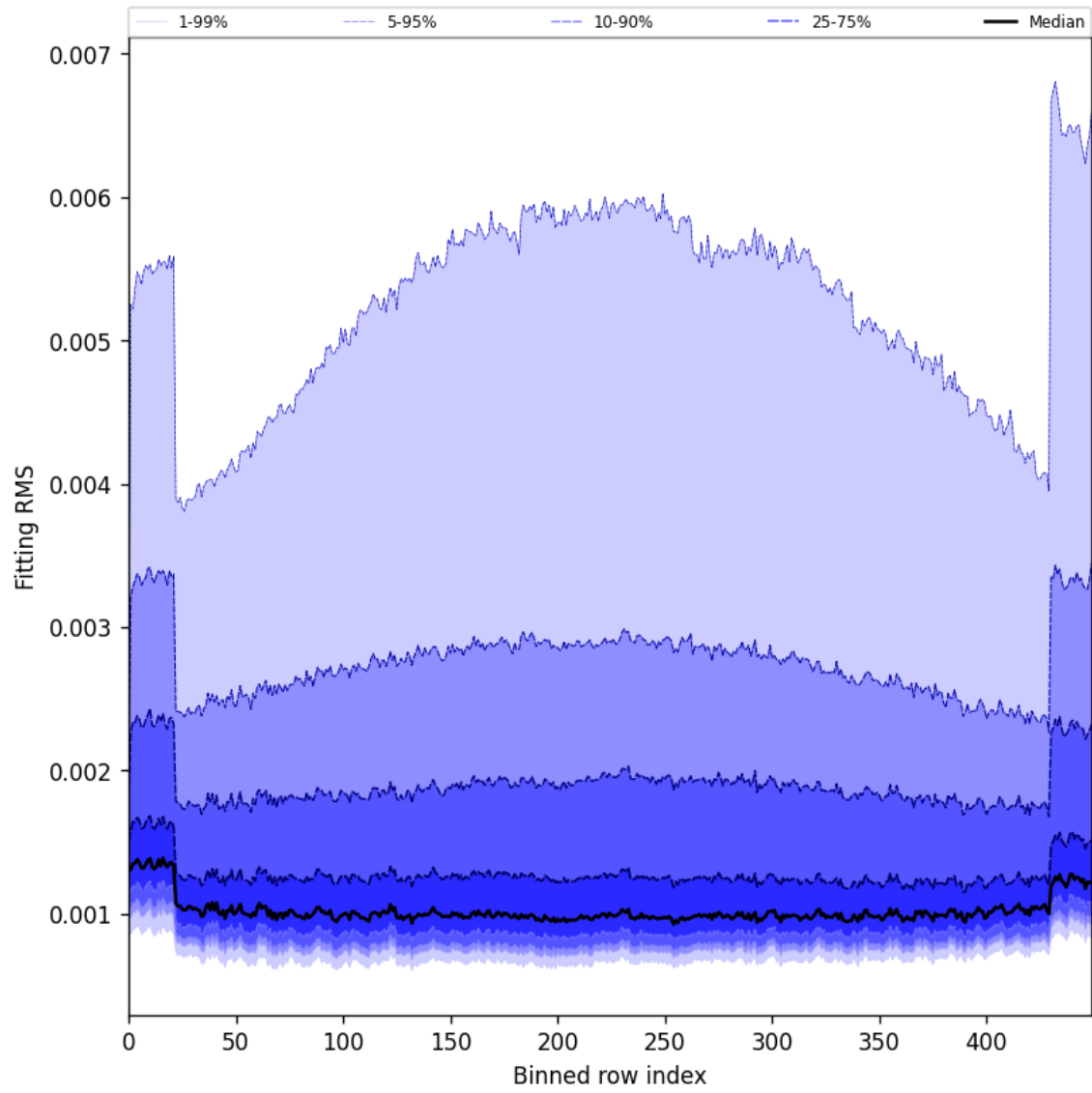
Figure 30: Along track statistics of “Fitting RMS” for 2025-06-30 to 2025-07-02
