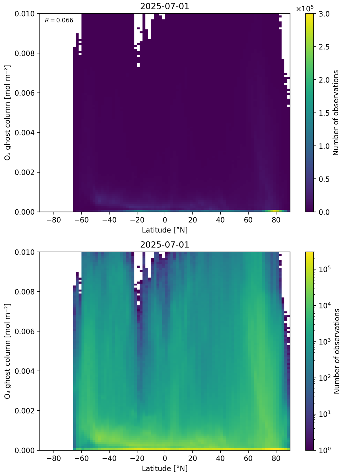
Figure 35: Scatter density plot of “Latitude” against “O 3 ghost column” for 2025-06-30 to 2025-07-02.
