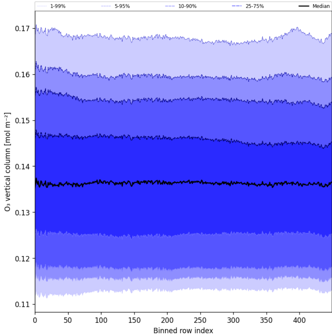
Figure 28: Along track statistics of “ O_3 vertical column” for 2025-06-30 to 2025-07-02
