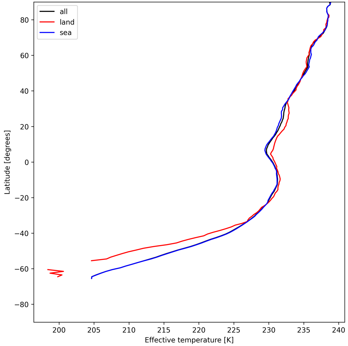
Figure 17: Zonal average of "Effective temperature" for 2025-06-30 to 2025-07-02.
