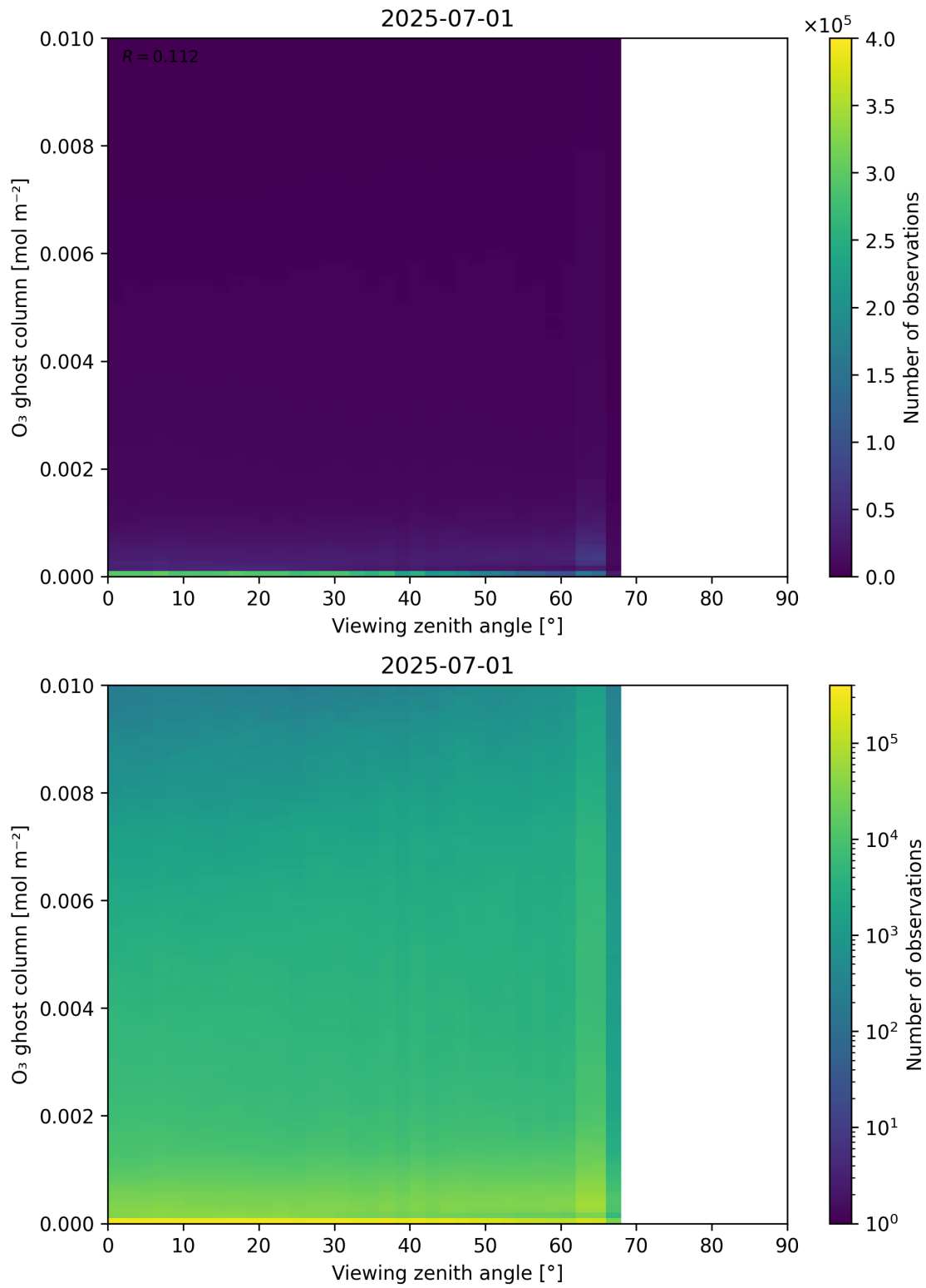
Figure 51: Scatter density plot of “Viewing zenith angle” against “O 3 ghost column” for 2025-06-30 to 2025-07-02.
