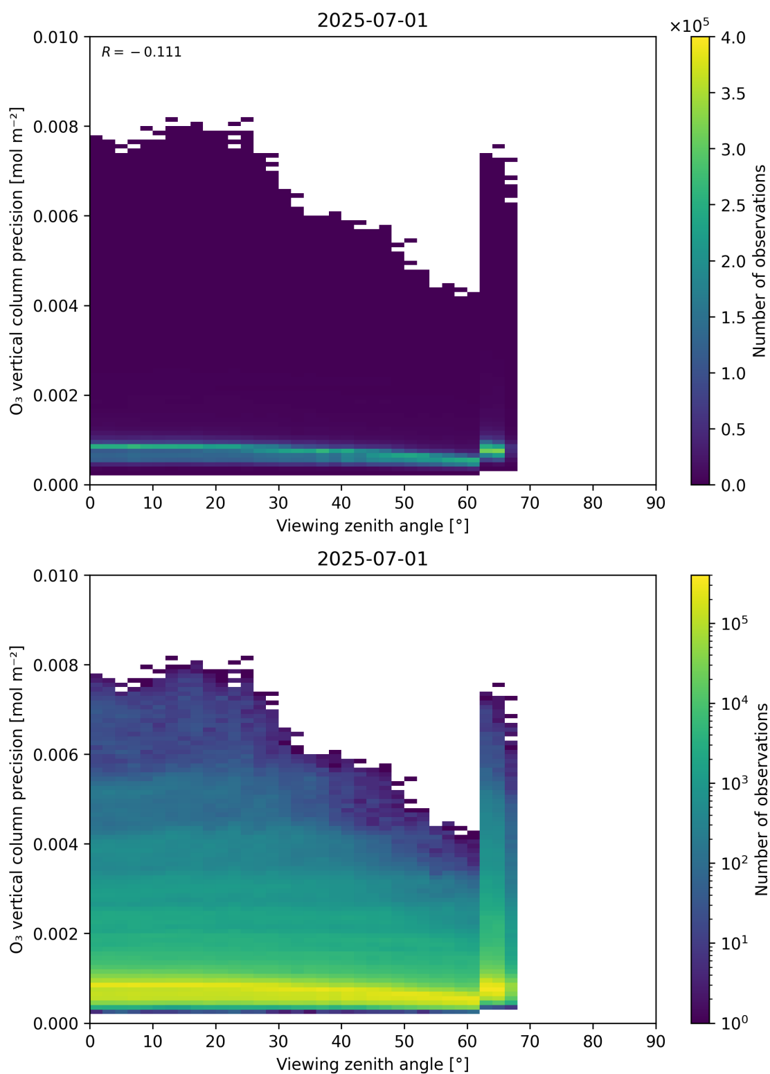
Figure 53: Scatter density plot of “Viewing zenith angle” against “O 3 vertical column precision” for 2025-06-30 to 2025-07-02.
