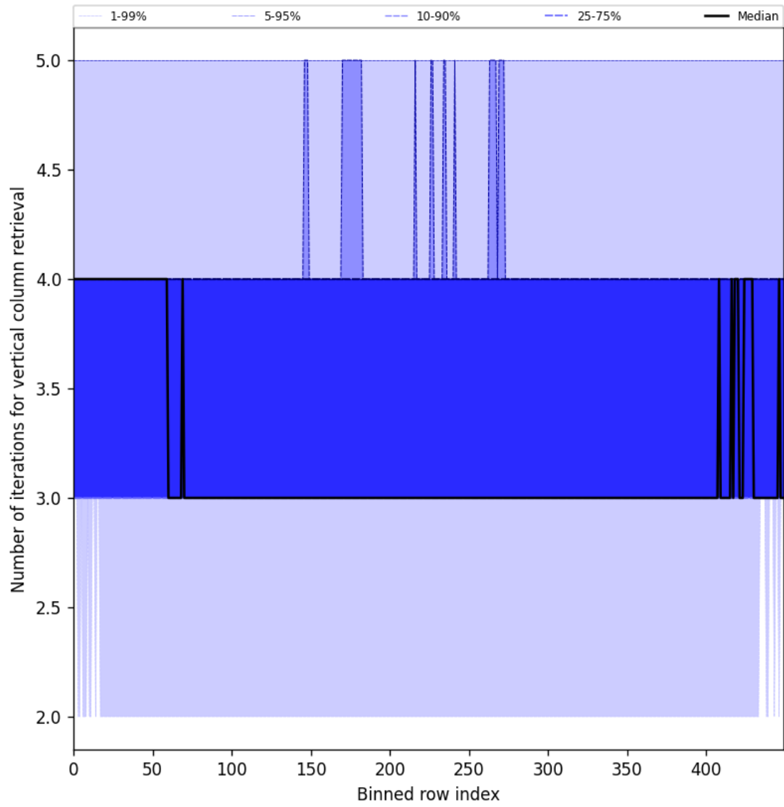
Figure 33: Along track statistics of “Number of iterations for vertical column retrieval” for 2025-06-30 to 2025-07-02
