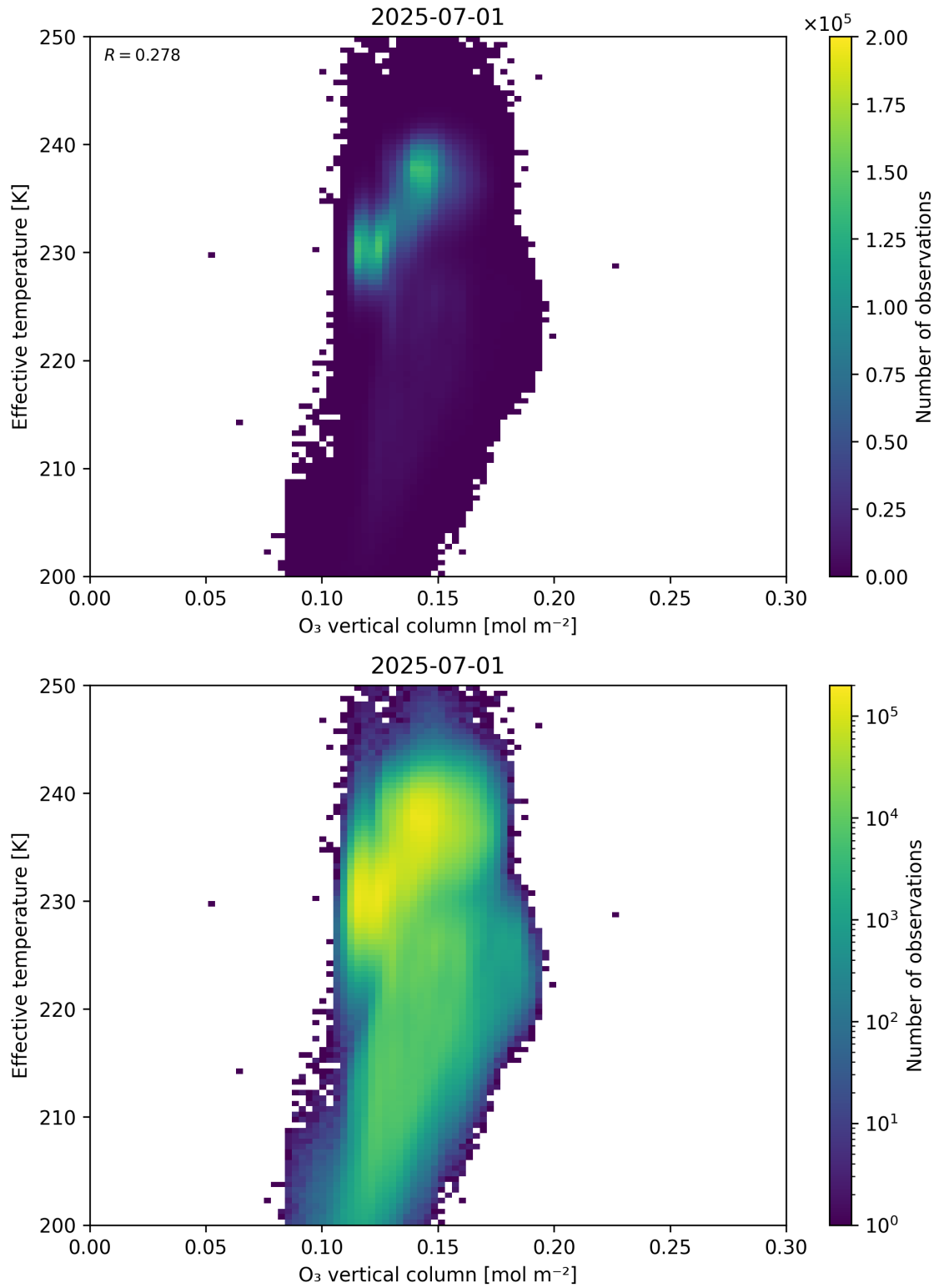
Figure 39: Scatter density plot of “O 3 vertical column” against “Effective temperature” for 2025-06-30 to 2025-07-02.
