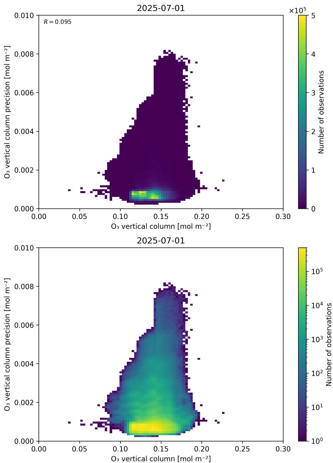
Figure 41: Scatter density plot of “O 3 vertical column” against “O 3 vertical column precision” for 2025-06-30 to 2025-07-02.
