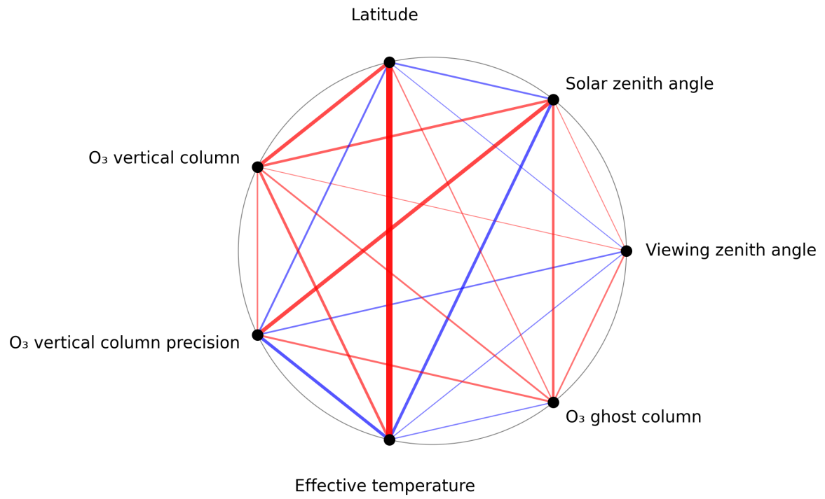
Figure 1: Map of correlation graph for 2025-06-30 to 2025-07-02.
