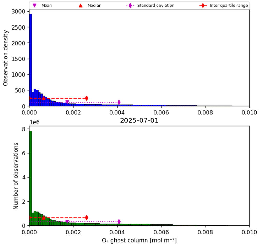
Figure 25: Histogram of “O 3 ghost column” for 2025-06-30 to 2025-07-02
