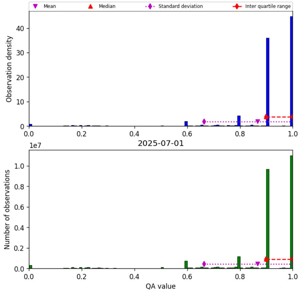
Figure 20: Histogram of “QA value” for 2025-06-30 to 2025-07-02
