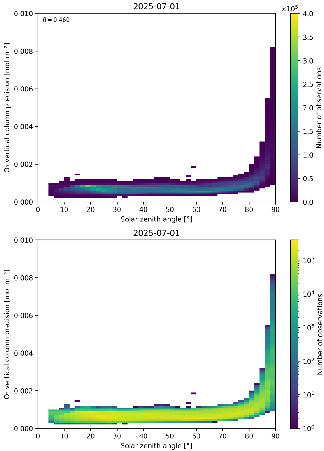
Figure 48: Scatter density plot of “Solar zenith angle” against “O 3 vertical column precision” for 2025-06-30 to 2025-07-02.
