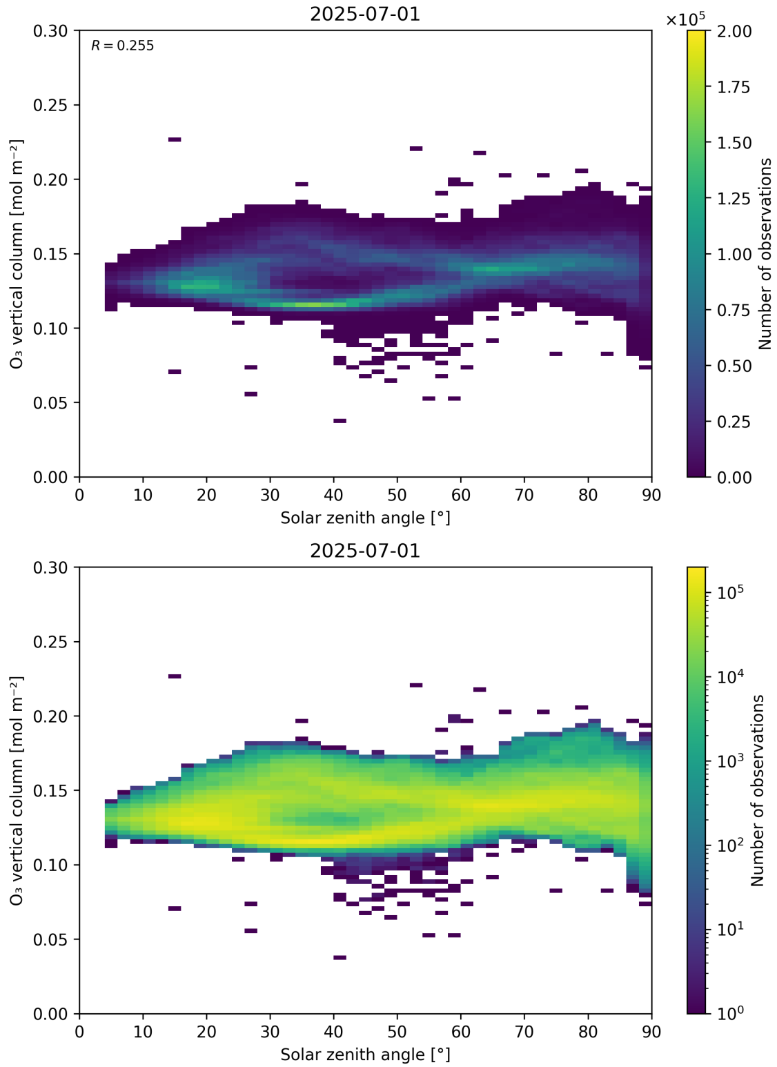
Figure 47: Scatter density plot of “Solar zenith angle” against “O 3 vertical column” for 2025-06-30 to 2025-07-02.
