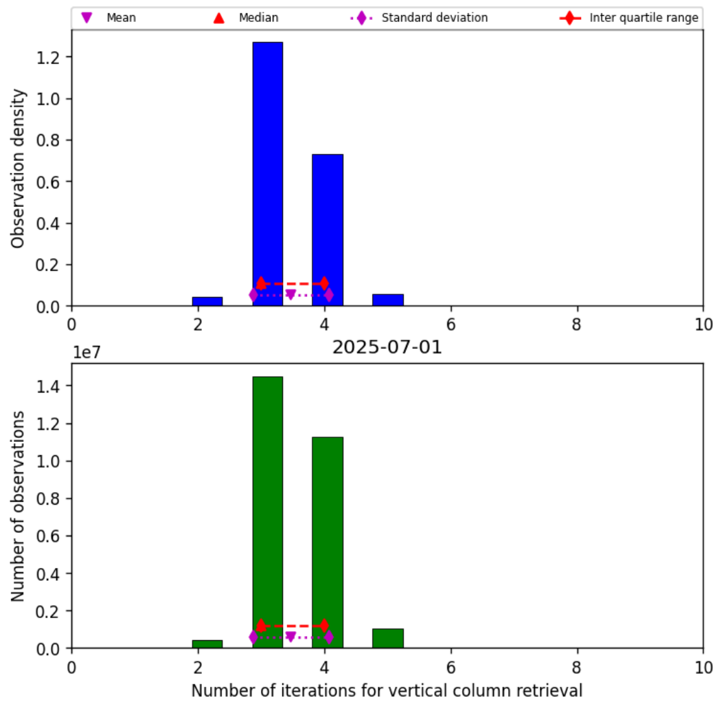
Figure 26: Histogram of “Number of iterations for vertical column retrieval” for 2025-06-30 to 2025-07-02
