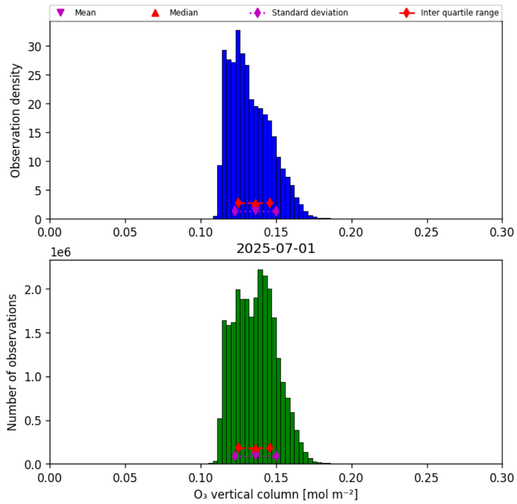
Figure 21: Histogram of “O 3 vertical column” for 2025-06-30 to 2025-07-02
