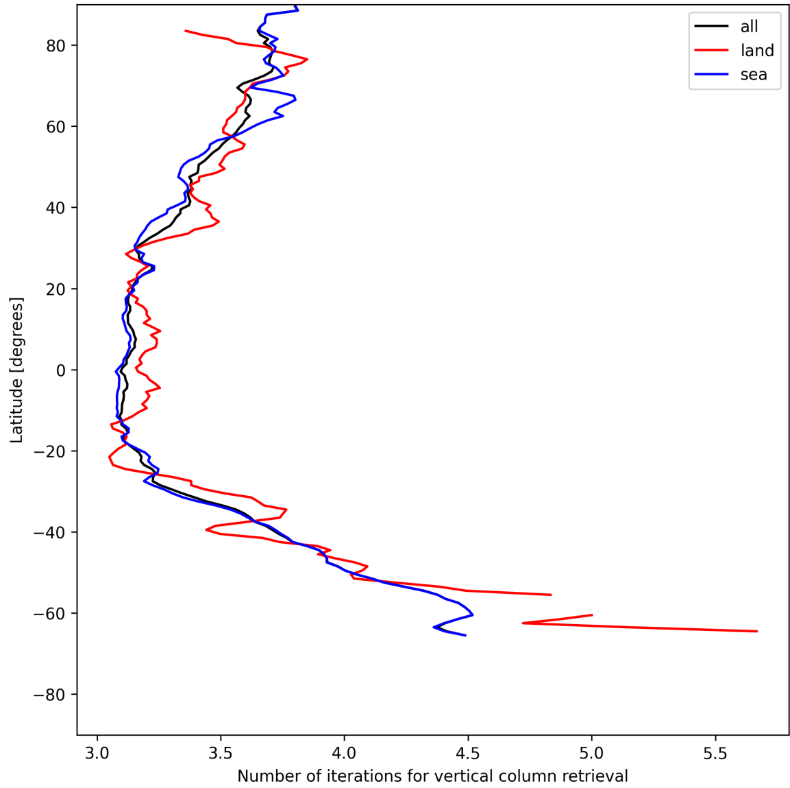
Figure 19: Zonal average of “Number of iterations for vertical column retrieval” for 2025-06-30 to 2025-07-02.
