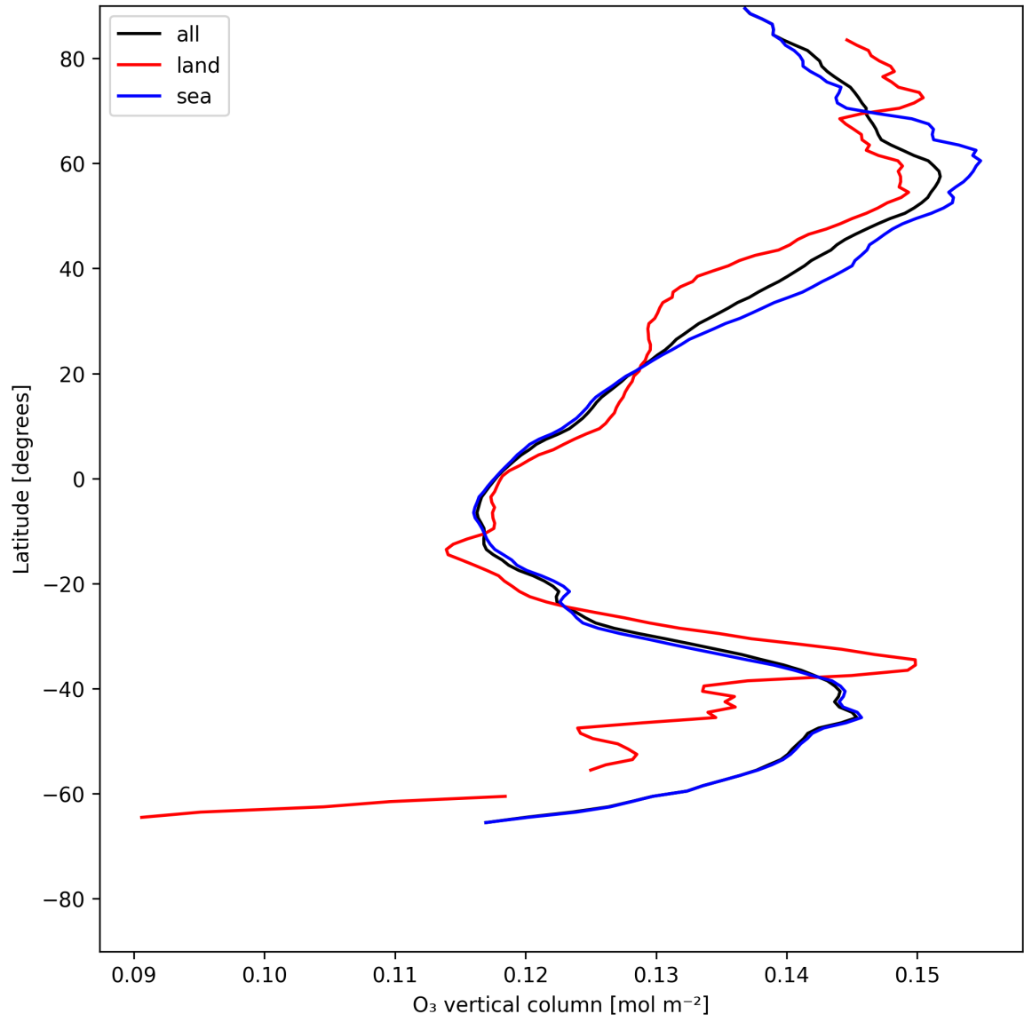
Figure 14: Zonal average of “O 3 vertical column” for 2025-06-30 to 2025-07-02.
