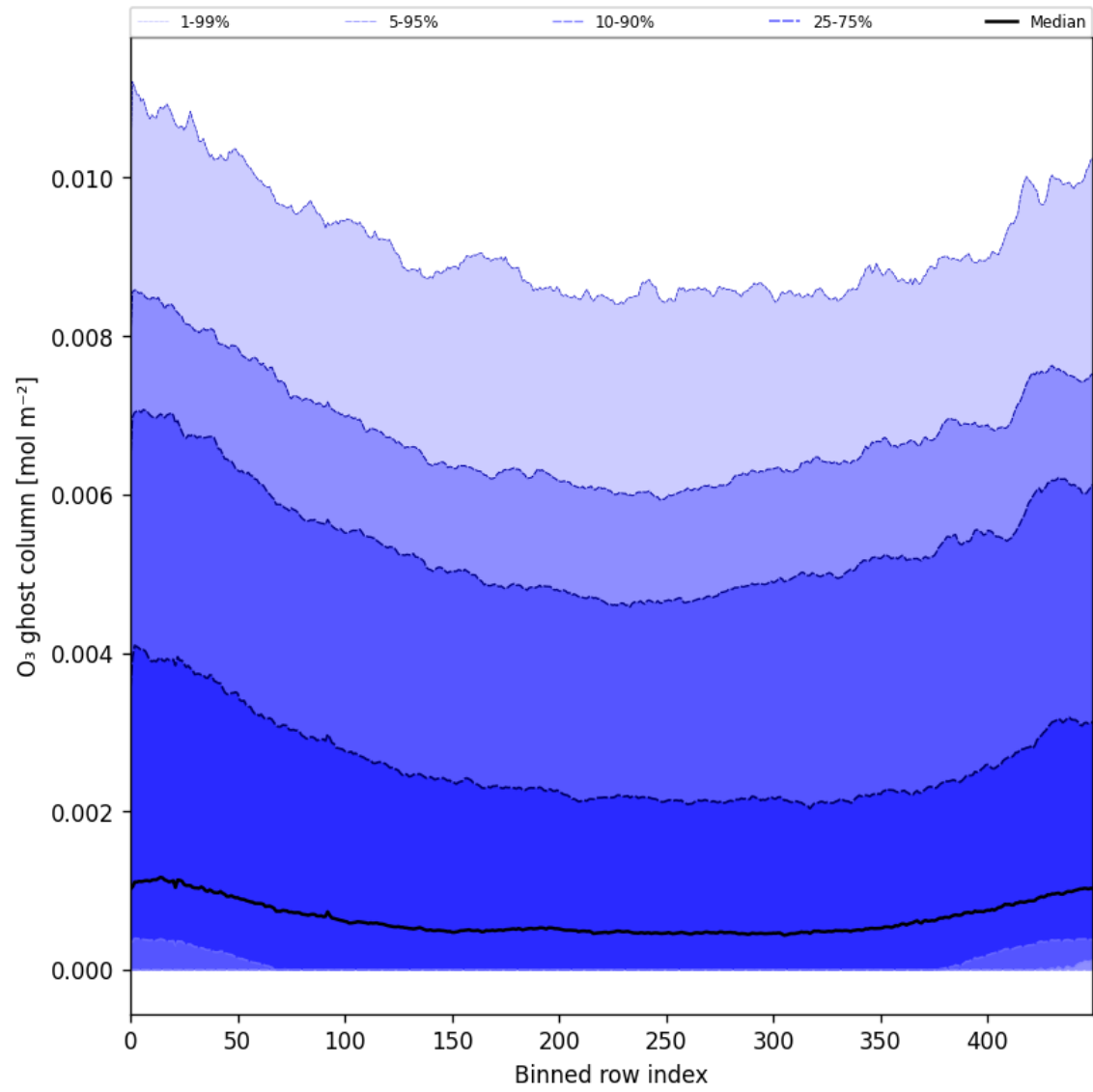
Figure 32: Along track statistics of “O 3 ghost column” for 2025-06-30 to 2025-07-02
