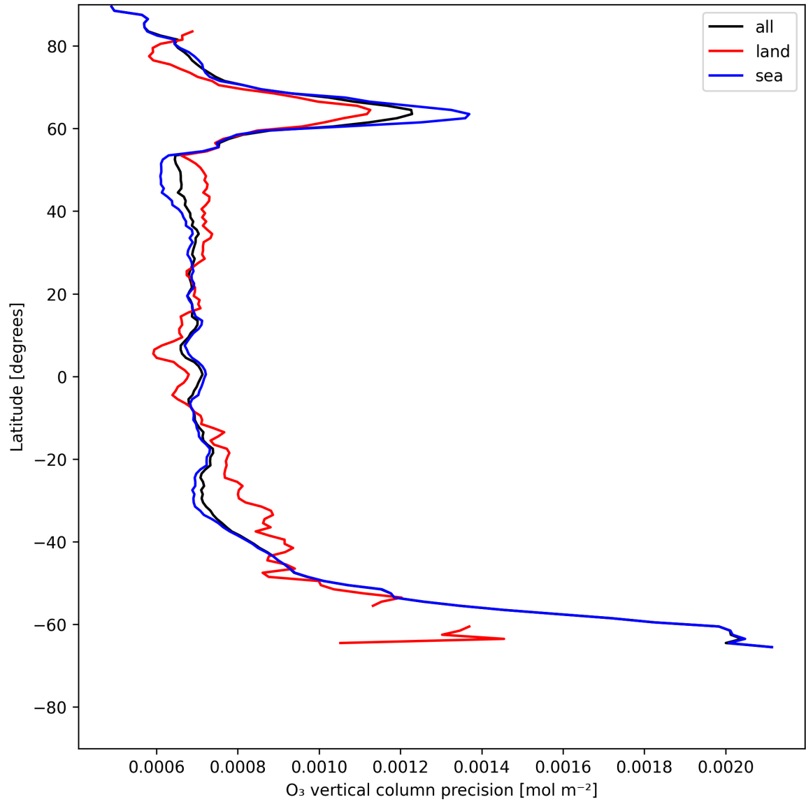
Figure 15: Zonal average of “O 3 vertical column precision” for 2025-06-30 to 2025-07-02.
