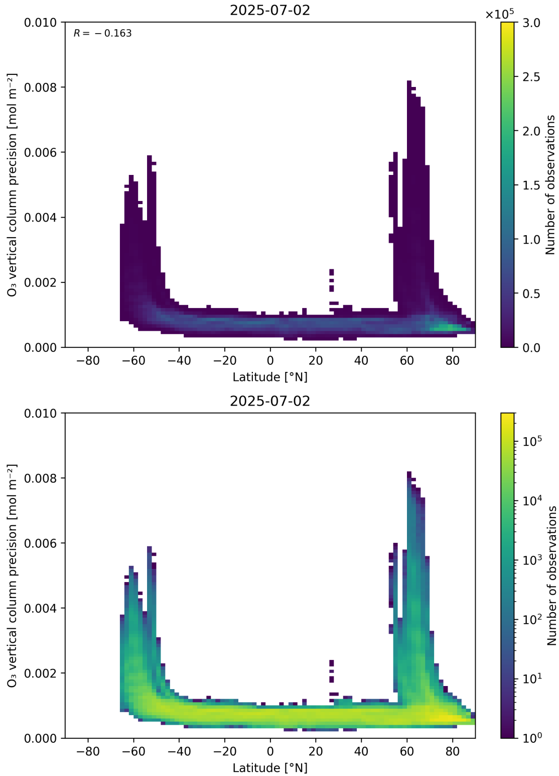
Figure 37: Scatter density plot of “Latitude” against “O 3 vertical column precision” for 2025-07-02 to 2025-07-03.
