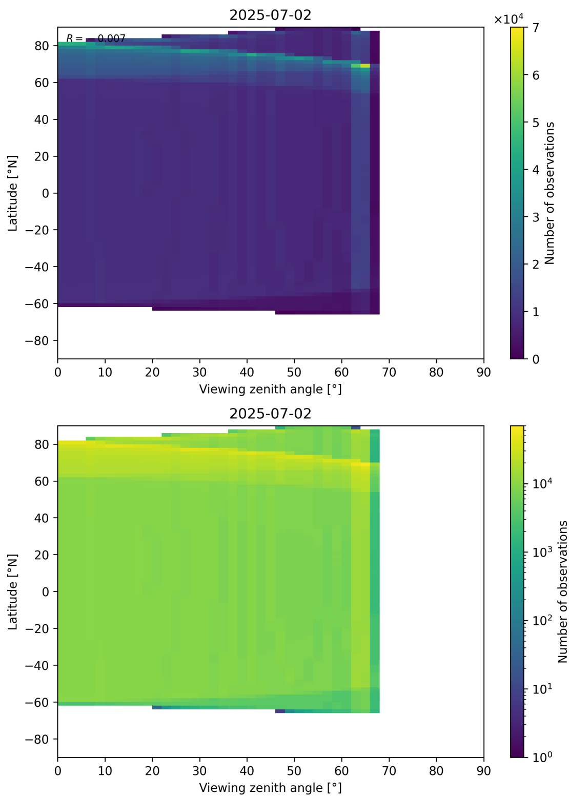
Figure 49: Scatter density plot of “Viewing zenith angle” against “Latitude” for 2025-07-02 to 2025-07-03.
