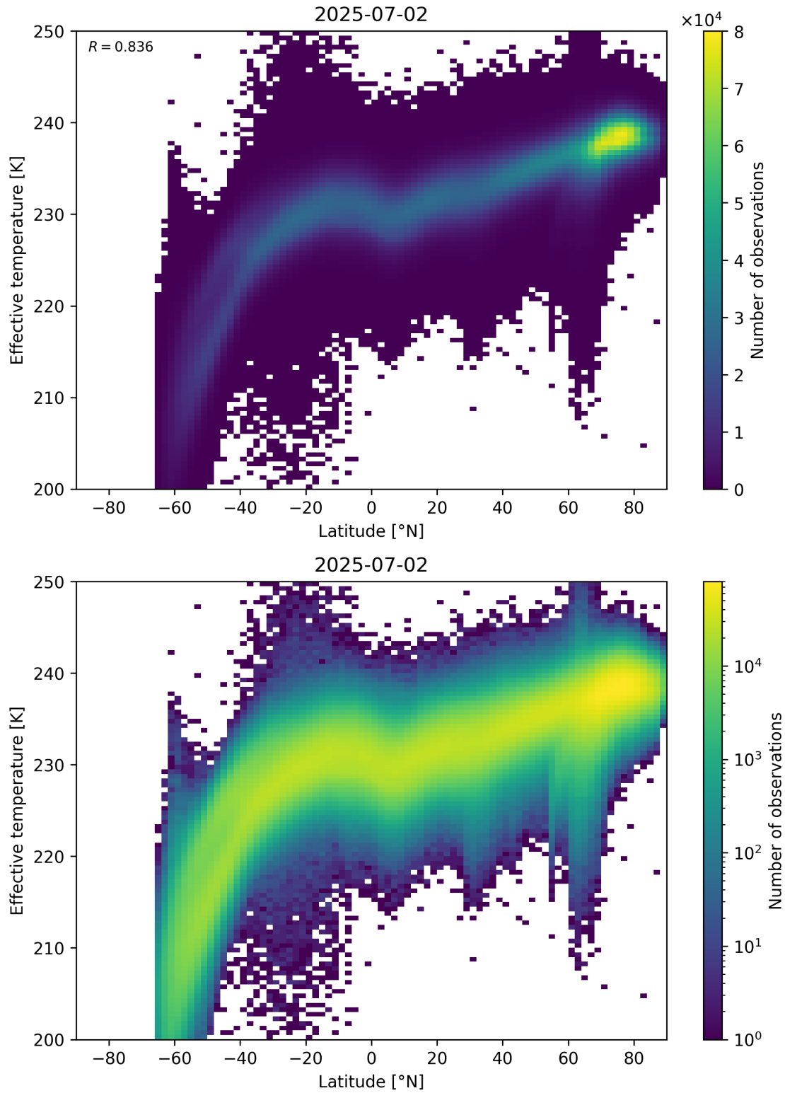
Figure 34: Scatter density plot of “Latitude” against “Effective temperature” for 2025-07-02 to 2025-07-03.
