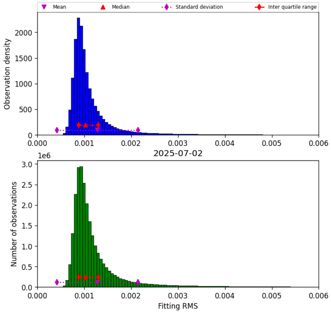
Figure 23: Histogram of “Fitting RMS” for 2025-07-02 to 2025-07-03
