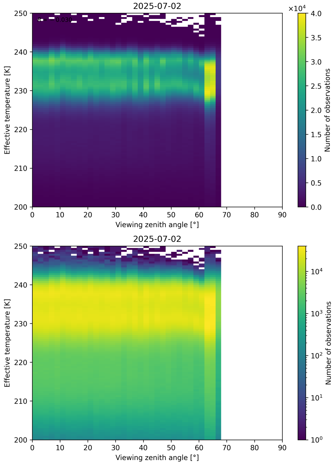
Figure 50: Scatter density plot of “Viewing zenith angle” against “Effective temperature” for 2025-07-02 to 2025-07-03.
