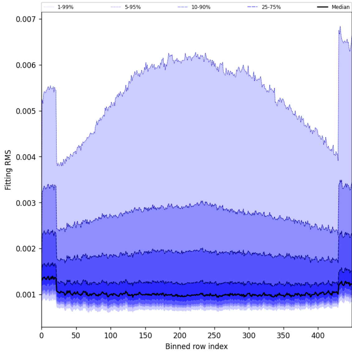
Figure 30: Along track statistics of “Fitting RMS” for 2025-07-02 to 2025-07-03
