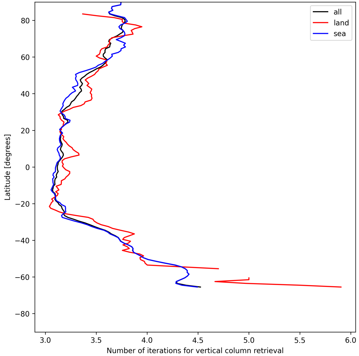
Figure 19: Zonal average of “Number of iterations for vertical column retrieval” for 2025-07-02 to 2025-07-03.
