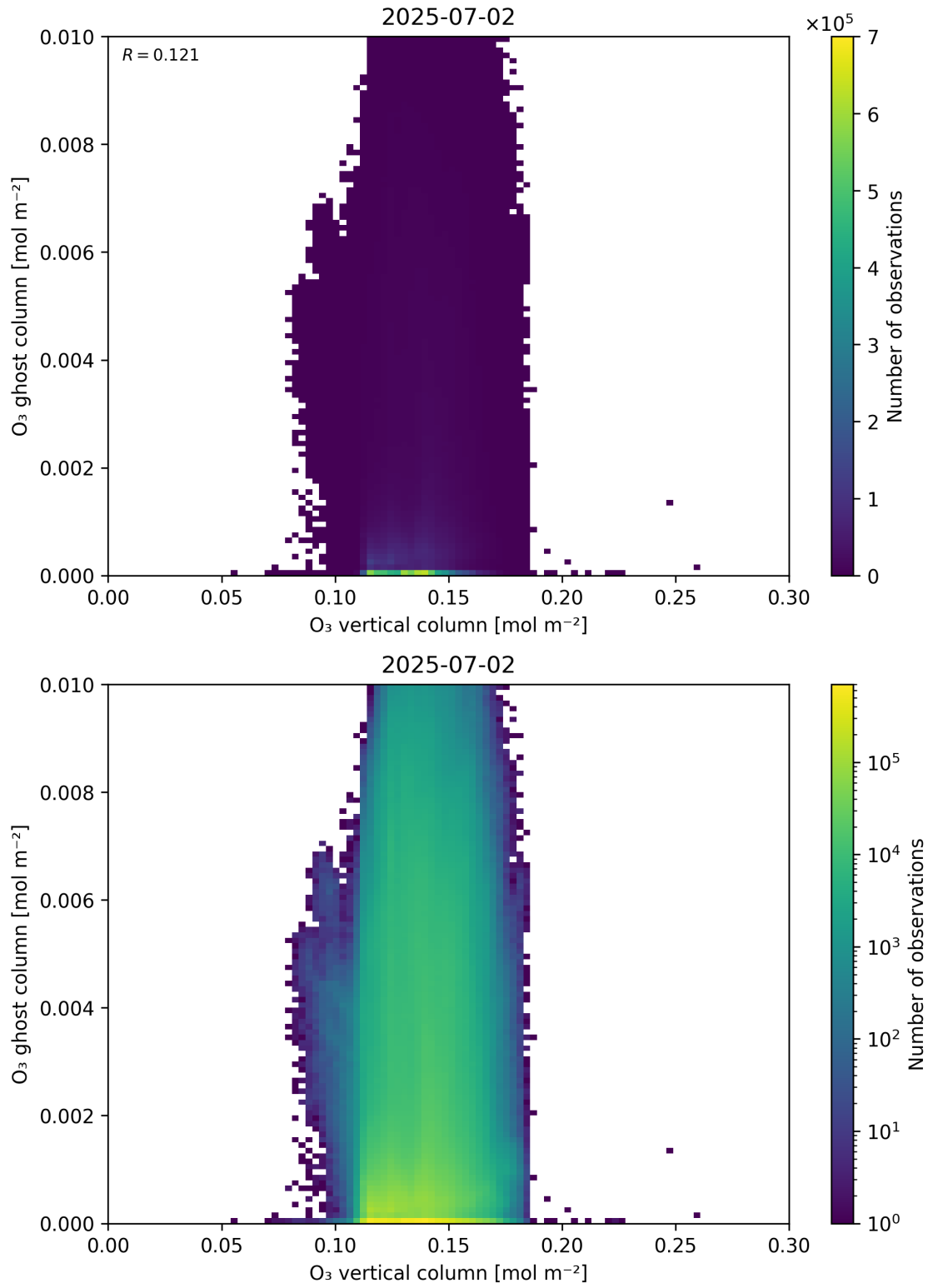
Figure 40: Scatter density plot of “O 3 vertical column” against “O 3 ghost column” for 2025-07-02 to 2025-07-03.
