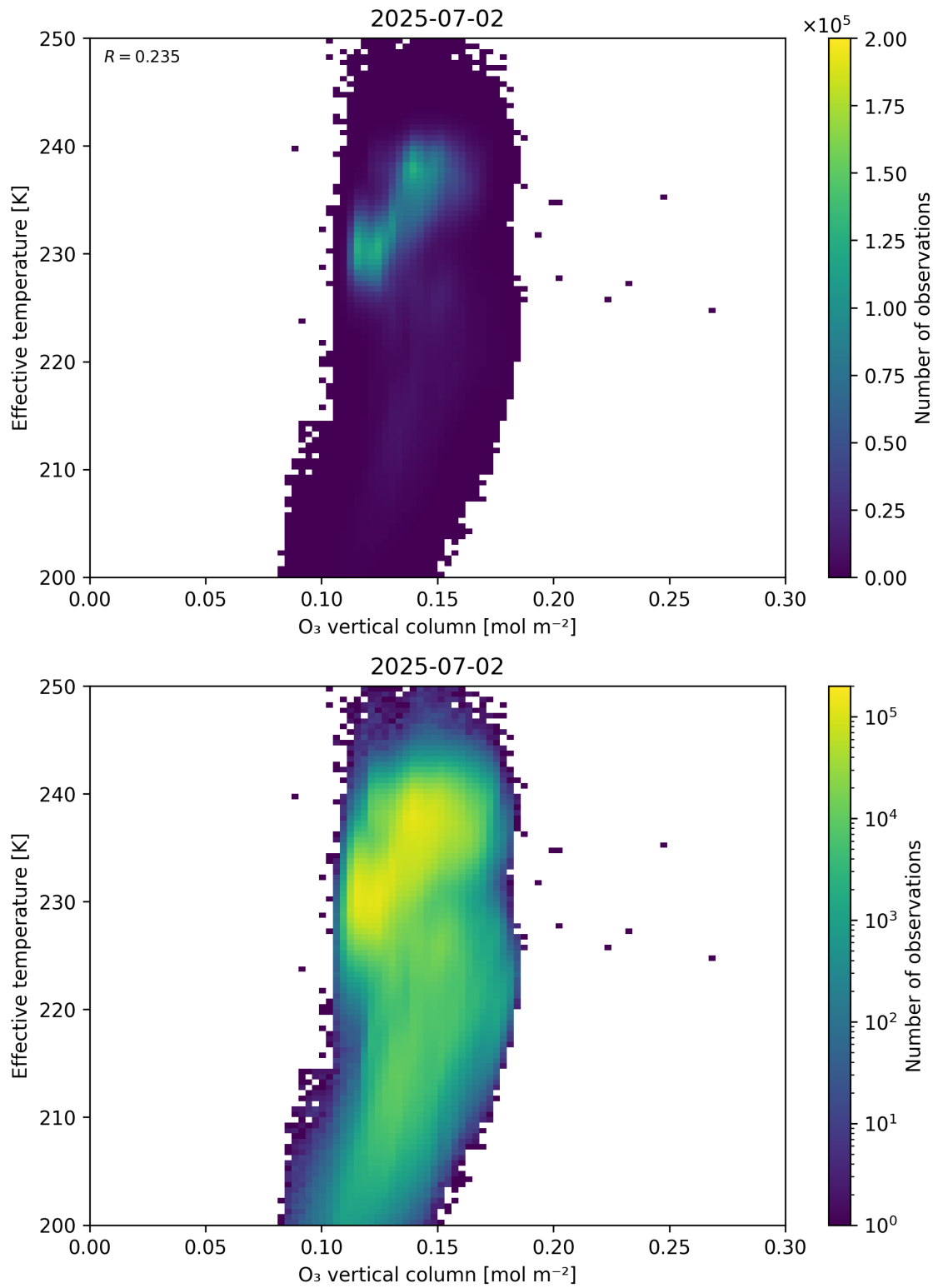
Figure 39: Scatter density plot of “O 3 vertical column” against “Effective temperature” for 2025-07-02 to 2025-07-03.
