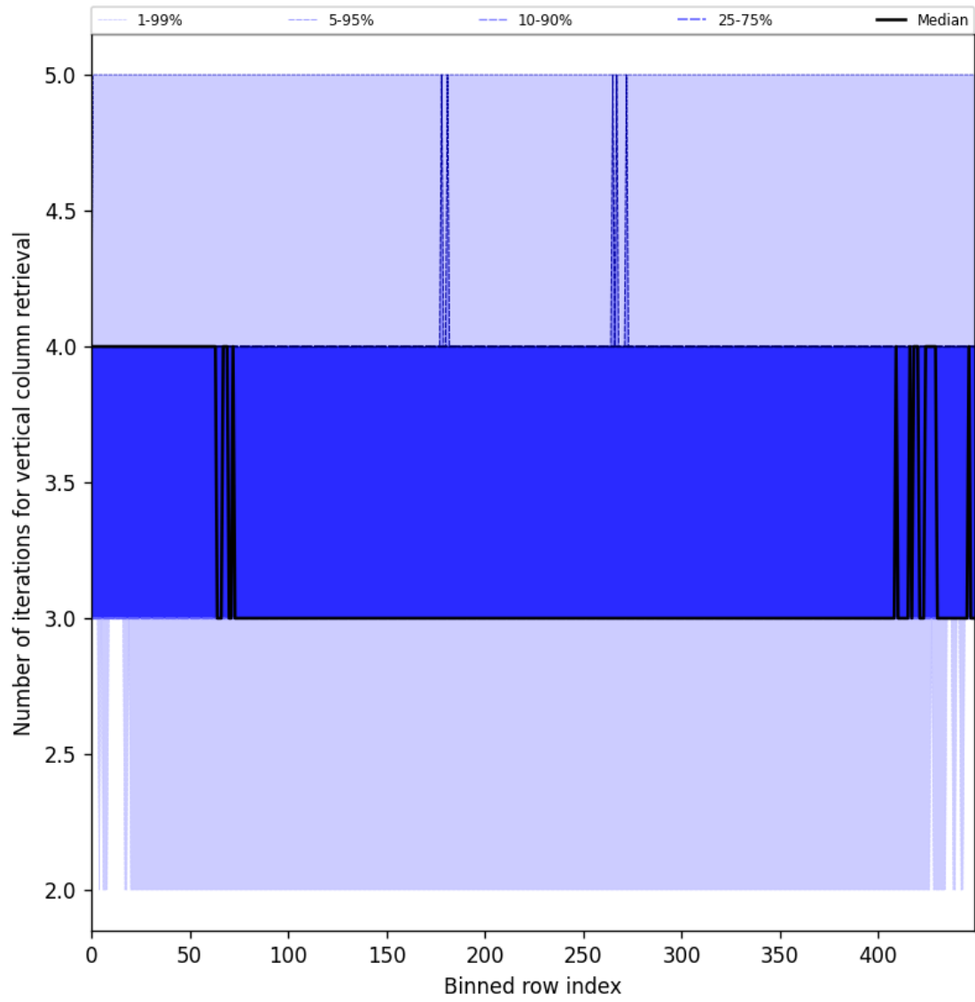
Figure 33: Along track statistics of “Number of iterations for vertical column retrieval” for 2025-07-02 to 2025-07-03
