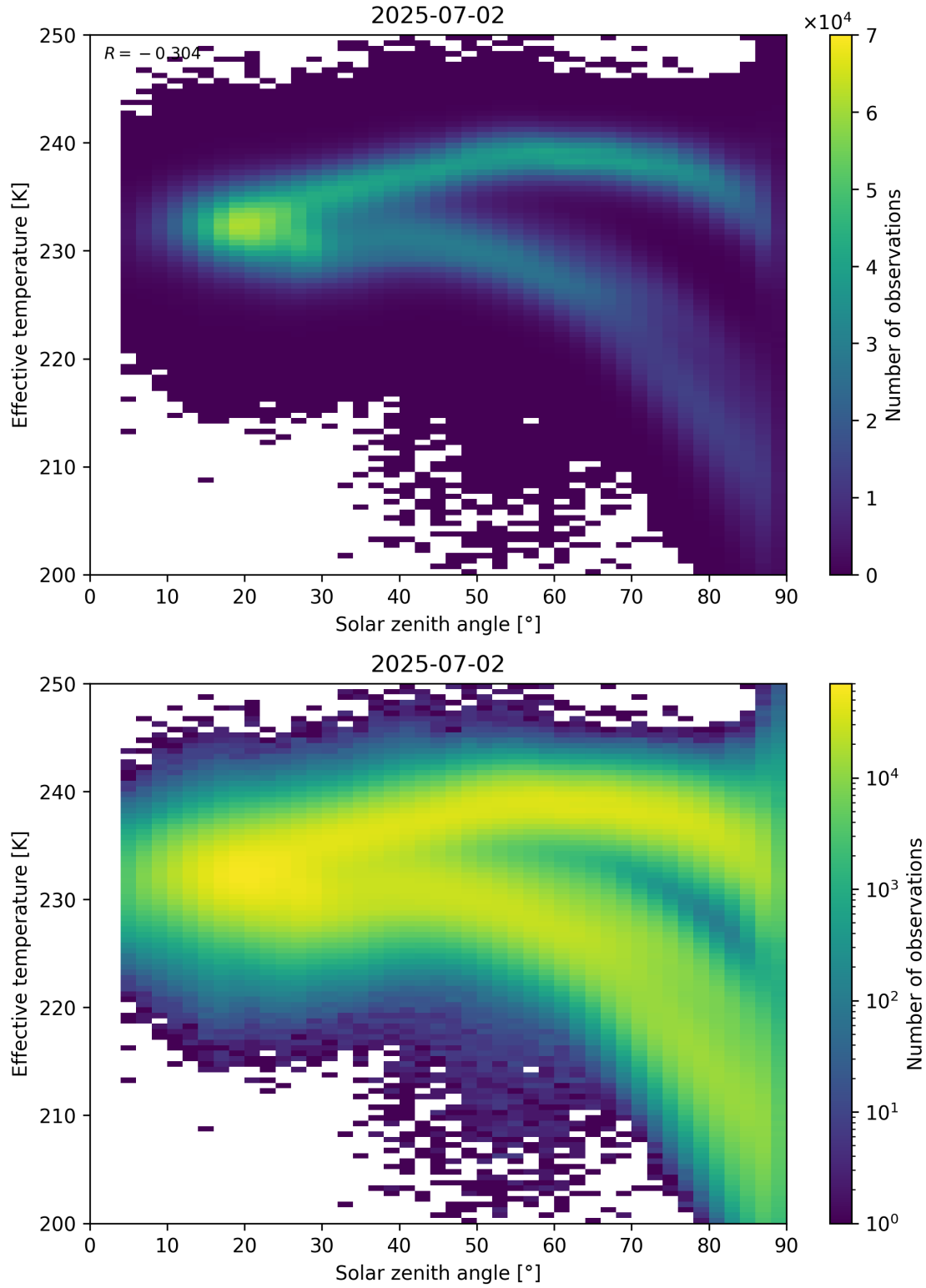
Figure 45: Scatter density plot of “Solar zenith angle” against “Effective temperature” for 2025-07-02 to 2025-07-03.
