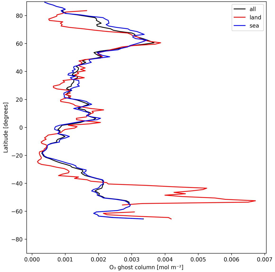
Figure 18: Zonal average of "O 3 ghost column" for 2025-07-02 to 2025-07-03.
