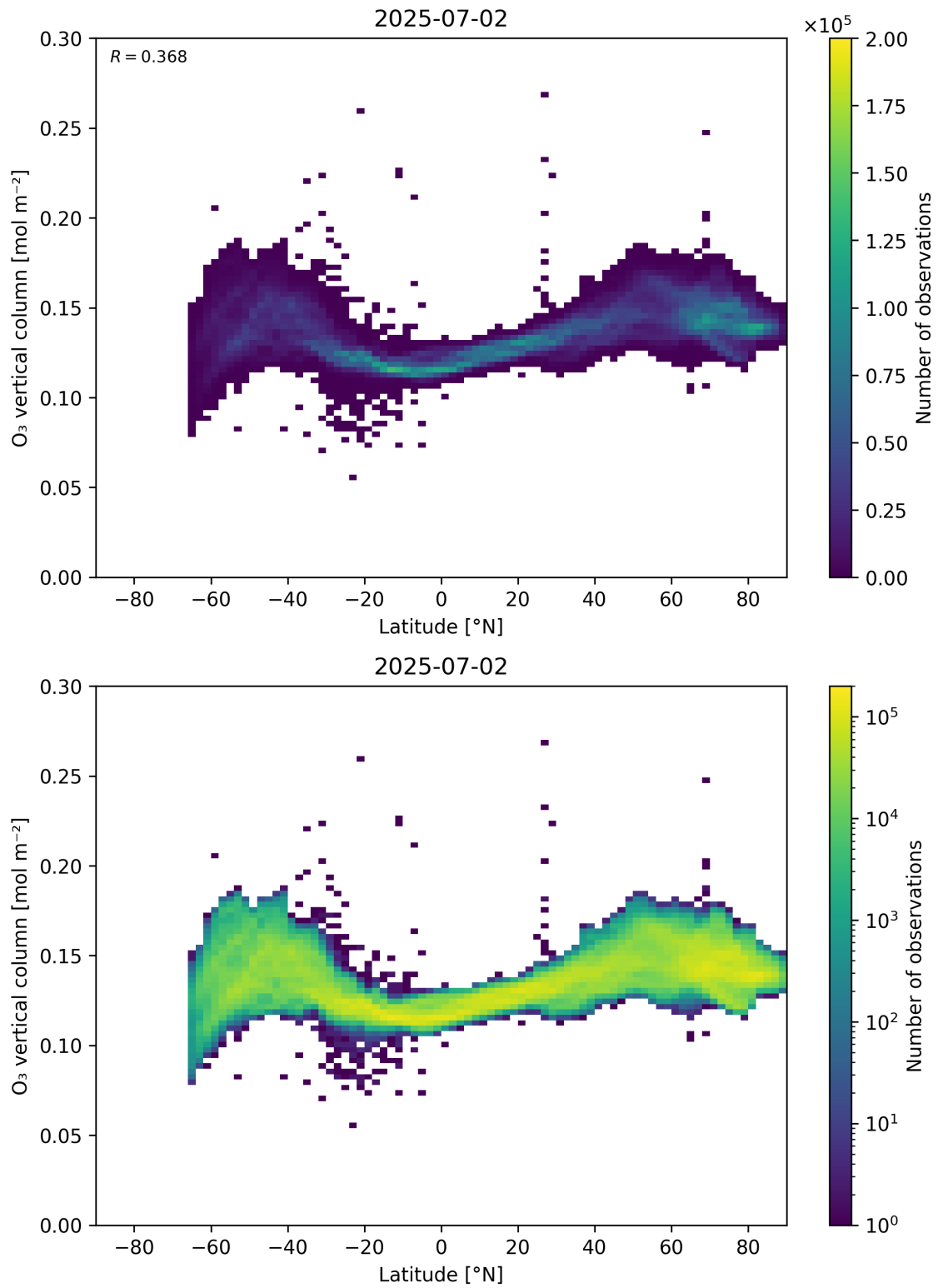
Figure 36: Scatter density plot of “Latitude” against “O 3 vertical column” for 2025-07-02 to 2025-07-03.
