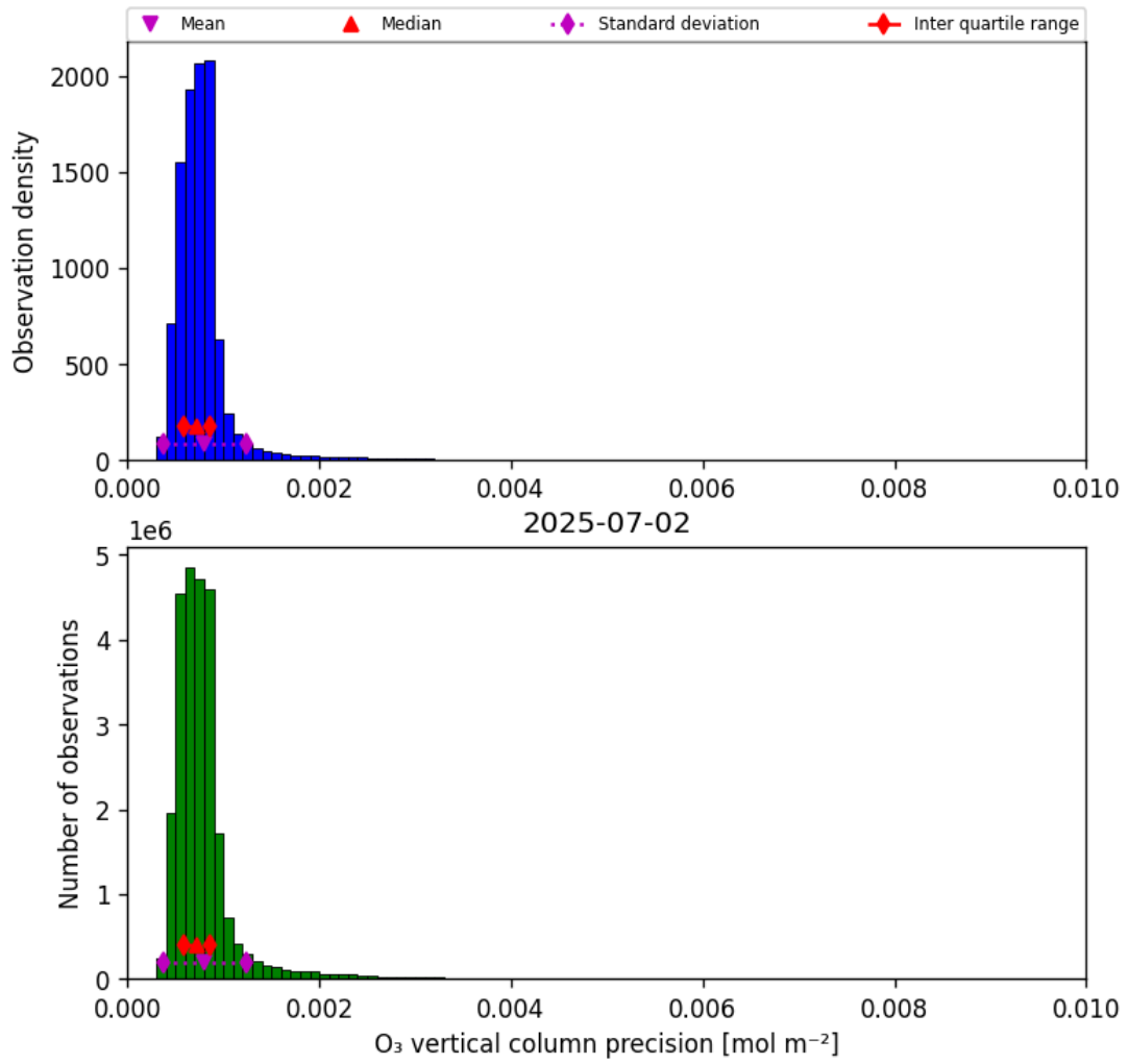
Figure 22: Histogram of “O 3 vertical column precision” for 2025-07-02 to 2025-07-03
