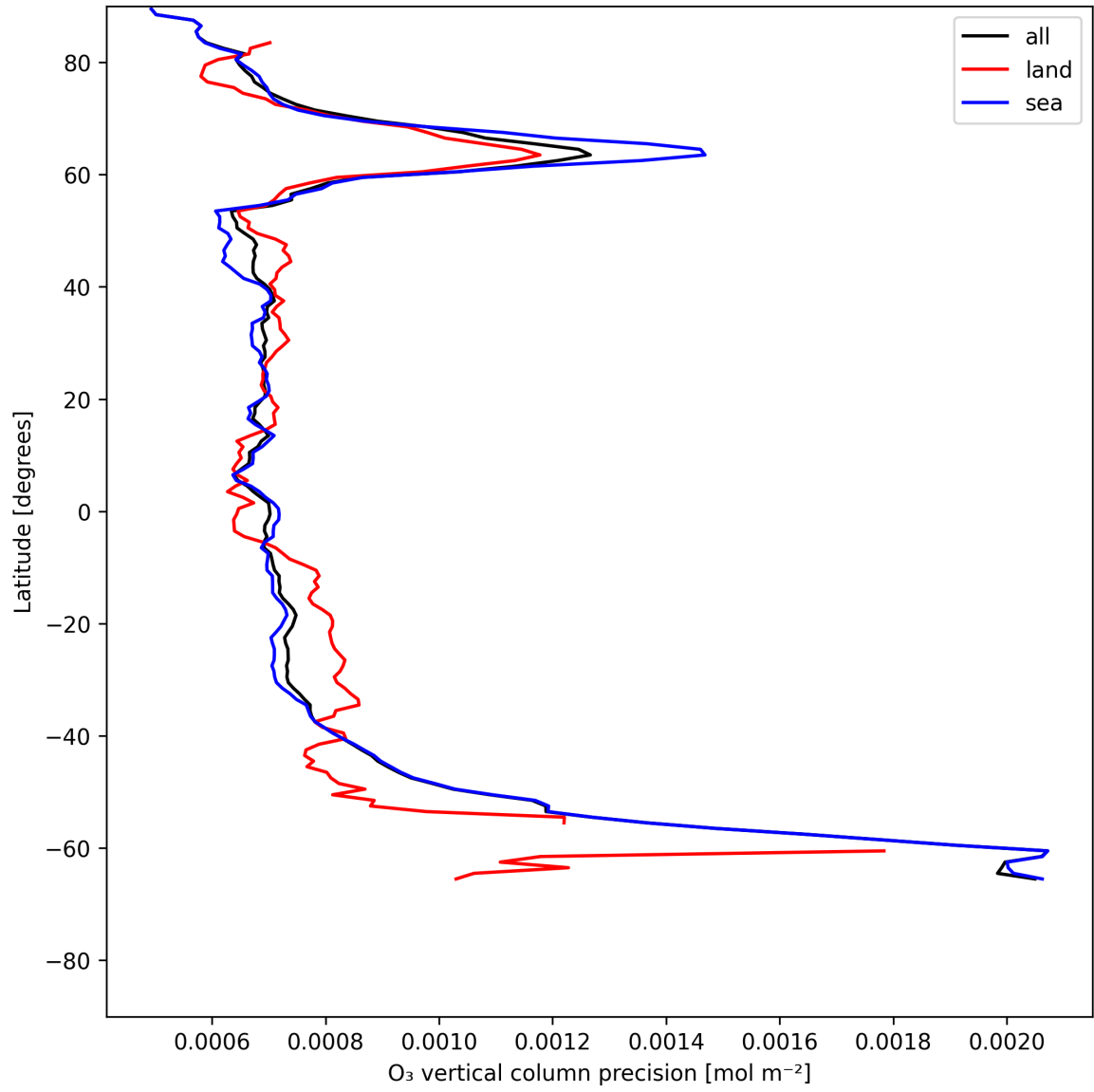
Figure 15: Zonal average of “O 3 vertical column precision” for 2025-07-02 to 2025-07-03.
