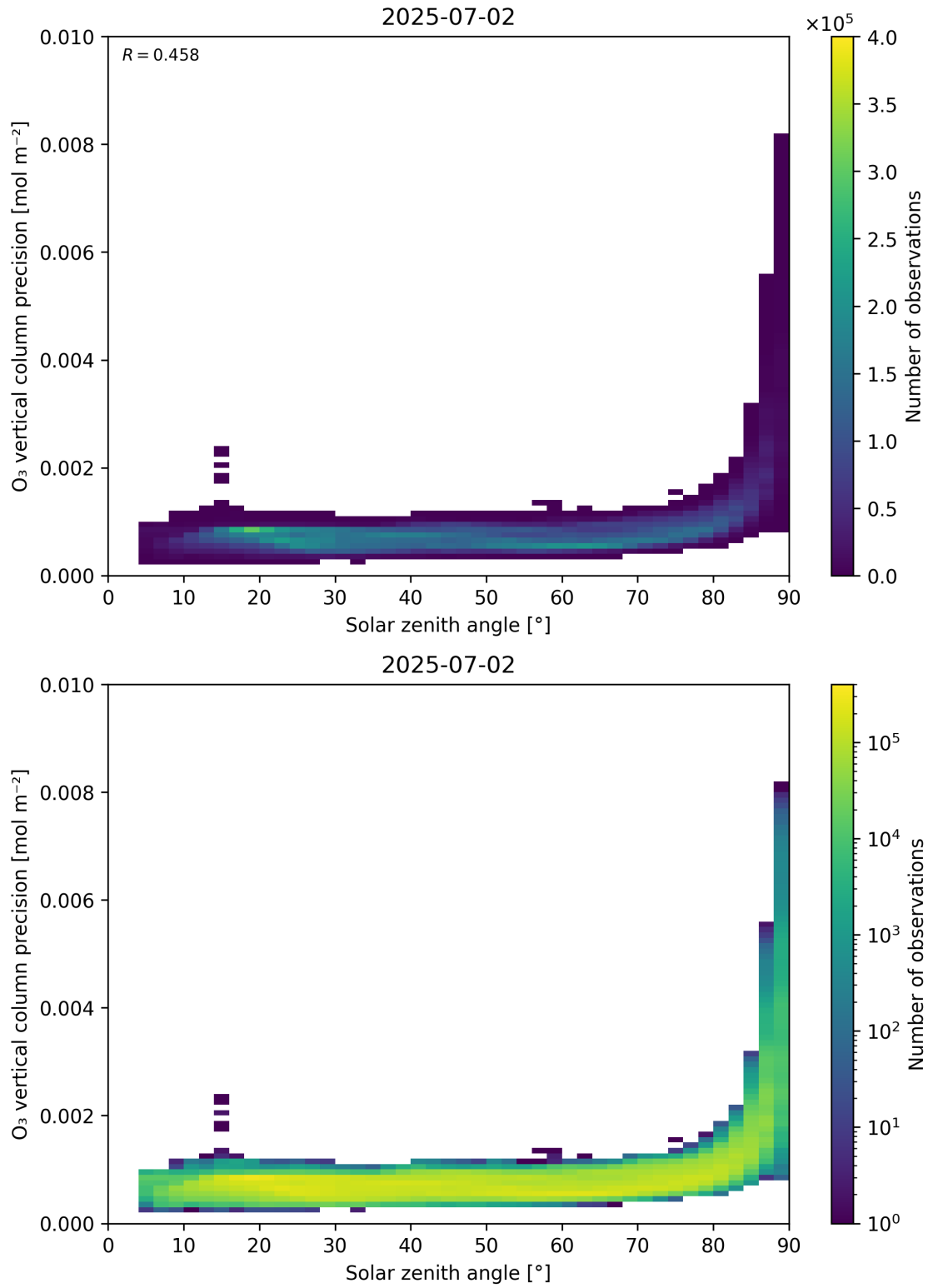
Figure 48: Scatter density plot of “Solar zenith angle” against “O 3 vertical column precision” for 2025-07-02 to 2025-07-03.
