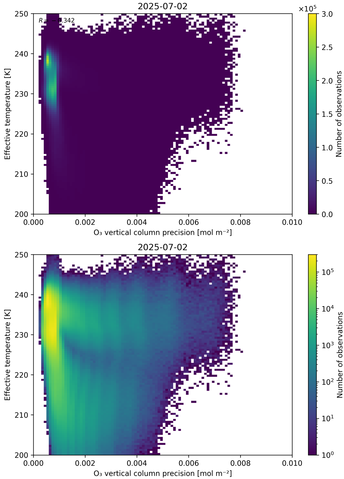
Figure 42: Scatter density plot of “O 3 vertical column precision” against “Effective temperature” for 2025-07-02 to 2025-07-03.
