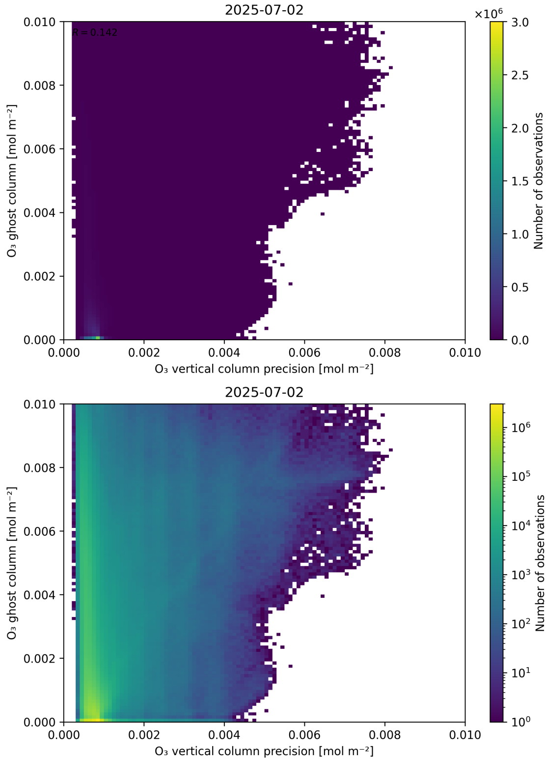
Figure 43: Scatter density plot of “ \text{O}_3 vertical column precision” against “ \text{O}_3 ghost column” for 2025-07-02 to 2025-07-03.
