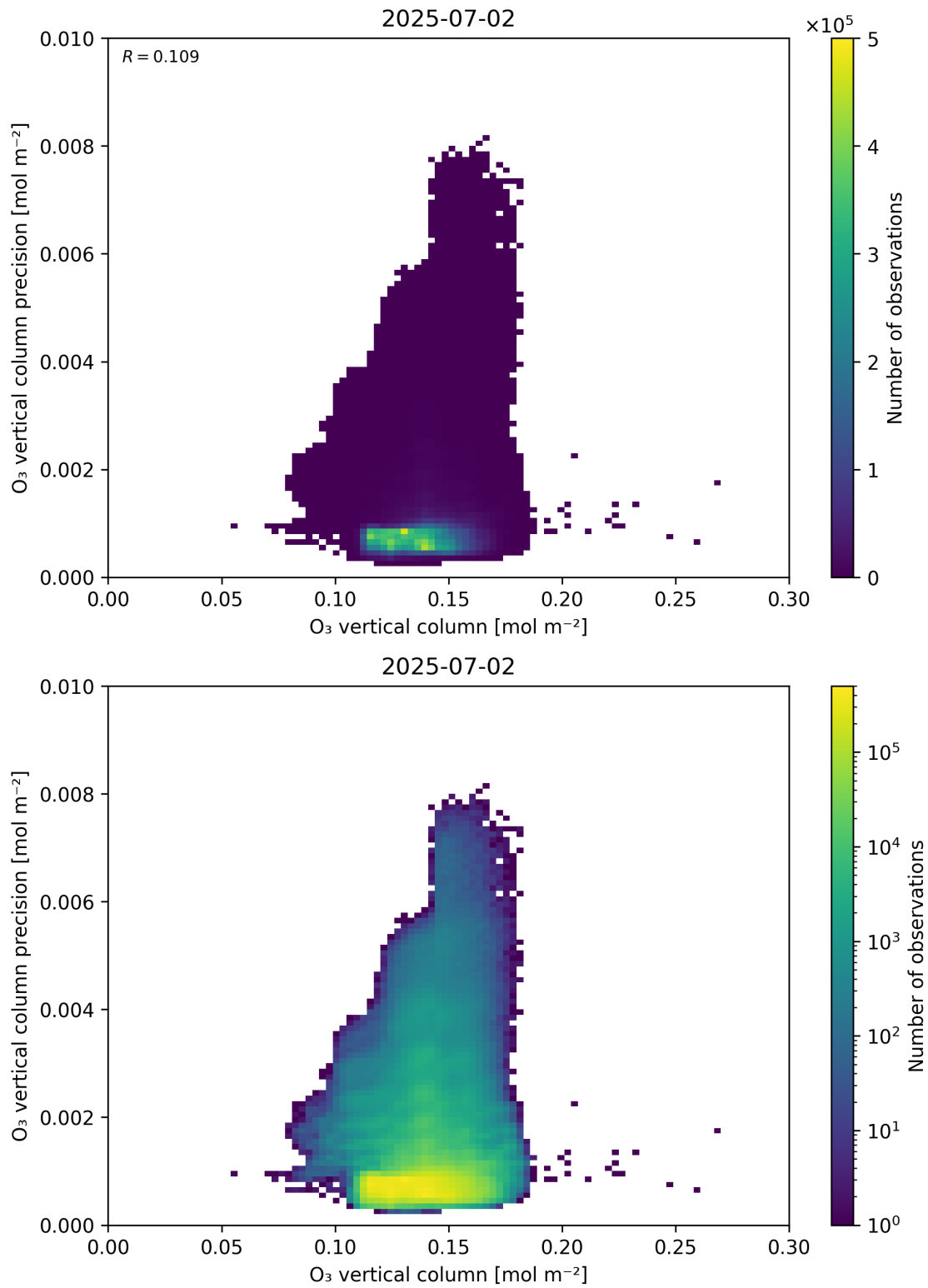
Figure 41: Scatter density plot of “O 3 vertical column” against “O 3 vertical column precision” for 2025-07-02 to 2025-07-03.
