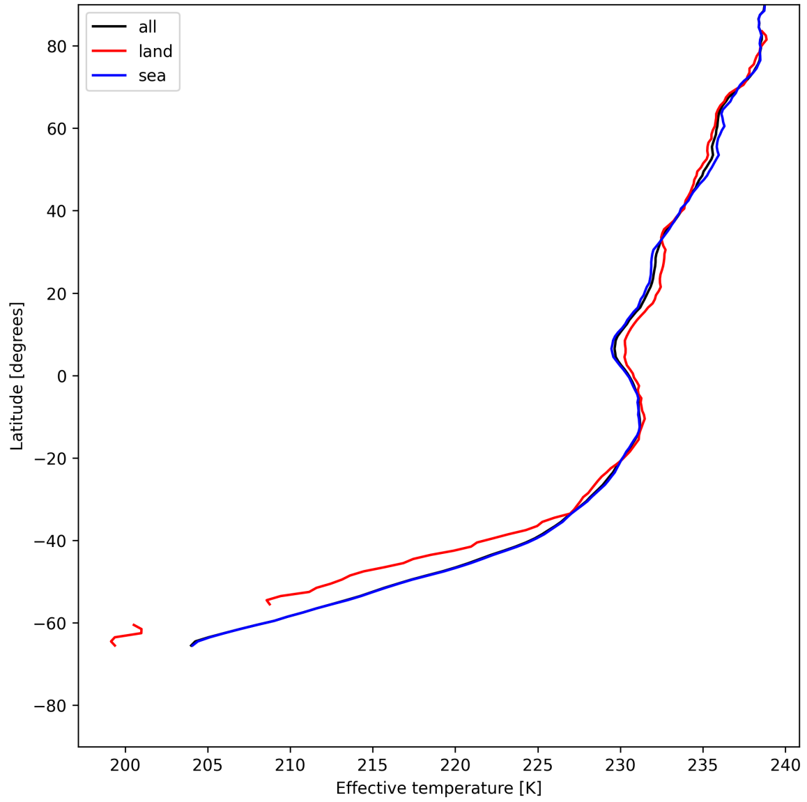
Figure 17: Zonal average of "Effective temperature" for 2025-07-02 to 2025-07-03.
