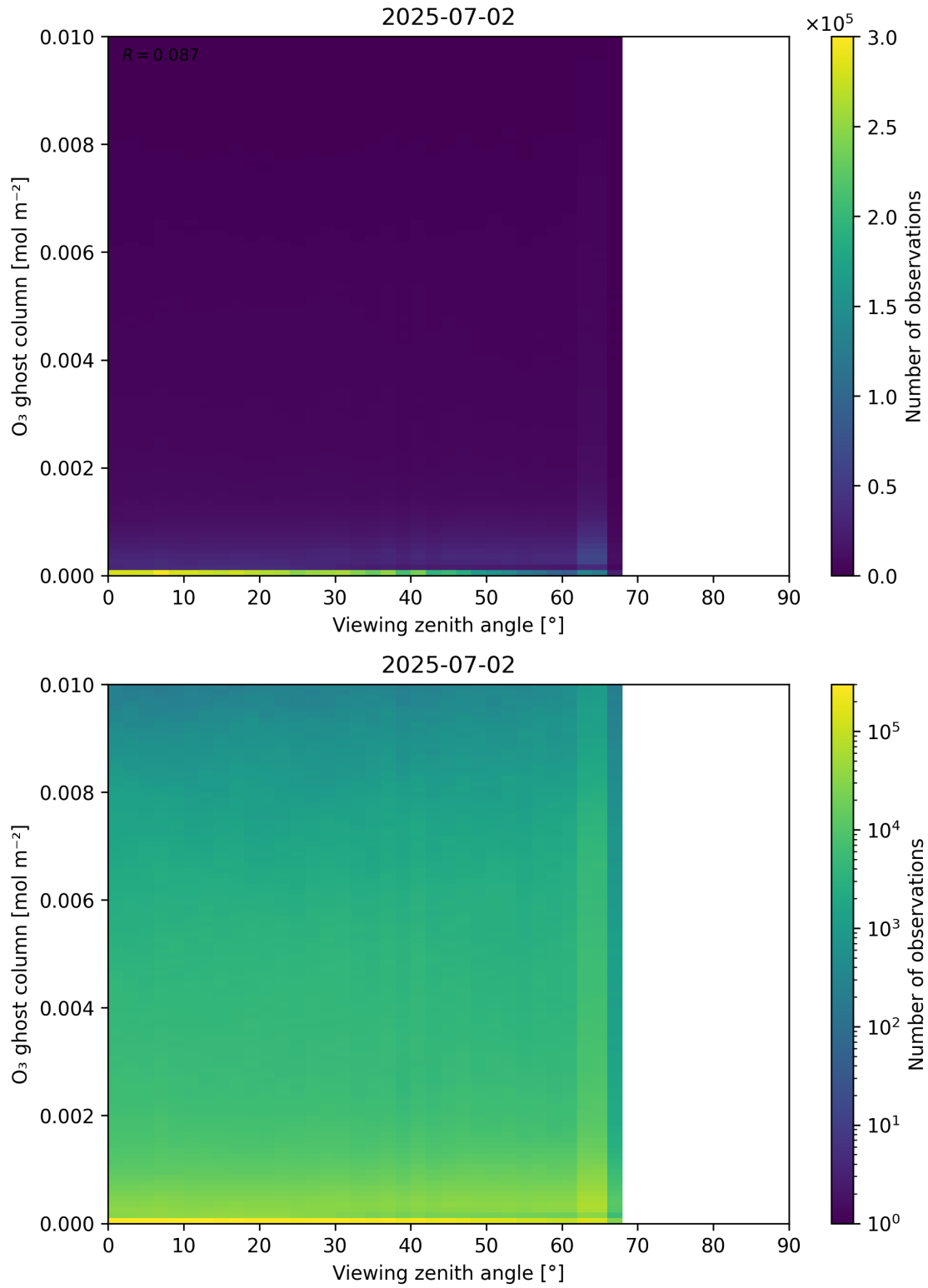
Figure 51: Scatter density plot of “Viewing zenith angle” against “O 3 ghost column” for 2025-07-02 to 2025-07-03.
