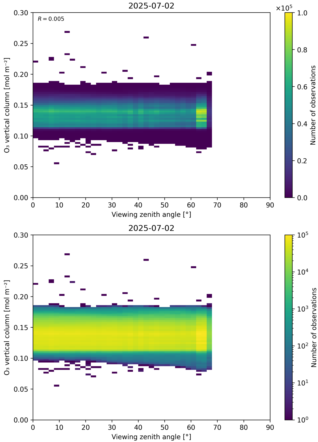
Figure 52: Scatter density plot of “Viewing zenith angle” against “O 3 vertical column” for 2025-07-02 to 2025-07-03.
