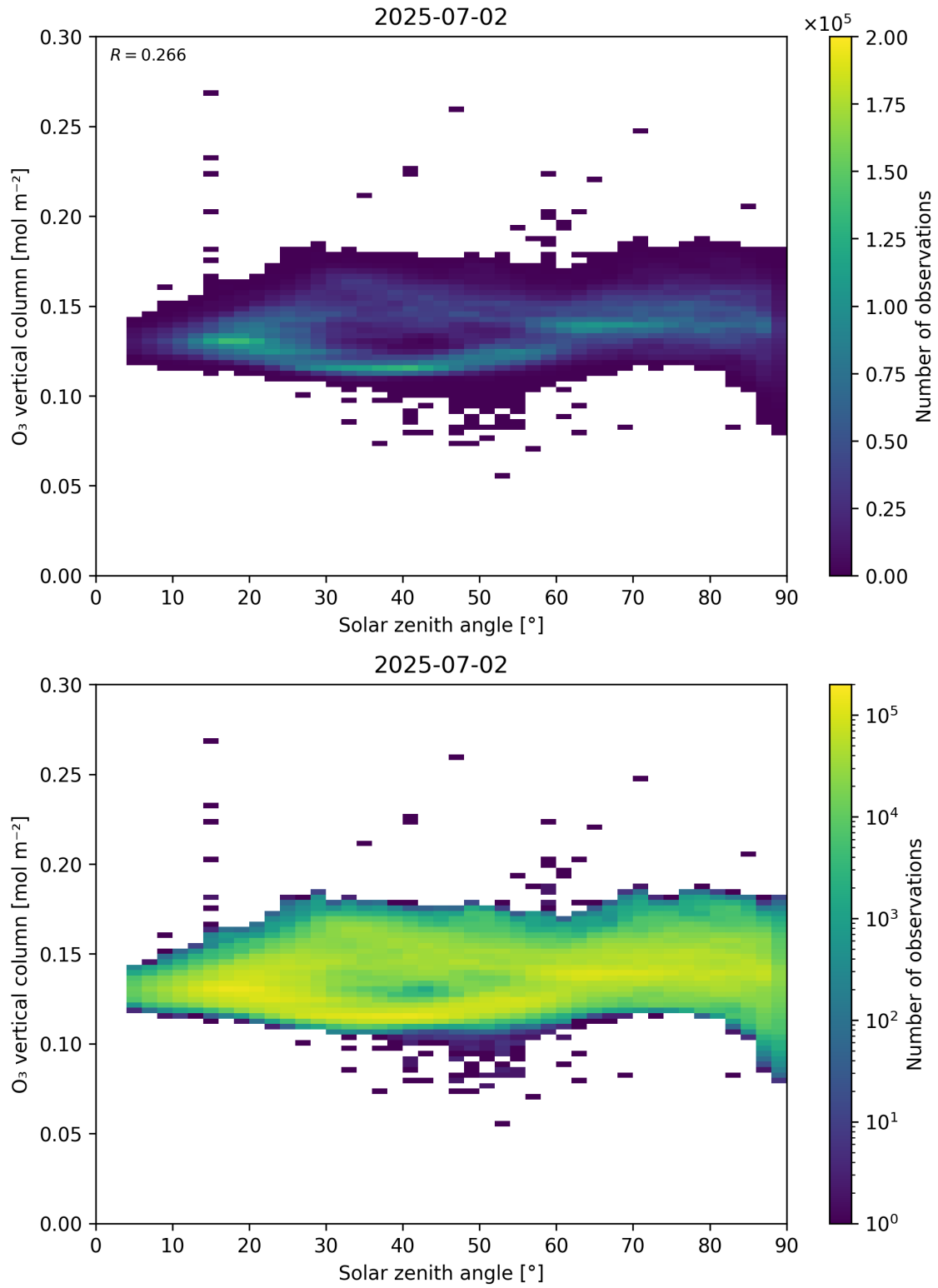
Figure 47: Scatter density plot of “Solar zenith angle” against “O 3 vertical column” for 2025-07-02 to 2025-07-03.
