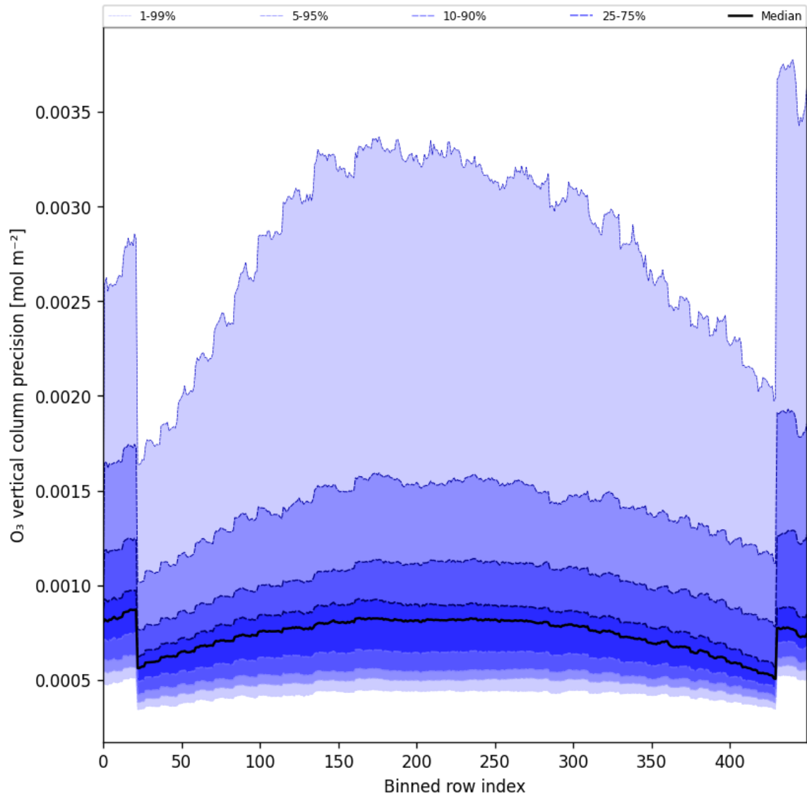
Figure 29: Along track statistics of “O 3 vertical column precision” for 2025-07-02 to 2025-07-03
