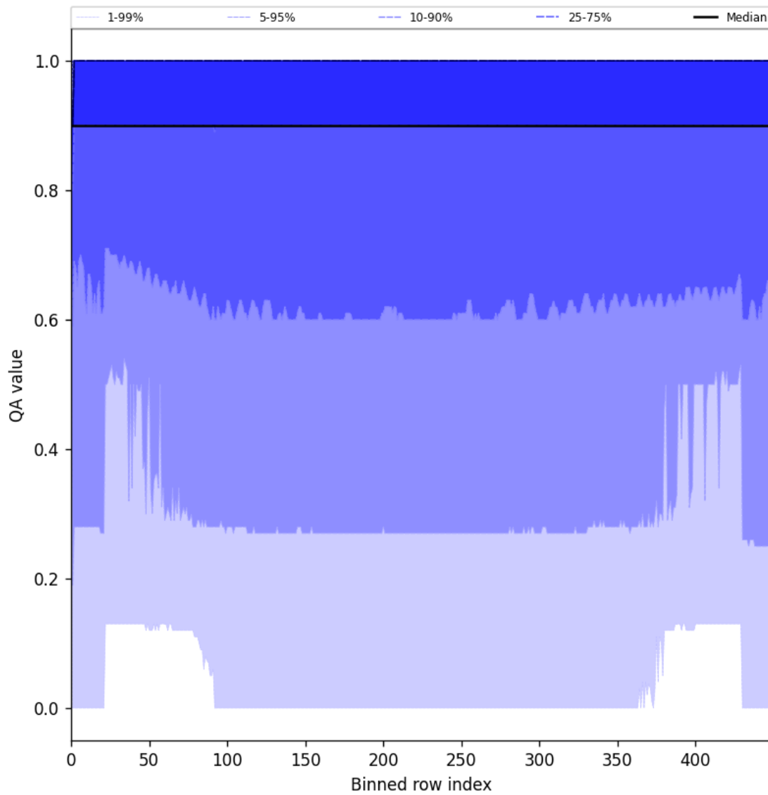
Figure 27: Along track statistics of “QA value” for 2025-07-02 to 2025-07-03
