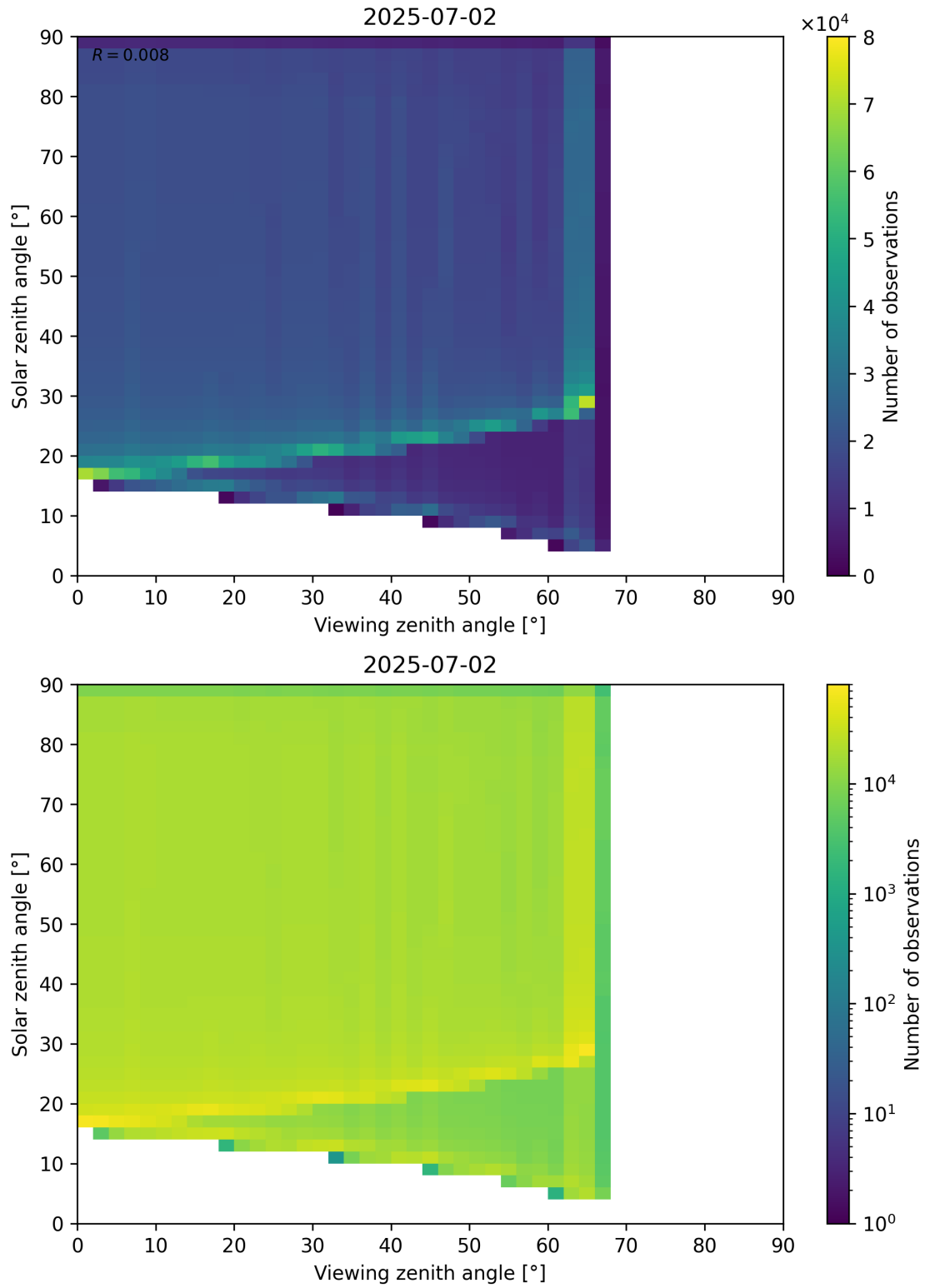
Figure 54: Scatter density plot of “Viewing zenith angle” against “Solar zenith angle” for 2025-07-02 to 2025-07-03.
