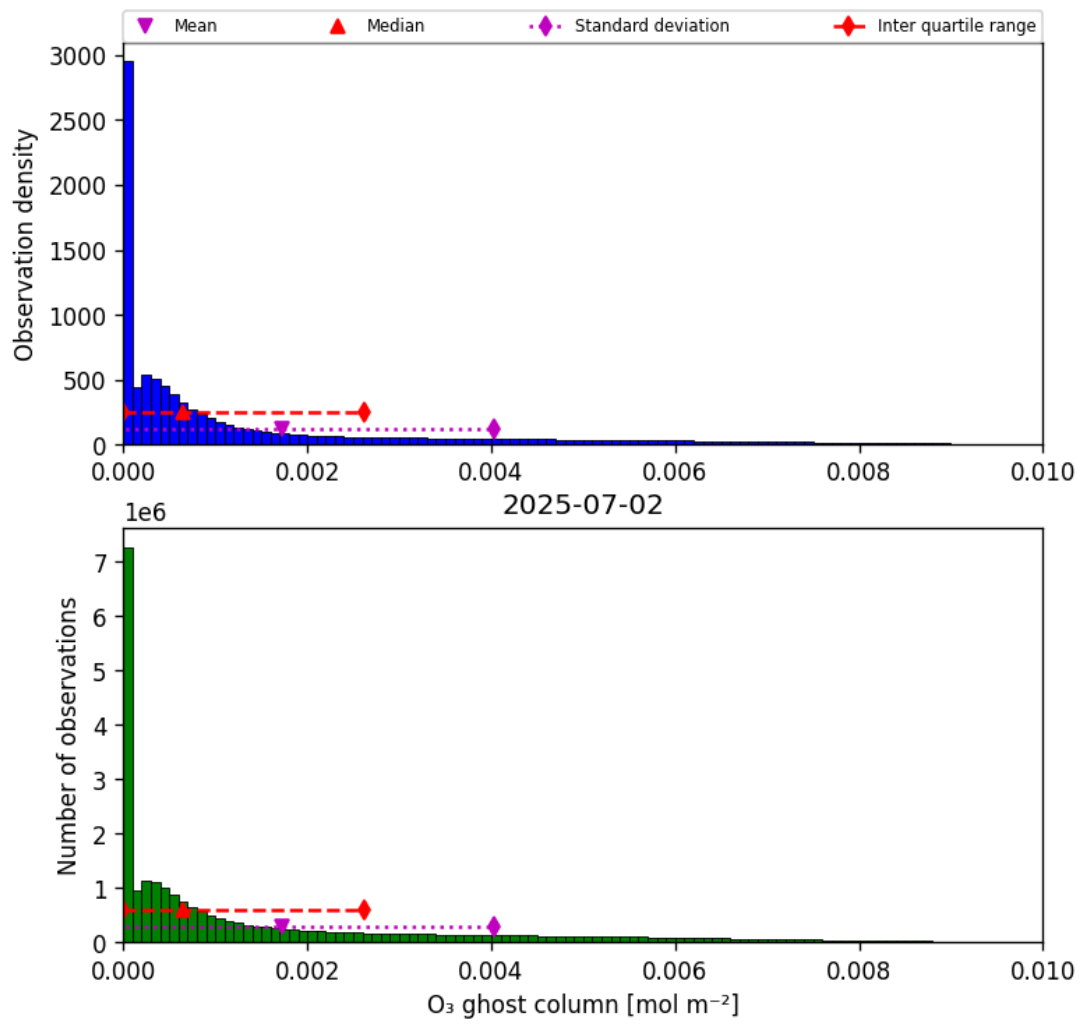
Figure 25: Histogram of “O 3 ghost column” for 2025-07-02 to 2025-07-03
