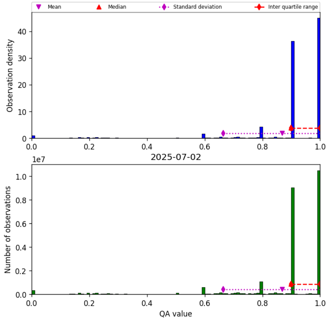
Figure 20: Histogram of “QA value” for 2025-07-02 to 2025-07-03
