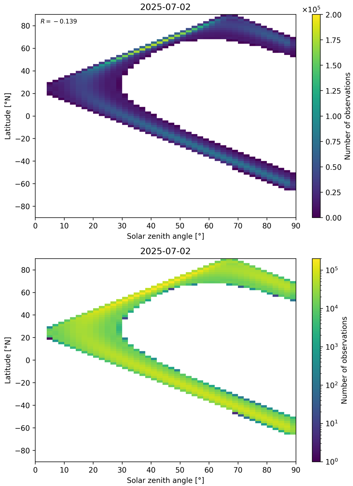
Figure 44: Scatter density plot of “Solar zenith angle” against “Latitude” for 2025-07-02 to 2025-07-03.
