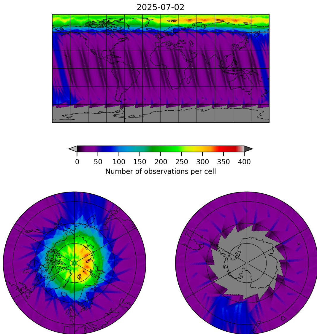
Figure 12: Map of the number of observations for 2025-07-02 to 2025-07-03
