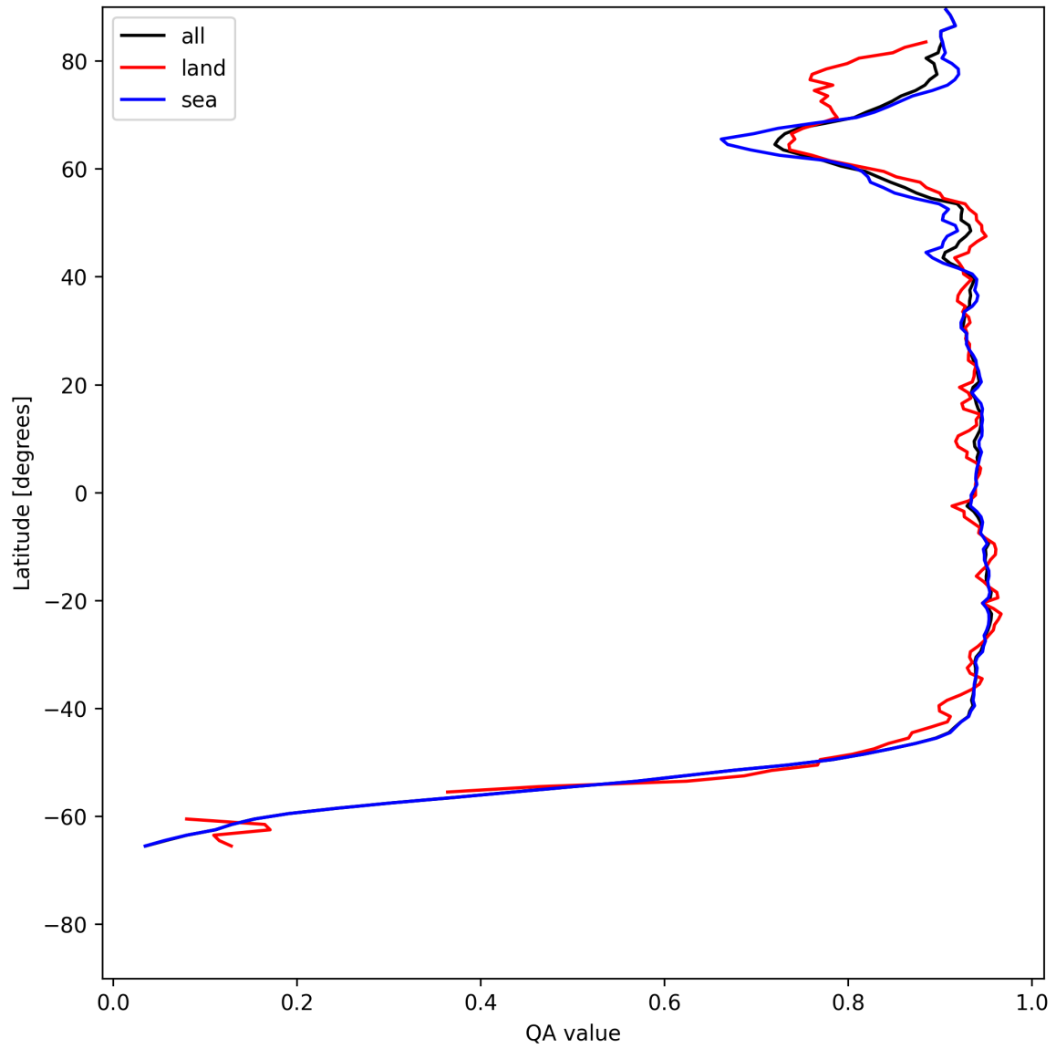
Figure 13: Zonal average of “QA value” for 2025-07-02 to 2025-07-03.
