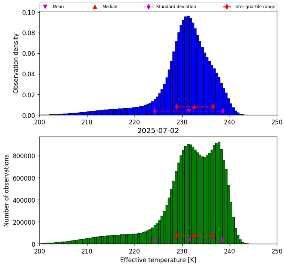
Figure 24: Histogram of “Effective temperature” for 2025-07-02 to 2025-07-03
