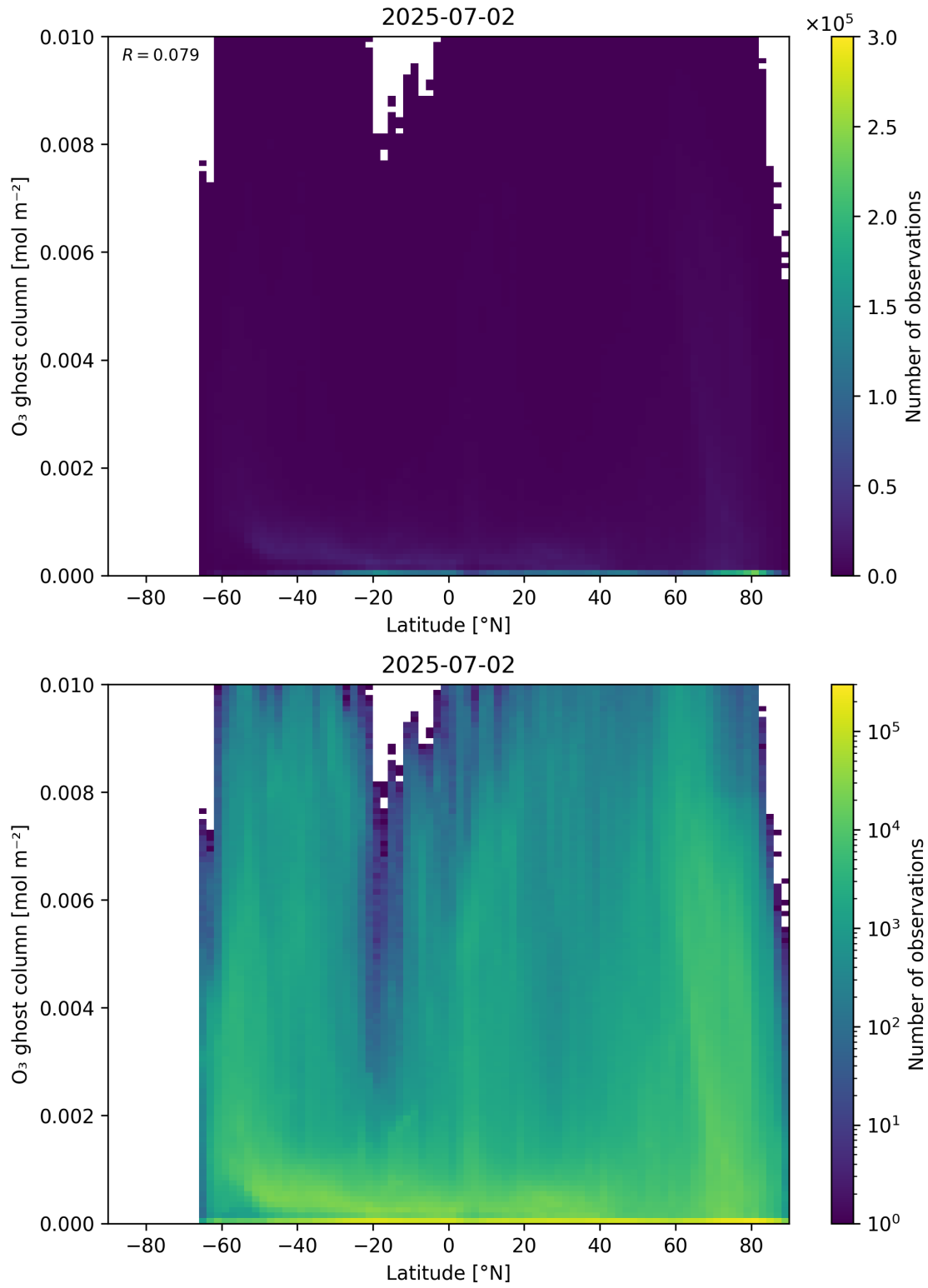
Figure 35: Scatter density plot of “Latitude” against “O 3 ghost column” for 2025-07-02 to 2025-07-03.
