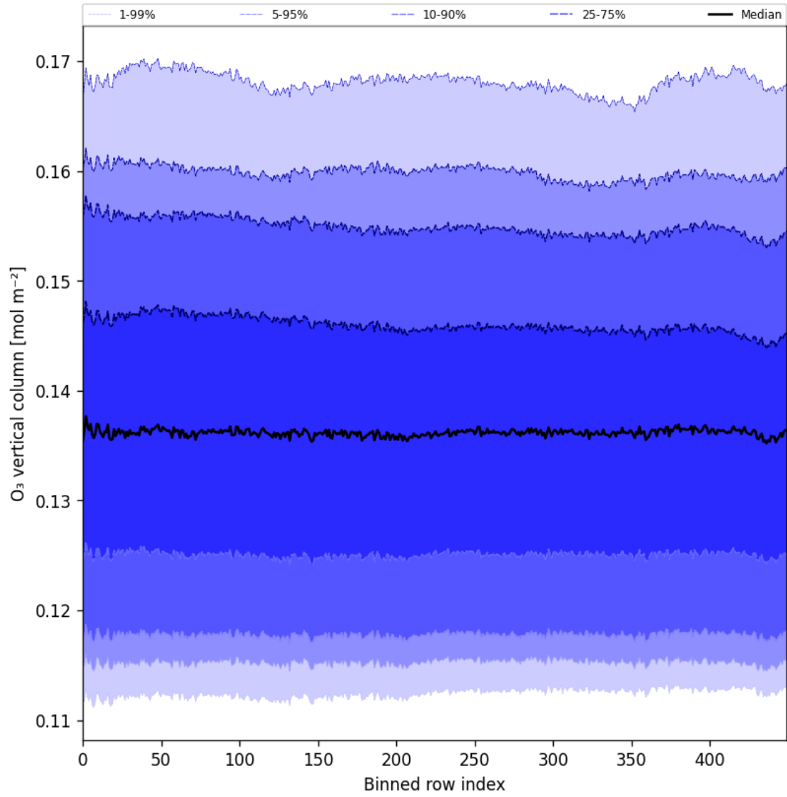
Figure 28: Along track statistics of “ O_3 vertical column” for 2025-07-02 to 2025-07-03
