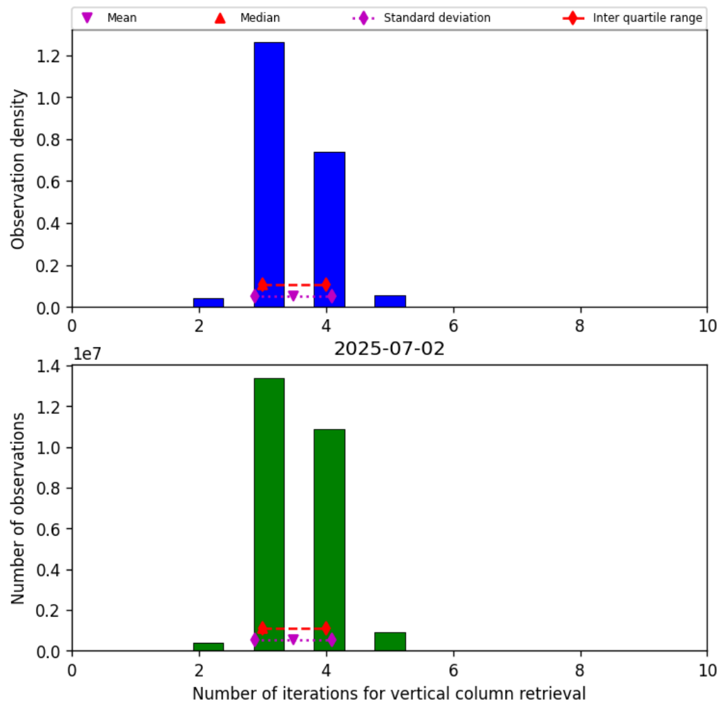
Figure 26: Histogram of “Number of iterations for vertical column retrieval” for 2025-07-02 to 2025-07-03
