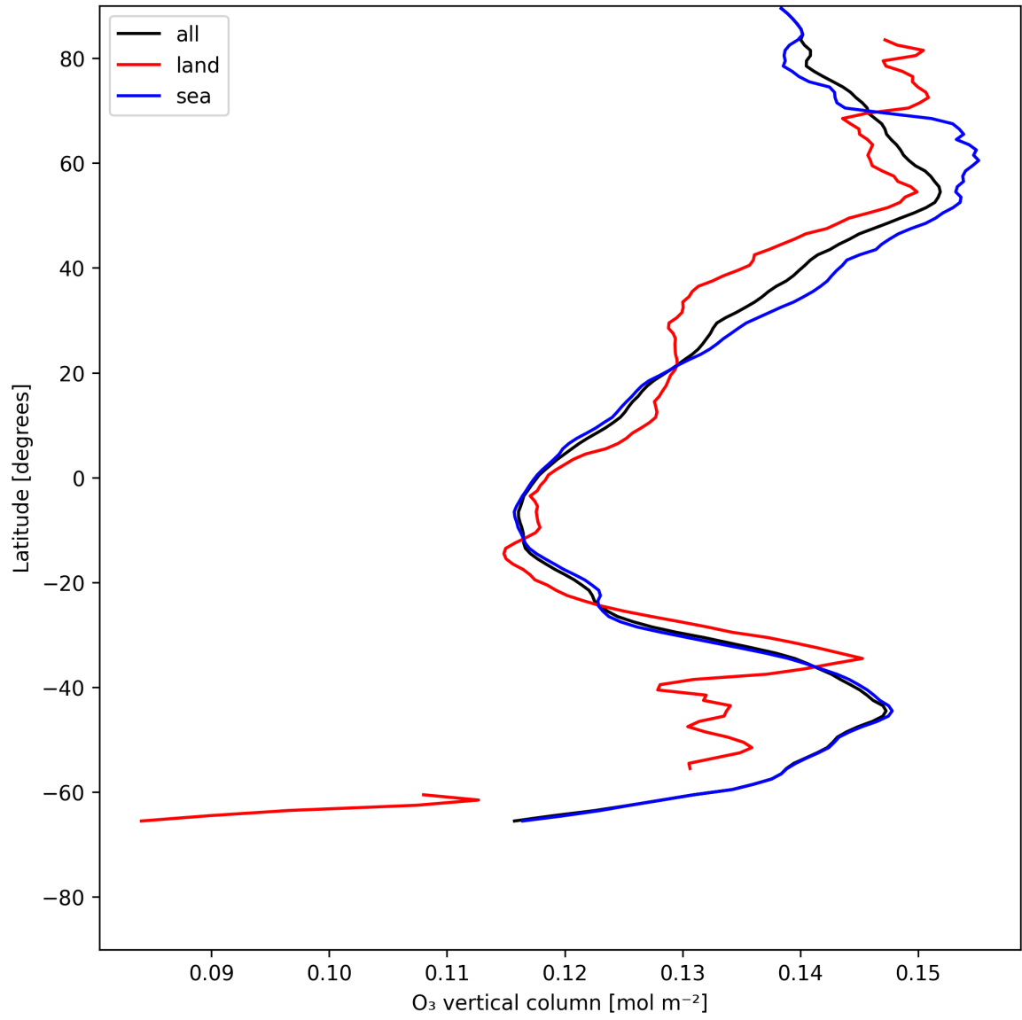
Figure 14: Zonal average of “O 3 vertical column” for 2025-07-02 to 2025-07-03.
