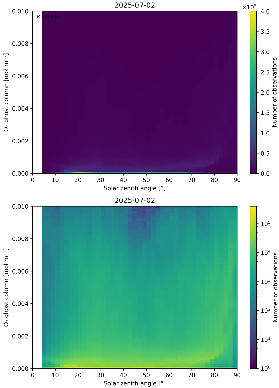
Figure 46: Scatter density plot of “Solar zenith angle” against “O 3 ghost column” for 2025-07-02 to 2025-07-03.
