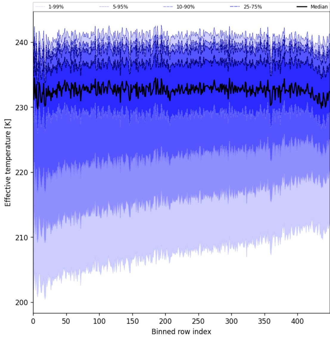
Figure 31: Along track statistics of “Effective temperature” for 2025-07-02 to 2025-07-03
