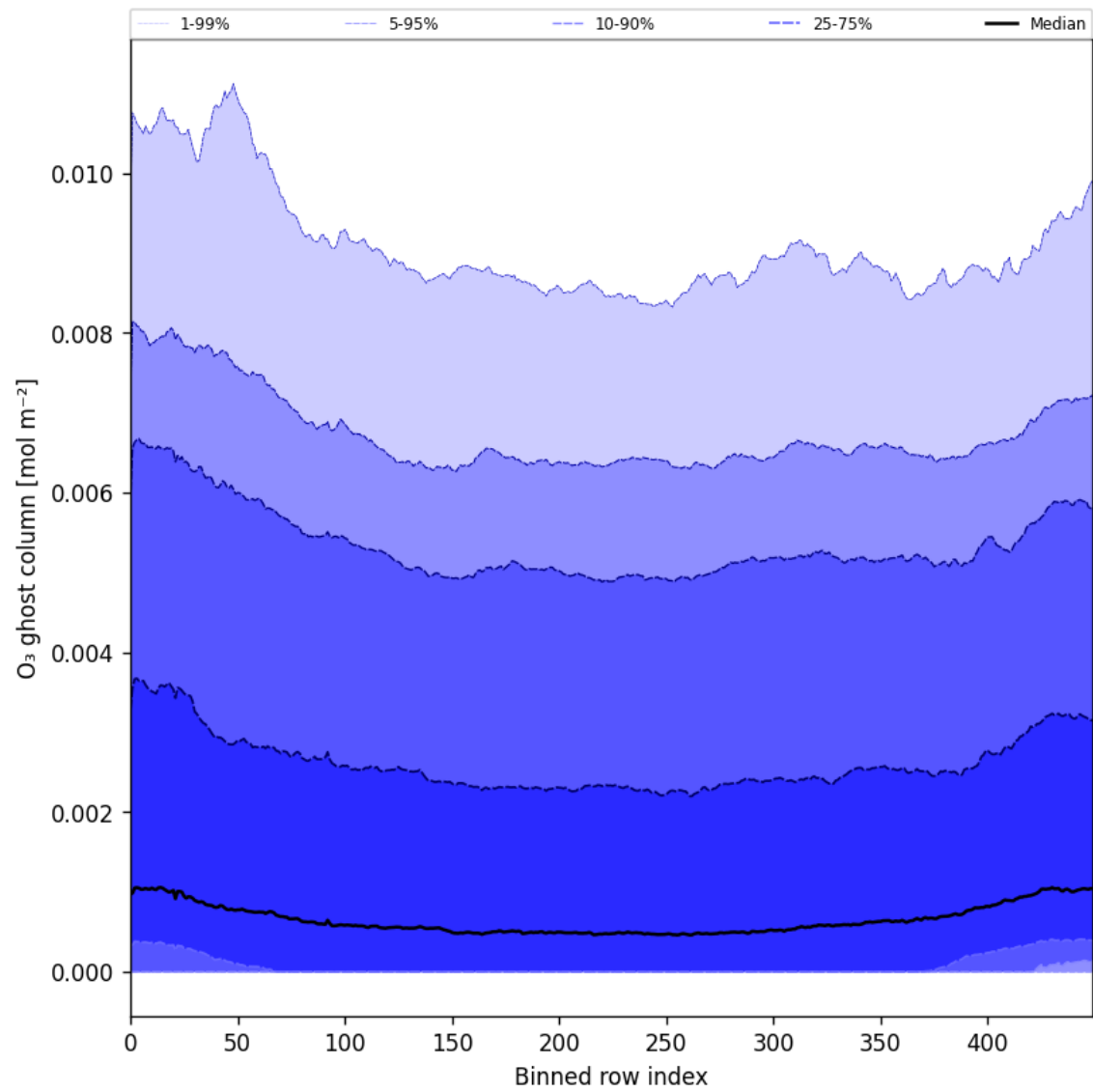
Figure 32: Along track statistics of “O 3 ghost column” for 2025-07-02 to 2025-07-03
