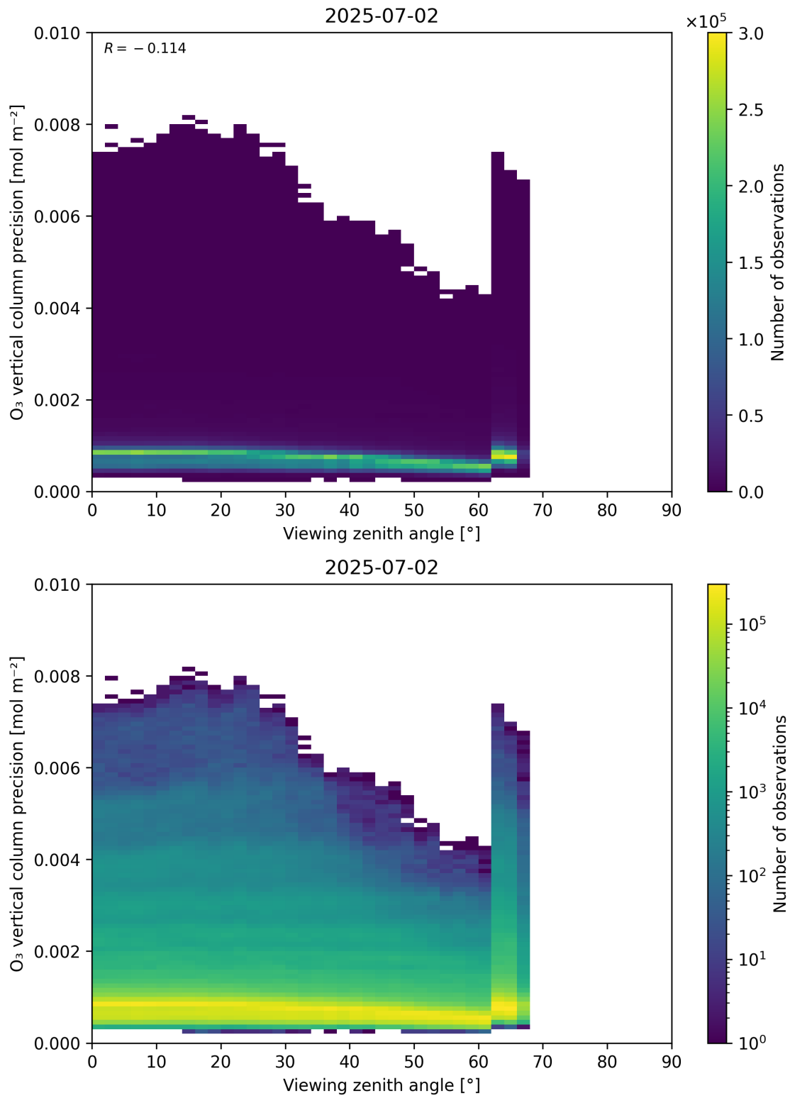
Figure 53: Scatter density plot of “Viewing zenith angle” against “O 3 vertical column precision” for 2025-07-02 to 2025-07-03.
