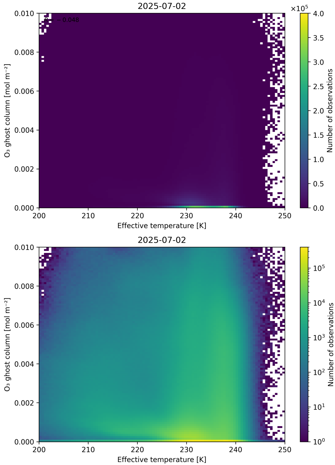
Figure 38: Scatter density plot of “Effective temperature” against “O 3 ghost column” for 2025-07-02 to 2025-07-03.
