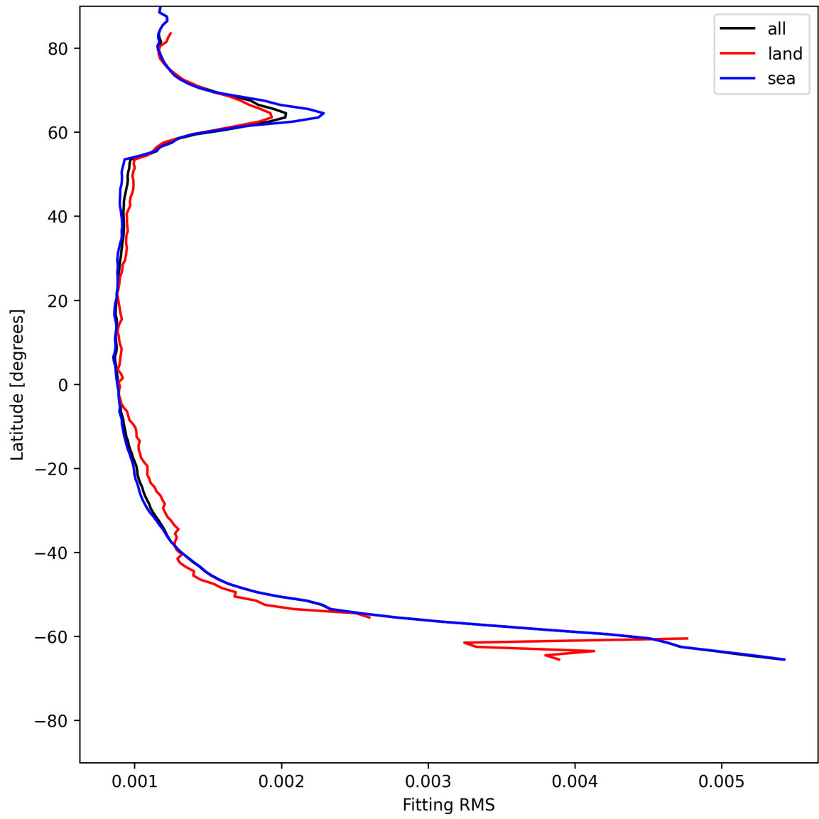
Figure 16: Zonal average of “Fitting RMS” for 2025-07-02 to 2025-07-03.
