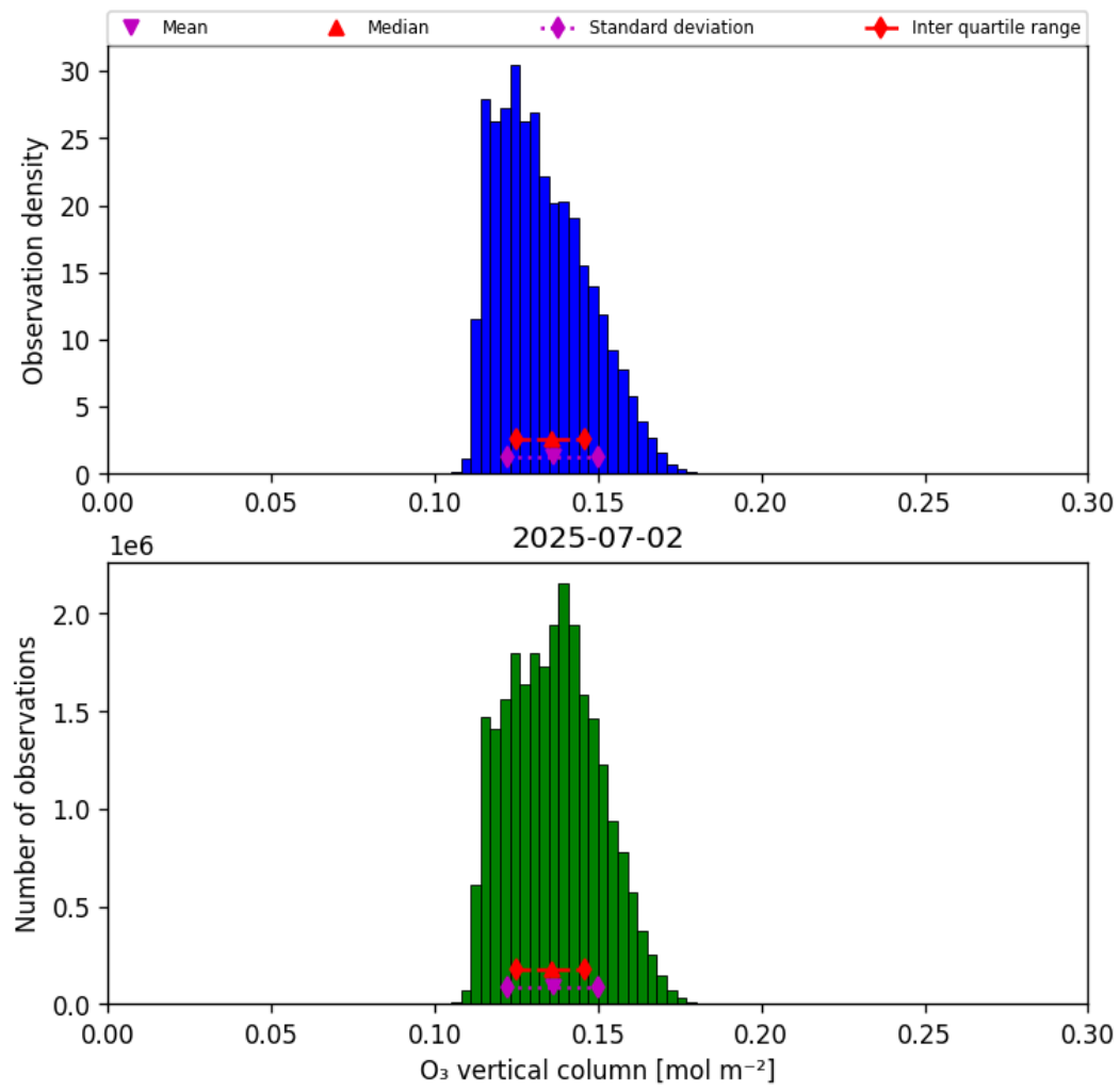
Figure 21: Histogram of “O 3 vertical column” for 2025-07-02 to 2025-07-03
