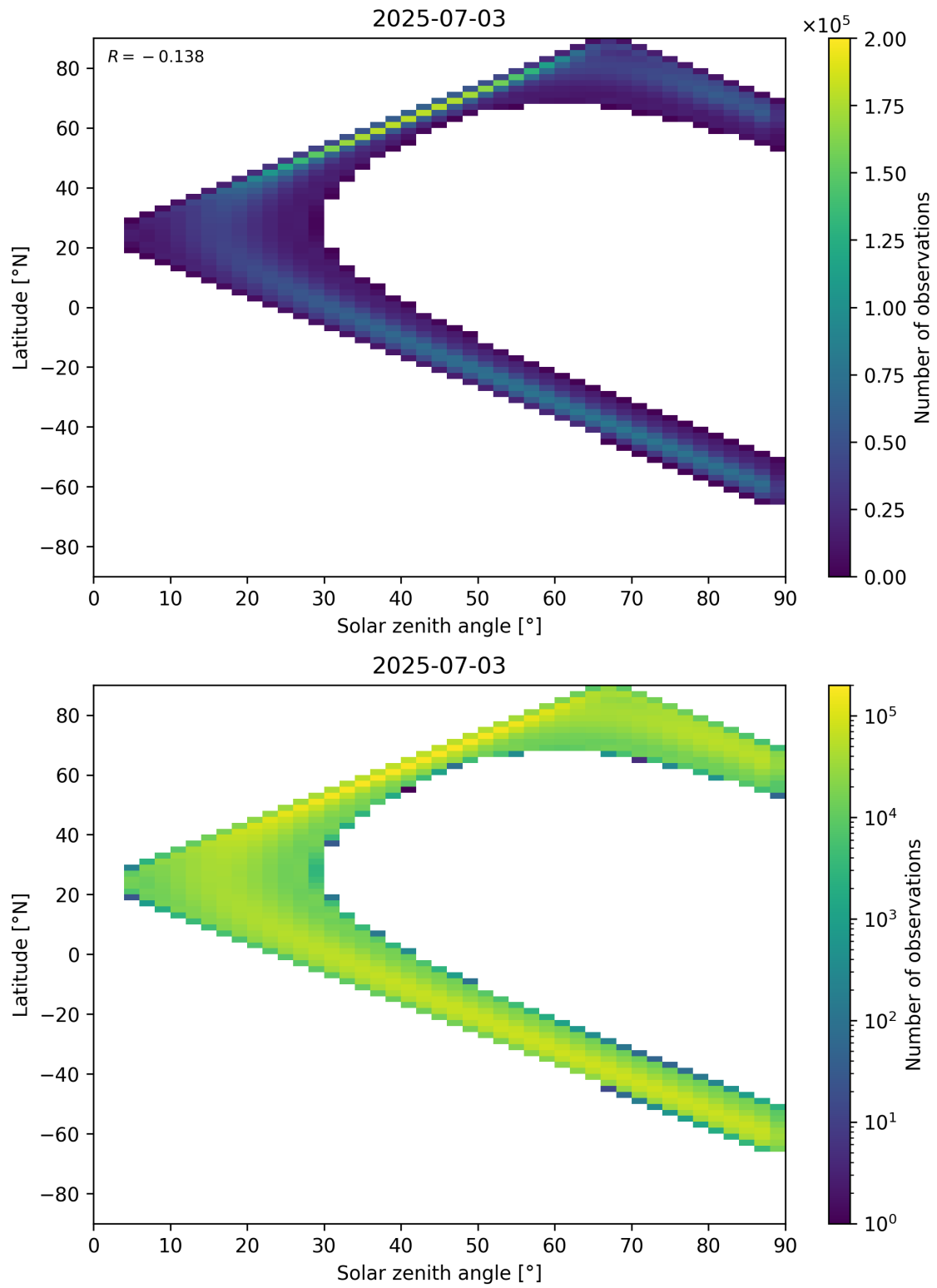
Figure 44: Scatter density plot of “Solar zenith angle” against “Latitude” for 2025-07-03 to 2025-07-04.
