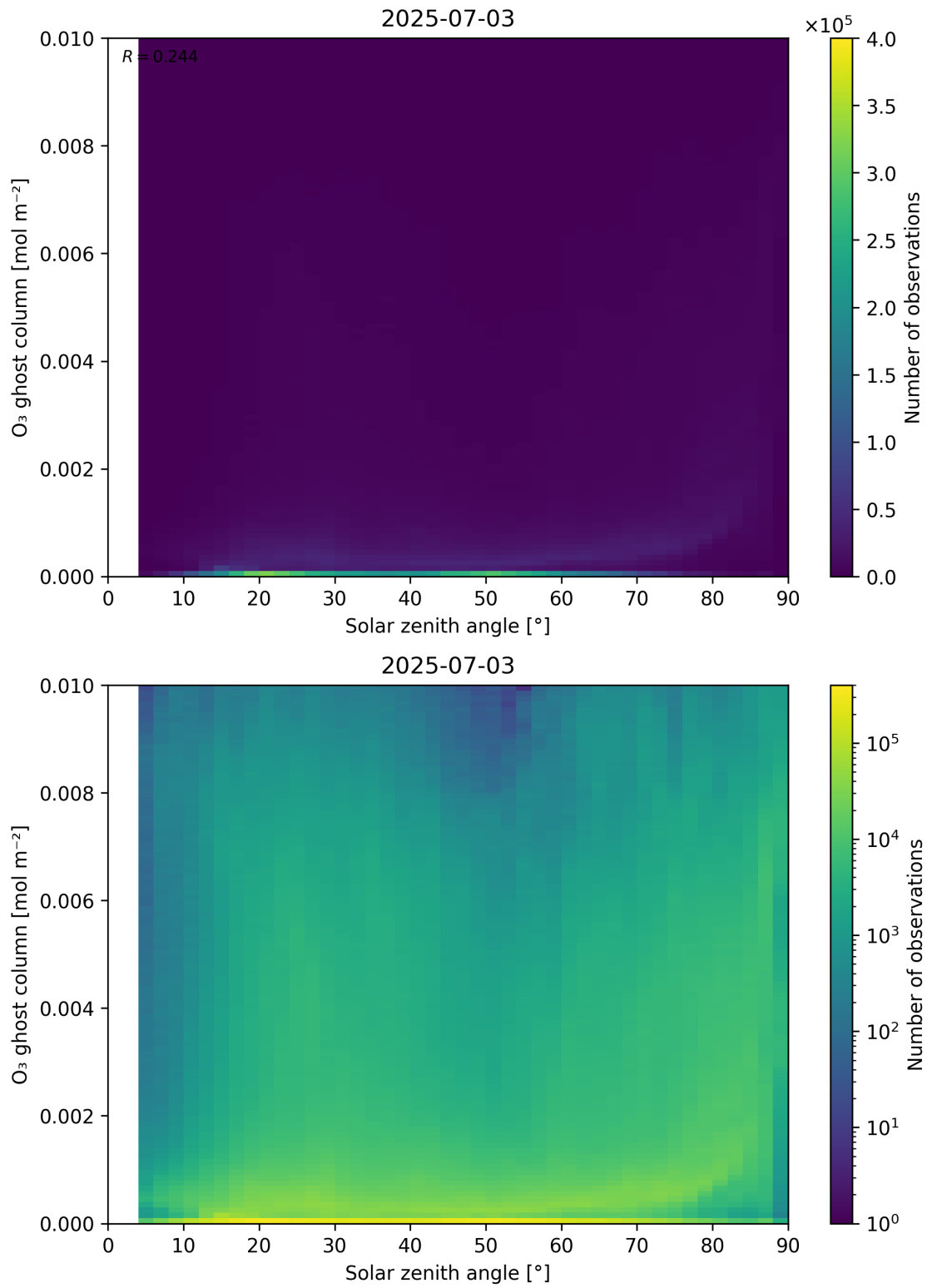
Figure 46: Scatter density plot of “Solar zenith angle” against “O 3 ghost column” for 2025-07-03 to 2025-07-04.
