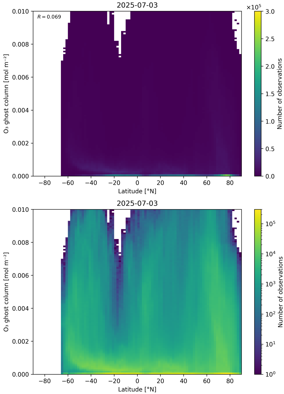
Figure 35: Scatter density plot of “Latitude” against “O 3 ghost column” for 2025-07-03 to 2025-07-04.
