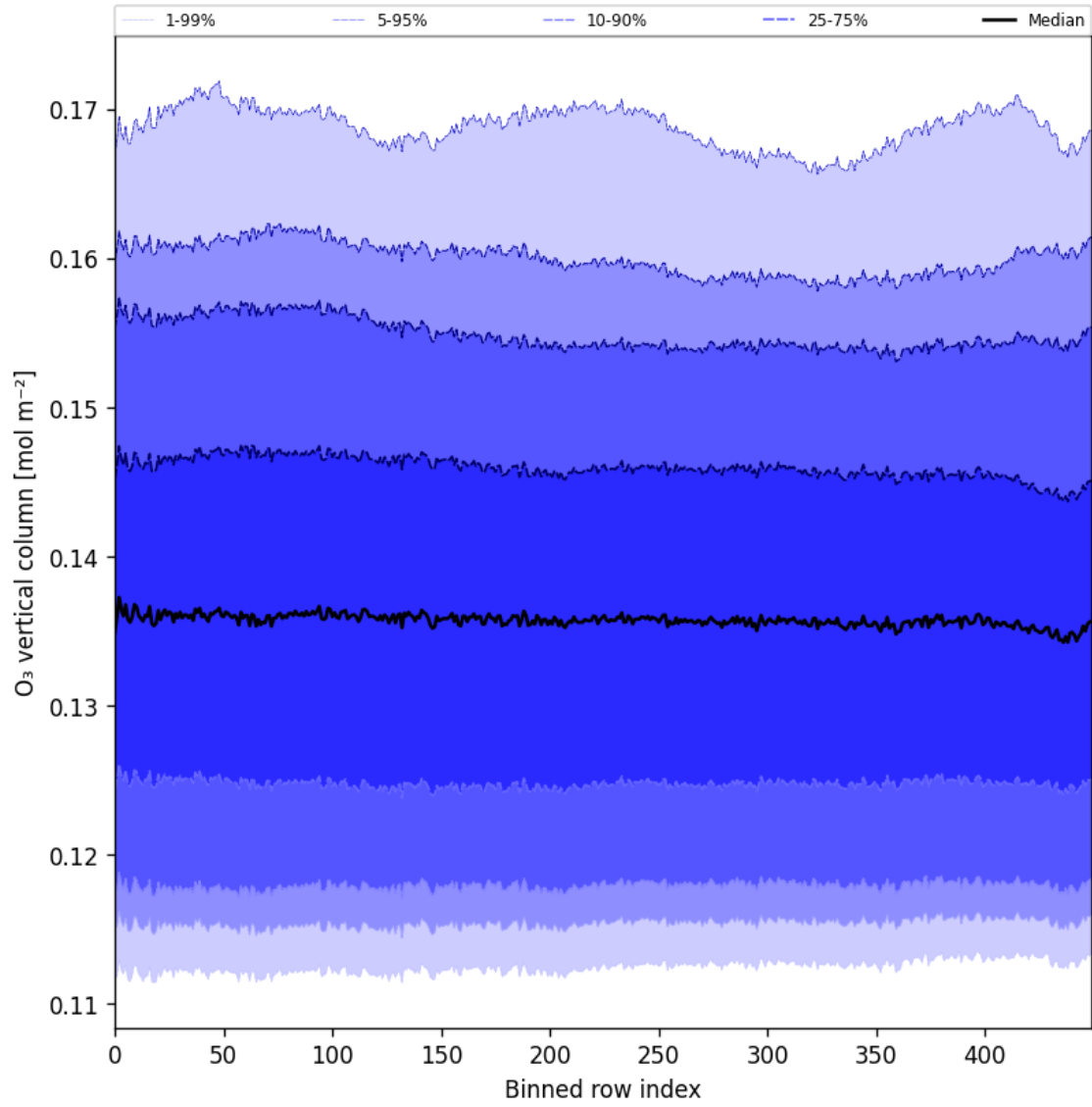
Figure 28: Along track statistics of “O 3 vertical column” for 2025-07-03 to 2025-07-04
