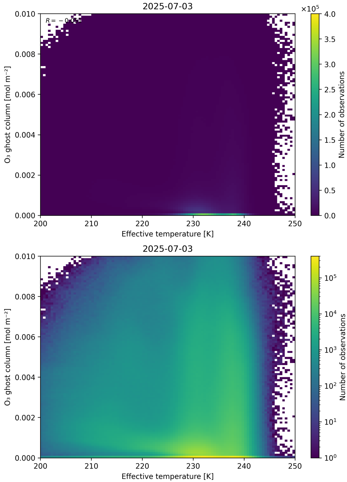
Figure 38: Scatter density plot of “Effective temperature” against “O 3 ghost column” for 2025-07-03 to 2025-07-04.
