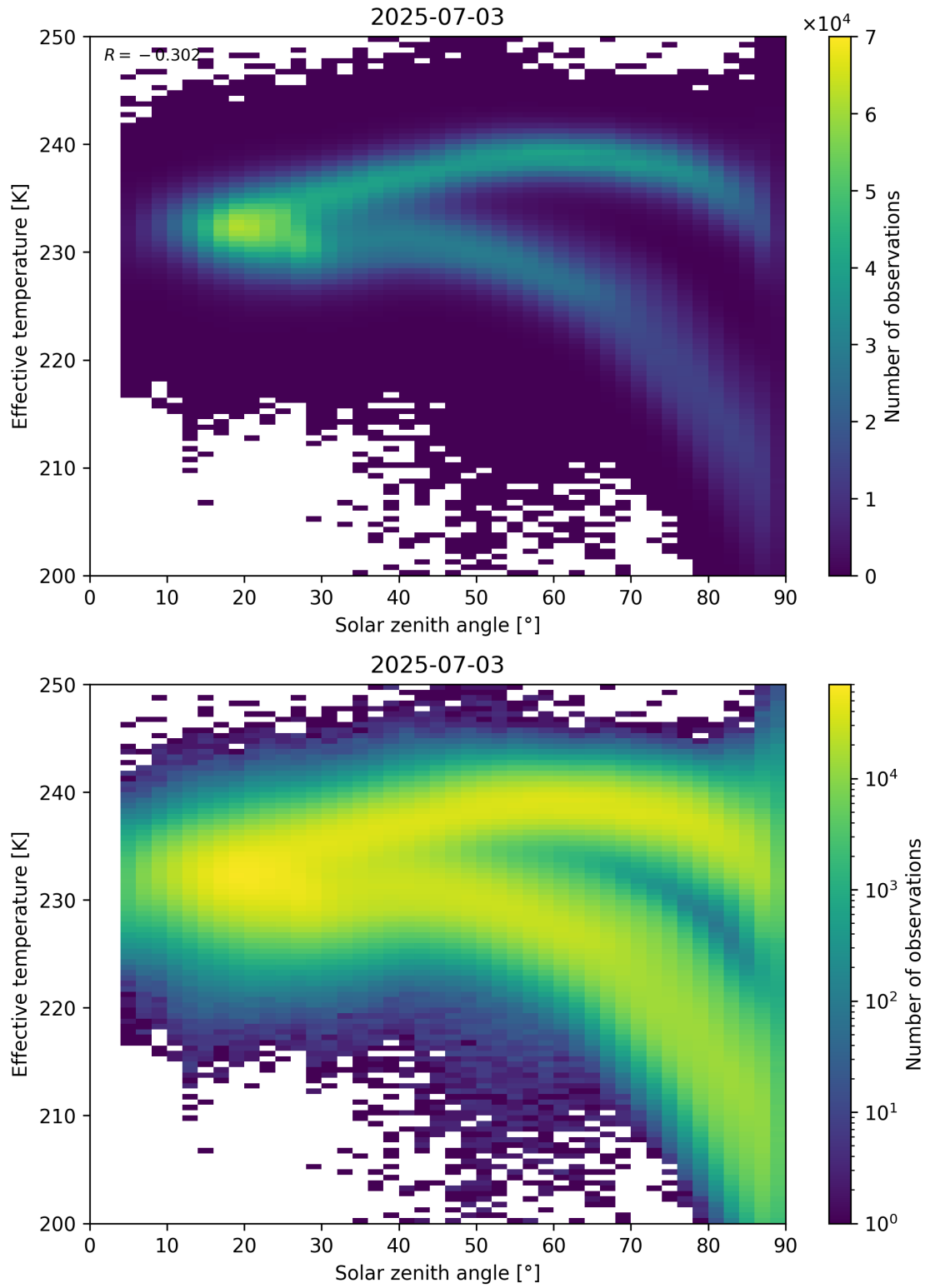
Figure 45: Scatter density plot of “Solar zenith angle” against “Effective temperature” for 2025-07-03 to 2025-07-04.
