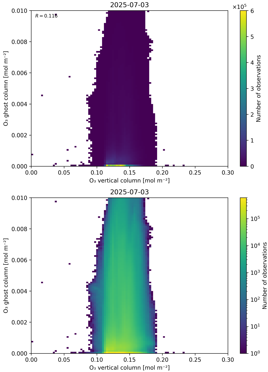
Figure 40: Scatter density plot of “O 3 vertical column” against “O 3 ghost column” for 2025-07-03 to 2025-07-04.
