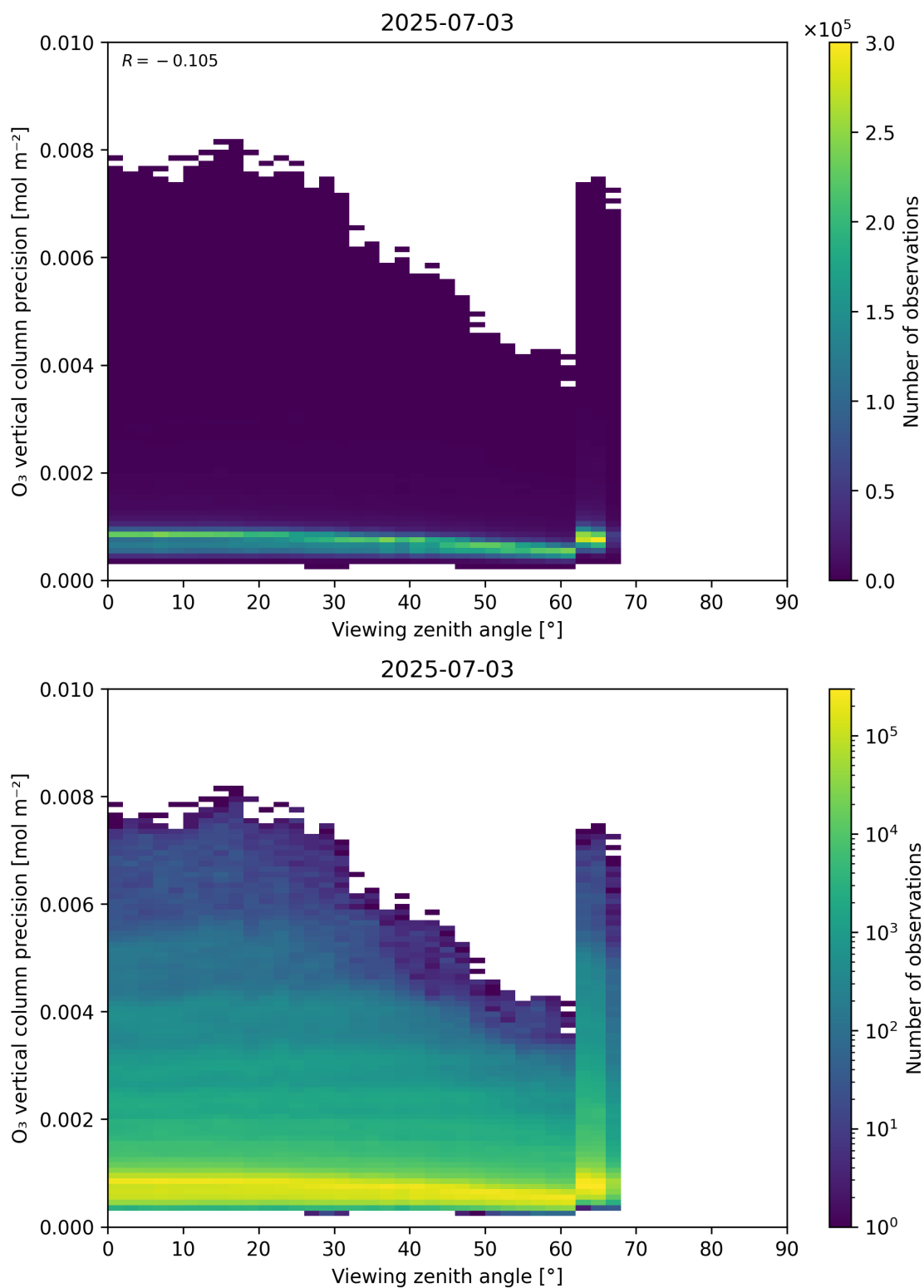
Figure 53: Scatter density plot of “Viewing zenith angle” against “O 3 vertical column precision” for 2025-07-03 to 2025-07-04.
