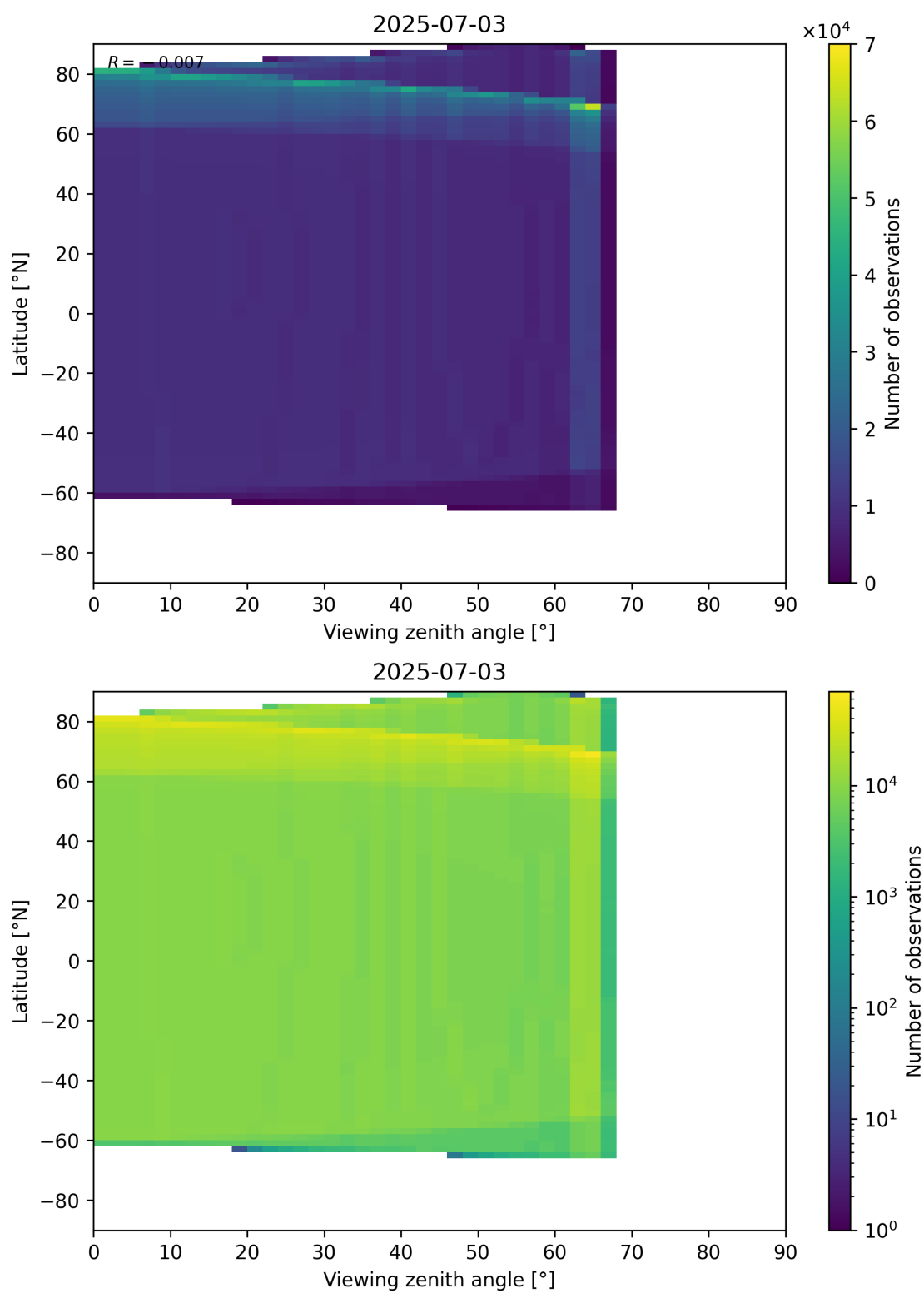
Figure 49: Scatter density plot of “Viewing zenith angle” against “Latitude” for 2025-07-03 to 2025-07-04.
