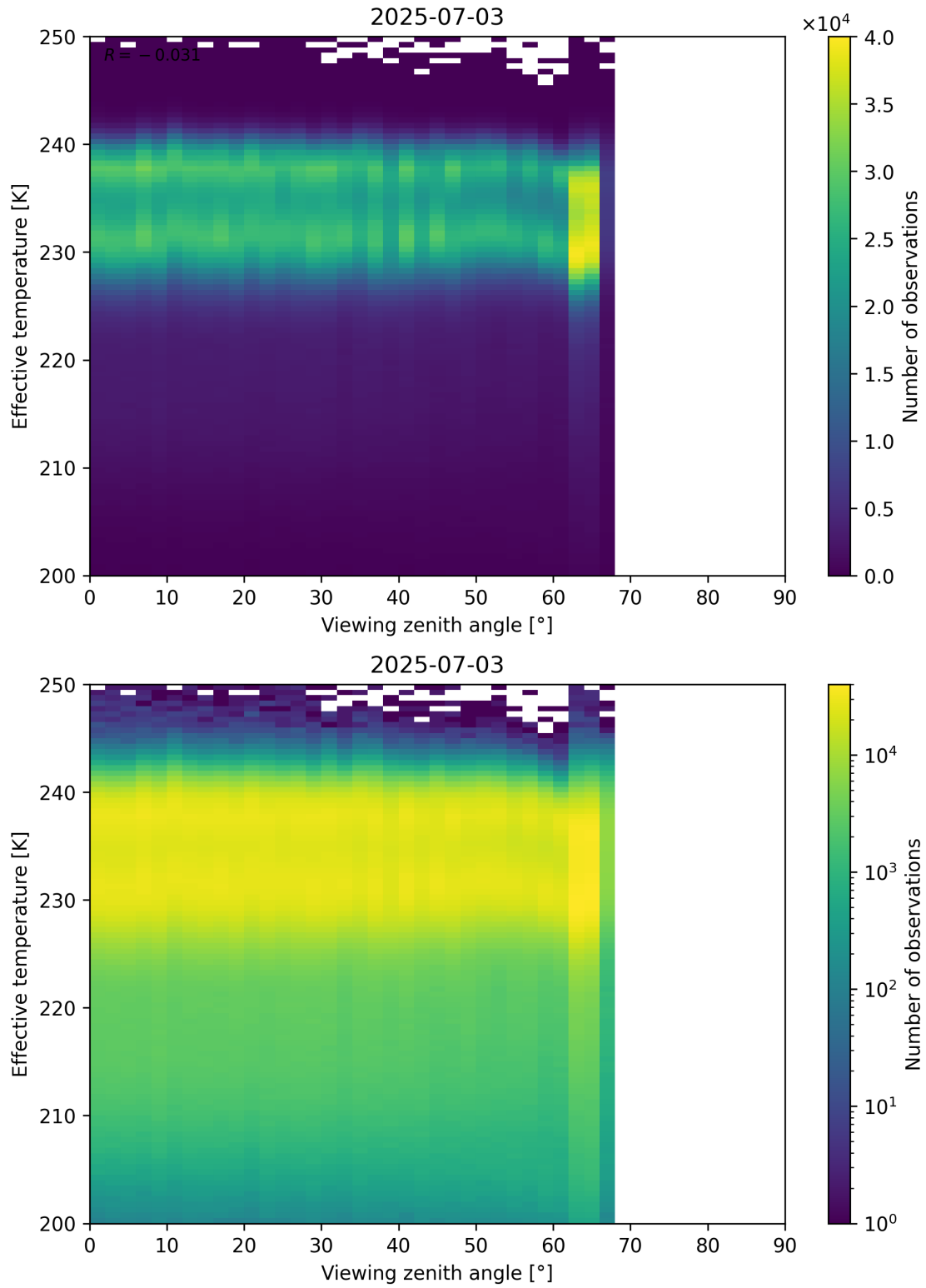
Figure 50: Scatter density plot of “Viewing zenith angle” against “Effective temperature” for 2025-07-03 to 2025-07-04.
