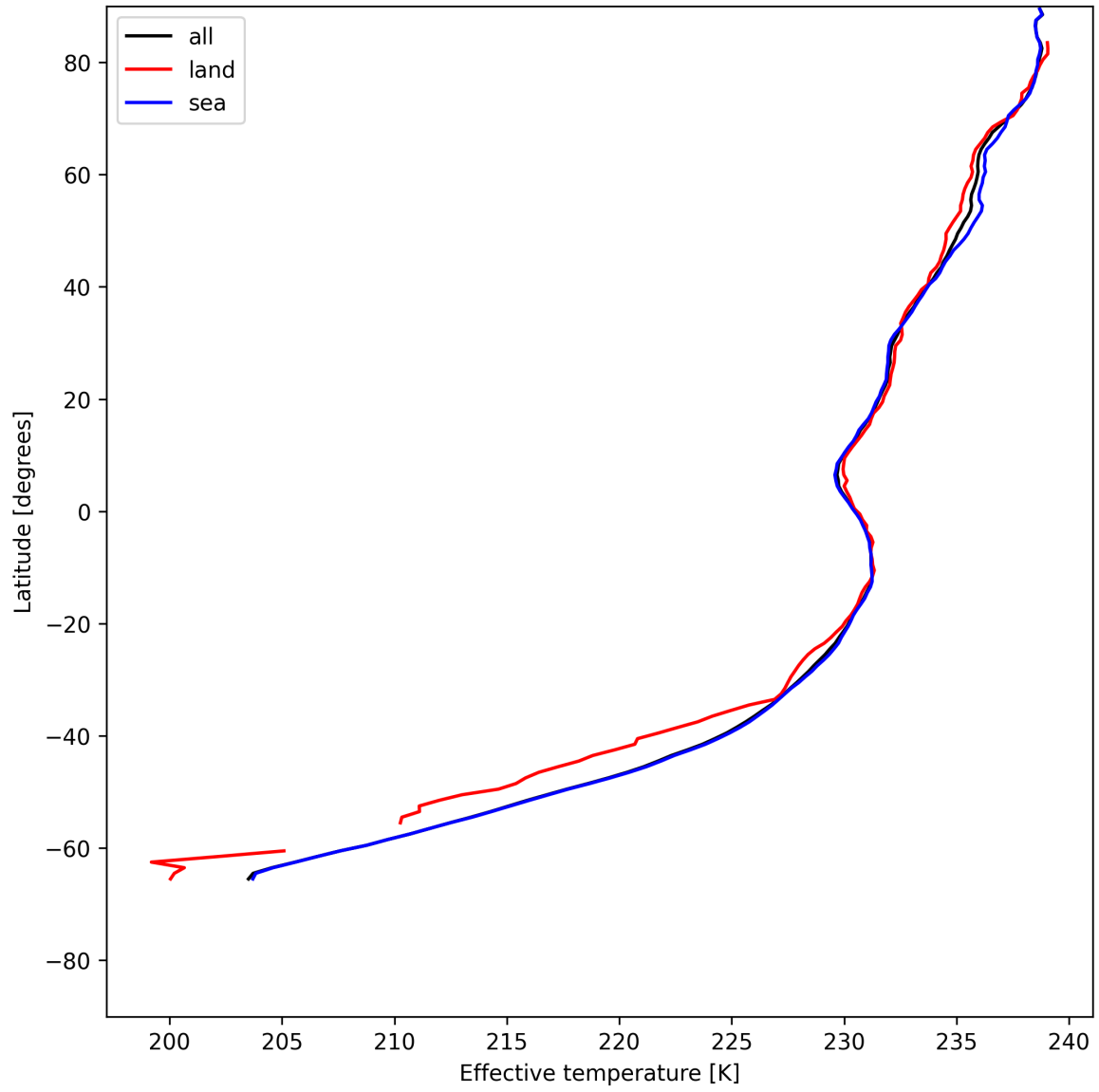
Figure 17: Zonal average of "Effective temperature" for 2025-07-03 to 2025-07-04.
