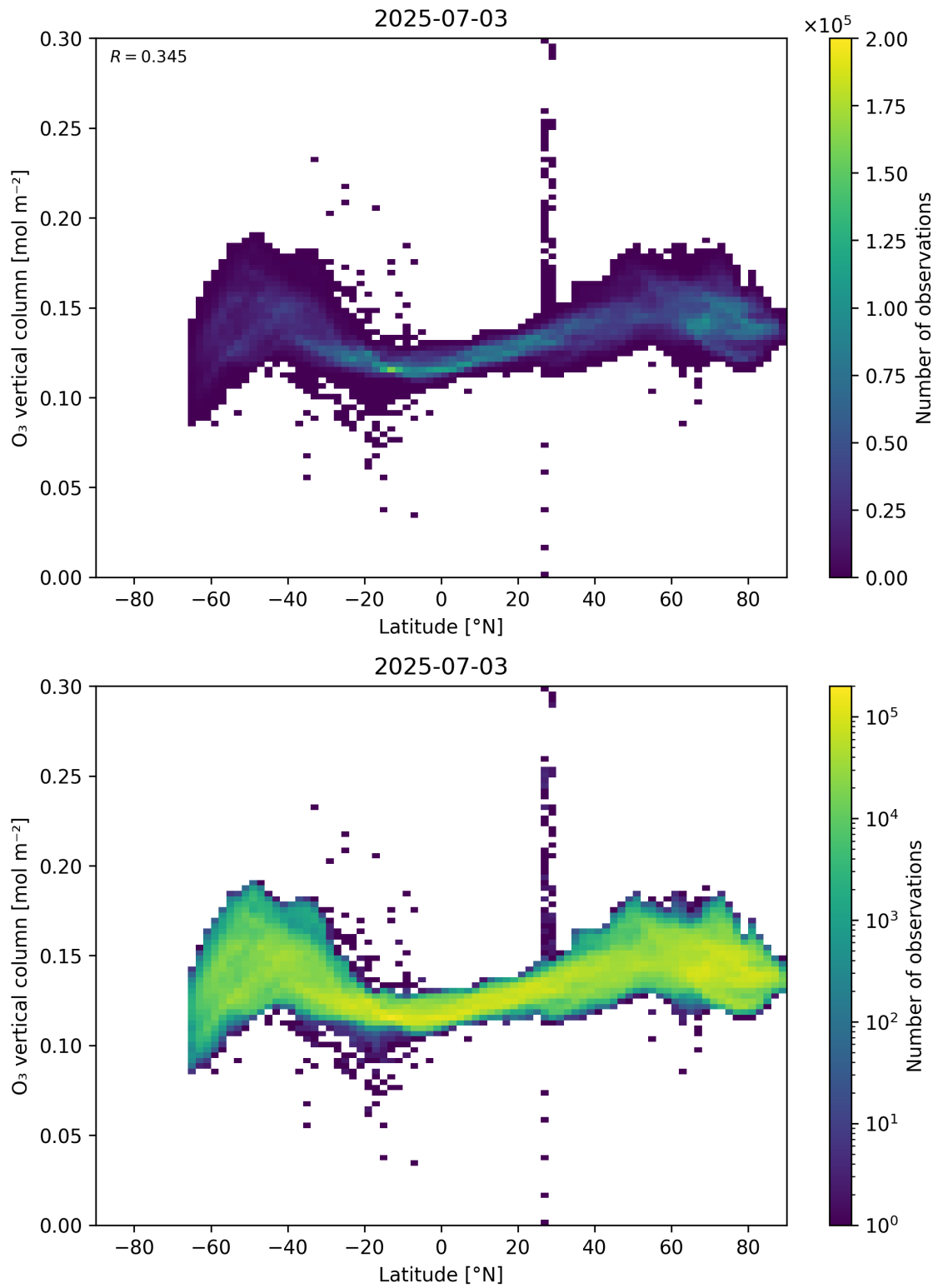
Figure 36: Scatter density plot of “Latitude” against “O 3 vertical column” for 2025-07-03 to 2025-07-04.
