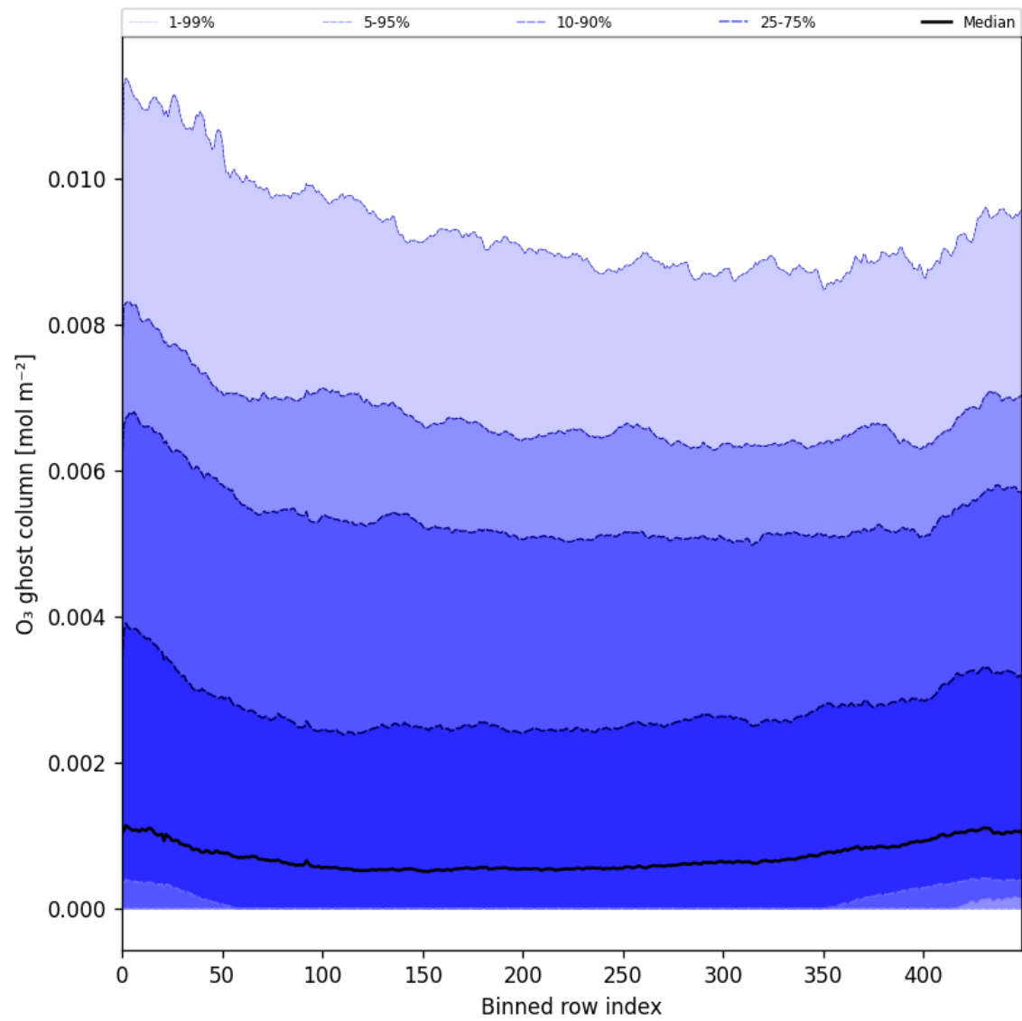
Figure 32: Along track statistics of “O 3 ghost column” for 2025-07-03 to 2025-07-04
