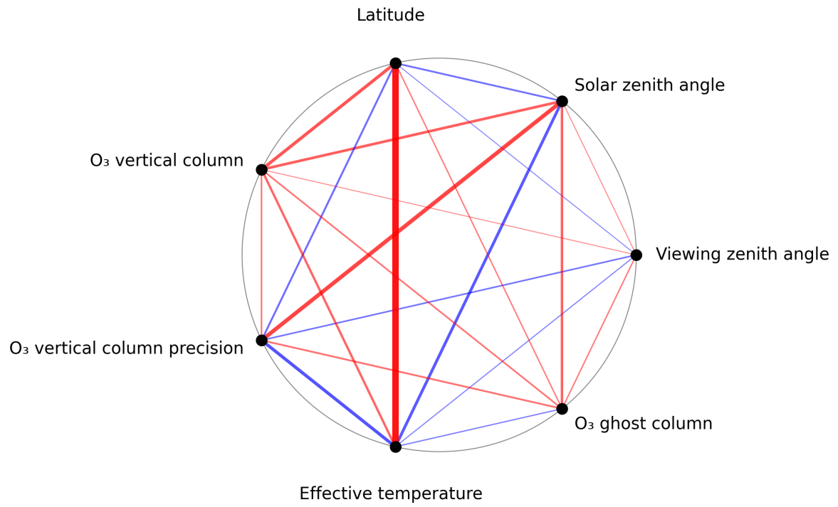
Figure 1: Map of correlation graph for 2025-07-03 to 2025-07-04.
