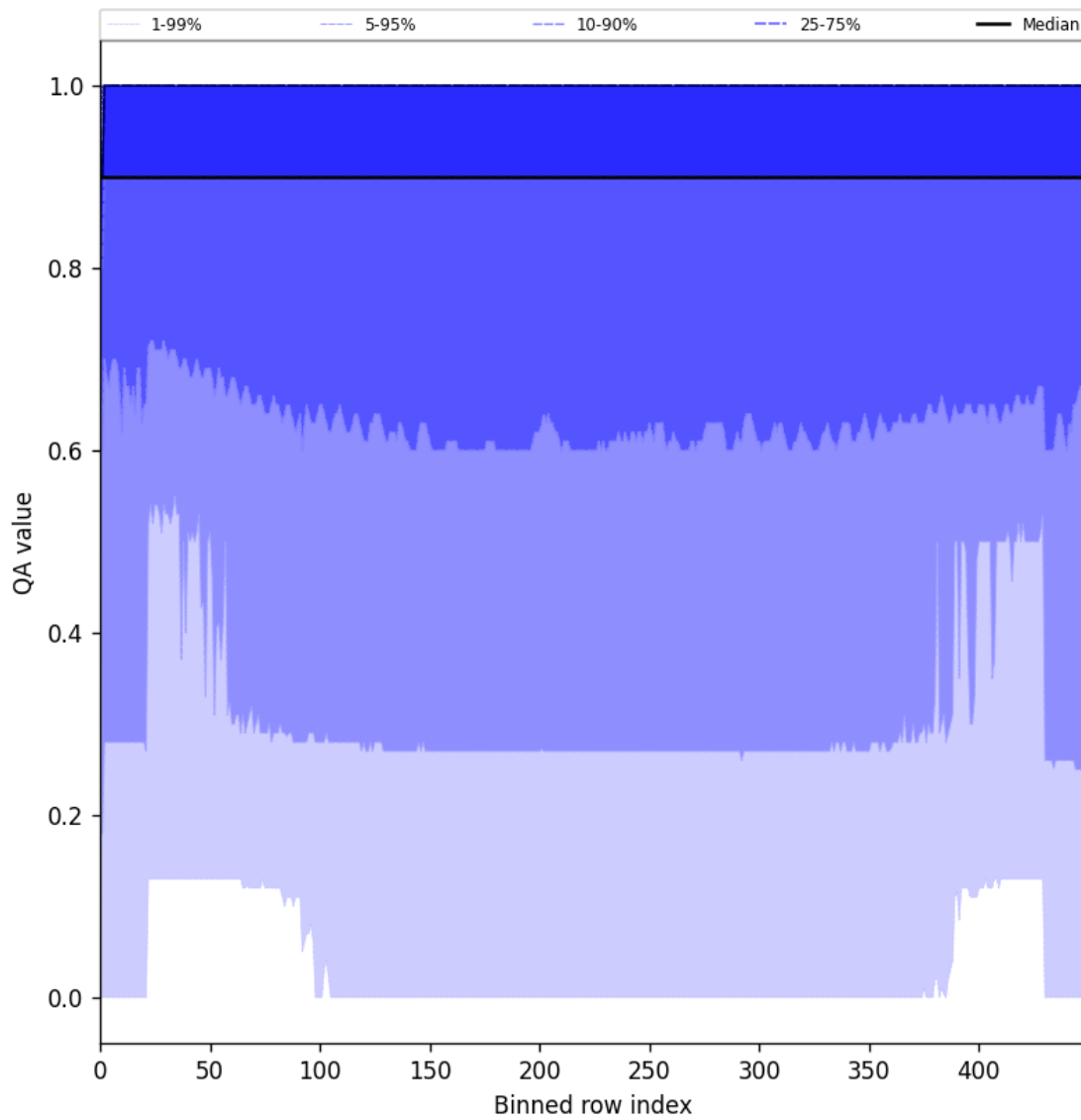
Figure 27: Along track statistics of “QA value” for 2025-07-03 to 2025-07-04
