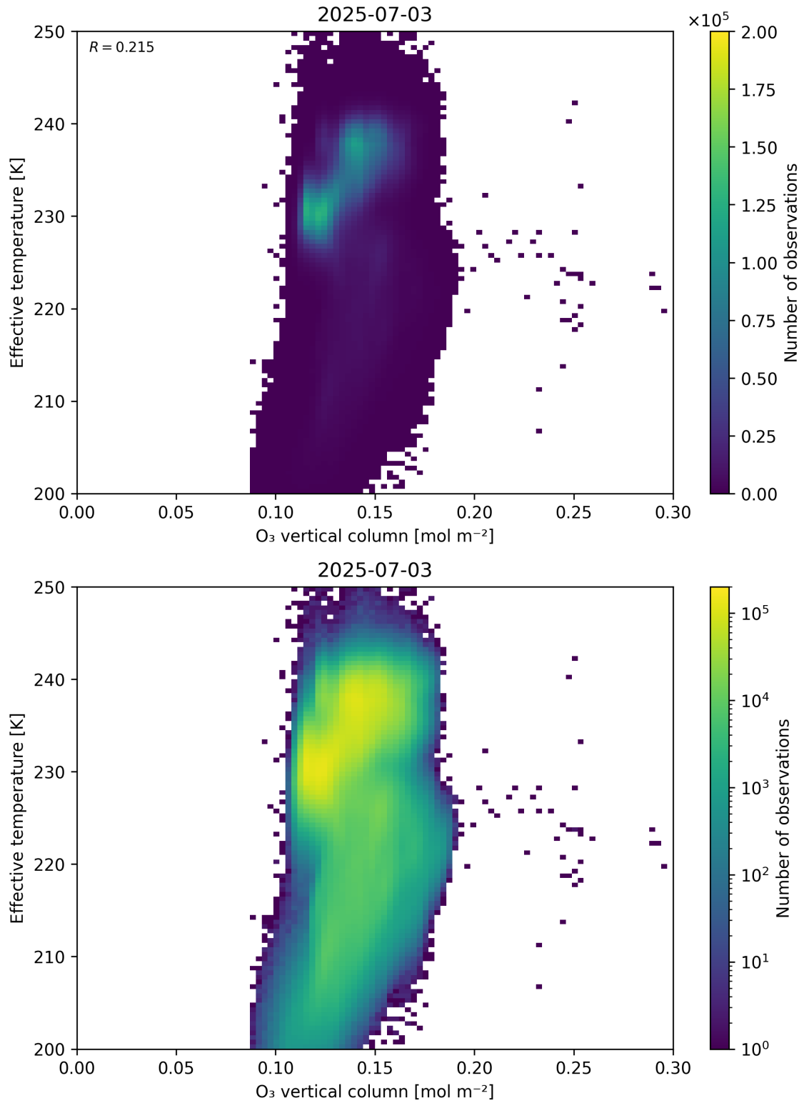
Figure 39: Scatter density plot of “O 3 vertical column” against “Effective temperature” for 2025-07-03 to 2025-07-04.
