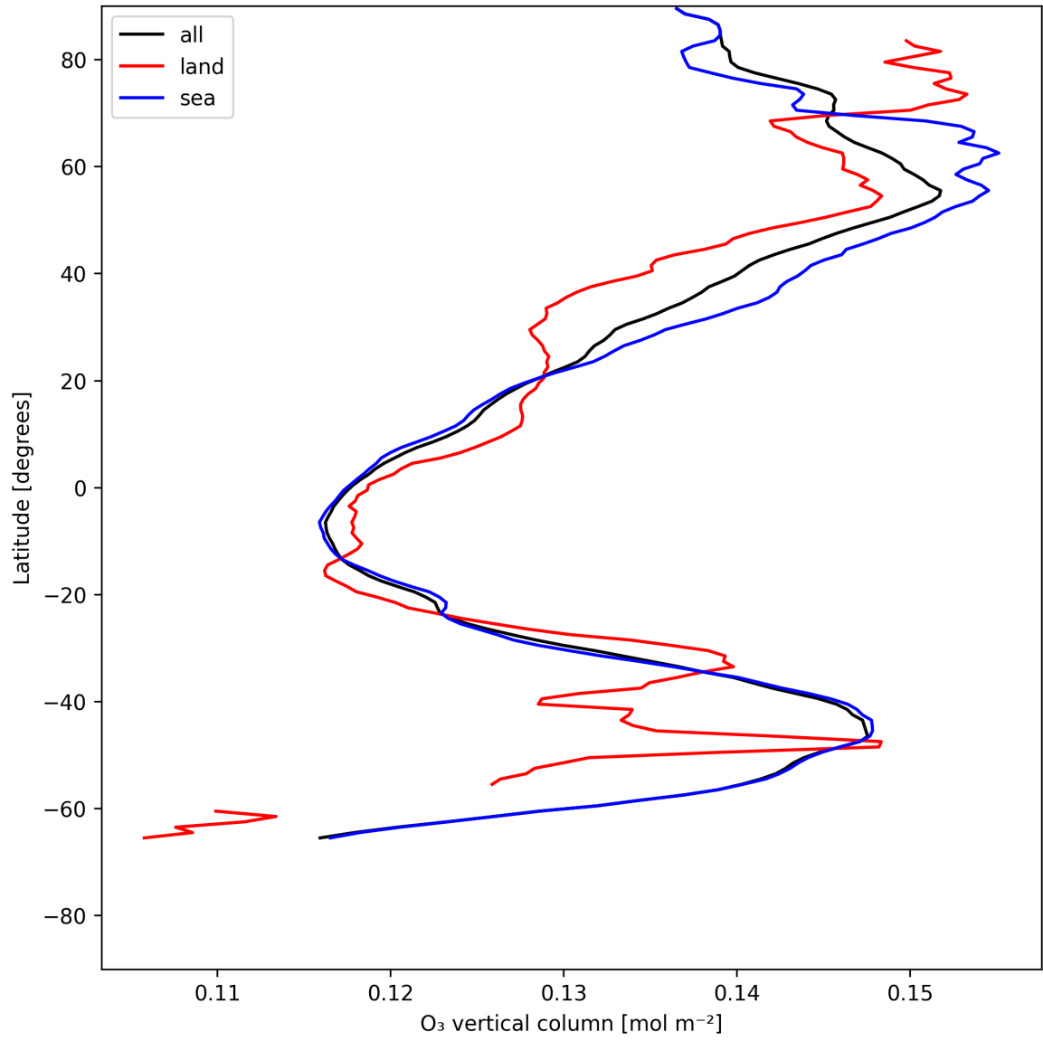
Figure 14: Zonal average of “O 3 vertical column” for 2025-07-03 to 2025-07-04.
