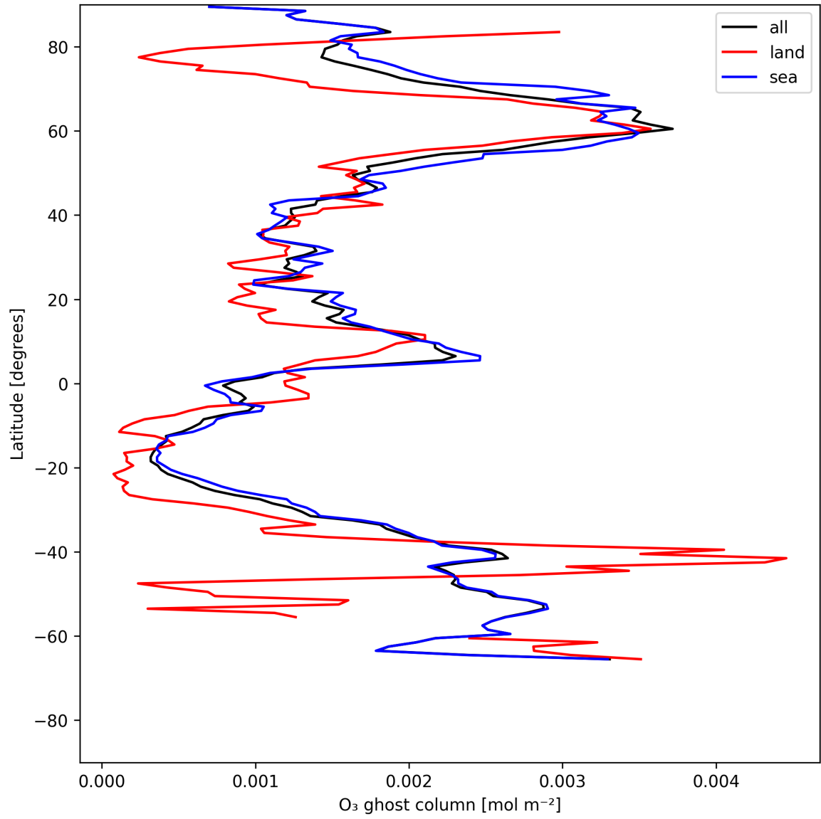
Figure 18: Zonal average of "O 3 ghost column" for 2025-07-03 to 2025-07-04.
