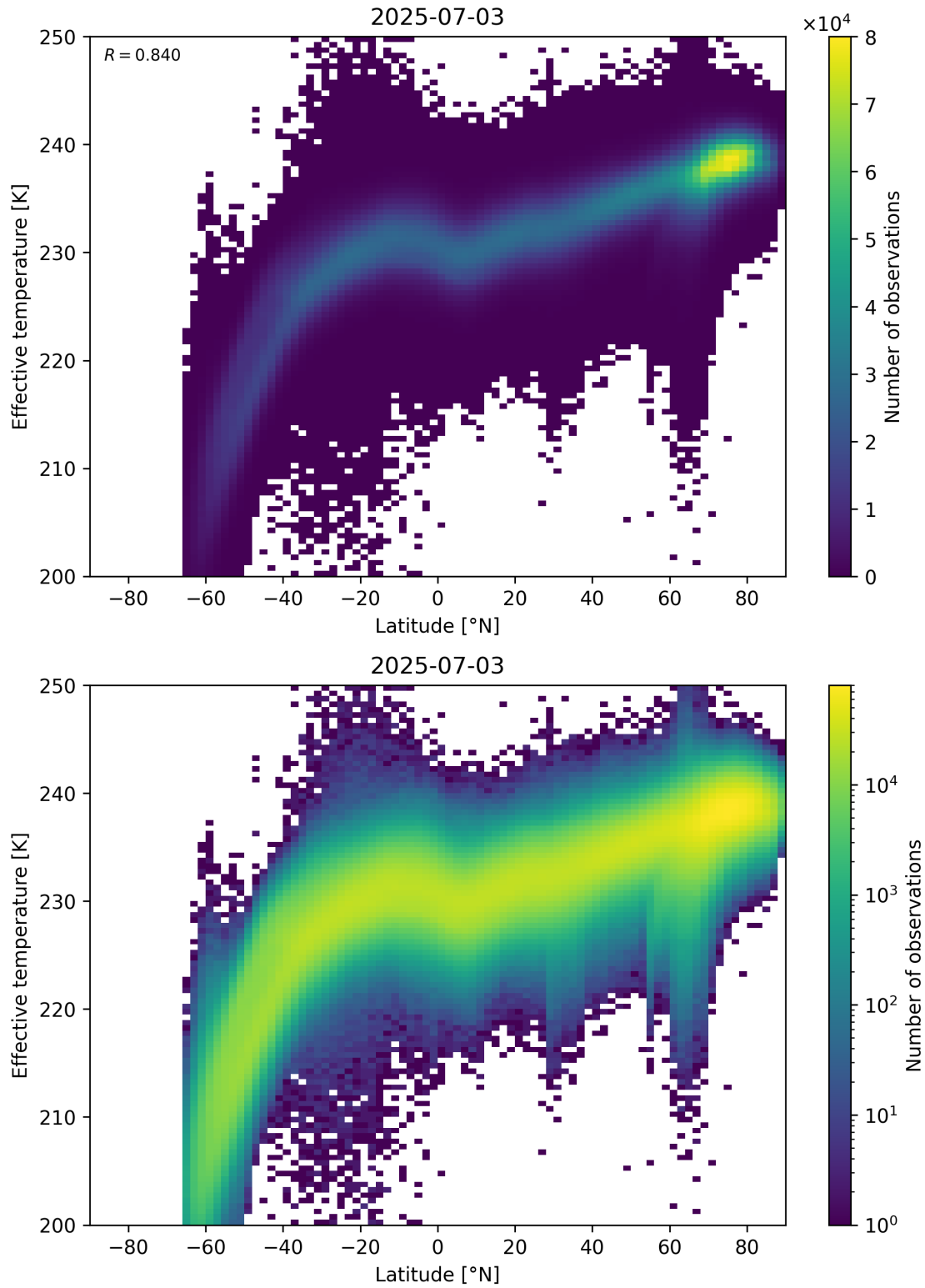
Figure 34: Scatter density plot of “Latitude” against “Effective temperature” for 2025-07-03 to 2025-07-04.
