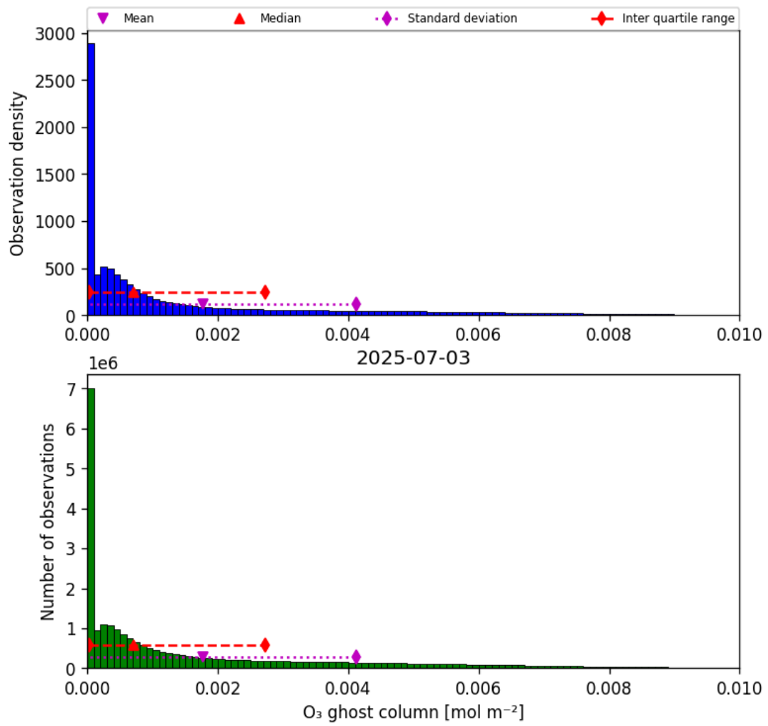
Figure 25: Histogram of “O 3 ghost column” for 2025-07-03 to 2025-07-04
