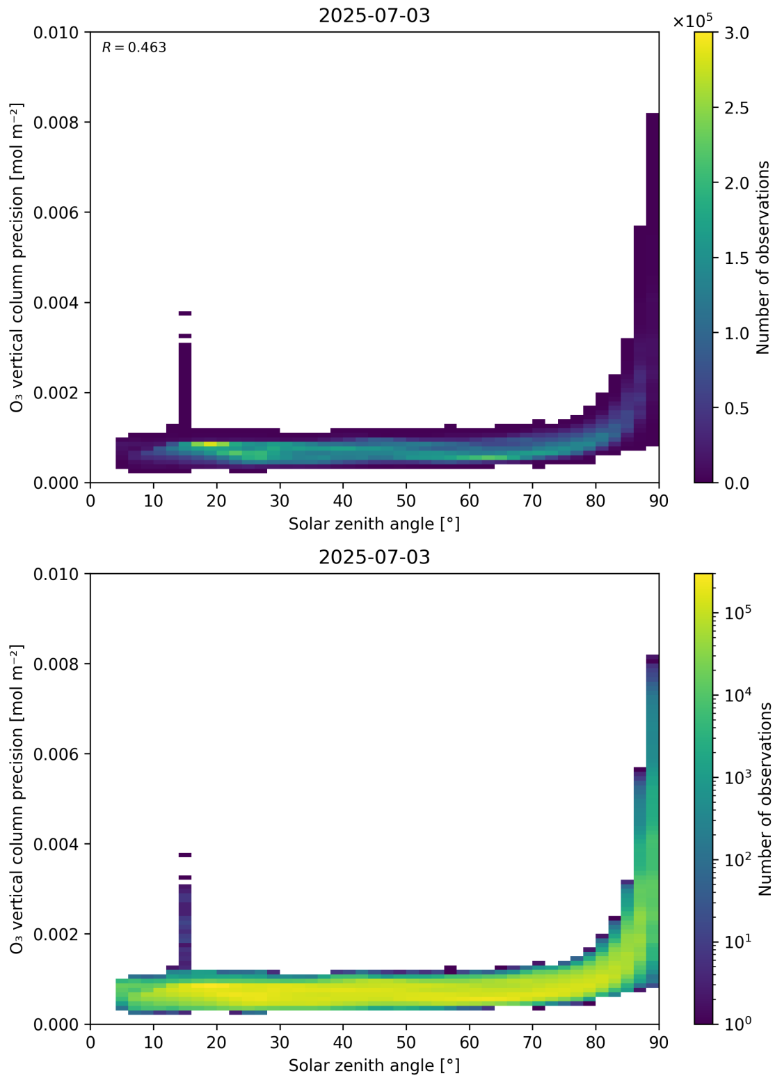
Figure 48: Scatter density plot of “Solar zenith angle” against “O 3 vertical column precision” for 2025-07-03 to 2025-07-04.
