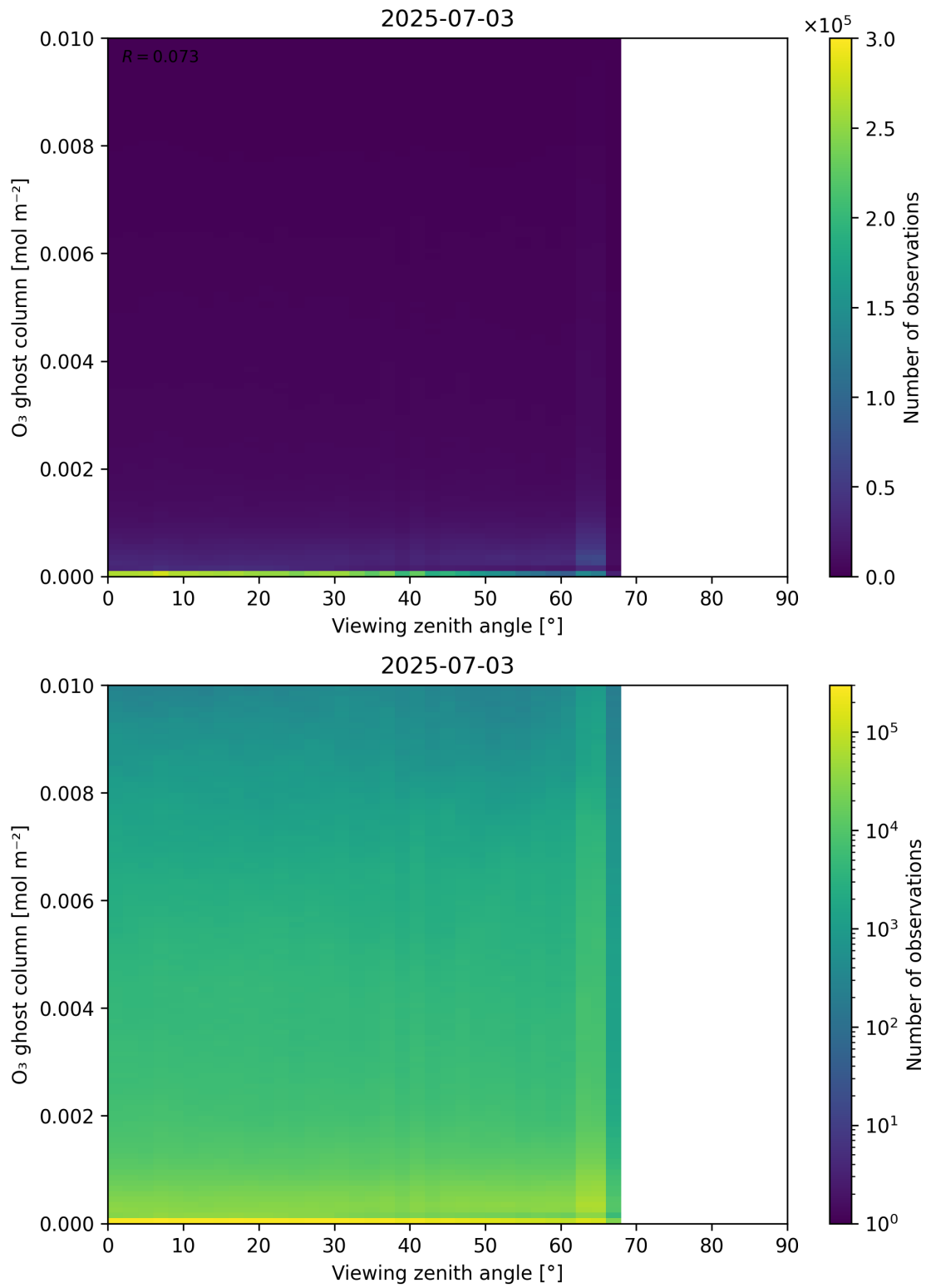
Figure 51: Scatter density plot of “Viewing zenith angle” against “O 3 ghost column” for 2025-07-03 to 2025-07-04.
