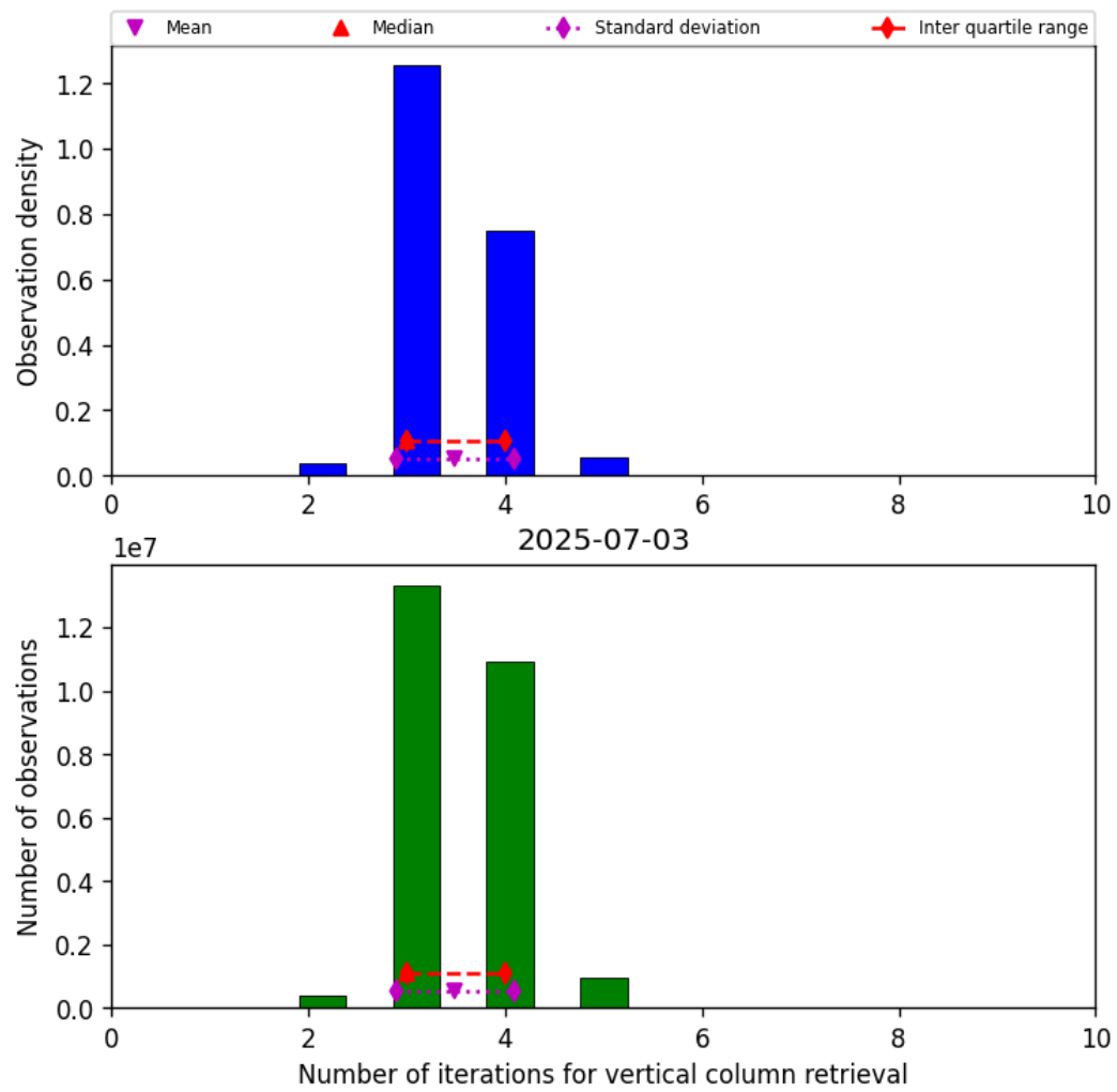
Figure 26: Histogram of “Number of iterations for vertical column retrieval” for 2025-07-03 to 2025-07-04
