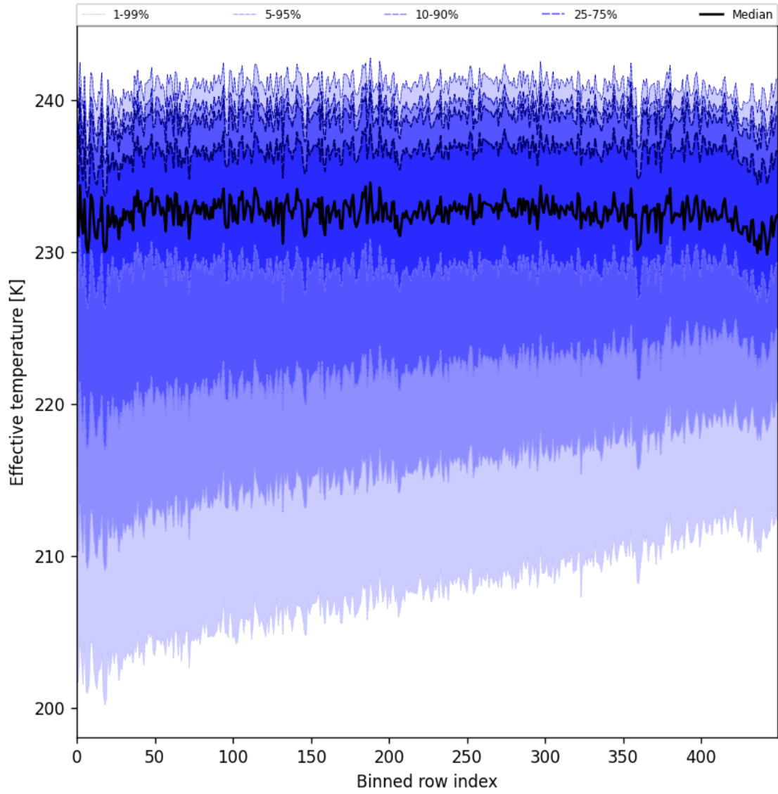
Figure 31: Along track statistics of “Effective temperature” for 2025-07-03 to 2025-07-04
