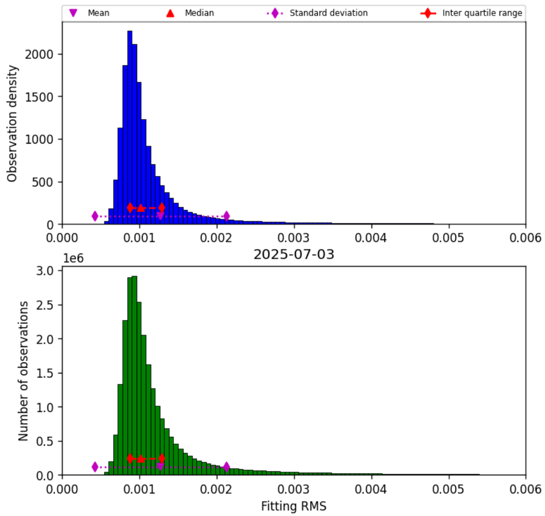
Figure 23: Histogram of “Fitting RMS” for 2025-07-03 to 2025-07-04
