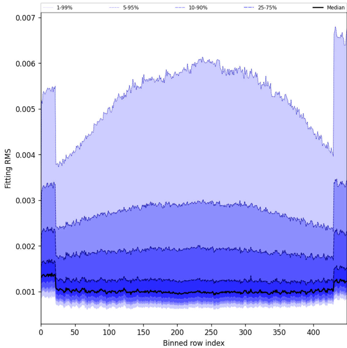
Figure 30: Along track statistics of “Fitting RMS” for 2025-07-03 to 2025-07-04
