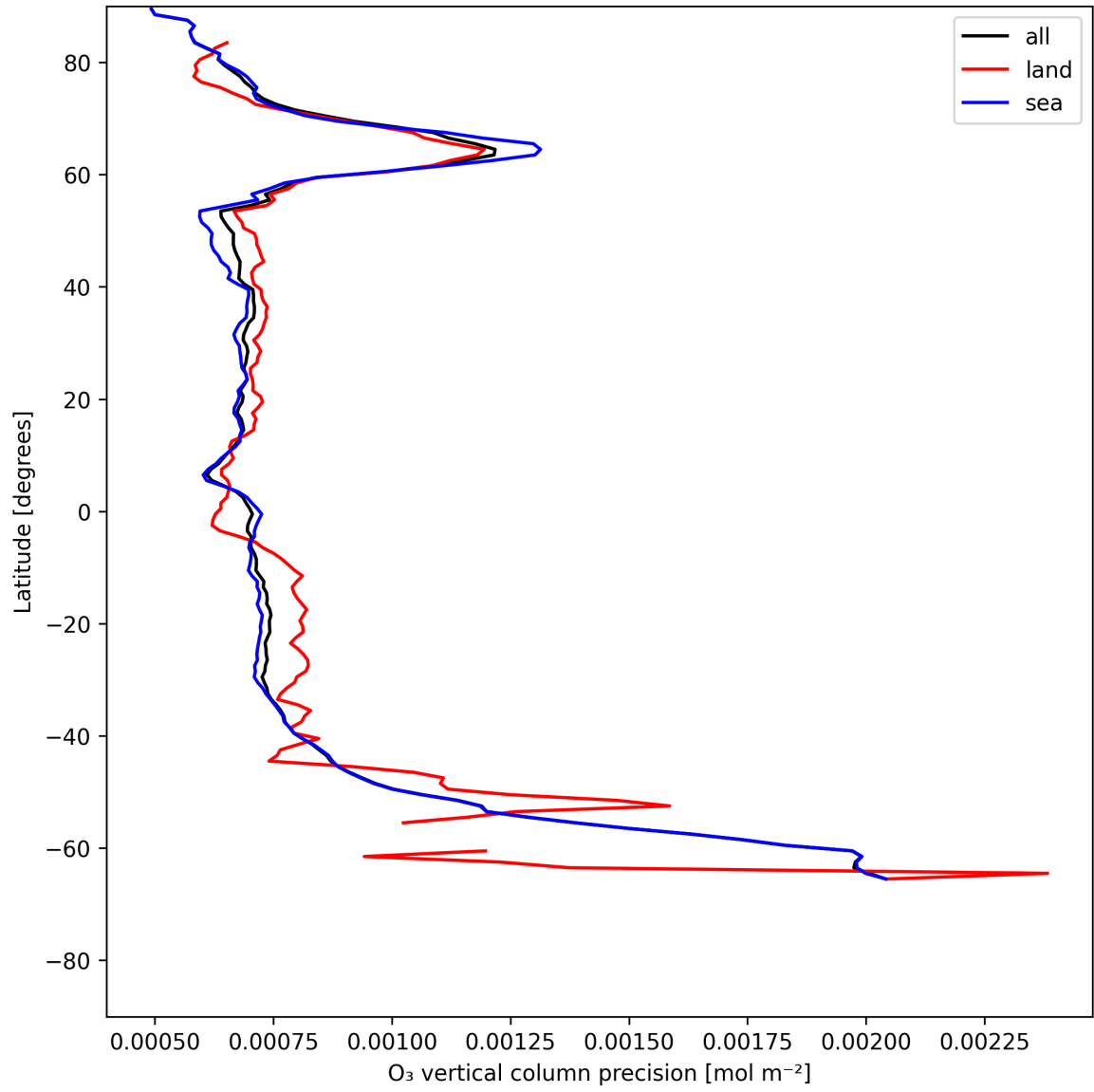
Figure 15: Zonal average of “O 3 vertical column precision” for 2025-07-03 to 2025-07-04.
