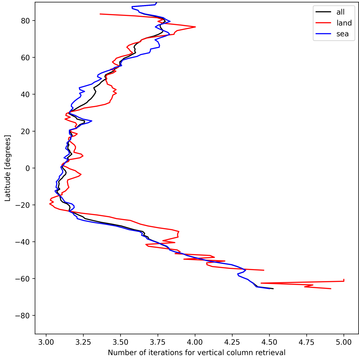
Figure 19: Zonal average of “Number of iterations for vertical column retrieval” for 2025-07-03 to 2025-07-04.
