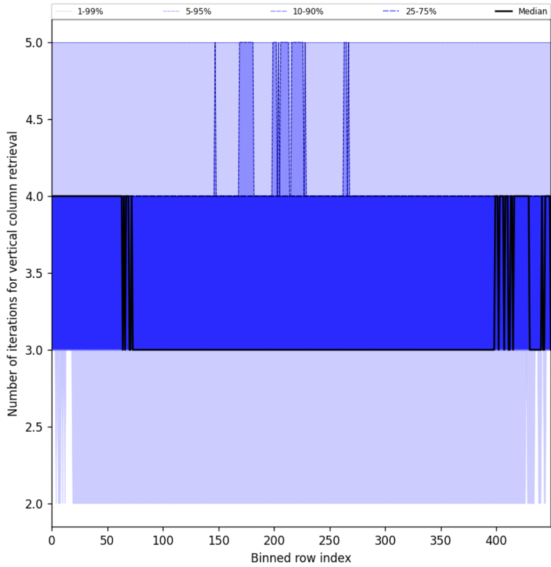
Figure 33: Along track statistics of “Number of iterations for vertical column retrieval” for 2025-07-03 to 2025-07-04
