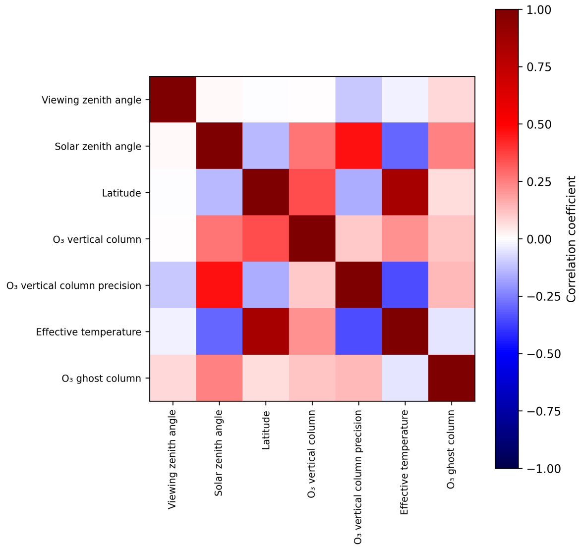
Figure 2: Map of correlation matrix for 2025-07-03 to 2025-07-04.
