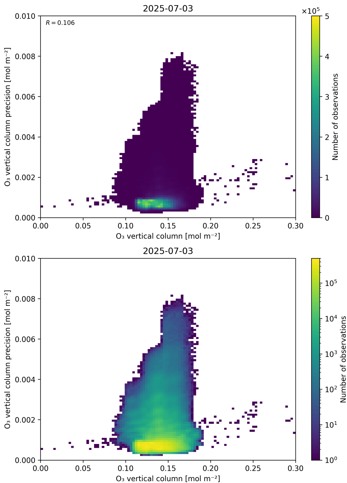
Figure 41: Scatter density plot of “O 3 vertical column” against “O 3 vertical column precision” for 2025-07-03 to 2025-07-04.
