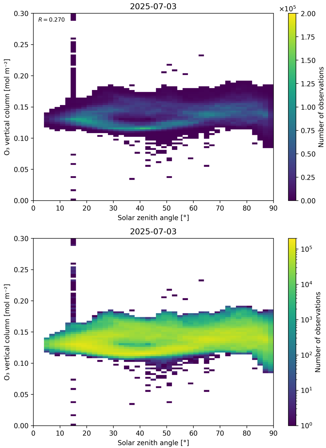
Figure 47: Scatter density plot of “Solar zenith angle” against “O 3 vertical column” for 2025-07-03 to 2025-07-04.
