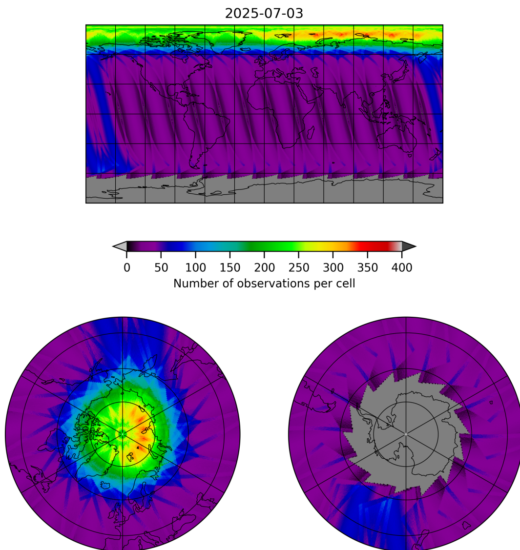
Figure 12: Map of the number of observations for 2025-07-03 to 2025-07-04
