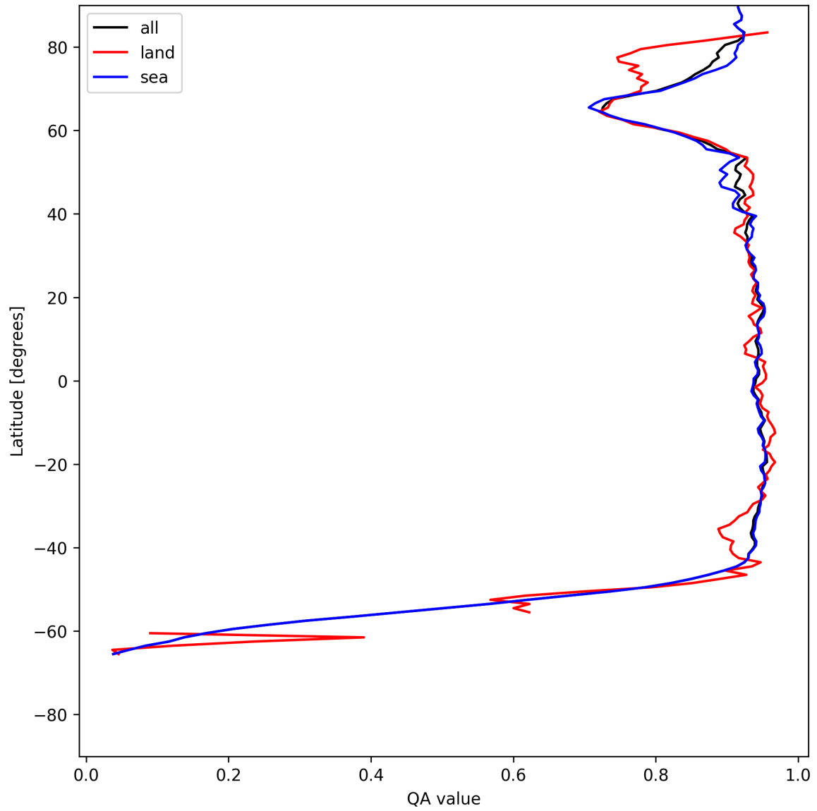
Figure 13: Zonal average of “QA value” for 2025-07-03 to 2025-07-04.
