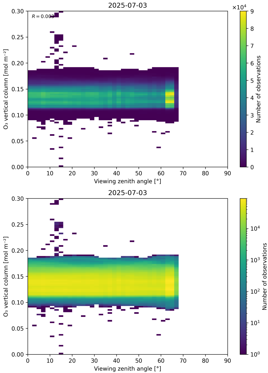
Figure 52: Scatter density plot of “Viewing zenith angle” against “O 3 vertical column” for 2025-07-03 to 2025-07-04.
