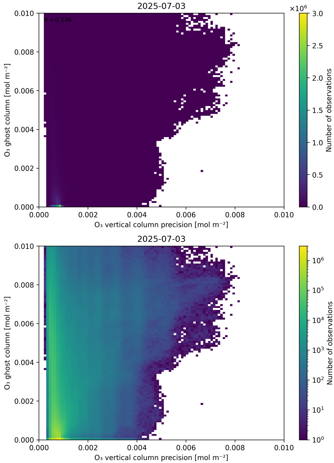
Figure 43: Scatter density plot of “ \text{O}_3 vertical column precision” against “ \text{O}_3 ghost column” for 2025-07-03 to 2025-07-04.
