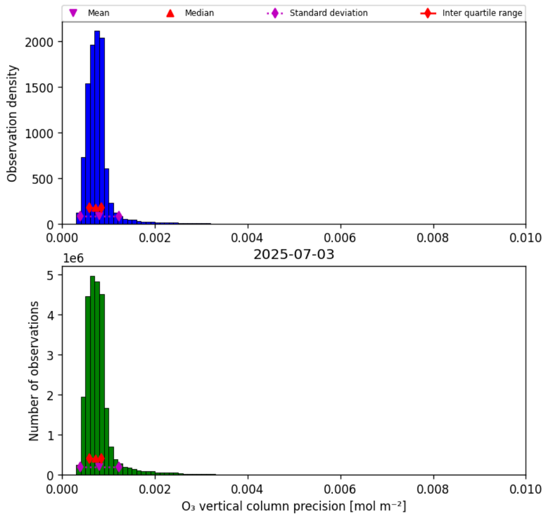
Figure 22: Histogram of “O 3 vertical column precision” for 2025-07-03 to 2025-07-04
