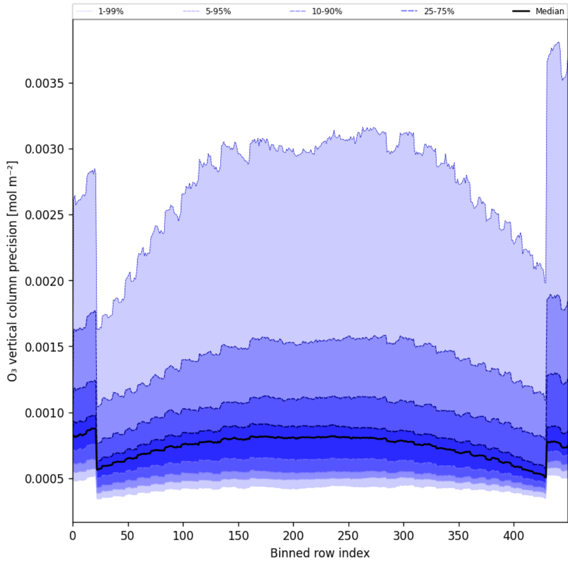
Figure 29: Along track statistics of “O 3 vertical column precision” for 2025-07-03 to 2025-07-04
