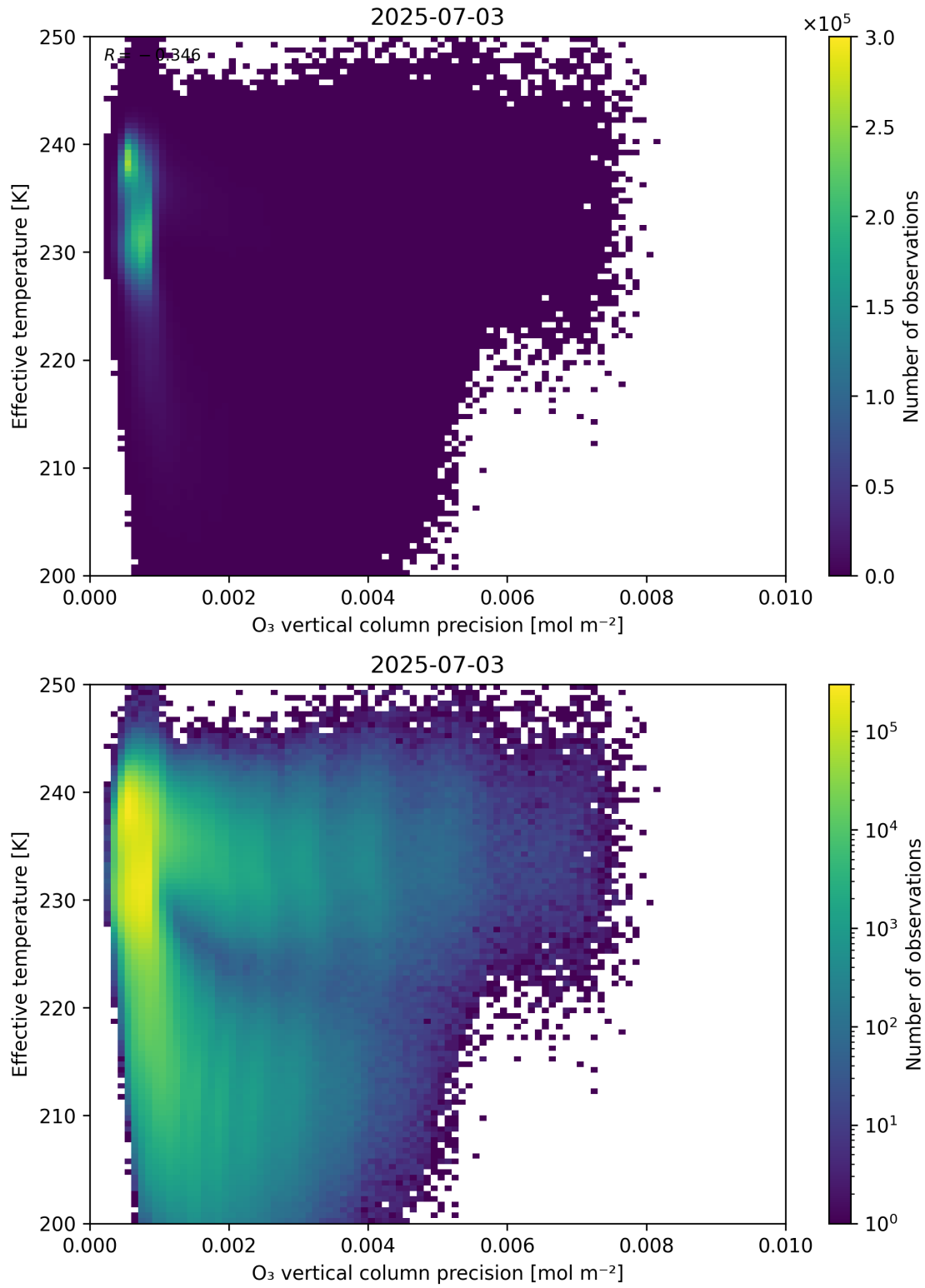
Figure 42: Scatter density plot of “ O_3 vertical column precision” against “Effective temperature” for 2025-07-03 to 2025-07-04.
