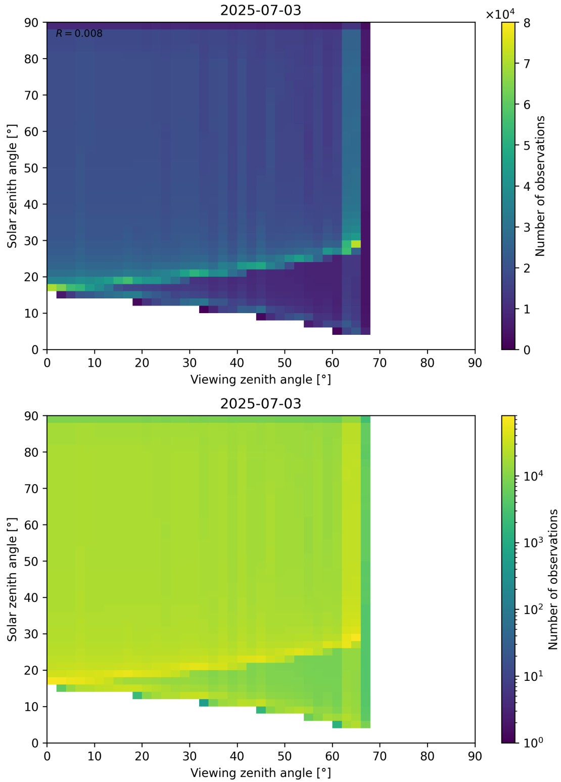
Figure 54: Scatter density plot of “Viewing zenith angle” against “Solar zenith angle” for 2025-07-03 to 2025-07-04.
