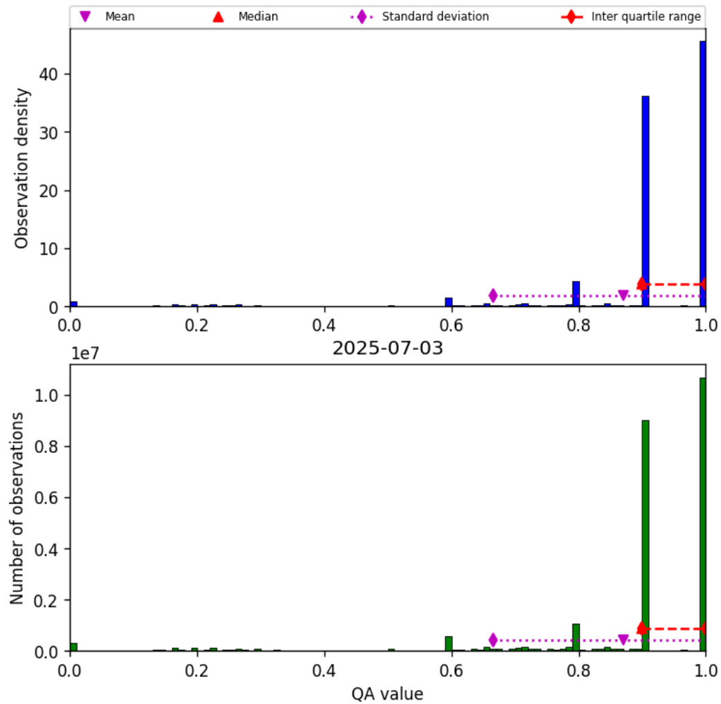
Figure 20: Histogram of “QA value” for 2025-07-03 to 2025-07-04
