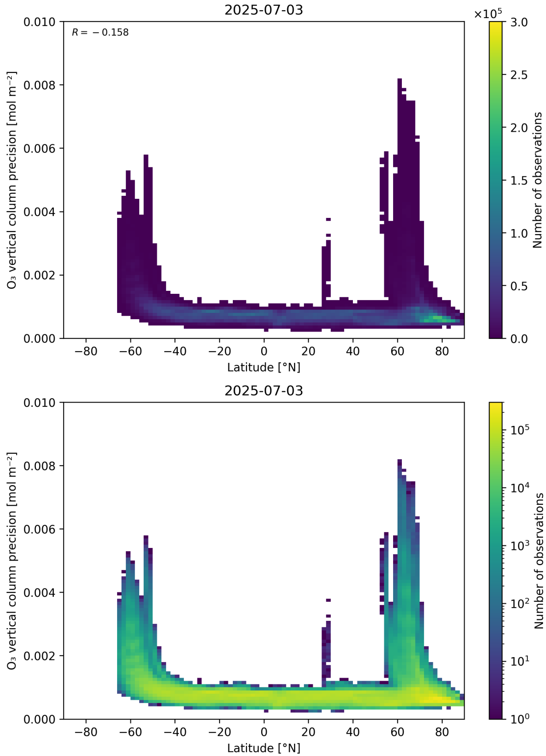
Figure 37: Scatter density plot of “Latitude” against “O 3 vertical column precision” for 2025-07-03 to 2025-07-04.
