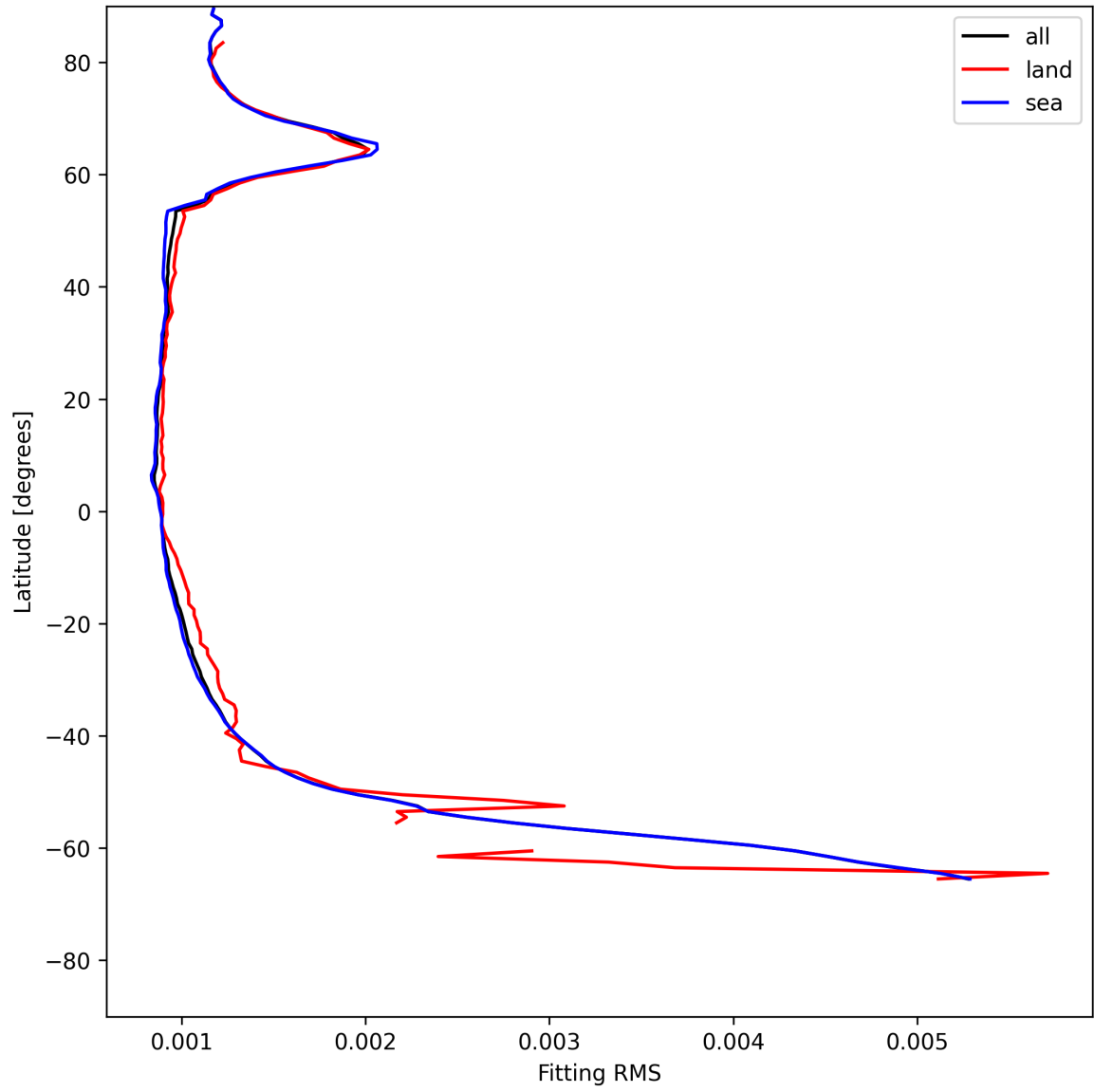
Figure 16: Zonal average of “Fitting RMS” for 2025-07-03 to 2025-07-04.
