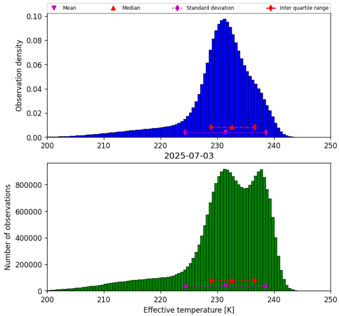
Figure 24: Histogram of “Effective temperature” for 2025-07-03 to 2025-07-04
