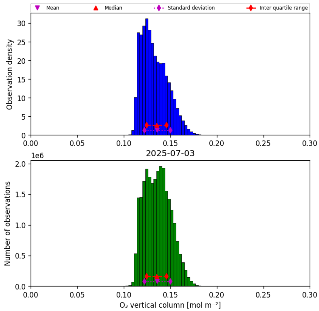
Figure 21: Histogram of “O 3 vertical column” for 2025-07-03 to 2025-07-04
