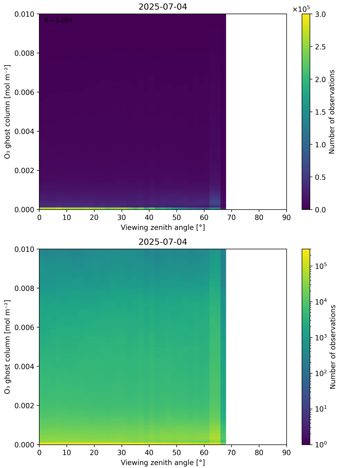
Figure 51: Scatter density plot of “Viewing zenith angle” against “O 3 ghost column” for 2025-07-03 to 2025-07-05.
