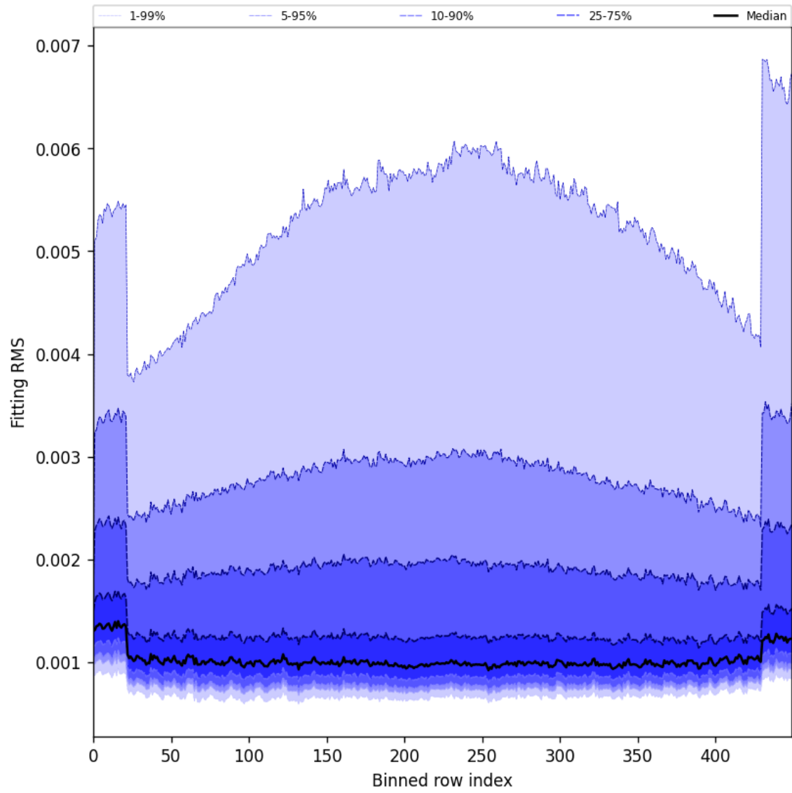
Figure 30: Along track statistics of “Fitting RMS” for 2025-07-03 to 2025-07-05
