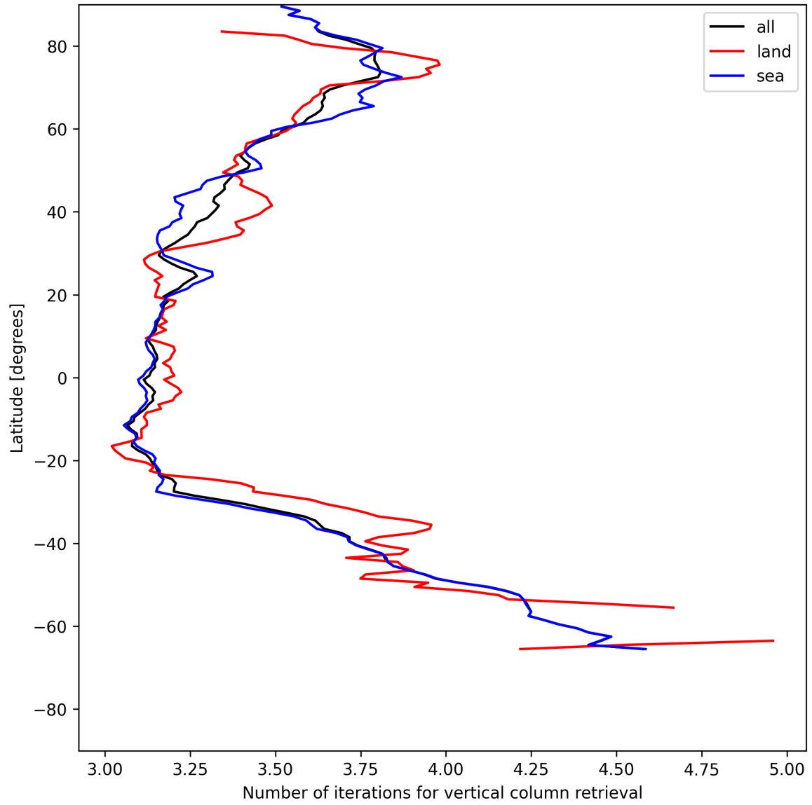
Figure 19: Zonal average of “Number of iterations for vertical column retrieval” for 2025-07-03 to 2025-07-05.
