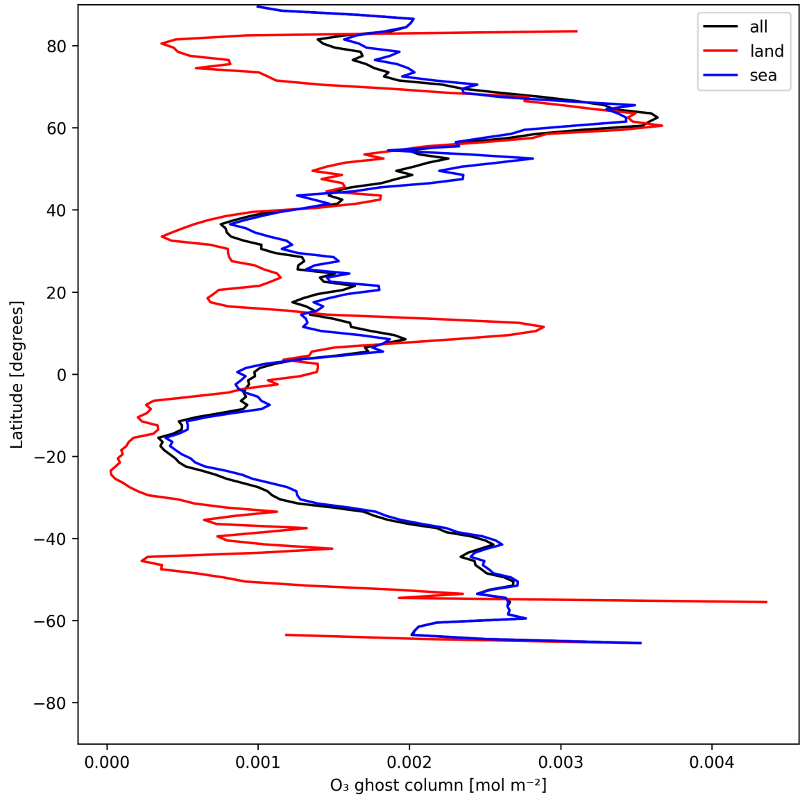
Figure 18: Zonal average of "O 3 ghost column" for 2025-07-03 to 2025-07-05.
