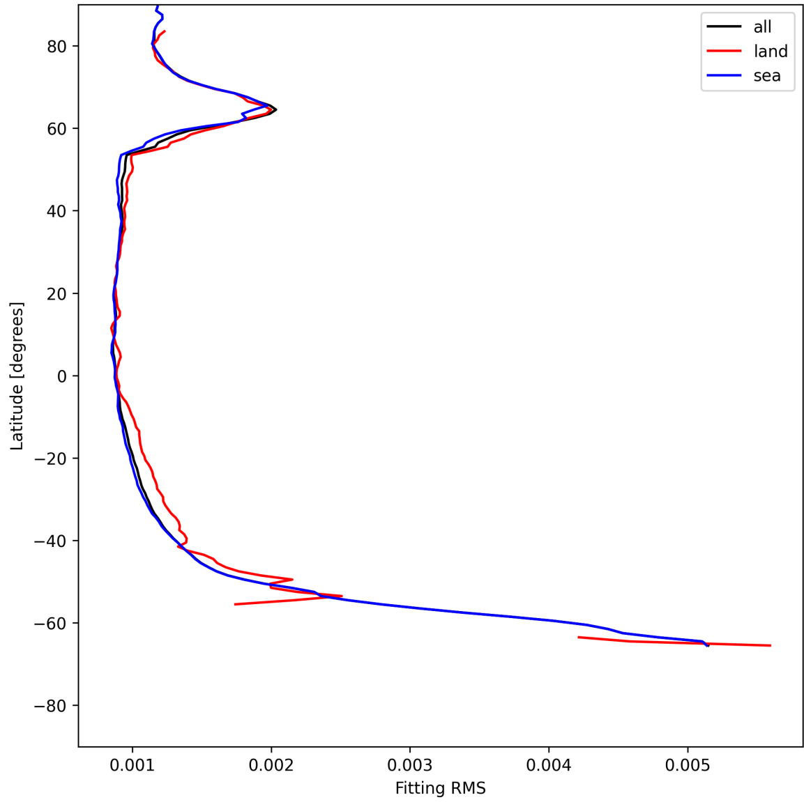
Figure 16: Zonal average of “Fitting RMS” for 2025-07-03 to 2025-07-05.
