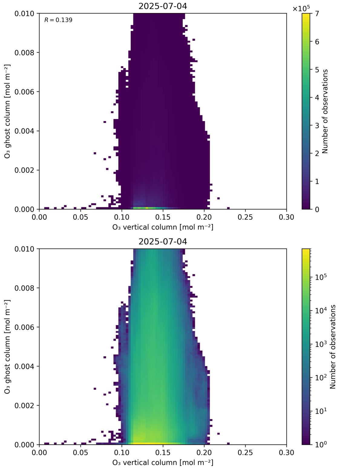
Figure 40: Scatter density plot of “O 3 vertical column” against “O 3 ghost column” for 2025-07-03 to 2025-07-05.
