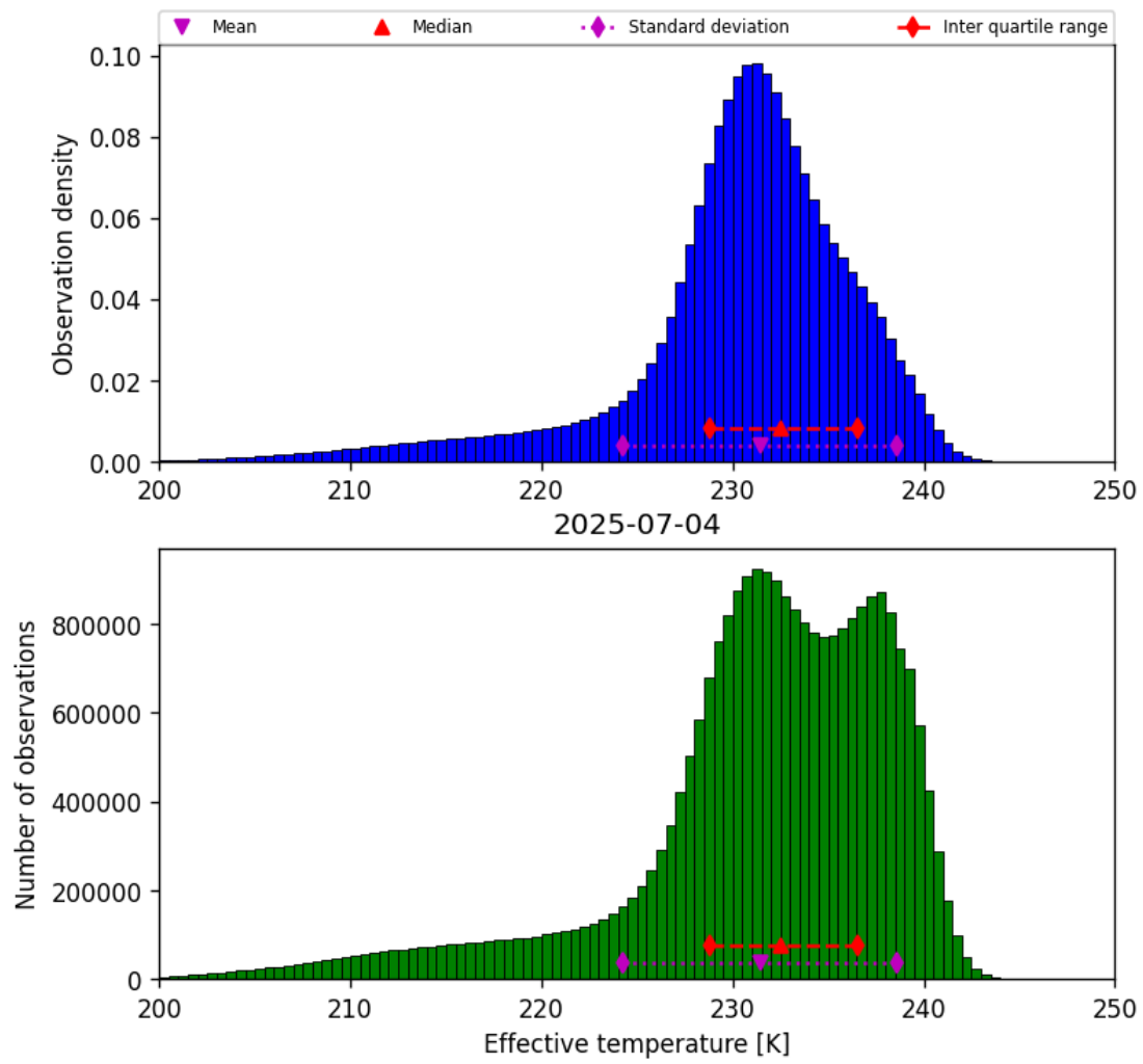
Figure 24: Histogram of “Effective temperature” for 2025-07-03 to 2025-07-05
