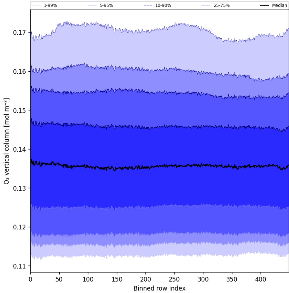
Figure 28: Along track statistics of “O 3 vertical column” for 2025-07-03 to 2025-07-05
