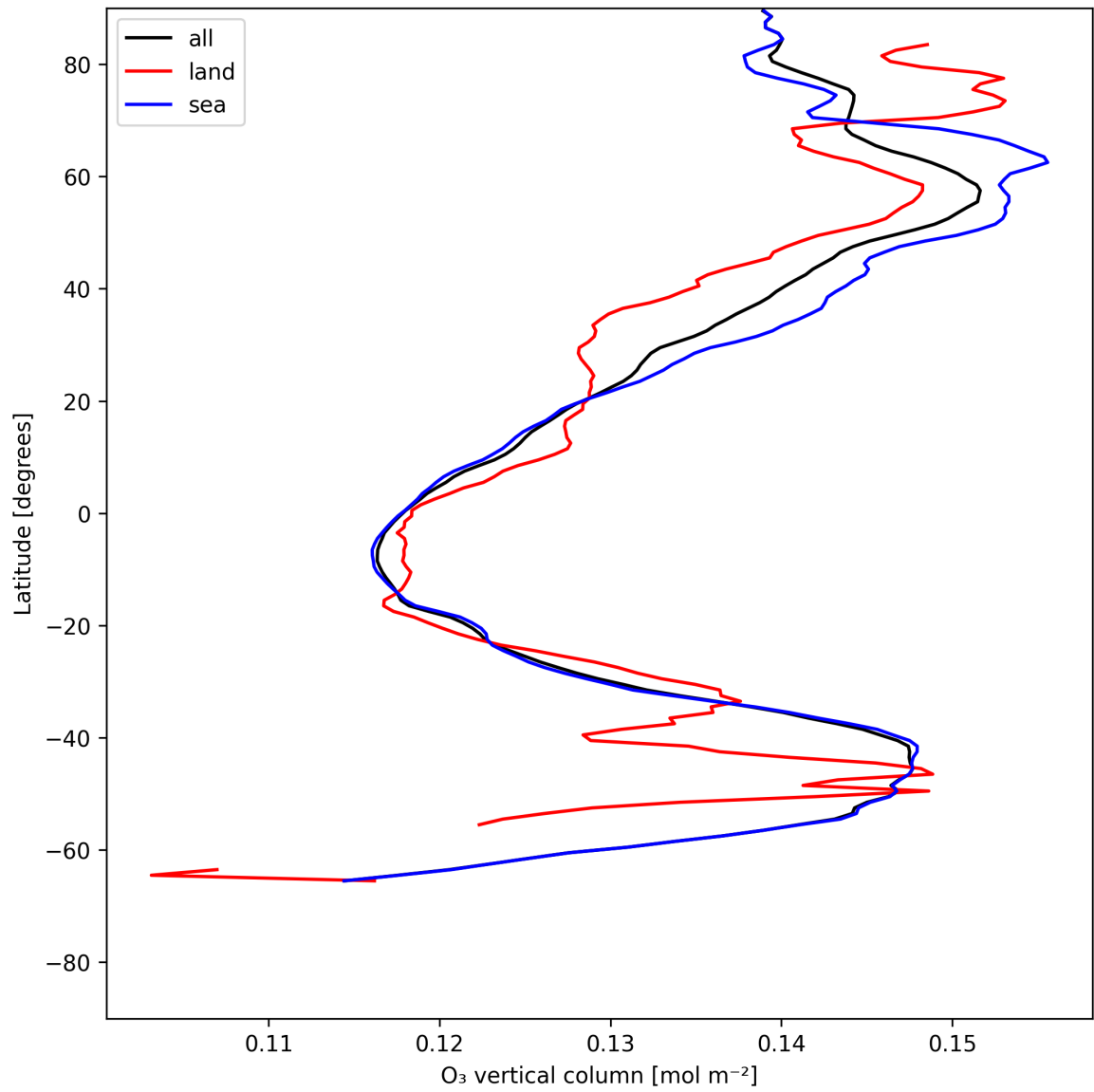
Figure 14: Zonal average of “O 3 vertical column” for 2025-07-03 to 2025-07-05.
