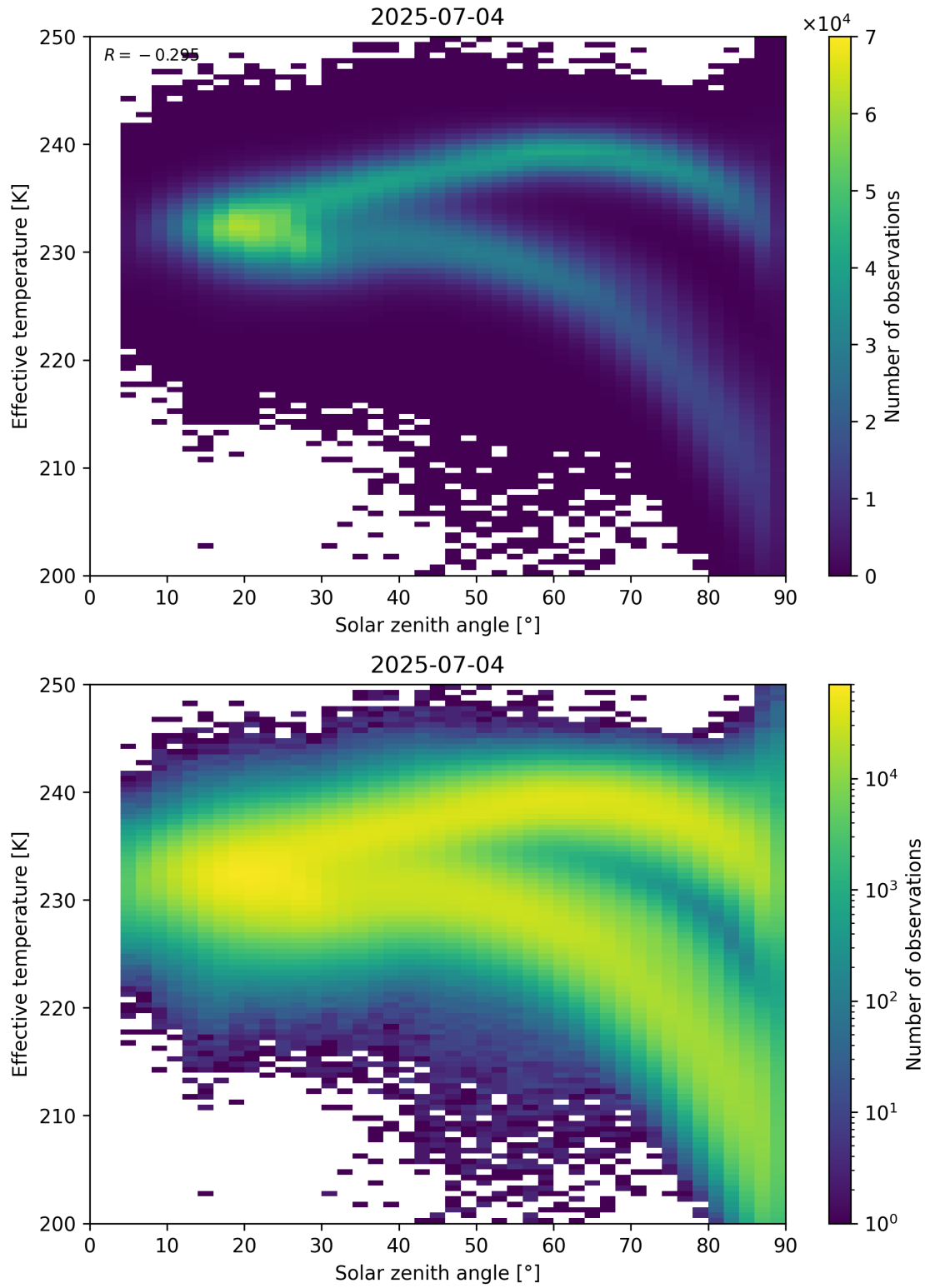
Figure 45: Scatter density plot of “Solar zenith angle” against “Effective temperature” for 2025-07-03 to 2025-07-05.
