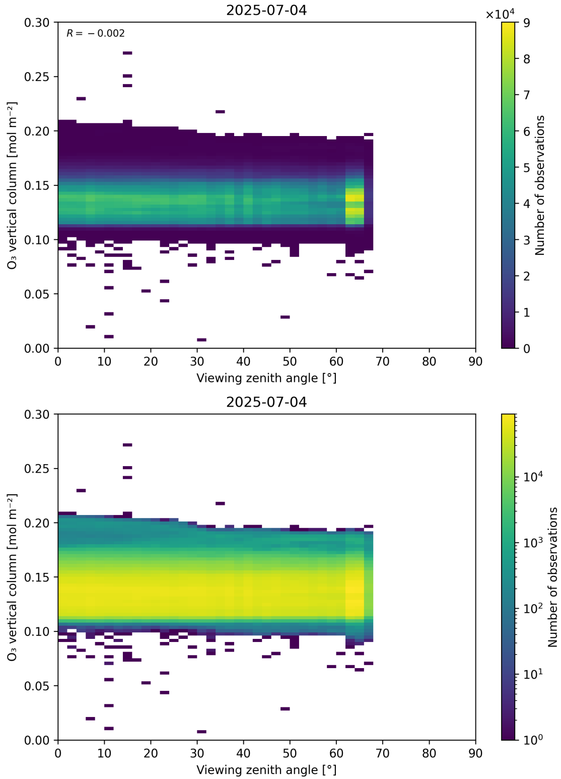
Figure 52: Scatter density plot of “Viewing zenith angle” against “O 3 vertical column” for 2025-07-03 to 2025-07-05.
