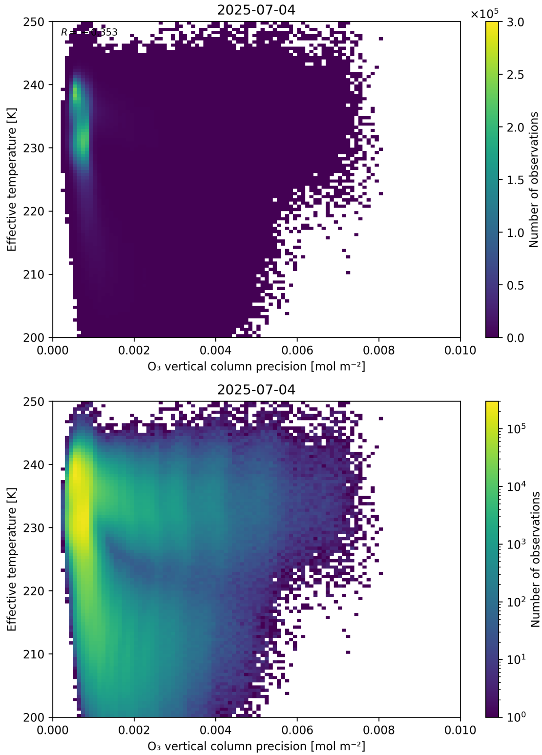
Figure 42: Scatter density plot of “O 3 vertical column precision” against “Effective temperature” for 2025-07-03 to 2025-07-05.
