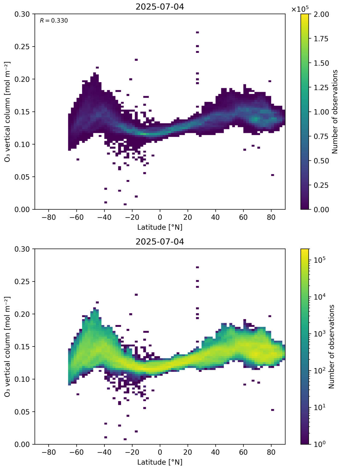
Figure 36: Scatter density plot of “Latitude” against “O 3 vertical column” for 2025-07-03 to 2025-07-05.
