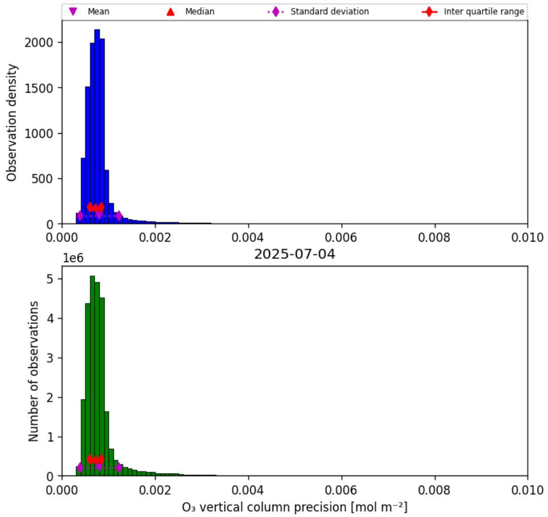
Figure 22: Histogram of “O 3 vertical column precision” for 2025-07-03 to 2025-07-05
