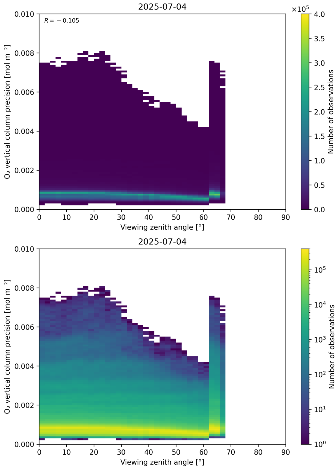
Figure 53: Scatter density plot of “Viewing zenith angle” against “O 3 vertical column precision” for 2025-07-03 to 2025-07-05.
