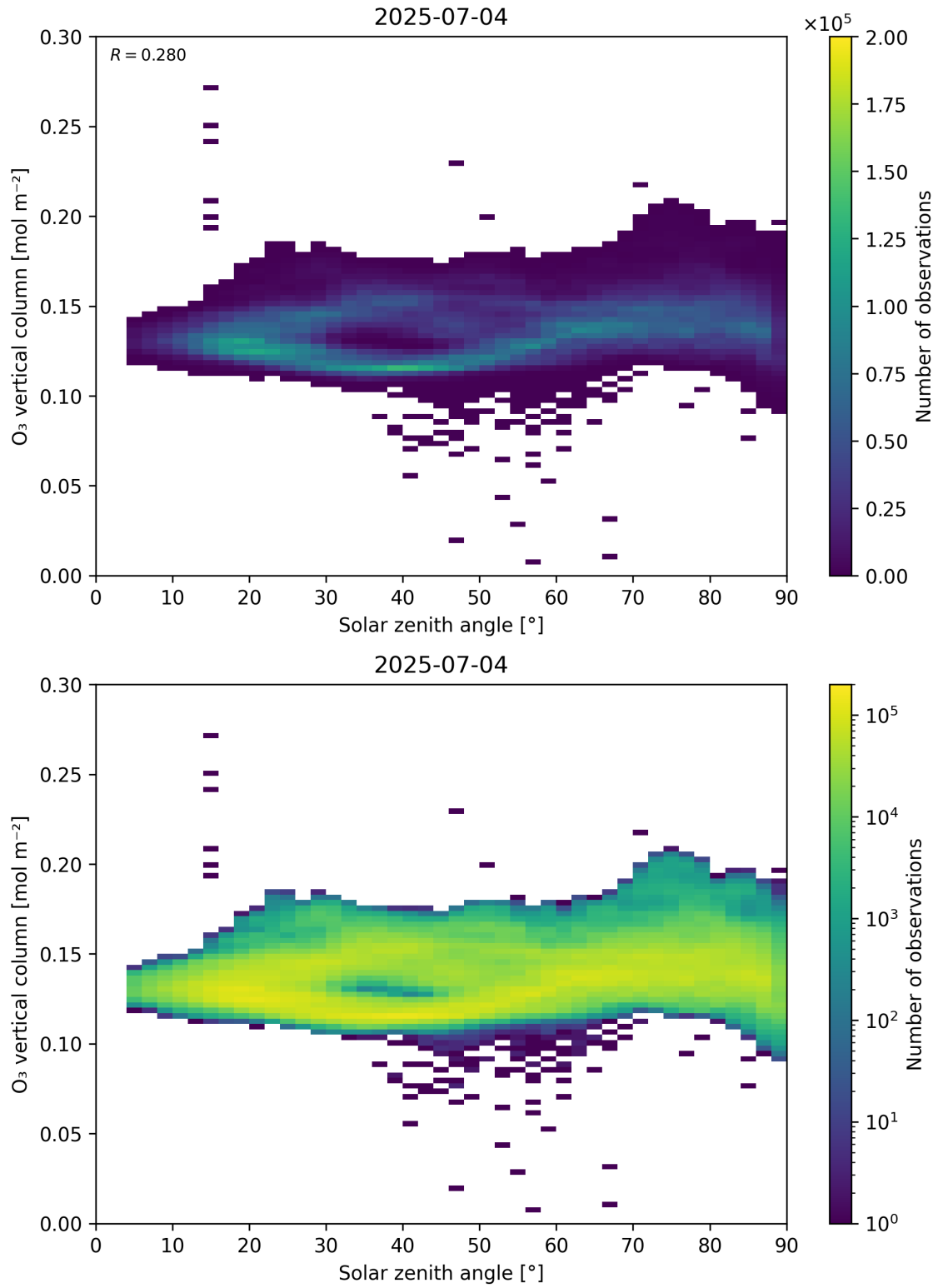
Figure 47: Scatter density plot of “Solar zenith angle” against “O 3 vertical column” for 2025-07-03 to 2025-07-05.
