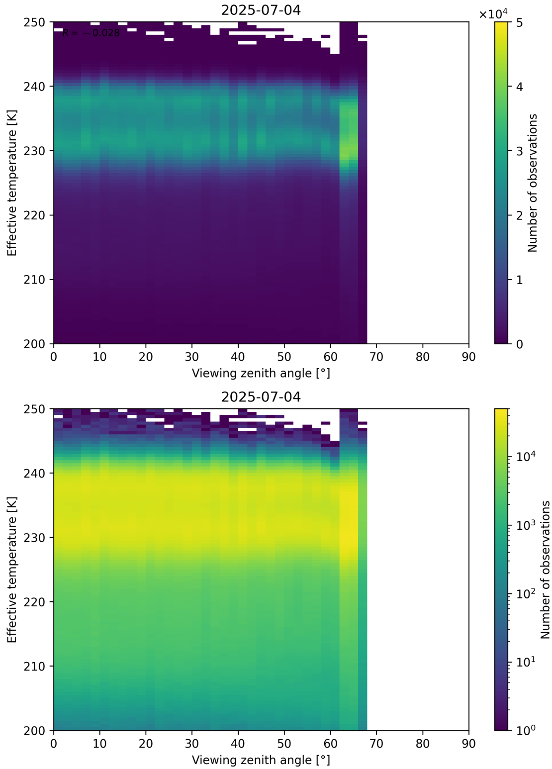
Figure 50: Scatter density plot of “Viewing zenith angle” against “Effective temperature” for 2025-07-03 to 2025-07-05.
