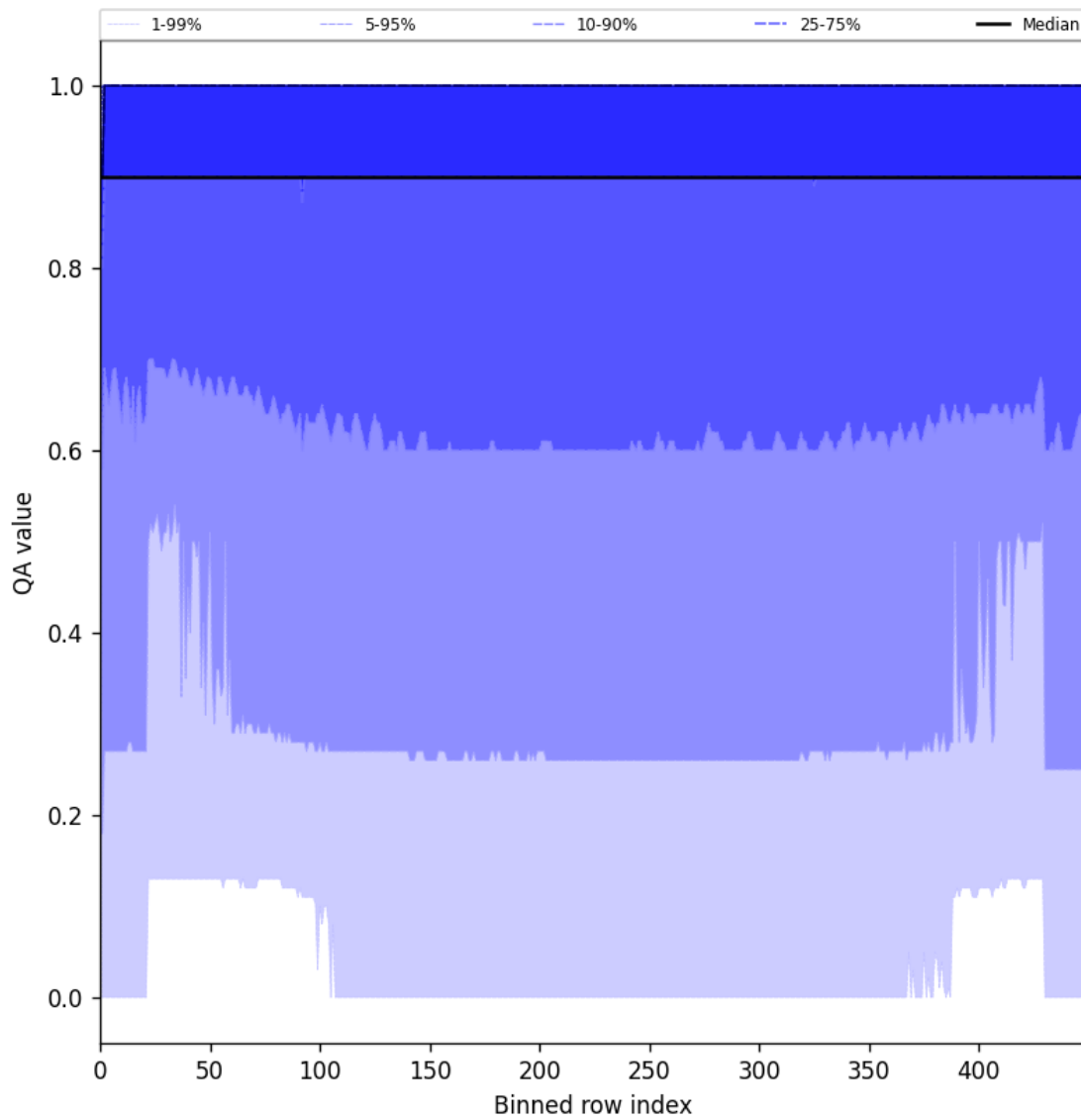
Figure 27: Along track statistics of “QA value” for 2025-07-03 to 2025-07-05
