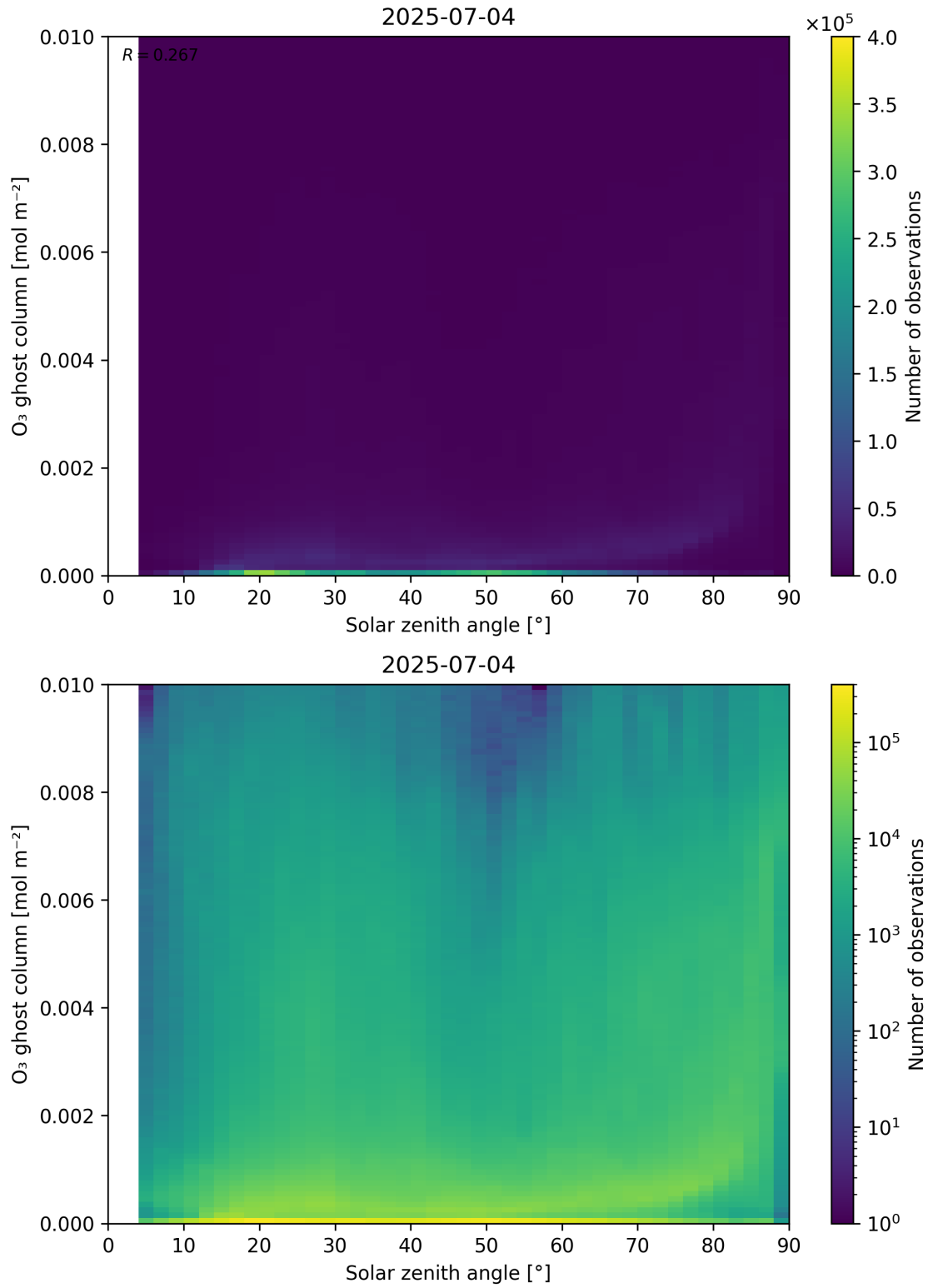
Figure 46: Scatter density plot of “Solar zenith angle” against “O 3 ghost column” for 2025-07-03 to 2025-07-05.
