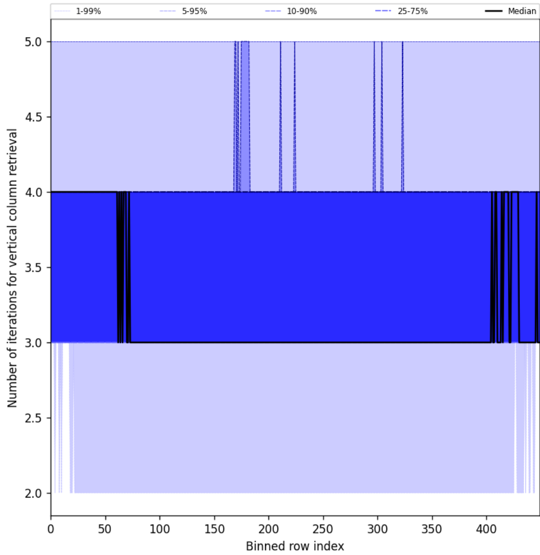
Figure 33: Along track statistics of “Number of iterations for vertical column retrieval” for 2025-07-03 to 2025-07-05
