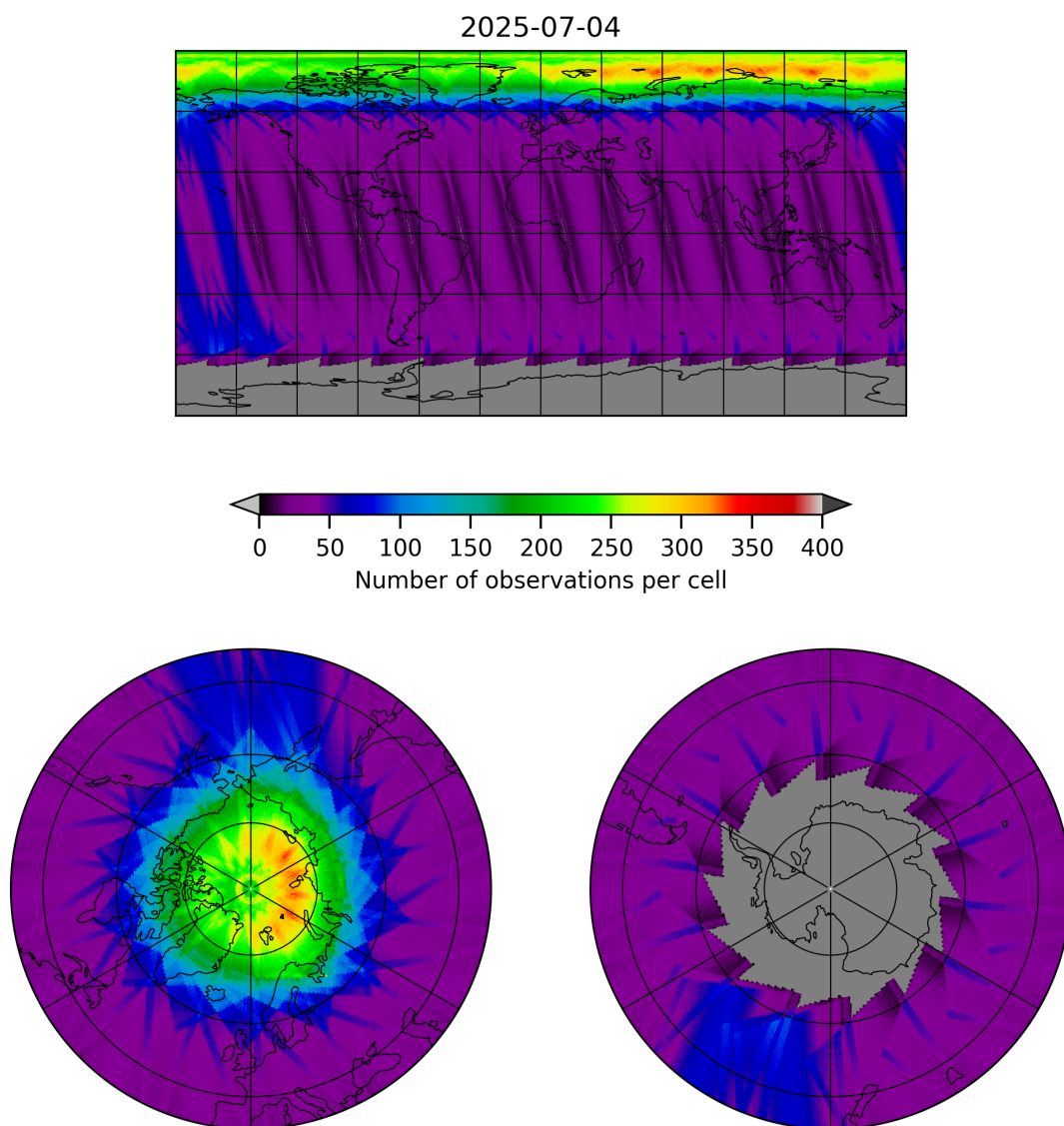
Figure 12: Map of the number of observations for 2025-07-03 to 2025-07-05
