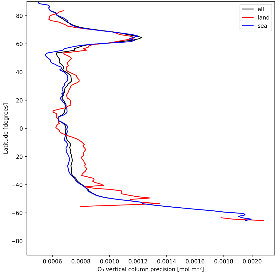
Figure 15: Zonal average of “O 3 vertical column precision” for 2025-07-03 to 2025-07-05.
