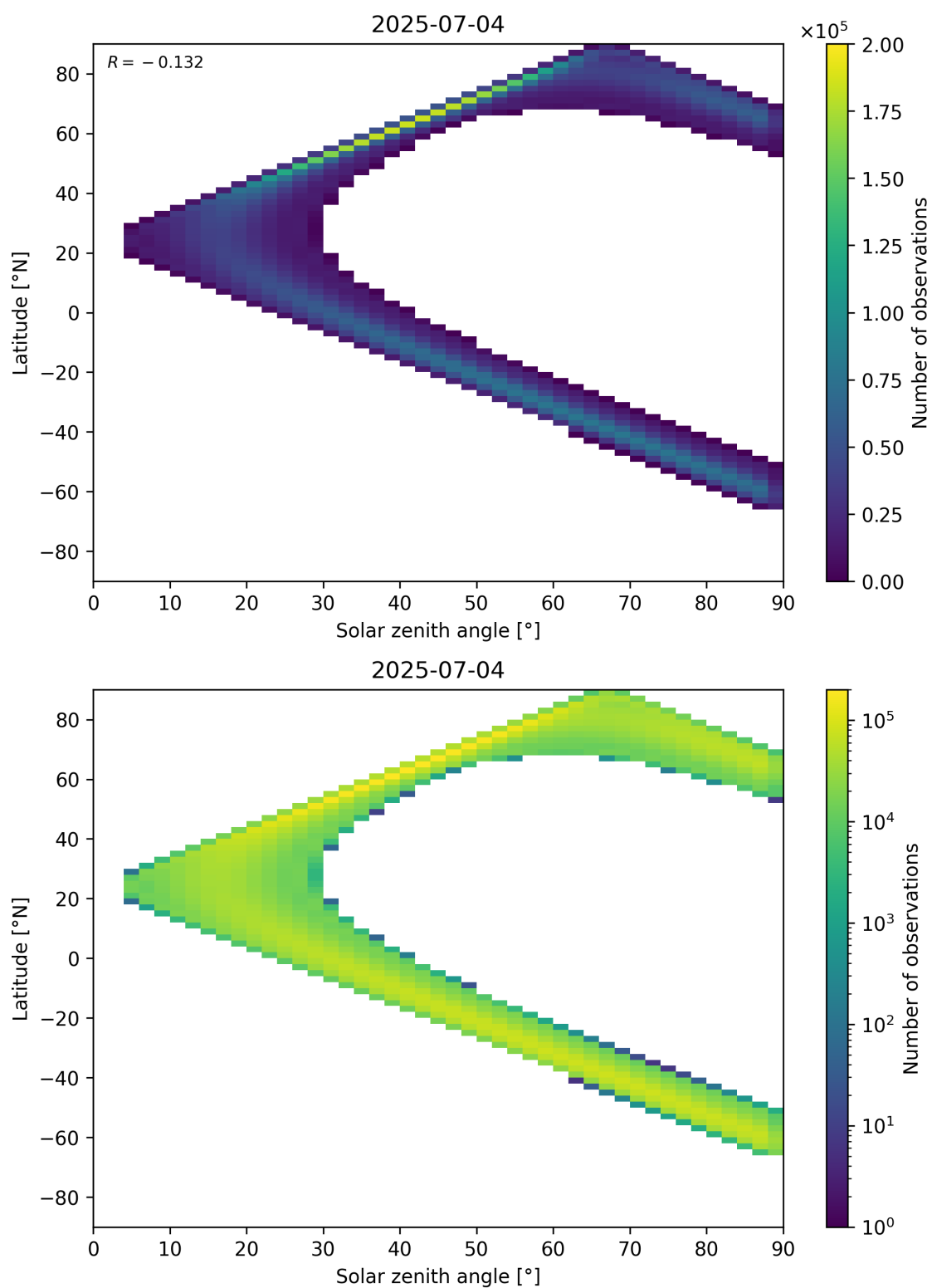
Figure 44: Scatter density plot of “Solar zenith angle” against “Latitude” for 2025-07-03 to 2025-07-05.
