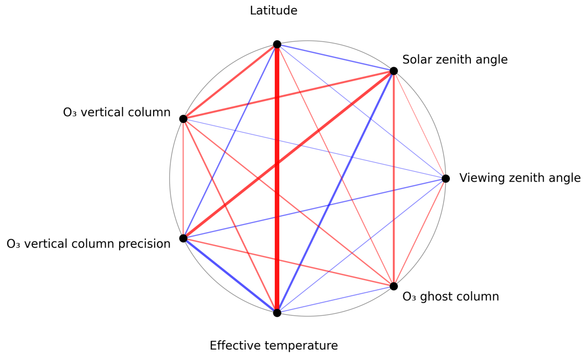
Figure 1: Map of correlation graph for 2025-07-03 to 2025-07-05.
