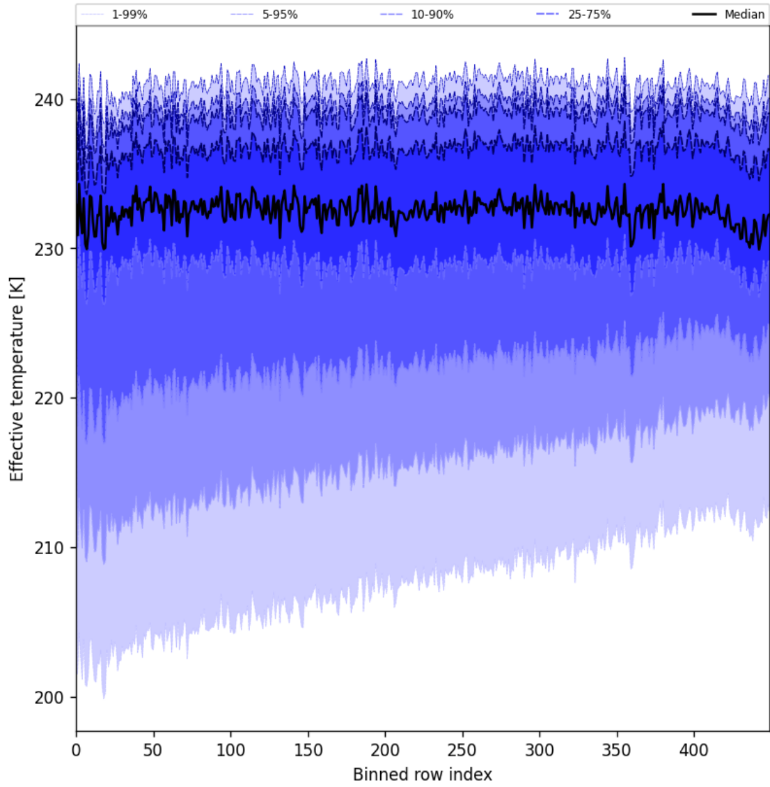
Figure 31: Along track statistics of “Effective temperature” for 2025-07-03 to 2025-07-05
