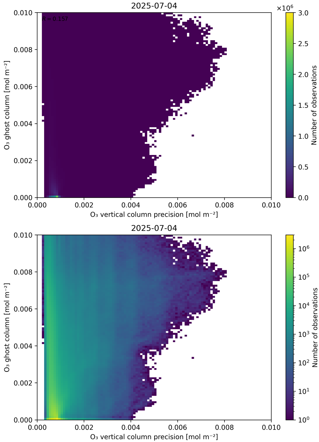
Figure 43: Scatter density plot of “ \text{O}_3 vertical column precision” against “ \text{O}_3 ghost column” for 2025-07-03 to 2025-07-05.
