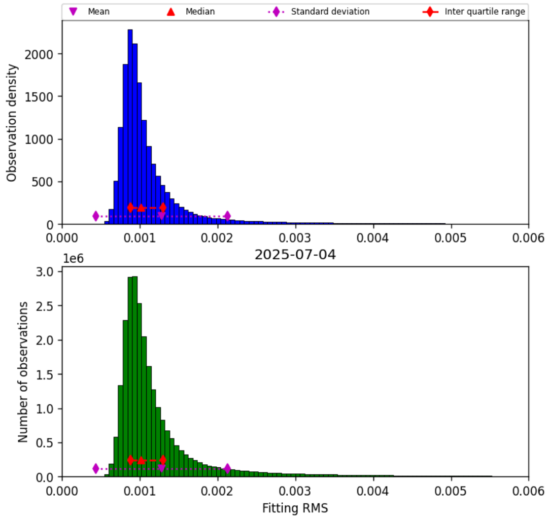
Figure 23: Histogram of “Fitting RMS” for 2025-07-03 to 2025-07-05
