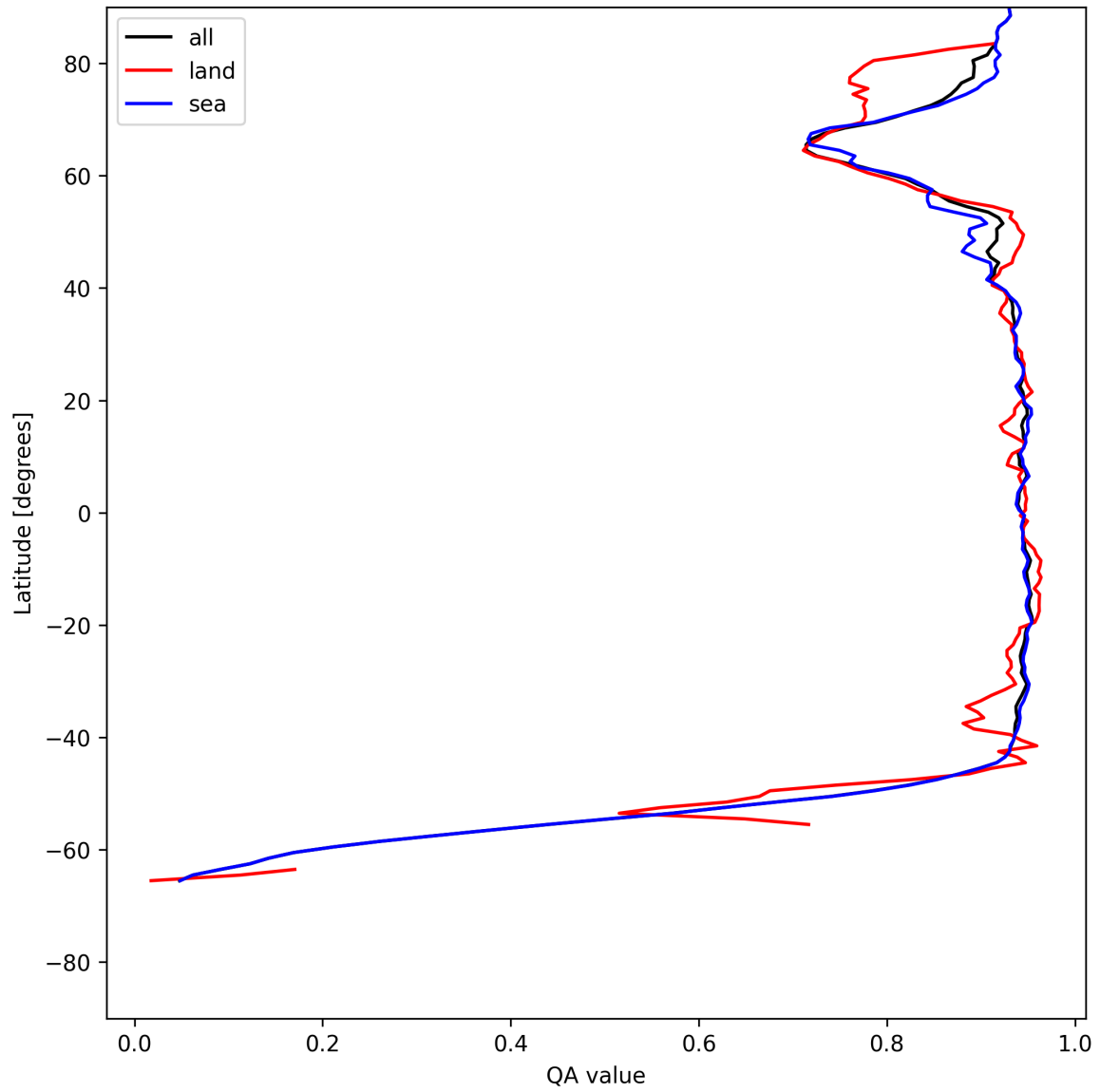
Figure 13: Zonal average of “QA value” for 2025-07-03 to 2025-07-05.
