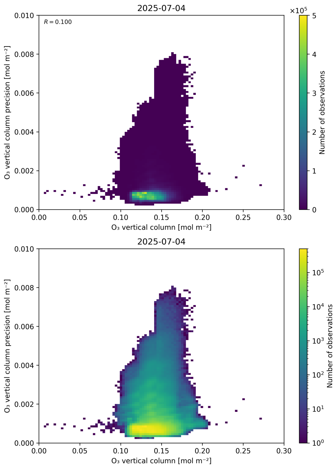
Figure 41: Scatter density plot of “O 3 vertical column” against “O 3 vertical column precision” for 2025-07-03 to 2025-07-05.
