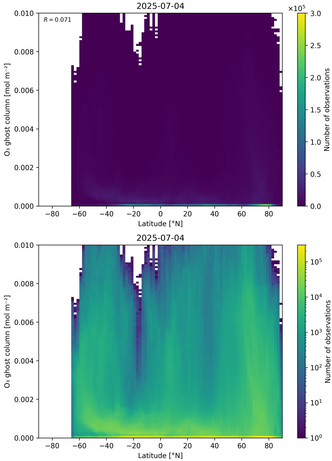
Figure 35: Scatter density plot of “Latitude” against “O 3 ghost column” for 2025-07-03 to 2025-07-05.
