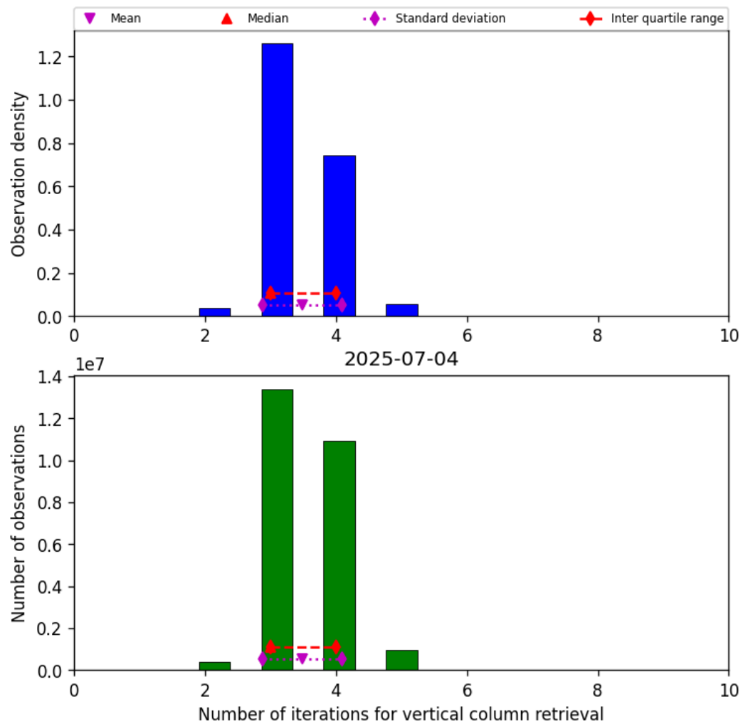
Figure 26: Histogram of “Number of iterations for vertical column retrieval” for 2025-07-03 to 2025-07-05
