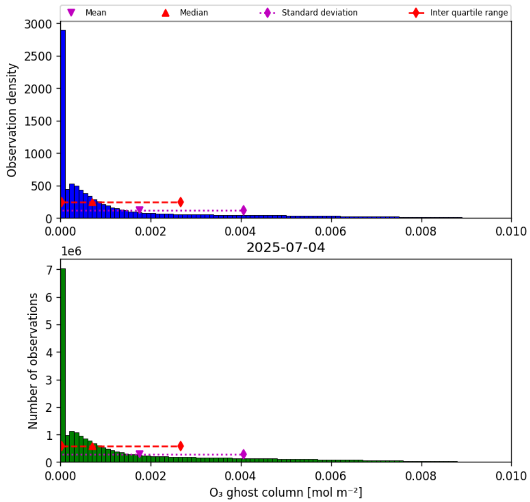
Figure 25: Histogram of “O 3 ghost column” for 2025-07-03 to 2025-07-05
