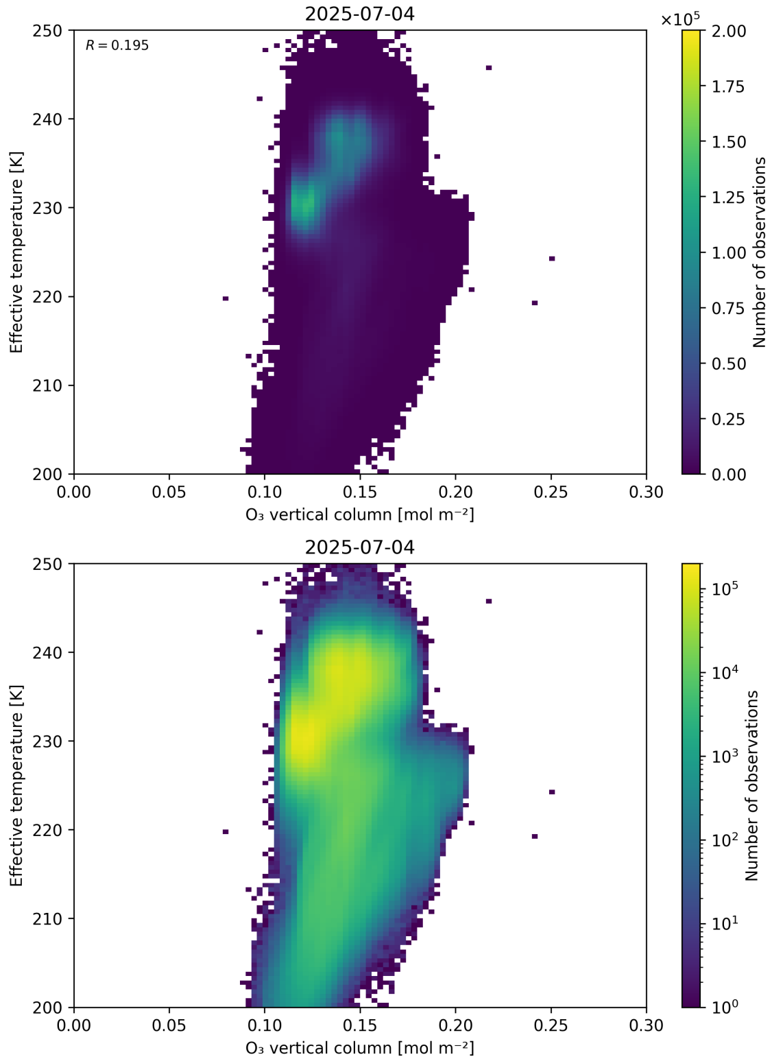
Figure 39: Scatter density plot of “O 3 vertical column” against “Effective temperature” for 2025-07-03 to 2025-07-05.
