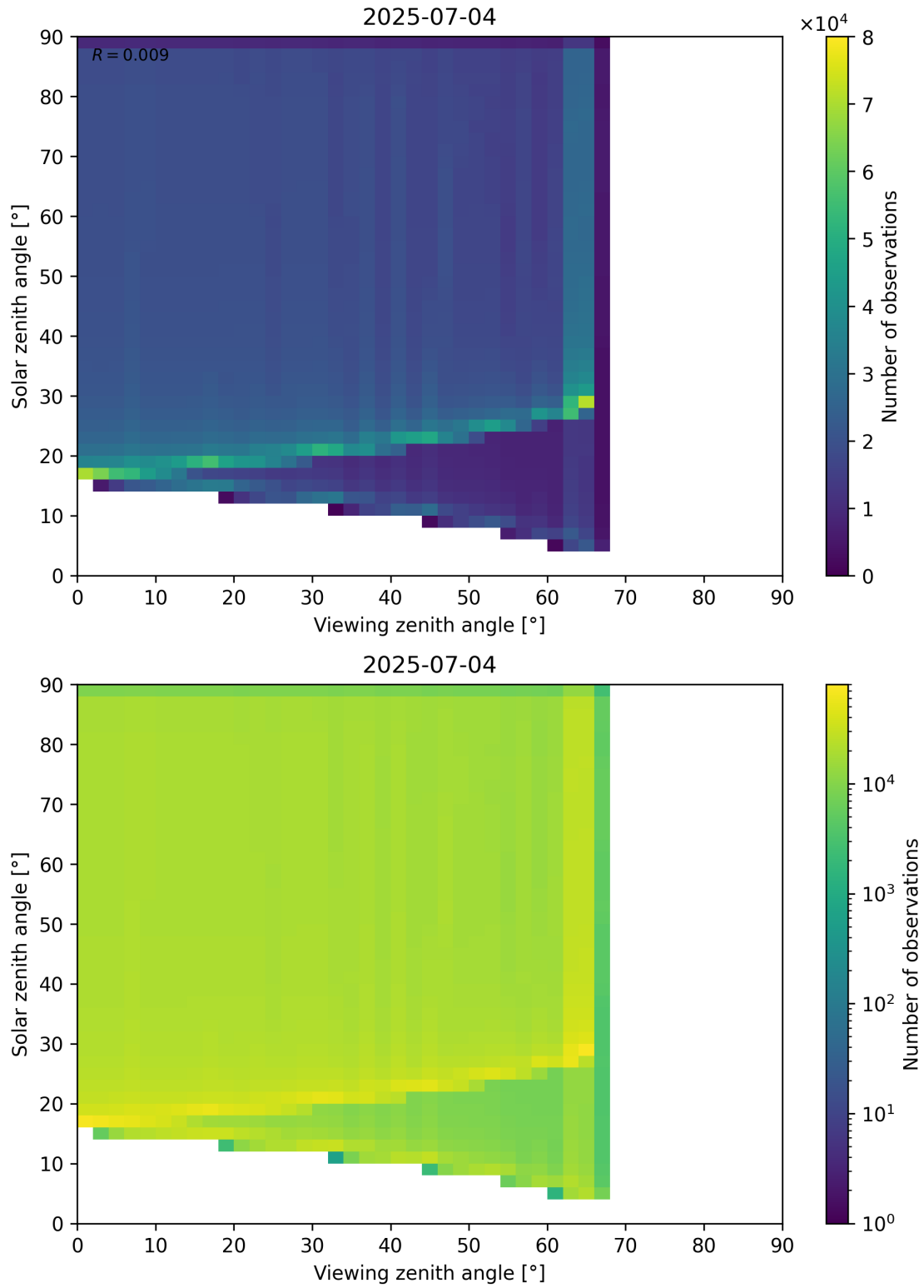
Figure 54: Scatter density plot of “Viewing zenith angle” against “Solar zenith angle” for 2025-07-03 to 2025-07-05.
