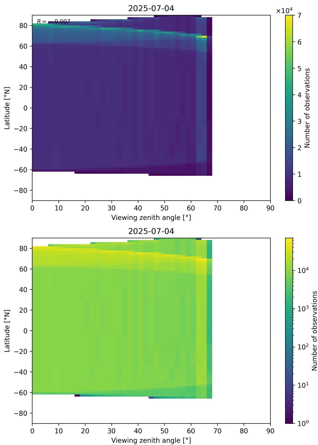
Figure 49: Scatter density plot of “Viewing zenith angle” against “Latitude” for 2025-07-03 to 2025-07-05.
