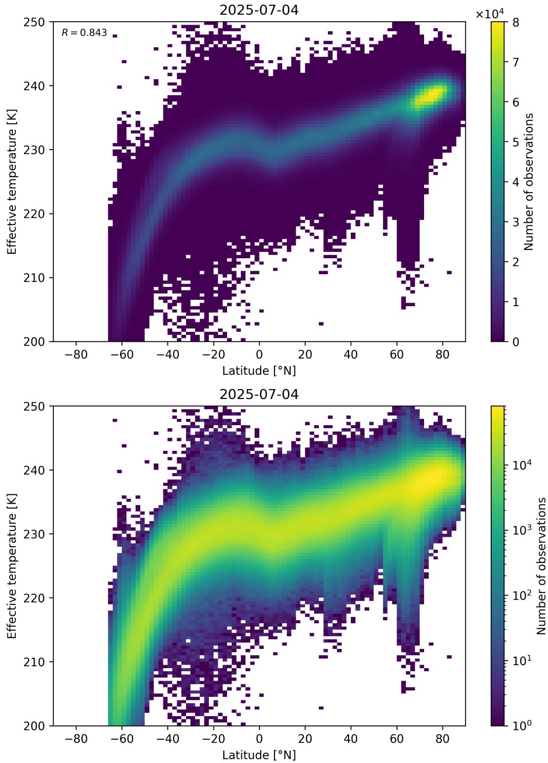
Figure 34: Scatter density plot of “Latitude” against “Effective temperature” for 2025-07-03 to 2025-07-05.
