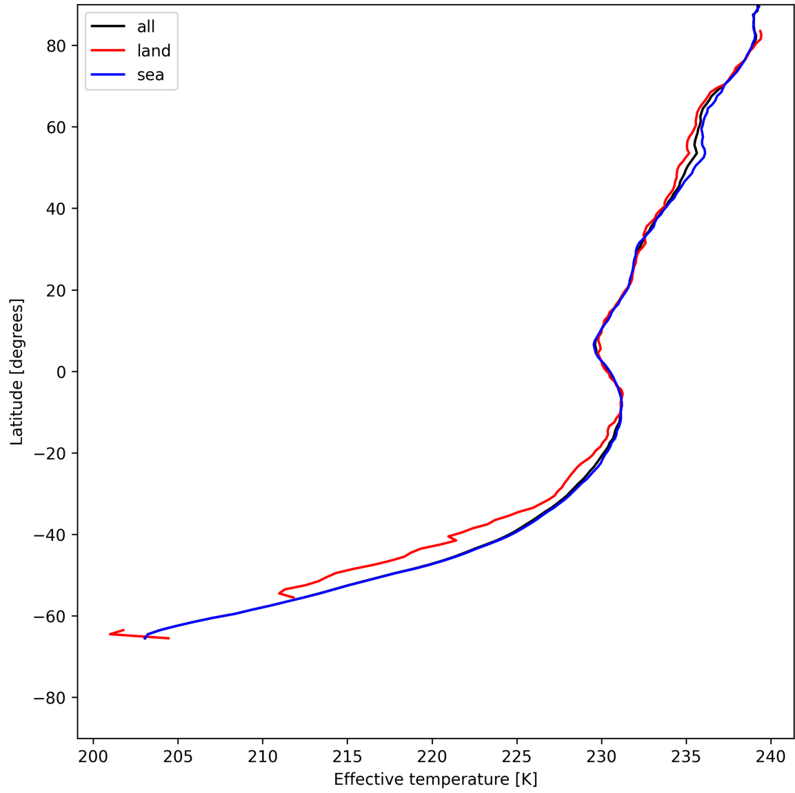
Figure 17: Zonal average of “Effective temperature” for 2025-07-03 to 2025-07-05.
