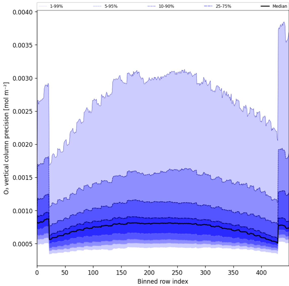
Figure 29: Along track statistics of “O 3 vertical column precision” for 2025-07-03 to 2025-07-05
