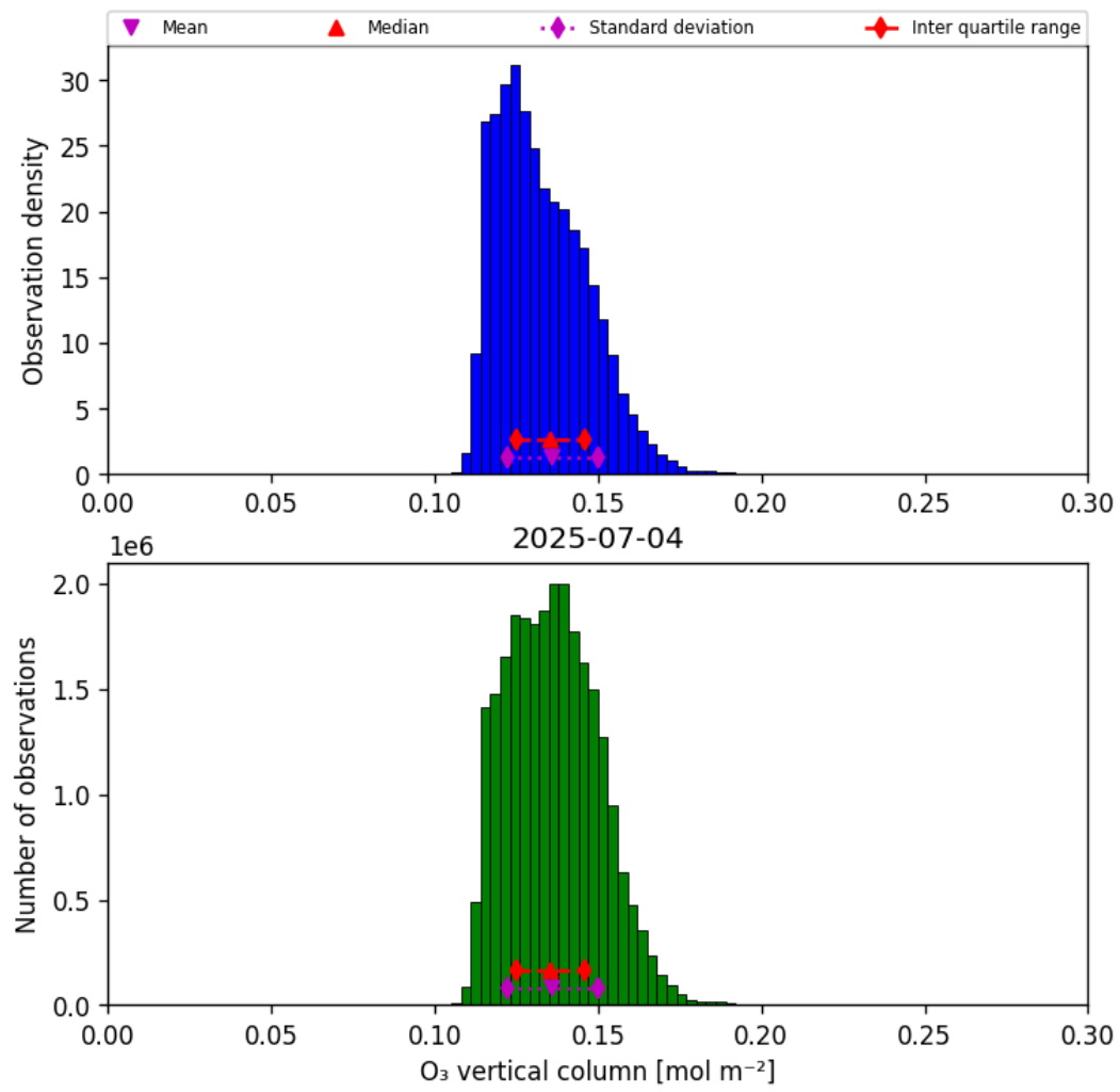
Figure 21: Histogram of “O 3 vertical column” for 2025-07-03 to 2025-07-05
