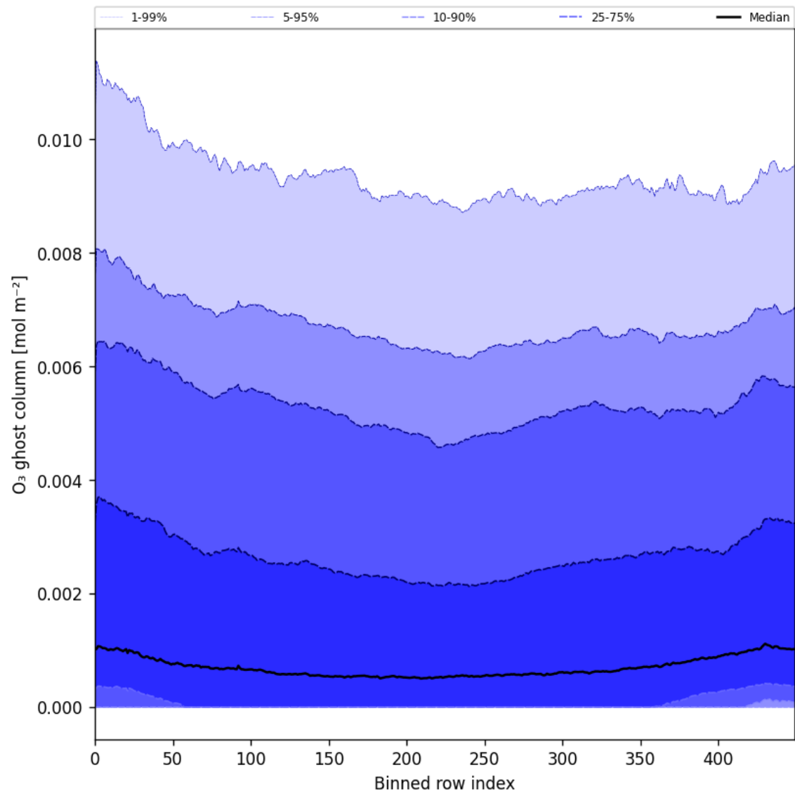
Figure 32: Along track statistics of “O 3 ghost column” for 2025-07-03 to 2025-07-05
