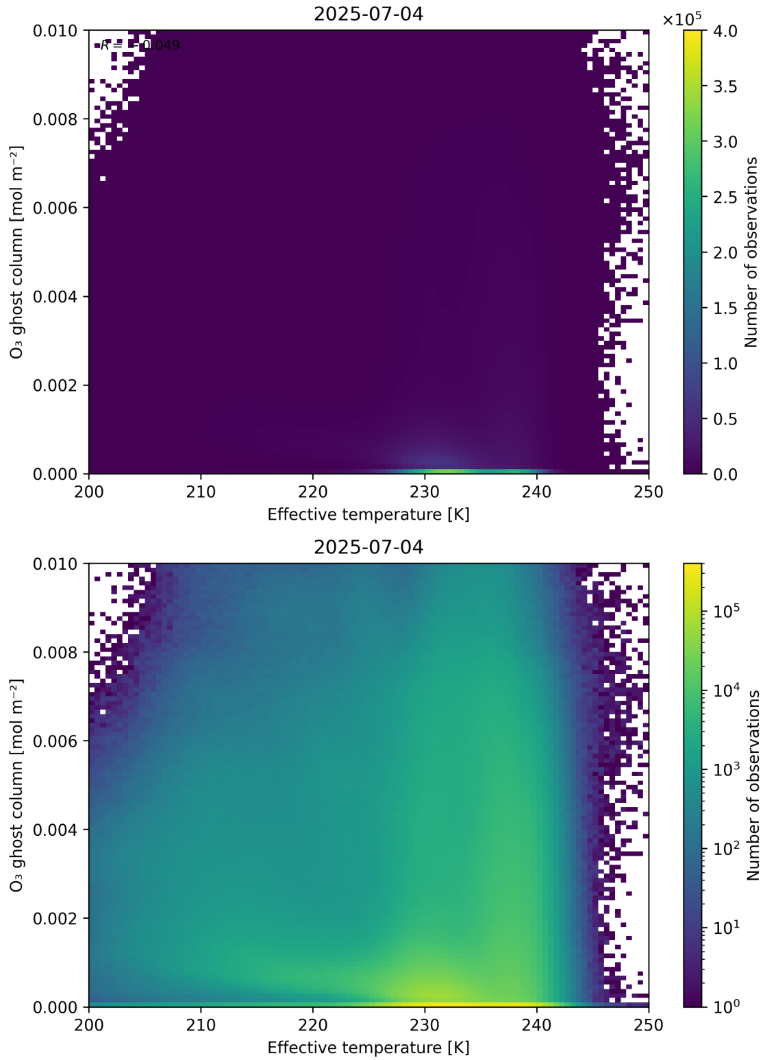
Figure 38: Scatter density plot of “Effective temperature” against “O 3 ghost column” for 2025-07-03 to 2025-07-05.
