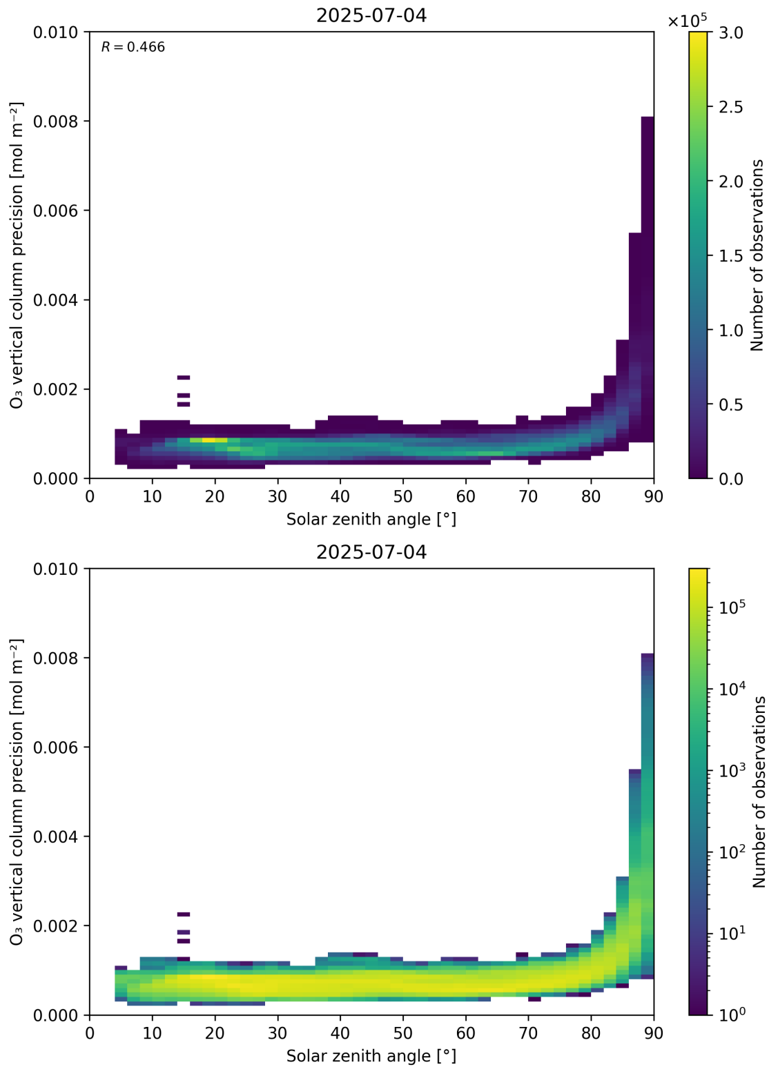
Figure 48: Scatter density plot of “Solar zenith angle” against “O 3 vertical column precision” for 2025-07-03 to 2025-07-05.
