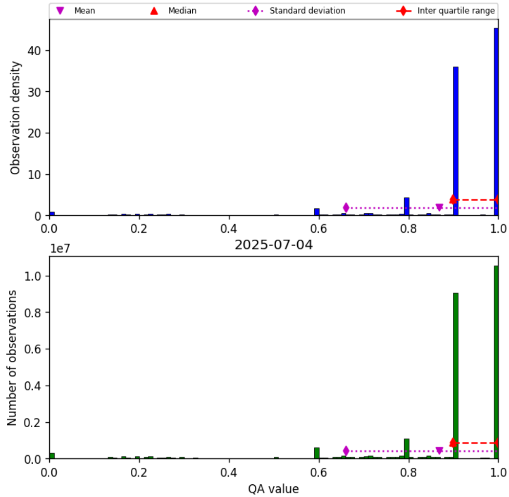
Figure 20: Histogram of “QA value” for 2025-07-03 to 2025-07-05
