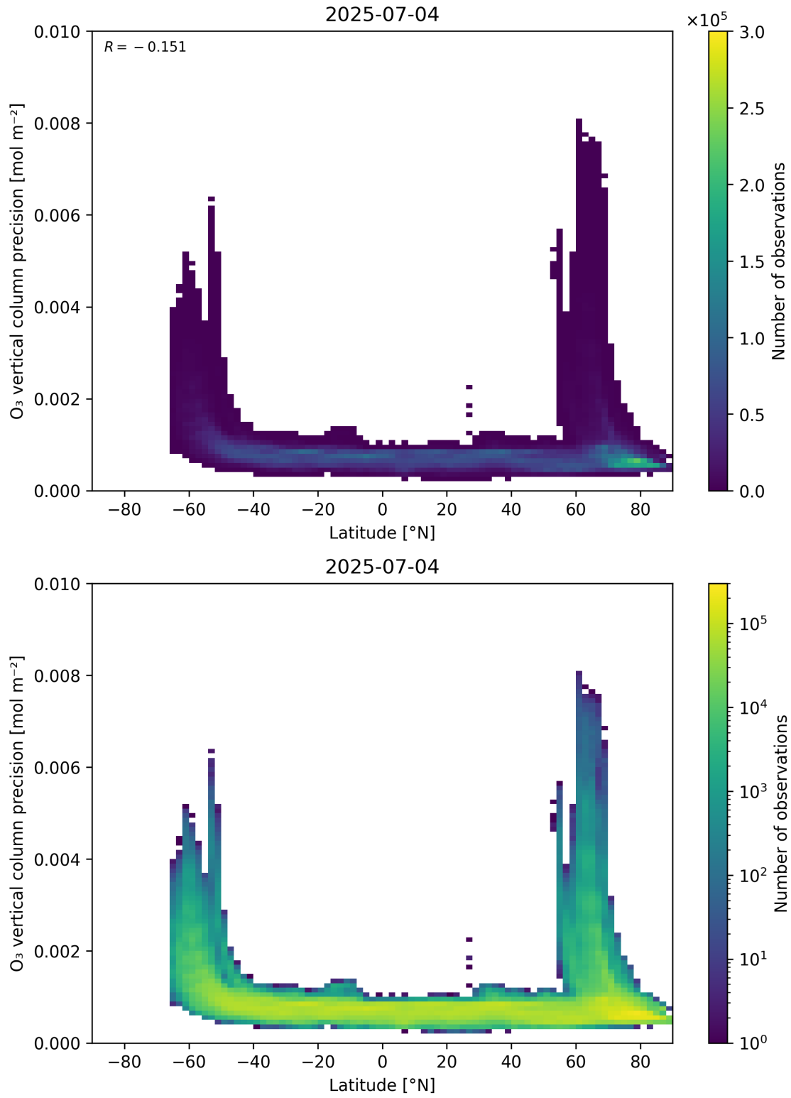
Figure 37: Scatter density plot of “Latitude” against “O 3 vertical column precision” for 2025-07-03 to 2025-07-05.
