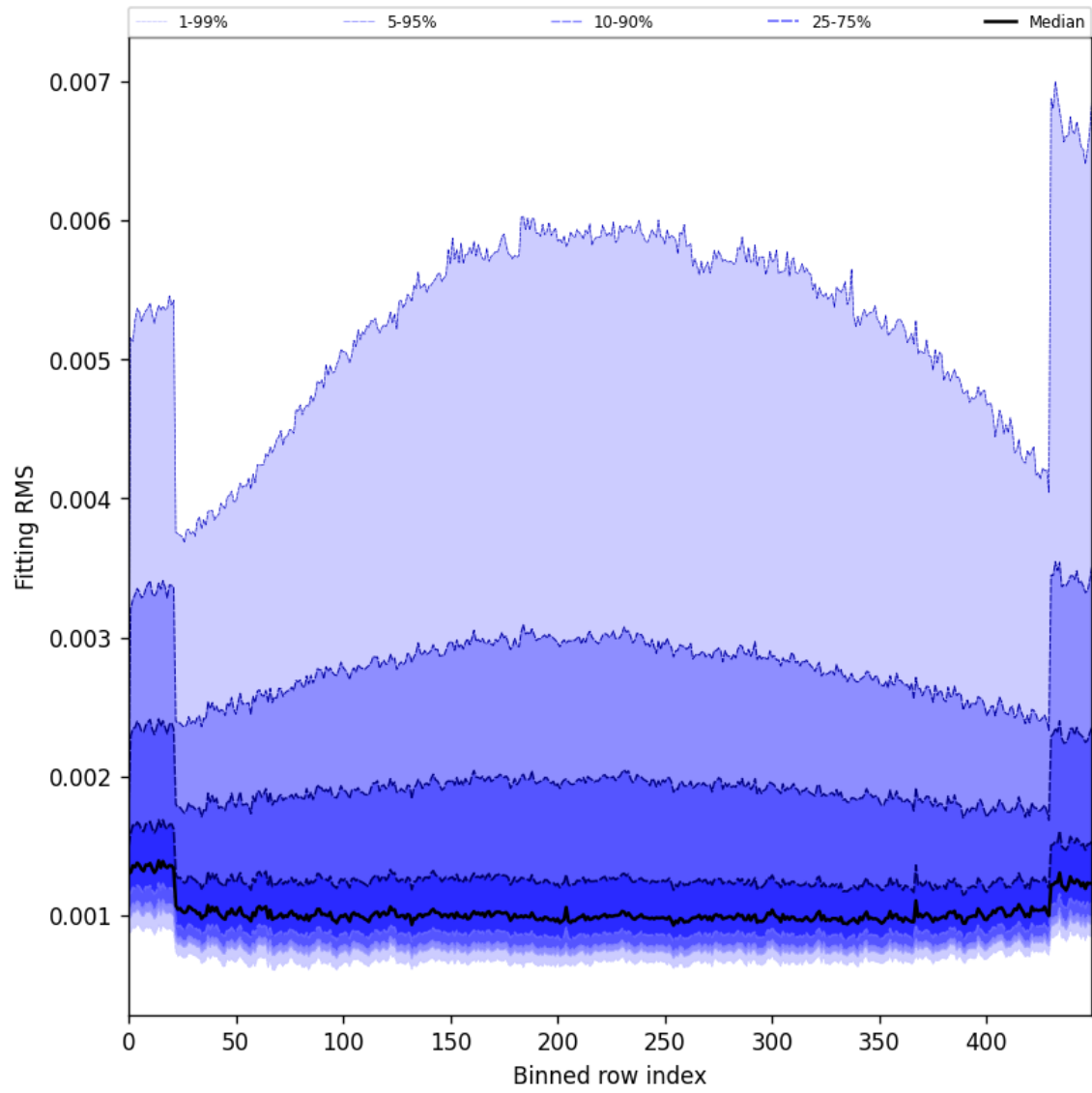
Figure 30: Along track statistics of “Fitting RMS” for 2025-07-04 to 2025-07-06
