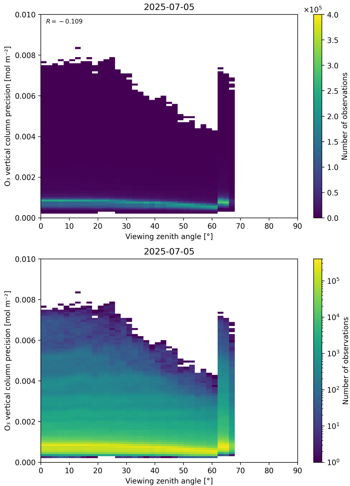
Figure 53: Scatter density plot of “Viewing zenith angle” against “O 3 vertical column precision” for 2025-07-04 to 2025-07-06.
