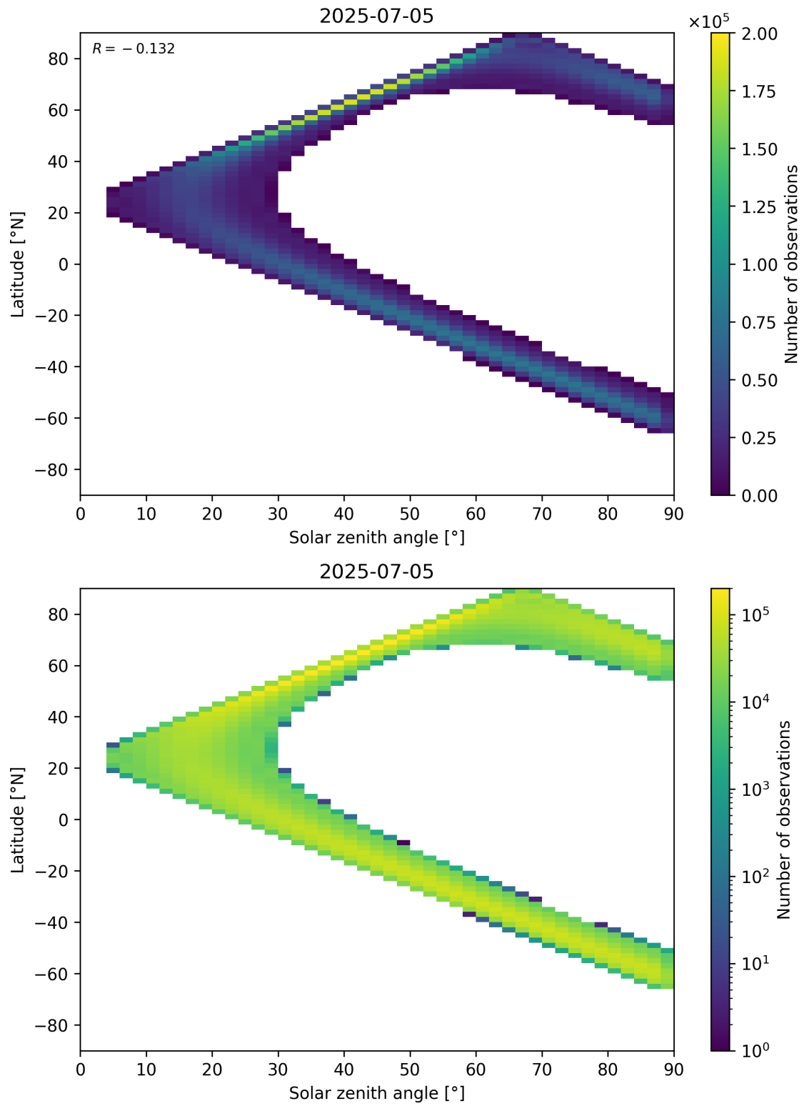
Figure 44: Scatter density plot of “Solar zenith angle” against “Latitude” for 2025-07-04 to 2025-07-06.
