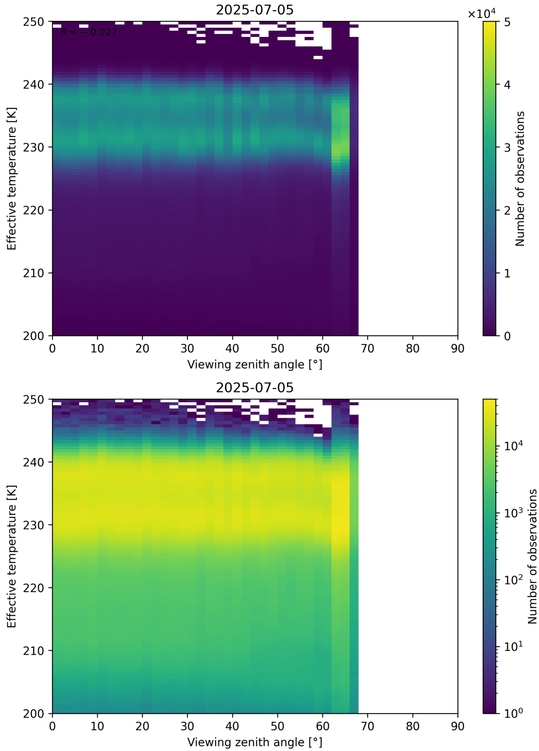
Figure 50: Scatter density plot of “Viewing zenith angle” against “Effective temperature” for 2025-07-04 to 2025-07-06.
