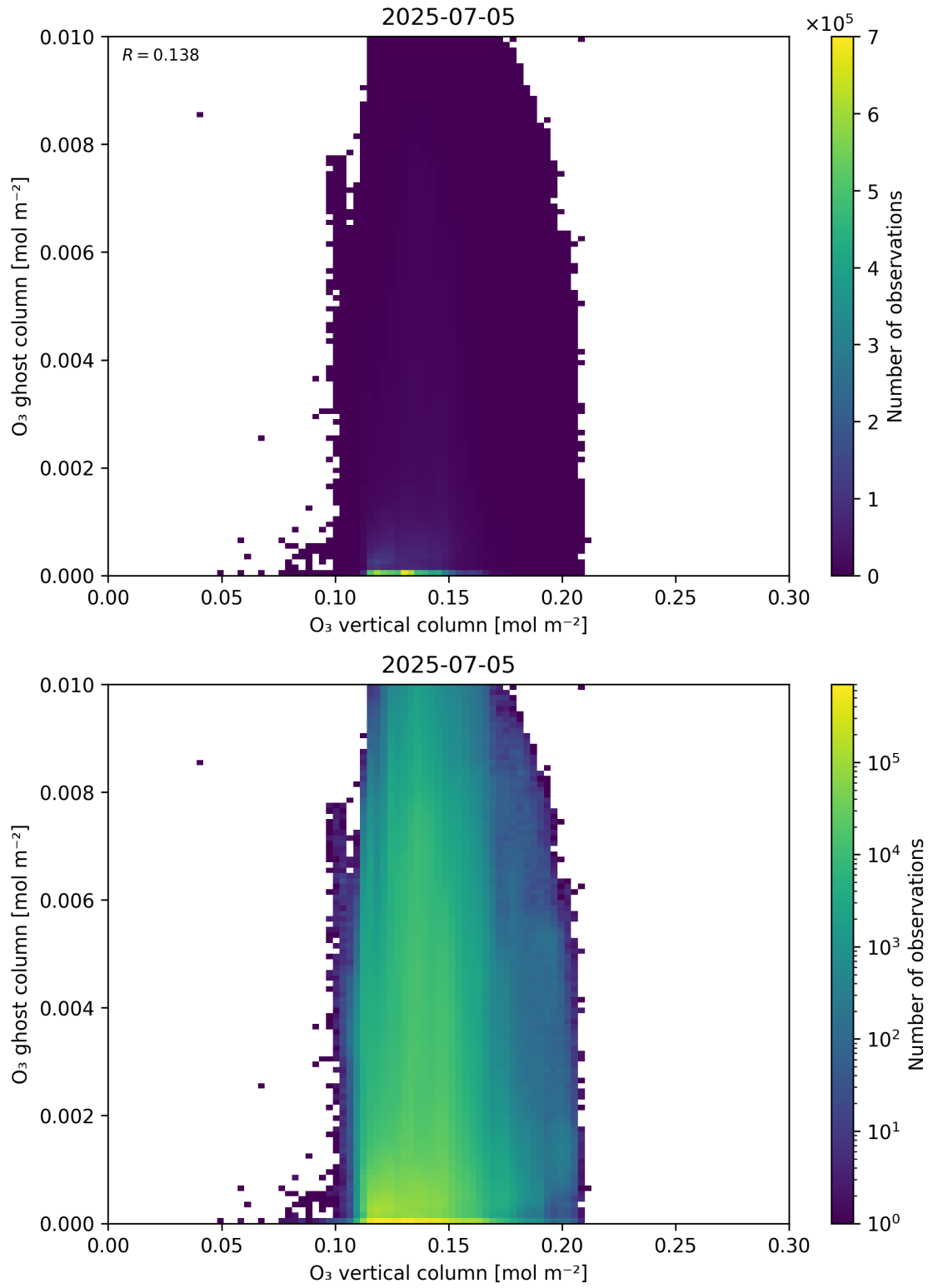
Figure 40: Scatter density plot of “O 3 vertical column” against “O 3 ghost column” for 2025-07-04 to 2025-07-06.
