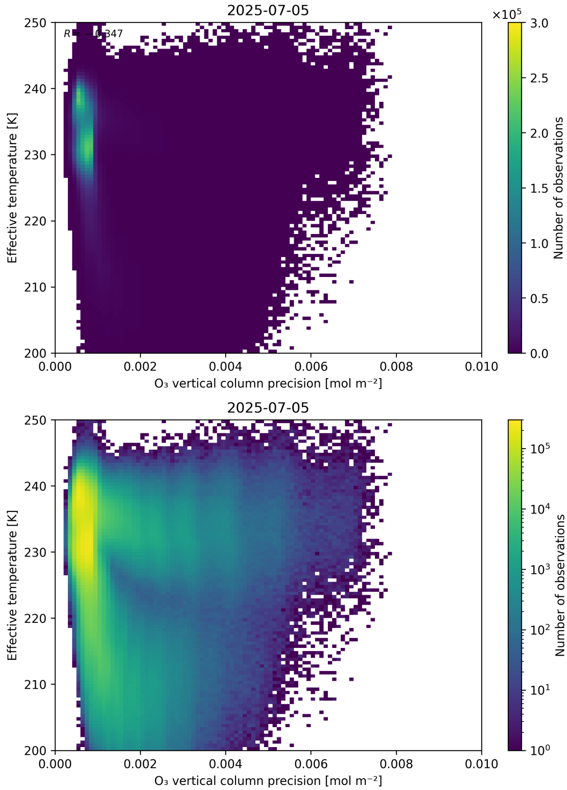
Figure 42: Scatter density plot of “O 3 vertical column precision” against “Effective temperature” for 2025-07-04 to 2025-07-06.
