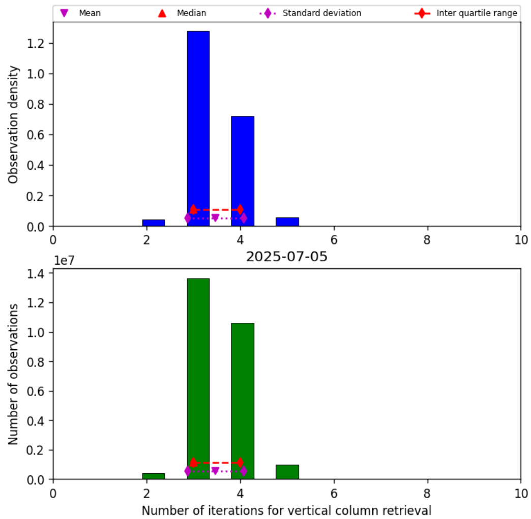
Figure 26: Histogram of “Number of iterations for vertical column retrieval” for 2025-07-04 to 2025-07-06
