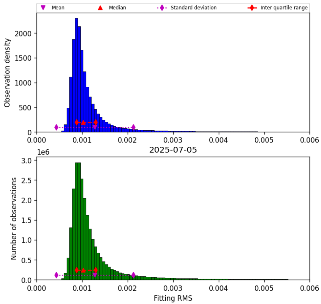
Figure 23: Histogram of “Fitting RMS” for 2025-07-04 to 2025-07-06
