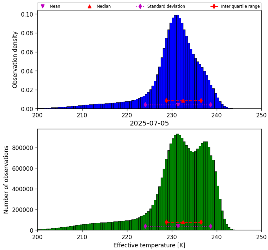
Figure 24: Histogram of “Effective temperature” for 2025-07-04 to 2025-07-06
