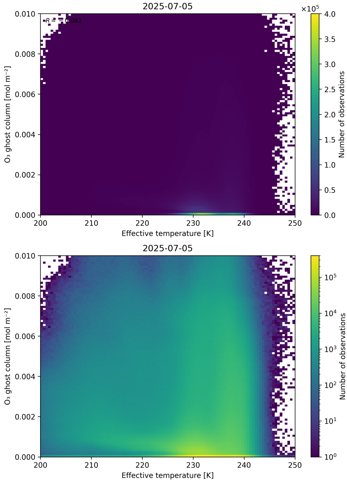
Figure 38: Scatter density plot of “Effective temperature” against “O 3 ghost column” for 2025-07-04 to 2025-07-06.
