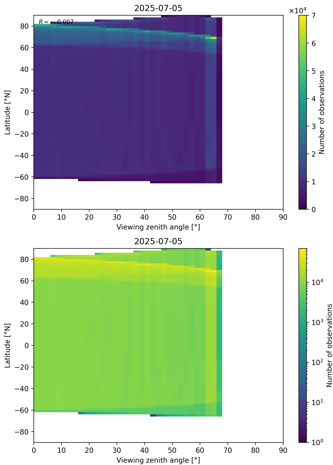
Figure 49: Scatter density plot of “Viewing zenith angle” against “Latitude” for 2025-07-04 to 2025-07-06.
