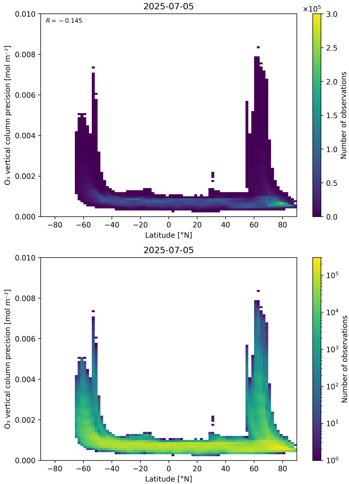
Figure 37: Scatter density plot of “Latitude” against “O 3 vertical column precision” for 2025-07-04 to 2025-07-06.
