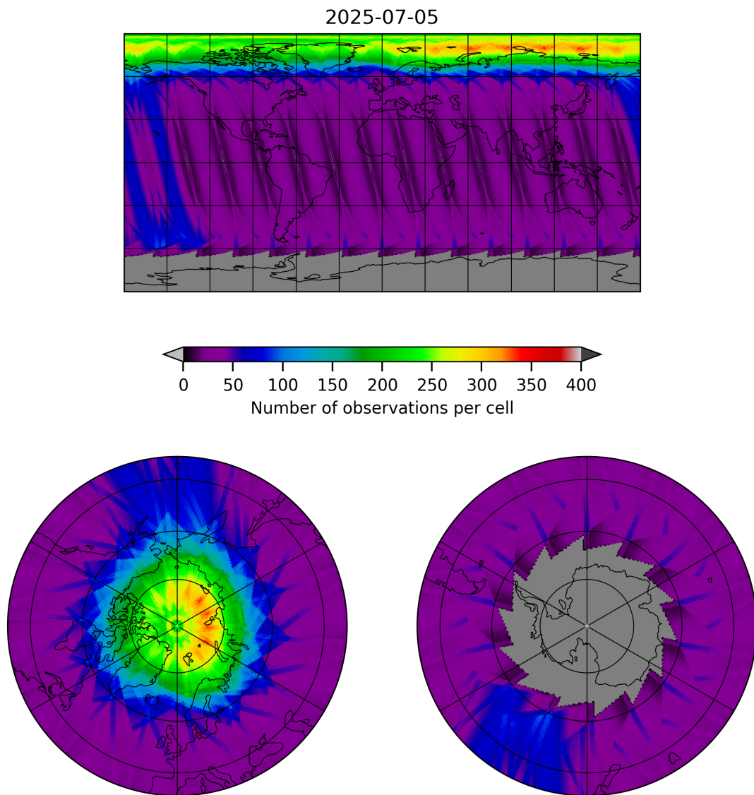
Figure 12: Map of the number of observations for 2025-07-04 to 2025-07-06
