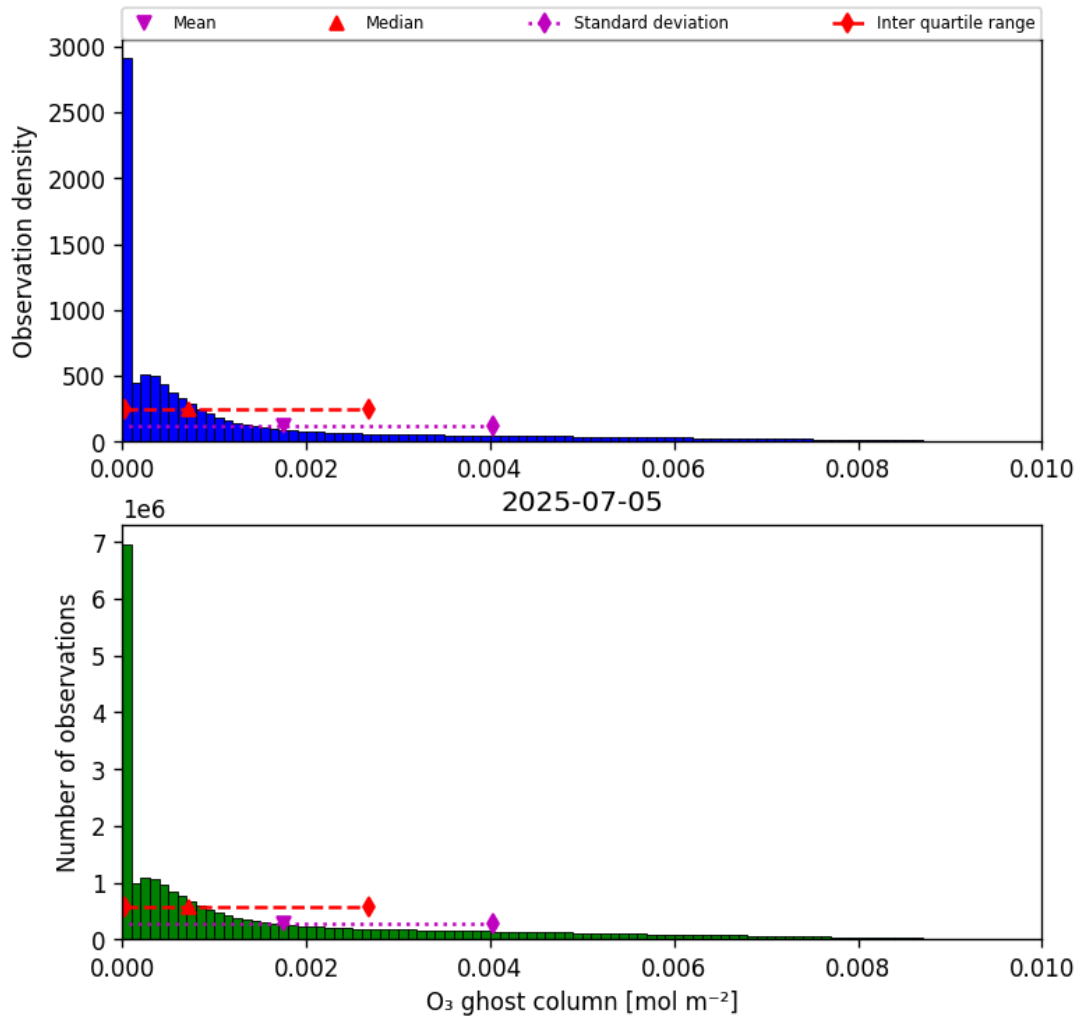
Figure 25: Histogram of “O 3 ghost column” for 2025-07-04 to 2025-07-06
