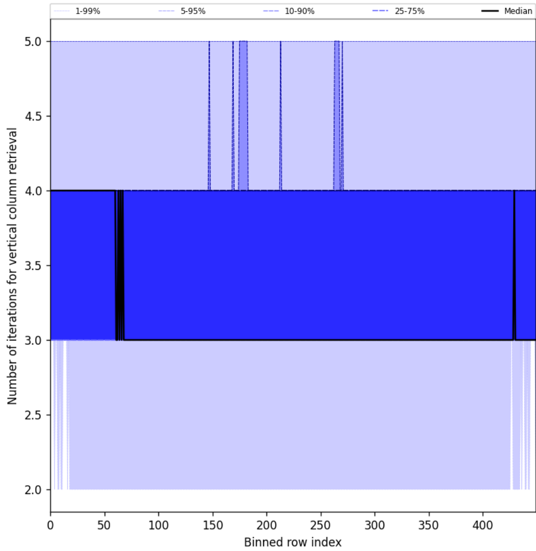
Figure 33: Along track statistics of “Number of iterations for vertical column retrieval” for 2025-07-04 to 2025-07-06
