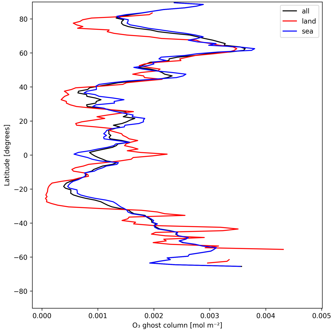
Figure 18: Zonal average of "O 3 ghost column" for 2025-07-04 to 2025-07-06.
