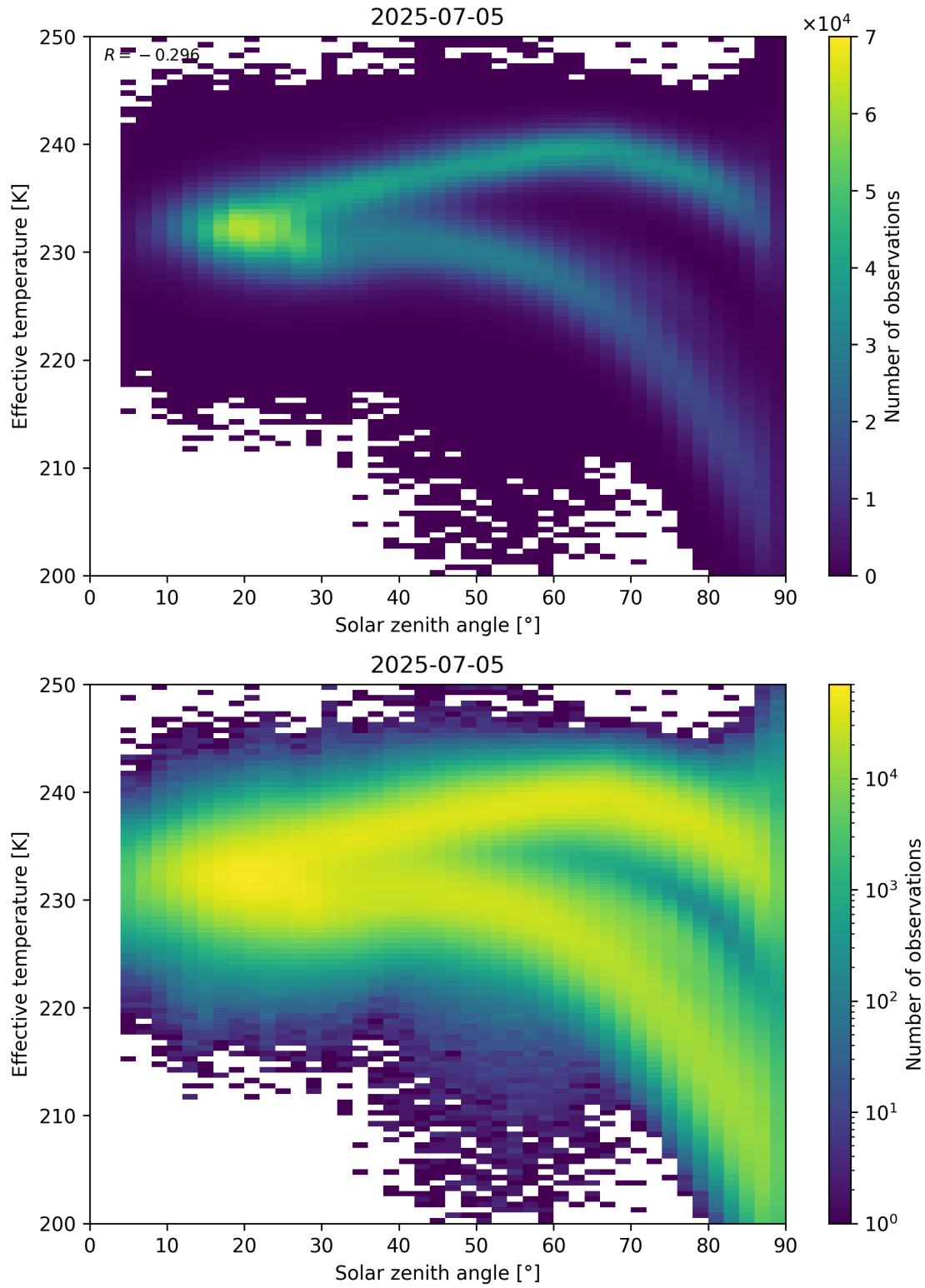
Figure 45: Scatter density plot of “Solar zenith angle” against “Effective temperature” for 2025-07-04 to 2025-07-06.
