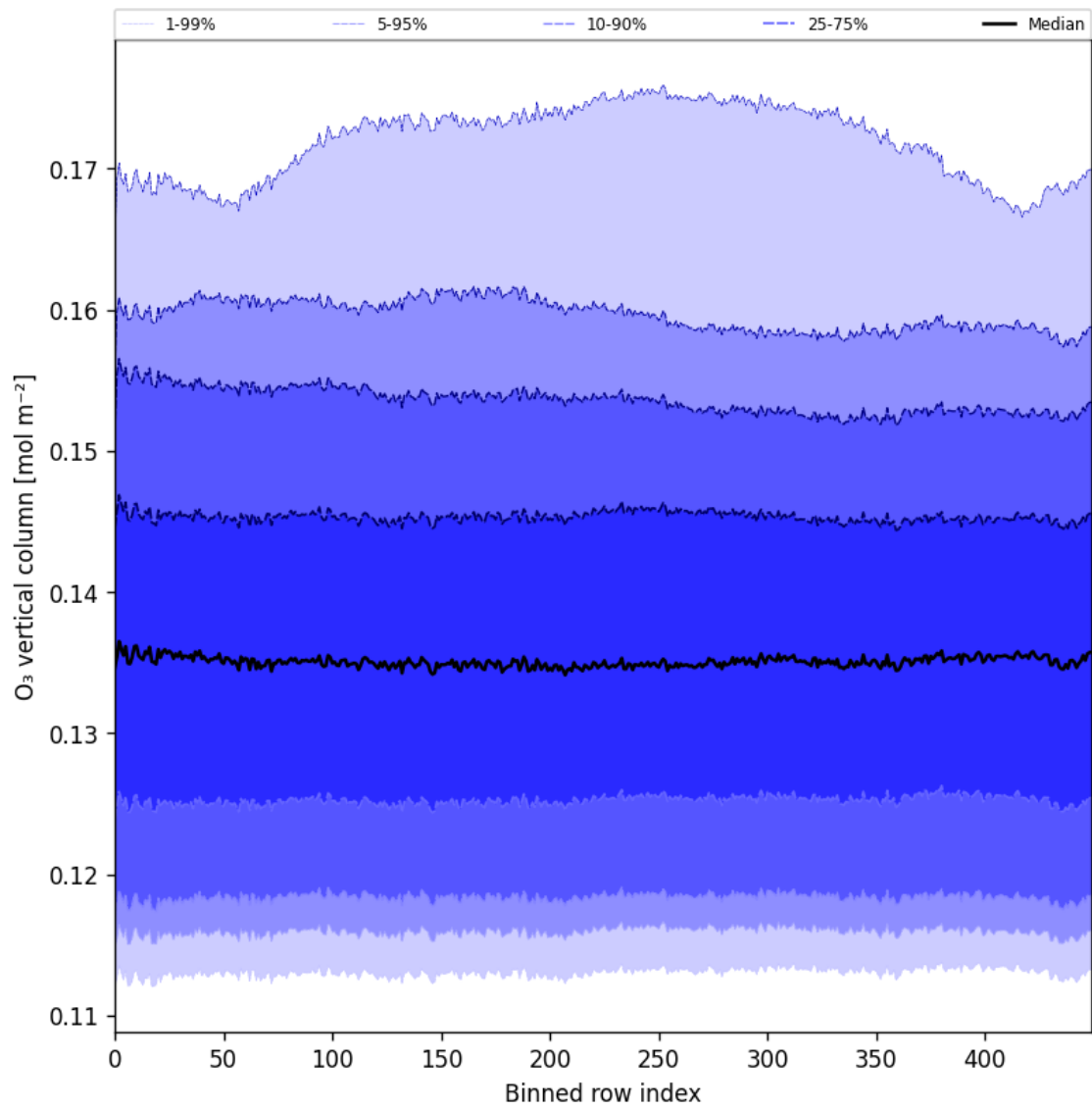
Figure 28: Along track statistics of “O 3 vertical column” for 2025-07-04 to 2025-07-06
