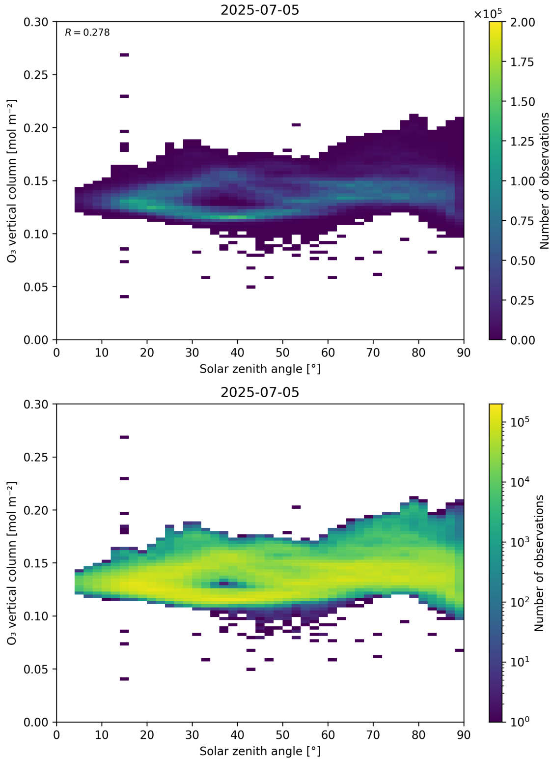
Figure 47: Scatter density plot of “Solar zenith angle” against “O 3 vertical column” for 2025-07-04 to 2025-07-06.
