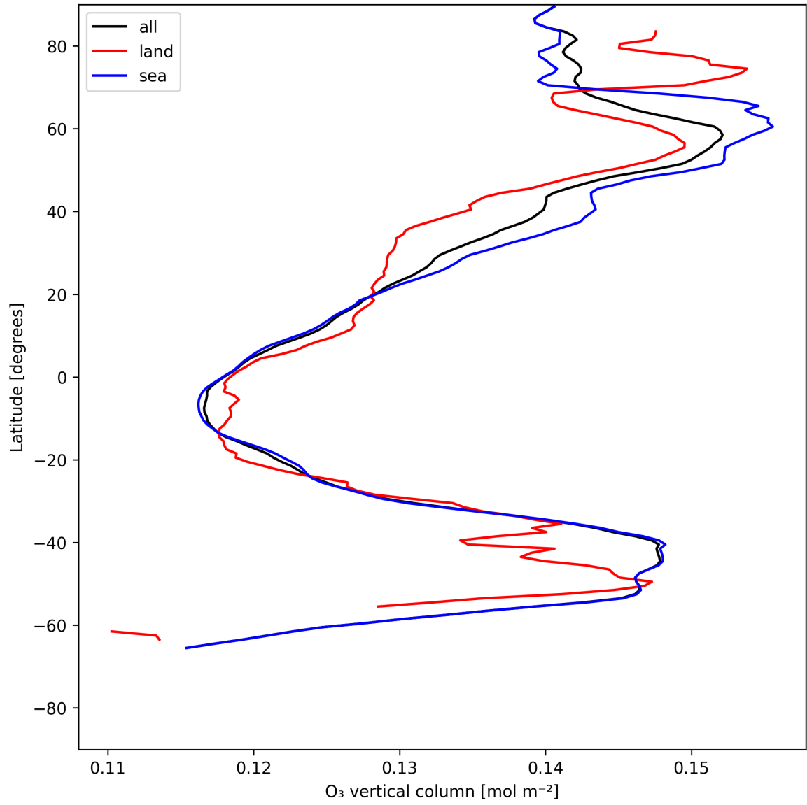
Figure 14: Zonal average of “O 3 vertical column” for 2025-07-04 to 2025-07-06.
