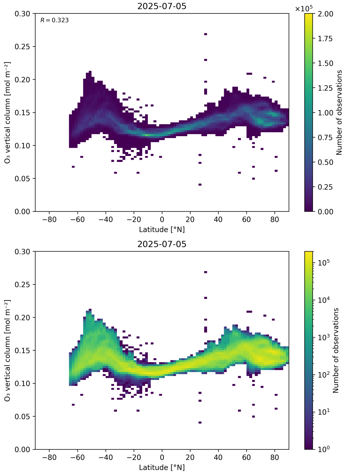
Figure 36: Scatter density plot of “Latitude” against “O 3 vertical column” for 2025-07-04 to 2025-07-06.
