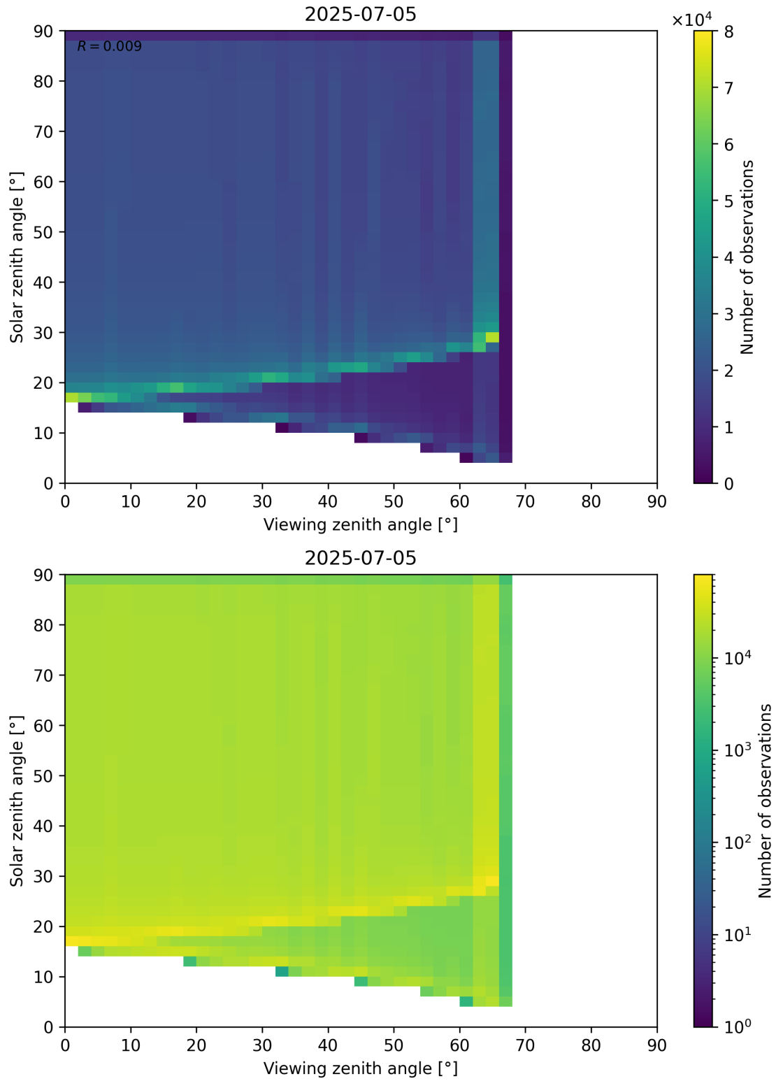
Figure 54: Scatter density plot of “Viewing zenith angle” against “Solar zenith angle” for 2025-07-04 to 2025-07-06.
