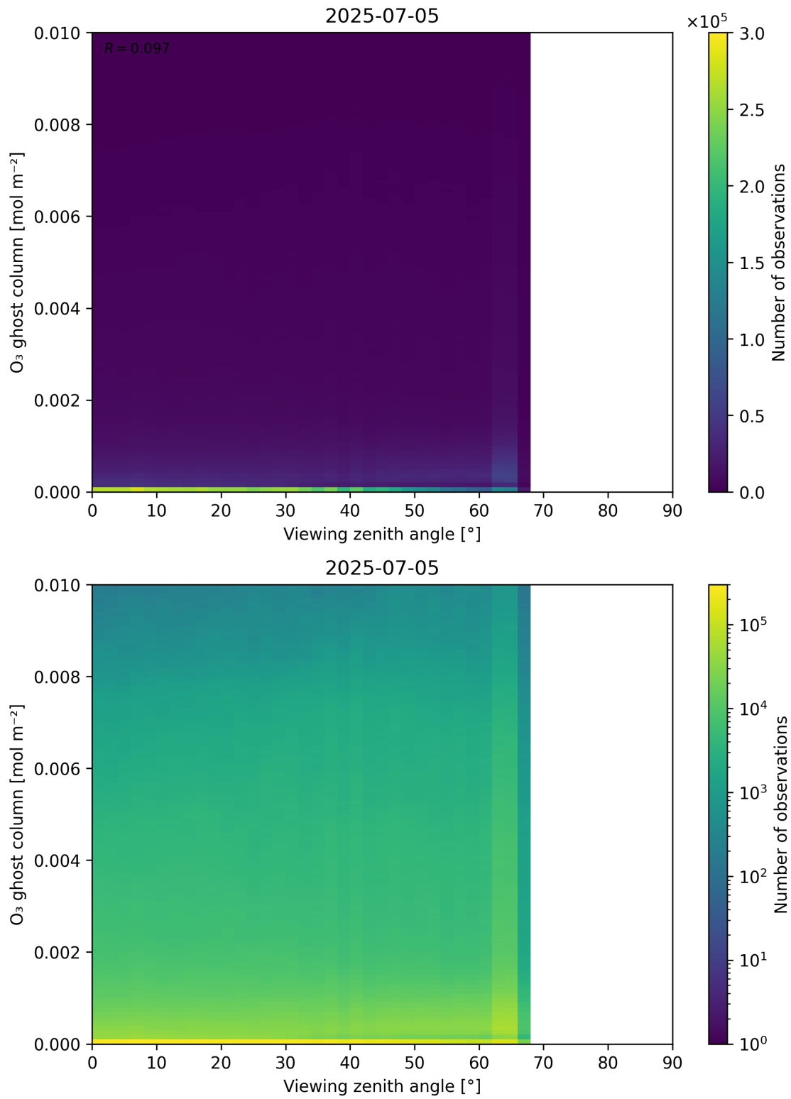
Figure 51: Scatter density plot of “Viewing zenith angle” against “O 3 ghost column” for 2025-07-04 to 2025-07-06.
