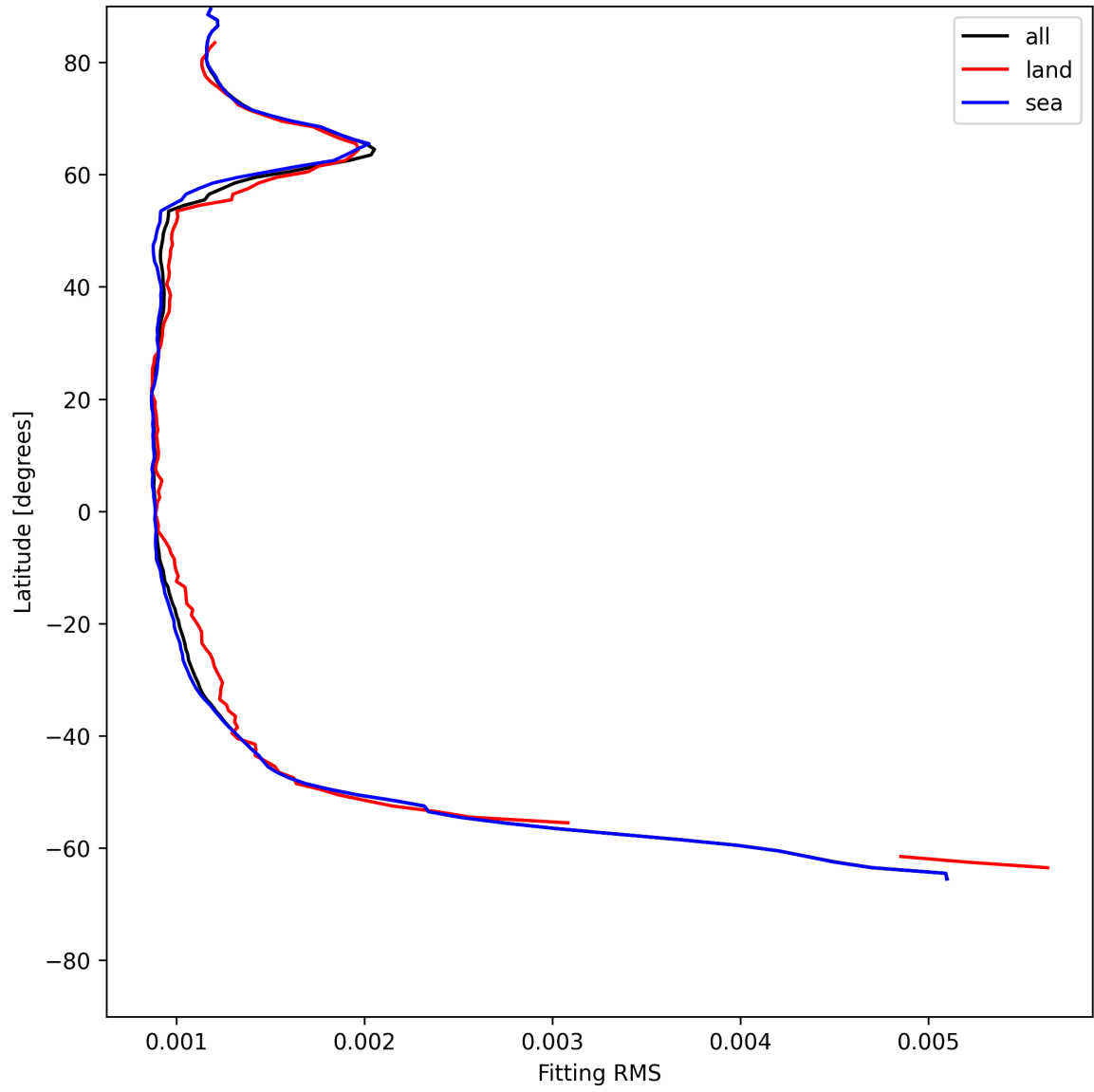
Figure 16: Zonal average of “Fitting RMS” for 2025-07-04 to 2025-07-06.
