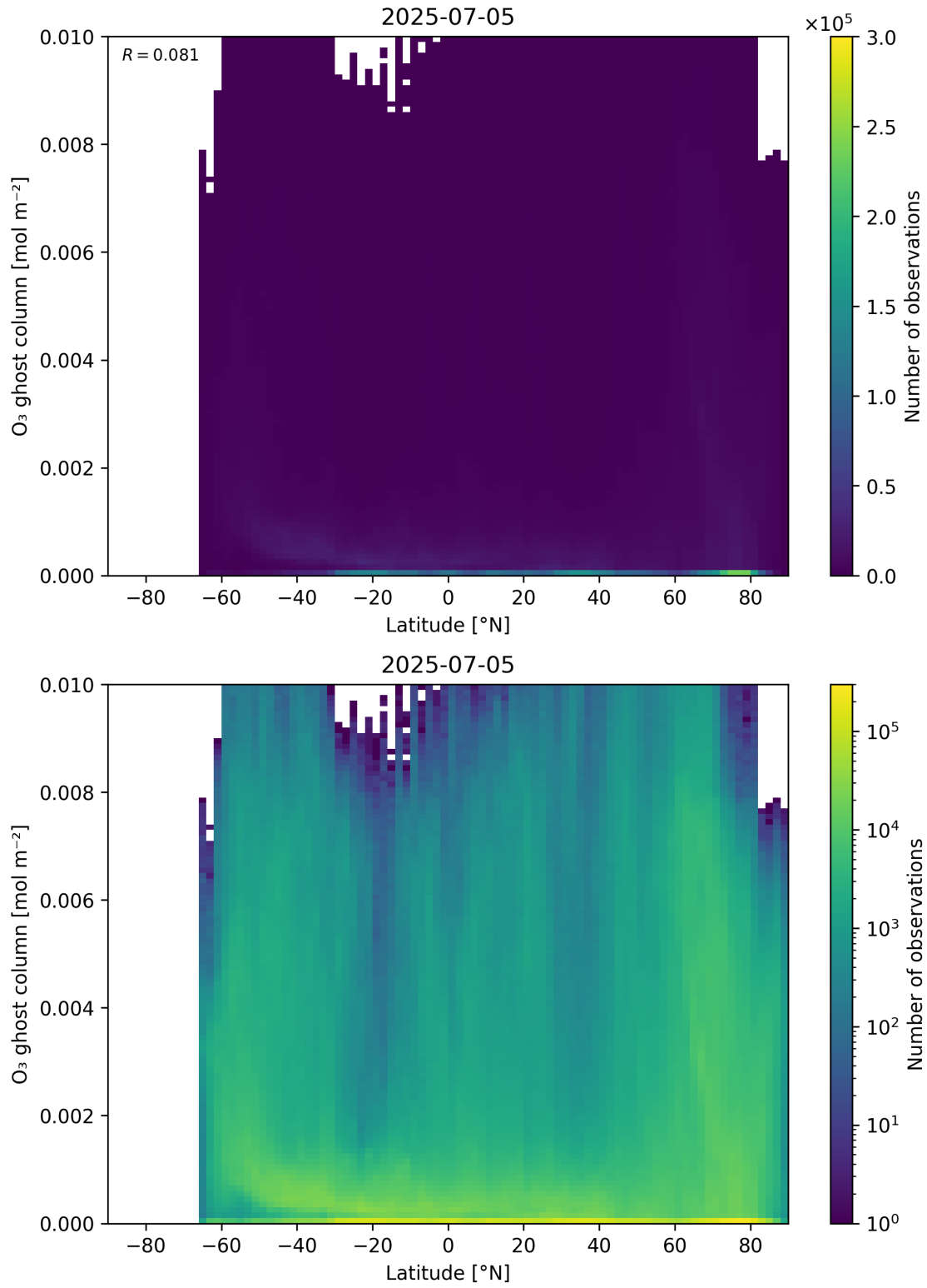
Figure 35: Scatter density plot of “Latitude” against “O 3 ghost column” for 2025-07-04 to 2025-07-06.
