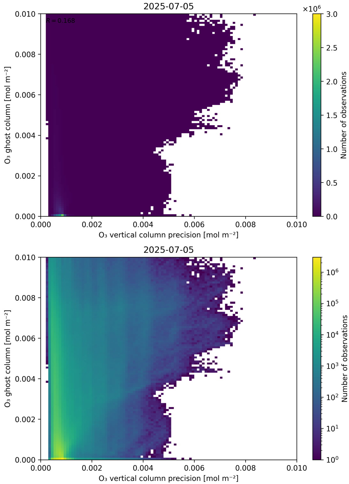
Figure 43: Scatter density plot of “ \text{O}_3 vertical column precision” against “ \text{O}_3 ghost column” for 2025-07-04 to 2025-07-06.
