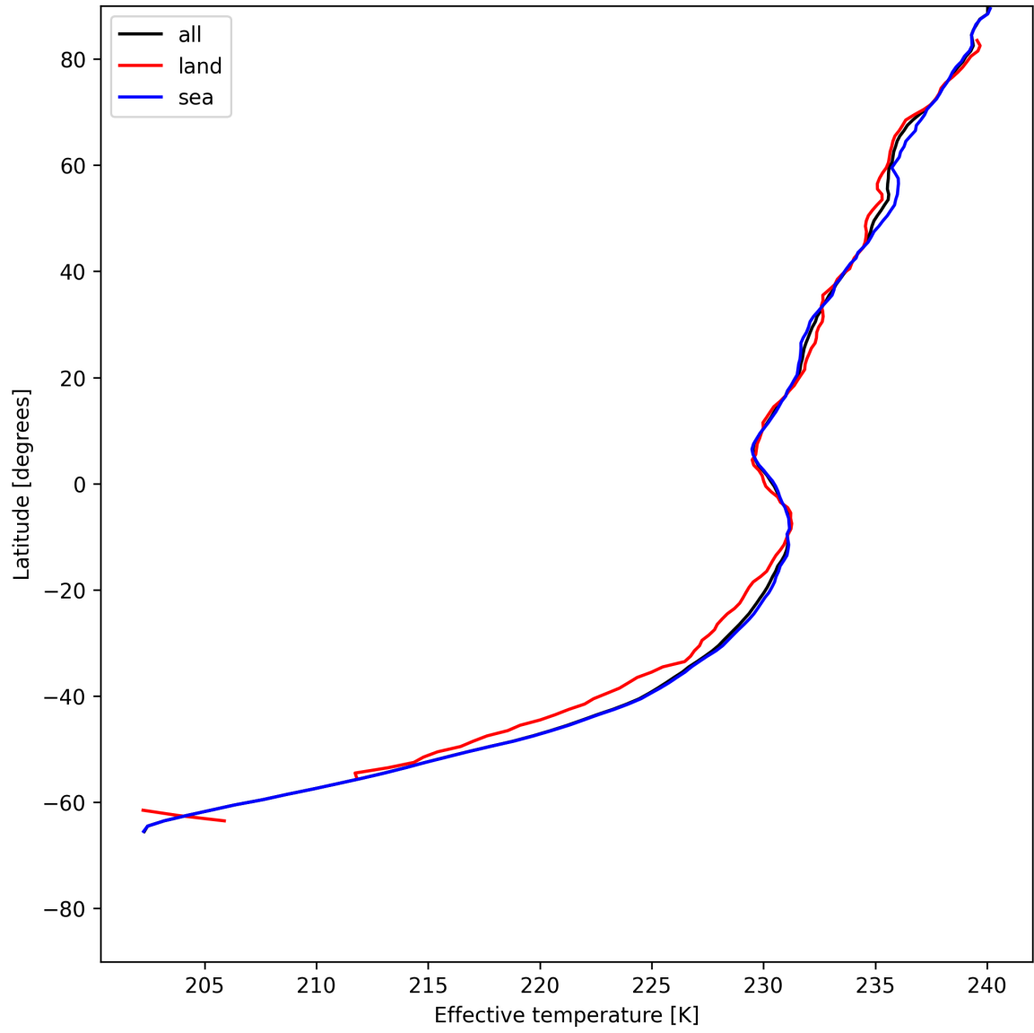
Figure 17: Zonal average of “Effective temperature” for 2025-07-04 to 2025-07-06.
