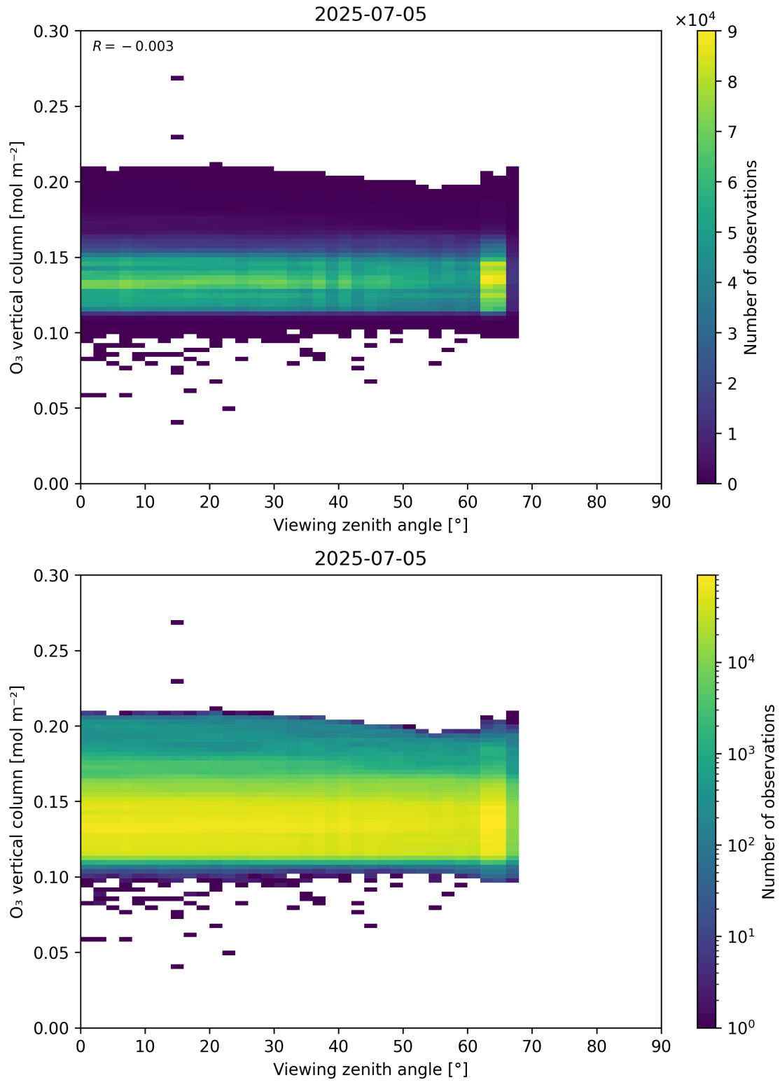
Figure 52: Scatter density plot of “Viewing zenith angle” against “O 3 vertical column” for 2025-07-04 to 2025-07-06.
