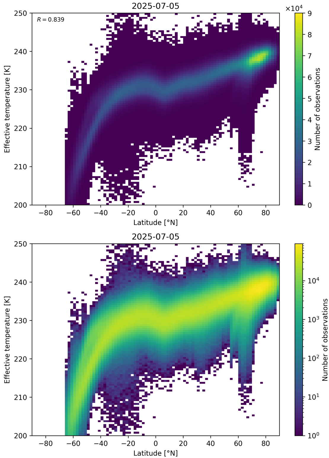
Figure 34: Scatter density plot of “Latitude” against “Effective temperature” for 2025-07-04 to 2025-07-06.
