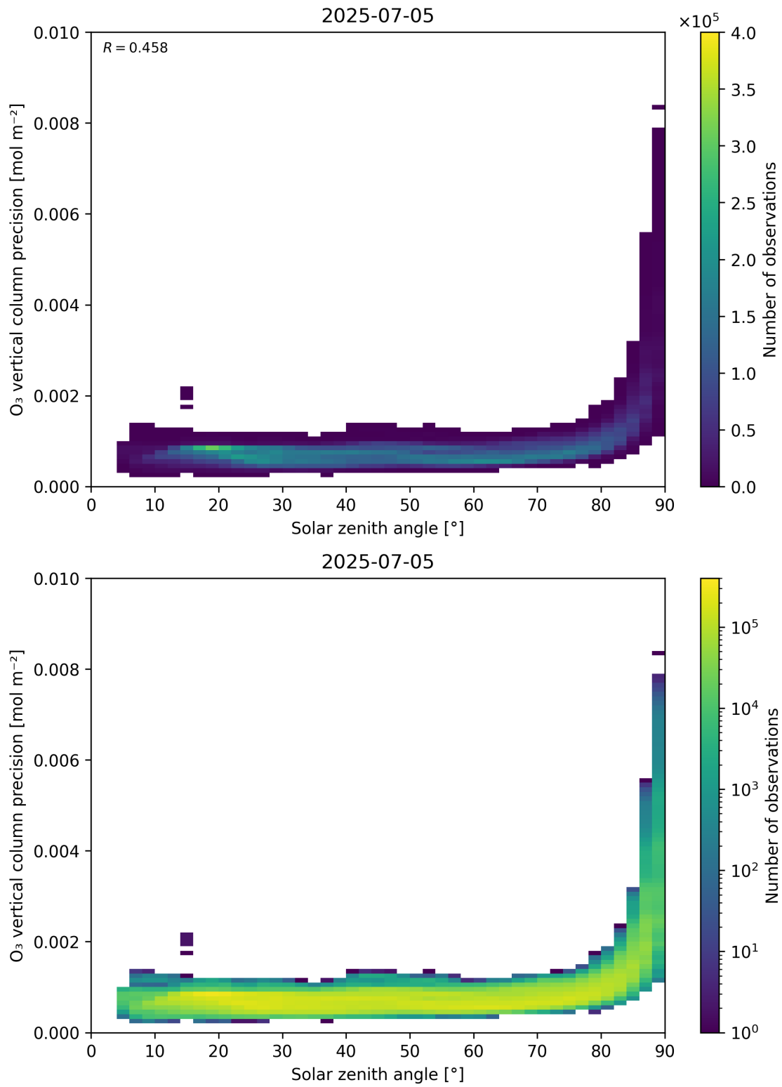
Figure 48: Scatter density plot of “Solar zenith angle” against “O 3 vertical column precision” for 2025-07-04 to 2025-07-06.
