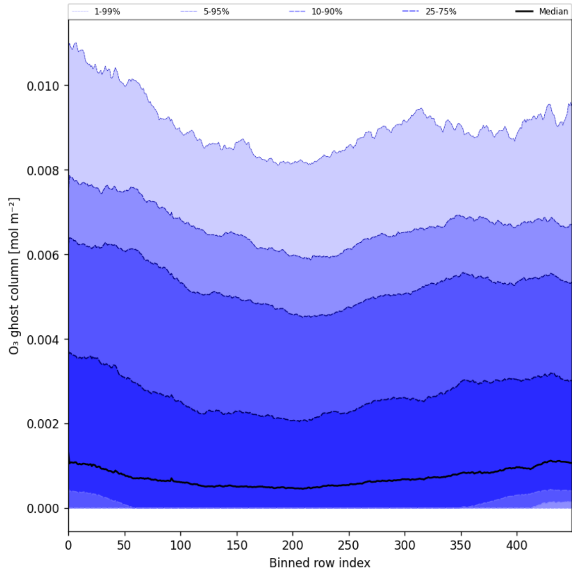
Figure 32: Along track statistics of “O 3 ghost column” for 2025-07-04 to 2025-07-06
