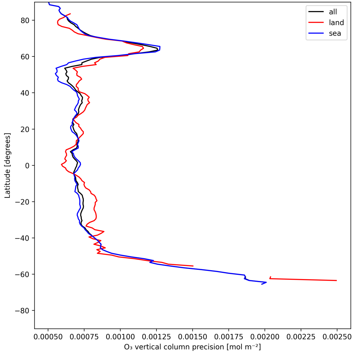
Figure 15: Zonal average of “O 3 vertical column precision” for 2025-07-04 to 2025-07-06.
