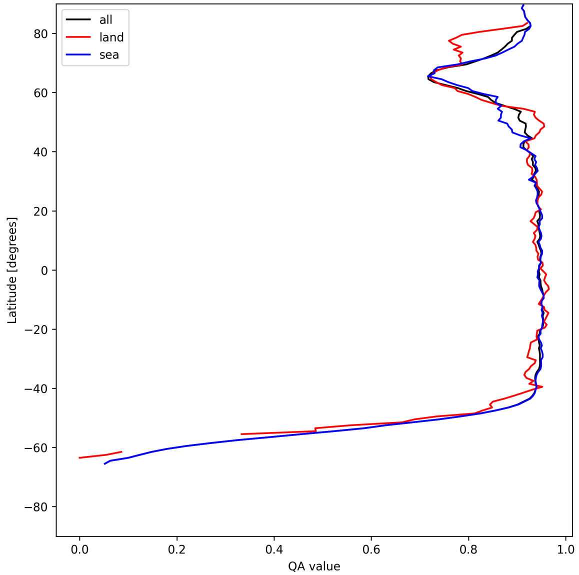
Figure 13: Zonal average of “QA value” for 2025-07-04 to 2025-07-06.
