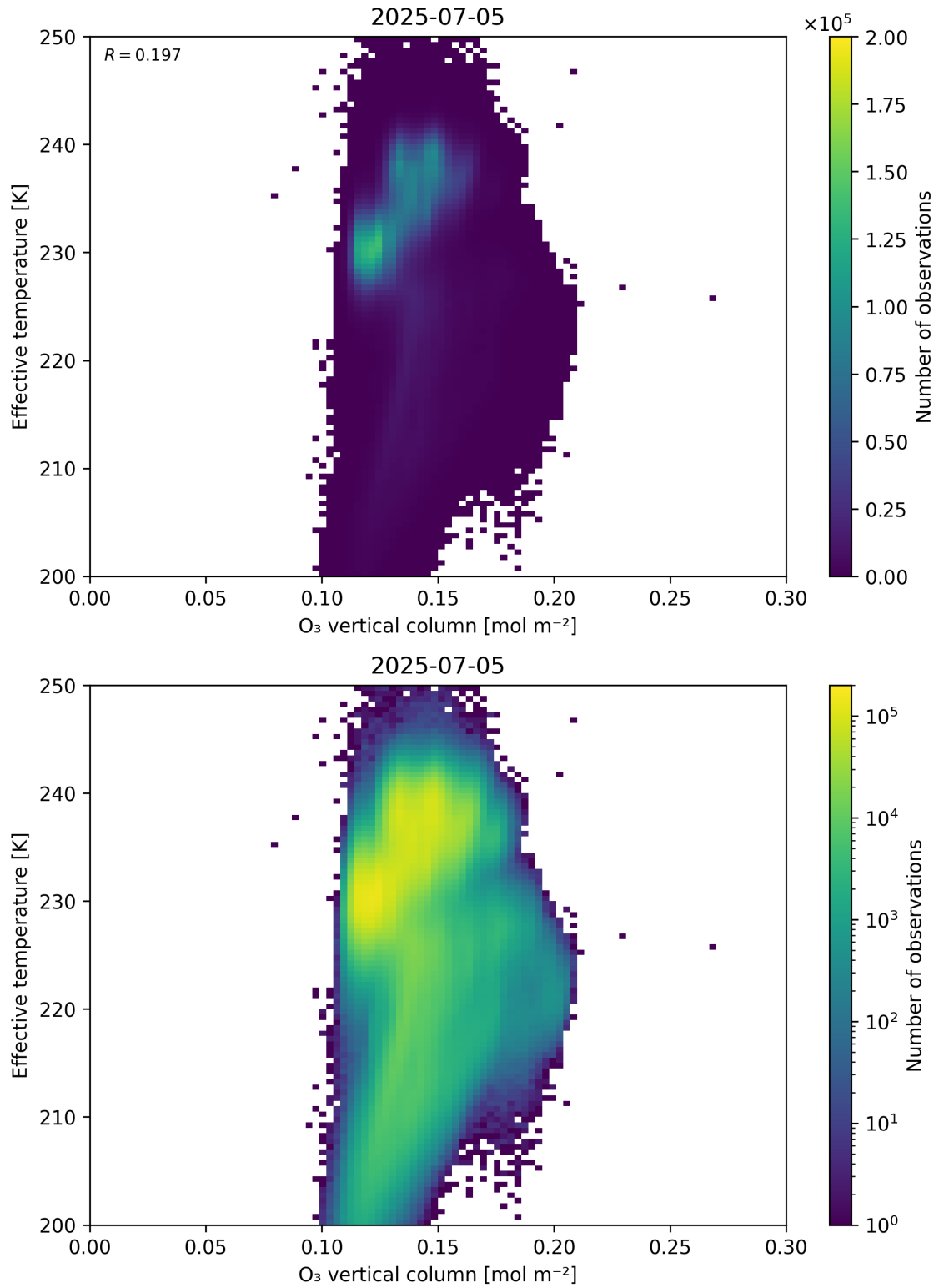
Figure 39: Scatter density plot of “O 3 vertical column” against “Effective temperature” for 2025-07-04 to 2025-07-06.
