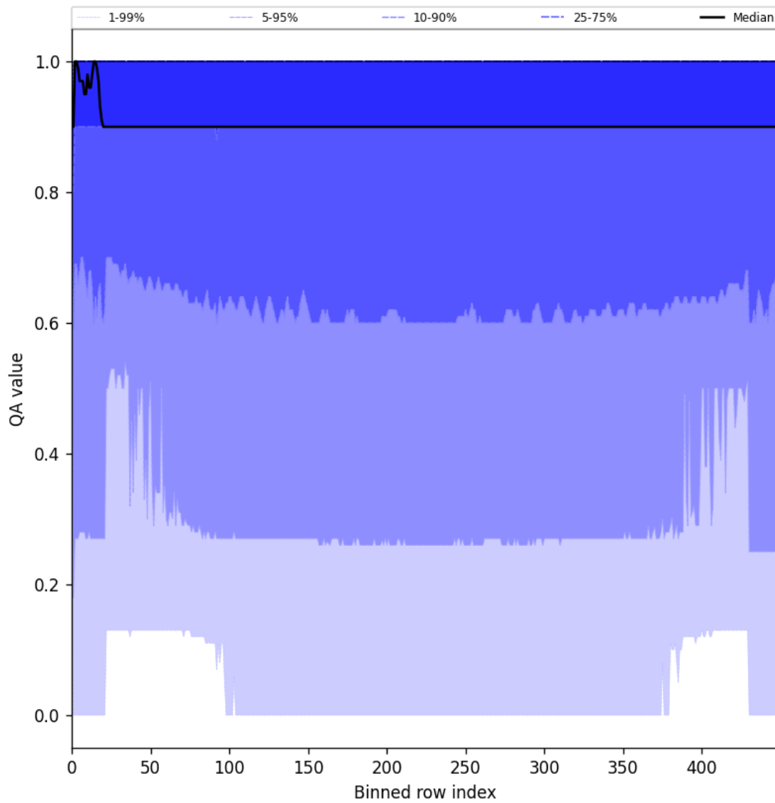
Figure 27: Along track statistics of “QA value” for 2025-07-04 to 2025-07-06
