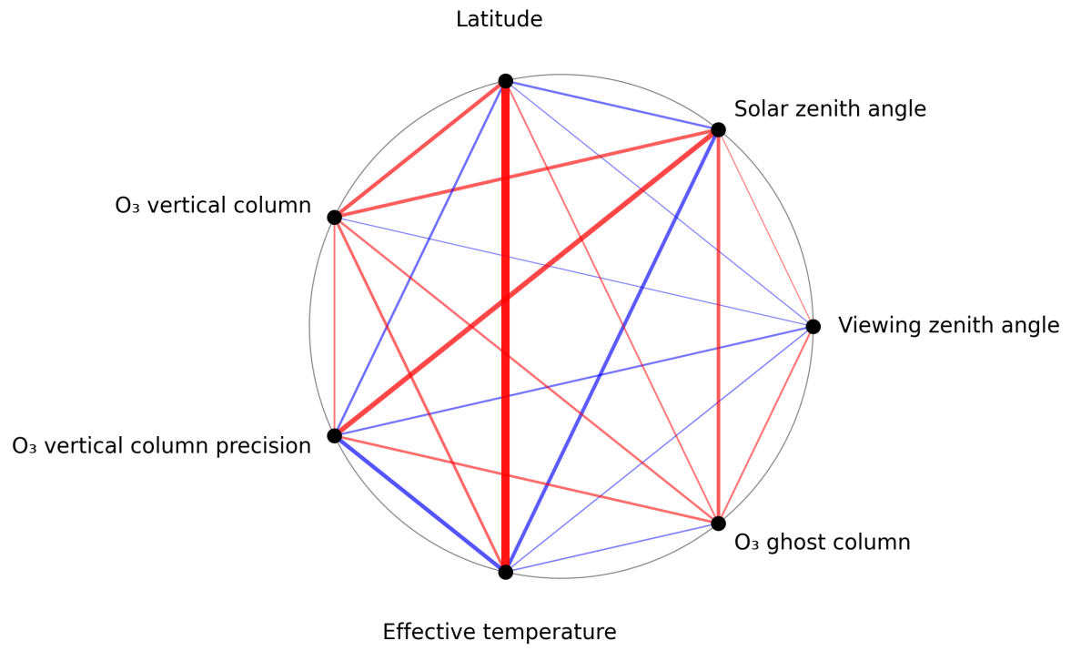
Figure 1: Map of correlation graph for 2025-07-04 to 2025-07-06.
