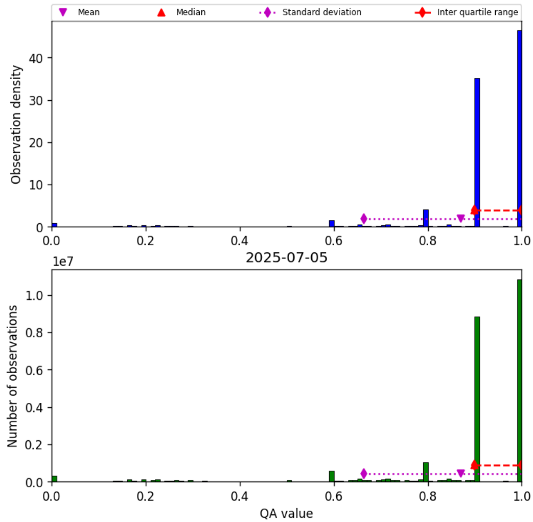
Figure 20: Histogram of “QA value” for 2025-07-04 to 2025-07-06
