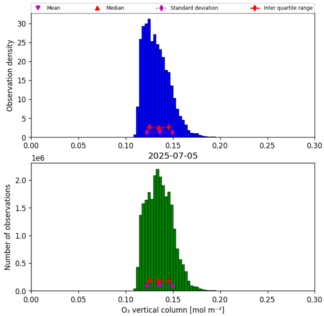
Figure 21: Histogram of “O 3 vertical column” for 2025-07-04 to 2025-07-06
