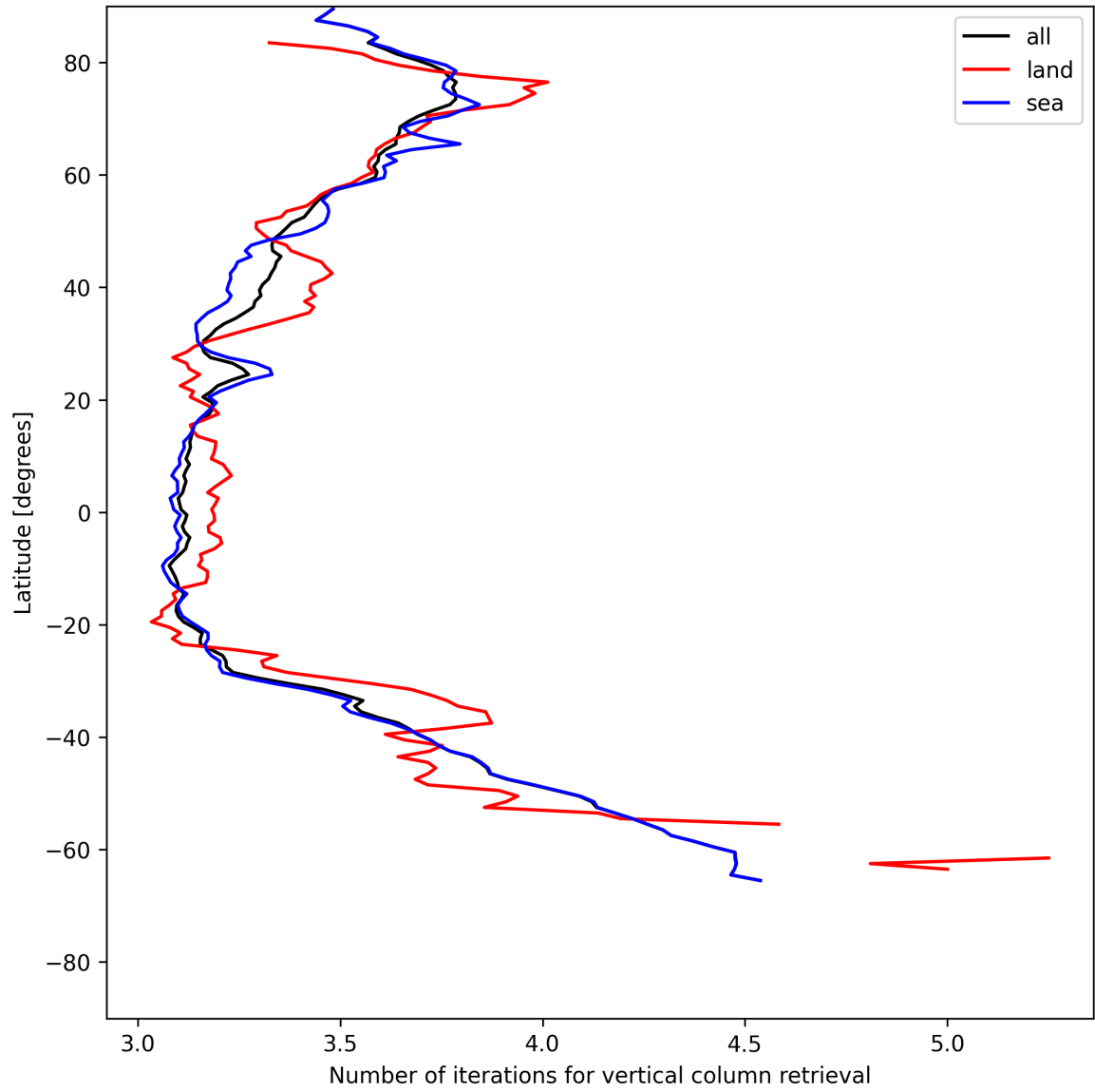
Figure 19: Zonal average of “Number of iterations for vertical column retrieval” for 2025-07-04 to 2025-07-06.
