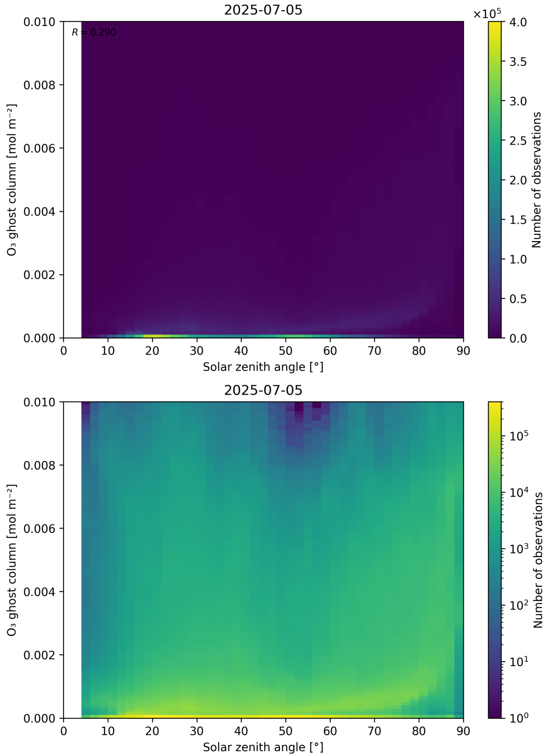
Figure 46: Scatter density plot of “Solar zenith angle” against “O 3 ghost column” for 2025-07-04 to 2025-07-06.
