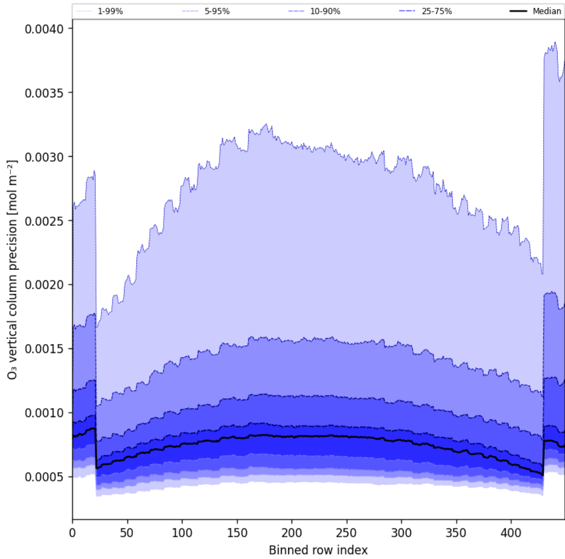
Figure 29: Along track statistics of “O 3 vertical column precision” for 2025-07-04 to 2025-07-06
