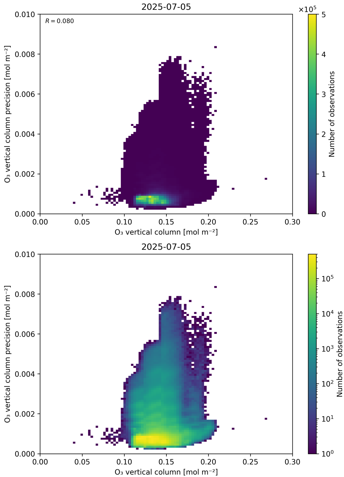
Figure 41: Scatter density plot of “O 3 vertical column” against “O 3 vertical column precision” for 2025-07-04 to 2025-07-06.
