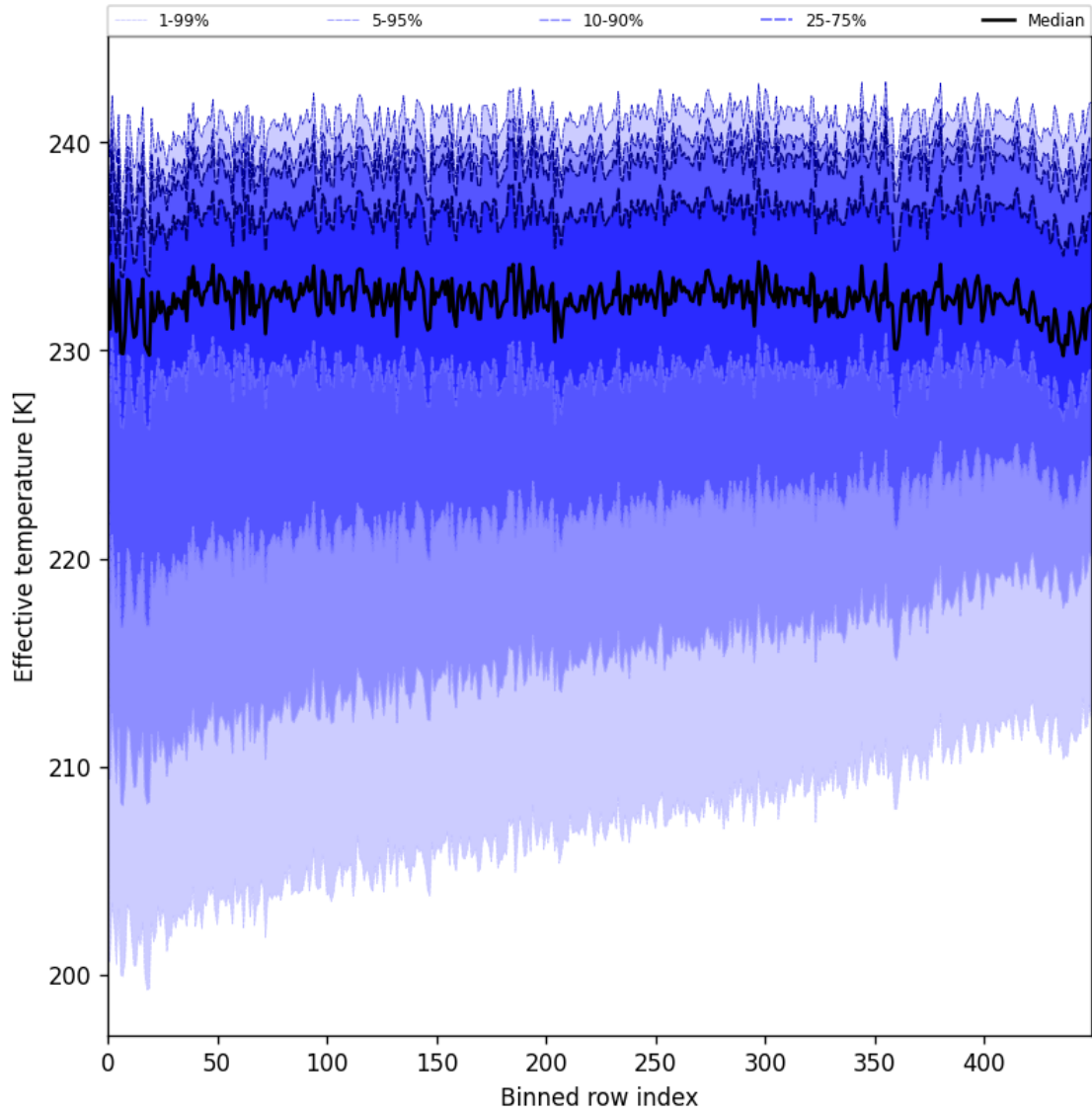
Figure 31: Along track statistics of “Effective temperature” for 2025-07-04 to 2025-07-06
