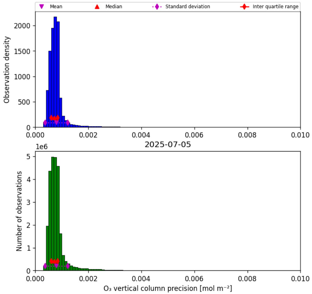
Figure 22: Histogram of “O 3 vertical column precision” for 2025-07-04 to 2025-07-06
