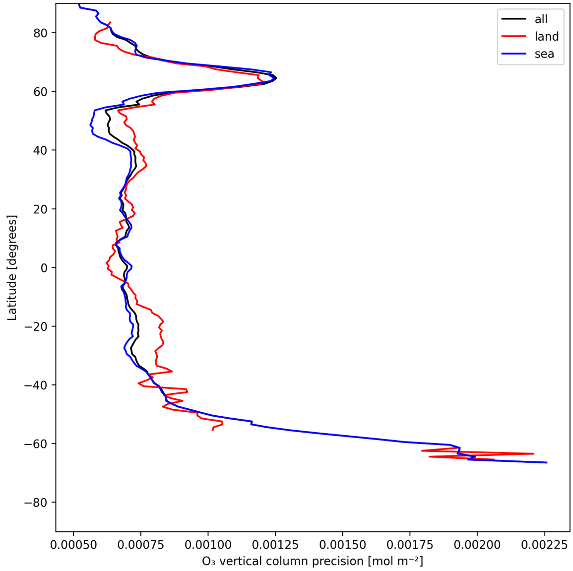
Figure 15: Zonal average of “O 3 vertical column precision” for 2025-07-05 to 2025-07-07.
