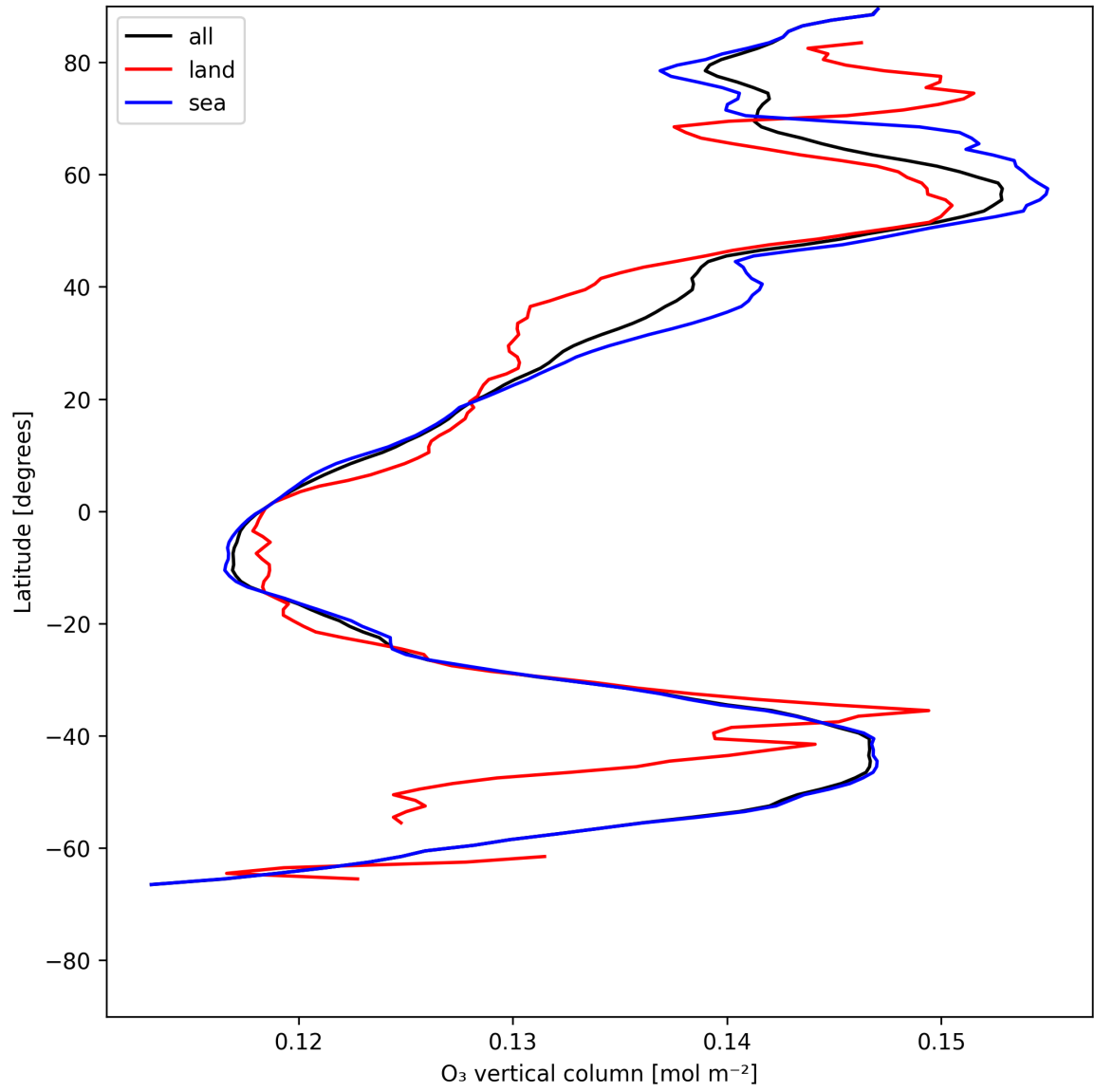
Figure 14: Zonal average of “O 3 vertical column” for 2025-07-05 to 2025-07-07.
