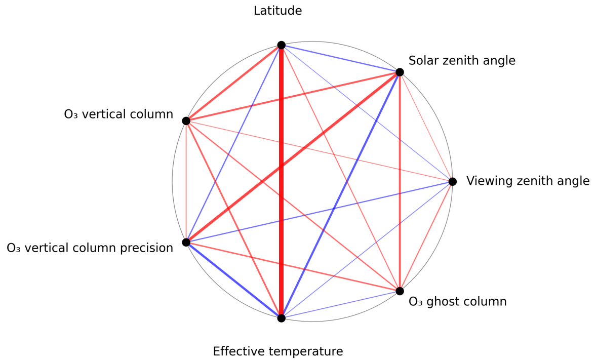
Figure 1: Map of correlation graph for 2025-07-05 to 2025-07-07.
