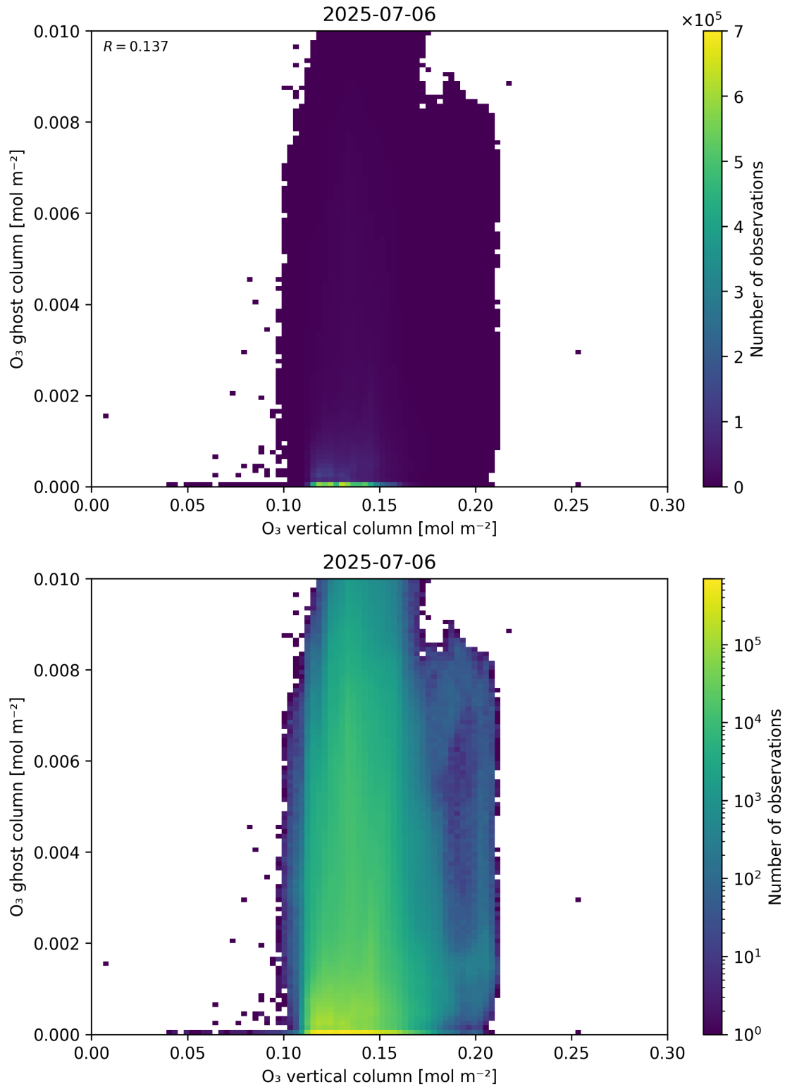
Figure 40: Scatter density plot of “O 3 vertical column” against “O 3 ghost column” for 2025-07-05 to 2025-07-07.
