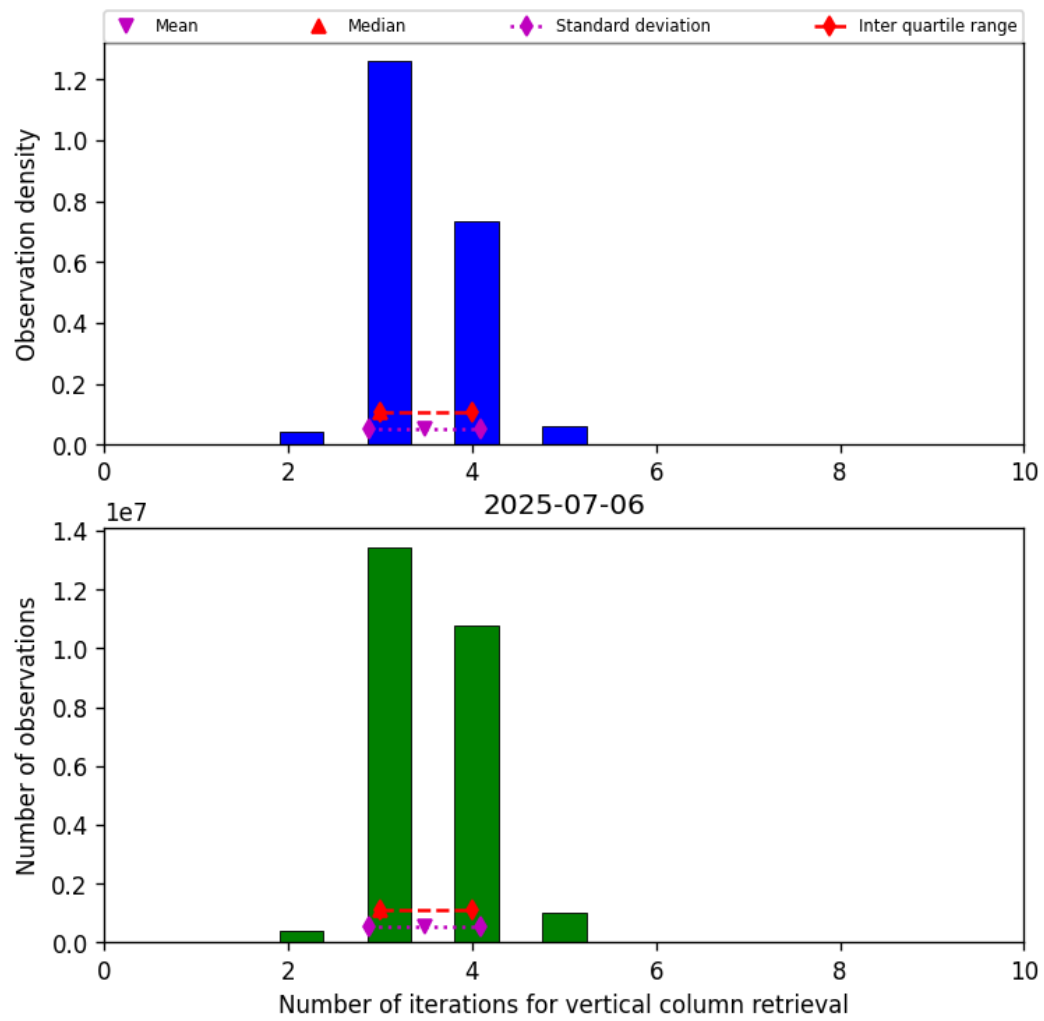
Figure 26: Histogram of “Number of iterations for vertical column retrieval” for 2025-07-05 to 2025-07-07
