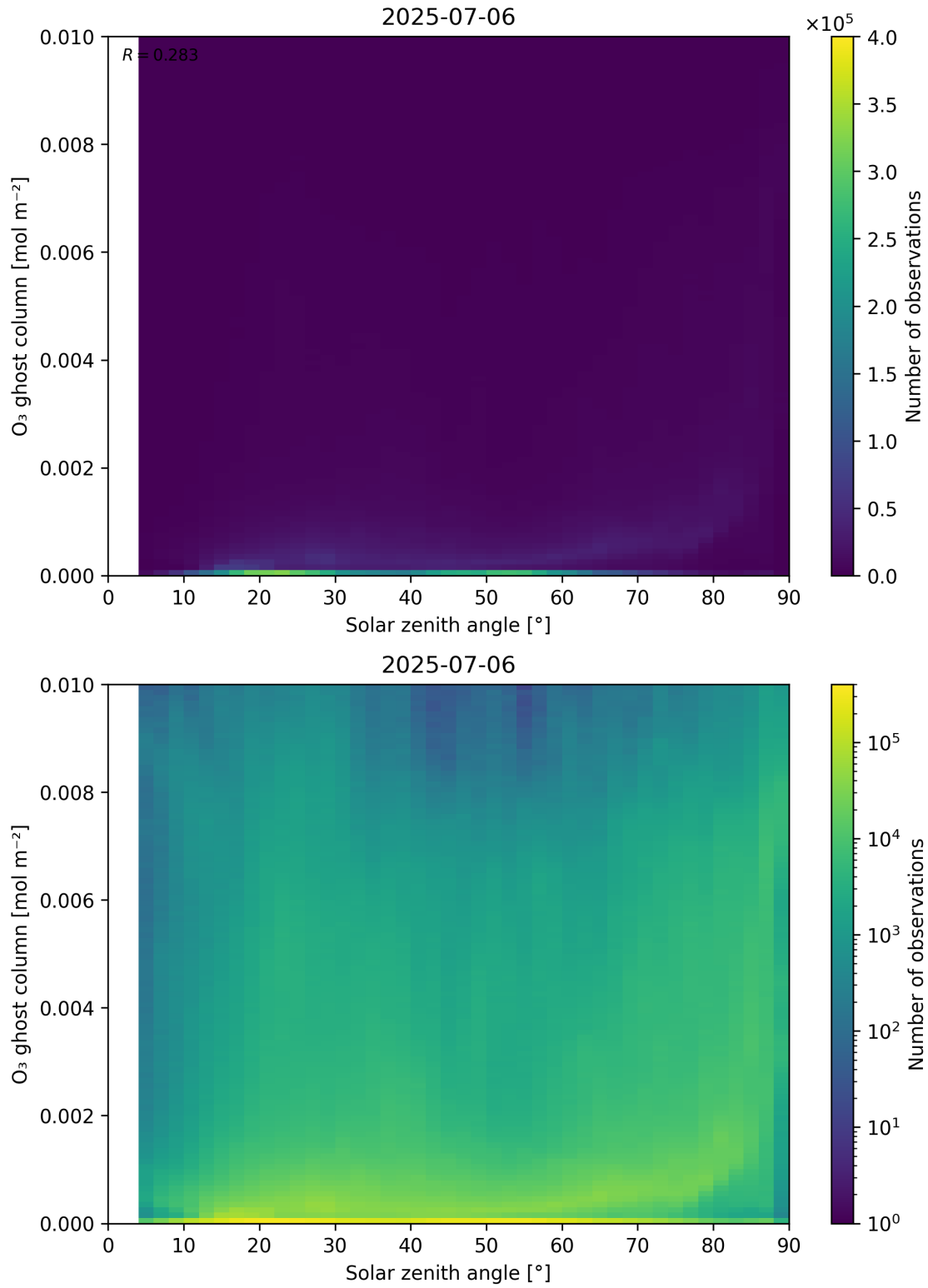
Figure 46: Scatter density plot of “Solar zenith angle” against “O 3 ghost column” for 2025-07-05 to 2025-07-07.
