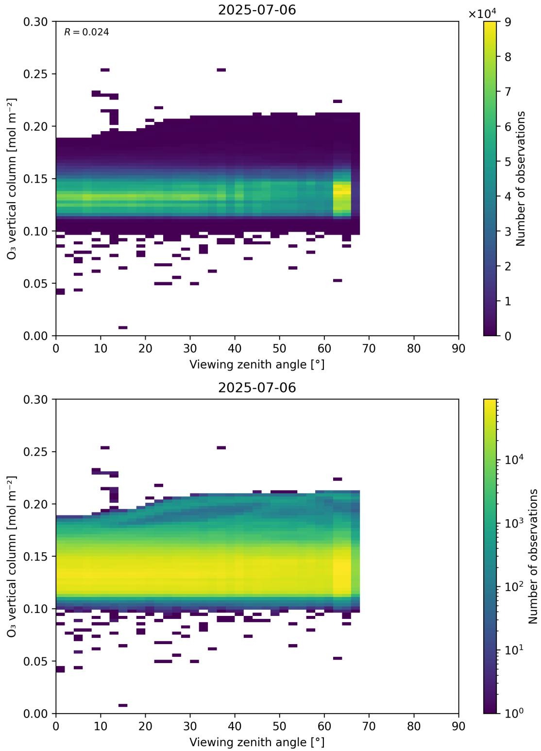
Figure 52: Scatter density plot of “Viewing zenith angle” against “O 3 vertical column” for 2025-07-05 to 2025-07-07.
