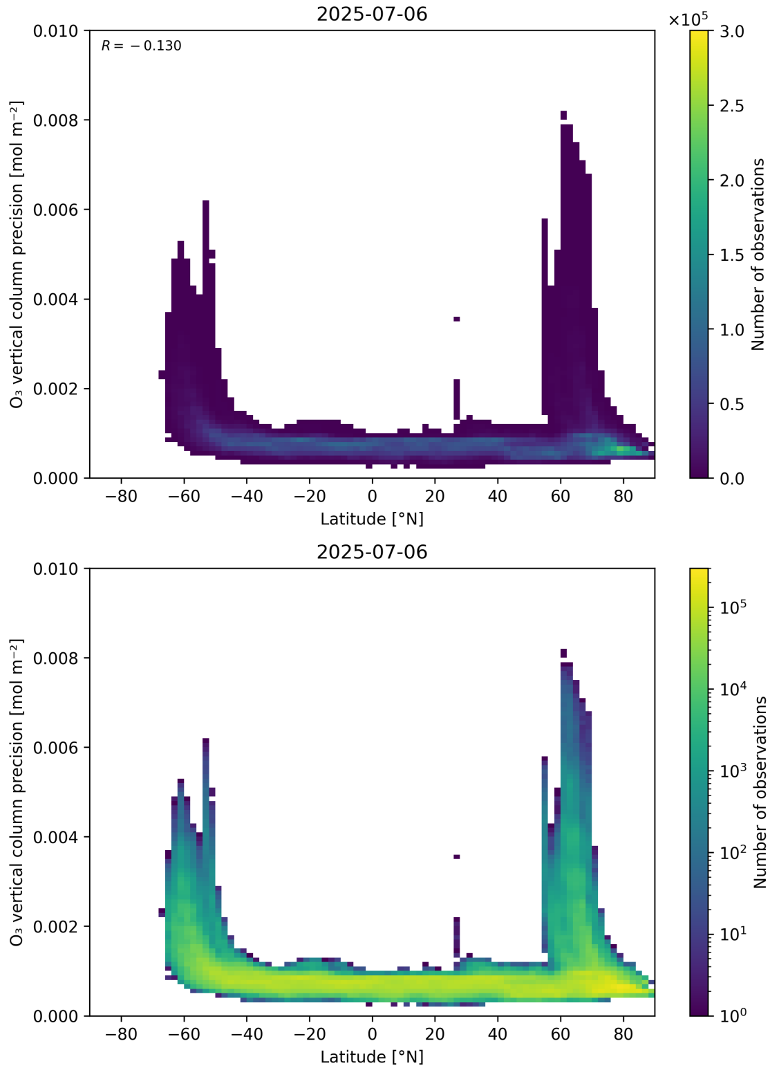
Figure 37: Scatter density plot of “Latitude” against “O 3 vertical column precision” for 2025-07-05 to 2025-07-07.
