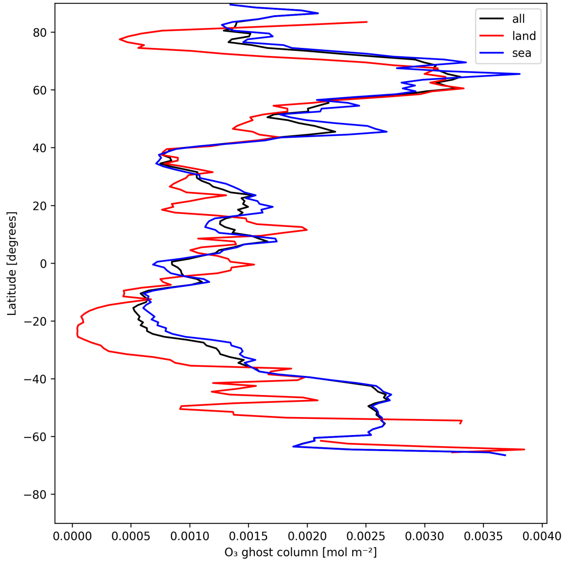
Figure 18: Zonal average of "O 3 ghost column" for 2025-07-05 to 2025-07-07.
