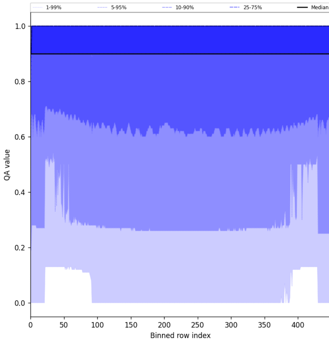
Figure 27: Along track statistics of “QA value” for 2025-07-05 to 2025-07-07
