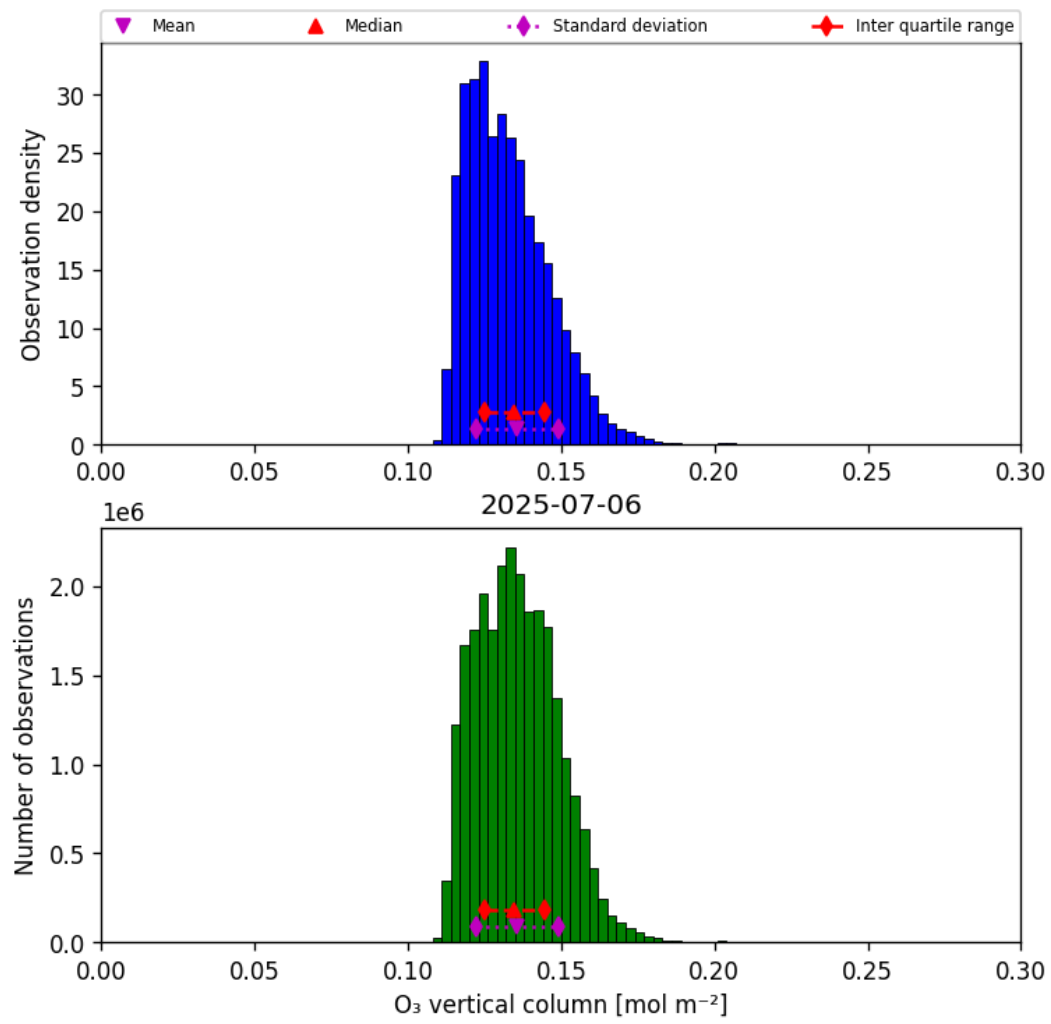
Figure 21: Histogram of “O 3 vertical column” for 2025-07-05 to 2025-07-07
