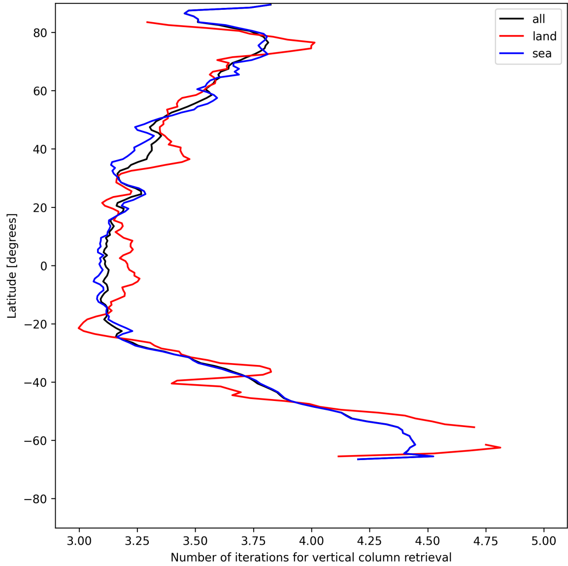
Figure 19: Zonal average of “Number of iterations for vertical column retrieval” for 2025-07-05 to 2025-07-07.
