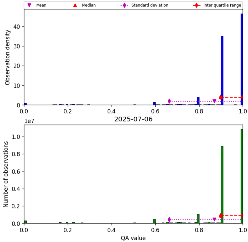
Figure 20: Histogram of “QA value” for 2025-07-05 to 2025-07-07
