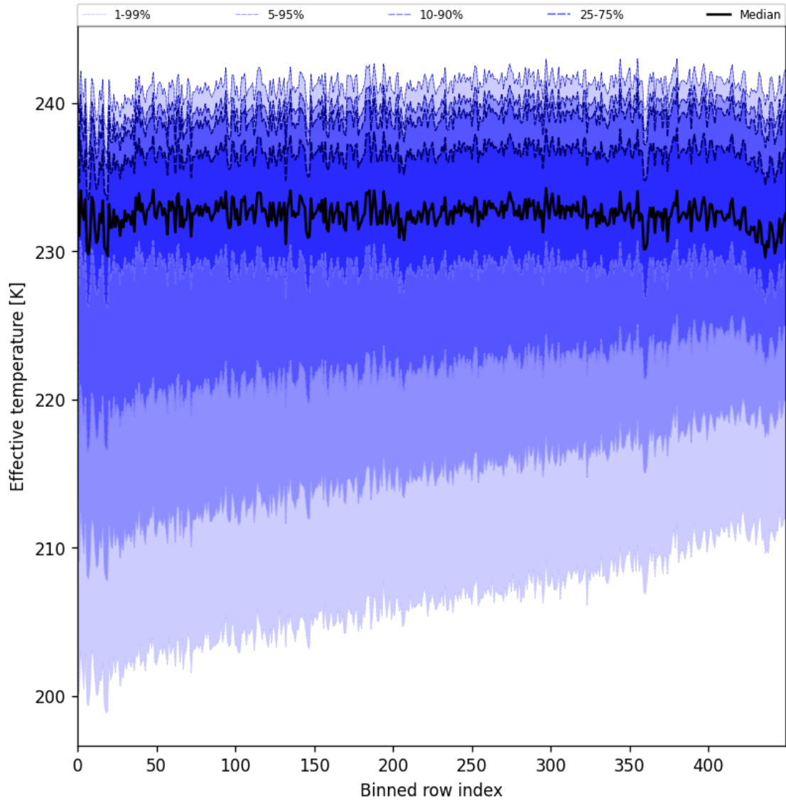
Figure 31: Along track statistics of “Effective temperature” for 2025-07-05 to 2025-07-07
