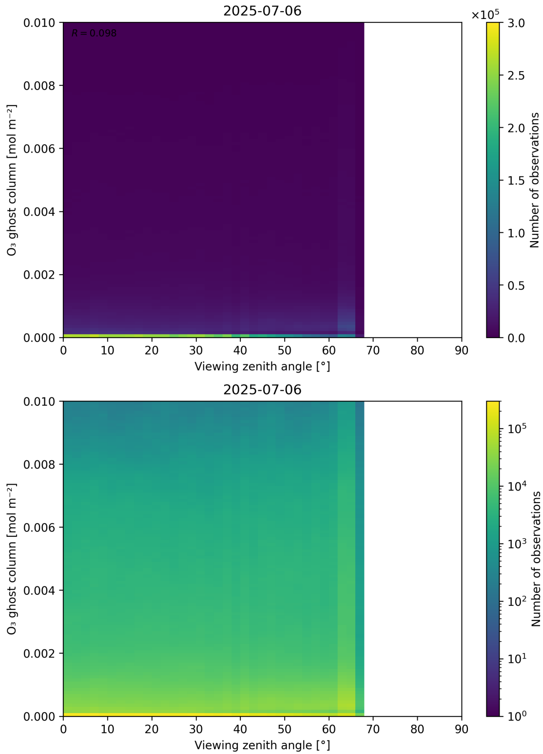
Figure 51: Scatter density plot of “Viewing zenith angle” against “O 3 ghost column” for 2025-07-05 to 2025-07-07.
