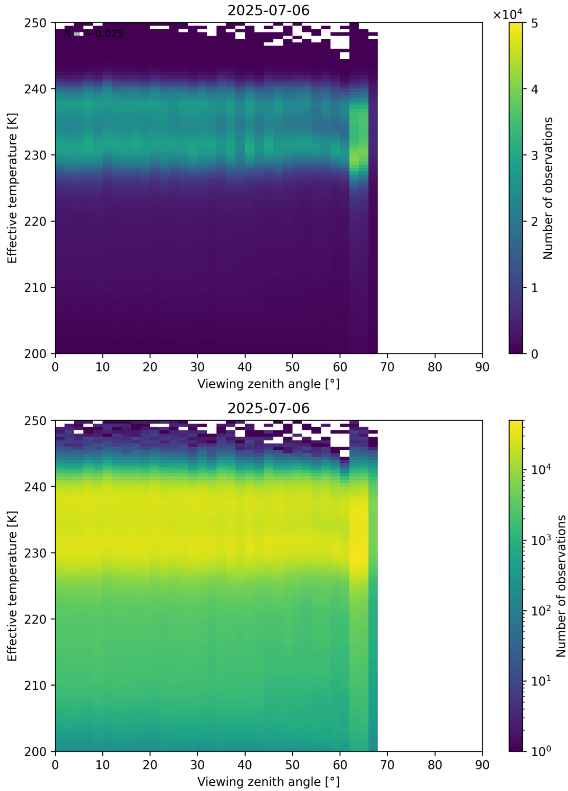
Figure 50: Scatter density plot of “Viewing zenith angle” against “Effective temperature” for 2025-07-05 to 2025-07-07.
