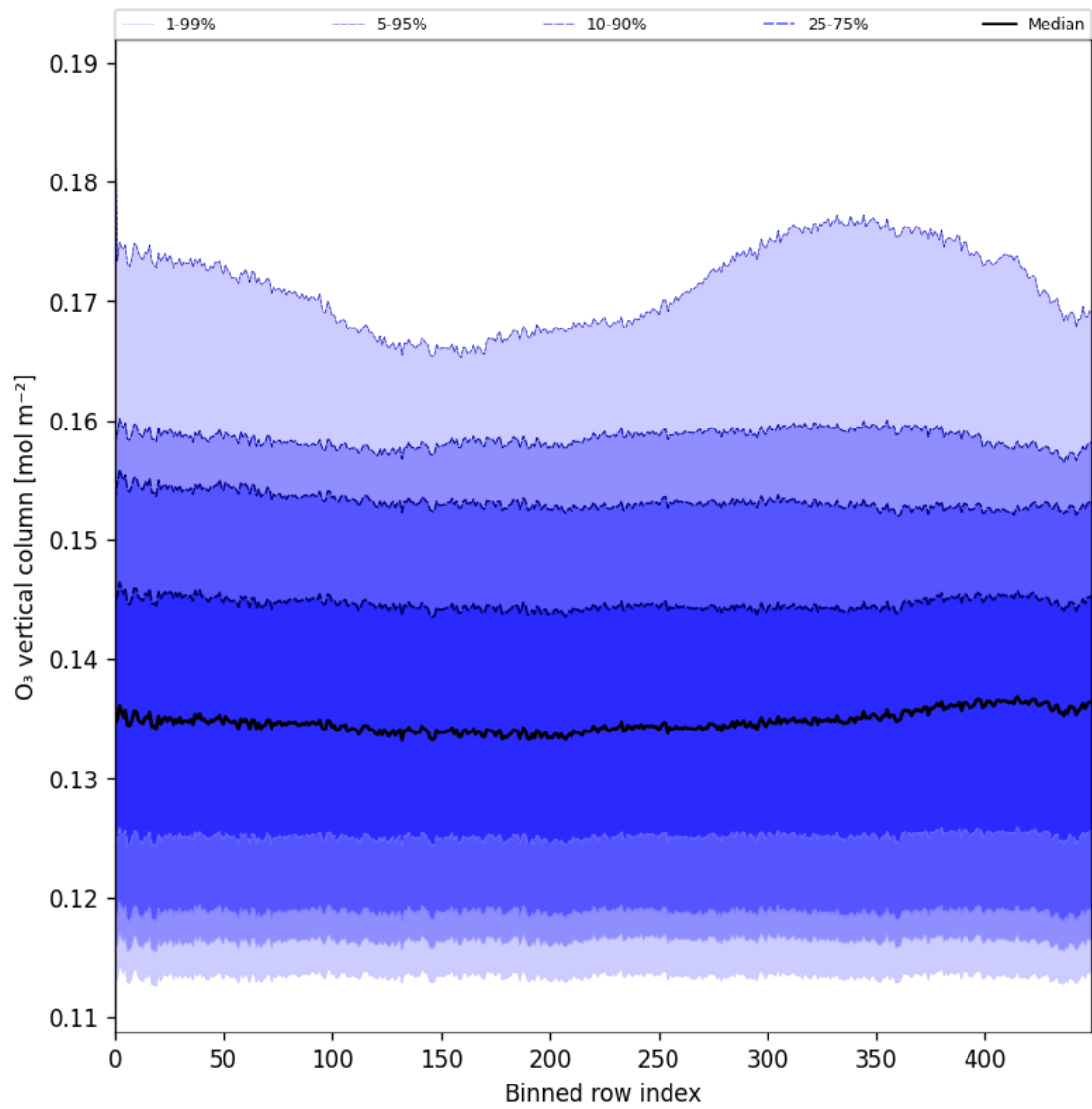
Figure 28: Along track statistics of “O 3 vertical column” for 2025-07-05 to 2025-07-07
