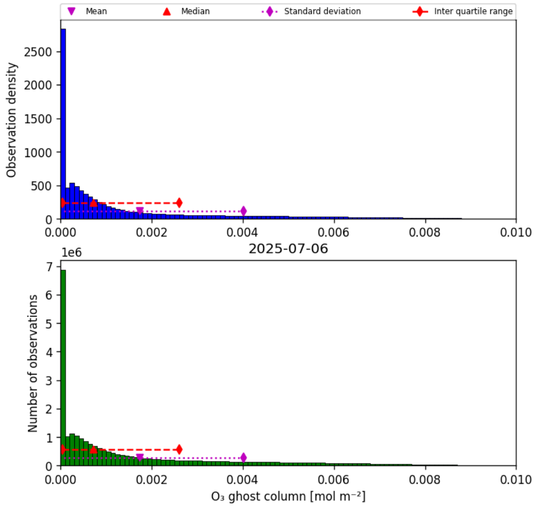
Figure 25: Histogram of “O 3 ghost column” for 2025-07-05 to 2025-07-07
