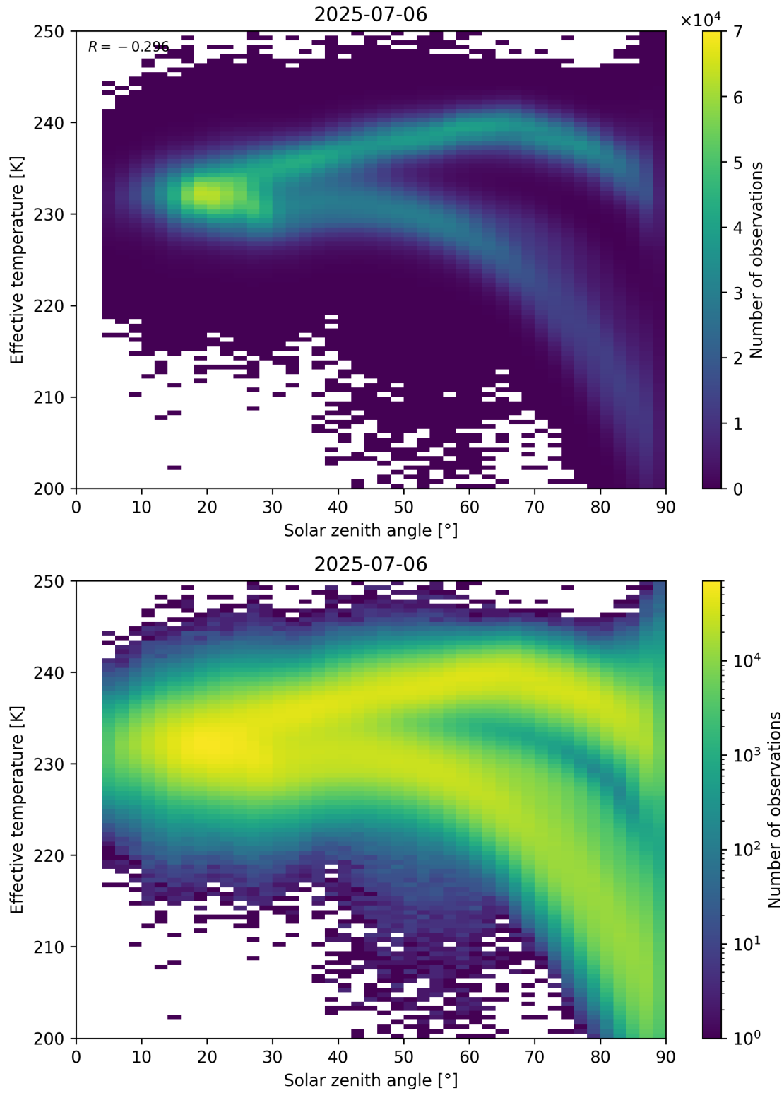
Figure 45: Scatter density plot of “Solar zenith angle” against “Effective temperature” for 2025-07-05 to 2025-07-07.
