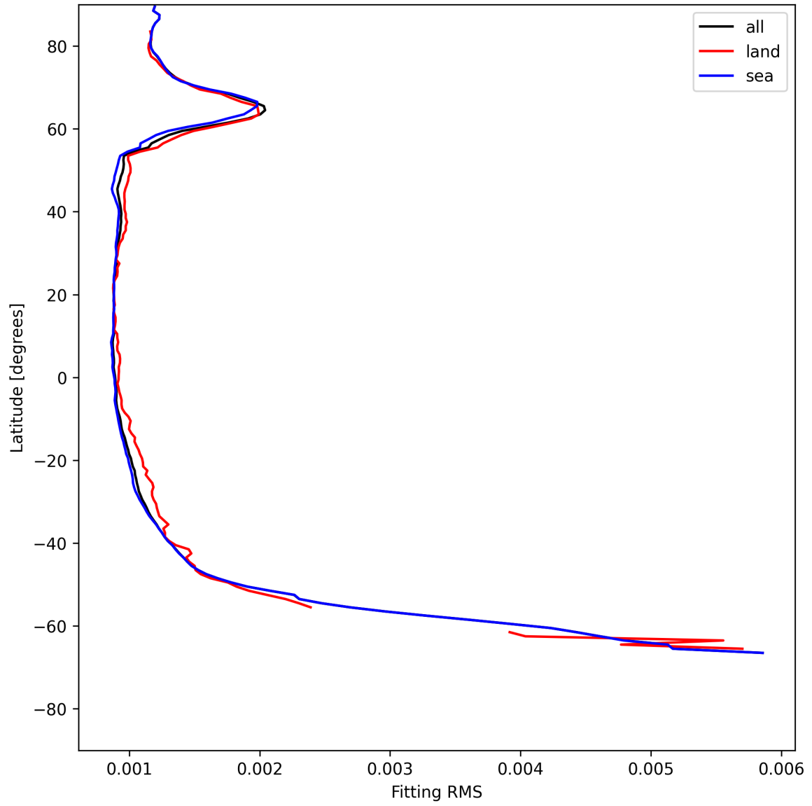
Figure 16: Zonal average of “Fitting RMS” for 2025-07-05 to 2025-07-07.
