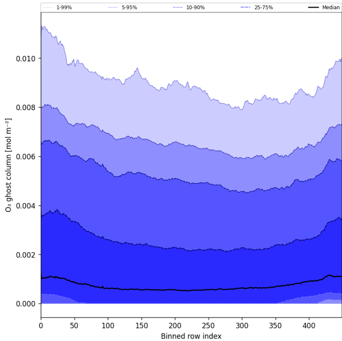
Figure 32: Along track statistics of “O 3 ghost column” for 2025-07-05 to 2025-07-07
