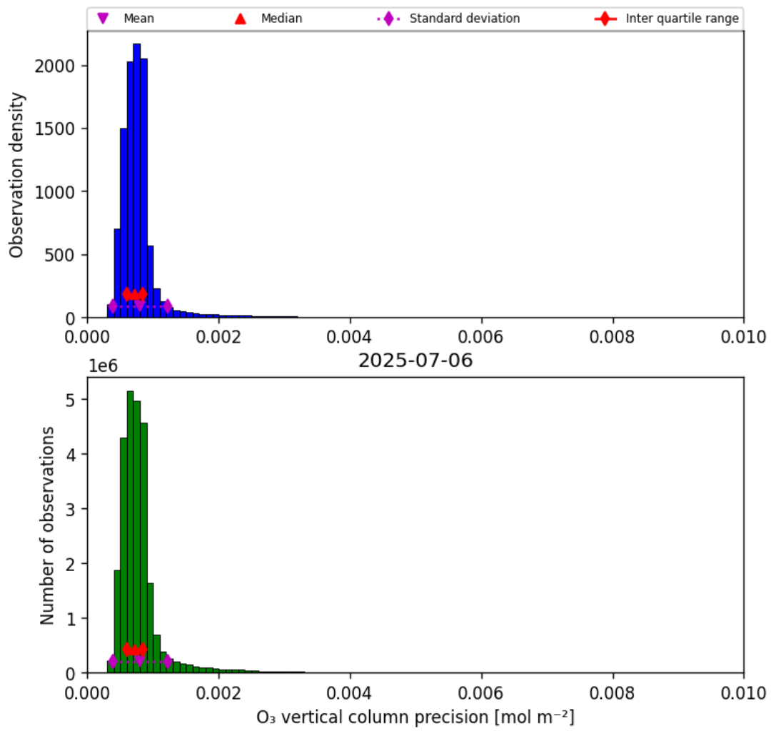
Figure 22: Histogram of “O 3 vertical column precision” for 2025-07-05 to 2025-07-07
