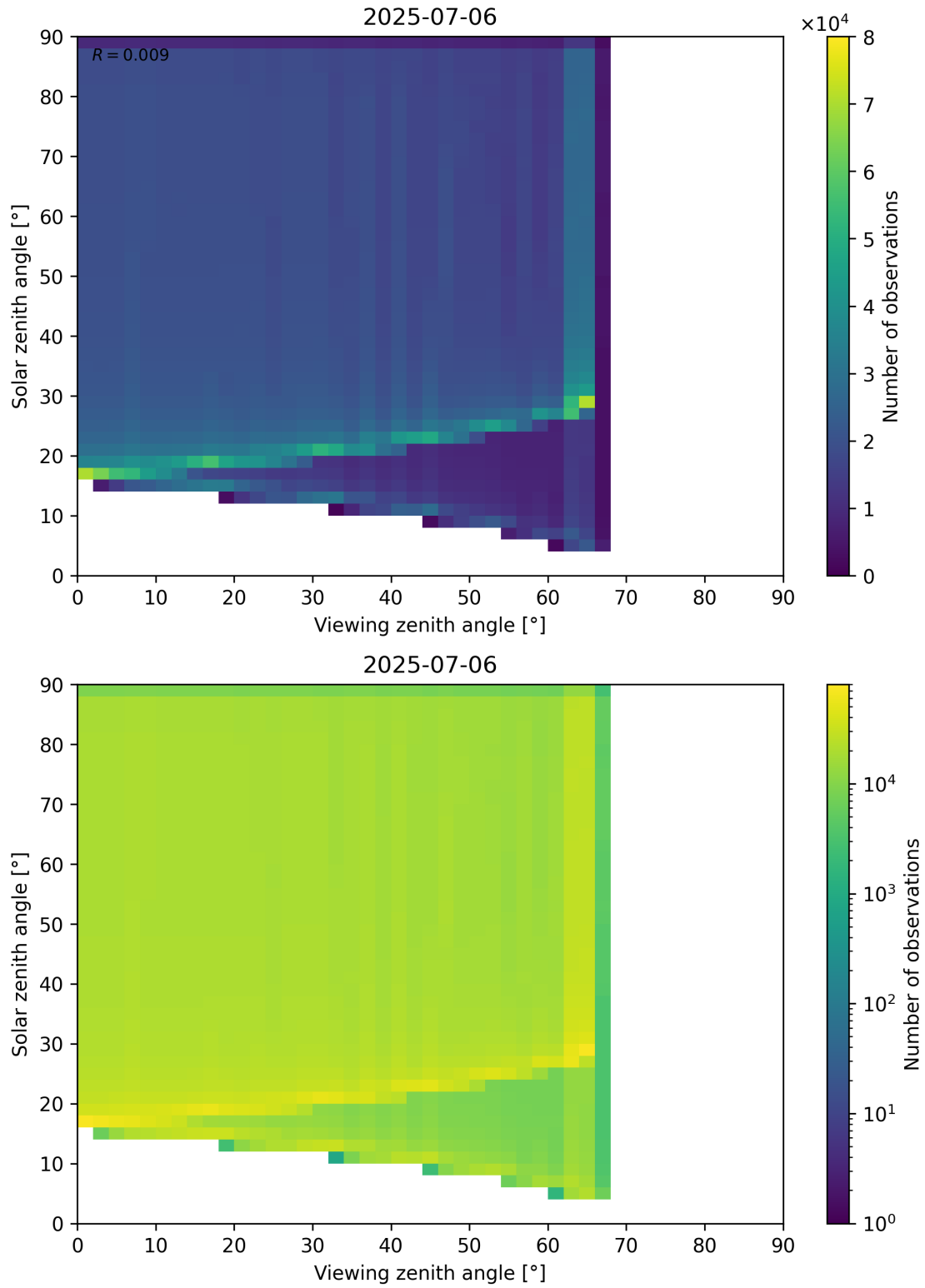
Figure 54: Scatter density plot of “Viewing zenith angle” against “Solar zenith angle” for 2025-07-05 to 2025-07-07.
