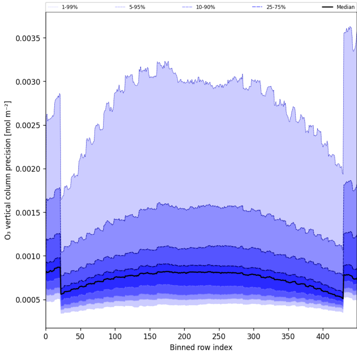
Figure 29: Along track statistics of “O 3 vertical column precision” for 2025-07-05 to 2025-07-07
