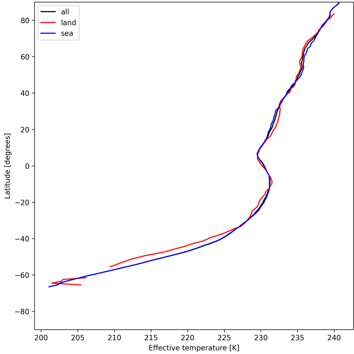
Figure 17: Zonal average of "Effective temperature" for 2025-07-05 to 2025-07-07.
