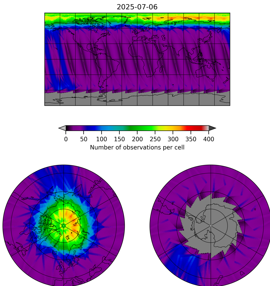
Figure 12: Map of the number of observations for 2025-07-05 to 2025-07-07
