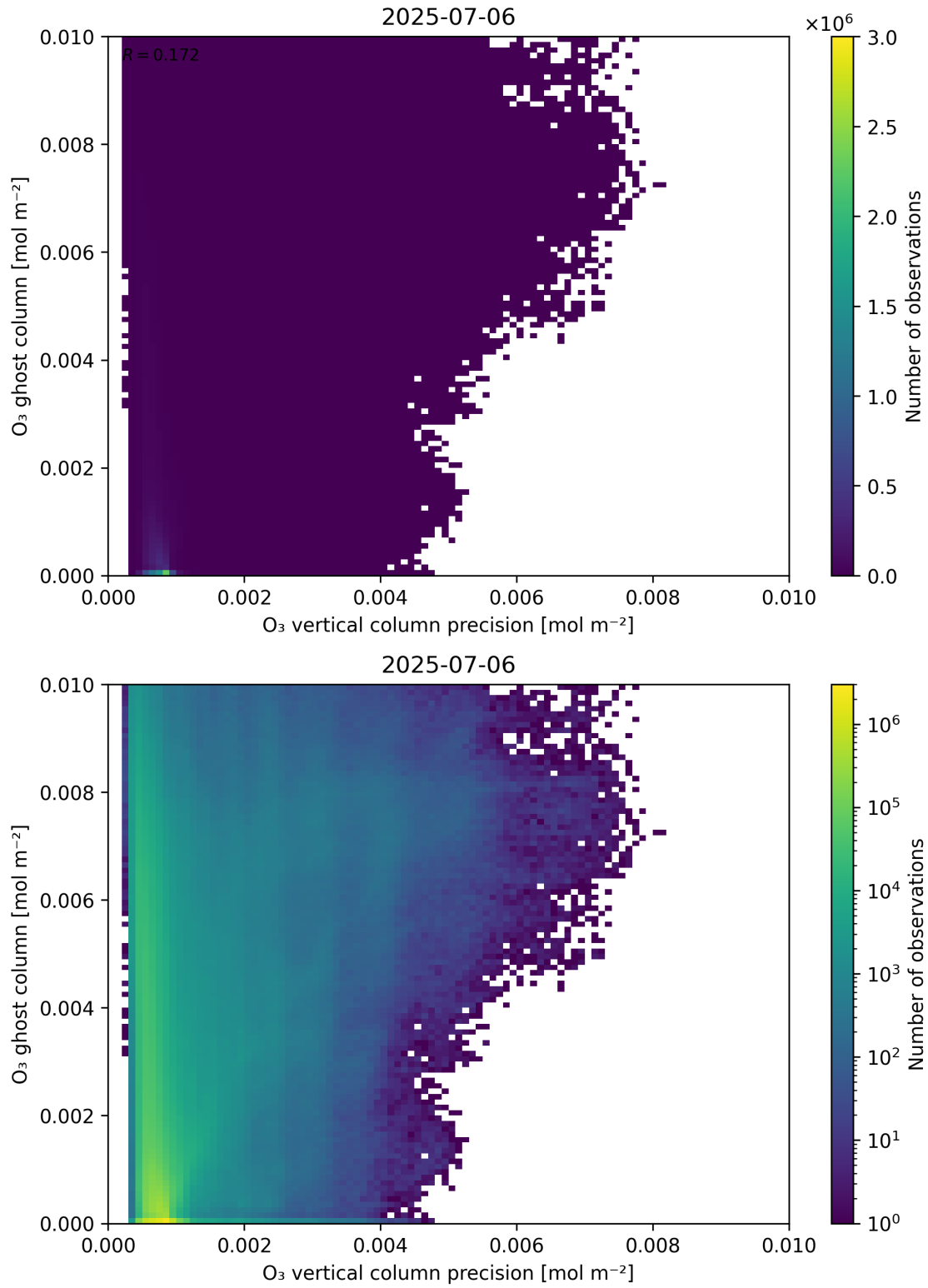
Figure 43: Scatter density plot of “O 3 vertical column precision” against “O 3 ghost column” for 2025-07-05 to 2025-07-07.
