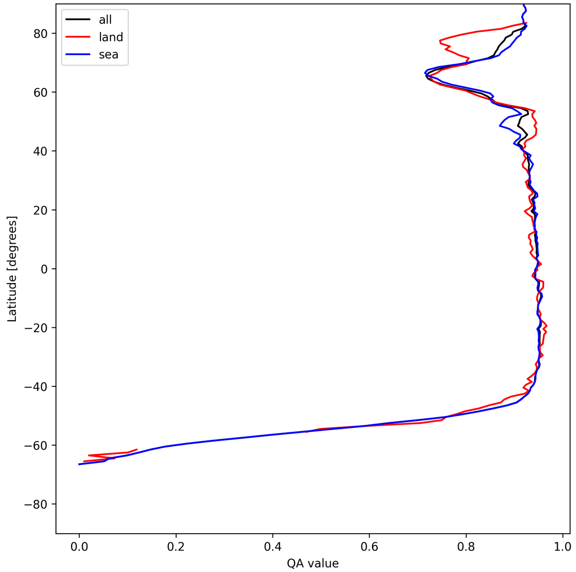
Figure 13: Zonal average of “QA value” for 2025-07-05 to 2025-07-07.
