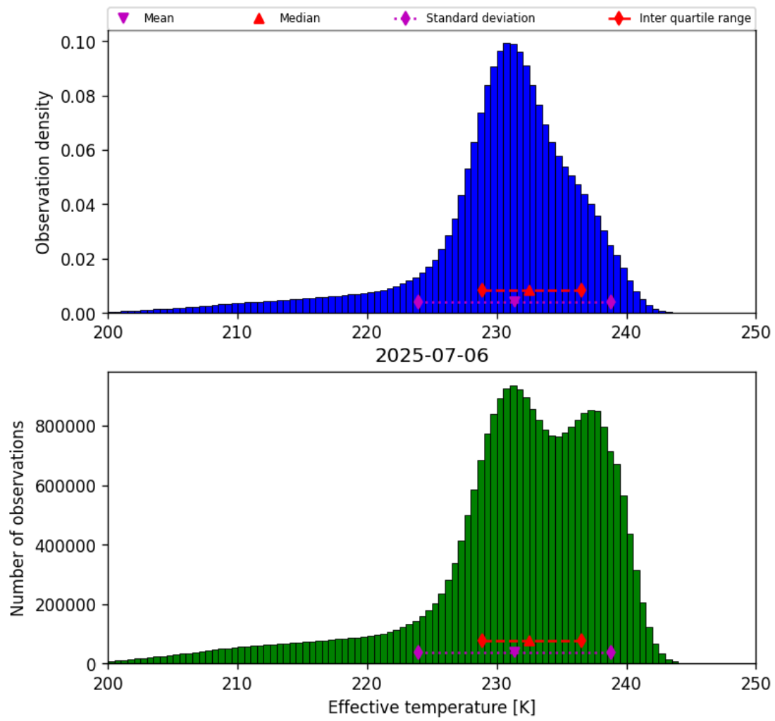
Figure 24: Histogram of “Effective temperature” for 2025-07-05 to 2025-07-07
