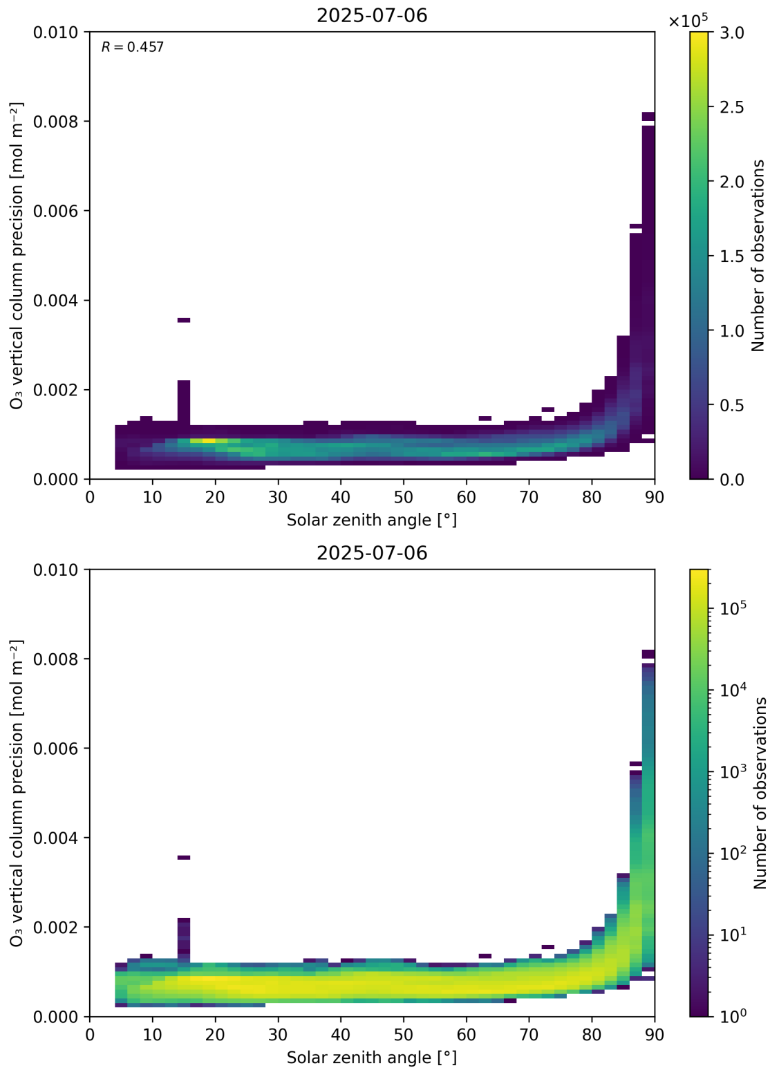
Figure 48: Scatter density plot of “Solar zenith angle” against “O 3 vertical column precision” for 2025-07-05 to 2025-07-07.
