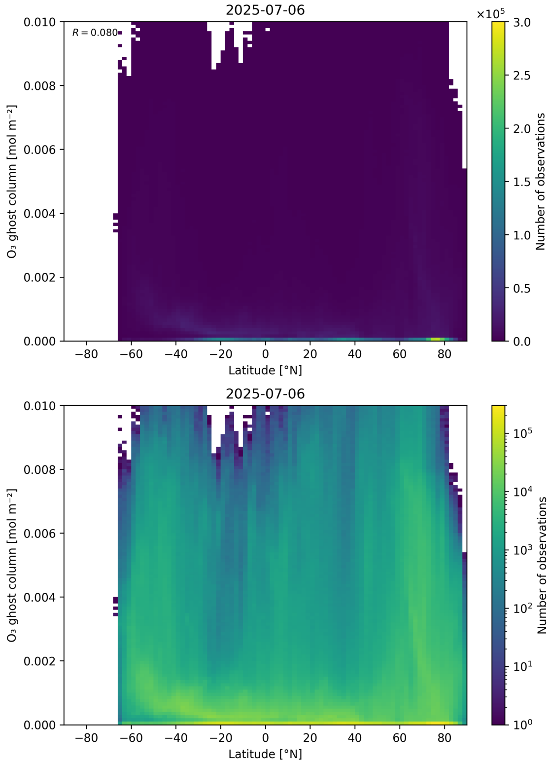
Figure 35: Scatter density plot of “Latitude” against “O 3 ghost column” for 2025-07-05 to 2025-07-07.
