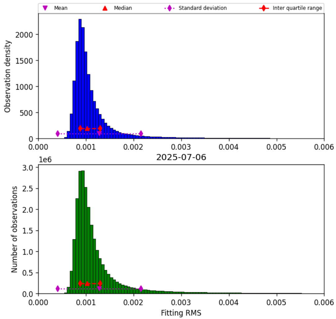
Figure 23: Histogram of “Fitting RMS” for 2025-07-05 to 2025-07-07
