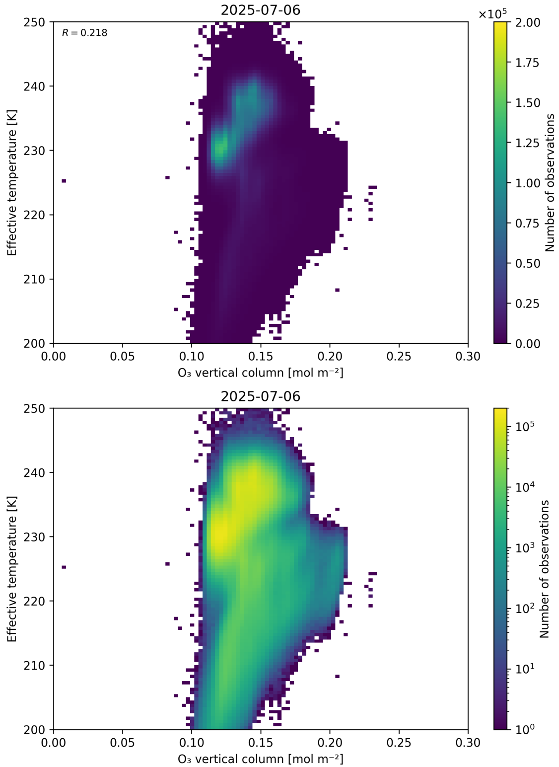
Figure 39: Scatter density plot of “O 3 vertical column” against “Effective temperature” for 2025-07-05 to 2025-07-07.
