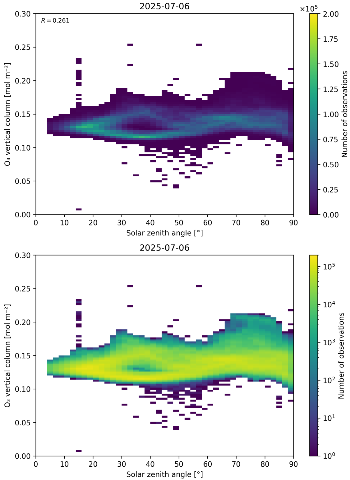
Figure 47: Scatter density plot of “Solar zenith angle” against “O 3 vertical column” for 2025-07-05 to 2025-07-07.
