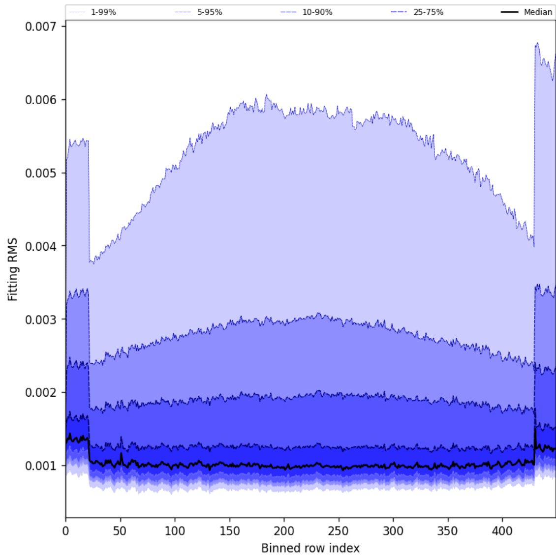
Figure 30: Along track statistics of “Fitting RMS” for 2025-07-05 to 2025-07-07
