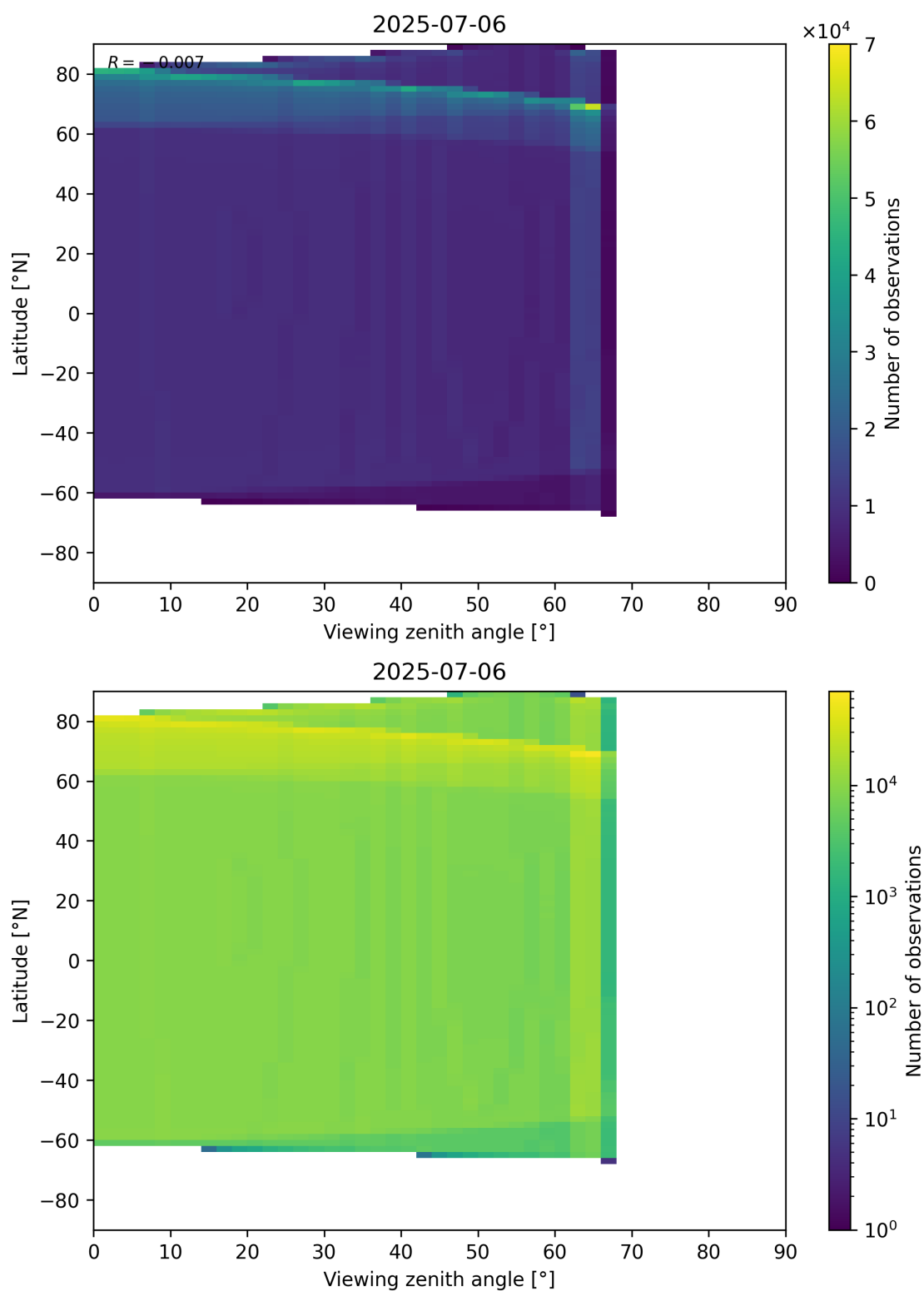
Figure 49: Scatter density plot of “Viewing zenith angle” against “Latitude” for 2025-07-05 to 2025-07-07.
