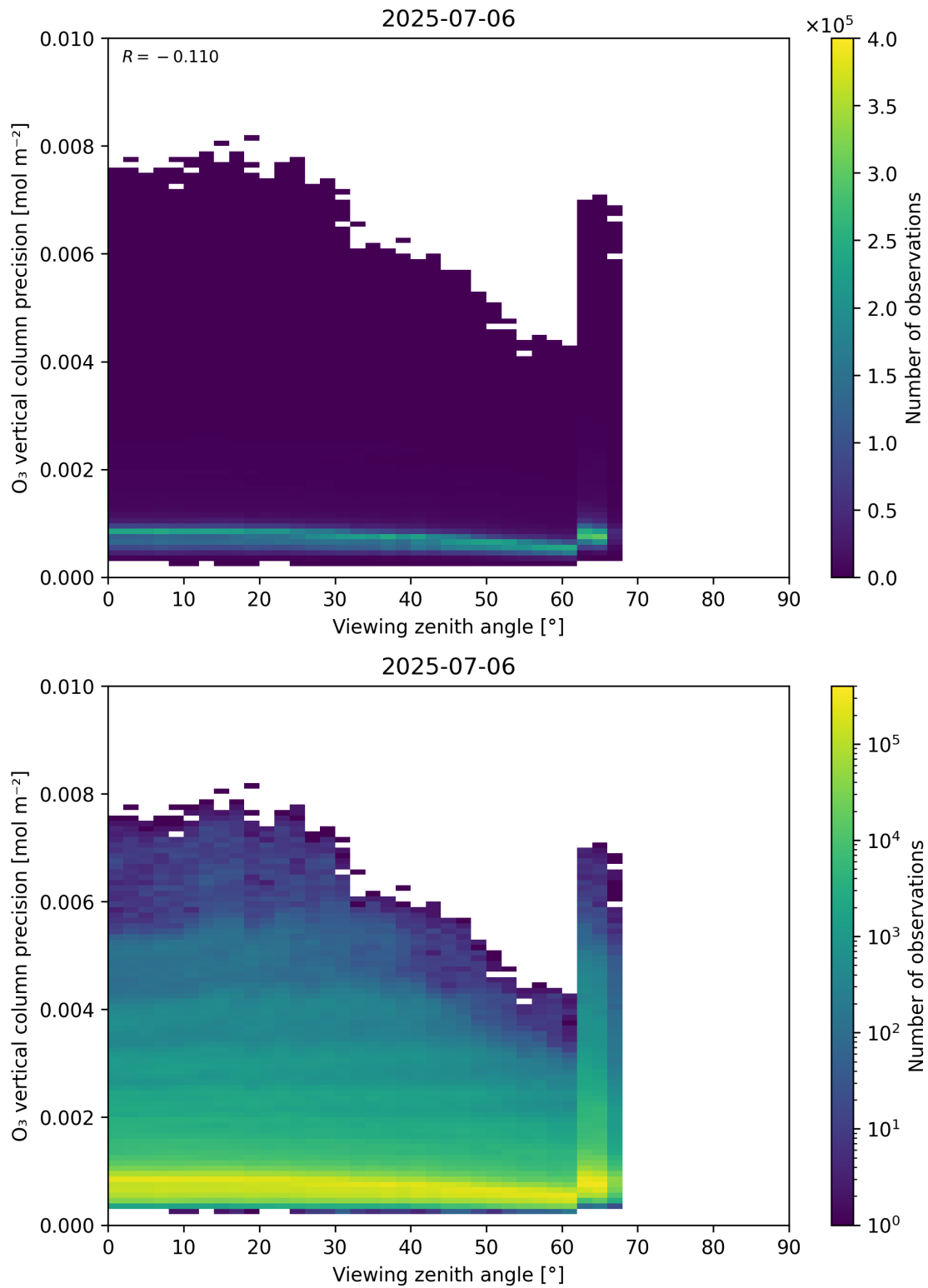
Figure 53: Scatter density plot of “Viewing zenith angle” against “O 3 vertical column precision” for 2025-07-05 to 2025-07-07.
