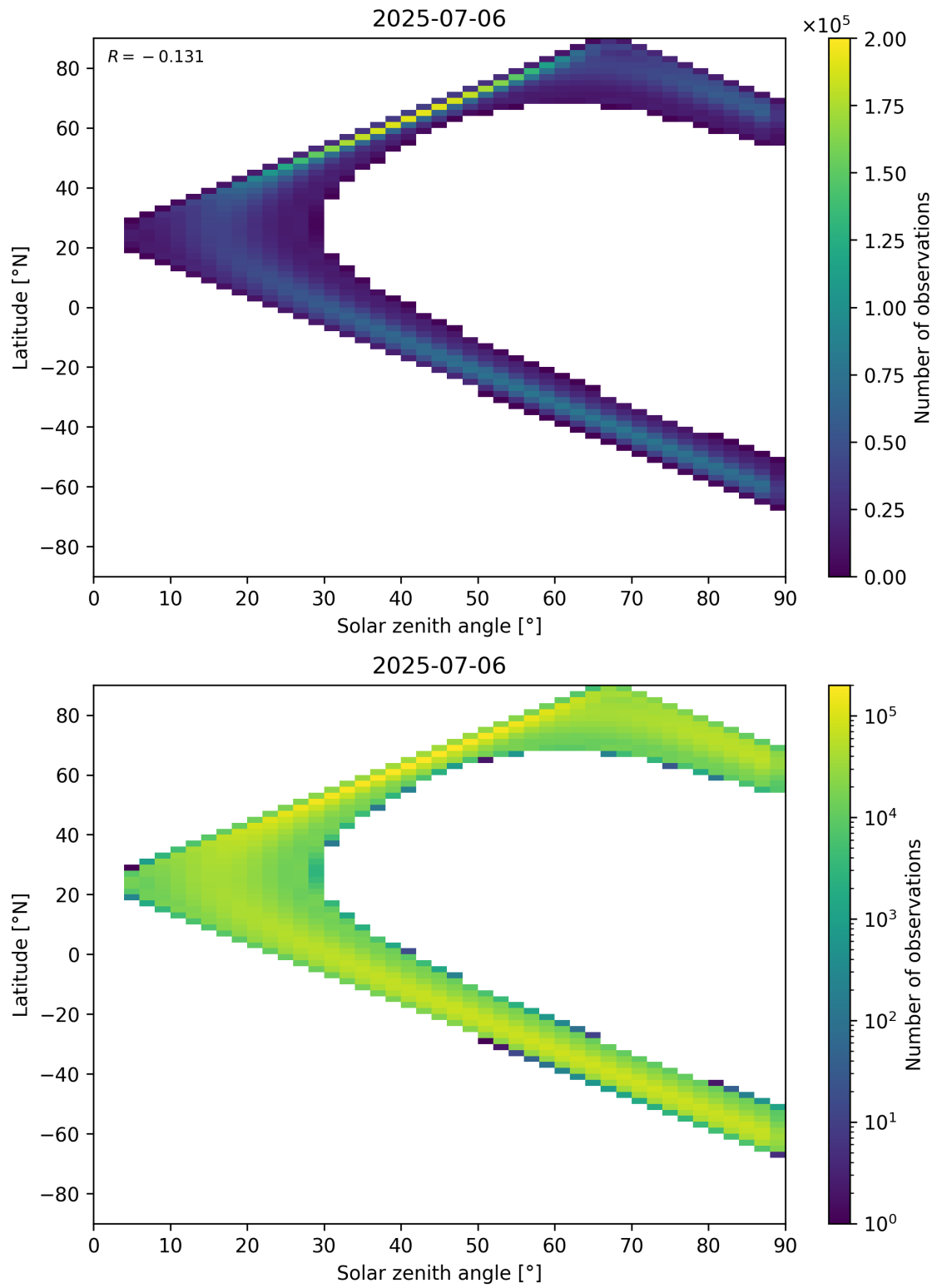
Figure 44: Scatter density plot of “Solar zenith angle” against “Latitude” for 2025-07-05 to 2025-07-07.
