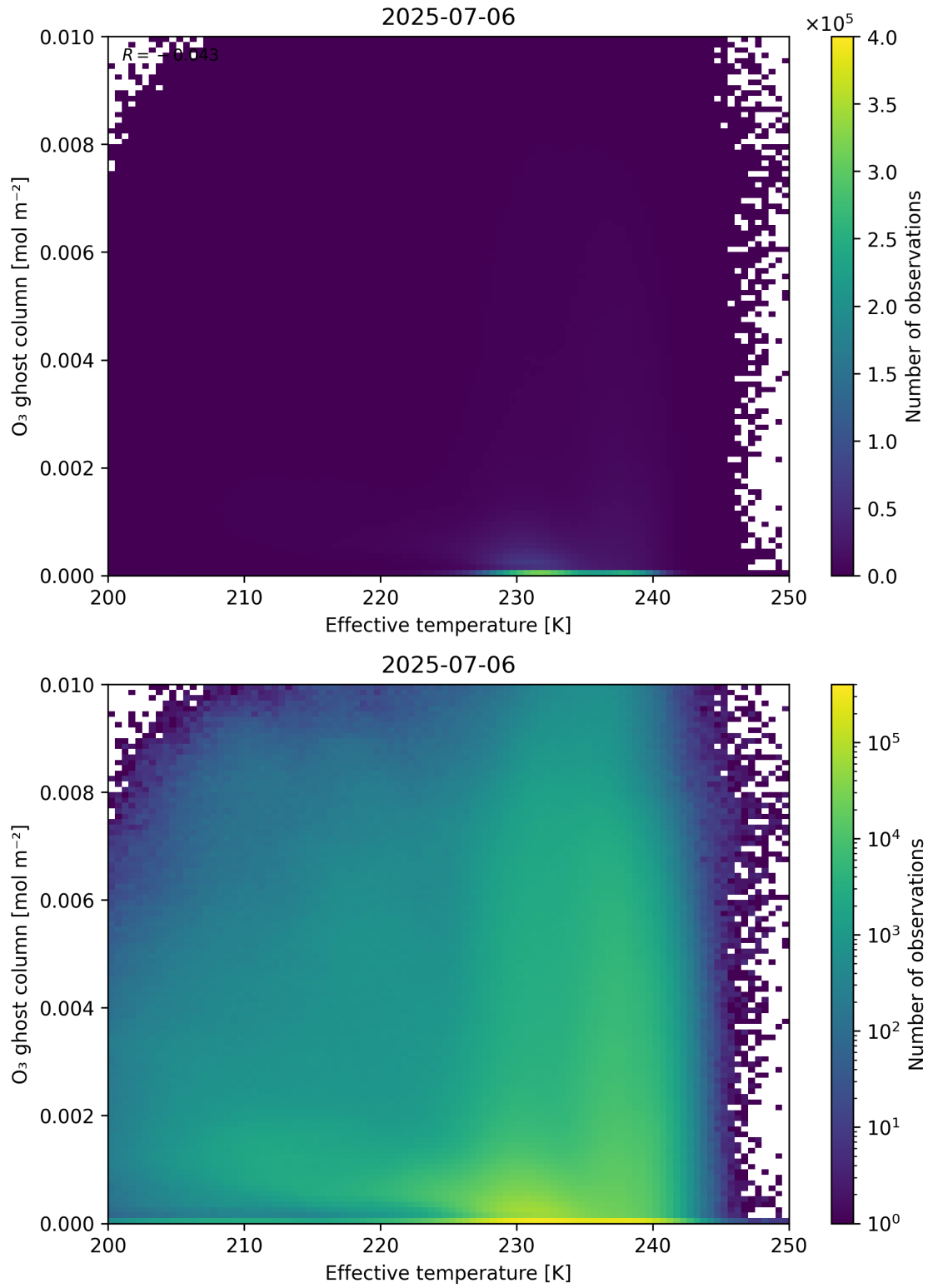
Figure 38: Scatter density plot of “Effective temperature” against “O 3 ghost column” for 2025-07-05 to 2025-07-07.
