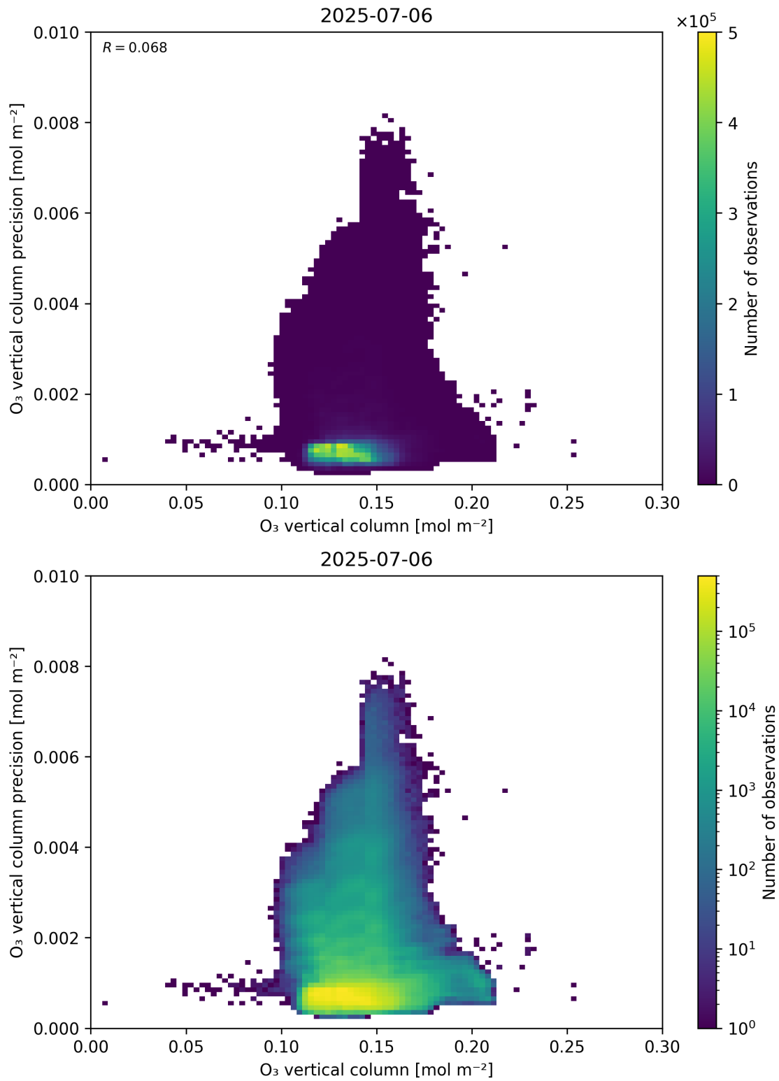
Figure 41: Scatter density plot of “O 3 vertical column” against “O 3 vertical column precision” for 2025-07-05 to 2025-07-07.
