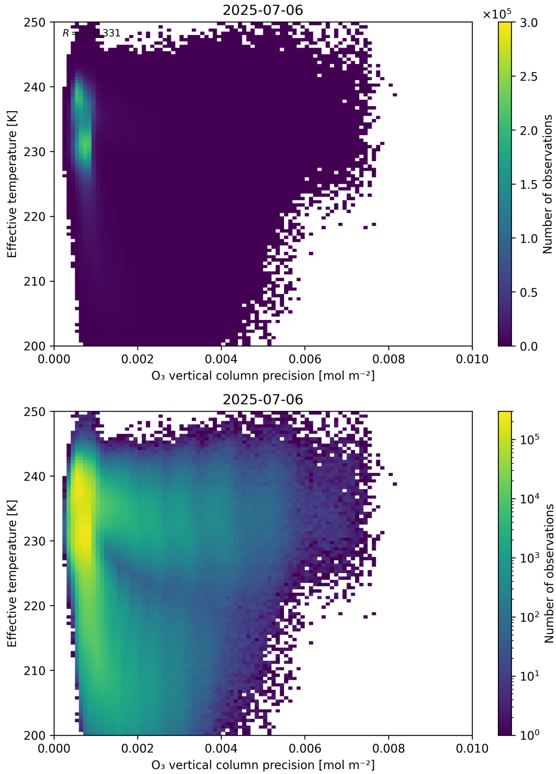
Figure 42: Scatter density plot of “O 3 vertical column precision” against “Effective temperature” for 2025-07-05 to 2025-07-07.
