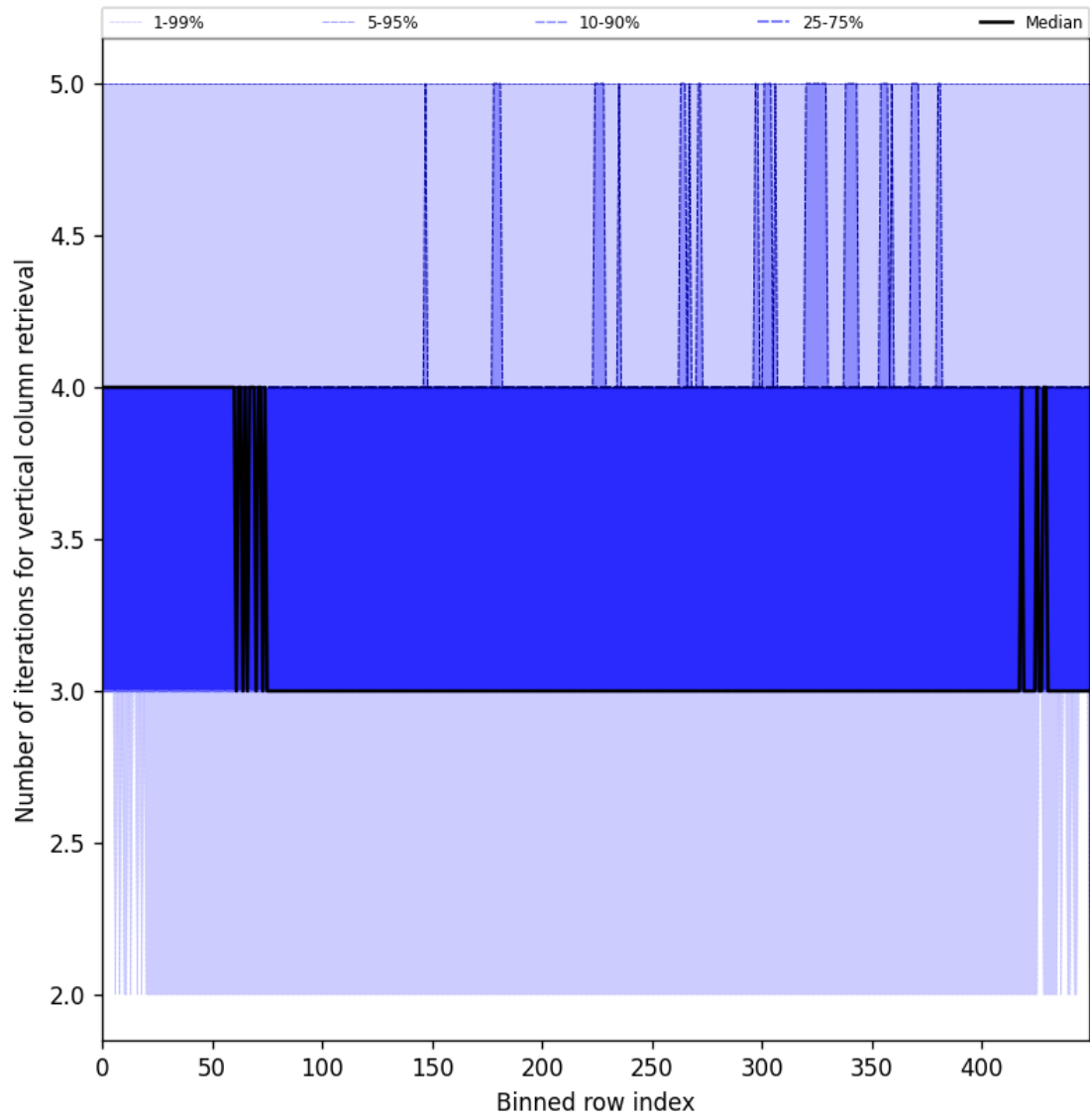
Figure 33: Along track statistics of “Number of iterations for vertical column retrieval” for 2025-07-05 to 2025-07-07
