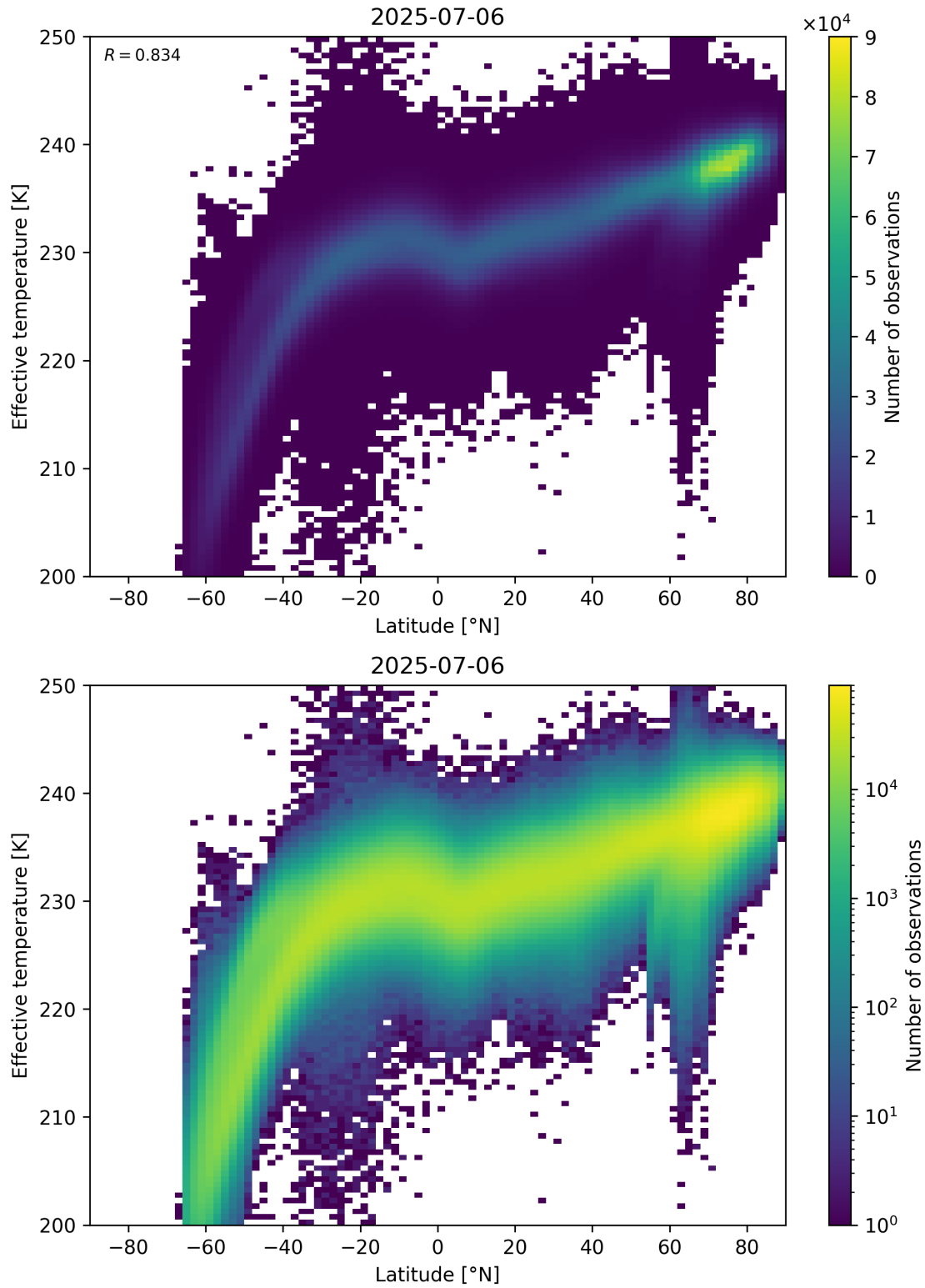
Figure 34: Scatter density plot of “Latitude” against “Effective temperature” for 2025-07-05 to 2025-07-07.
