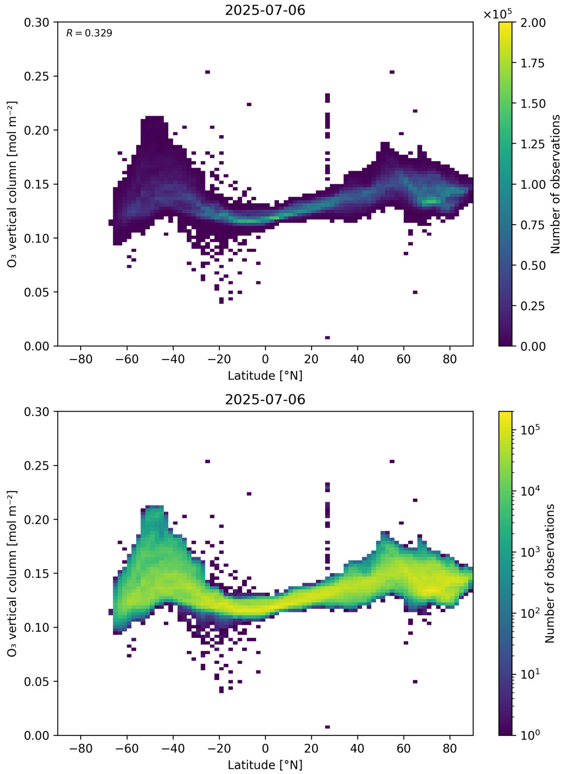
Figure 36: Scatter density plot of “Latitude” against “O 3 vertical column” for 2025-07-05 to 2025-07-07.
