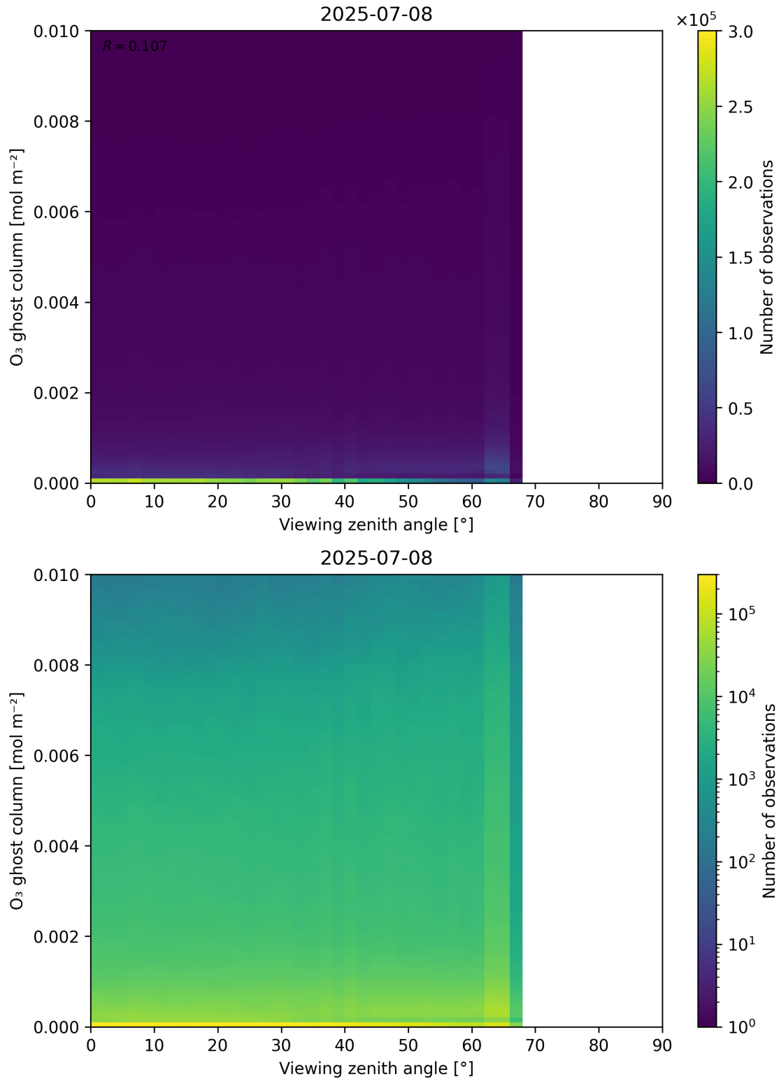
Figure 51: Scatter density plot of “Viewing zenith angle” against “O 3 ghost column” for 2025-07-08 to 2025-07-09.
