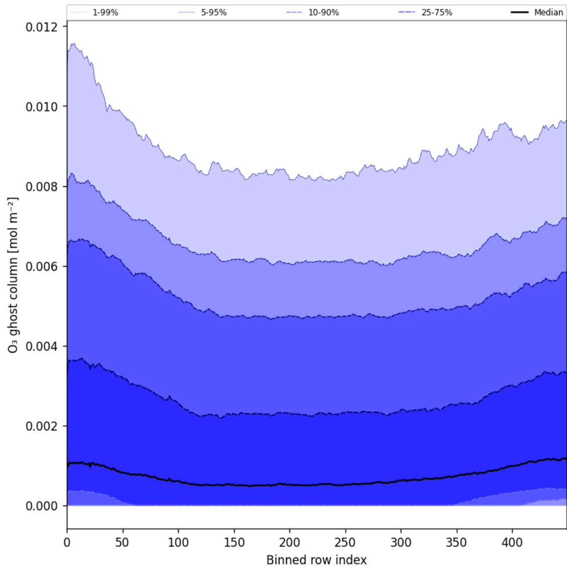
Figure 32: Along track statistics of “O 3 ghost column” for 2025-07-08 to 2025-07-09
