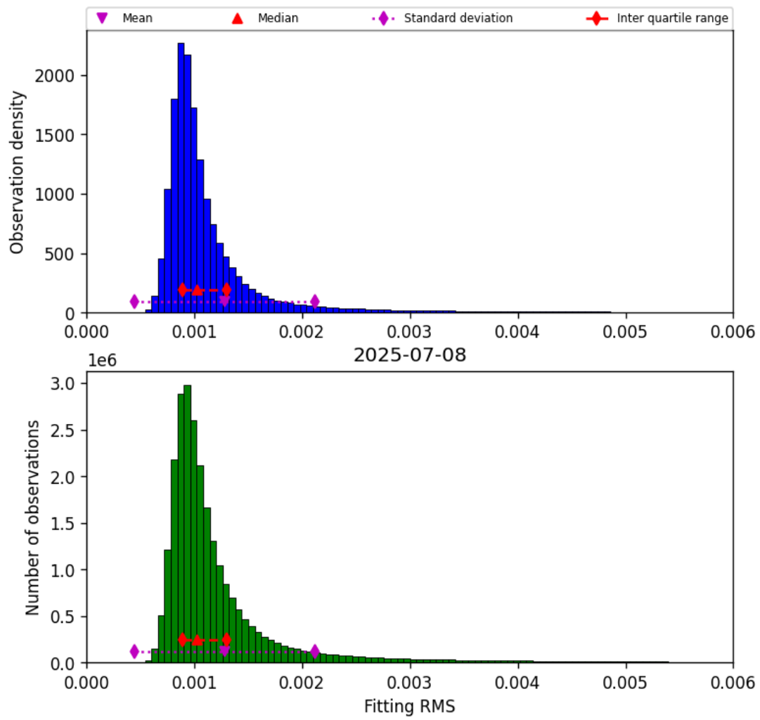
Figure 23: Histogram of “Fitting RMS” for 2025-07-08 to 2025-07-09
