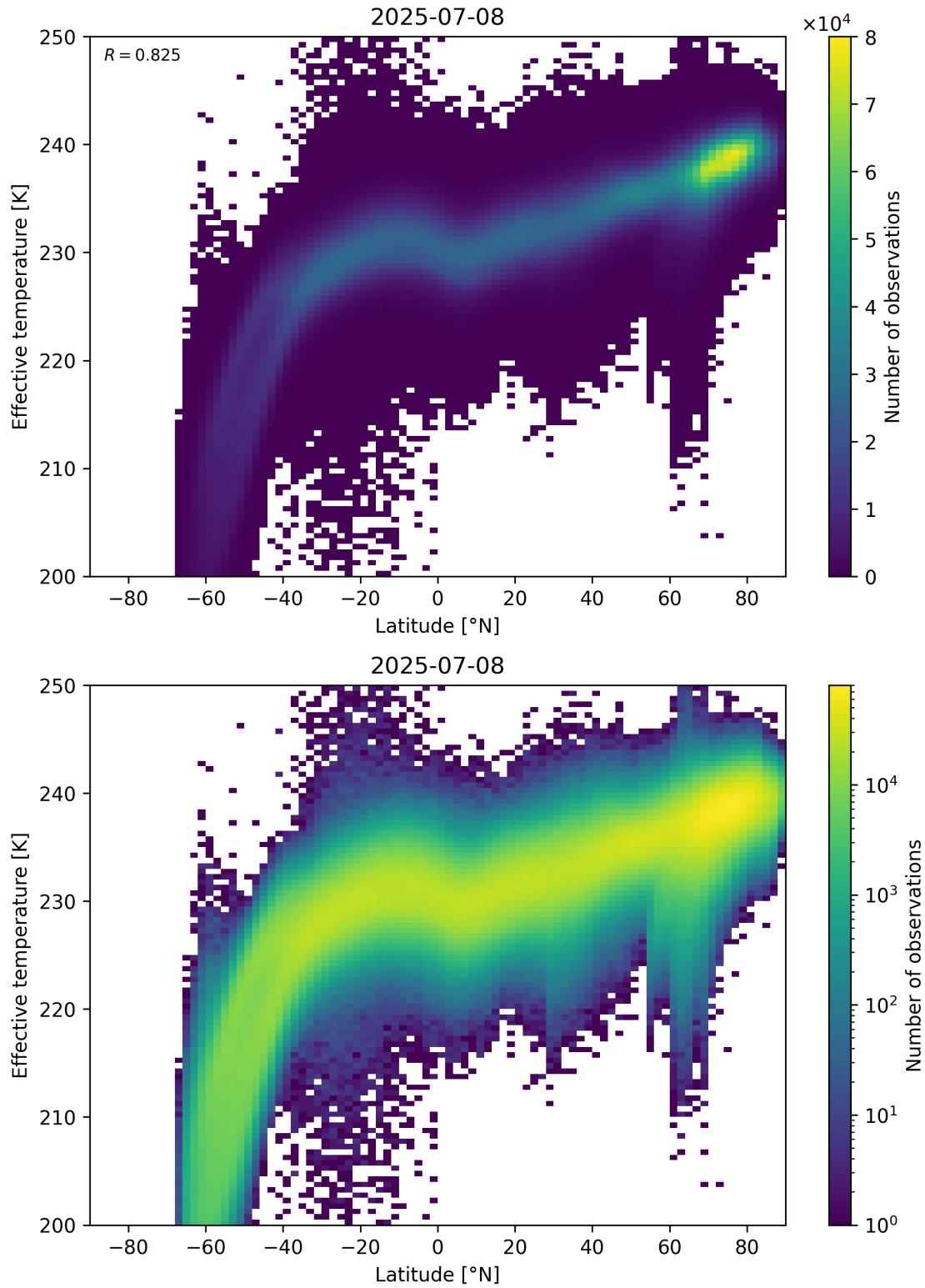
Figure 34: Scatter density plot of “Latitude” against “Effective temperature” for 2025-07-08 to 2025-07-09.
