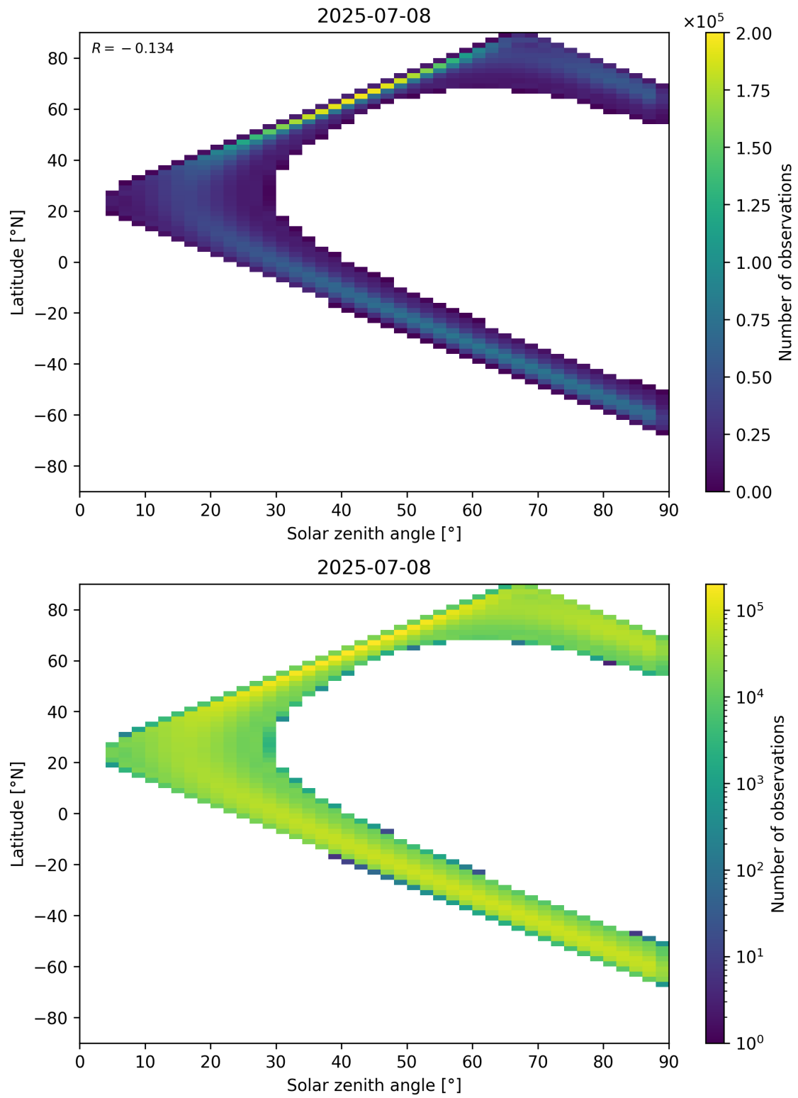
Figure 44: Scatter density plot of “Solar zenith angle” against “Latitude” for 2025-07-08 to 2025-07-09.
