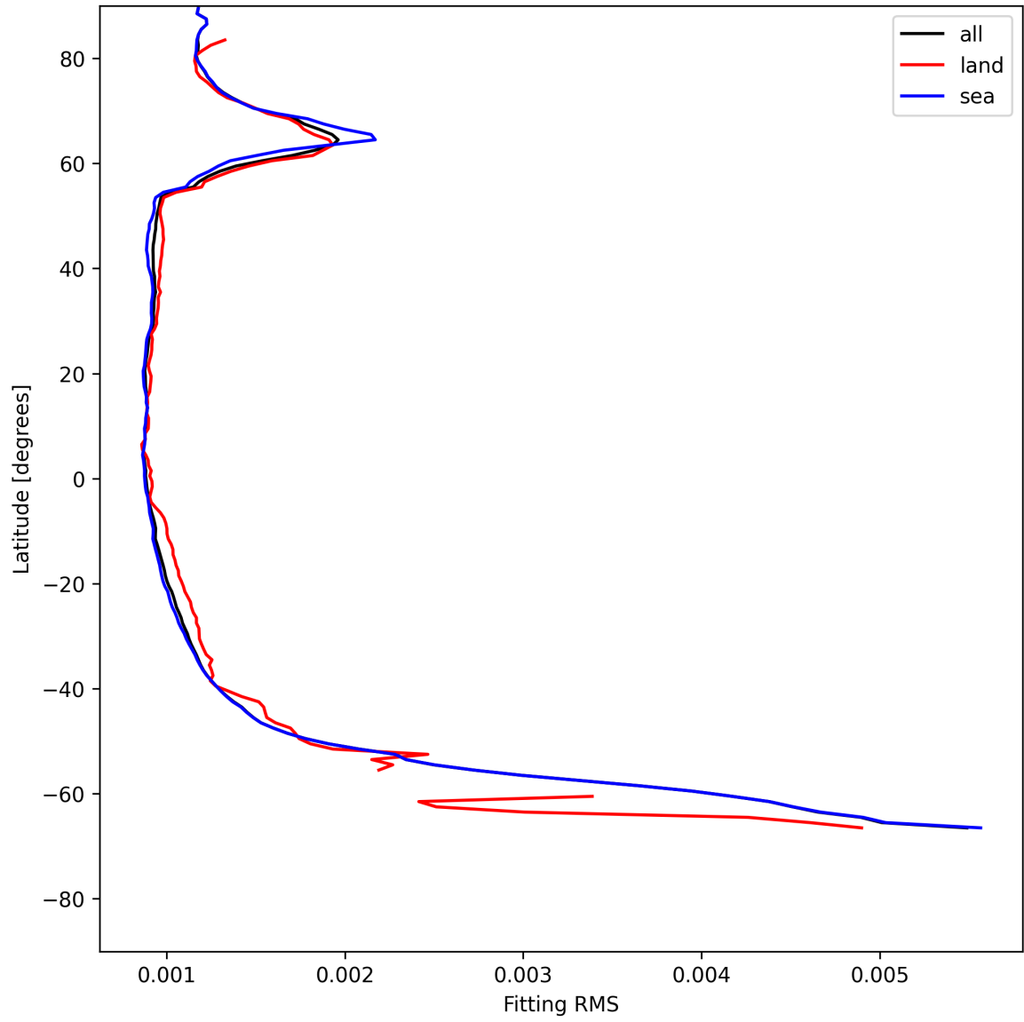
Figure 16: Zonal average of "Fitting RMS" for 2025-07-08 to 2025-07-09.
