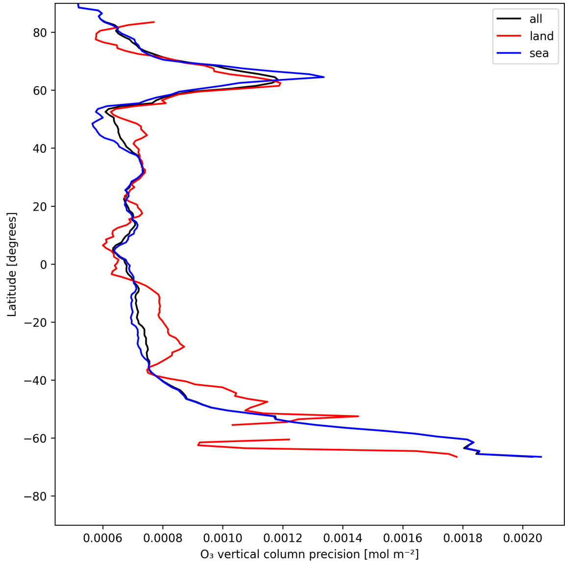
Figure 15: Zonal average of “O 3 vertical column precision” for 2025-07-08 to 2025-07-09.
