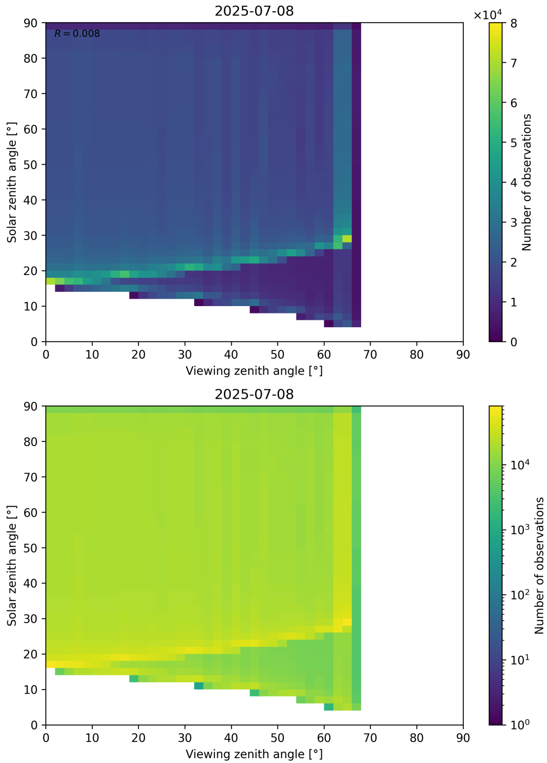
Figure 54: Scatter density plot of “Viewing zenith angle” against “Solar zenith angle” for 2025-07-08 to 2025-07-09.
