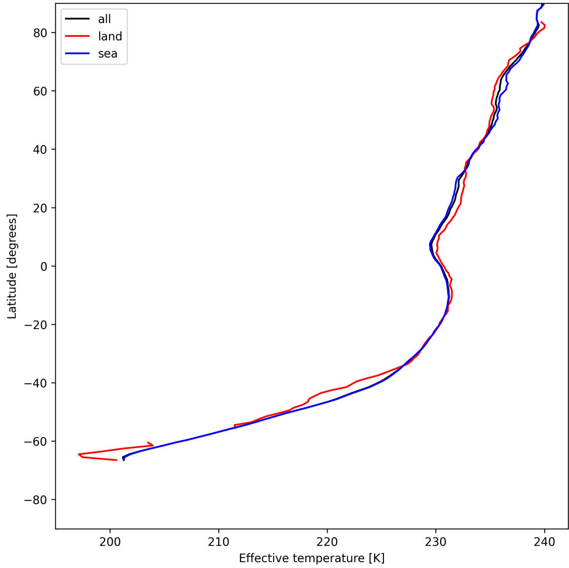
Figure 17: Zonal average of "Effective temperature" for 2025-07-08 to 2025-07-09.
