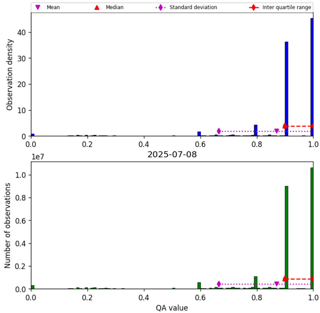
Figure 20: Histogram of “QA value” for 2025-07-08 to 2025-07-09
