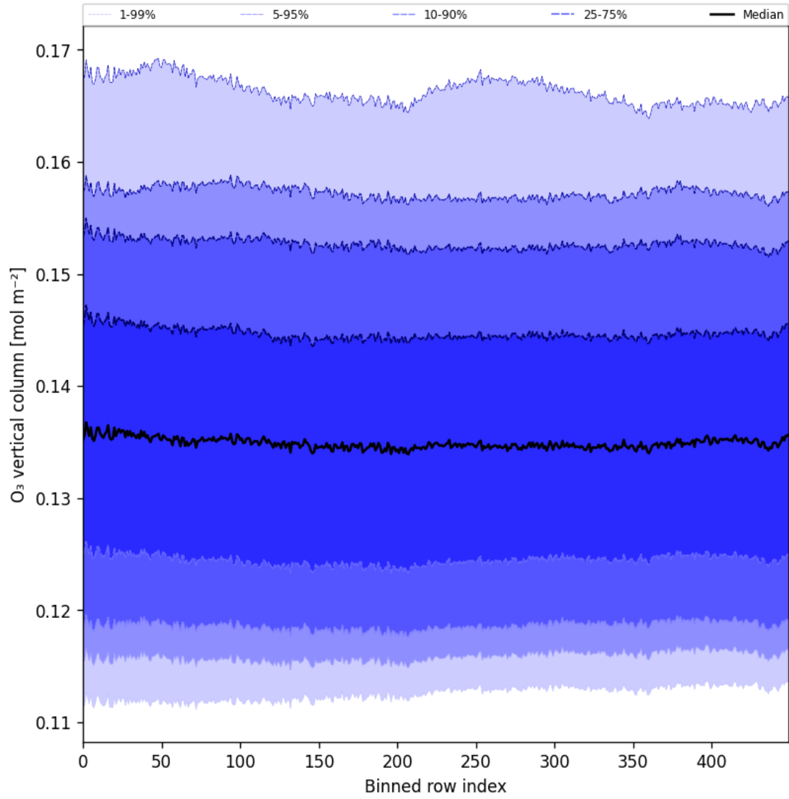
Figure 28: Along track statistics of “O 3 vertical column” for 2025-07-08 to 2025-07-09
