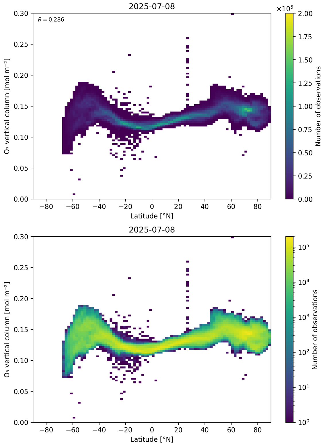
Figure 36: Scatter density plot of “Latitude” against “O 3 vertical column” for 2025-07-08 to 2025-07-09.
