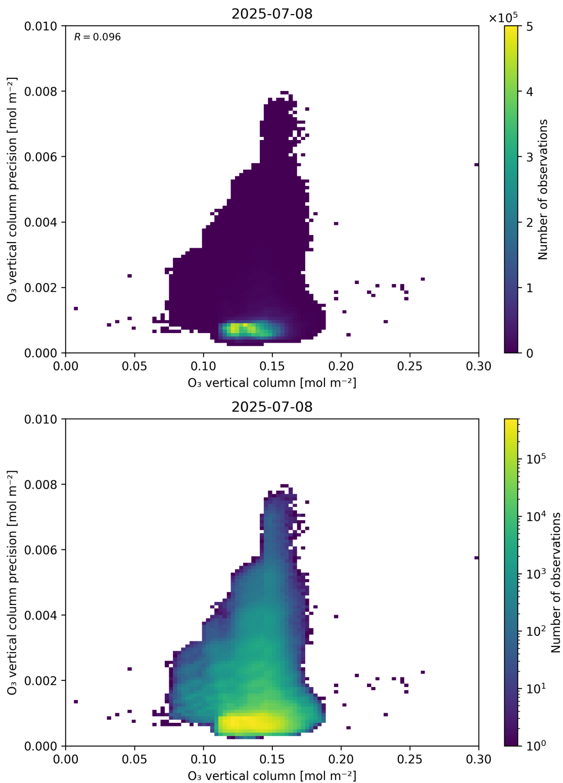
Figure 41: Scatter density plot of “O 3 vertical column” against “O 3 vertical column precision” for 2025-07-08 to 2025-07-09.
