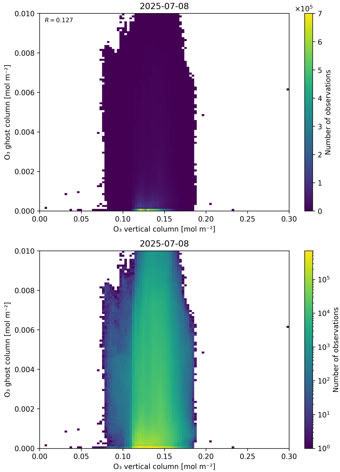
Figure 40: Scatter density plot of “O 3 vertical column” against “O 3 ghost column” for 2025-07-08 to 2025-07-09.
