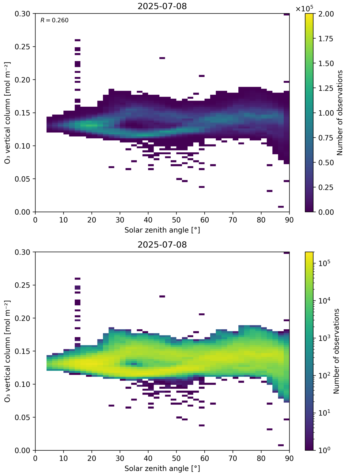
Figure 47: Scatter density plot of “Solar zenith angle” against “O 3 vertical column” for 2025-07-08 to 2025-07-09.
