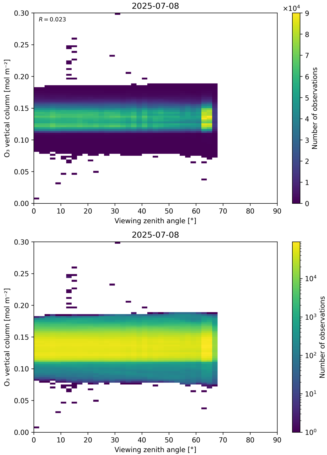
Figure 52: Scatter density plot of “Viewing zenith angle” against “O 3 vertical column” for 2025-07-08 to 2025-07-09.
