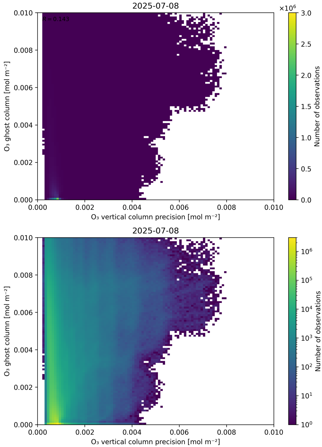
Figure 43: Scatter density plot of “O 3 vertical column precision” against “O 3 ghost column” for 2025-07-08 to 2025-07-09.
