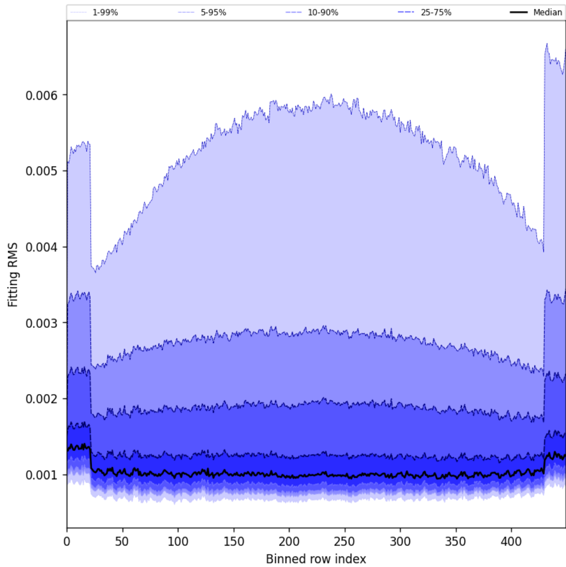
Figure 30: Along track statistics of “Fitting RMS” for 2025-07-08 to 2025-07-09
