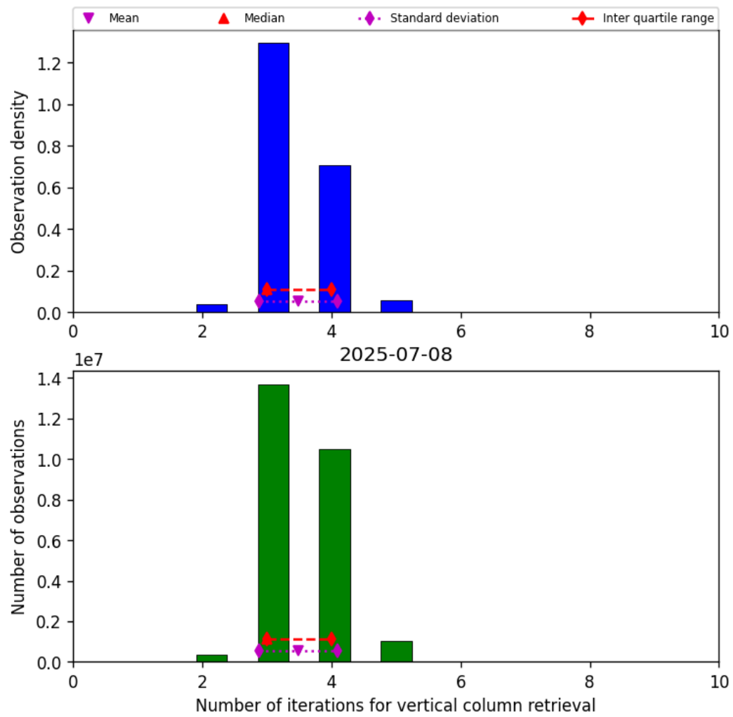
Figure 26: Histogram of “Number of iterations for vertical column retrieval” for 2025-07-08 to 2025-07-09
