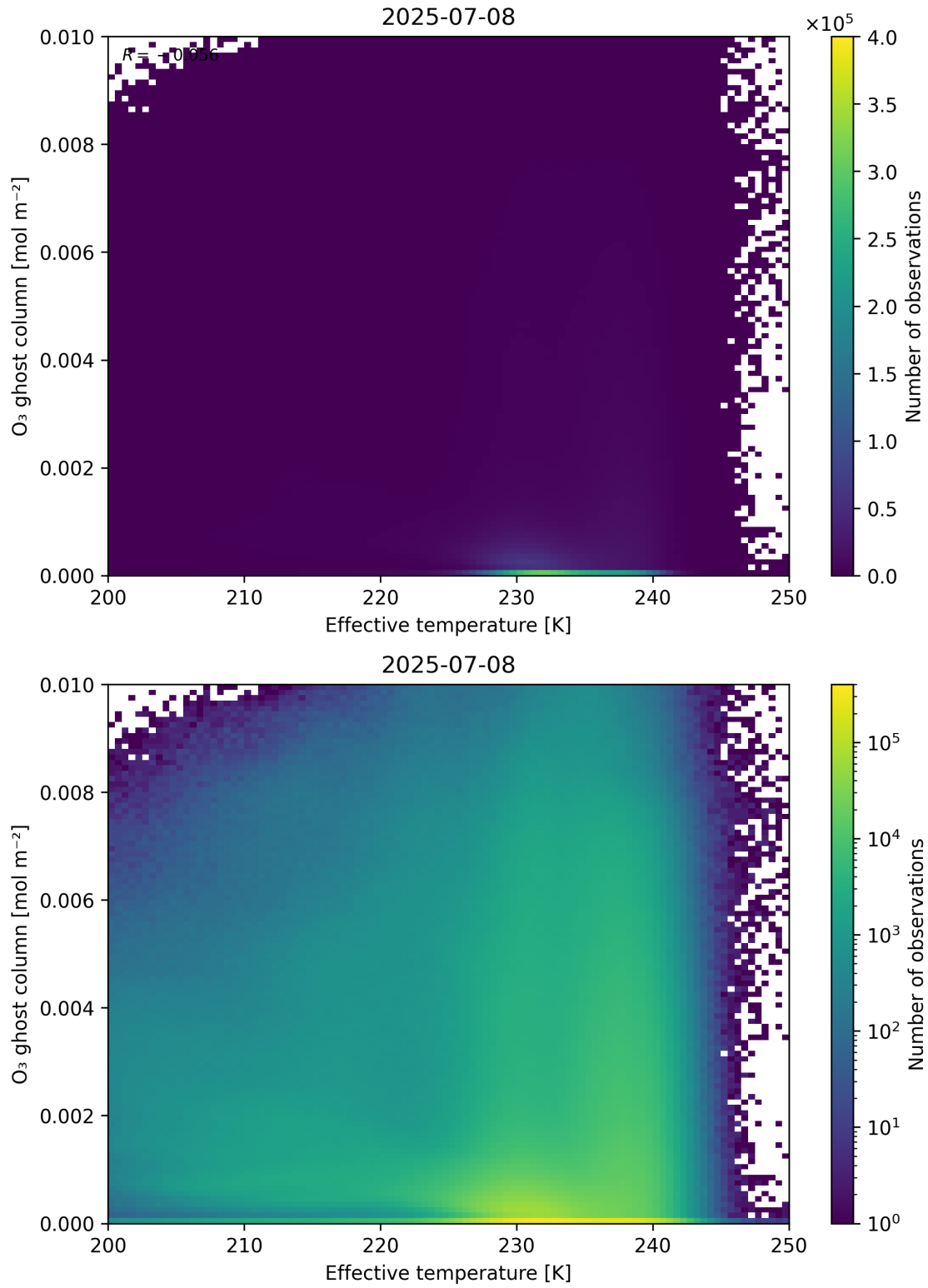
Figure 38: Scatter density plot of “Effective temperature” against “O 3 ghost column” for 2025-07-08 to 2025-07-09.
