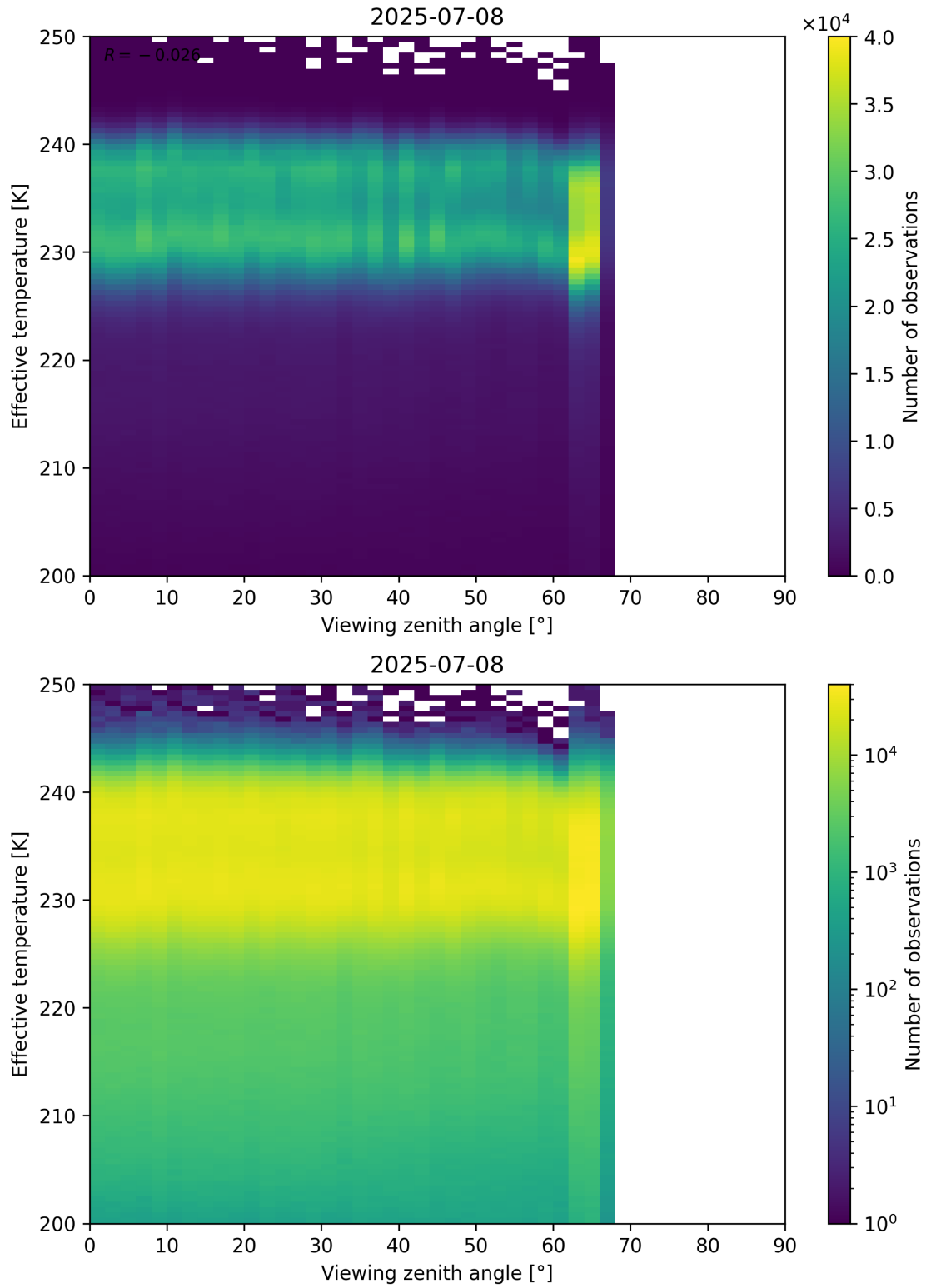
Figure 50: Scatter density plot of “Viewing zenith angle” against “Effective temperature” for 2025-07-08 to 2025-07-09.
