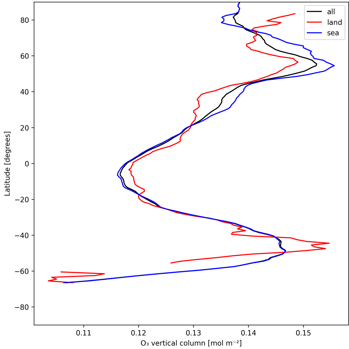
Figure 14: Zonal average of “O 3 vertical column” for 2025-07-08 to 2025-07-09.
