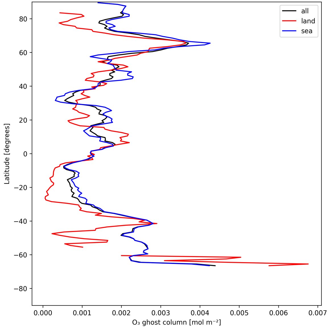
Figure 18: Zonal average of "O 3 ghost column" for 2025-07-08 to 2025-07-09.
