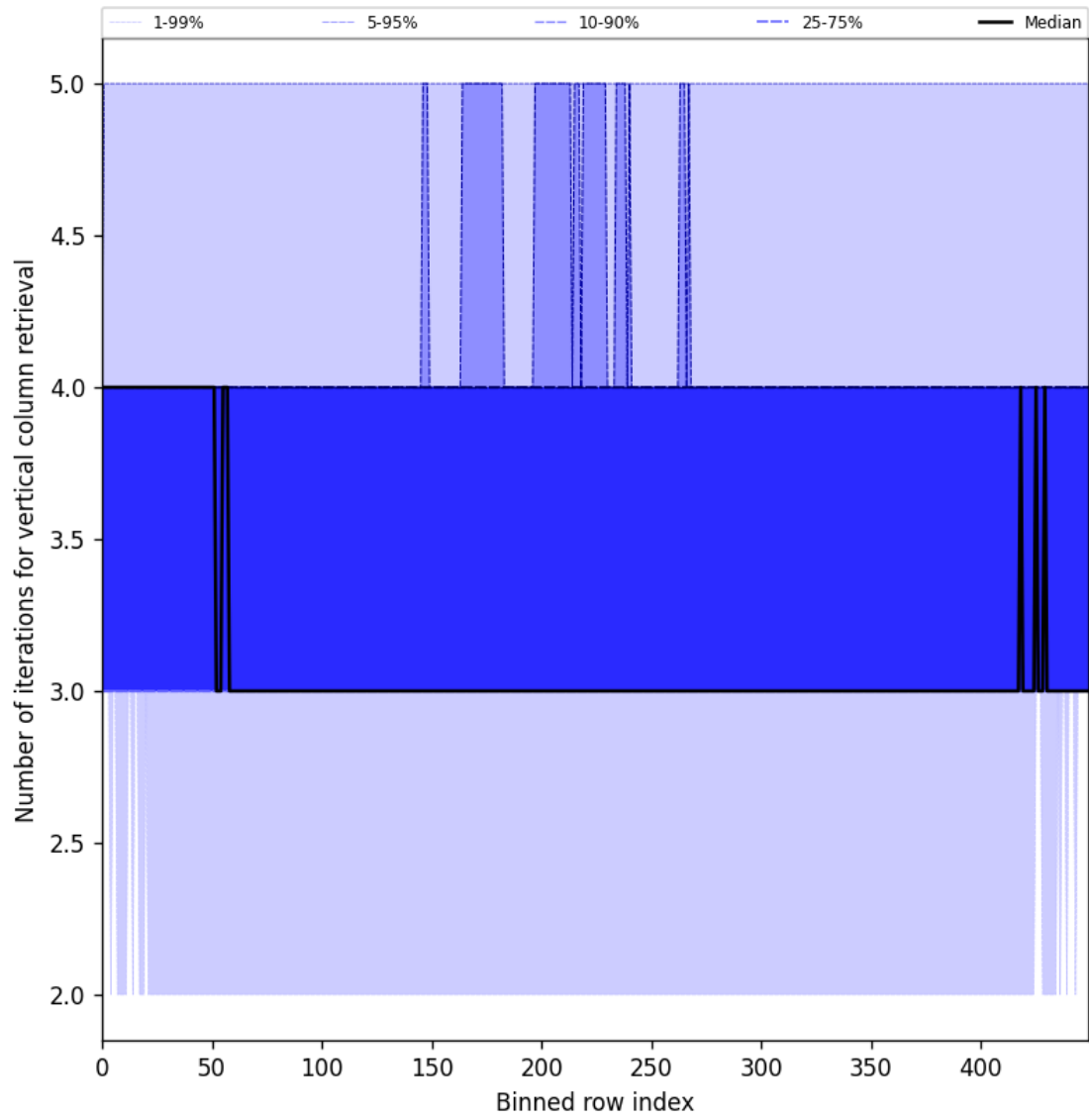
Figure 33: Along track statistics of “Number of iterations for vertical column retrieval” for 2025-07-08 to 2025-07-09
