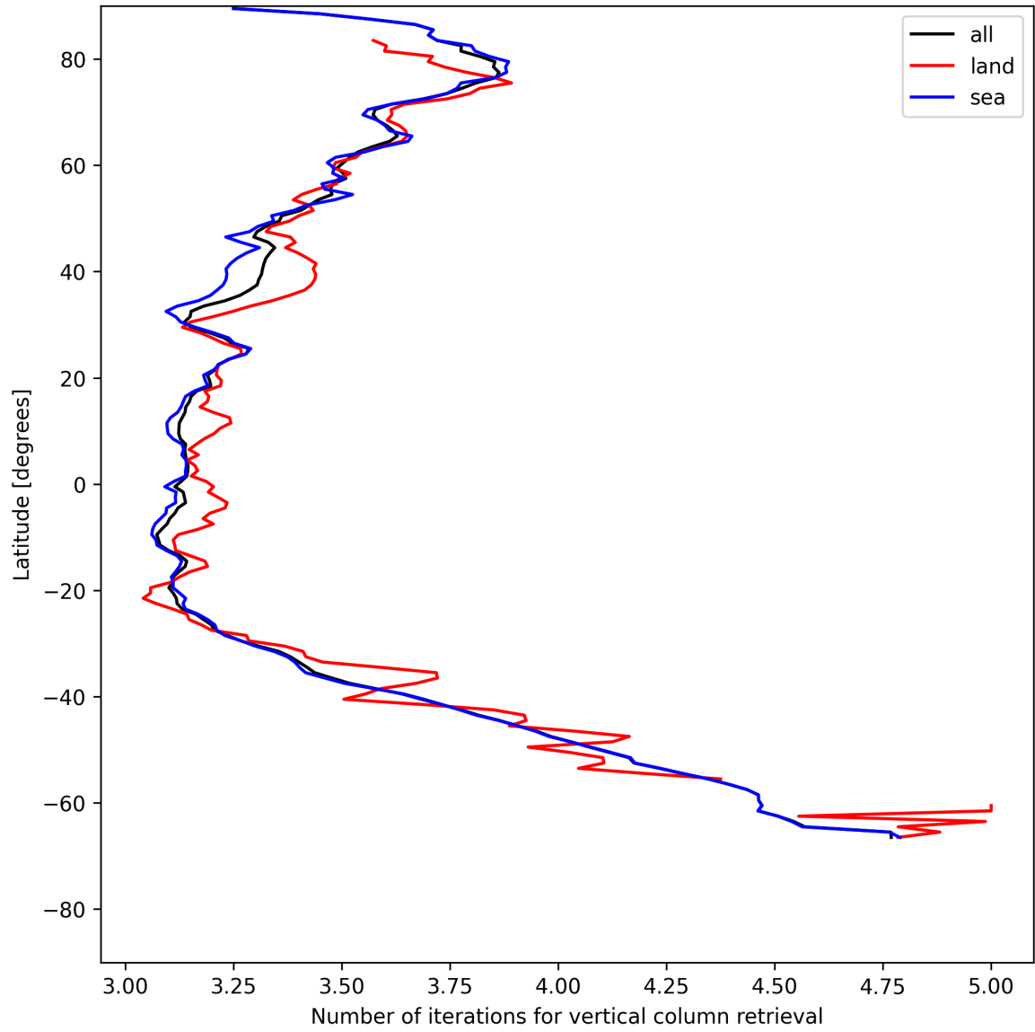
Figure 19: Zonal average of “Number of iterations for vertical column retrieval” for 2025-07-08 to 2025-07-09.
