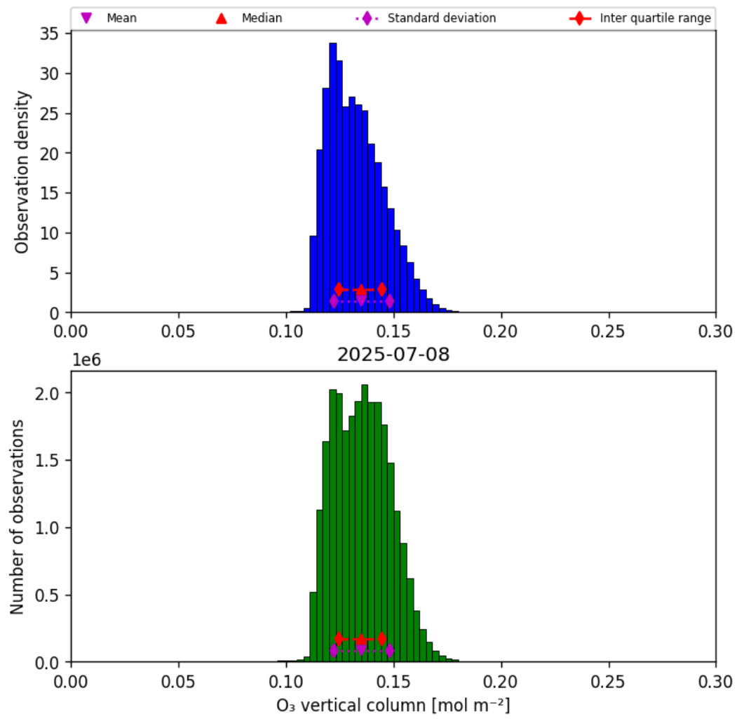
Figure 21: Histogram of “O 3 vertical column” for 2025-07-08 to 2025-07-09
