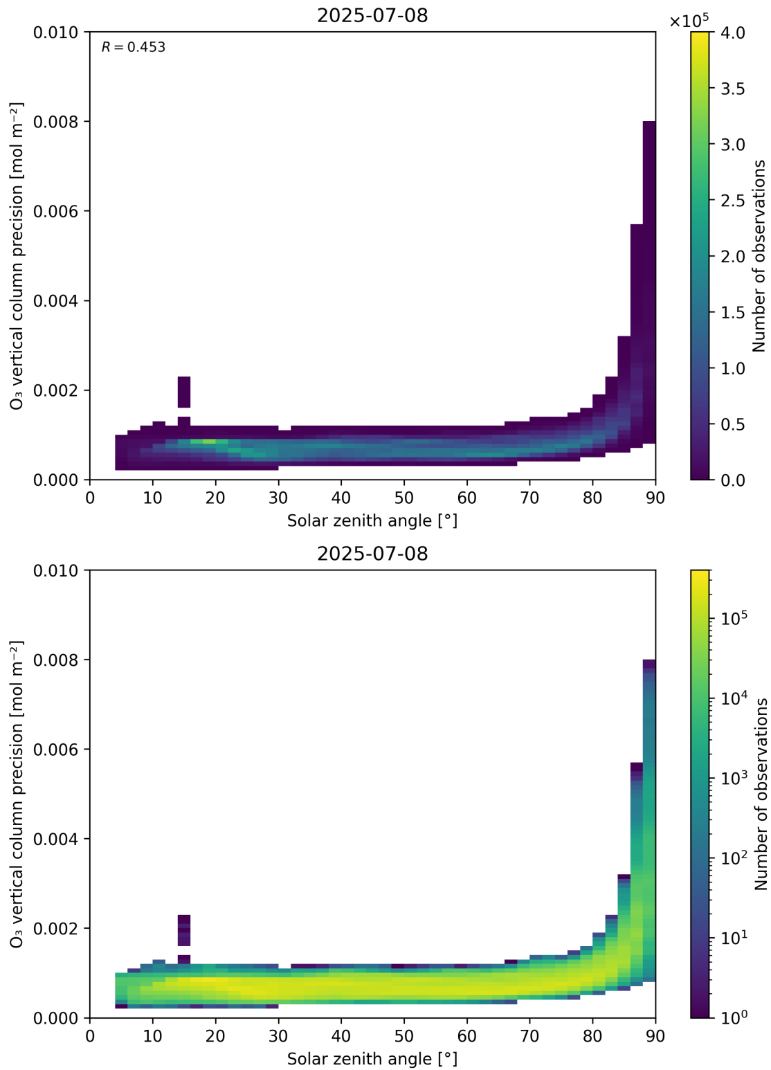
Figure 48: Scatter density plot of “Solar zenith angle” against “O 3 vertical column precision” for 2025-07-08 to 2025-07-09.
