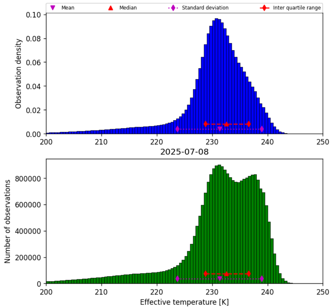
Figure 24: Histogram of “Effective temperature” for 2025-07-08 to 2025-07-09
