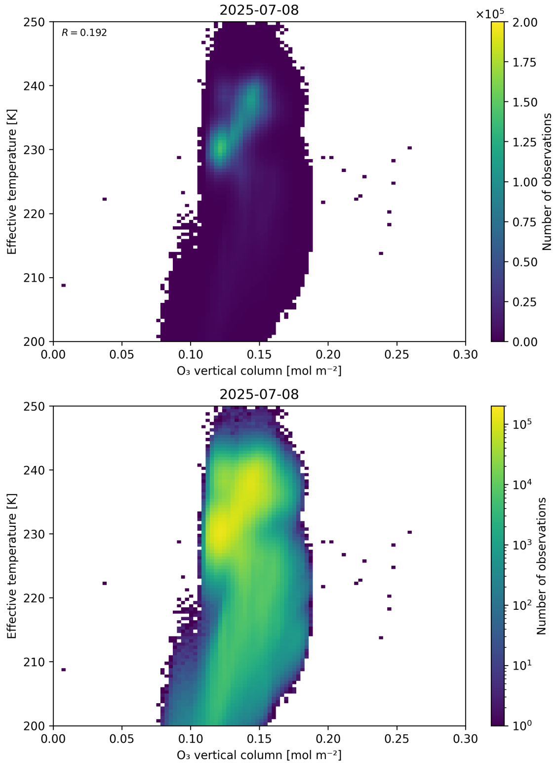
Figure 39: Scatter density plot of “O 3 vertical column” against “Effective temperature” for 2025-07-08 to 2025-07-09.
