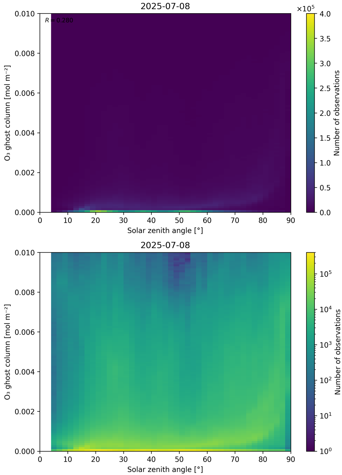
Figure 46: Scatter density plot of “Solar zenith angle” against “O 3 ghost column” for 2025-07-08 to 2025-07-09.
