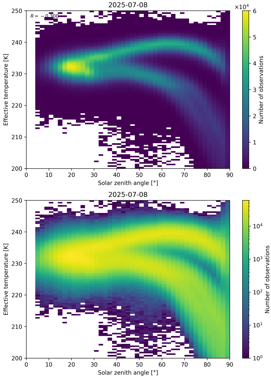
Figure 45: Scatter density plot of “Solar zenith angle” against “Effective temperature” for 2025-07-08 to 2025-07-09.
