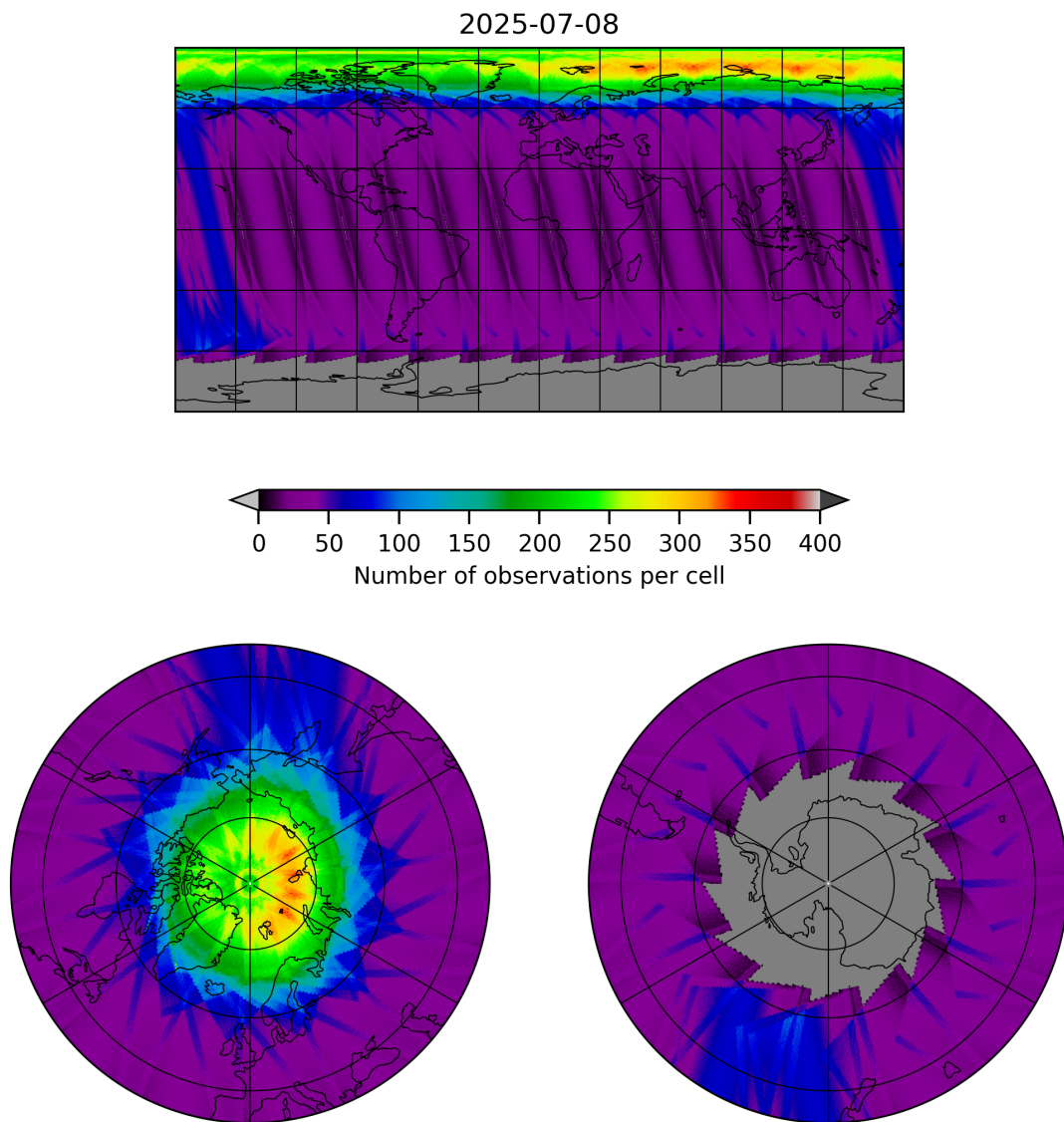
Figure 12: Map of the number of observations for 2025-07-08 to 2025-07-09
