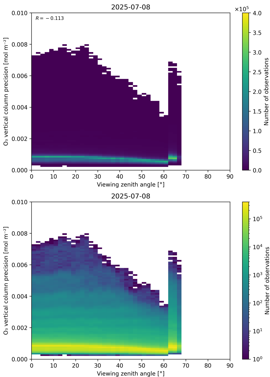
Figure 53: Scatter density plot of “Viewing zenith angle” against “O 3 vertical column precision” for 2025-07-08 to 2025-07-09.
