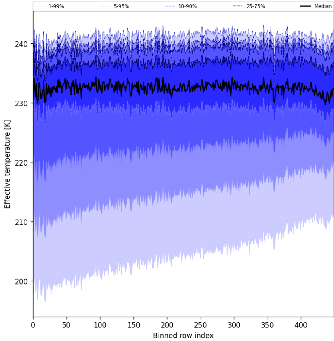
Figure 31: Along track statistics of “Effective temperature” for 2025-07-08 to 2025-07-09
