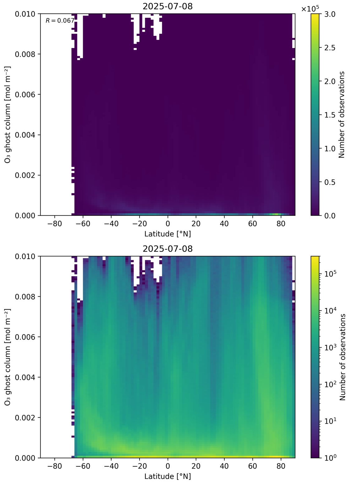
Figure 35: Scatter density plot of “Latitude” against “O 3 ghost column” for 2025-07-08 to 2025-07-09.
