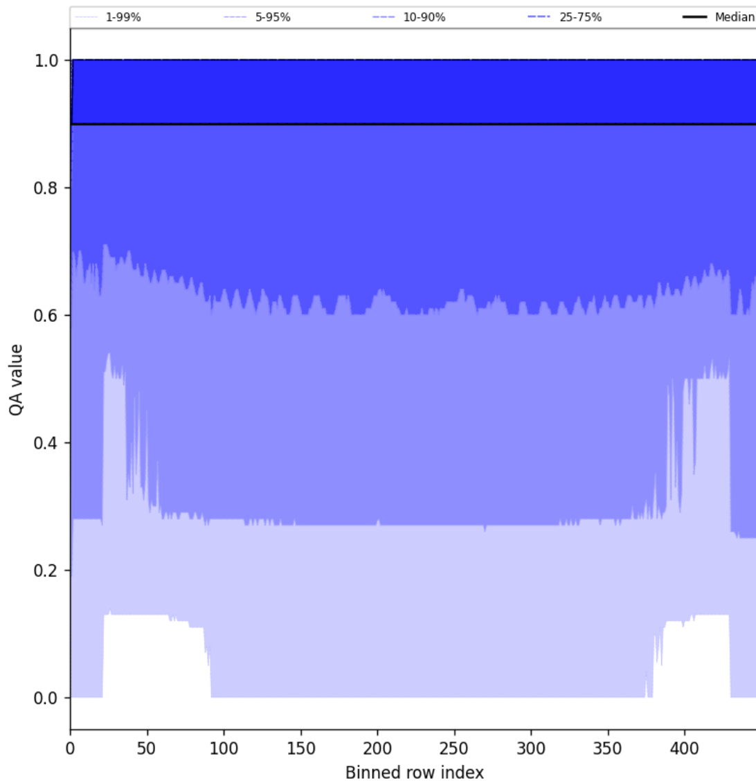
Figure 27: Along track statistics of “QA value” for 2025-07-08 to 2025-07-09
