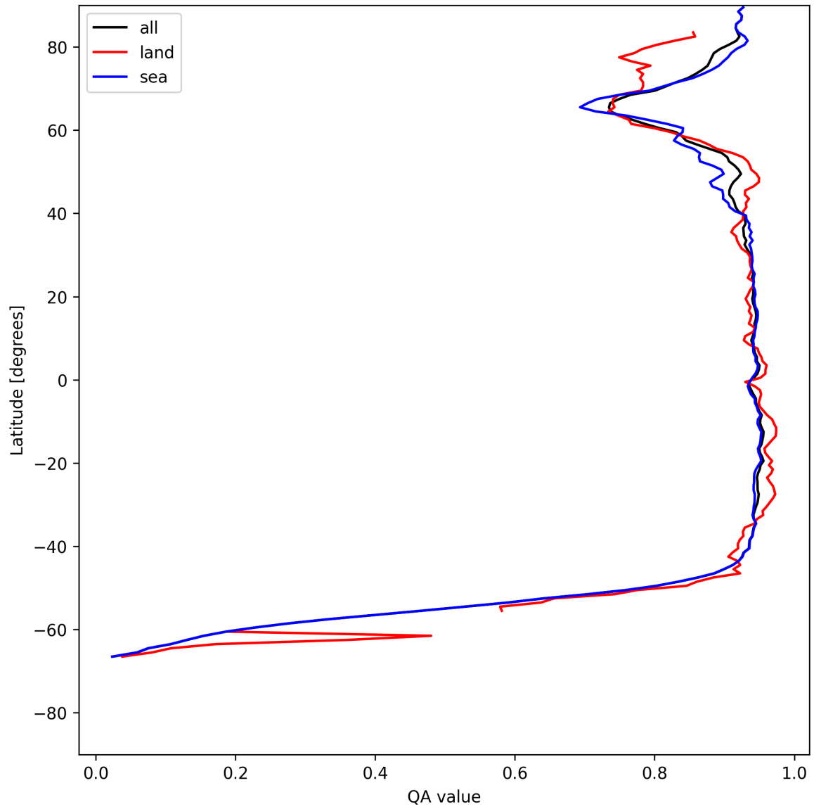
Figure 13: Zonal average of “QA value” for 2025-07-08 to 2025-07-09.
