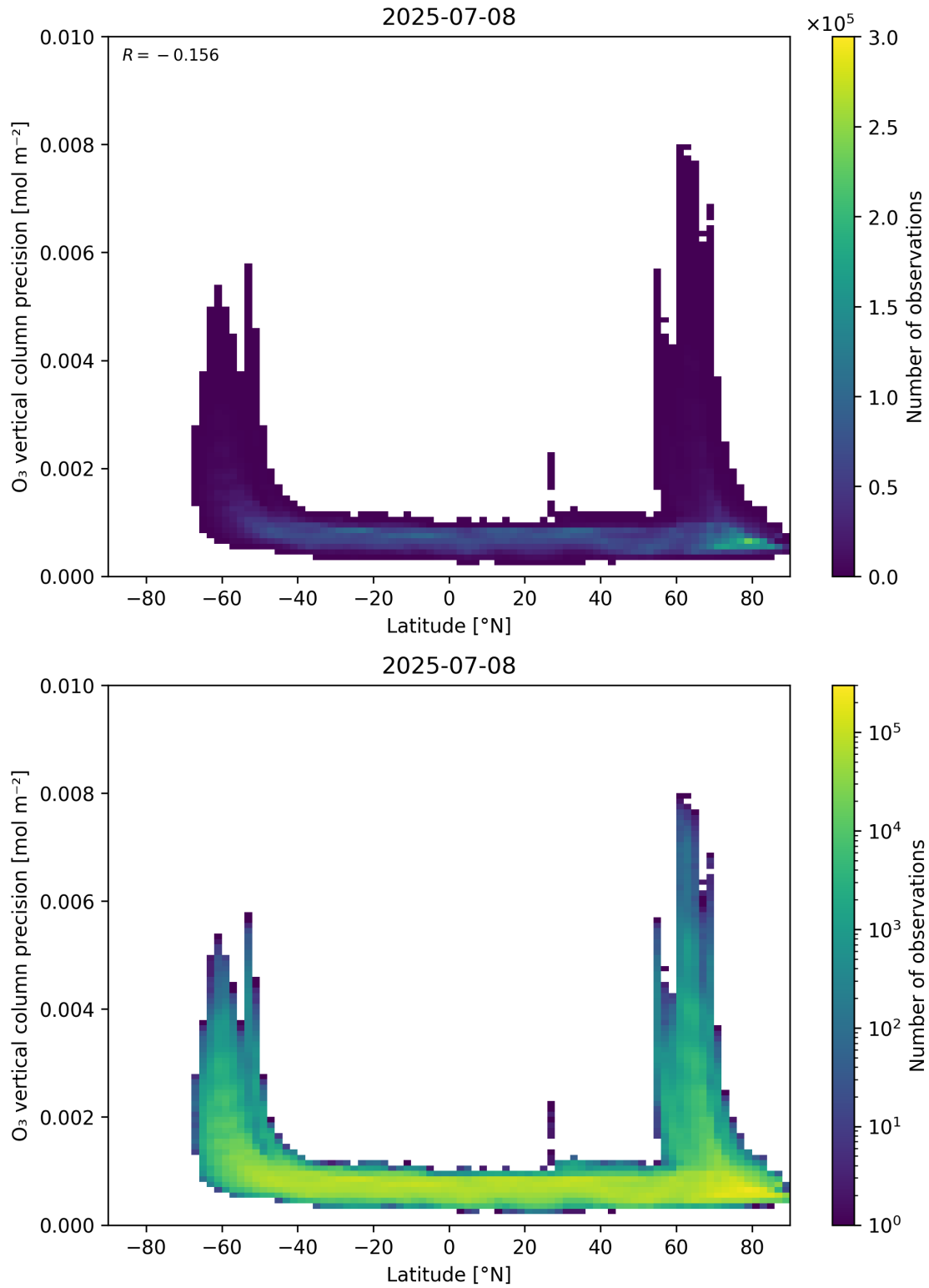
Figure 37: Scatter density plot of “Latitude” against “O 3 vertical column precision” for 2025-07-08 to 2025-07-09.
