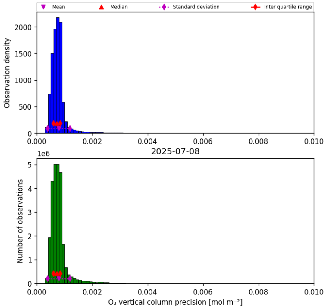
Figure 22: Histogram of “O 3 vertical column precision” for 2025-07-08 to 2025-07-09
