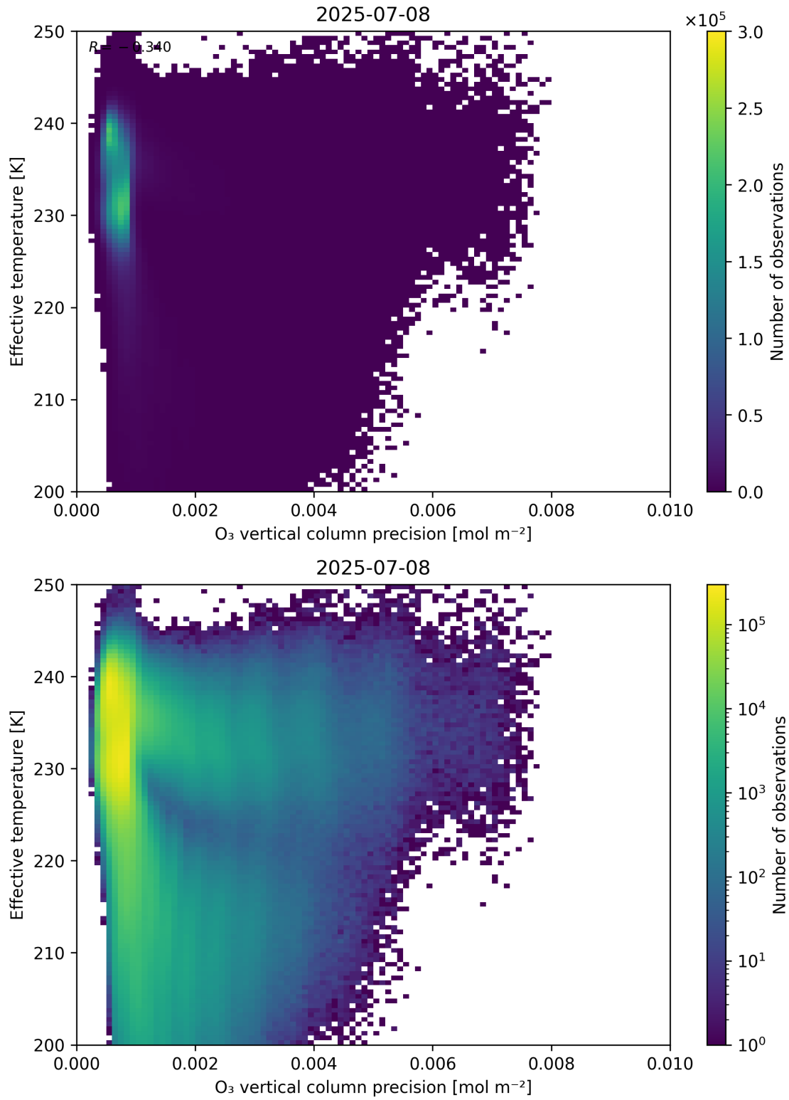
Figure 42: Scatter density plot of “O 3 vertical column precision” against “Effective temperature” for 2025-07-08 to 2025-07-09.
