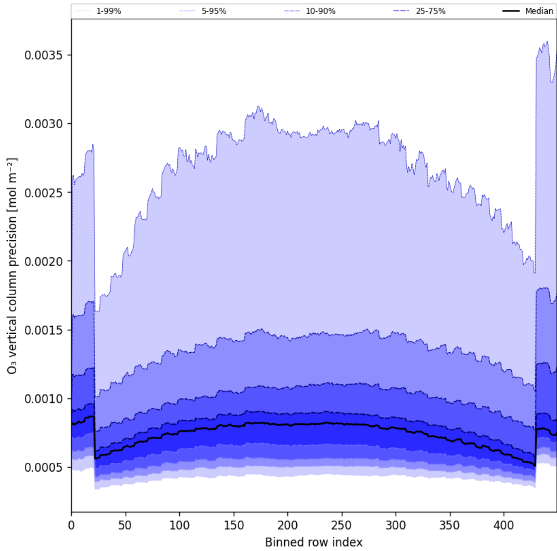
Figure 29: Along track statistics of "O 3 vertical column precision" for 2025-07-08 to 2025-07-09
