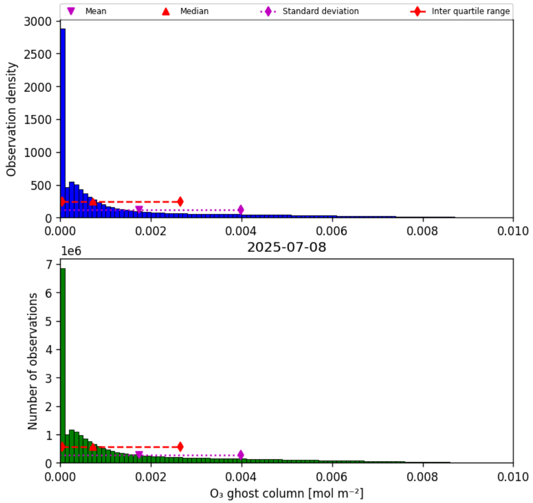
Figure 25: Histogram of “O 3 ghost column” for 2025-07-08 to 2025-07-09
