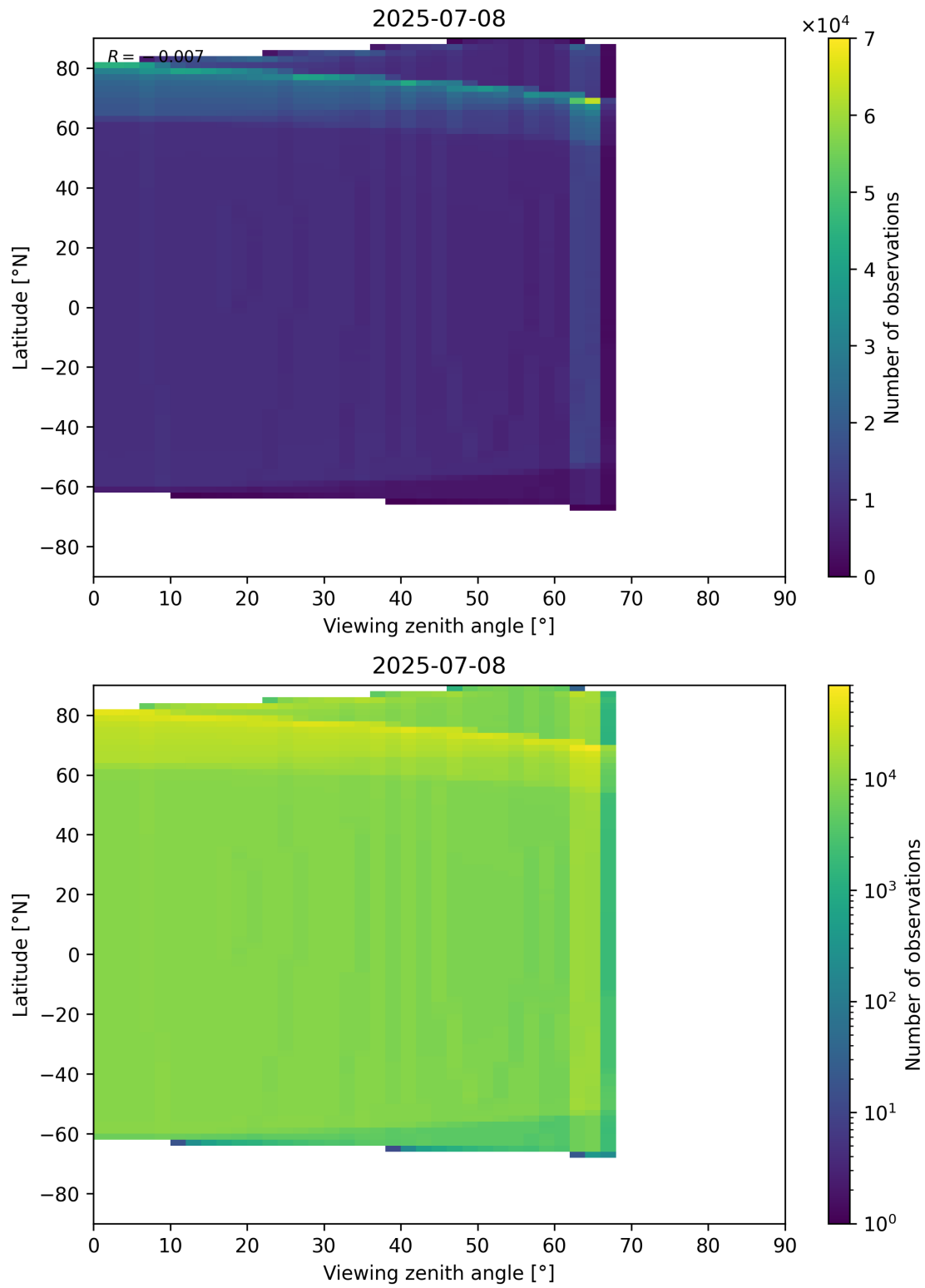
Figure 49: Scatter density plot of “Viewing zenith angle” against “Latitude” for 2025-07-08 to 2025-07-09.
