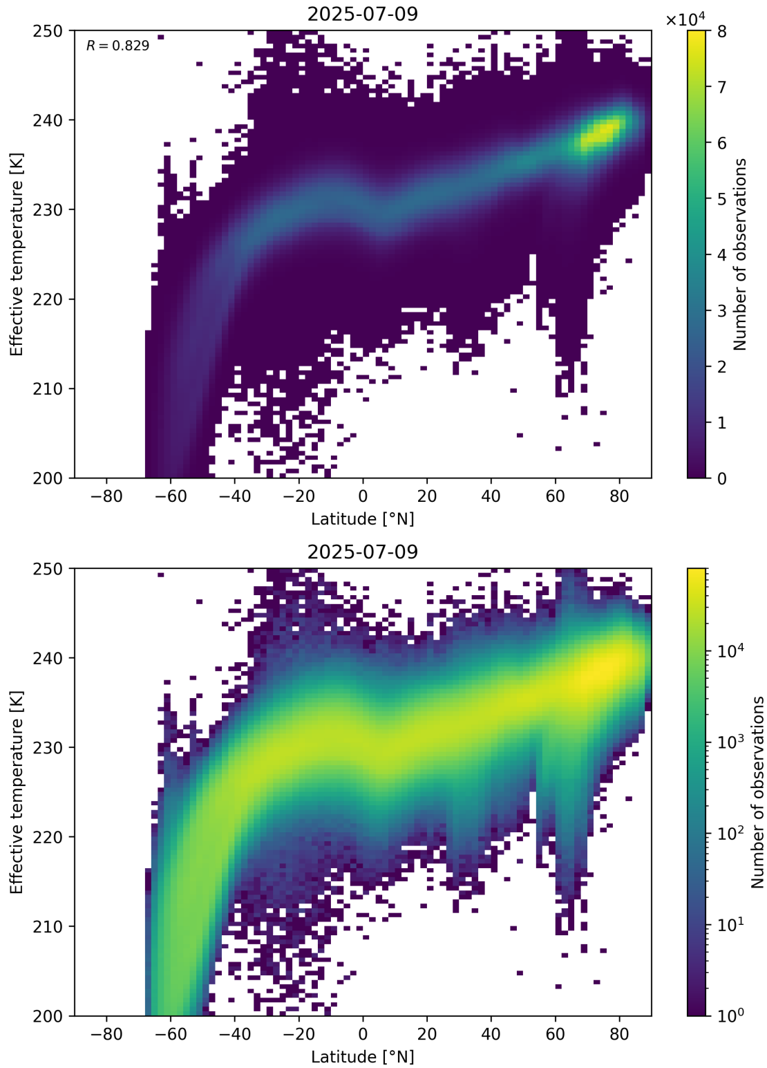
Figure 34: Scatter density plot of “Latitude” against “Effective temperature” for 2025-07-08 to 2025-07-10.
