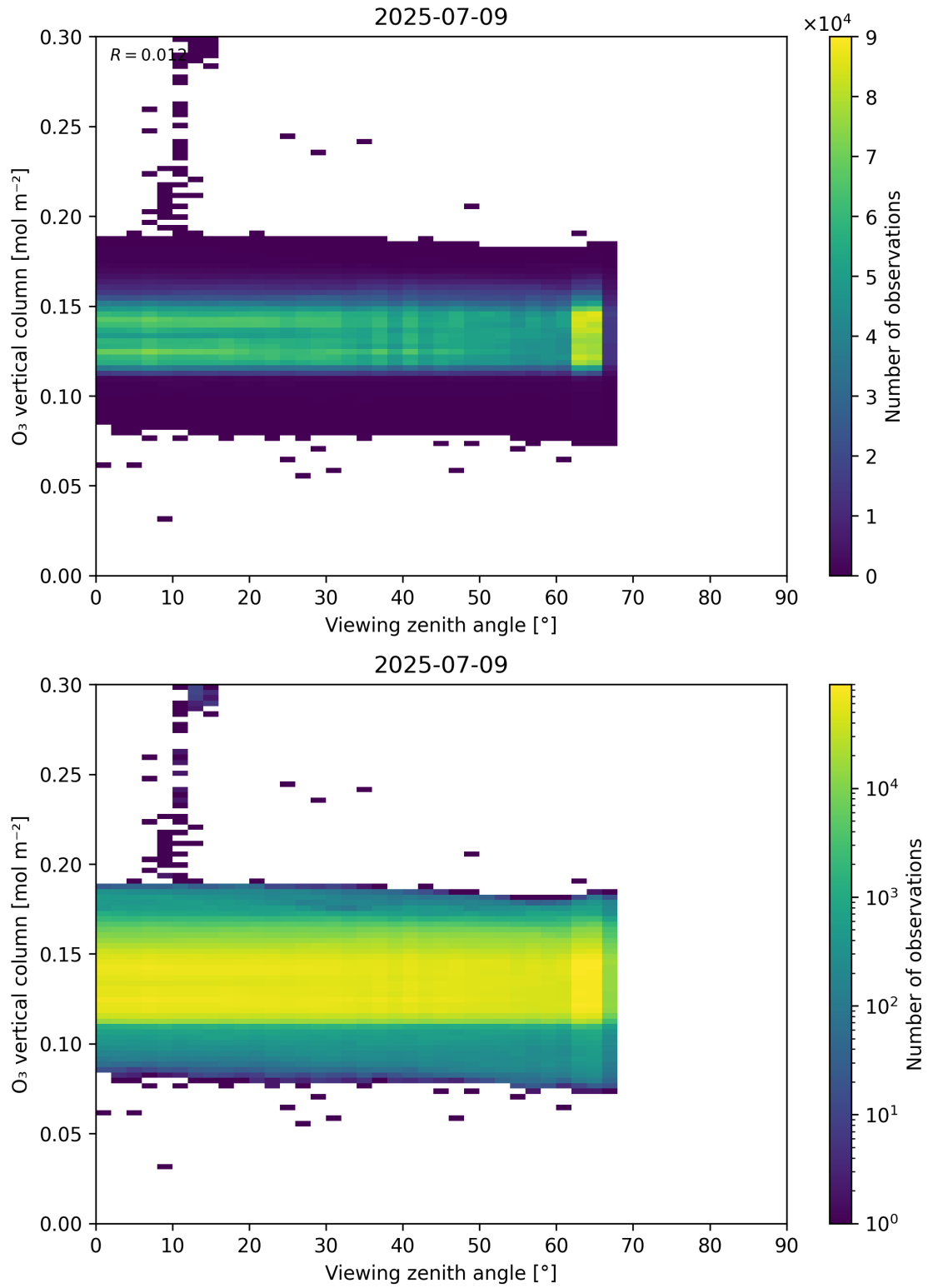
Figure 52: Scatter density plot of “Viewing zenith angle” against “O 3 vertical column” for 2025-07-08 to 2025-07-10.
