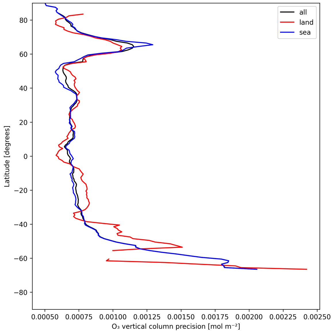
Figure 15: Zonal average of “O 3 vertical column precision” for 2025-07-08 to 2025-07-10.
