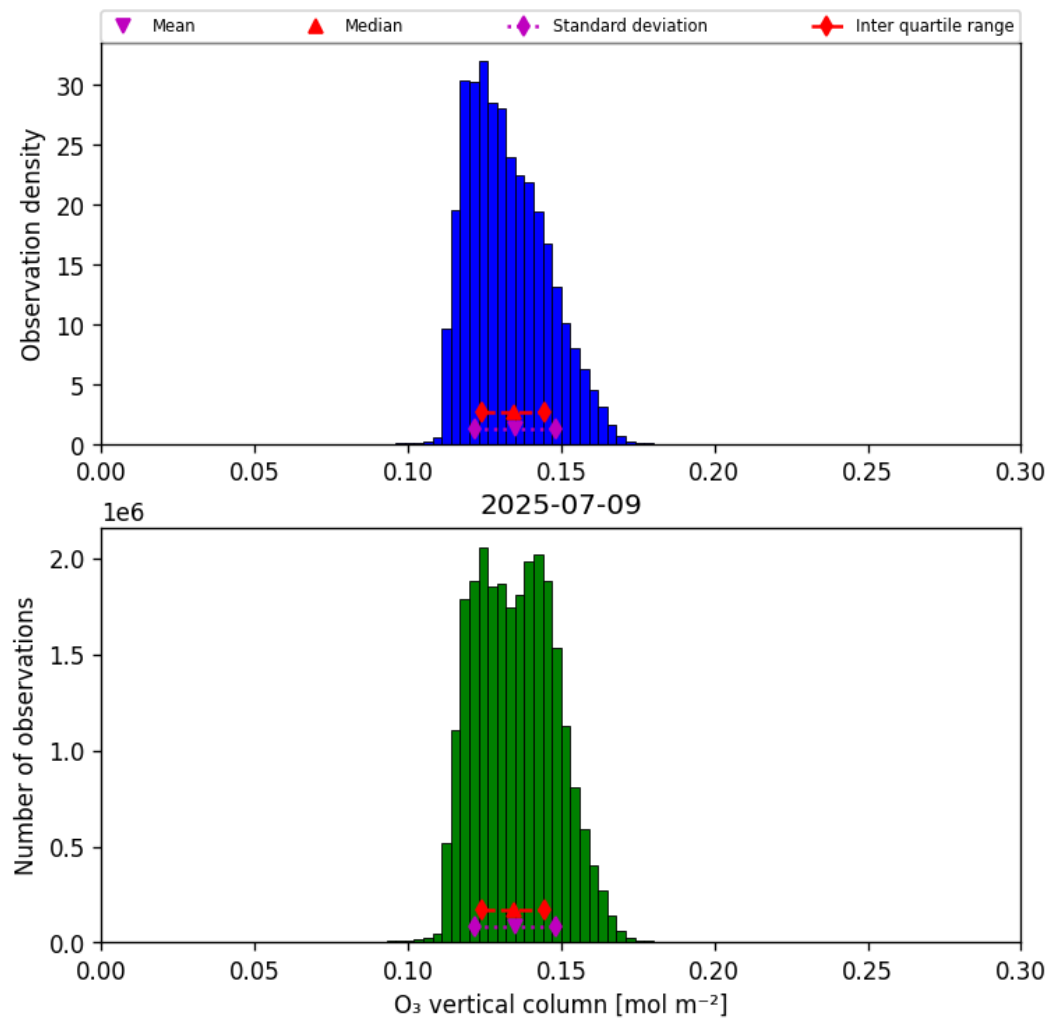
Figure 21: Histogram of “O 3 vertical column” for 2025-07-08 to 2025-07-10
