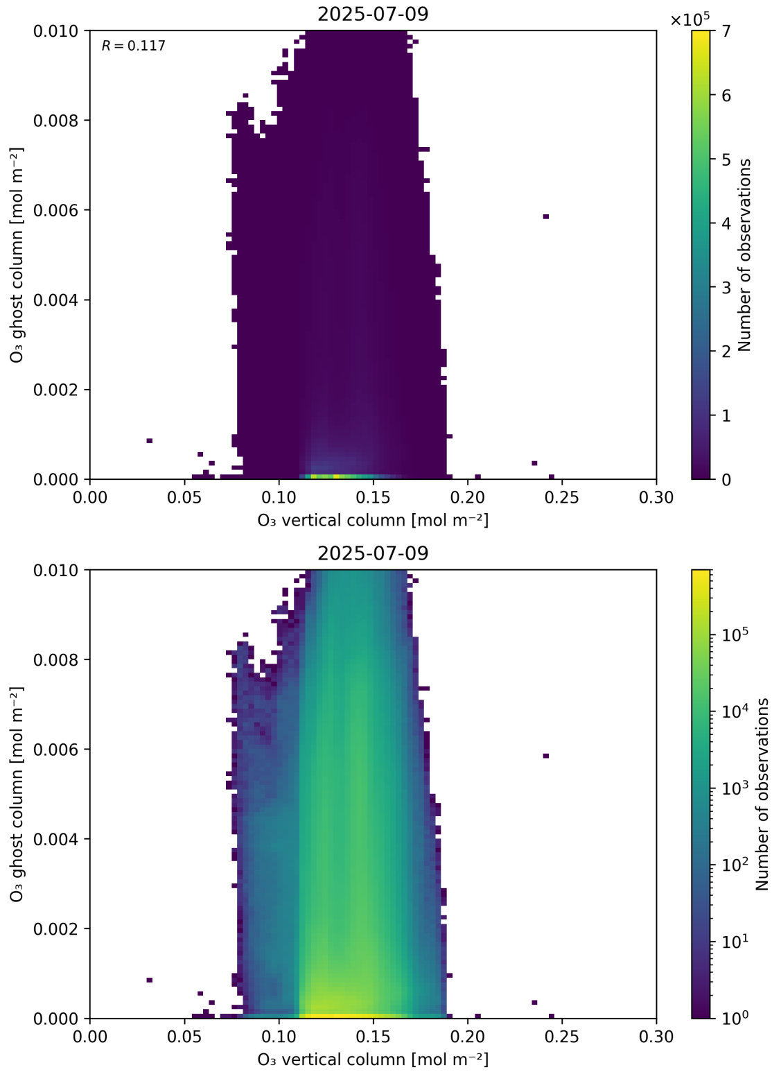
Figure 40: Scatter density plot of “O 3 vertical column” against “O 3 ghost column” for 2025-07-08 to 2025-07-10.
