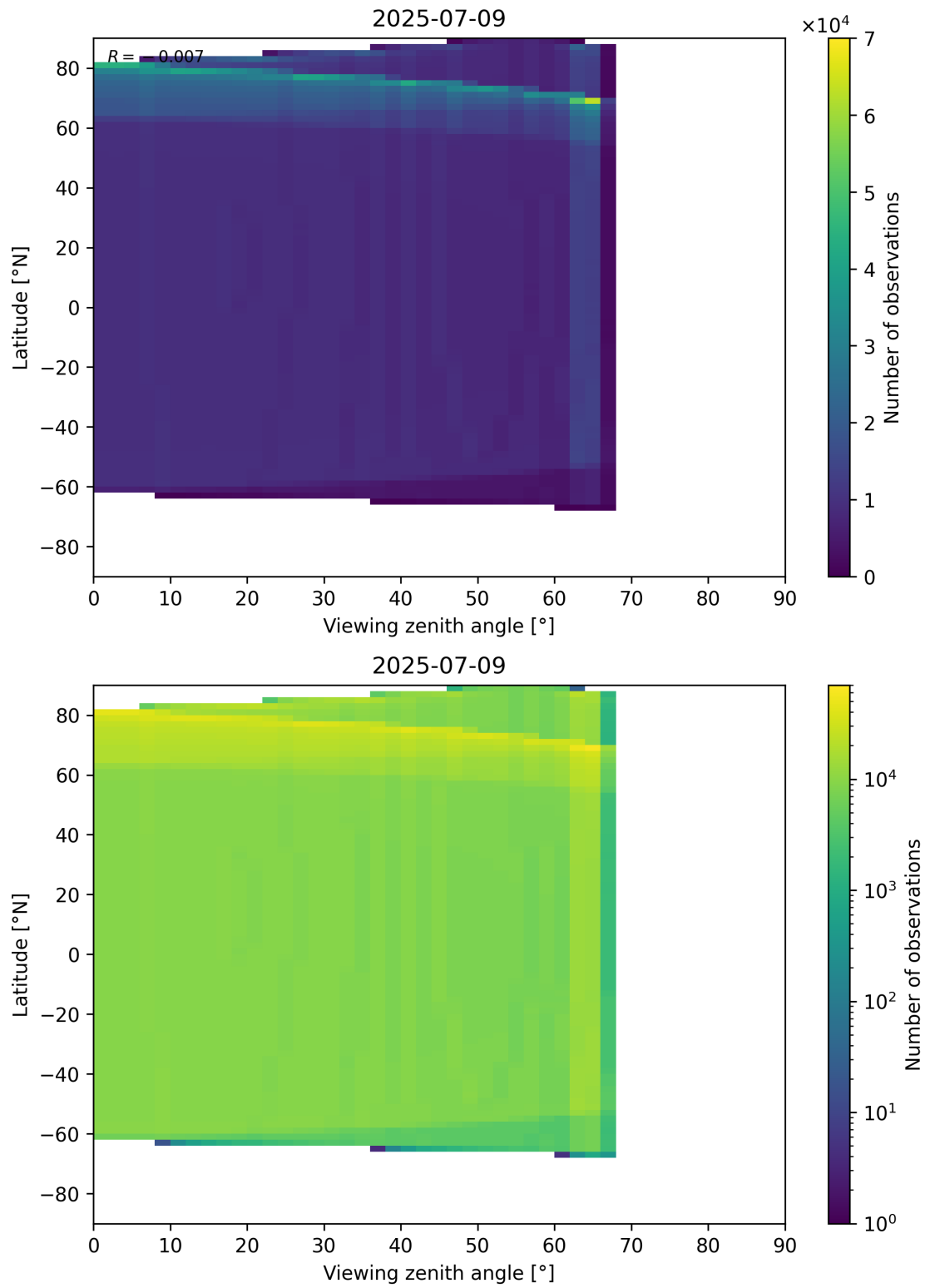
Figure 49: Scatter density plot of “Viewing zenith angle” against “Latitude” for 2025-07-08 to 2025-07-10.
