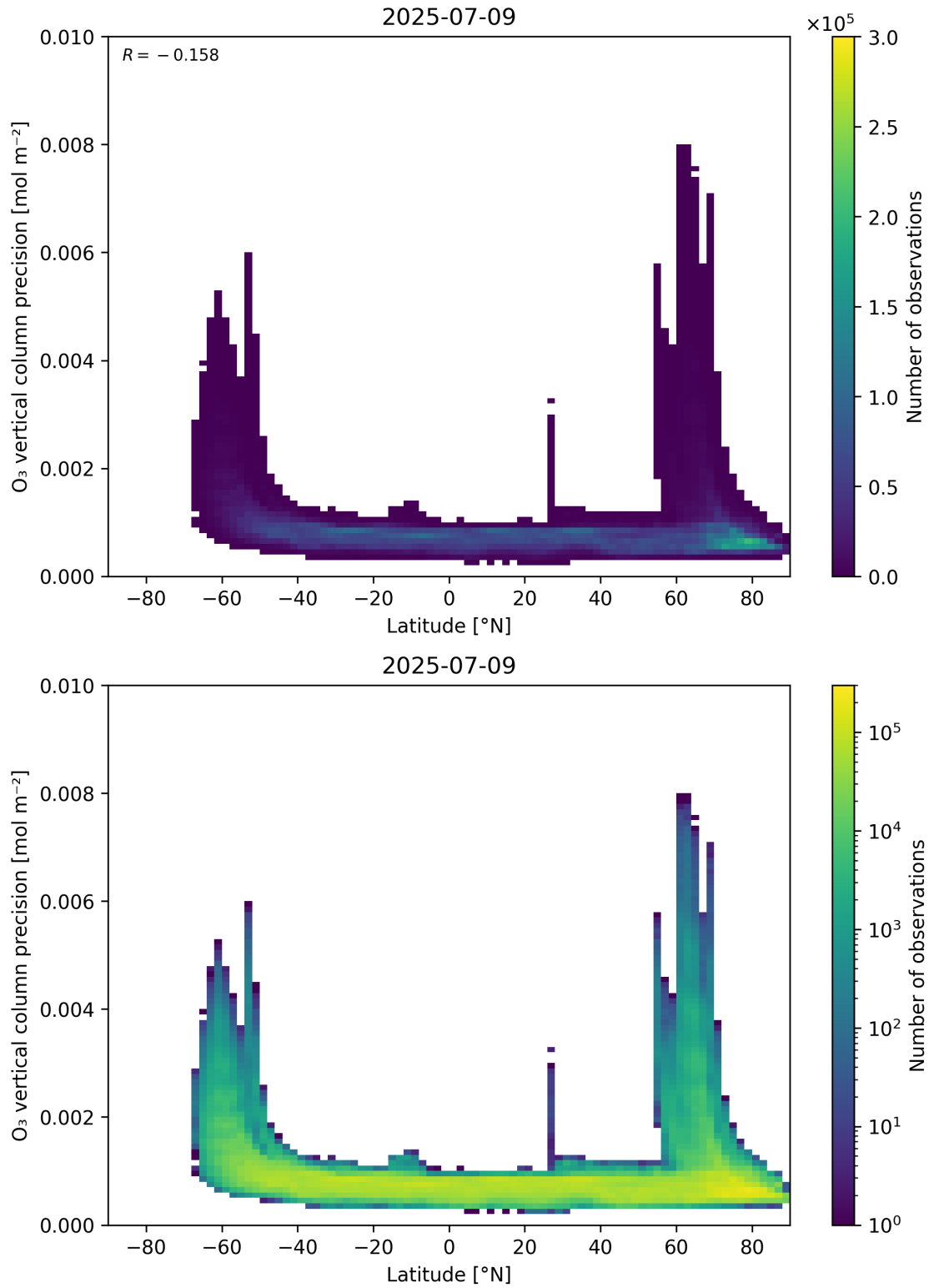
Figure 37: Scatter density plot of “Latitude” against “O 3 vertical column precision” for 2025-07-08 to 2025-07-10.
