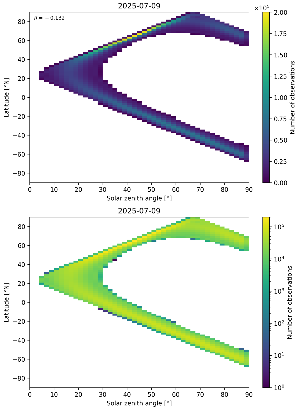
Figure 44: Scatter density plot of “Solar zenith angle” against “Latitude” for 2025-07-08 to 2025-07-10.
