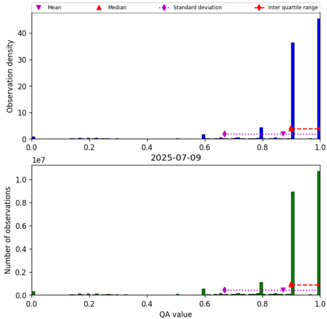
Figure 20: Histogram of “QA value” for 2025-07-08 to 2025-07-10
