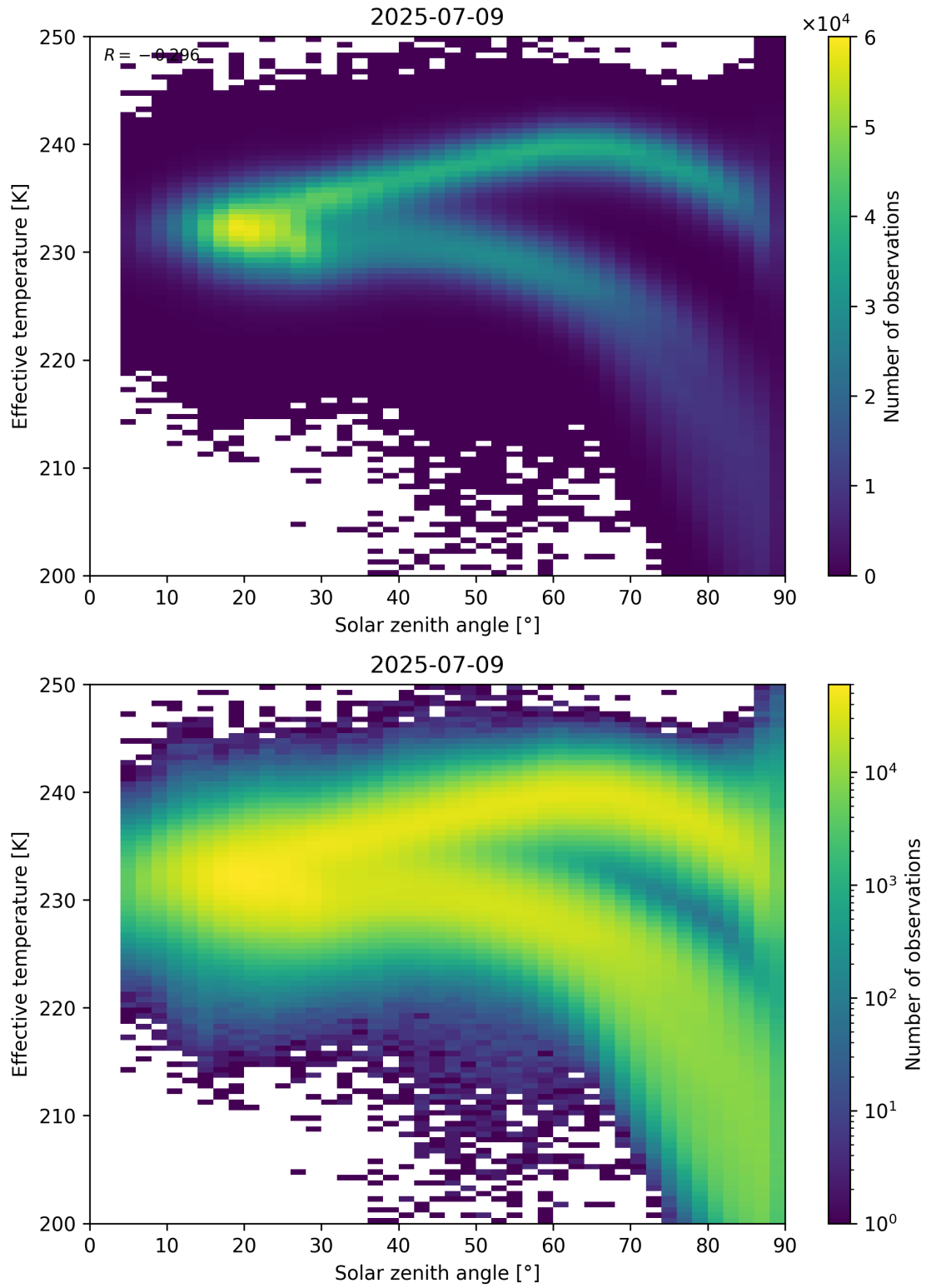
Figure 45: Scatter density plot of “Solar zenith angle” against “Effective temperature” for 2025-07-08 to 2025-07-10.
