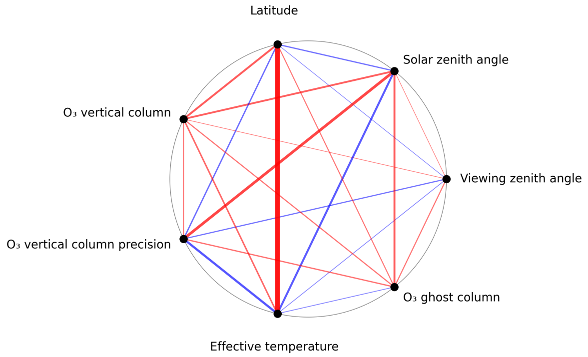
Figure 1: Map of correlation graph for 2025-07-08 to 2025-07-10.
