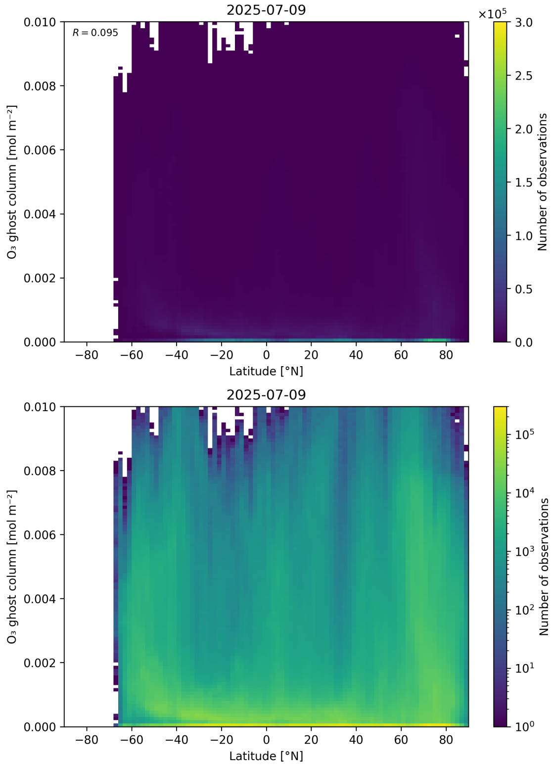
Figure 35: Scatter density plot of “Latitude” against “O 3 ghost column” for 2025-07-08 to 2025-07-10.
