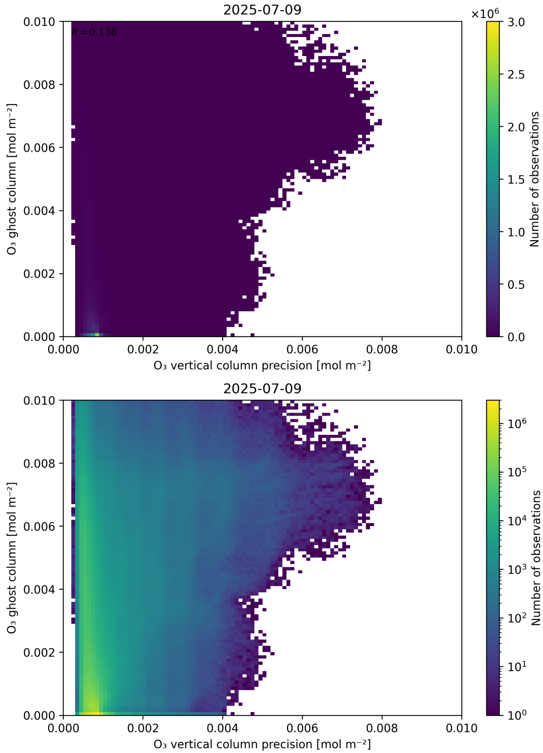
Figure 43: Scatter density plot of “ \text{O}_3 vertical column precision” against “ \text{O}_3 ghost column” for 2025-07-08 to 2025-07-10.
