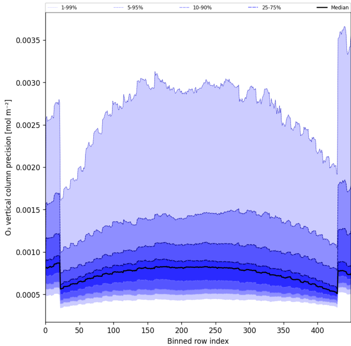
Figure 29: Along track statistics of “O 3 vertical column precision” for 2025-07-08 to 2025-07-10
