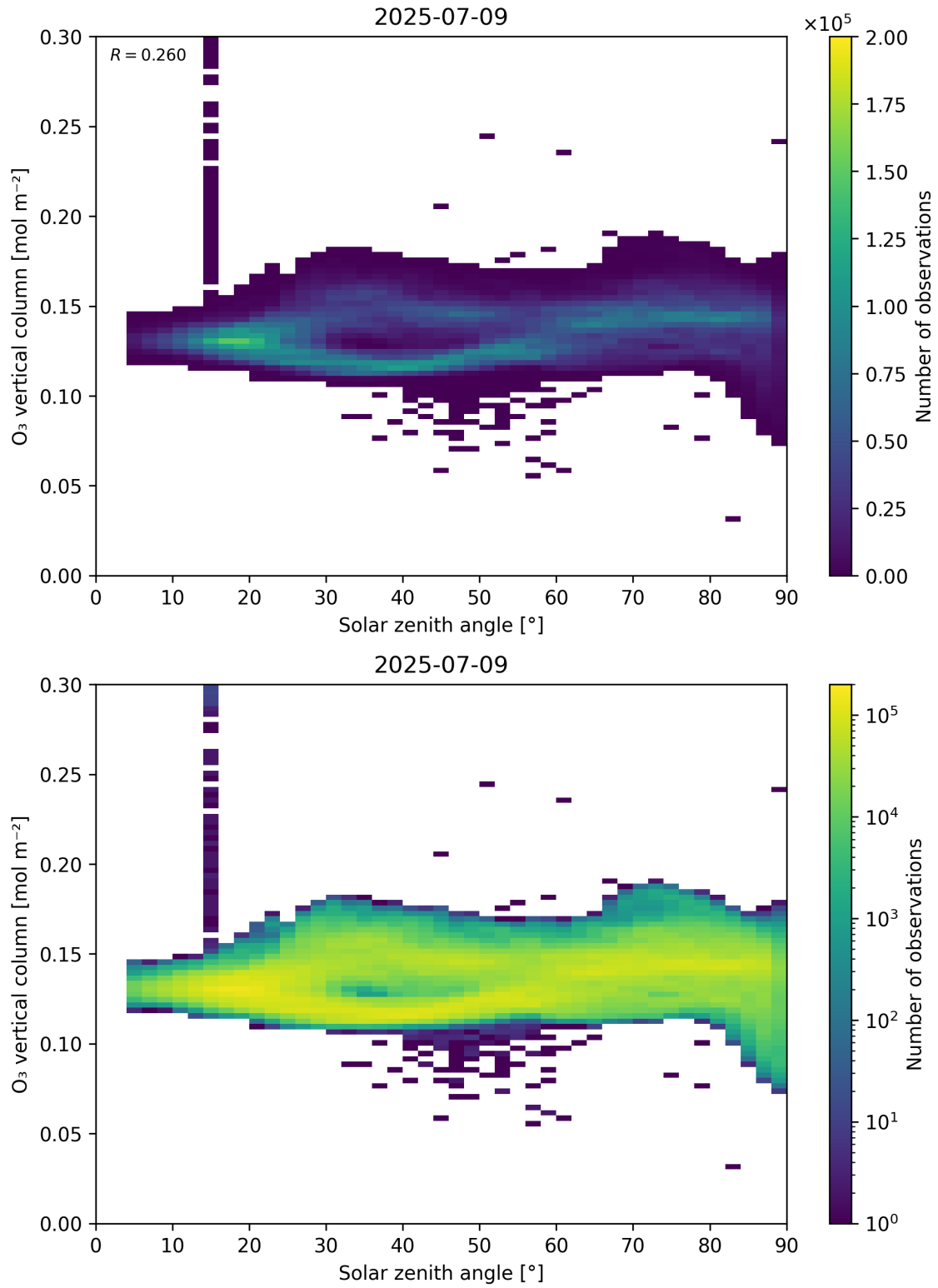
Figure 47: Scatter density plot of “Solar zenith angle” against “O 3 vertical column” for 2025-07-08 to 2025-07-10.
