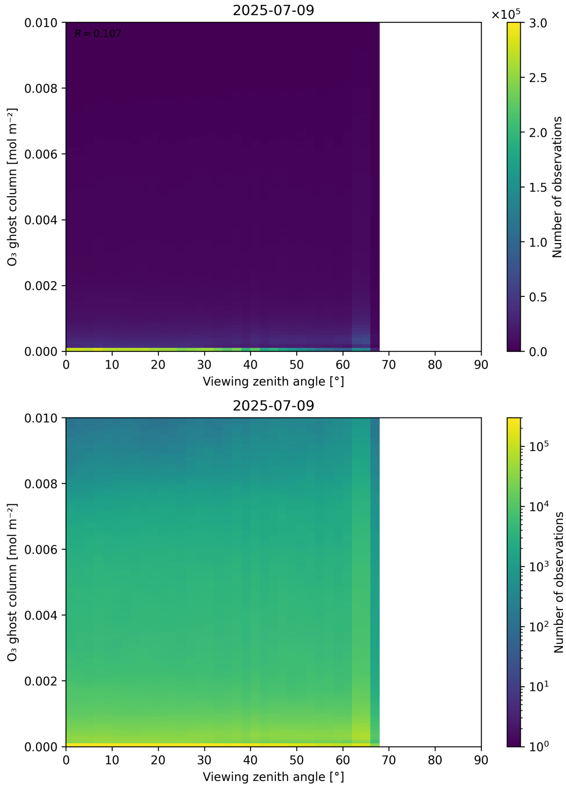
Figure 51: Scatter density plot of “Viewing zenith angle” against “O 3 ghost column” for 2025-07-08 to 2025-07-10.
