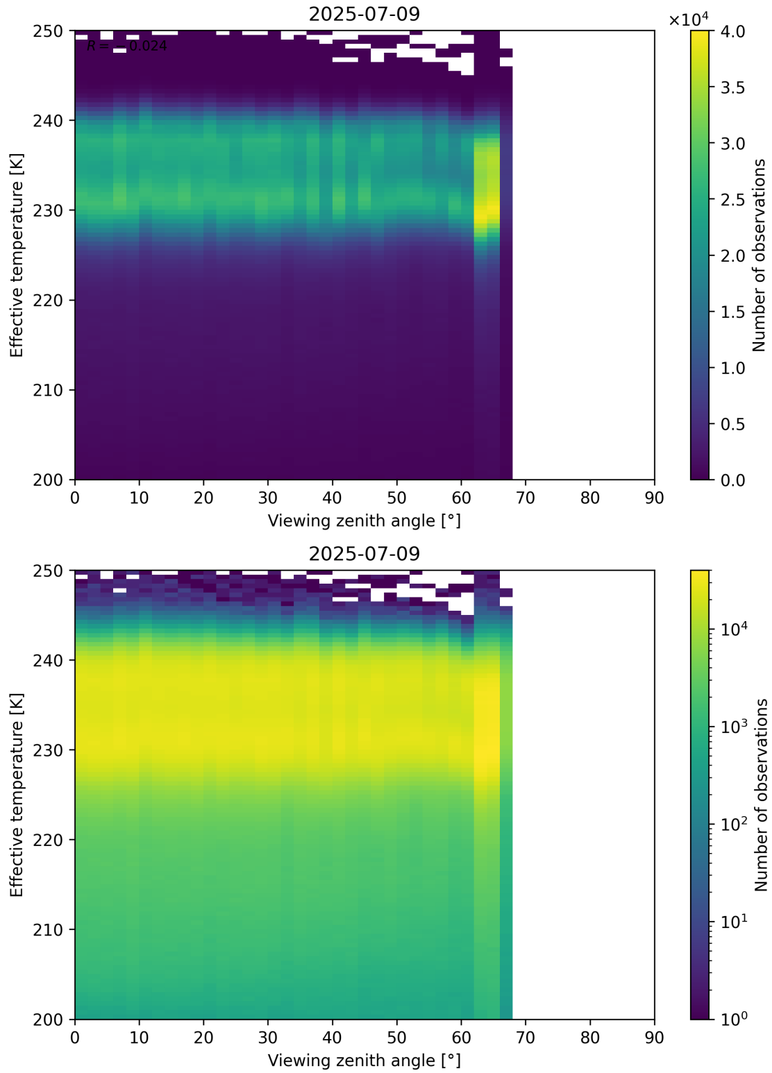
Figure 50: Scatter density plot of “Viewing zenith angle” against “Effective temperature” for 2025-07-08 to 2025-07-10.
