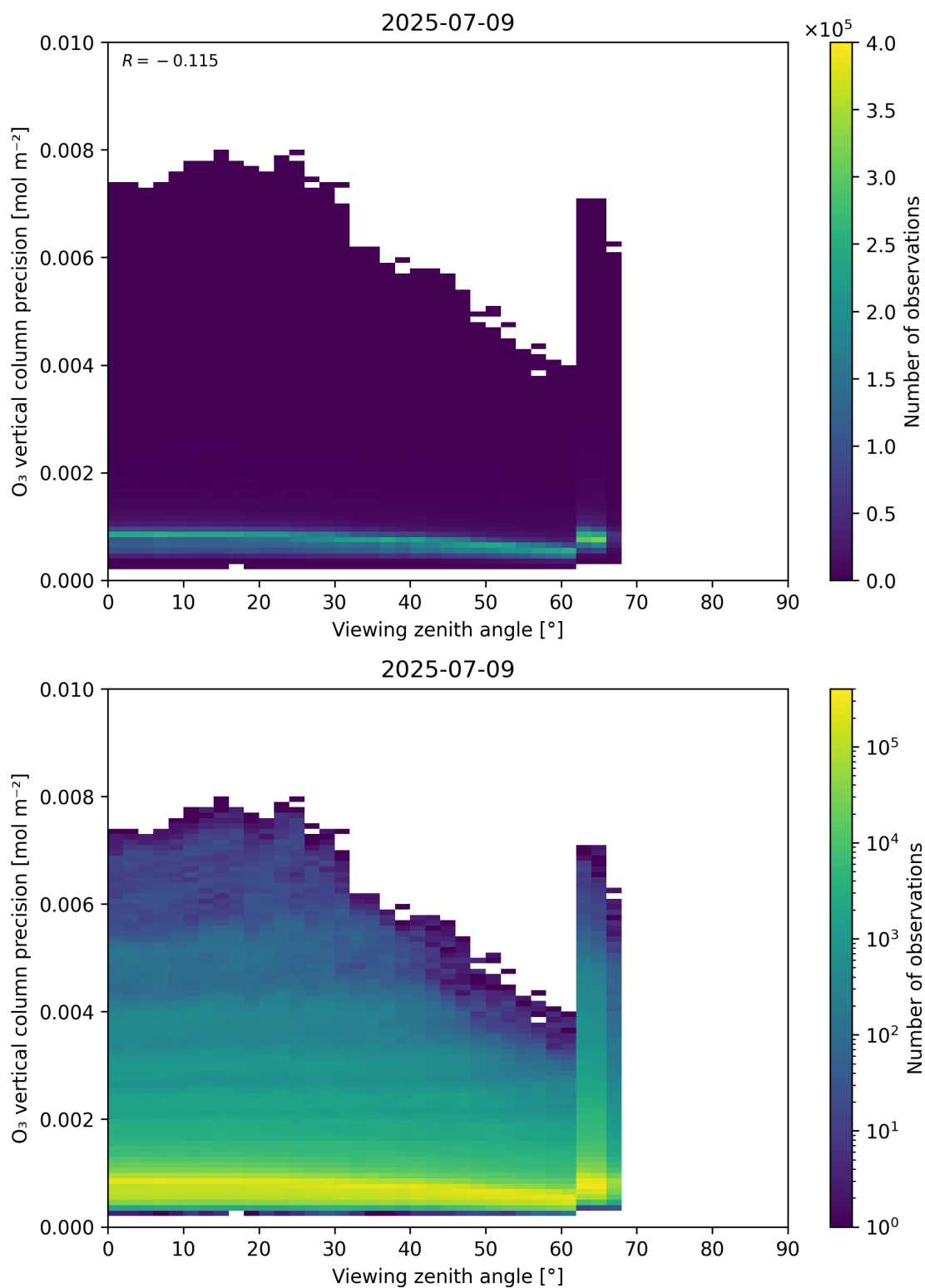
Figure 53: Scatter density plot of “Viewing zenith angle” against “O 3 vertical column precision” for 2025-07-08 to 2025-07-10.
