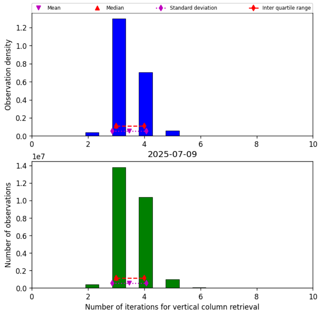
Figure 26: Histogram of “Number of iterations for vertical column retrieval” for 2025-07-08 to 2025-07-10
