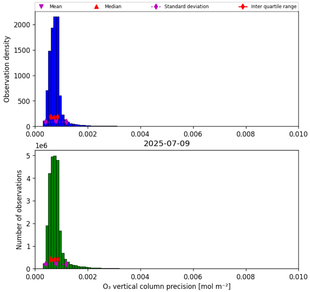
Figure 22: Histogram of “O 3 vertical column precision” for 2025-07-08 to 2025-07-10
