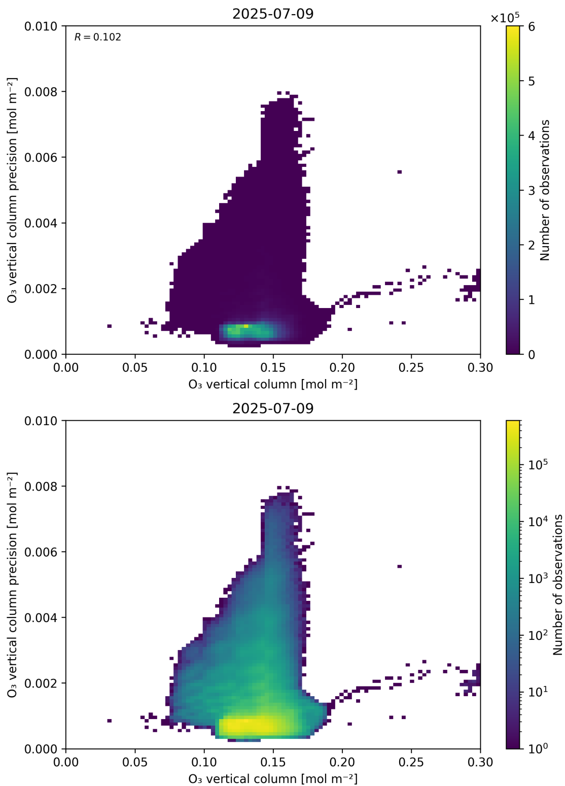
Figure 41: Scatter density plot of “O 3 vertical column” against “O 3 vertical column precision” for 2025-07-08 to 2025-07-10.
