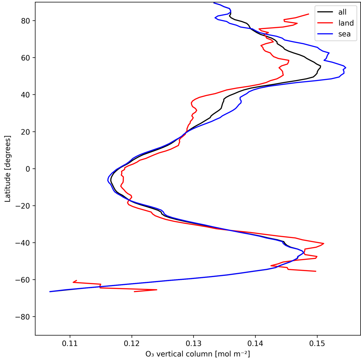
Figure 14: Zonal average of “O 3 vertical column” for 2025-07-08 to 2025-07-10.
