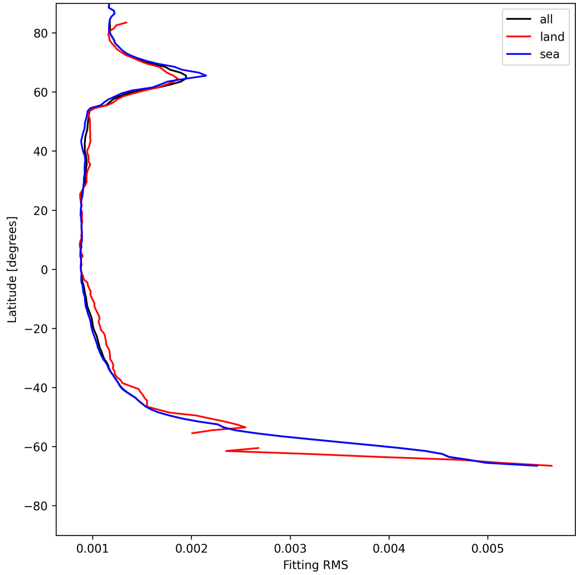
Figure 16: Zonal average of “Fitting RMS” for 2025-07-08 to 2025-07-10.
