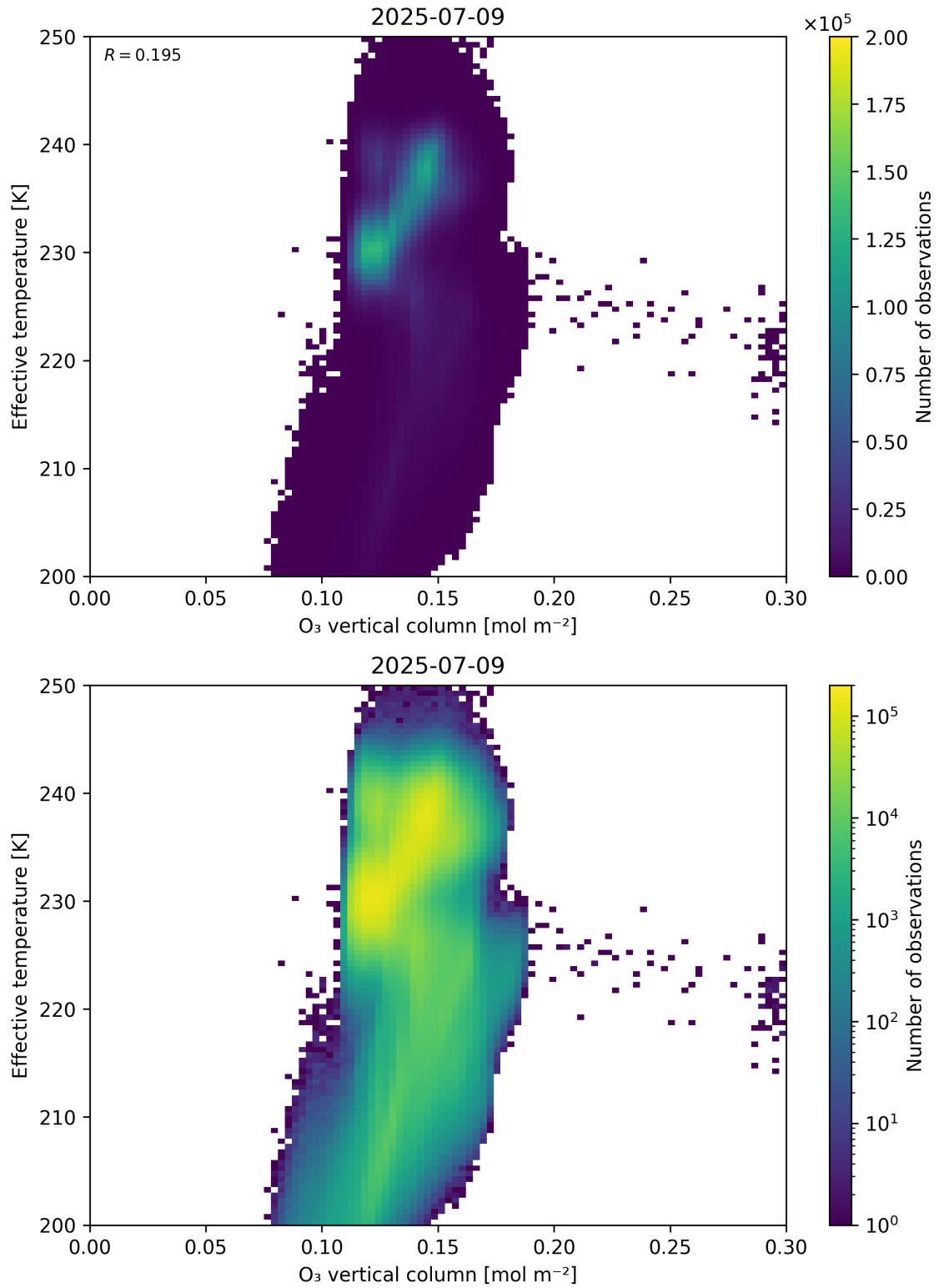
Figure 39: Scatter density plot of “O 3 vertical column” against “Effective temperature” for 2025-07-08 to 2025-07-10.
