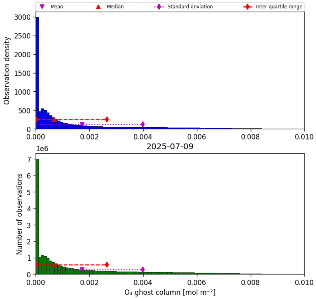
Figure 25: Histogram of “O 3 ghost column” for 2025-07-08 to 2025-07-10
