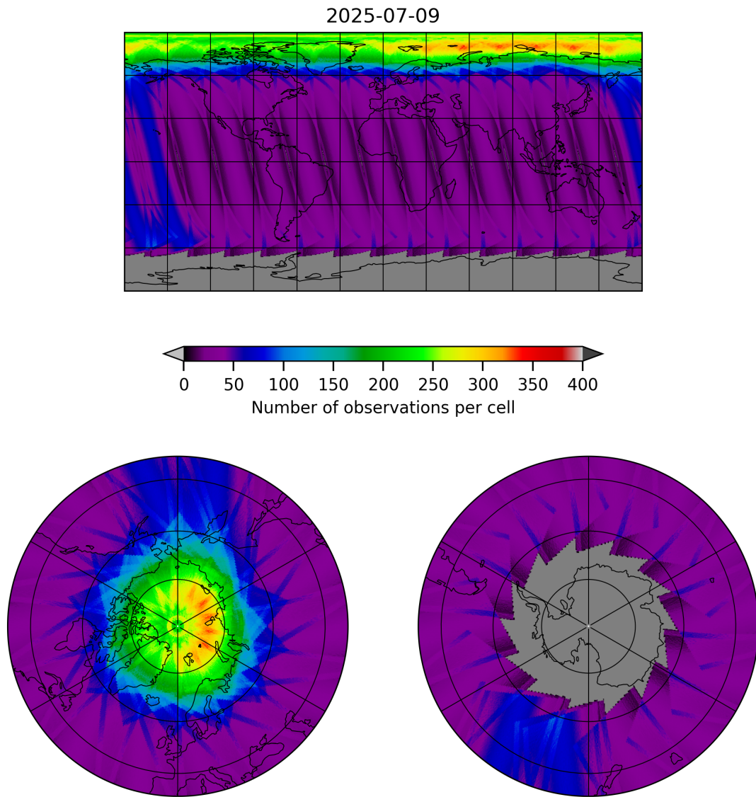
Figure 12: Map of the number of observations for 2025-07-08 to 2025-07-10
