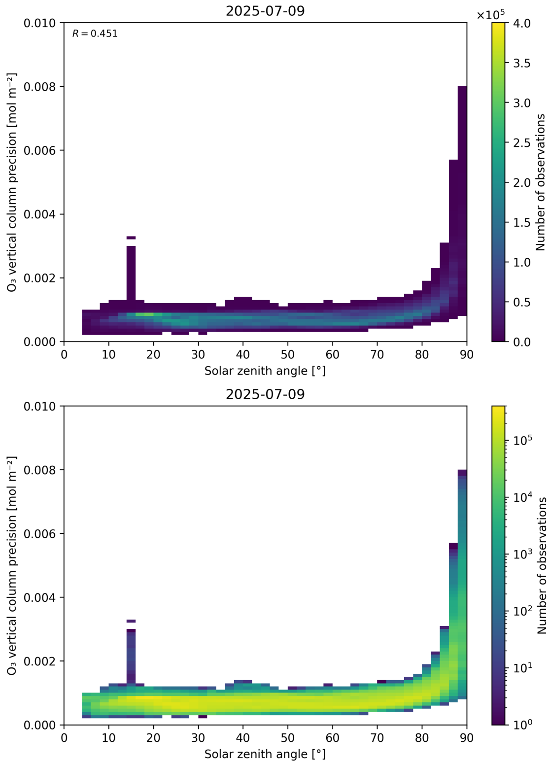
Figure 48: Scatter density plot of “Solar zenith angle” against “O 3 vertical column precision” for 2025-07-08 to 2025-07-10.
