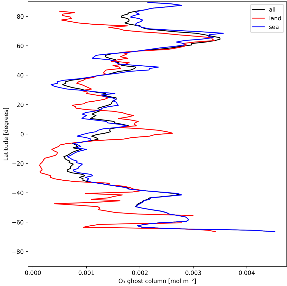
Figure 18: Zonal average of "O 3 ghost column" for 2025-07-08 to 2025-07-10.
