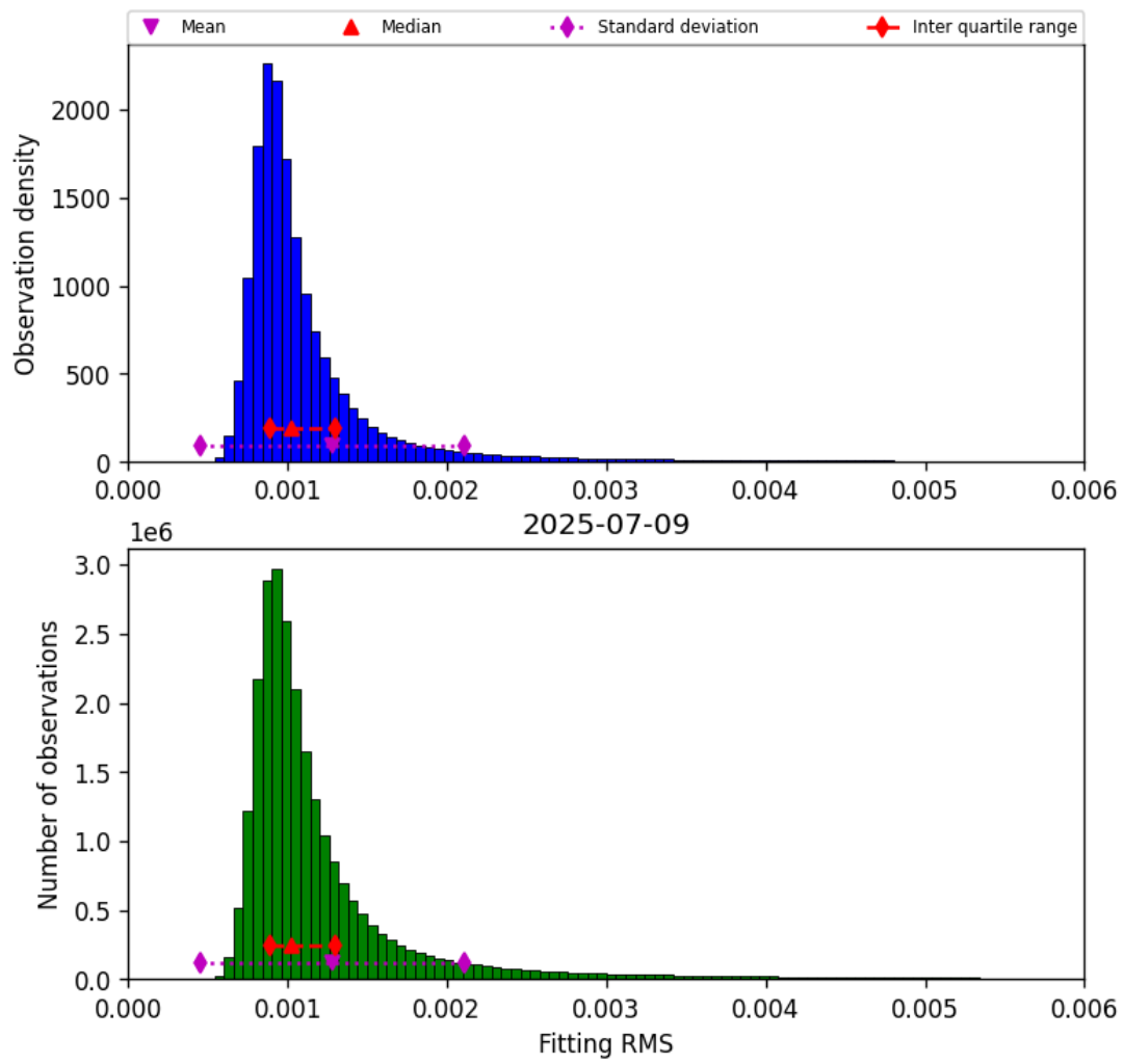
Figure 23: Histogram of “Fitting RMS” for 2025-07-08 to 2025-07-10
