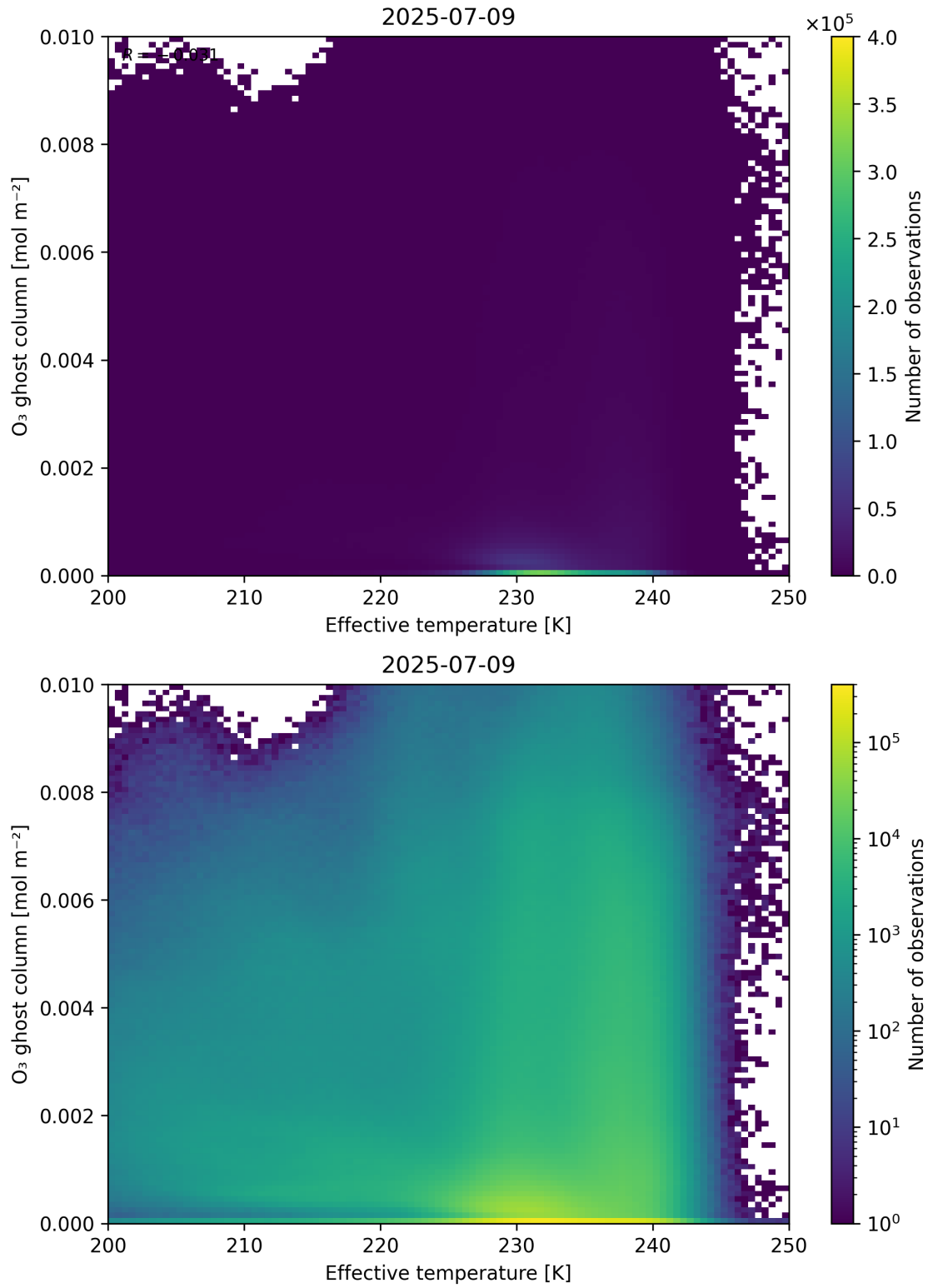
Figure 38: Scatter density plot of “Effective temperature” against “O 3 ghost column” for 2025-07-08 to 2025-07-10.
