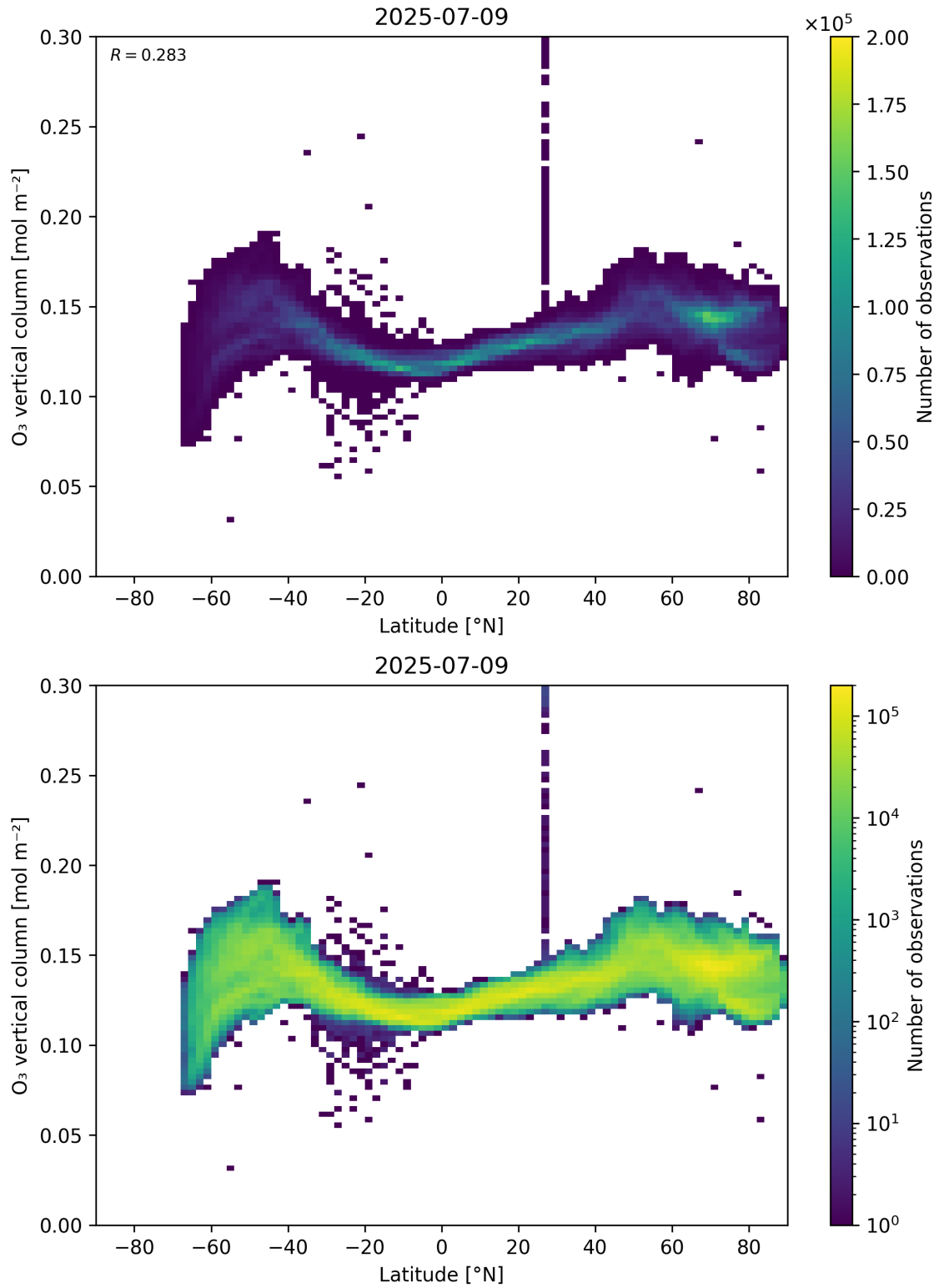
Figure 36: Scatter density plot of “Latitude” against “O 3 vertical column” for 2025-07-08 to 2025-07-10.
