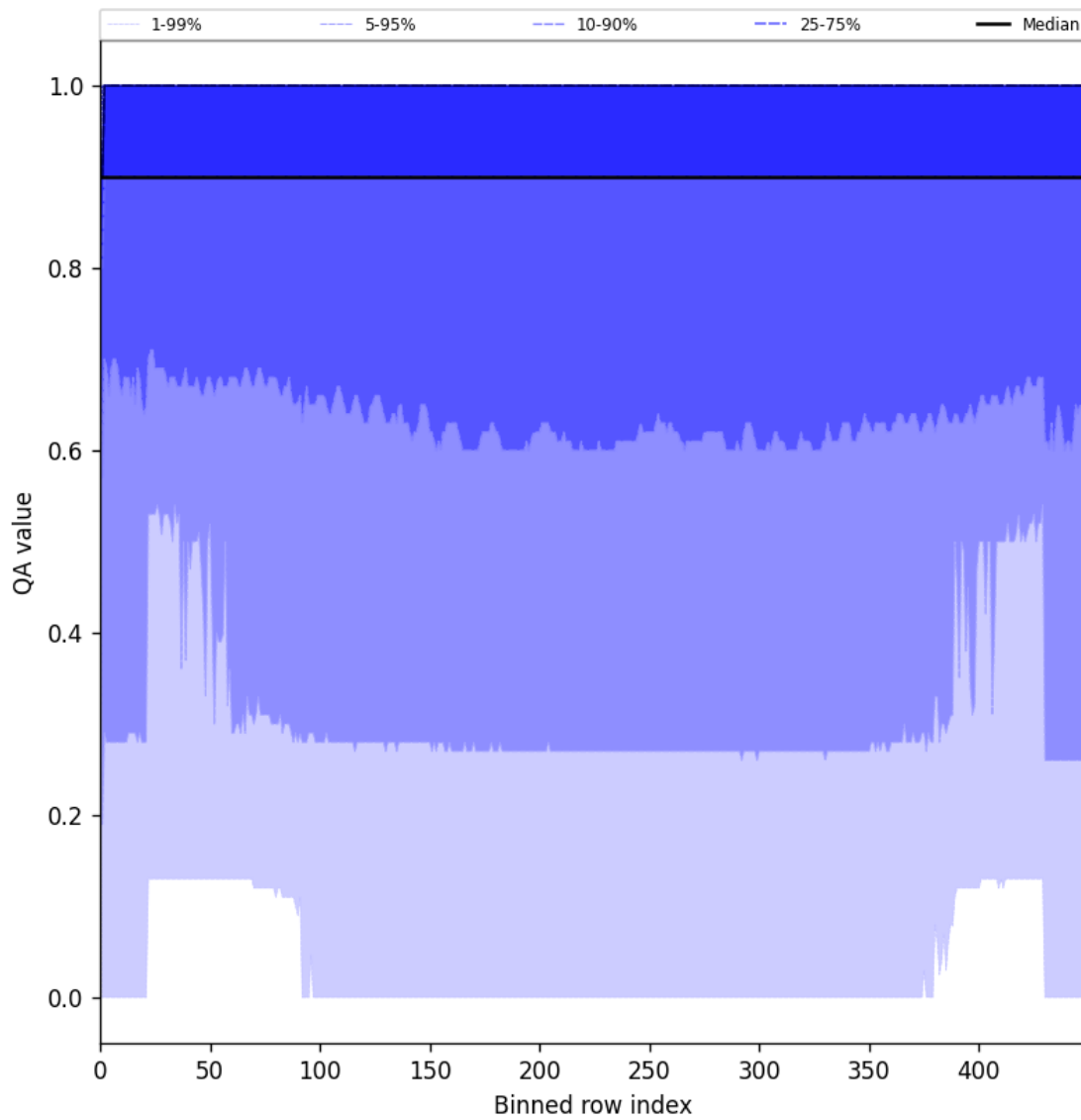
Figure 27: Along track statistics of “QA value” for 2025-07-08 to 2025-07-10
