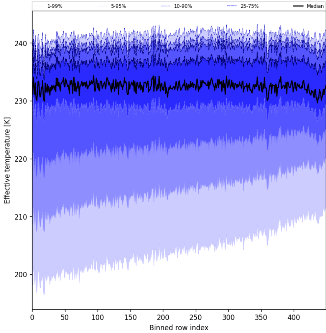
Figure 31: Along track statistics of “Effective temperature” for 2025-07-08 to 2025-07-10
