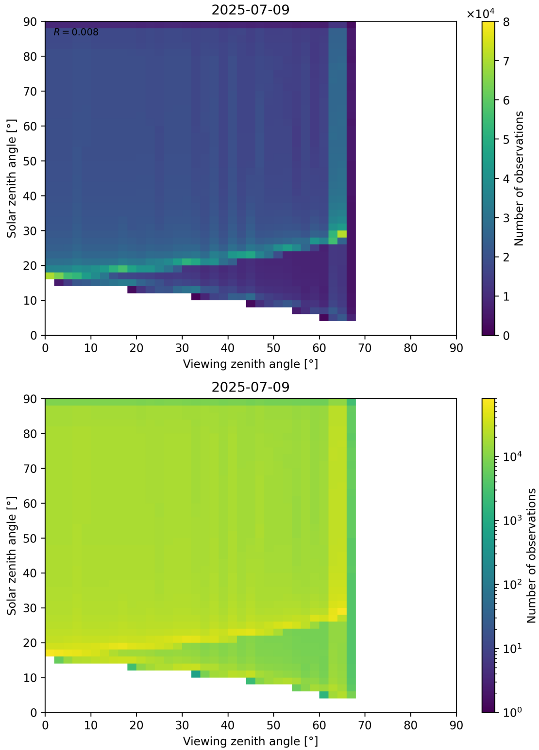
Figure 54: Scatter density plot of “Viewing zenith angle” against “Solar zenith angle” for 2025-07-08 to 2025-07-10.
