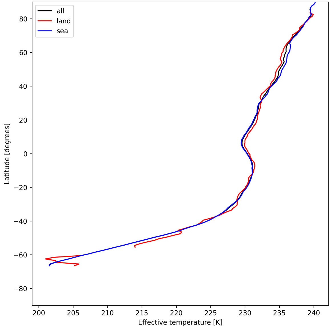
Figure 17: Zonal average of "Effective temperature" for 2025-07-08 to 2025-07-10.
