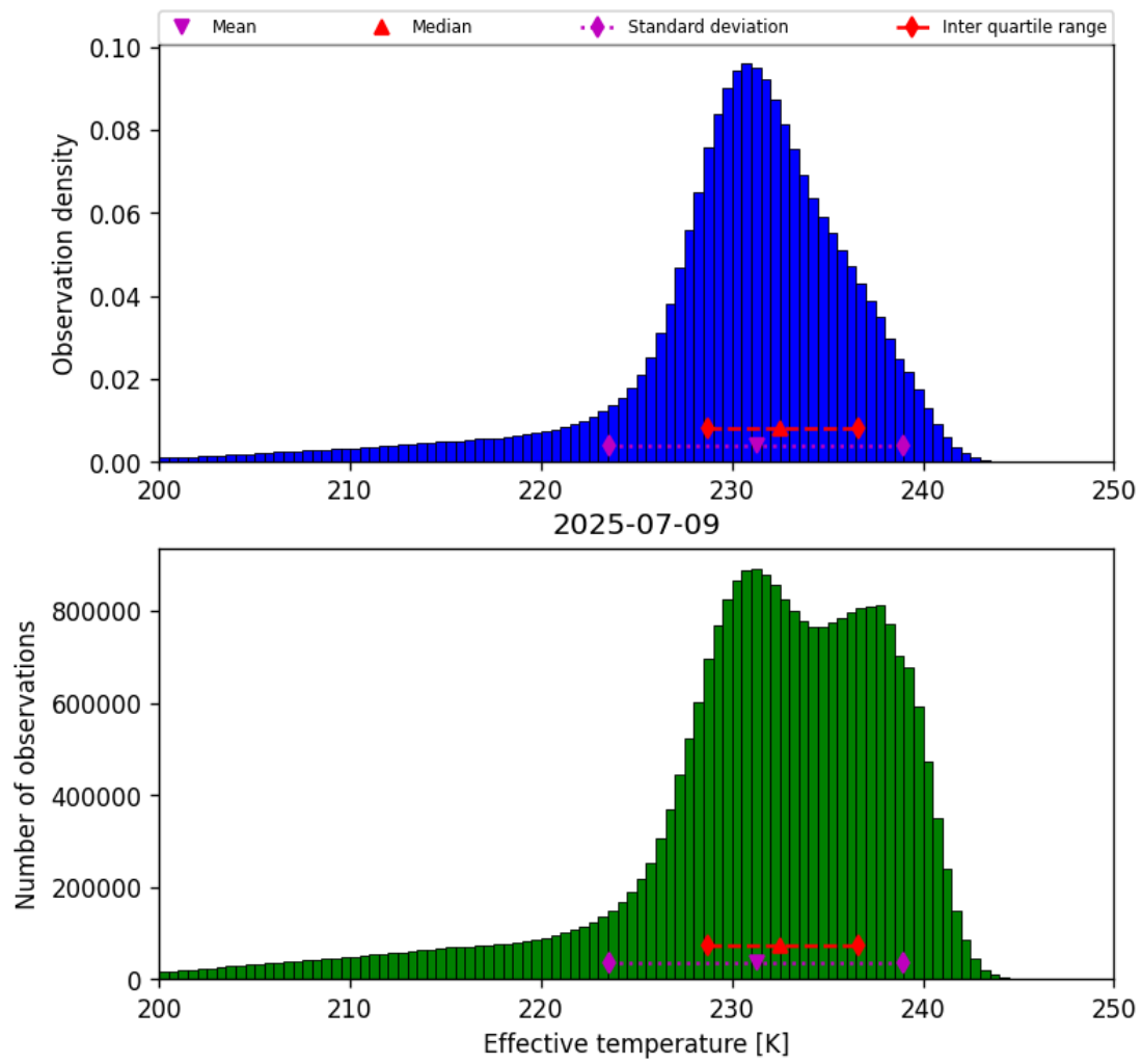
Figure 24: Histogram of “Effective temperature” for 2025-07-08 to 2025-07-10
