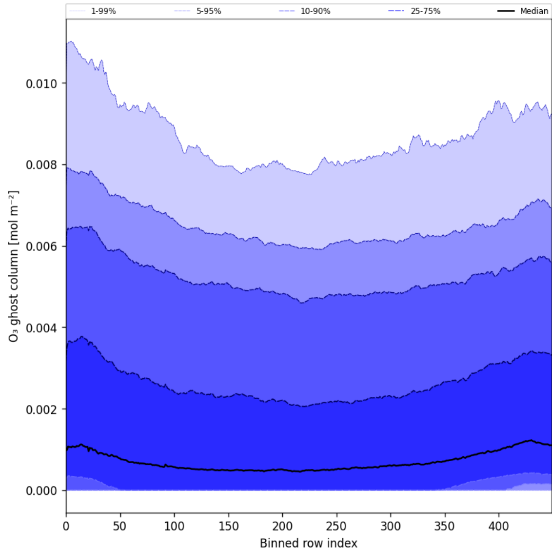
Figure 32: Along track statistics of “O 3 ghost column” for 2025-07-08 to 2025-07-10
