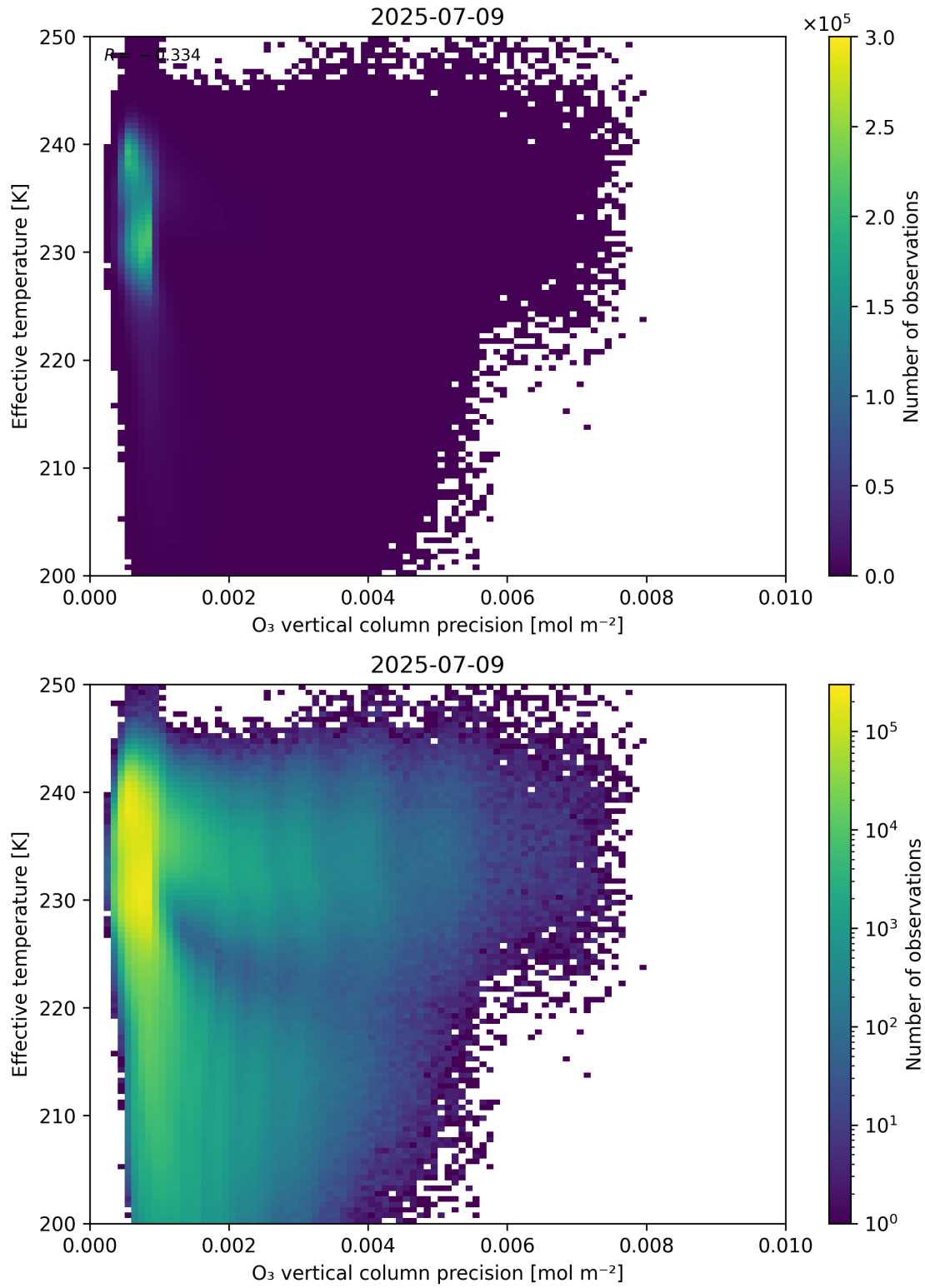
Figure 42: Scatter density plot of “O 3 vertical column precision” against “Effective temperature” for 2025-07-08 to 2025-07-10.
