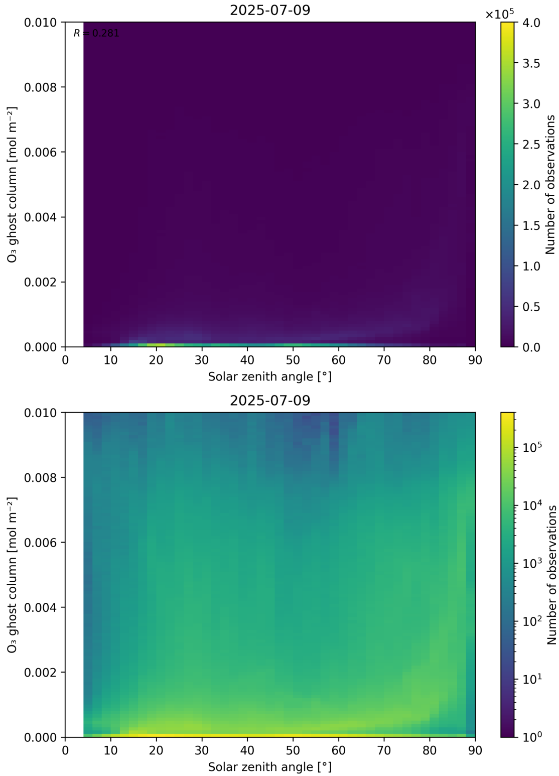
Figure 46: Scatter density plot of “Solar zenith angle” against “O 3 ghost column” for 2025-07-08 to 2025-07-10.
