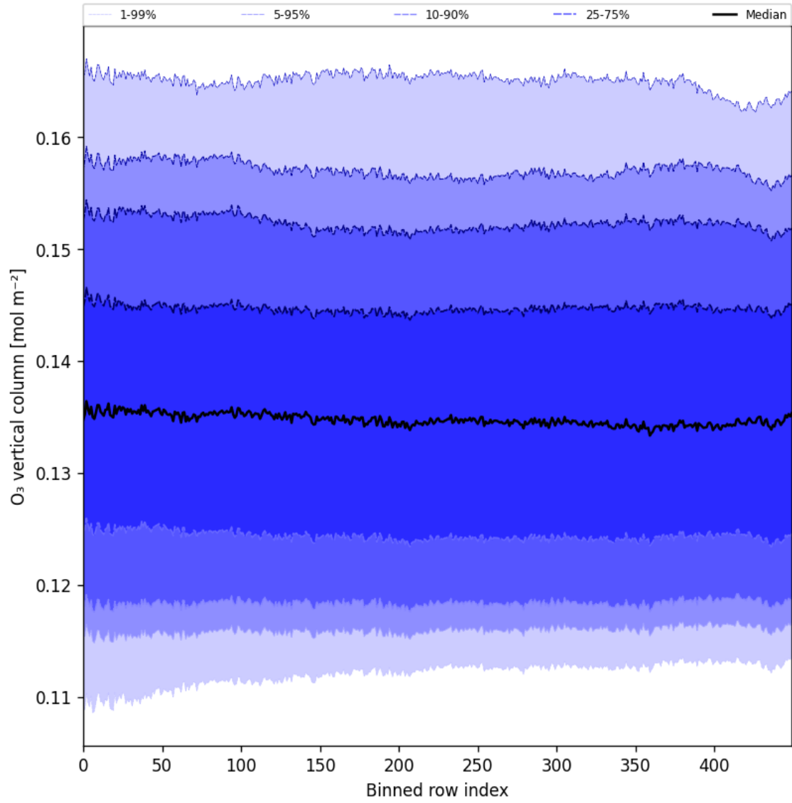
Figure 28: Along track statistics of “O 3 vertical column” for 2025-07-08 to 2025-07-10
