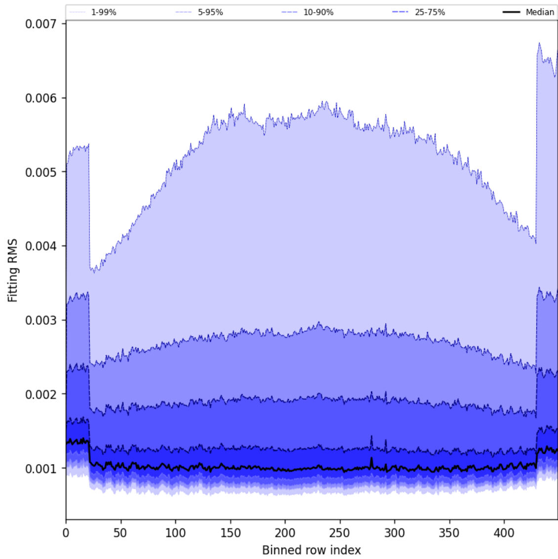
Figure 30: Along track statistics of “Fitting RMS” for 2025-07-08 to 2025-07-10
