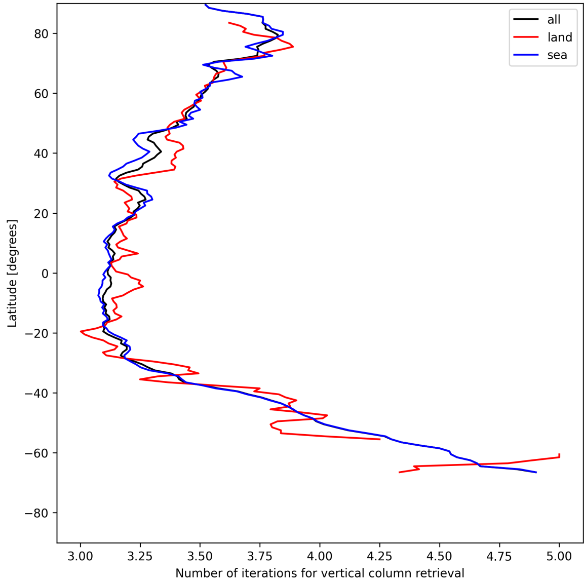
Figure 19: Zonal average of “Number of iterations for vertical column retrieval” for 2025-07-08 to 2025-07-10.
