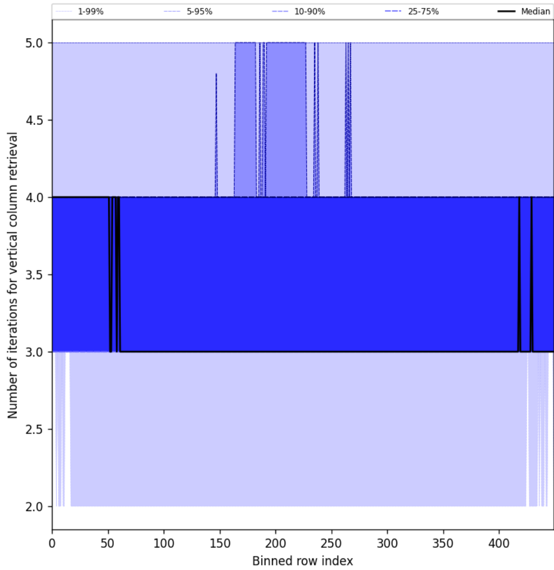
Figure 33: Along track statistics of “Number of iterations for vertical column retrieval” for 2025-07-08 to 2025-07-10
