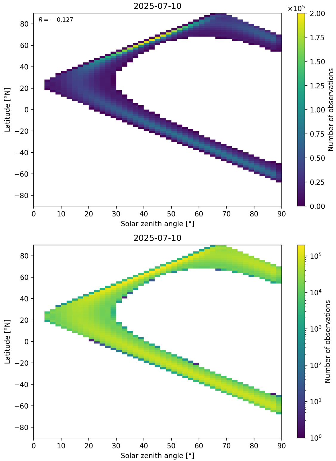
Figure 44: Scatter density plot of “Solar zenith angle” against “Latitude” for 2025-07-09 to 2025-07-11.
