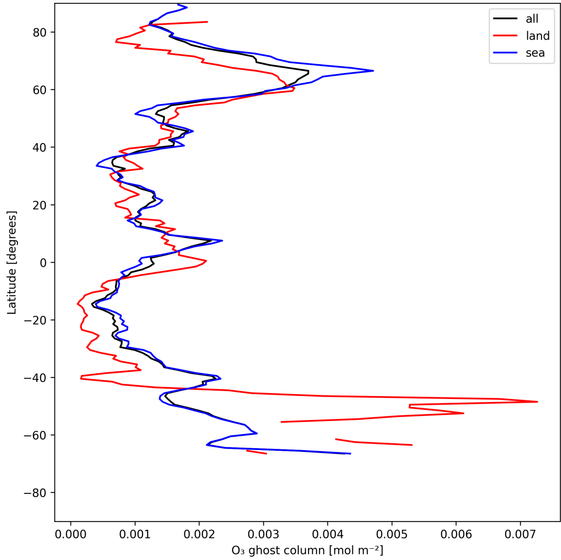
Figure 18: Zonal average of "O 3 ghost column" for 2025-07-09 to 2025-07-11.
