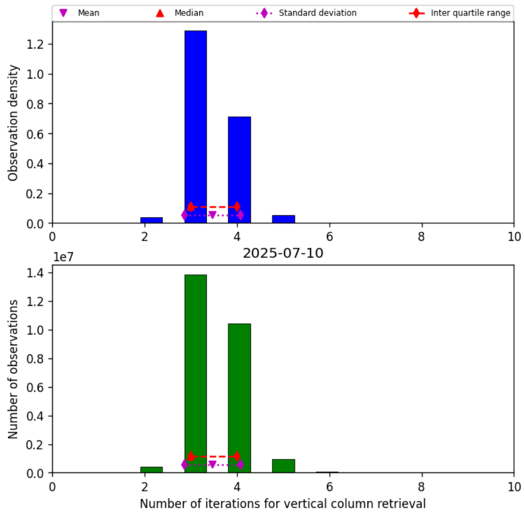
Figure 26: Histogram of “Number of iterations for vertical column retrieval” for 2025-07-09 to 2025-07-11
