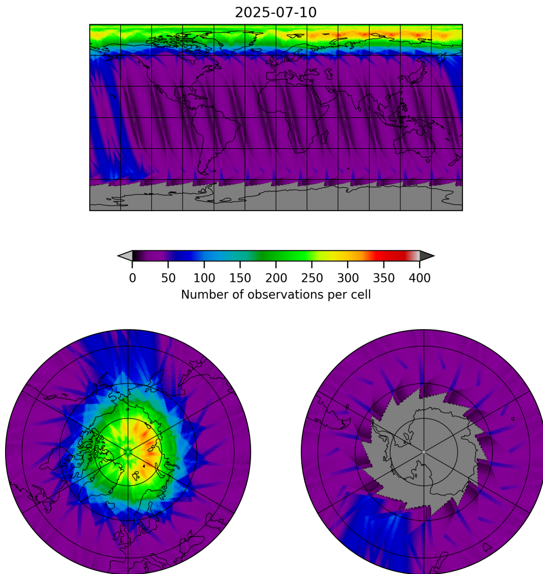
Figure 12: Map of the number of observations for 2025-07-09 to 2025-07-11
