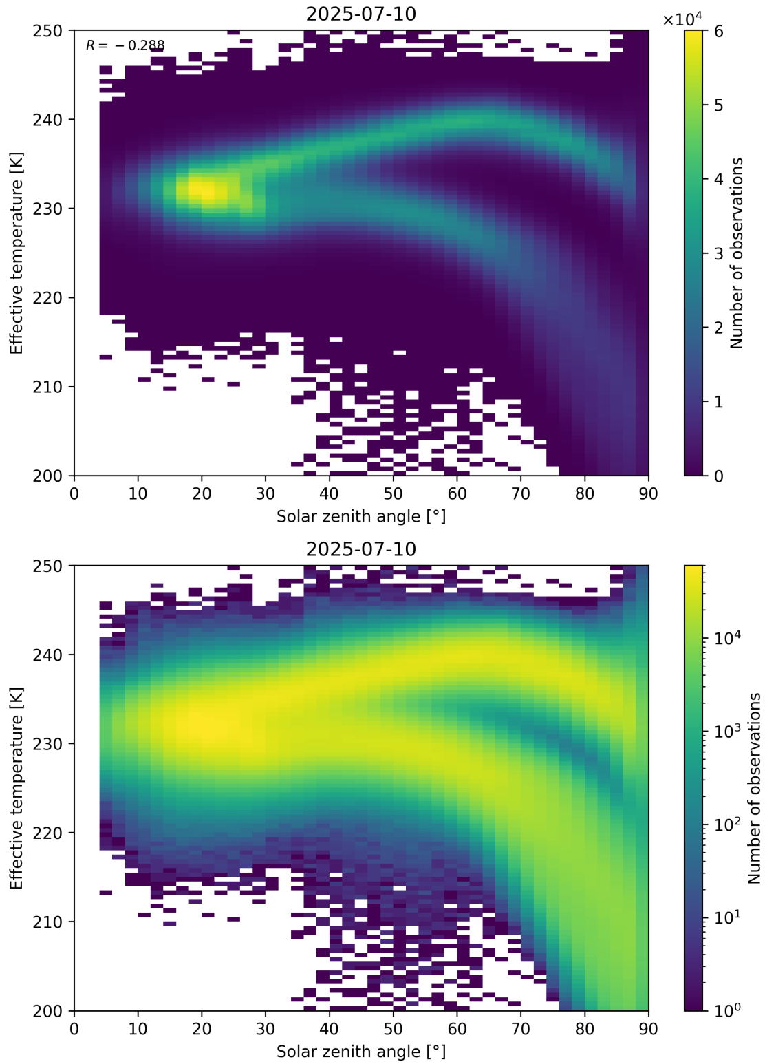
Figure 45: Scatter density plot of “Solar zenith angle” against “Effective temperature” for 2025-07-09 to 2025-07-11.
