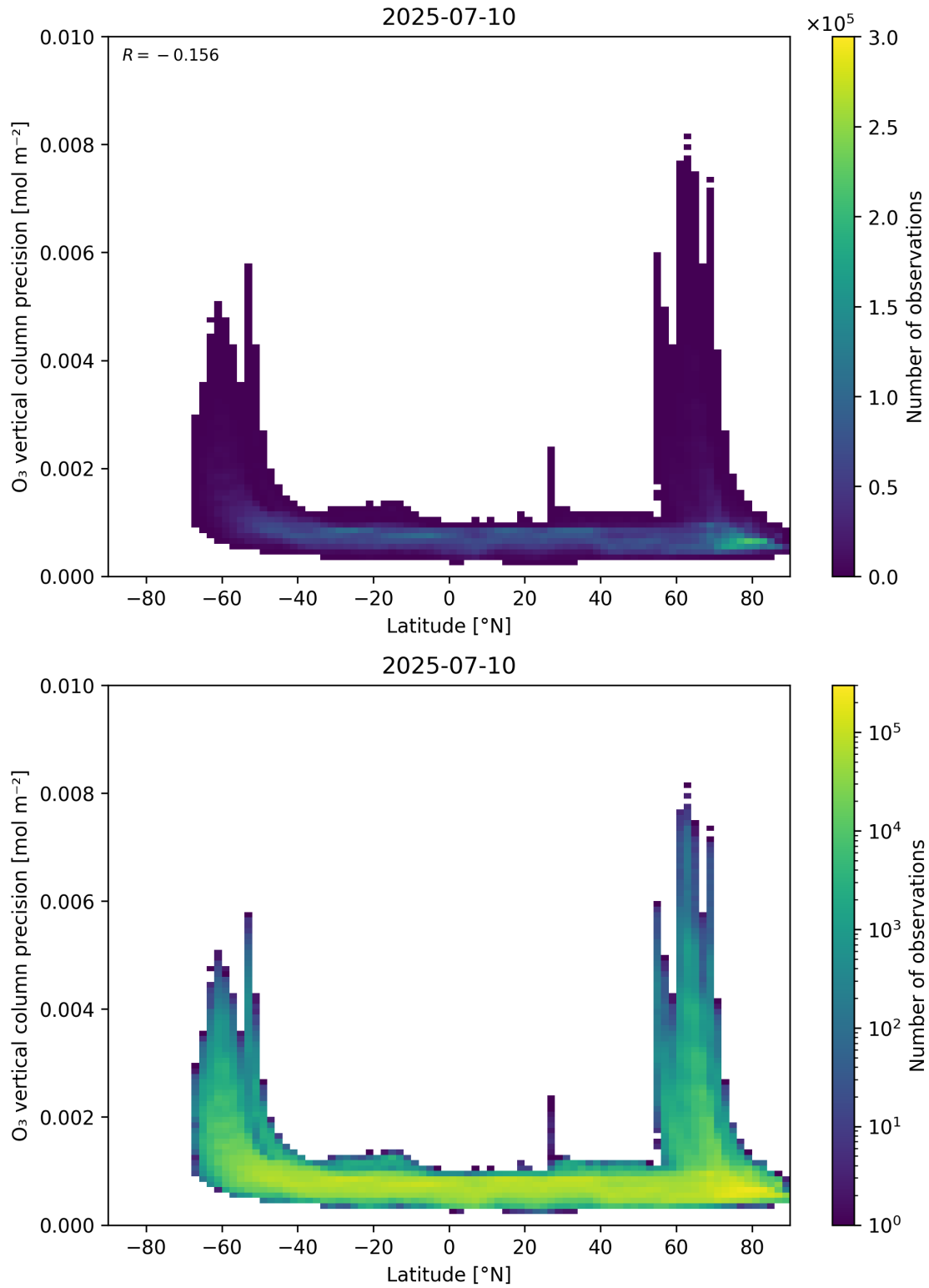
Figure 37: Scatter density plot of “Latitude” against “O 3 vertical column precision” for 2025-07-09 to 2025-07-11.
