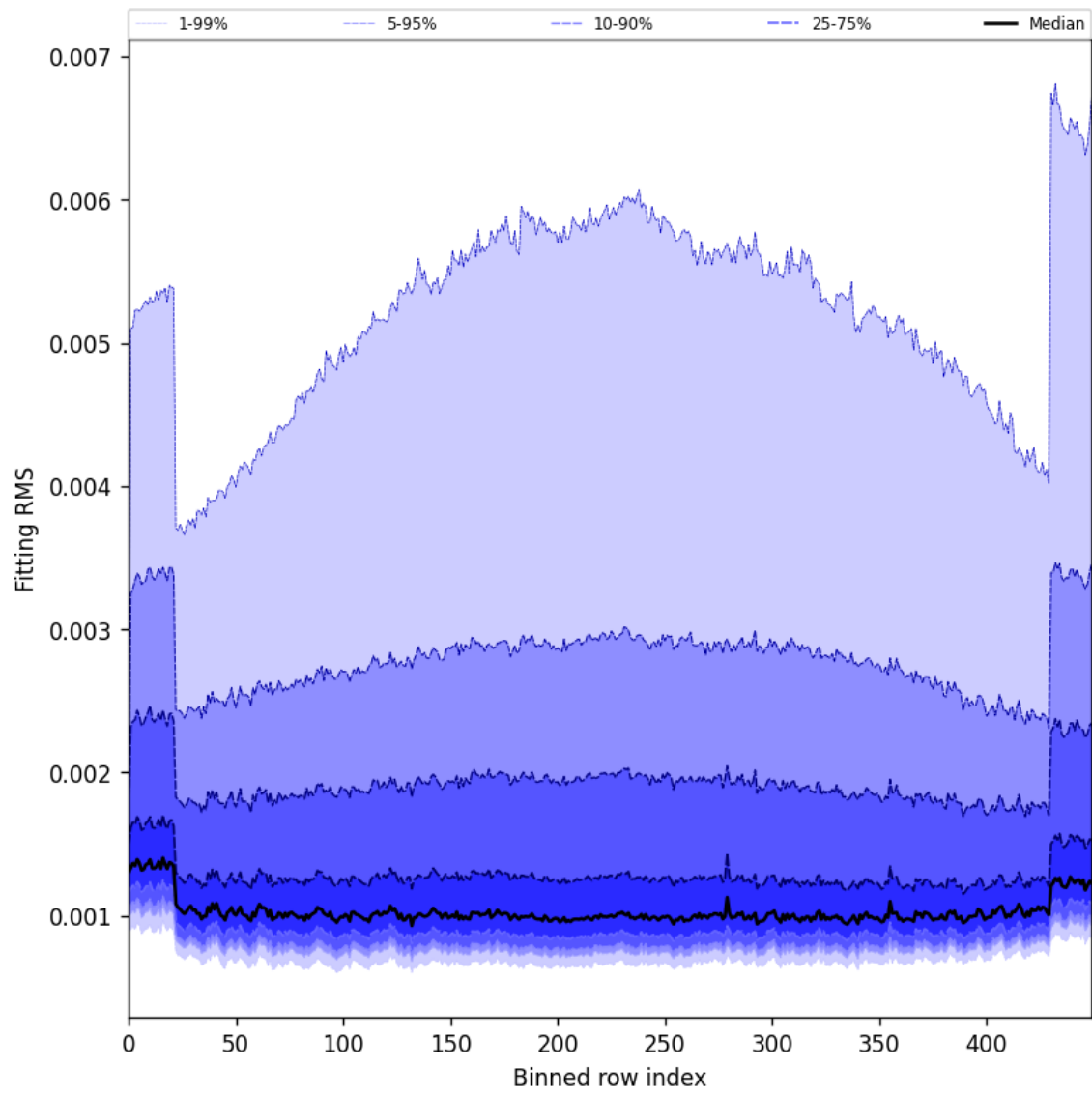
Figure 30: Along track statistics of “Fitting RMS” for 2025-07-09 to 2025-07-11
