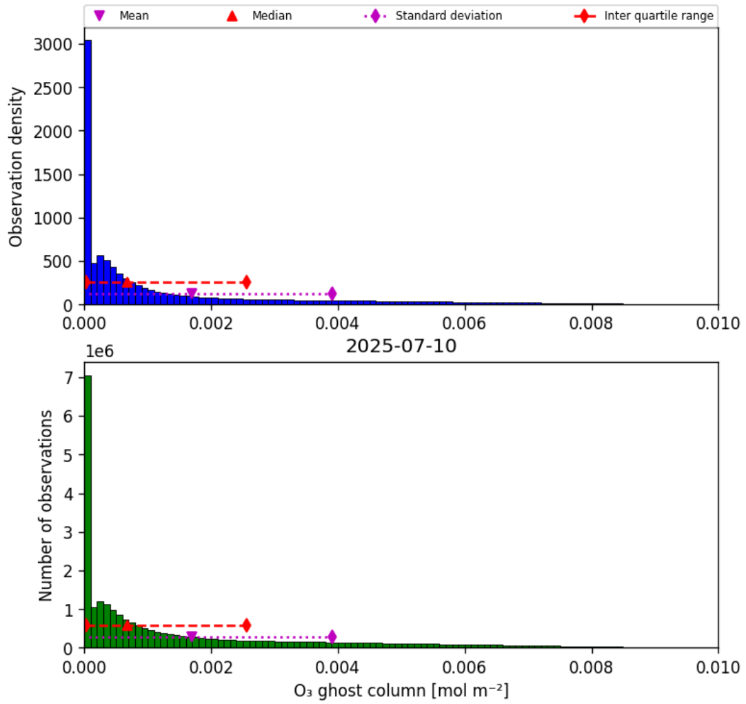
Figure 25: Histogram of “O 3 ghost column” for 2025-07-09 to 2025-07-11
