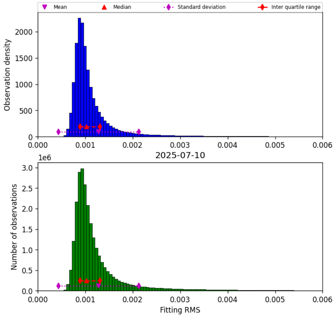
Figure 23: Histogram of “Fitting RMS” for 2025-07-09 to 2025-07-11
