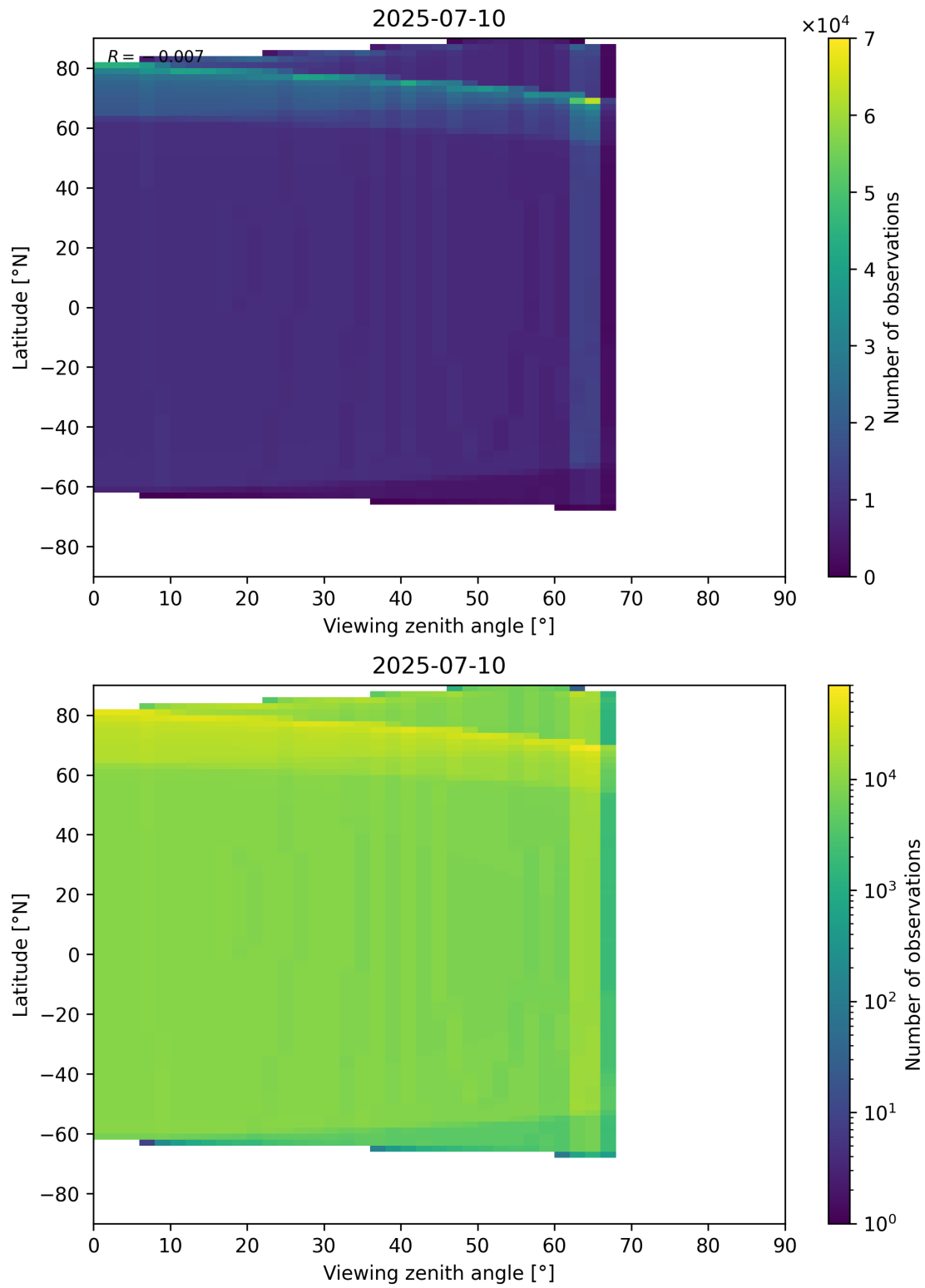
Figure 49: Scatter density plot of “Viewing zenith angle” against “Latitude” for 2025-07-09 to 2025-07-11.
