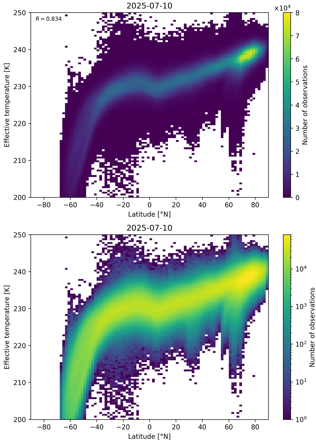
Figure 34: Scatter density plot of “Latitude” against “Effective temperature” for 2025-07-09 to 2025-07-11.
