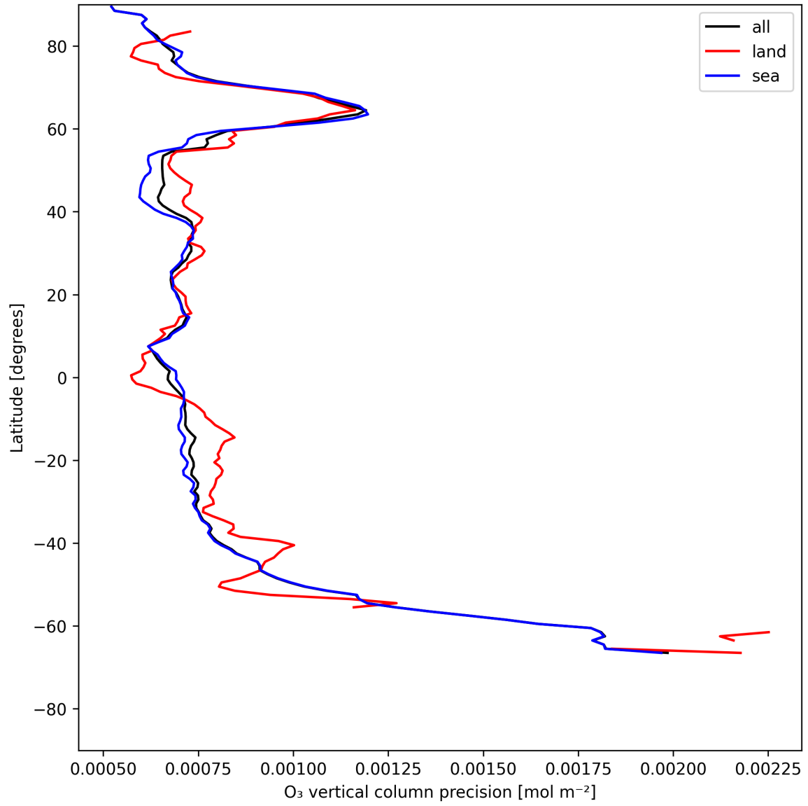
Figure 15: Zonal average of “O 3 vertical column precision” for 2025-07-09 to 2025-07-11.
