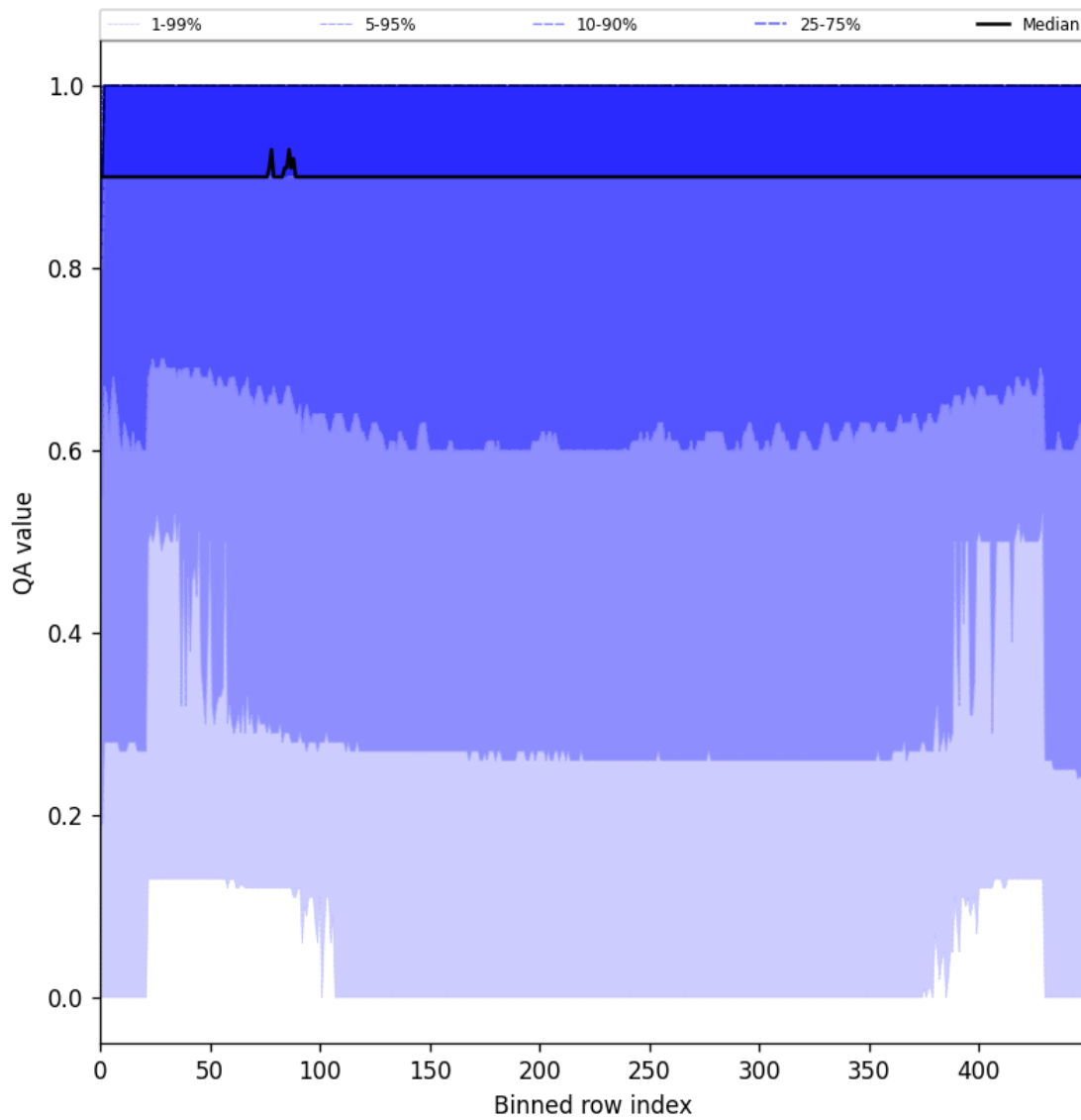
Figure 27: Along track statistics of “QA value” for 2025-07-09 to 2025-07-11
