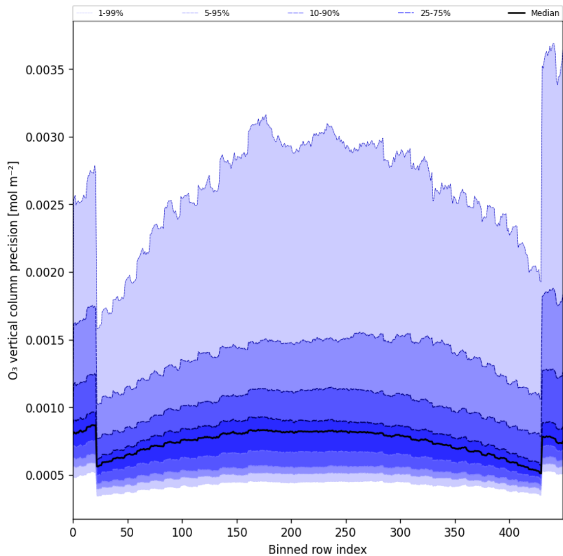
Figure 29: Along track statistics of “O 3 vertical column precision” for 2025-07-09 to 2025-07-11
