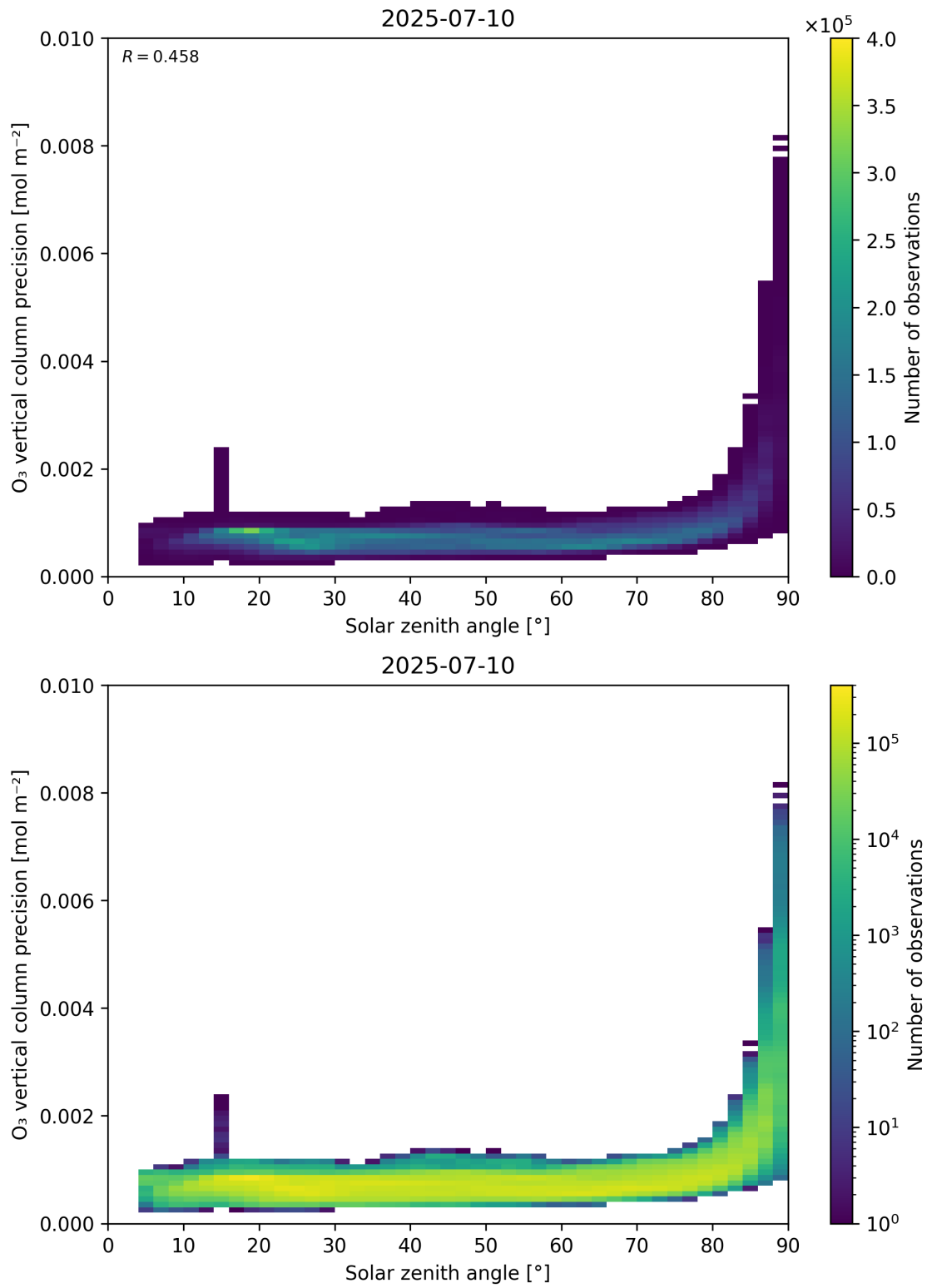
Figure 48: Scatter density plot of “Solar zenith angle” against “O 3 vertical column precision” for 2025-07-09 to 2025-07-11.
