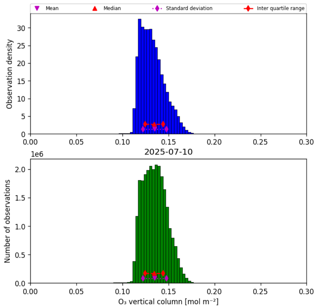
Figure 21: Histogram of “O 3 vertical column” for 2025-07-09 to 2025-07-11
