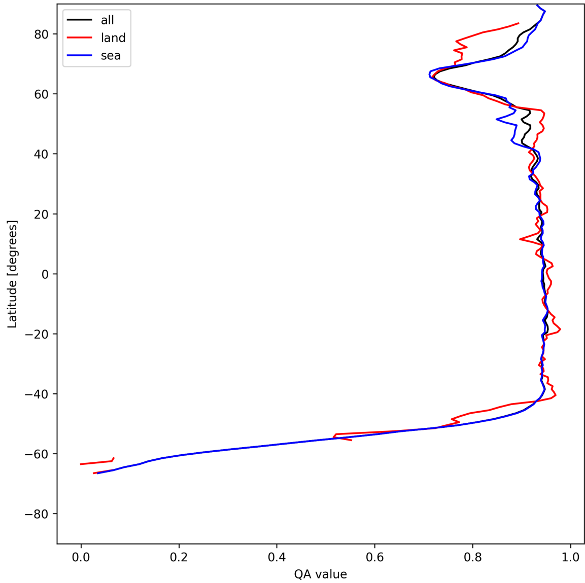
Figure 13: Zonal average of “QA value” for 2025-07-09 to 2025-07-11.
