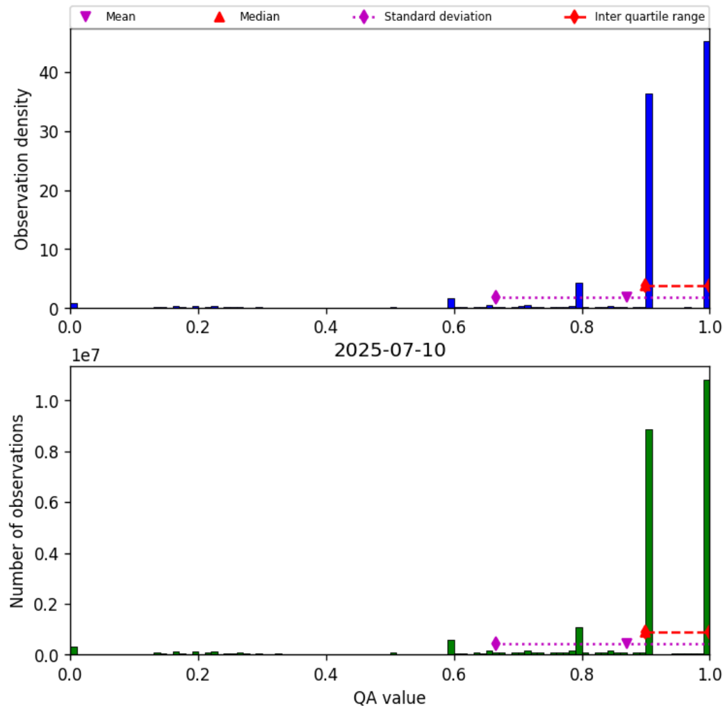
Figure 20: Histogram of “QA value” for 2025-07-09 to 2025-07-11
