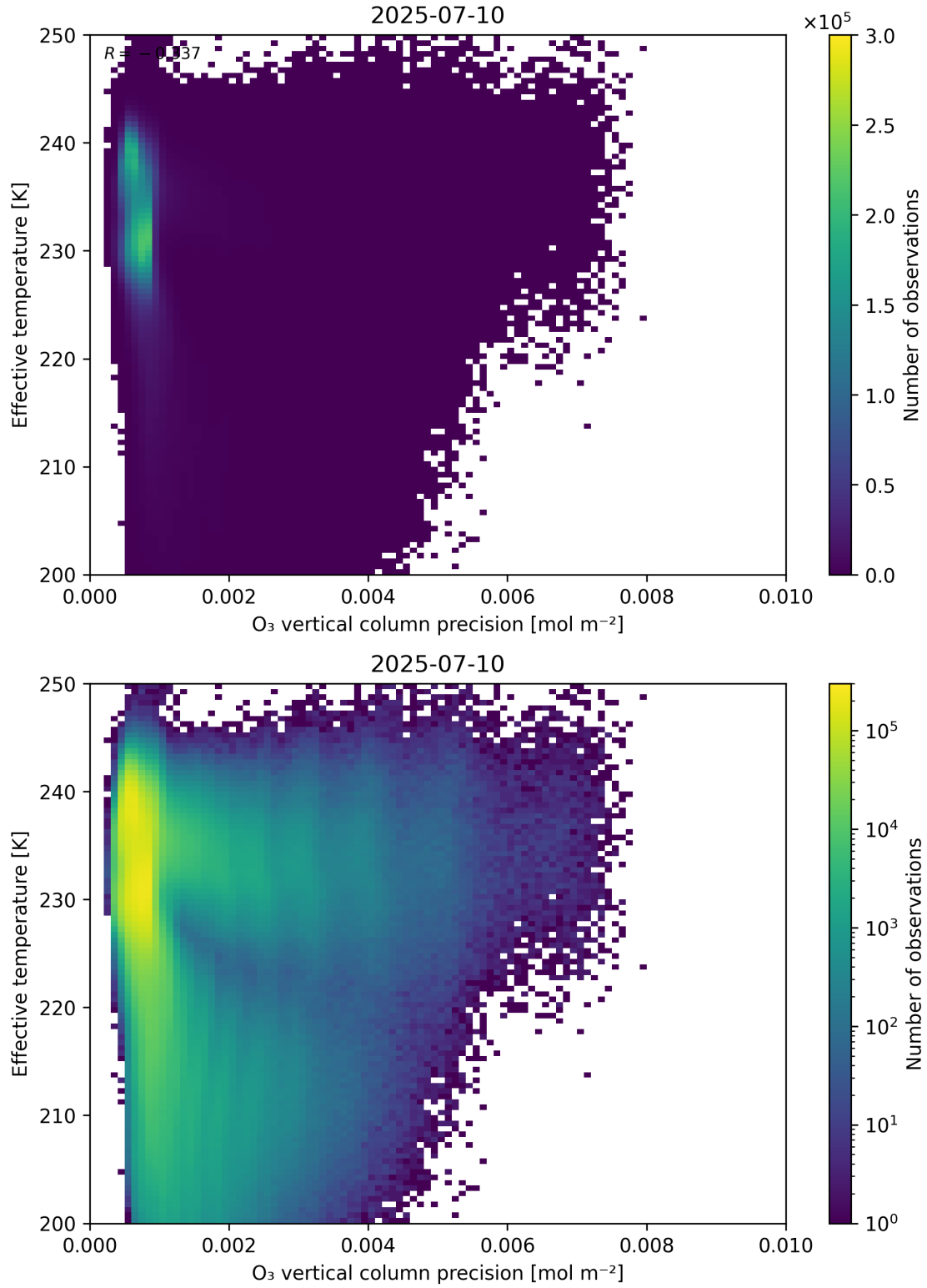
Figure 42: Scatter density plot of “O 3 vertical column precision” against “Effective temperature” for 2025-07-09 to 2025-07-11.
