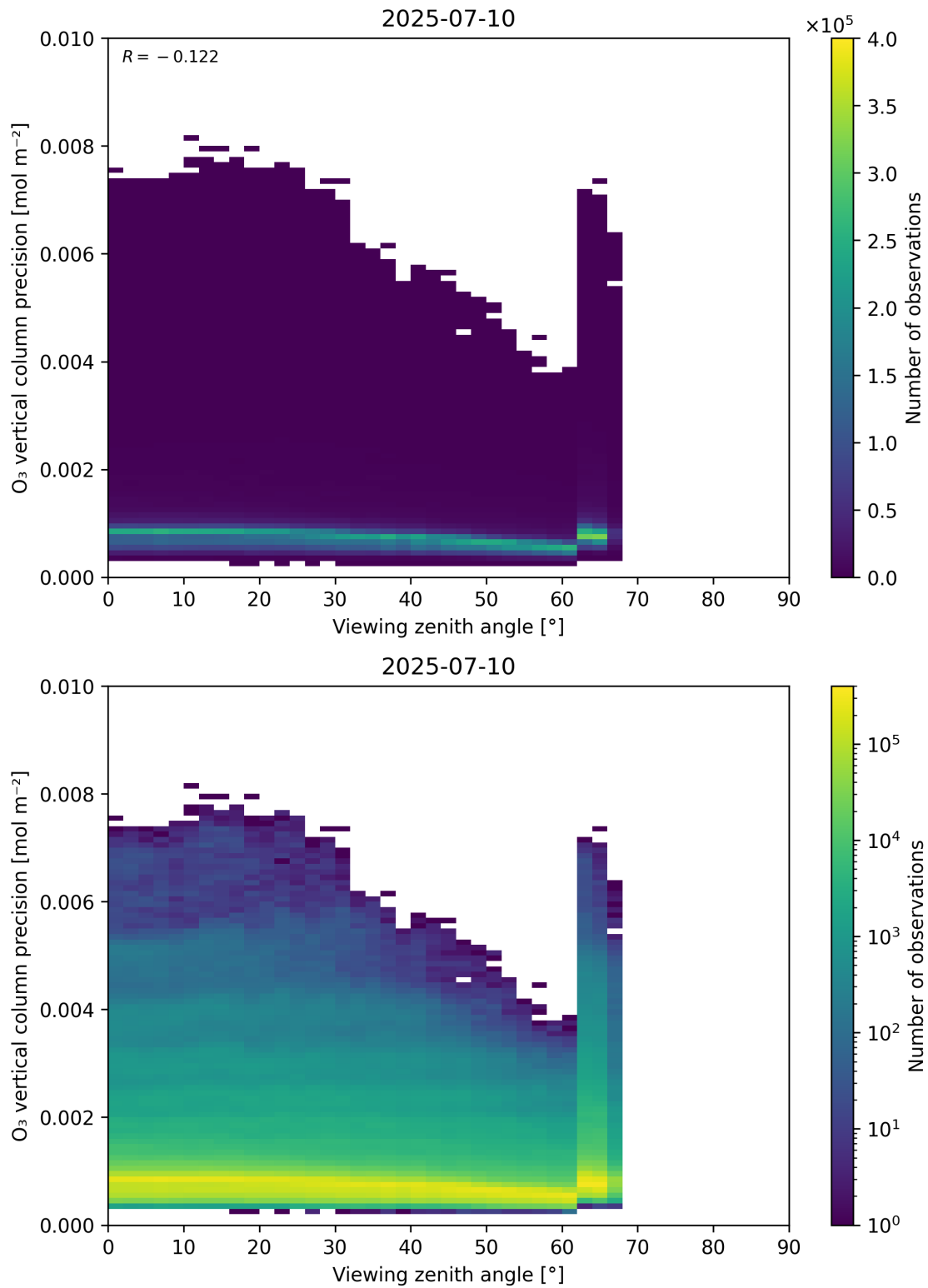
Figure 53: Scatter density plot of “Viewing zenith angle” against “O 3 vertical column precision” for 2025-07-09 to 2025-07-11.
