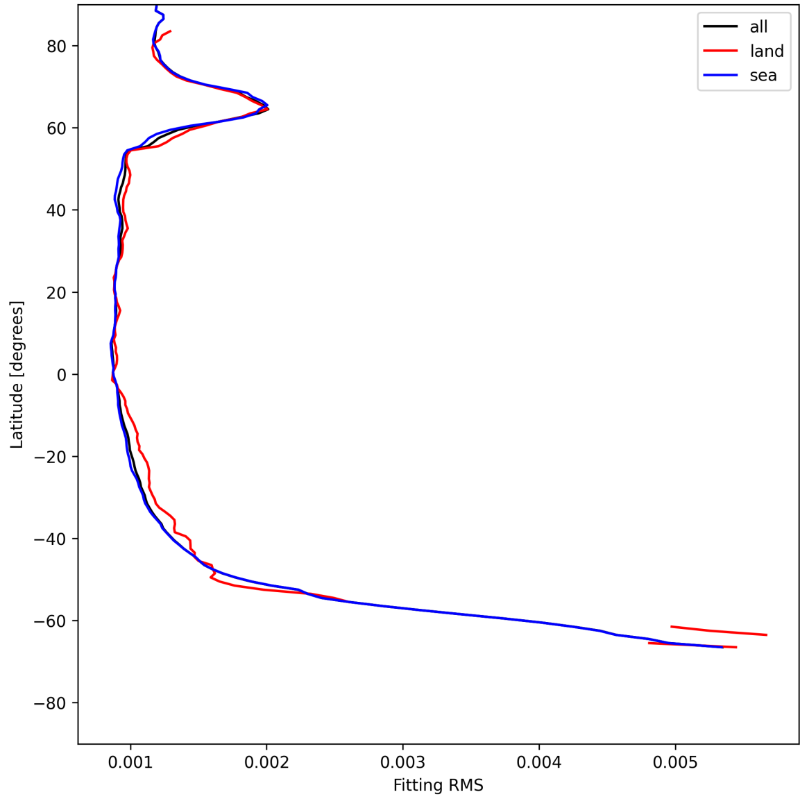
Figure 16: Zonal average of “Fitting RMS” for 2025-07-09 to 2025-07-11.
