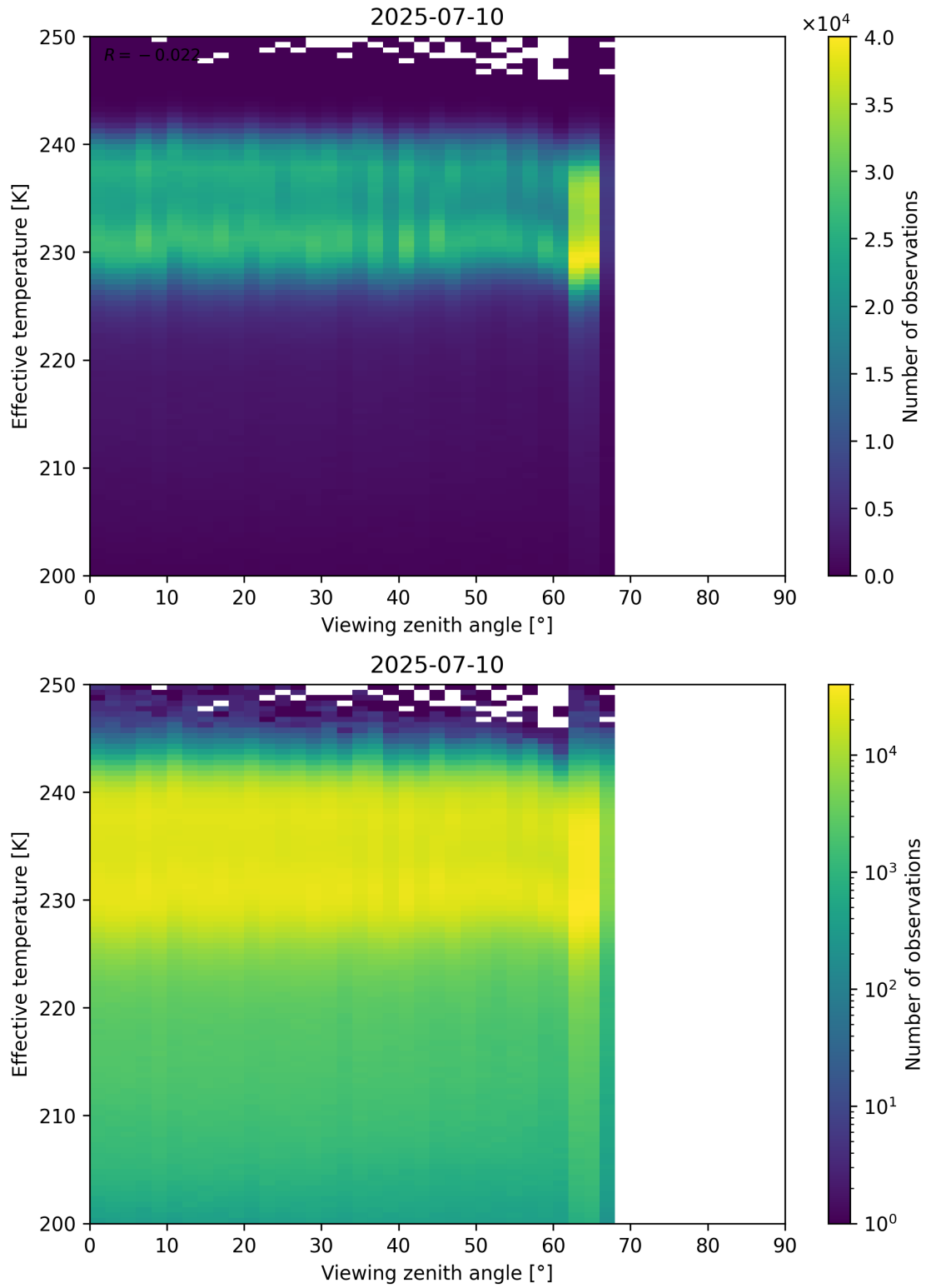
Figure 50: Scatter density plot of “Viewing zenith angle” against “Effective temperature” for 2025-07-09 to 2025-07-11.
