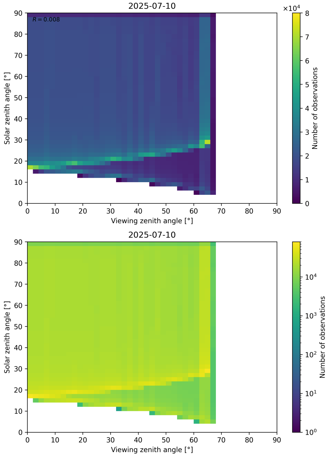
Figure 54: Scatter density plot of “Viewing zenith angle” against “Solar zenith angle” for 2025-07-09 to 2025-07-11.
