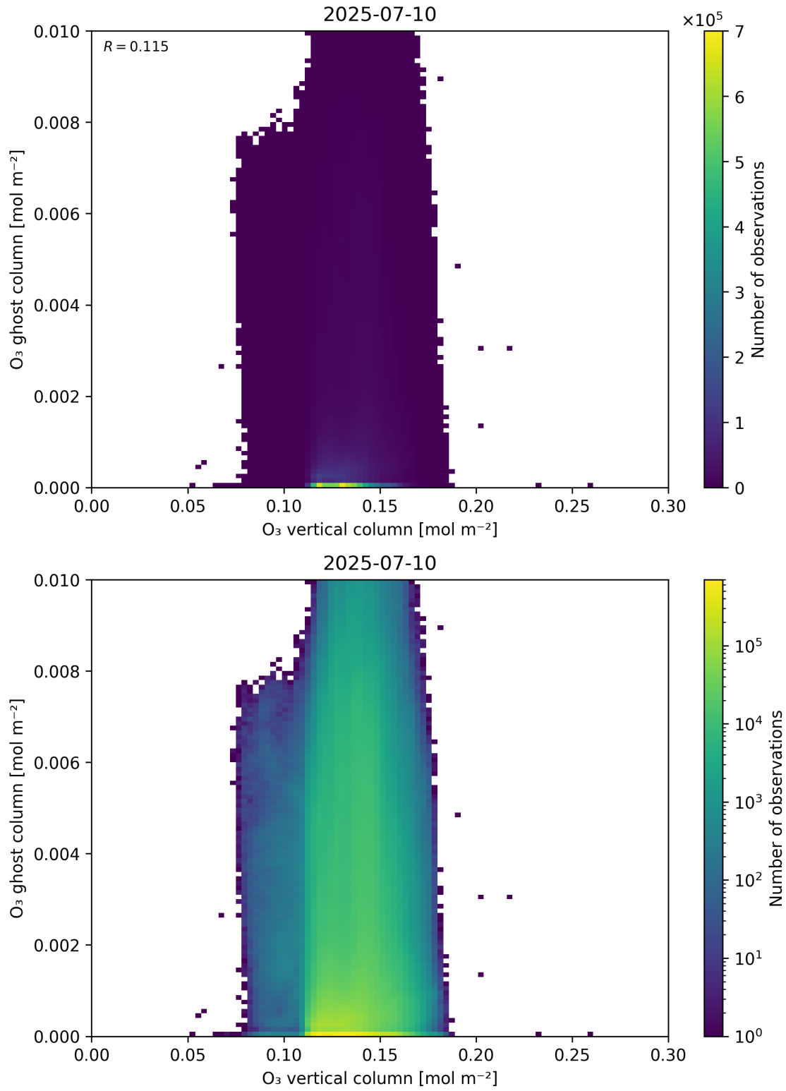
Figure 40: Scatter density plot of “O 3 vertical column” against “O 3 ghost column” for 2025-07-09 to 2025-07-11.
