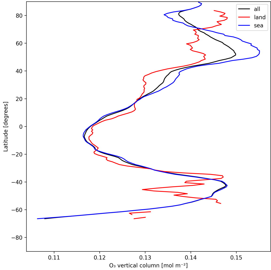
Figure 14: Zonal average of “O 3 vertical column” for 2025-07-09 to 2025-07-11.
