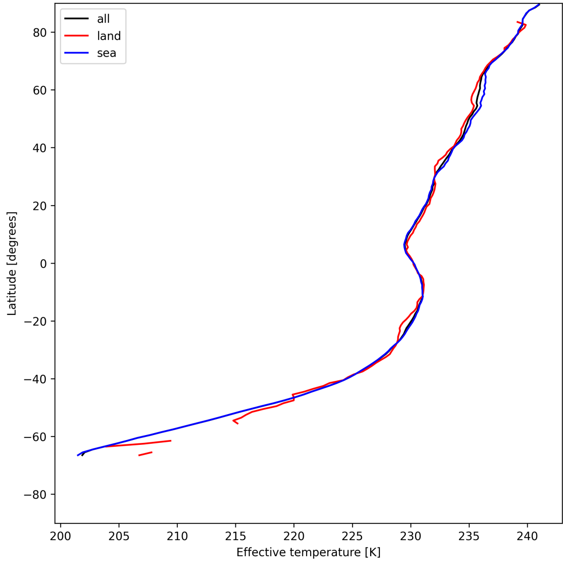
Figure 17: Zonal average of "Effective temperature" for 2025-07-09 to 2025-07-11.
