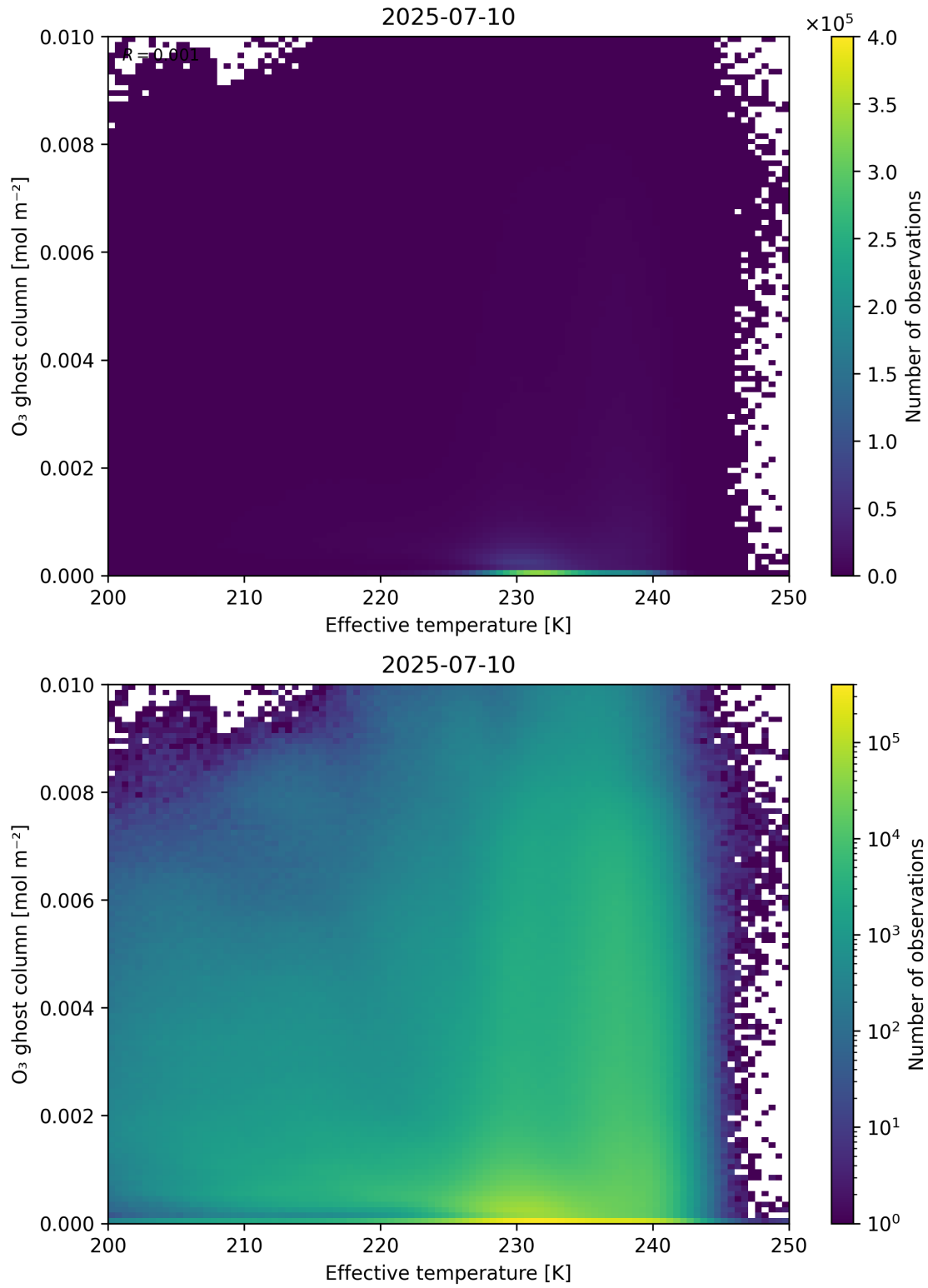
Figure 38: Scatter density plot of “Effective temperature” against “O 3 ghost column” for 2025-07-09 to 2025-07-11.
