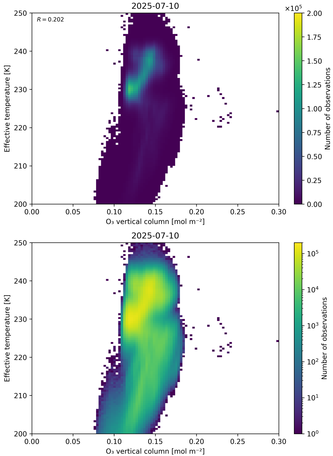
Figure 39: Scatter density plot of “O 3 vertical column” against “Effective temperature” for 2025-07-09 to 2025-07-11.
