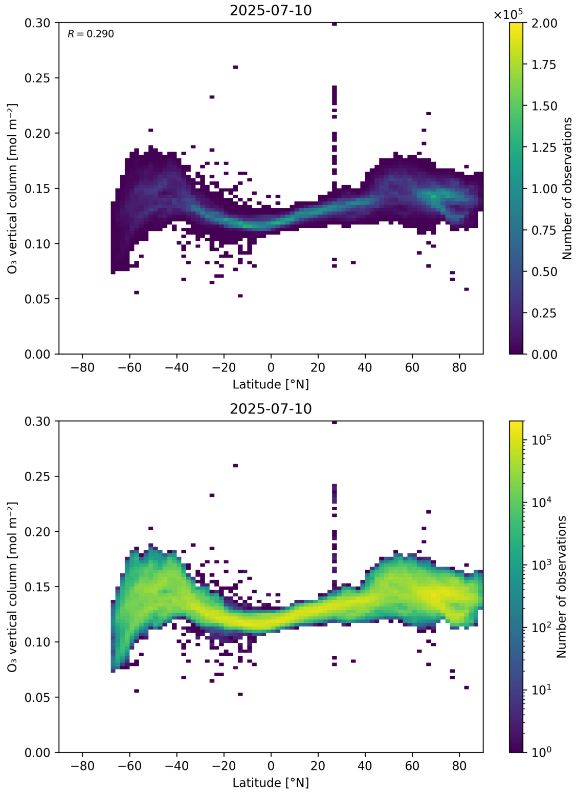
Figure 36: Scatter density plot of “Latitude” against “O 3 vertical column” for 2025-07-09 to 2025-07-11.
