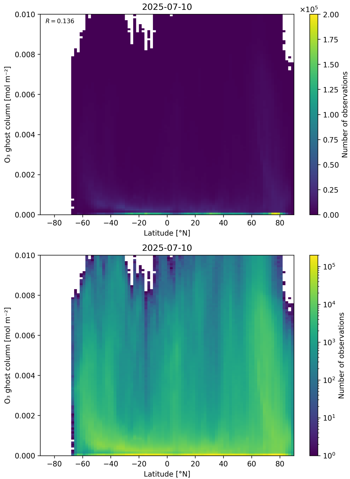
Figure 35: Scatter density plot of “Latitude” against “O 3 ghost column” for 2025-07-09 to 2025-07-11.
