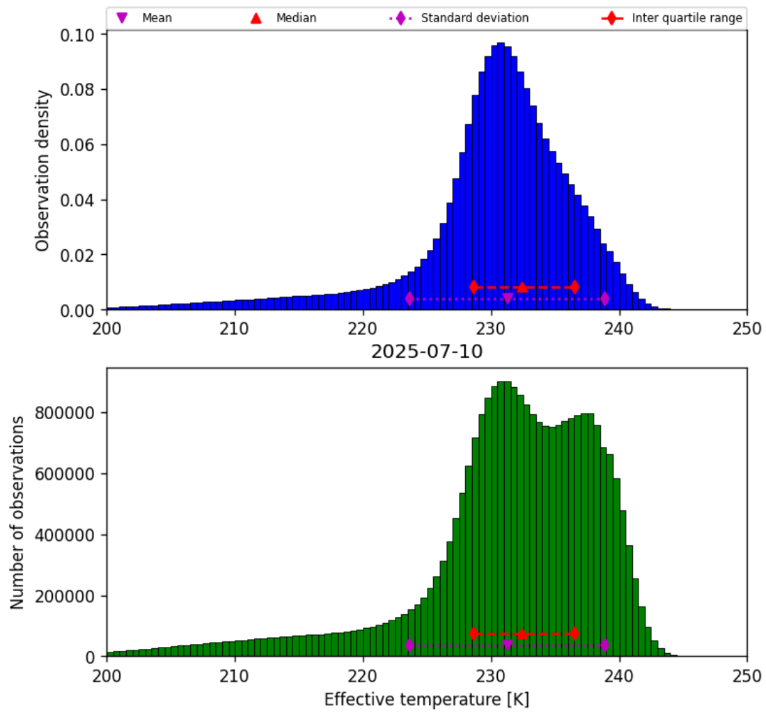
Figure 24: Histogram of “Effective temperature” for 2025-07-09 to 2025-07-11
