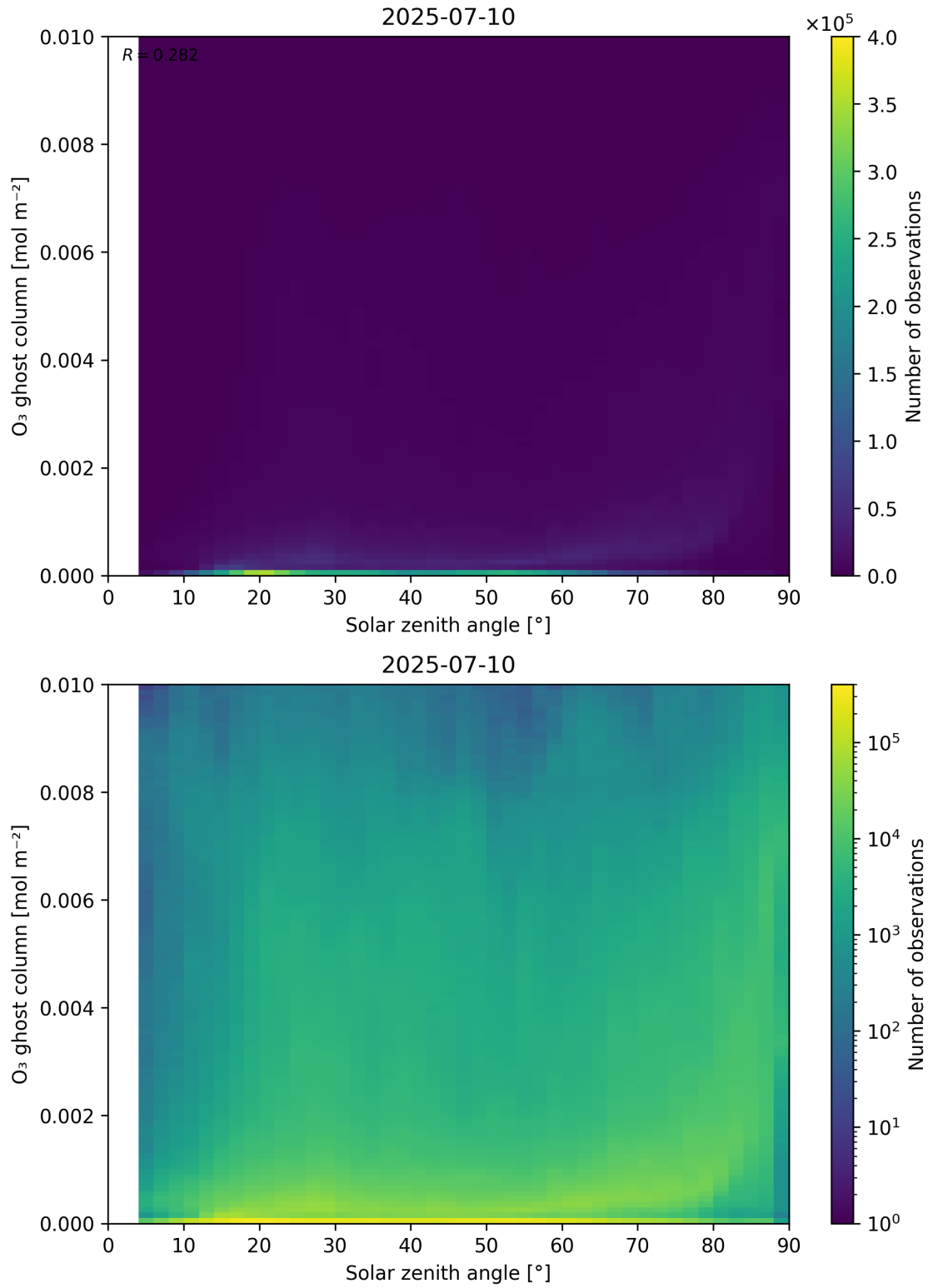
Figure 46: Scatter density plot of “Solar zenith angle” against “O 3 ghost column” for 2025-07-09 to 2025-07-11.
