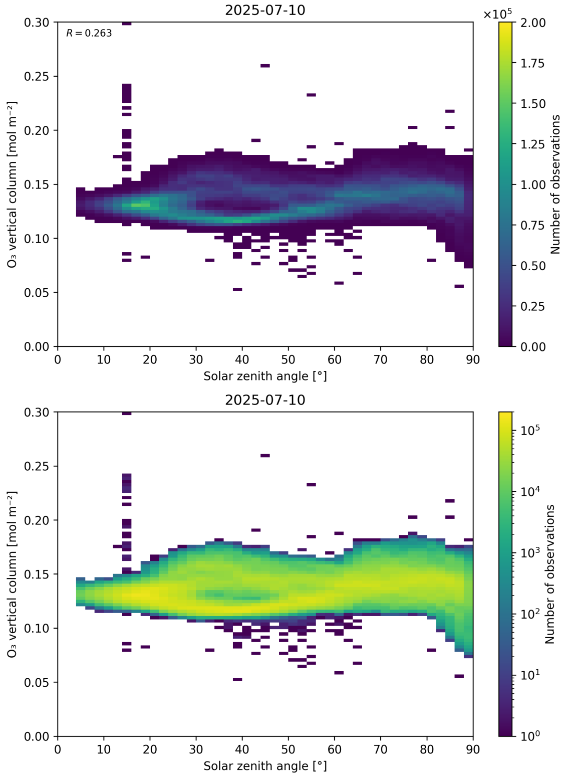
Figure 47: Scatter density plot of “Solar zenith angle” against “O 3 vertical column” for 2025-07-09 to 2025-07-11.
