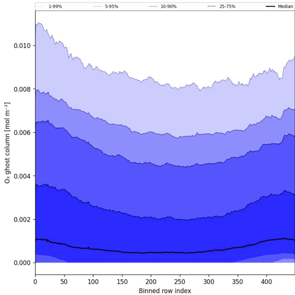
Figure 32: Along track statistics of “O 3 ghost column” for 2025-07-09 to 2025-07-11
