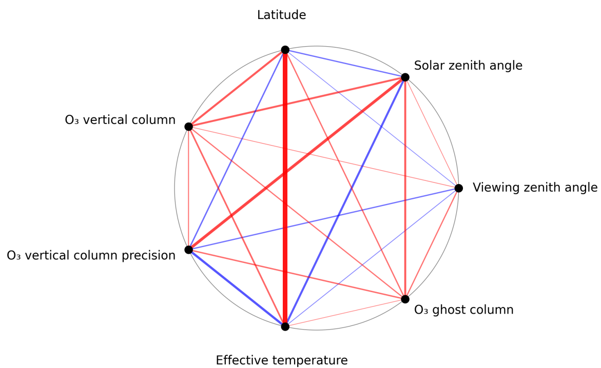
Figure 1: Map of correlation graph for 2025-07-09 to 2025-07-11.
