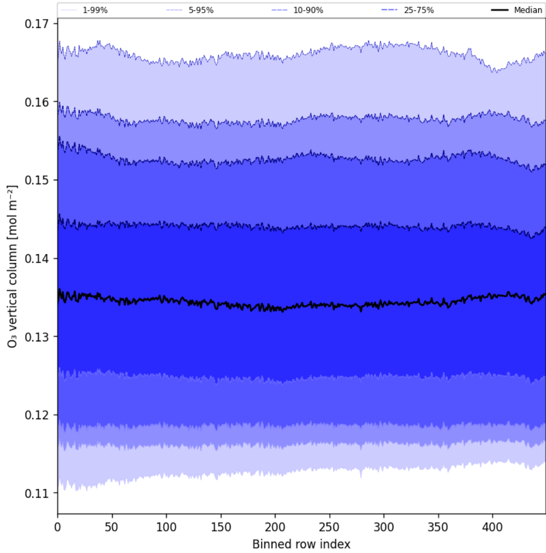
Figure 28: Along track statistics of “O 3 vertical column” for 2025-07-09 to 2025-07-11
