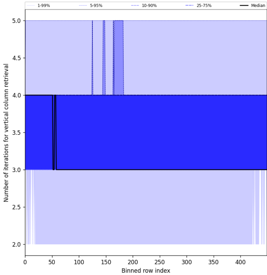
Figure 33: Along track statistics of “Number of iterations for vertical column retrieval” for 2025-07-09 to 2025-07-11
