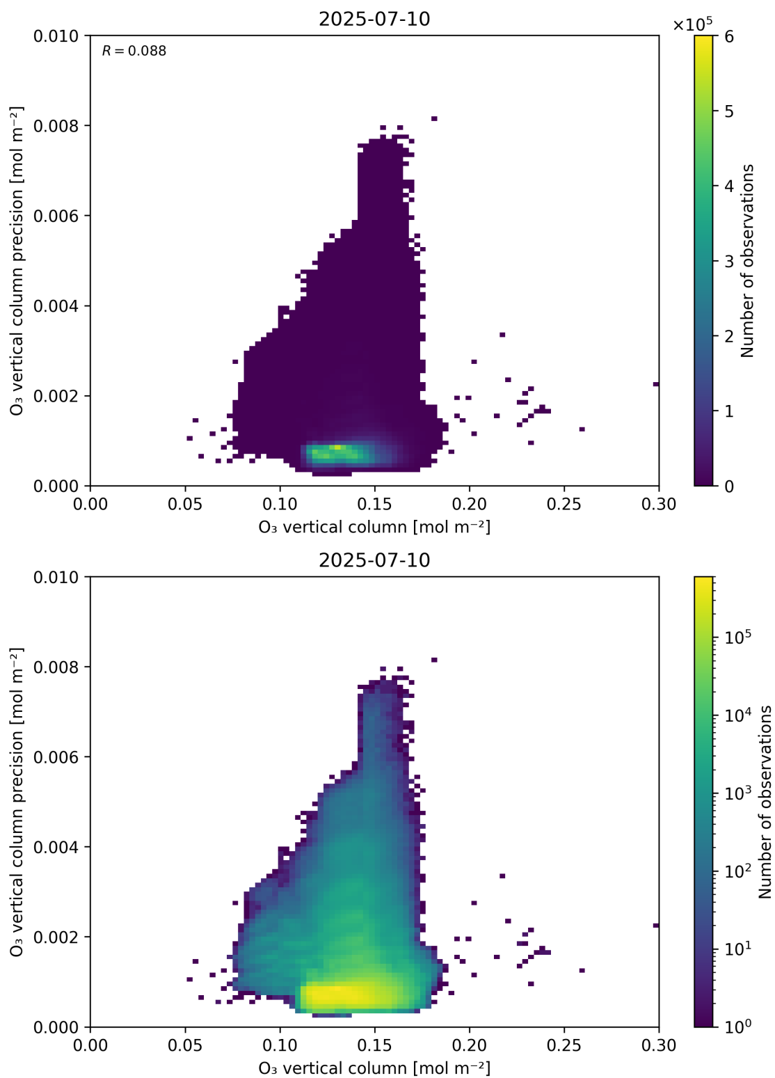
Figure 41: Scatter density plot of “O 3 vertical column” against “O 3 vertical column precision” for 2025-07-09 to 2025-07-11.
