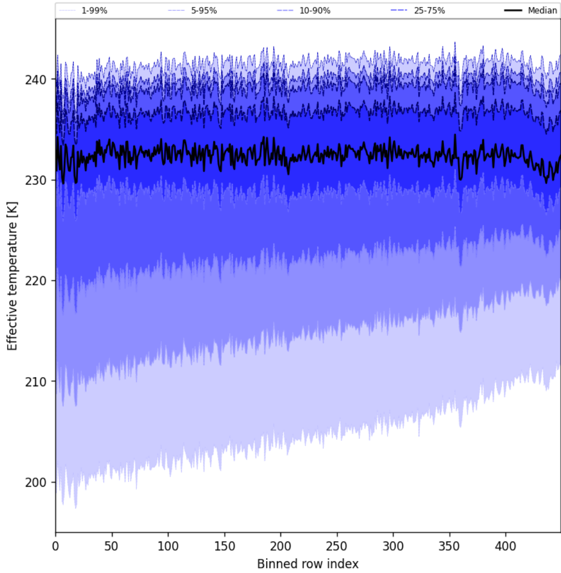
Figure 31: Along track statistics of “Effective temperature” for 2025-07-09 to 2025-07-11
