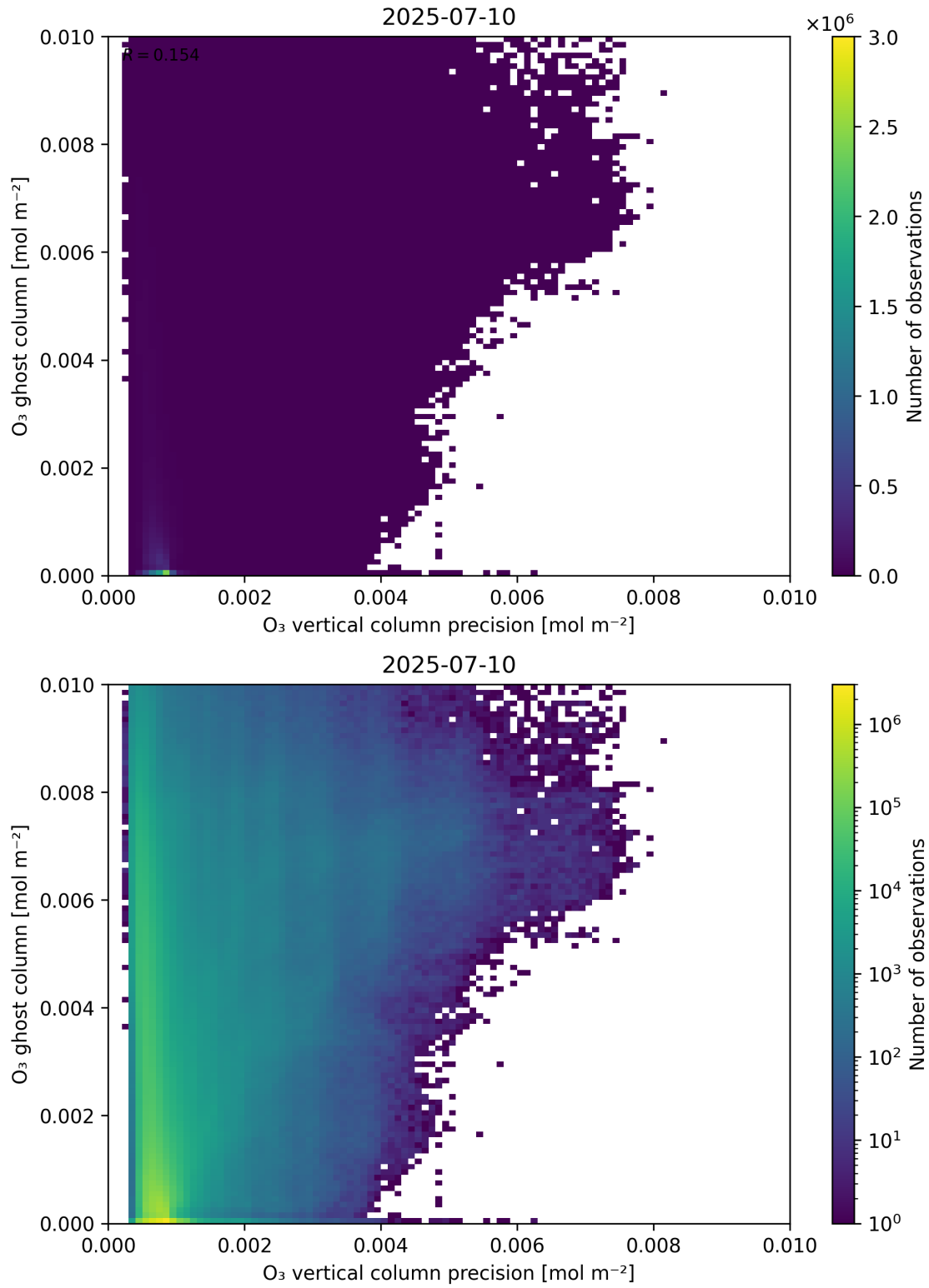
Figure 43: Scatter density plot of “ O_3 vertical column precision” against “ O_3 ghost column” for 2025-07-09 to 2025-07-11.
