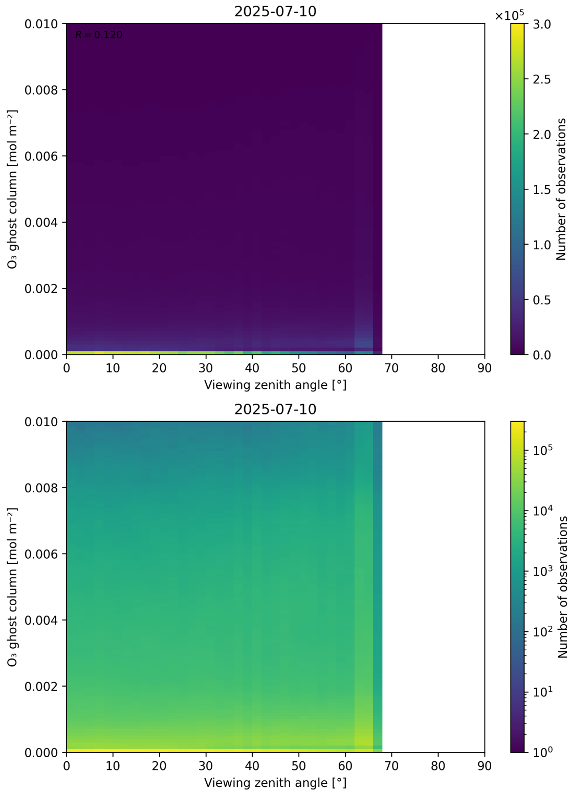
Figure 51: Scatter density plot of “Viewing zenith angle” against “O 3 ghost column” for 2025-07-09 to 2025-07-11.
