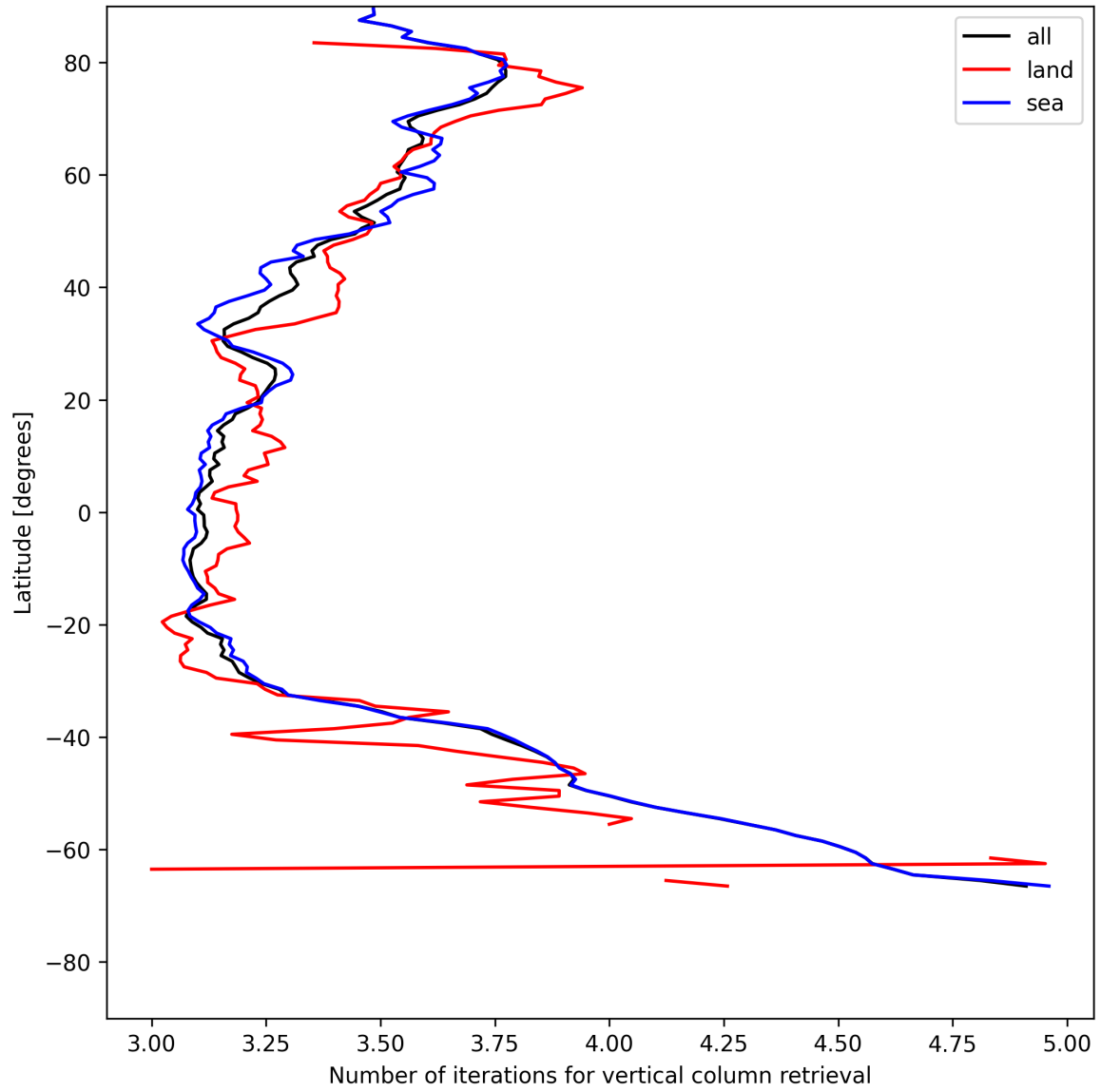
Figure 19: Zonal average of “Number of iterations for vertical column retrieval” for 2025-07-09 to 2025-07-11.
