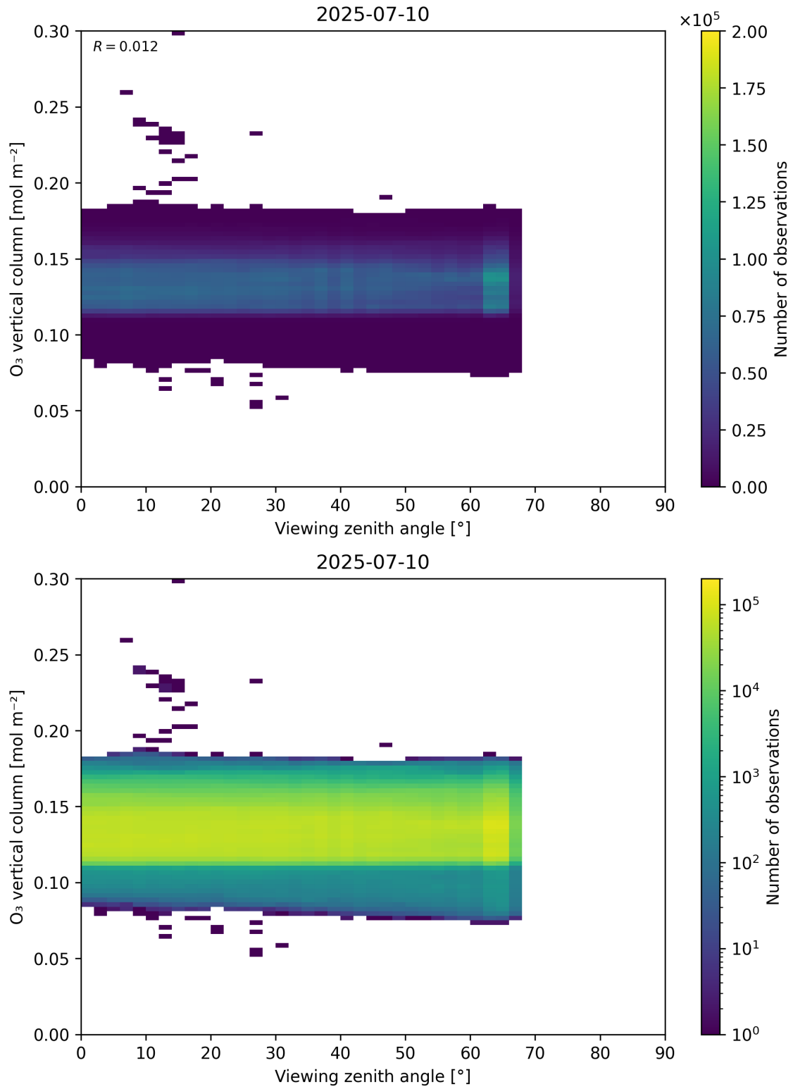
Figure 52: Scatter density plot of “Viewing zenith angle” against “O 3 vertical column” for 2025-07-09 to 2025-07-11.
