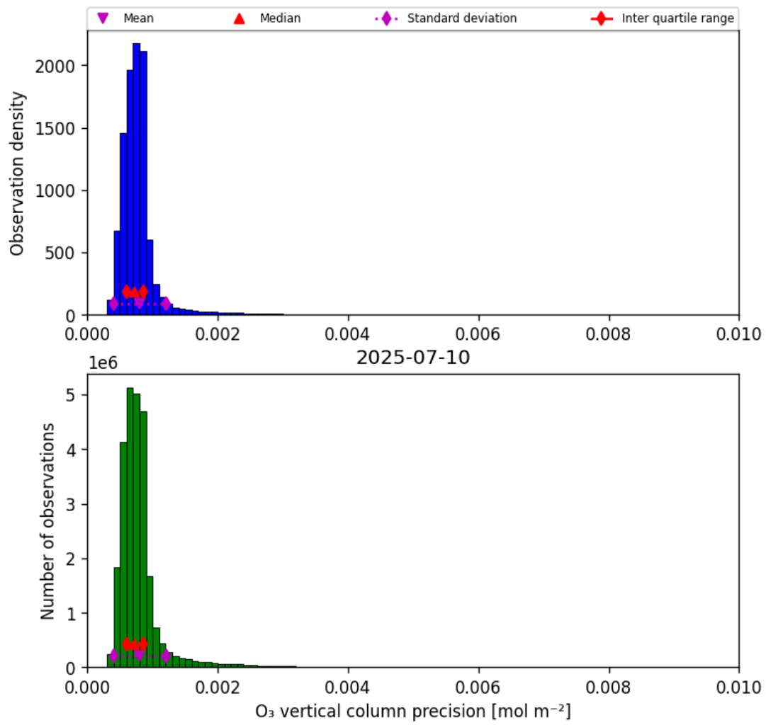
Figure 22: Histogram of “O 3 vertical column precision” for 2025-07-09 to 2025-07-11
