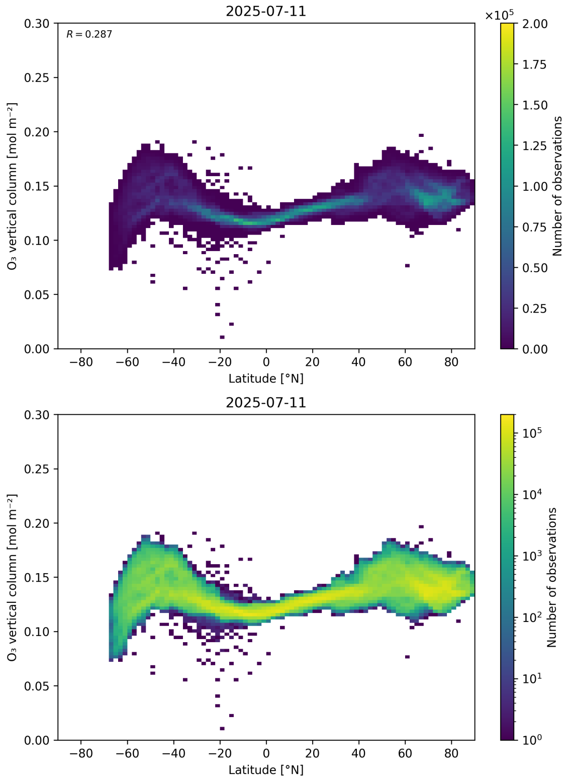
Figure 36: Scatter density plot of “Latitude” against “O 3 vertical column” for 2025-07-10 to 2025-07-12.
