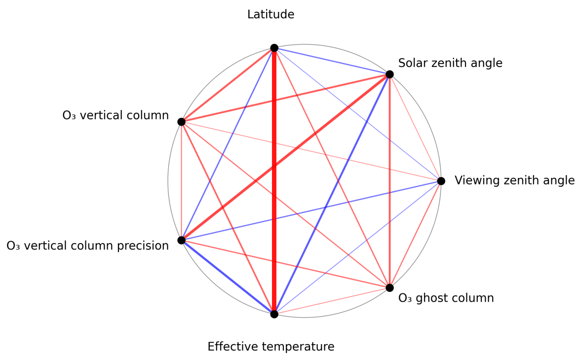
Figure 1: Map of correlation graph for 2025-07-10 to 2025-07-12.
