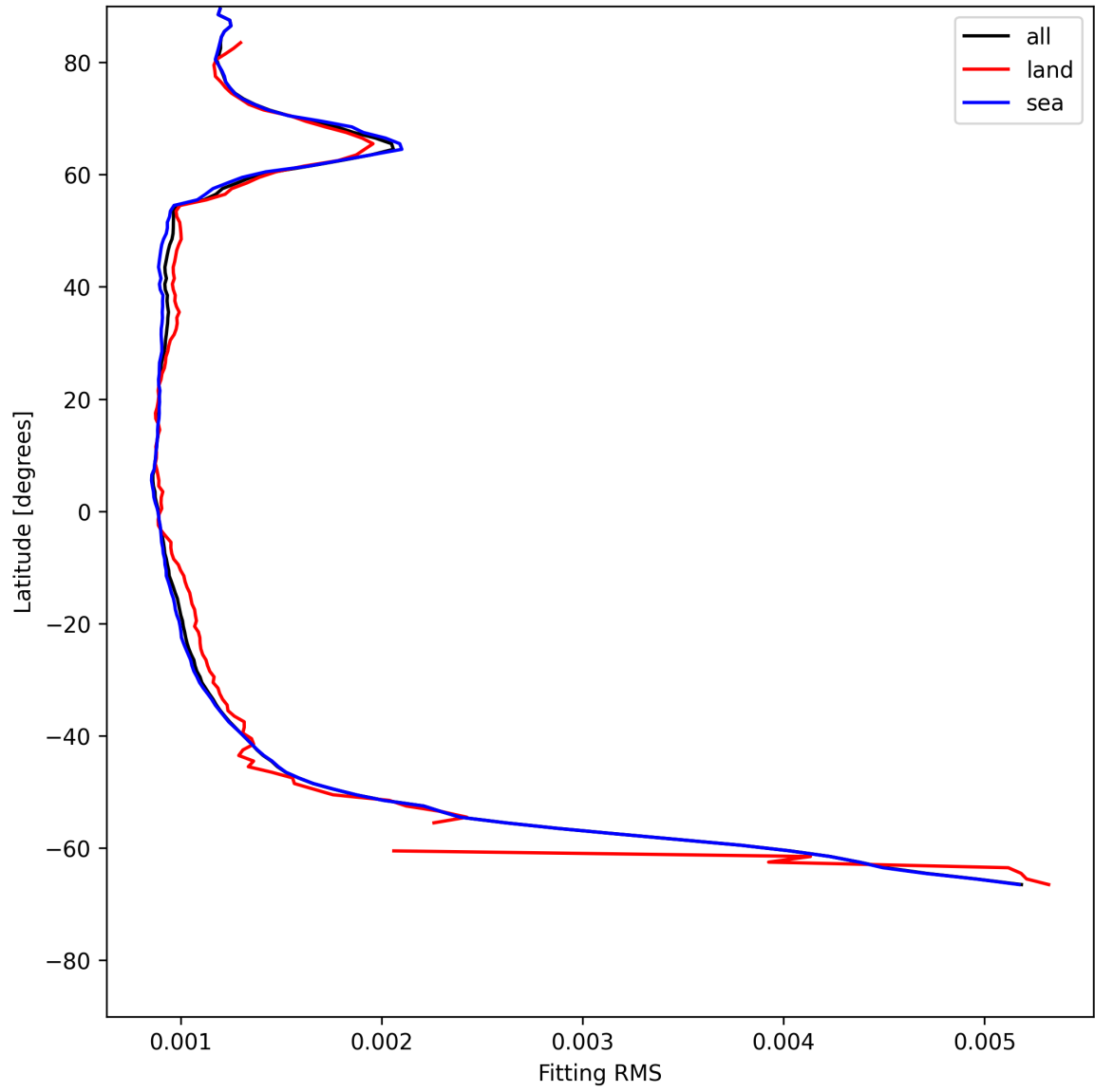
Figure 16: Zonal average of “Fitting RMS” for 2025-07-10 to 2025-07-12.
