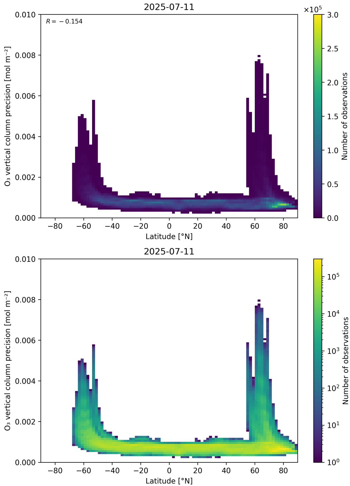
Figure 37: Scatter density plot of “Latitude” against “O 3 vertical column precision” for 2025-07-10 to 2025-07-12.
