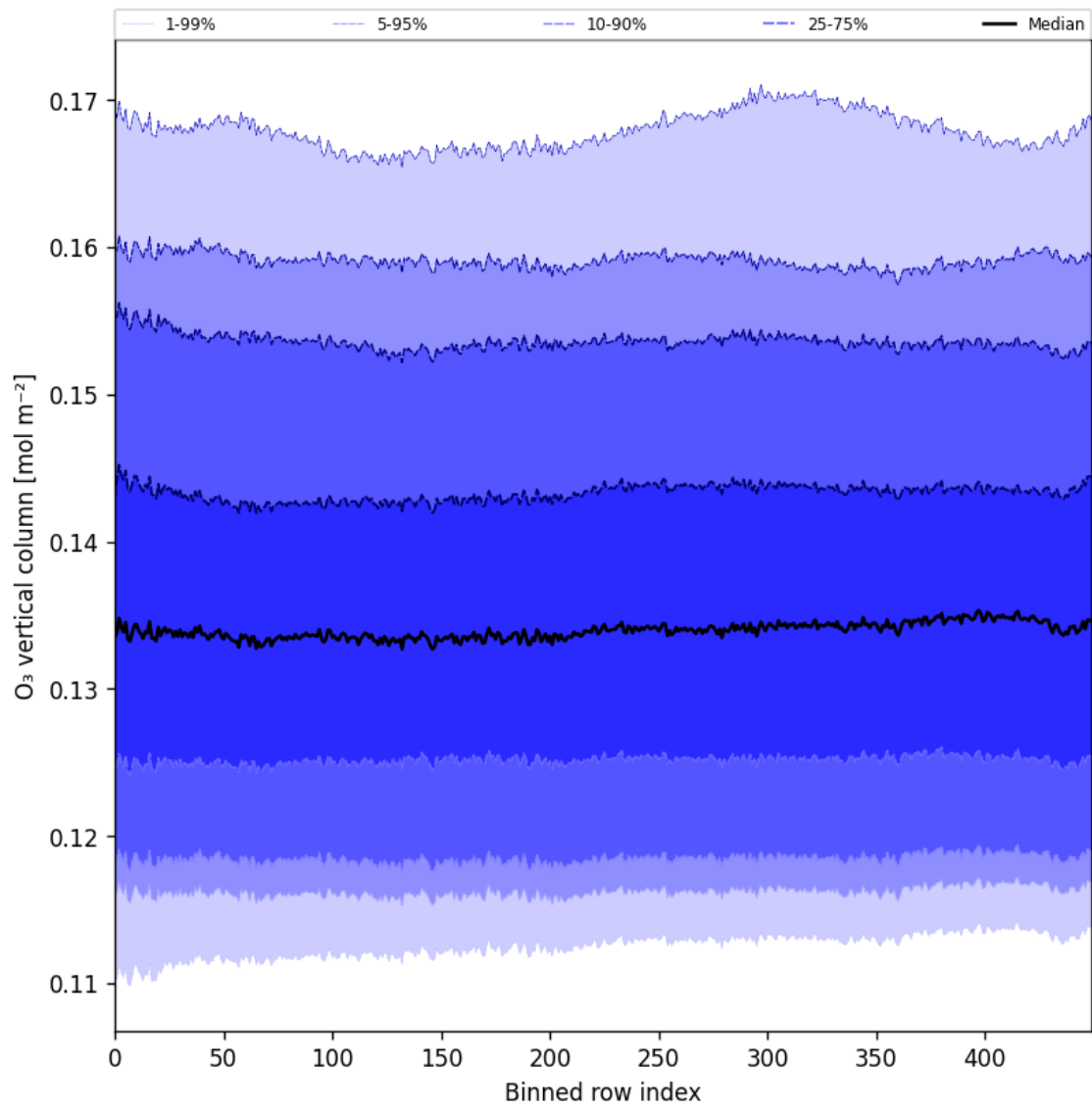
Figure 28: Along track statistics of “O 3 vertical column” for 2025-07-10 to 2025-07-12
