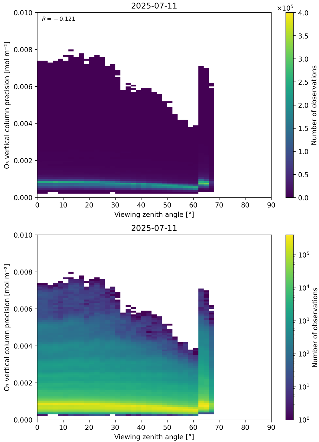
Figure 53: Scatter density plot of “Viewing zenith angle” against “O 3 vertical column precision” for 2025-07-10 to 2025-07-12.
