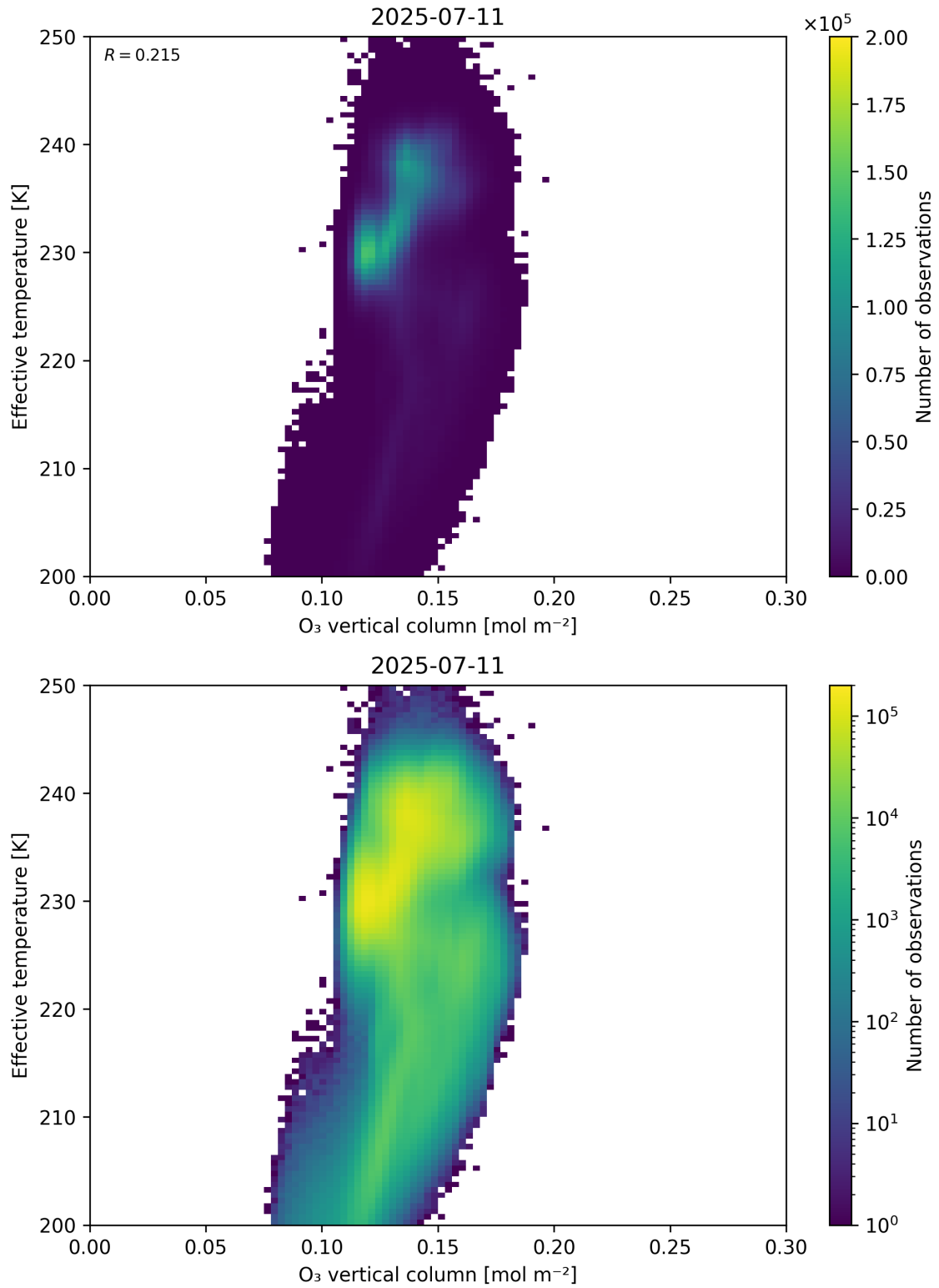
Figure 39: Scatter density plot of “O 3 vertical column” against “Effective temperature” for 2025-07-10 to 2025-07-12.
