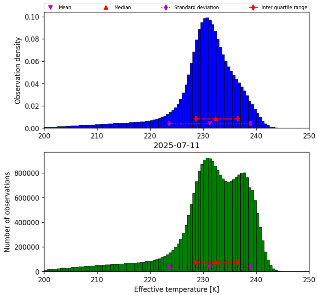
Figure 24: Histogram of “Effective temperature” for 2025-07-10 to 2025-07-12
