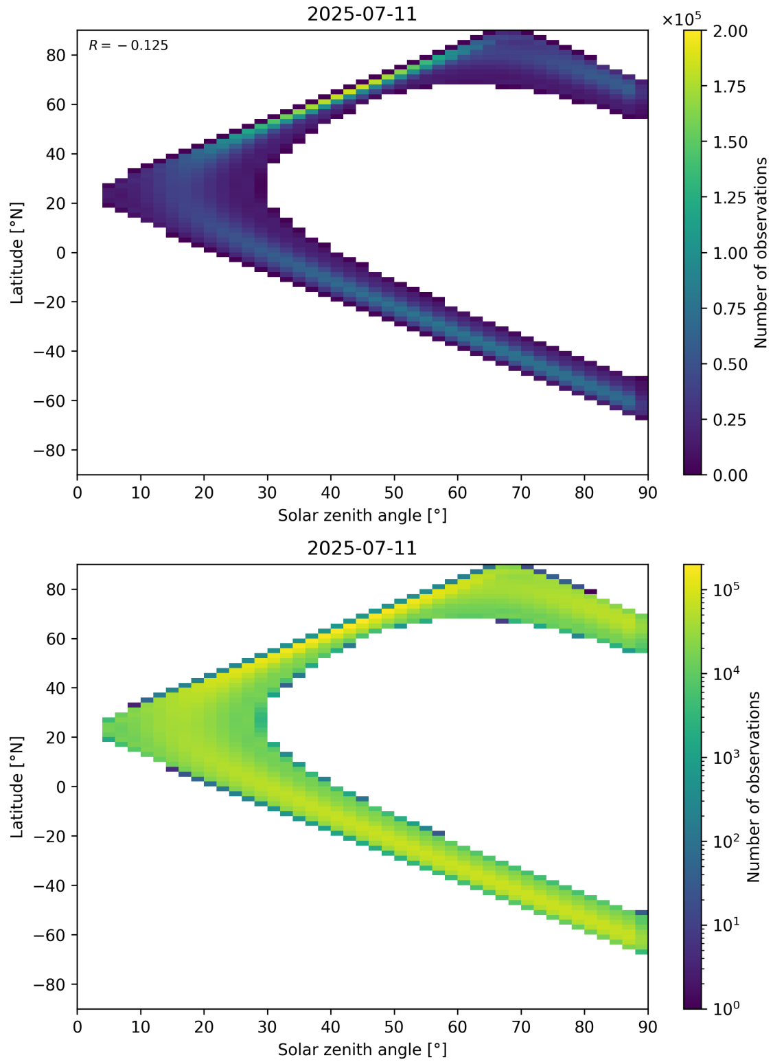
Figure 44: Scatter density plot of “Solar zenith angle” against “Latitude” for 2025-07-10 to 2025-07-12.
