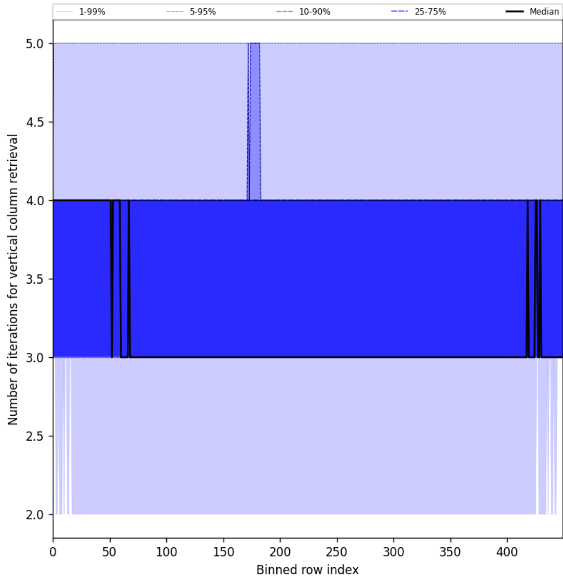
Figure 33: Along track statistics of “Number of iterations for vertical column retrieval” for 2025-07-10 to 2025-07-12
