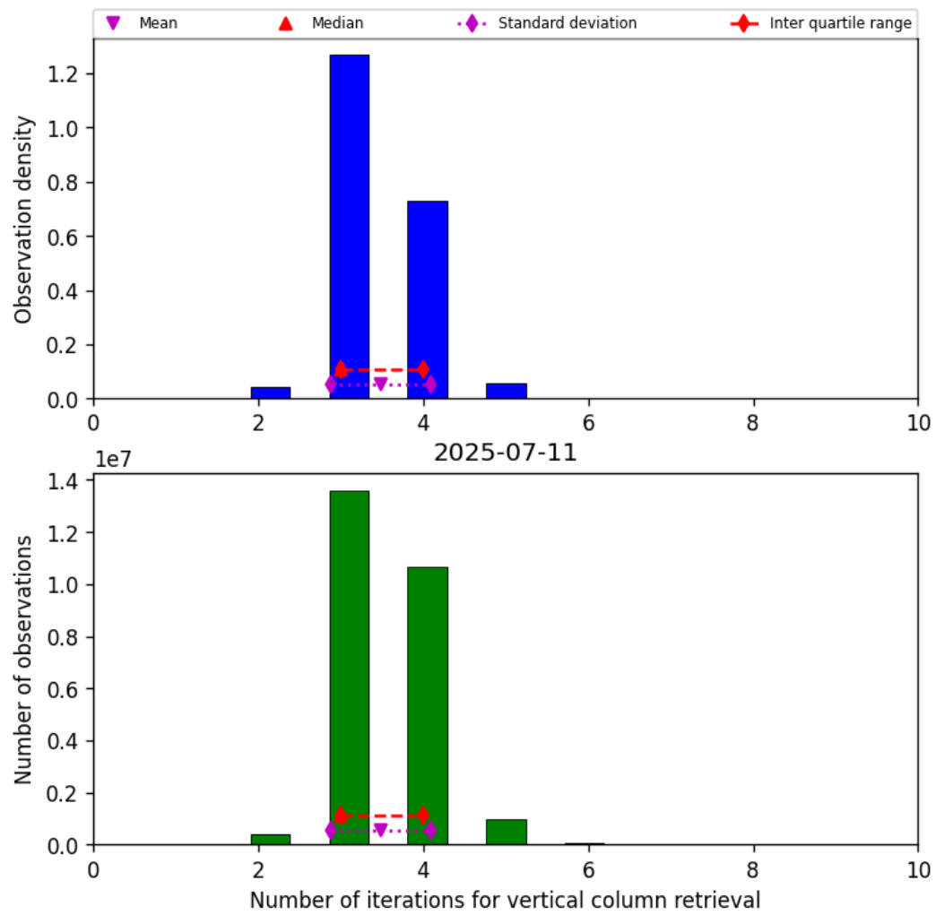
Figure 26: Histogram of “Number of iterations for vertical column retrieval” for 2025-07-10 to 2025-07-12
