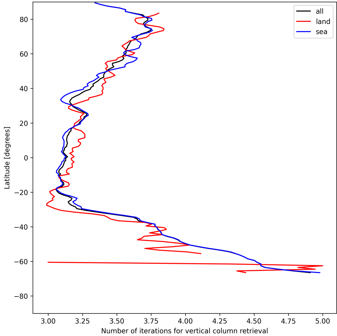
Figure 19: Zonal average of “Number of iterations for vertical column retrieval” for 2025-07-10 to 2025-07-12.
