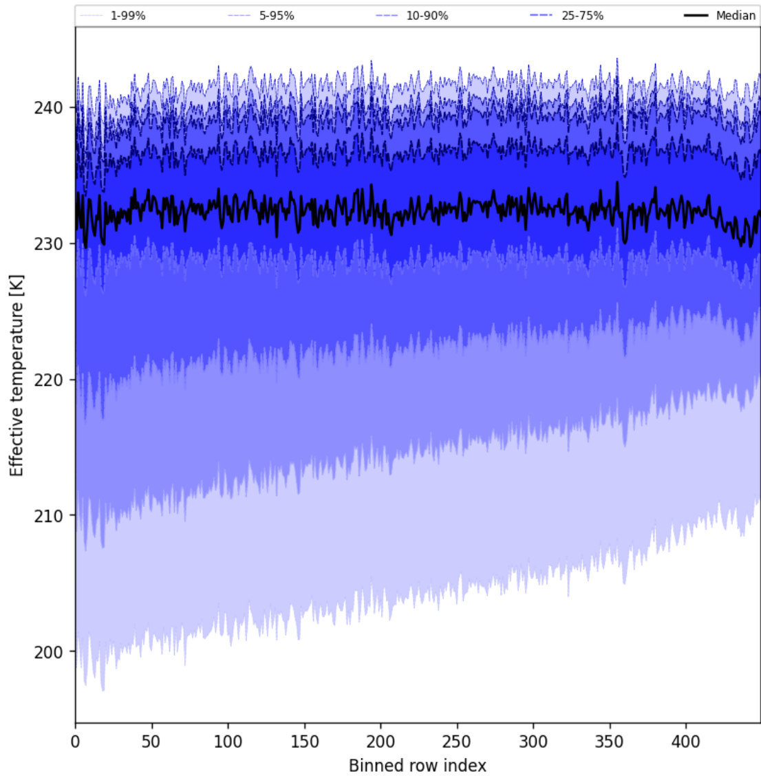
Figure 31: Along track statistics of “Effective temperature” for 2025-07-10 to 2025-07-12
