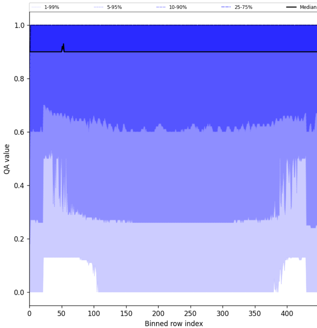
Figure 27: Along track statistics of “QA value” for 2025-07-10 to 2025-07-12
