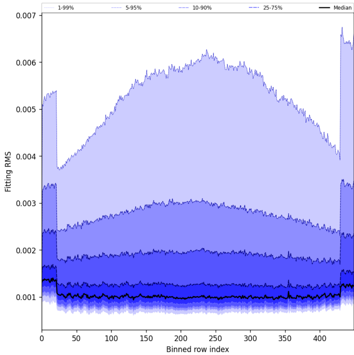
Figure 30: Along track statistics of “Fitting RMS” for 2025-07-10 to 2025-07-12
