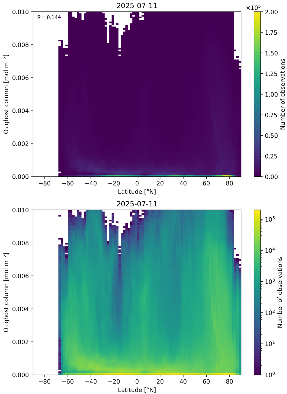
Figure 35: Scatter density plot of “Latitude” against “O 3 ghost column” for 2025-07-10 to 2025-07-12.
