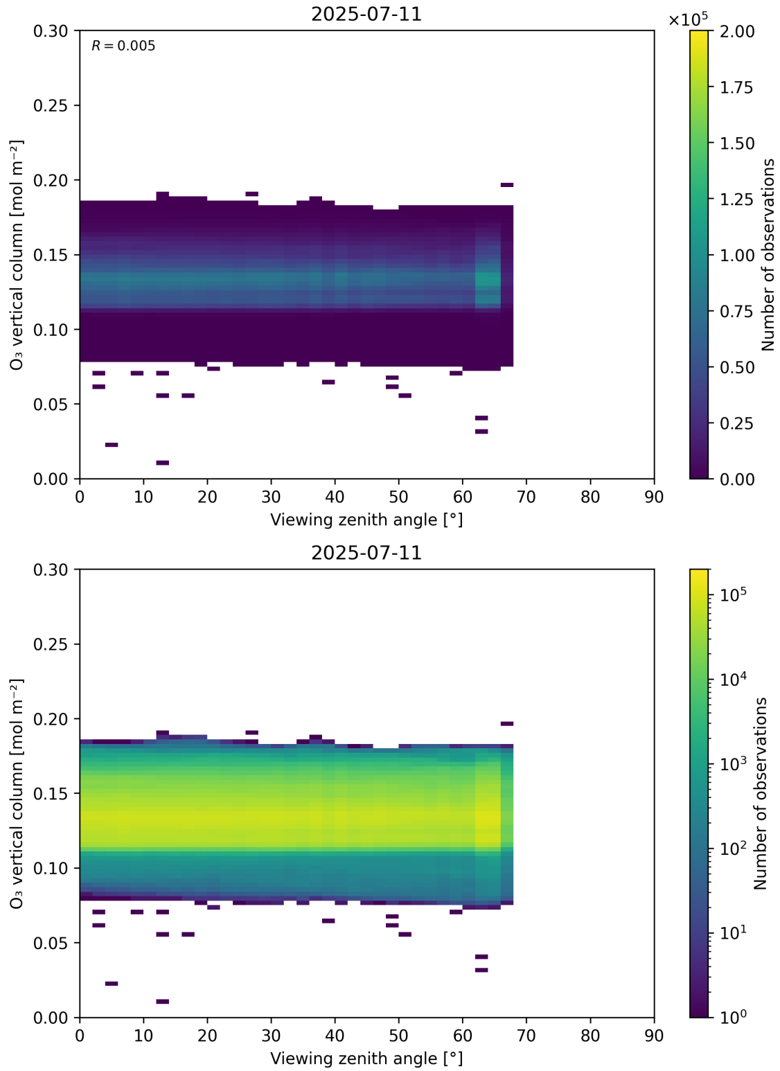
Figure 52: Scatter density plot of “Viewing zenith angle” against “O 3 vertical column” for 2025-07-10 to 2025-07-12.
