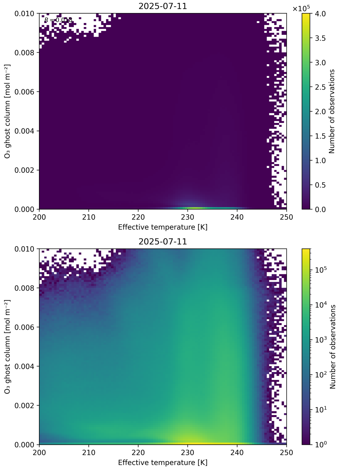
Figure 38: Scatter density plot of “Effective temperature” against “O 3 ghost column” for 2025-07-10 to 2025-07-12.
