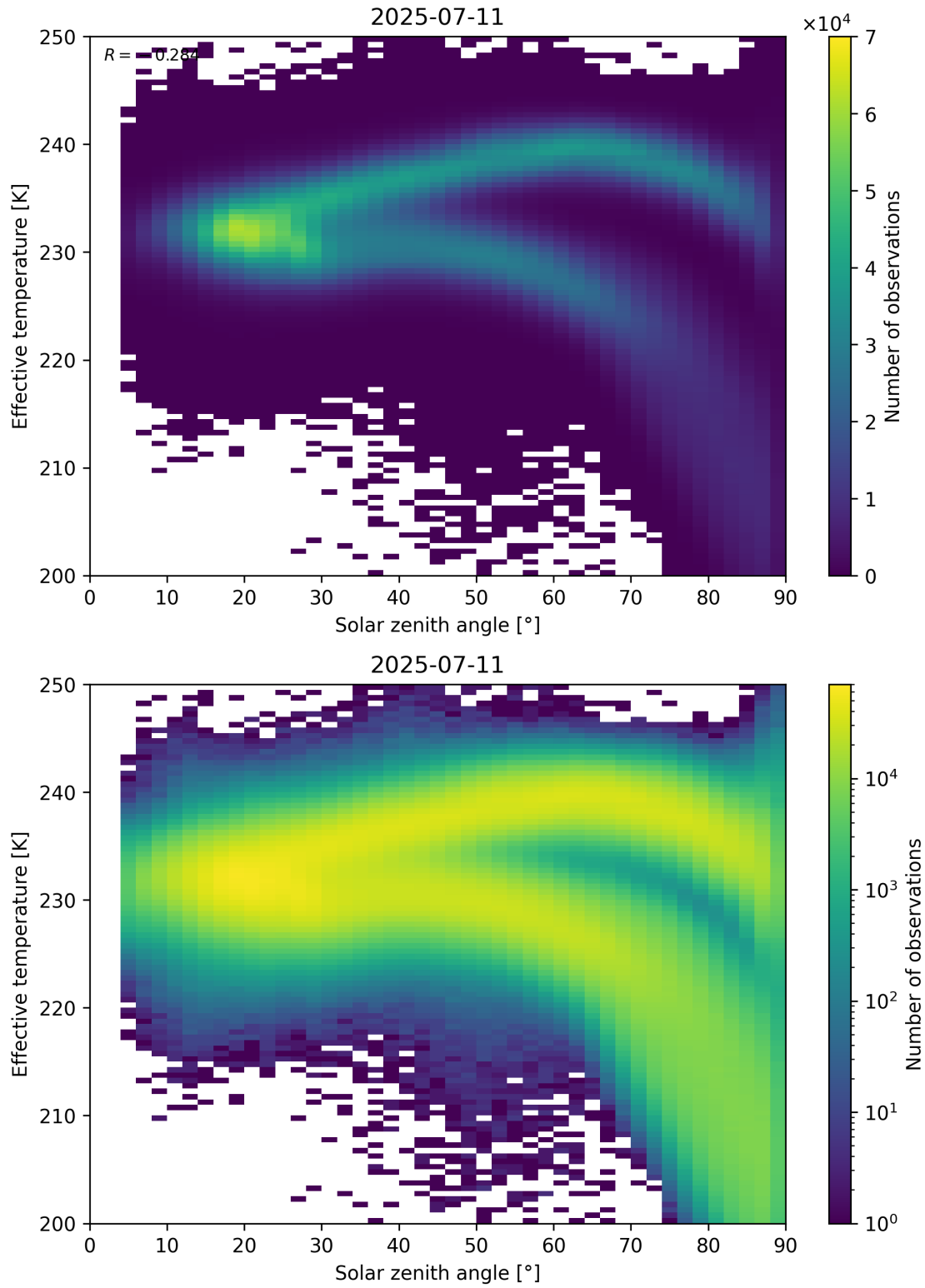
Figure 45: Scatter density plot of “Solar zenith angle” against “Effective temperature” for 2025-07-10 to 2025-07-12.
