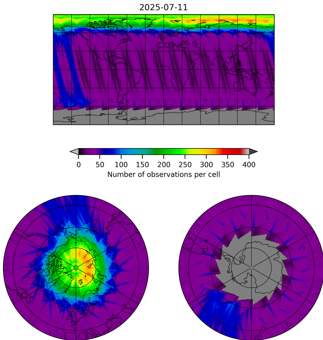
Figure 12: Map of the number of observations for 2025-07-10 to 2025-07-12
