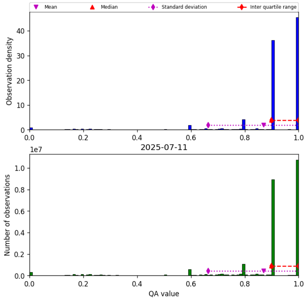
Figure 20: Histogram of “QA value” for 2025-07-10 to 2025-07-12
