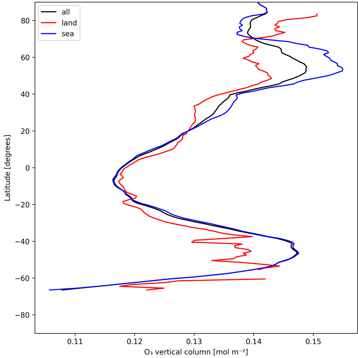
Figure 14: Zonal average of “O 3 vertical column” for 2025-07-10 to 2025-07-12.
