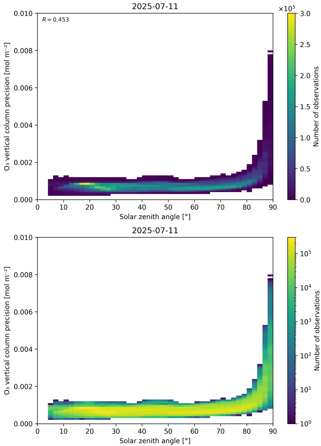
Figure 48: Scatter density plot of “Solar zenith angle” against “O 3 vertical column precision” for 2025-07-10 to 2025-07-12.
