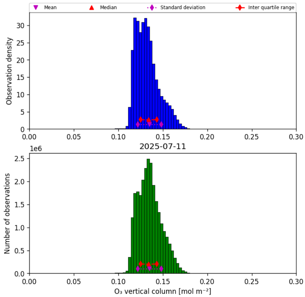
Figure 21: Histogram of “O 3 vertical column” for 2025-07-10 to 2025-07-12
