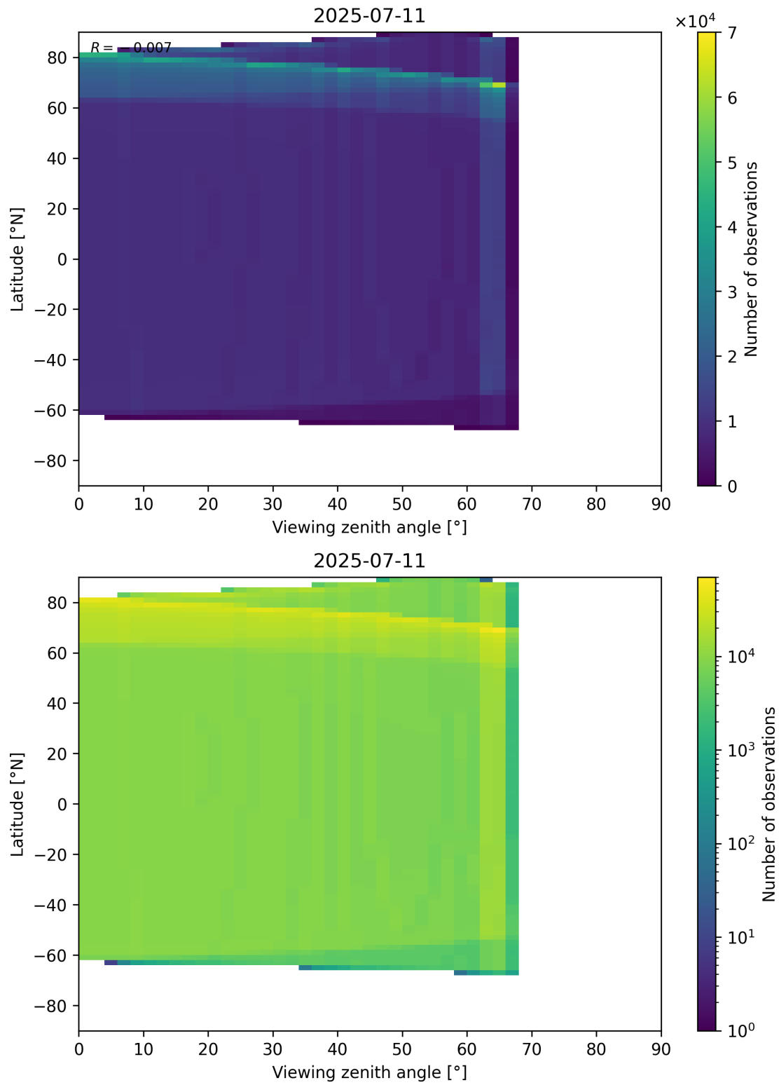
Figure 49: Scatter density plot of “Viewing zenith angle” against “Latitude” for 2025-07-10 to 2025-07-12.
