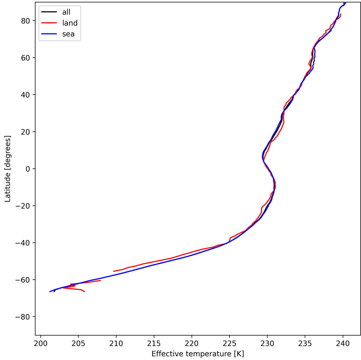
Figure 17: Zonal average of "Effective temperature" for 2025-07-10 to 2025-07-12.
