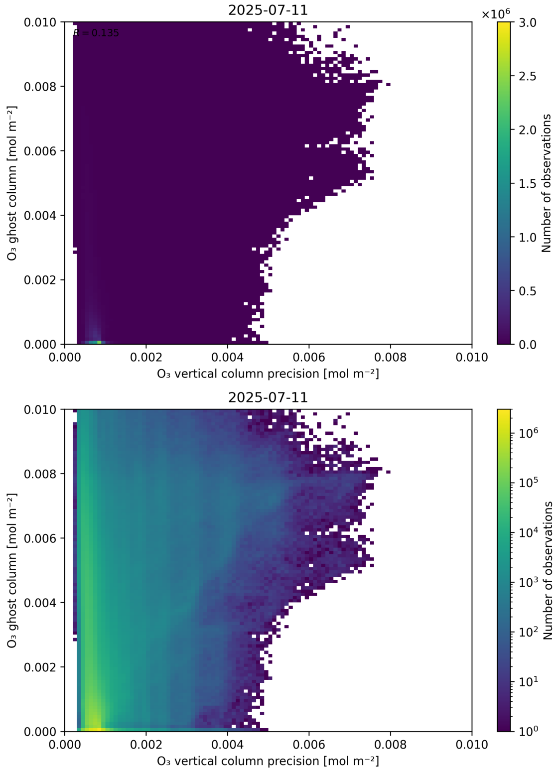
Figure 43: Scatter density plot of “O 3 vertical column precision” against “O 3 ghost column” for 2025-07-10 to 2025-07-12.
