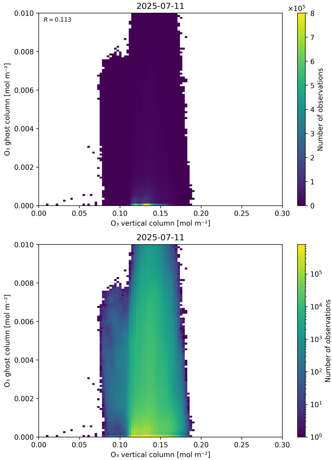
Figure 40: Scatter density plot of “O 3 vertical column” against “O 3 ghost column” for 2025-07-10 to 2025-07-12.
