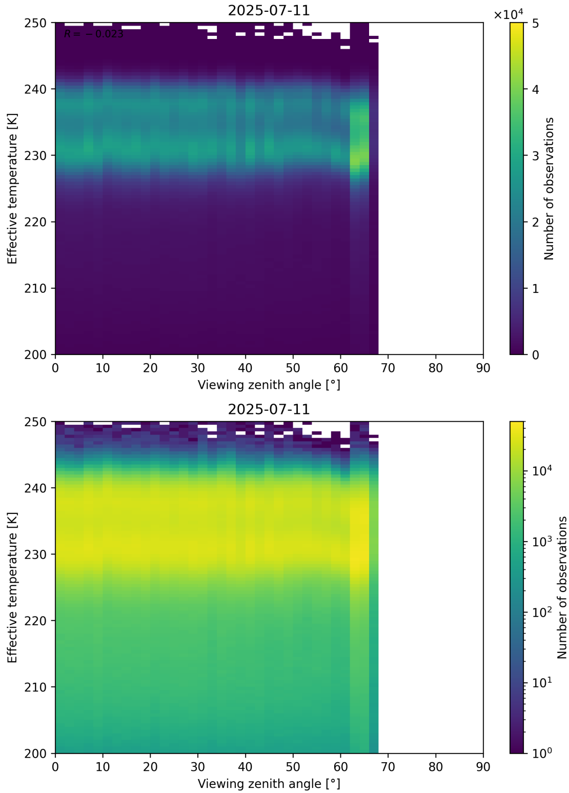
Figure 50: Scatter density plot of “Viewing zenith angle” against “Effective temperature” for 2025-07-10 to 2025-07-12.
