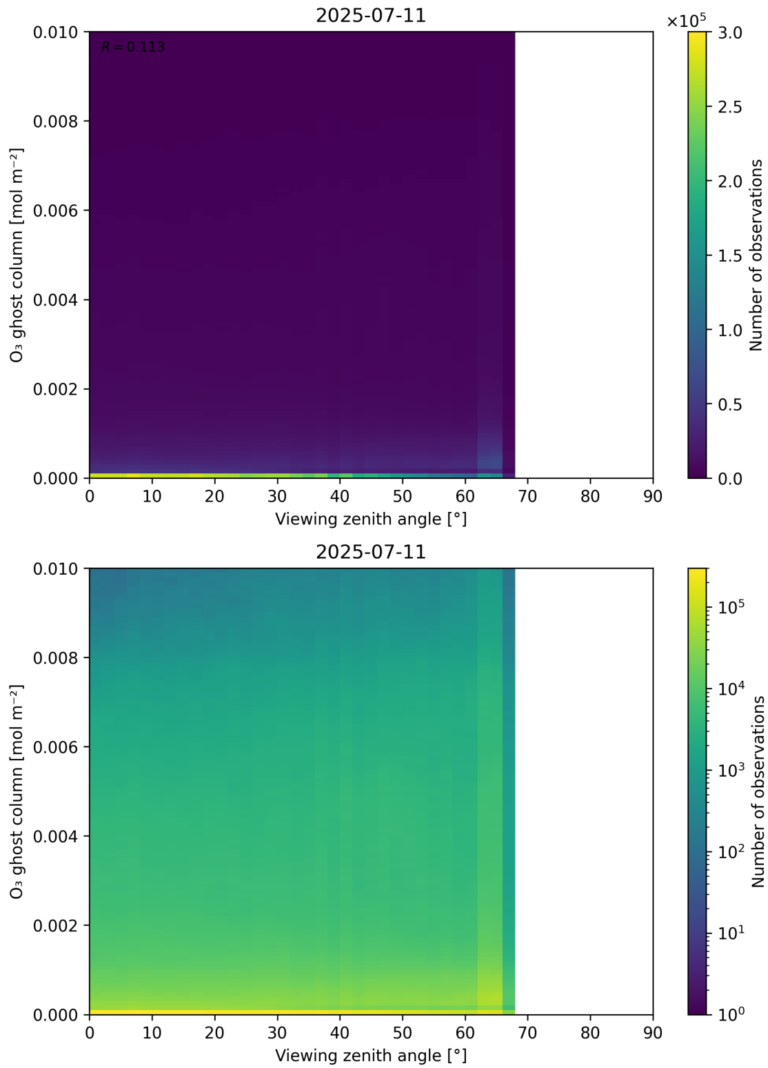
Figure 51: Scatter density plot of “Viewing zenith angle” against “O 3 ghost column” for 2025-07-10 to 2025-07-12.
