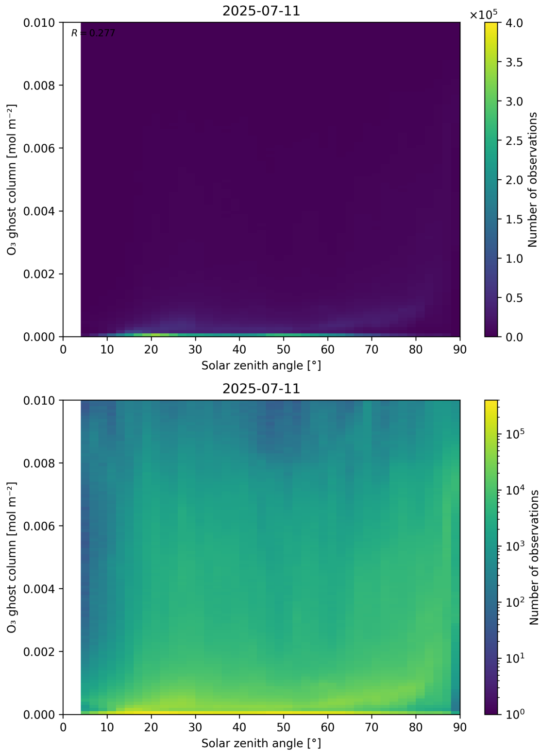
Figure 46: Scatter density plot of “Solar zenith angle” against “O 3 ghost column” for 2025-07-10 to 2025-07-12.
