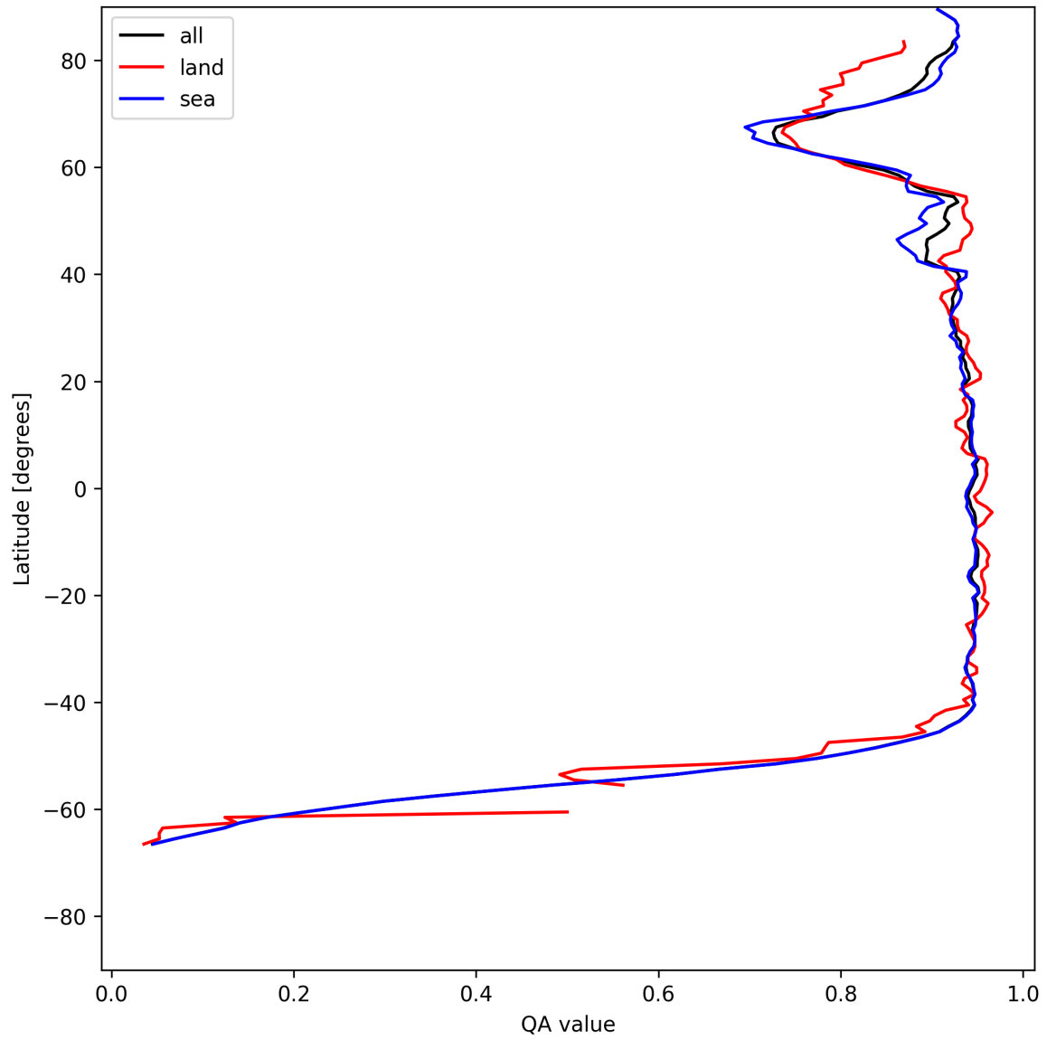
Figure 13: Zonal average of “QA value” for 2025-07-10 to 2025-07-12.
