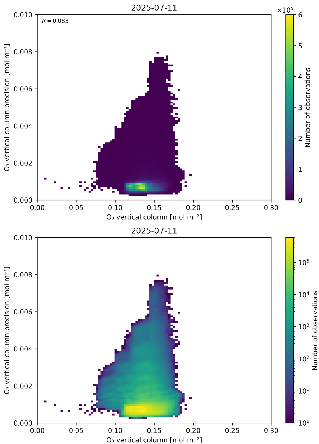
Figure 41: Scatter density plot of “O 3 vertical column” against “O 3 vertical column precision” for 2025-07-10 to 2025-07-12.
