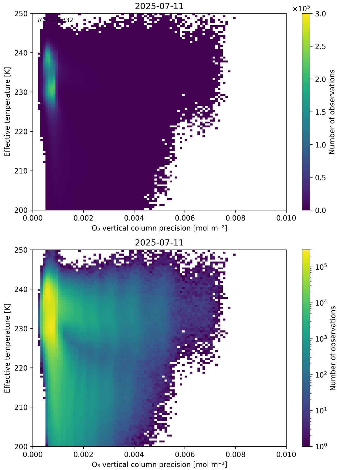
Figure 42: Scatter density plot of “O 3 vertical column precision” against “Effective temperature” for 2025-07-10 to 2025-07-12.
