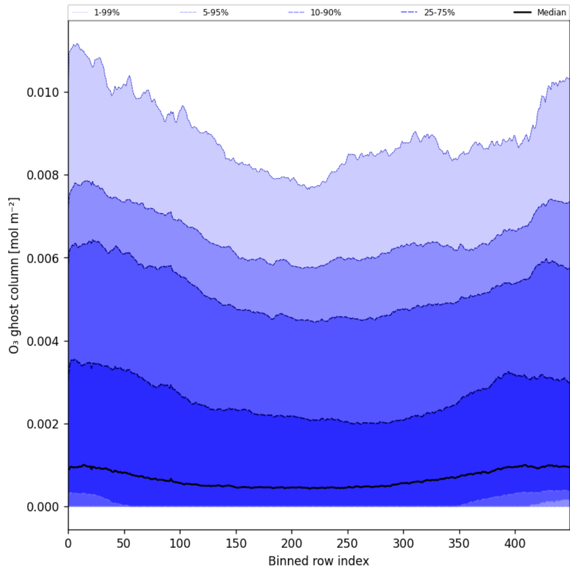
Figure 32: Along track statistics of “O 3 ghost column” for 2025-07-10 to 2025-07-12
