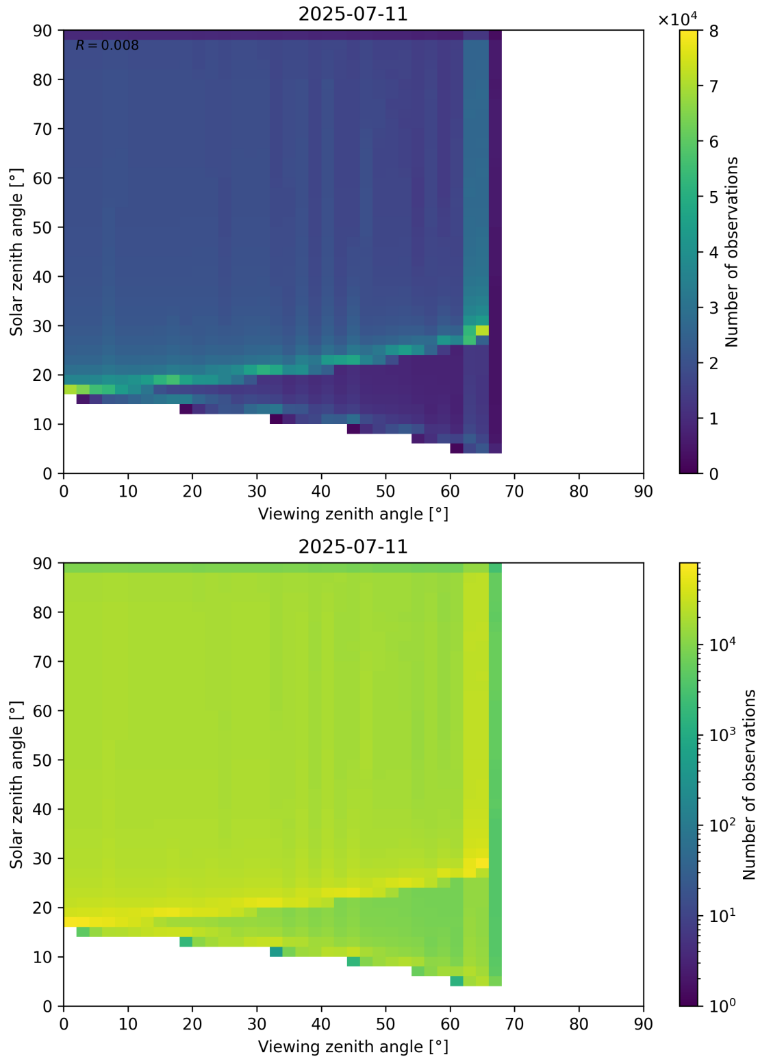
Figure 54: Scatter density plot of “Viewing zenith angle” against “Solar zenith angle” for 2025-07-10 to 2025-07-12.
