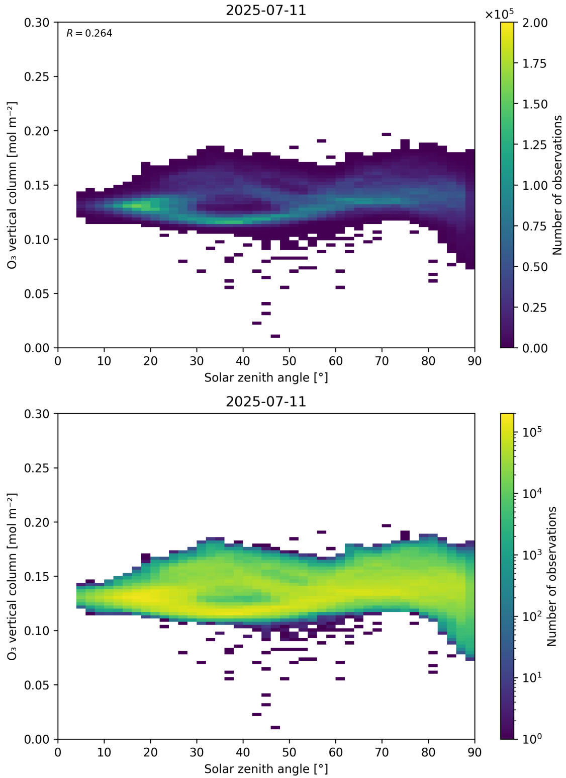
Figure 47: Scatter density plot of “Solar zenith angle” against “O 3 vertical column” for 2025-07-10 to 2025-07-12.
