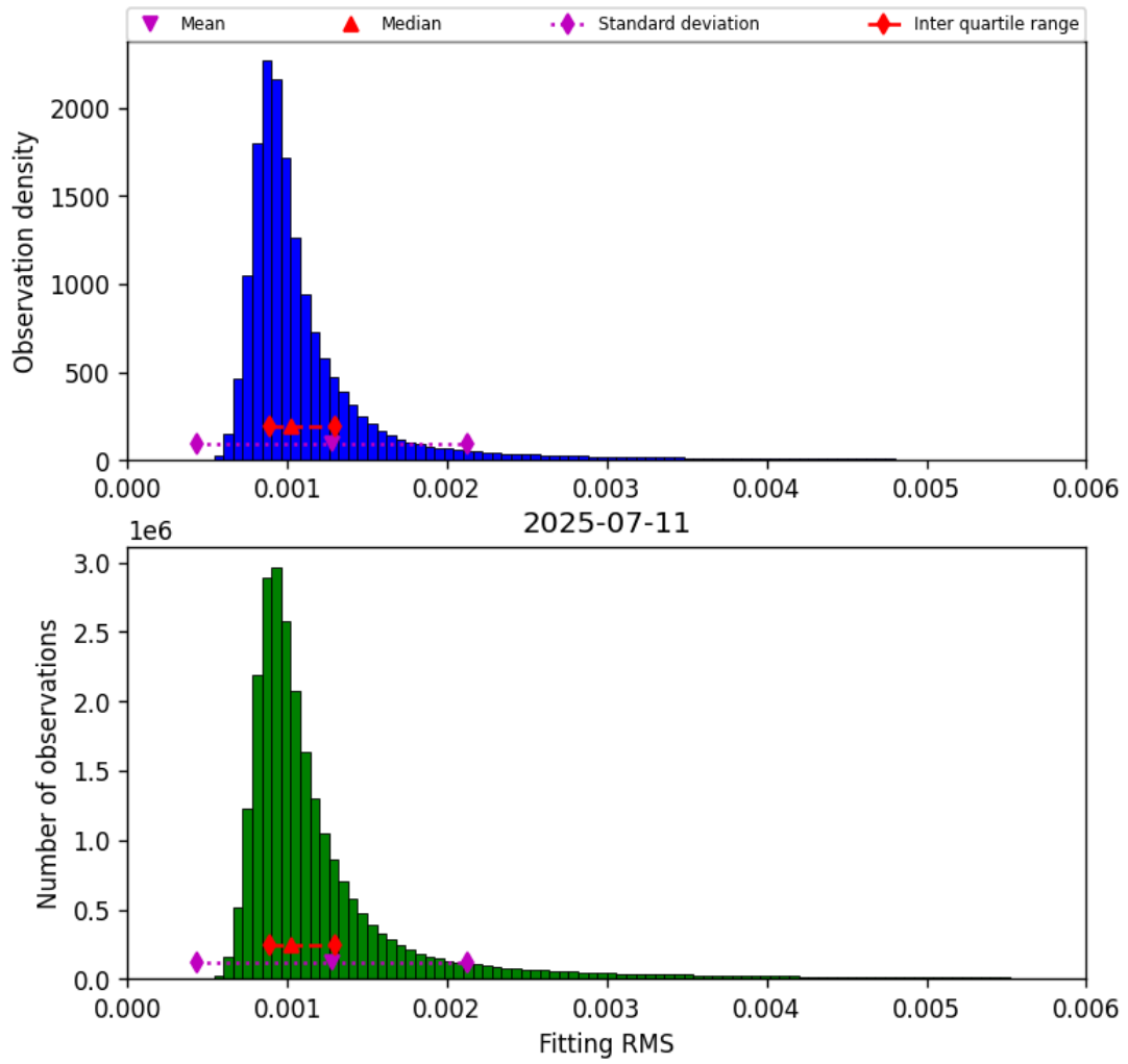
Figure 23: Histogram of “Fitting RMS” for 2025-07-10 to 2025-07-12
