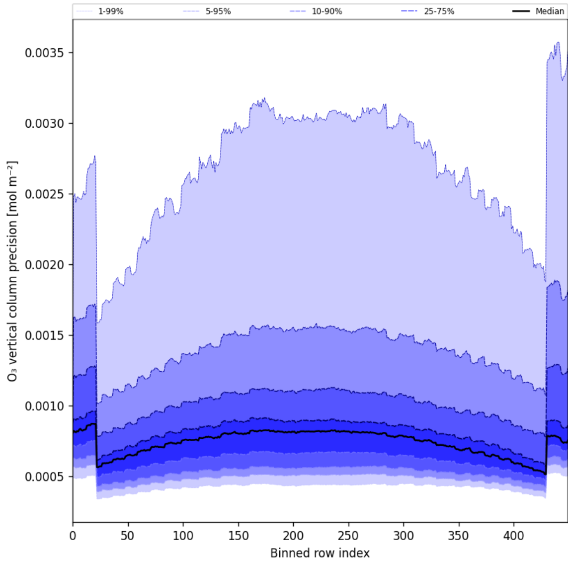
Figure 29: Along track statistics of “O 3 vertical column precision” for 2025-07-10 to 2025-07-12
