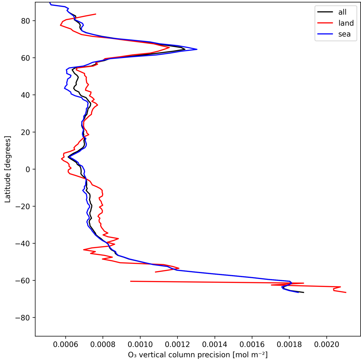
Figure 15: Zonal average of “O 3 vertical column precision” for 2025-07-10 to 2025-07-12.
