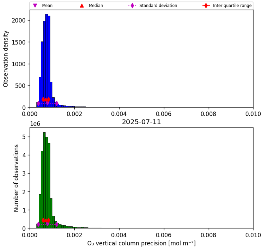
Figure 22: Histogram of “O 3 vertical column precision” for 2025-07-10 to 2025-07-12
