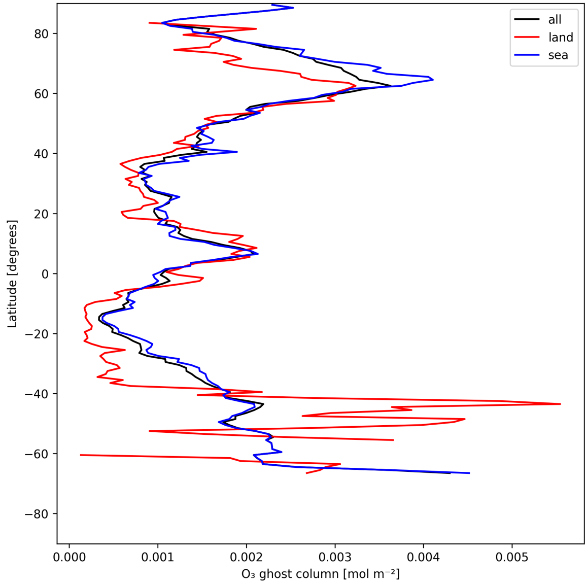
Figure 18: Zonal average of "O 3 ghost column" for 2025-07-10 to 2025-07-12.
