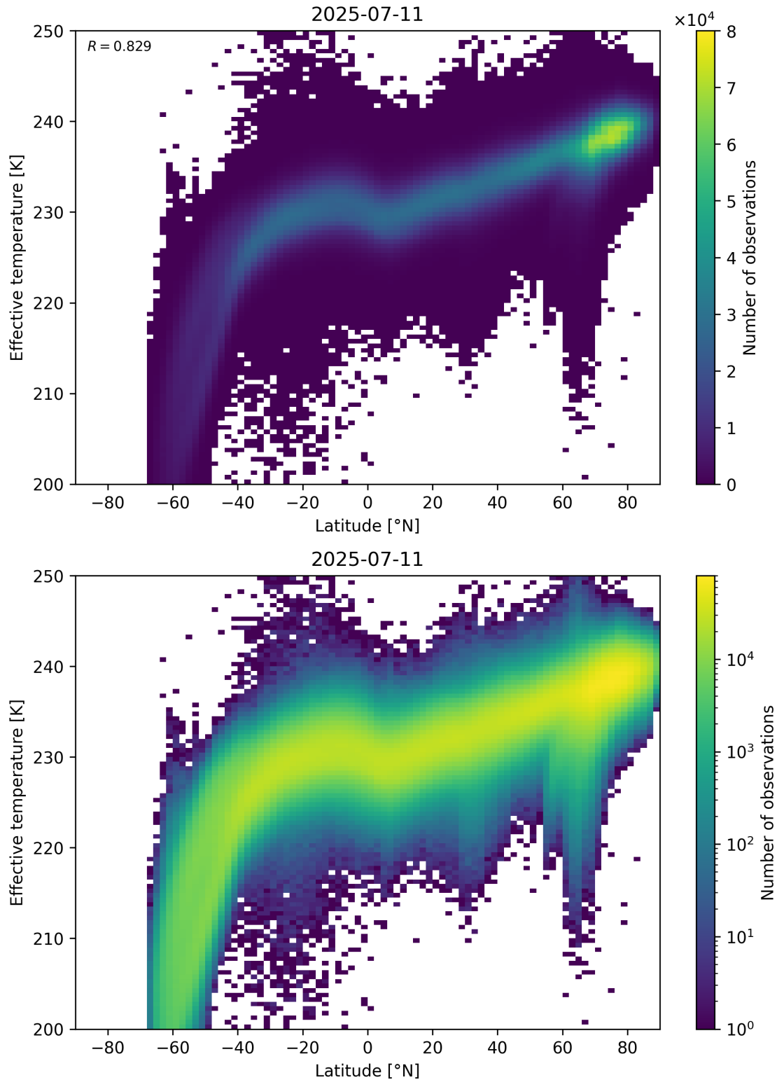
Figure 34: Scatter density plot of “Latitude” against “Effective temperature” for 2025-07-10 to 2025-07-12.
