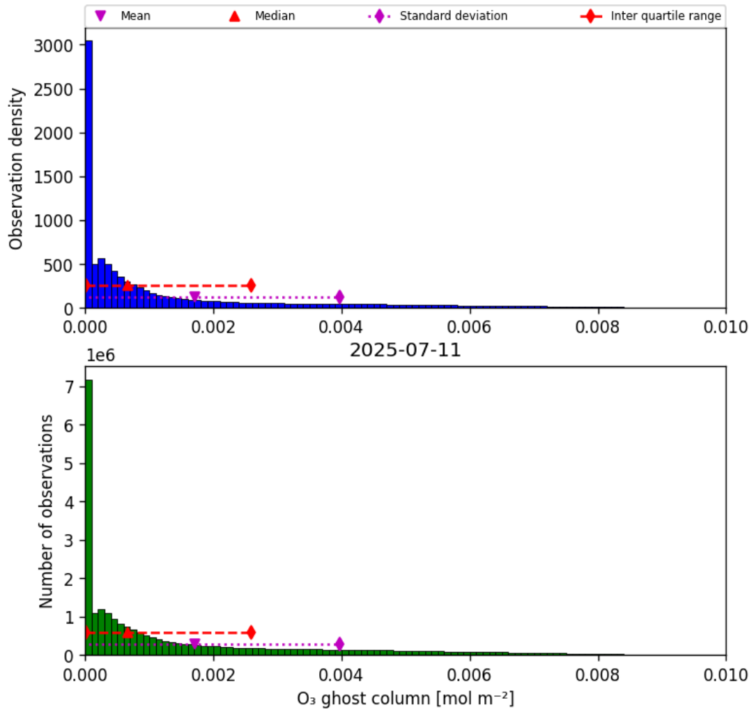
Figure 25: Histogram of “O 3 ghost column” for 2025-07-10 to 2025-07-12
