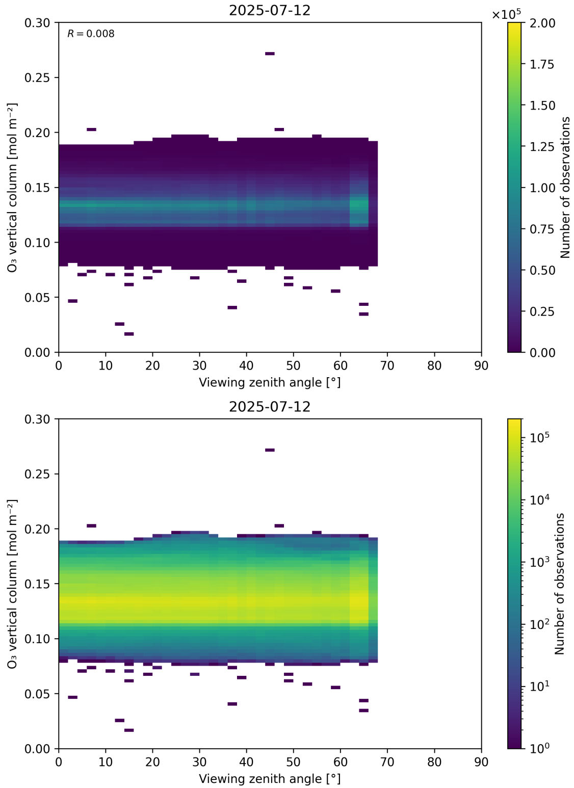
Figure 52: Scatter density plot of “Viewing zenith angle” against “O 3 vertical column” for 2025-07-11 to 2025-07-13.
