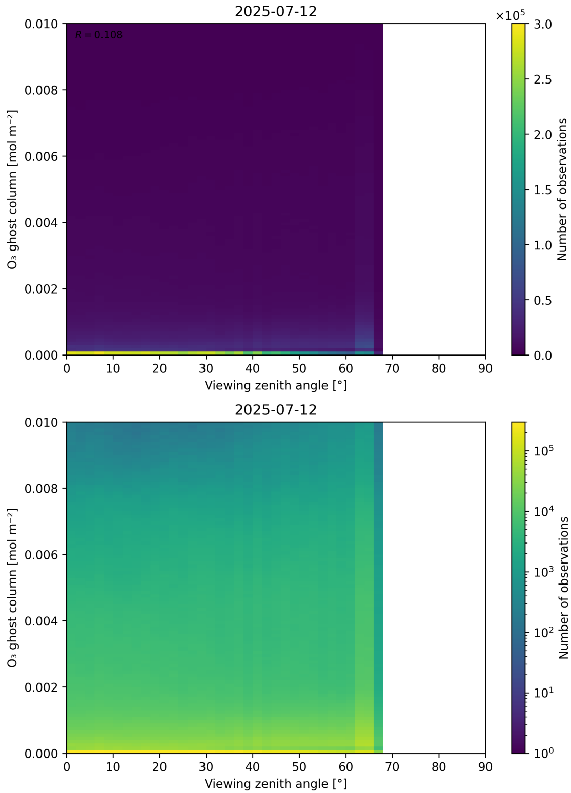
Figure 51: Scatter density plot of “Viewing zenith angle” against “O 3 ghost column” for 2025-07-11 to 2025-07-13.
