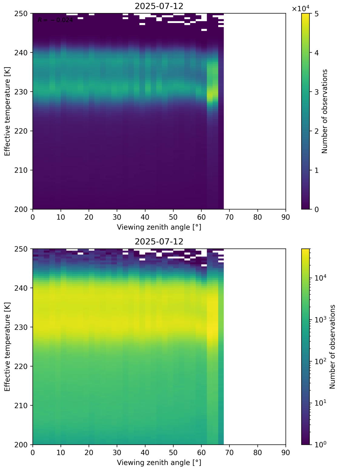
Figure 50: Scatter density plot of “Viewing zenith angle” against “Effective temperature” for 2025-07-11 to 2025-07-13.
