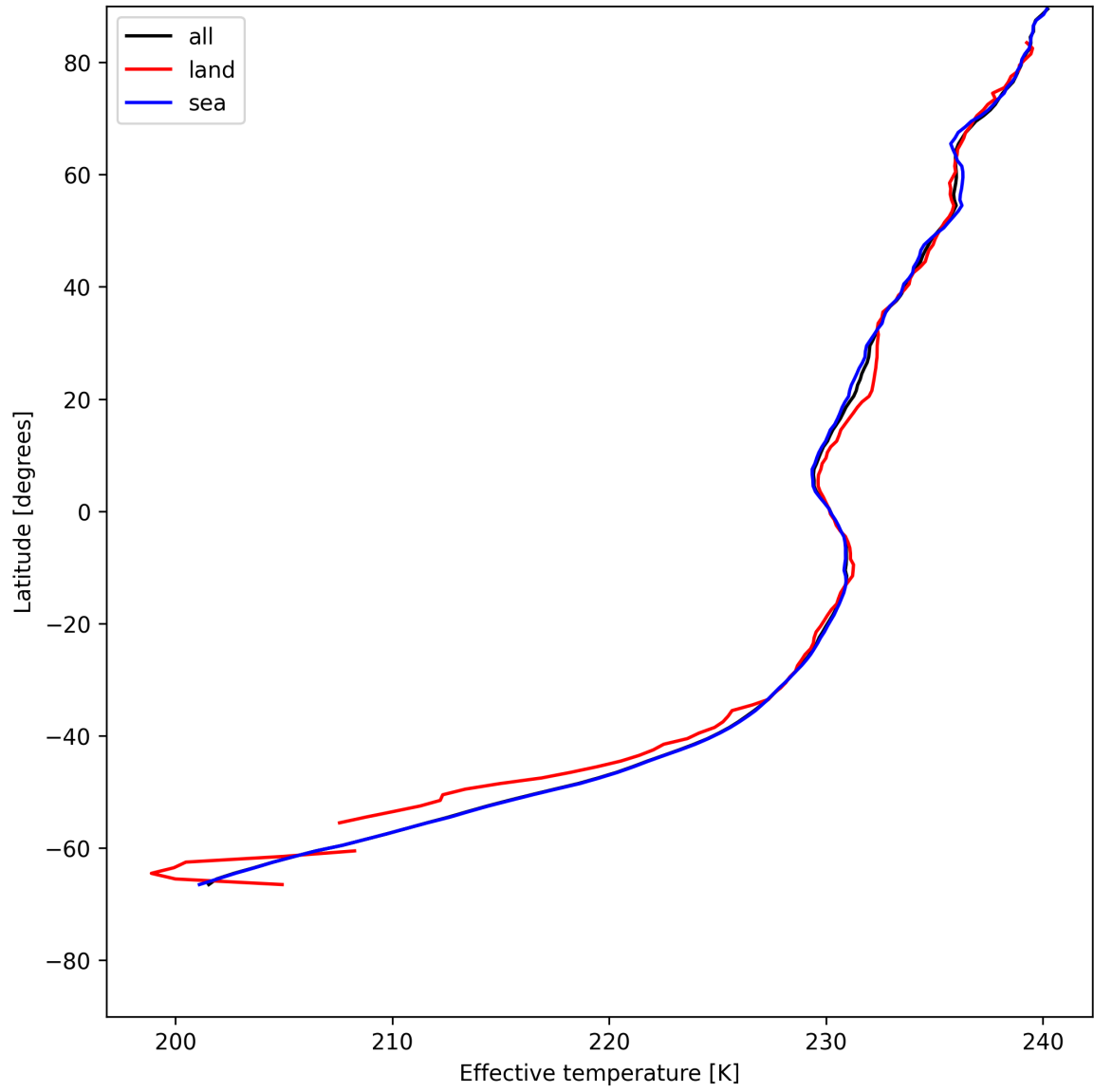
Figure 17: Zonal average of "Effective temperature" for 2025-07-11 to 2025-07-13.
