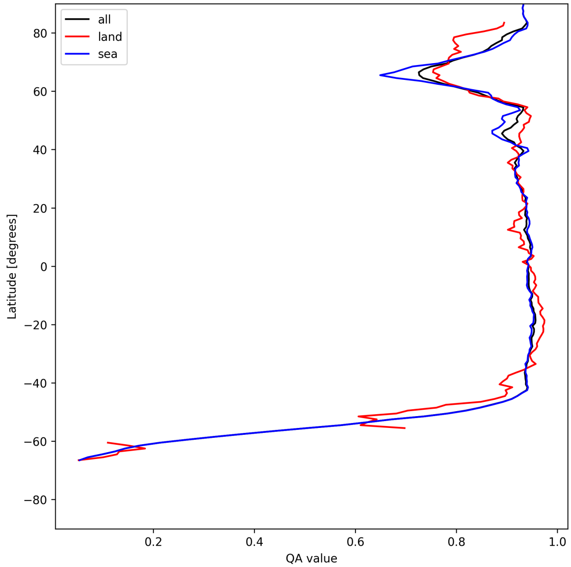
Figure 13: Zonal average of “QA value” for 2025-07-11 to 2025-07-13.
