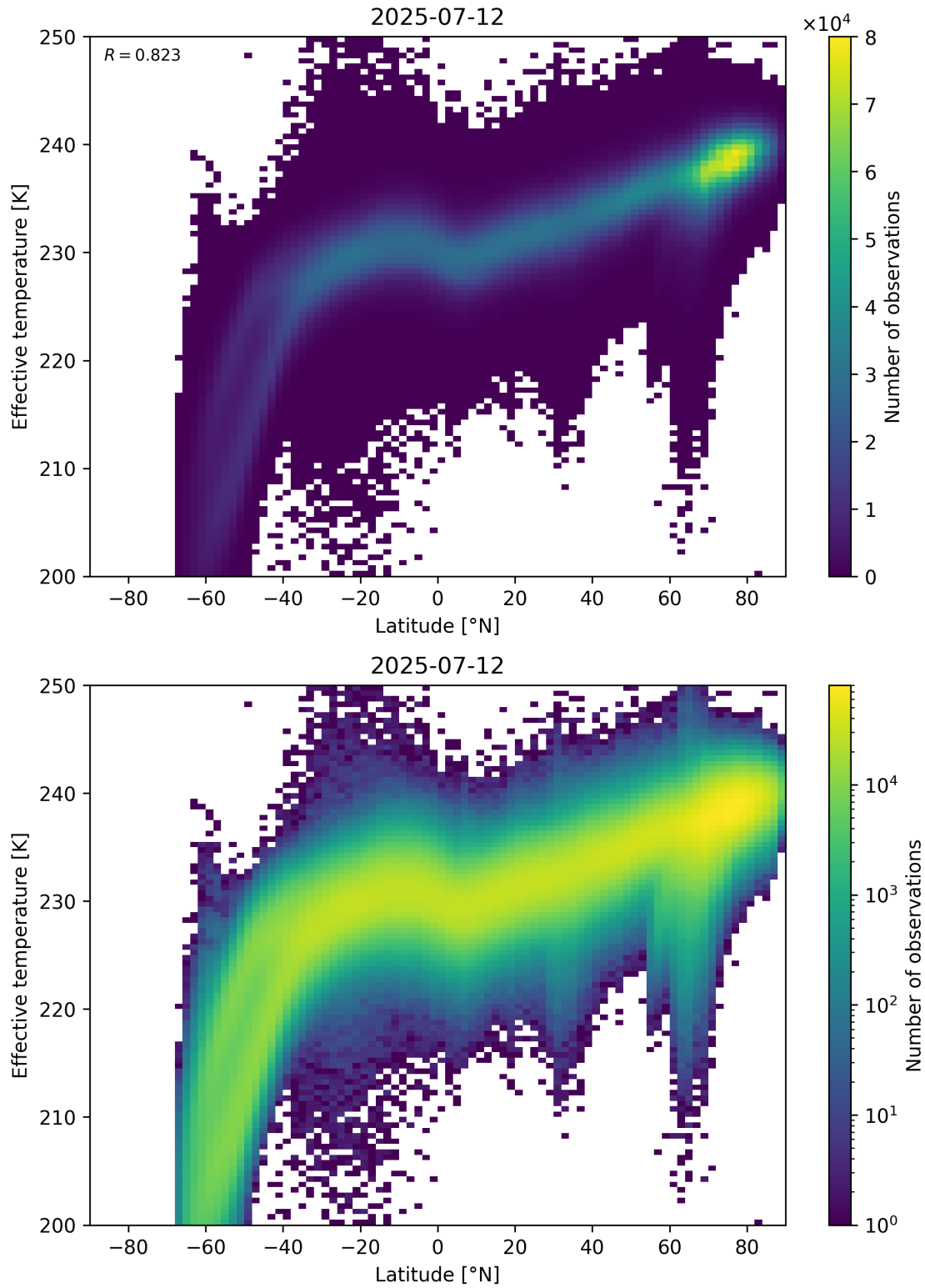
Figure 34: Scatter density plot of “Latitude” against “Effective temperature” for 2025-07-11 to 2025-07-13.
