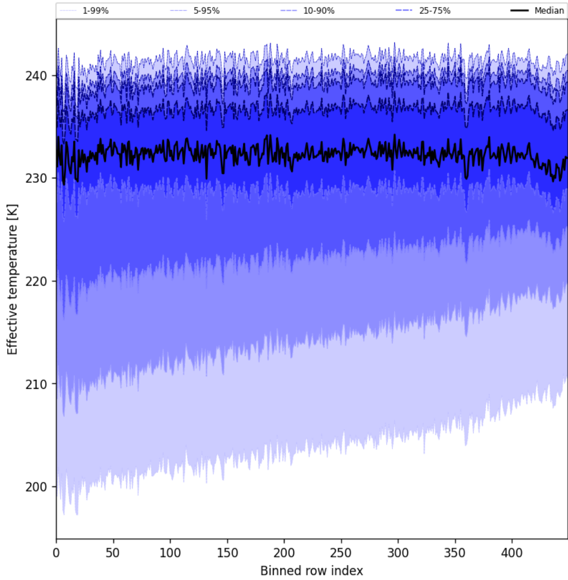
Figure 31: Along track statistics of “Effective temperature” for 2025-07-11 to 2025-07-13
