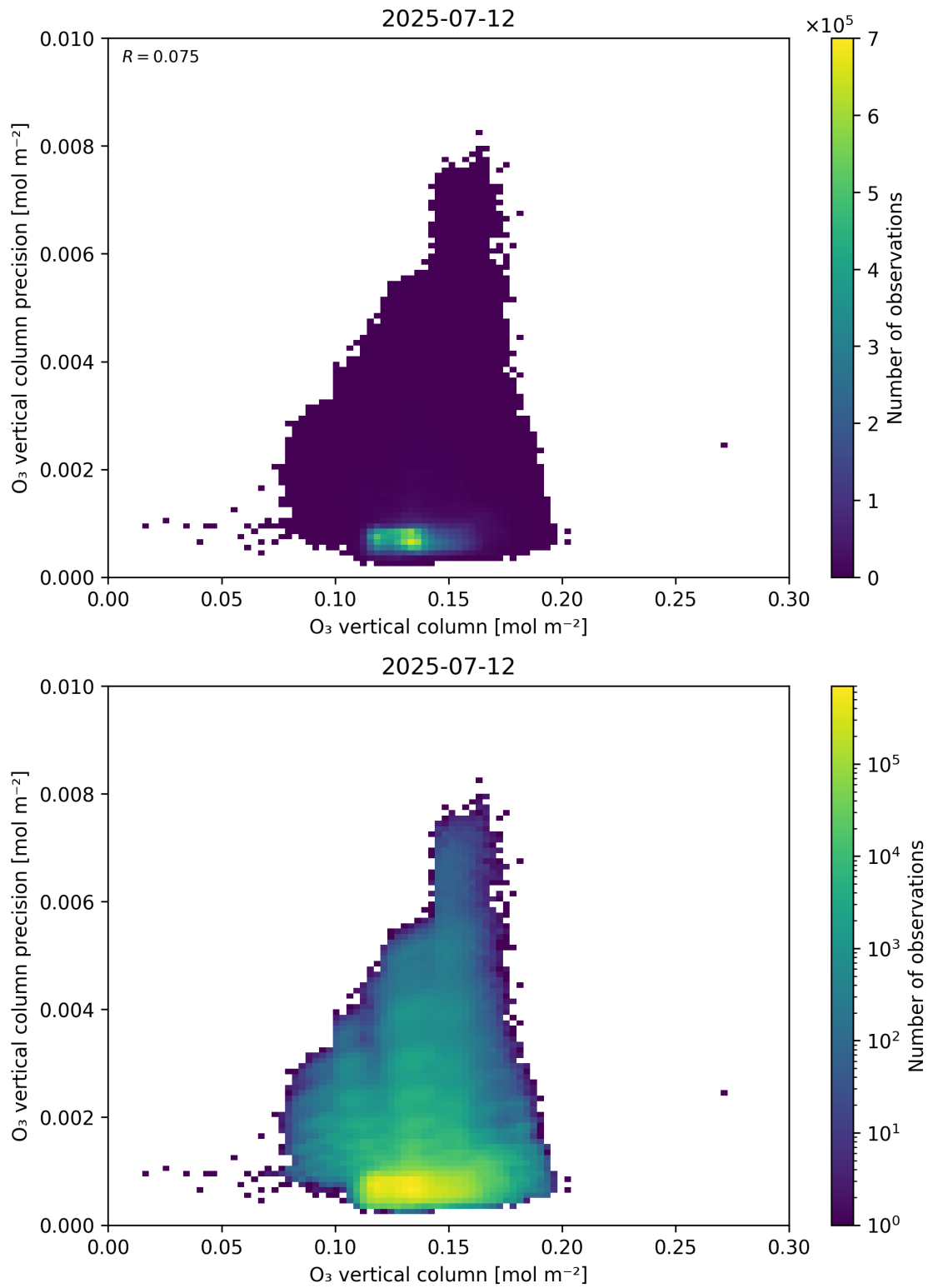
Figure 41: Scatter density plot of “O 3 vertical column” against “O 3 vertical column precision” for 2025-07-11 to 2025-07-13.
