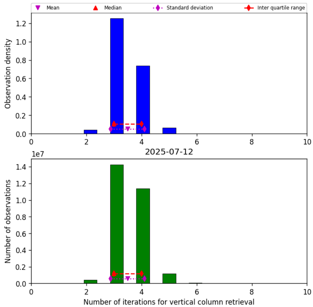
Figure 26: Histogram of “Number of iterations for vertical column retrieval” for 2025-07-11 to 2025-07-13
