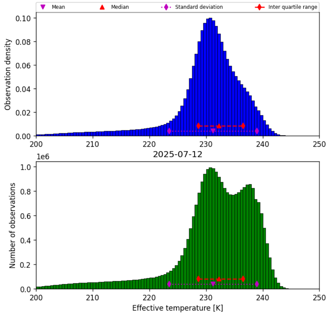
Figure 24: Histogram of “Effective temperature” for 2025-07-11 to 2025-07-13
