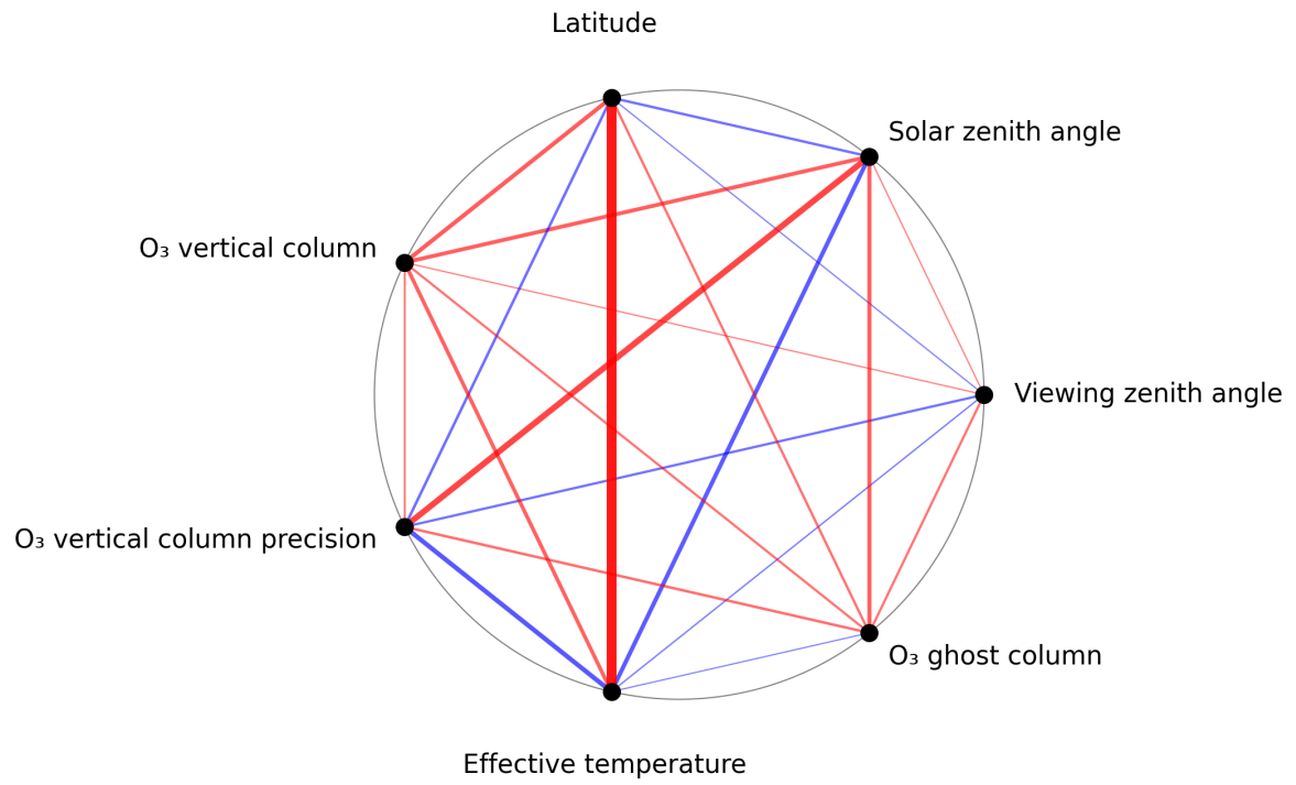
Figure 1: Map of correlation graph for 2025-07-11 to 2025-07-13.
