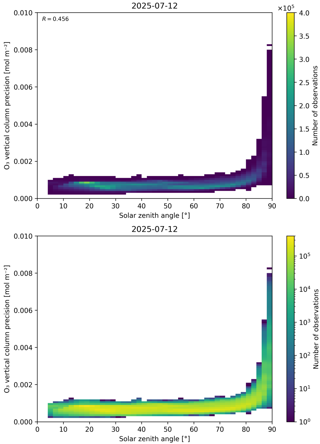
Figure 48: Scatter density plot of “Solar zenith angle” against “O 3 vertical column precision” for 2025-07-11 to 2025-07-13.
