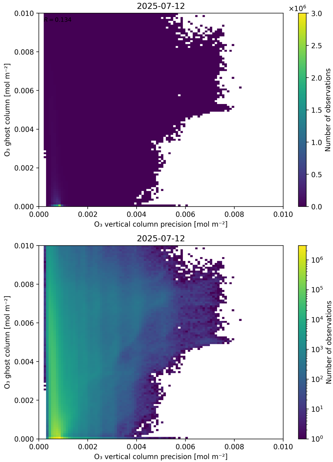
Figure 43: Scatter density plot of “ \text{O}_3 vertical column precision” against “ \text{O}_3 ghost column” for 2025-07-11 to 2025-07-13.
