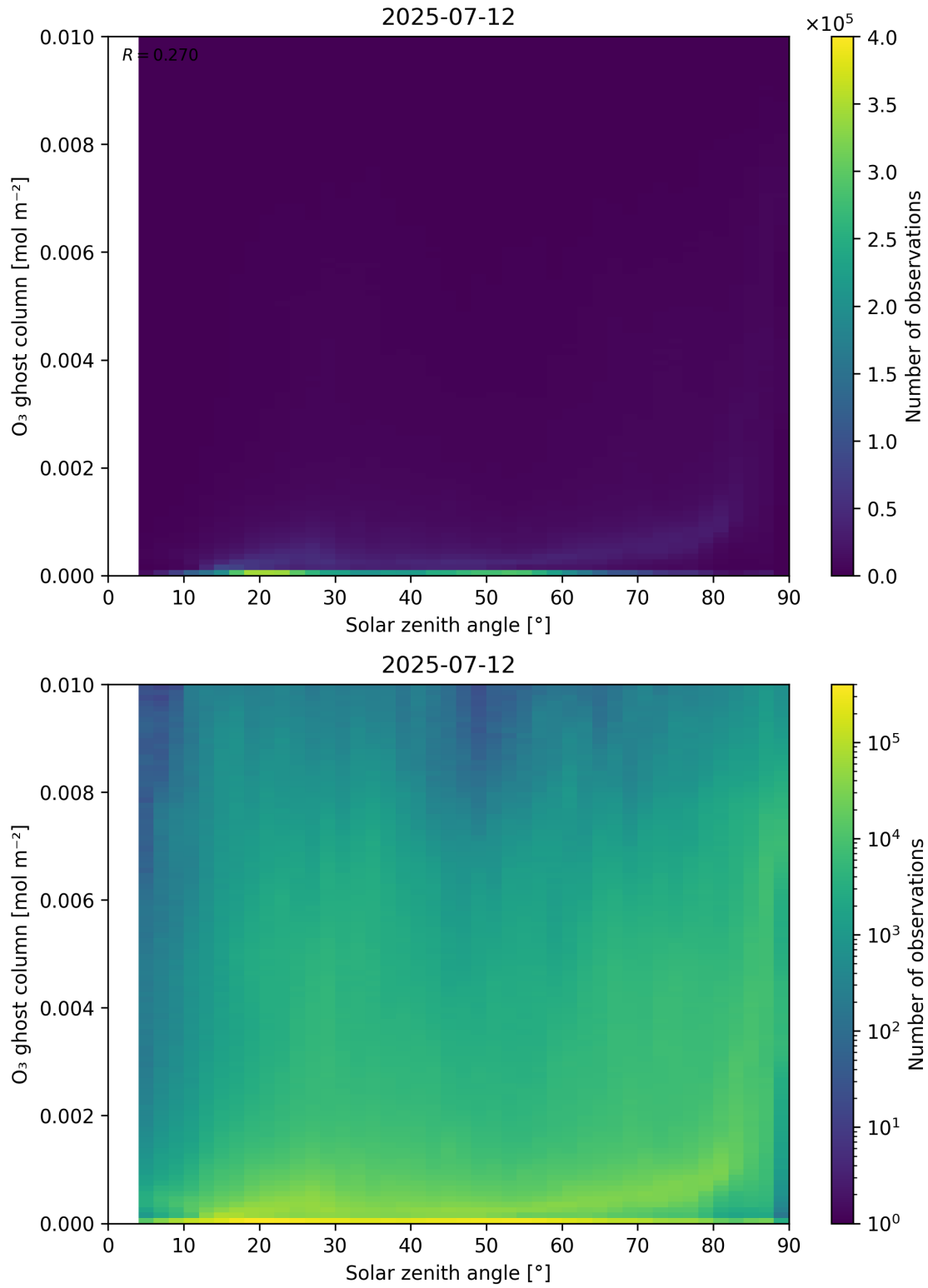
Figure 46: Scatter density plot of “Solar zenith angle” against “O 3 ghost column” for 2025-07-11 to 2025-07-13.
