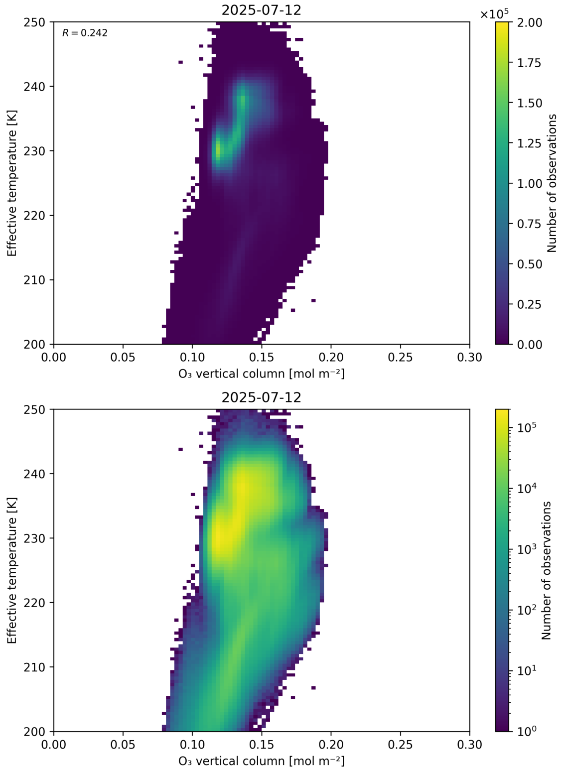
Figure 39: Scatter density plot of “O 3 vertical column” against “Effective temperature” for 2025-07-11 to 2025-07-13.
