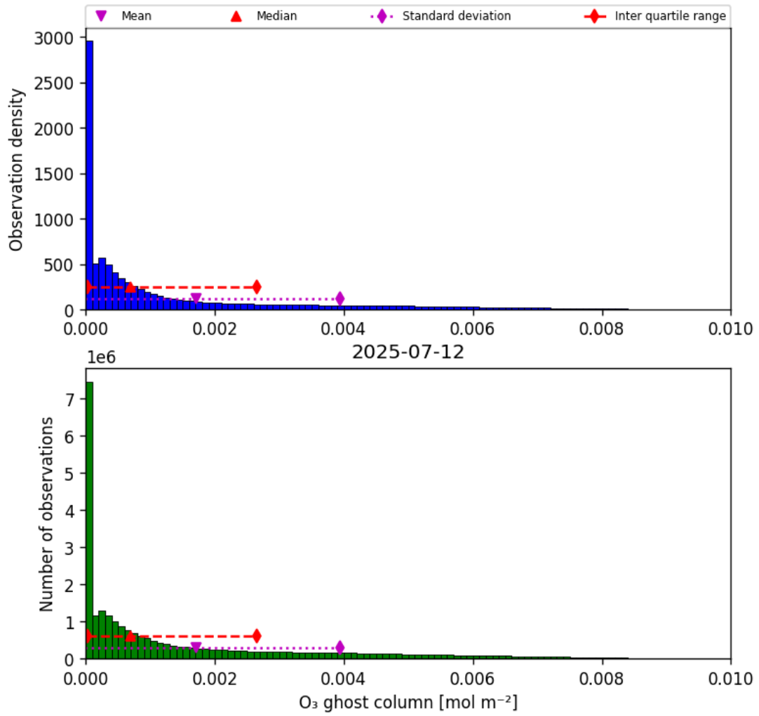
Figure 25: Histogram of “O 3 ghost column” for 2025-07-11 to 2025-07-13
