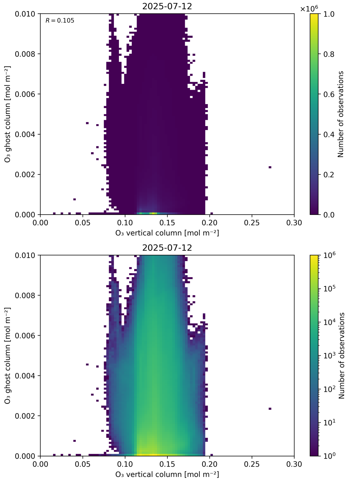
Figure 40: Scatter density plot of “O 3 vertical column” against “O 3 ghost column” for 2025-07-11 to 2025-07-13.
