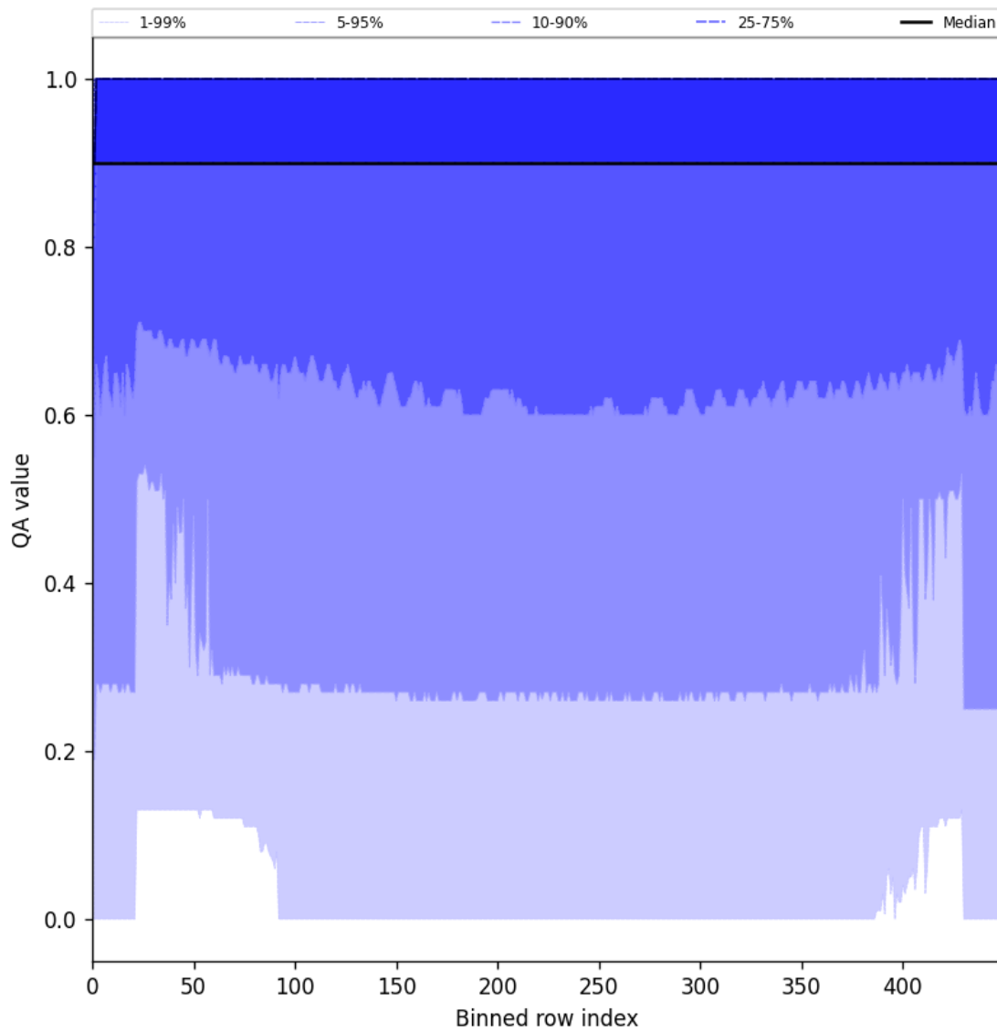
Figure 27: Along track statistics of “QA value” for 2025-07-11 to 2025-07-13
