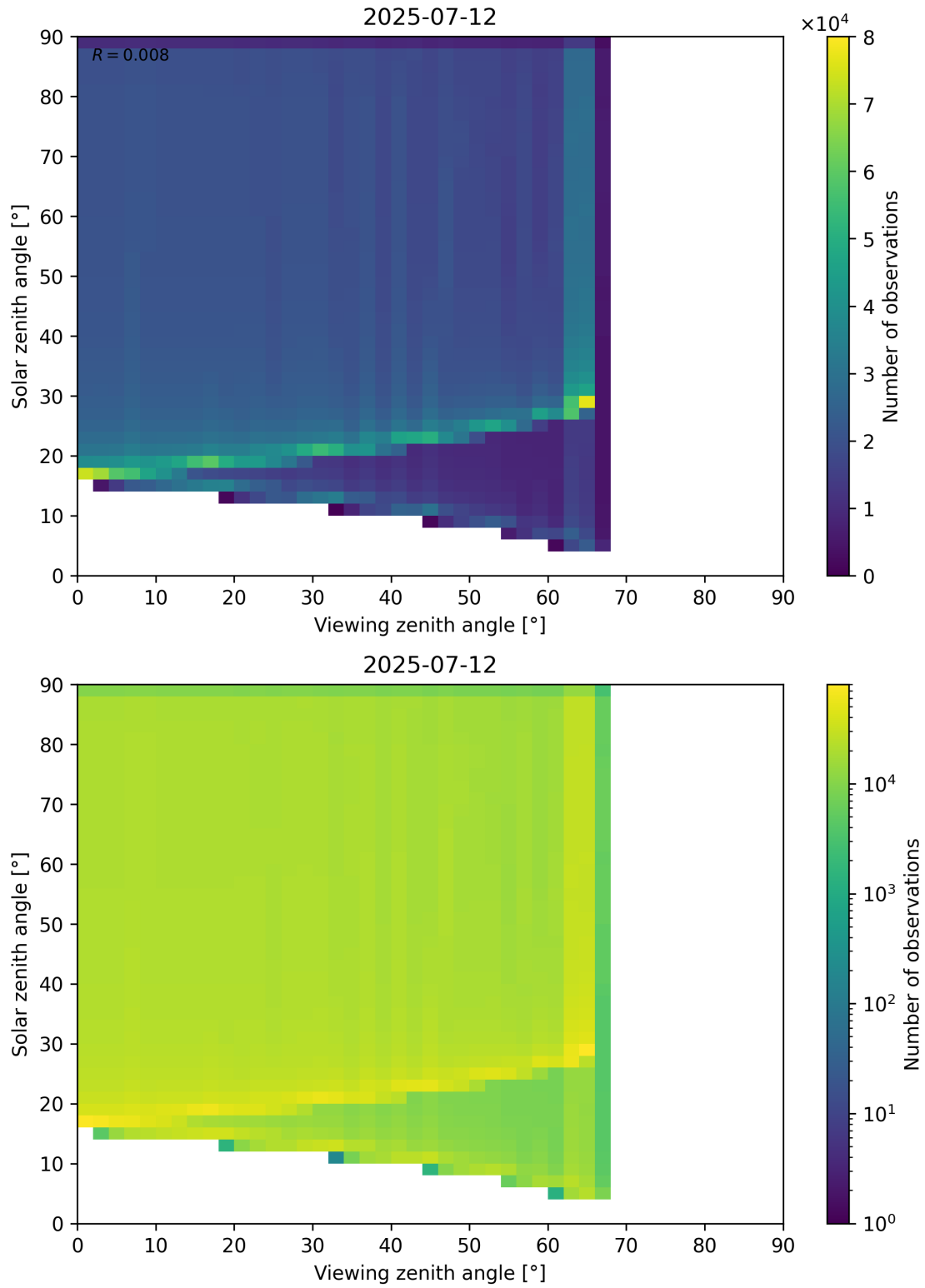
Figure 54: Scatter density plot of “Viewing zenith angle” against “Solar zenith angle” for 2025-07-11 to 2025-07-13.
