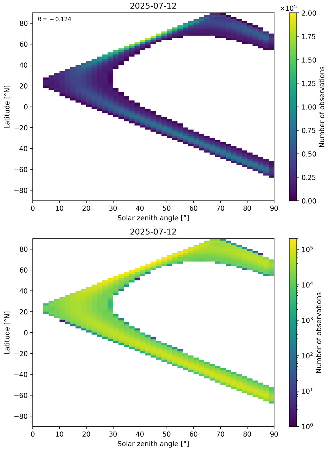
Figure 44: Scatter density plot of “Solar zenith angle” against “Latitude” for 2025-07-11 to 2025-07-13.
