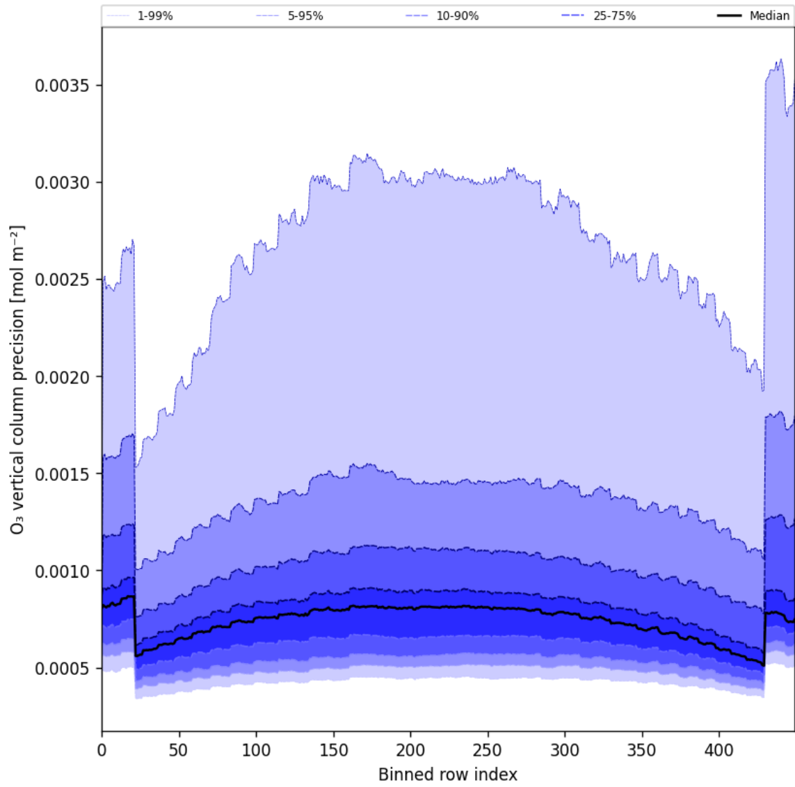
Figure 29: Along track statistics of “O 3 vertical column precision” for 2025-07-11 to 2025-07-13
