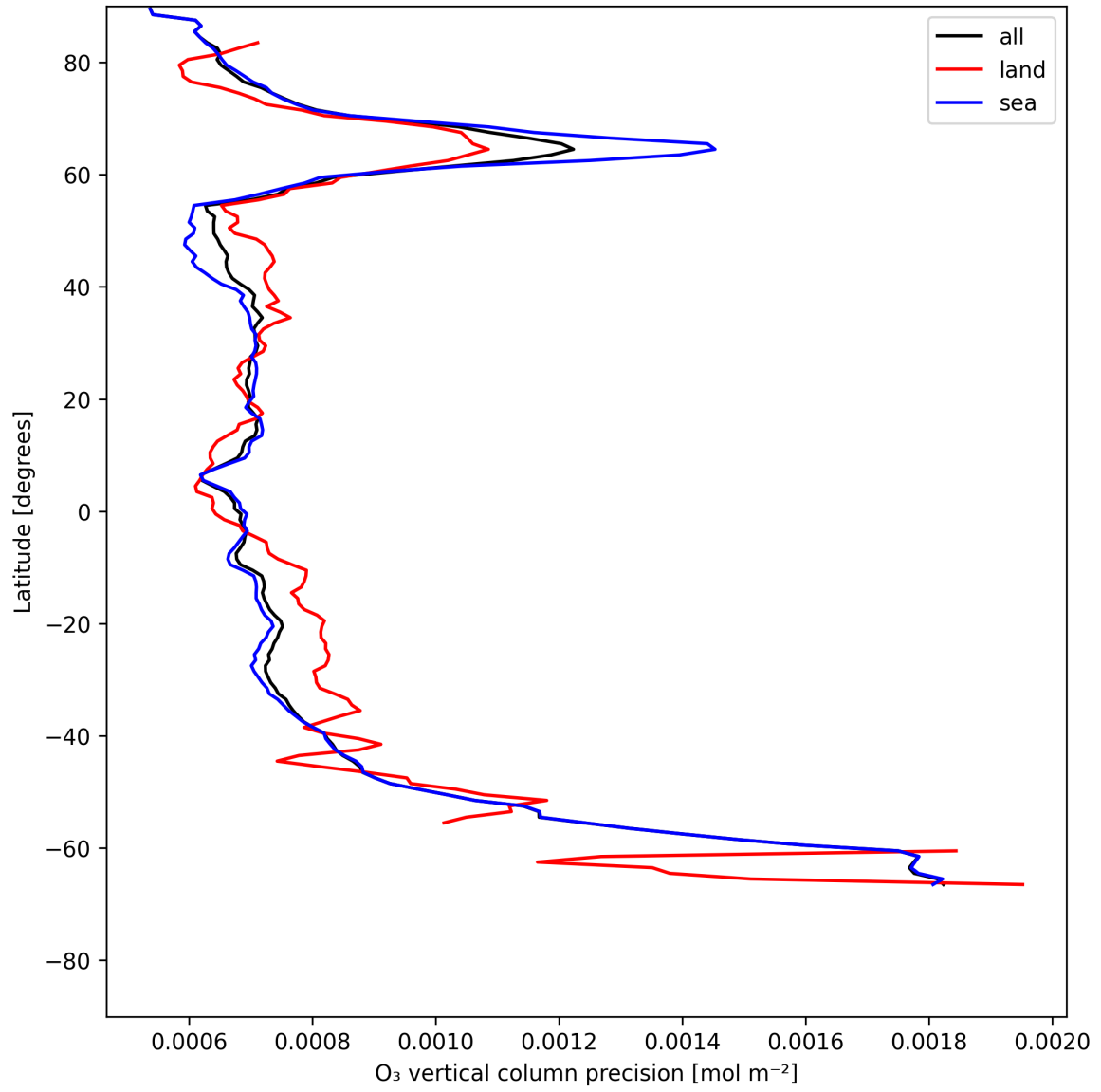
Figure 15: Zonal average of “O 3 vertical column precision” for 2025-07-11 to 2025-07-13.
