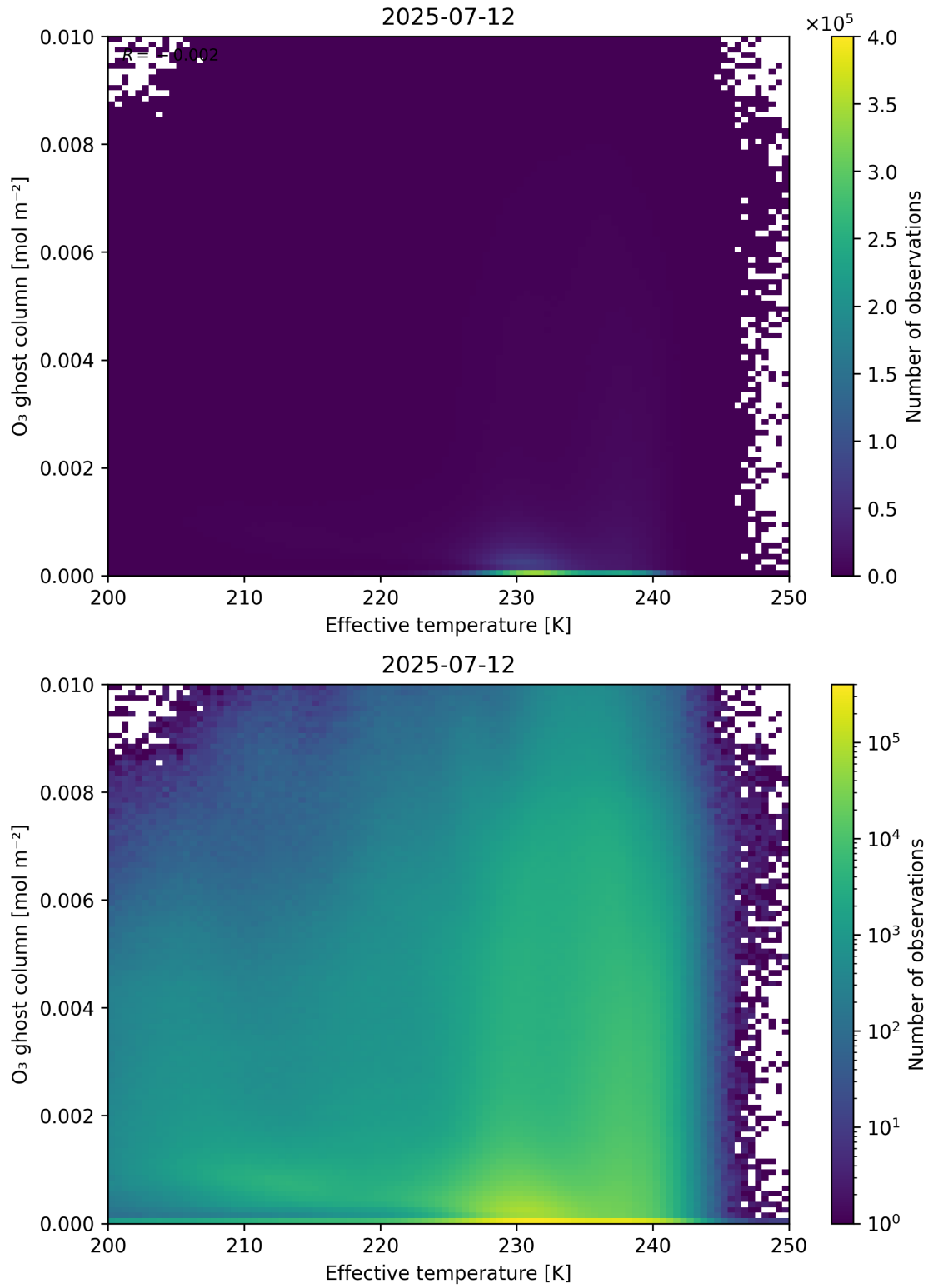
Figure 38: Scatter density plot of “Effective temperature” against “O 3 ghost column” for 2025-07-11 to 2025-07-13.
