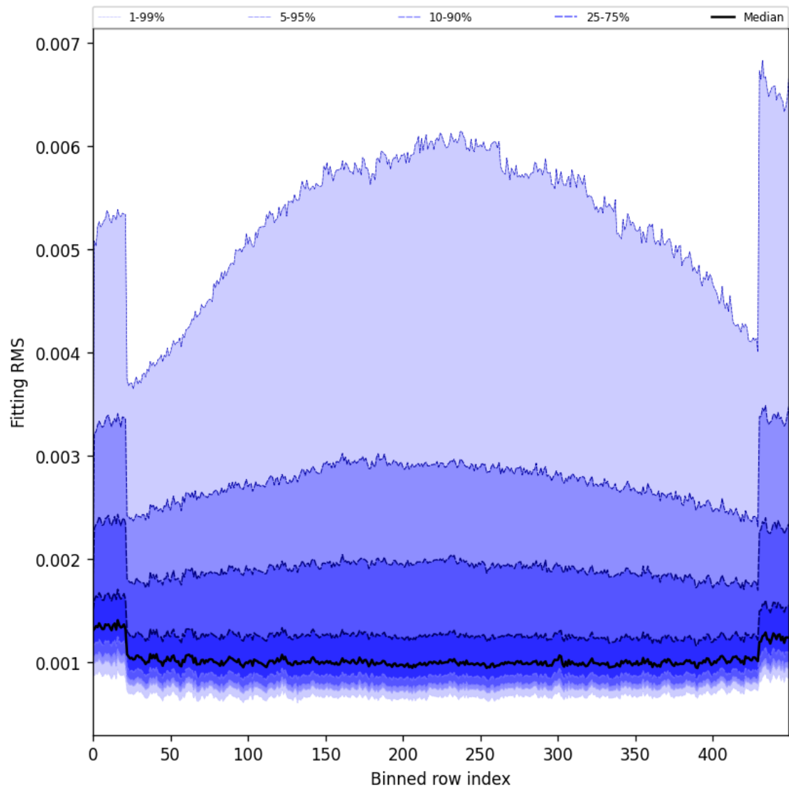
Figure 30: Along track statistics of “Fitting RMS” for 2025-07-11 to 2025-07-13
