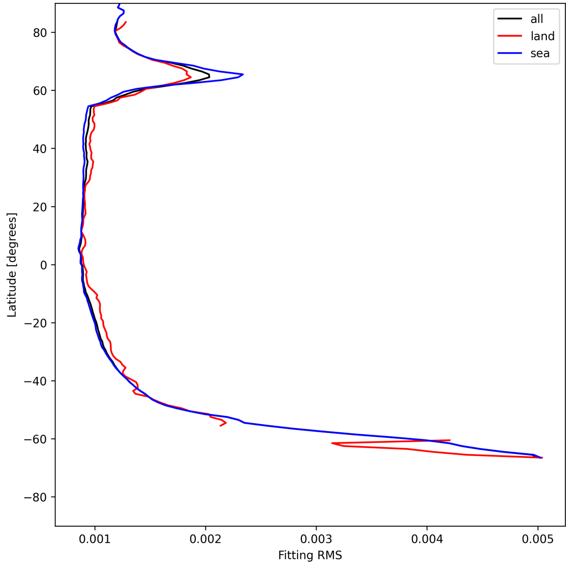
Figure 16: Zonal average of “Fitting RMS” for 2025-07-11 to 2025-07-13.
