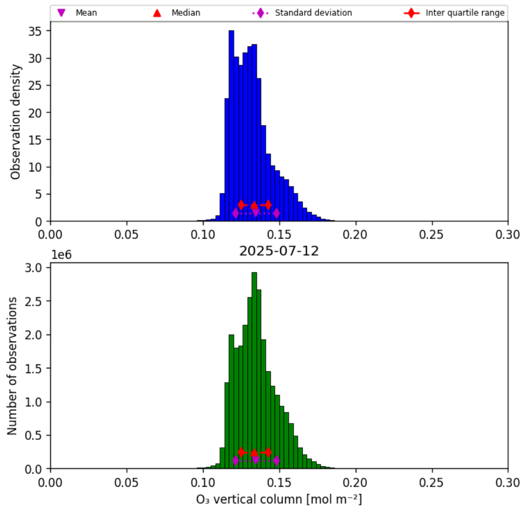
Figure 21: Histogram of “O 3 vertical column” for 2025-07-11 to 2025-07-13
