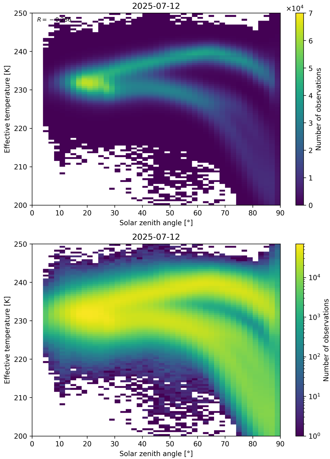
Figure 45: Scatter density plot of “Solar zenith angle” against “Effective temperature” for 2025-07-11 to 2025-07-13.
