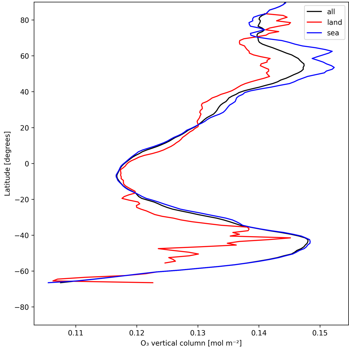
Figure 14: Zonal average of “O 3 vertical column” for 2025-07-11 to 2025-07-13.
