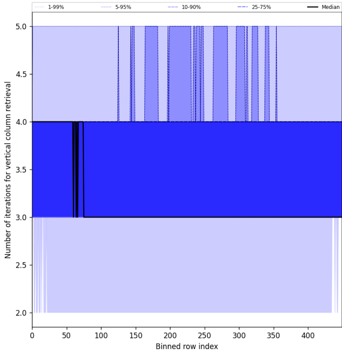
Figure 33: Along track statistics of “Number of iterations for vertical column retrieval” for 2025-07-11 to 2025-07-13
