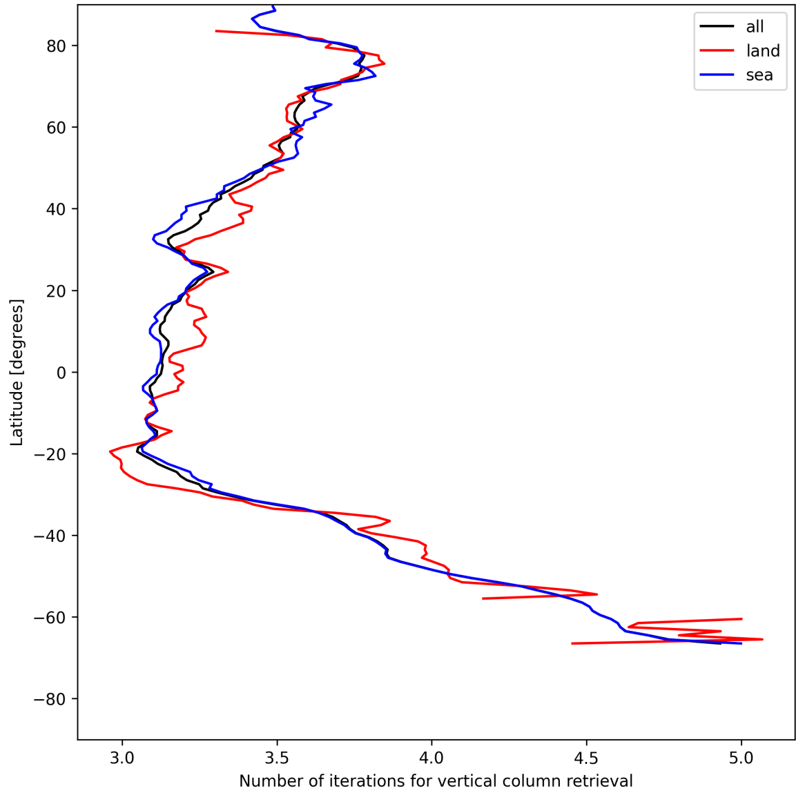
Figure 19: Zonal average of “Number of iterations for vertical column retrieval” for 2025-07-11 to 2025-07-13.
