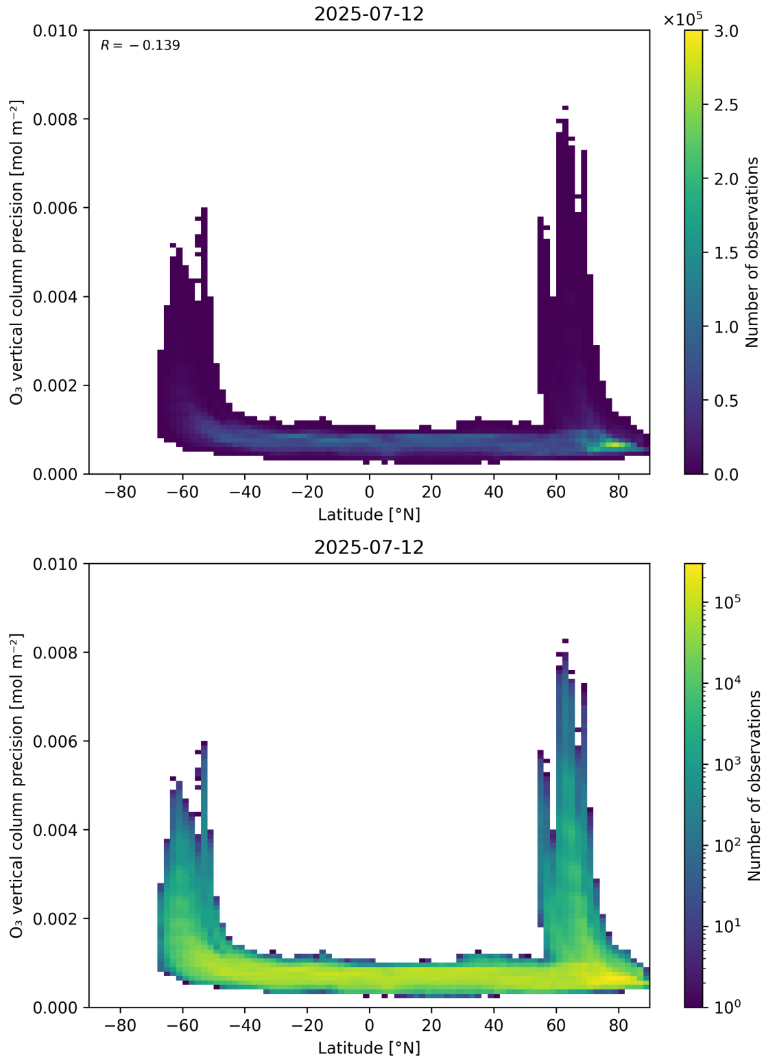
Figure 37: Scatter density plot of “Latitude” against “O 3 vertical column precision” for 2025-07-11 to 2025-07-13.
