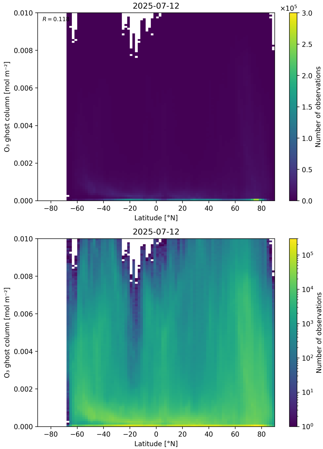
Figure 35: Scatter density plot of “Latitude” against “O 3 ghost column” for 2025-07-11 to 2025-07-13.
