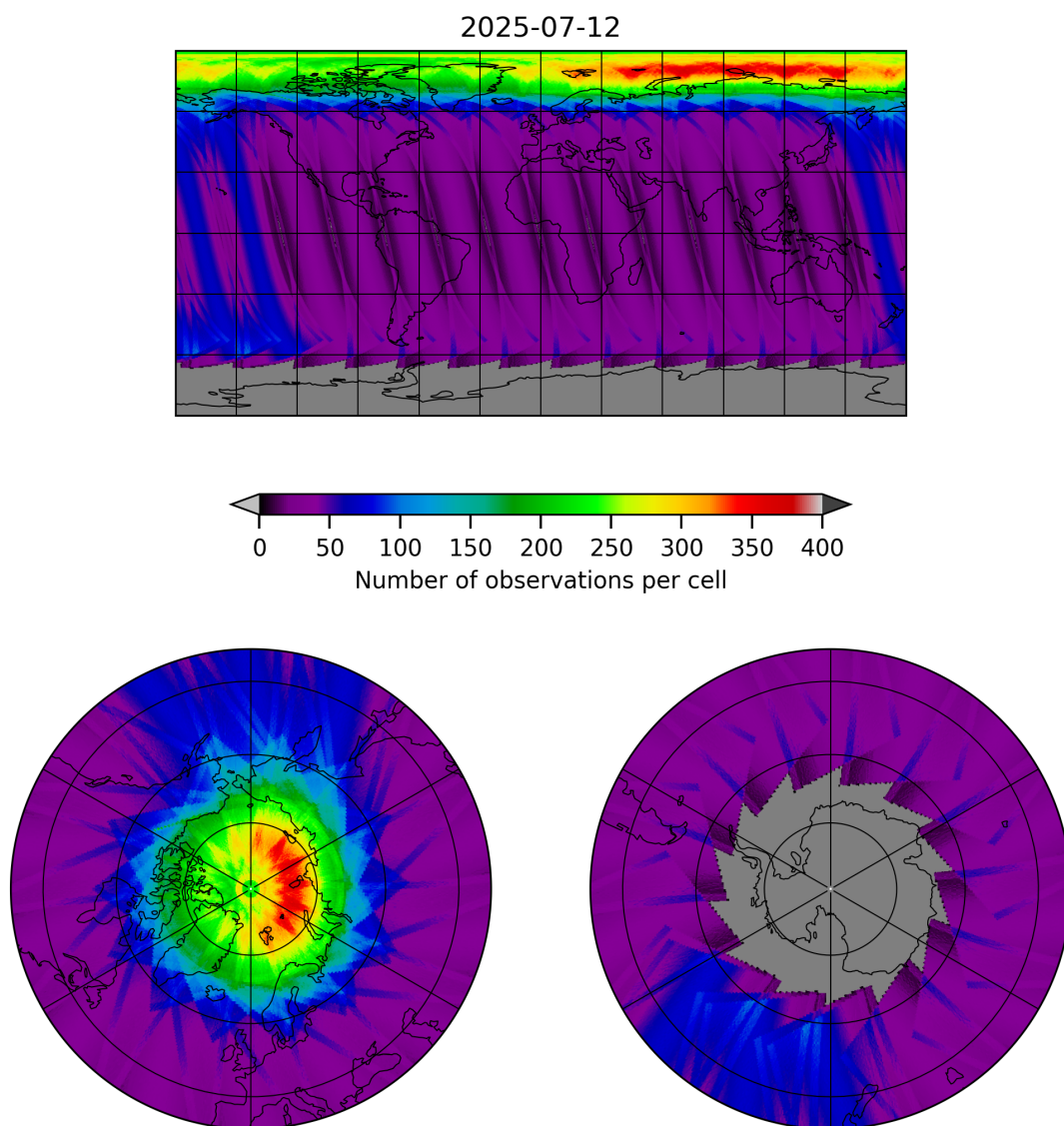
Figure 12: Map of the number of observations for 2025-07-11 to 2025-07-13
