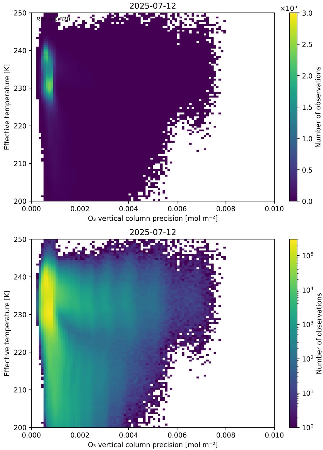
Figure 42: Scatter density plot of “O 3 vertical column precision” against “Effective temperature” for 2025-07-11 to 2025-07-13.
