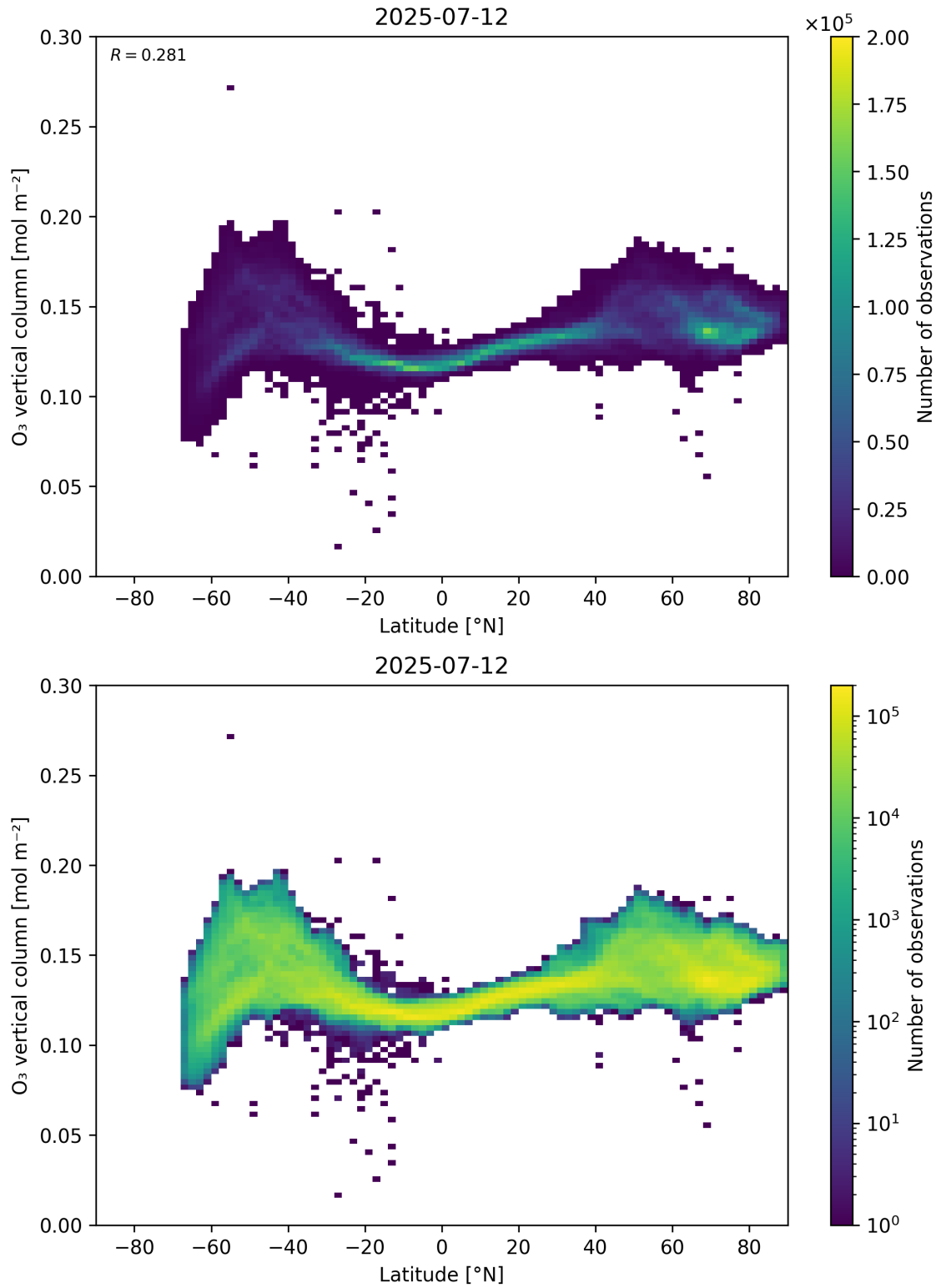
Figure 36: Scatter density plot of “Latitude” against “O 3 vertical column” for 2025-07-11 to 2025-07-13.
