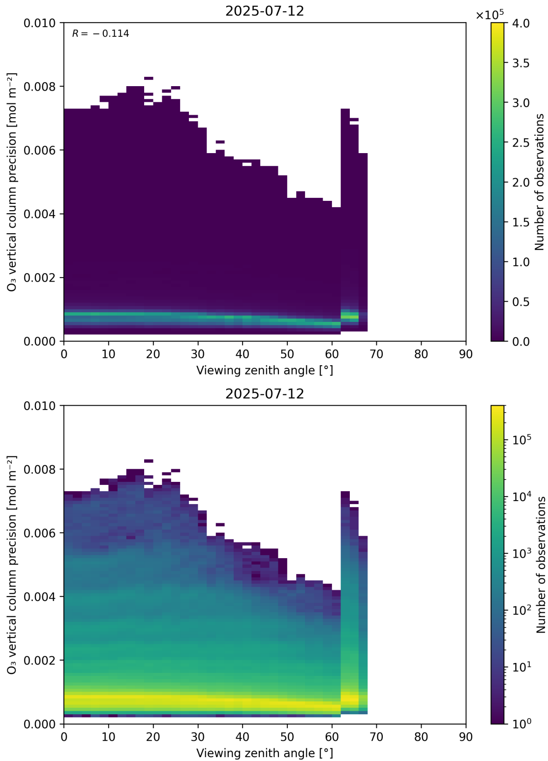
Figure 53: Scatter density plot of “Viewing zenith angle” against “O 3 vertical column precision” for 2025-07-11 to 2025-07-13.
