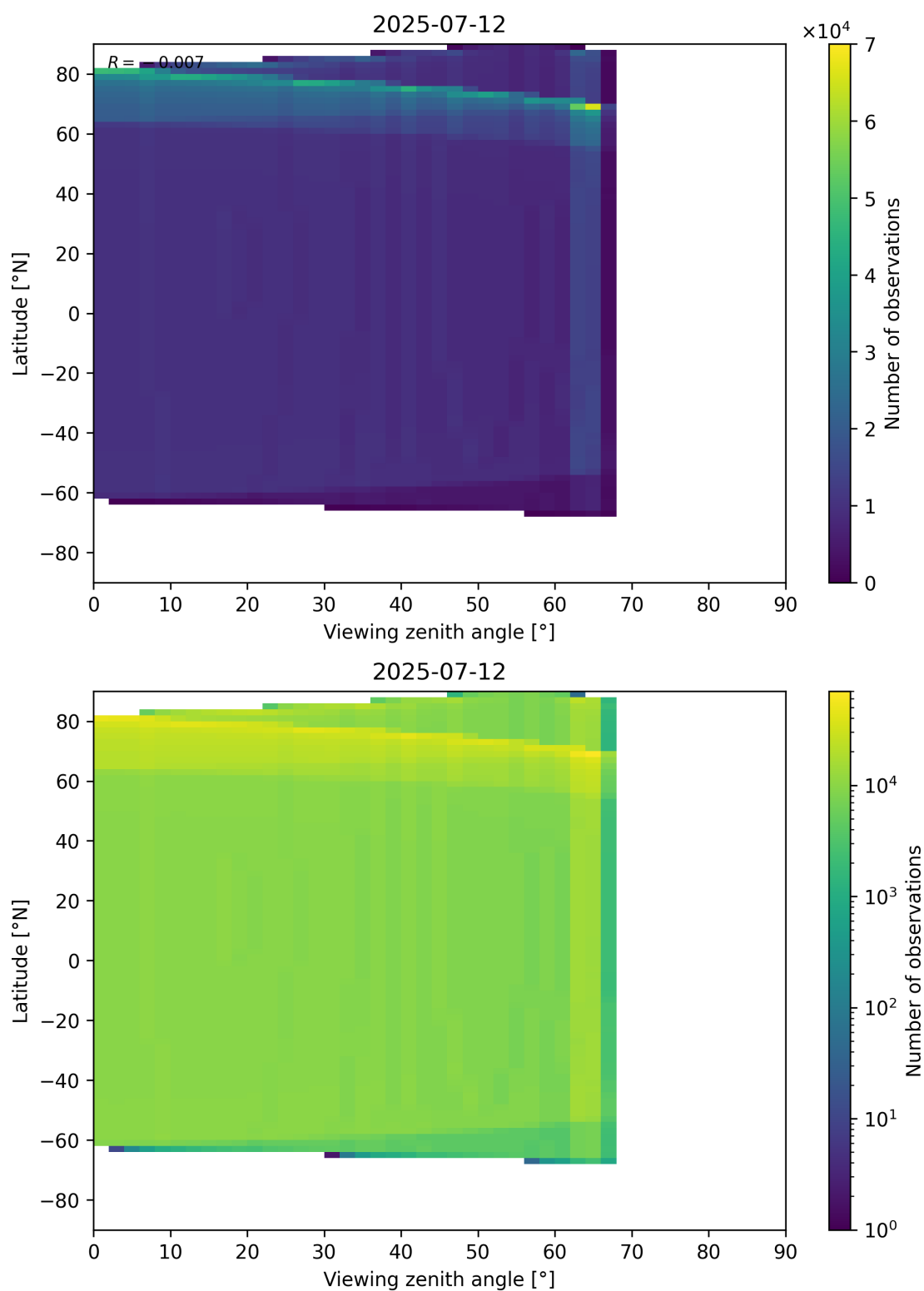
Figure 49: Scatter density plot of “Viewing zenith angle” against “Latitude” for 2025-07-11 to 2025-07-13.
