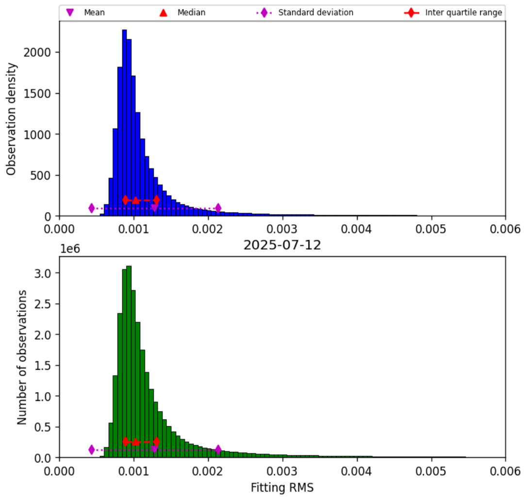
Figure 23: Histogram of “Fitting RMS” for 2025-07-11 to 2025-07-13
