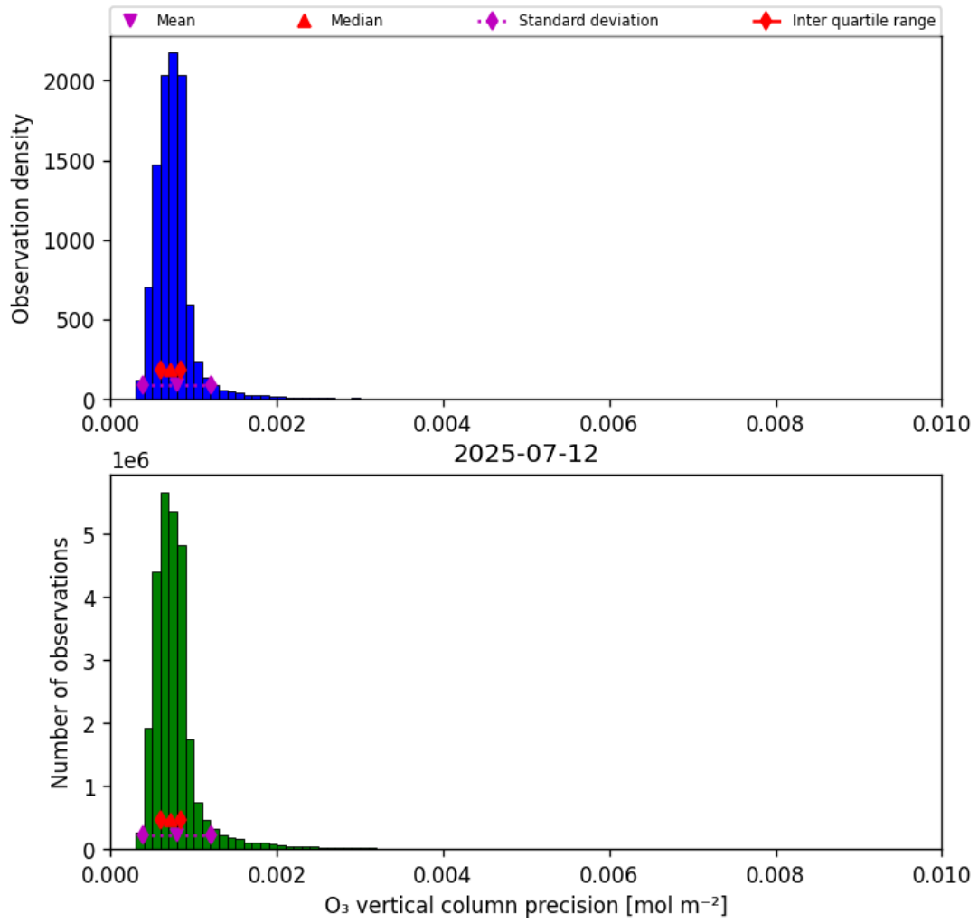
Figure 22: Histogram of “O 3 vertical column precision” for 2025-07-11 to 2025-07-13
