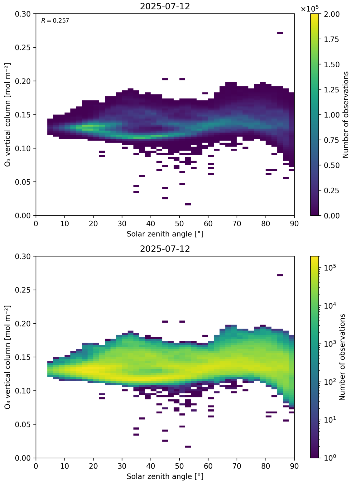
Figure 47: Scatter density plot of “Solar zenith angle” against “O 3 vertical column” for 2025-07-11 to 2025-07-13.
