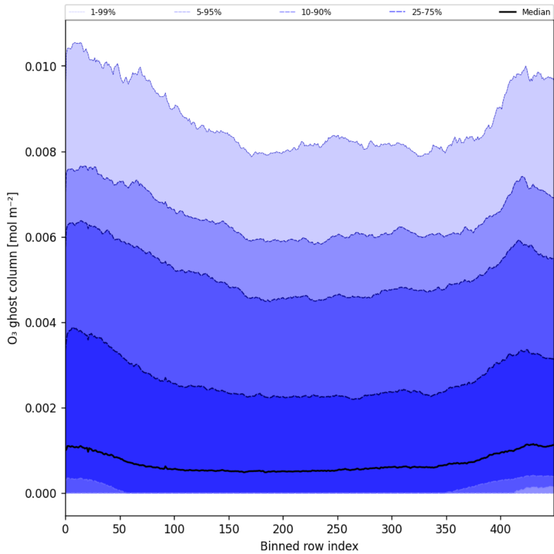
Figure 32: Along track statistics of “O 3 ghost column” for 2025-07-11 to 2025-07-13
