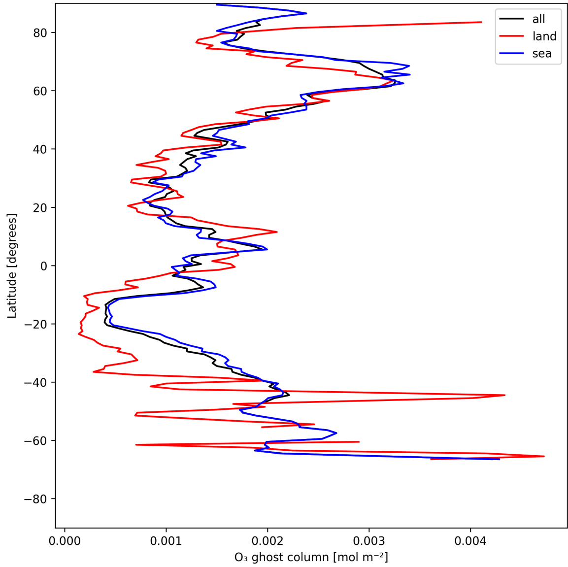
Figure 18: Zonal average of "O 3 ghost column" for 2025-07-11 to 2025-07-13.
