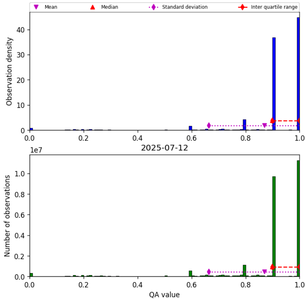
Figure 20: Histogram of “QA value” for 2025-07-11 to 2025-07-13
