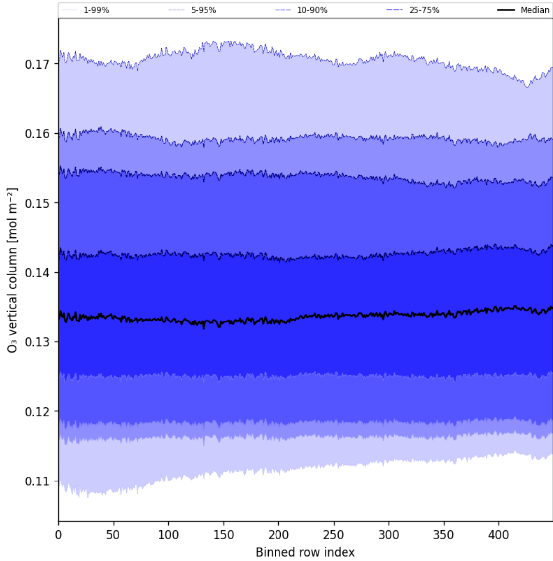
Figure 28: Along track statistics of “O 3 vertical column” for 2025-07-11 to 2025-07-13
