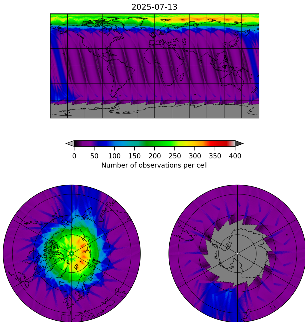
Figure 12: Map of the number of observations for 2025-07-13 to 2025-07-14
