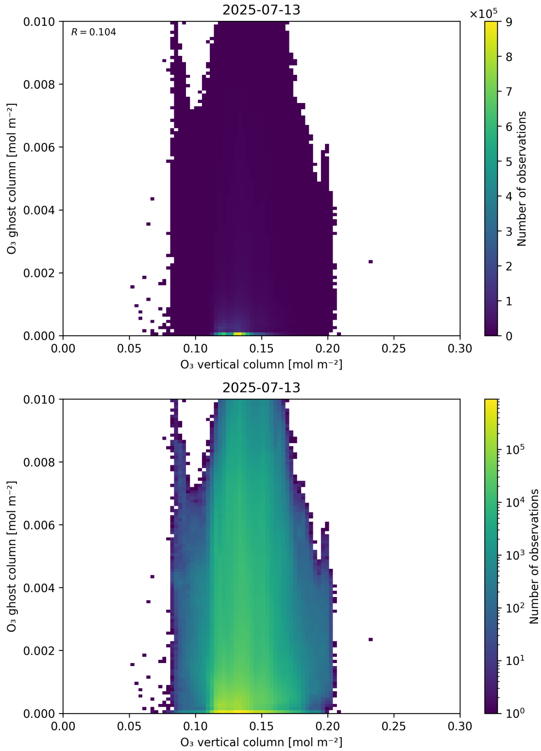
Figure 40: Scatter density plot of “O 3 vertical column” against “O 3 ghost column” for 2025-07-13 to 2025-07-14.
