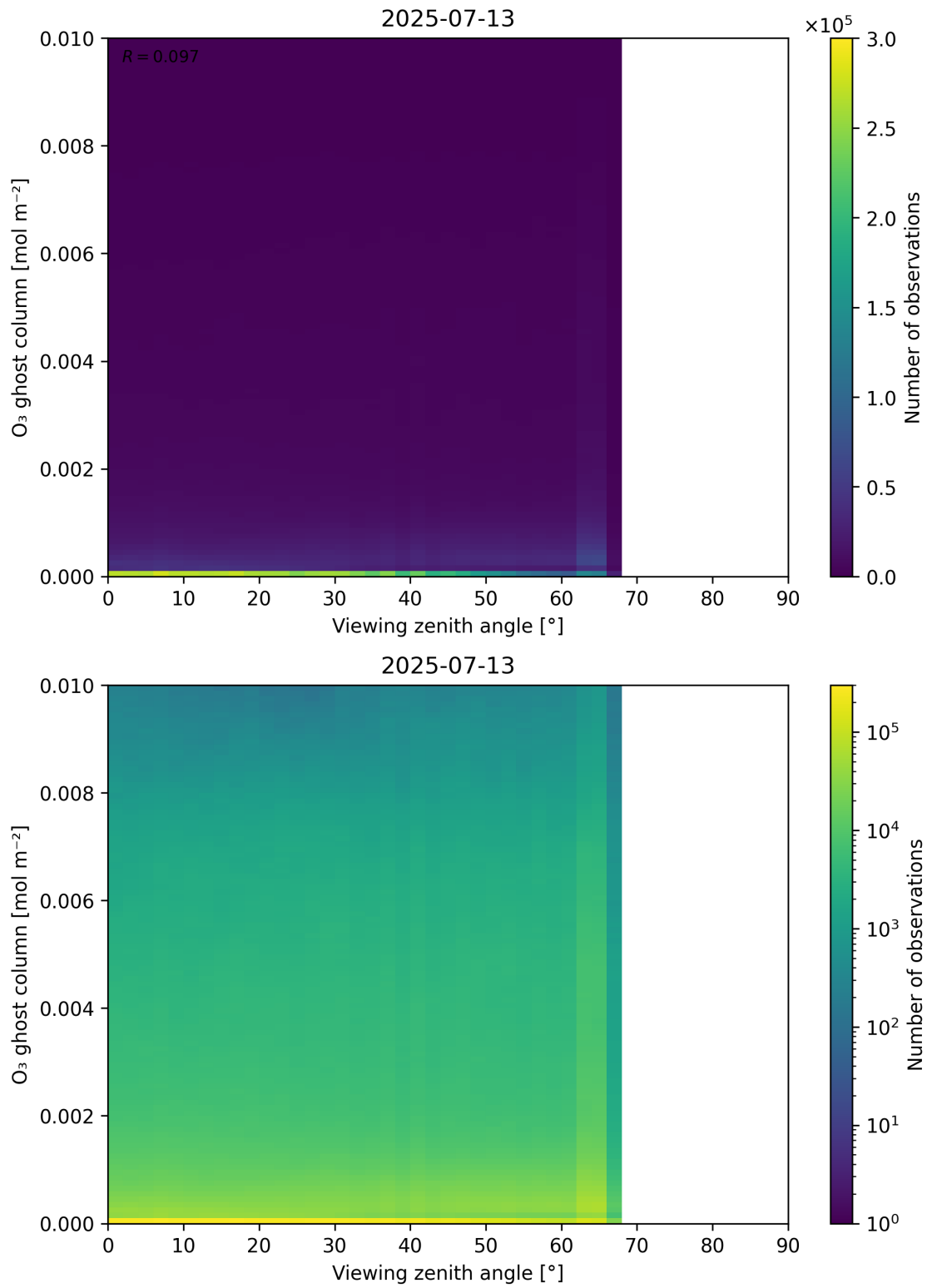
Figure 51: Scatter density plot of “Viewing zenith angle” against “O 3 ghost column” for 2025-07-13 to 2025-07-14.
