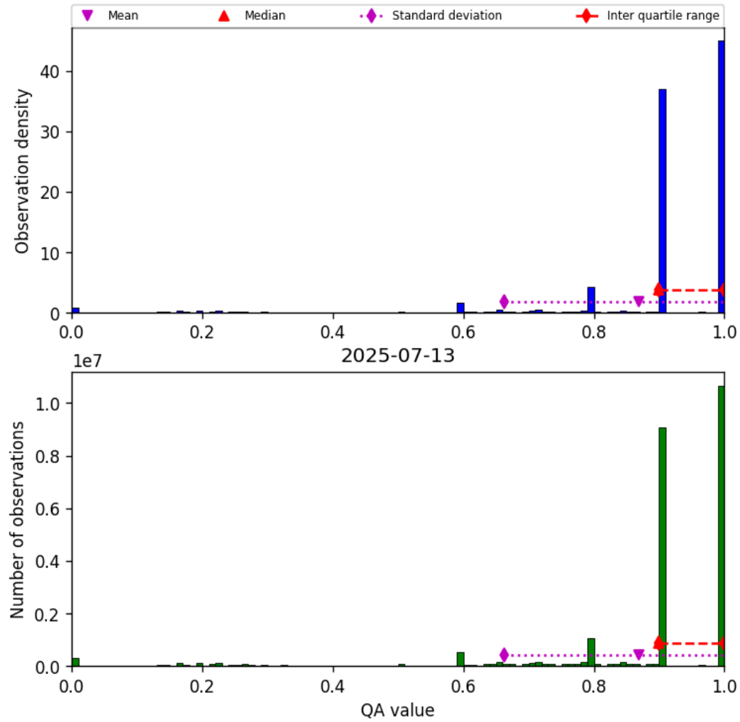
Figure 20: Histogram of “QA value” for 2025-07-13 to 2025-07-14
