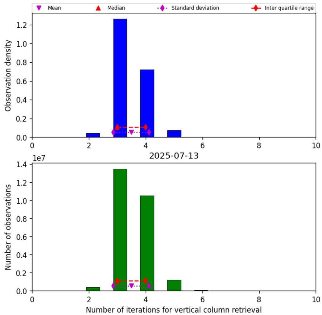
Figure 26: Histogram of “Number of iterations for vertical column retrieval” for 2025-07-13 to 2025-07-14
