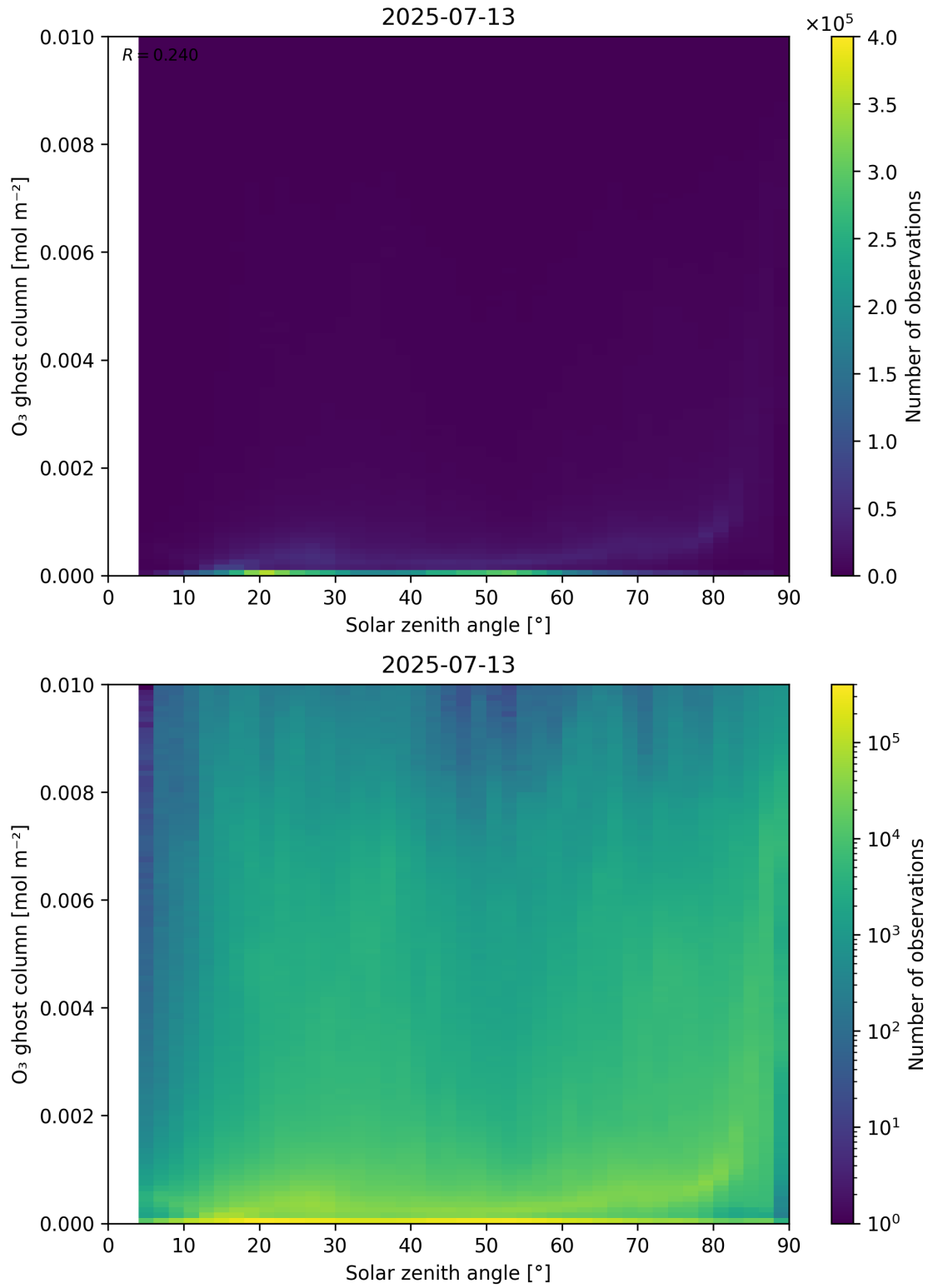
Figure 46: Scatter density plot of “Solar zenith angle” against “O 3 ghost column” for 2025-07-13 to 2025-07-14.
