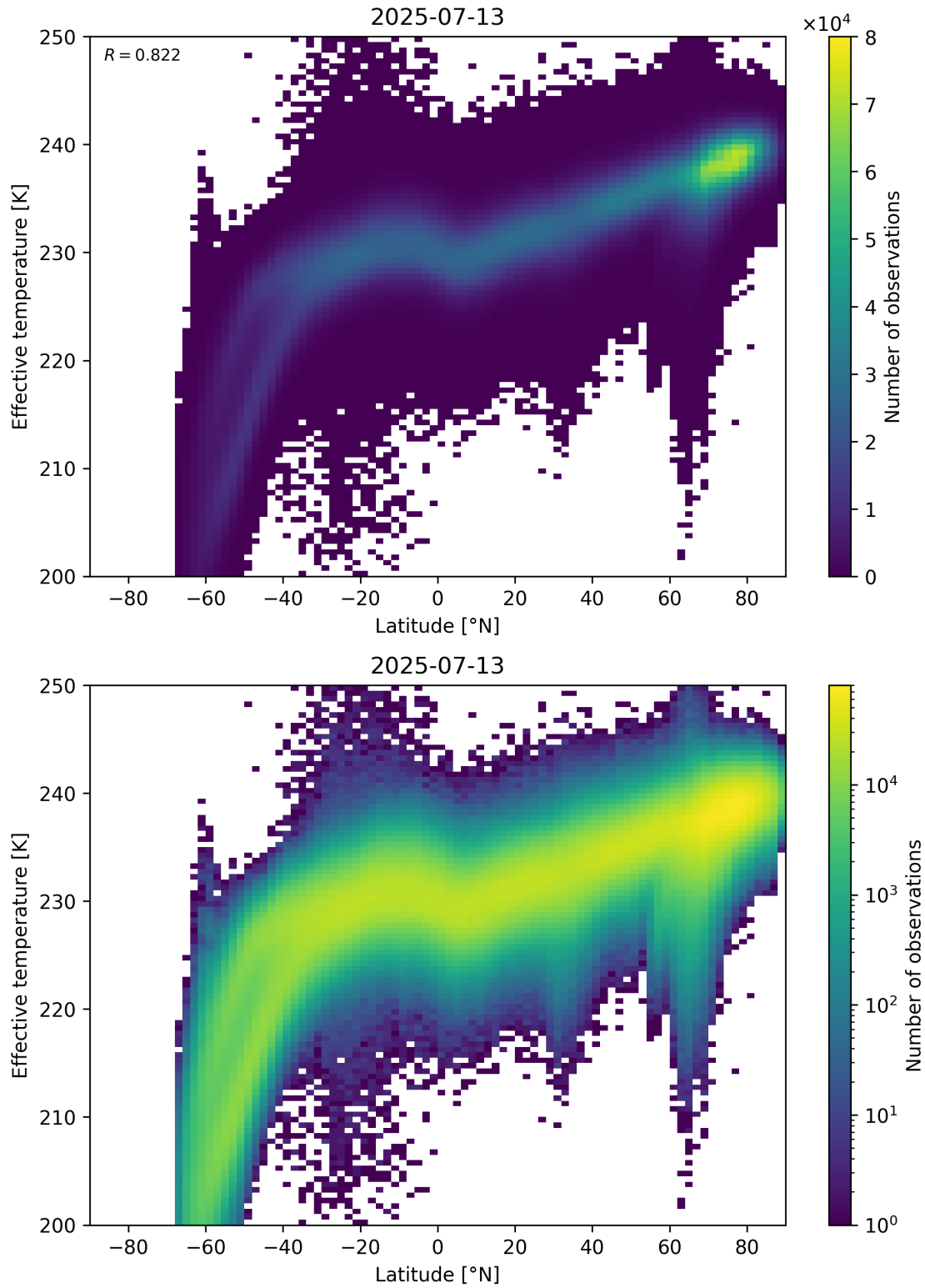
Figure 34: Scatter density plot of “Latitude” against “Effective temperature” for 2025-07-13 to 2025-07-14.
