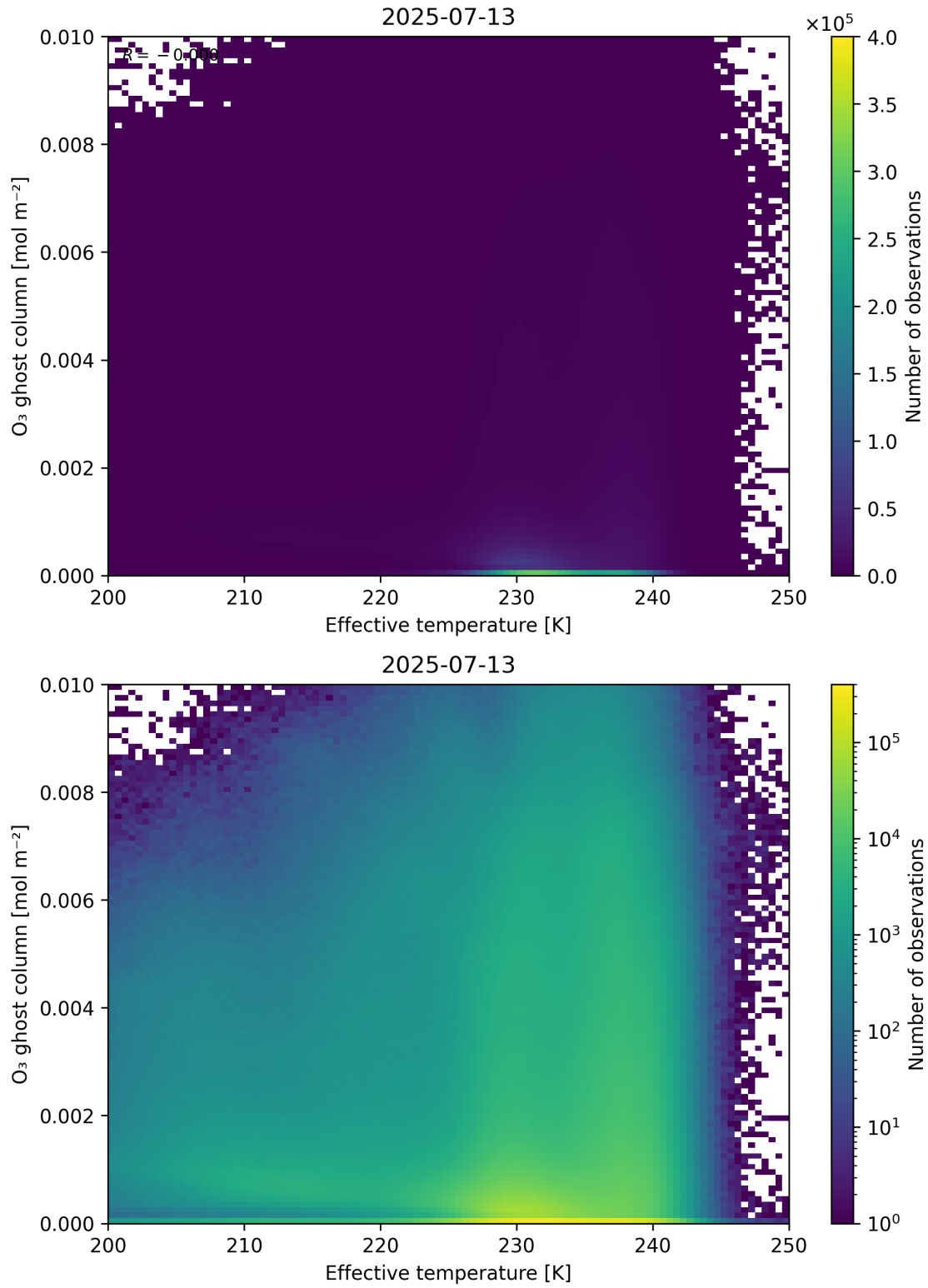
Figure 38: Scatter density plot of “Effective temperature” against “O 3 ghost column” for 2025-07-13 to 2025-07-14.
