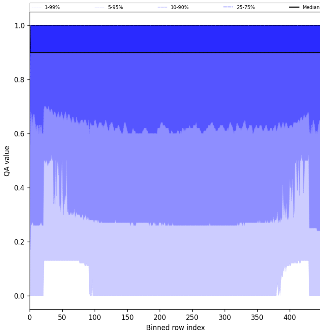
Figure 27: Along track statistics of “QA value” for 2025-07-13 to 2025-07-14
