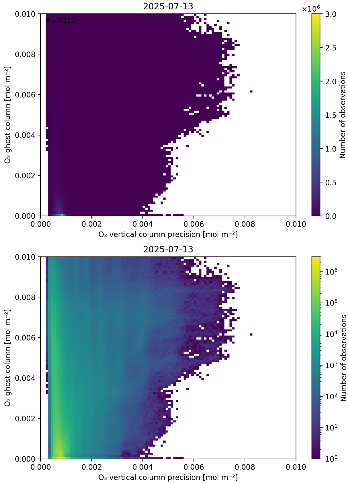
Figure 43: Scatter density plot of “ O_3 vertical column precision” against “ O_3 ghost column” for 2025-07-13 to 2025-07-14.
