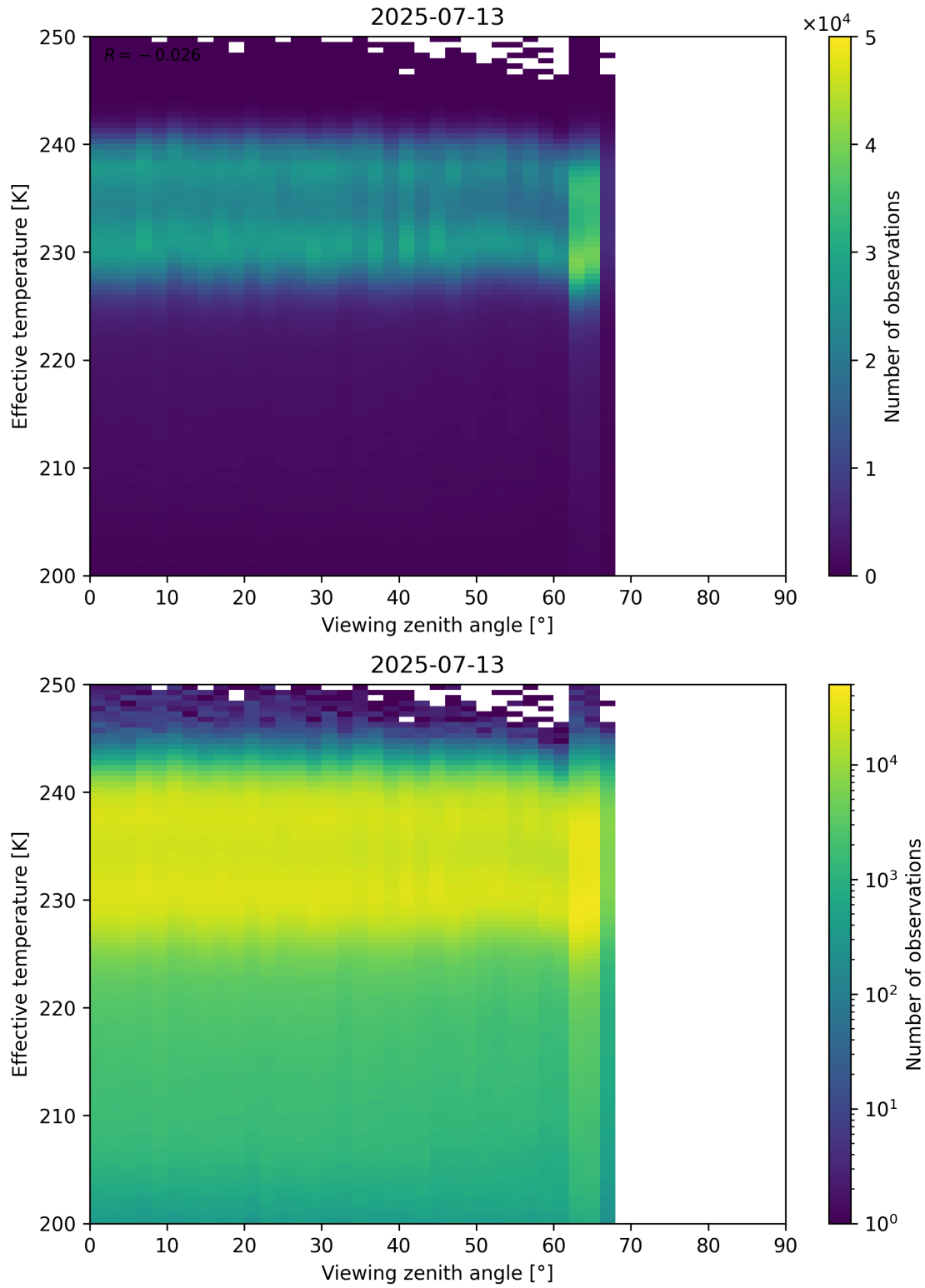
Figure 50: Scatter density plot of “Viewing zenith angle” against “Effective temperature” for 2025-07-13 to 2025-07-14.
