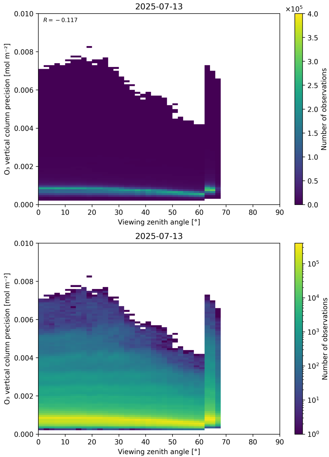
Figure 53: Scatter density plot of “Viewing zenith angle” against “O 3 vertical column precision” for 2025-07-13 to 2025-07-14.
