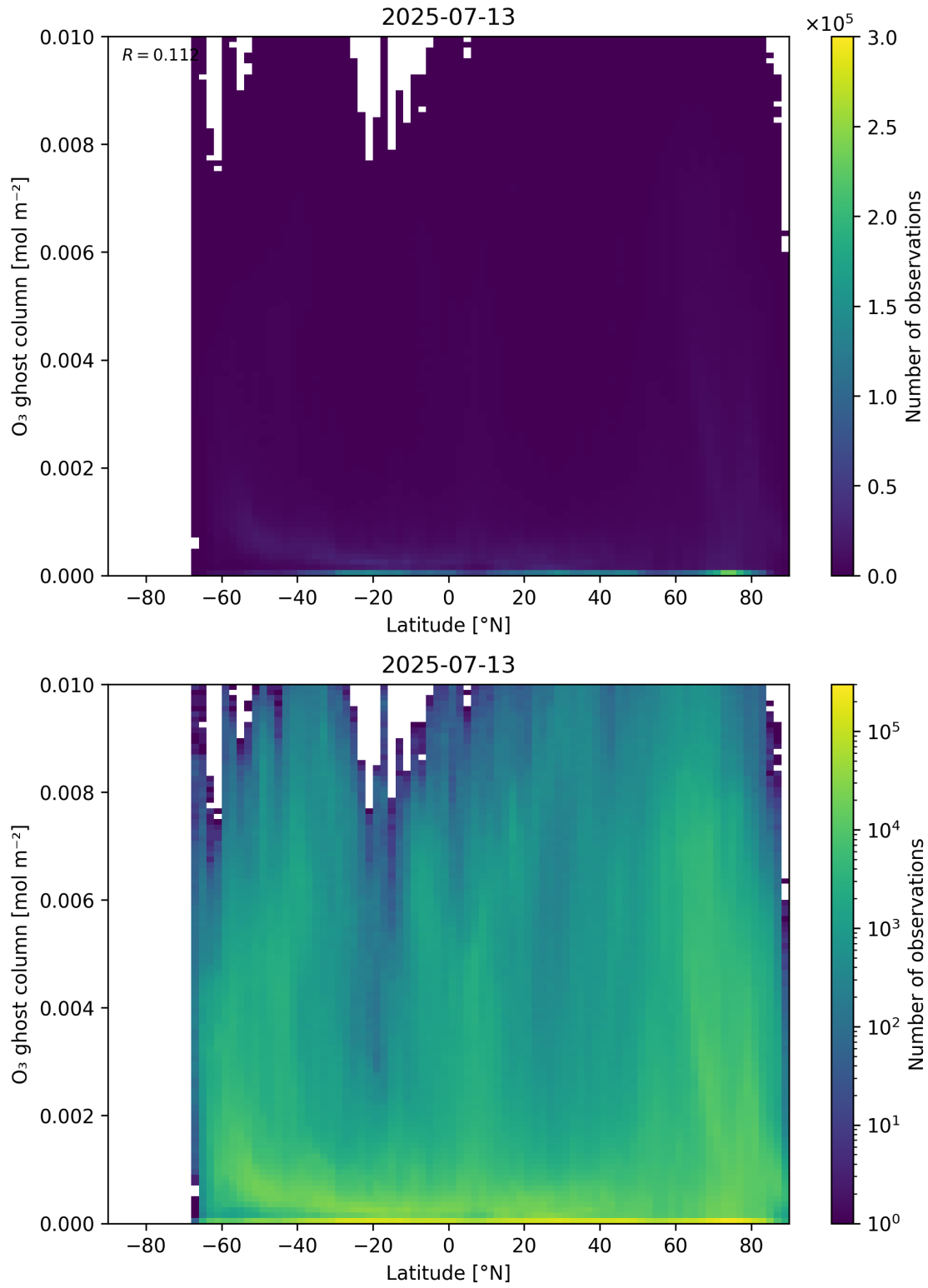
Figure 35: Scatter density plot of “Latitude” against “O 3 ghost column” for 2025-07-13 to 2025-07-14.
