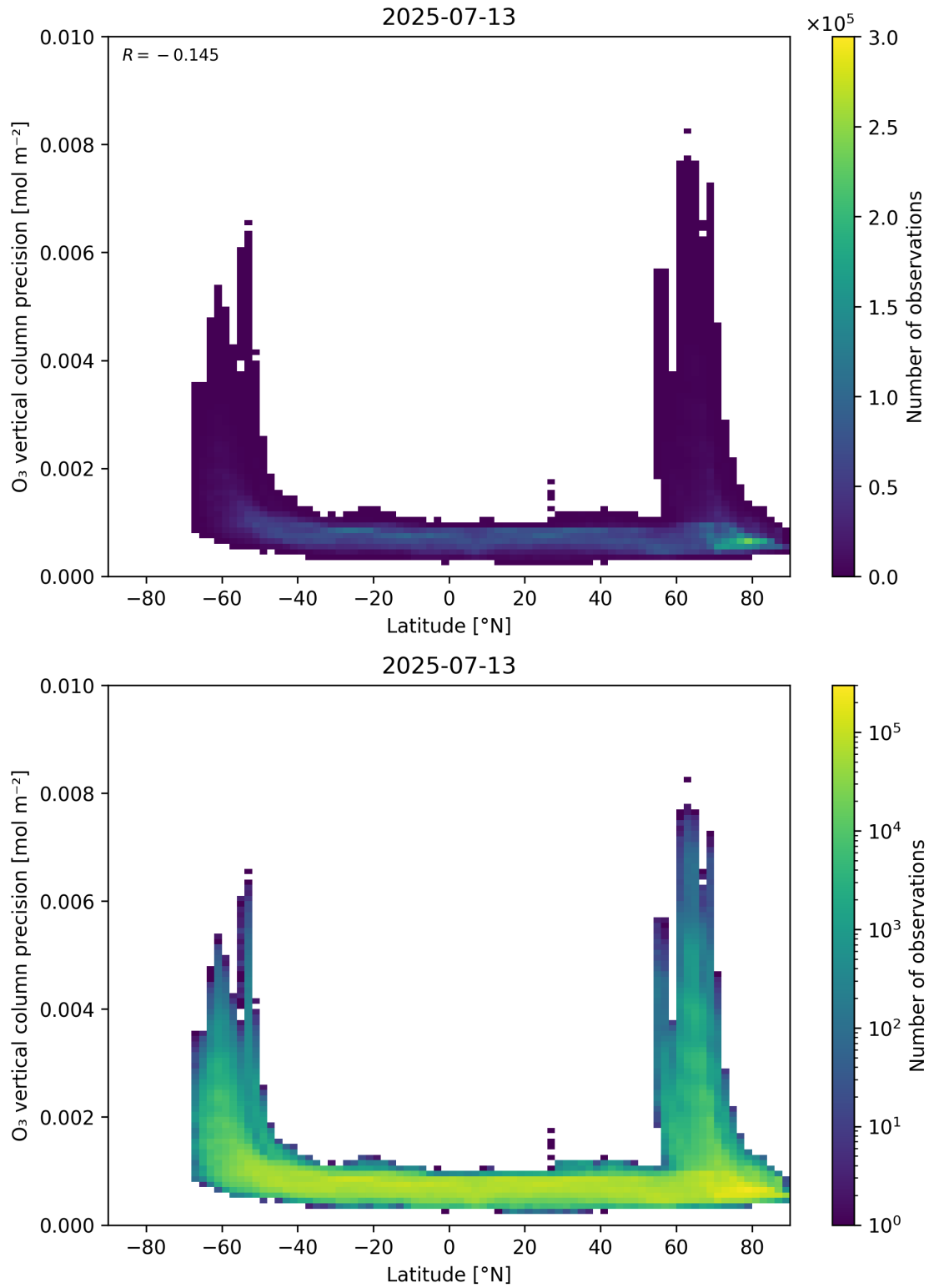
Figure 37: Scatter density plot of “Latitude” against “O 3 vertical column precision” for 2025-07-13 to 2025-07-14.
