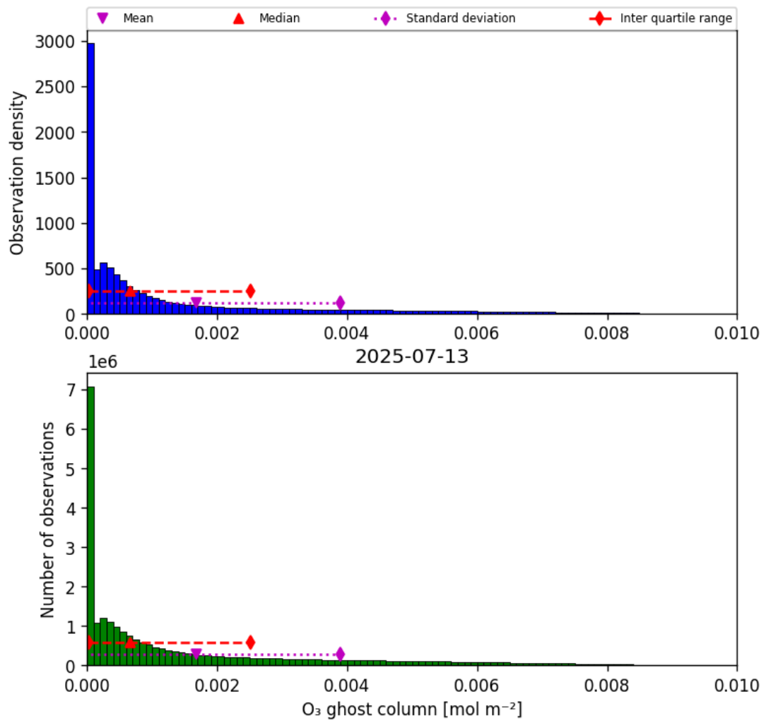
Figure 25: Histogram of “O 3 ghost column” for 2025-07-13 to 2025-07-14
