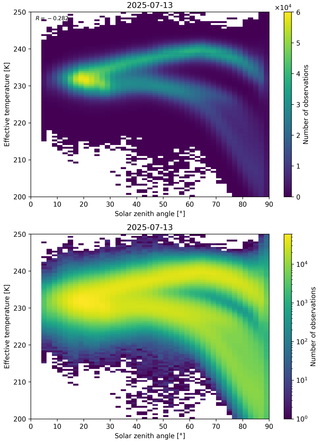
Figure 45: Scatter density plot of “Solar zenith angle” against “Effective temperature” for 2025-07-13 to 2025-07-14.
