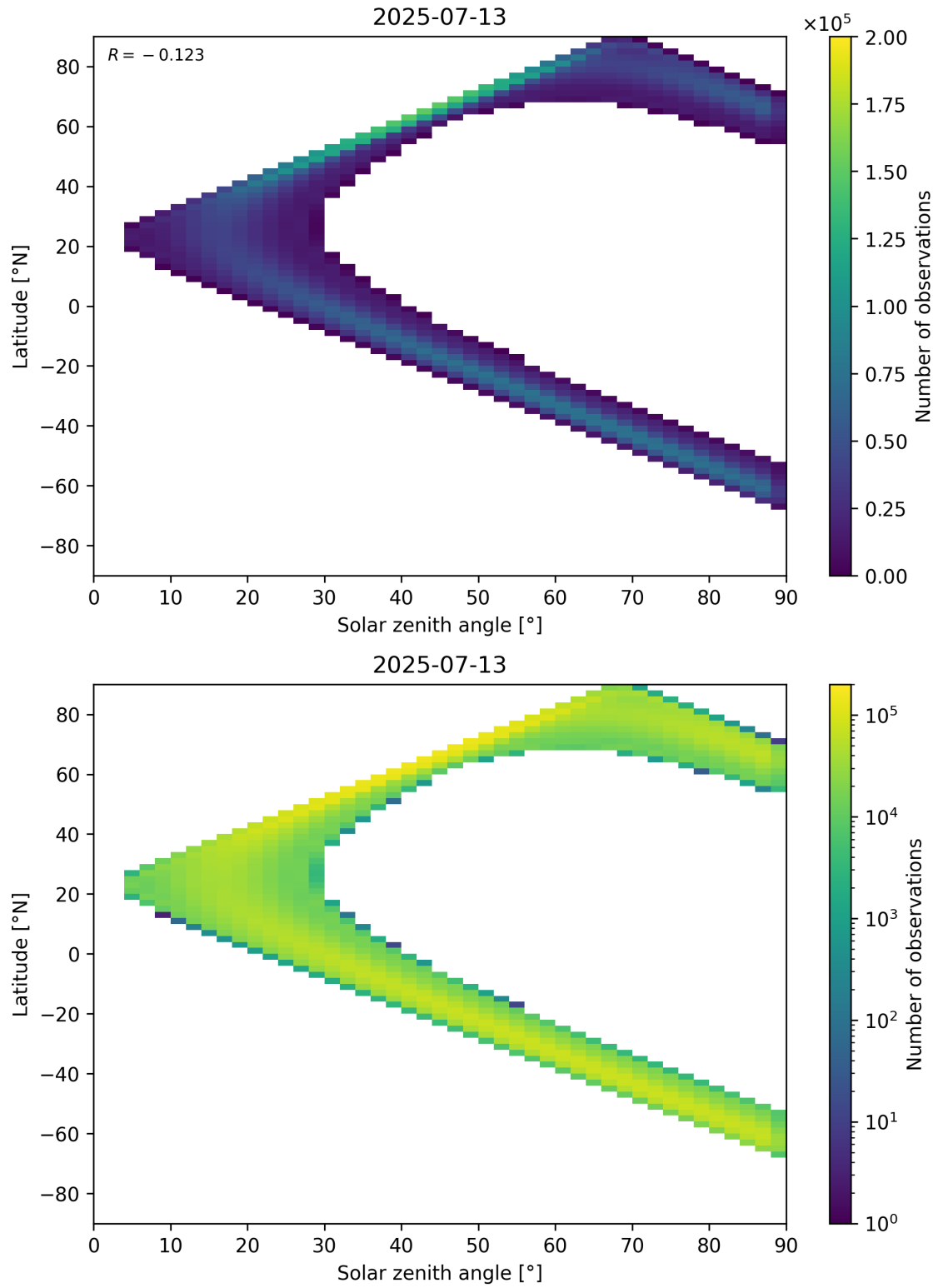
Figure 44: Scatter density plot of “Solar zenith angle” against “Latitude” for 2025-07-13 to 2025-07-14.
