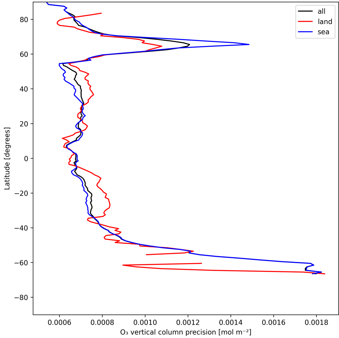
Figure 15: Zonal average of “O 3 vertical column precision” for 2025-07-13 to 2025-07-14.
