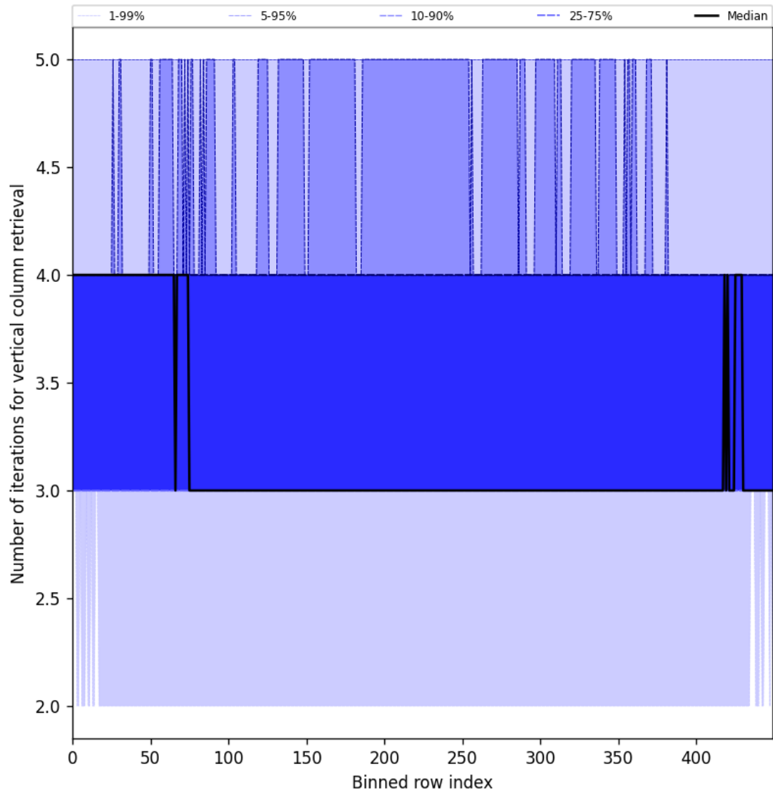
Figure 33: Along track statistics of “Number of iterations for vertical column retrieval” for 2025-07-13 to 2025-07-14
