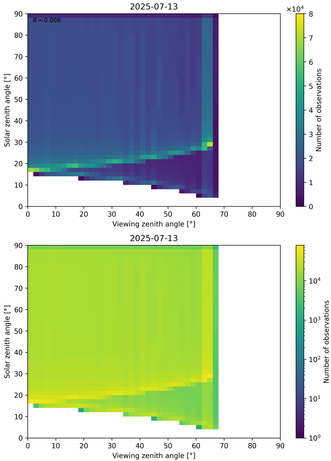
Figure 54: Scatter density plot of “Viewing zenith angle” against “Solar zenith angle” for 2025-07-13 to 2025-07-14.
