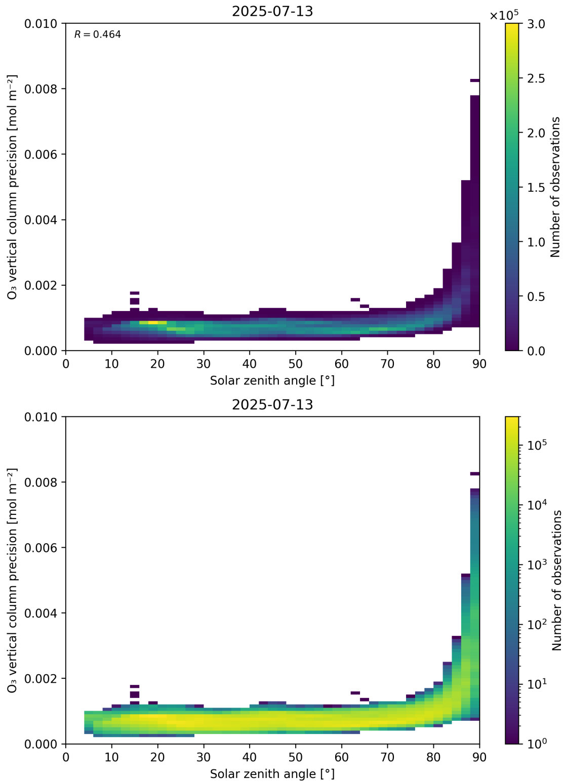
Figure 48: Scatter density plot of “Solar zenith angle” against “O 3 vertical column precision” for 2025-07-13 to 2025-07-14.
