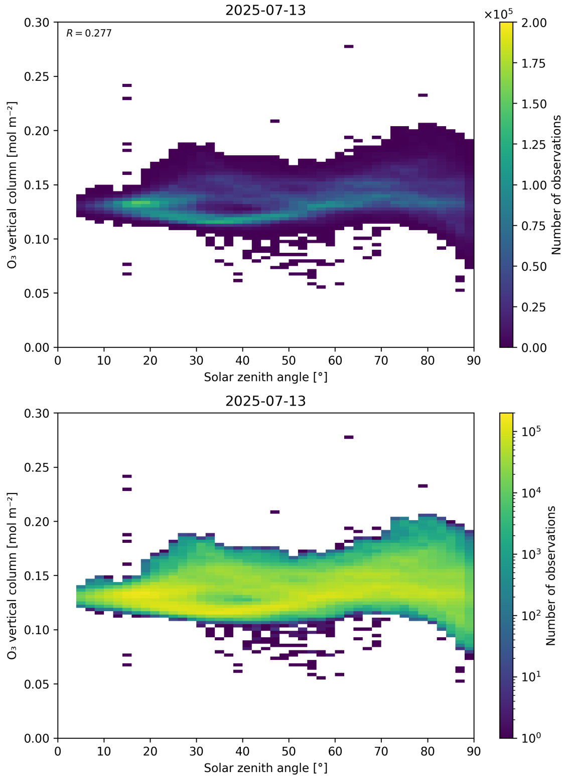
Figure 47: Scatter density plot of “Solar zenith angle” against “O 3 vertical column” for 2025-07-13 to 2025-07-14.
