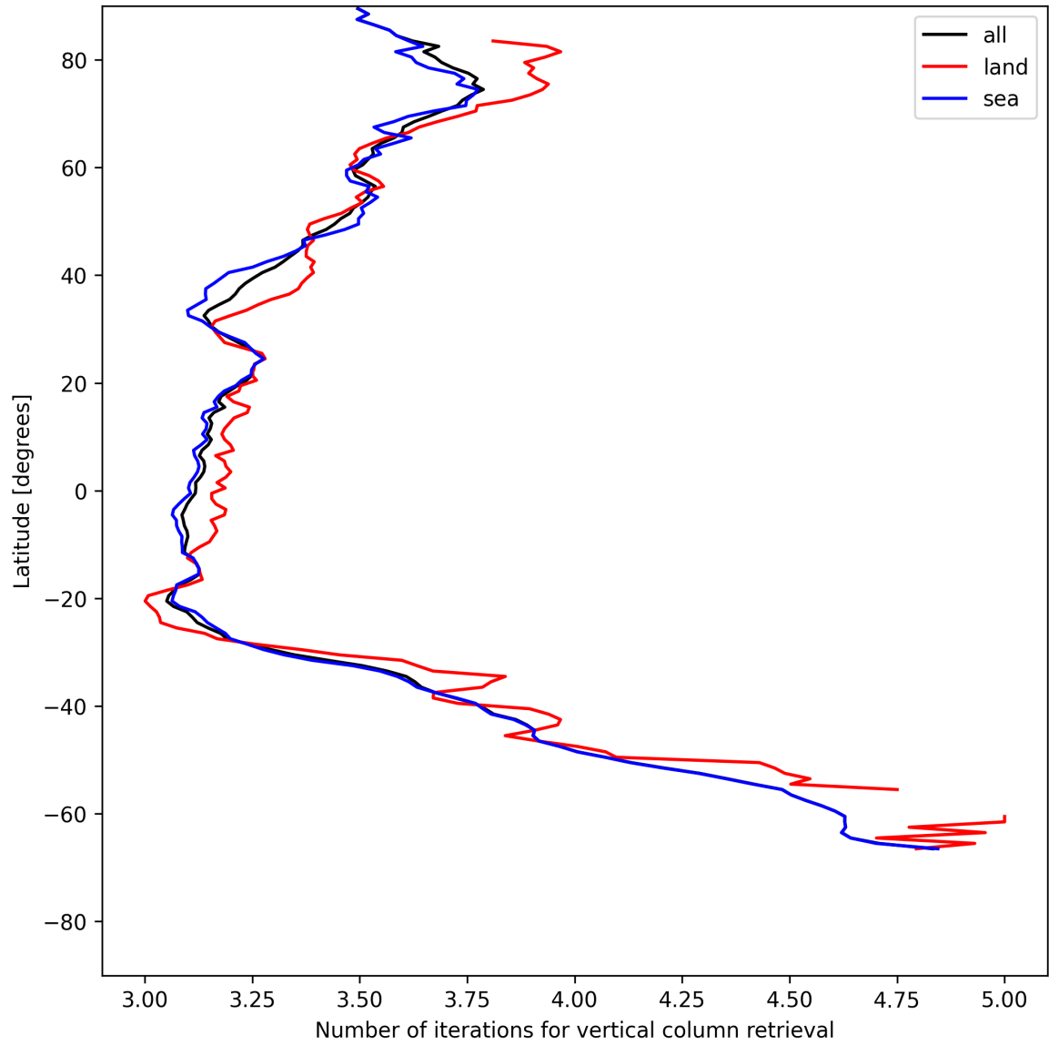
Figure 19: Zonal average of “Number of iterations for vertical column retrieval” for 2025-07-13 to 2025-07-14.
