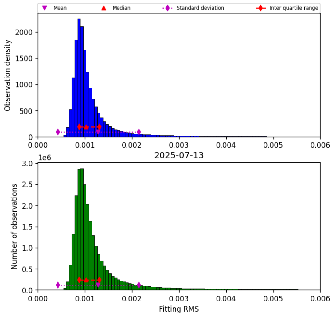
Figure 23: Histogram of “Fitting RMS” for 2025-07-13 to 2025-07-14
