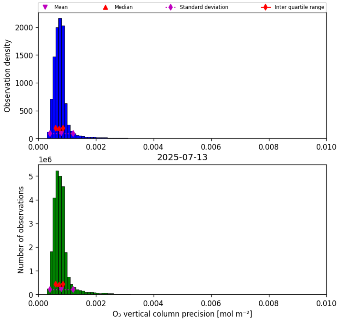
Figure 22: Histogram of “O 3 vertical column precision” for 2025-07-13 to 2025-07-14
