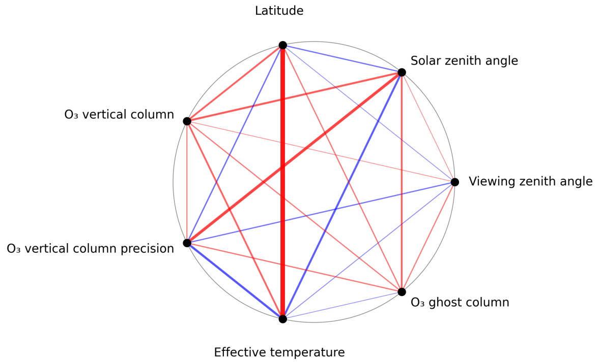
Figure 1: Map of correlation graph for 2025-07-13 to 2025-07-14.
