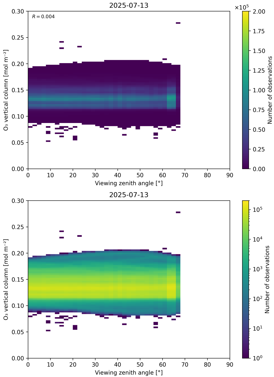
Figure 52: Scatter density plot of “Viewing zenith angle” against “O 3 vertical column” for 2025-07-13 to 2025-07-14.
