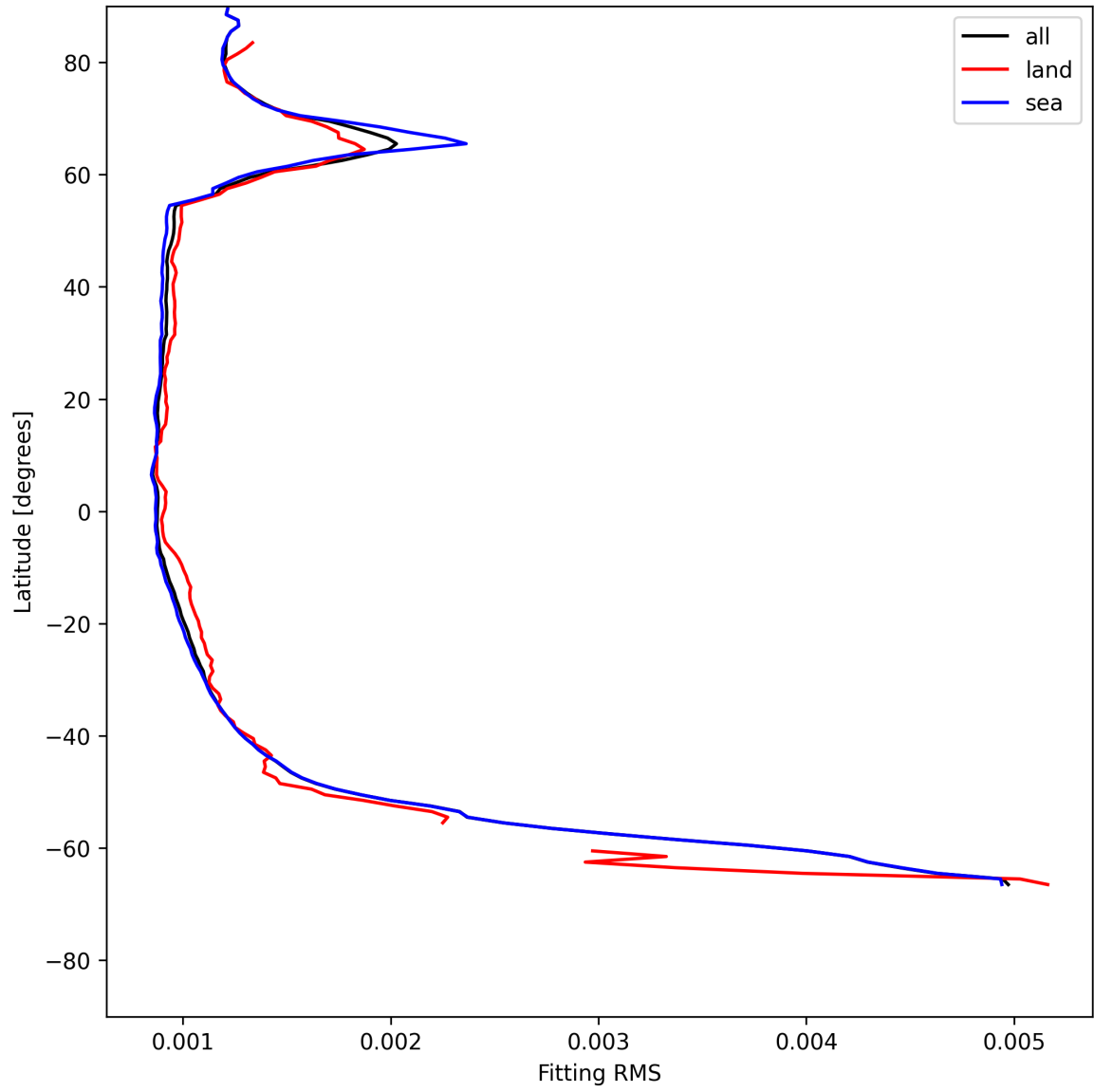
Figure 16: Zonal average of “Fitting RMS” for 2025-07-13 to 2025-07-14.
