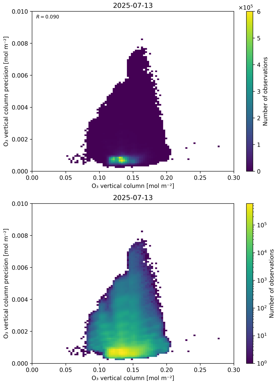
Figure 41: Scatter density plot of “O 3 vertical column” against “O 3 vertical column precision” for 2025-07-13 to 2025-07-14.
