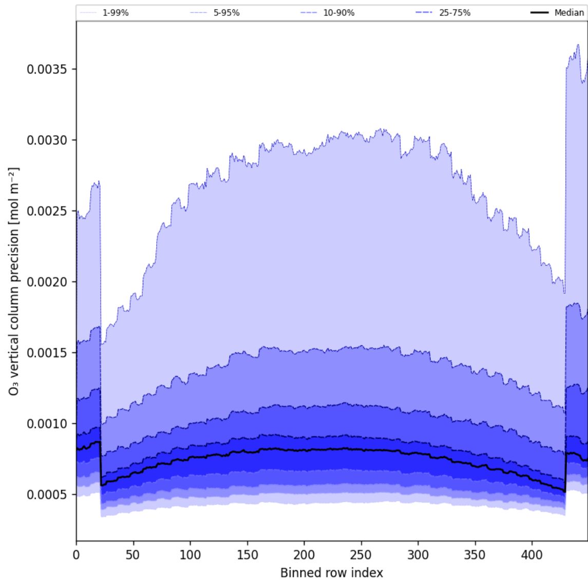
Figure 29: Along track statistics of “O 3 vertical column precision” for 2025-07-13 to 2025-07-14
