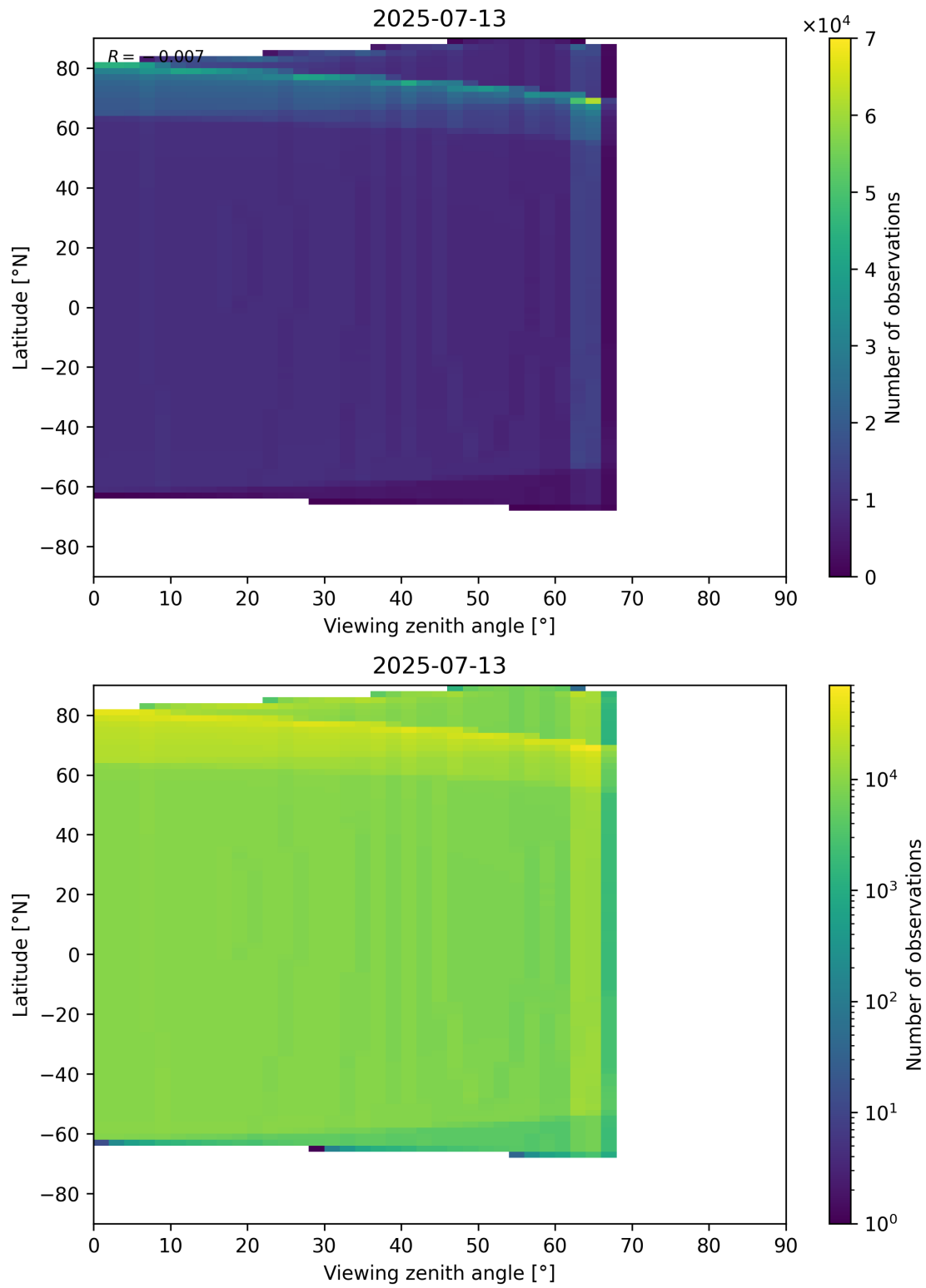
Figure 49: Scatter density plot of “Viewing zenith angle” against “Latitude” for 2025-07-13 to 2025-07-14.
