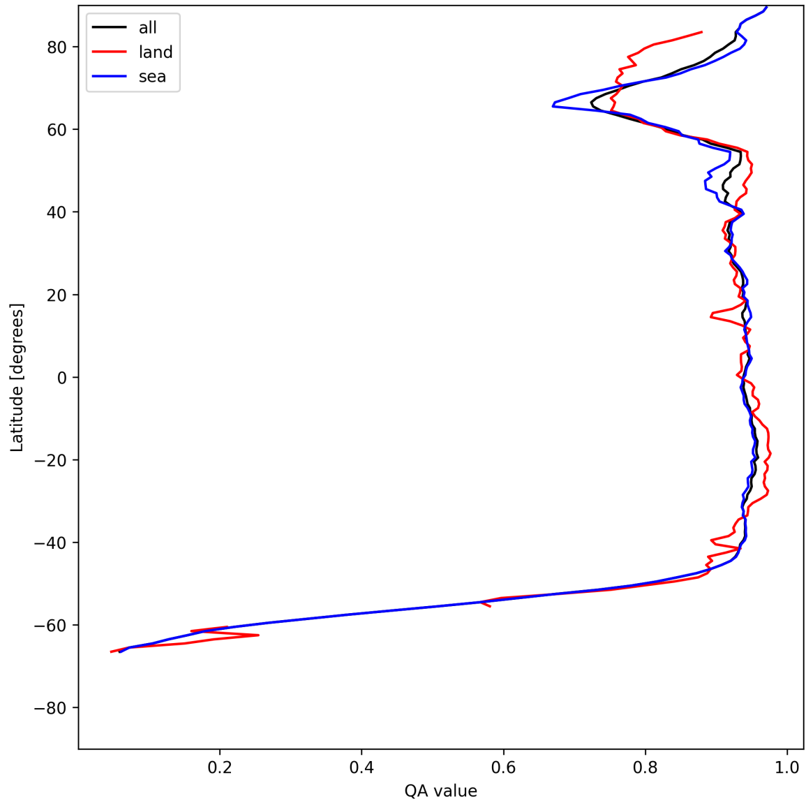
Figure 13: Zonal average of “QA value” for 2025-07-13 to 2025-07-14.
