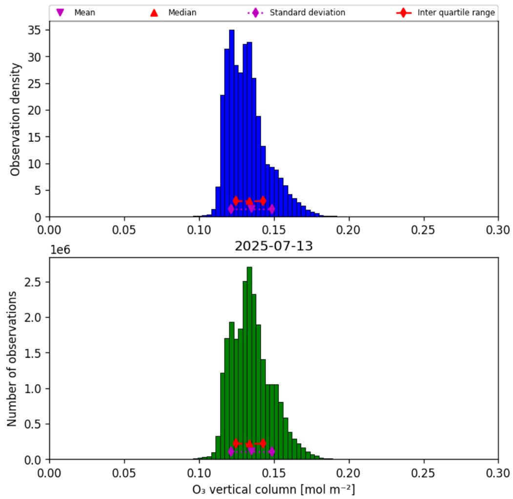
Figure 21: Histogram of “O 3 vertical column” for 2025-07-13 to 2025-07-14
