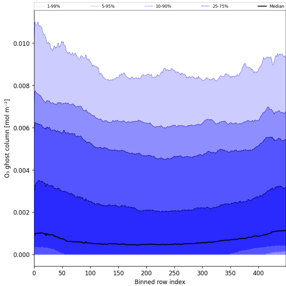
Figure 32: Along track statistics of “O 3 ghost column” for 2025-07-13 to 2025-07-14
