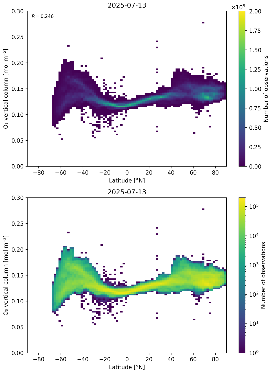
Figure 36: Scatter density plot of “Latitude” against “O 3 vertical column” for 2025-07-13 to 2025-07-14.
