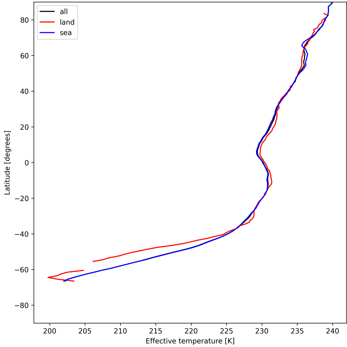
Figure 17: Zonal average of “Effective temperature” for 2025-07-13 to 2025-07-14.
