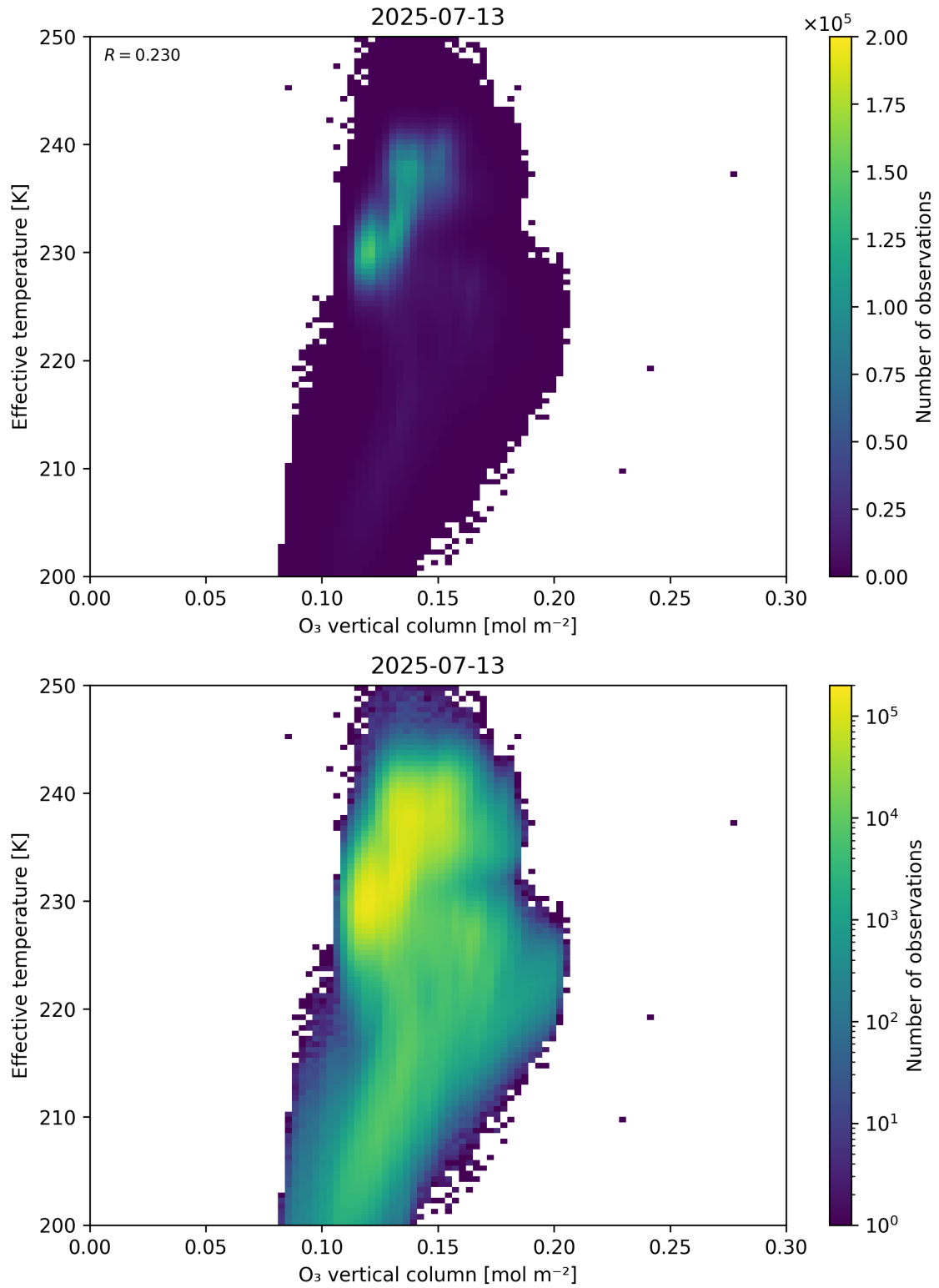
Figure 39: Scatter density plot of “O 3 vertical column” against “Effective temperature” for 2025-07-13 to 2025-07-14.
