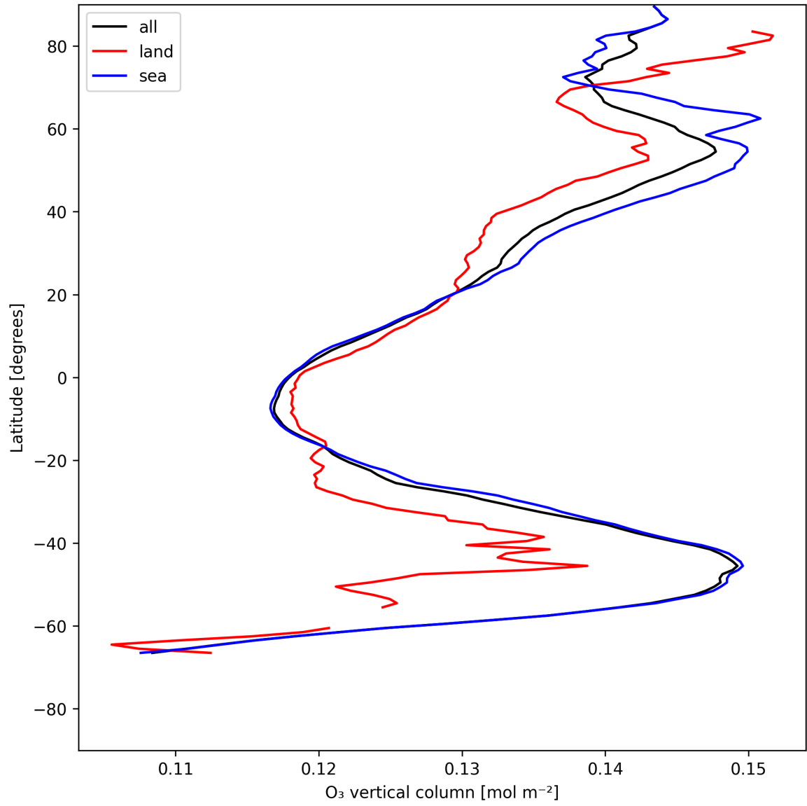
Figure 14: Zonal average of “O 3 vertical column” for 2025-07-13 to 2025-07-14.
