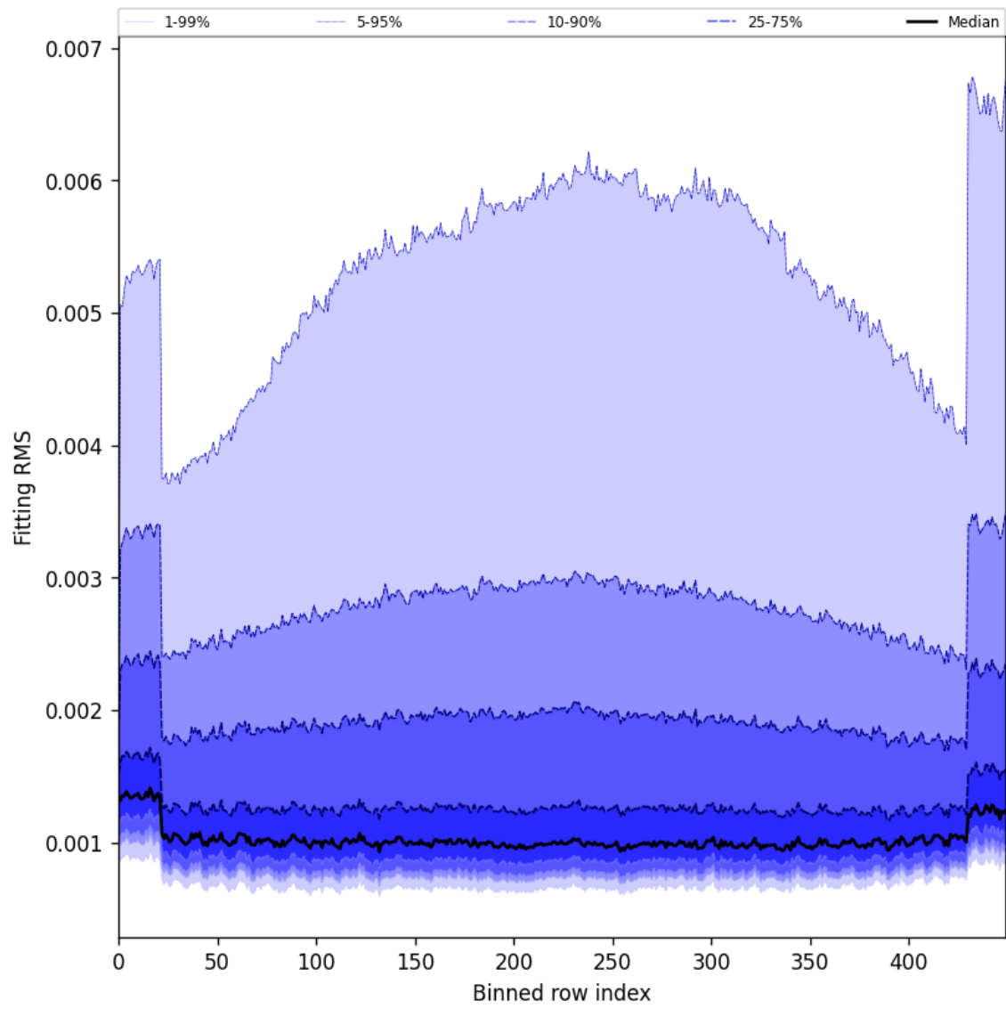
Figure 30: Along track statistics of “Fitting RMS” for 2025-07-13 to 2025-07-14
