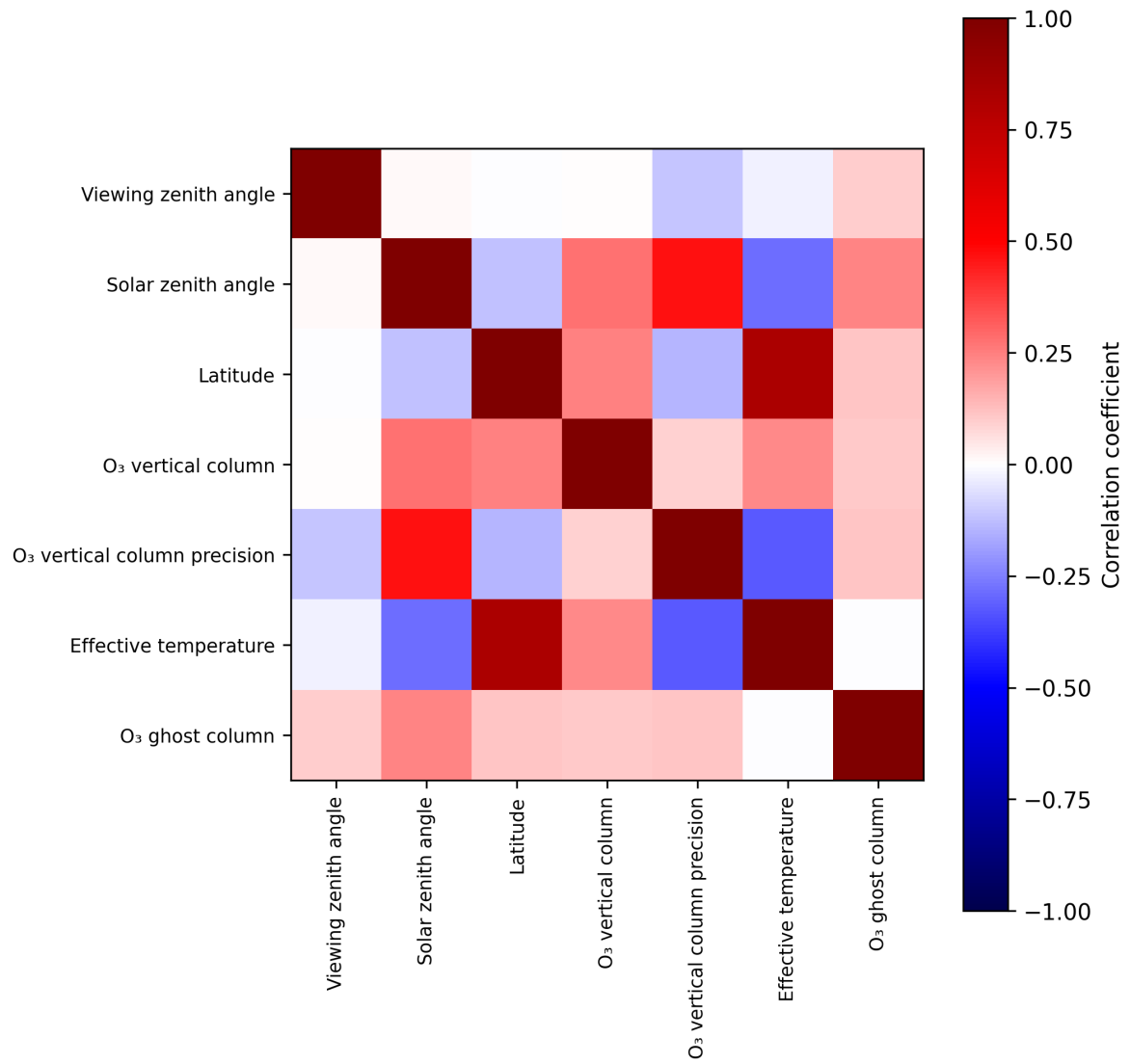
Figure 2: Map of correlation matrix for 2025-07-13 to 2025-07-14.
