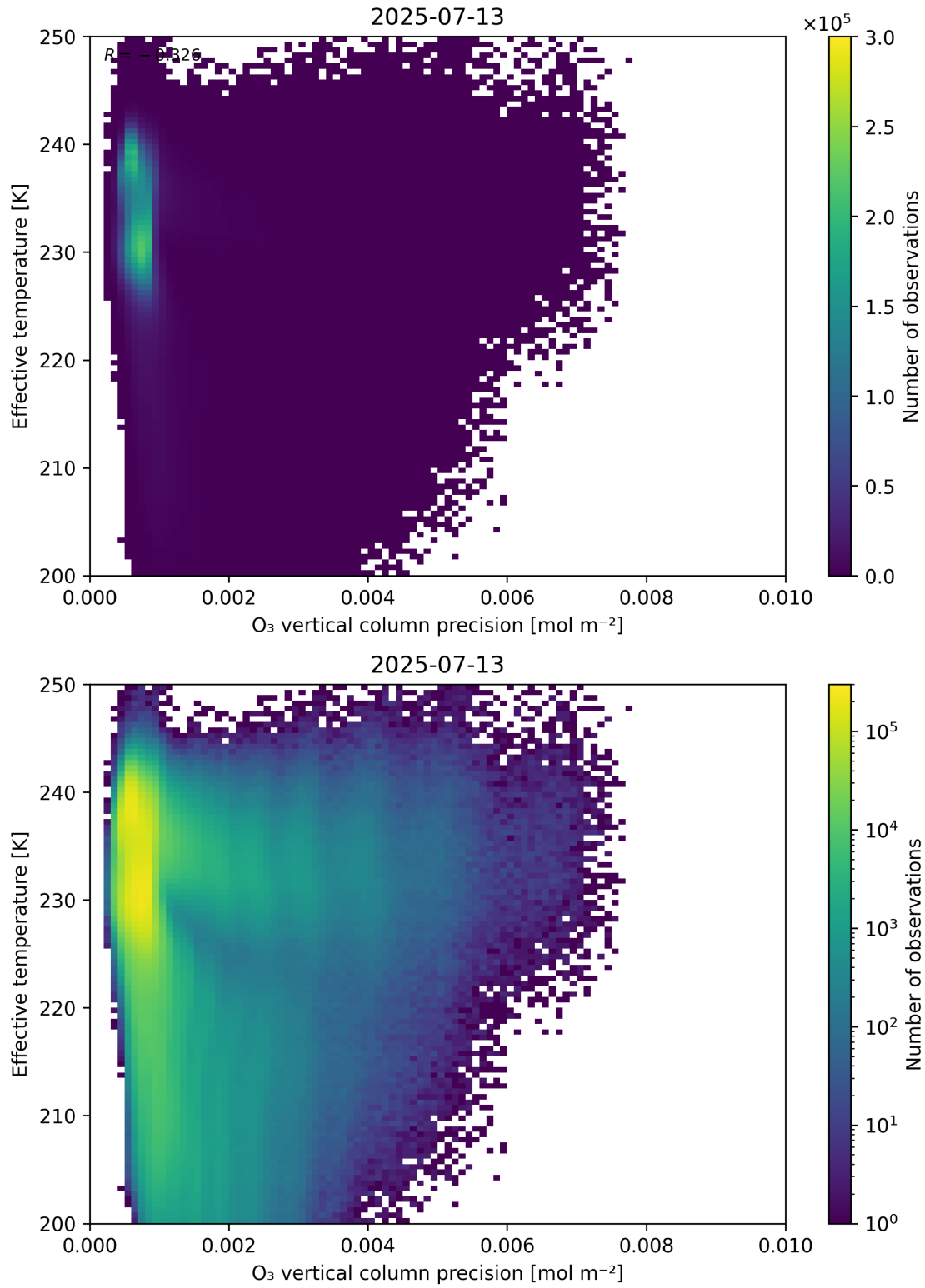
Figure 42: Scatter density plot of “O 3 vertical column precision” against “Effective temperature” for 2025-07-13 to 2025-07-14.
