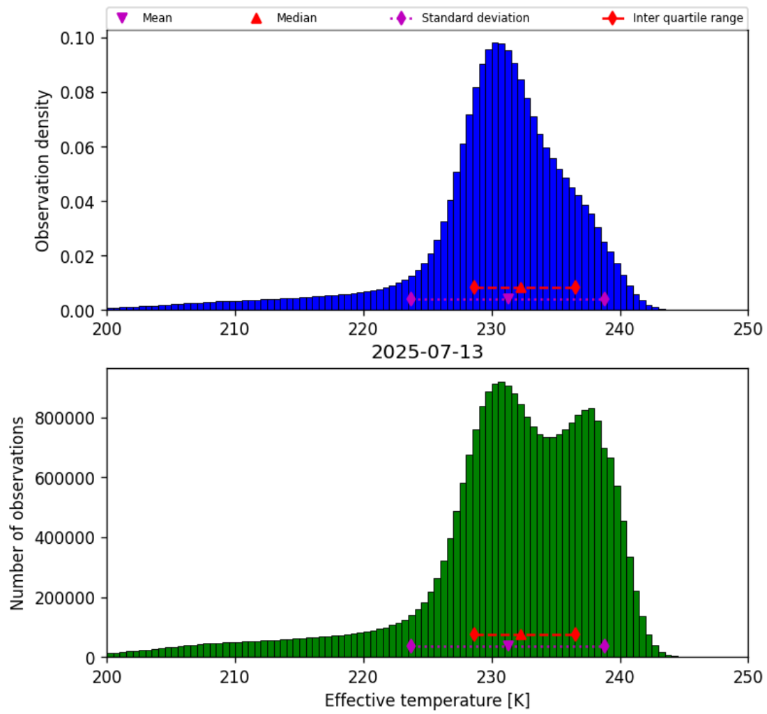
Figure 24: Histogram of “Effective temperature” for 2025-07-13 to 2025-07-14
