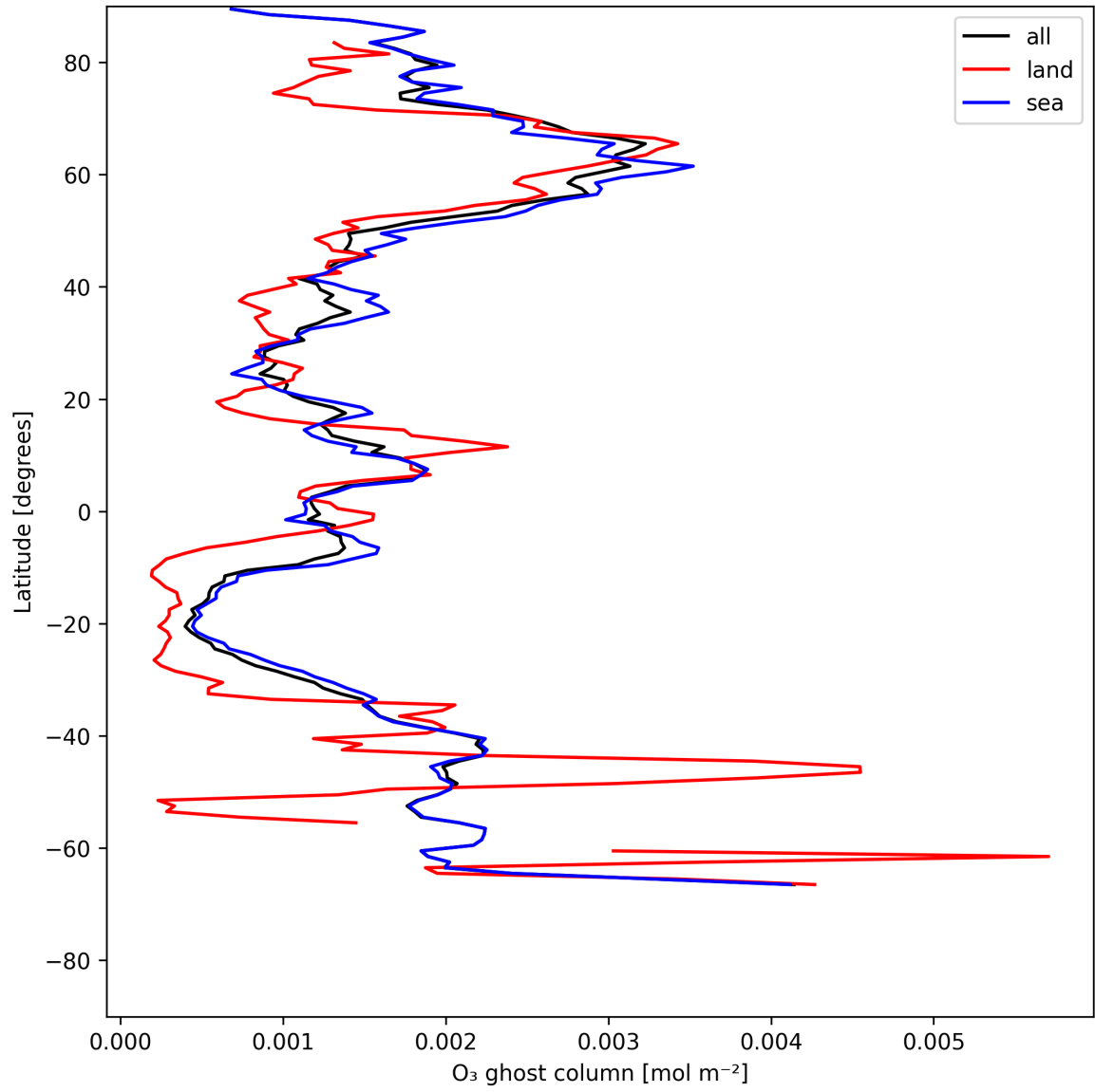
Figure 18: Zonal average of "O 3 ghost column" for 2025-07-13 to 2025-07-14.
