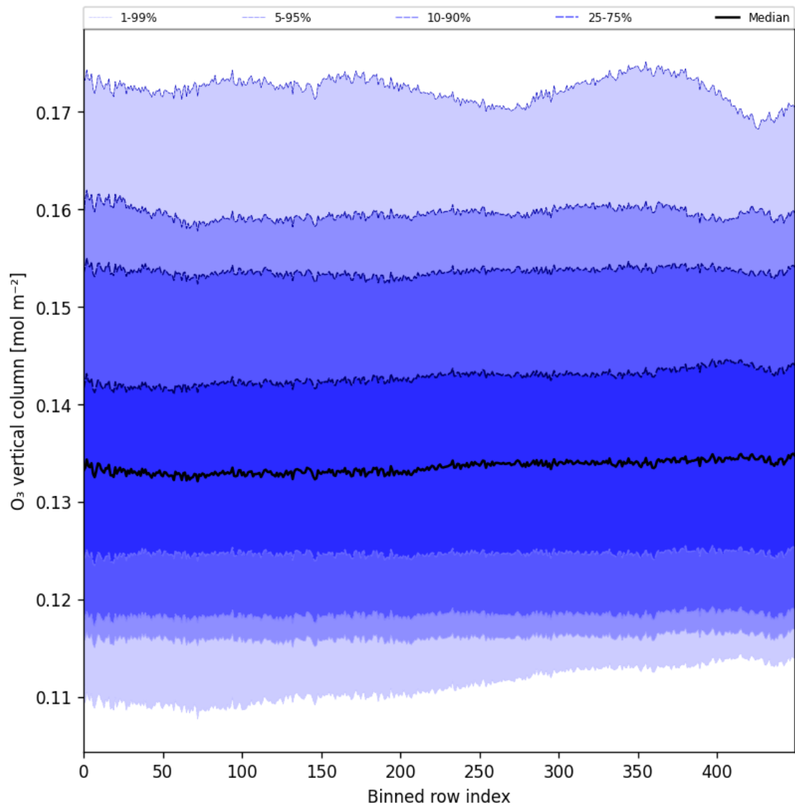
Figure 28: Along track statistics of “O 3 vertical column” for 2025-07-13 to 2025-07-14
