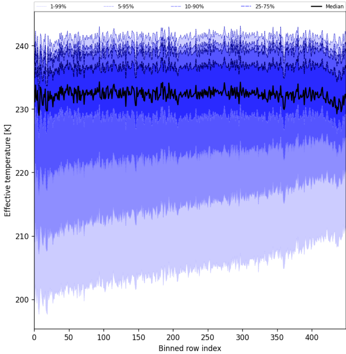
Figure 31: Along track statistics of “Effective temperature” for 2025-07-13 to 2025-07-14
