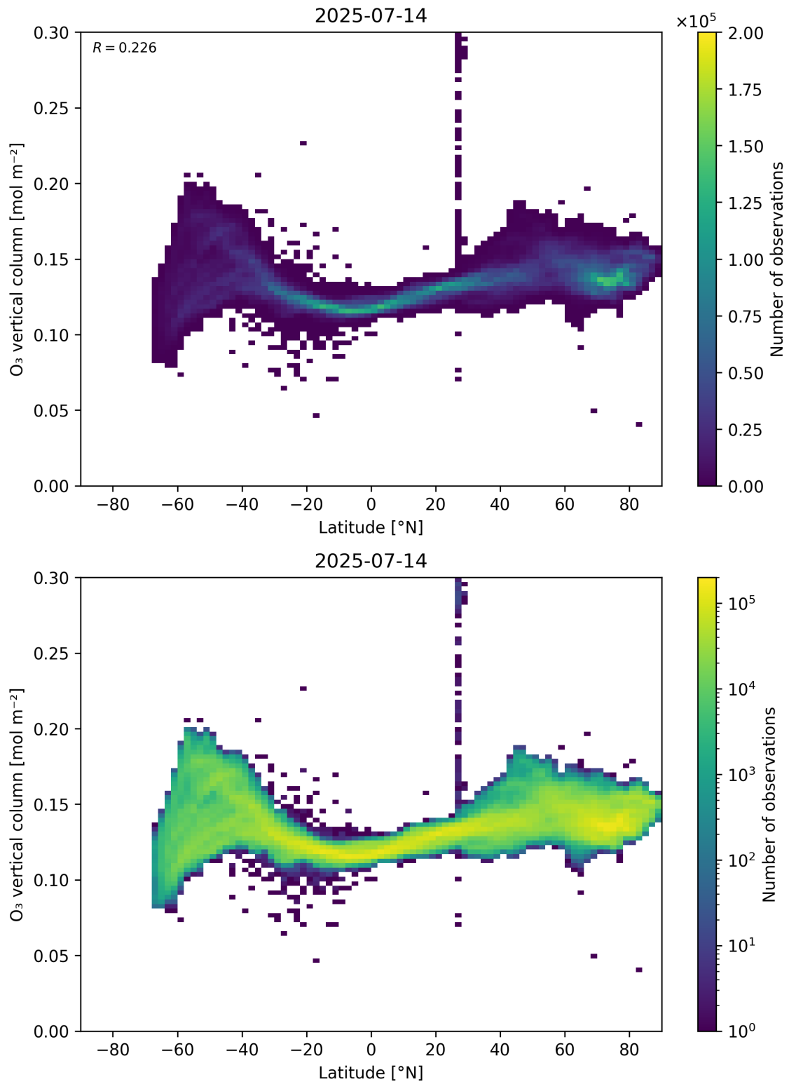
Figure 36: Scatter density plot of “Latitude” against “O 3 vertical column” for 2025-07-13 to 2025-07-15.
