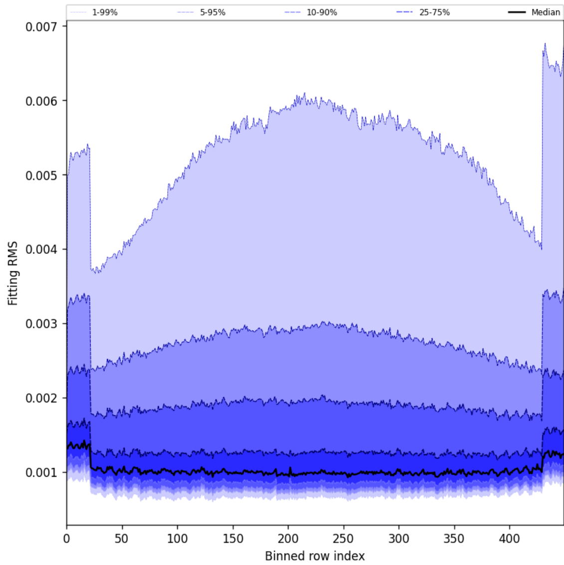
Figure 30: Along track statistics of “Fitting RMS” for 2025-07-13 to 2025-07-15
