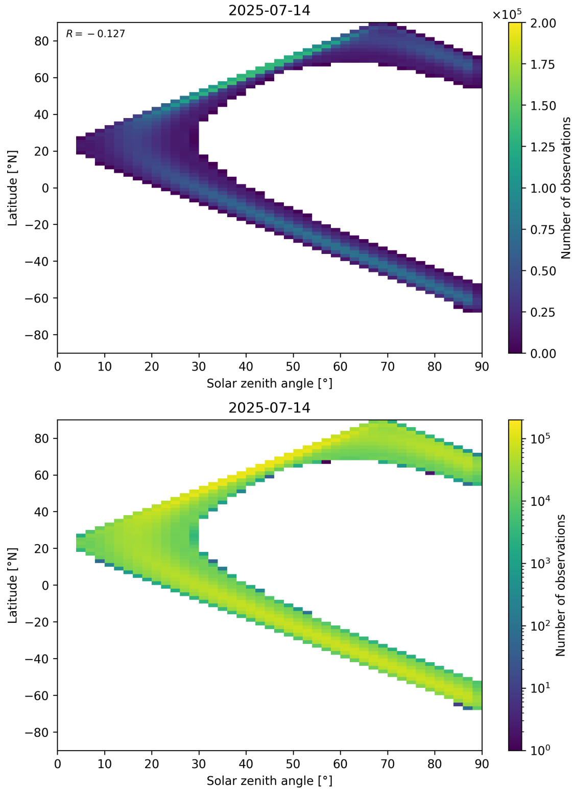
Figure 44: Scatter density plot of “Solar zenith angle” against “Latitude” for 2025-07-13 to 2025-07-15.
