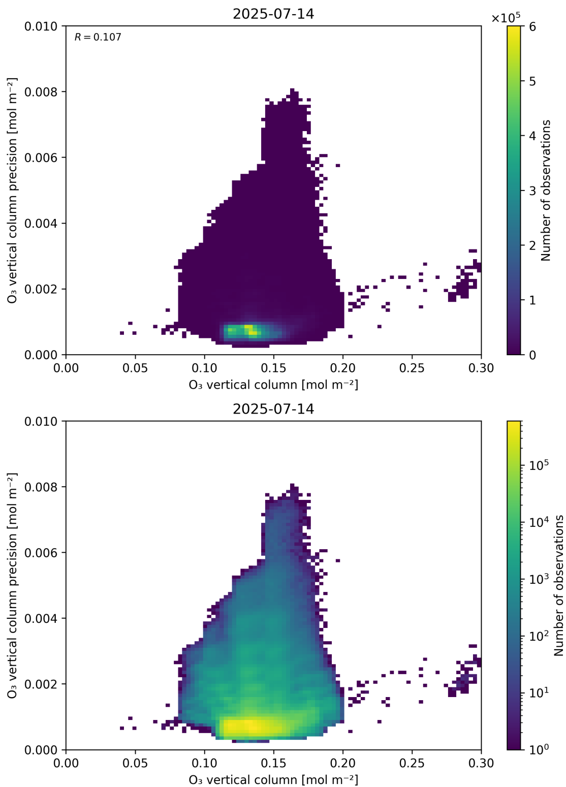
Figure 41: Scatter density plot of “O 3 vertical column” against “O 3 vertical column precision” for 2025-07-13 to 2025-07-15.
