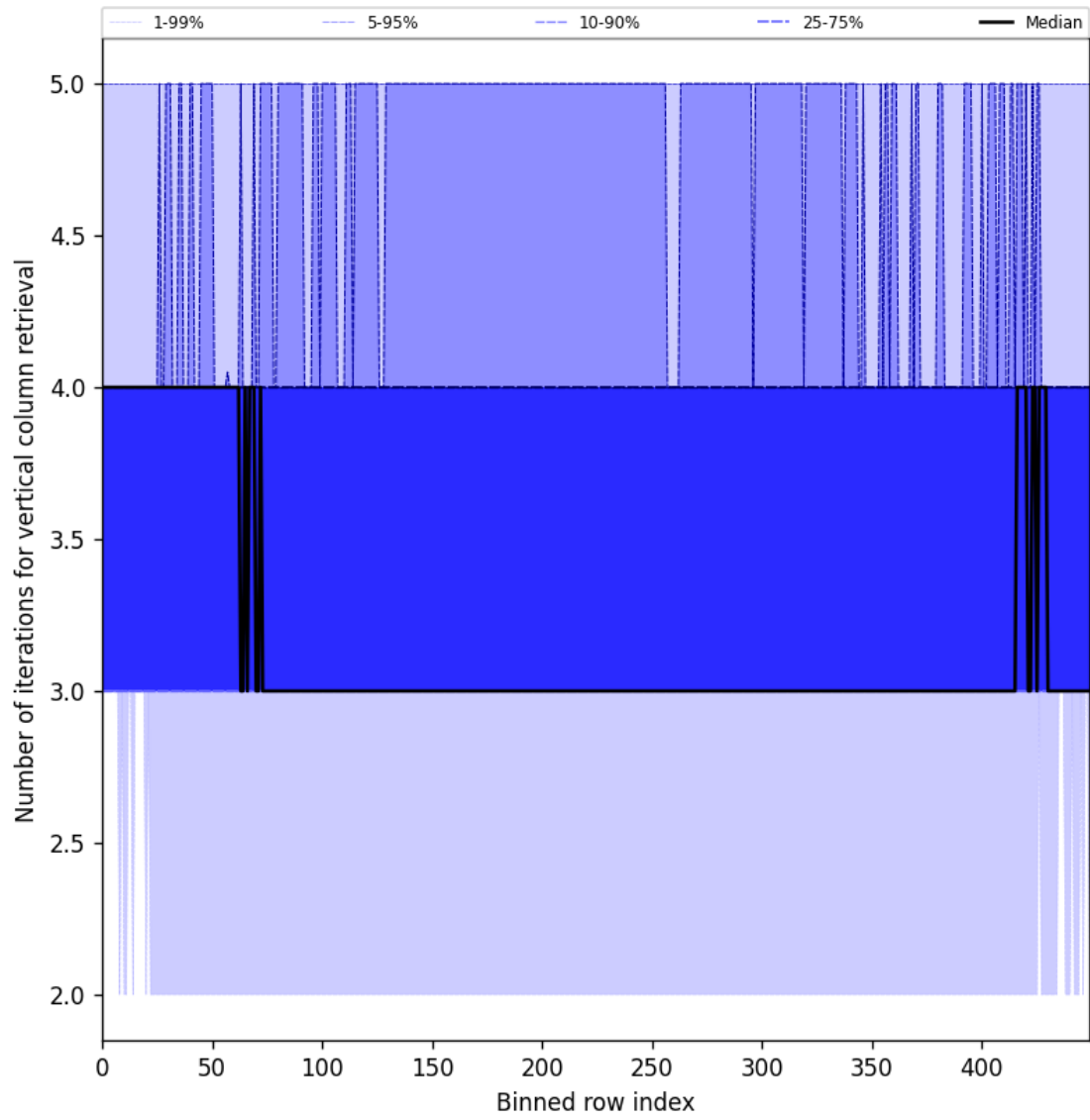
Figure 33: Along track statistics of “Number of iterations for vertical column retrieval” for 2025-07-13 to 2025-07-15
