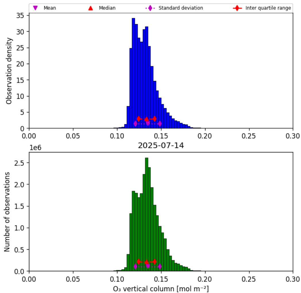
Figure 21: Histogram of “O 3 vertical column” for 2025-07-13 to 2025-07-15
