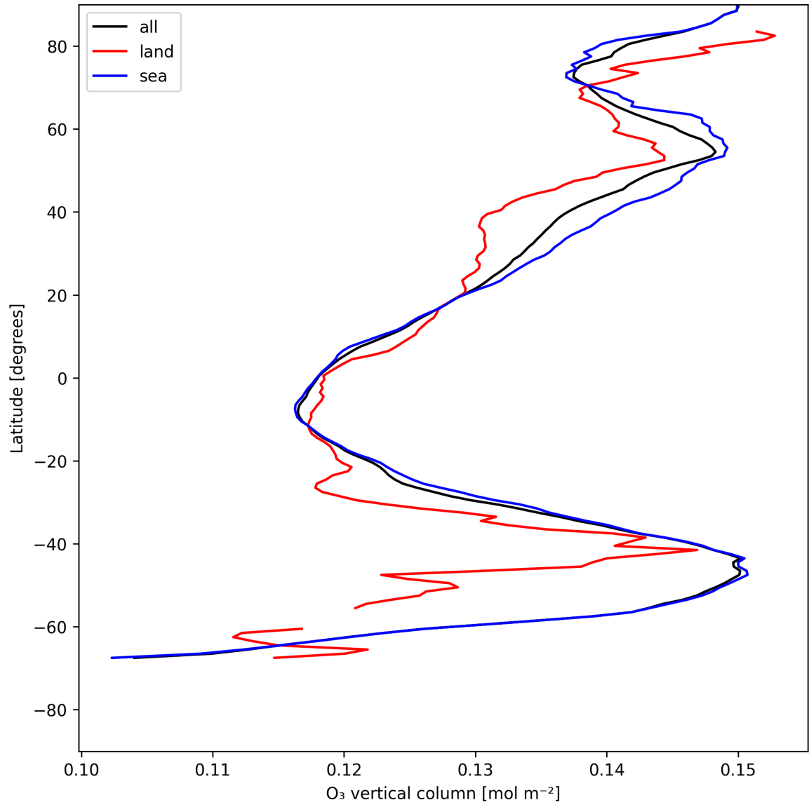
Figure 14: Zonal average of “O 3 vertical column” for 2025-07-13 to 2025-07-15.
