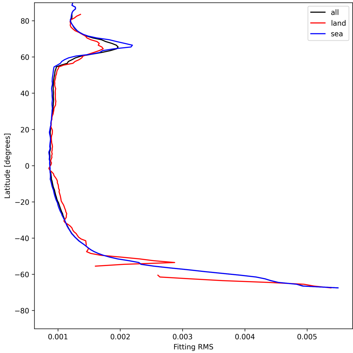
Figure 16: Zonal average of “Fitting RMS” for 2025-07-13 to 2025-07-15.
