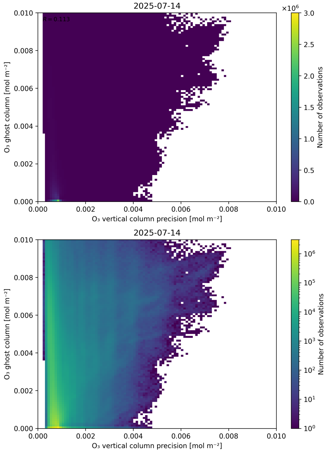
Figure 43: Scatter density plot of “ \text{O}_3 vertical column precision” against “ \text{O}_3 ghost column” for 2025-07-13 to 2025-07-15.
