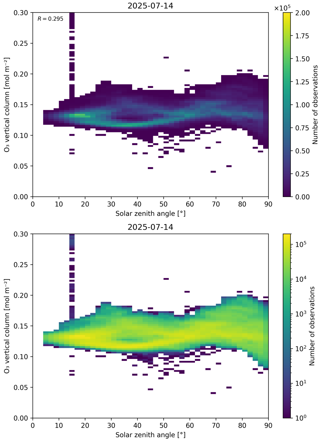
Figure 47: Scatter density plot of “Solar zenith angle” against “O 3 vertical column” for 2025-07-13 to 2025-07-15.
