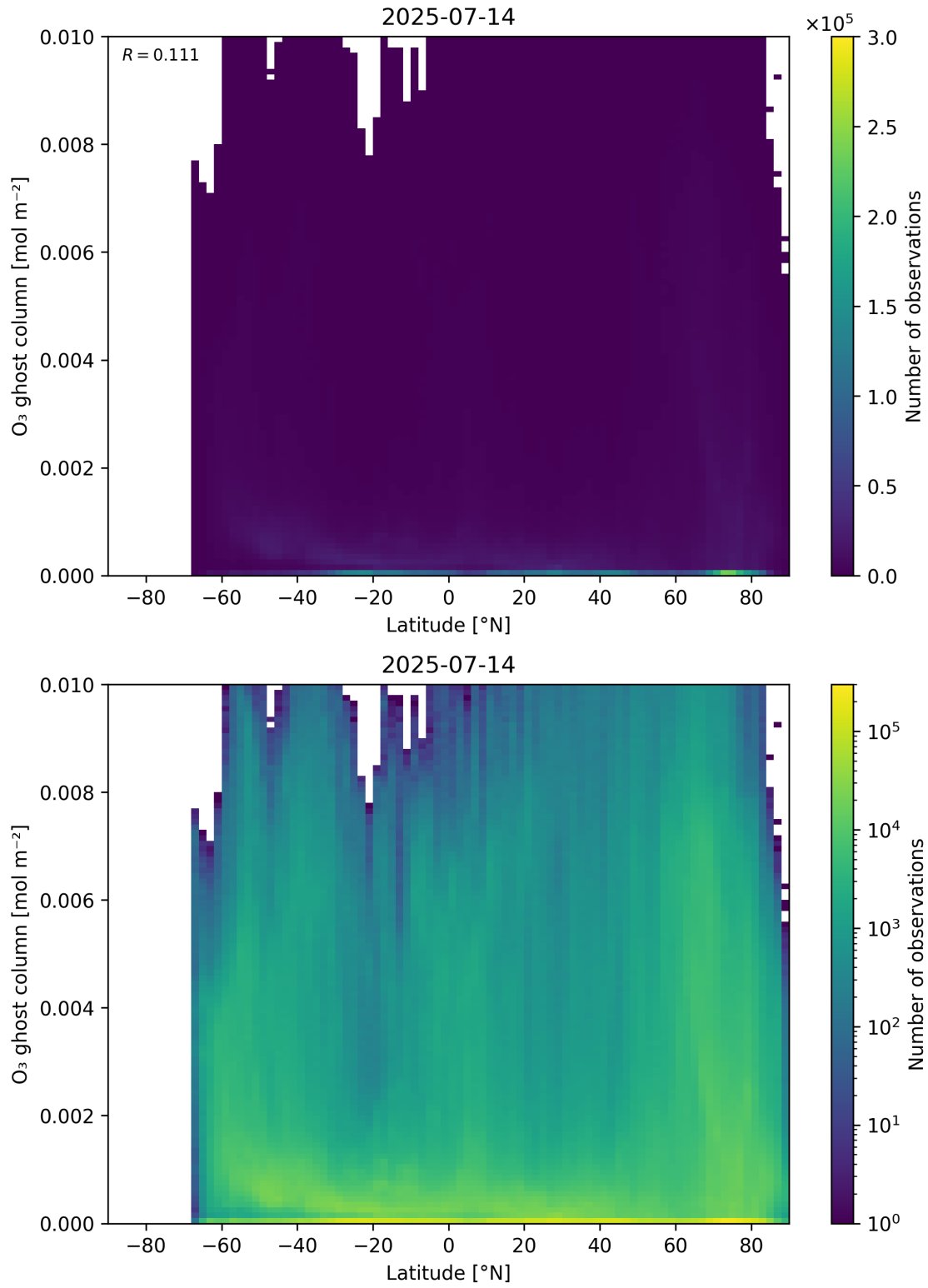
Figure 35: Scatter density plot of “Latitude” against “O 3 ghost column” for 2025-07-13 to 2025-07-15.
