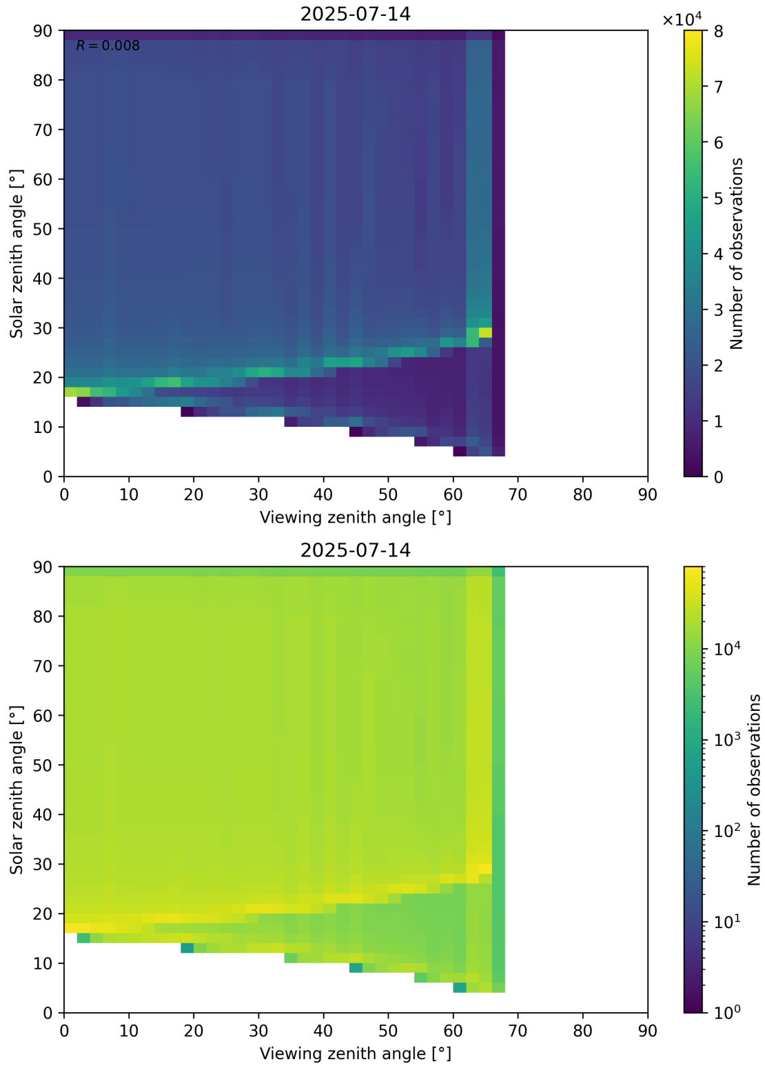
Figure 54: Scatter density plot of “Viewing zenith angle” against “Solar zenith angle” for 2025-07-13 to 2025-07-15.
