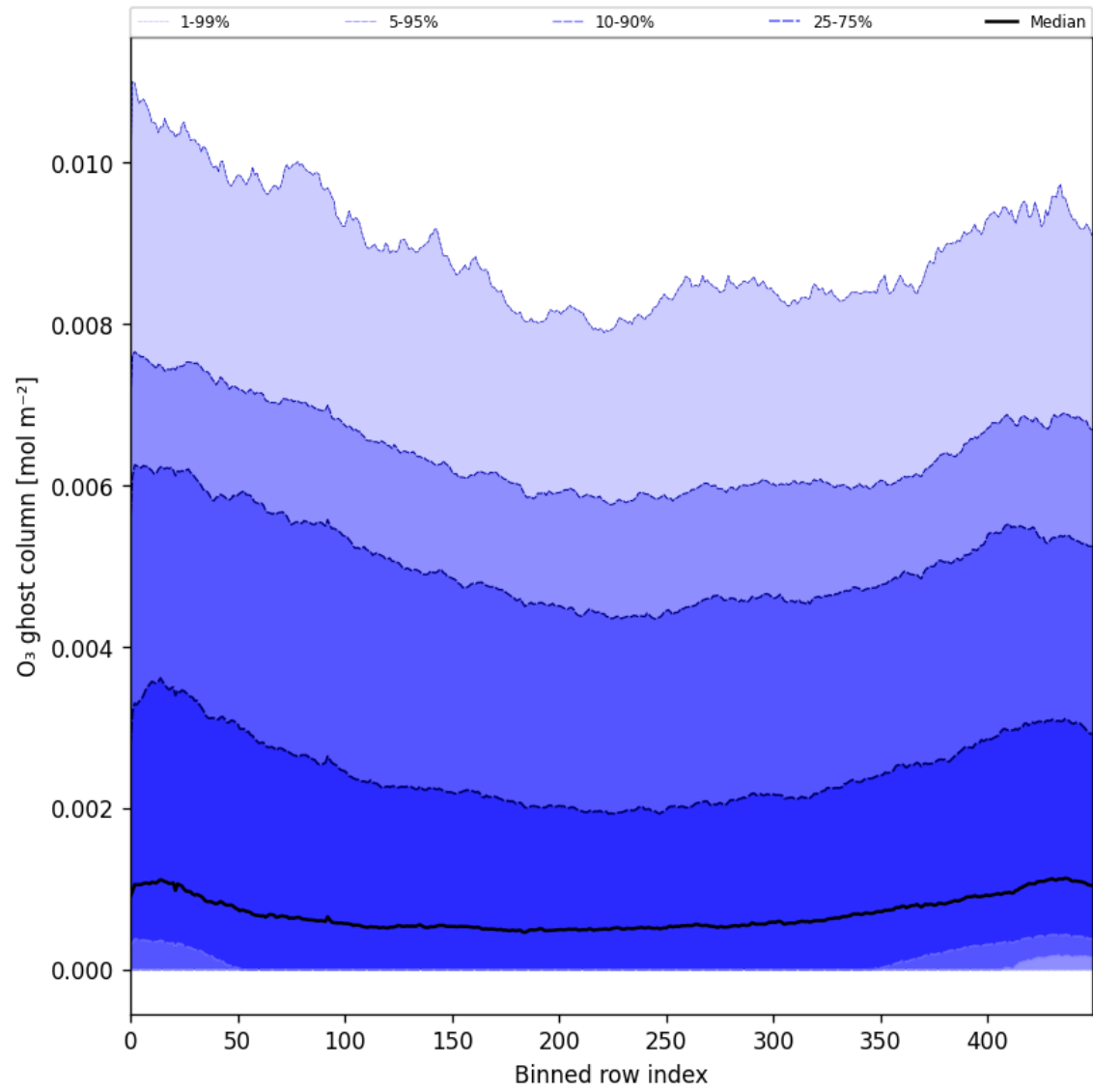
Figure 32: Along track statistics of “O 3 ghost column” for 2025-07-13 to 2025-07-15
