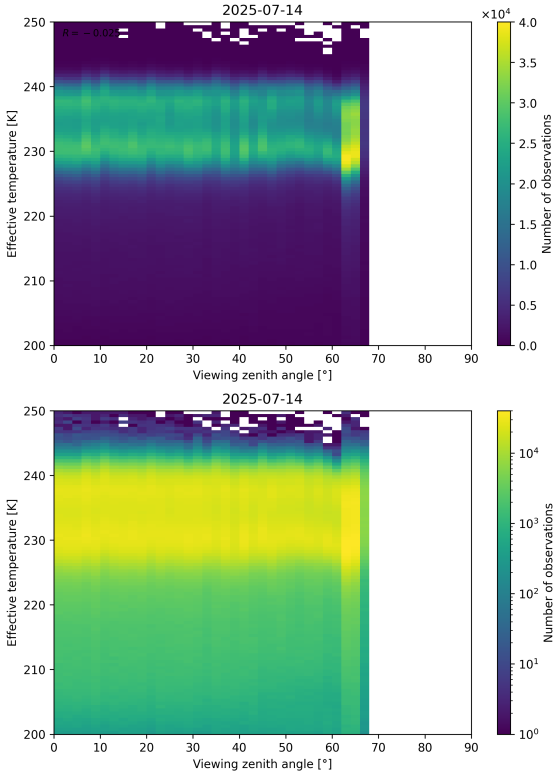
Figure 50: Scatter density plot of “Viewing zenith angle” against “Effective temperature” for 2025-07-13 to 2025-07-15.
