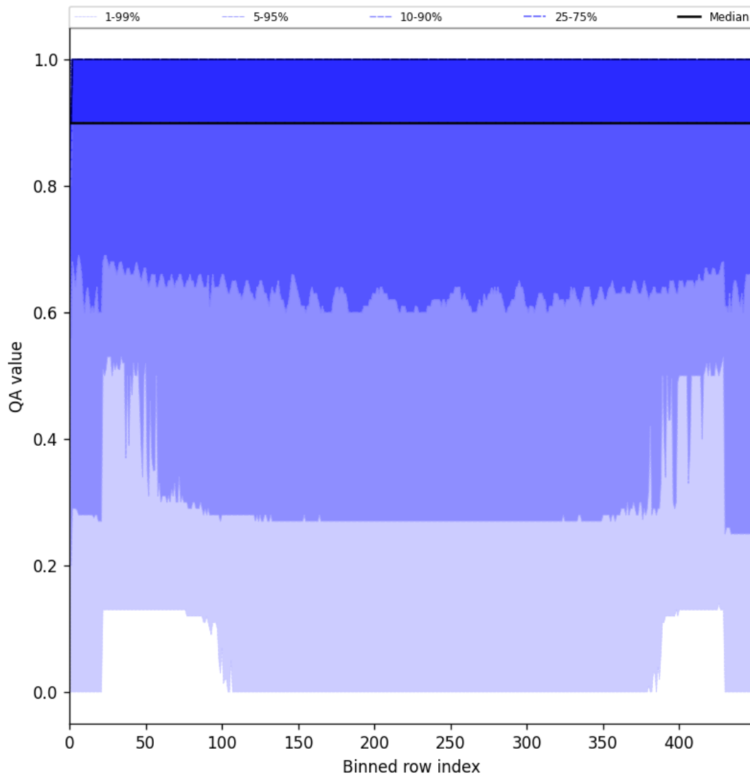
Figure 27: Along track statistics of “QA value” for 2025-07-13 to 2025-07-15
