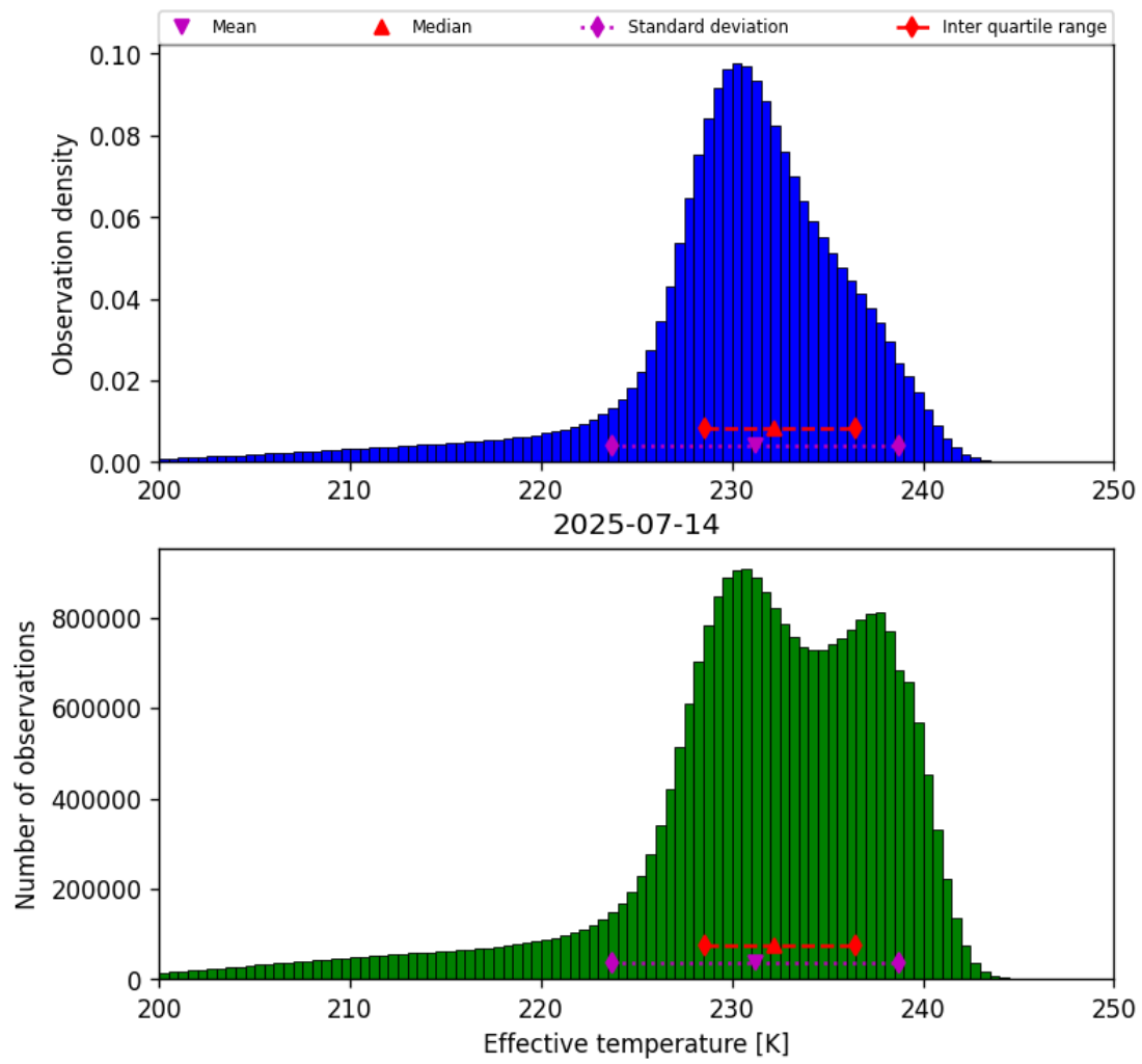
Figure 24: Histogram of “Effective temperature” for 2025-07-13 to 2025-07-15
