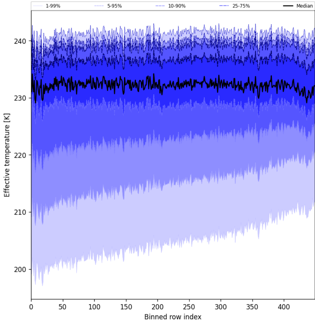
Figure 31: Along track statistics of “Effective temperature” for 2025-07-13 to 2025-07-15
