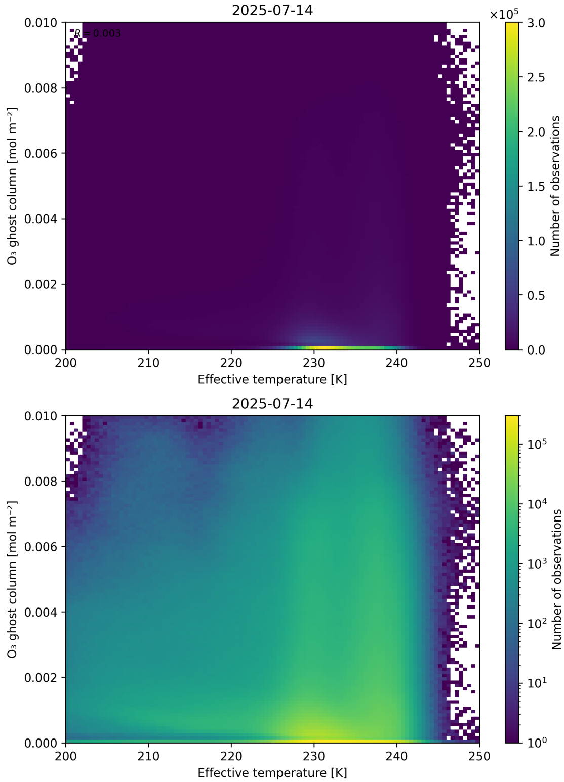
Figure 38: Scatter density plot of “Effective temperature” against “O 3 ghost column” for 2025-07-13 to 2025-07-15.
