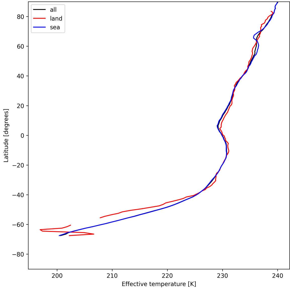
Figure 17: Zonal average of “Effective temperature” for 2025-07-13 to 2025-07-15.
