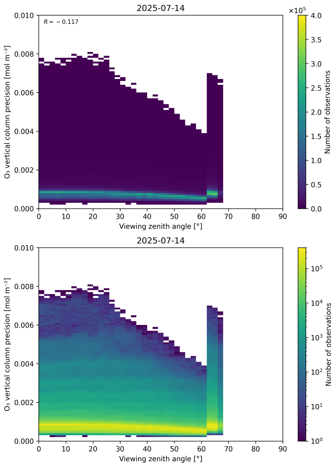
Figure 53: Scatter density plot of “Viewing zenith angle” against “O 3 vertical column precision” for 2025-07-13 to 2025-07-15.
