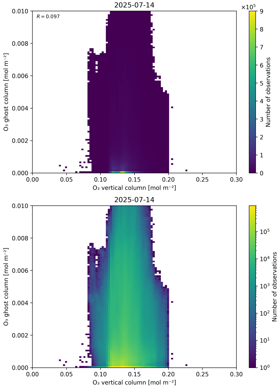
Figure 40: Scatter density plot of “O 3 vertical column” against “O 3 ghost column” for 2025-07-13 to 2025-07-15.
