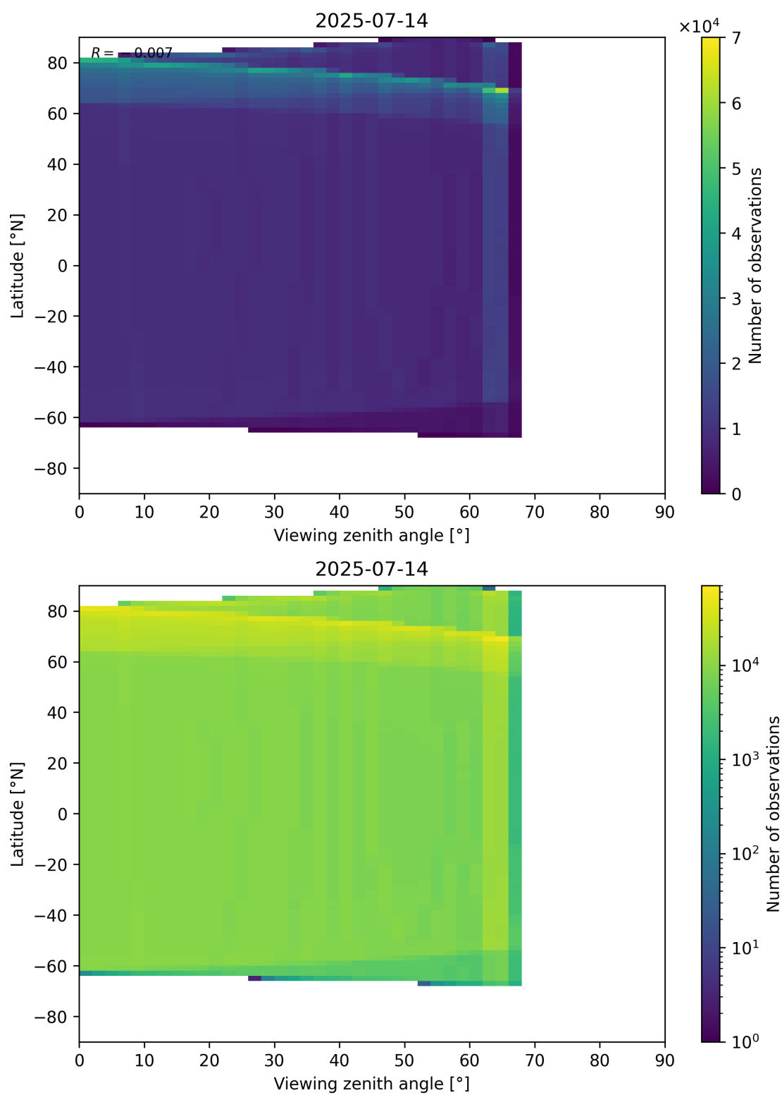
Figure 49: Scatter density plot of “Viewing zenith angle” against “Latitude” for 2025-07-13 to 2025-07-15.
