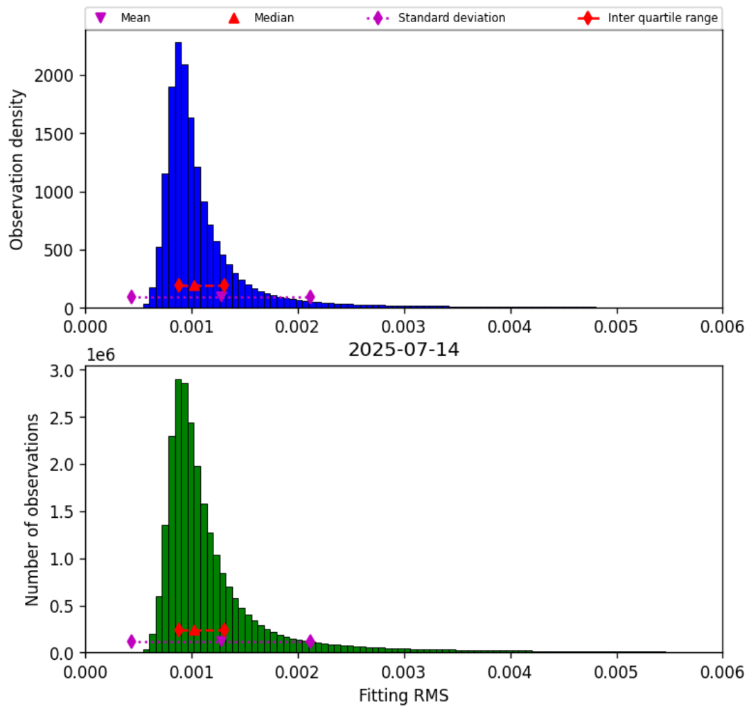
Figure 23: Histogram of “Fitting RMS” for 2025-07-13 to 2025-07-15
