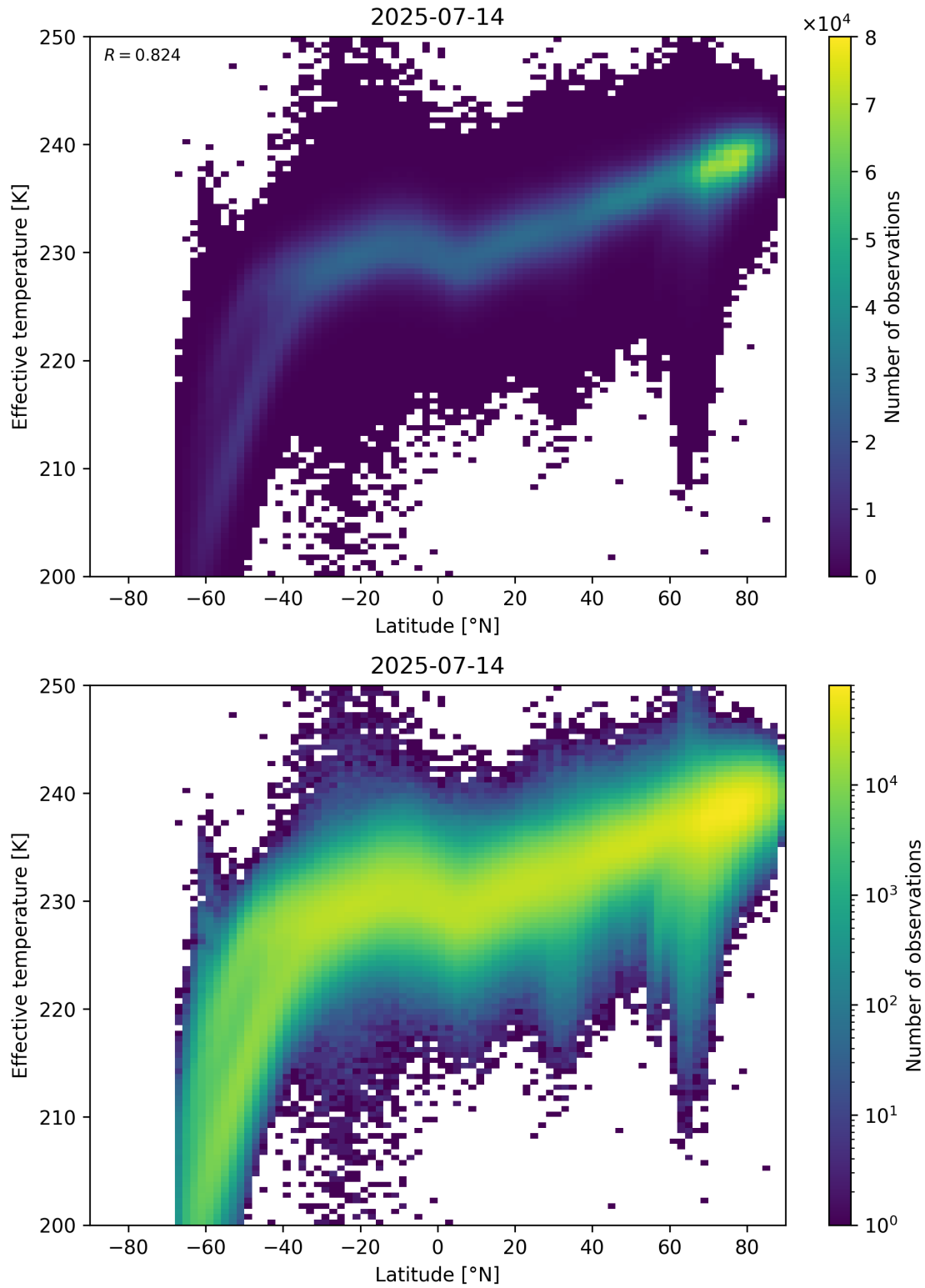
Figure 34: Scatter density plot of “Latitude” against “Effective temperature” for 2025-07-13 to 2025-07-15.
