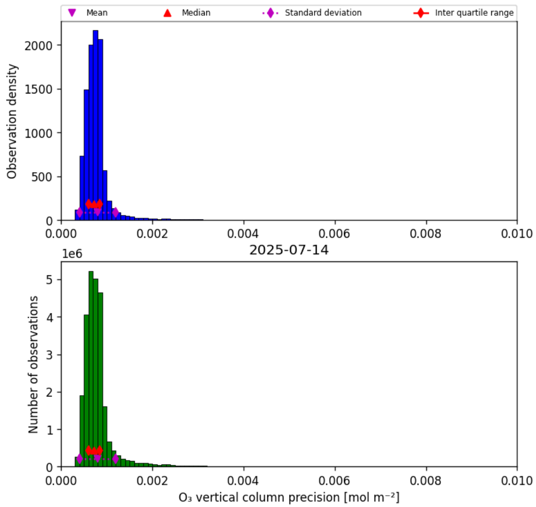
Figure 22: Histogram of “O 3 vertical column precision” for 2025-07-13 to 2025-07-15
