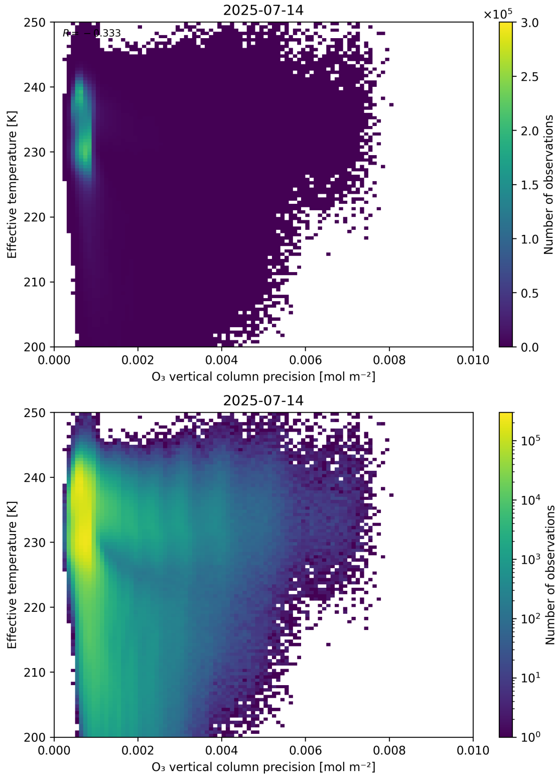
Figure 42: Scatter density plot of “O 3 vertical column precision” against “Effective temperature” for 2025-07-13 to 2025-07-15.
