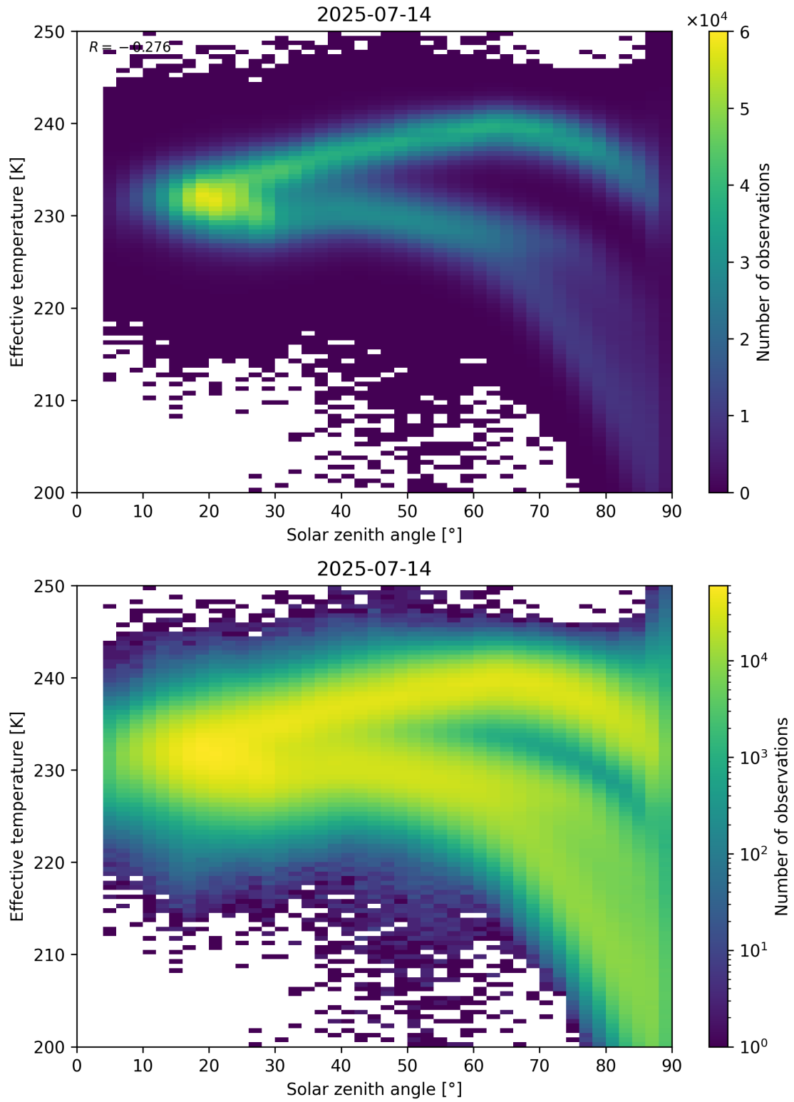
Figure 45: Scatter density plot of “Solar zenith angle” against “Effective temperature” for 2025-07-13 to 2025-07-15.
