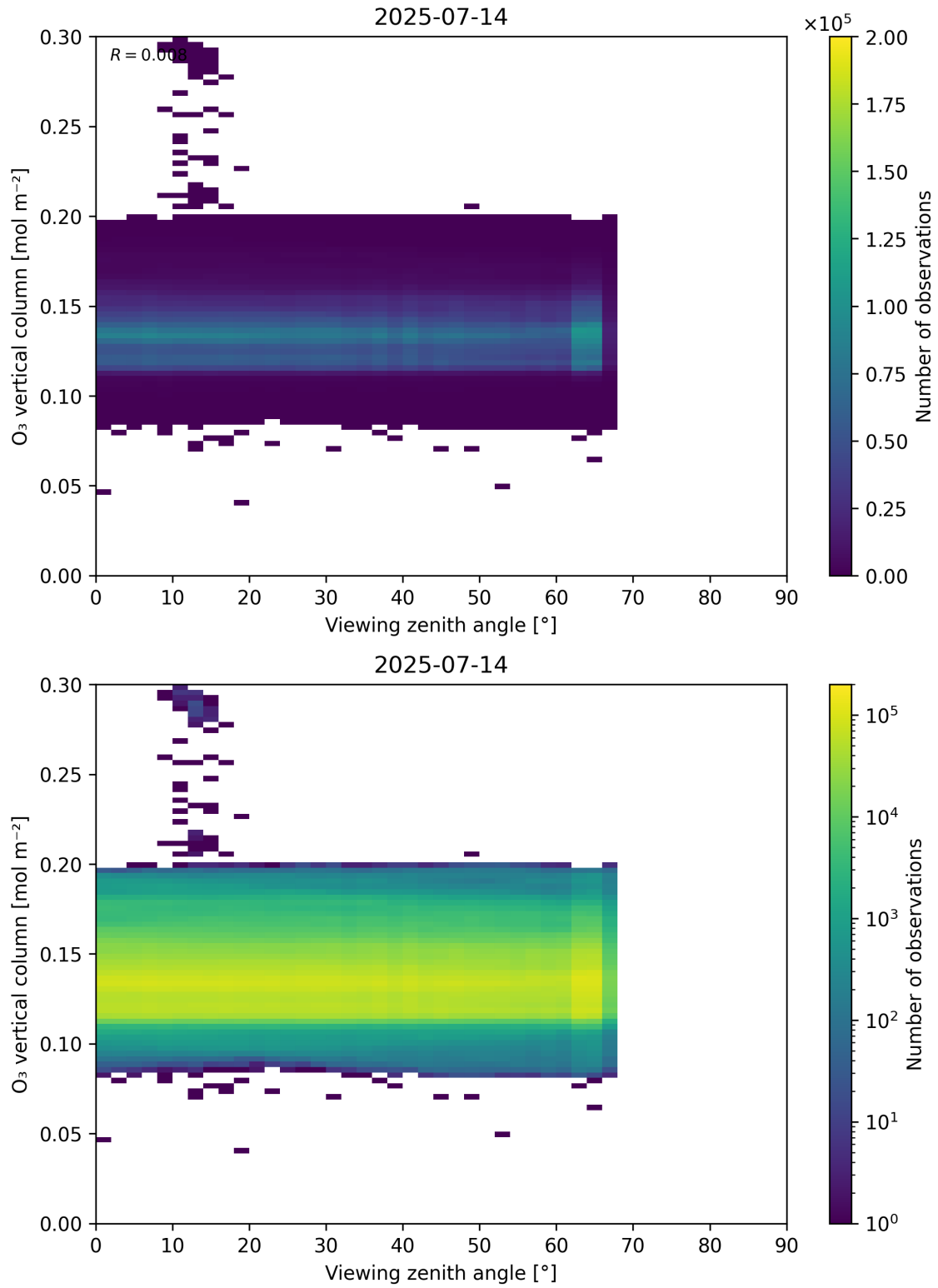
Figure 52: Scatter density plot of “Viewing zenith angle” against “O 3 vertical column” for 2025-07-13 to 2025-07-15.
