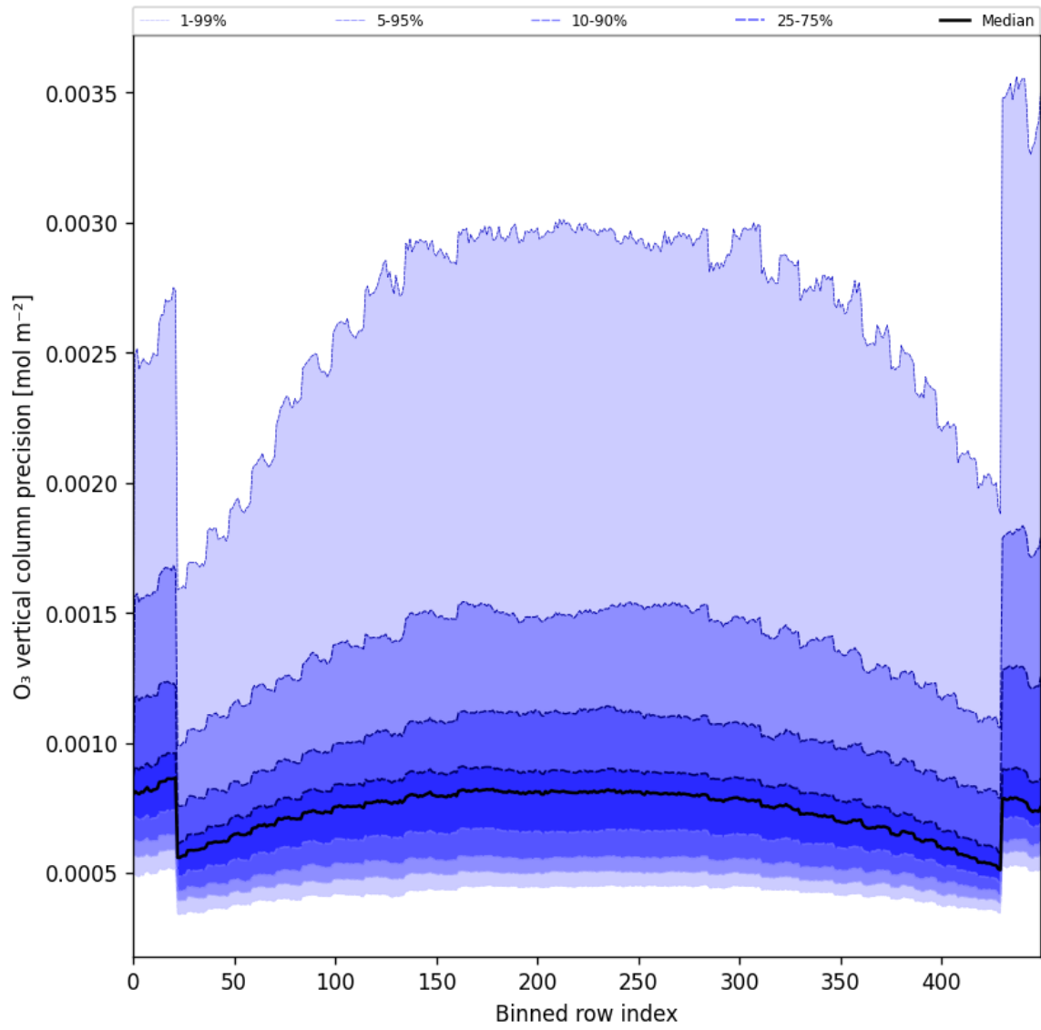
Figure 29: Along track statistics of “O 3 vertical column precision” for 2025-07-13 to 2025-07-15
