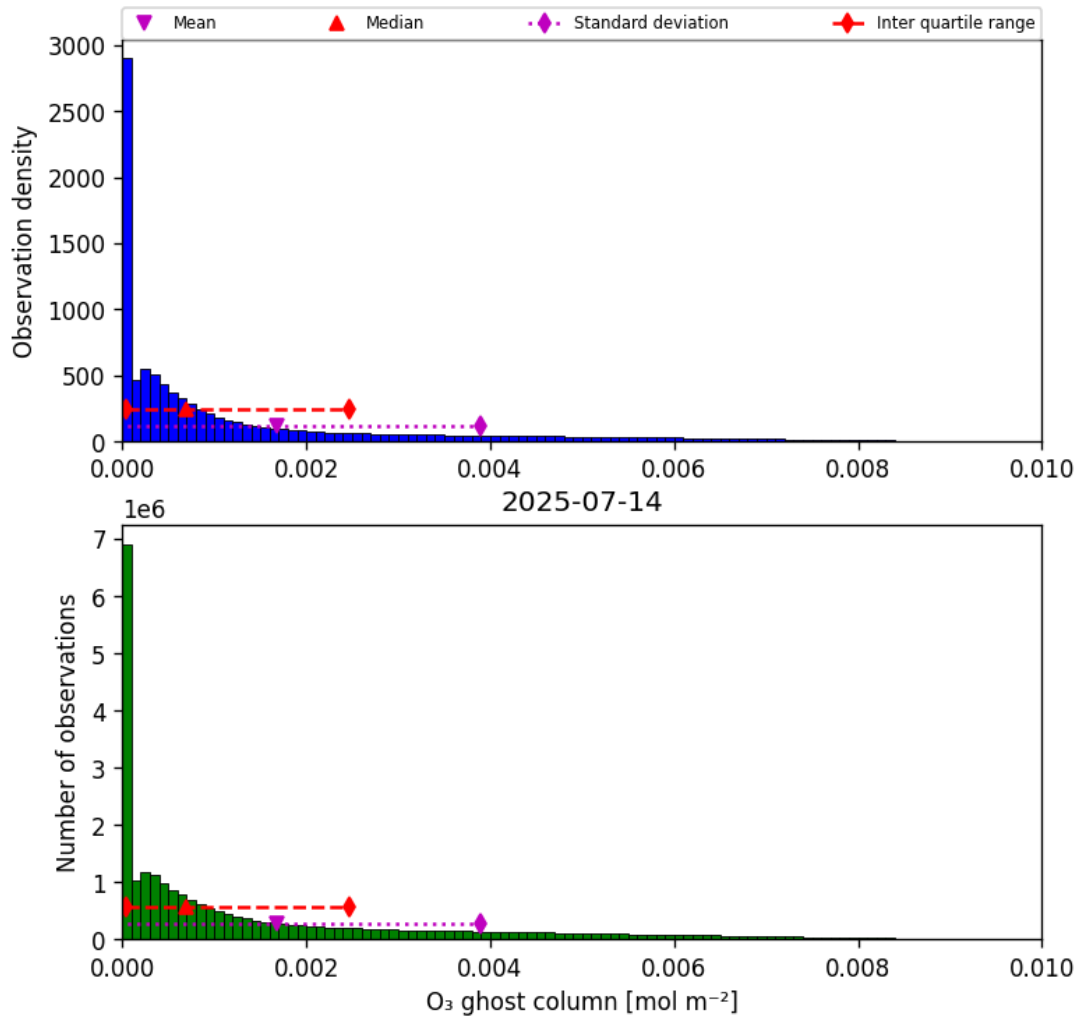
Figure 25: Histogram of “O 3 ghost column” for 2025-07-13 to 2025-07-15
