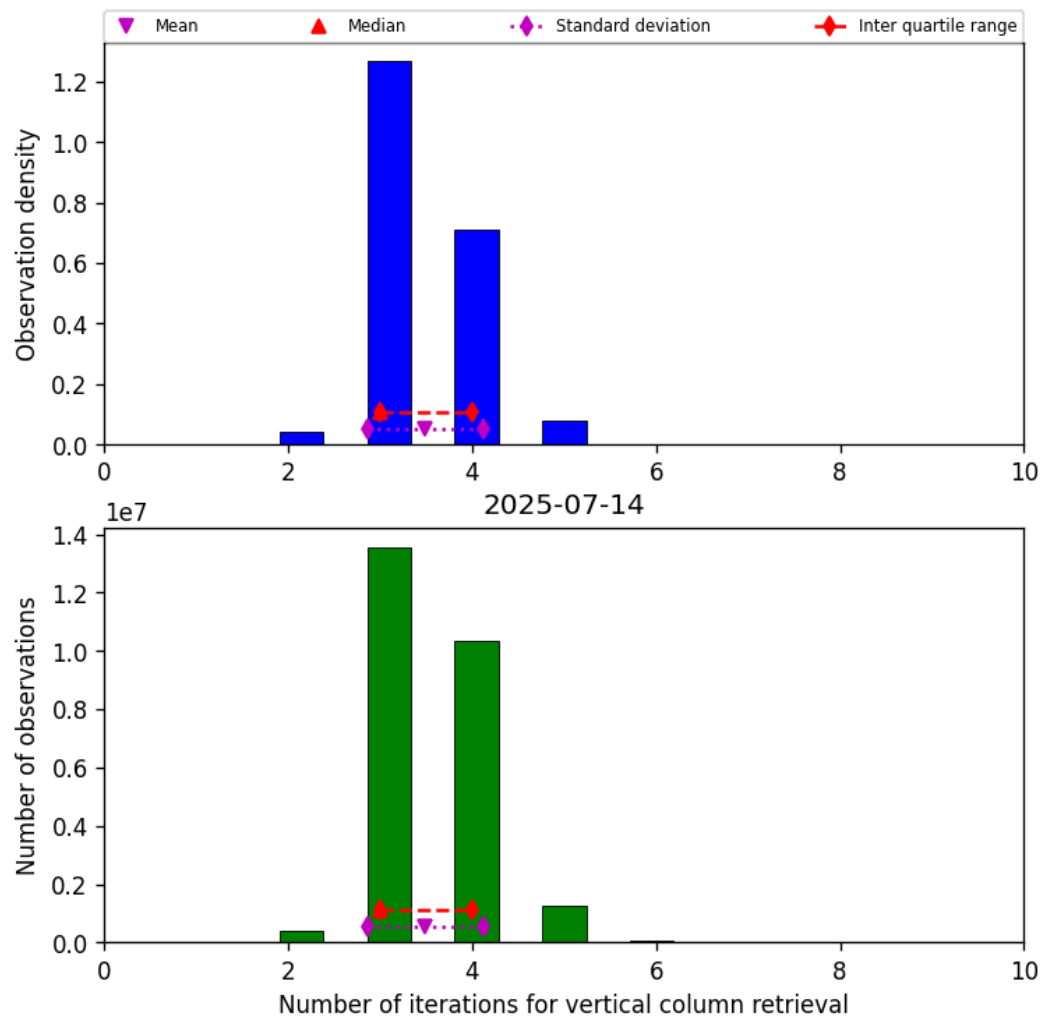
Figure 26: Histogram of “Number of iterations for vertical column retrieval” for 2025-07-13 to 2025-07-15
