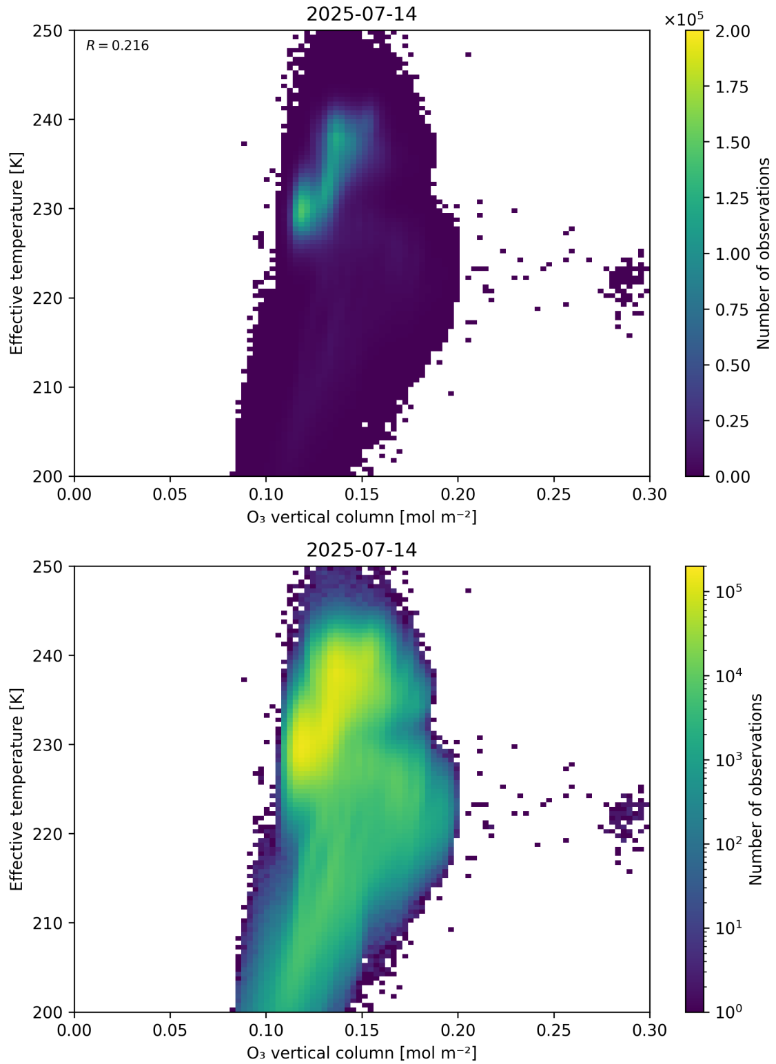
Figure 39: Scatter density plot of “O 3 vertical column” against “Effective temperature” for 2025-07-13 to 2025-07-15.
