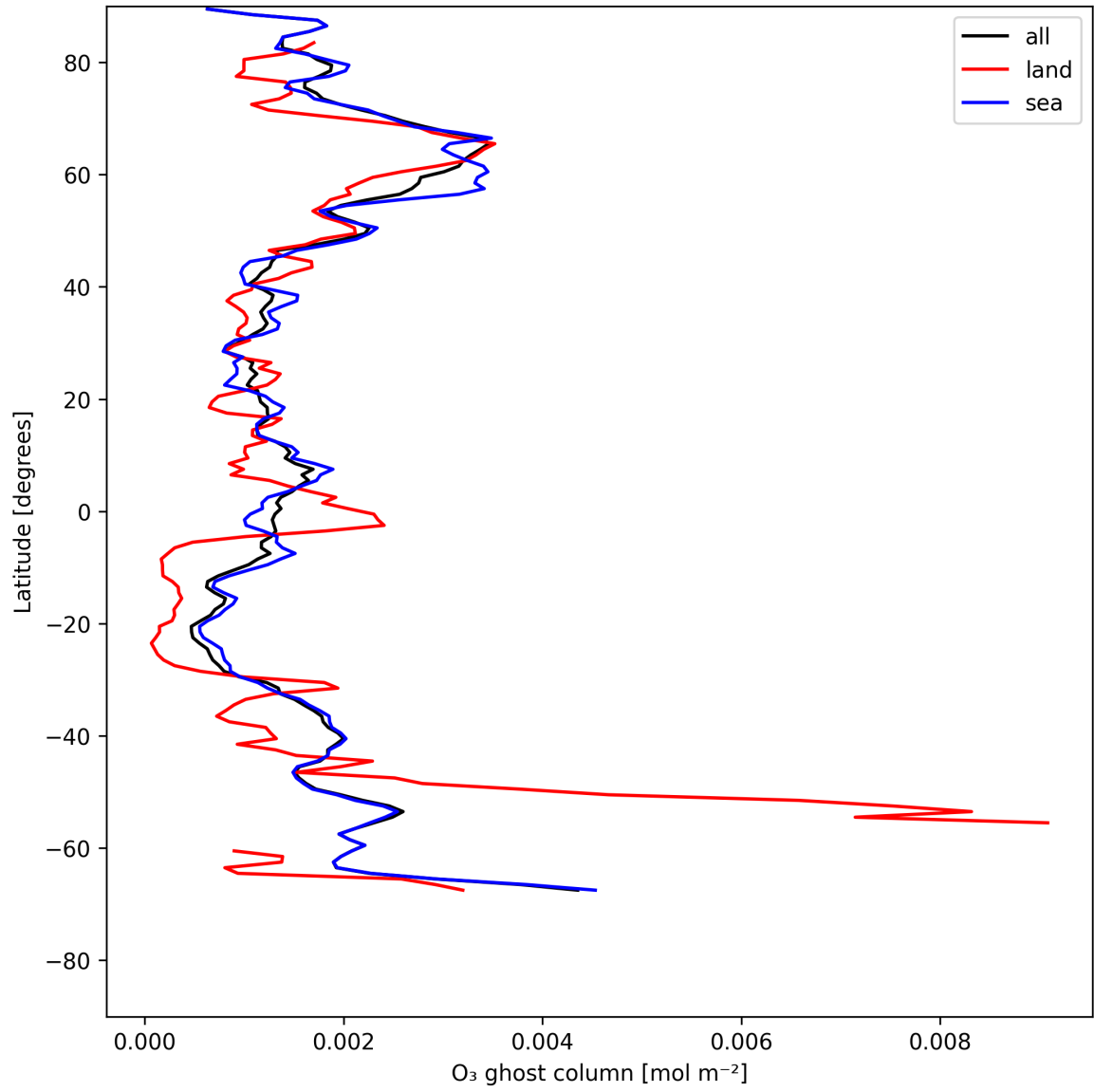
Figure 18: Zonal average of “O 3 ghost column” for 2025-07-13 to 2025-07-15.
