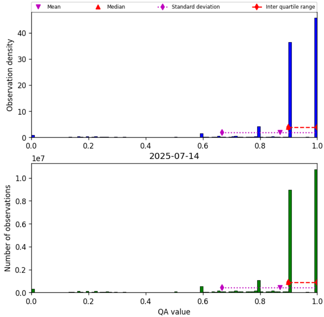
Figure 20: Histogram of “QA value” for 2025-07-13 to 2025-07-15
