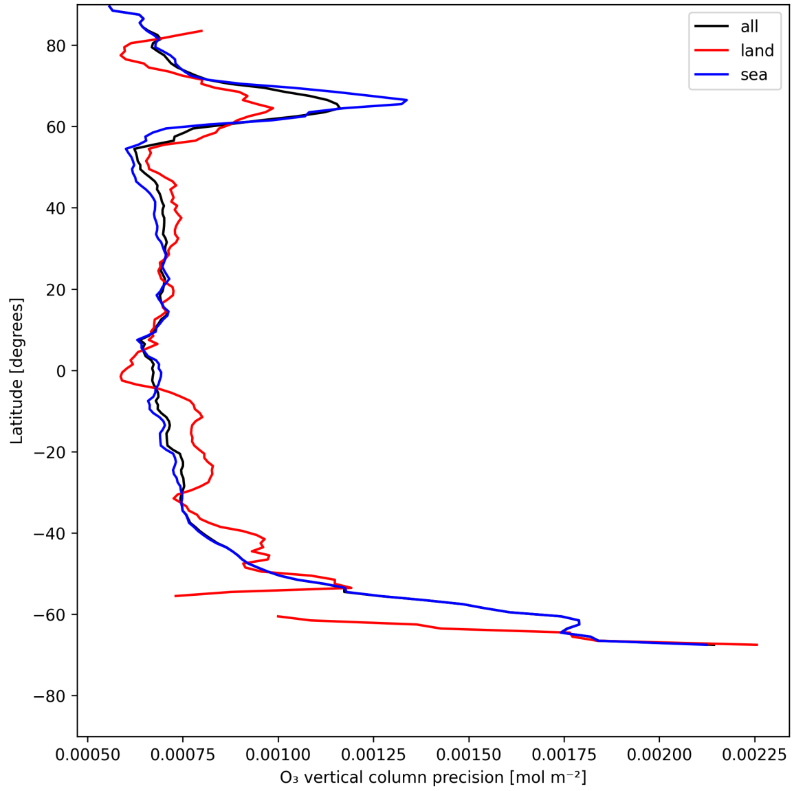
Figure 15: Zonal average of “O 3 vertical column precision” for 2025-07-13 to 2025-07-15.
