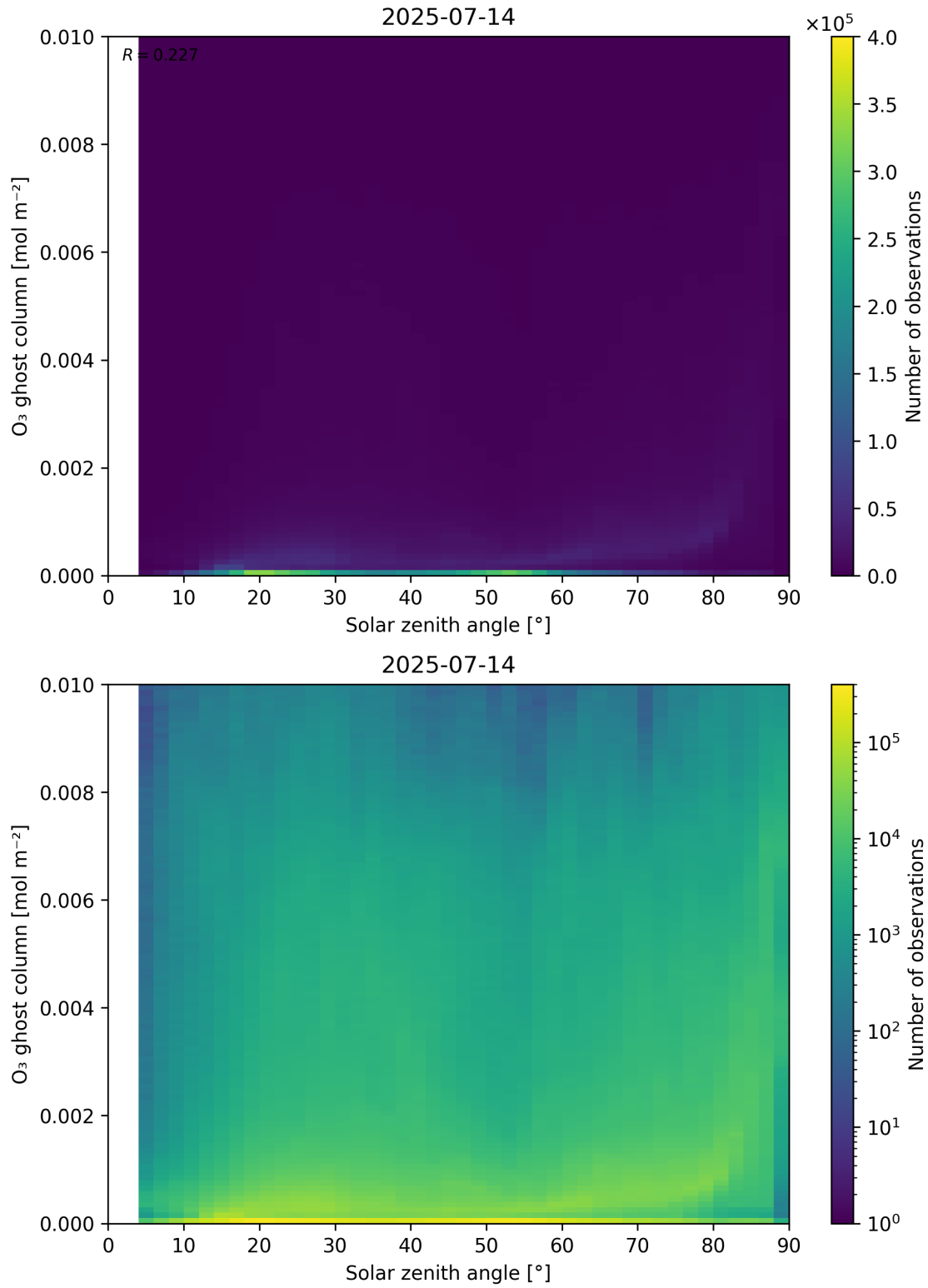
Figure 46: Scatter density plot of “Solar zenith angle” against “O 3 ghost column” for 2025-07-13 to 2025-07-15.
