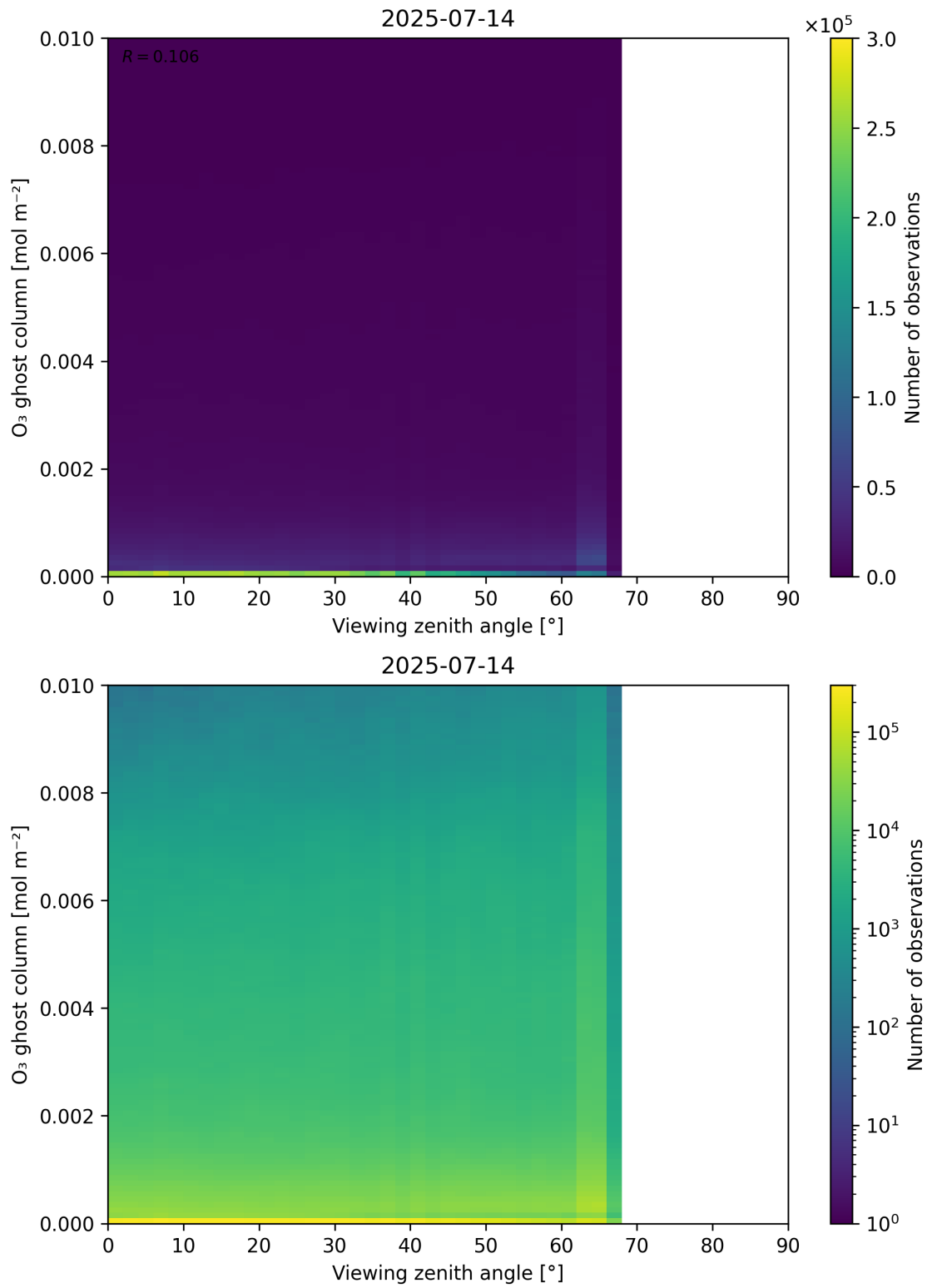
Figure 51: Scatter density plot of “Viewing zenith angle” against “O 3 ghost column” for 2025-07-13 to 2025-07-15.
