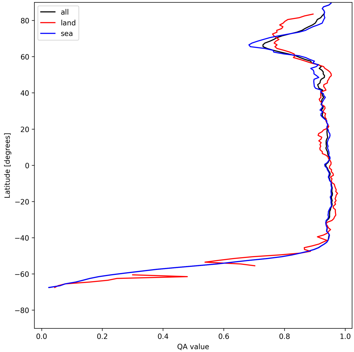
Figure 13: Zonal average of “QA value” for 2025-07-13 to 2025-07-15.
