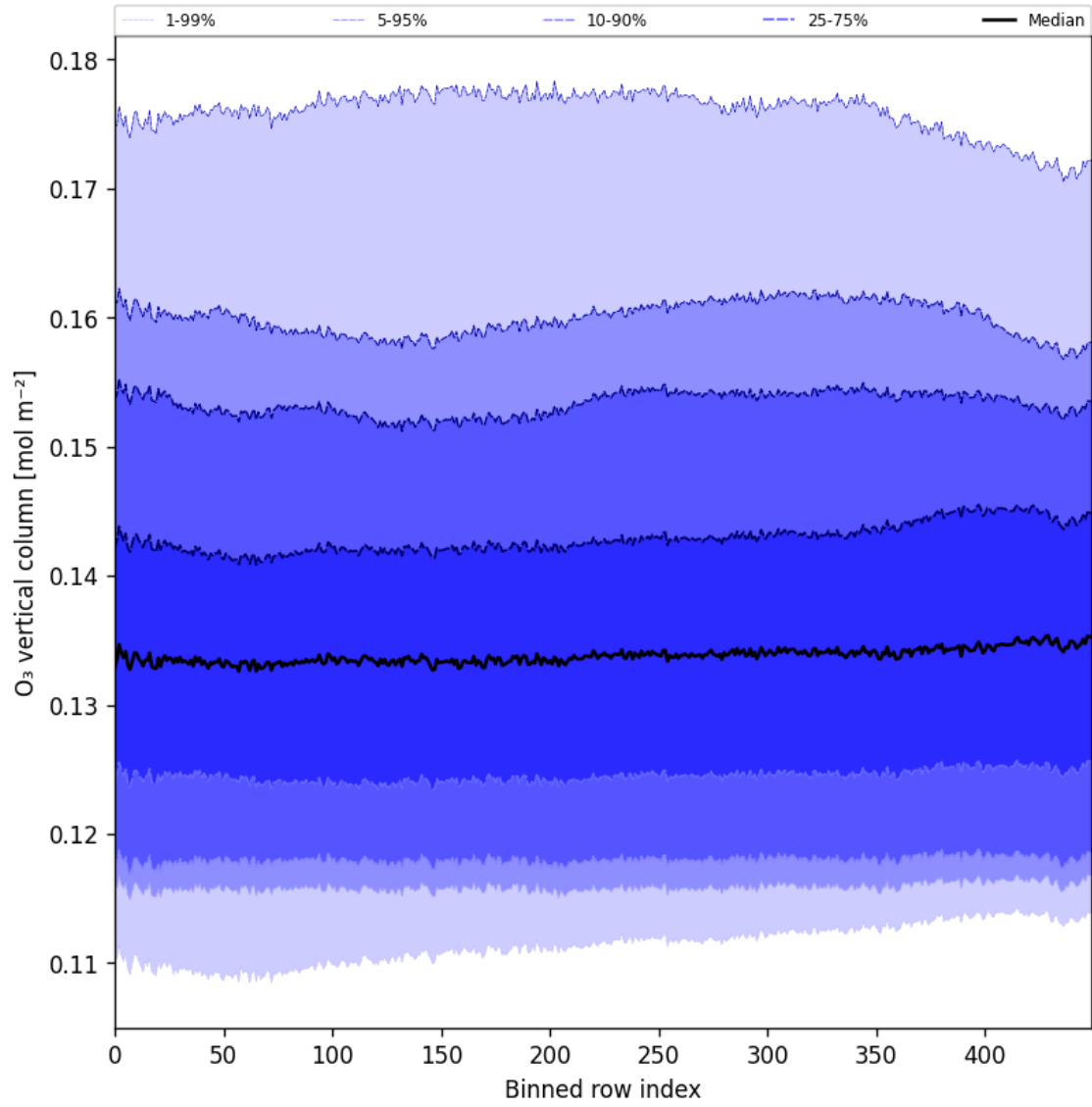
Figure 28: Along track statistics of “O 3 vertical column” for 2025-07-13 to 2025-07-15
