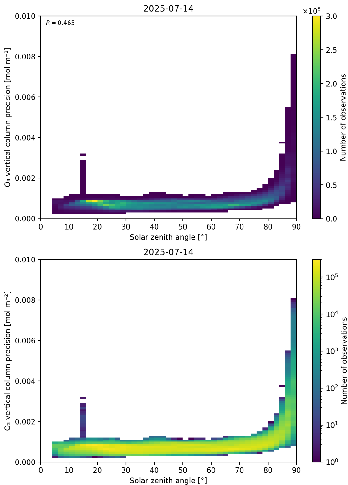
Figure 48: Scatter density plot of “Solar zenith angle” against “O 3 vertical column precision” for 2025-07-13 to 2025-07-15.
