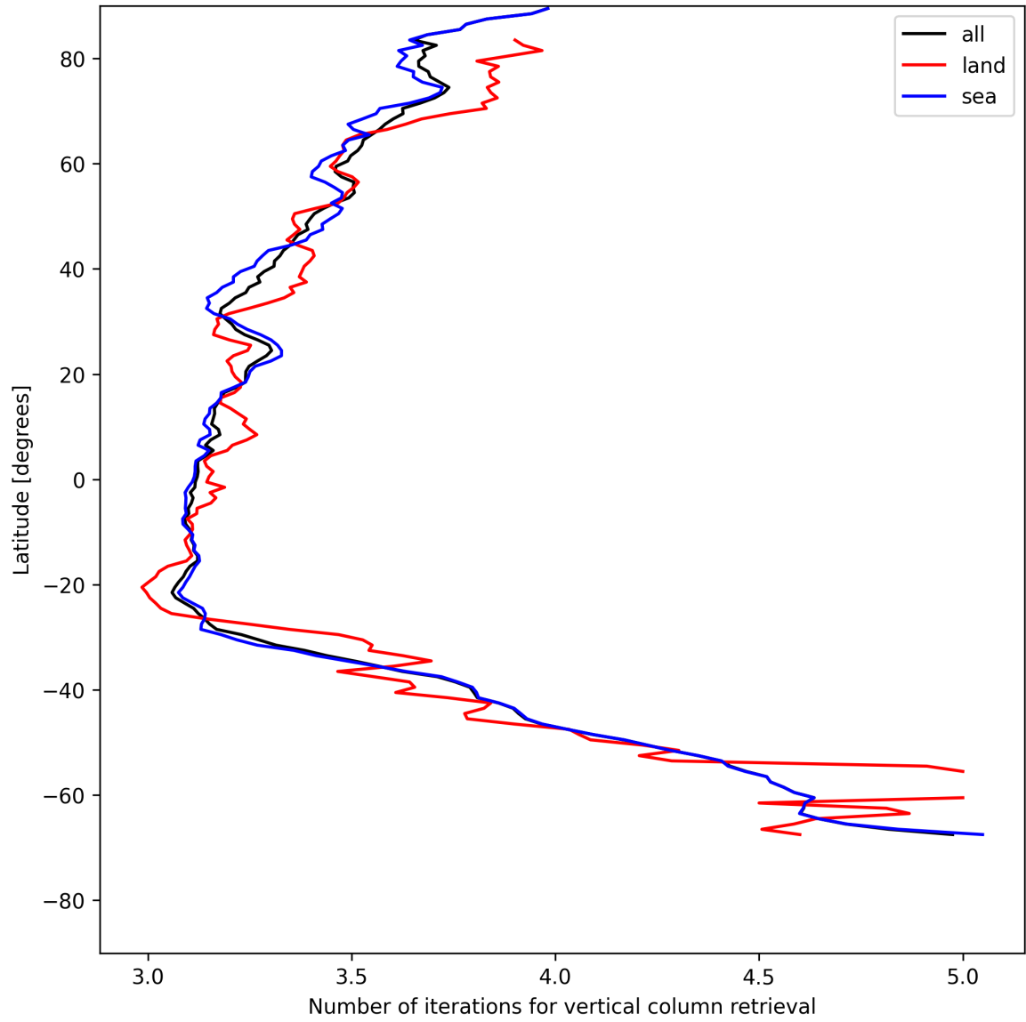
Figure 19: Zonal average of “Number of iterations for vertical column retrieval” for 2025-07-13 to 2025-07-15.
