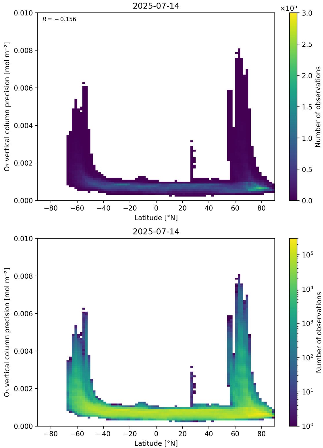
Figure 37: Scatter density plot of “Latitude” against “O 3 vertical column precision” for 2025-07-13 to 2025-07-15.
