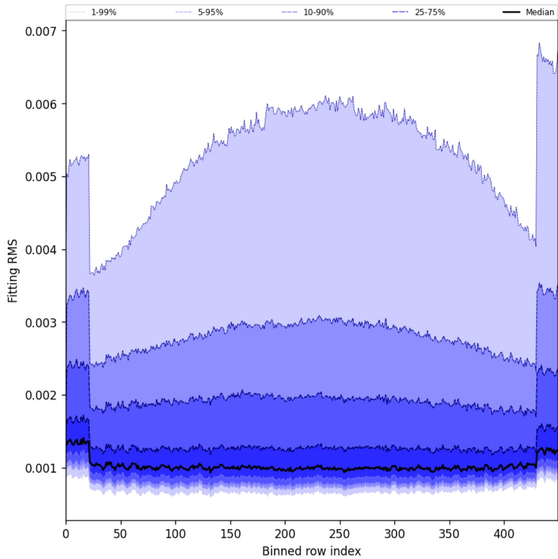
Figure 30: Along track statistics of “Fitting RMS” for 2025-07-14 to 2025-07-16
