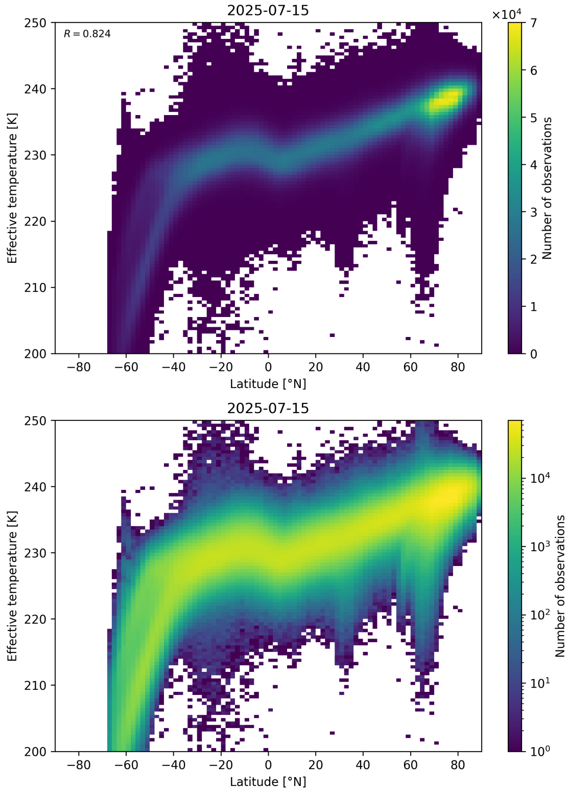
Figure 34: Scatter density plot of “Latitude” against “Effective temperature” for 2025-07-14 to 2025-07-16.
