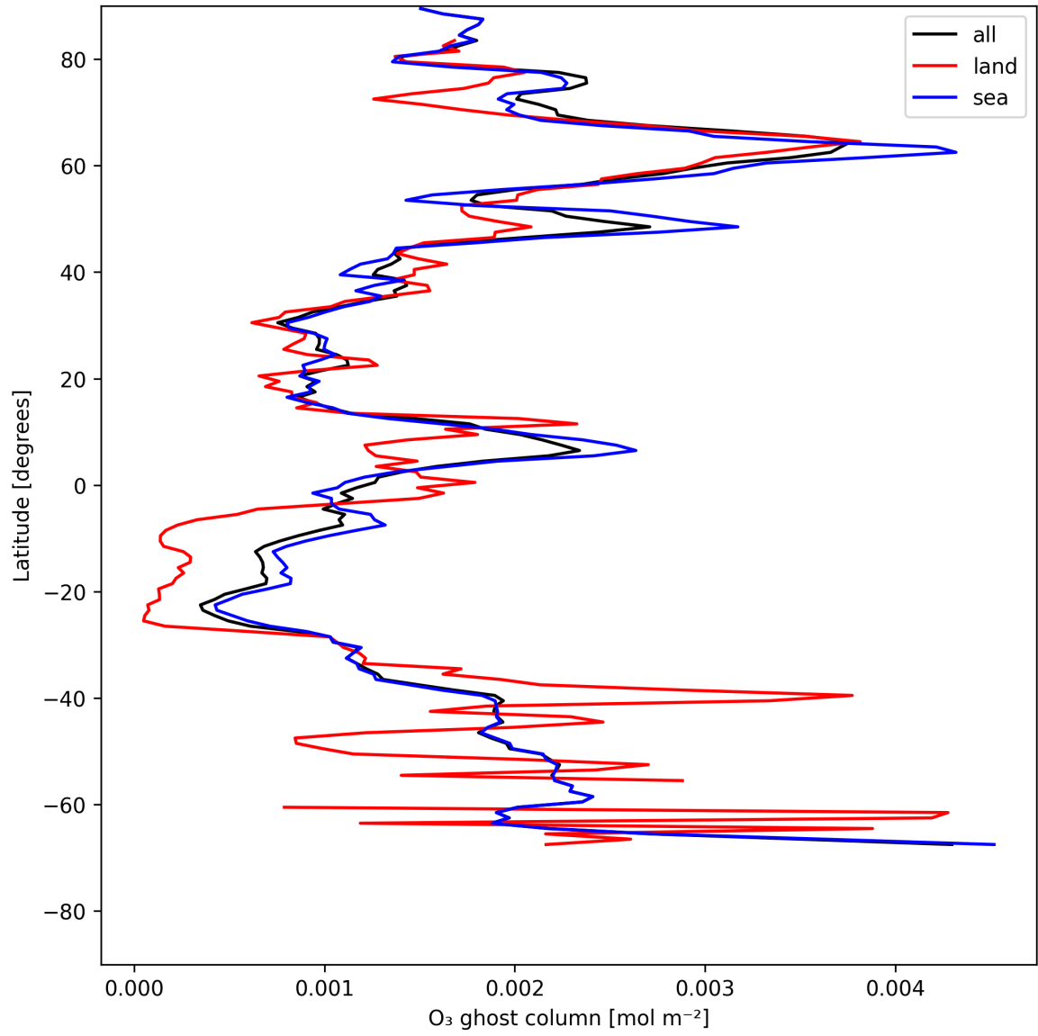
Figure 18: Zonal average of "O 3 ghost column" for 2025-07-14 to 2025-07-16.
