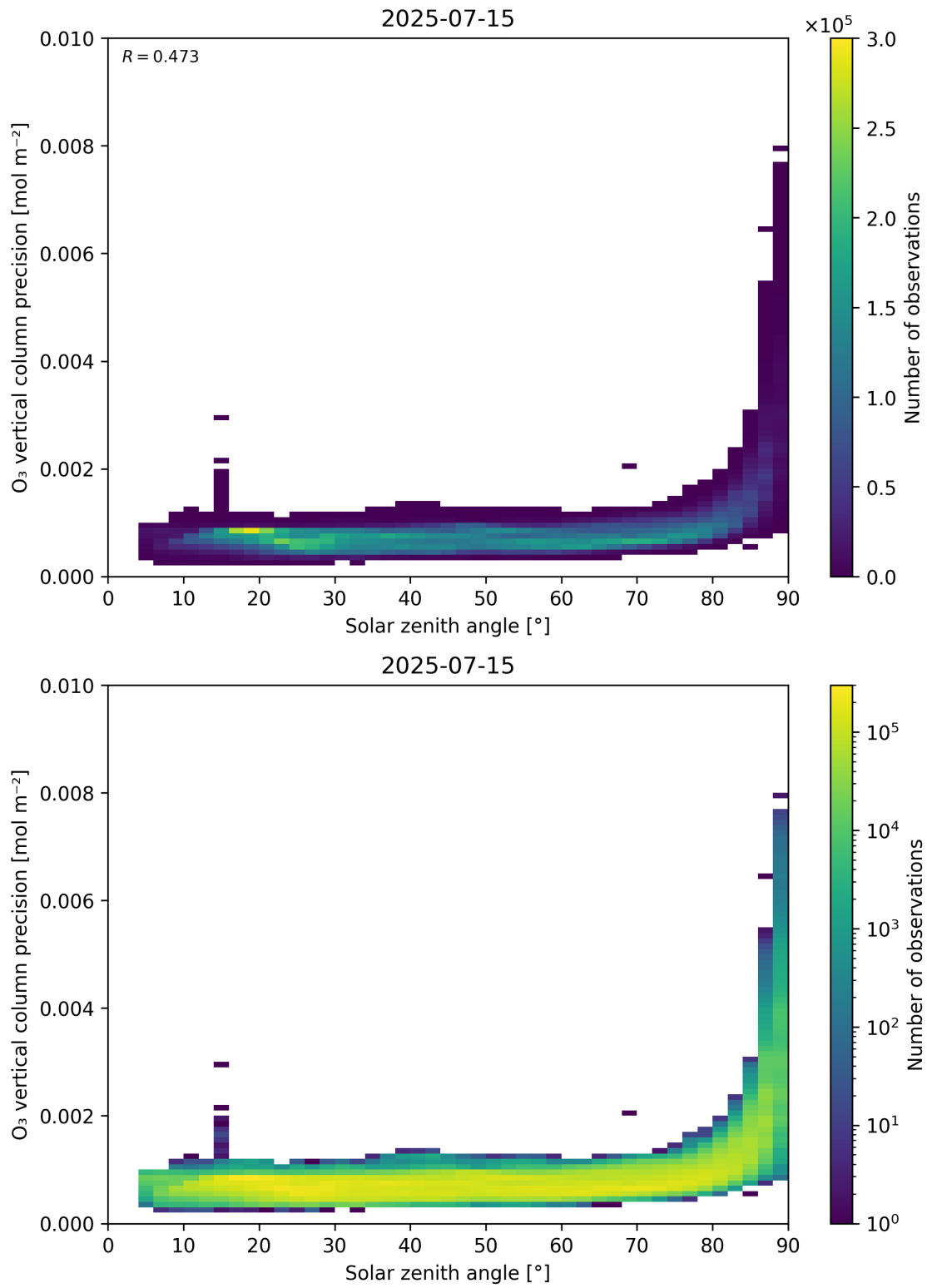
Figure 48: Scatter density plot of “Solar zenith angle” against “O 3 vertical column precision” for 2025-07-14 to 2025-07-16.
