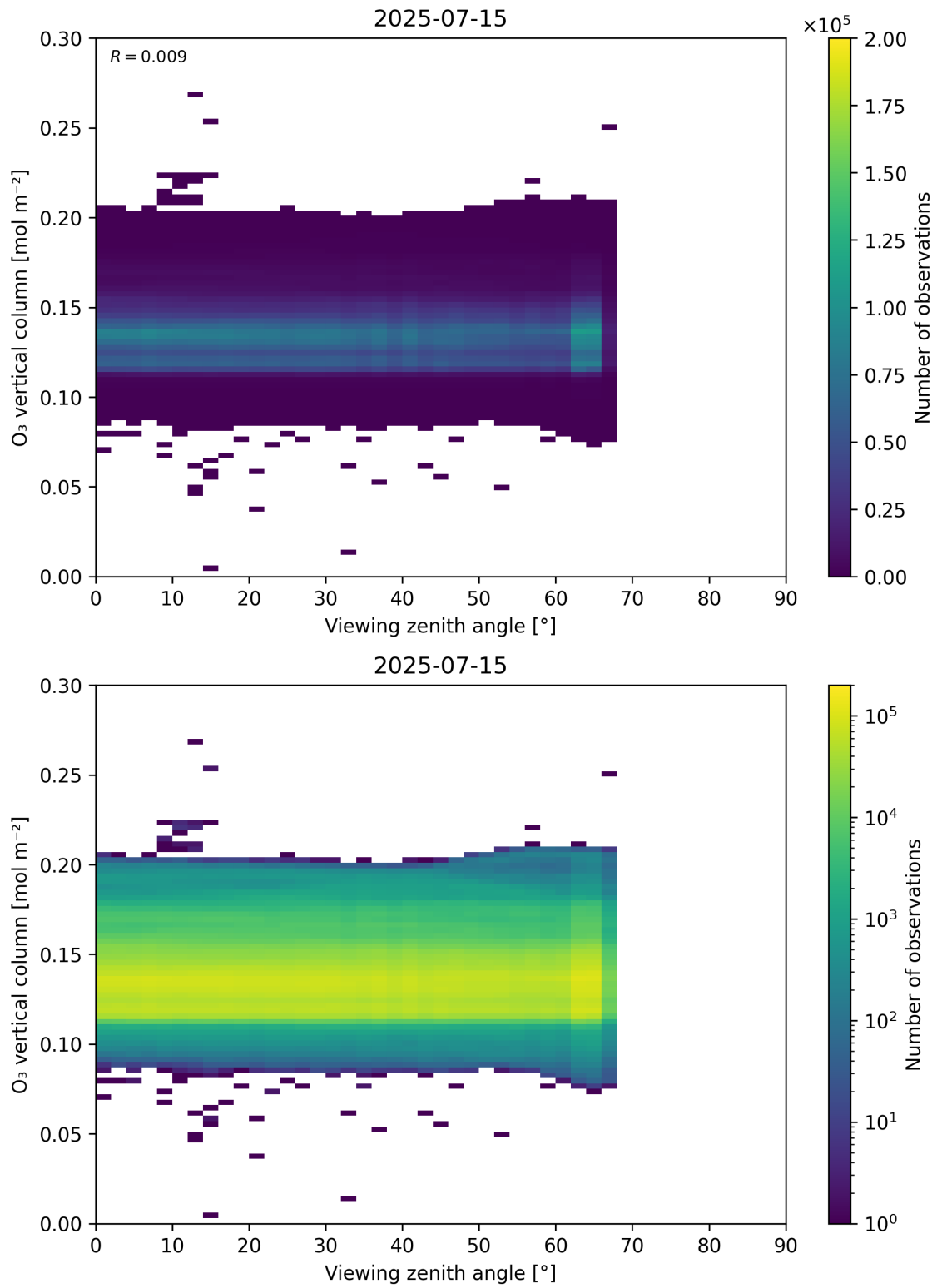
Figure 52: Scatter density plot of “Viewing zenith angle” against “O 3 vertical column” for 2025-07-14 to 2025-07-16.
