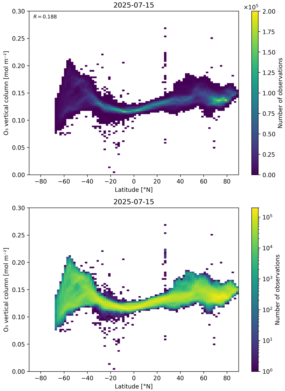
Figure 36: Scatter density plot of “Latitude” against “O 3 vertical column” for 2025-07-14 to 2025-07-16.
