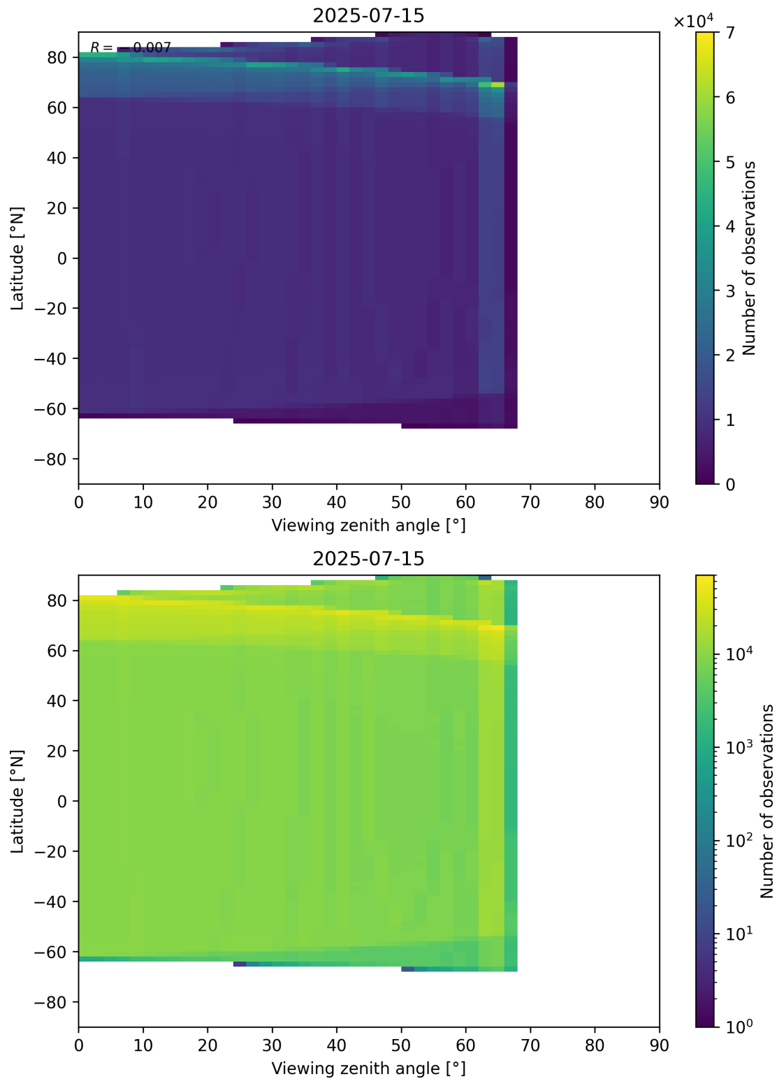
Figure 49: Scatter density plot of “Viewing zenith angle” against “Latitude” for 2025-07-14 to 2025-07-16.
