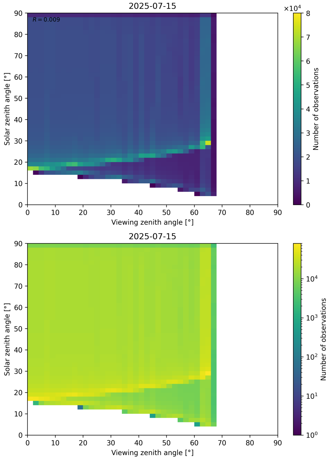
Figure 54: Scatter density plot of “Viewing zenith angle” against “Solar zenith angle” for 2025-07-14 to 2025-07-16.
