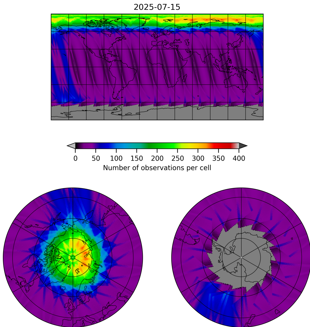
Figure 12: Map of the number of observations for 2025-07-14 to 2025-07-16
