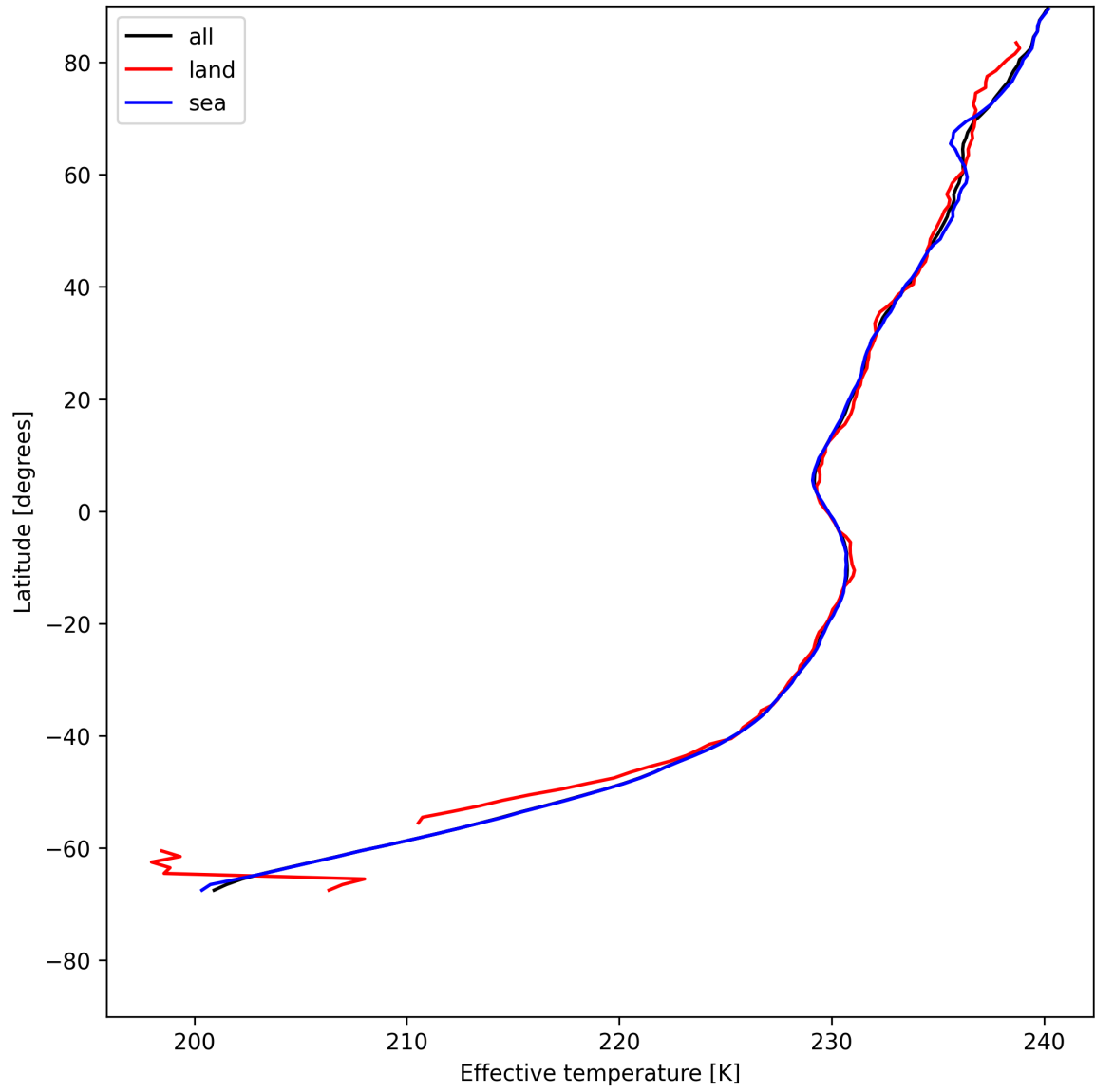
Figure 17: Zonal average of "Effective temperature" for 2025-07-14 to 2025-07-16.
