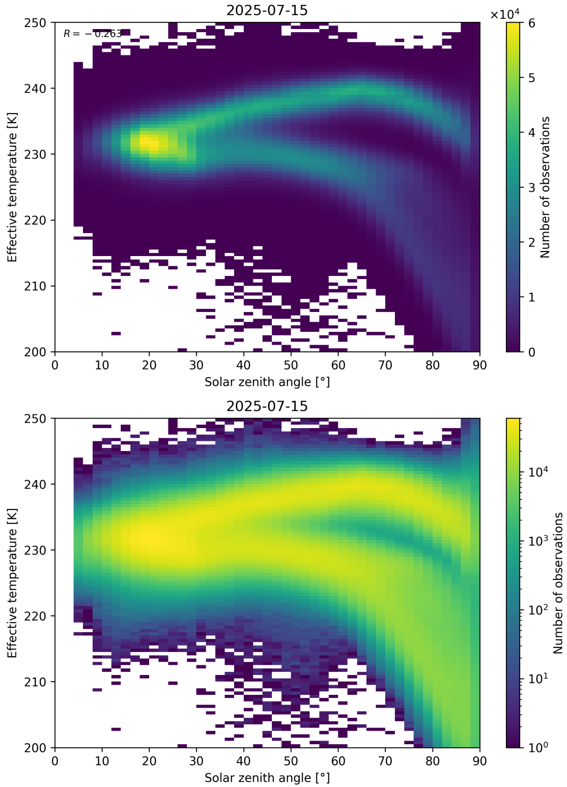
Figure 45: Scatter density plot of “Solar zenith angle” against “Effective temperature” for 2025-07-14 to 2025-07-16.
