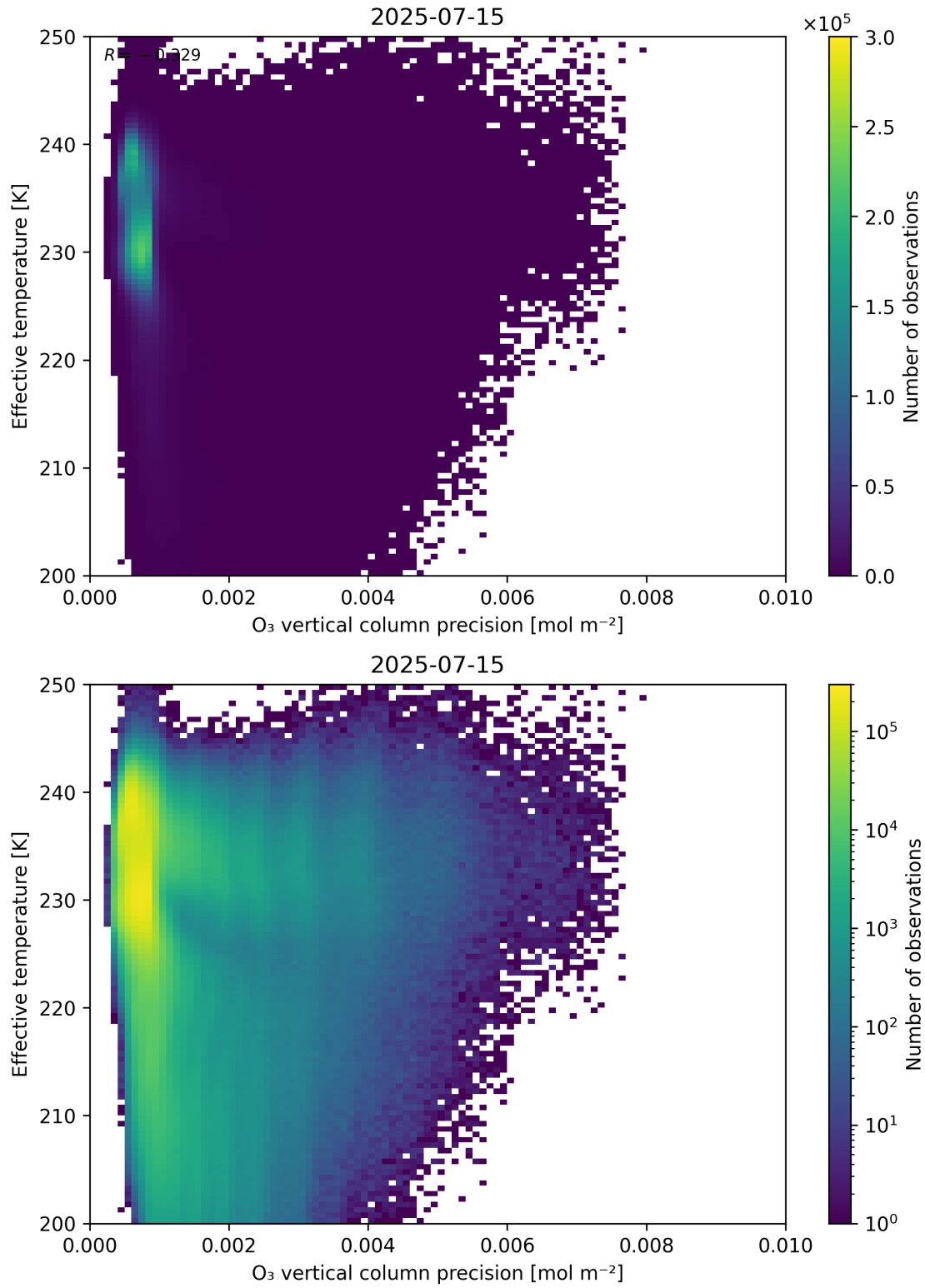
Figure 42: Scatter density plot of “O 3 vertical column precision” against “Effective temperature” for 2025-07-14 to 2025-07-16.
