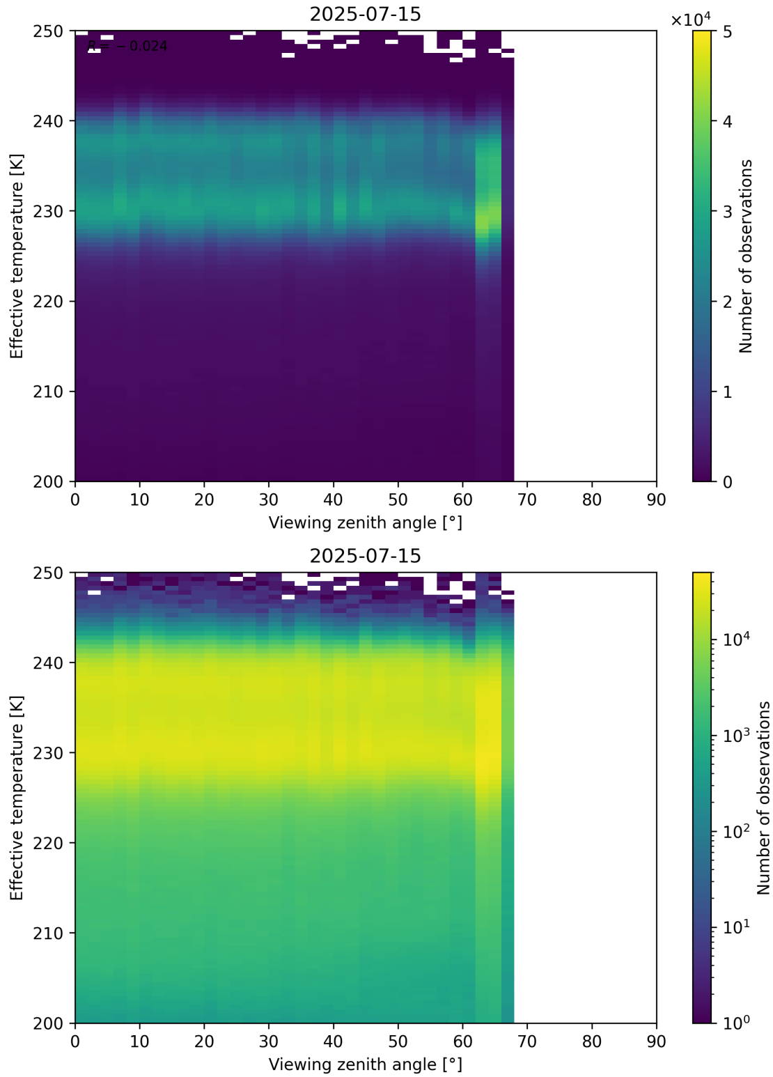
Figure 50: Scatter density plot of “Viewing zenith angle” against “Effective temperature” for 2025-07-14 to 2025-07-16.
