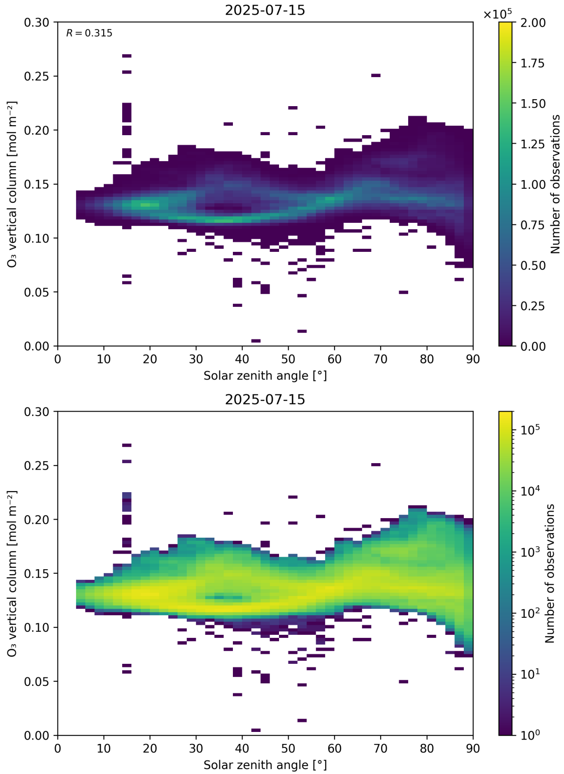
Figure 47: Scatter density plot of “Solar zenith angle” against “O 3 vertical column” for 2025-07-14 to 2025-07-16.
