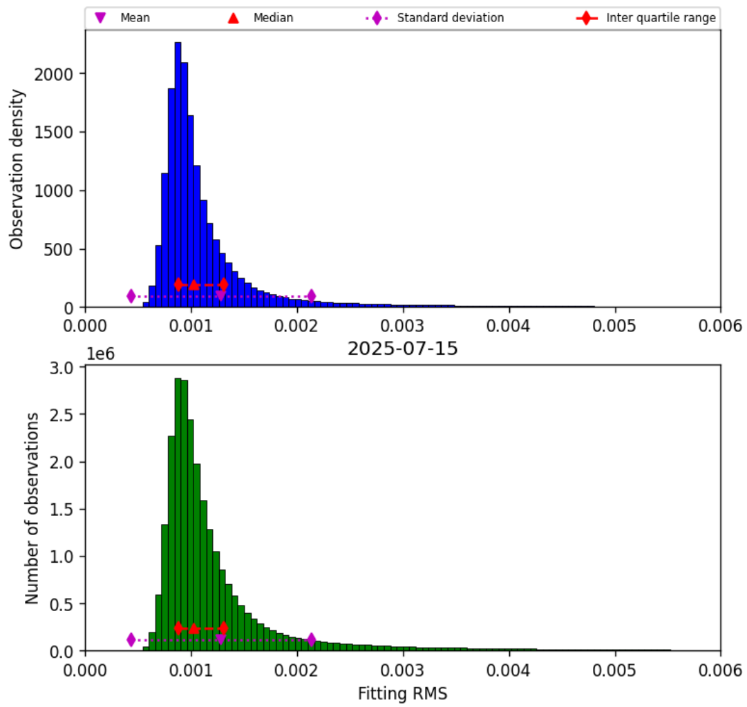
Figure 23: Histogram of “Fitting RMS” for 2025-07-14 to 2025-07-16
