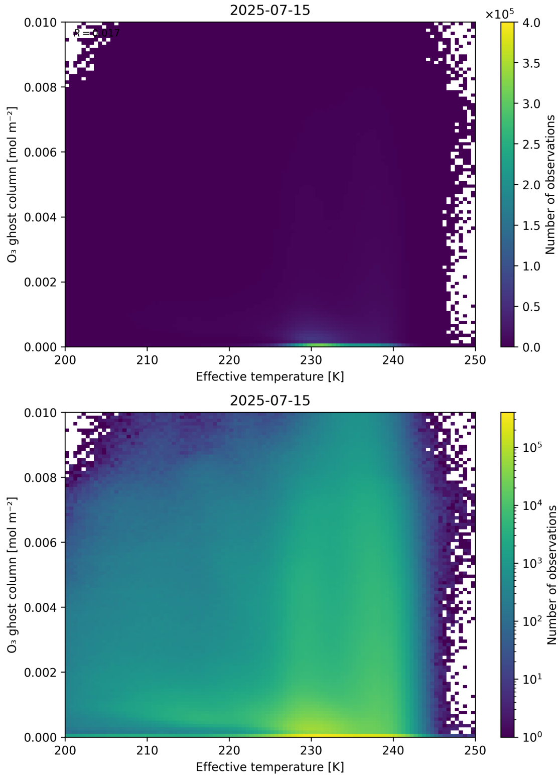
Figure 38: Scatter density plot of “Effective temperature” against “O 3 ghost column” for 2025-07-14 to 2025-07-16.
