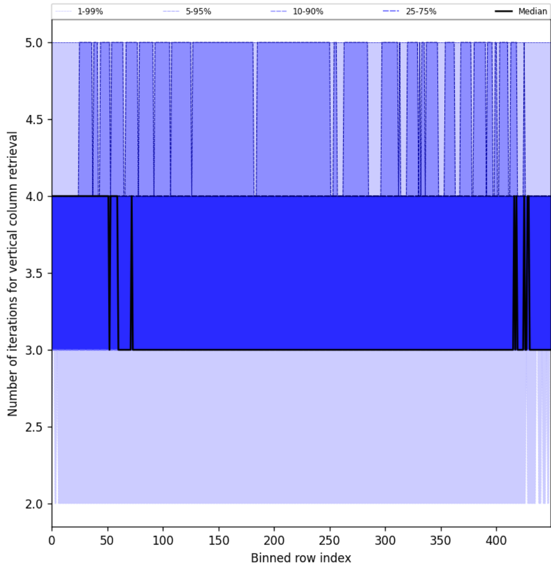
Figure 33: Along track statistics of “Number of iterations for vertical column retrieval” for 2025-07-14 to 2025-07-16
