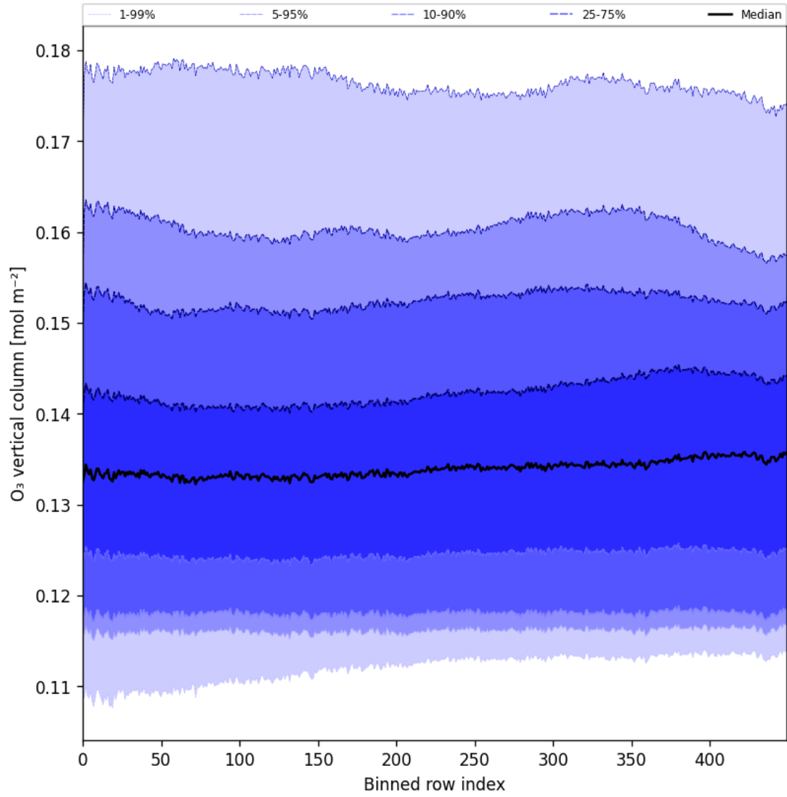
Figure 28: Along track statistics of “ O_3 vertical column” for 2025-07-14 to 2025-07-16
