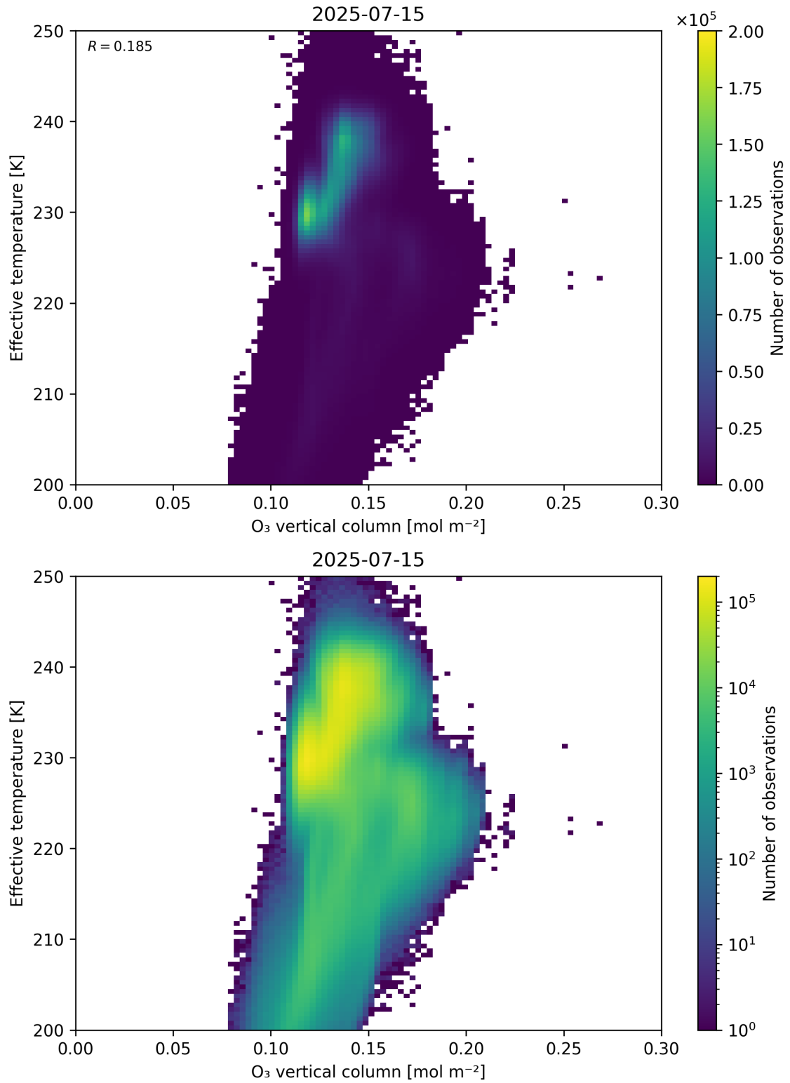
Figure 39: Scatter density plot of “O 3 vertical column” against “Effective temperature” for 2025-07-14 to 2025-07-16.
