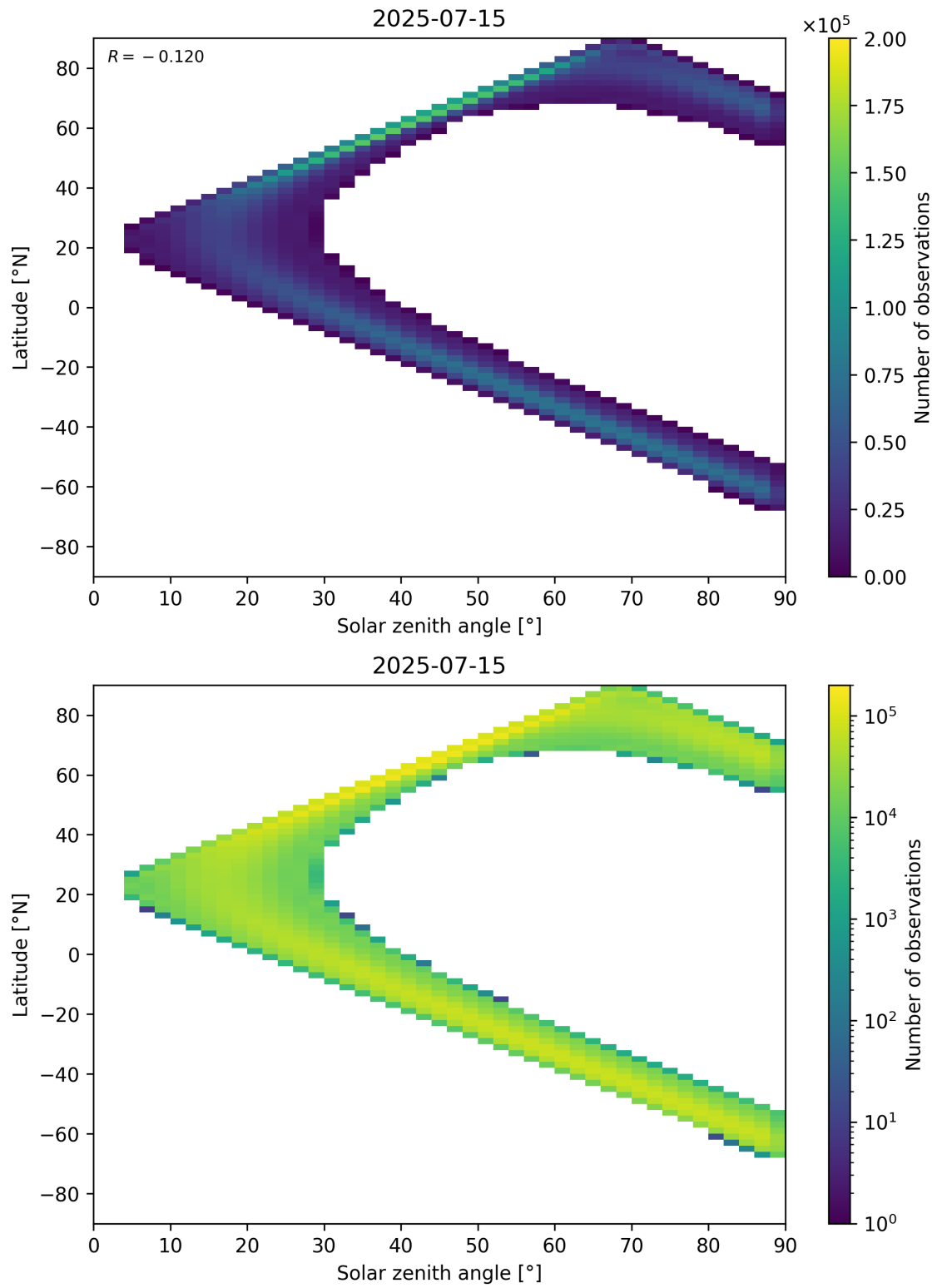
Figure 44: Scatter density plot of “Solar zenith angle” against “Latitude” for 2025-07-14 to 2025-07-16.
