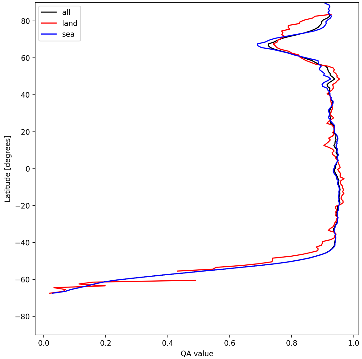
Figure 13: Zonal average of “QA value” for 2025-07-14 to 2025-07-16.
