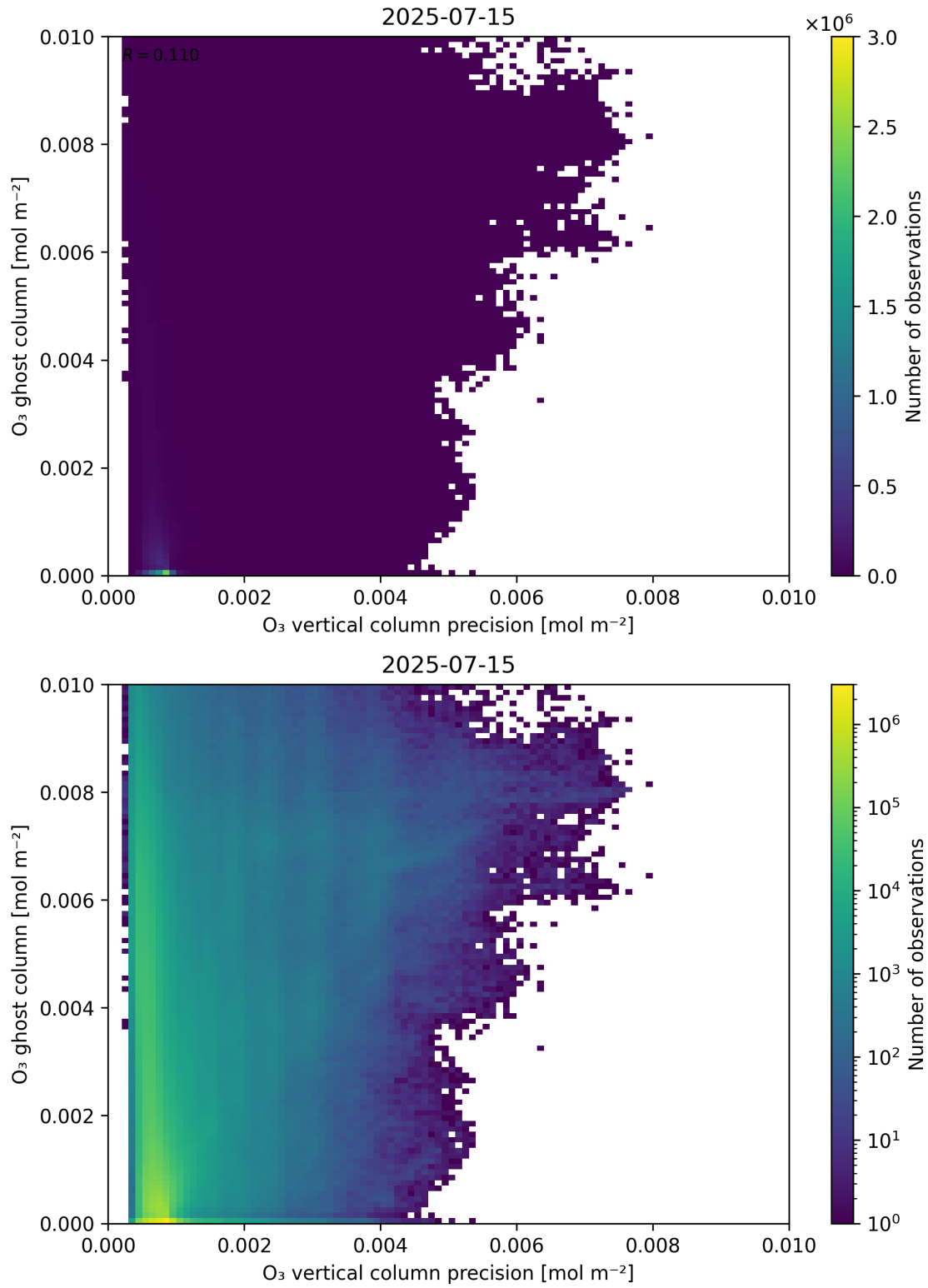
Figure 43: Scatter density plot of “O 3 vertical column precision” against “O 3 ghost column” for 2025-07-14 to 2025-07-16.
