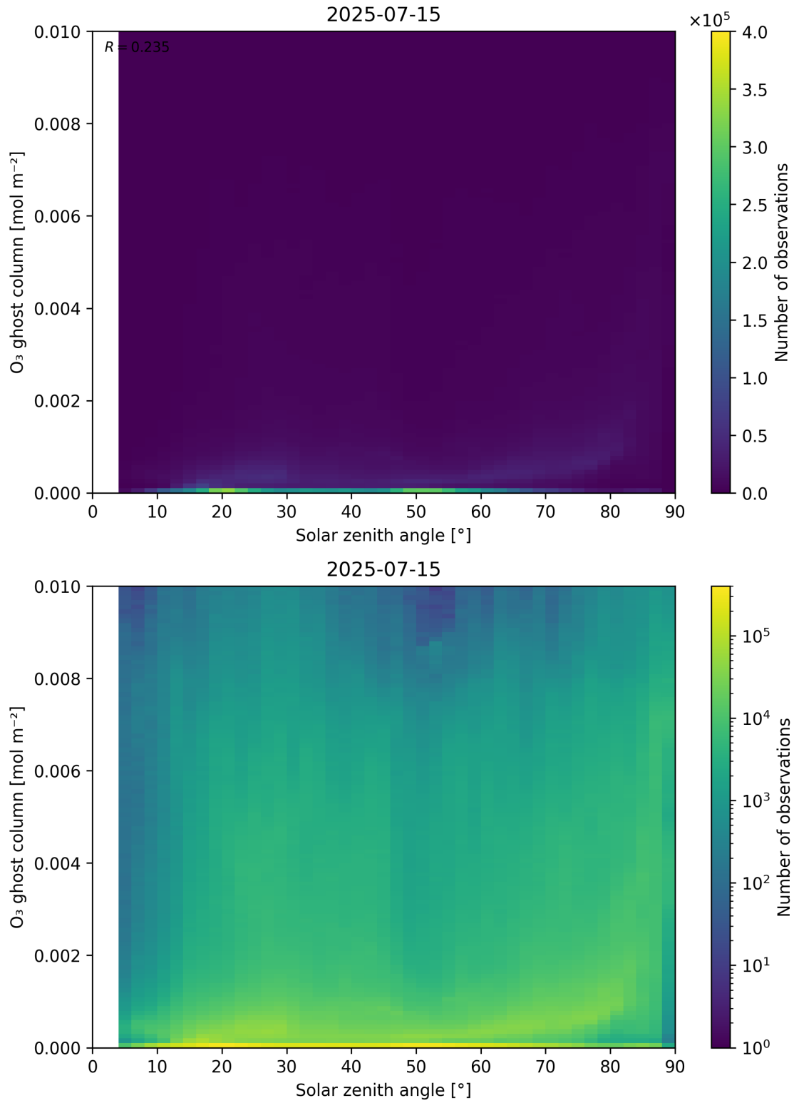
Figure 46: Scatter density plot of “Solar zenith angle” against “O 3 ghost column” for 2025-07-14 to 2025-07-16.
