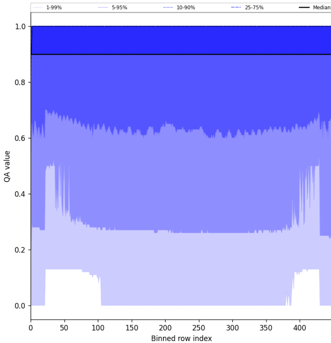
Figure 27: Along track statistics of “QA value” for 2025-07-14 to 2025-07-16
