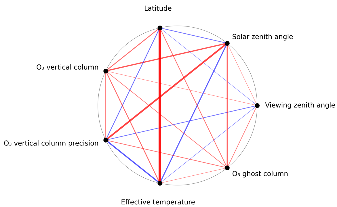
Figure 1: Map of correlation graph for 2025-07-14 to 2025-07-16.
