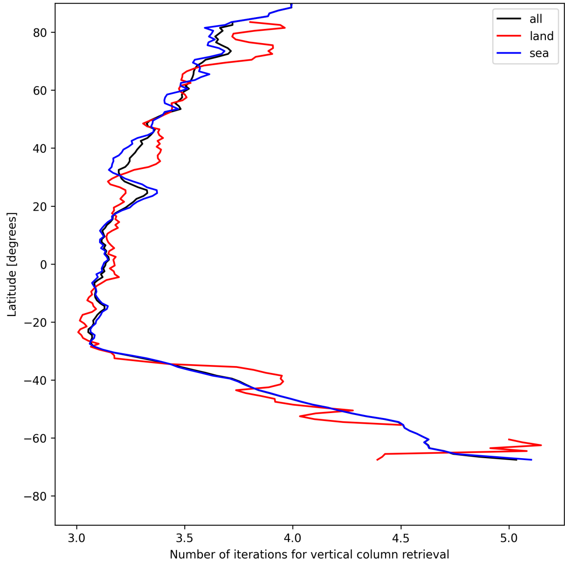
Figure 19: Zonal average of “Number of iterations for vertical column retrieval” for 2025-07-14 to 2025-07-16.
