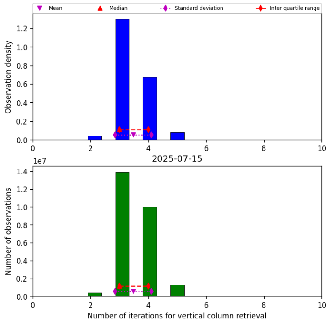
Figure 26: Histogram of “Number of iterations for vertical column retrieval” for 2025-07-14 to 2025-07-16
