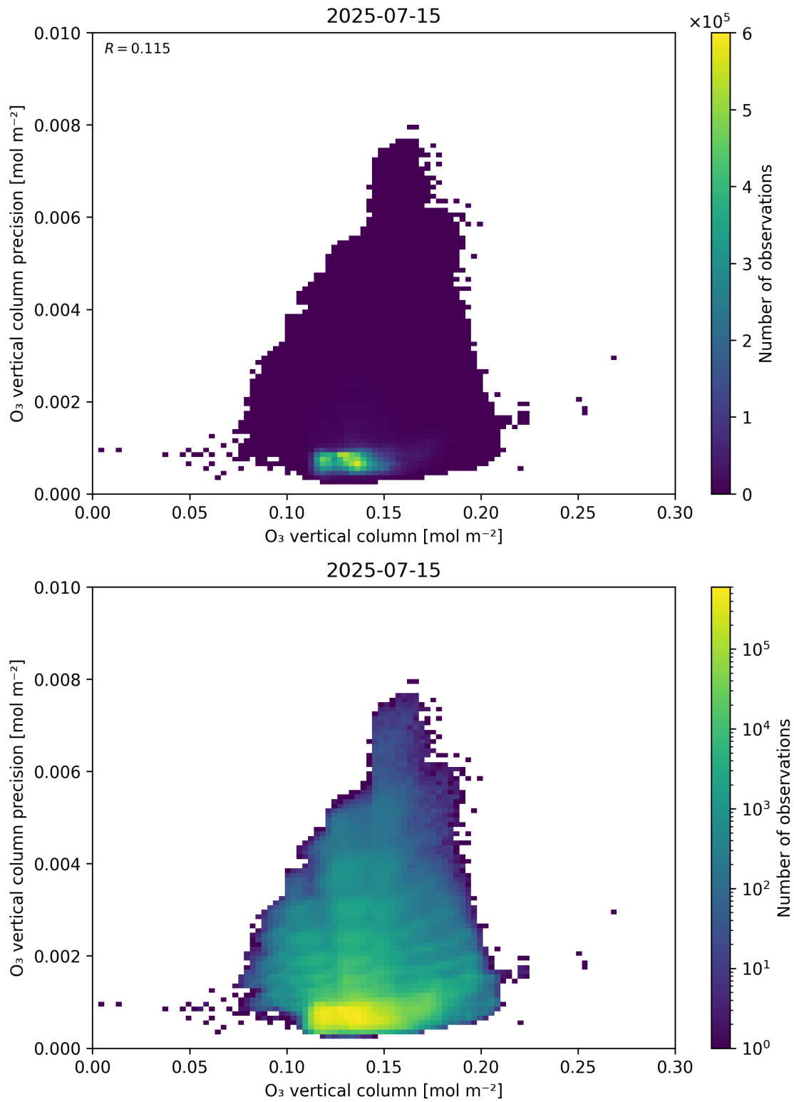
Figure 41: Scatter density plot of “O 3 vertical column” against “O 3 vertical column precision” for 2025-07-14 to 2025-07-16.
