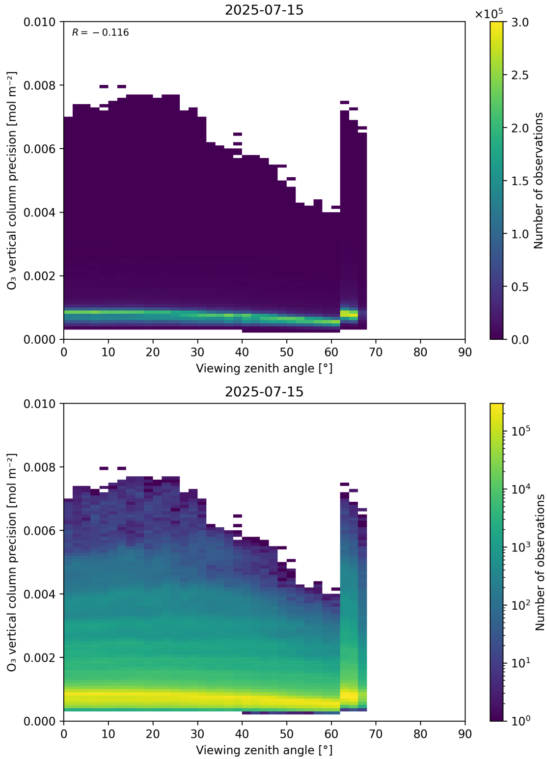
Figure 53: Scatter density plot of “Viewing zenith angle” against “O 3 vertical column precision” for 2025-07-14 to 2025-07-16.
