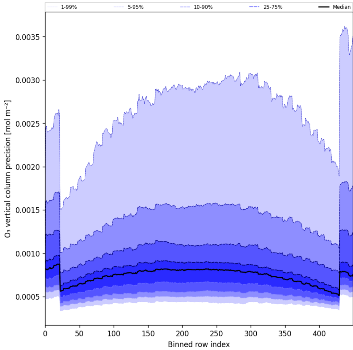
Figure 29: Along track statistics of “O 3 vertical column precision” for 2025-07-14 to 2025-07-16
