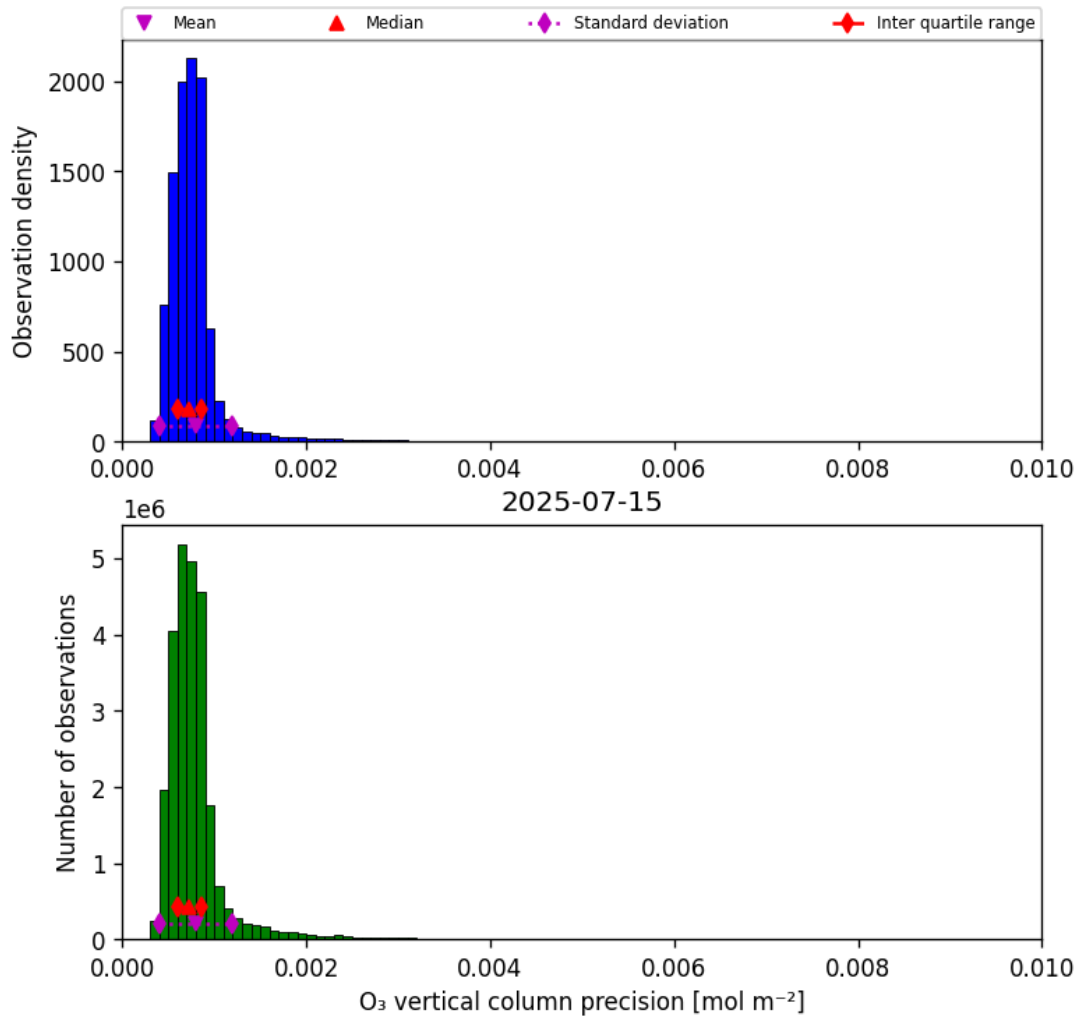
Figure 22: Histogram of “O 3 vertical column precision” for 2025-07-14 to 2025-07-16
