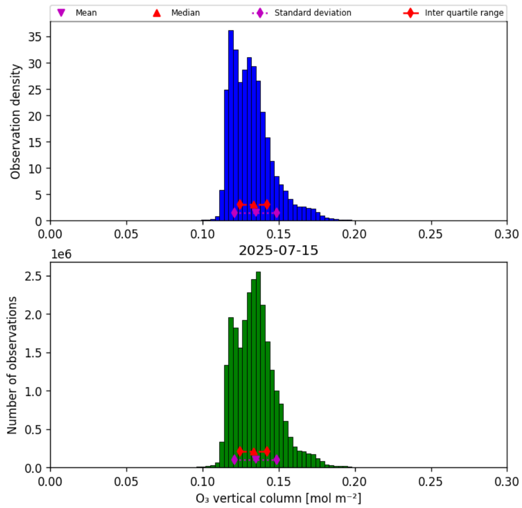
Figure 21: Histogram of “O 3 vertical column” for 2025-07-14 to 2025-07-16
