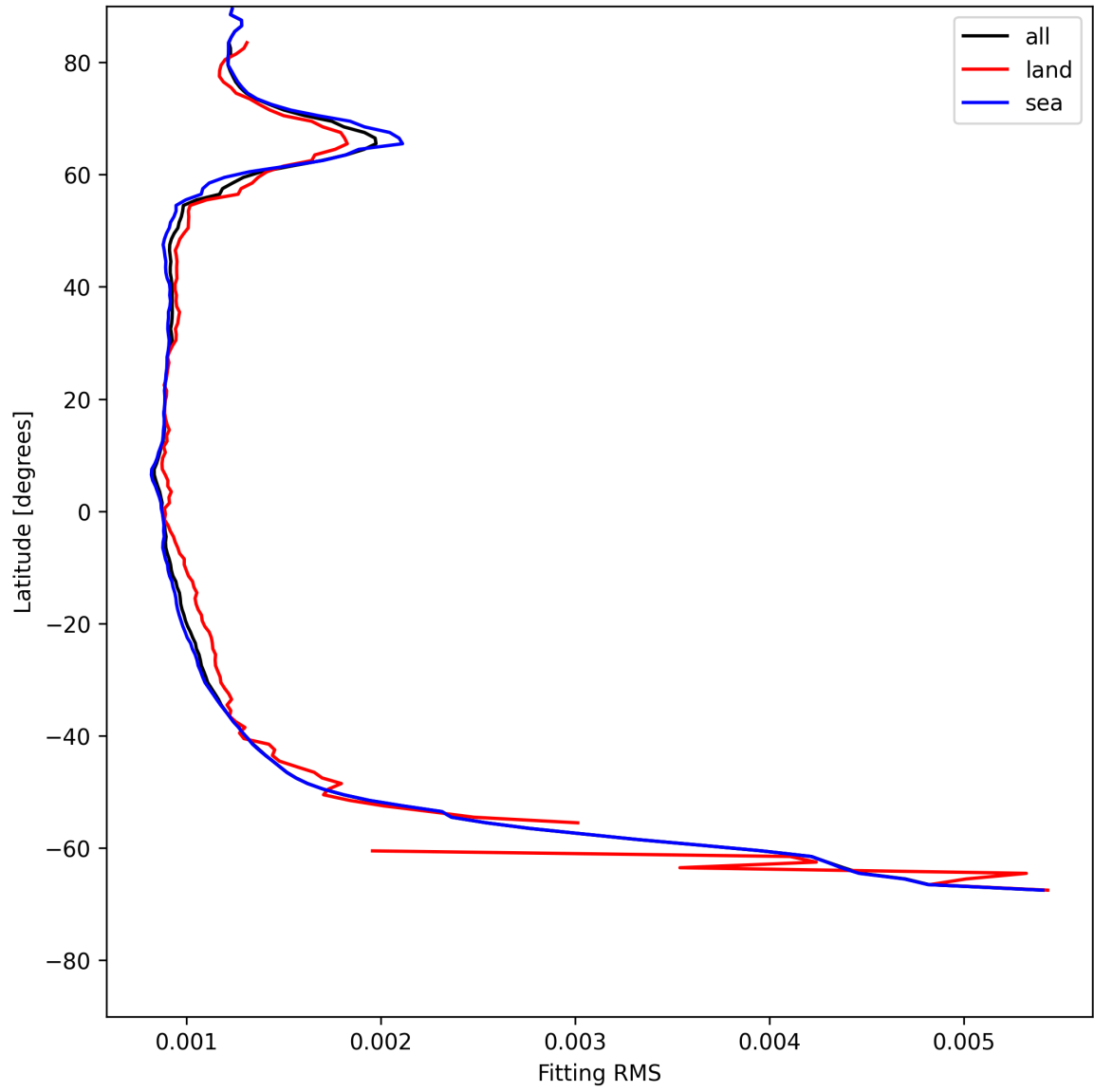
Figure 16: Zonal average of “Fitting RMS” for 2025-07-14 to 2025-07-16.
