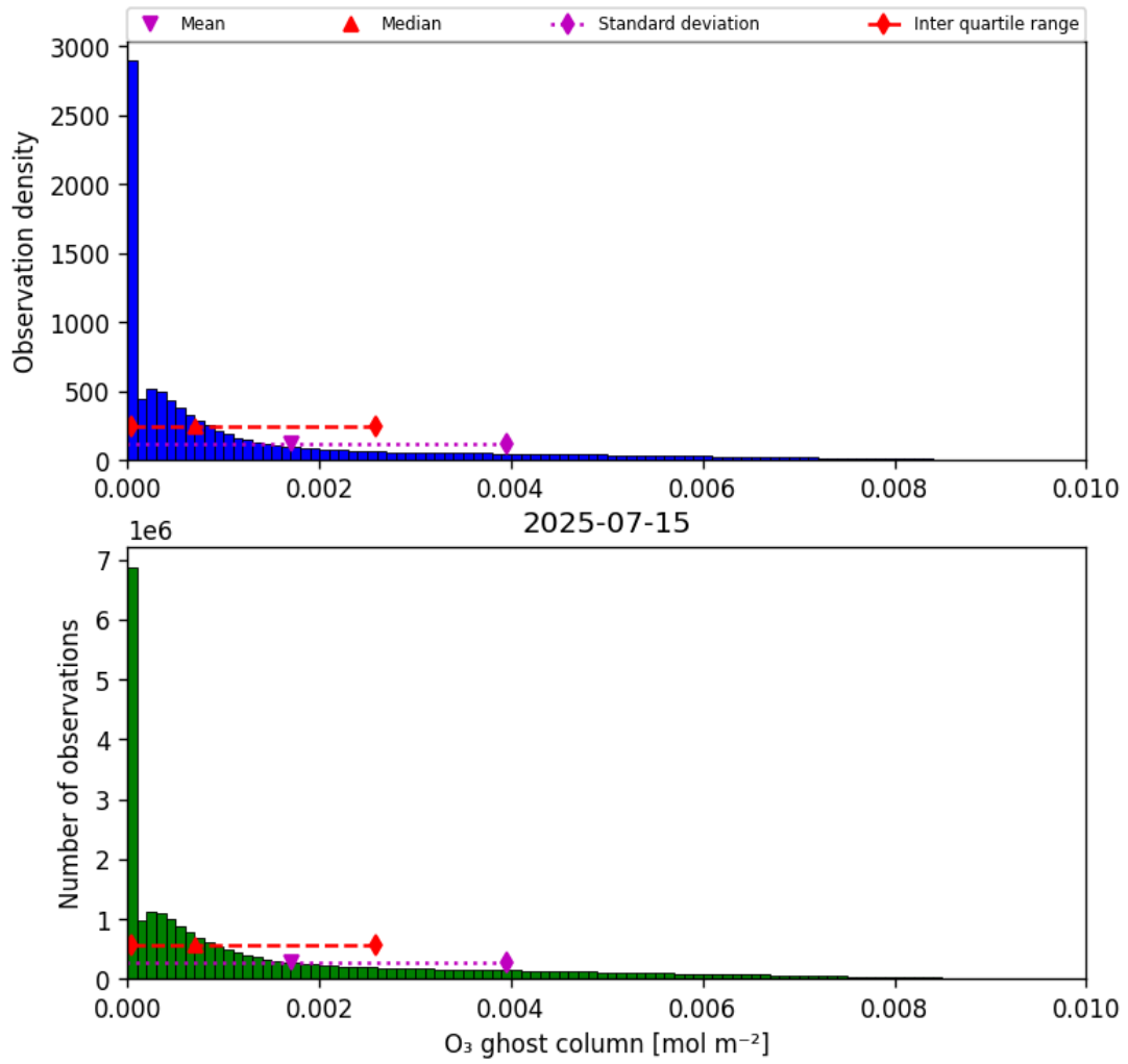
Figure 25: Histogram of “O 3 ghost column” for 2025-07-14 to 2025-07-16
