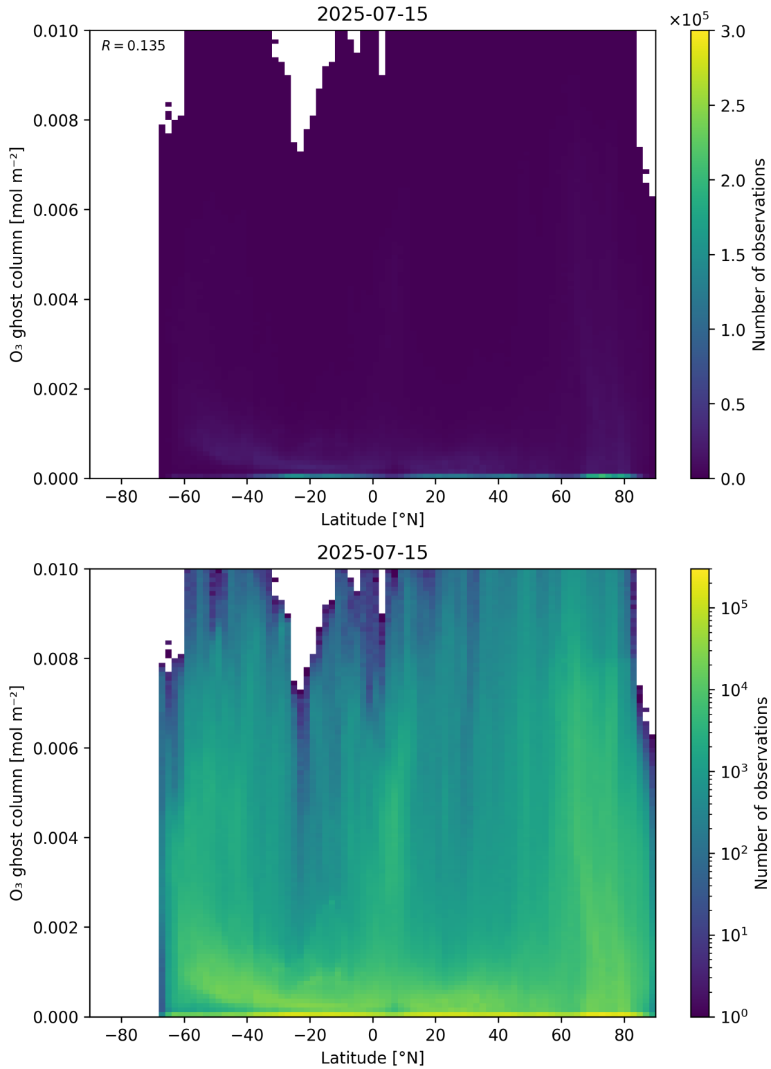
Figure 35: Scatter density plot of “Latitude” against “O 3 ghost column” for 2025-07-14 to 2025-07-16.
