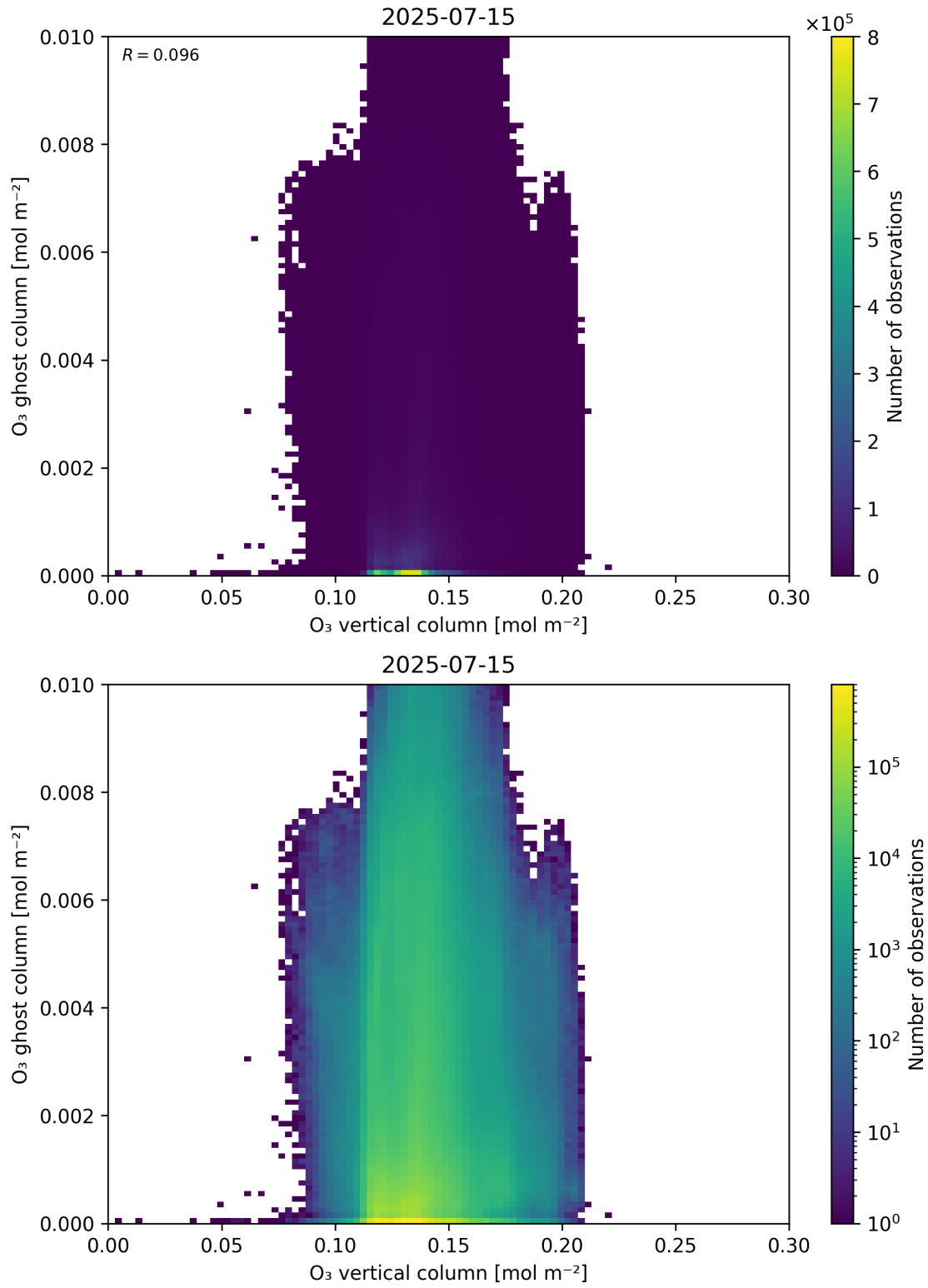
Figure 40: Scatter density plot of “O 3 vertical column” against “O 3 ghost column” for 2025-07-14 to 2025-07-16.
