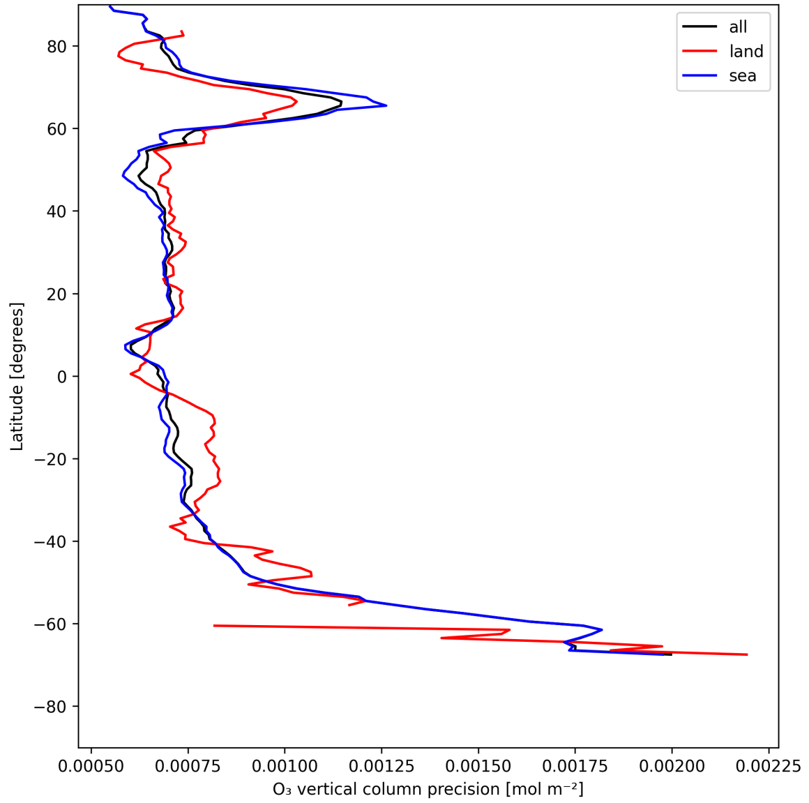
Figure 15: Zonal average of "O 3 vertical column precision" for 2025-07-14 to 2025-07-16.
