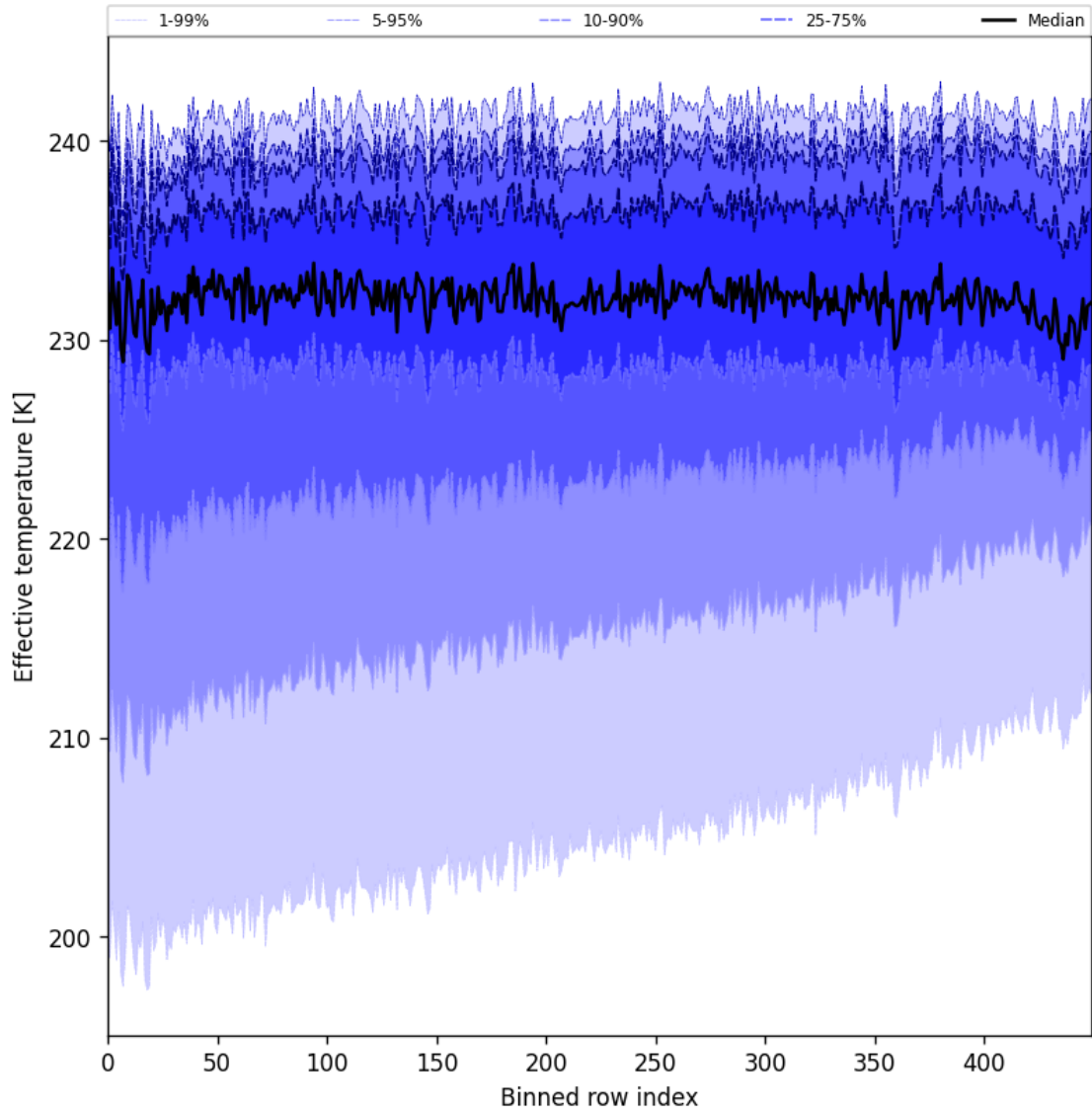
Figure 31: Along track statistics of “Effective temperature” for 2025-07-14 to 2025-07-16
