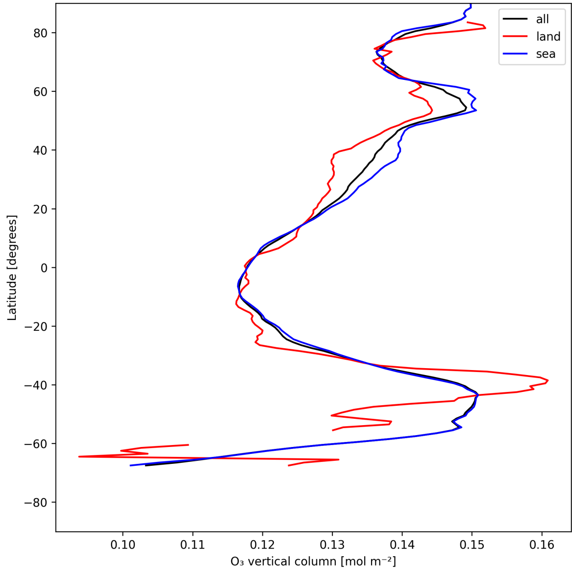
Figure 14: Zonal average of “O 3 vertical column” for 2025-07-14 to 2025-07-16.
