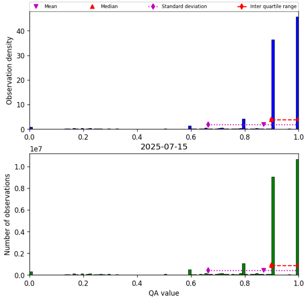
Figure 20: Histogram of “QA value” for 2025-07-14 to 2025-07-16
