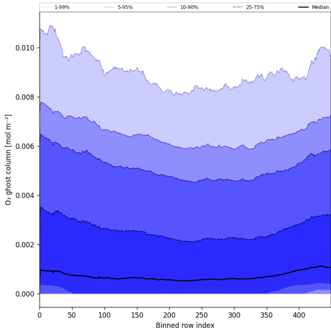
Figure 32: Along track statistics of “O 3 ghost column” for 2025-07-14 to 2025-07-16
