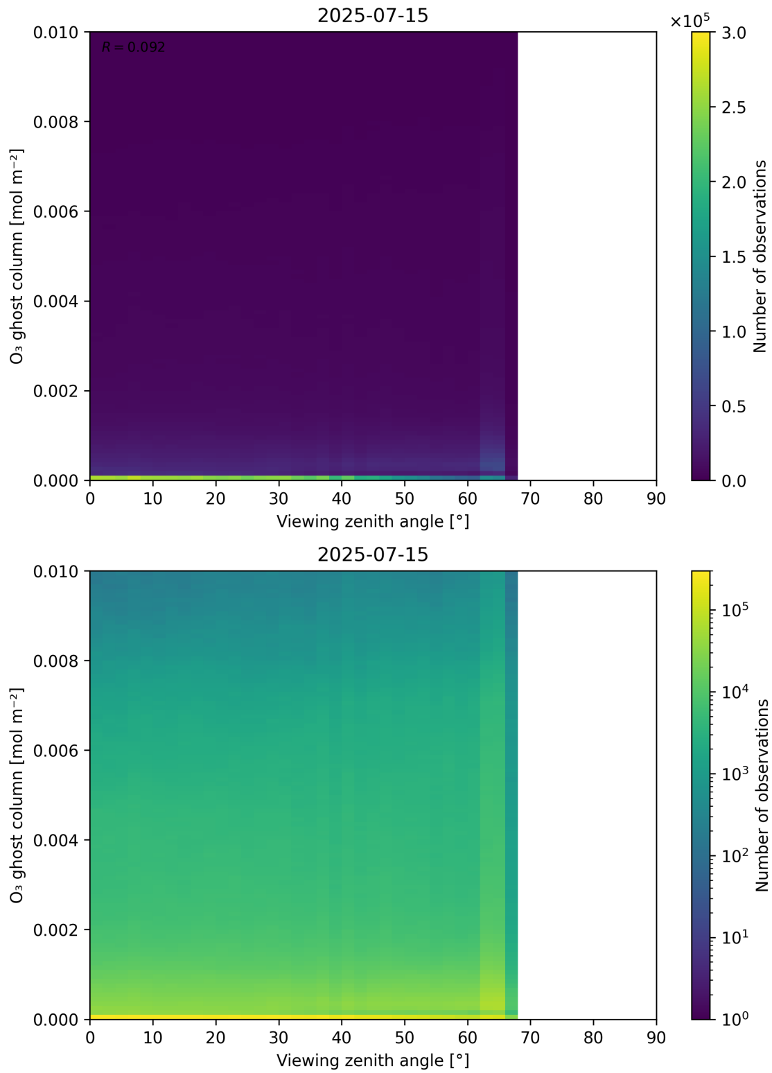
Figure 51: Scatter density plot of “Viewing zenith angle” against “O 3 ghost column” for 2025-07-14 to 2025-07-16.
