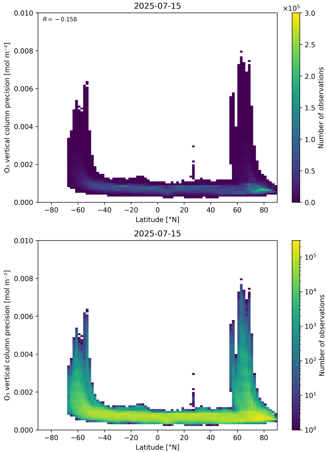
Figure 37: Scatter density plot of “Latitude” against “O 3 vertical column precision” for 2025-07-14 to 2025-07-16.
