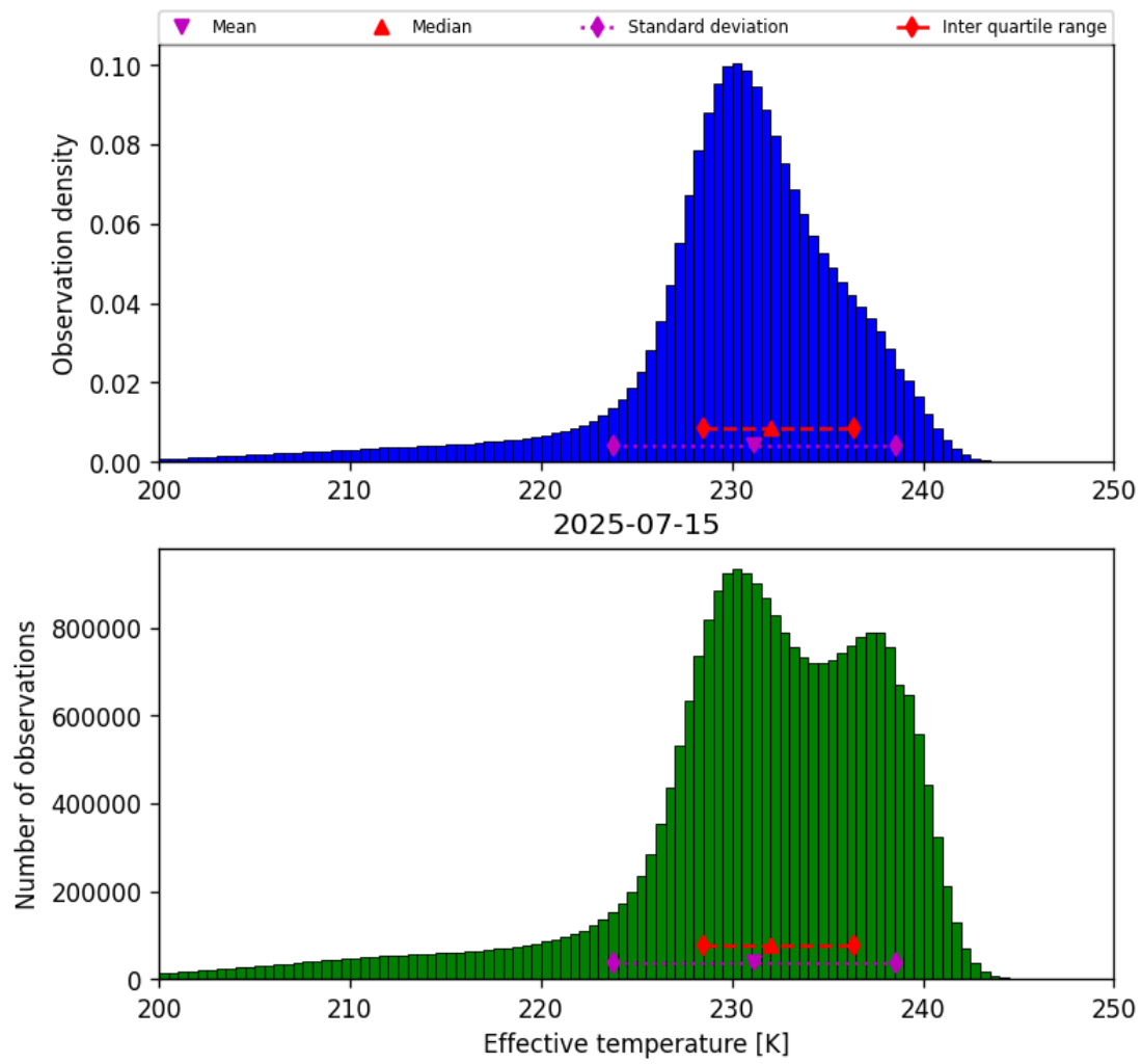
Figure 24: Histogram of “Effective temperature” for 2025-07-14 to 2025-07-16
