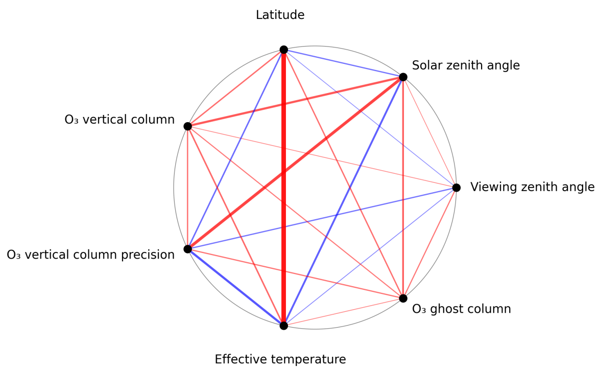
Figure 1: Map of correlation graph for 2025-07-15 to 2025-07-17.
