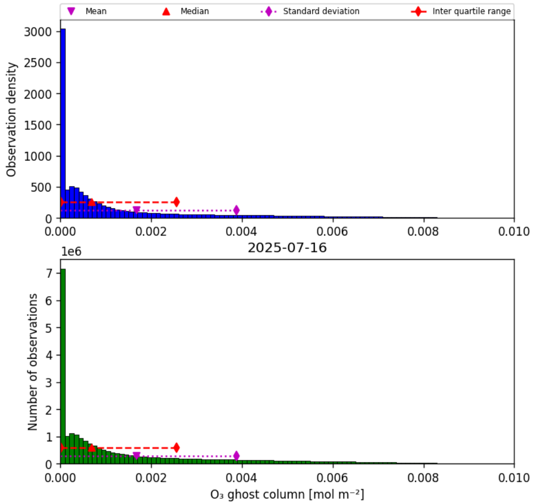
Figure 25: Histogram of “O 3 ghost column” for 2025-07-15 to 2025-07-17
