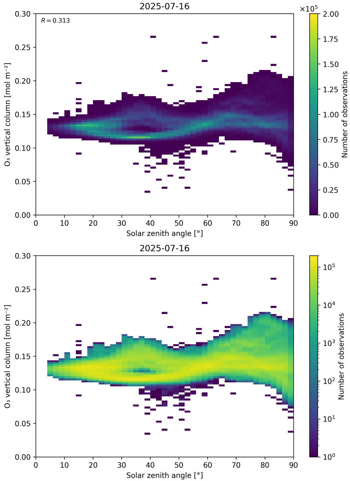
Figure 47: Scatter density plot of “Solar zenith angle” against “O 3 vertical column” for 2025-07-15 to 2025-07-17.
