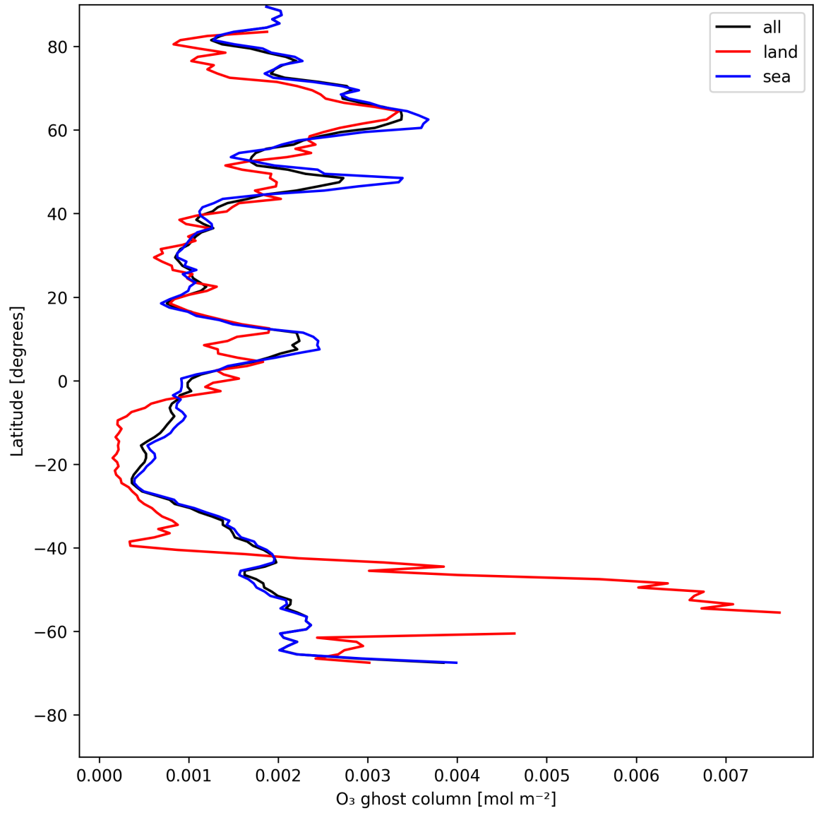
Figure 18: Zonal average of “O 3 ghost column” for 2025-07-15 to 2025-07-17.
