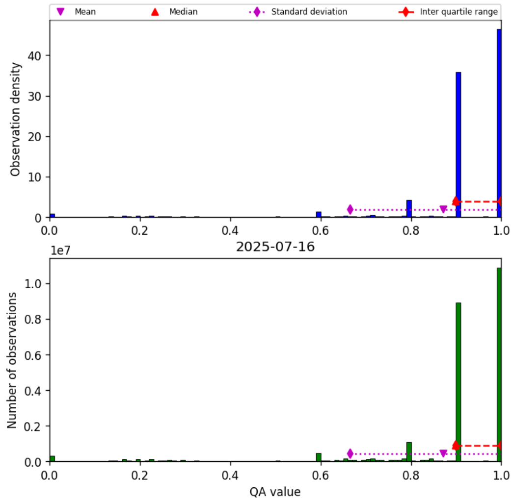
Figure 20: Histogram of “QA value” for 2025-07-15 to 2025-07-17
