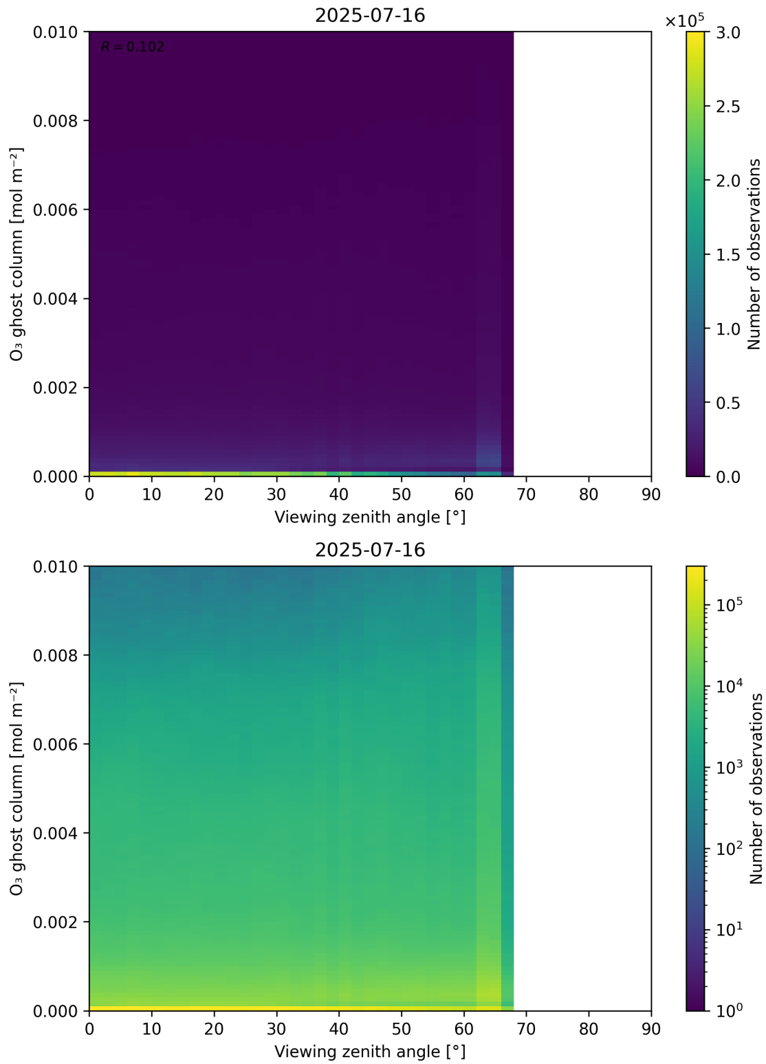
Figure 51: Scatter density plot of “Viewing zenith angle” against “O 3 ghost column” for 2025-07-15 to 2025-07-17.
