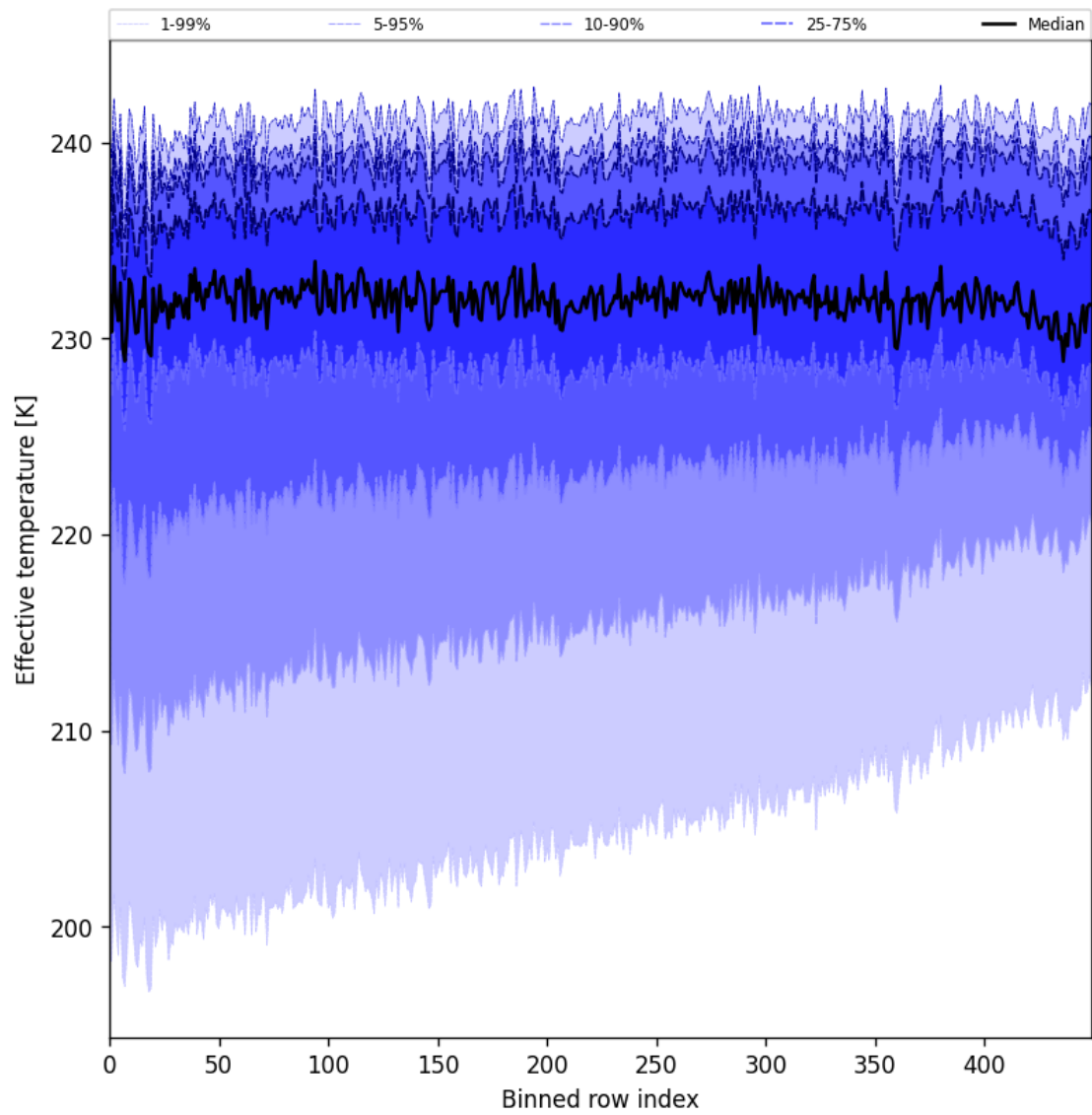
Figure 31: Along track statistics of “Effective temperature” for 2025-07-15 to 2025-07-17
