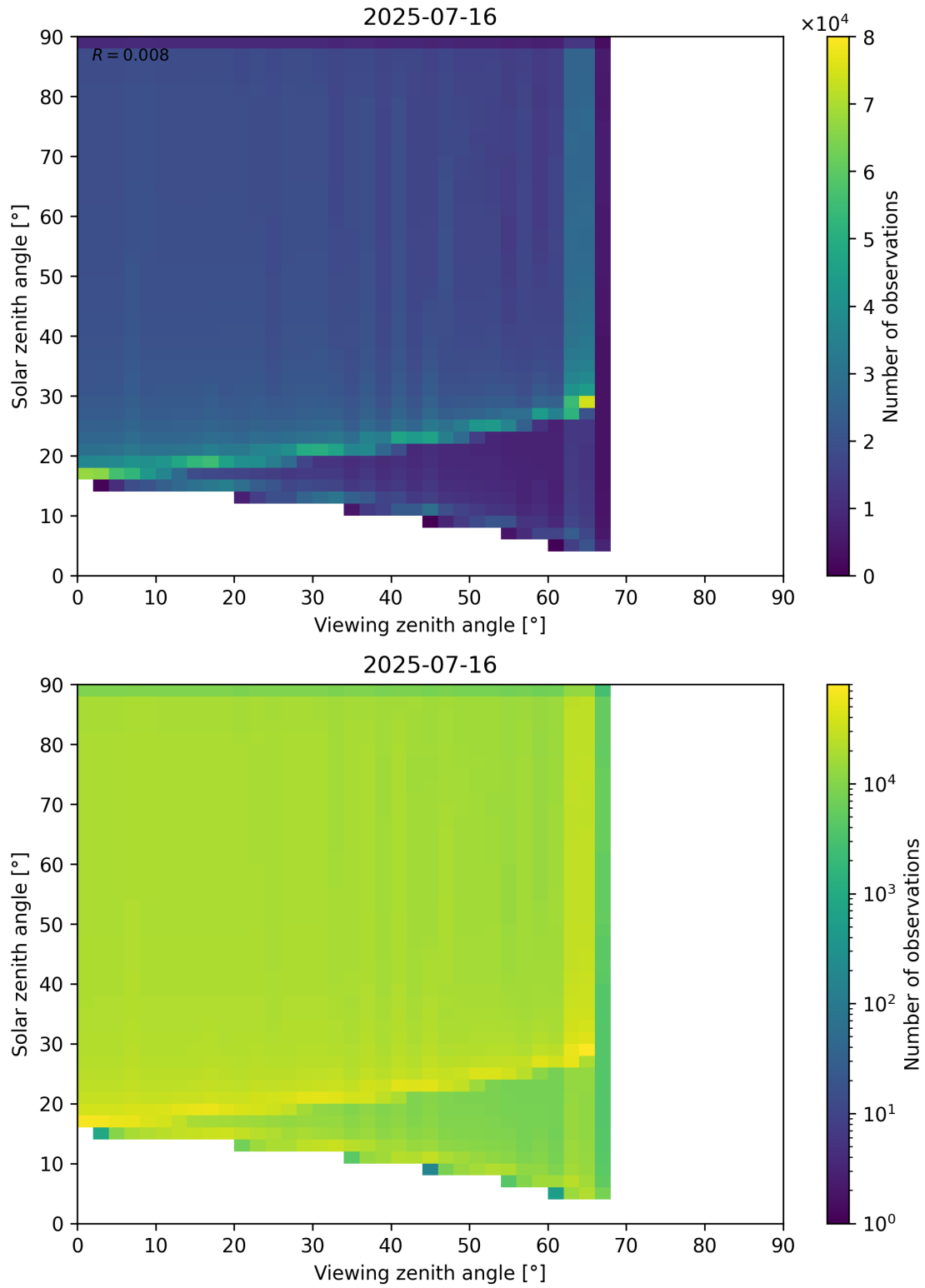
Figure 54: Scatter density plot of “Viewing zenith angle” against “Solar zenith angle” for 2025-07-15 to 2025-07-17.
