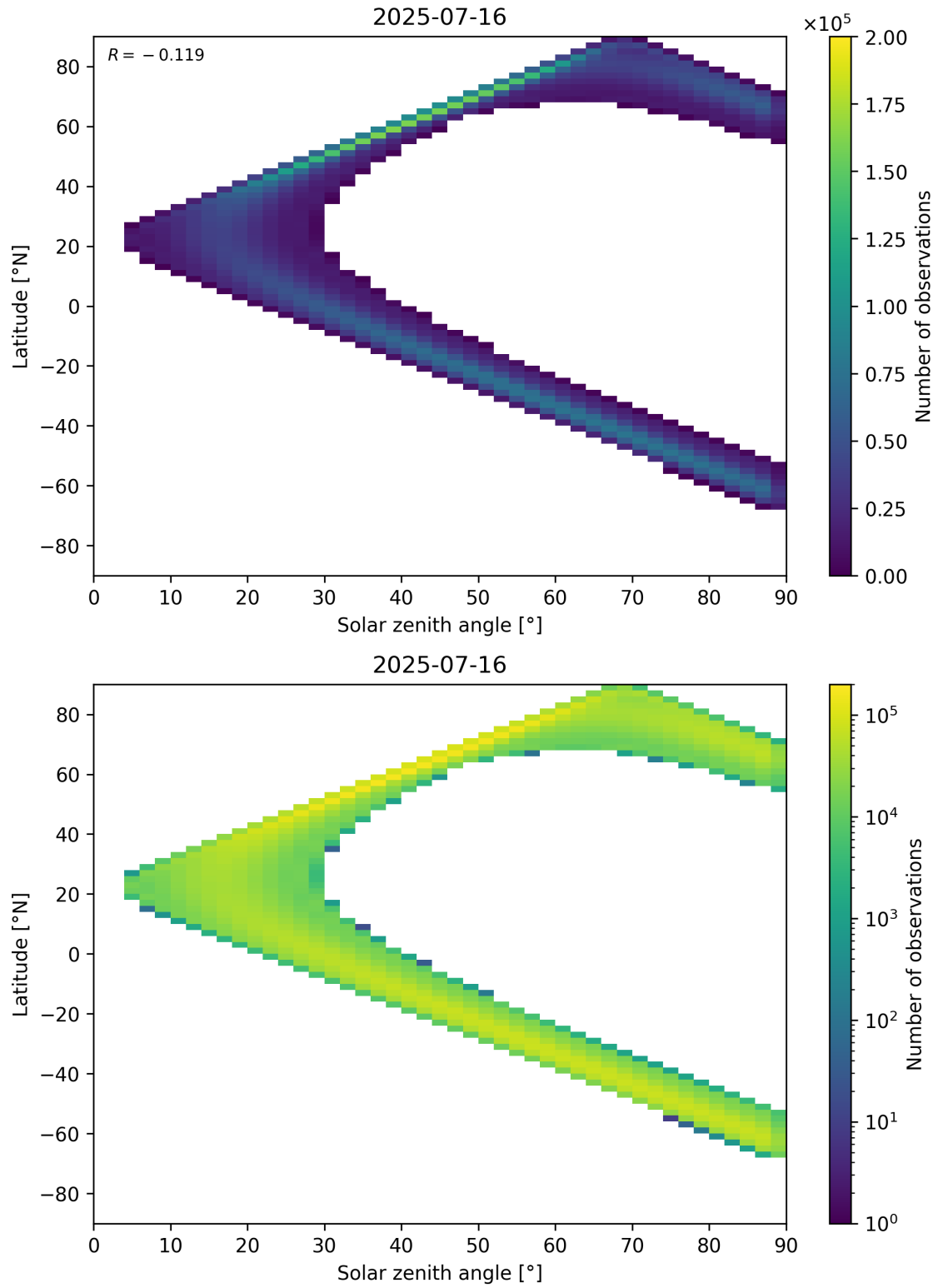
Figure 44: Scatter density plot of “Solar zenith angle” against “Latitude” for 2025-07-15 to 2025-07-17.
