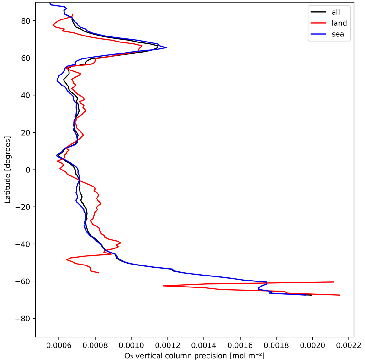
Figure 15: Zonal average of "O 3 vertical column precision" for 2025-07-15 to 2025-07-17.
