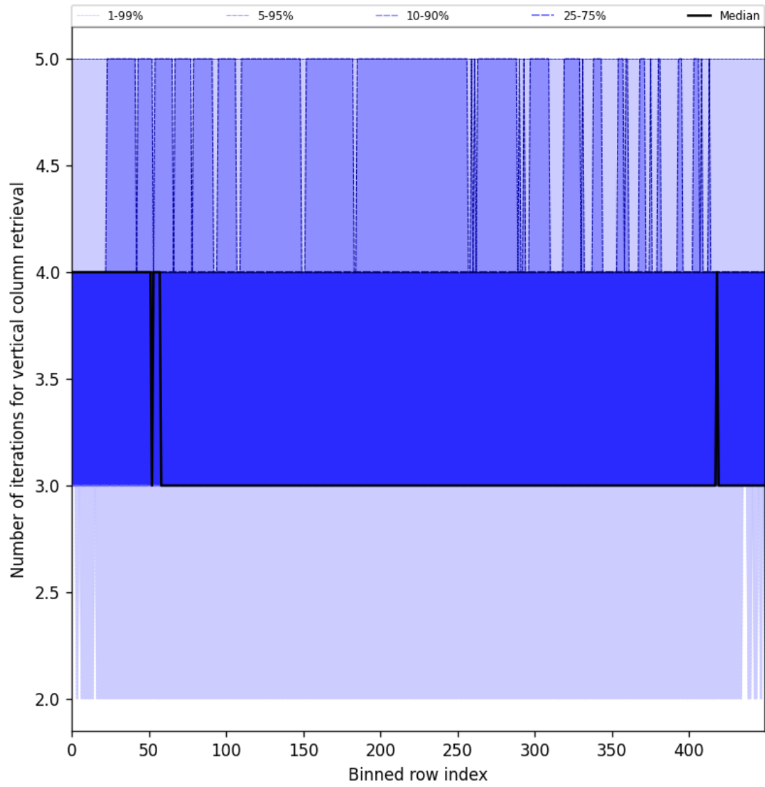
Figure 33: Along track statistics of “Number of iterations for vertical column retrieval” for 2025-07-15 to 2025-07-17
