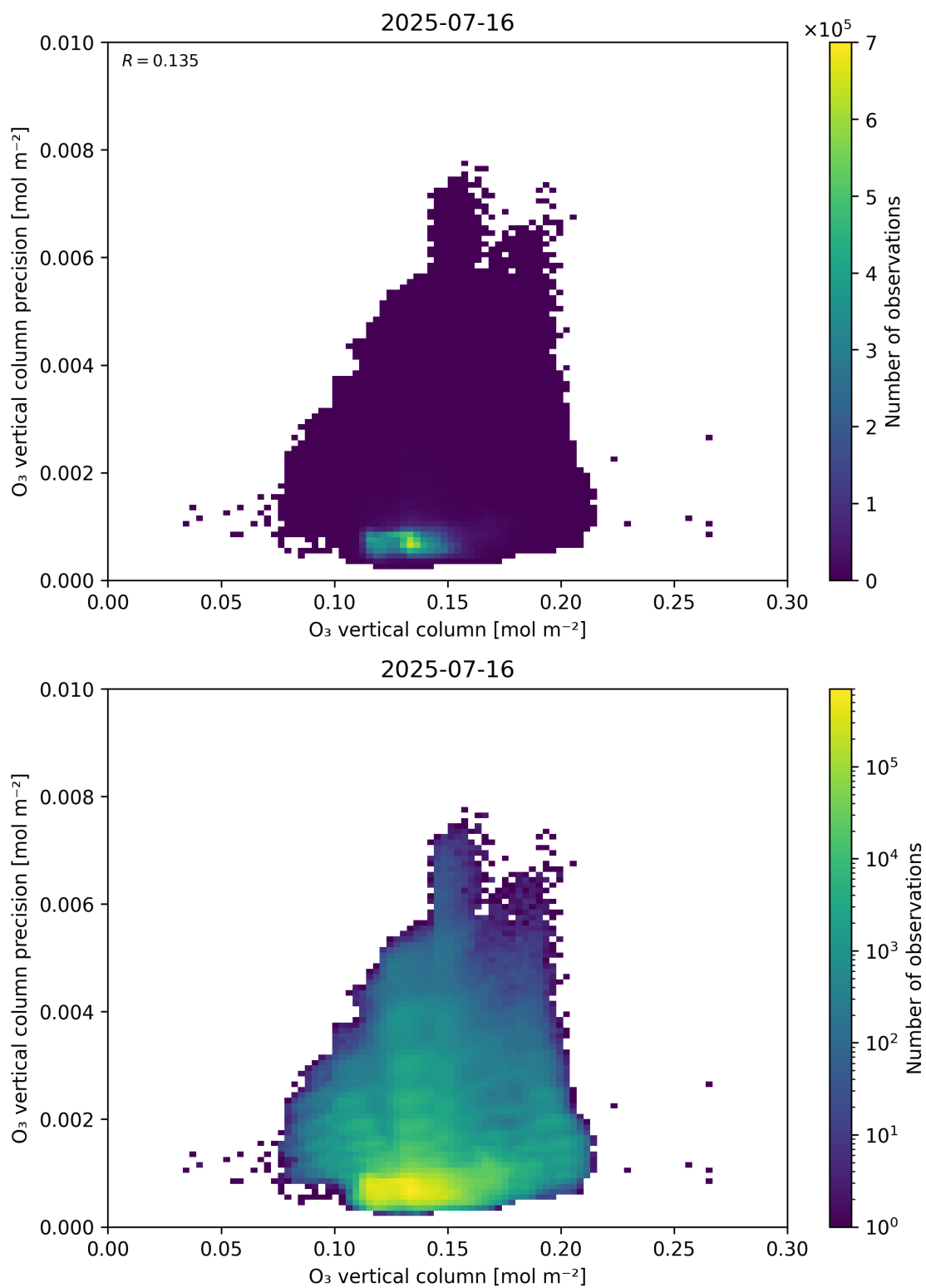
Figure 41: Scatter density plot of “O 3 vertical column” against “O 3 vertical column precision” for 2025-07-15 to 2025-07-17.
