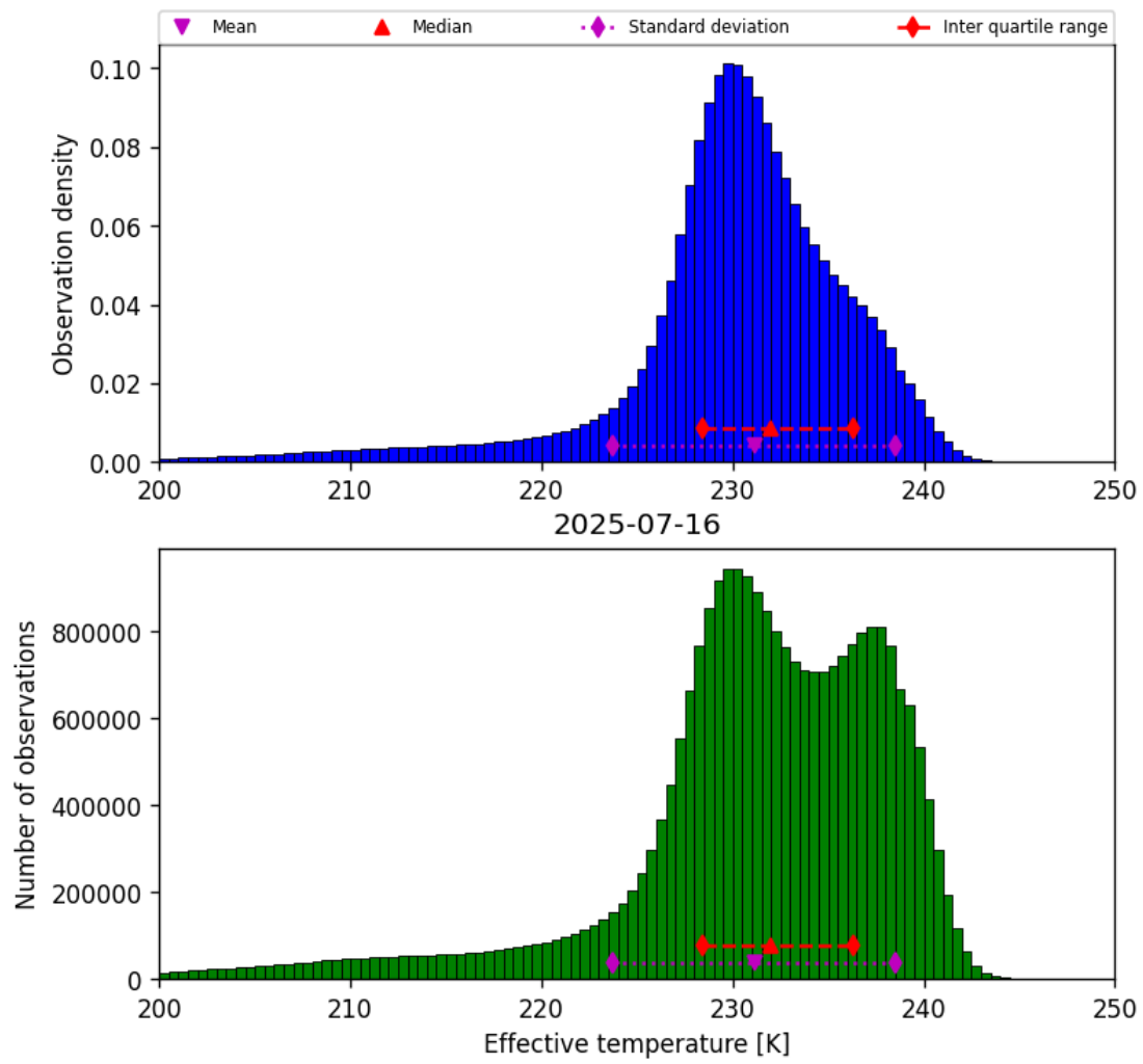
Figure 24: Histogram of “Effective temperature” for 2025-07-15 to 2025-07-17
