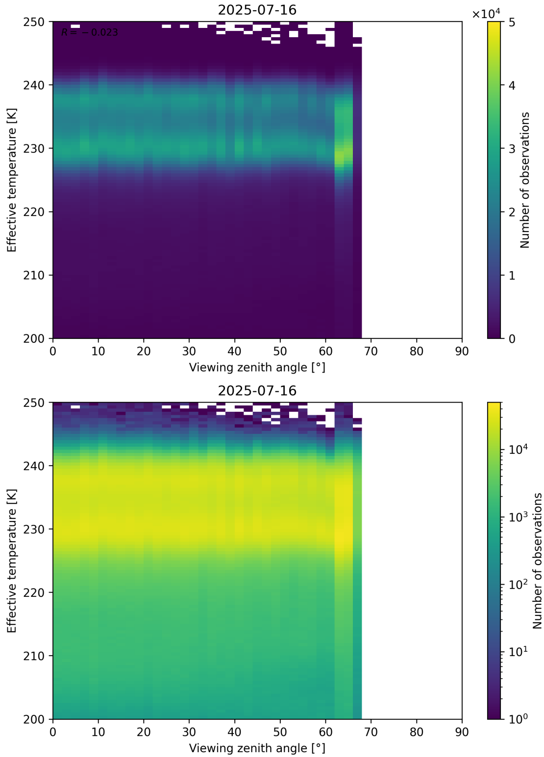
Figure 50: Scatter density plot of “Viewing zenith angle” against “Effective temperature” for 2025-07-15 to 2025-07-17.
