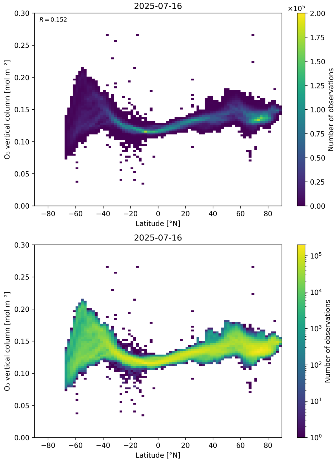
Figure 36: Scatter density plot of “Latitude” against “O 3 vertical column” for 2025-07-15 to 2025-07-17.
