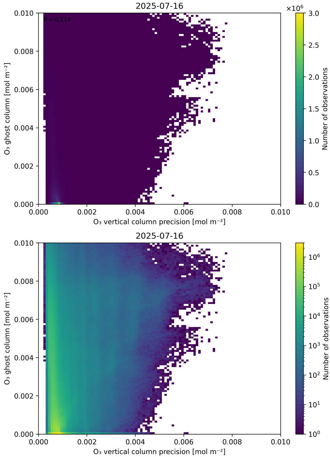
Figure 43: Scatter density plot of “ \text{O}_3 vertical column precision” against “ \text{O}_3 ghost column” for 2025-07-15 to 2025-07-17.
