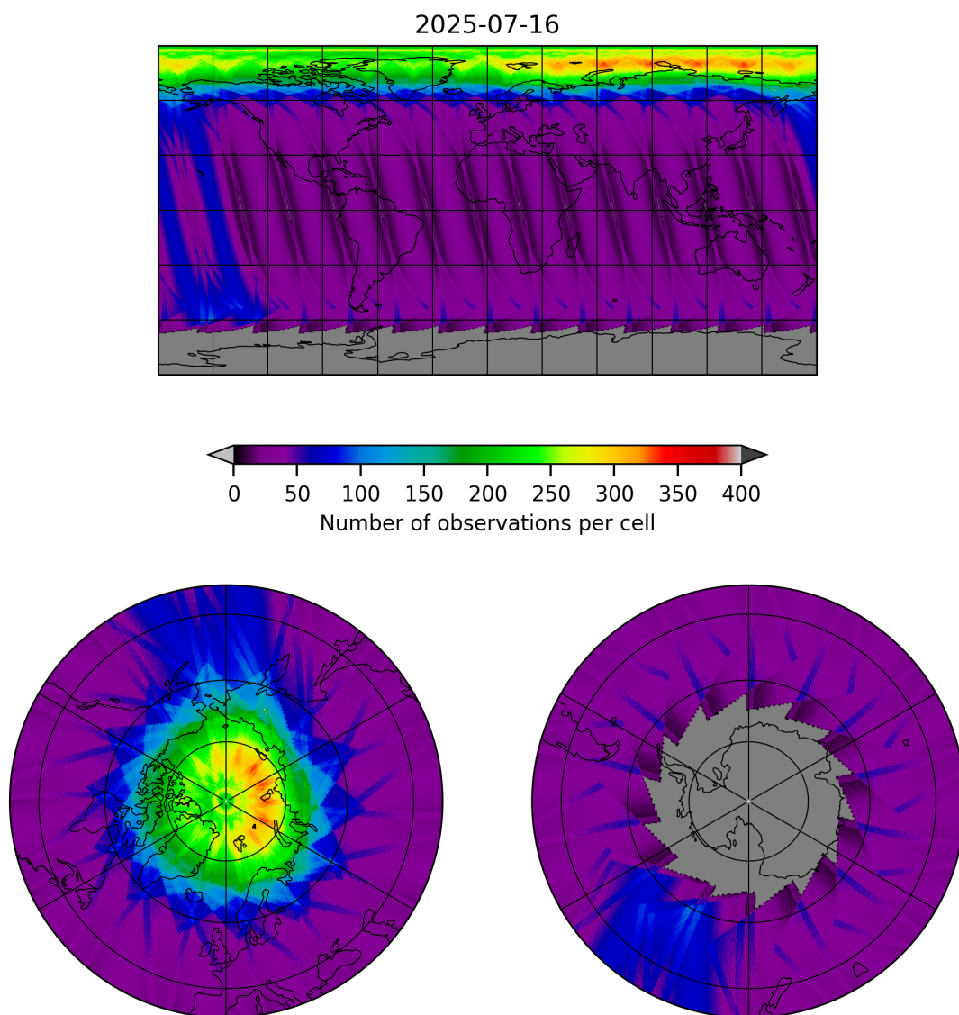
Figure 12: Map of the number of observations for 2025-07-15 to 2025-07-17
