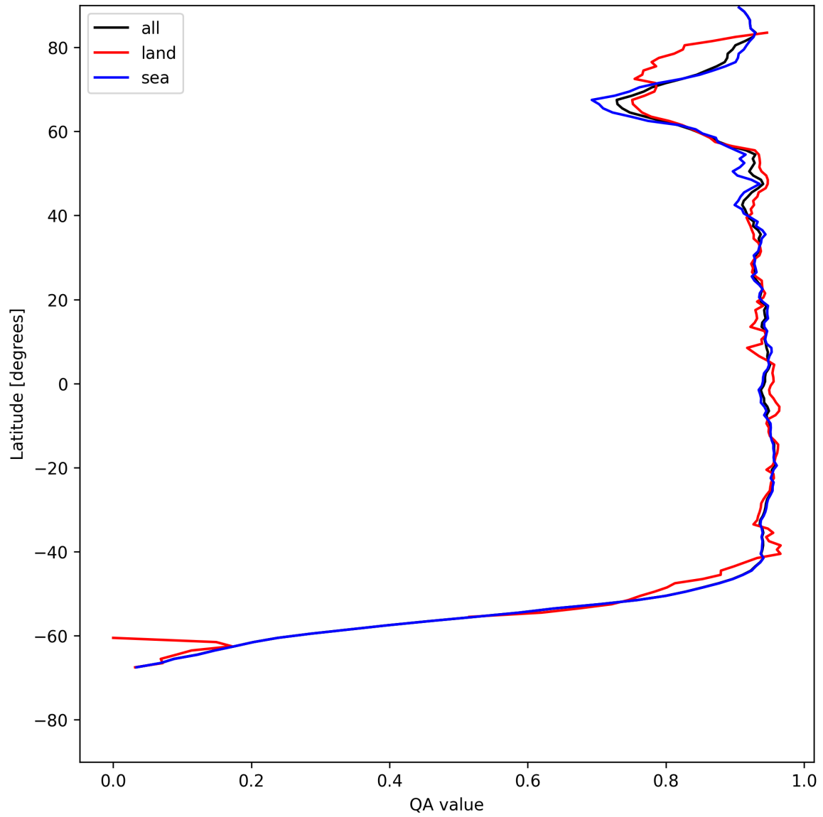
Figure 13: Zonal average of “QA value” for 2025-07-15 to 2025-07-17.
