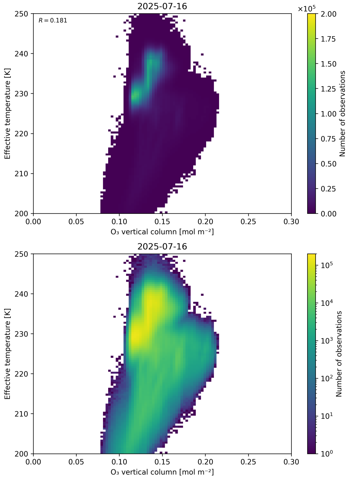
Figure 39: Scatter density plot of “O 3 vertical column” against “Effective temperature” for 2025-07-15 to 2025-07-17.
