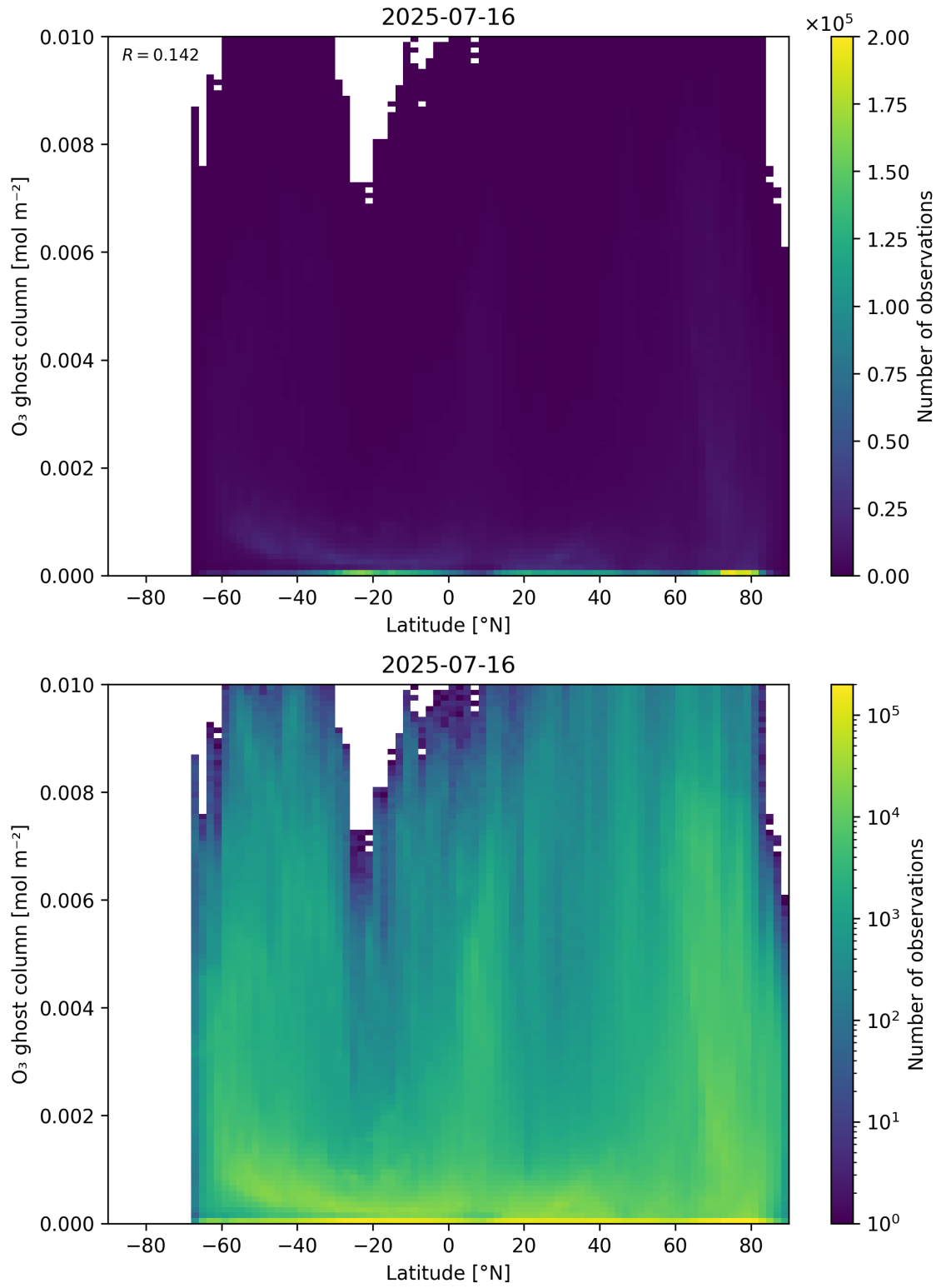
Figure 35: Scatter density plot of “Latitude” against “O 3 ghost column” for 2025-07-15 to 2025-07-17.
