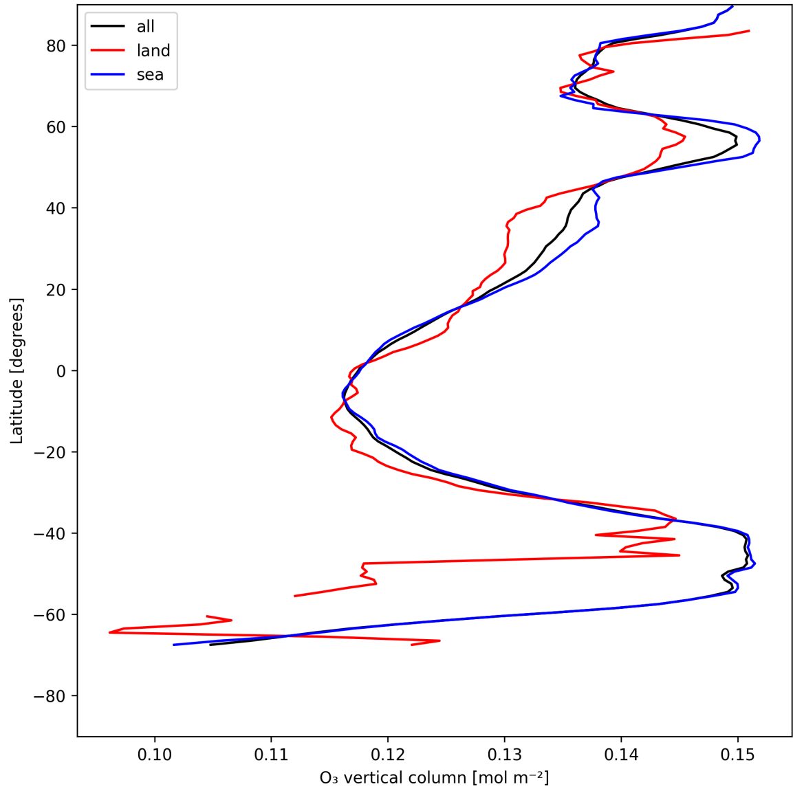
Figure 14: Zonal average of “O 3 vertical column” for 2025-07-15 to 2025-07-17.
