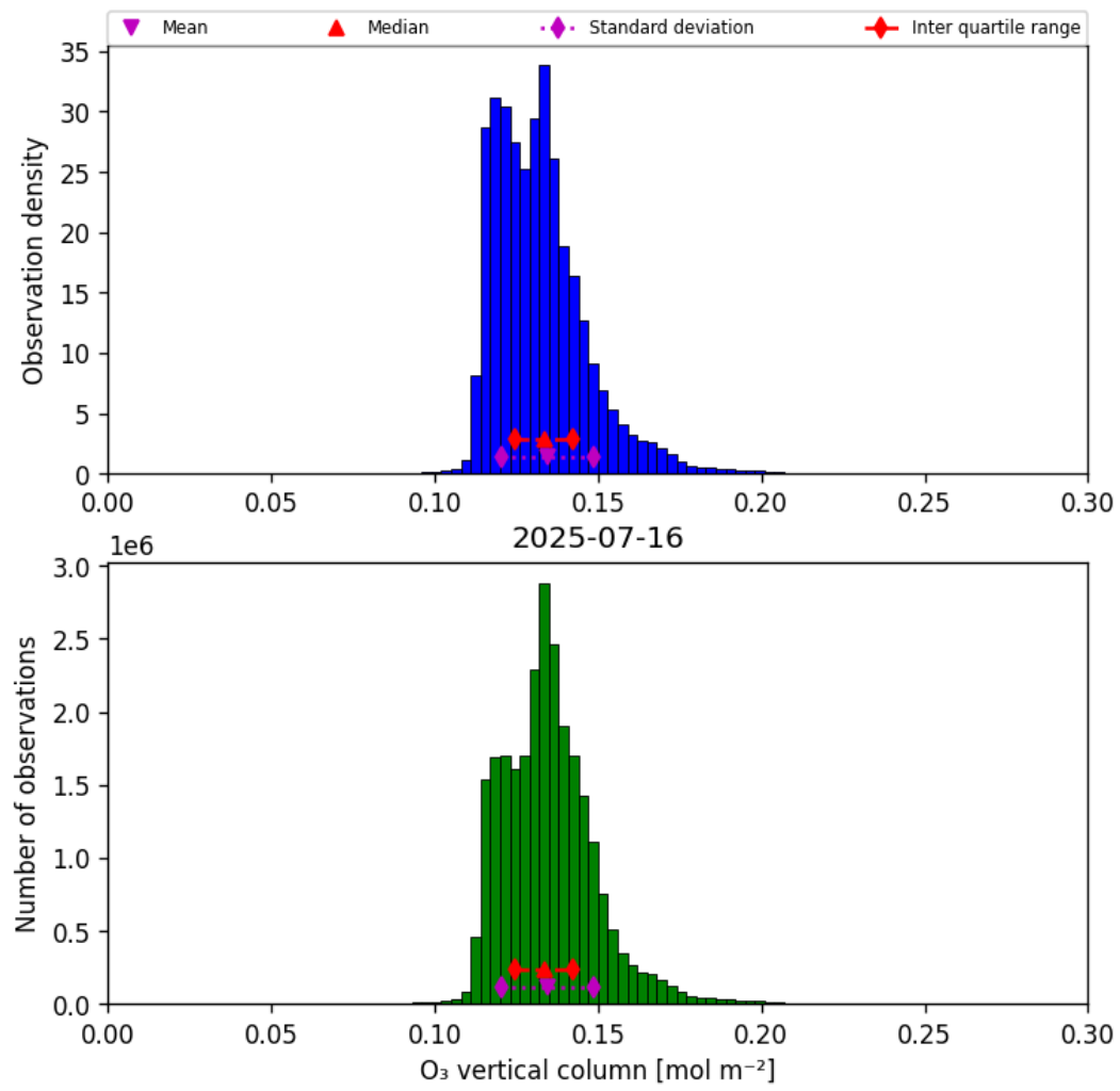
Figure 21: Histogram of “O 3 vertical column” for 2025-07-15 to 2025-07-17
