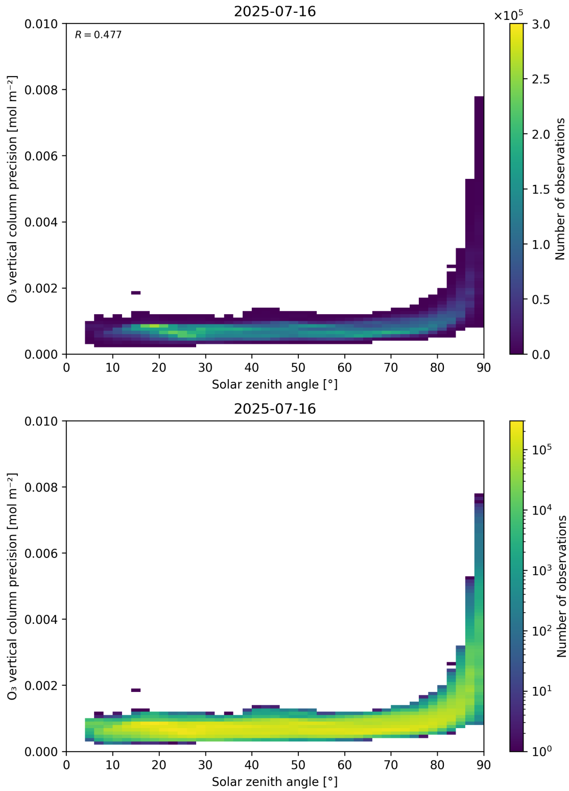
Figure 48: Scatter density plot of “Solar zenith angle” against “O 3 vertical column precision” for 2025-07-15 to 2025-07-17.
