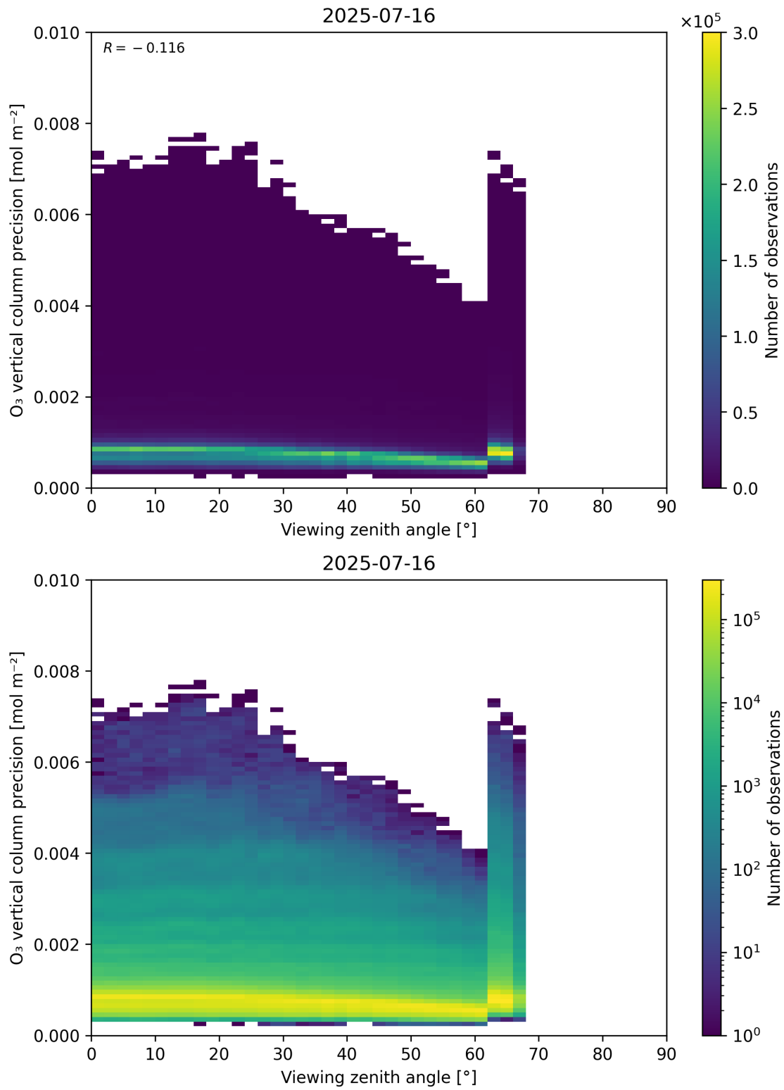
Figure 53: Scatter density plot of “Viewing zenith angle” against “O 3 vertical column precision” for 2025-07-15 to 2025-07-17.
