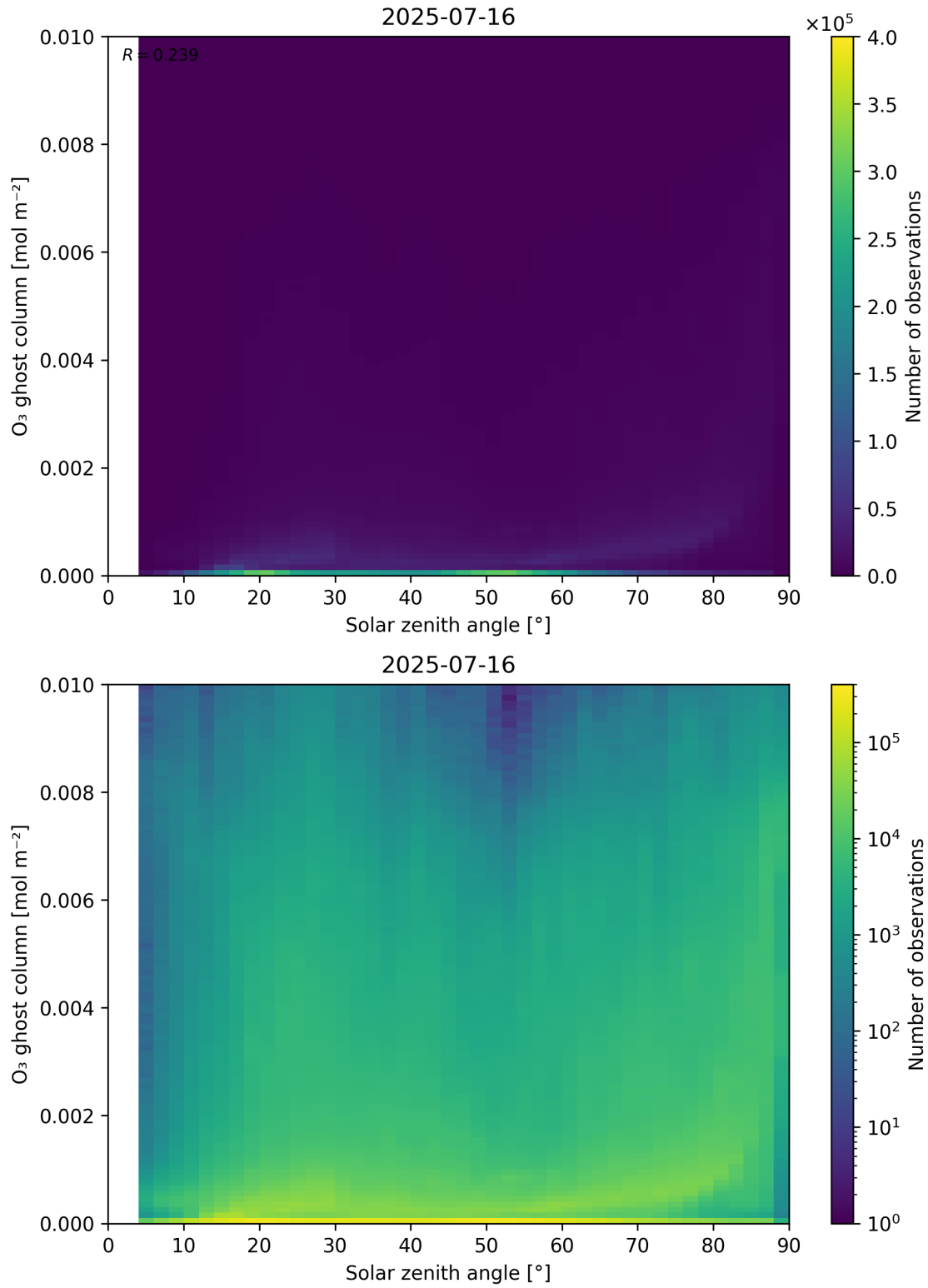
Figure 46: Scatter density plot of “Solar zenith angle” against “O 3 ghost column” for 2025-07-15 to 2025-07-17.
