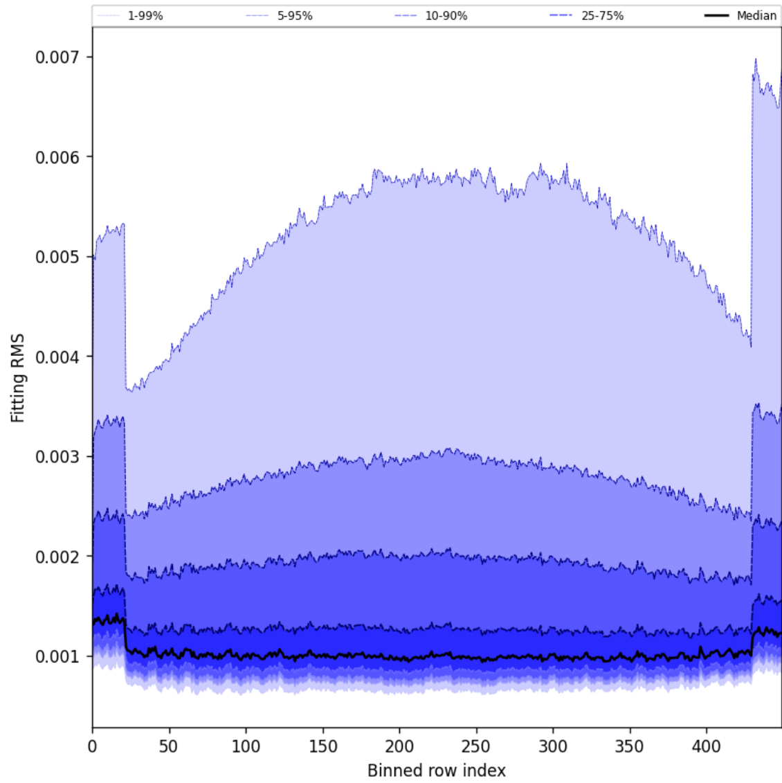
Figure 30: Along track statistics of “Fitting RMS” for 2025-07-15 to 2025-07-17
