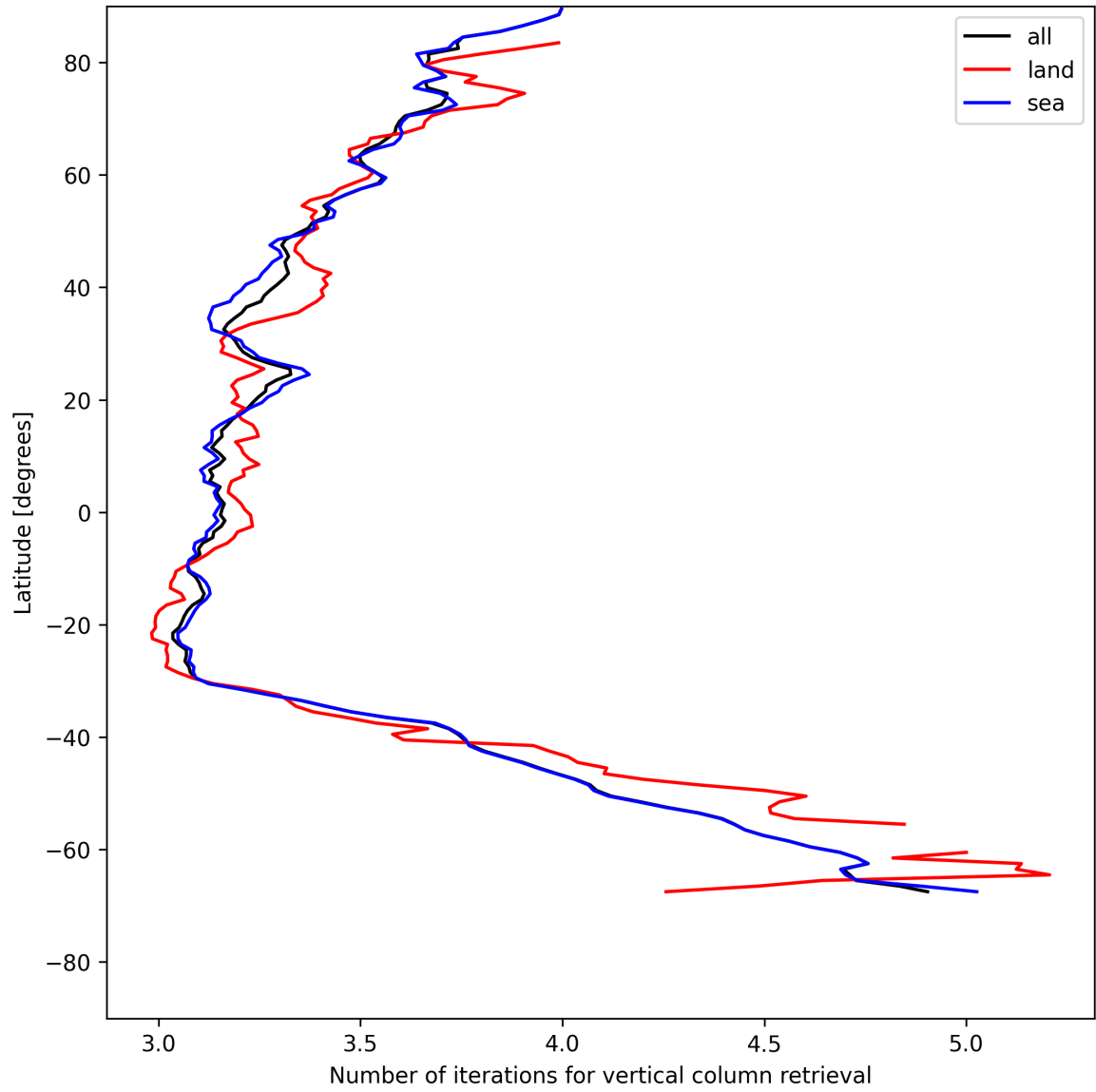
Figure 19: Zonal average of “Number of iterations for vertical column retrieval” for 2025-07-15 to 2025-07-17.
