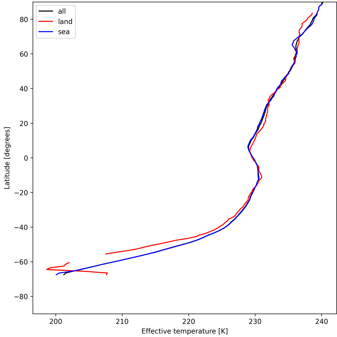
Figure 17: Zonal average of "Effective temperature" for 2025-07-15 to 2025-07-17.
