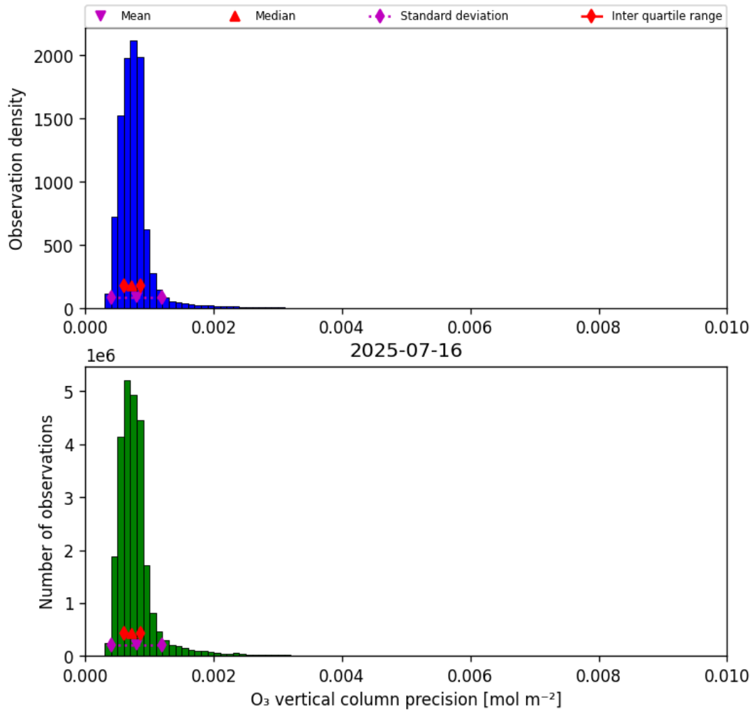
Figure 22: Histogram of “O 3 vertical column precision” for 2025-07-15 to 2025-07-17
