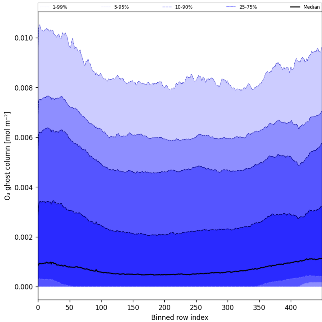
Figure 32: Along track statistics of “O 3 ghost column” for 2025-07-15 to 2025-07-17
