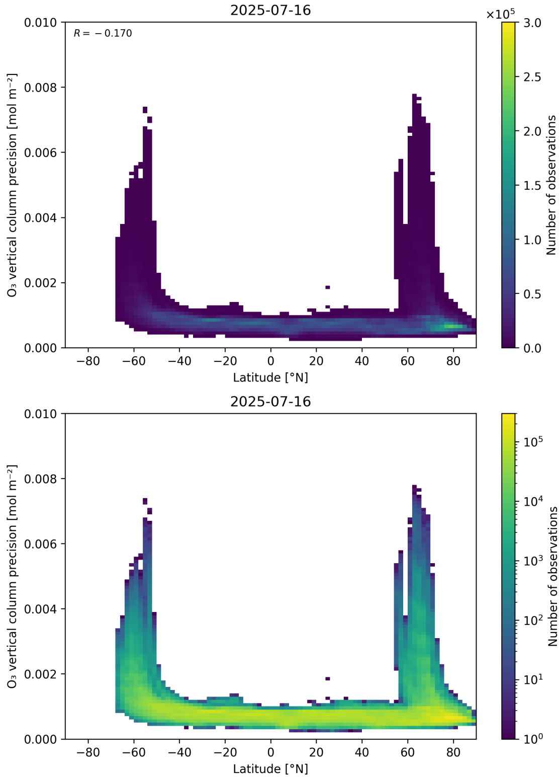
Figure 37: Scatter density plot of “Latitude” against “O 3 vertical column precision” for 2025-07-15 to 2025-07-17.
