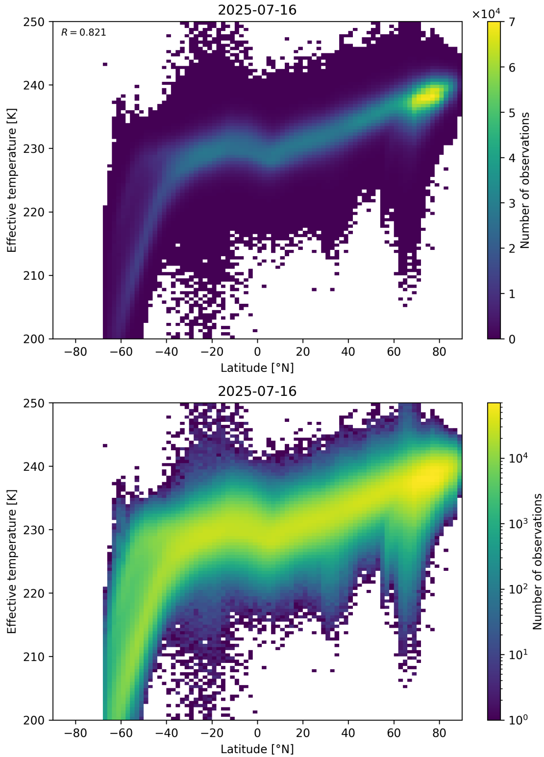
Figure 34: Scatter density plot of “Latitude” against “Effective temperature” for 2025-07-15 to 2025-07-17.
