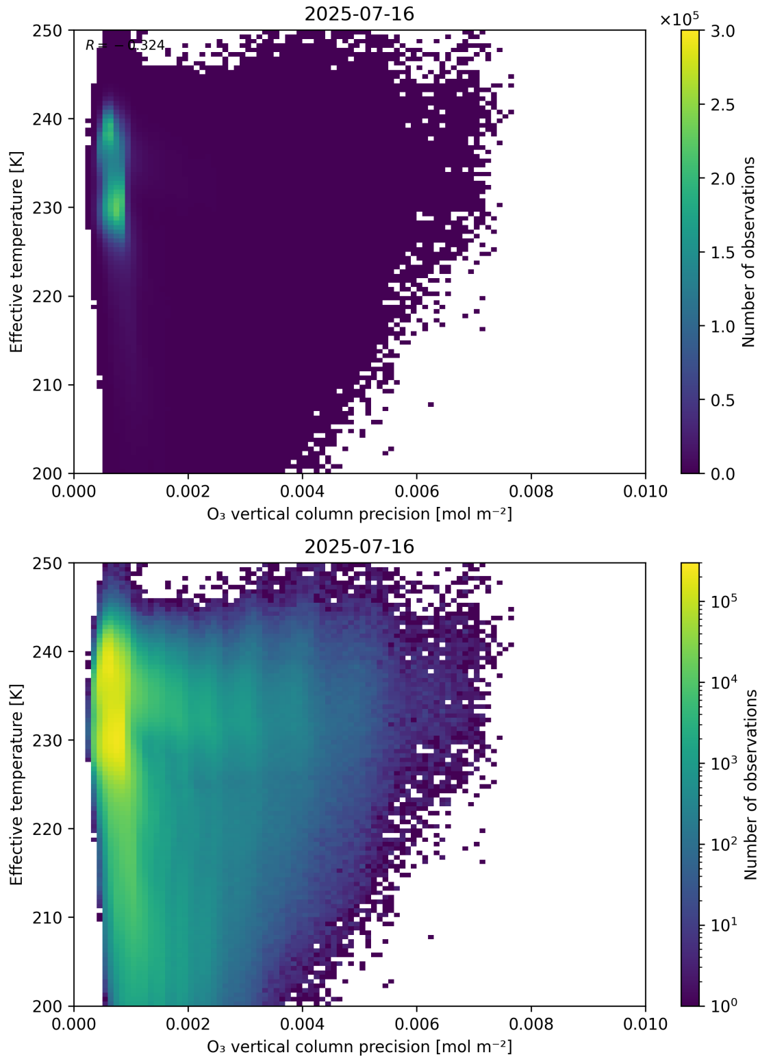
Figure 42: Scatter density plot of “O 3 vertical column precision” against “Effective temperature” for 2025-07-15 to 2025-07-17.
