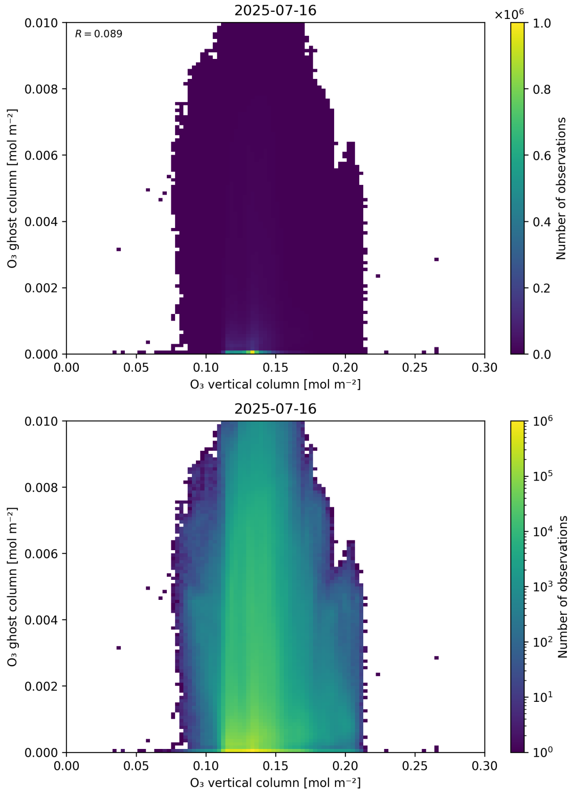
Figure 40: Scatter density plot of “O 3 vertical column” against “O 3 ghost column” for 2025-07-15 to 2025-07-17.
