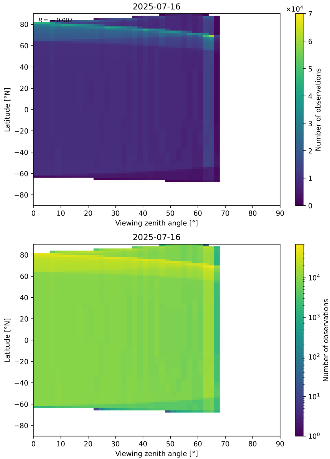
Figure 49: Scatter density plot of “Viewing zenith angle” against “Latitude” for 2025-07-15 to 2025-07-17.
