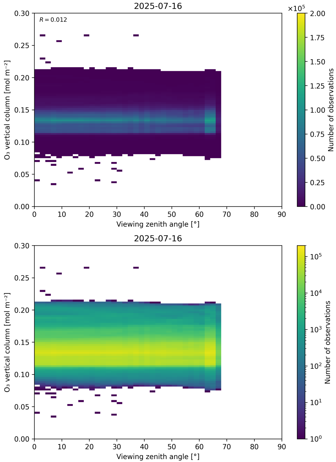
Figure 52: Scatter density plot of “Viewing zenith angle” against “O 3 vertical column” for 2025-07-15 to 2025-07-17.
