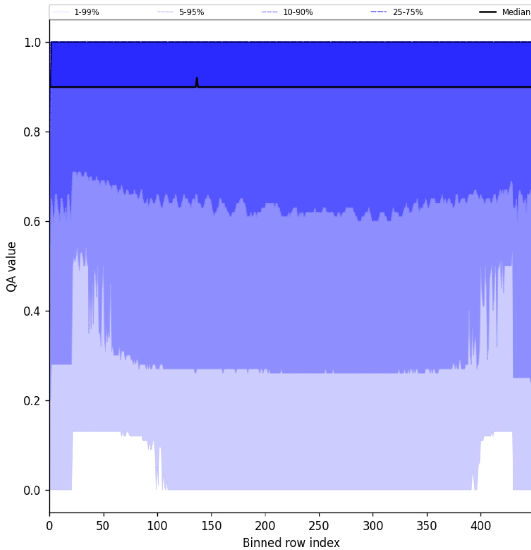
Figure 27: Along track statistics of “QA value” for 2025-07-15 to 2025-07-17
