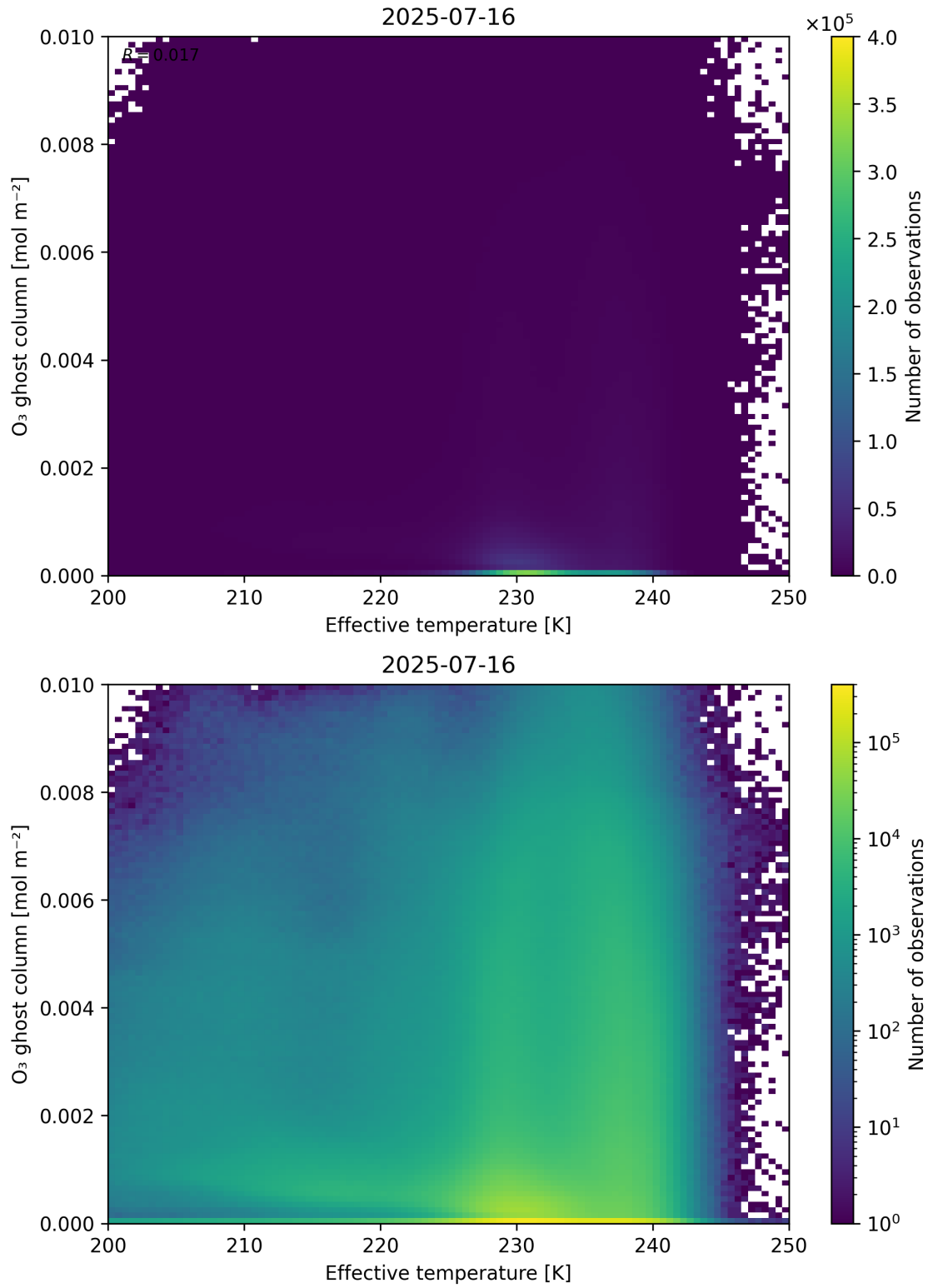
Figure 38: Scatter density plot of “Effective temperature” against “O 3 ghost column” for 2025-07-15 to 2025-07-17.
