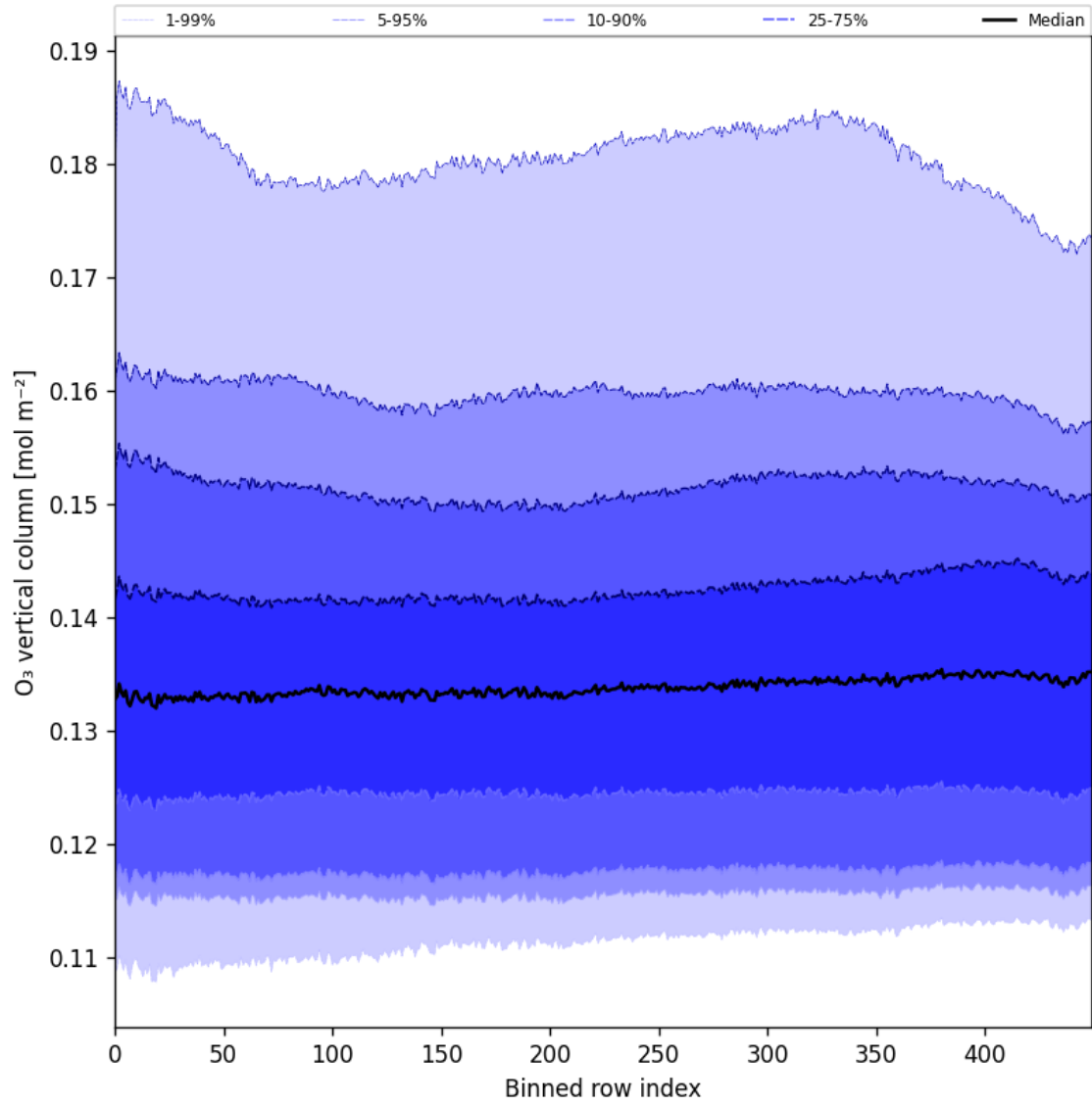
Figure 28: Along track statistics of “O 3 vertical column” for 2025-07-15 to 2025-07-17
