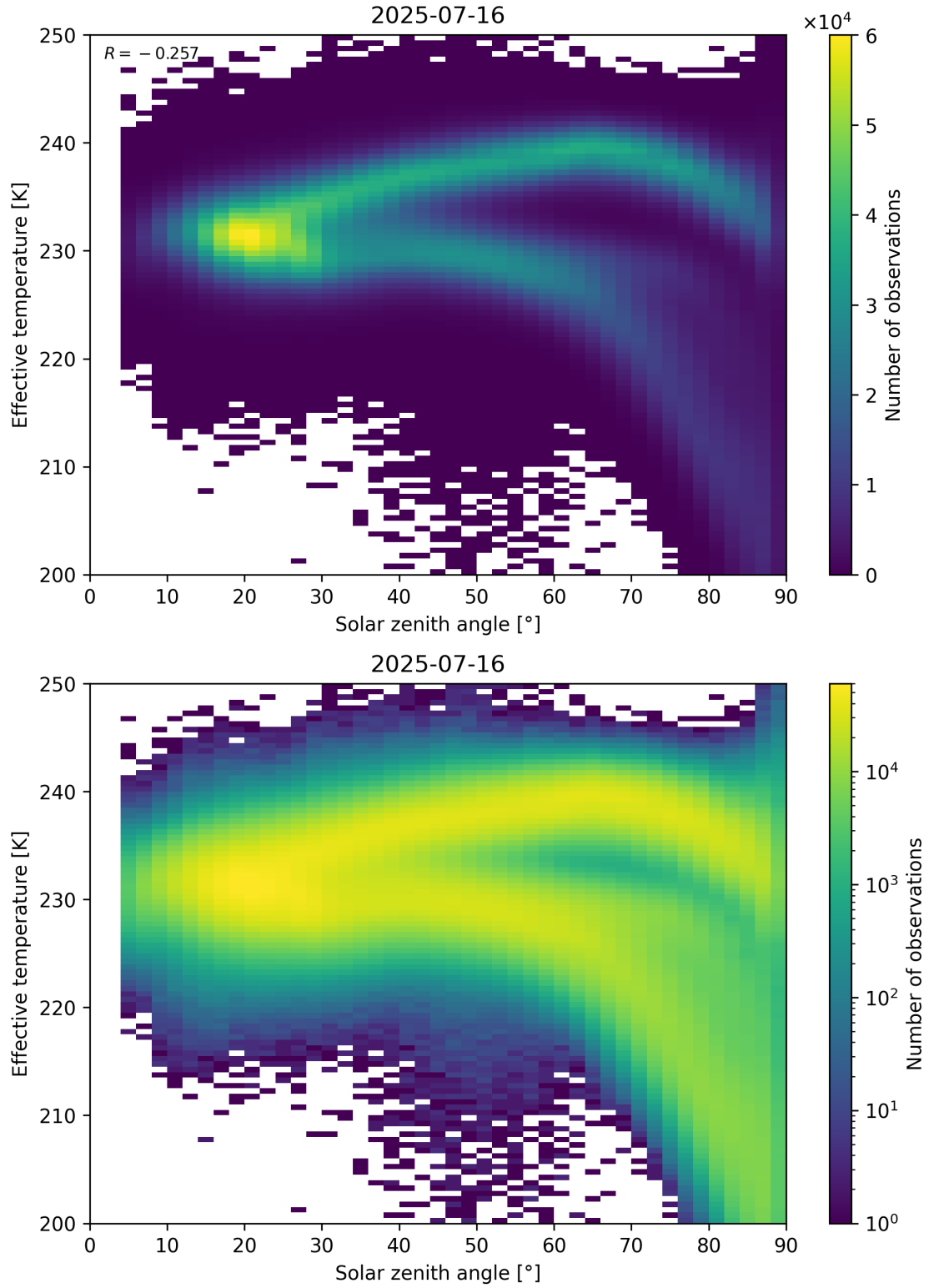
Figure 45: Scatter density plot of “Solar zenith angle” against “Effective temperature” for 2025-07-15 to 2025-07-17.
