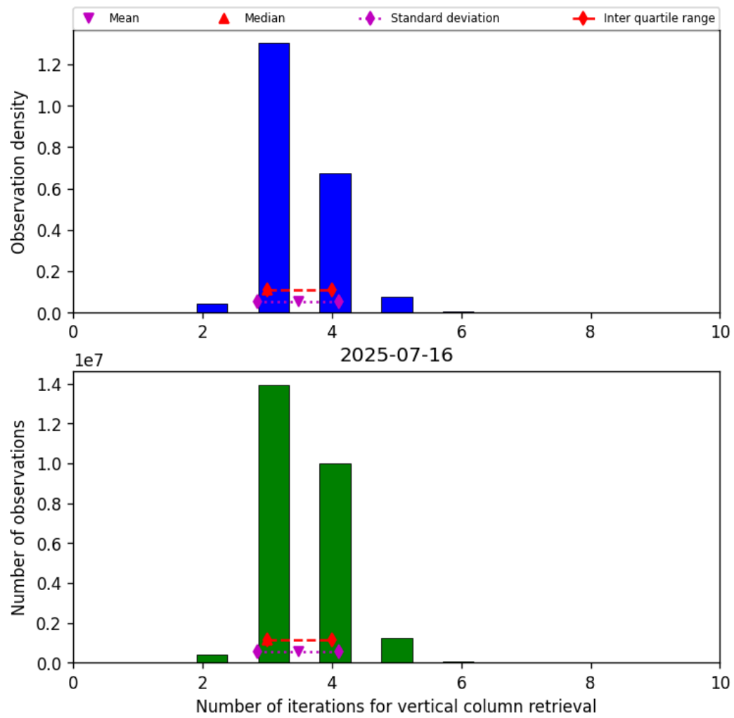
Figure 26: Histogram of “Number of iterations for vertical column retrieval” for 2025-07-15 to 2025-07-17
