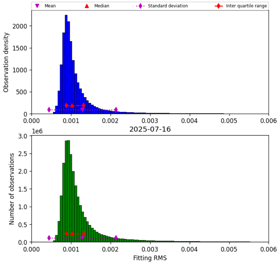
Figure 23: Histogram of “Fitting RMS” for 2025-07-15 to 2025-07-17
