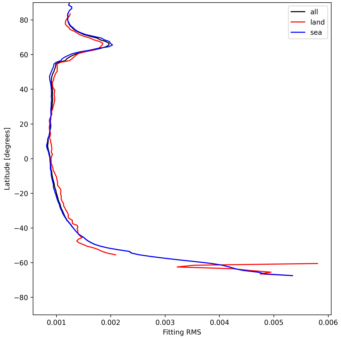
Figure 16: Zonal average of “Fitting RMS” for 2025-07-15 to 2025-07-17.
