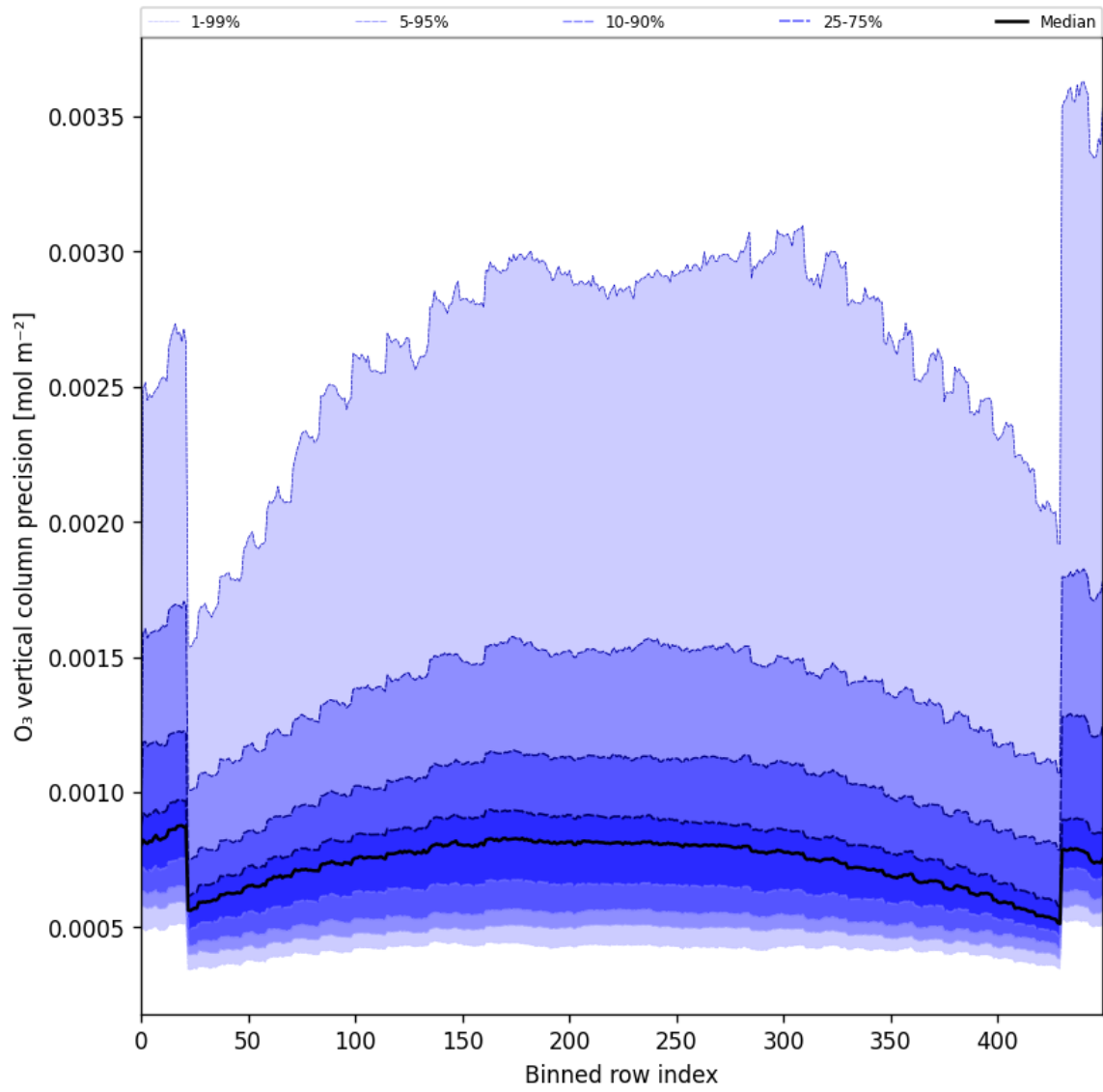
Figure 29: Along track statistics of “O 3 vertical column precision” for 2025-07-15 to 2025-07-17
