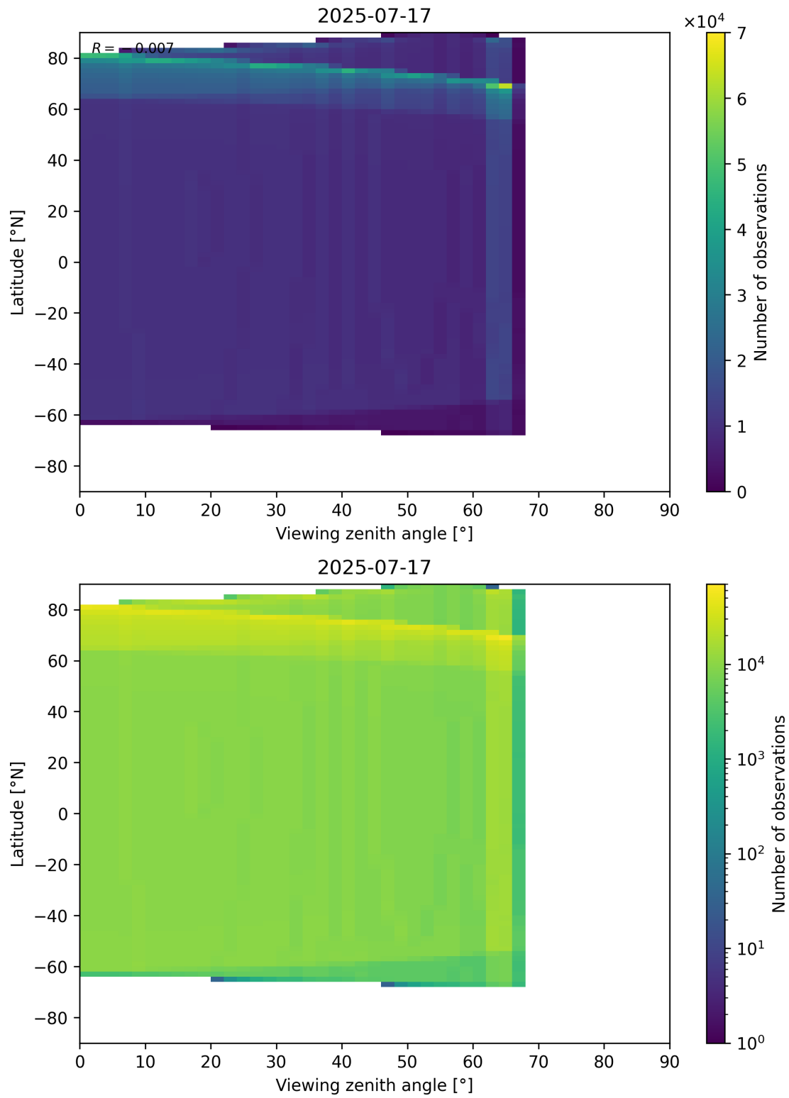
Figure 49: Scatter density plot of “Viewing zenith angle” against “Latitude” for 2025-07-16 to 2025-07-18.
