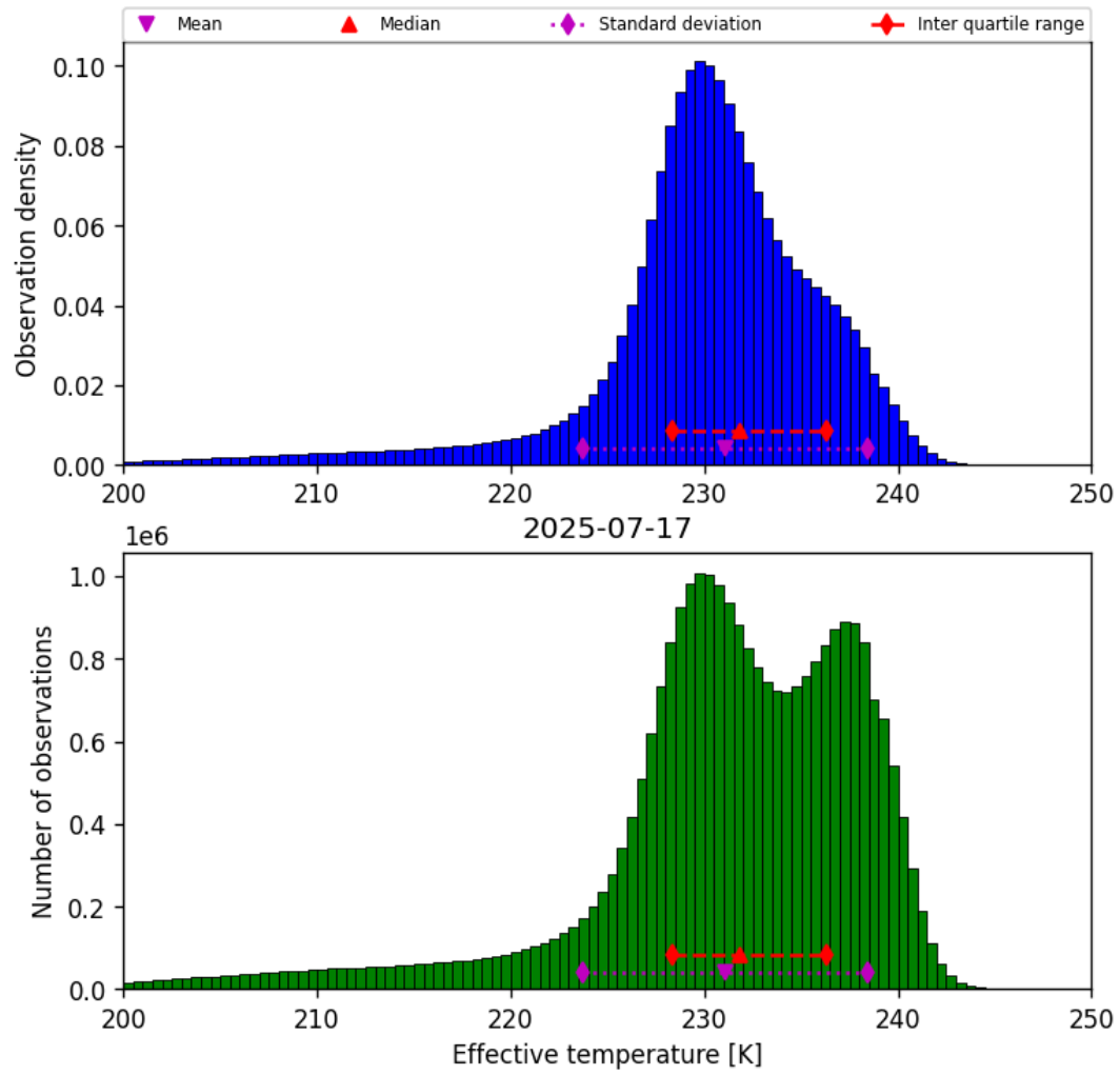
Figure 24: Histogram of “Effective temperature” for 2025-07-16 to 2025-07-18
