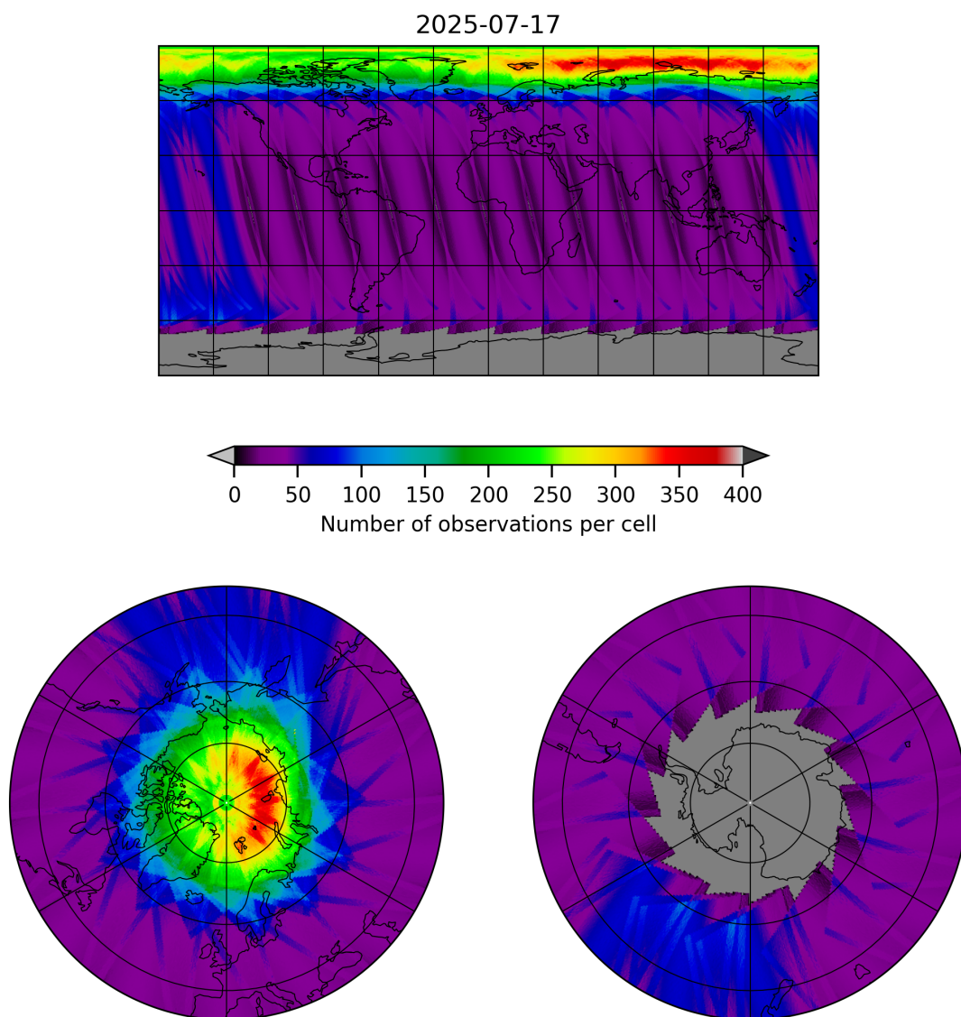
Figure 12: Map of the number of observations for 2025-07-16 to 2025-07-18
