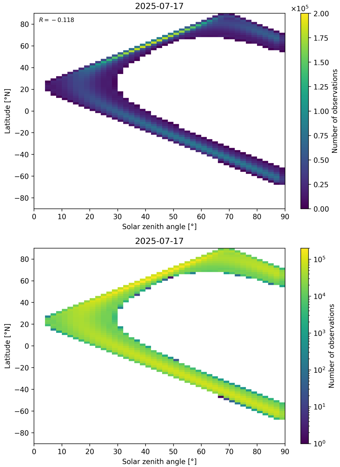
Figure 44: Scatter density plot of “Solar zenith angle” against “Latitude” for 2025-07-16 to 2025-07-18.
