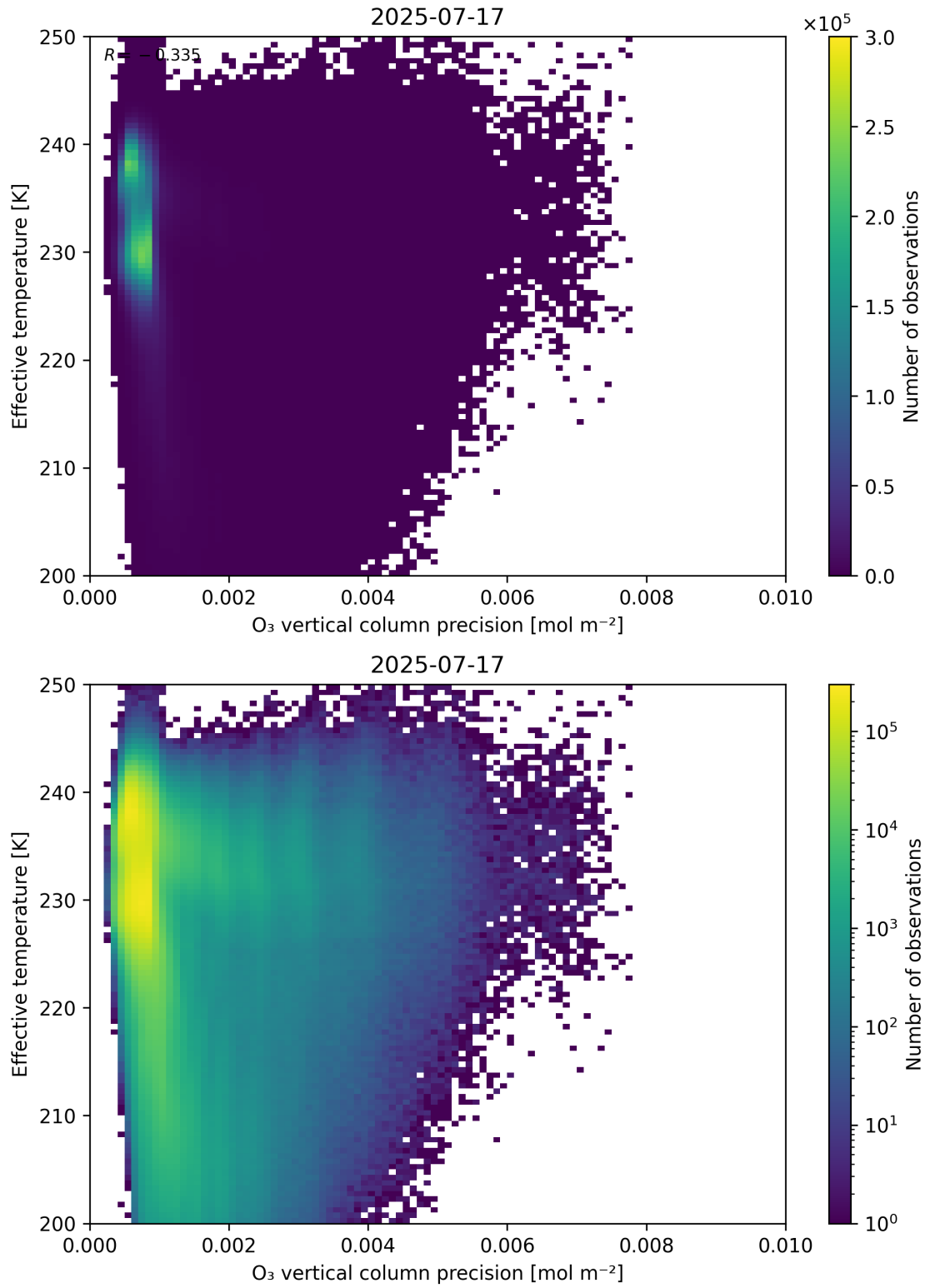
Figure 42: Scatter density plot of “O 3 vertical column precision” against “Effective temperature” for 2025-07-16 to 2025-07-18.
