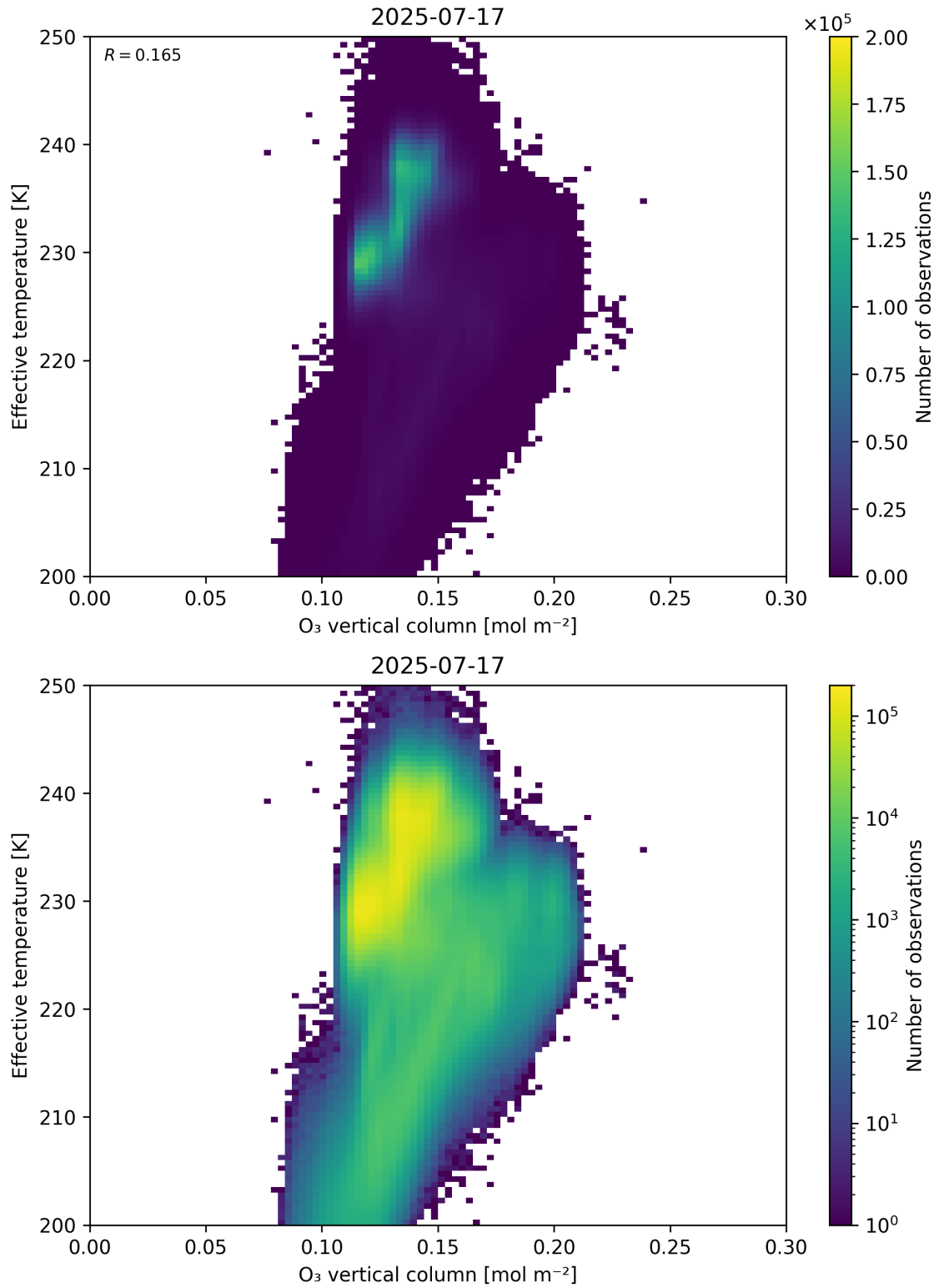
Figure 39: Scatter density plot of “O 3 vertical column” against “Effective temperature” for 2025-07-16 to 2025-07-18.
