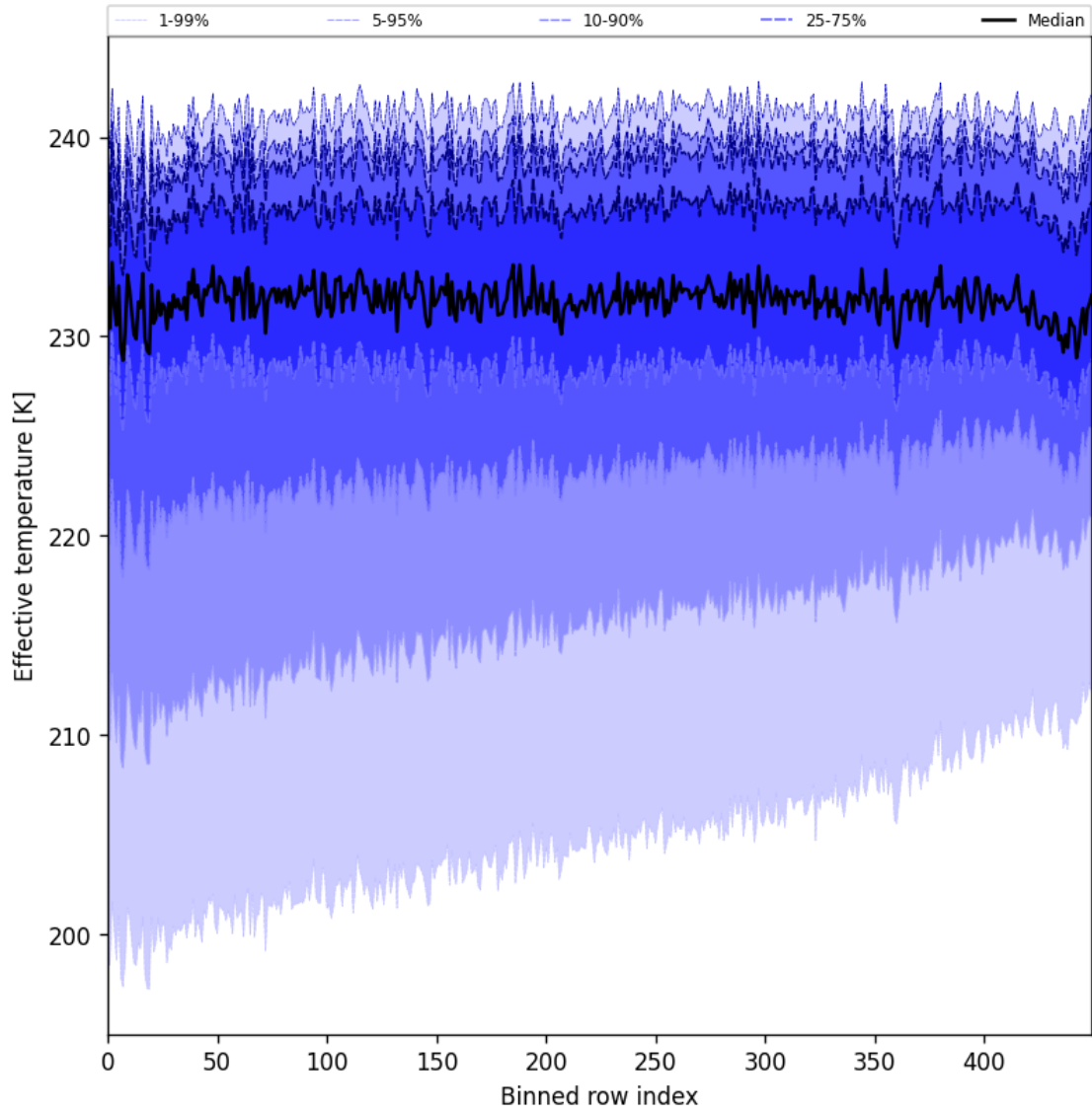
Figure 31: Along track statistics of “Effective temperature” for 2025-07-16 to 2025-07-18
