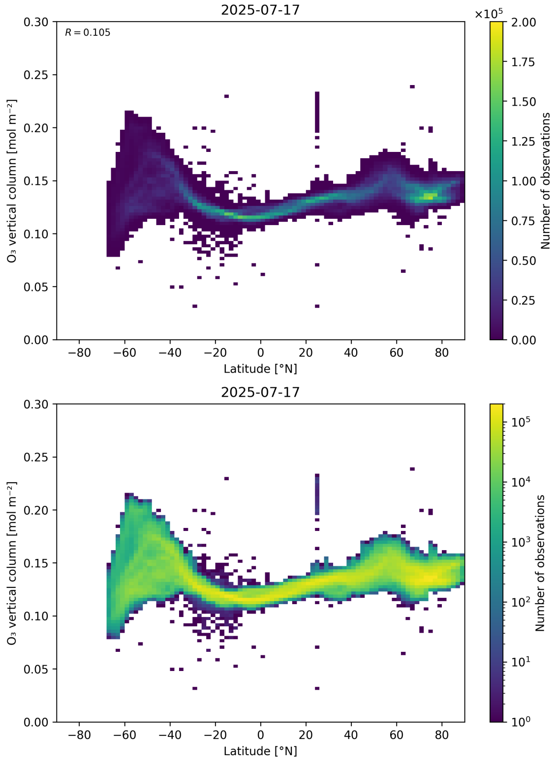
Figure 36: Scatter density plot of “Latitude” against “O 3 vertical column” for 2025-07-16 to 2025-07-18.
