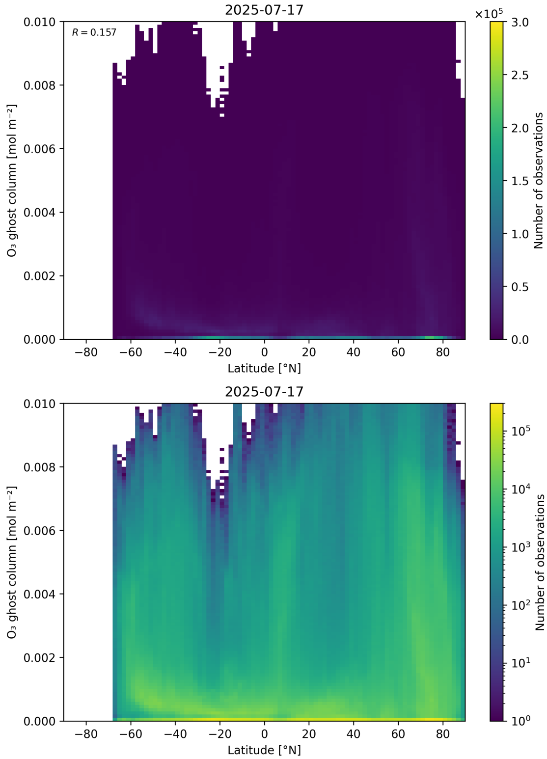
Figure 35: Scatter density plot of “Latitude” against “O 3 ghost column” for 2025-07-16 to 2025-07-18.
