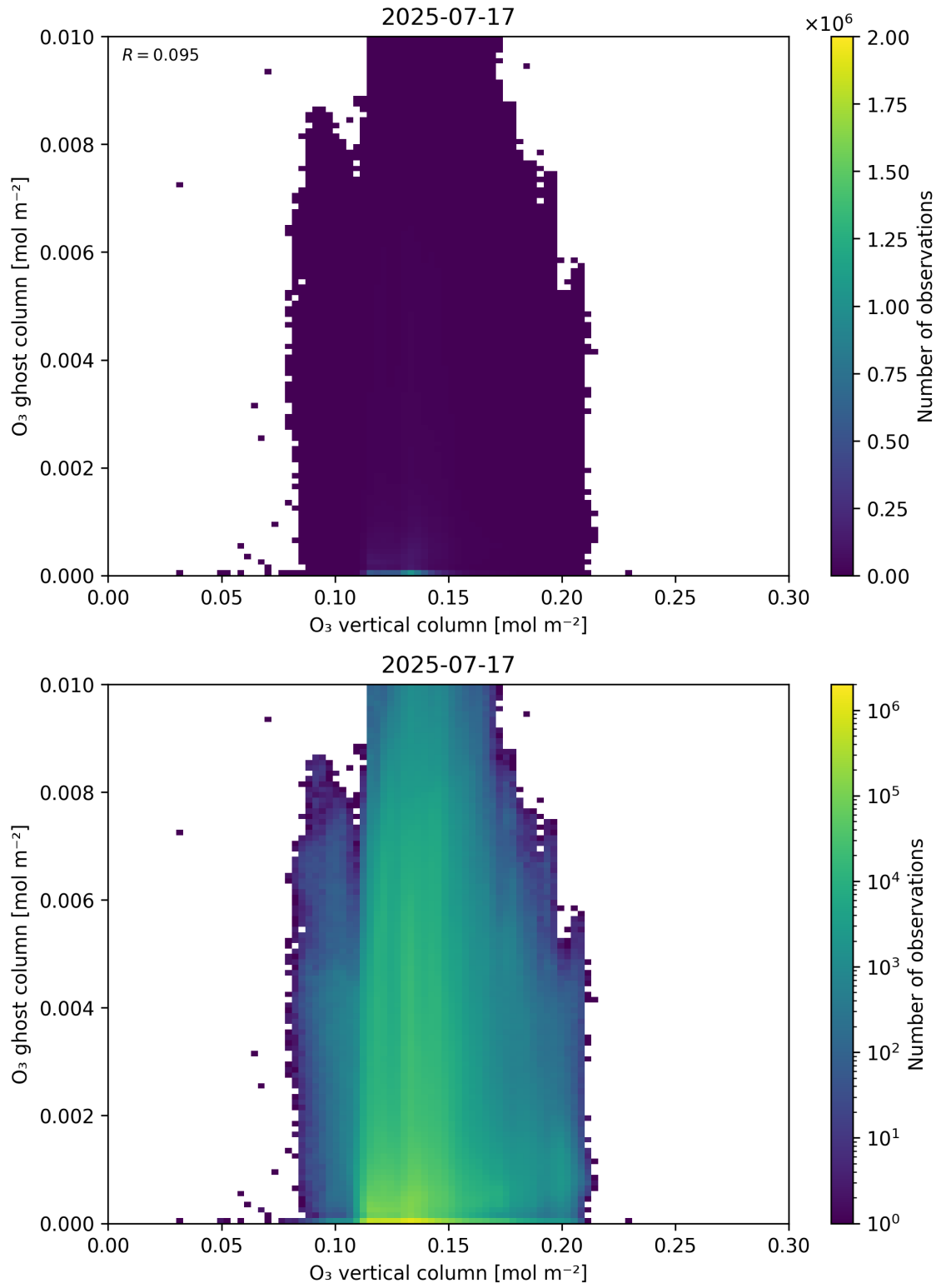
Figure 40: Scatter density plot of “O 3 vertical column” against “O 3 ghost column” for 2025-07-16 to 2025-07-18.
