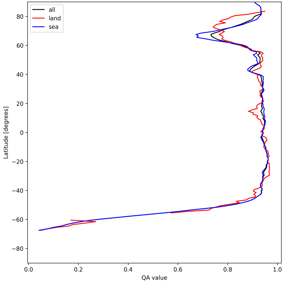
Figure 13: Zonal average of “QA value” for 2025-07-16 to 2025-07-18.
