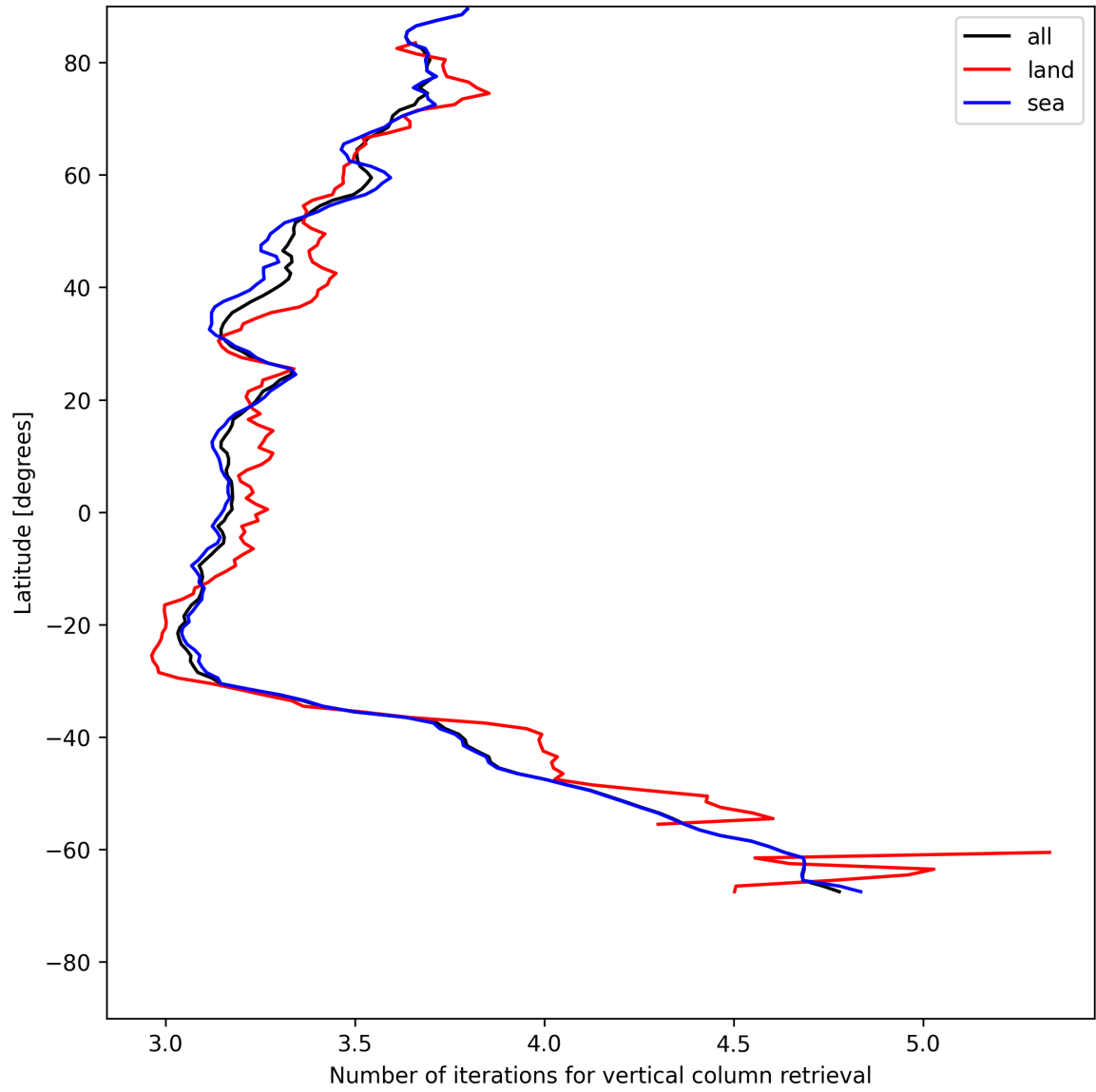
Figure 19: Zonal average of “Number of iterations for vertical column retrieval” for 2025-07-16 to 2025-07-18.
