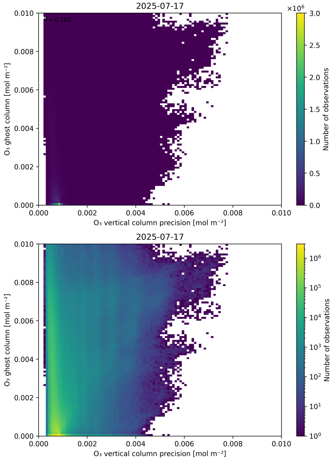
Figure 43: Scatter density plot of “ \text{O}_3 vertical column precision” against “ \text{O}_3 ghost column” for 2025-07-16 to 2025-07-18.
