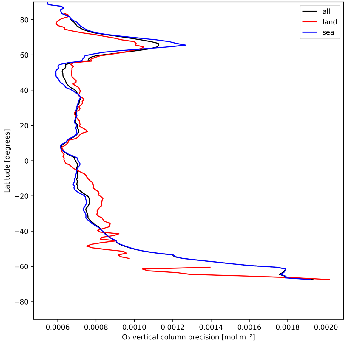
Figure 15: Zonal average of “O 3 vertical column precision” for 2025-07-16 to 2025-07-18.
