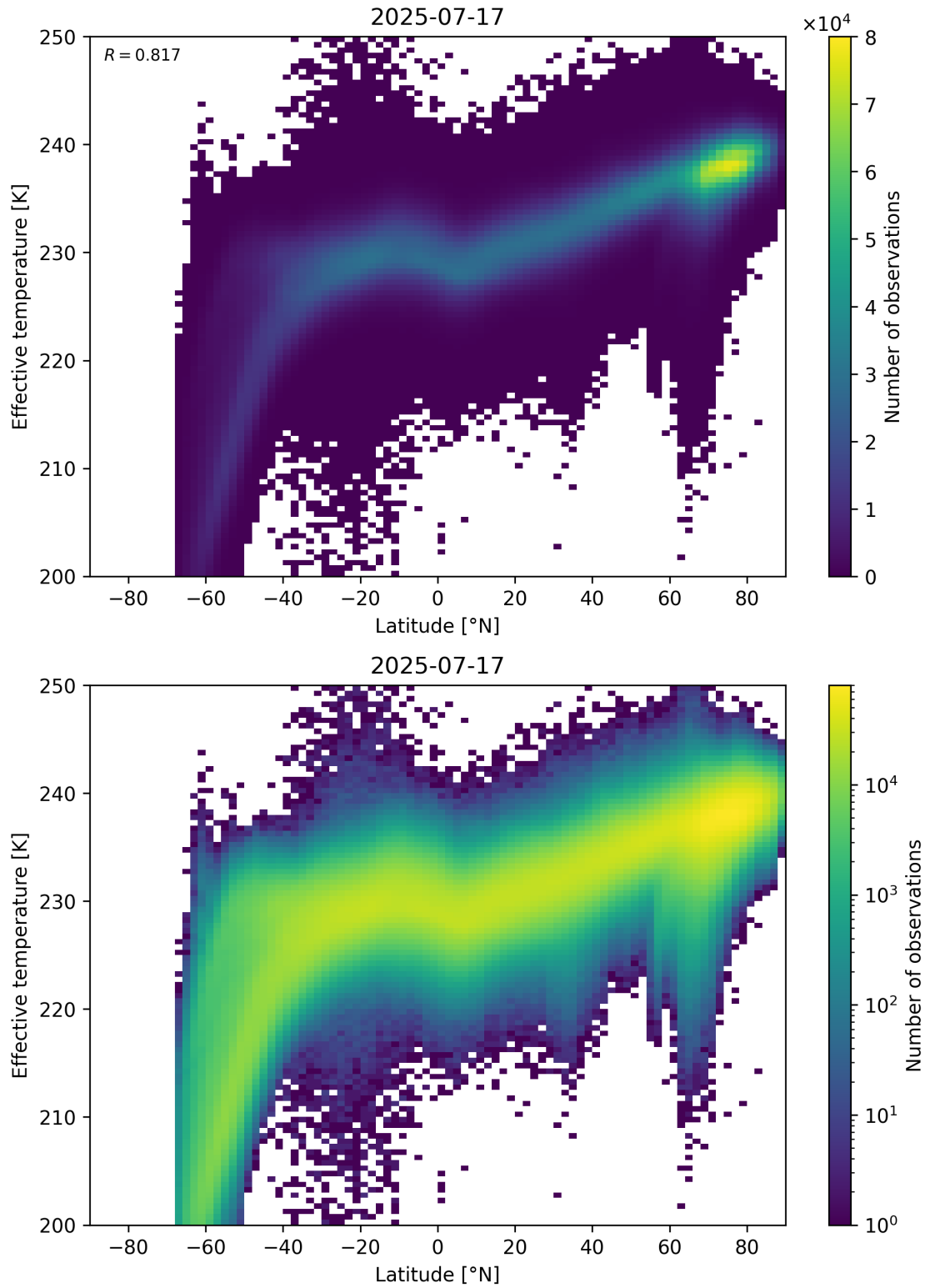
Figure 34: Scatter density plot of “Latitude” against “Effective temperature” for 2025-07-16 to 2025-07-18.
