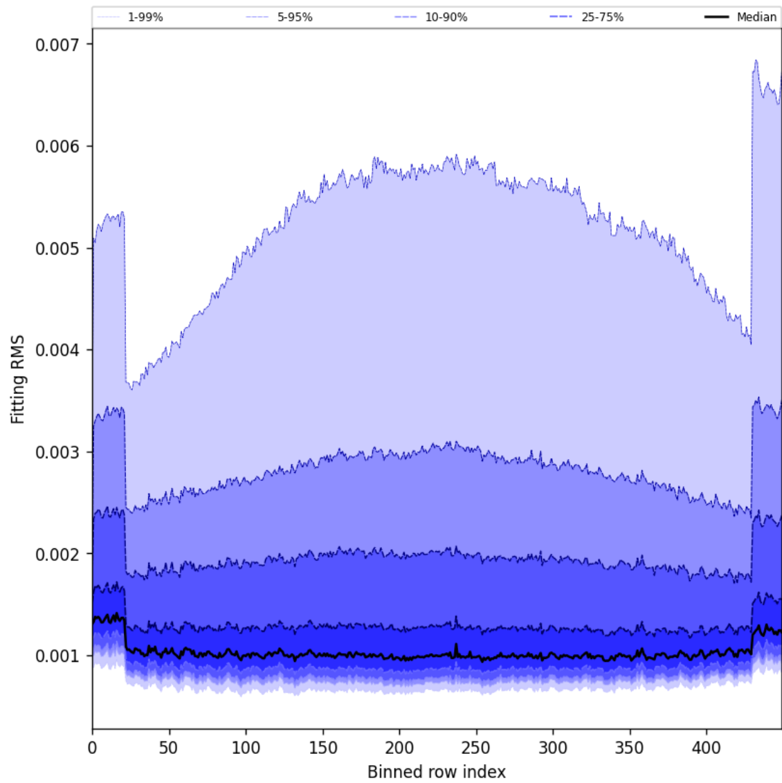
Figure 30: Along track statistics of “Fitting RMS” for 2025-07-16 to 2025-07-18
