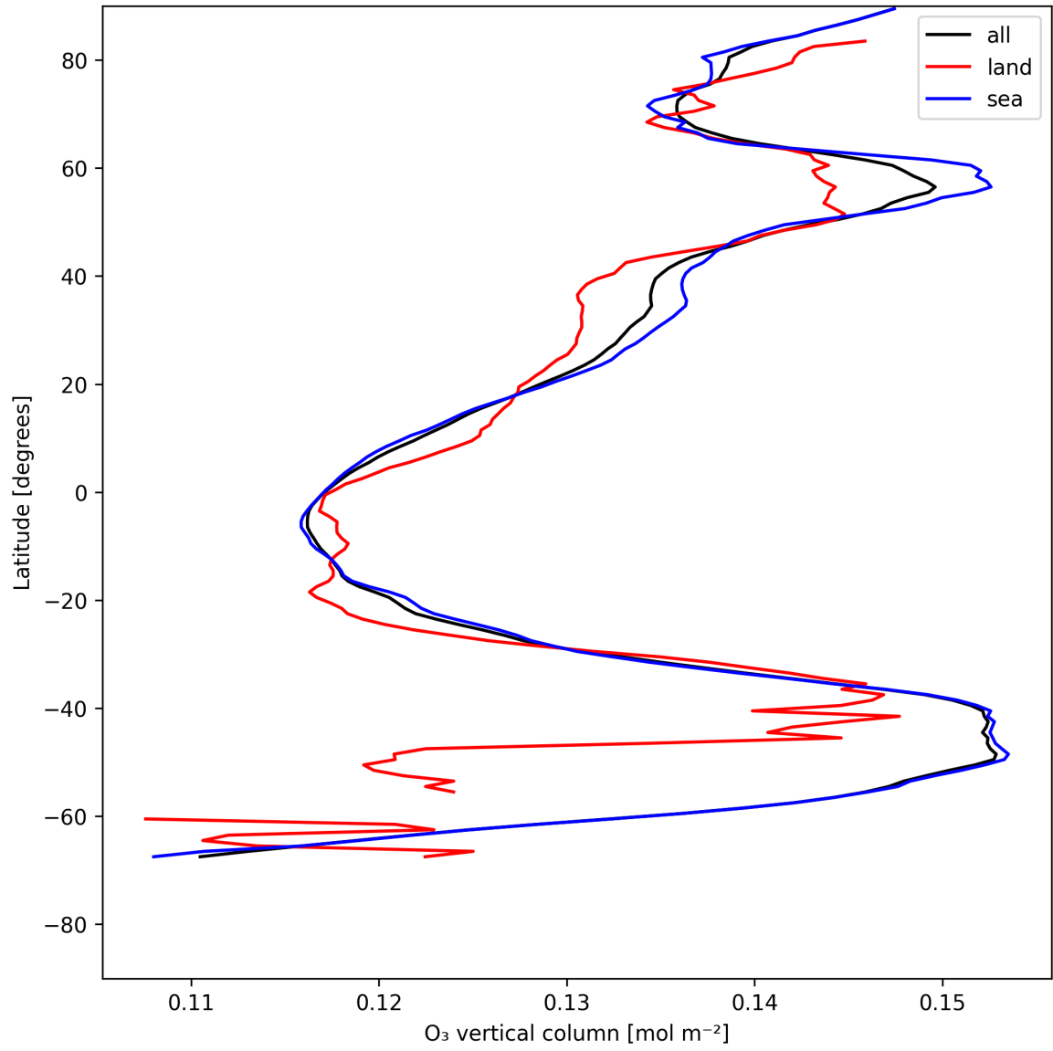
Figure 14: Zonal average of “O 3 vertical column” for 2025-07-16 to 2025-07-18.
