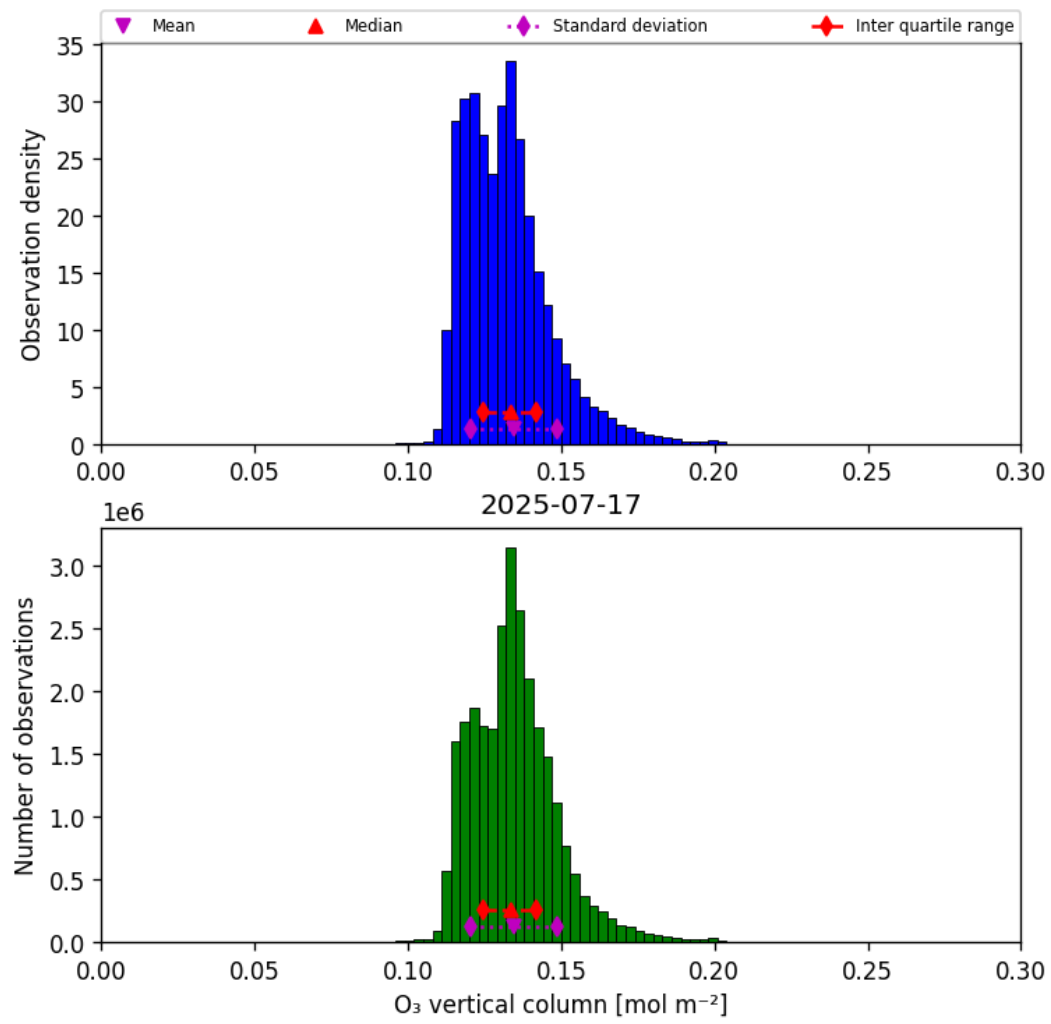
Figure 21: Histogram of “O 3 vertical column” for 2025-07-16 to 2025-07-18
