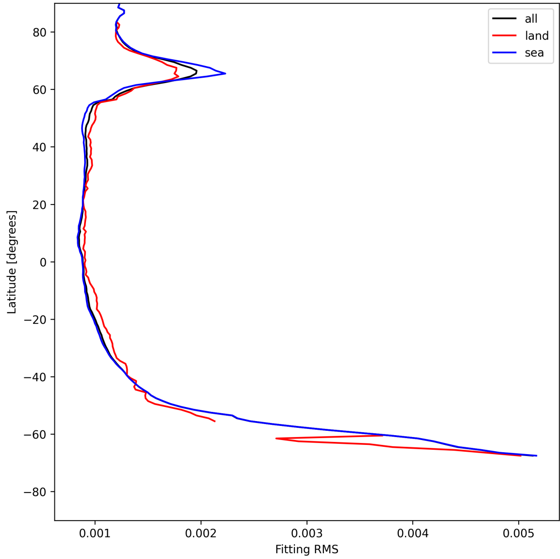
Figure 16: Zonal average of “Fitting RMS” for 2025-07-16 to 2025-07-18.
