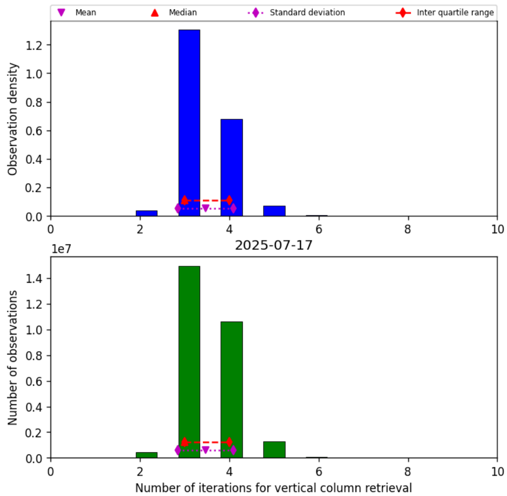
Figure 26: Histogram of “Number of iterations for vertical column retrieval” for 2025-07-16 to 2025-07-18
