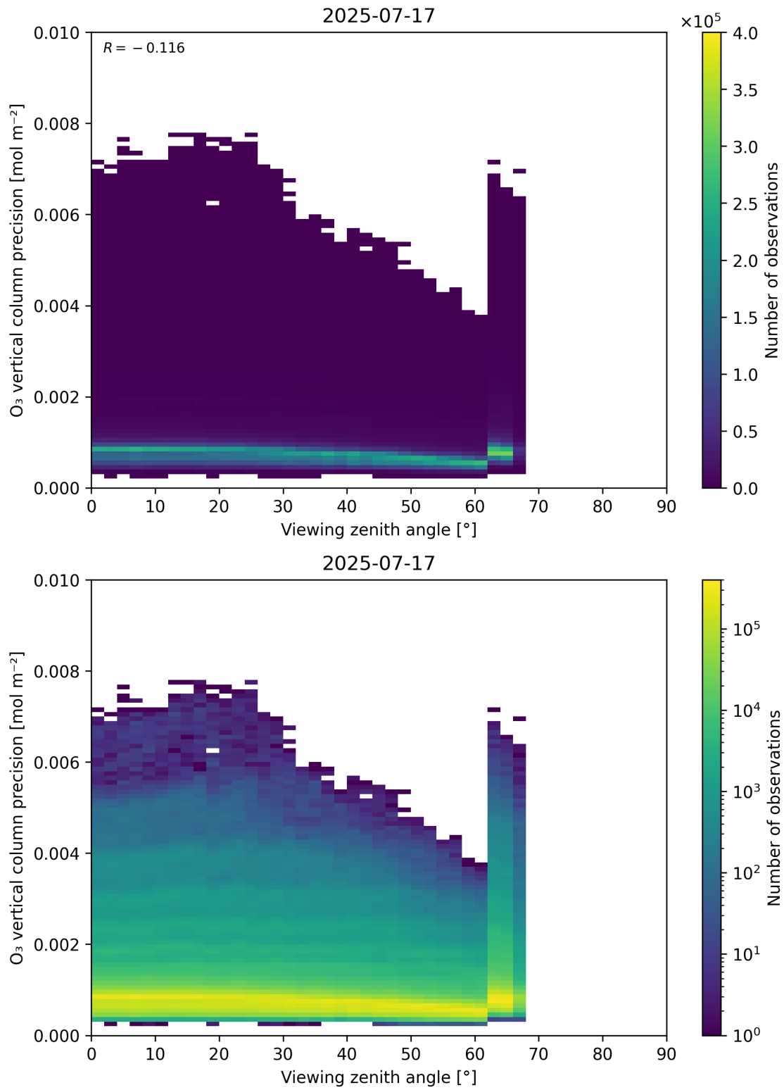
Figure 53: Scatter density plot of “Viewing zenith angle” against “O 3 vertical column precision” for 2025-07-16 to 2025-07-18.
