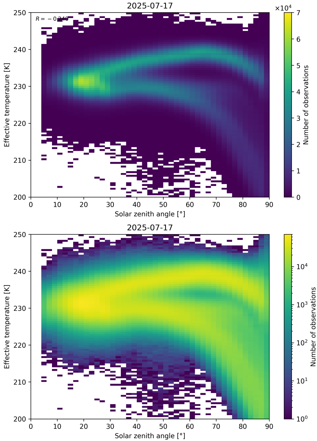
Figure 45: Scatter density plot of “Solar zenith angle” against “Effective temperature” for 2025-07-16 to 2025-07-18.
