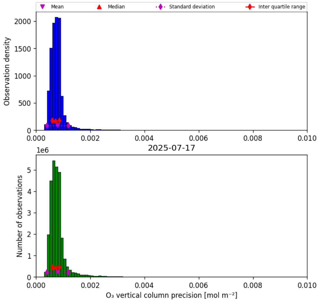
Figure 22: Histogram of “O 3 vertical column precision” for 2025-07-16 to 2025-07-18
