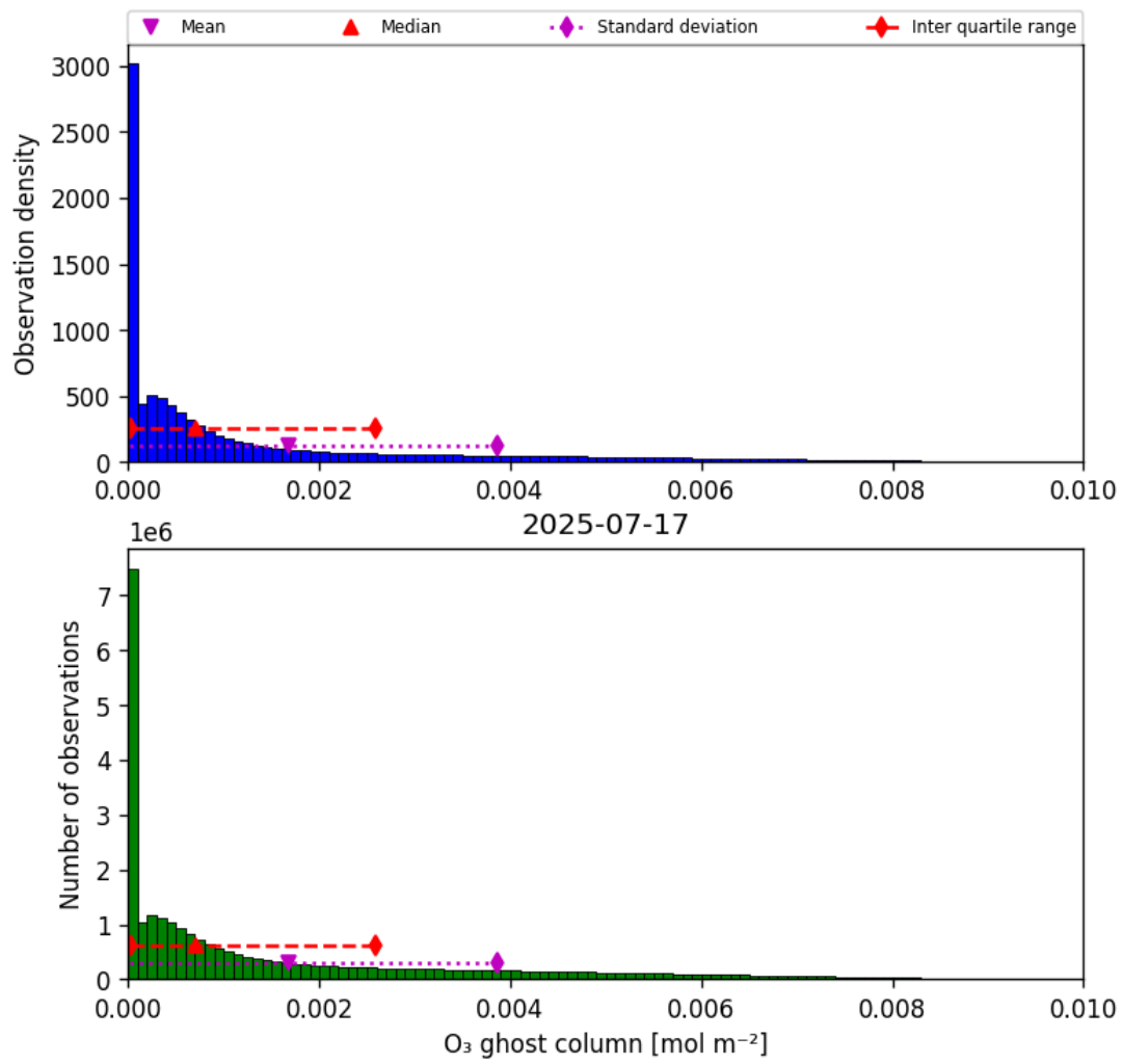
Figure 25: Histogram of “O 3 ghost column” for 2025-07-16 to 2025-07-18
