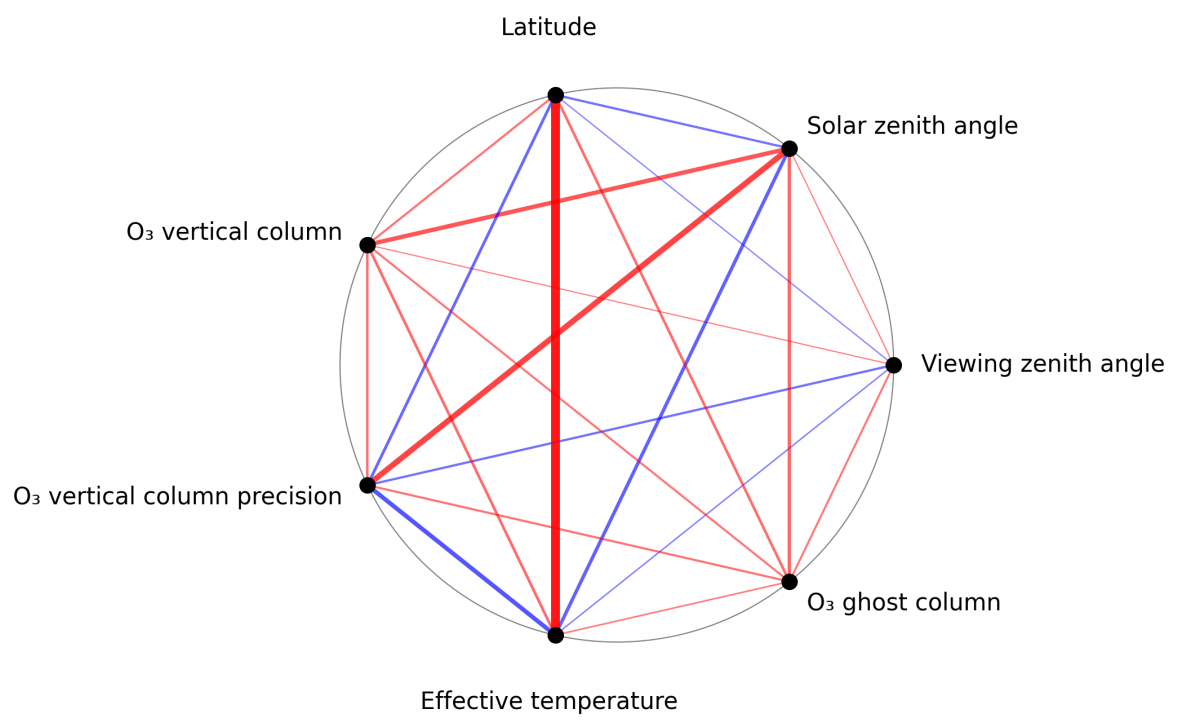
Figure 1: Map of correlation graph for 2025-07-16 to 2025-07-18.
