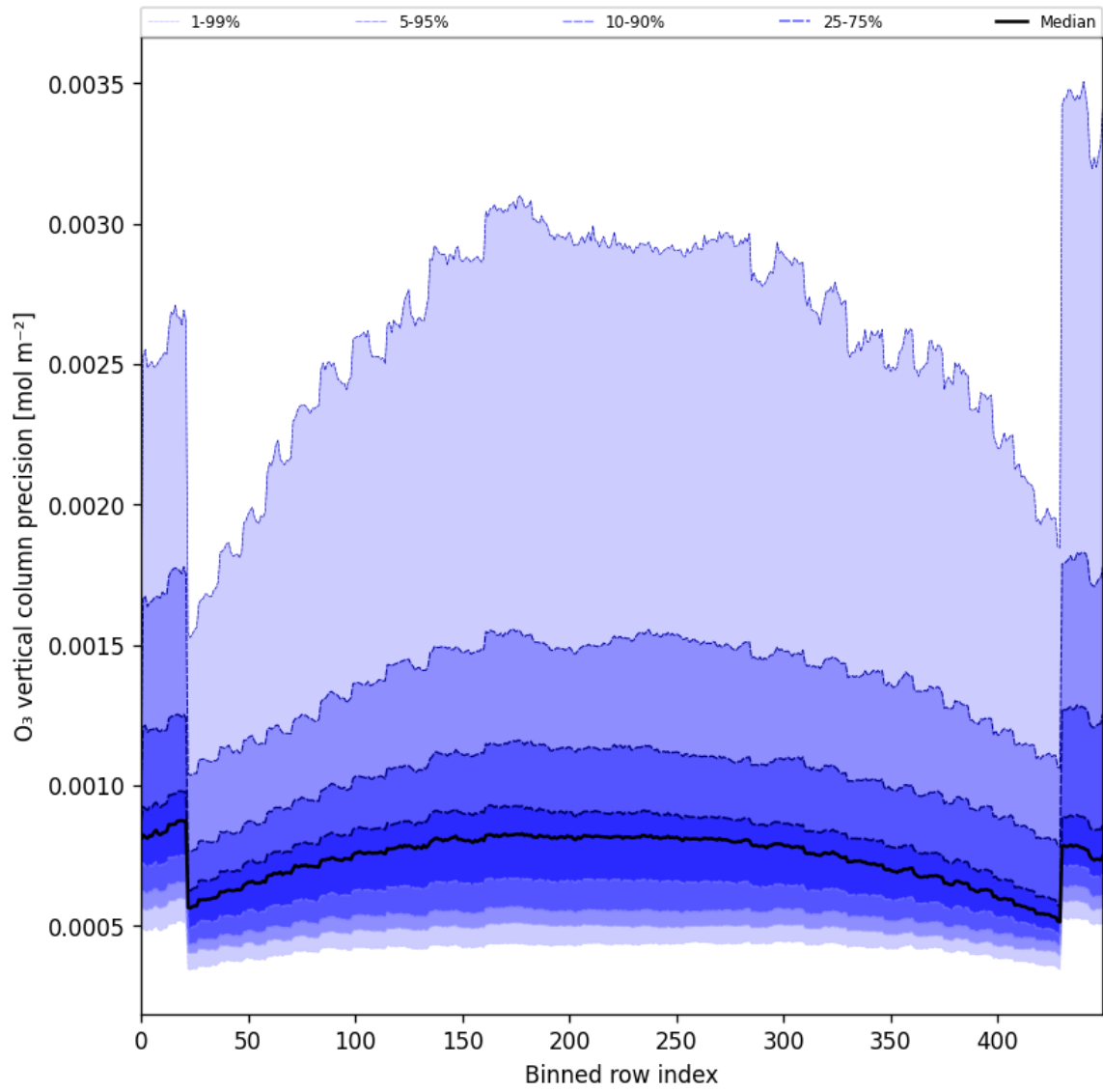
Figure 29: Along track statistics of “O 3 vertical column precision” for 2025-07-16 to 2025-07-18
