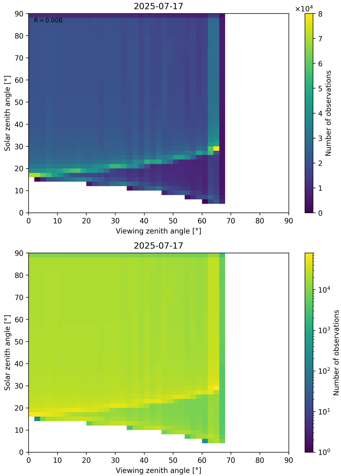
Figure 54: Scatter density plot of “Viewing zenith angle” against “Solar zenith angle” for 2025-07-16 to 2025-07-18.
