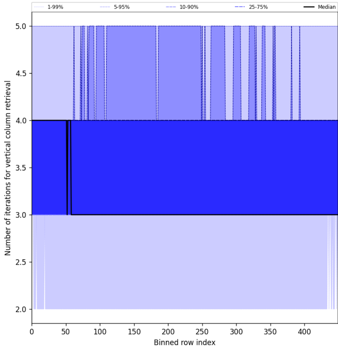
Figure 33: Along track statistics of “Number of iterations for vertical column retrieval” for 2025-07-16 to 2025-07-18
