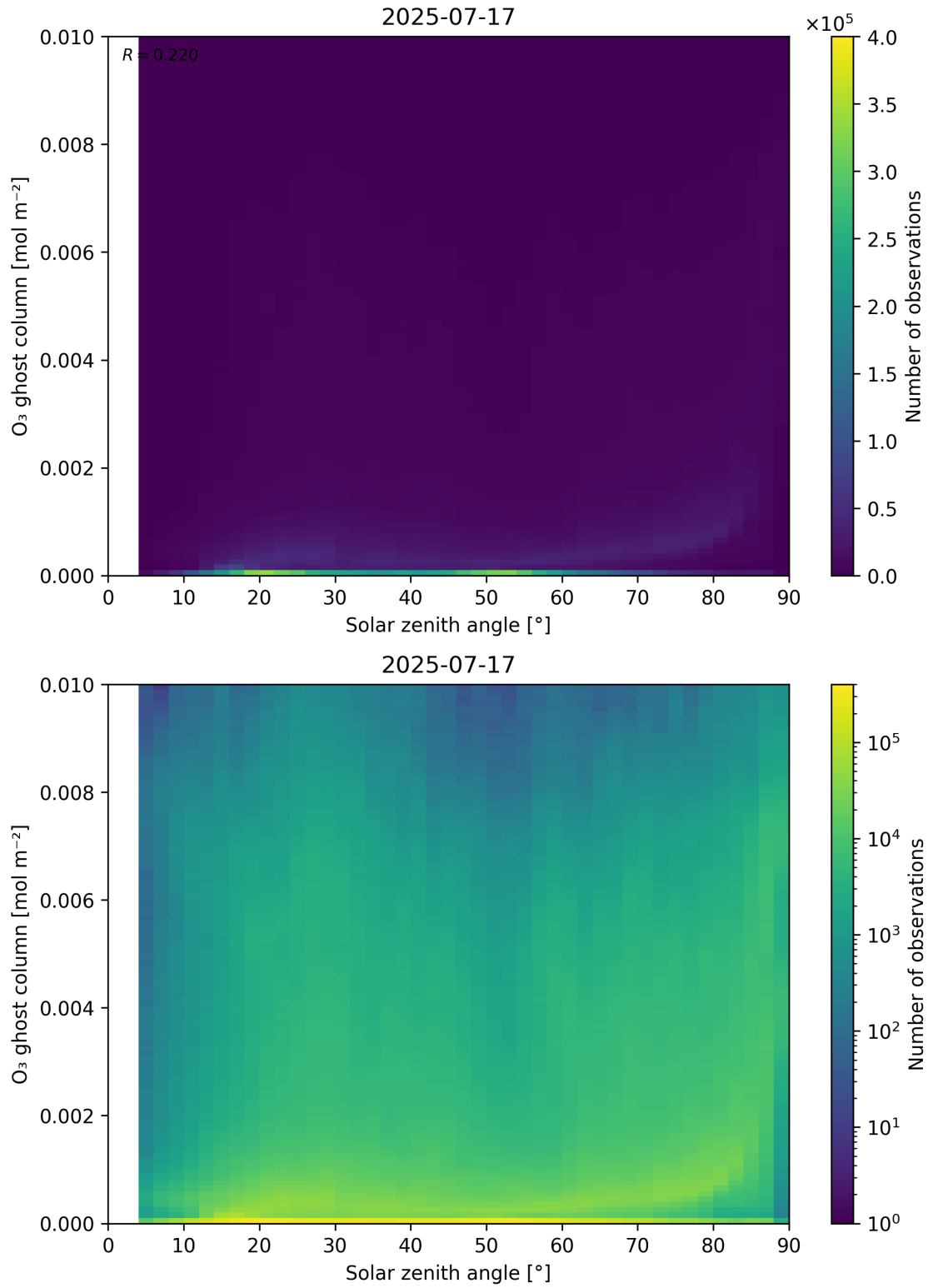
Figure 46: Scatter density plot of “Solar zenith angle” against “O 3 ghost column” for 2025-07-16 to 2025-07-18.
