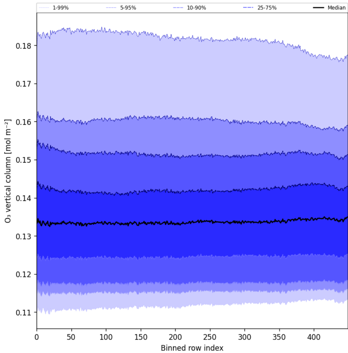
Figure 28: Along track statistics of “O 3 vertical column” for 2025-07-16 to 2025-07-18
