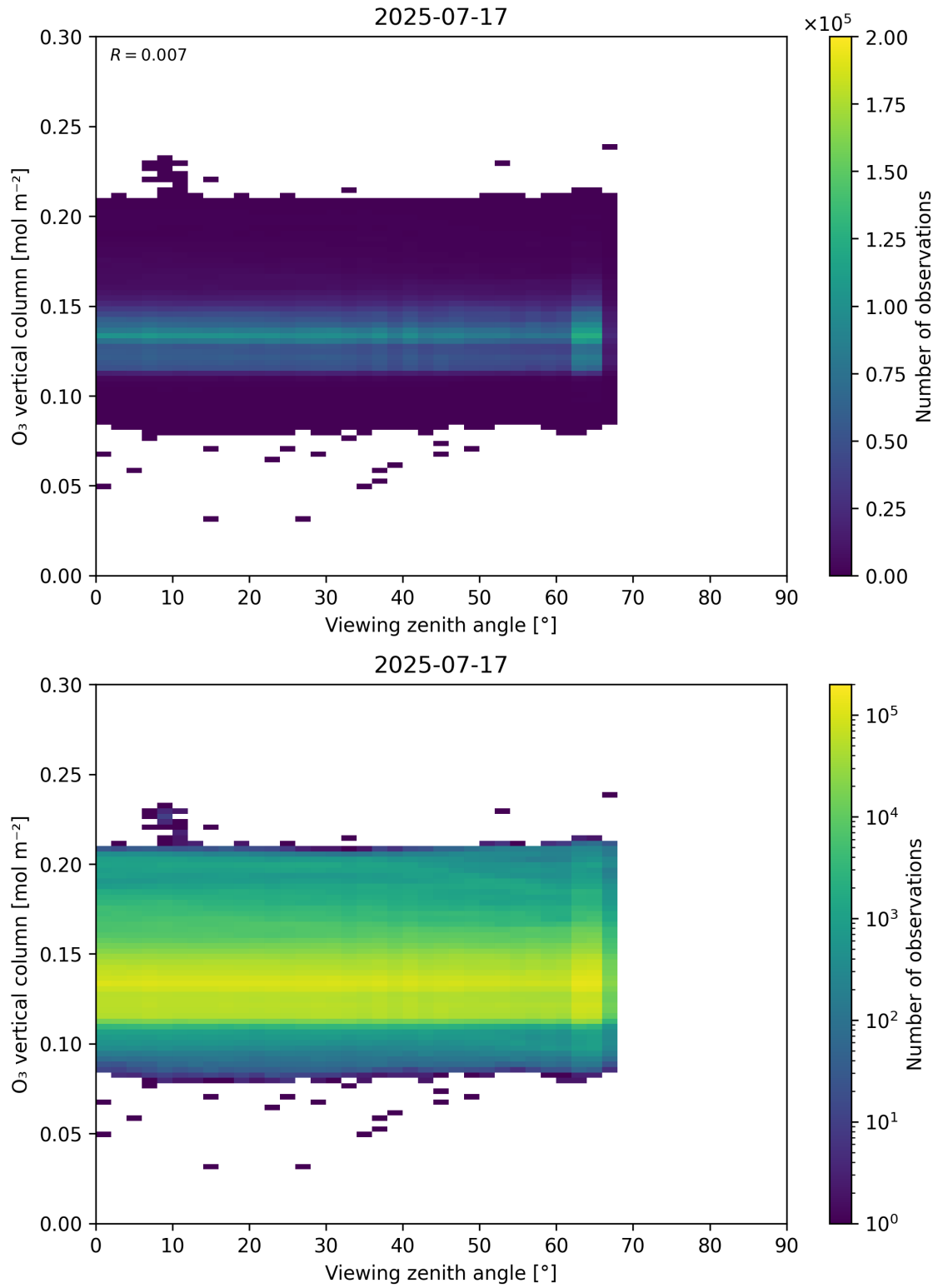
Figure 52: Scatter density plot of “Viewing zenith angle” against “O 3 vertical column” for 2025-07-16 to 2025-07-18.
