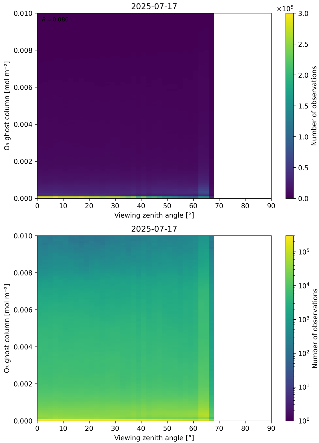
Figure 51: Scatter density plot of “Viewing zenith angle” against “O 3 ghost column” for 2025-07-16 to 2025-07-18.
