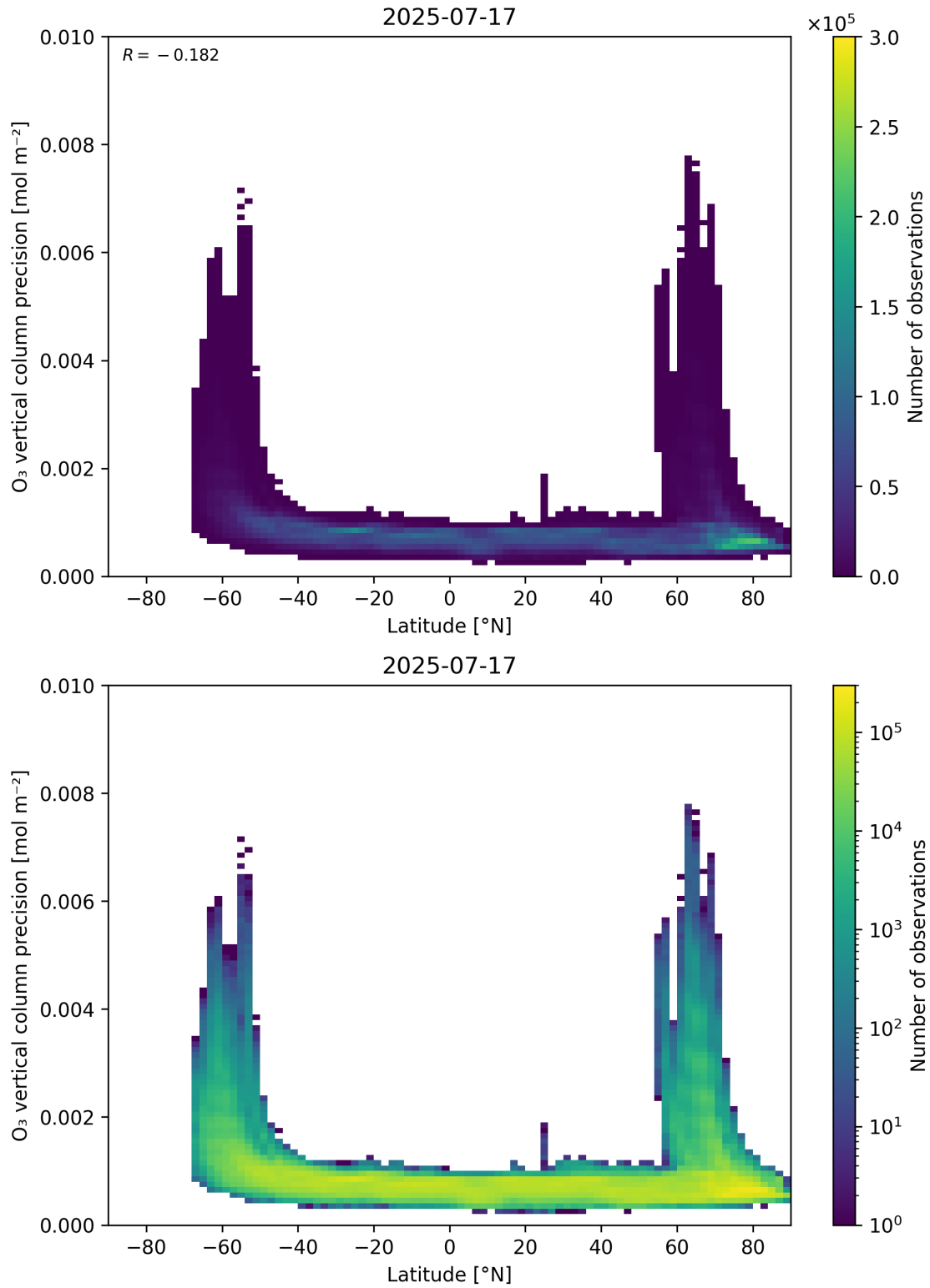
Figure 37: Scatter density plot of “Latitude” against “O 3 vertical column precision” for 2025-07-16 to 2025-07-18.
