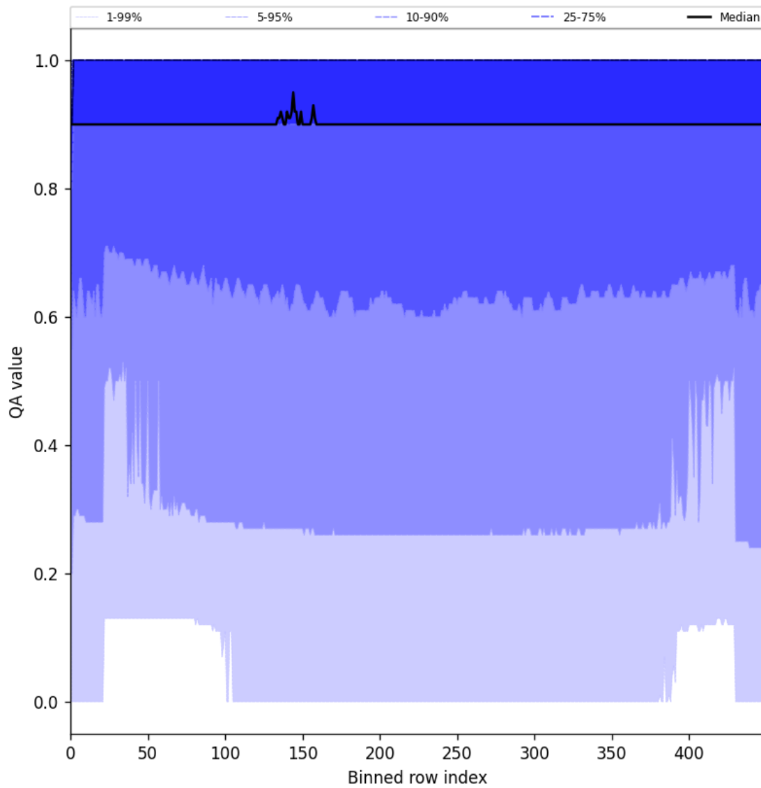
Figure 27: Along track statistics of “QA value” for 2025-07-16 to 2025-07-18
