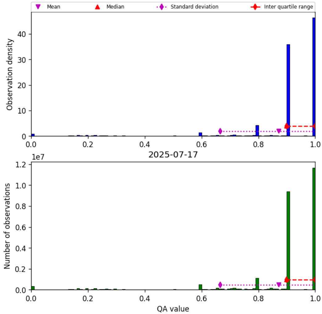
Figure 20: Histogram of “QA value” for 2025-07-16 to 2025-07-18
