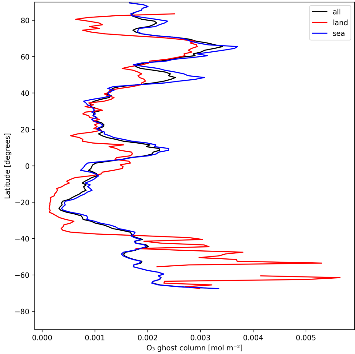
Figure 18: Zonal average of "O 3 ghost column" for 2025-07-16 to 2025-07-18.
