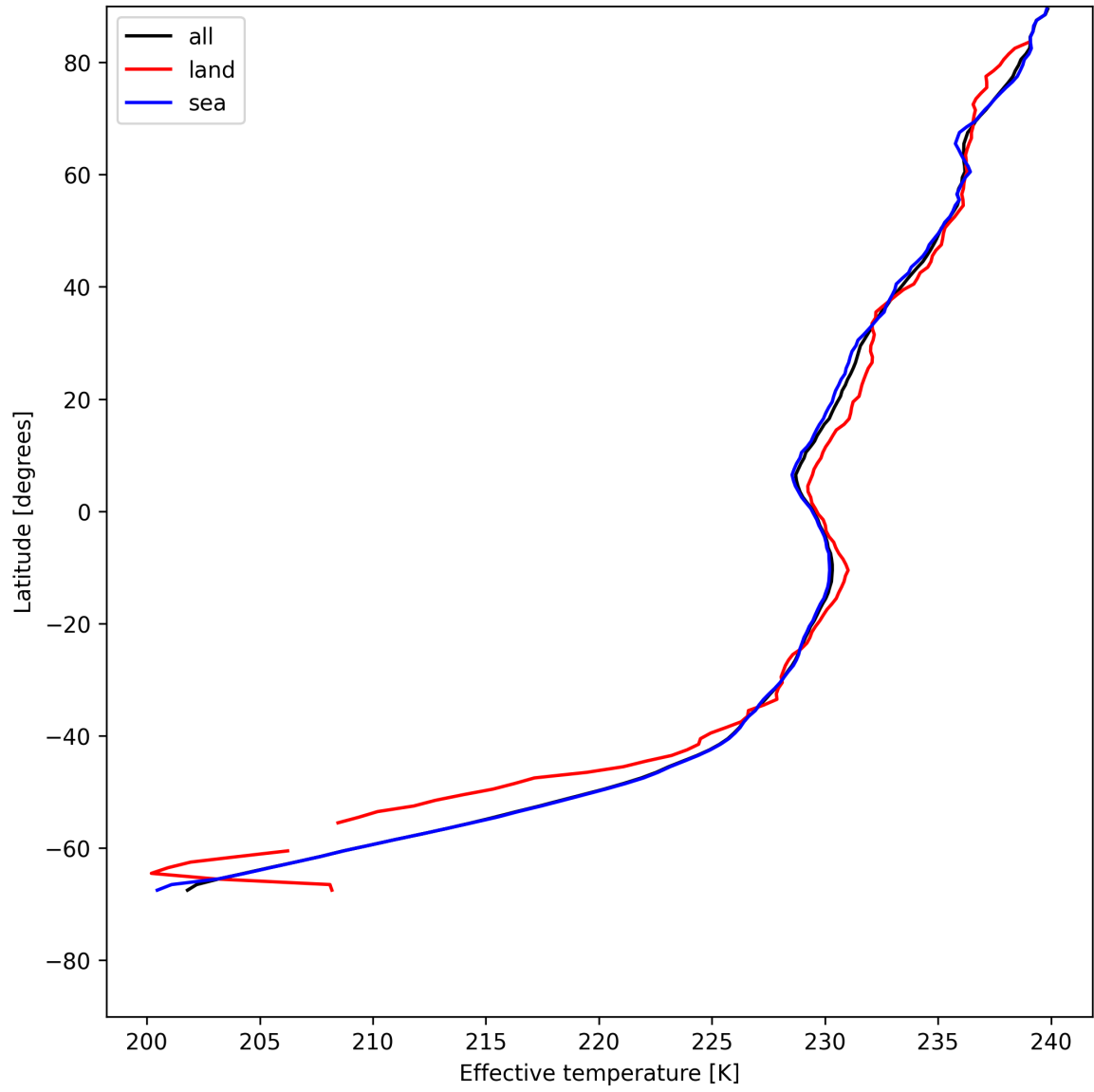
Figure 17: Zonal average of "Effective temperature" for 2025-07-16 to 2025-07-18.
