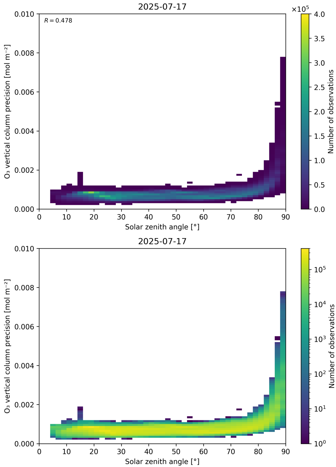
Figure 48: Scatter density plot of “Solar zenith angle” against “O 3 vertical column precision” for 2025-07-16 to 2025-07-18.
