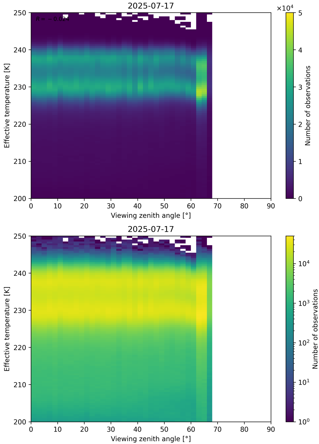
Figure 50: Scatter density plot of “Viewing zenith angle” against “Effective temperature” for 2025-07-16 to 2025-07-18.
