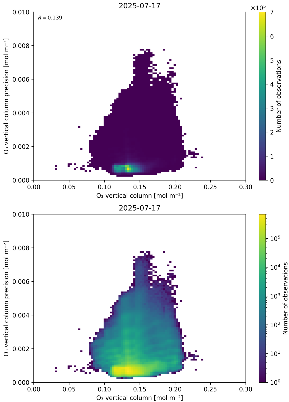
Figure 41: Scatter density plot of “O 3 vertical column” against “O 3 vertical column precision” for 2025-07-16 to 2025-07-18.
