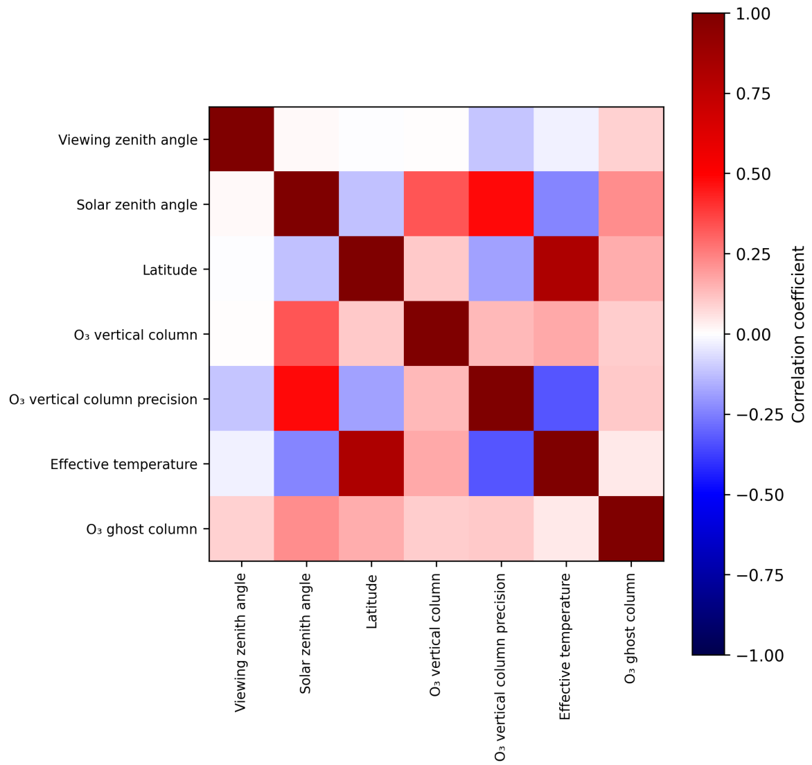
Figure 2: Map of correlation matrix for 2025-07-16 to 2025-07-18.
