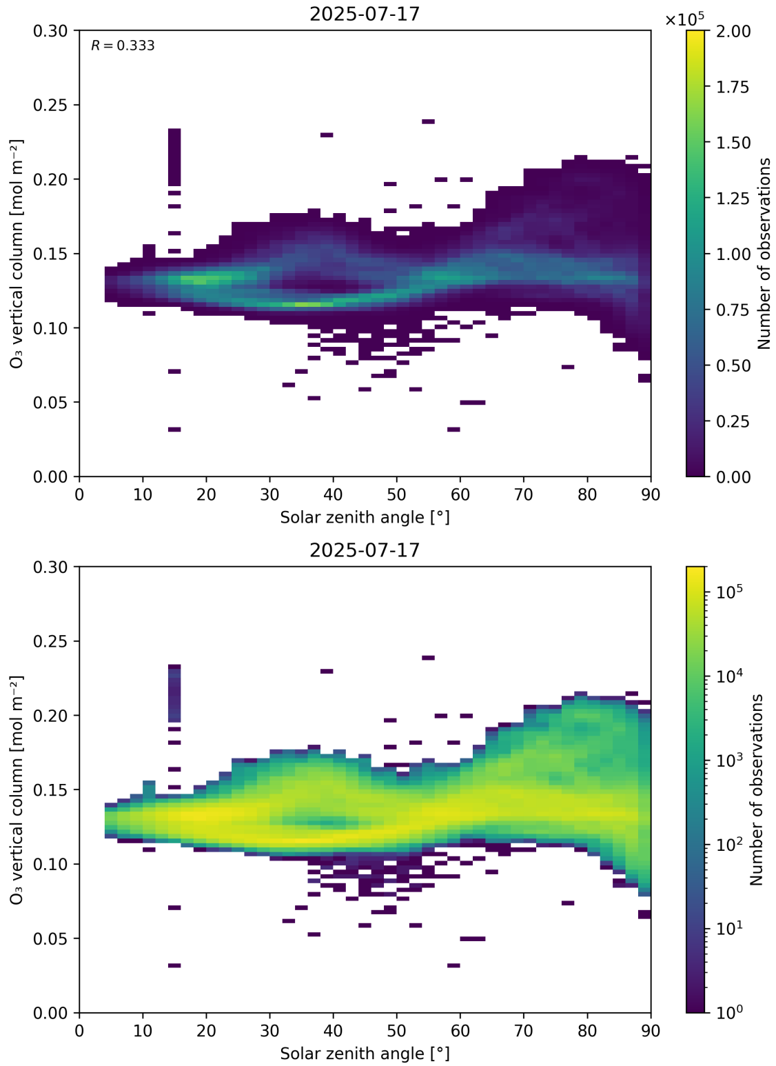
Figure 47: Scatter density plot of “Solar zenith angle” against “O 3 vertical column” for 2025-07-16 to 2025-07-18.
