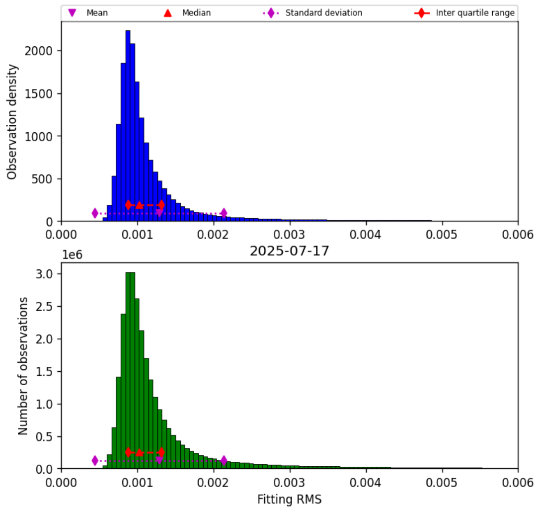
Figure 23: Histogram of “Fitting RMS” for 2025-07-16 to 2025-07-18
