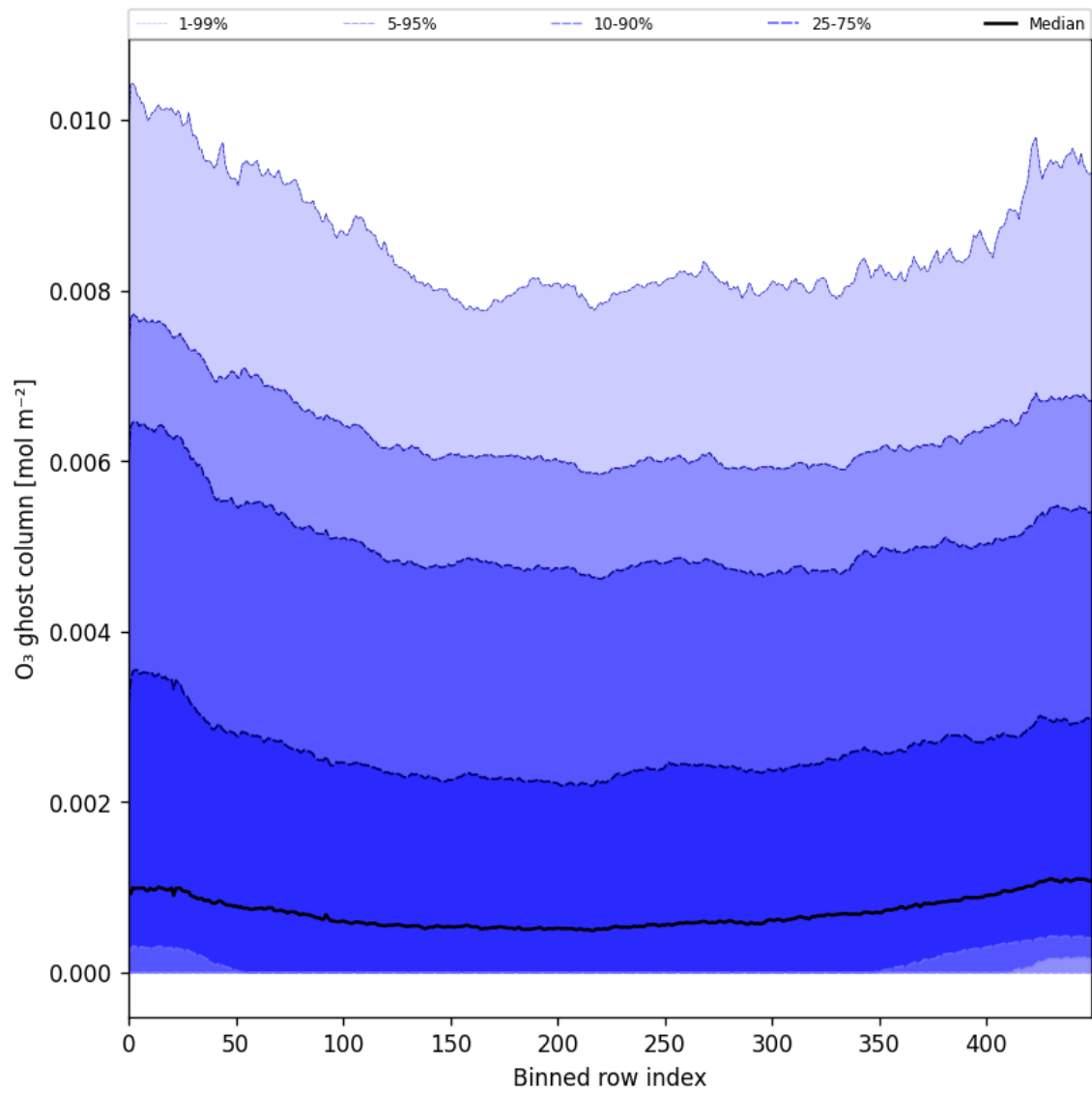
Figure 32: Along track statistics of “O 3 ghost column” for 2025-07-16 to 2025-07-18
