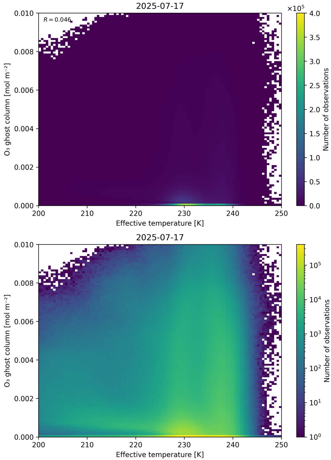
Figure 38: Scatter density plot of “Effective temperature” against “O 3 ghost column” for 2025-07-16 to 2025-07-18.
