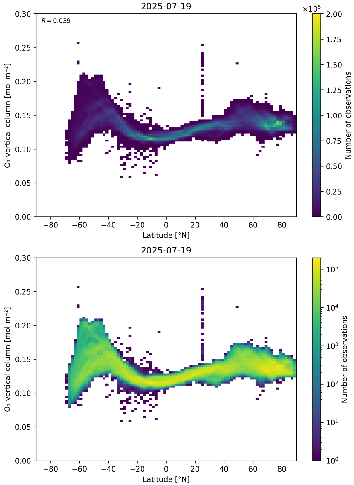
Figure 36: Scatter density plot of “Latitude” against “O 3 vertical column” for 2025-07-19 to 2025-07-20.
