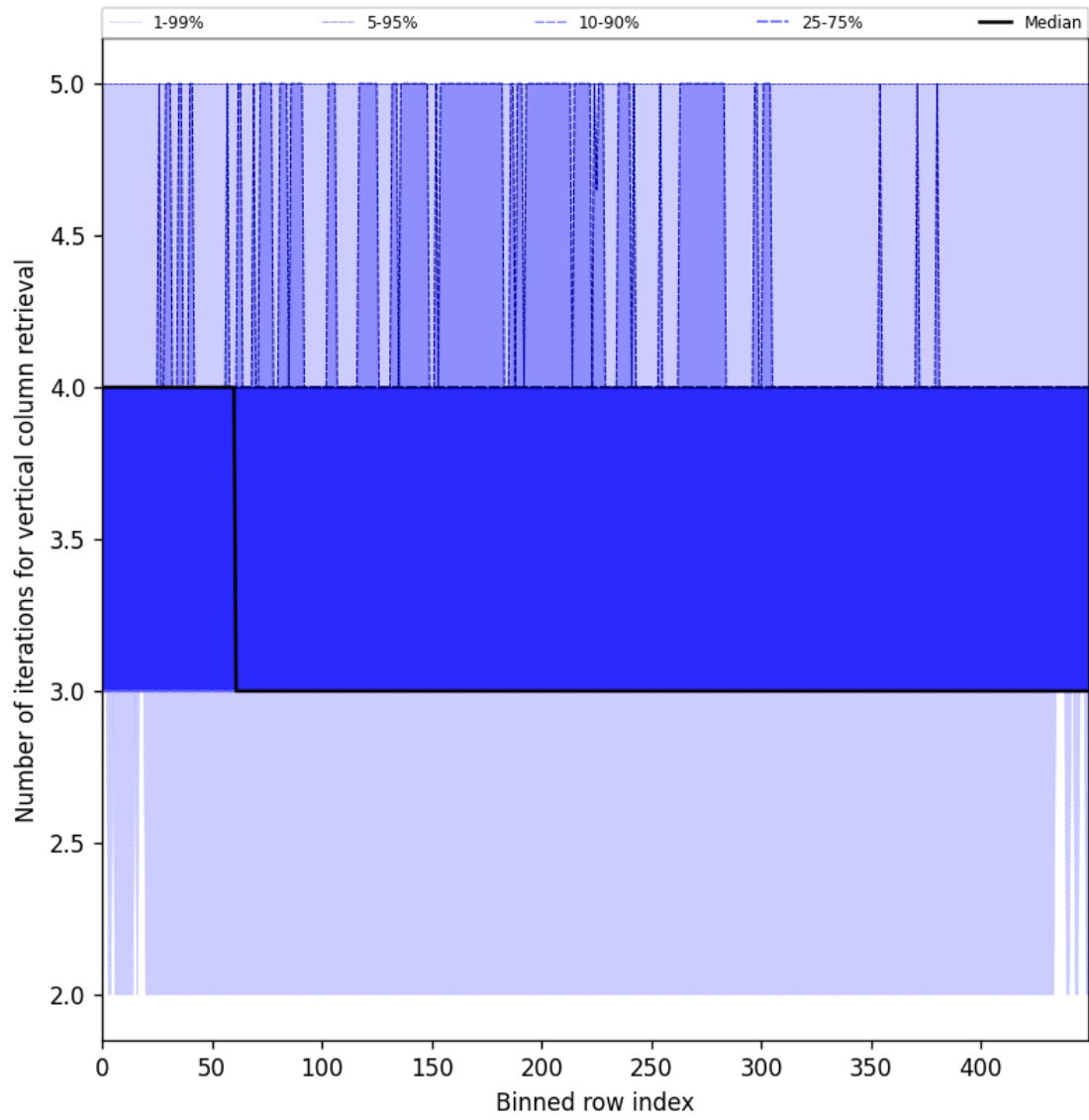
Figure 33: Along track statistics of “Number of iterations for vertical column retrieval” for 2025-07-19 to 2025-07-20
