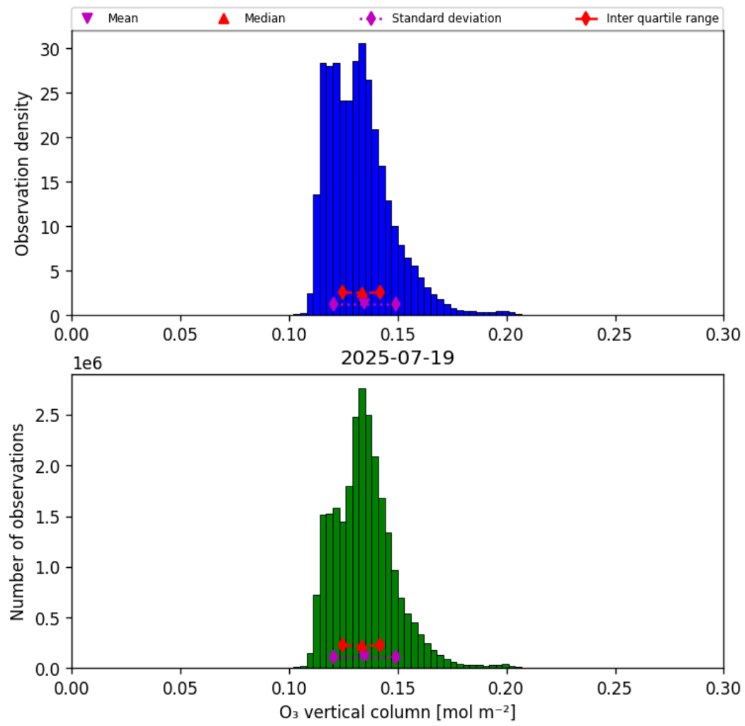
Figure 21: Histogram of “O 3 vertical column” for 2025-07-19 to 2025-07-20
