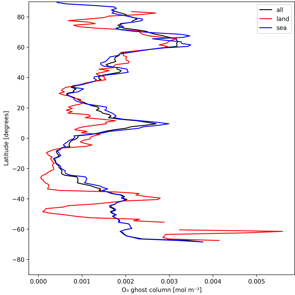
Figure 18: Zonal average of “O 3 ghost column” for 2025-07-19 to 2025-07-20.
