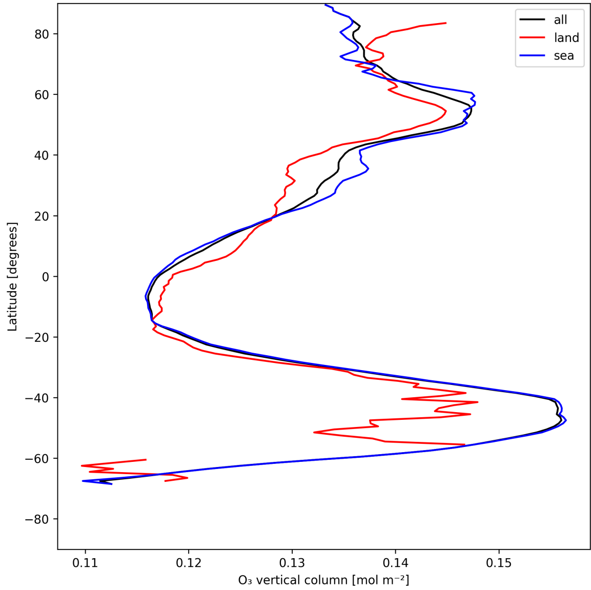
Figure 14: Zonal average of “O 3 vertical column” for 2025-07-19 to 2025-07-20.
