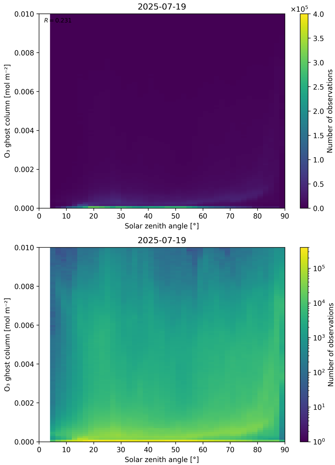
Figure 46: Scatter density plot of “Solar zenith angle” against “O 3 ghost column” for 2025-07-19 to 2025-07-20.
