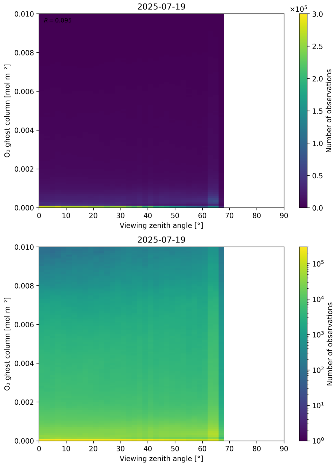
Figure 51: Scatter density plot of “Viewing zenith angle” against “O 3 ghost column” for 2025-07-19 to 2025-07-20.
