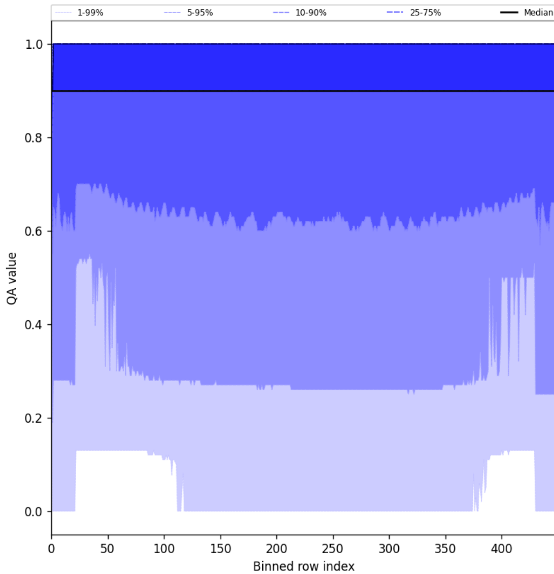
Figure 27: Along track statistics of “QA value” for 2025-07-19 to 2025-07-20
