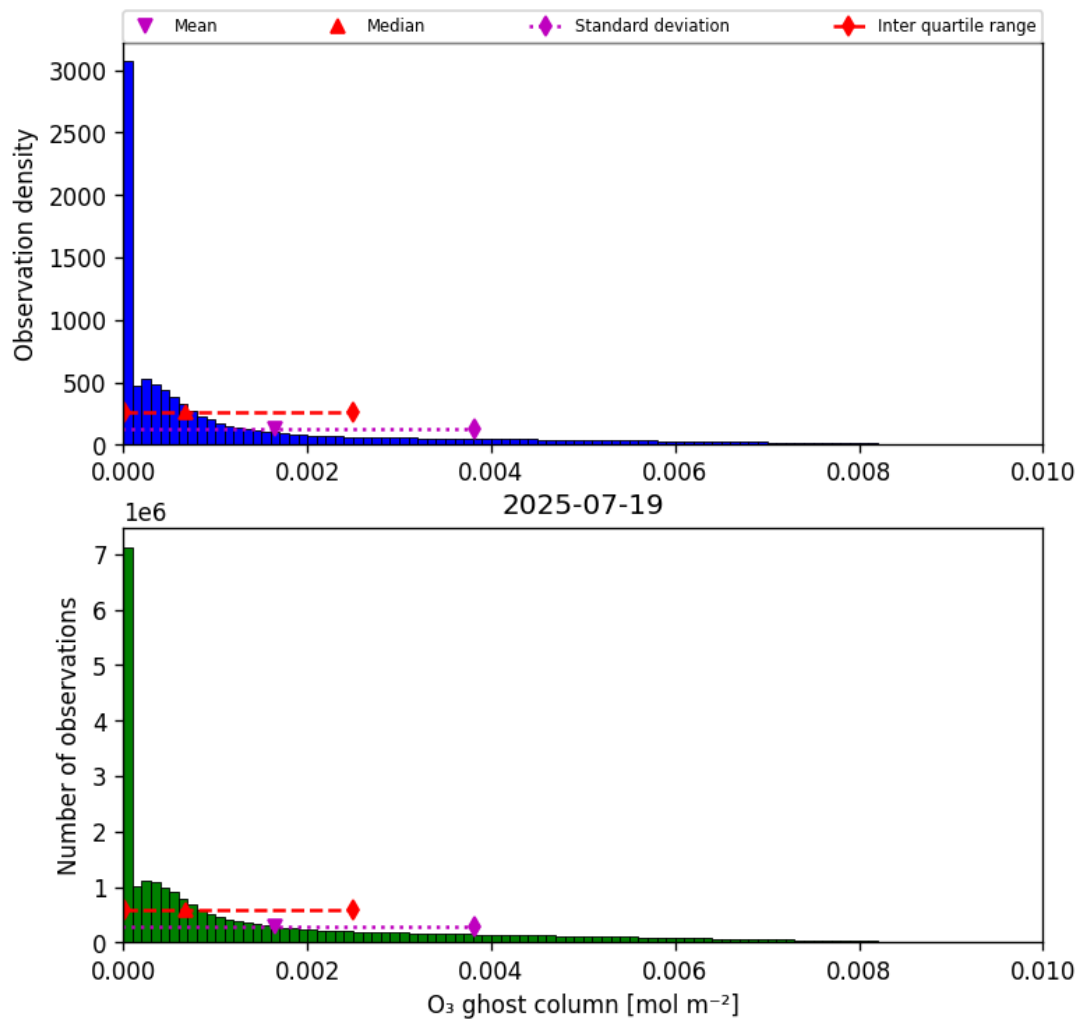
Figure 25: Histogram of “O 3 ghost column” for 2025-07-19 to 2025-07-20
