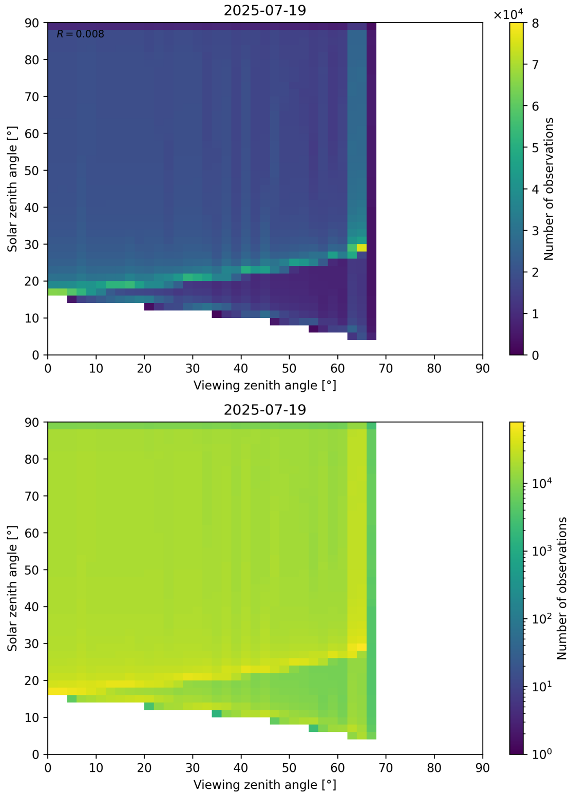
Figure 54: Scatter density plot of “Viewing zenith angle” against “Solar zenith angle” for 2025-07-19 to 2025-07-20.
