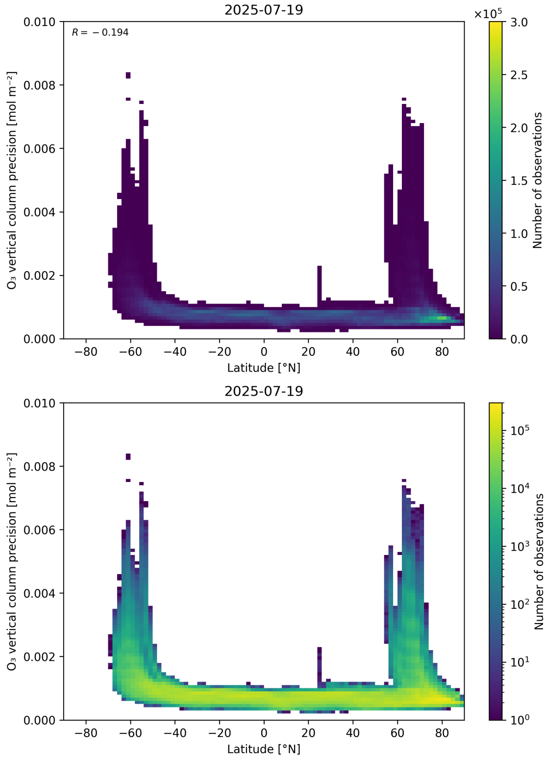
Figure 37: Scatter density plot of “Latitude” against “O 3 vertical column precision” for 2025-07-19 to 2025-07-20.
