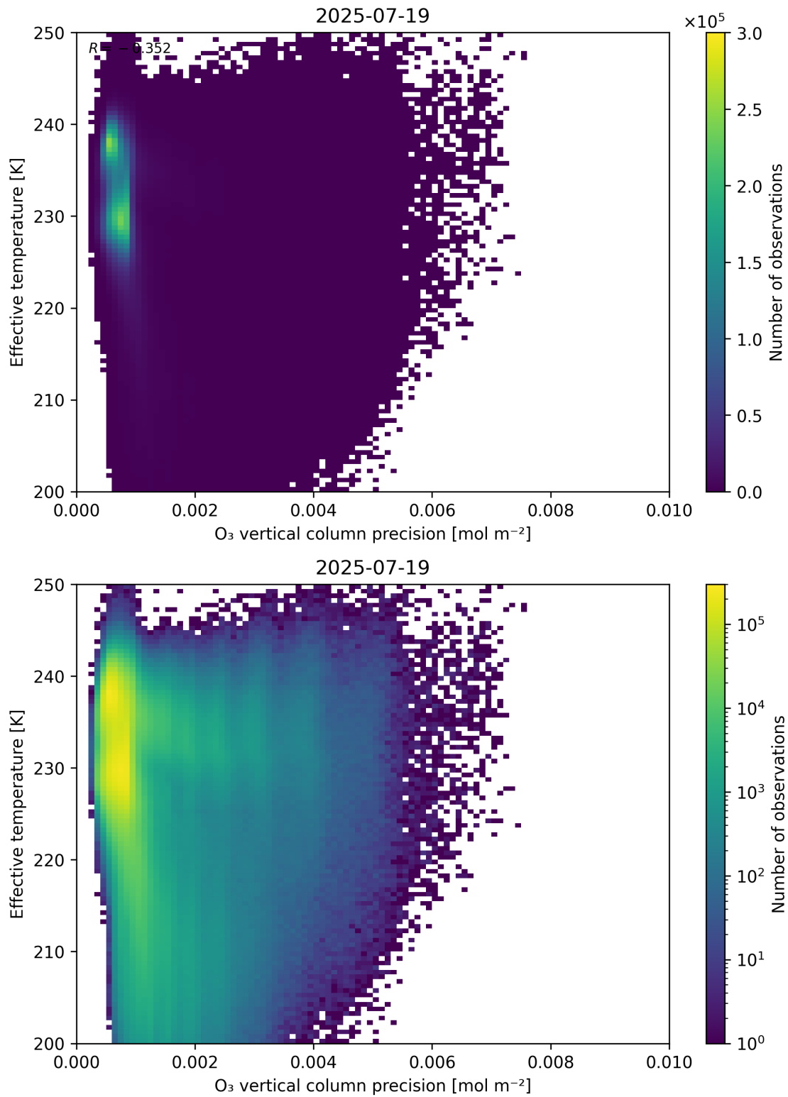
Figure 42: Scatter density plot of “ O_3 vertical column precision” against “Effective temperature” for 2025-07-19 to 2025-07-20.
