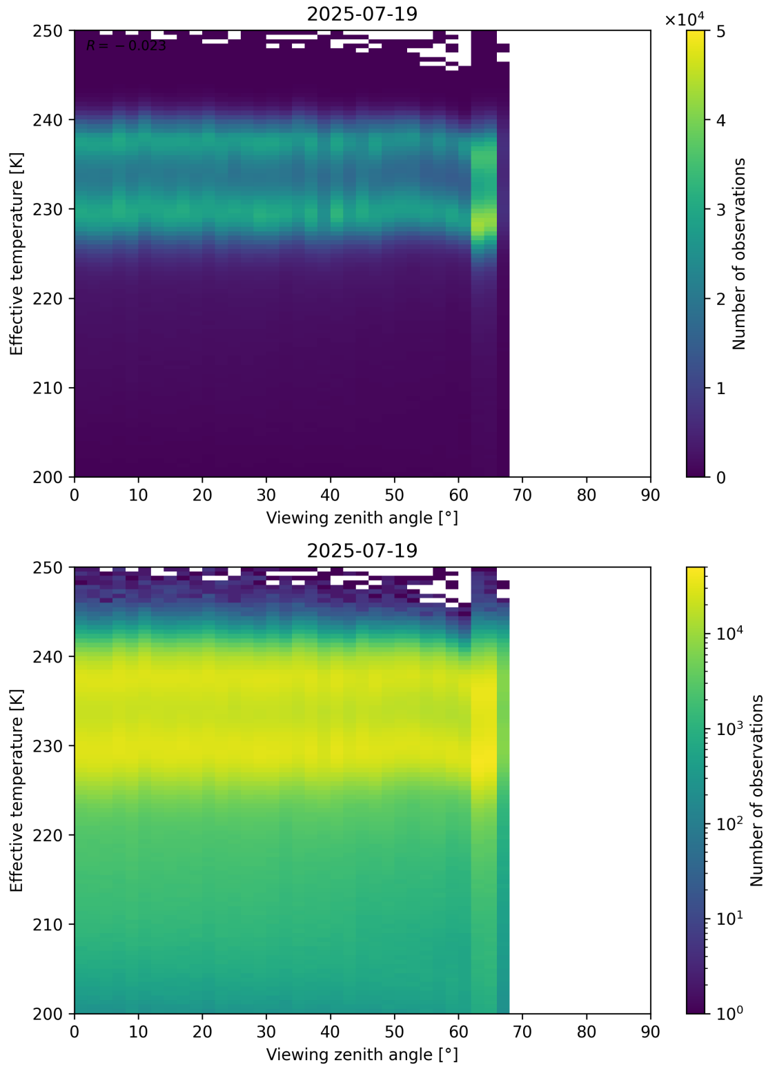
Figure 50: Scatter density plot of “Viewing zenith angle” against “Effective temperature” for 2025-07-19 to 2025-07-20.
