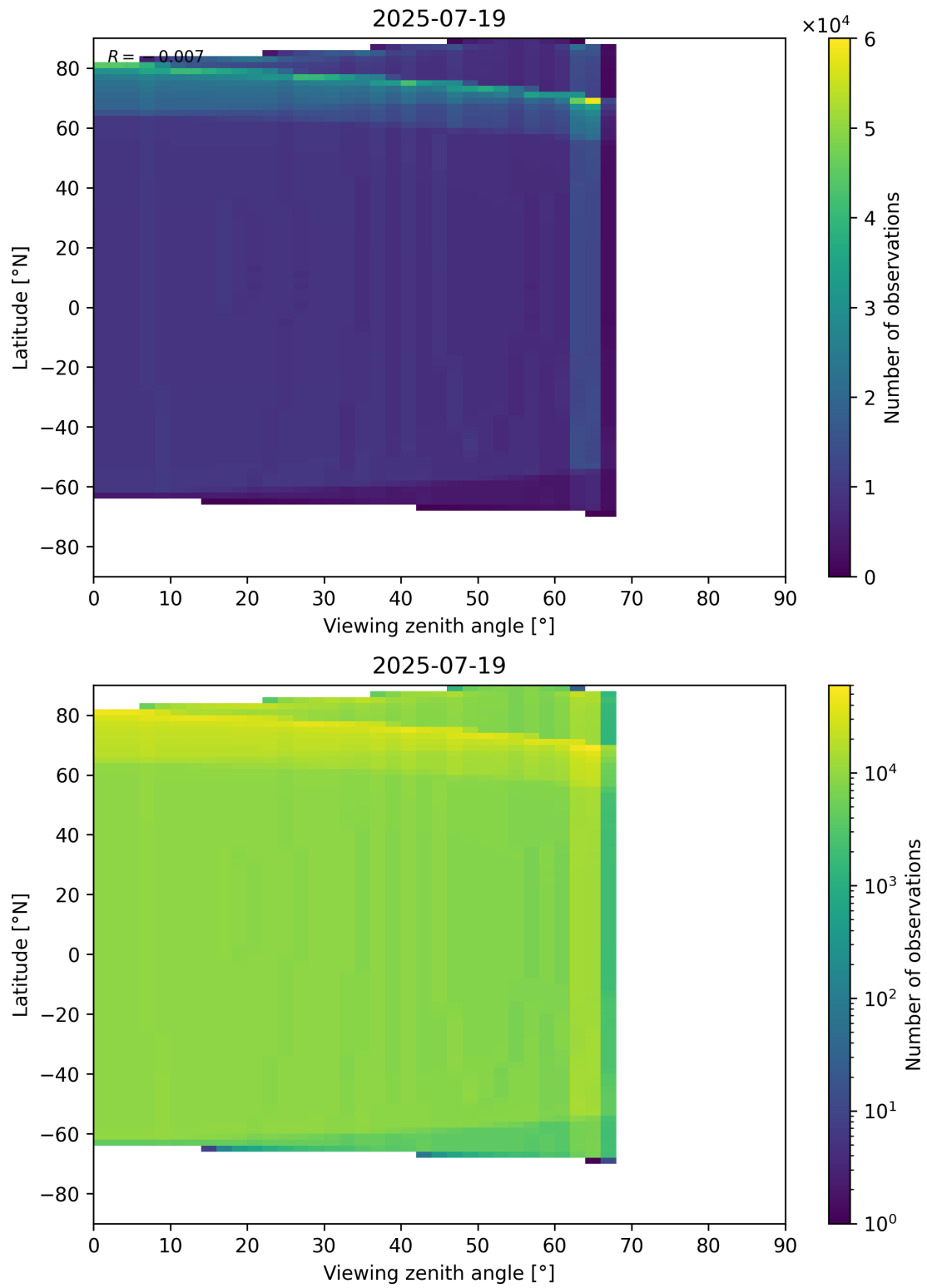
Figure 49: Scatter density plot of “Viewing zenith angle” against “Latitude” for 2025-07-19 to 2025-07-20.
