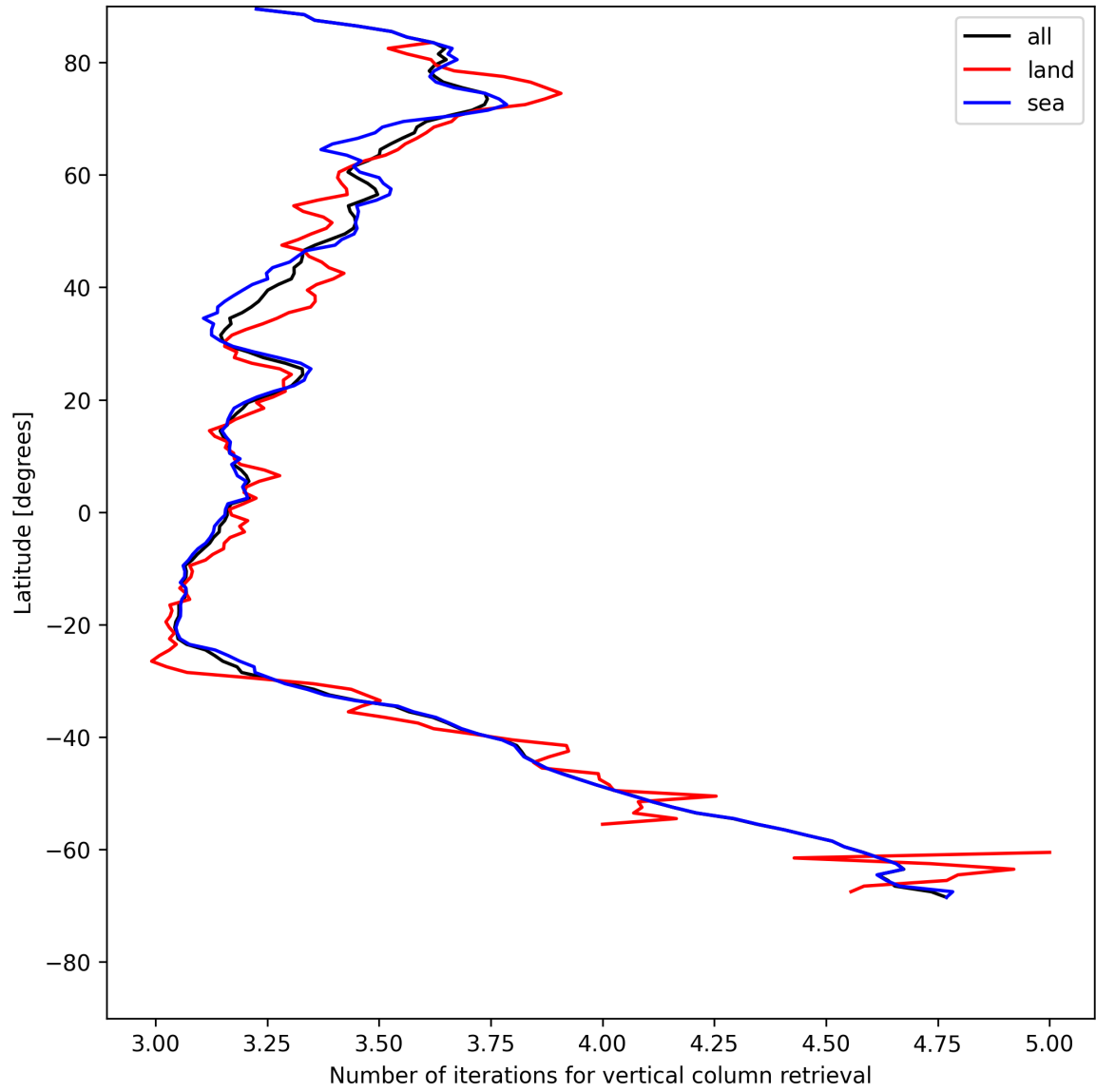
Figure 19: Zonal average of “Number of iterations for vertical column retrieval” for 2025-07-19 to 2025-07-20.
