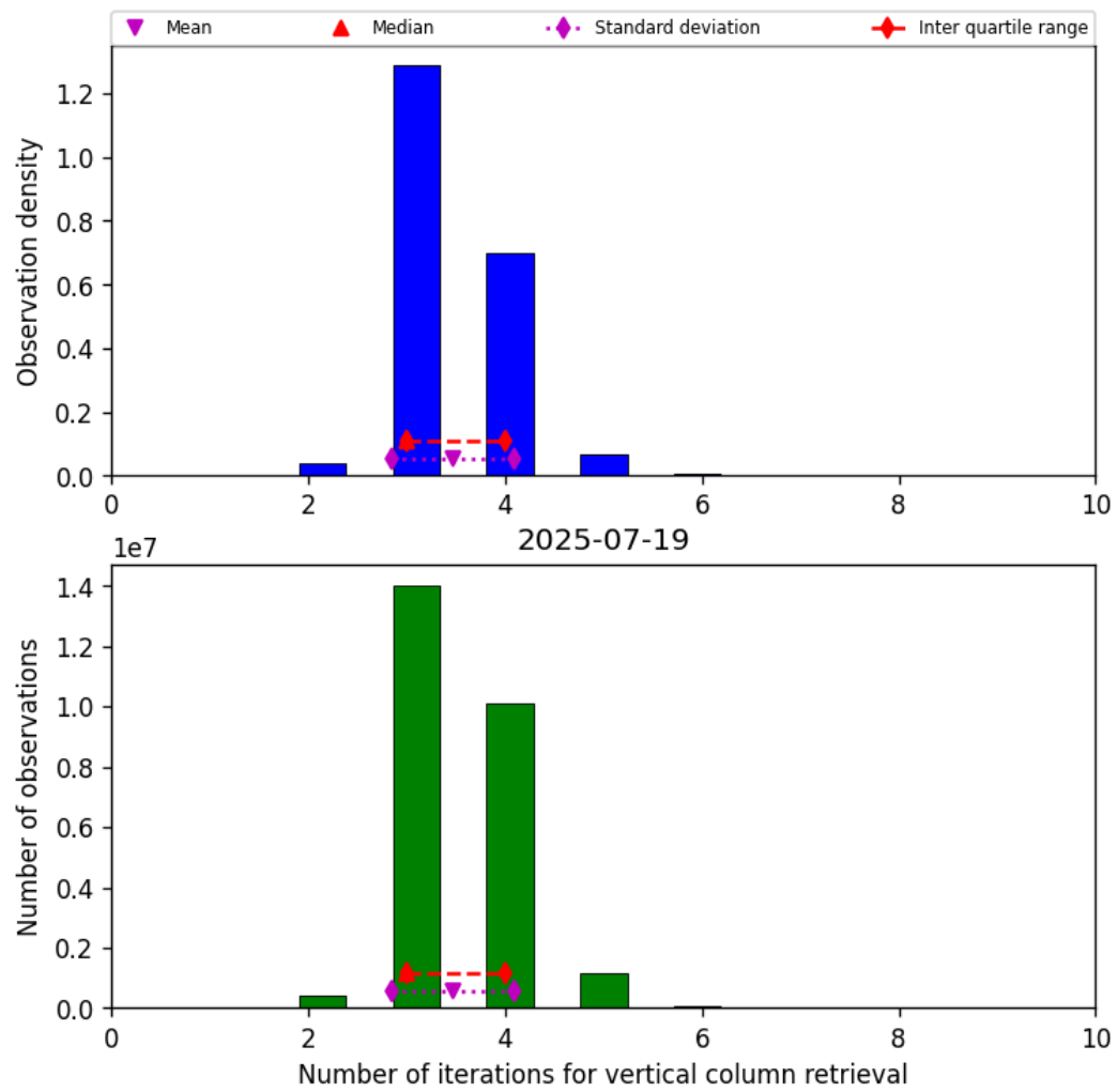
Figure 26: Histogram of “Number of iterations for vertical column retrieval” for 2025-07-19 to 2025-07-20
