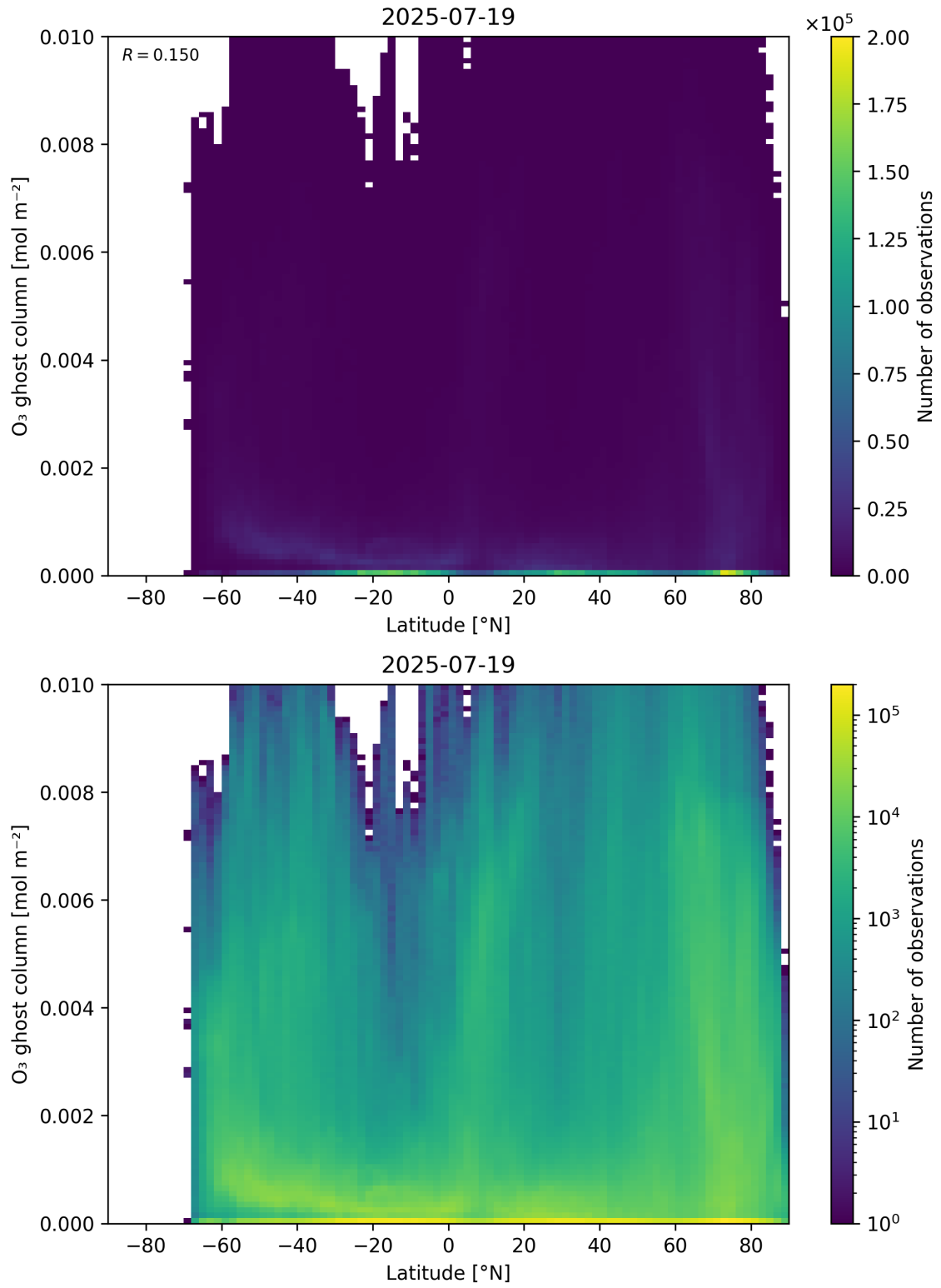
Figure 35: Scatter density plot of “Latitude” against “O 3 ghost column” for 2025-07-19 to 2025-07-20.
