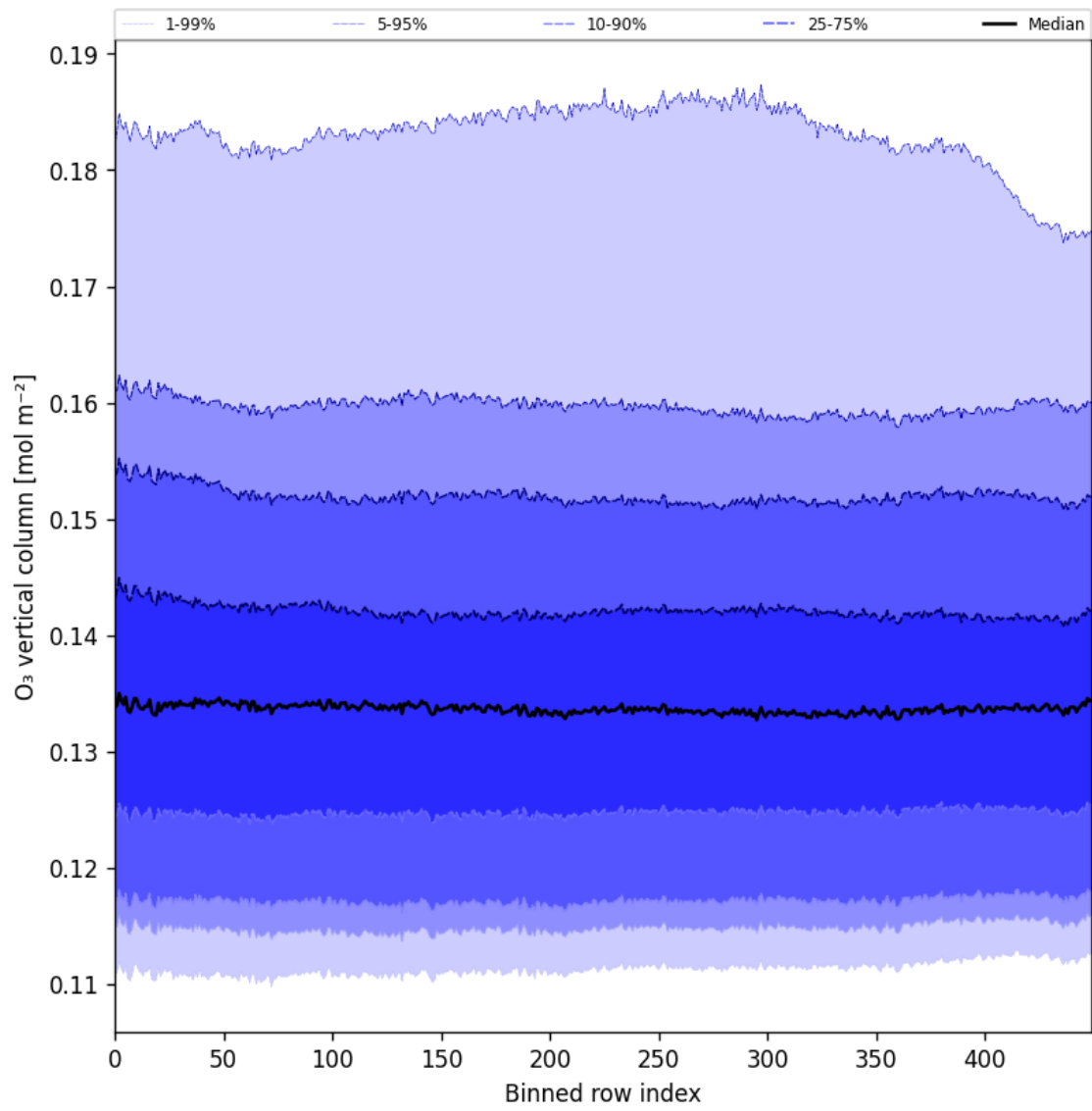
Figure 28: Along track statistics of “O 3 vertical column” for 2025-07-19 to 2025-07-20
