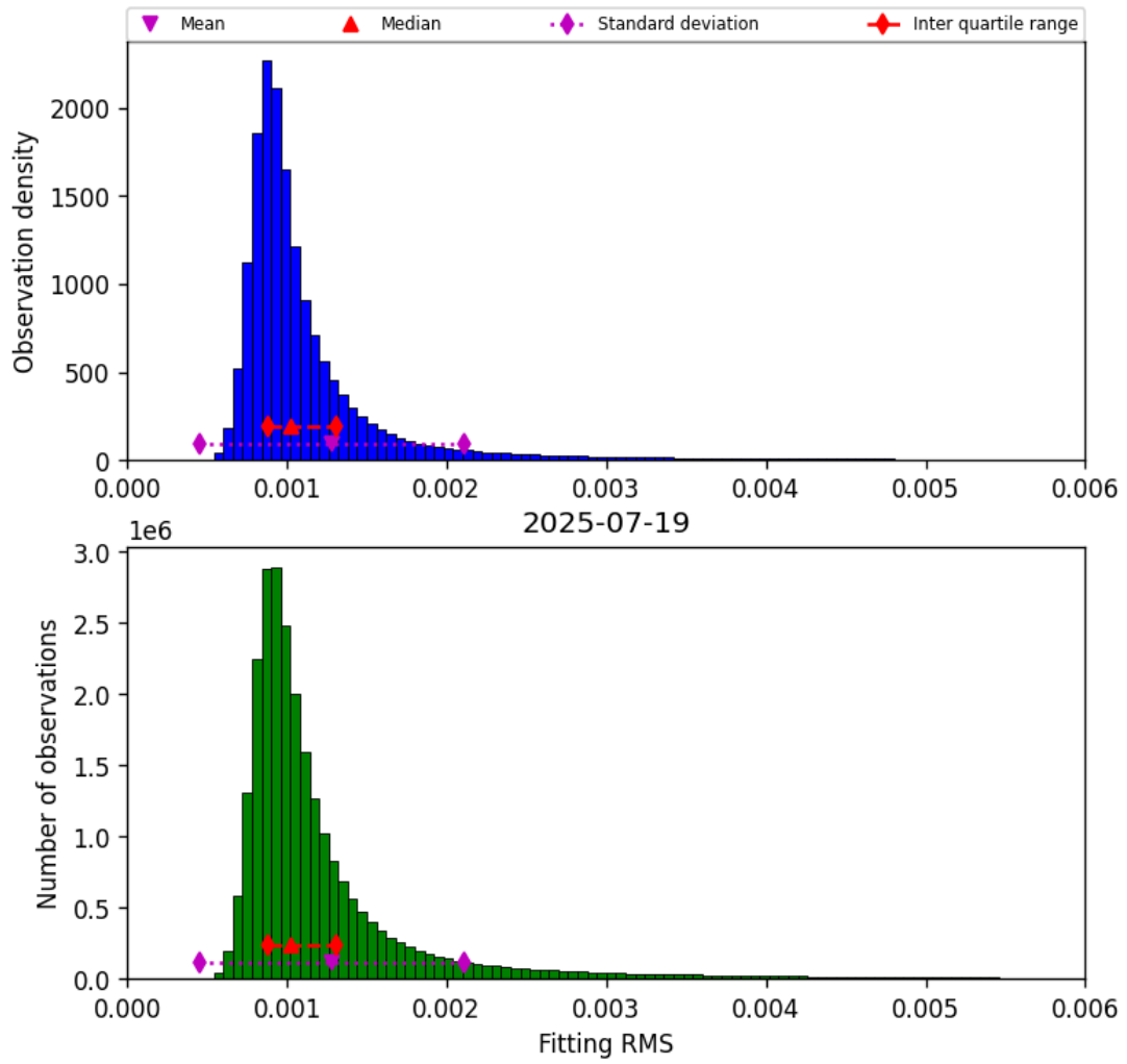
Figure 23: Histogram of “Fitting RMS” for 2025-07-19 to 2025-07-20
