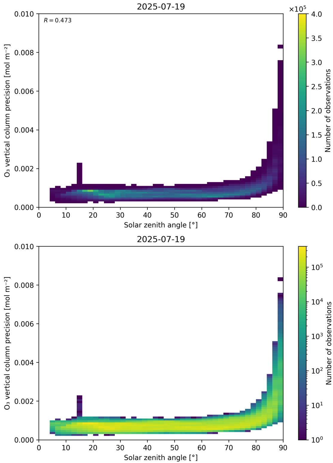
Figure 48: Scatter density plot of “Solar zenith angle” against “O 3 vertical column precision” for 2025-07-19 to 2025-07-20.
