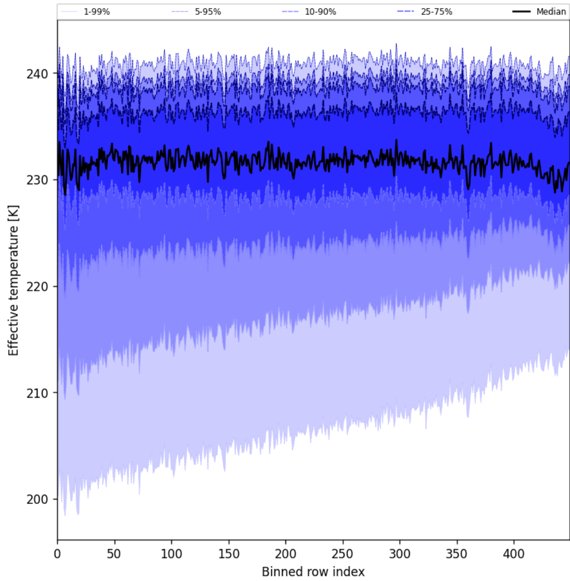
Figure 31: Along track statistics of “Effective temperature” for 2025-07-19 to 2025-07-20
