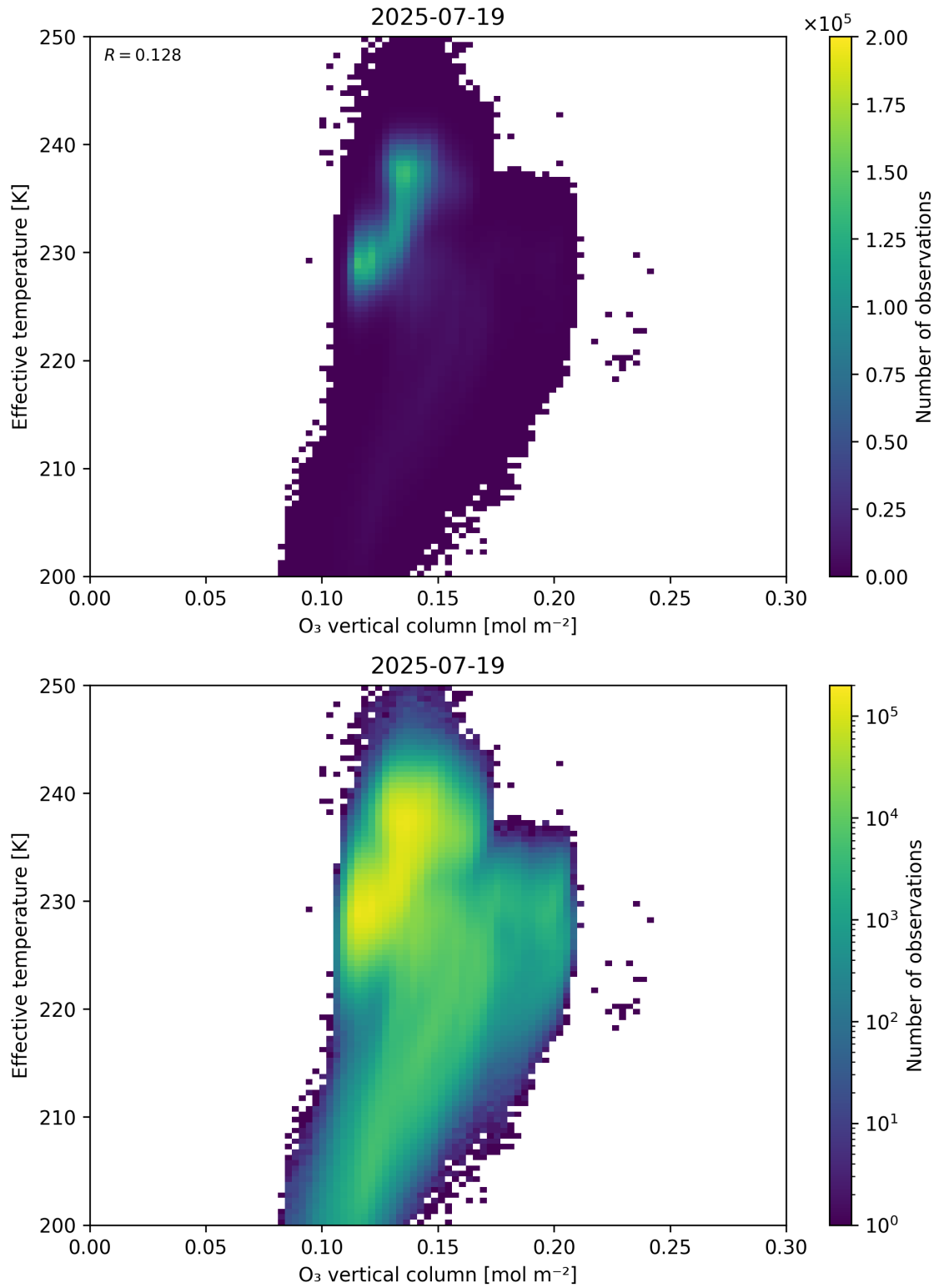
Figure 39: Scatter density plot of “O 3 vertical column” against “Effective temperature” for 2025-07-19 to 2025-07-20.
