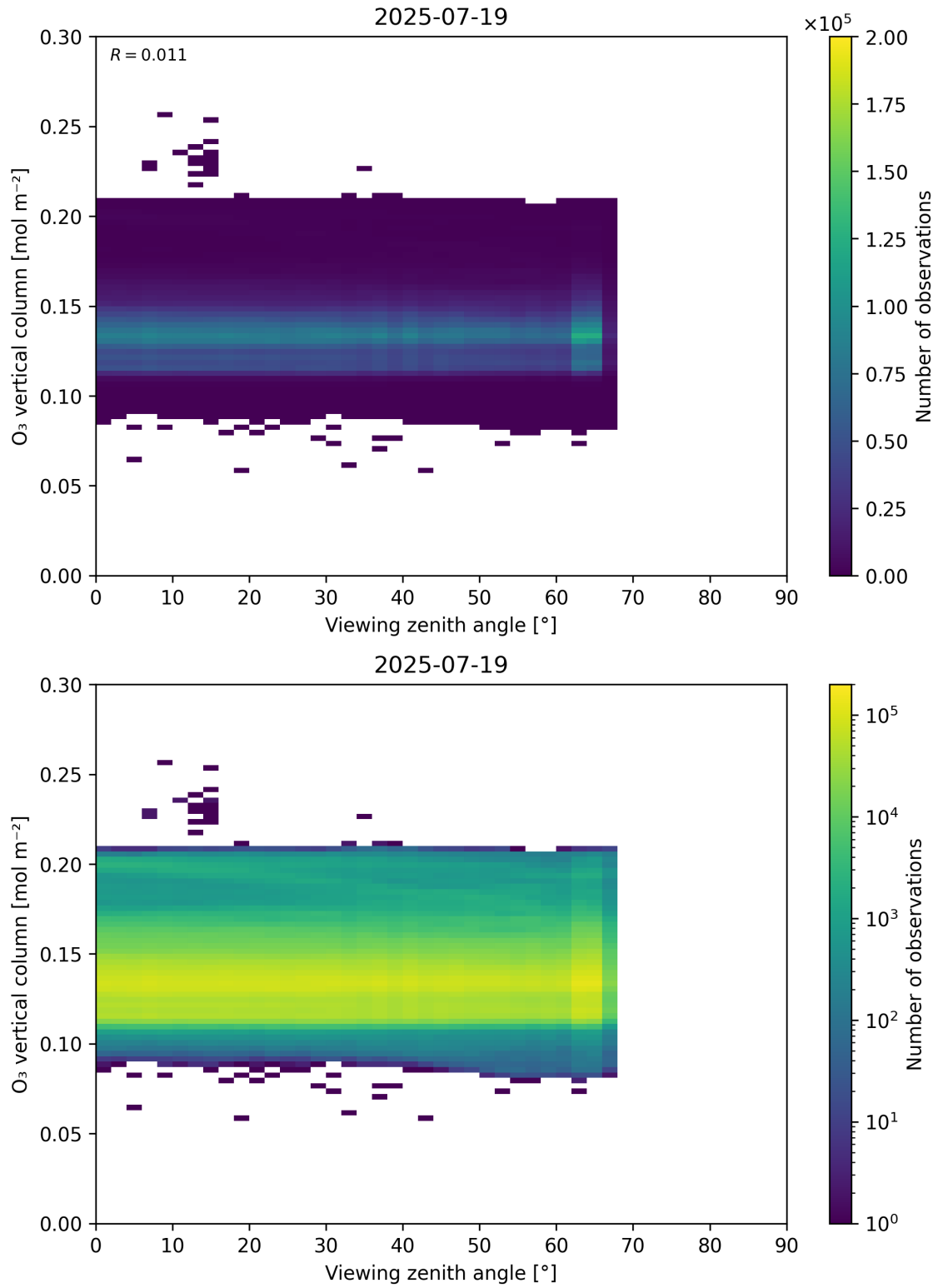
Figure 52: Scatter density plot of “Viewing zenith angle” against “O 3 vertical column” for 2025-07-19 to 2025-07-20.
