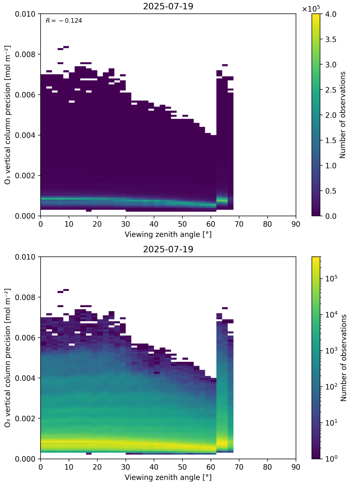
Figure 53: Scatter density plot of “Viewing zenith angle” against “O 3 vertical column precision” for 2025-07-19 to 2025-07-20.
