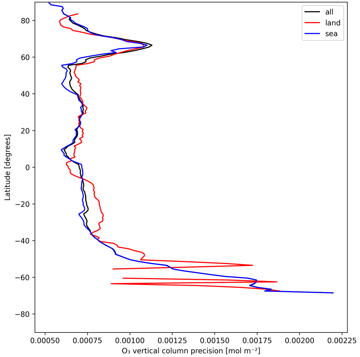
Figure 15: Zonal average of "O 3 vertical column precision" for 2025-07-19 to 2025-07-20.
