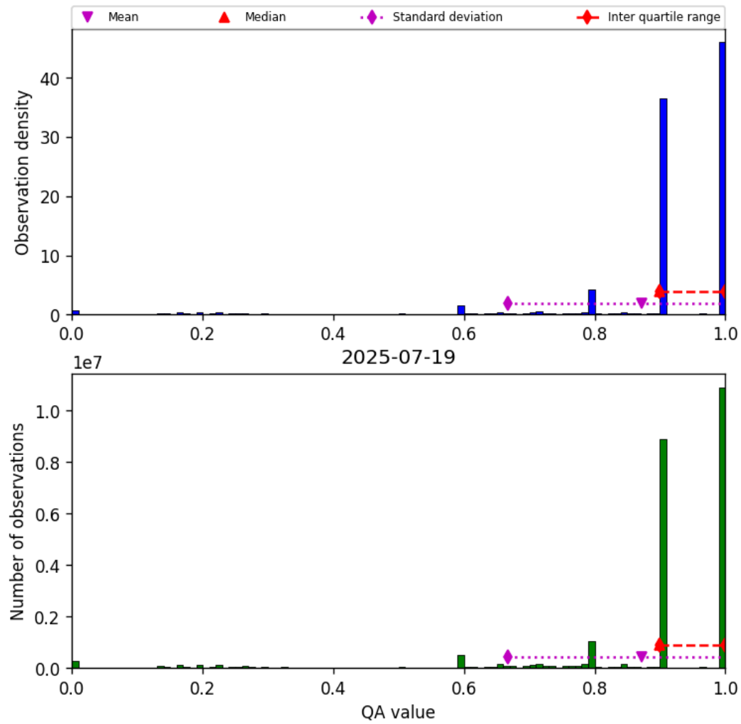
Figure 20: Histogram of “QA value” for 2025-07-19 to 2025-07-20
