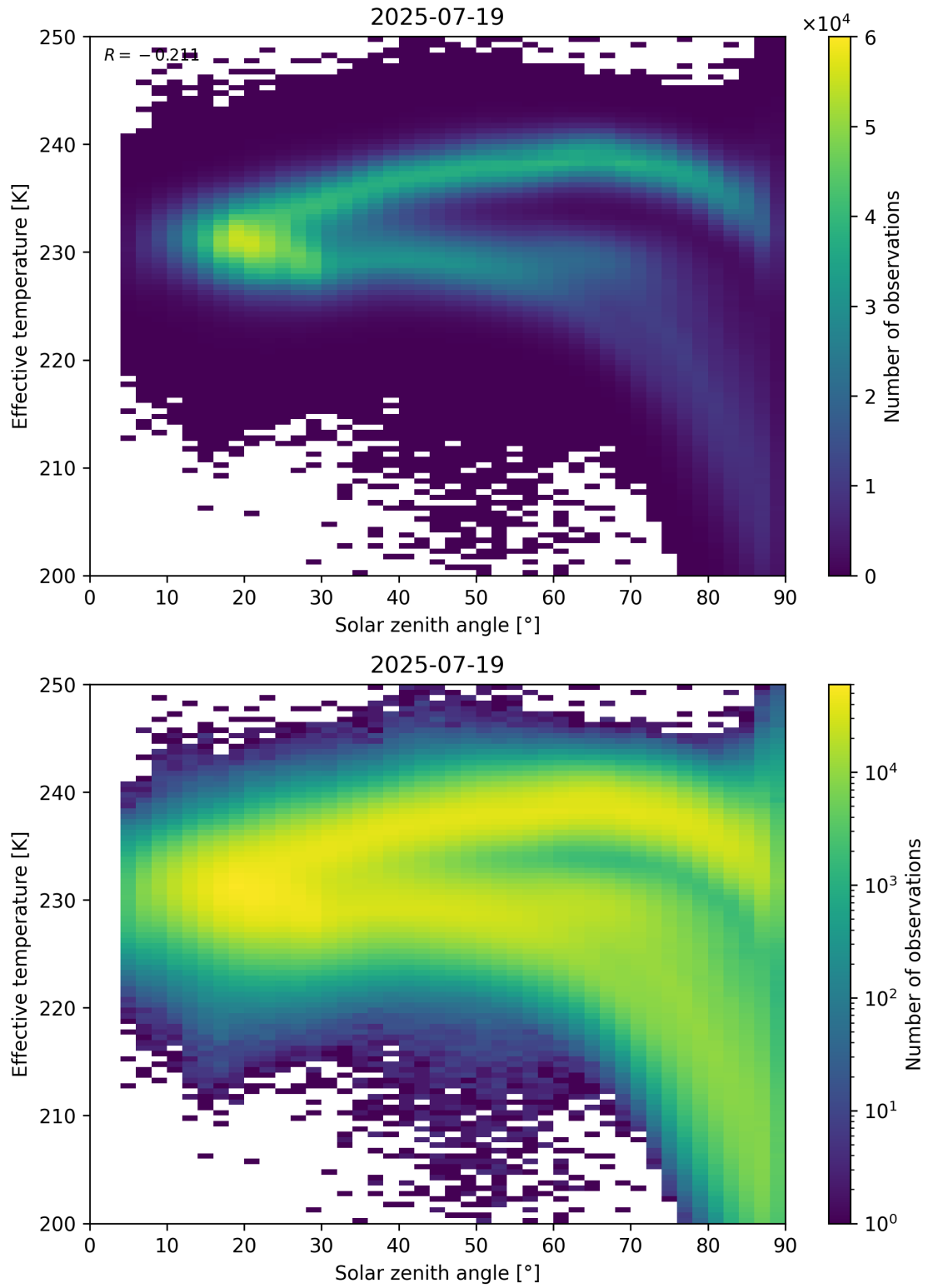
Figure 45: Scatter density plot of “Solar zenith angle” against “Effective temperature” for 2025-07-19 to 2025-07-20.
