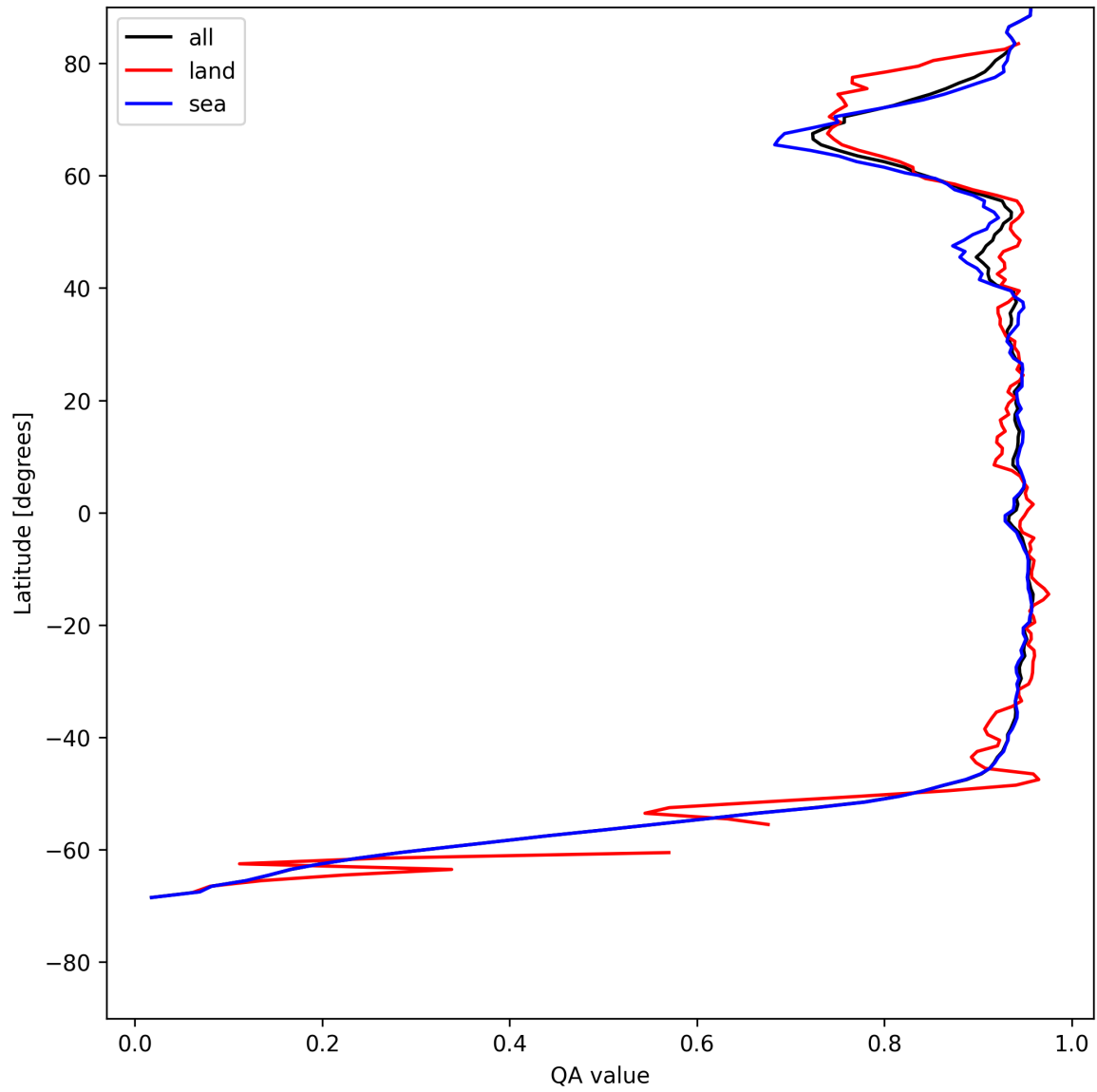
Figure 13: Zonal average of “QA value” for 2025-07-19 to 2025-07-20.
