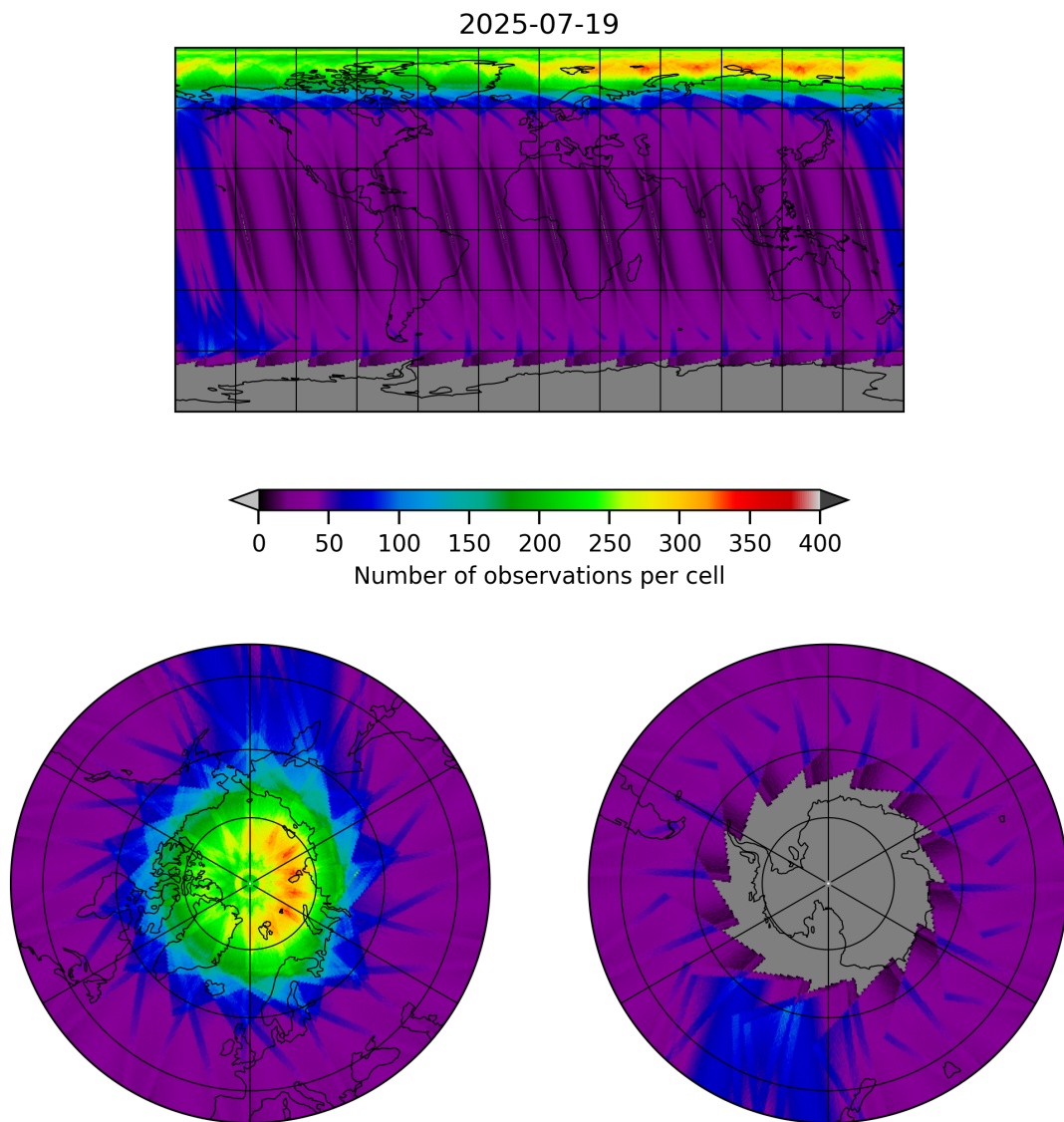
Figure 12: Map of the number of observations for 2025-07-19 to 2025-07-20
