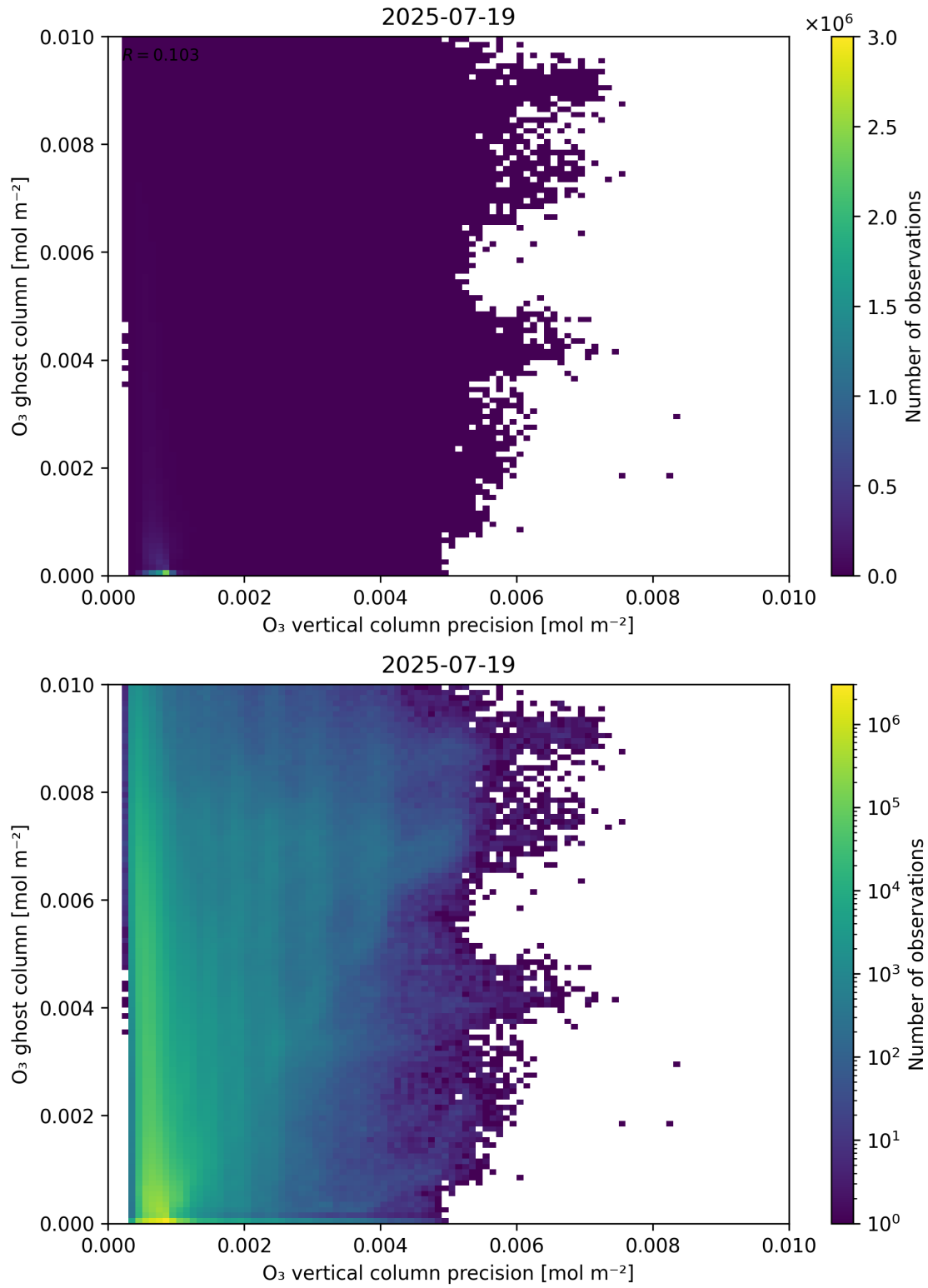
Figure 43: Scatter density plot of “O 3 vertical column precision” against “O 3 ghost column” for 2025-07-19 to 2025-07-20.
