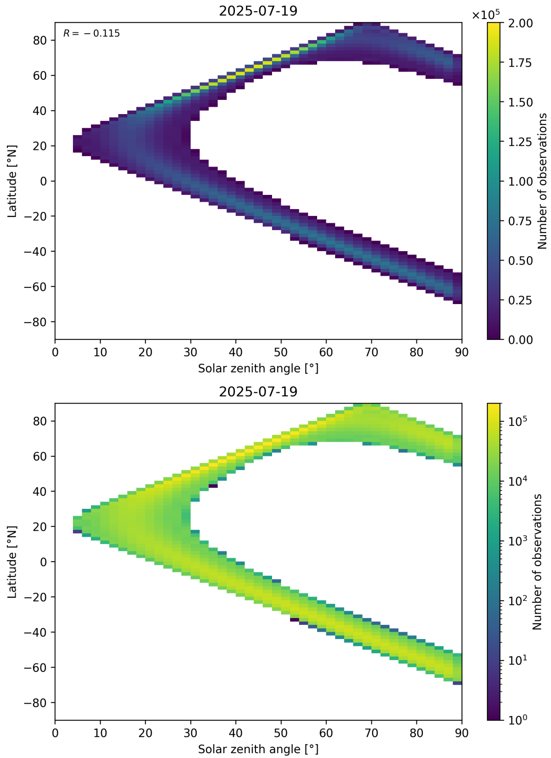
Figure 44: Scatter density plot of “Solar zenith angle” against “Latitude” for 2025-07-19 to 2025-07-20.
