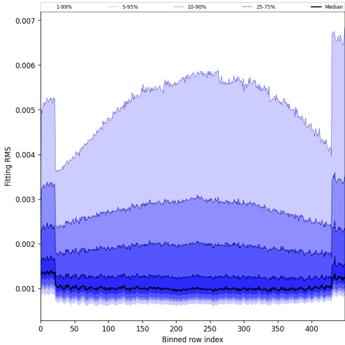
Figure 30: Along track statistics of “Fitting RMS” for 2025-07-19 to 2025-07-20
