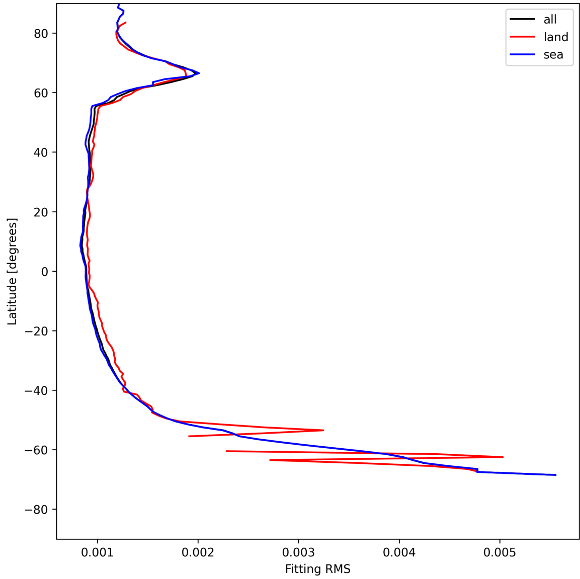
Figure 16: Zonal average of “Fitting RMS” for 2025-07-19 to 2025-07-20.
