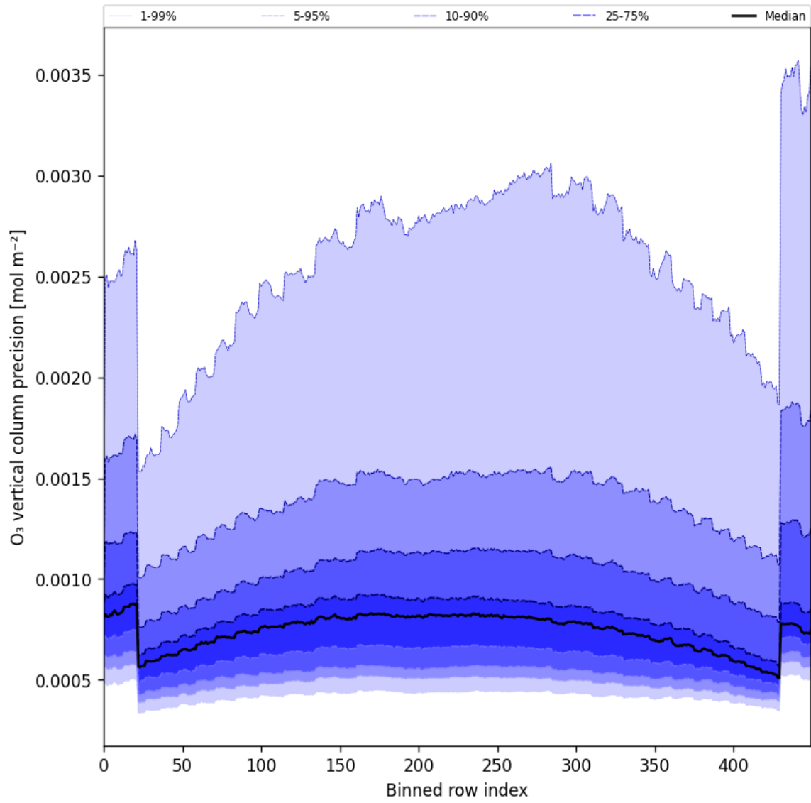
Figure 29: Along track statistics of “O 3 vertical column precision” for 2025-07-19 to 2025-07-20
