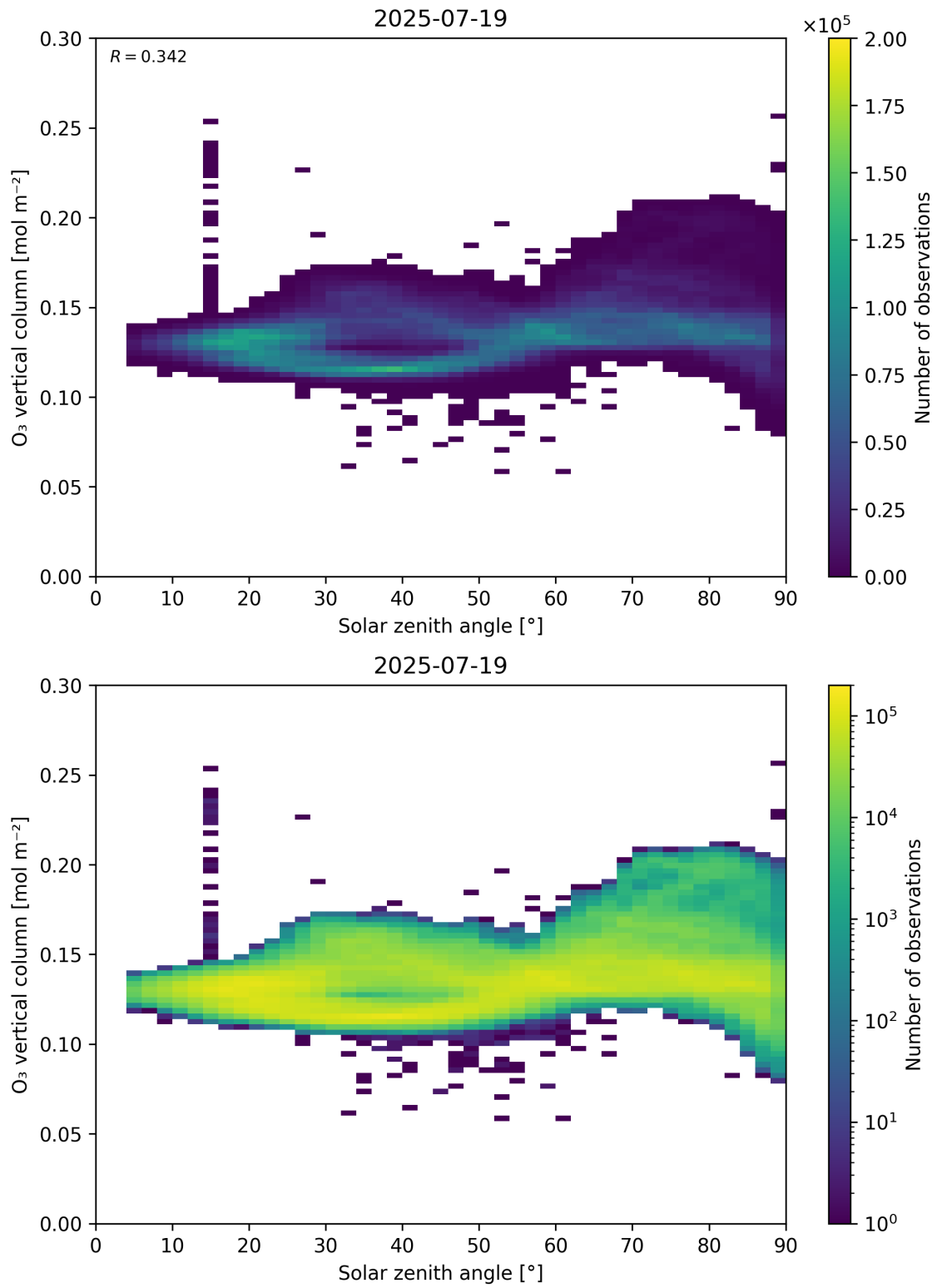
Figure 47: Scatter density plot of “Solar zenith angle” against “O 3 vertical column” for 2025-07-19 to 2025-07-20.
