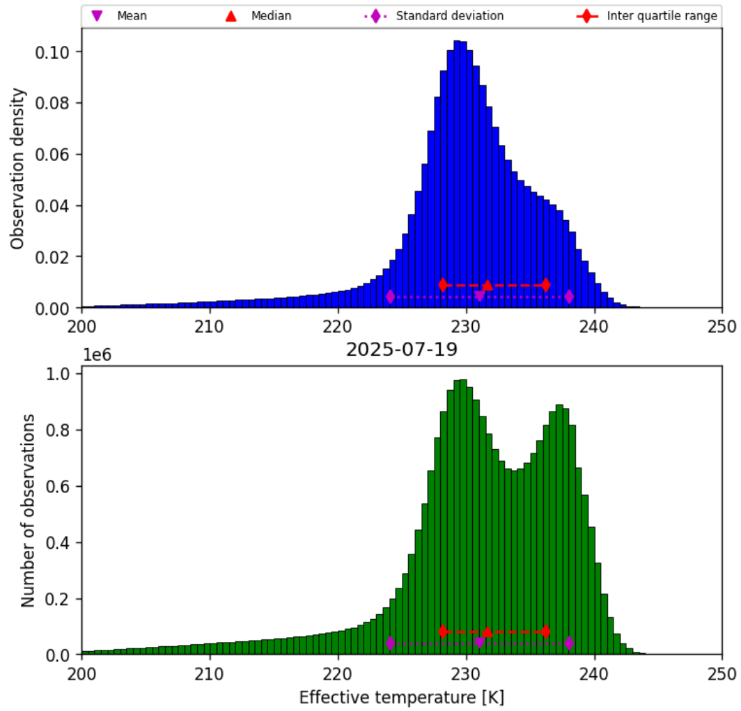
Figure 24: Histogram of “Effective temperature” for 2025-07-19 to 2025-07-20
