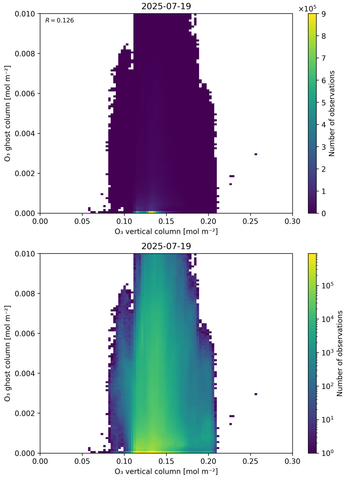
Figure 40: Scatter density plot of “O 3 vertical column” against “O 3 ghost column” for 2025-07-19 to 2025-07-20.
