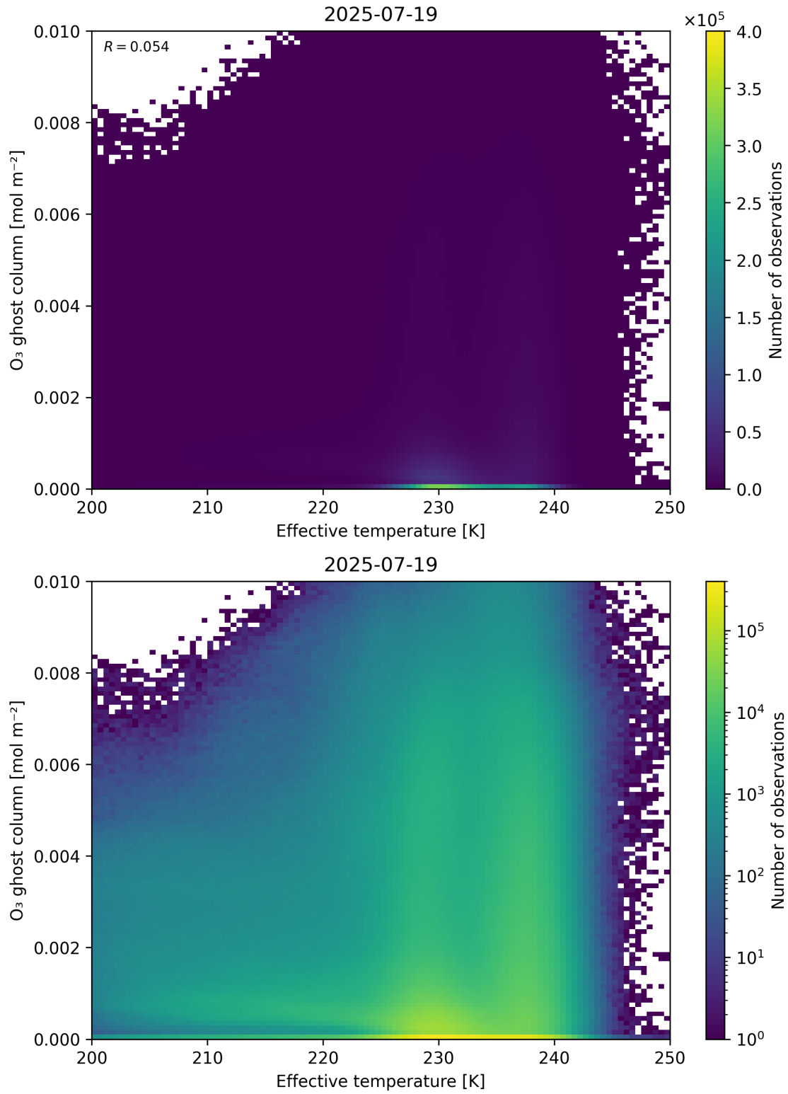
Figure 38: Scatter density plot of “Effective temperature” against “O 3 ghost column” for 2025-07-19 to 2025-07-20.
