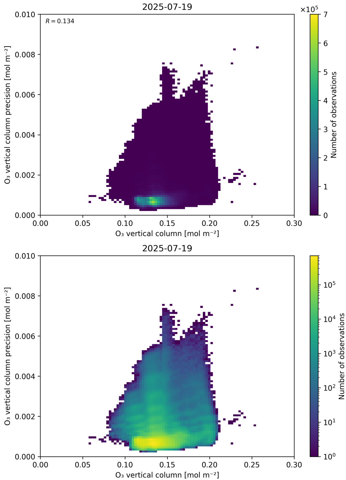
Figure 41: Scatter density plot of “O 3 vertical column” against “O 3 vertical column precision” for 2025-07-19 to 2025-07-20.
