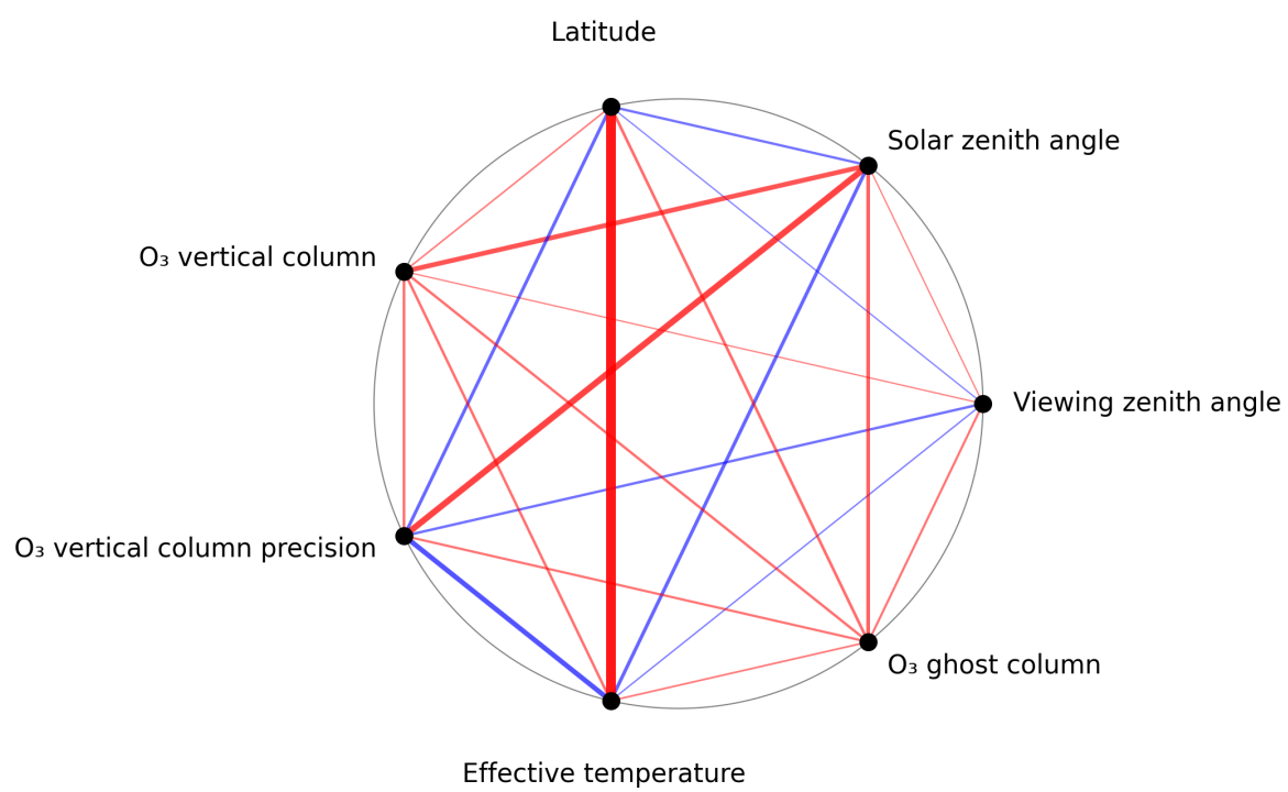
Figure 1: Map of correlation graph for 2025-07-19 to 2025-07-20.
