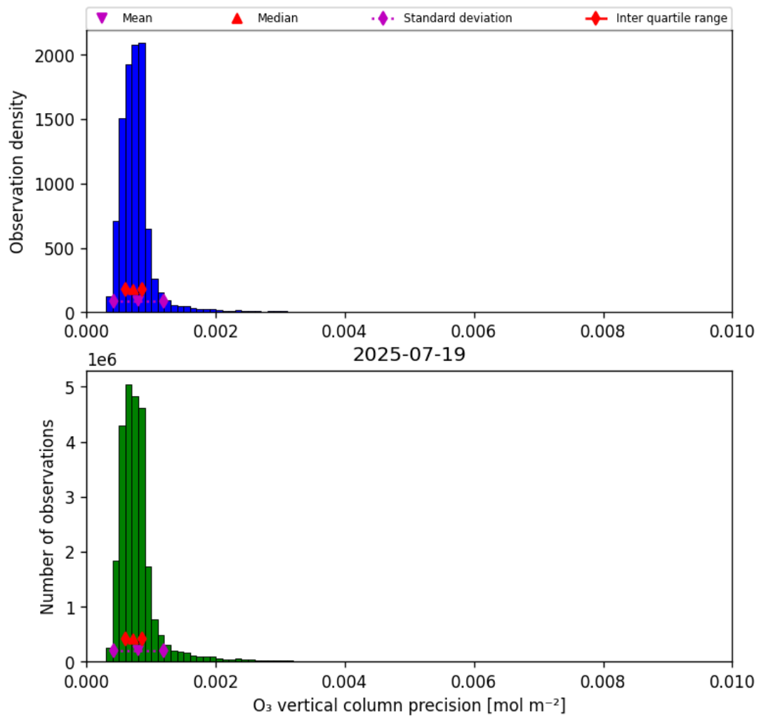
Figure 22: Histogram of “O 3 vertical column precision” for 2025-07-19 to 2025-07-20
