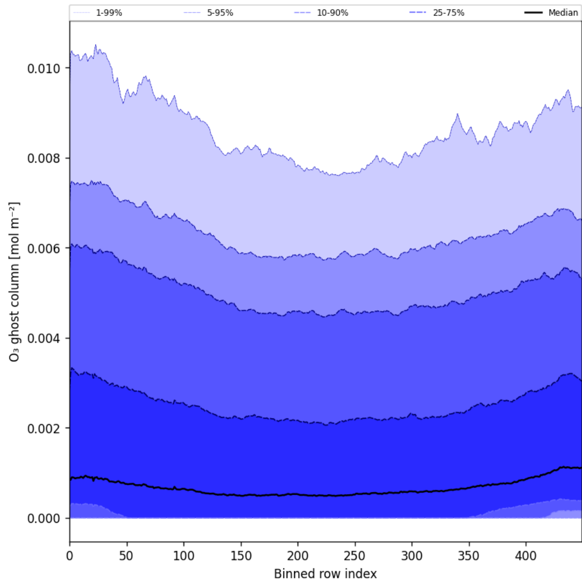
Figure 32: Along track statistics of “O 3 ghost column” for 2025-07-19 to 2025-07-20
