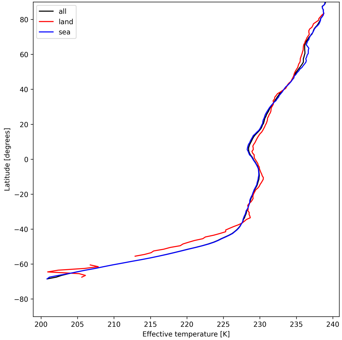
Figure 17: Zonal average of “Effective temperature” for 2025-07-19 to 2025-07-20.
