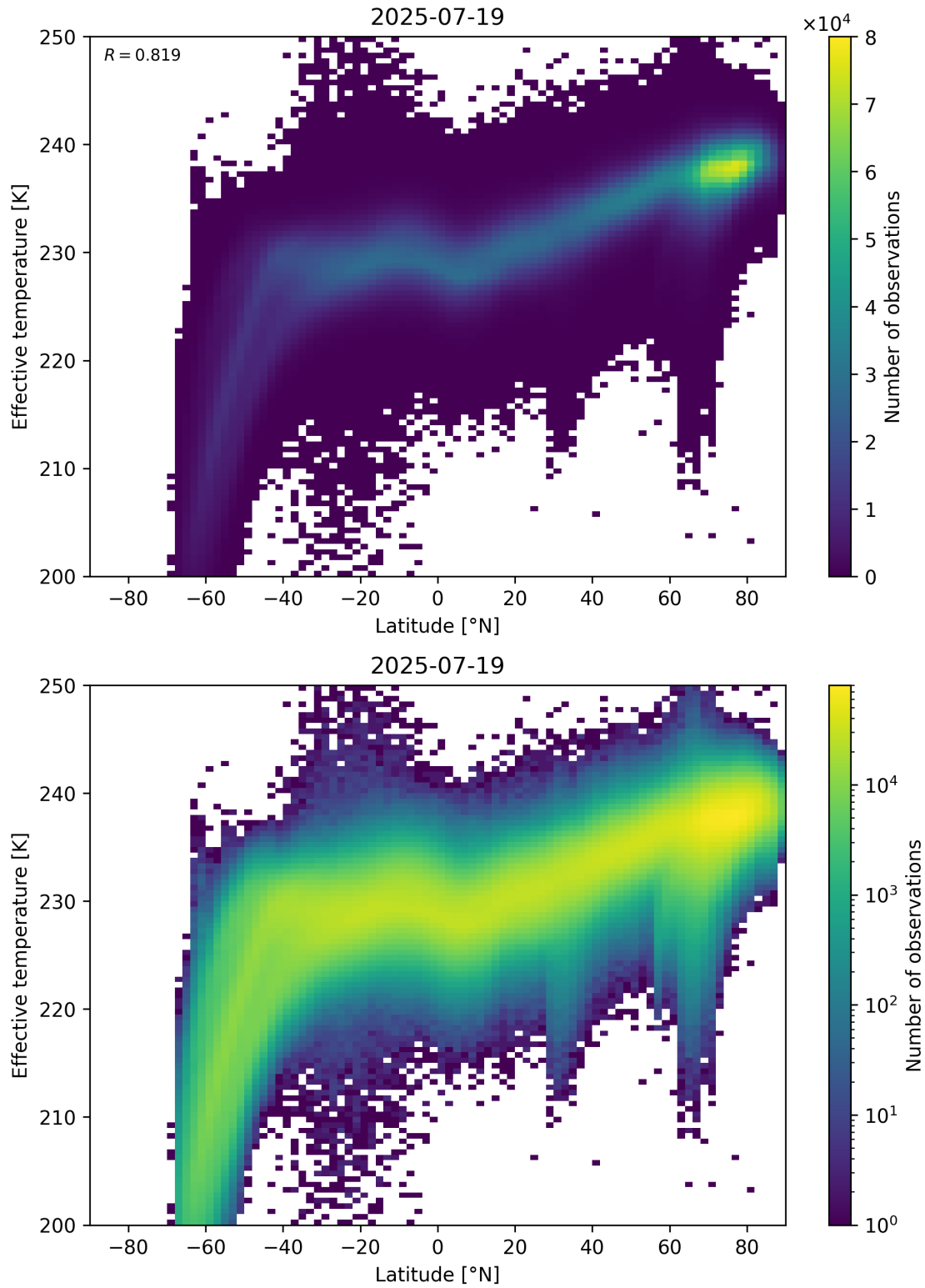
Figure 34: Scatter density plot of “Latitude” against “Effective temperature” for 2025-07-19 to 2025-07-20.
