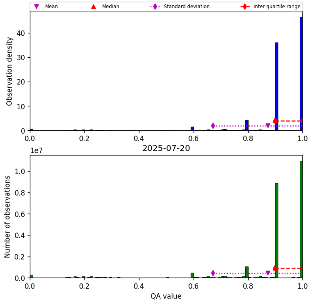
Figure 20: Histogram of “QA value” for 2025-07-19 to 2025-07-21
