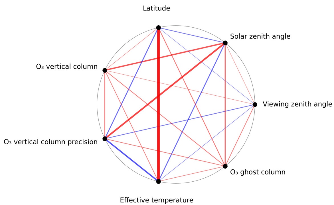
Figure 1: Map of correlation graph for 2025-07-19 to 2025-07-21.
