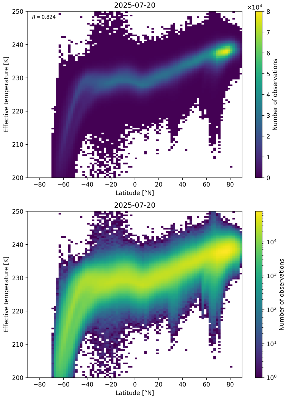
Figure 34: Scatter density plot of “Latitude” against “Effective temperature” for 2025-07-19 to 2025-07-21.
