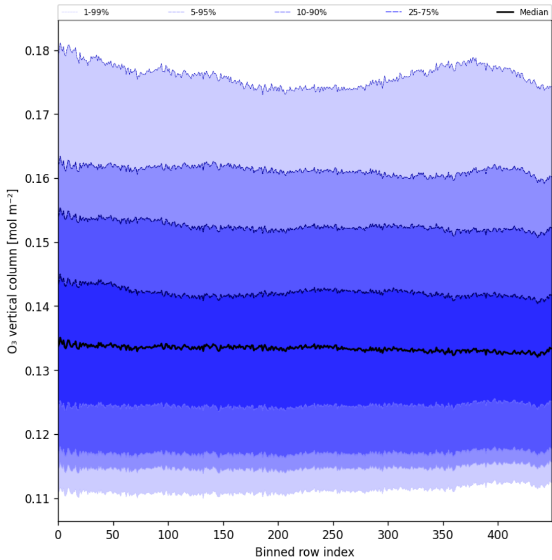
Figure 28: Along track statistics of “O 3 vertical column” for 2025-07-19 to 2025-07-21
