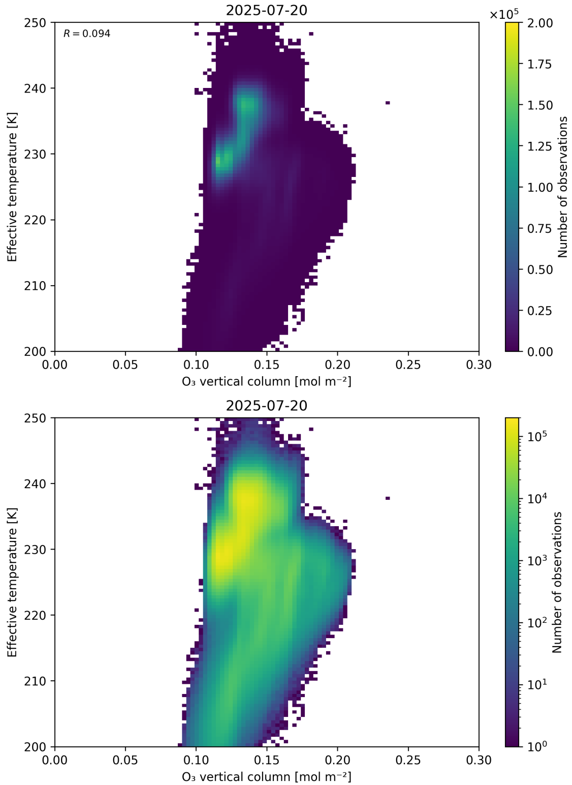
Figure 39: Scatter density plot of “O 3 vertical column” against “Effective temperature” for 2025-07-19 to 2025-07-21.
