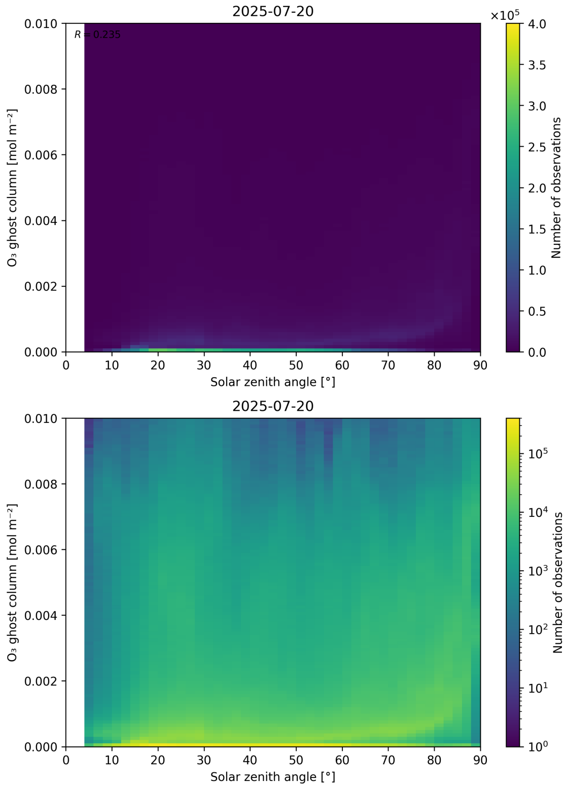
Figure 46: Scatter density plot of “Solar zenith angle” against “O 3 ghost column” for 2025-07-19 to 2025-07-21.
