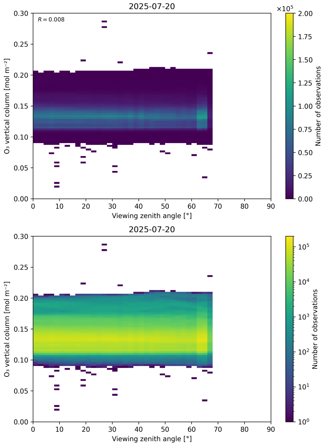
Figure 52: Scatter density plot of “Viewing zenith angle” against “O 3 vertical column” for 2025-07-19 to 2025-07-21.
