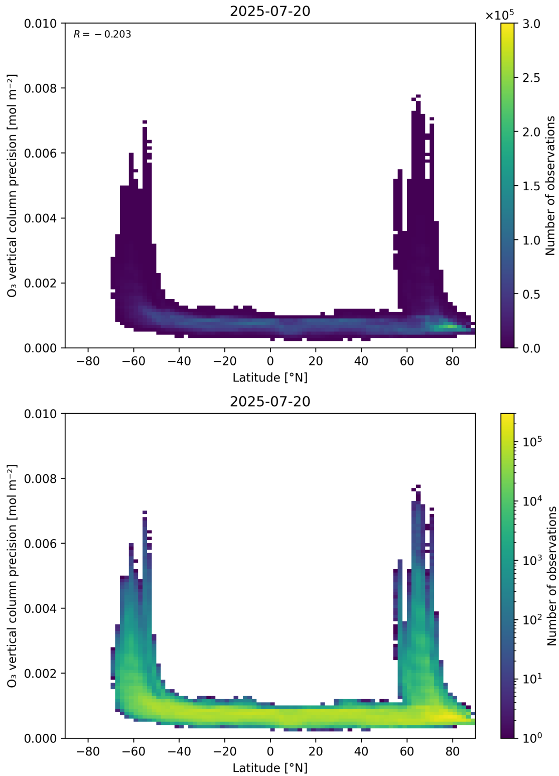
Figure 37: Scatter density plot of “Latitude” against “O 3 vertical column precision” for 2025-07-19 to 2025-07-21.
