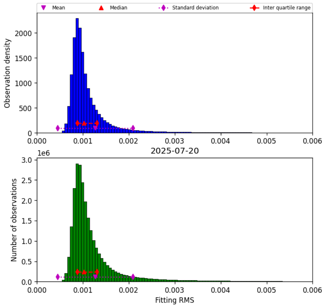
Figure 23: Histogram of “Fitting RMS” for 2025-07-19 to 2025-07-21
