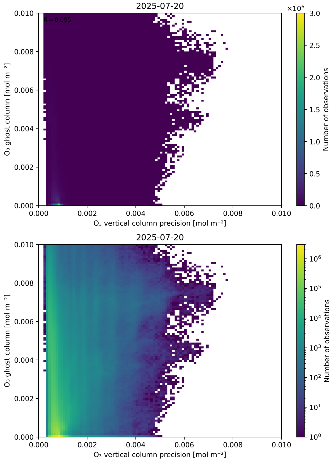
Figure 43: Scatter density plot of “ \text{O}_3 vertical column precision” against “ \text{O}_3 ghost column” for 2025-07-19 to 2025-07-21.
