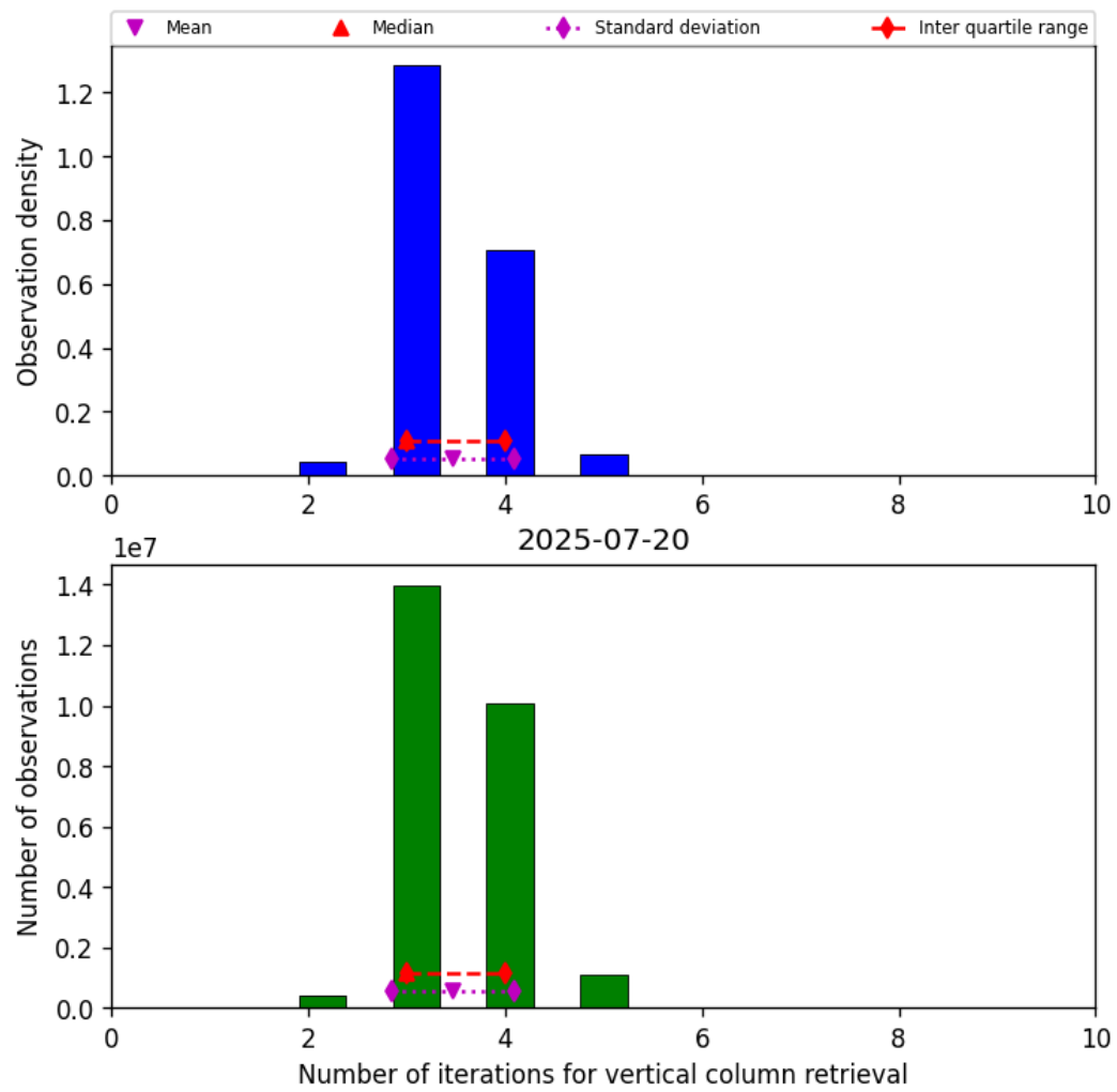
Figure 26: Histogram of “Number of iterations for vertical column retrieval” for 2025-07-19 to 2025-07-21
