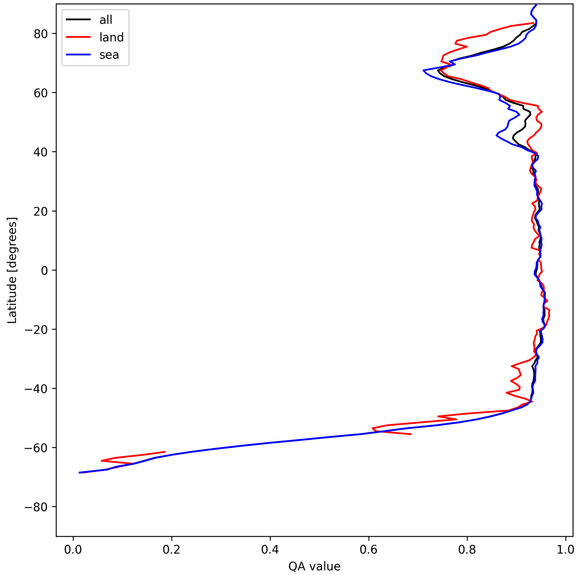
Figure 13: Zonal average of “QA value” for 2025-07-19 to 2025-07-21.
