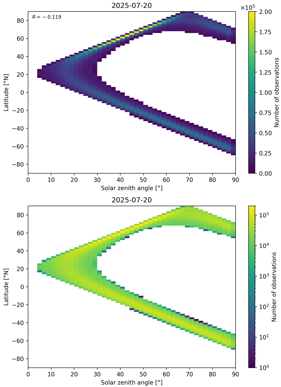
Figure 44: Scatter density plot of “Solar zenith angle” against “Latitude” for 2025-07-19 to 2025-07-21.
