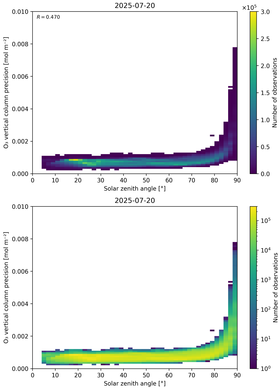
Figure 48: Scatter density plot of “Solar zenith angle” against “O 3 vertical column precision” for 2025-07-19 to 2025-07-21.
