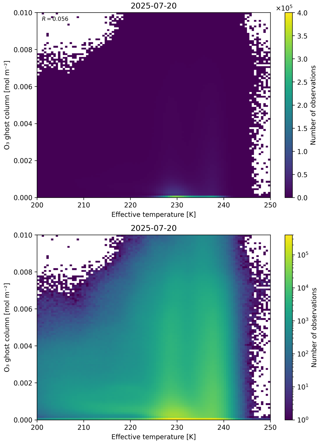
Figure 38: Scatter density plot of “Effective temperature” against “O 3 ghost column” for 2025-07-19 to 2025-07-21.
