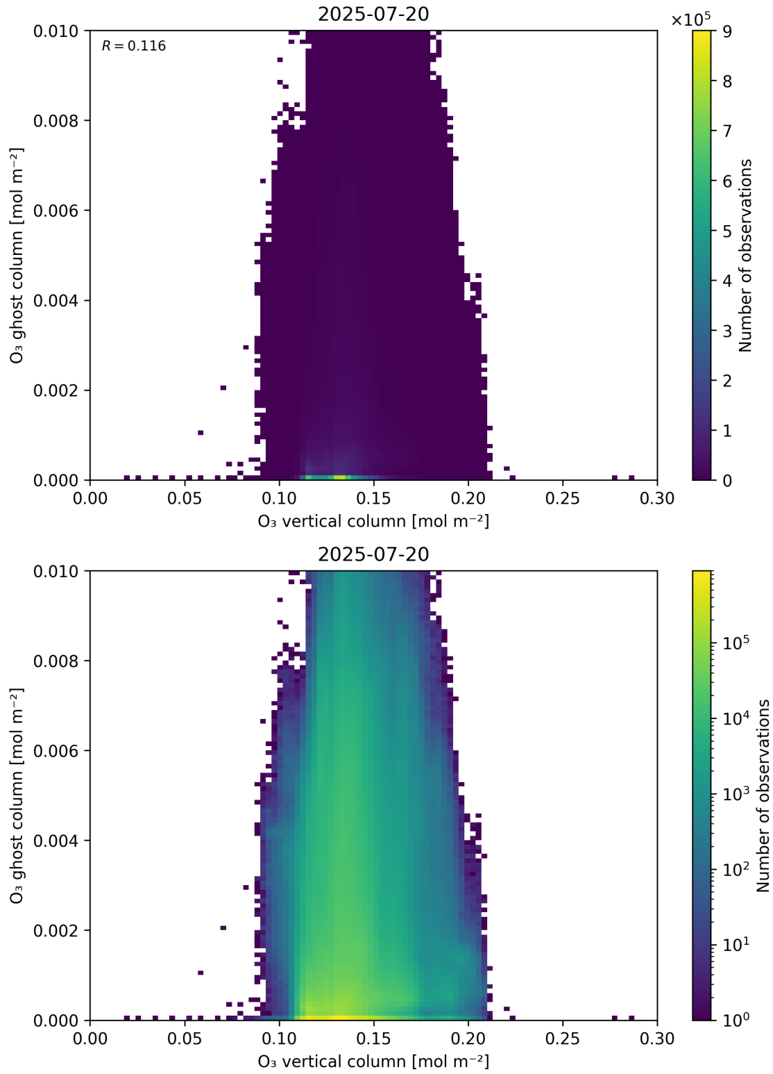
Figure 40: Scatter density plot of “O 3 vertical column” against “O 3 ghost column” for 2025-07-19 to 2025-07-21.
