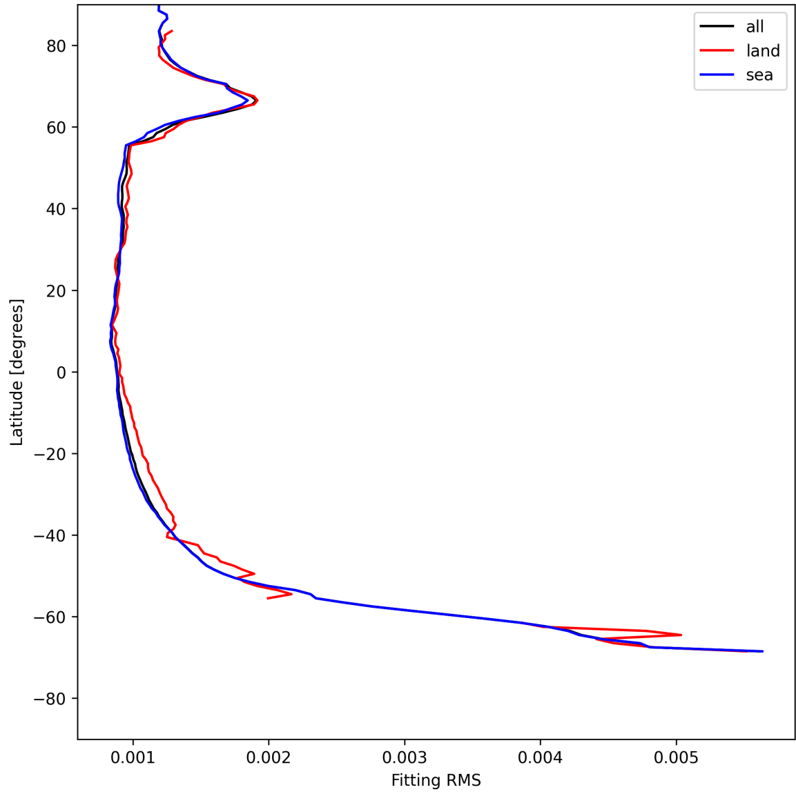
Figure 16: Zonal average of “Fitting RMS” for 2025-07-19 to 2025-07-21.
