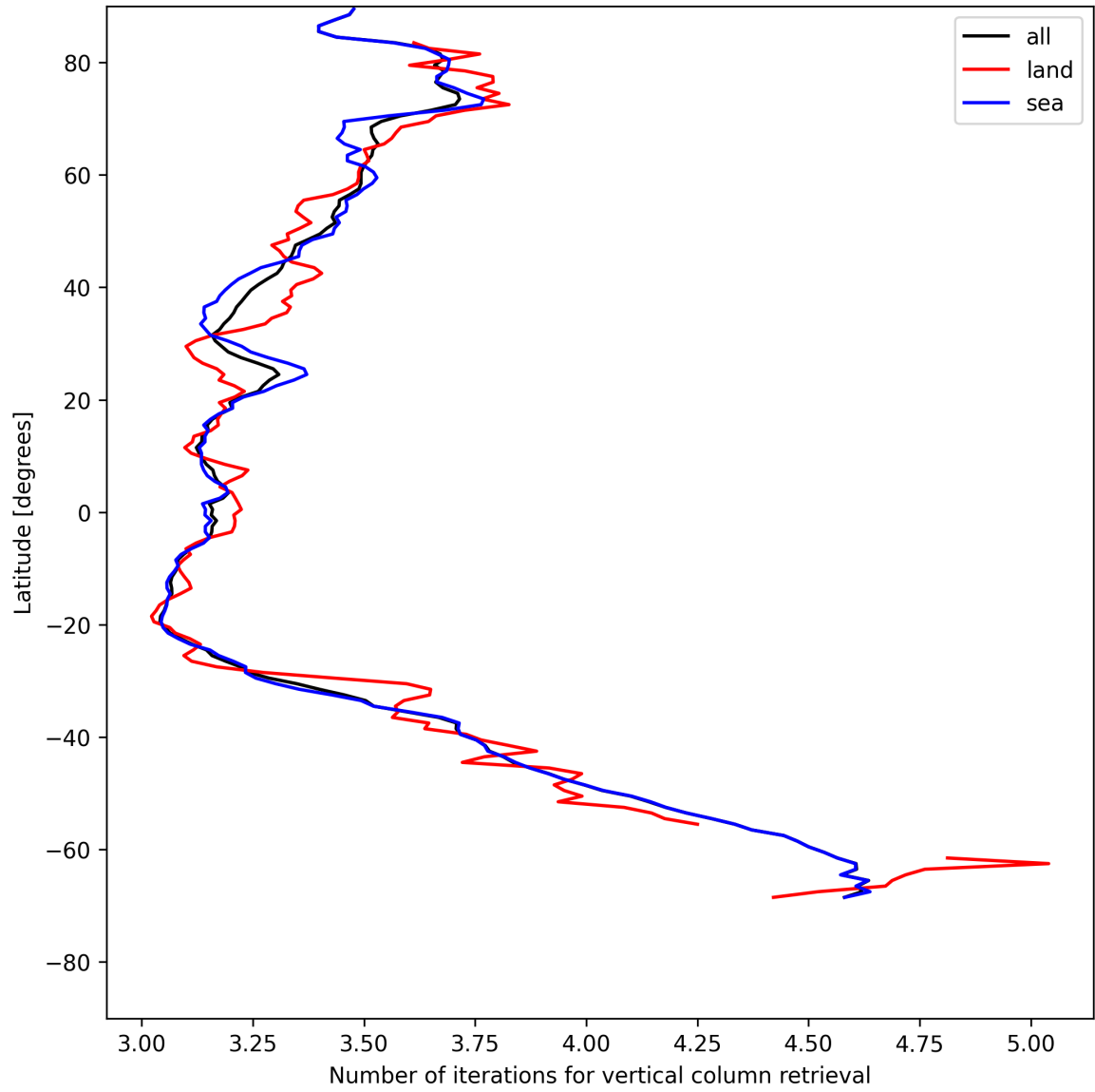
Figure 19: Zonal average of “Number of iterations for vertical column retrieval” for 2025-07-19 to 2025-07-21.
