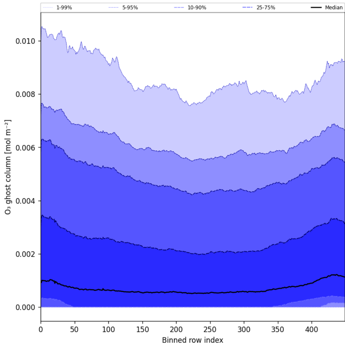
Figure 32: Along track statistics of “O 3 ghost column” for 2025-07-19 to 2025-07-21
