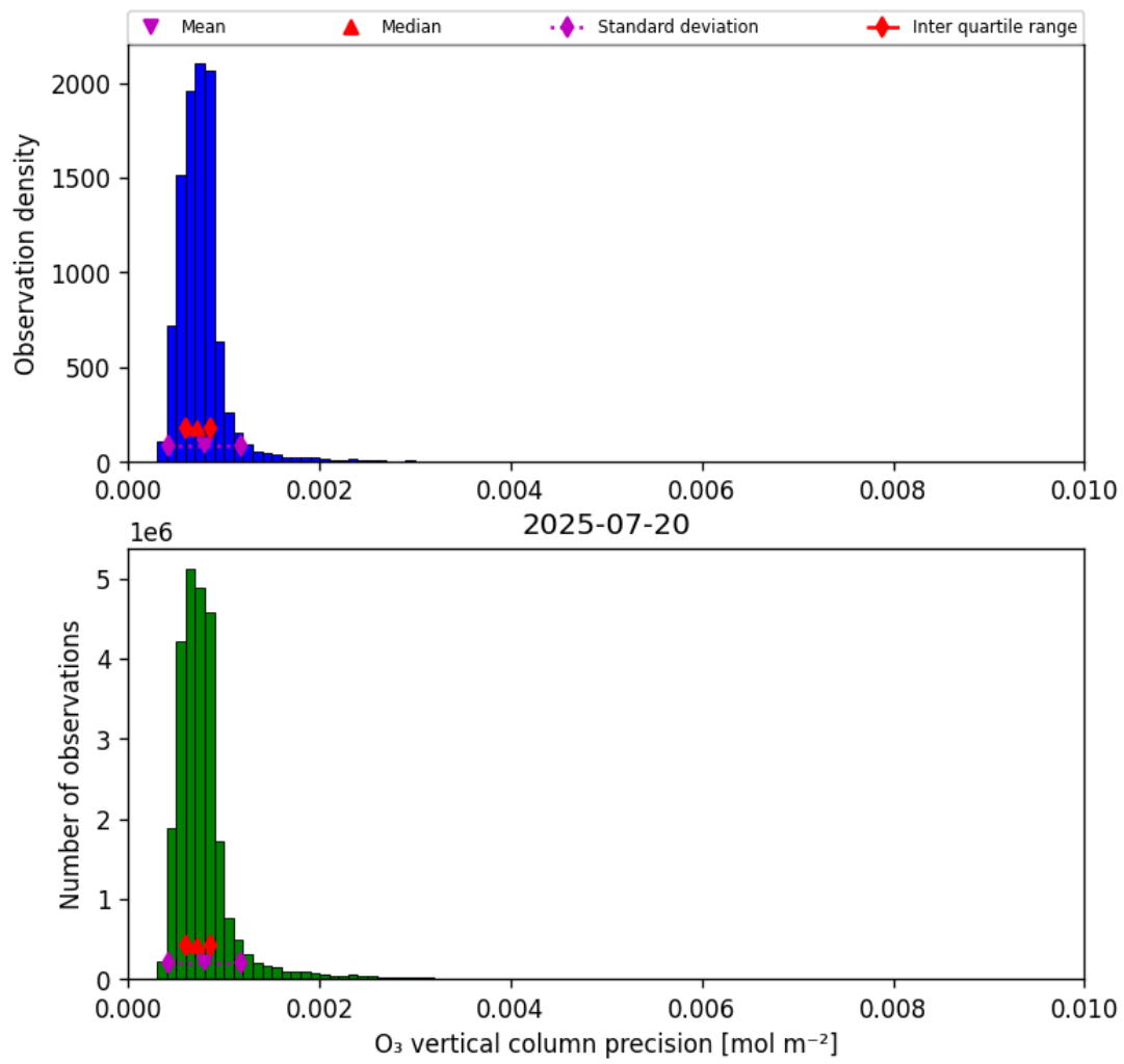
Figure 22: Histogram of “O 3 vertical column precision” for 2025-07-19 to 2025-07-21
