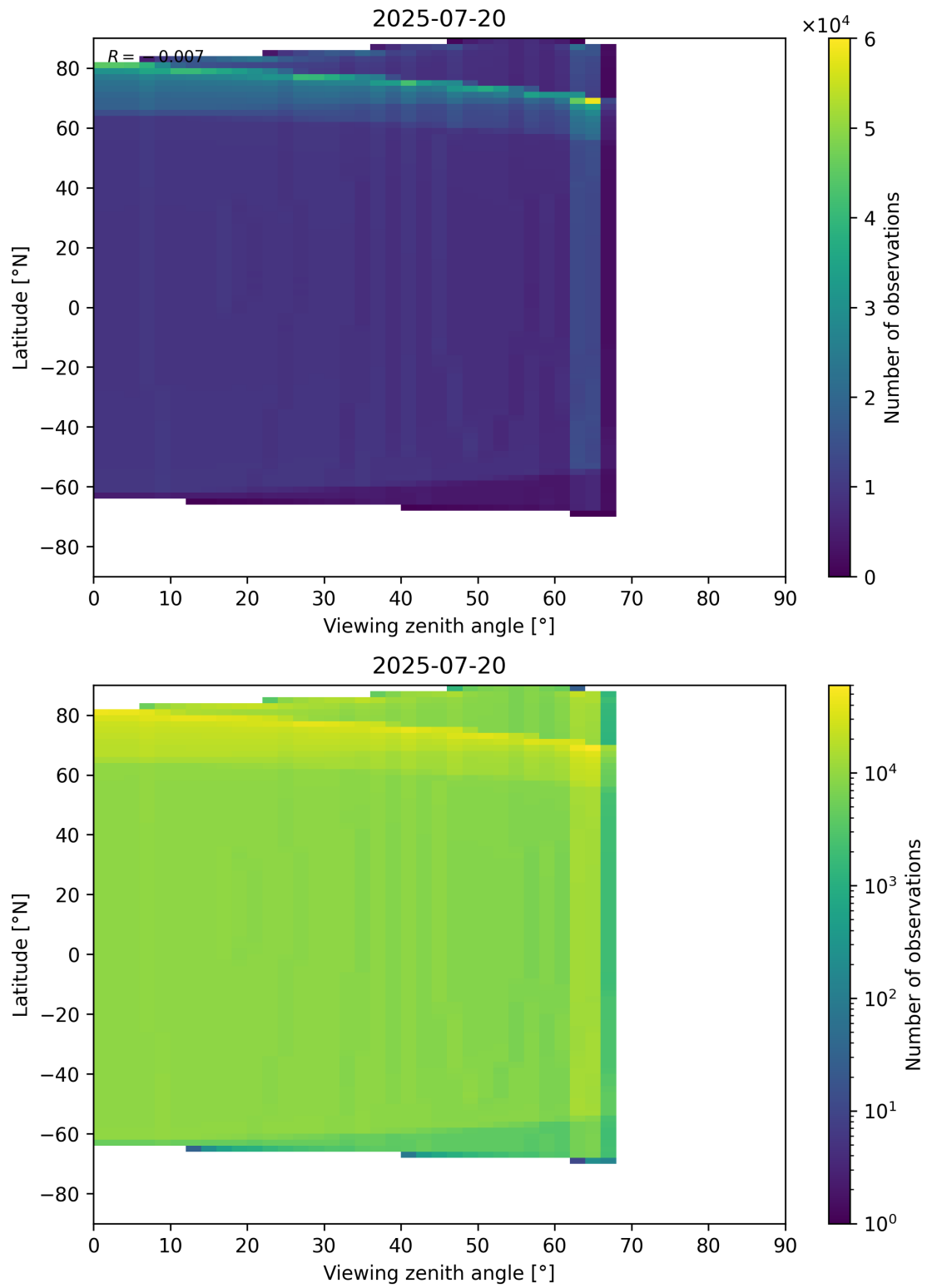
Figure 49: Scatter density plot of “Viewing zenith angle” against “Latitude” for 2025-07-19 to 2025-07-21.
