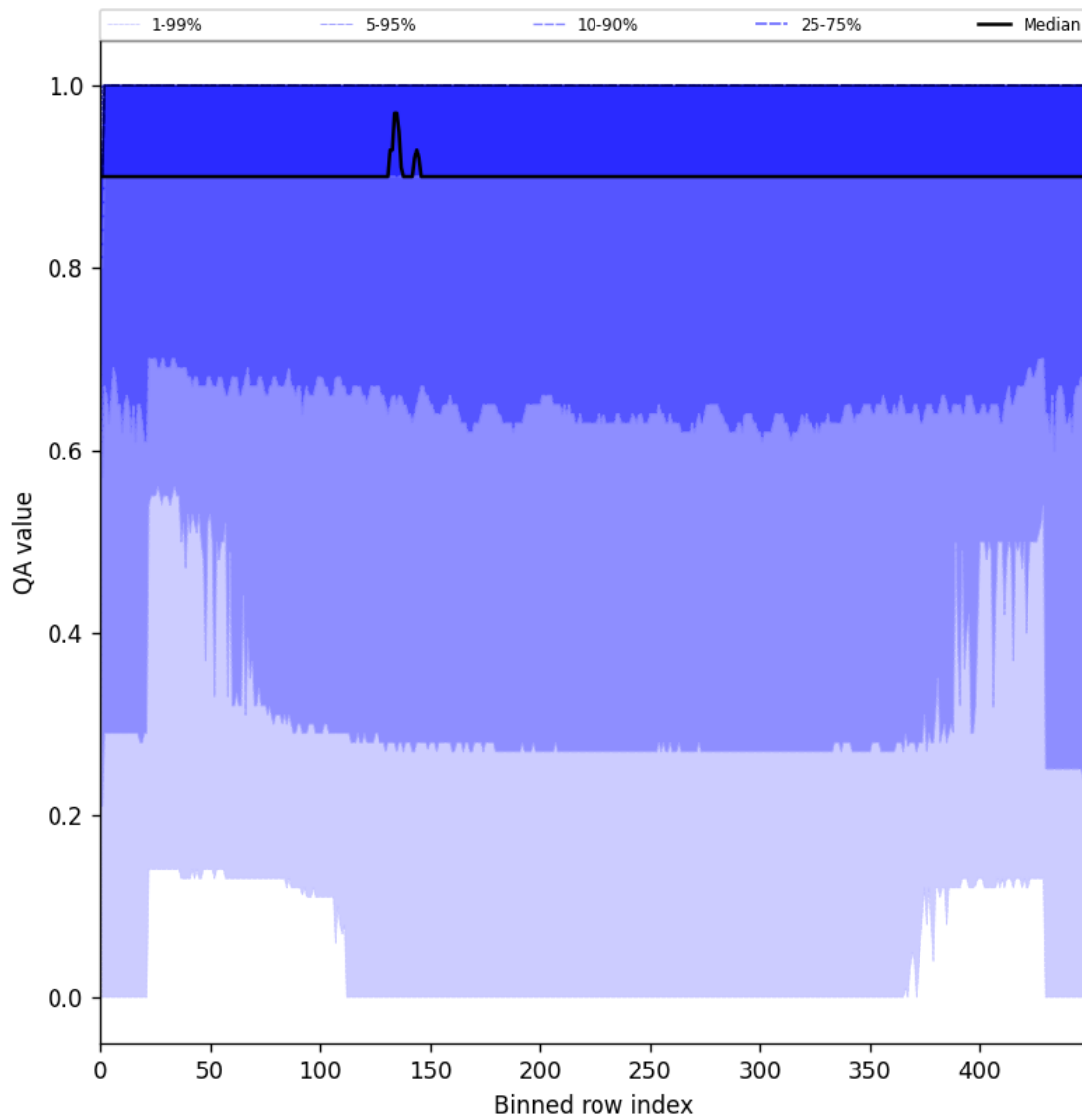
Figure 27: Along track statistics of “QA value” for 2025-07-19 to 2025-07-21
