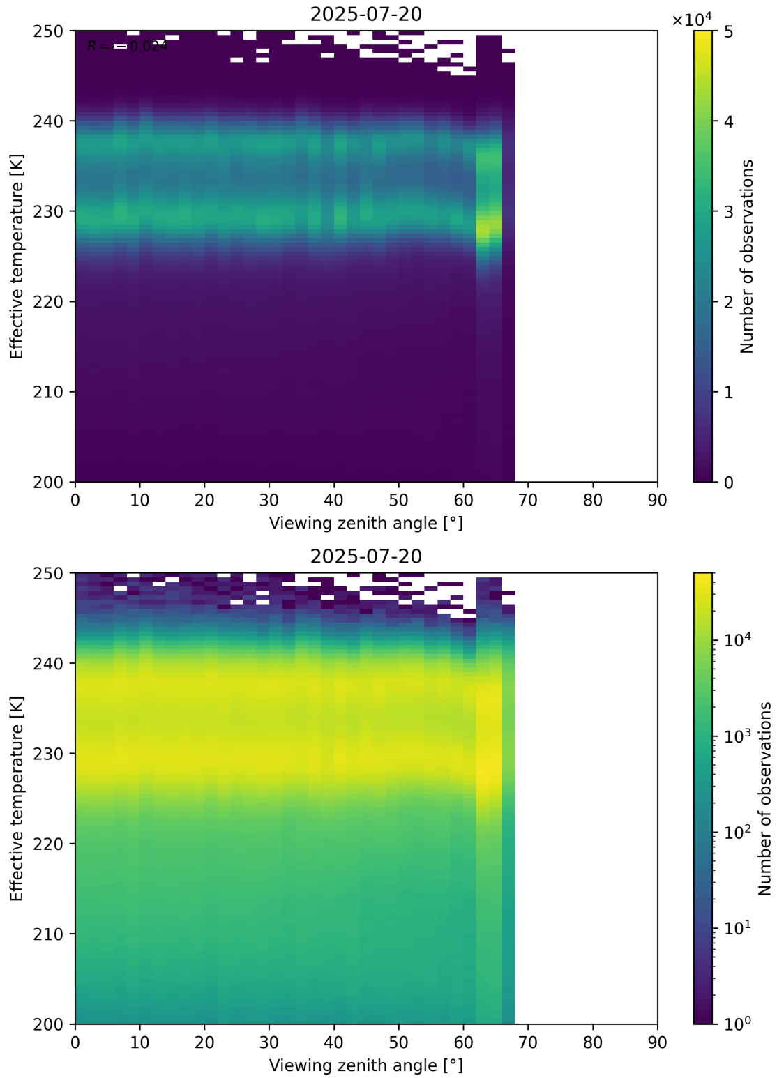
Figure 50: Scatter density plot of “Viewing zenith angle” against “Effective temperature” for 2025-07-19 to 2025-07-21.
