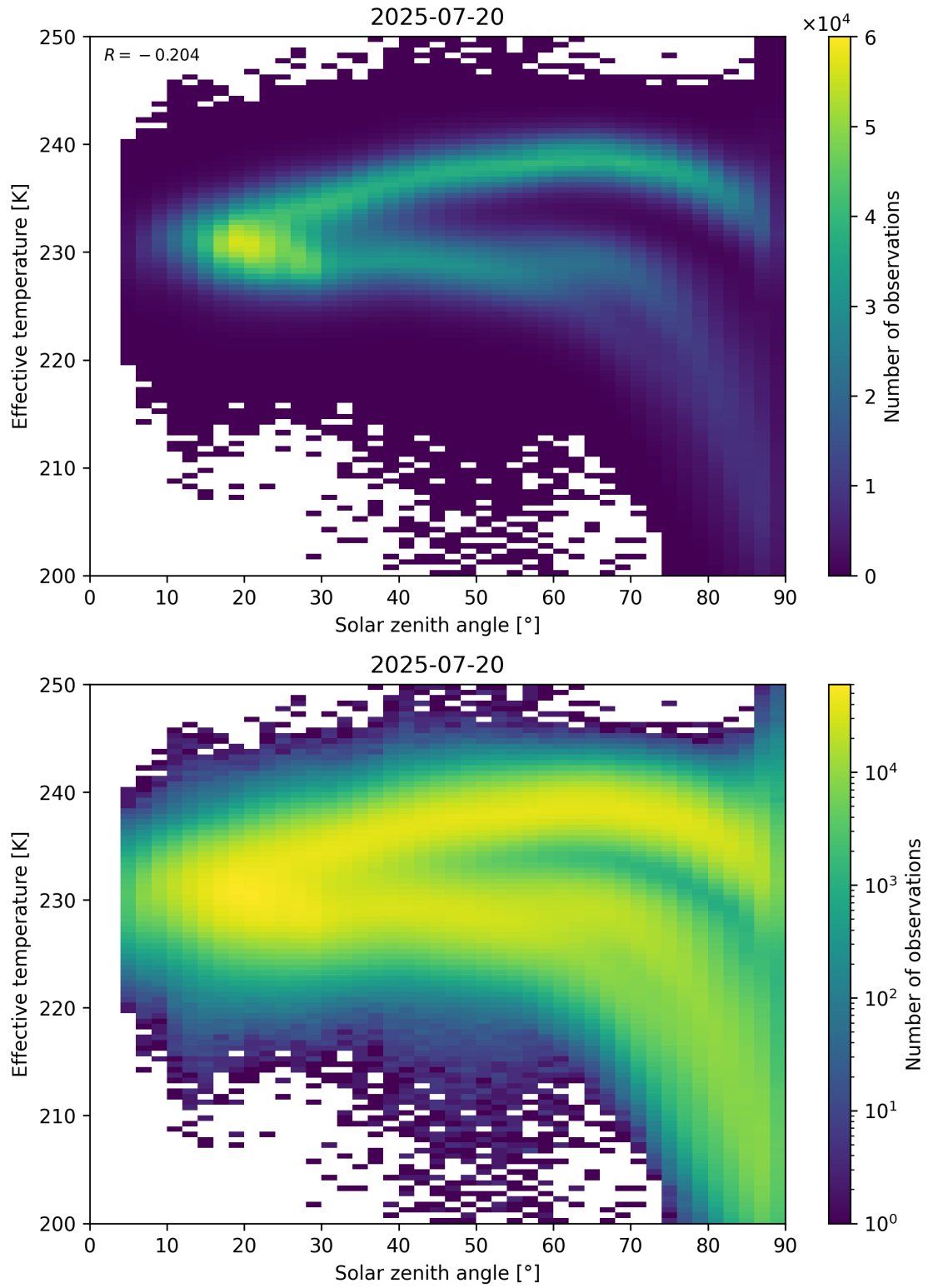
Figure 45: Scatter density plot of “Solar zenith angle” against “Effective temperature” for 2025-07-19 to 2025-07-21.
