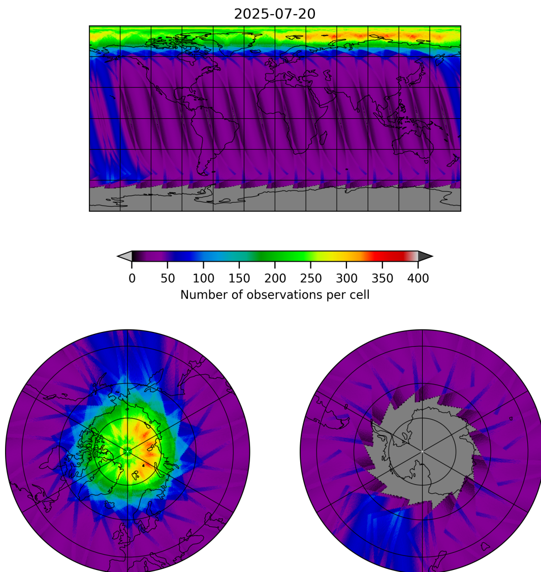
Figure 12: Map of the number of observations for 2025-07-19 to 2025-07-21
