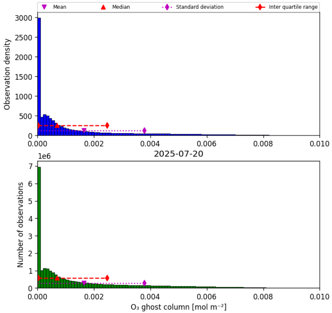
Figure 25: Histogram of “O 3 ghost column” for 2025-07-19 to 2025-07-21
