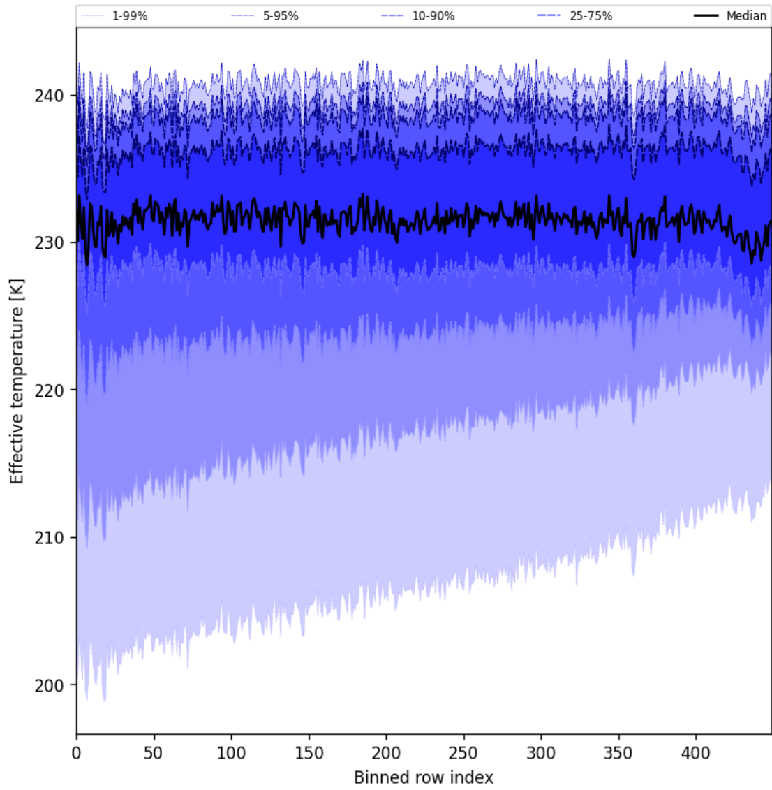
Figure 31: Along track statistics of “Effective temperature” for 2025-07-19 to 2025-07-21
