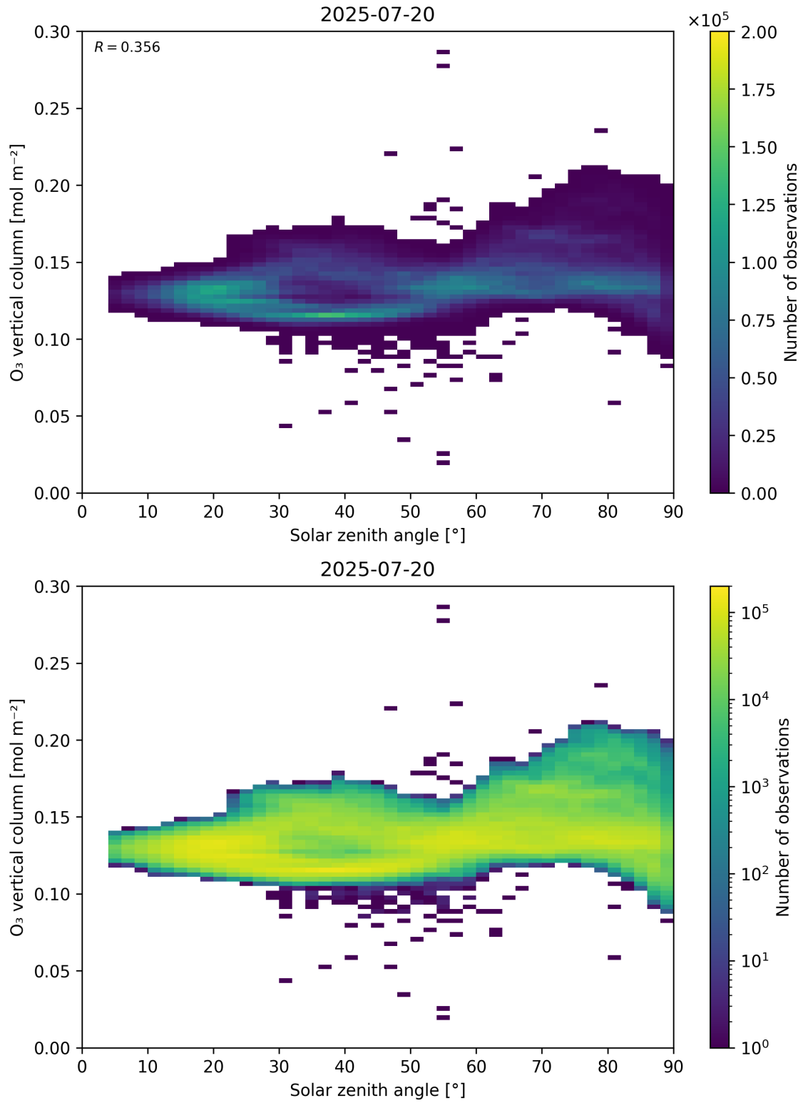
Figure 47: Scatter density plot of “Solar zenith angle” against “O 3 vertical column” for 2025-07-19 to 2025-07-21.
