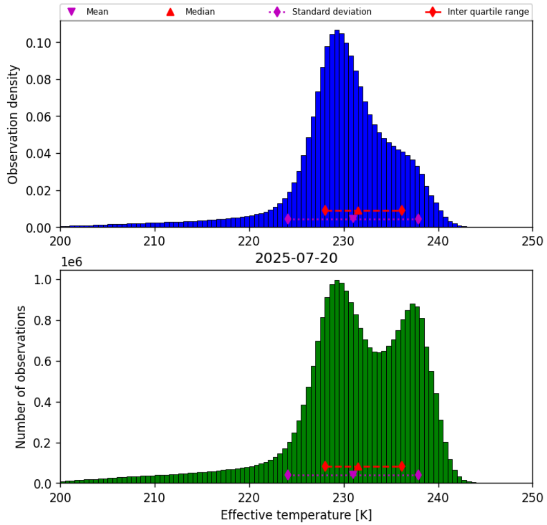
Figure 24: Histogram of “Effective temperature” for 2025-07-19 to 2025-07-21
