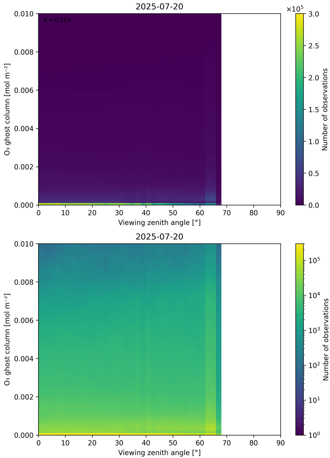
Figure 51: Scatter density plot of “Viewing zenith angle” against “O 3 ghost column” for 2025-07-19 to 2025-07-21.
