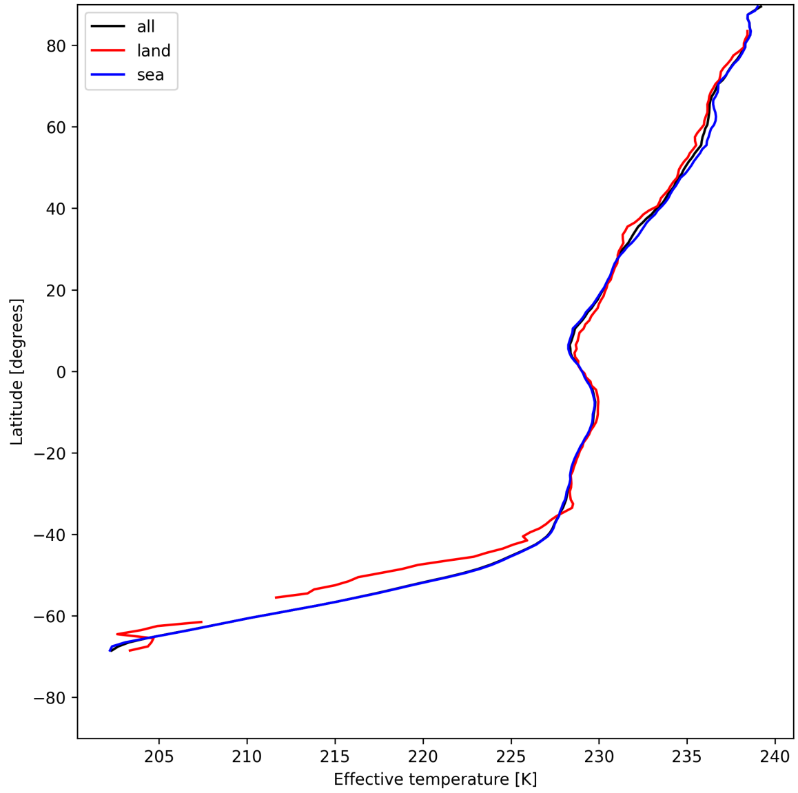
Figure 17: Zonal average of "Effective temperature" for 2025-07-19 to 2025-07-21.
