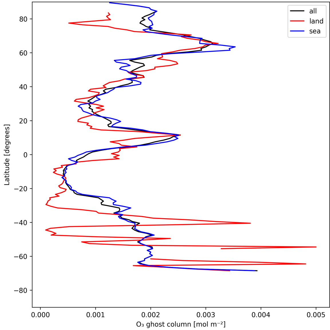
Figure 18: Zonal average of “O 3 ghost column” for 2025-07-19 to 2025-07-21.
