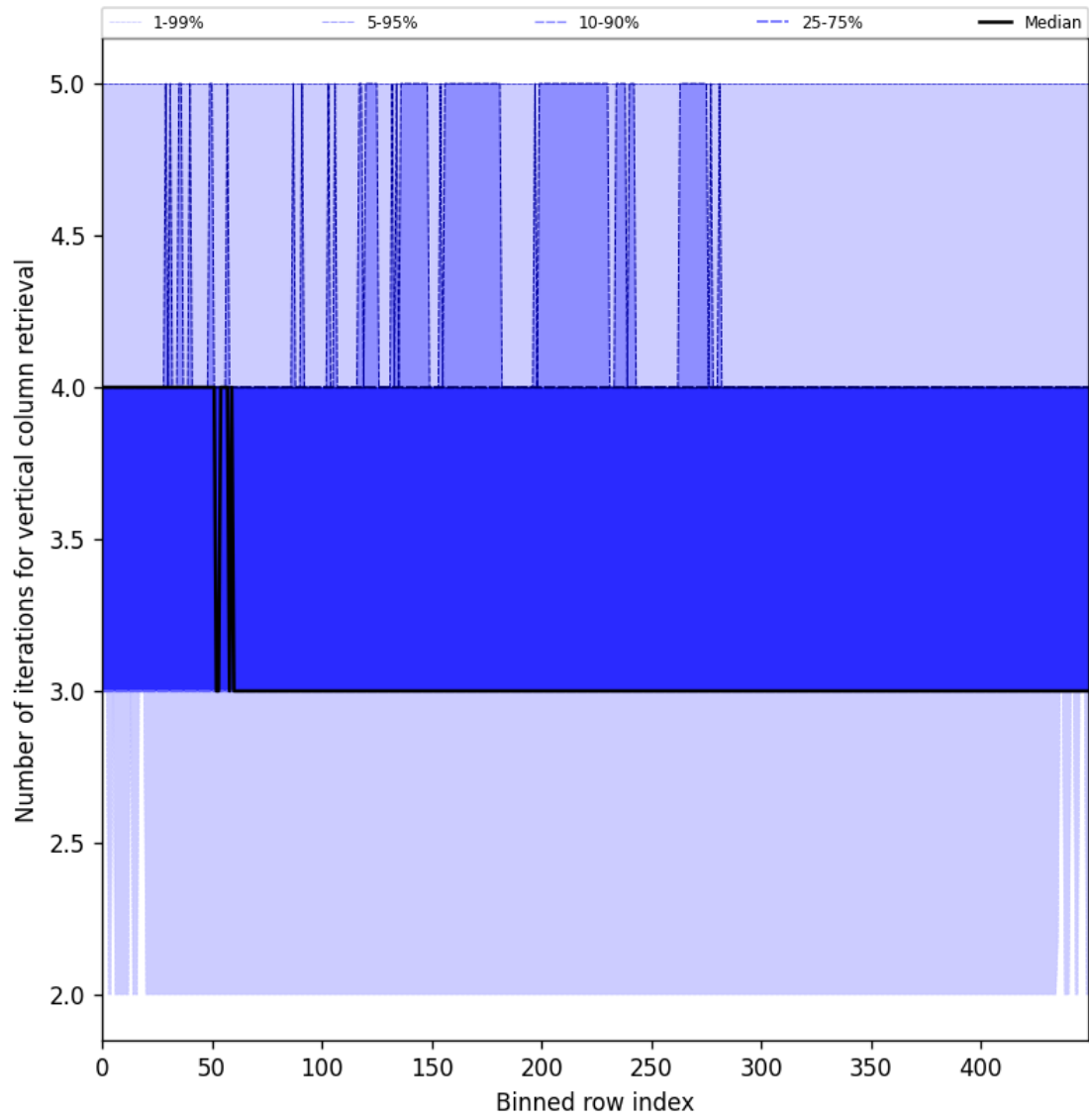
Figure 33: Along track statistics of “Number of iterations for vertical column retrieval” for 2025-07-19 to 2025-07-21
