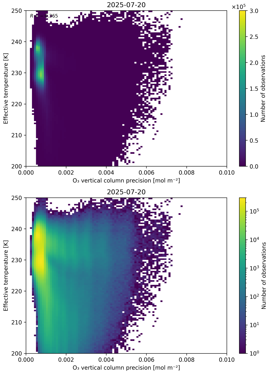
Figure 42: Scatter density plot of “O 3 vertical column precision” against “Effective temperature” for 2025-07-19 to 2025-07-21.
