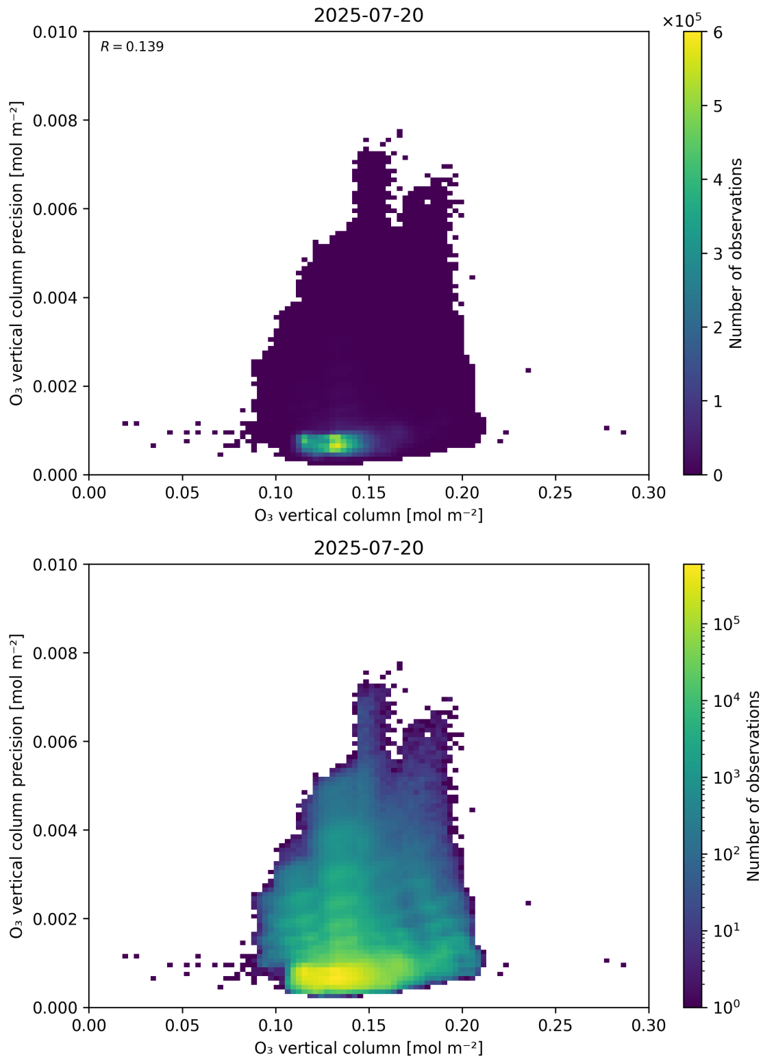
Figure 41: Scatter density plot of “O 3 vertical column” against “O 3 vertical column precision” for 2025-07-19 to 2025-07-21.
