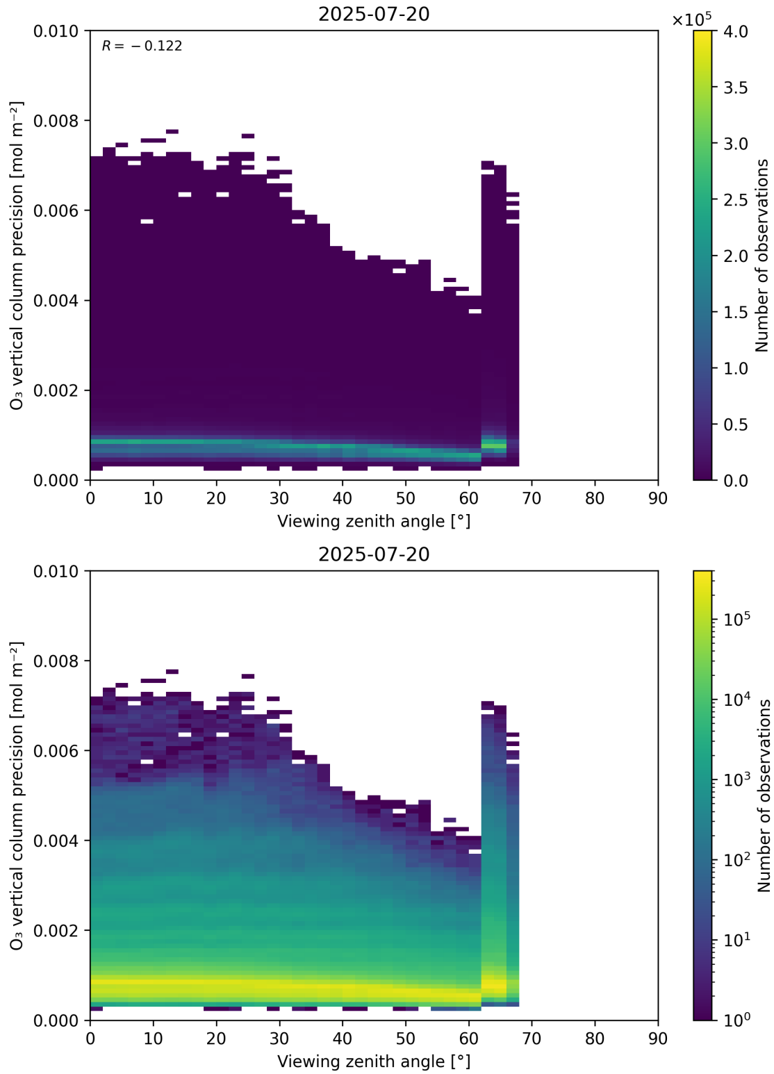
Figure 53: Scatter density plot of “Viewing zenith angle” against “O 3 vertical column precision” for 2025-07-19 to 2025-07-21.
