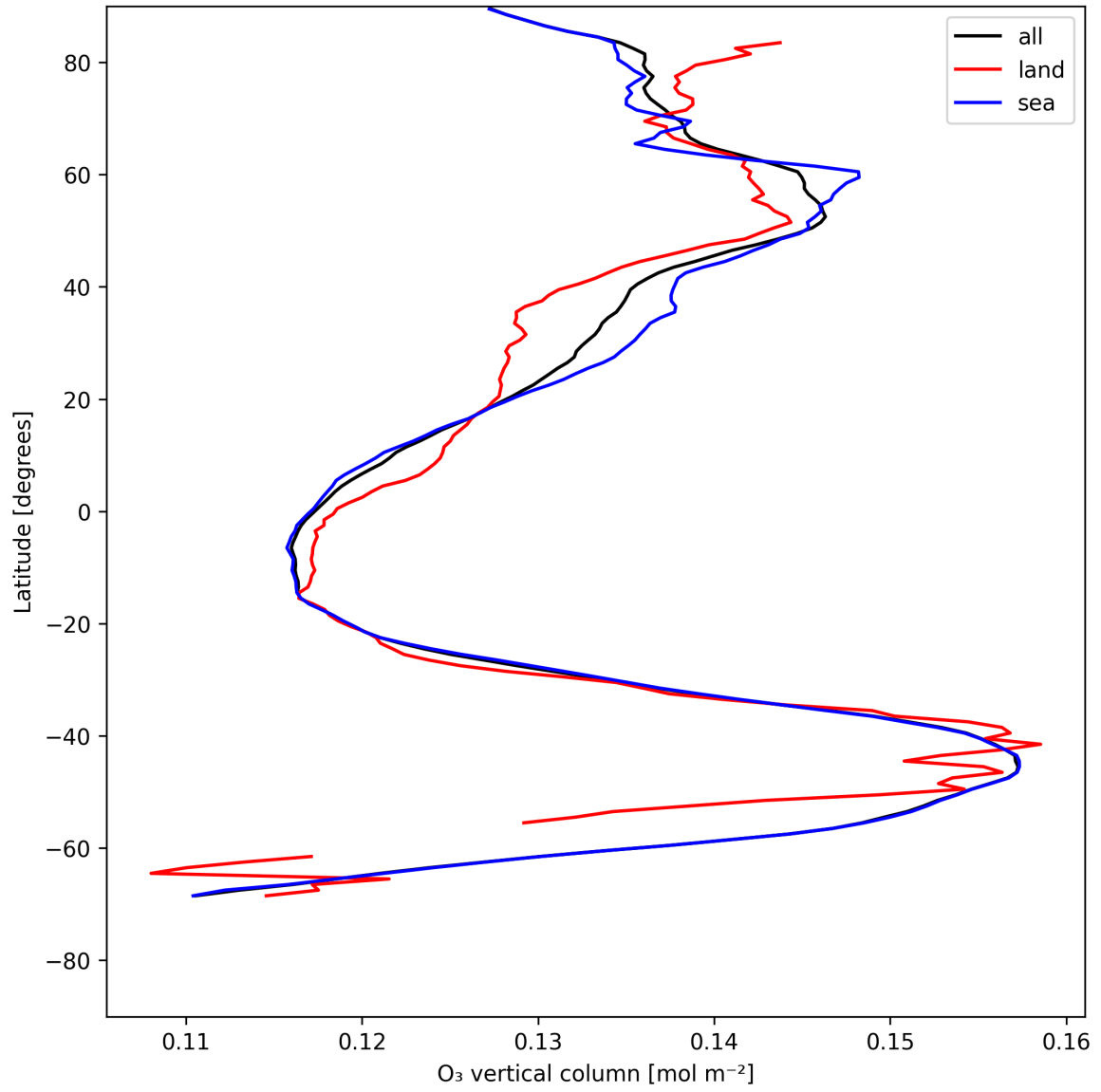
Figure 14: Zonal average of “O 3 vertical column” for 2025-07-19 to 2025-07-21.
