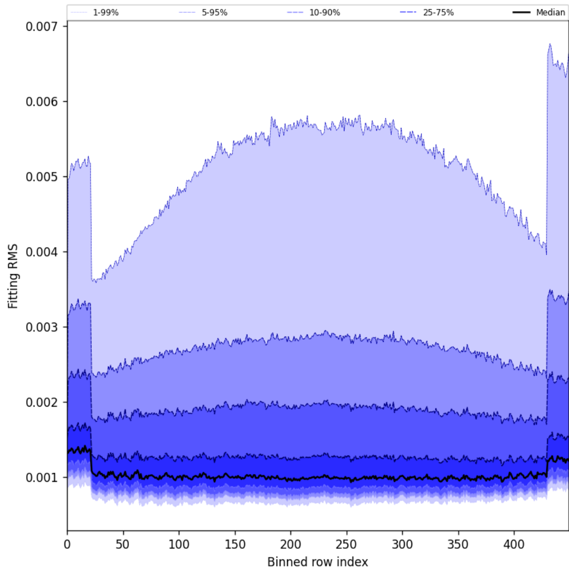
Figure 30: Along track statistics of “Fitting RMS” for 2025-07-19 to 2025-07-21
