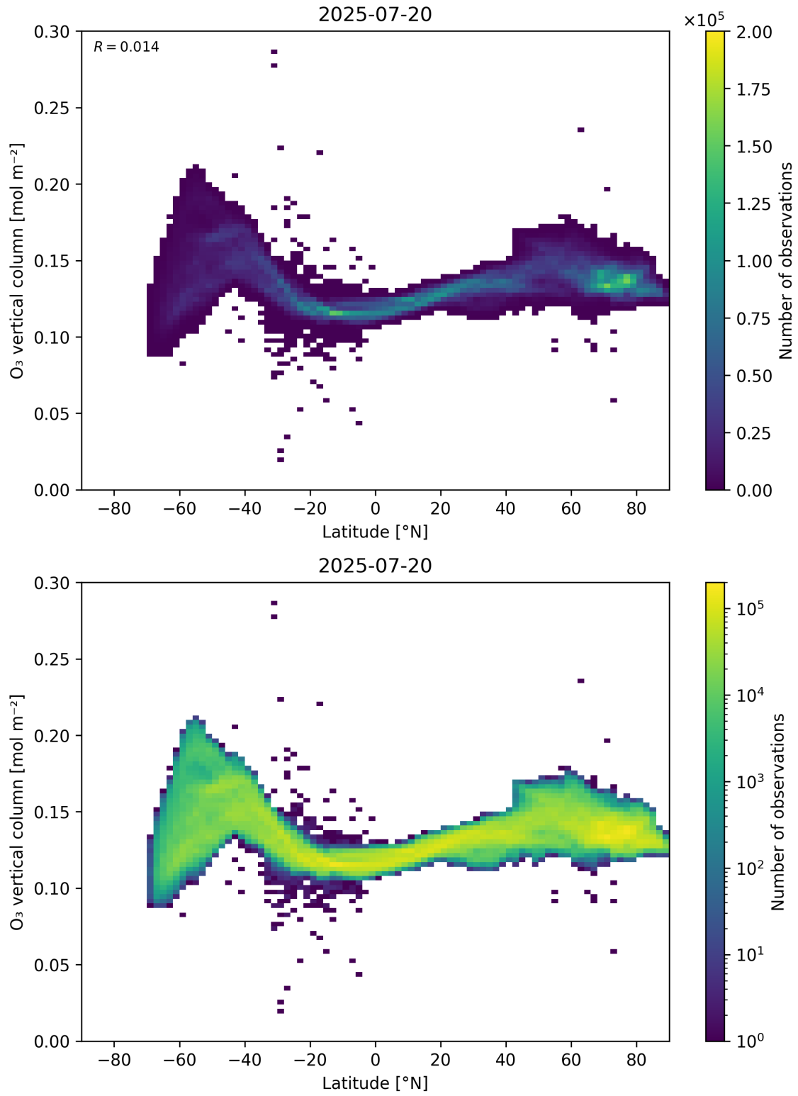
Figure 36: Scatter density plot of “Latitude” against “O 3 vertical column” for 2025-07-19 to 2025-07-21.
