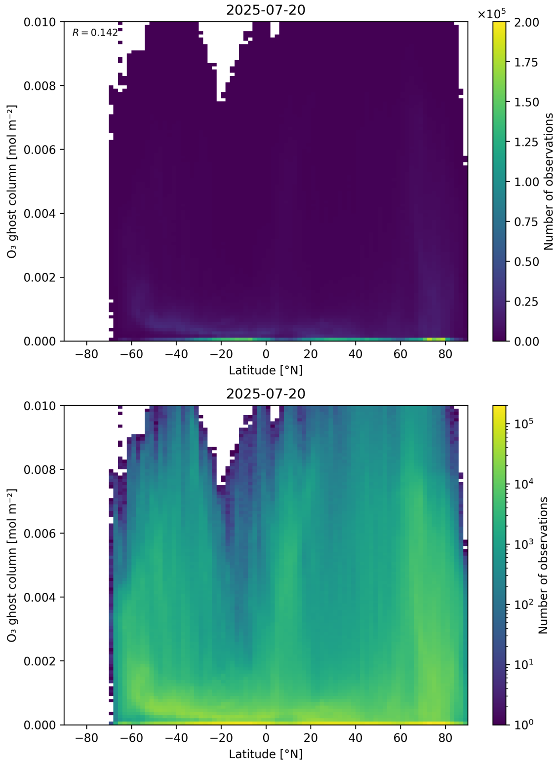
Figure 35: Scatter density plot of “Latitude” against “O 3 ghost column” for 2025-07-19 to 2025-07-21.
