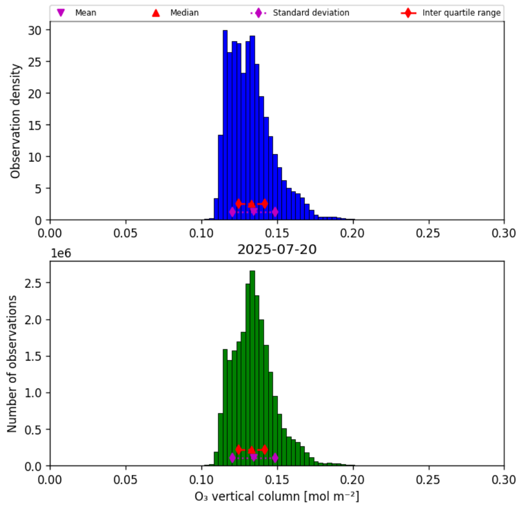
Figure 21: Histogram of “O 3 vertical column” for 2025-07-19 to 2025-07-21
