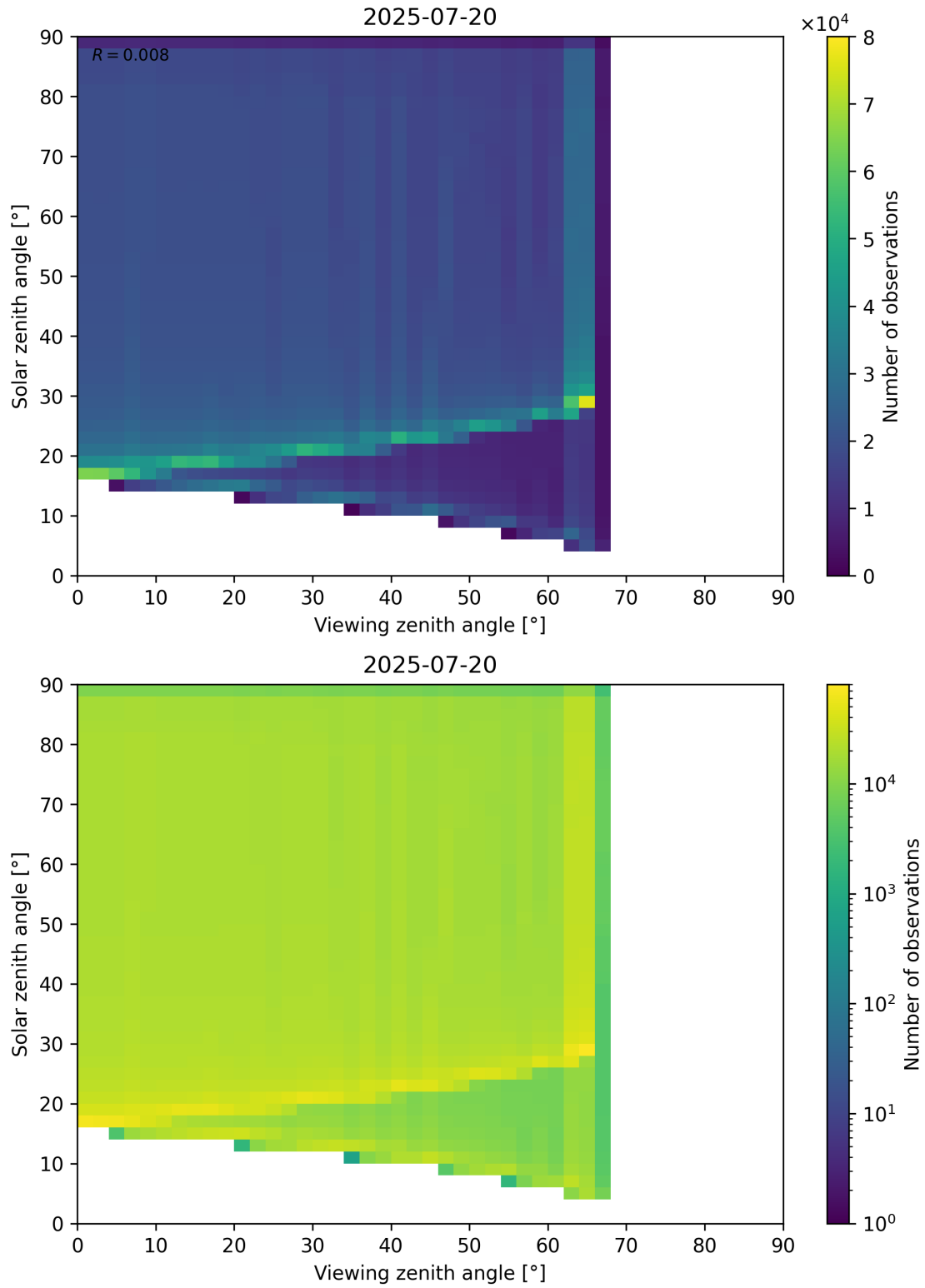
Figure 54: Scatter density plot of “Viewing zenith angle” against “Solar zenith angle” for 2025-07-19 to 2025-07-21.
