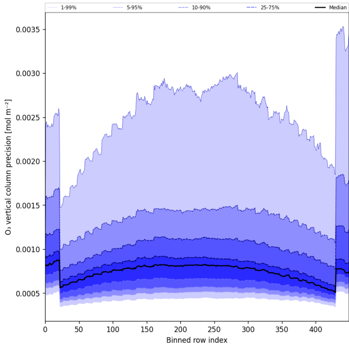
Figure 29: Along track statistics of “O 3 vertical column precision” for 2025-07-19 to 2025-07-21
