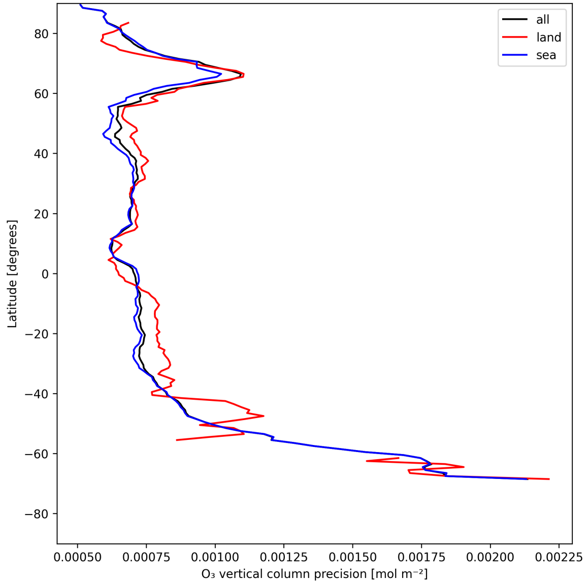
Figure 15: Zonal average of "O 3 vertical column precision" for 2025-07-19 to 2025-07-21.
