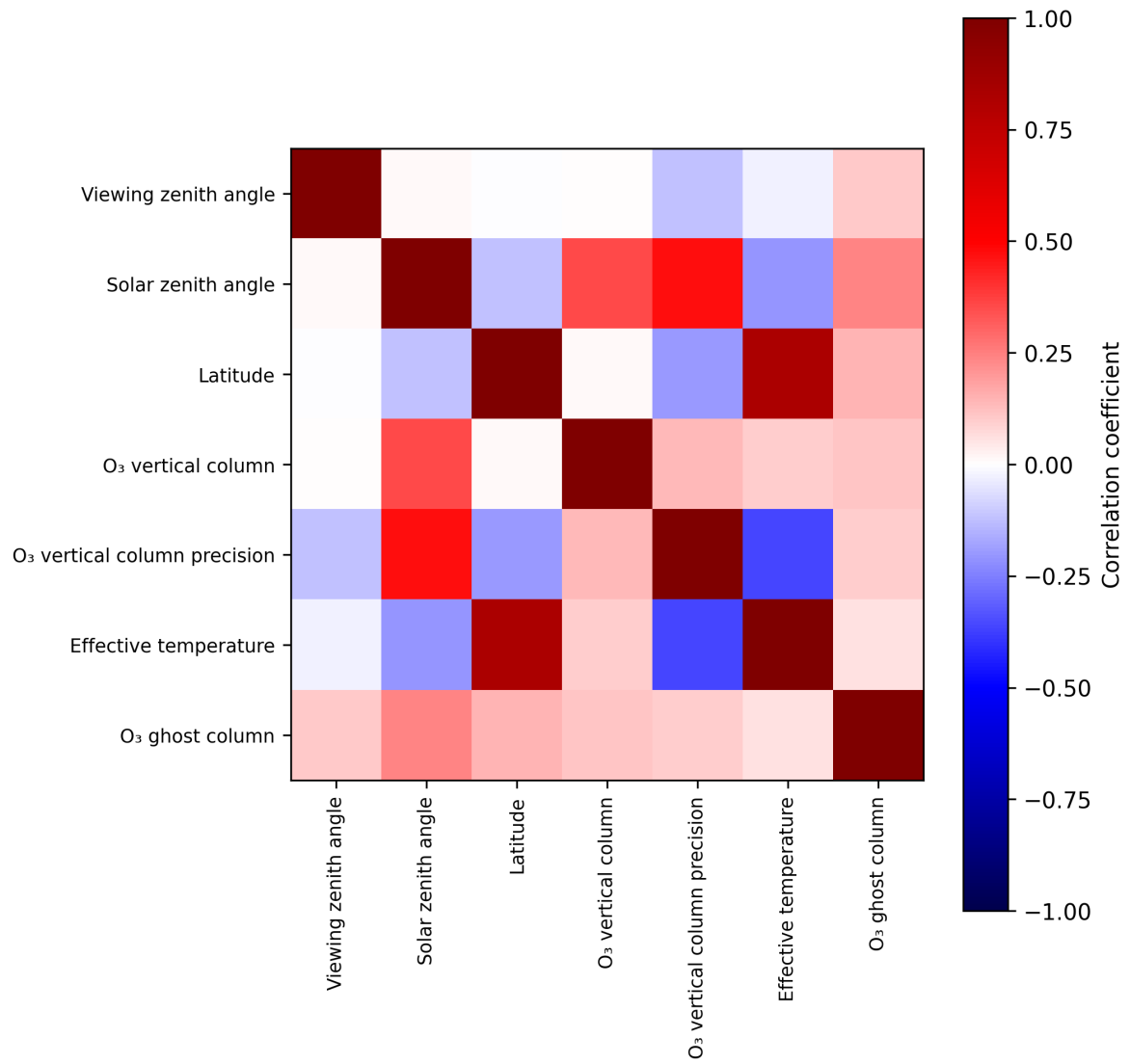
Figure 2: Map of correlation matrix for 2025-07-19 to 2025-07-21.
