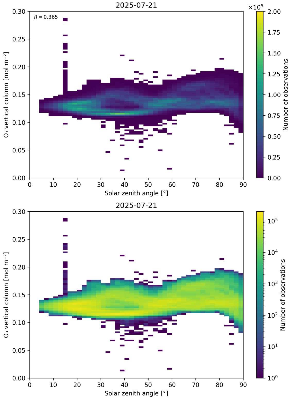
Figure 47: Scatter density plot of “Solar zenith angle” against “O 3 vertical column” for 2025-07-20 to 2025-07-22.
