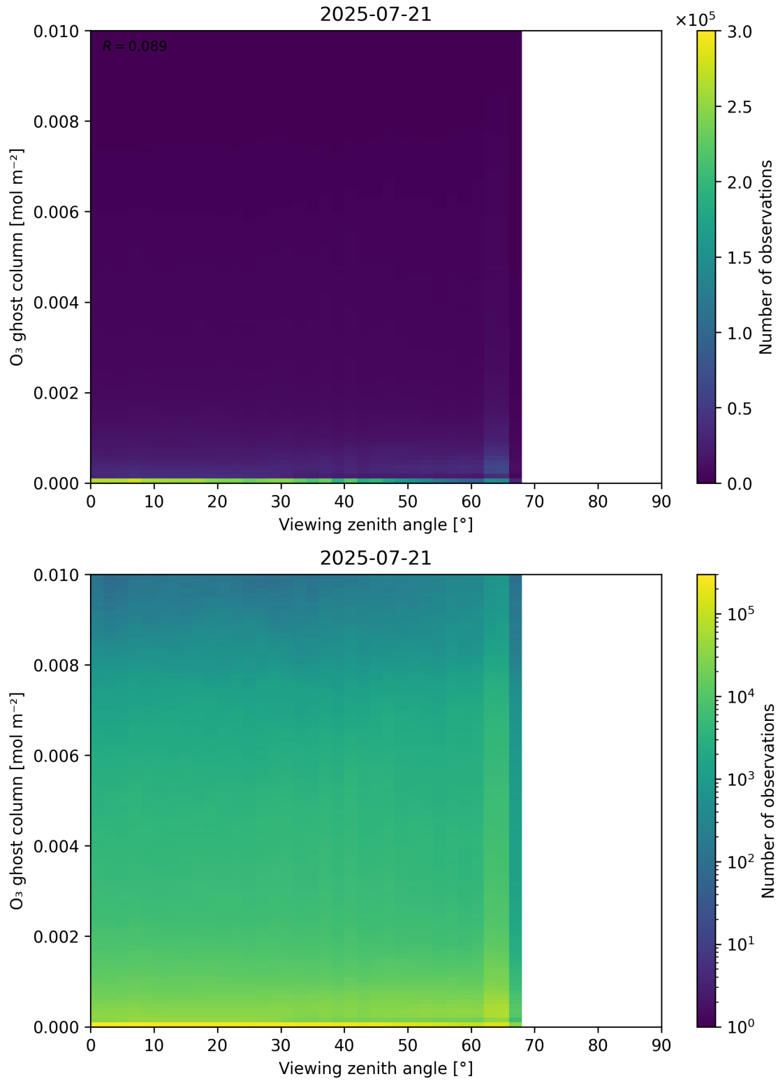
Figure 51: Scatter density plot of “Viewing zenith angle” against “O 3 ghost column” for 2025-07-20 to 2025-07-22.
