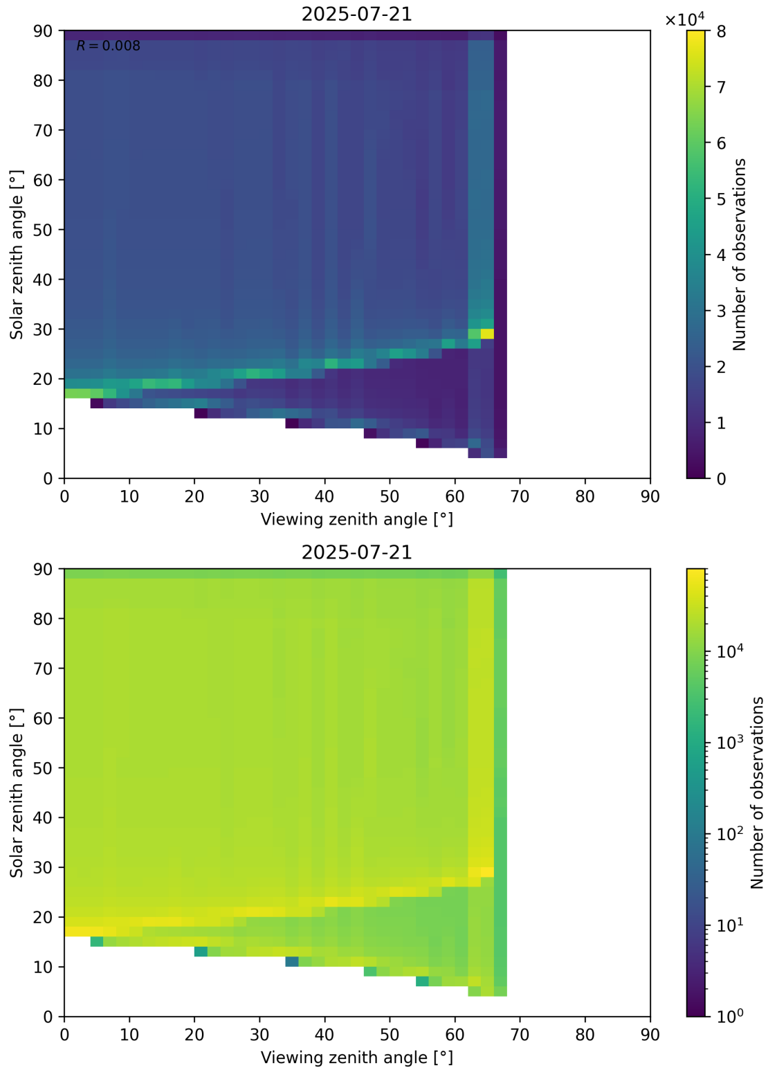
Figure 54: Scatter density plot of “Viewing zenith angle” against “Solar zenith angle” for 2025-07-20 to 2025-07-22.
