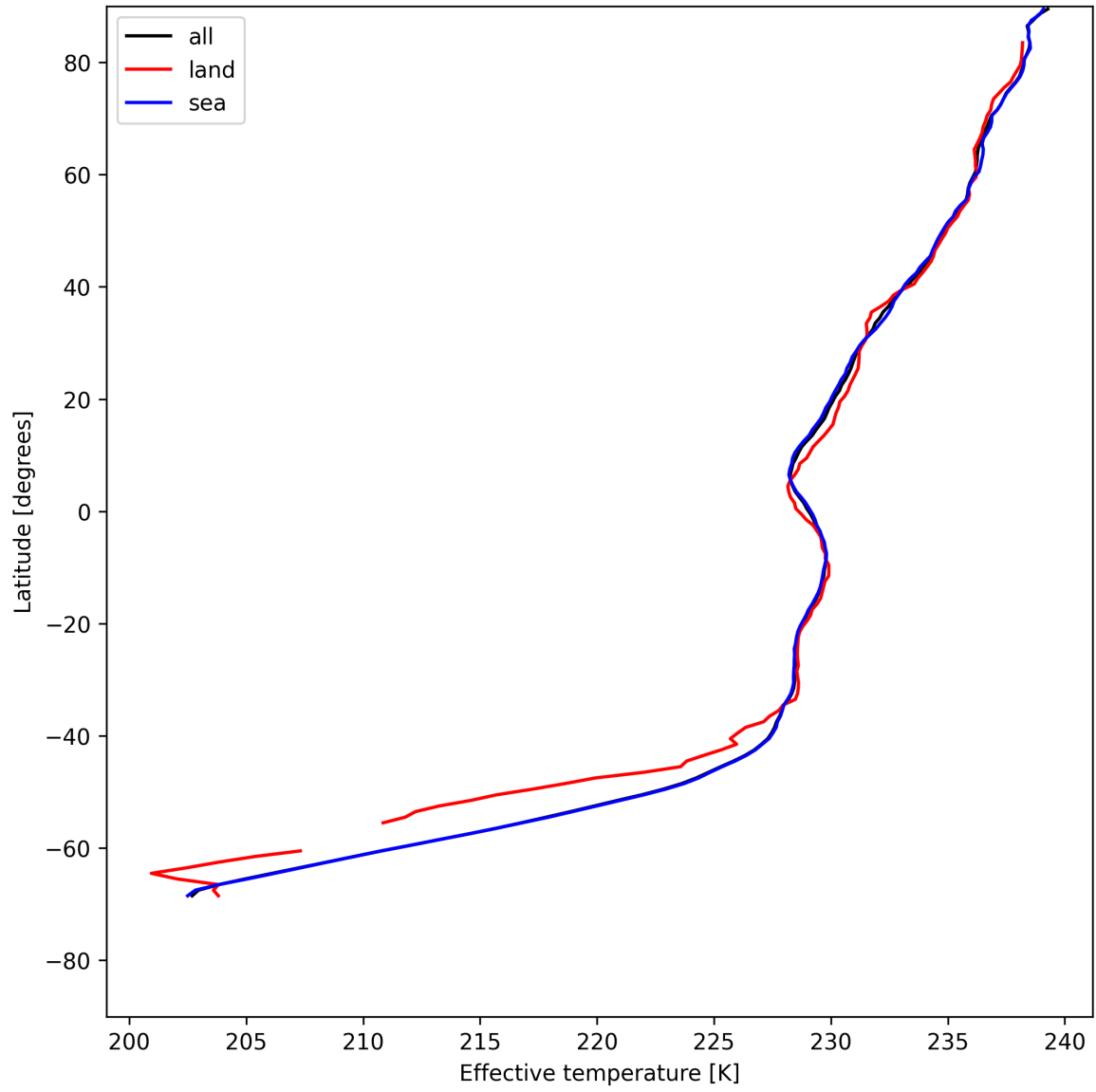
Figure 17: Zonal average of "Effective temperature" for 2025-07-20 to 2025-07-22.
