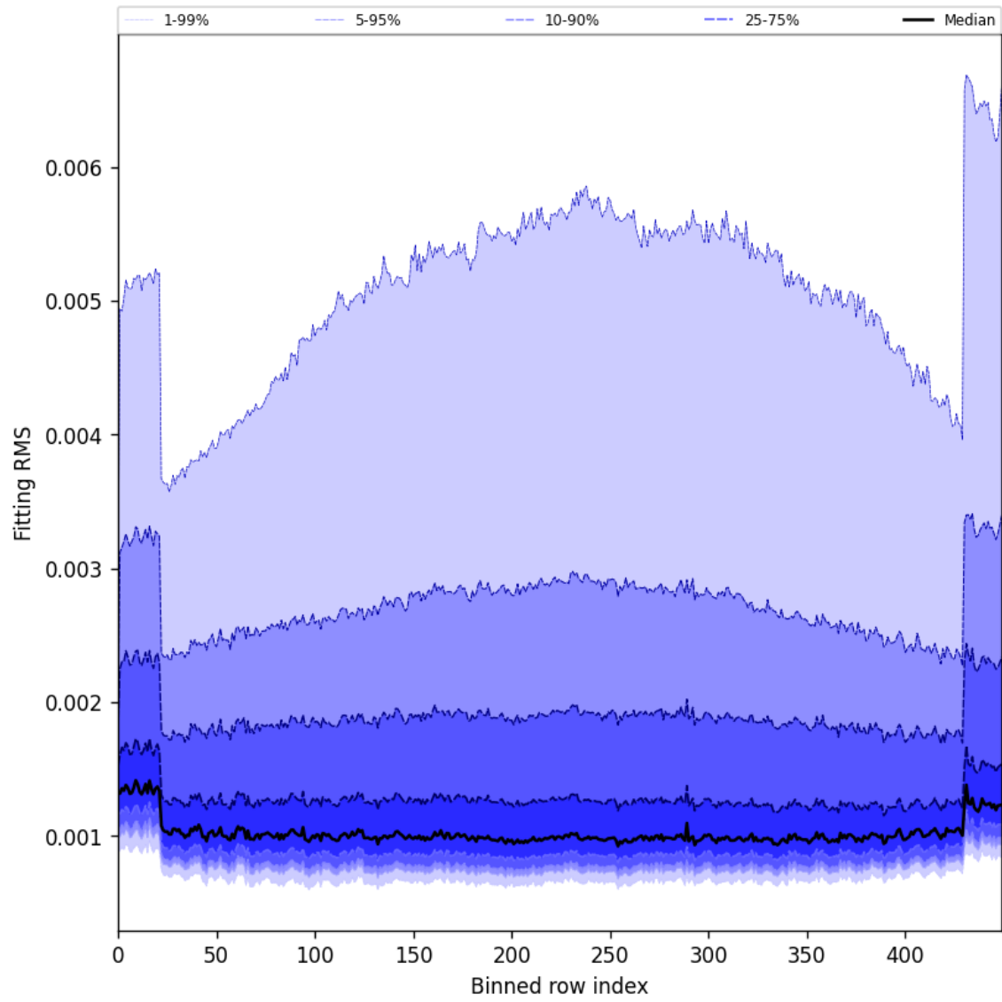
Figure 30: Along track statistics of “Fitting RMS” for 2025-07-20 to 2025-07-22
