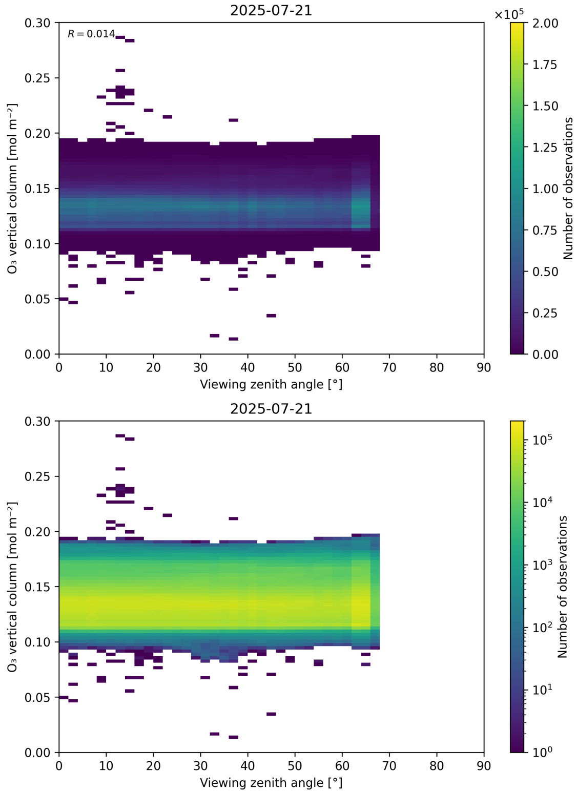
Figure 52: Scatter density plot of “Viewing zenith angle” against “O 3 vertical column” for 2025-07-20 to 2025-07-22.
