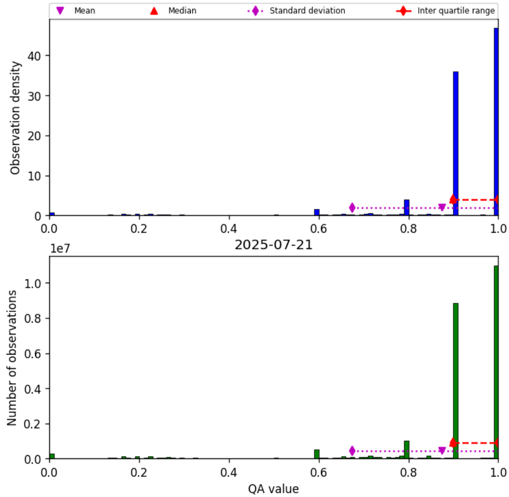
Figure 20: Histogram of “QA value” for 2025-07-20 to 2025-07-22
