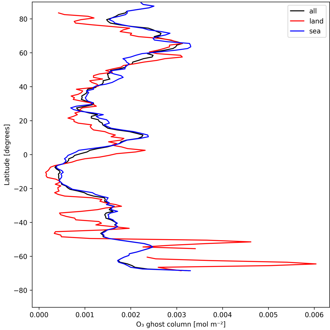
Figure 18: Zonal average of "O 3 ghost column" for 2025-07-20 to 2025-07-22.
