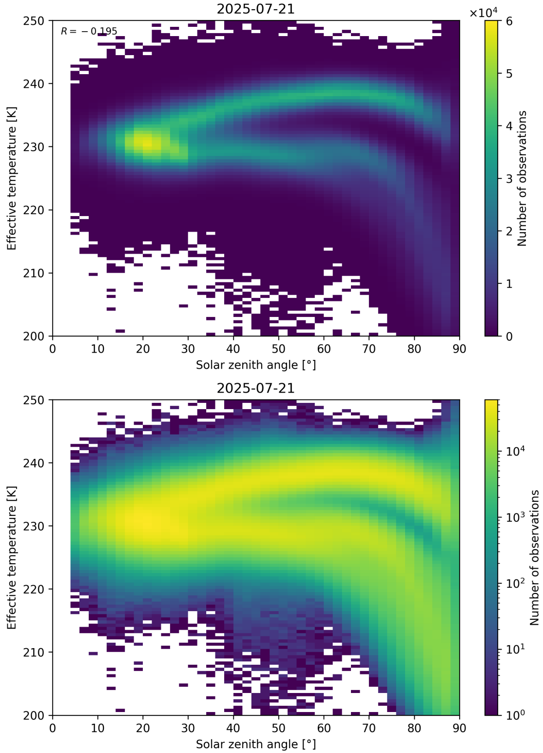
Figure 45: Scatter density plot of “Solar zenith angle” against “Effective temperature” for 2025-07-20 to 2025-07-22.
