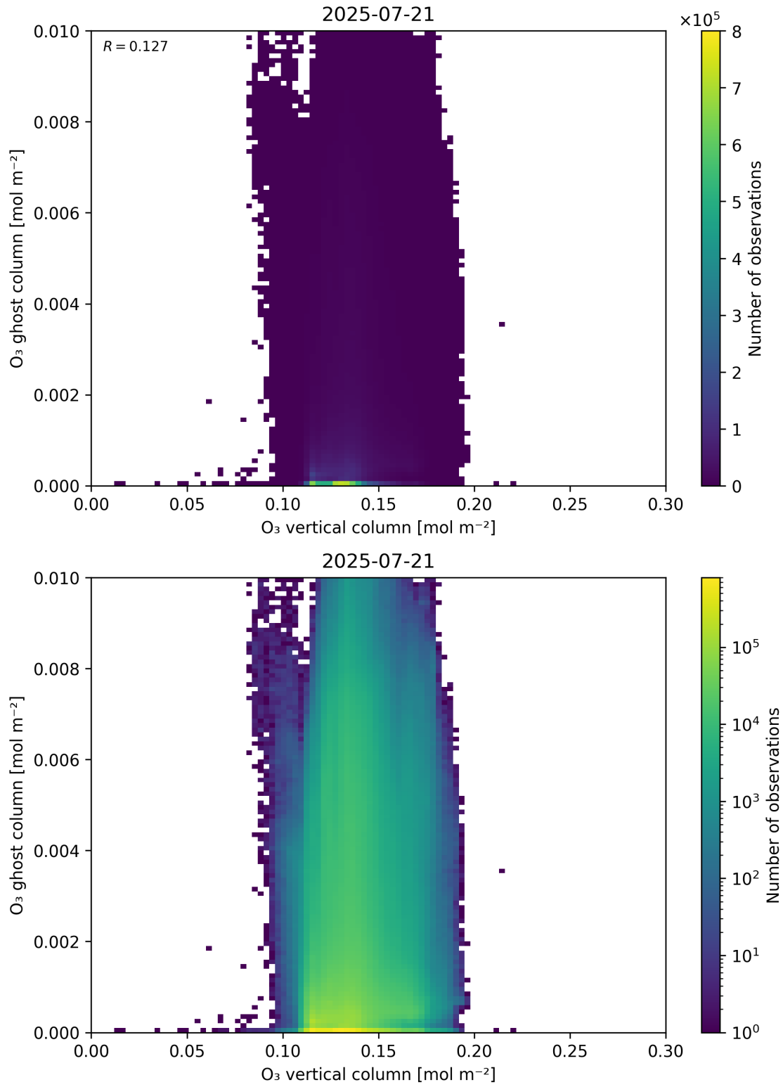
Figure 40: Scatter density plot of “O 3 vertical column” against “O 3 ghost column” for 2025-07-20 to 2025-07-22.
