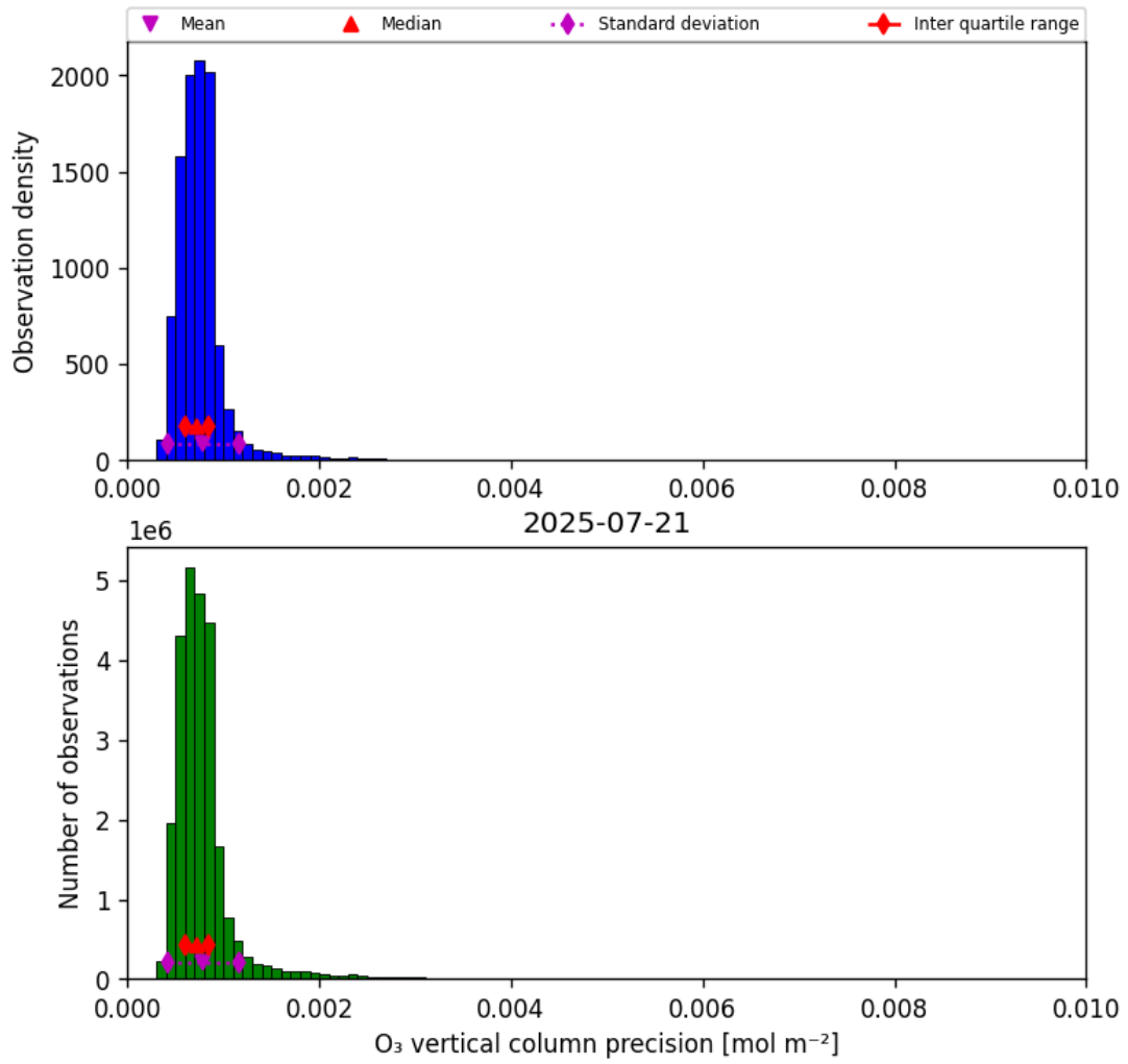
Figure 22: Histogram of “O 3 vertical column precision” for 2025-07-20 to 2025-07-22
