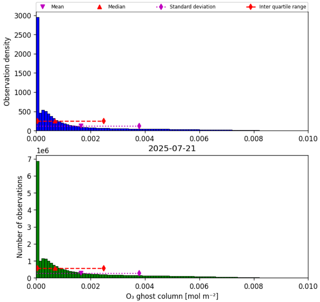
Figure 25: Histogram of “O 3 ghost column” for 2025-07-20 to 2025-07-22
