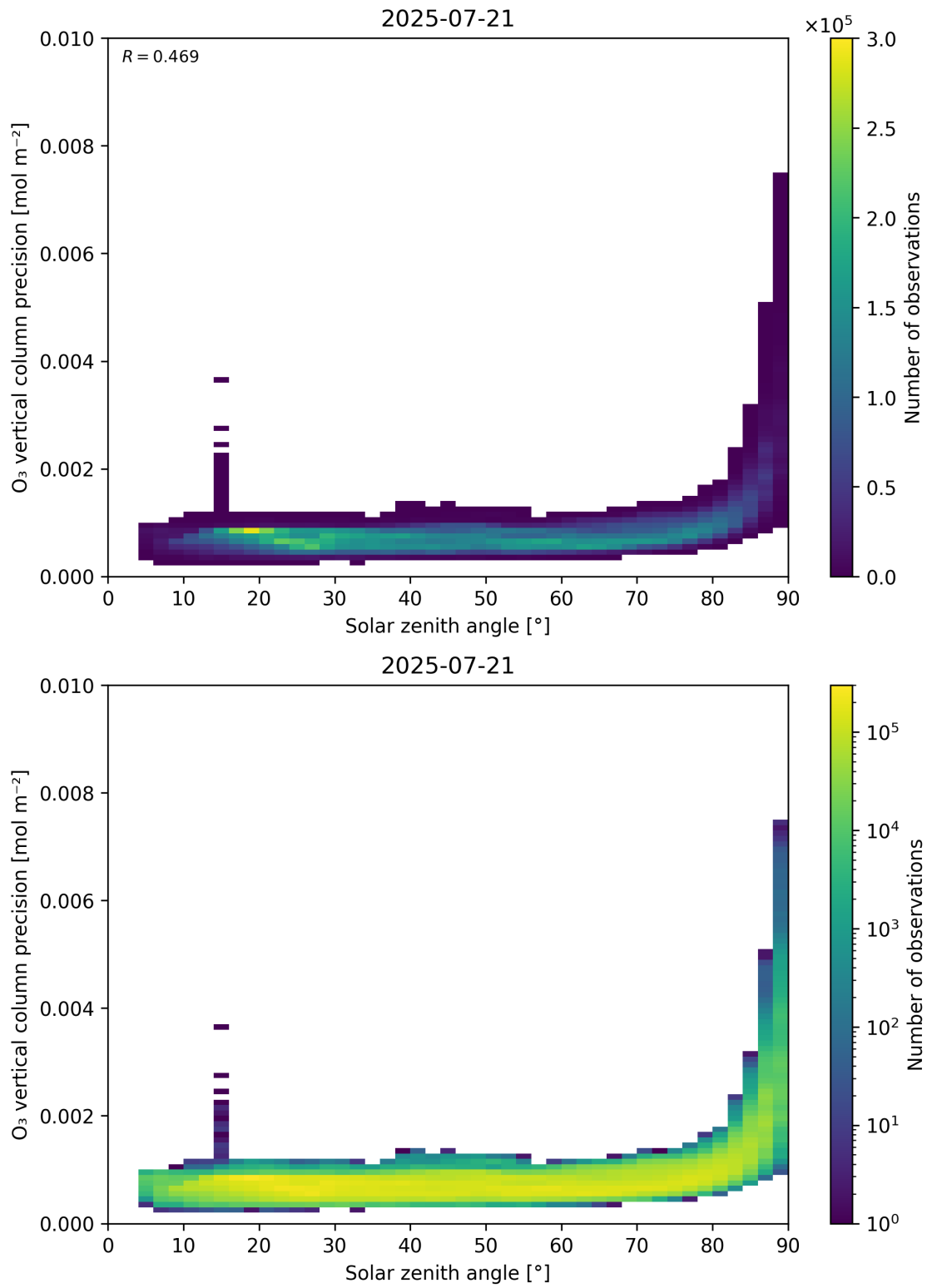
Figure 48: Scatter density plot of “Solar zenith angle” against “O 3 vertical column precision” for 2025-07-20 to 2025-07-22.
