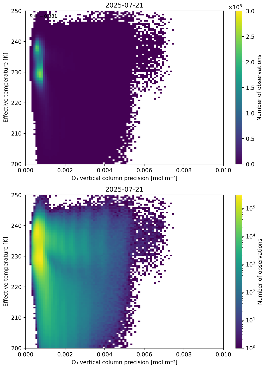
Figure 42: Scatter density plot of “O 3 vertical column precision” against “Effective temperature” for 2025-07-20 to 2025-07-22.
