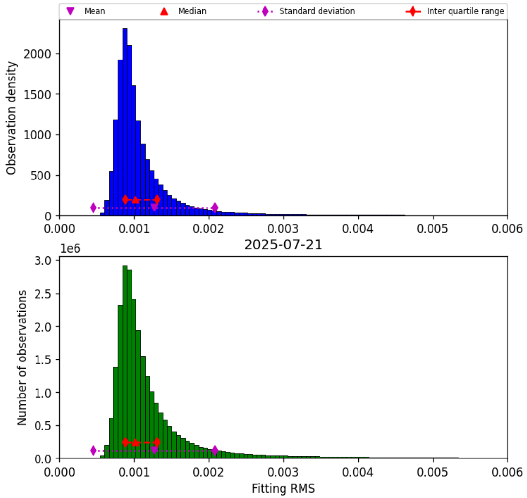
Figure 23: Histogram of “Fitting RMS” for 2025-07-20 to 2025-07-22
