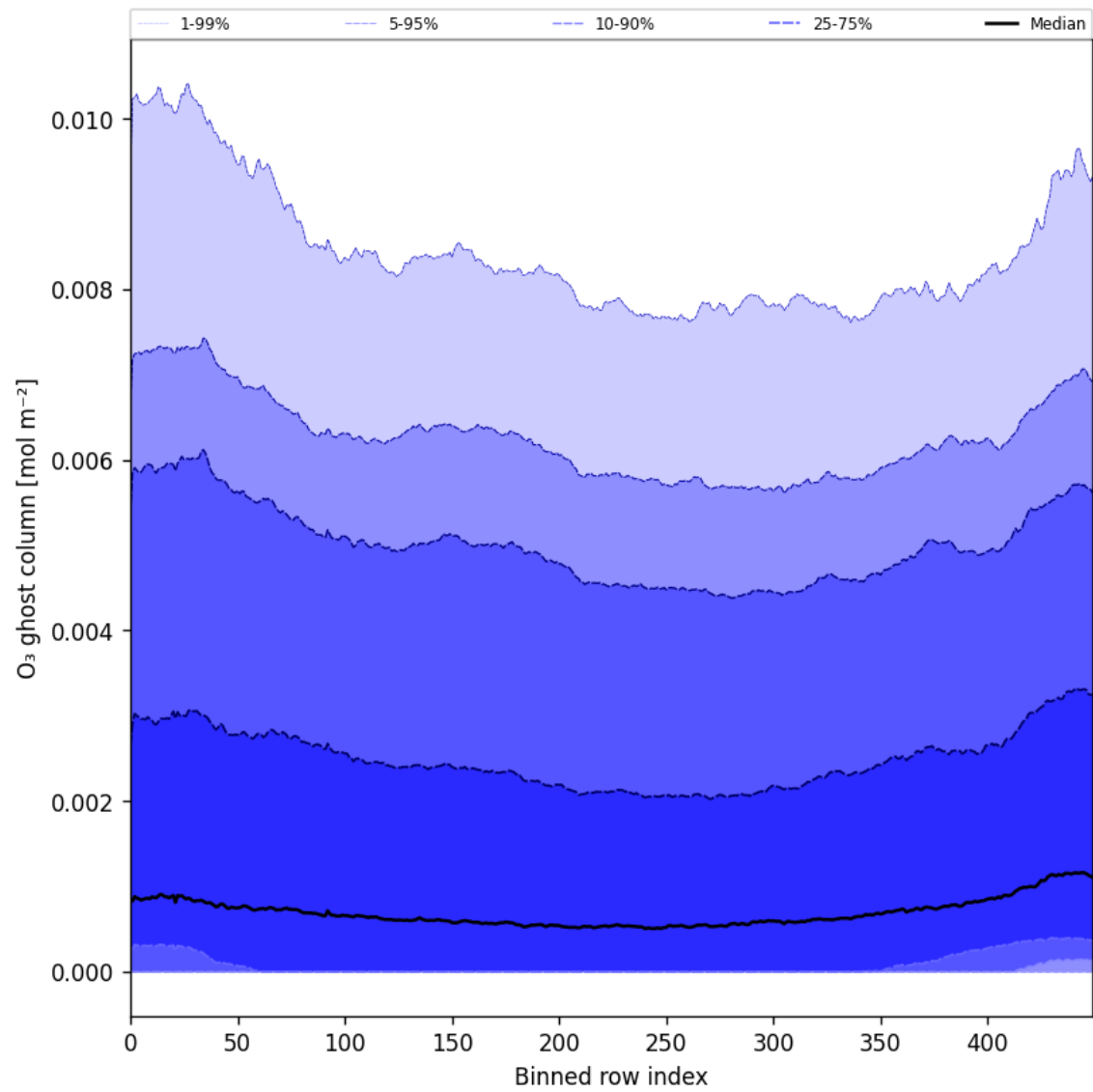
Figure 32: Along track statistics of “O 3 ghost column” for 2025-07-20 to 2025-07-22
