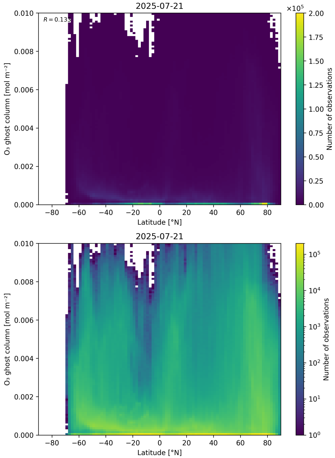
Figure 35: Scatter density plot of “Latitude” against “O 3 ghost column” for 2025-07-20 to 2025-07-22.
