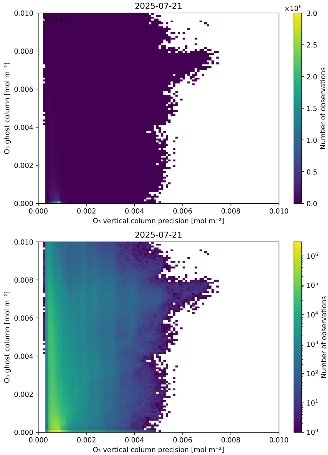
Figure 43: Scatter density plot of “O 3 vertical column precision” against “O 3 ghost column” for 2025-07-20 to 2025-07-22.
