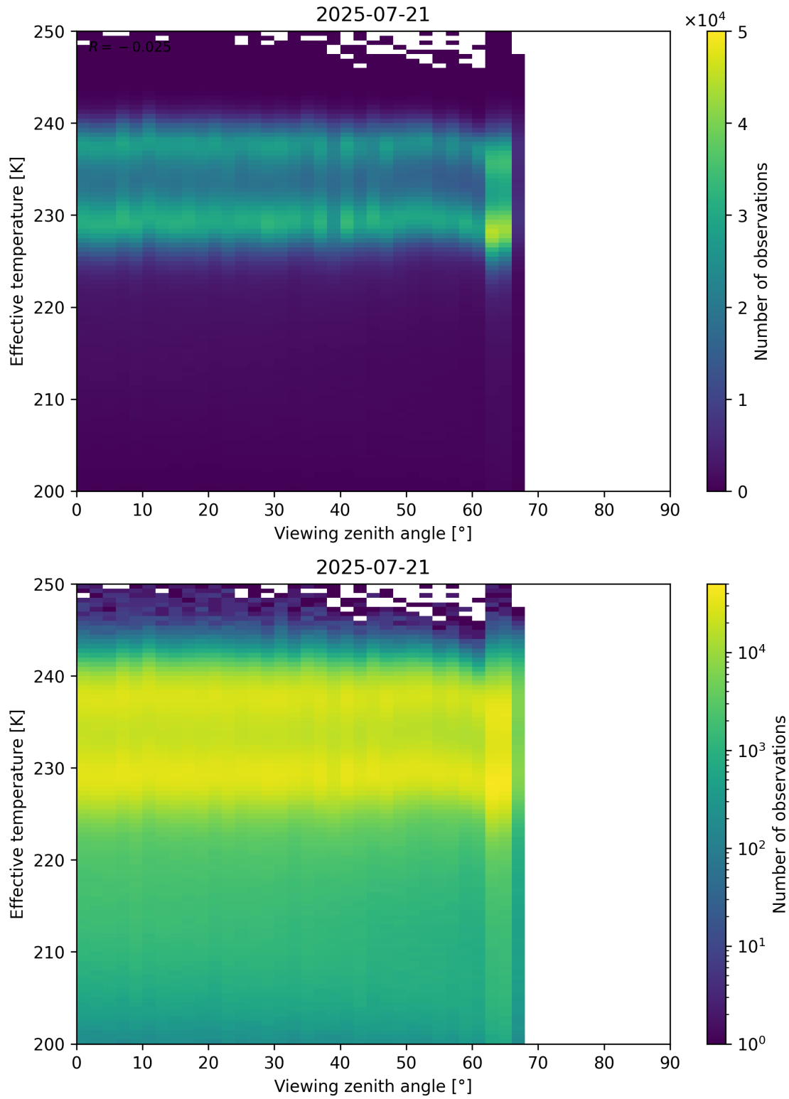
Figure 50: Scatter density plot of “Viewing zenith angle” against “Effective temperature” for 2025-07-20 to 2025-07-22.
