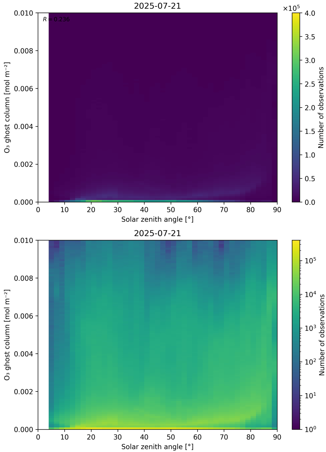
Figure 46: Scatter density plot of “Solar zenith angle” against “O 3 ghost column” for 2025-07-20 to 2025-07-22.
