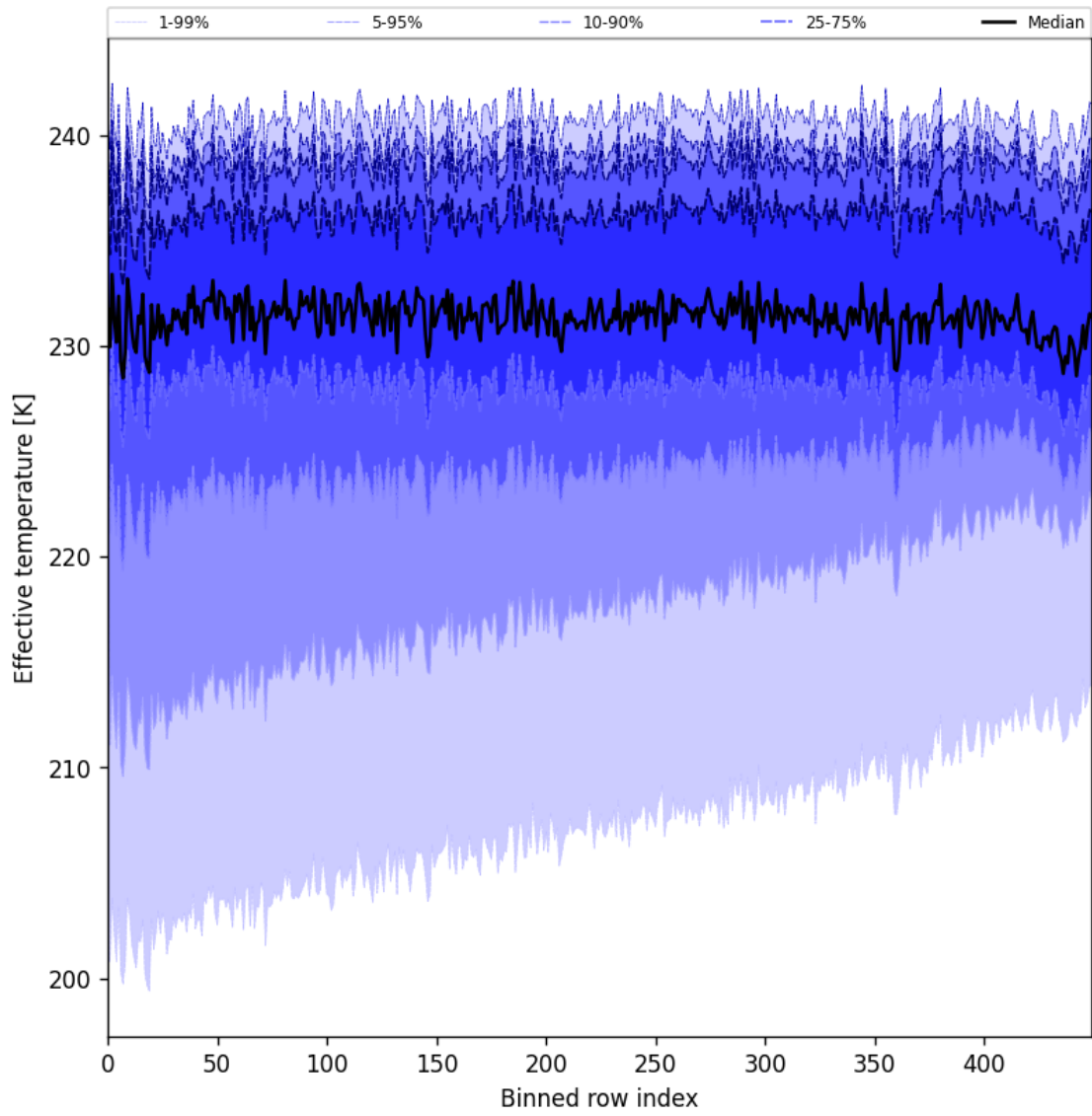
Figure 31: Along track statistics of “Effective temperature” for 2025-07-20 to 2025-07-22
