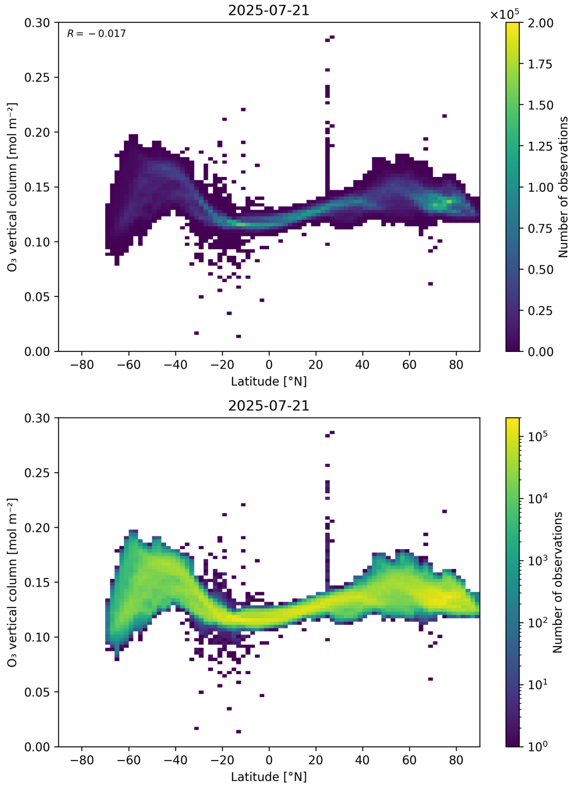
Figure 36: Scatter density plot of “Latitude” against “O 3 vertical column” for 2025-07-20 to 2025-07-22.
