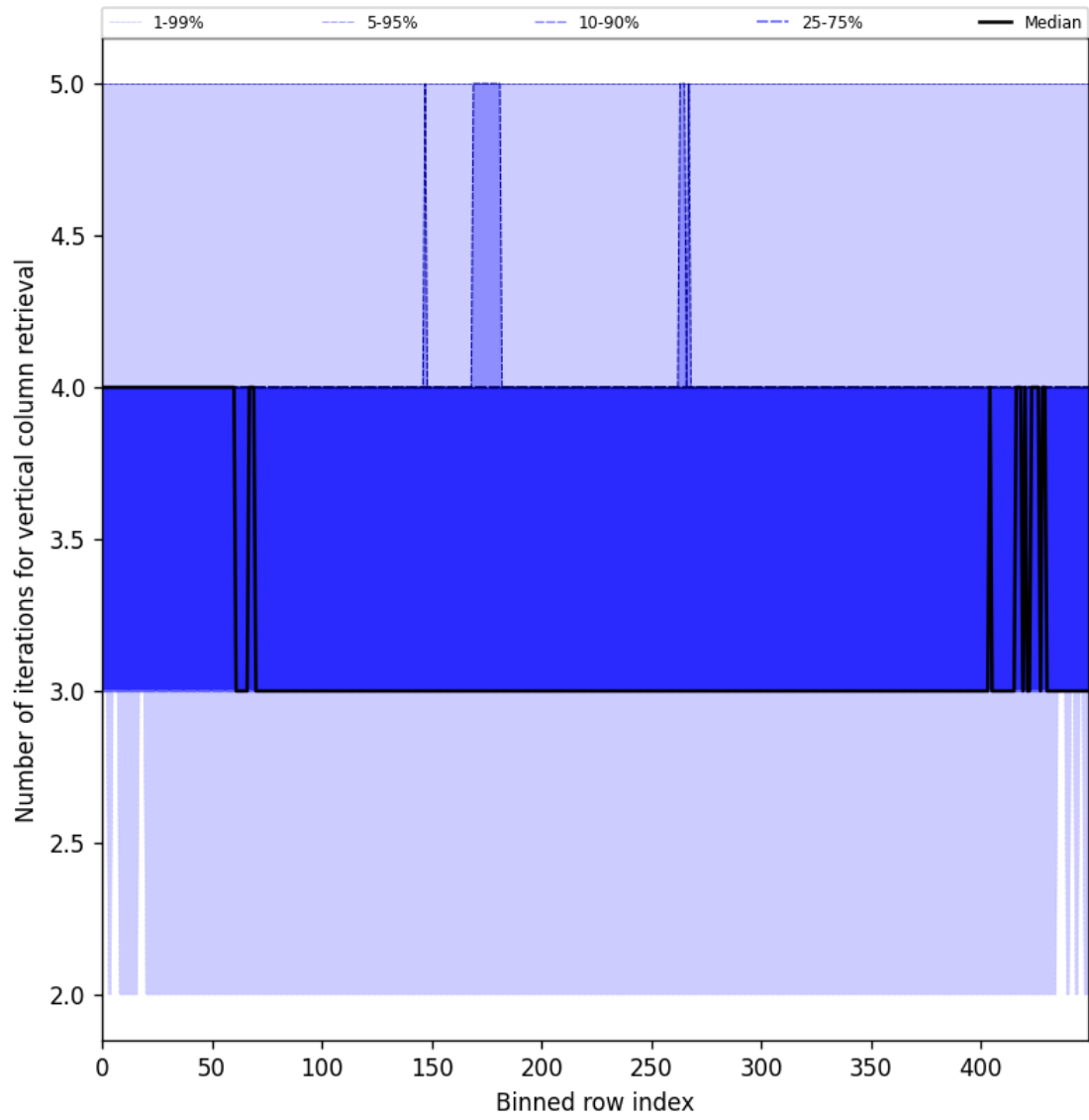
Figure 33: Along track statistics of “Number of iterations for vertical column retrieval” for 2025-07-20 to 2025-07-22
