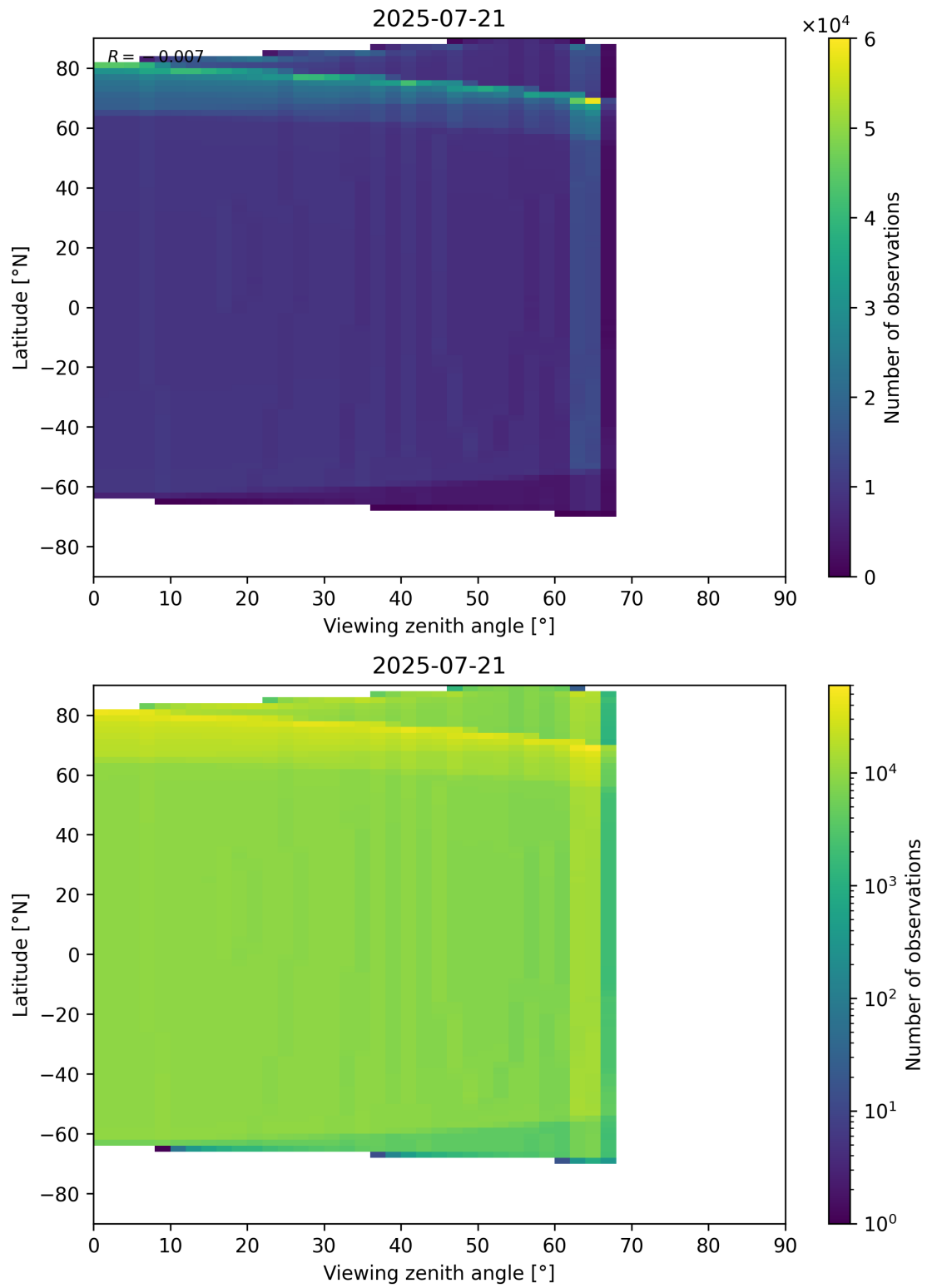
Figure 49: Scatter density plot of “Viewing zenith angle” against “Latitude” for 2025-07-20 to 2025-07-22.
