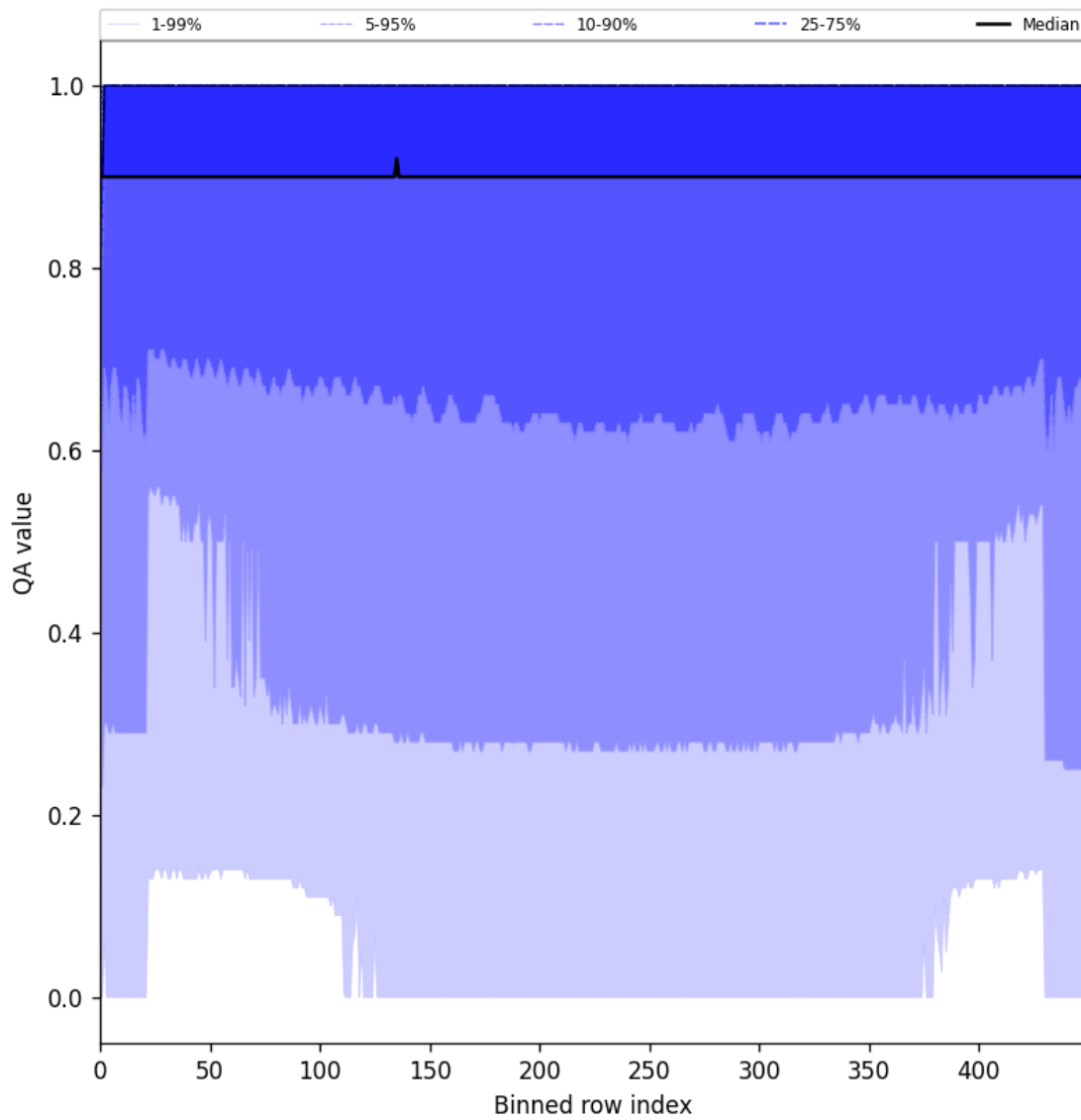
Figure 27: Along track statistics of “QA value” for 2025-07-20 to 2025-07-22
