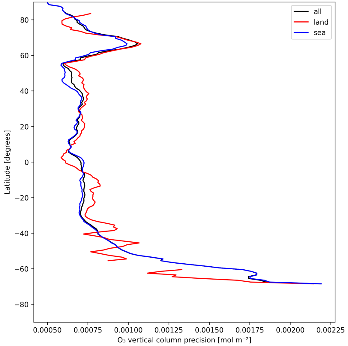
Figure 15: Zonal average of “O 3 vertical column precision” for 2025-07-20 to 2025-07-22.
