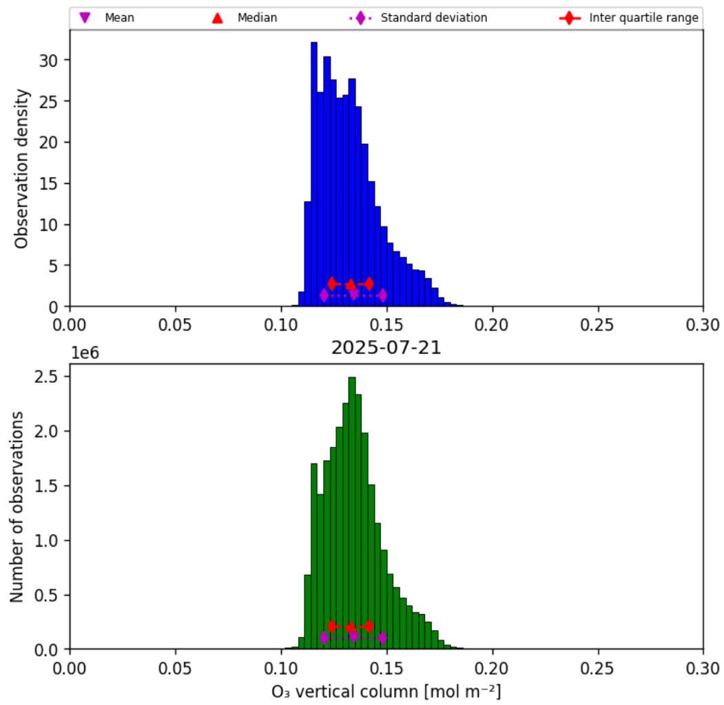
Figure 21: Histogram of “O 3 vertical column” for 2025-07-20 to 2025-07-22
