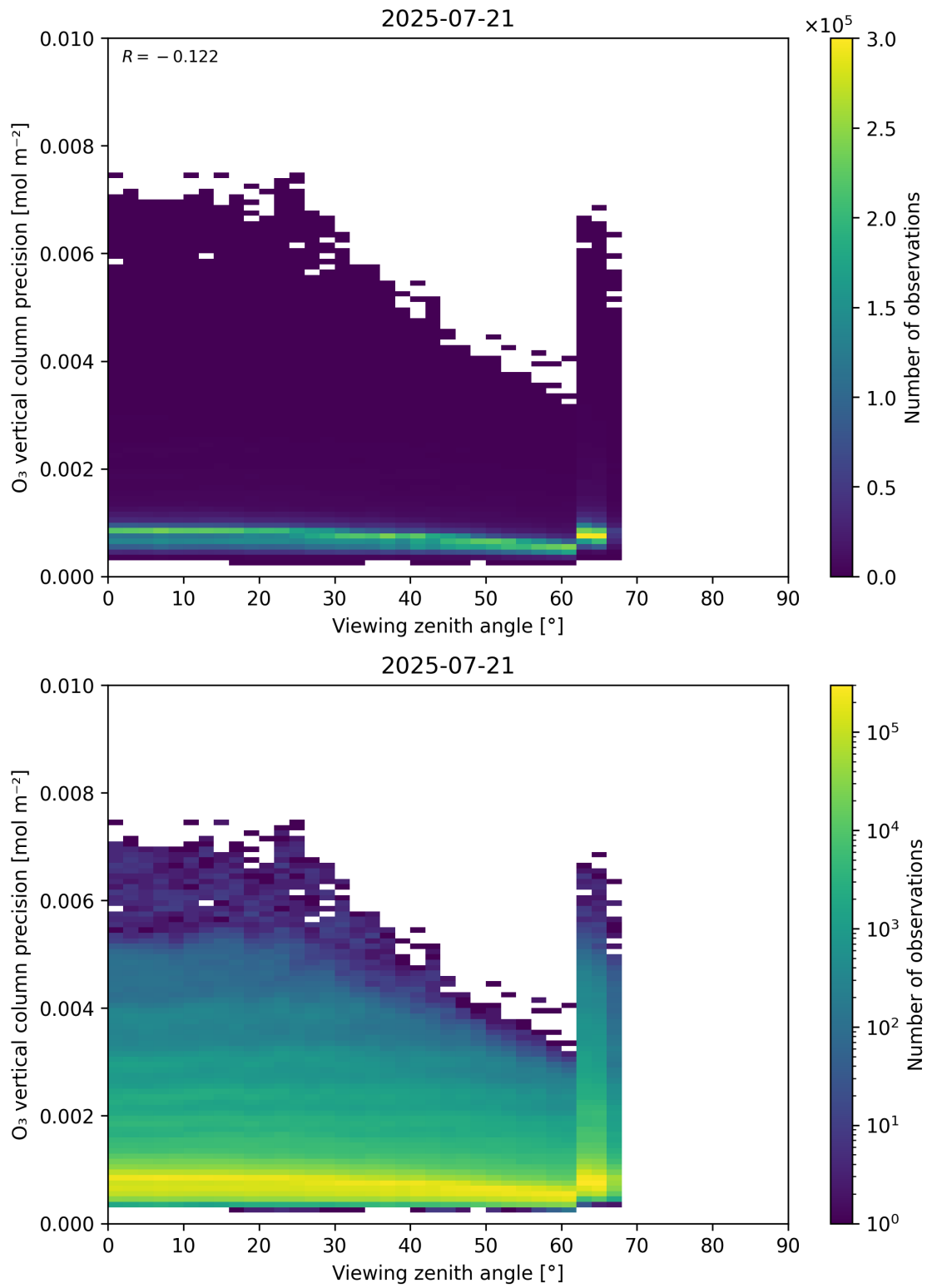
Figure 53: Scatter density plot of “Viewing zenith angle” against “O 3 vertical column precision” for 2025-07-20 to 2025-07-22.
