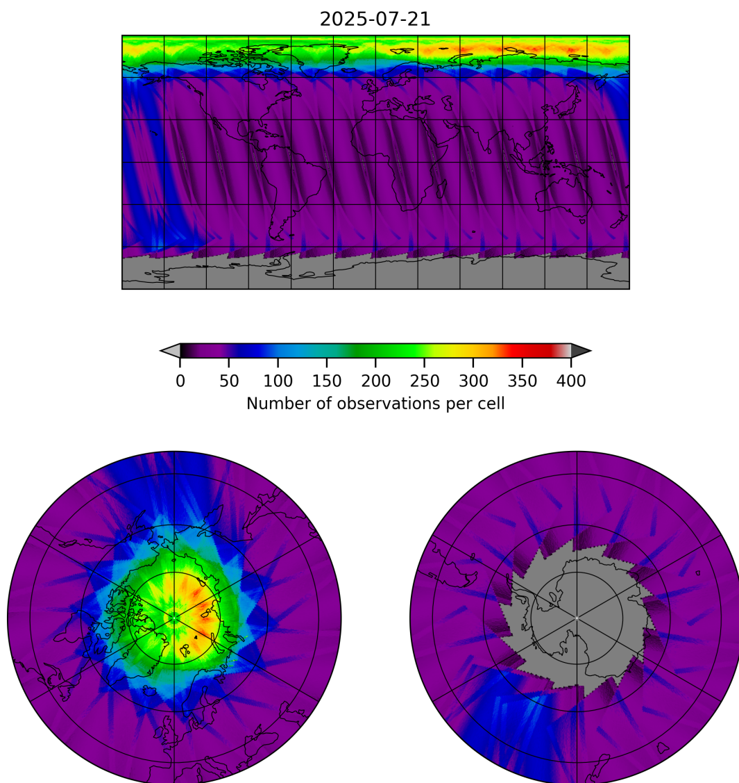
Figure 12: Map of the number of observations for 2025-07-20 to 2025-07-22
