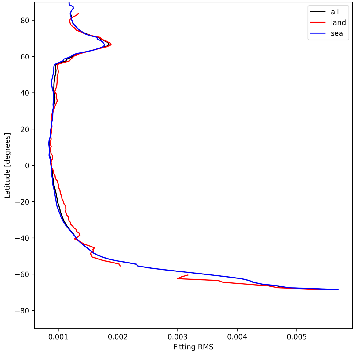
Figure 16: Zonal average of “Fitting RMS” for 2025-07-20 to 2025-07-22.
