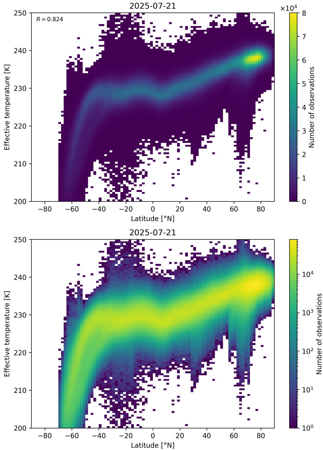
Figure 34: Scatter density plot of “Latitude” against “Effective temperature” for 2025-07-20 to 2025-07-22.
