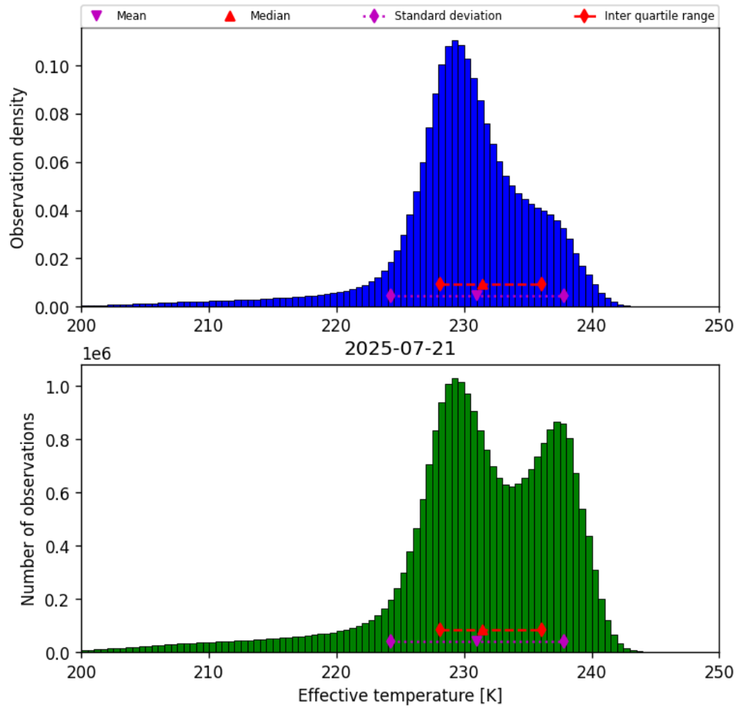
Figure 24: Histogram of “Effective temperature” for 2025-07-20 to 2025-07-22
