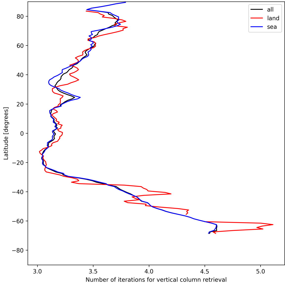
Figure 19: Zonal average of “Number of iterations for vertical column retrieval” for 2025-07-20 to 2025-07-22.
