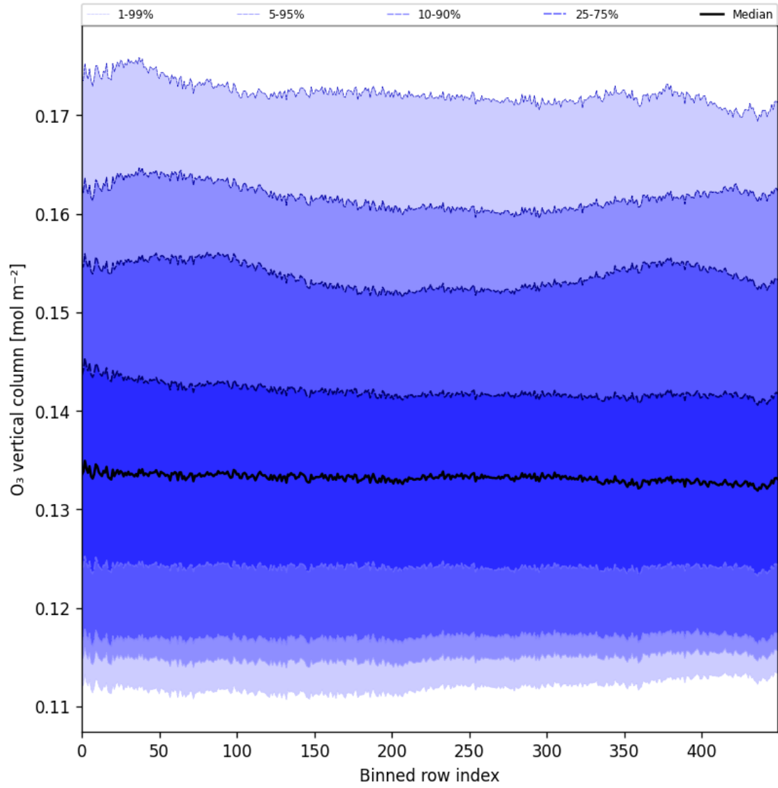
Figure 28: Along track statistics of “O 3 vertical column” for 2025-07-20 to 2025-07-22
