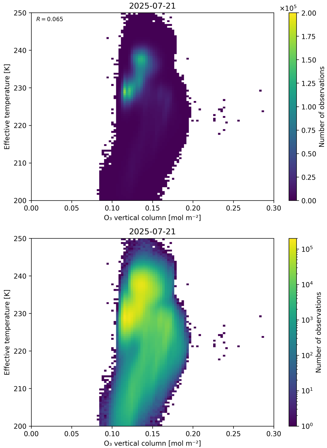
Figure 39: Scatter density plot of “O 3 vertical column” against “Effective temperature” for 2025-07-20 to 2025-07-22.
