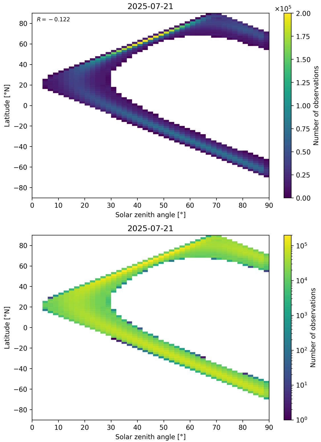
Figure 44: Scatter density plot of “Solar zenith angle” against “Latitude” for 2025-07-20 to 2025-07-22.
