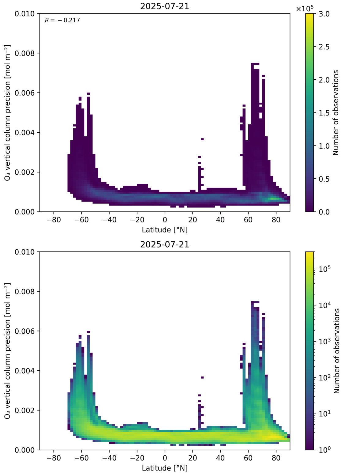
Figure 37: Scatter density plot of “Latitude” against “O 3 vertical column precision” for 2025-07-20 to 2025-07-22.
