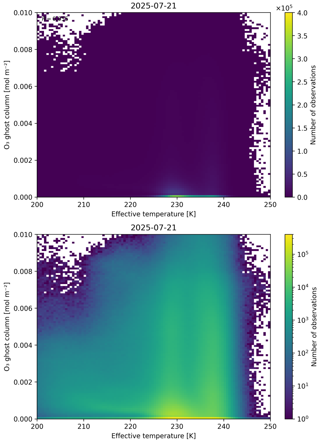
Figure 38: Scatter density plot of “Effective temperature” against “O 3 ghost column” for 2025-07-20 to 2025-07-22.
