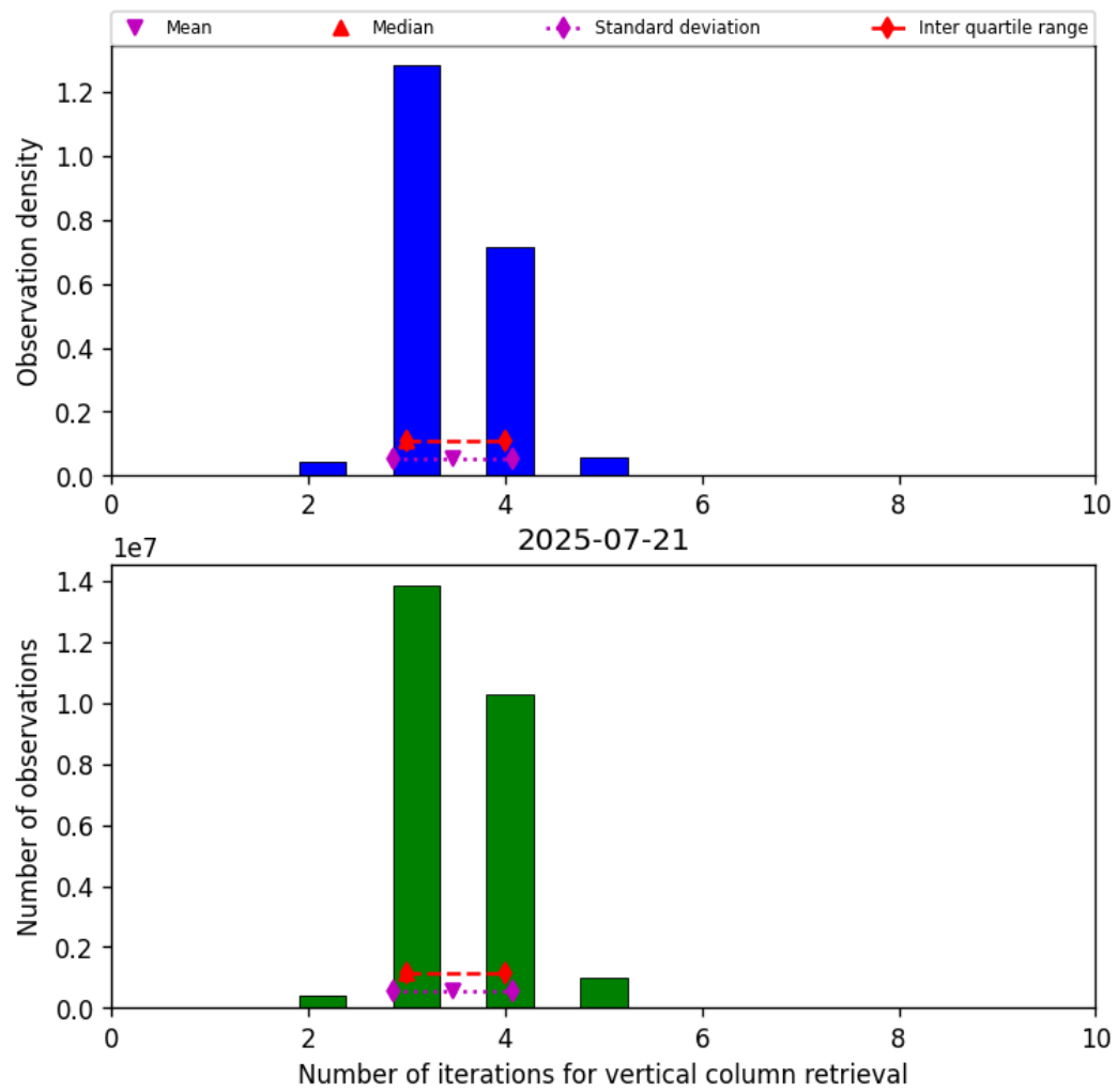
Figure 26: Histogram of “Number of iterations for vertical column retrieval” for 2025-07-20 to 2025-07-22
