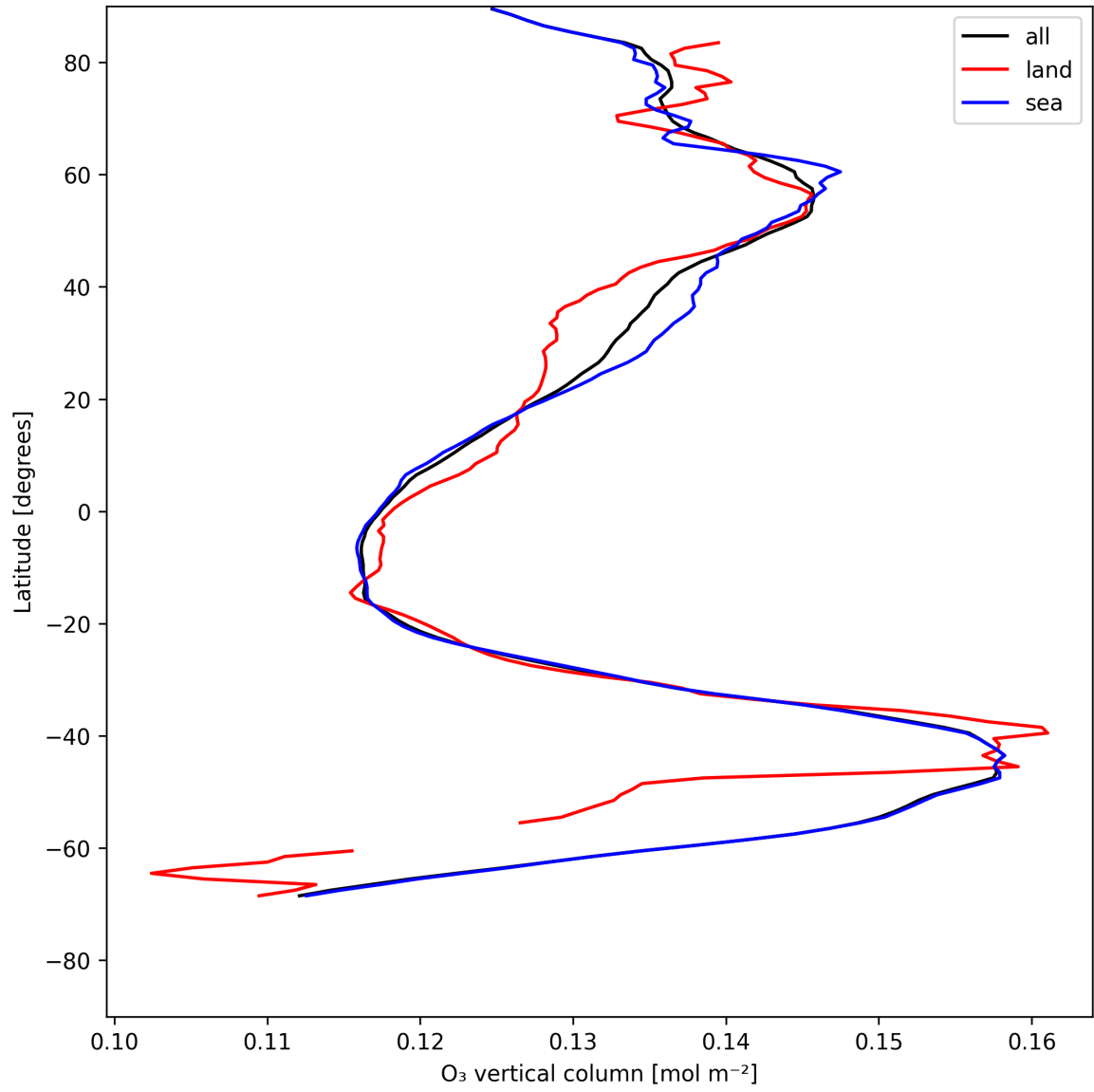
Figure 14: Zonal average of “O 3 vertical column” for 2025-07-20 to 2025-07-22.
