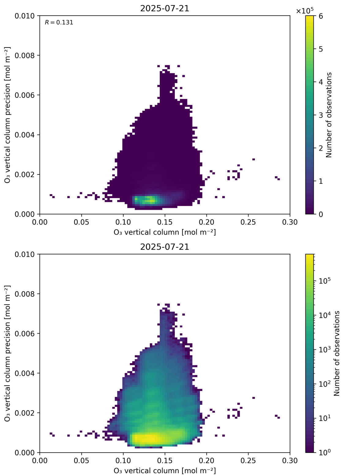
Figure 41: Scatter density plot of “O 3 vertical column” against “O 3 vertical column precision” for 2025-07-20 to 2025-07-22.
