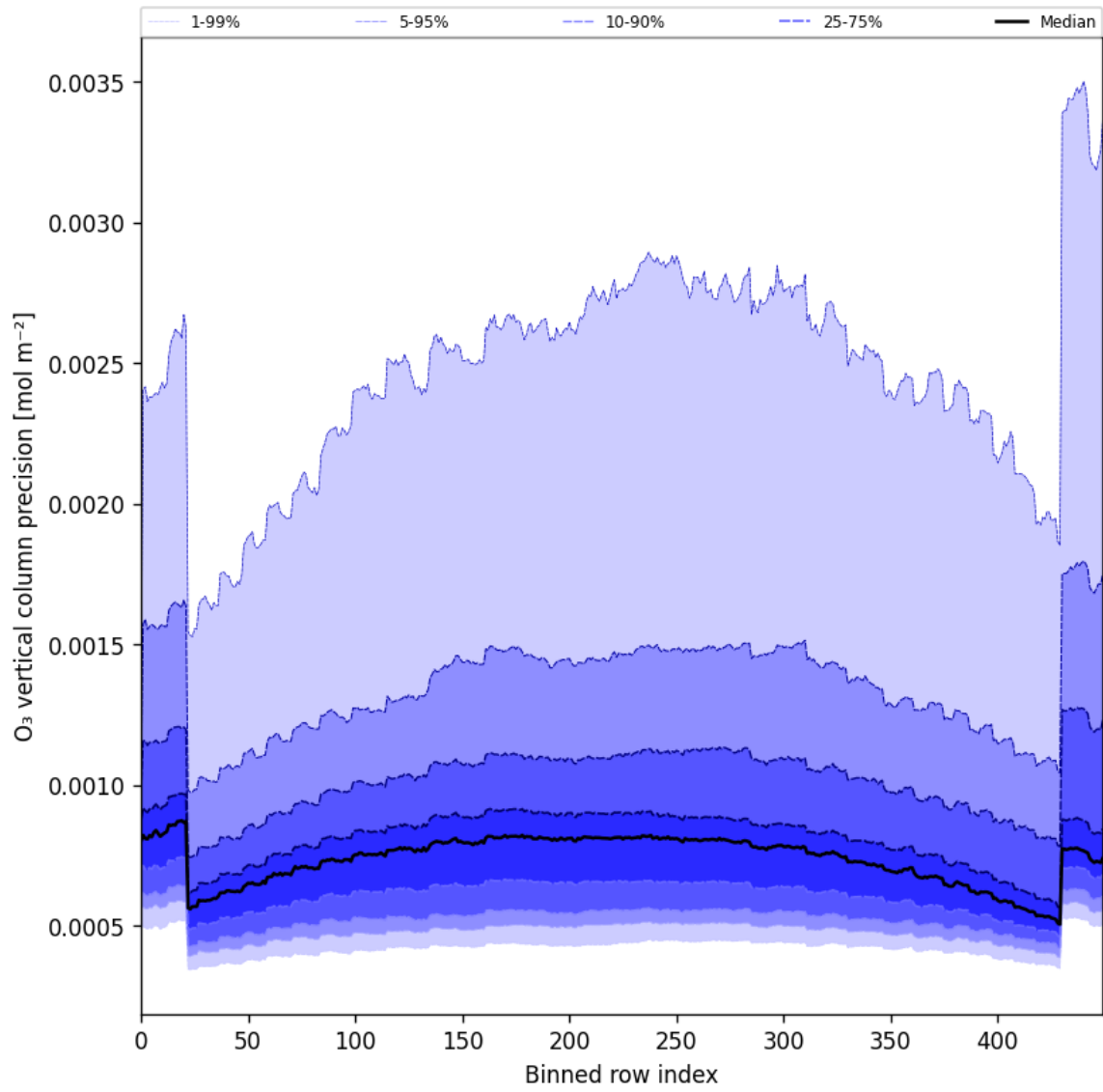
Figure 29: Along track statistics of “O 3 vertical column precision” for 2025-07-20 to 2025-07-22
