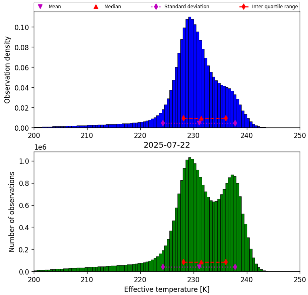
Figure 24: Histogram of “Effective temperature” for 2025-07-21 to 2025-07-23
