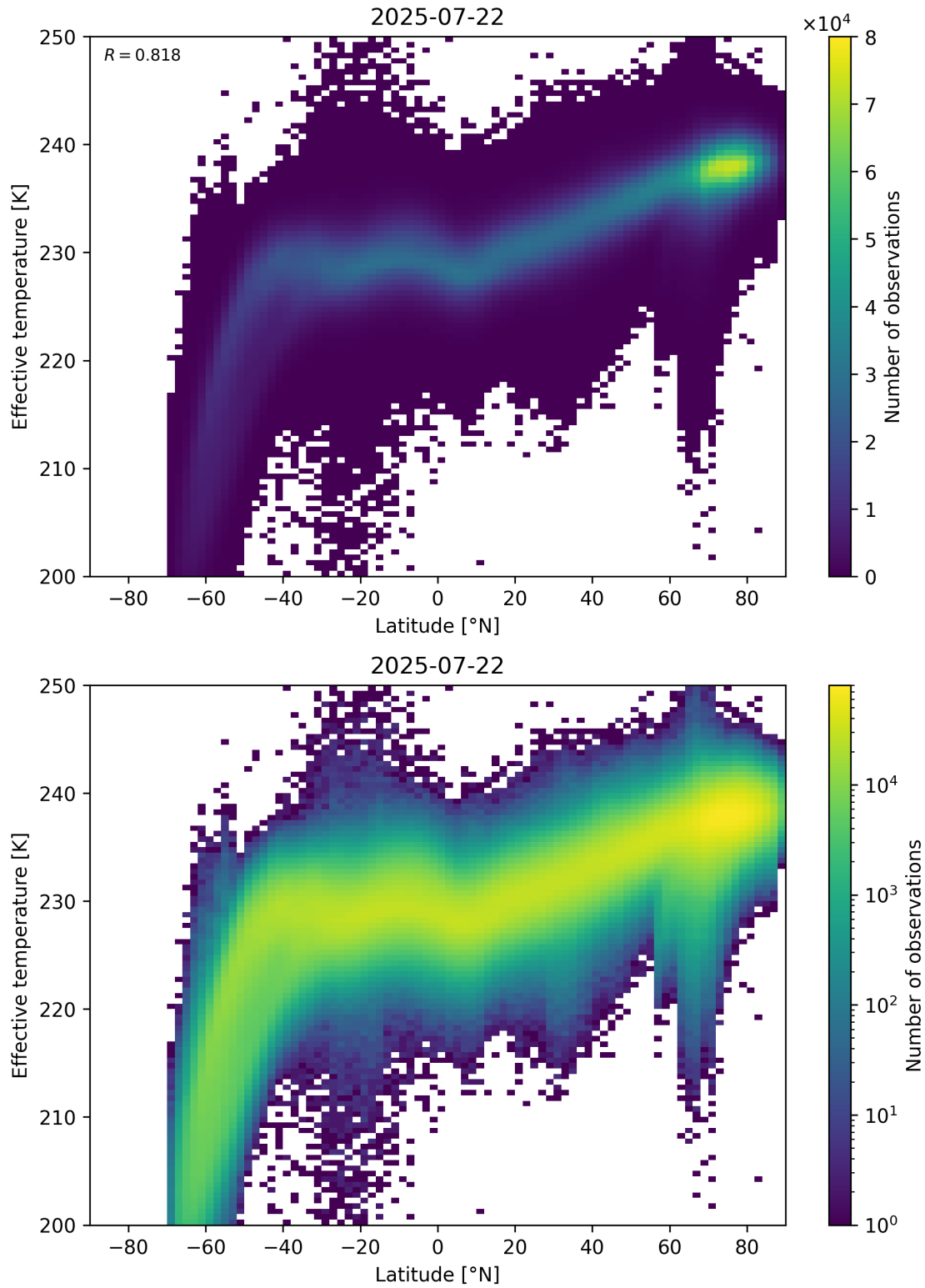
Figure 34: Scatter density plot of “Latitude” against “Effective temperature” for 2025-07-21 to 2025-07-23.
