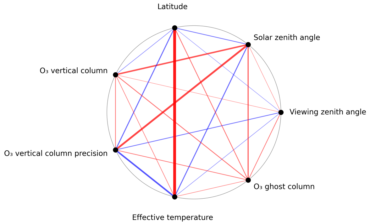
Figure 1: Map of correlation graph for 2025-07-21 to 2025-07-23.
