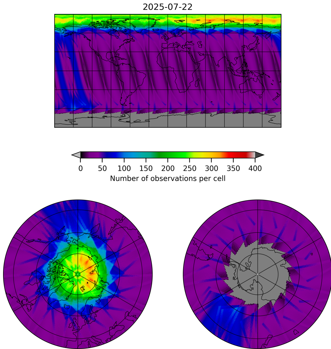
Figure 12: Map of the number of observations for 2025-07-21 to 2025-07-23
