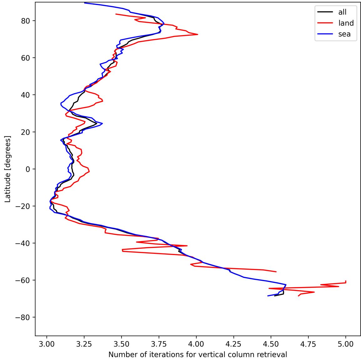
Figure 19: Zonal average of “Number of iterations for vertical column retrieval” for 2025-07-21 to 2025-07-23.
