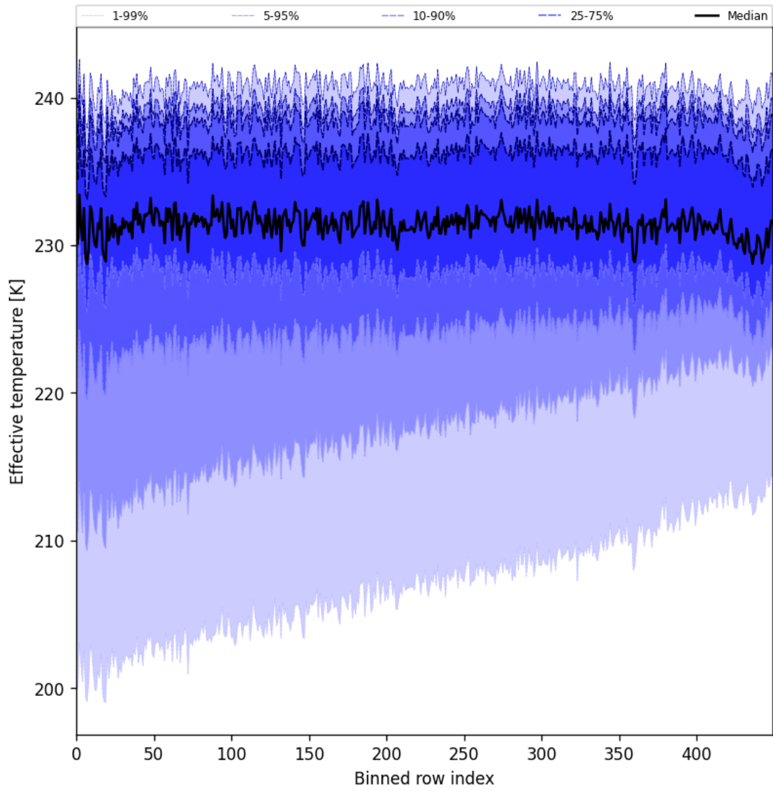
Figure 31: Along track statistics of “Effective temperature” for 2025-07-21 to 2025-07-23
