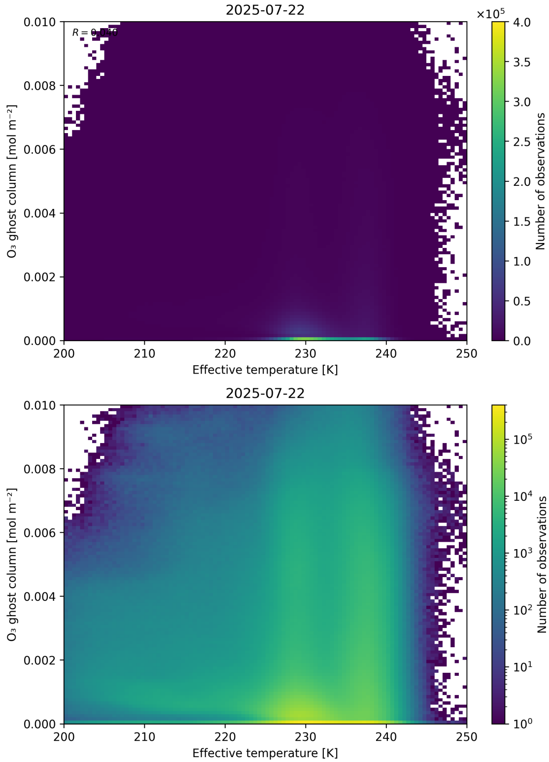
Figure 38: Scatter density plot of “Effective temperature” against “O 3 ghost column” for 2025-07-21 to 2025-07-23.
