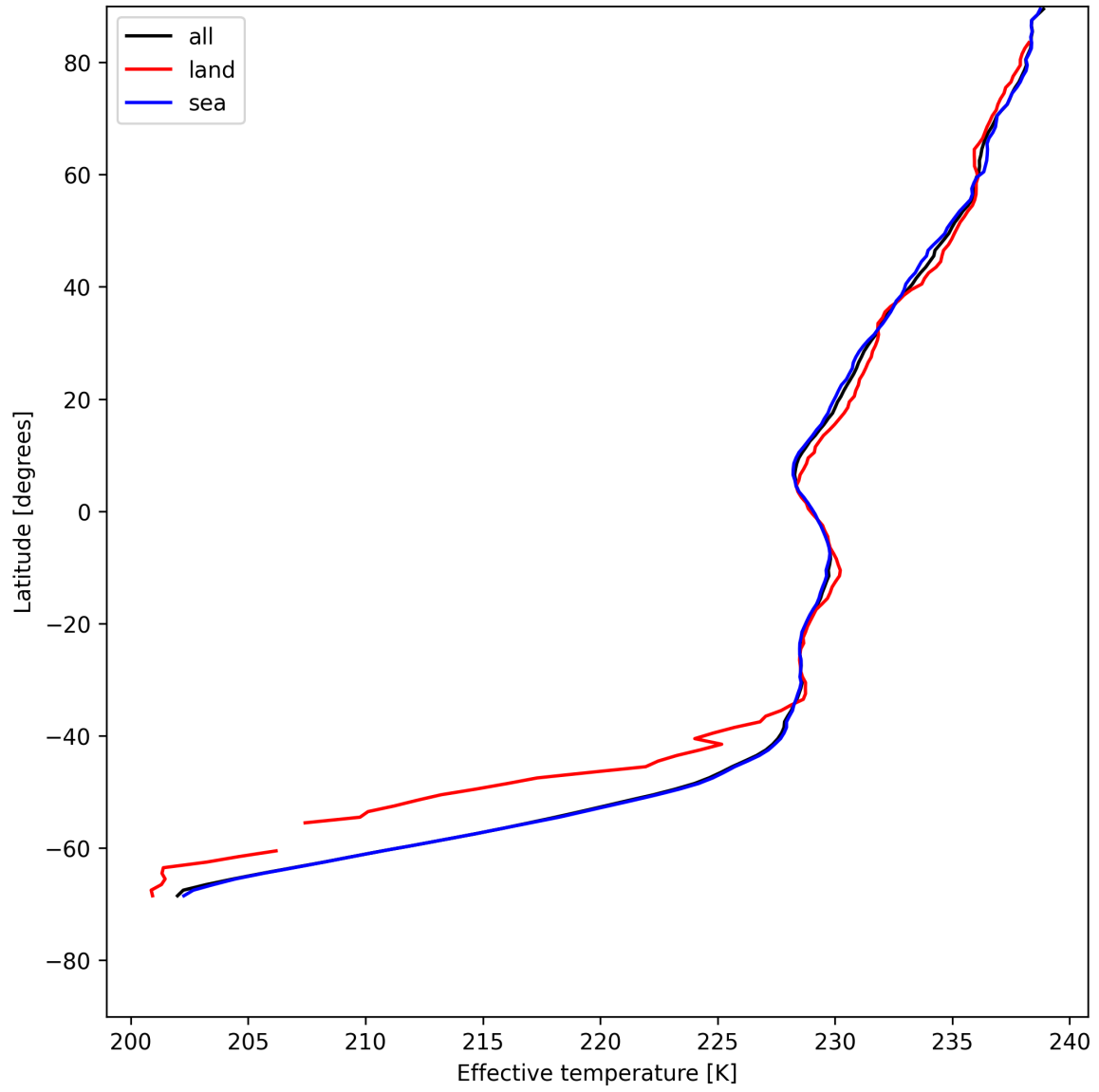
Figure 17: Zonal average of "Effective temperature" for 2025-07-21 to 2025-07-23.
