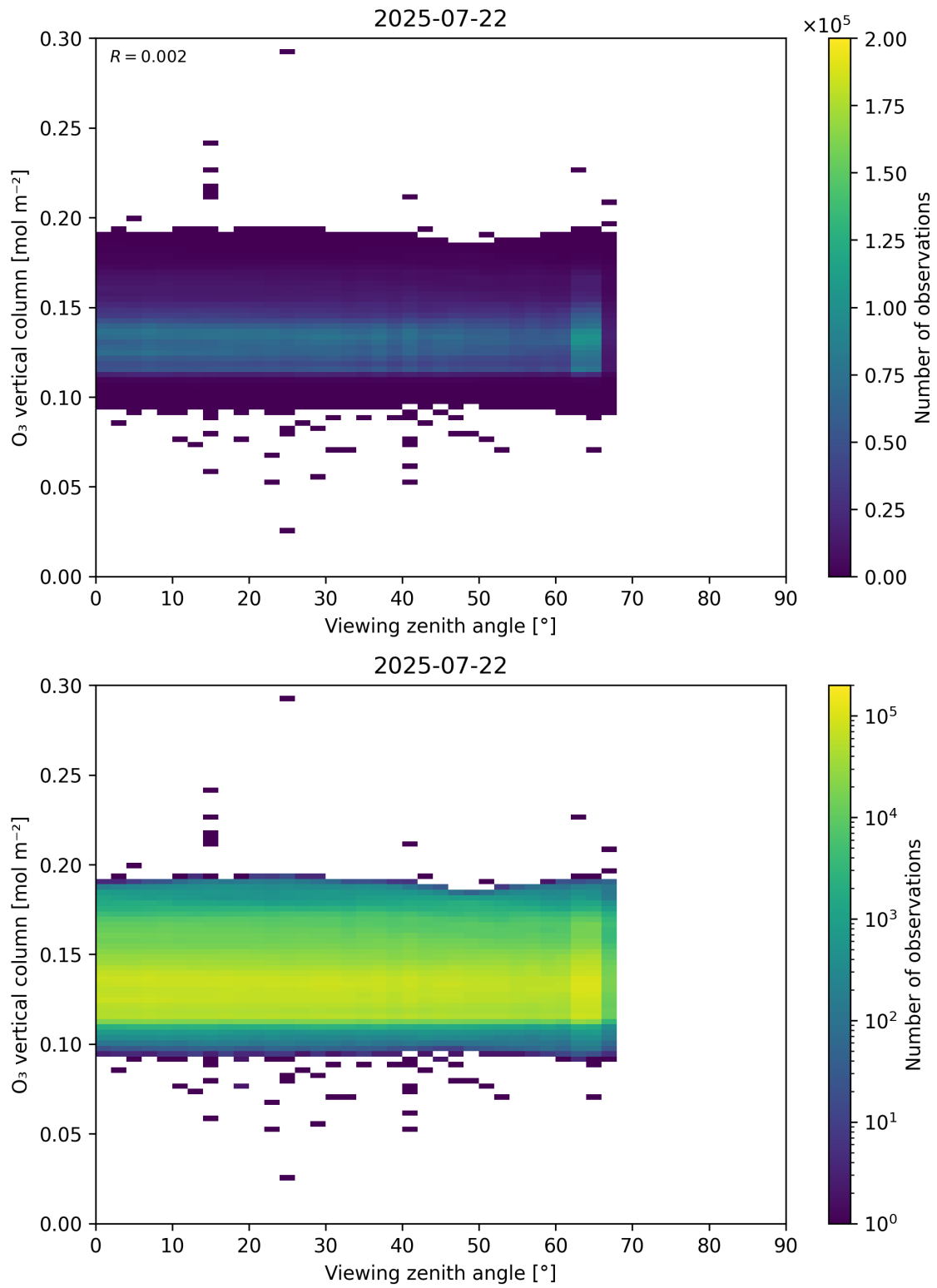
Figure 52: Scatter density plot of “Viewing zenith angle” against “O 3 vertical column” for 2025-07-21 to 2025-07-23.
