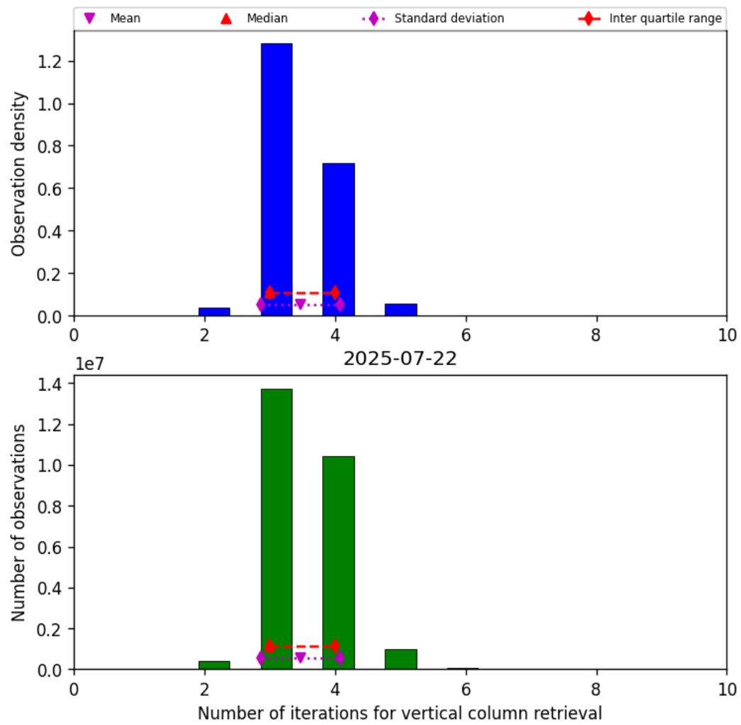
Figure 26: Histogram of “Number of iterations for vertical column retrieval” for 2025-07-21 to 2025-07-23
