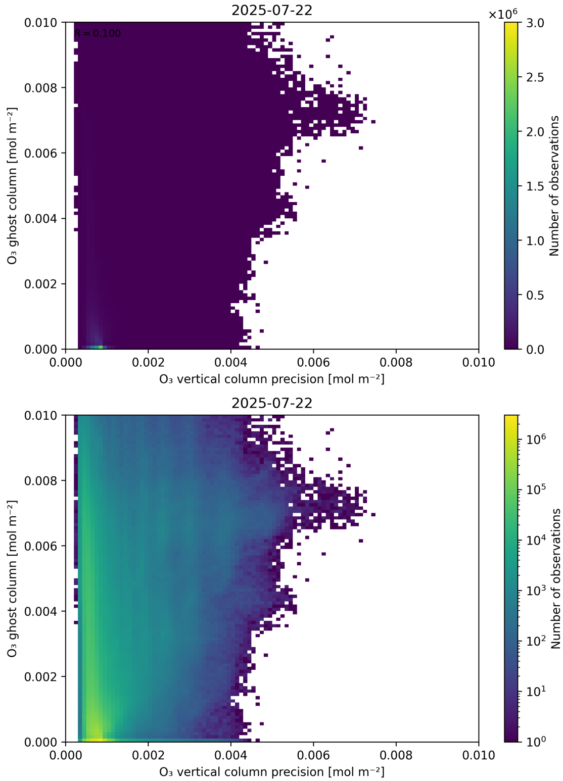
Figure 43: Scatter density plot of “O 3 vertical column precision” against “O 3 ghost column” for 2025-07-21 to 2025-07-23.
