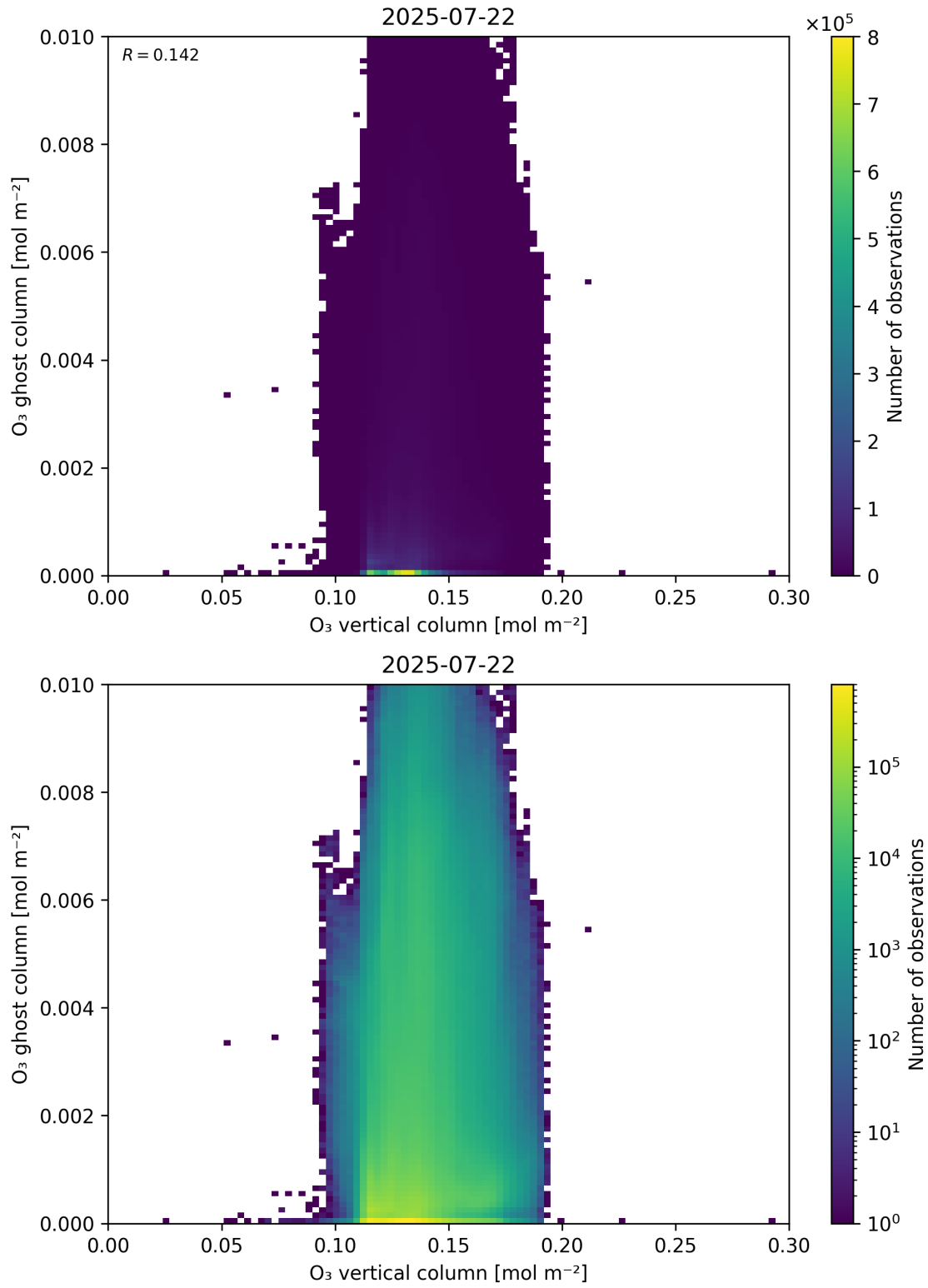
Figure 40: Scatter density plot of “O 3 vertical column” against “O 3 ghost column” for 2025-07-21 to 2025-07-23.
