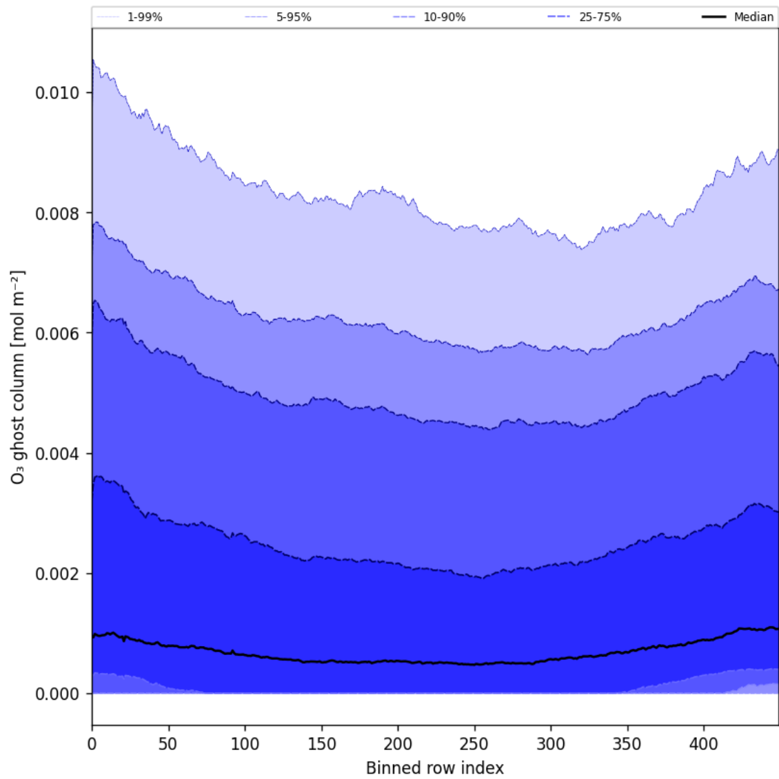
Figure 32: Along track statistics of “O 3 ghost column” for 2025-07-21 to 2025-07-23
