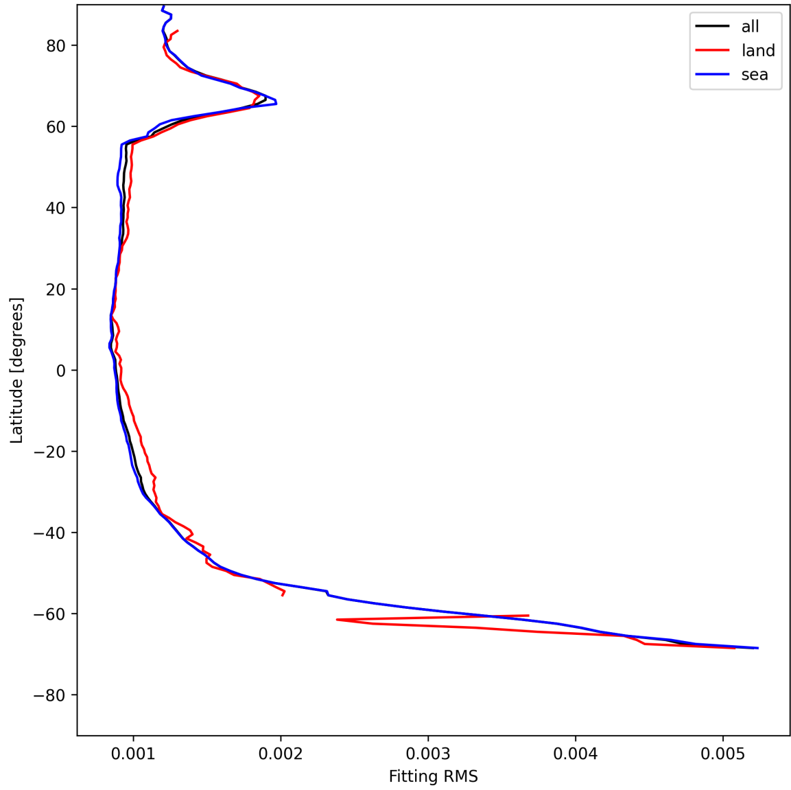
Figure 16: Zonal average of “Fitting RMS” for 2025-07-21 to 2025-07-23.
