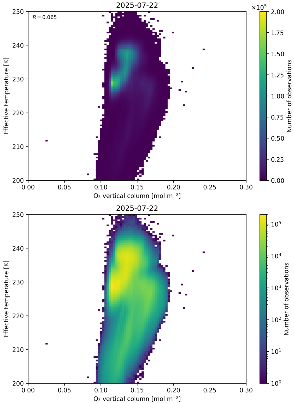
Figure 39: Scatter density plot of “O 3 vertical column” against “Effective temperature” for 2025-07-21 to 2025-07-23.
