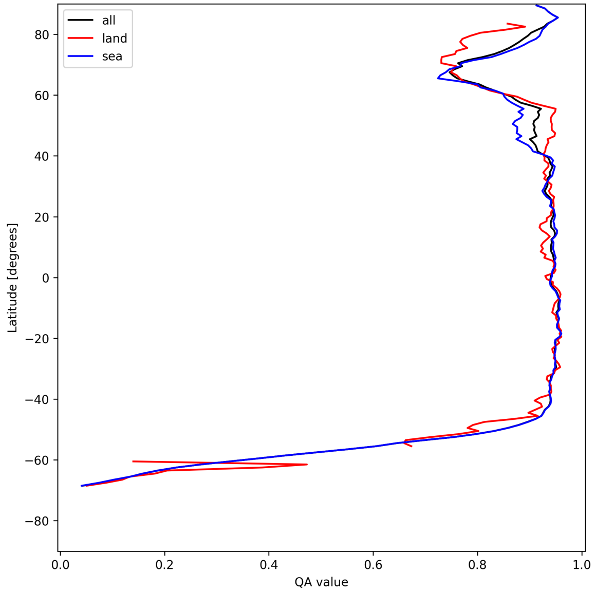
Figure 13: Zonal average of “QA value” for 2025-07-21 to 2025-07-23.
