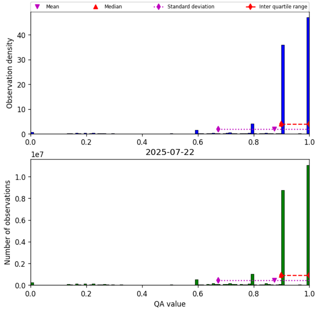
Figure 20: Histogram of “QA value” for 2025-07-21 to 2025-07-23
