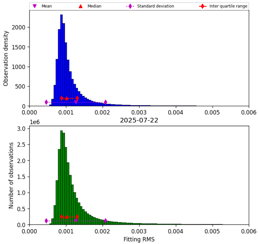
Figure 23: Histogram of “Fitting RMS” for 2025-07-21 to 2025-07-23
