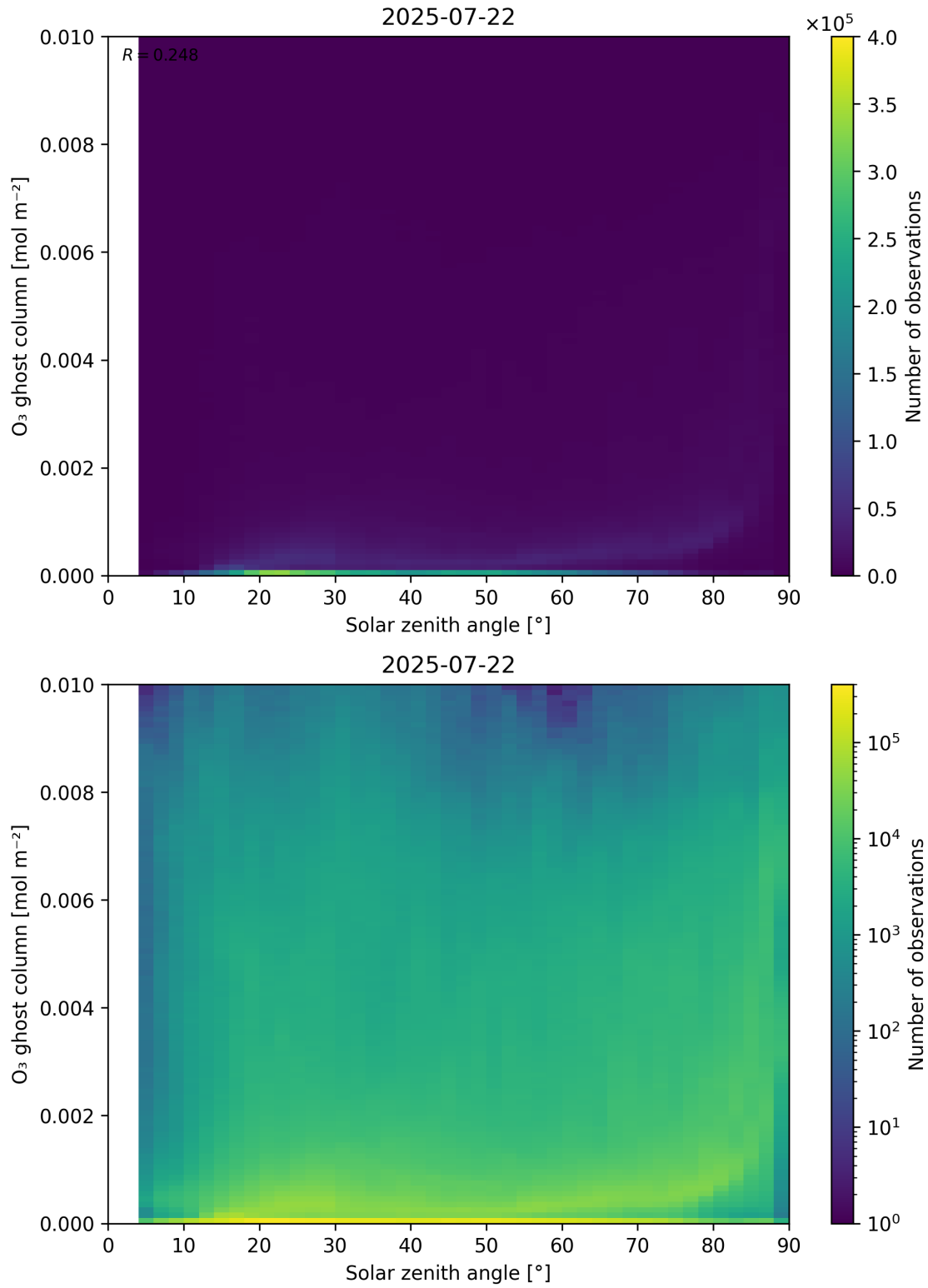
Figure 46: Scatter density plot of “Solar zenith angle” against “O 3 ghost column” for 2025-07-21 to 2025-07-23.
