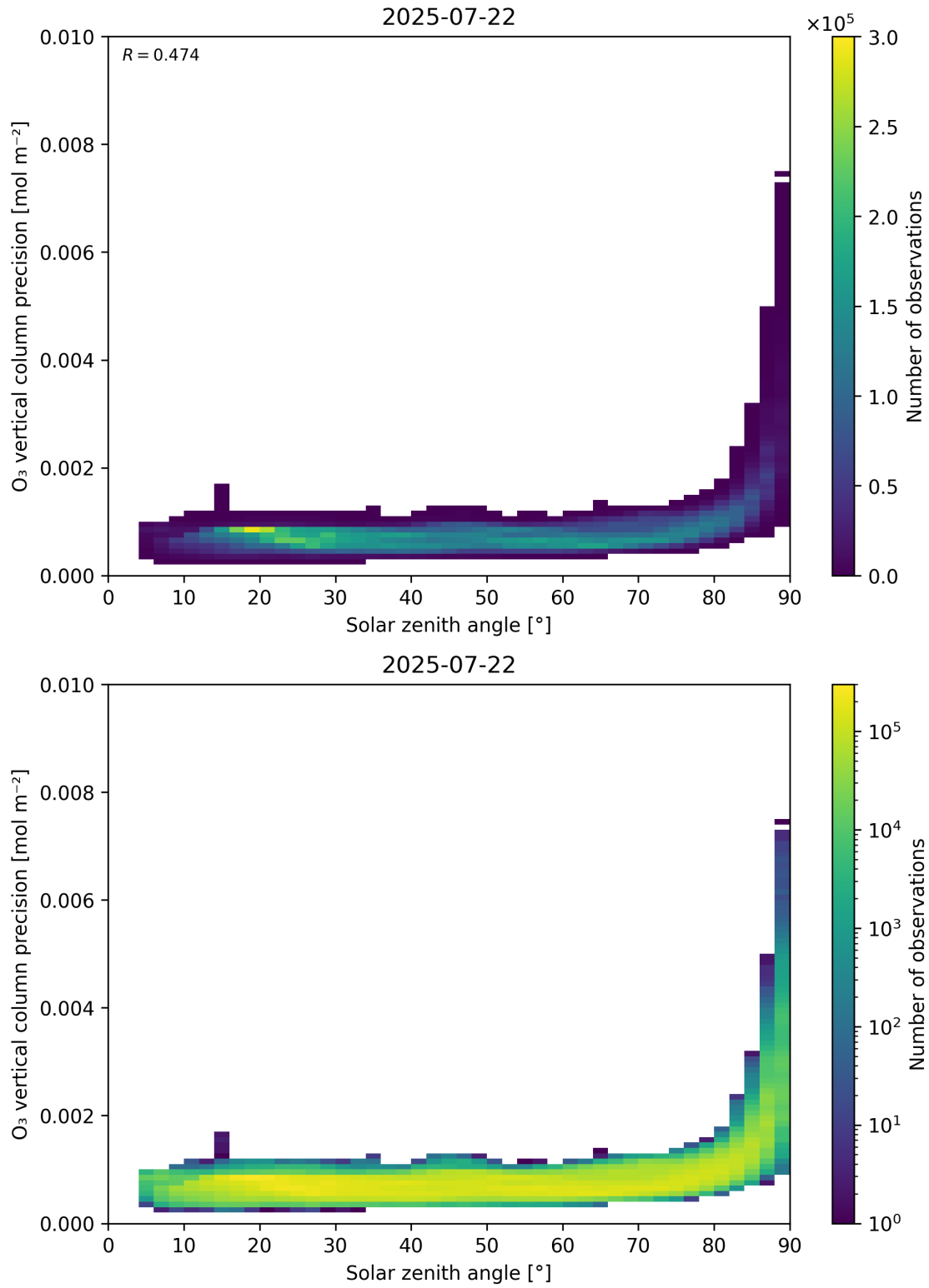
Figure 48: Scatter density plot of “Solar zenith angle” against “O 3 vertical column precision” for 2025-07-21 to 2025-07-23.
