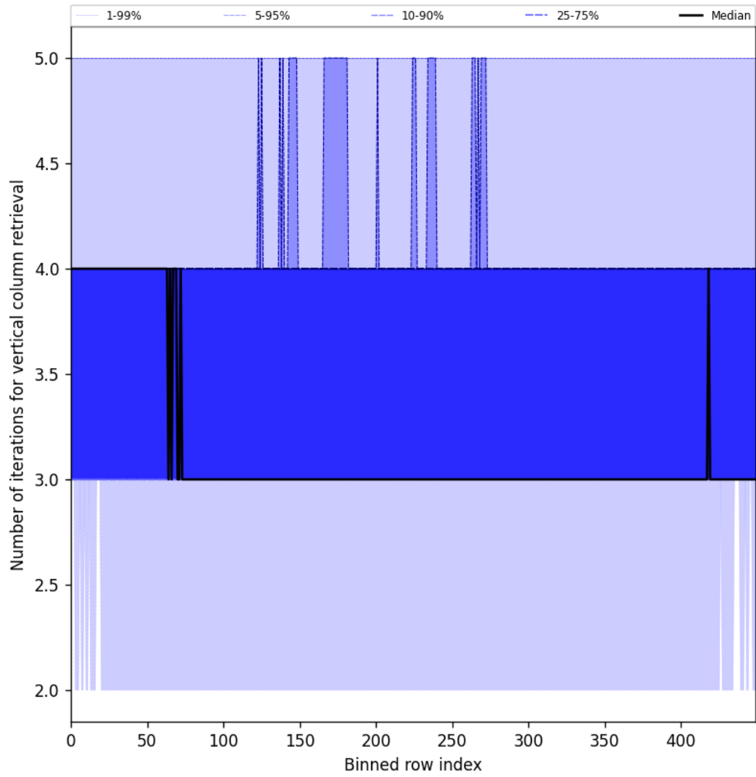
Figure 33: Along track statistics of “Number of iterations for vertical column retrieval” for 2025-07-21 to 2025-07-23
