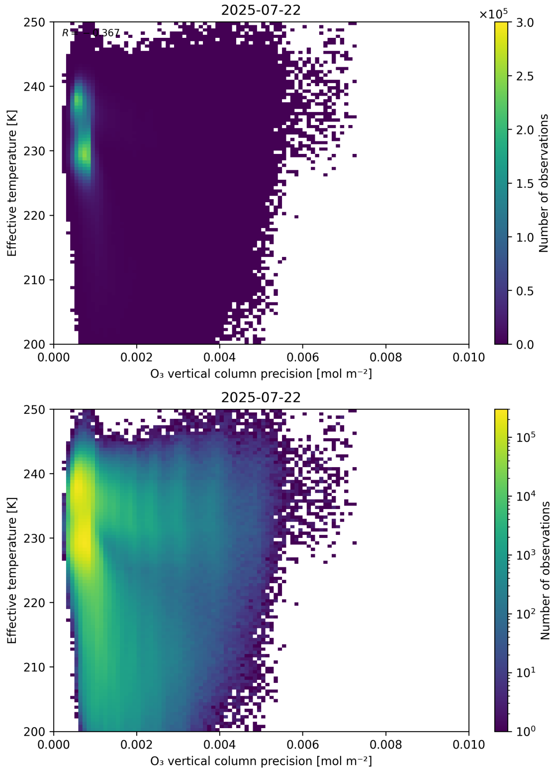
Figure 42: Scatter density plot of “O 3 vertical column precision” against “Effective temperature” for 2025-07-21 to 2025-07-23.
