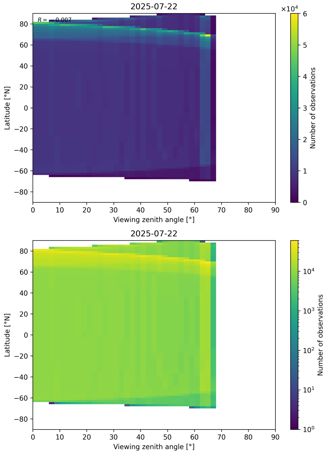
Figure 49: Scatter density plot of “Viewing zenith angle” against “Latitude” for 2025-07-21 to 2025-07-23.
