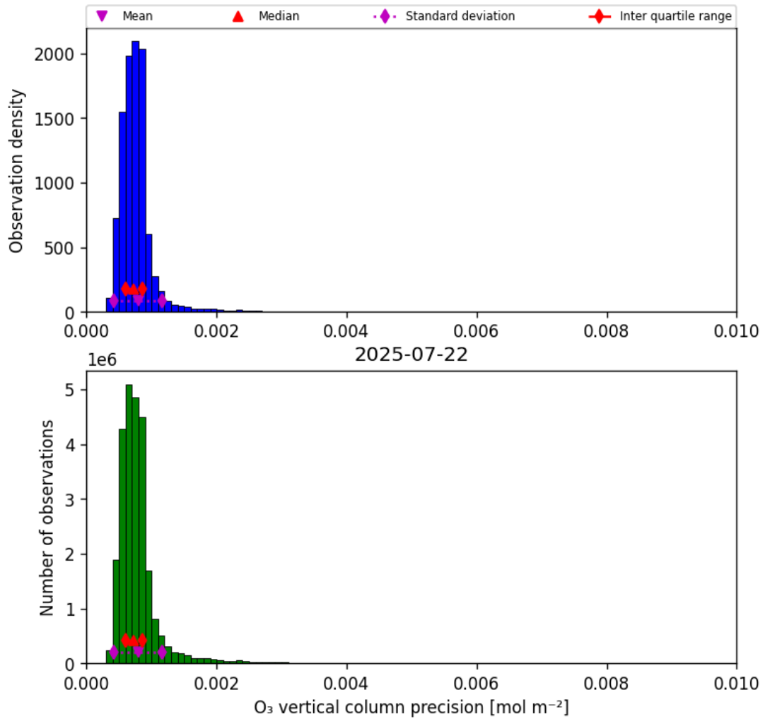
Figure 22: Histogram of “O 3 vertical column precision” for 2025-07-21 to 2025-07-23
