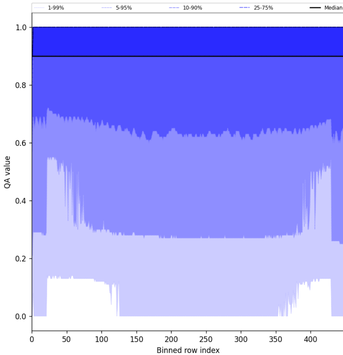
Figure 27: Along track statistics of “QA value” for 2025-07-21 to 2025-07-23
