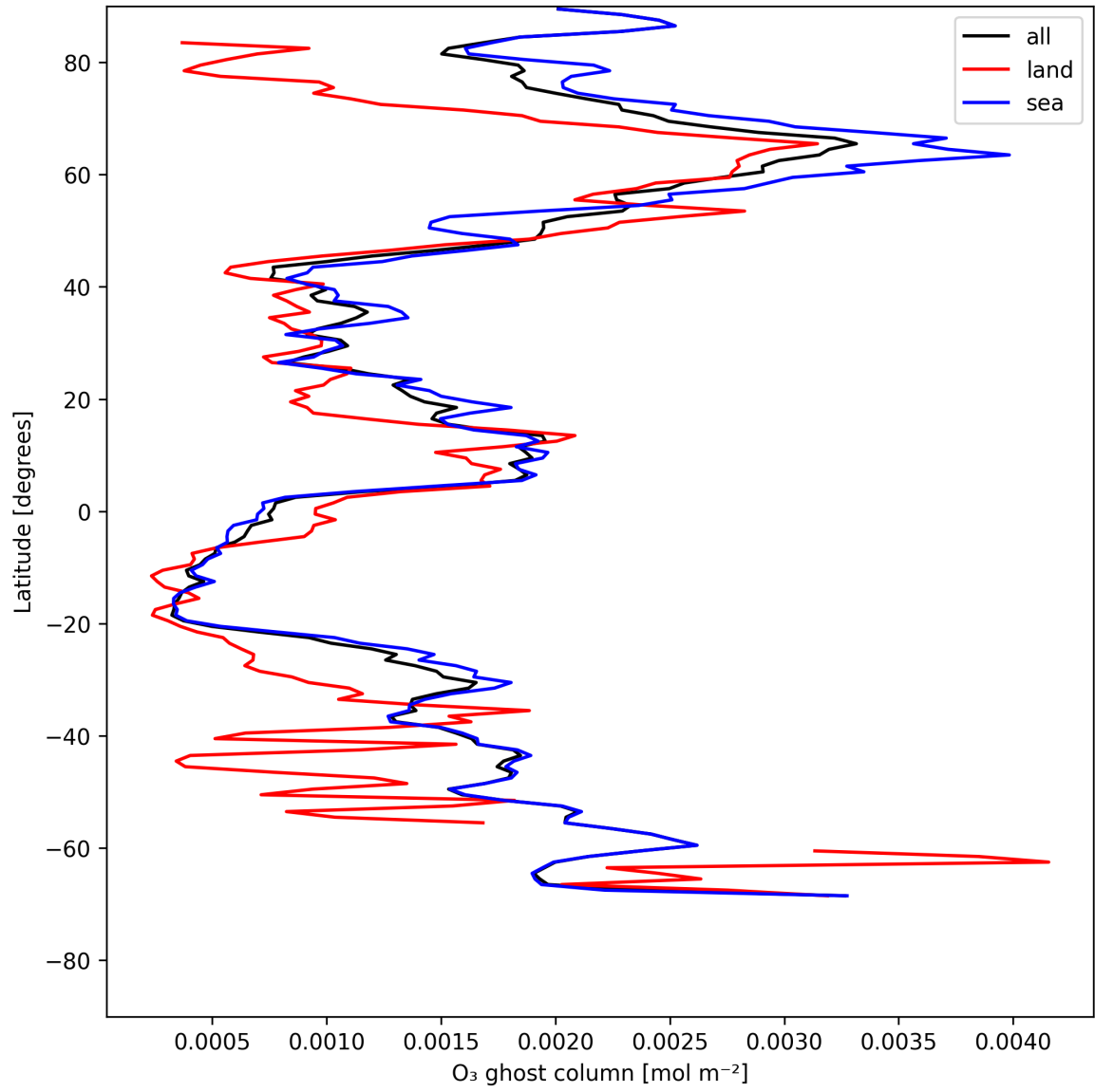
Figure 18: Zonal average of “O 3 ghost column” for 2025-07-21 to 2025-07-23.
