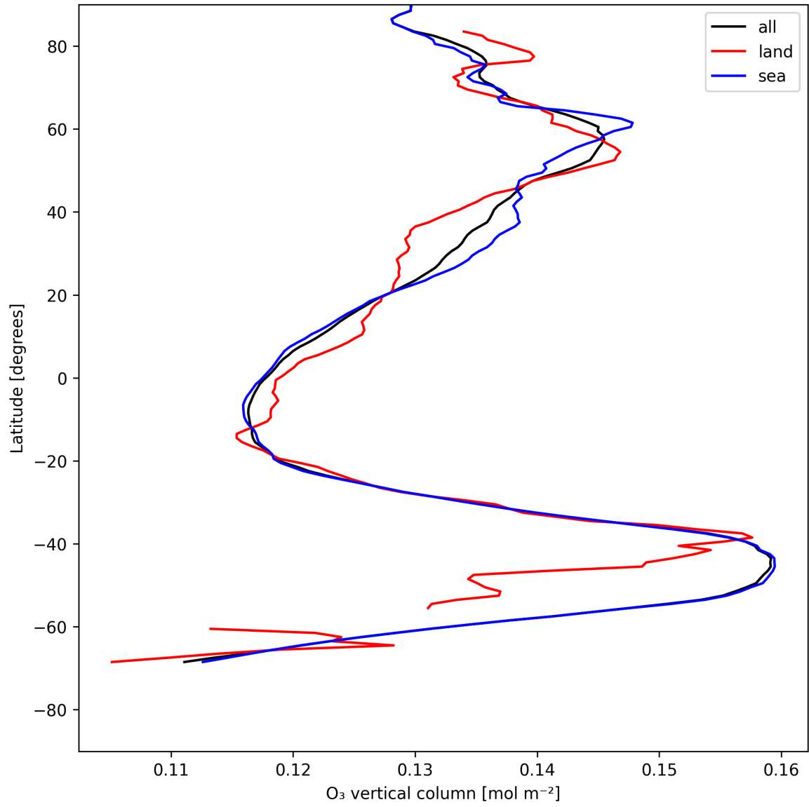
Figure 14: Zonal average of “O 3 vertical column” for 2025-07-21 to 2025-07-23.
