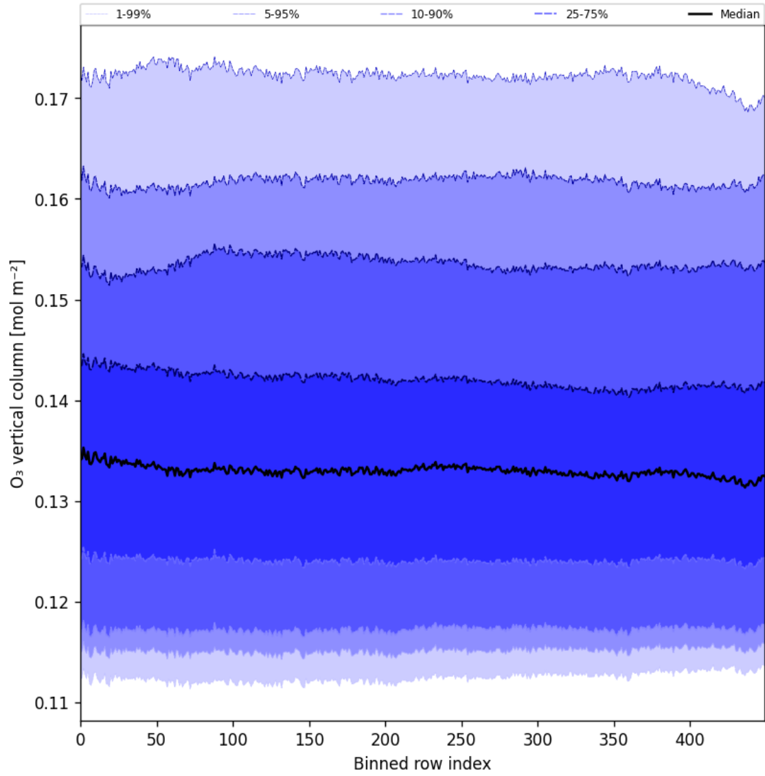
Figure 28: Along track statistics of “O 3 vertical column” for 2025-07-21 to 2025-07-23
