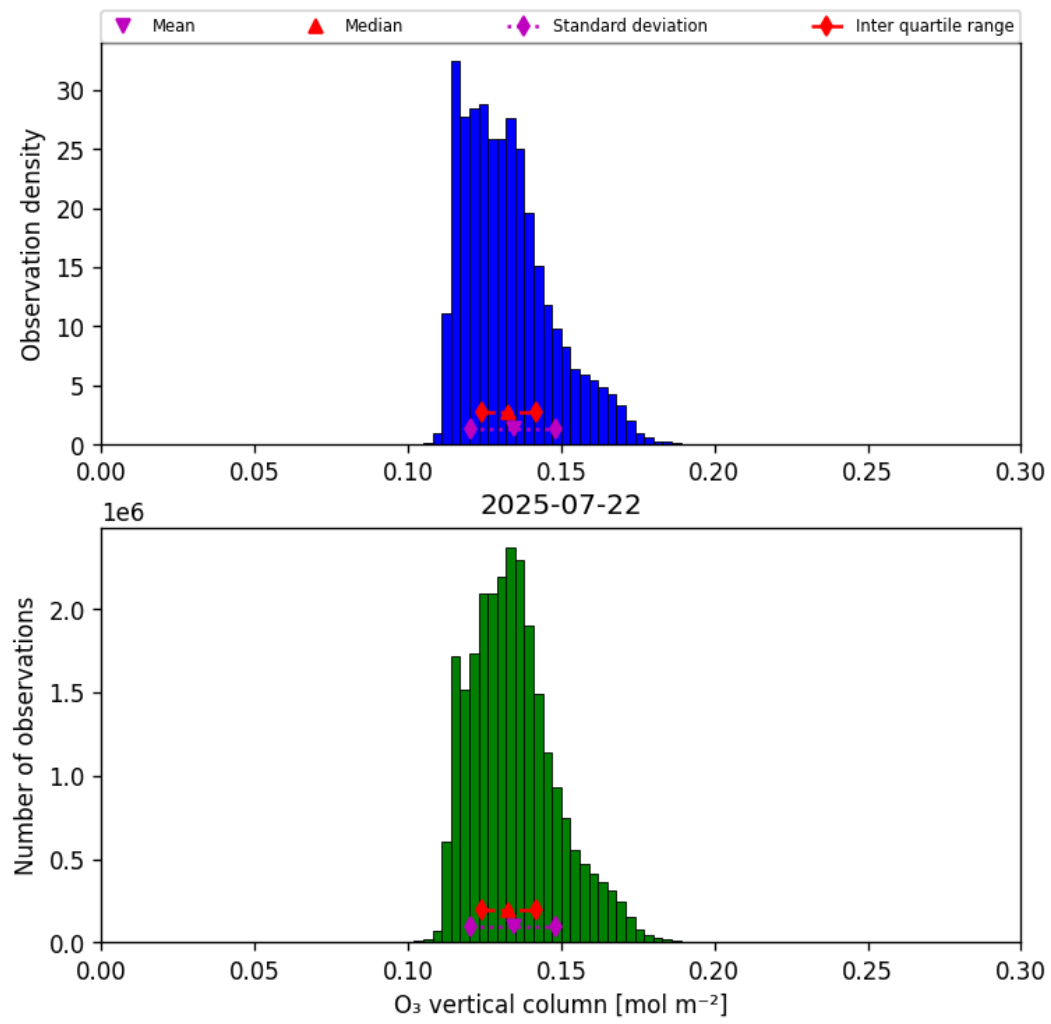
Figure 21: Histogram of “O 3 vertical column” for 2025-07-21 to 2025-07-23
