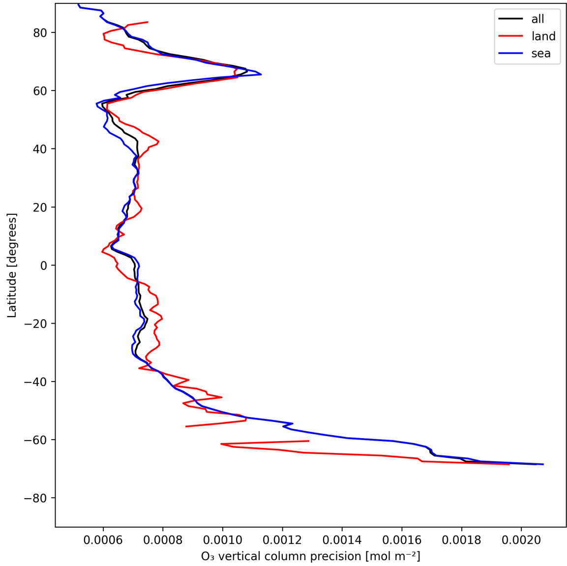
Figure 15: Zonal average of “O 3 vertical column precision” for 2025-07-21 to 2025-07-23.
