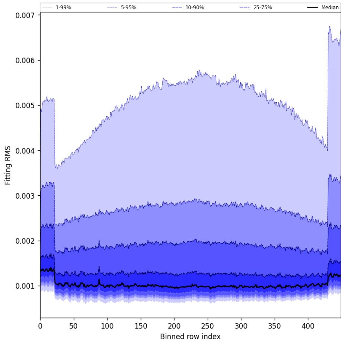
Figure 30: Along track statistics of “Fitting RMS” for 2025-07-21 to 2025-07-23
