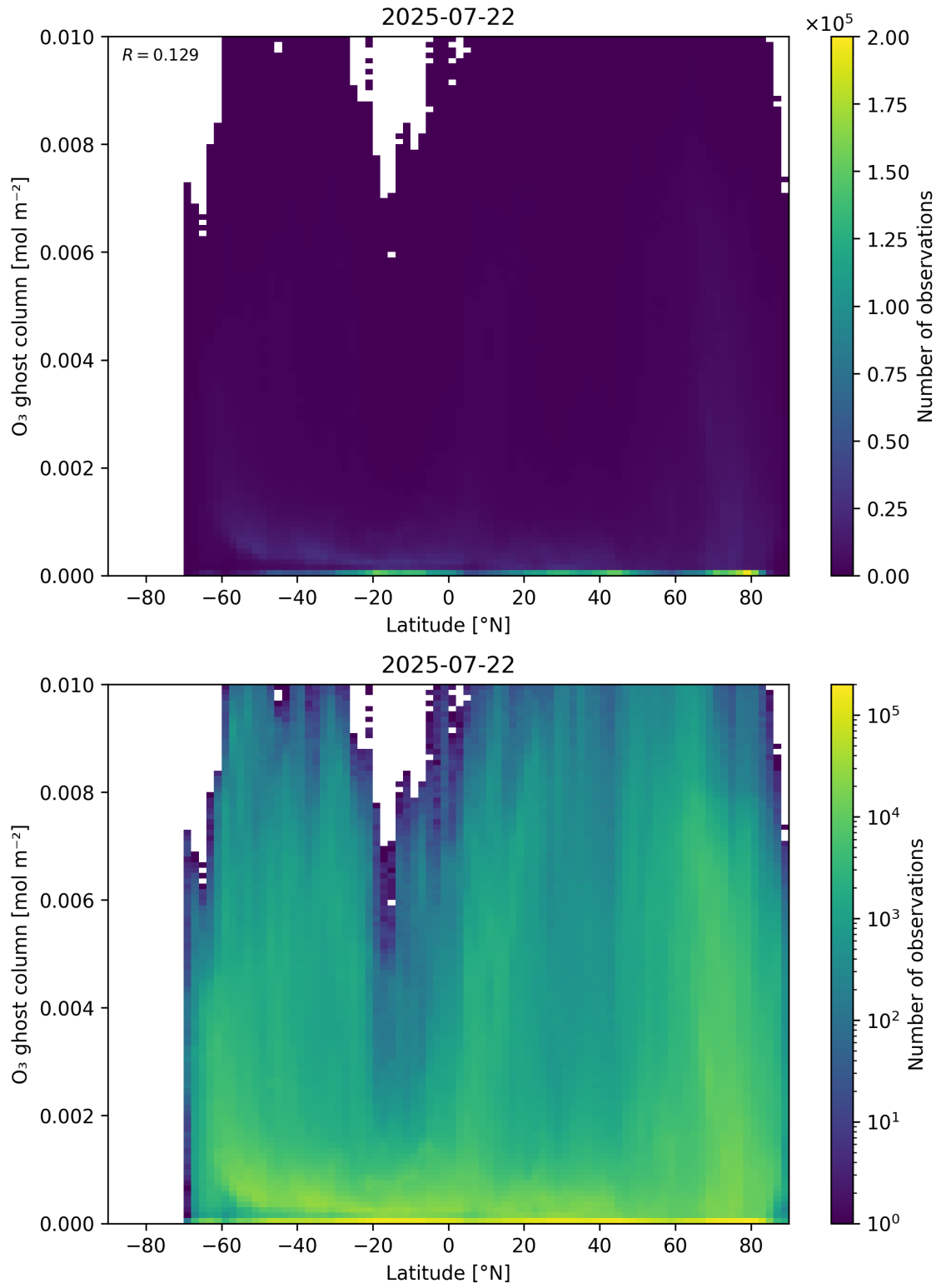
Figure 35: Scatter density plot of “Latitude” against “O 3 ghost column” for 2025-07-21 to 2025-07-23.
