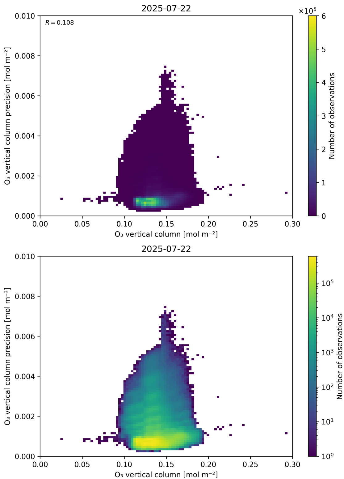
Figure 41: Scatter density plot of “O 3 vertical column” against “O 3 vertical column precision” for 2025-07-21 to 2025-07-23.
