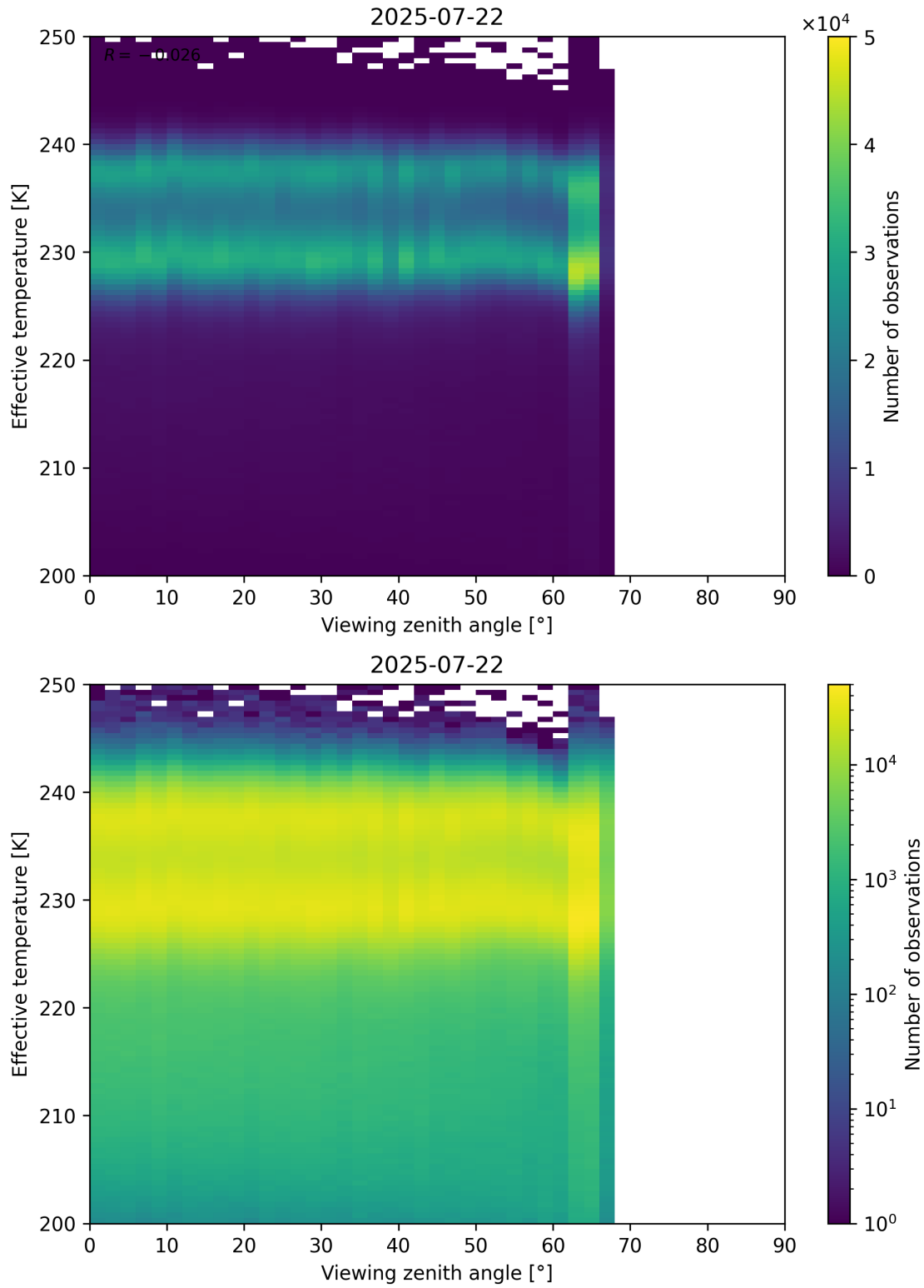
Figure 50: Scatter density plot of “Viewing zenith angle” against “Effective temperature” for 2025-07-21 to 2025-07-23.
