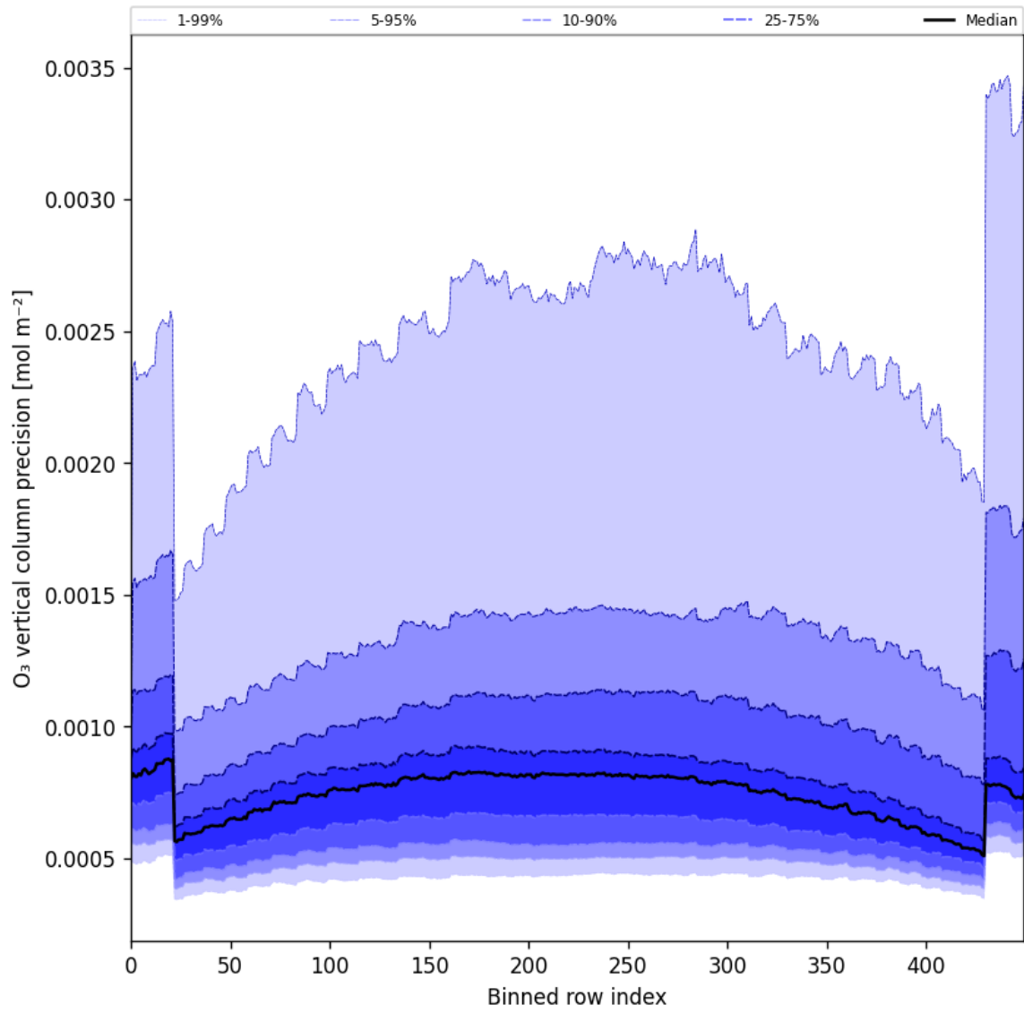
Figure 29: Along track statistics of “O 3 vertical column precision” for 2025-07-21 to 2025-07-23
