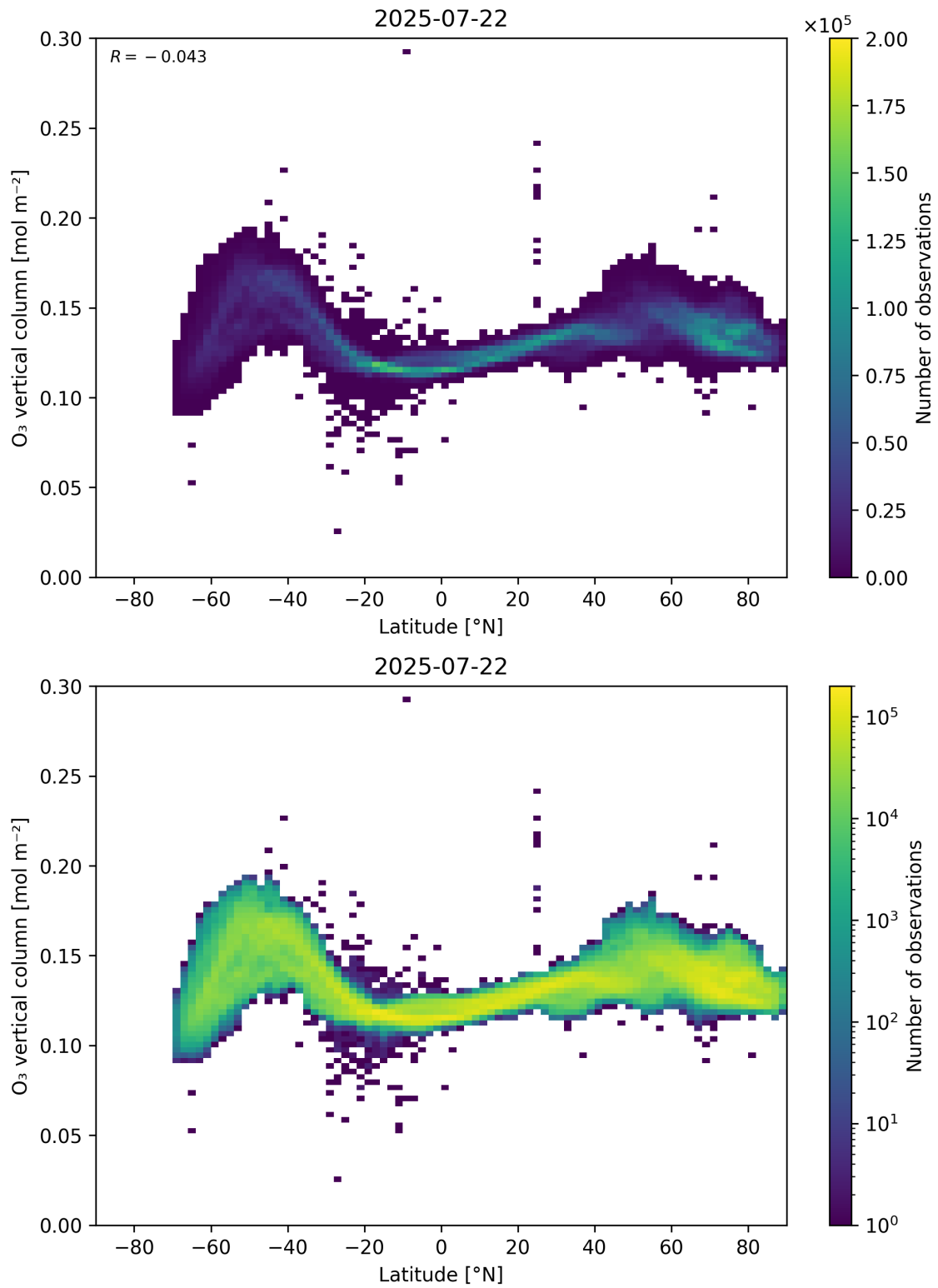
Figure 36: Scatter density plot of “Latitude” against “O 3 vertical column” for 2025-07-21 to 2025-07-23.
