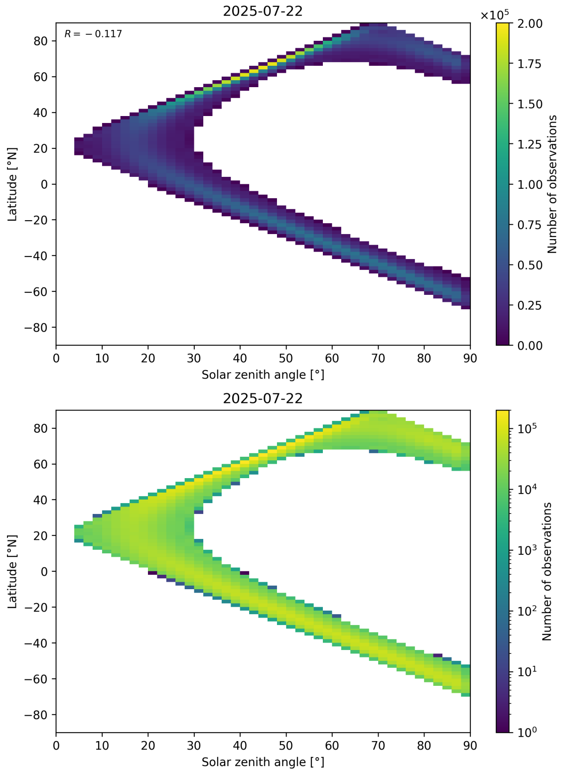
Figure 44: Scatter density plot of “Solar zenith angle” against “Latitude” for 2025-07-21 to 2025-07-23.
