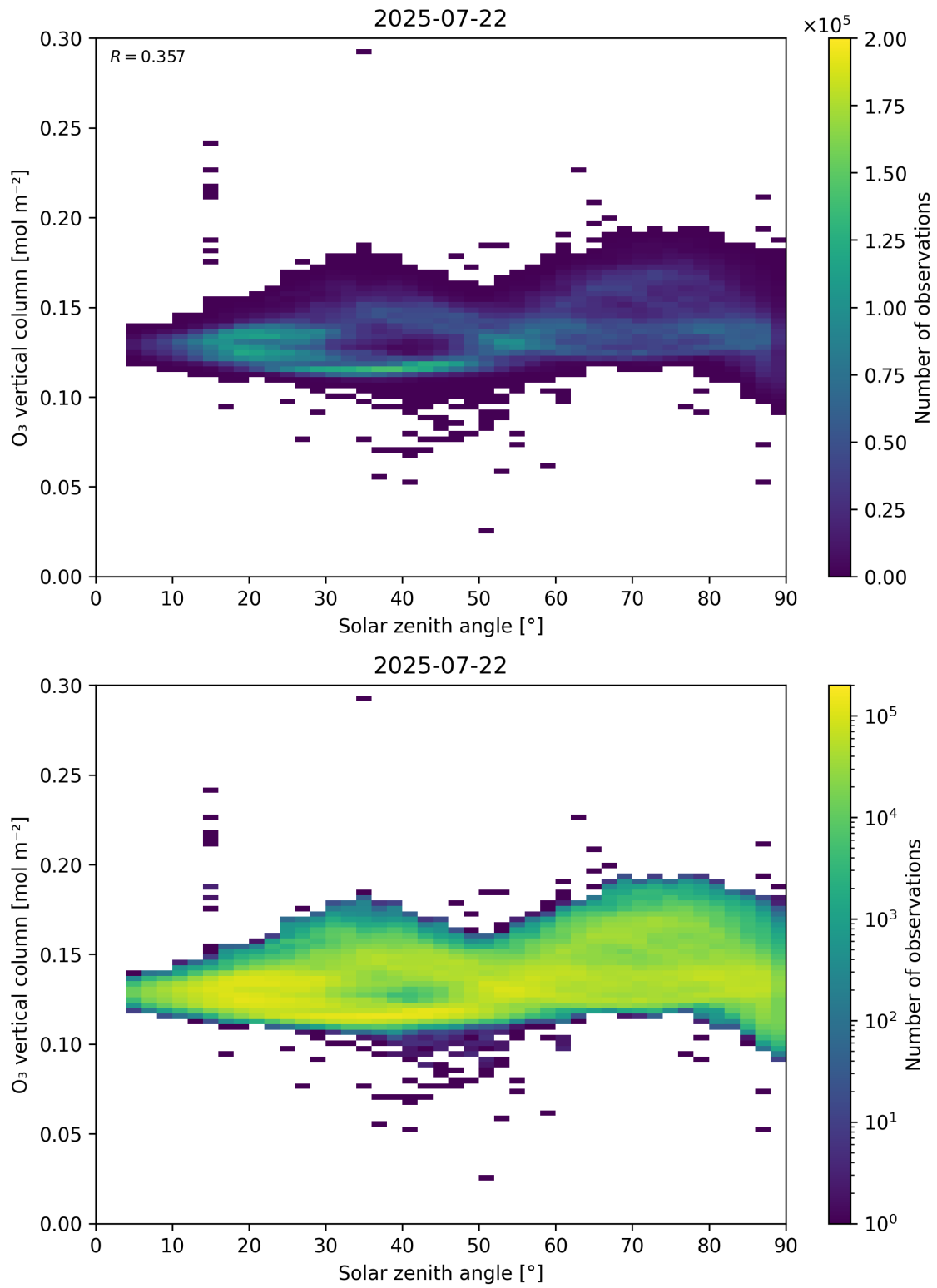
Figure 47: Scatter density plot of “Solar zenith angle” against “O 3 vertical column” for 2025-07-21 to 2025-07-23.
