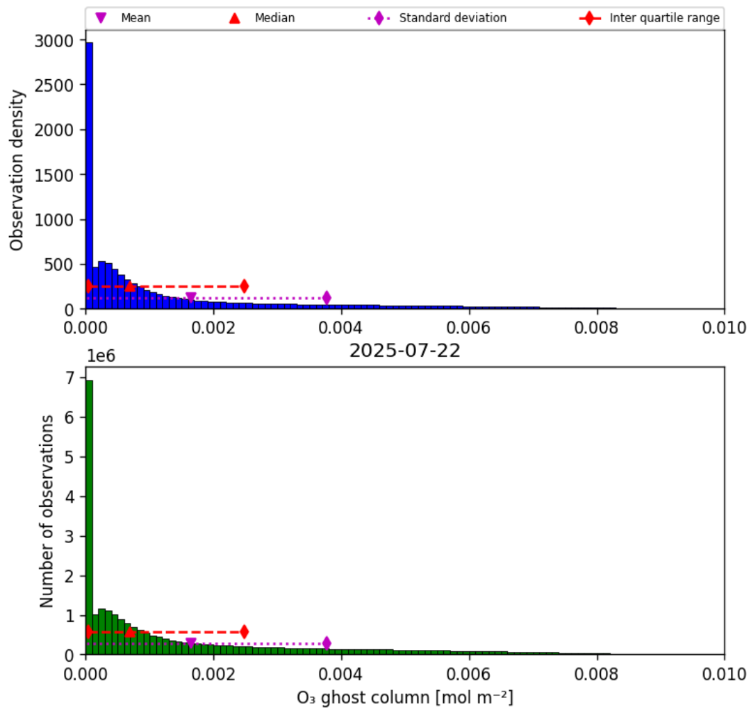
Figure 25: Histogram of “O 3 ghost column” for 2025-07-21 to 2025-07-23
