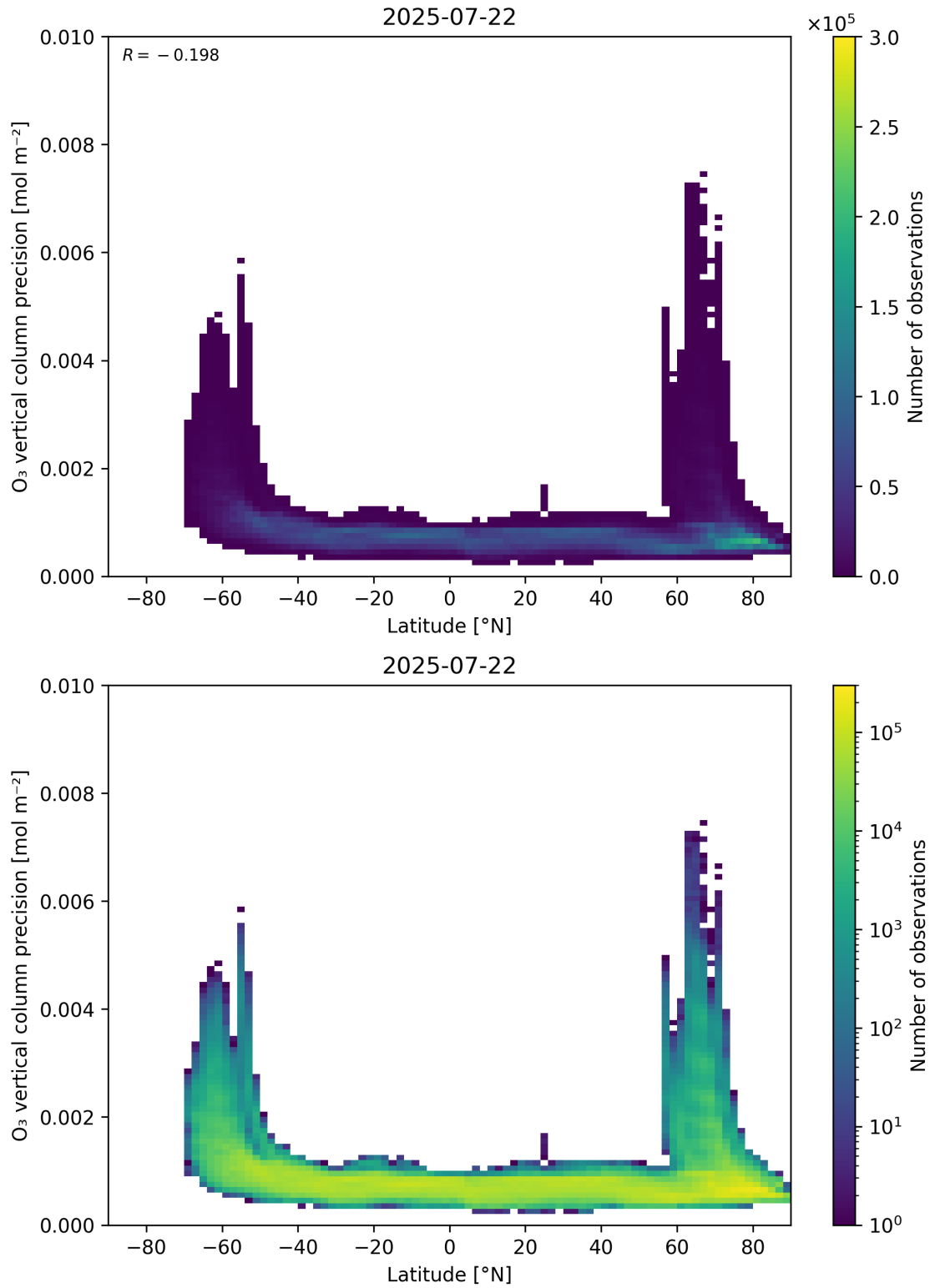
Figure 37: Scatter density plot of “Latitude” against “O 3 vertical column precision” for 2025-07-21 to 2025-07-23.
