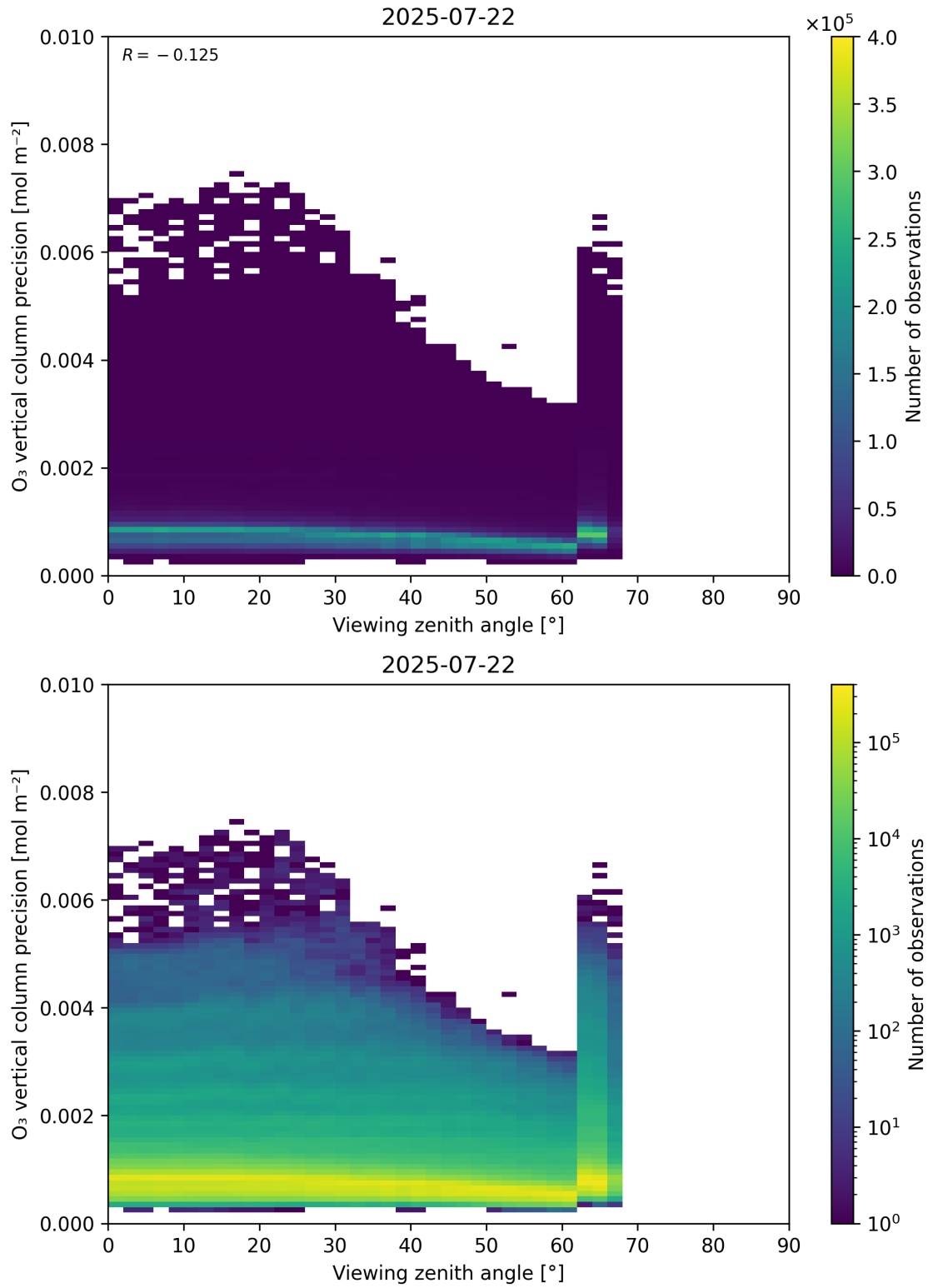
Figure 53: Scatter density plot of “Viewing zenith angle” against “O 3 vertical column precision” for 2025-07-21 to 2025-07-23.
