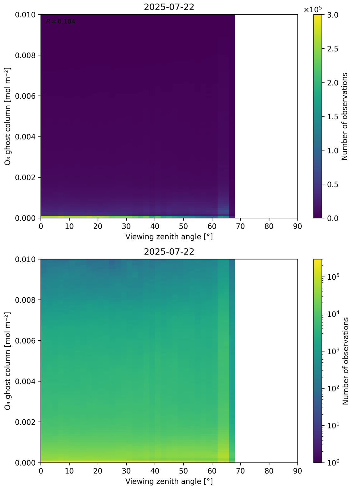
Figure 51: Scatter density plot of “Viewing zenith angle” against “O 3 ghost column” for 2025-07-21 to 2025-07-23.
