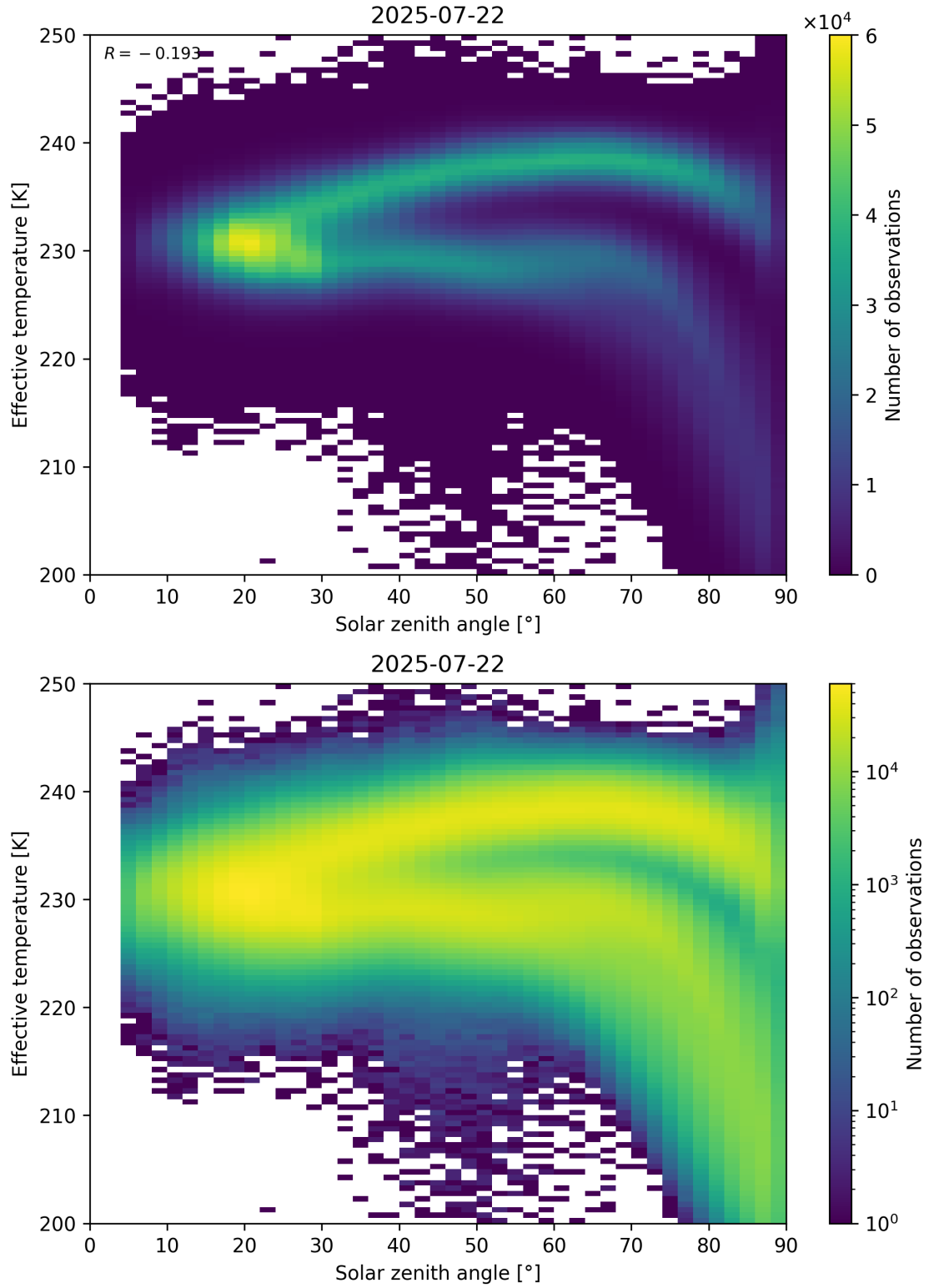
Figure 45: Scatter density plot of “Solar zenith angle” against “Effective temperature” for 2025-07-21 to 2025-07-23.
