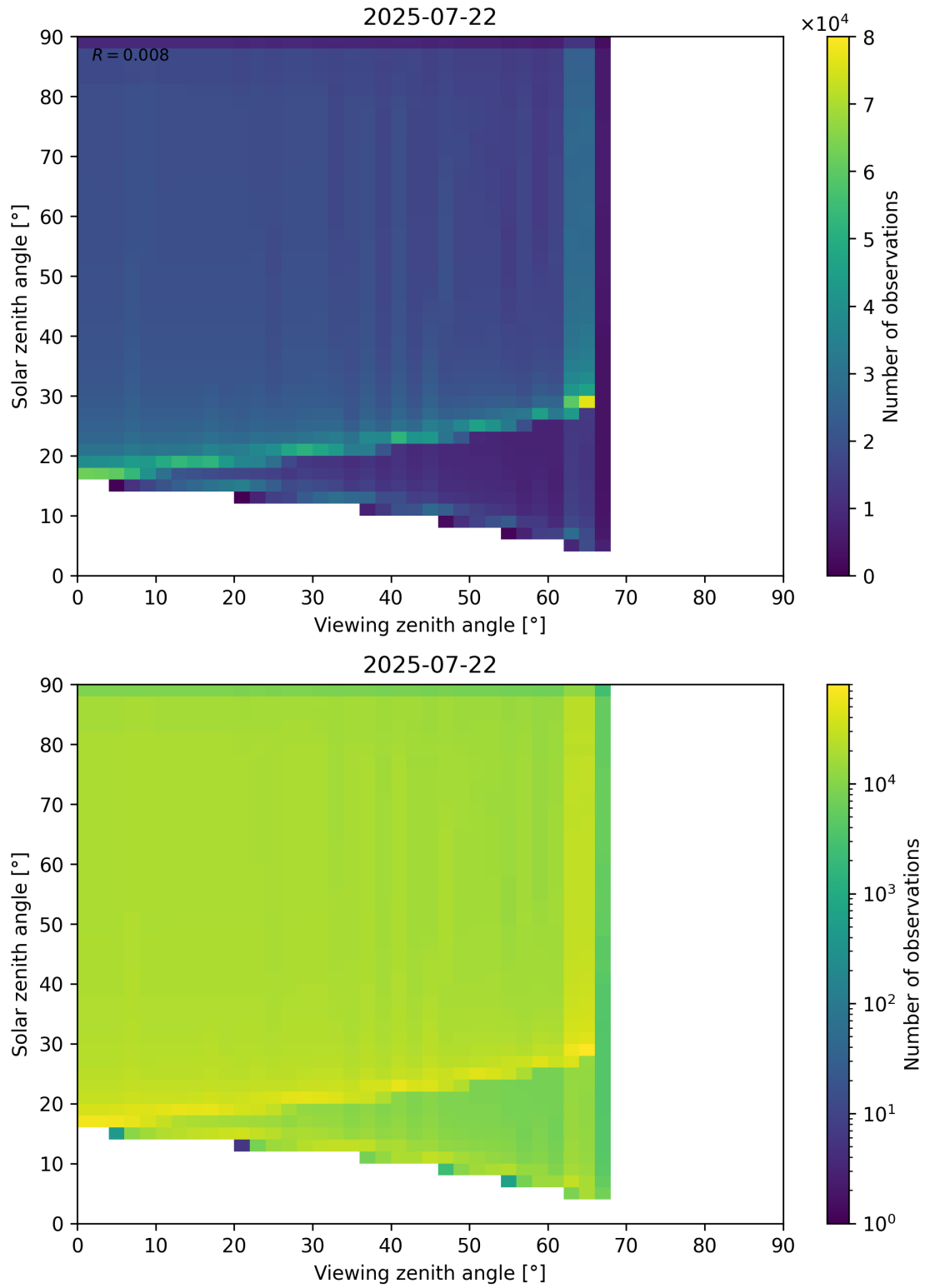
Figure 54: Scatter density plot of “Viewing zenith angle” against “Solar zenith angle” for 2025-07-21 to 2025-07-23.
