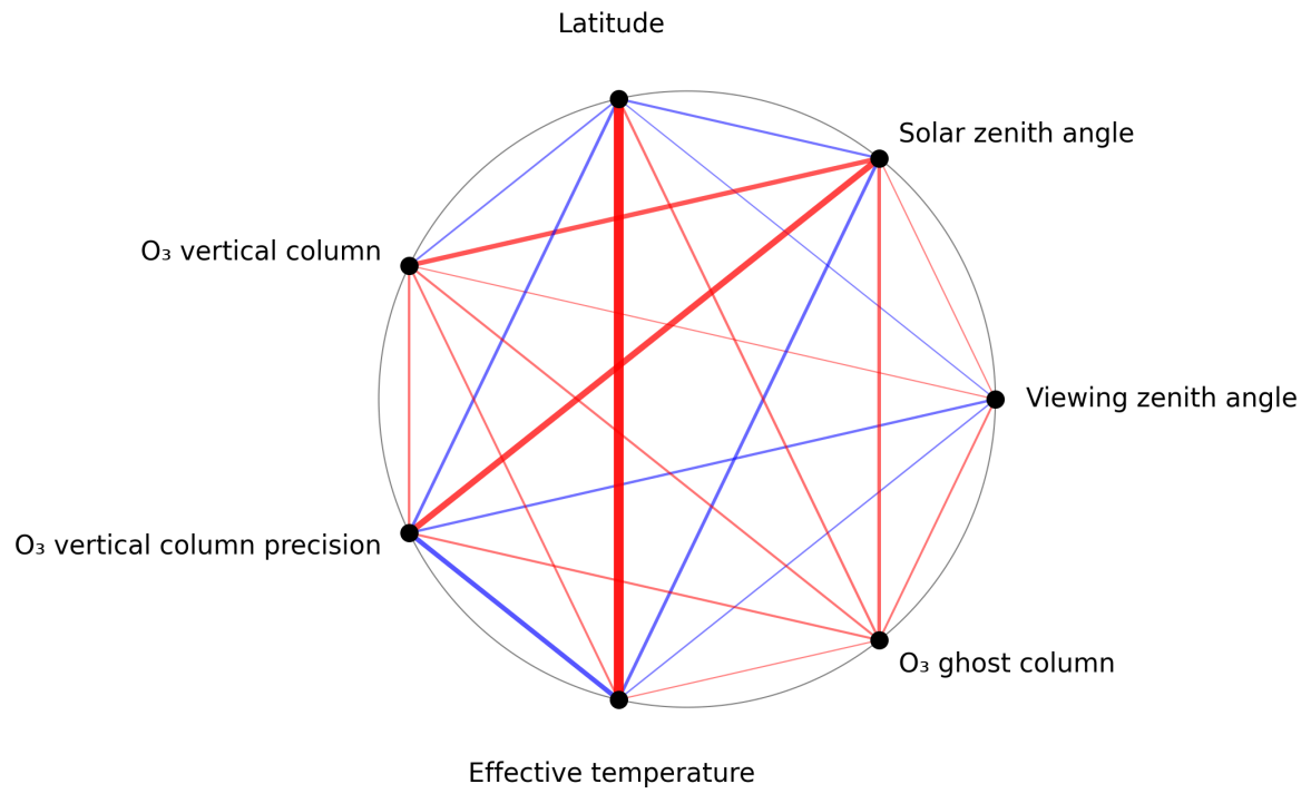
Figure 1: Map of correlation graph for 2025-07-24 to 2025-07-25.
