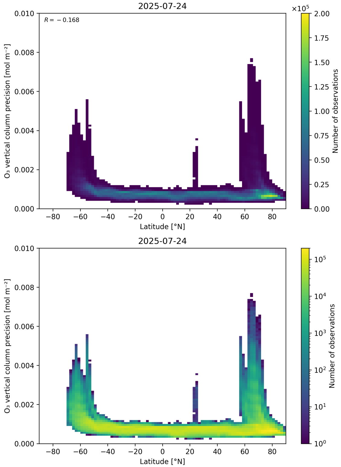
Figure 37: Scatter density plot of “Latitude” against “O 3 vertical column precision” for 2025-07-24 to 2025-07-25.
