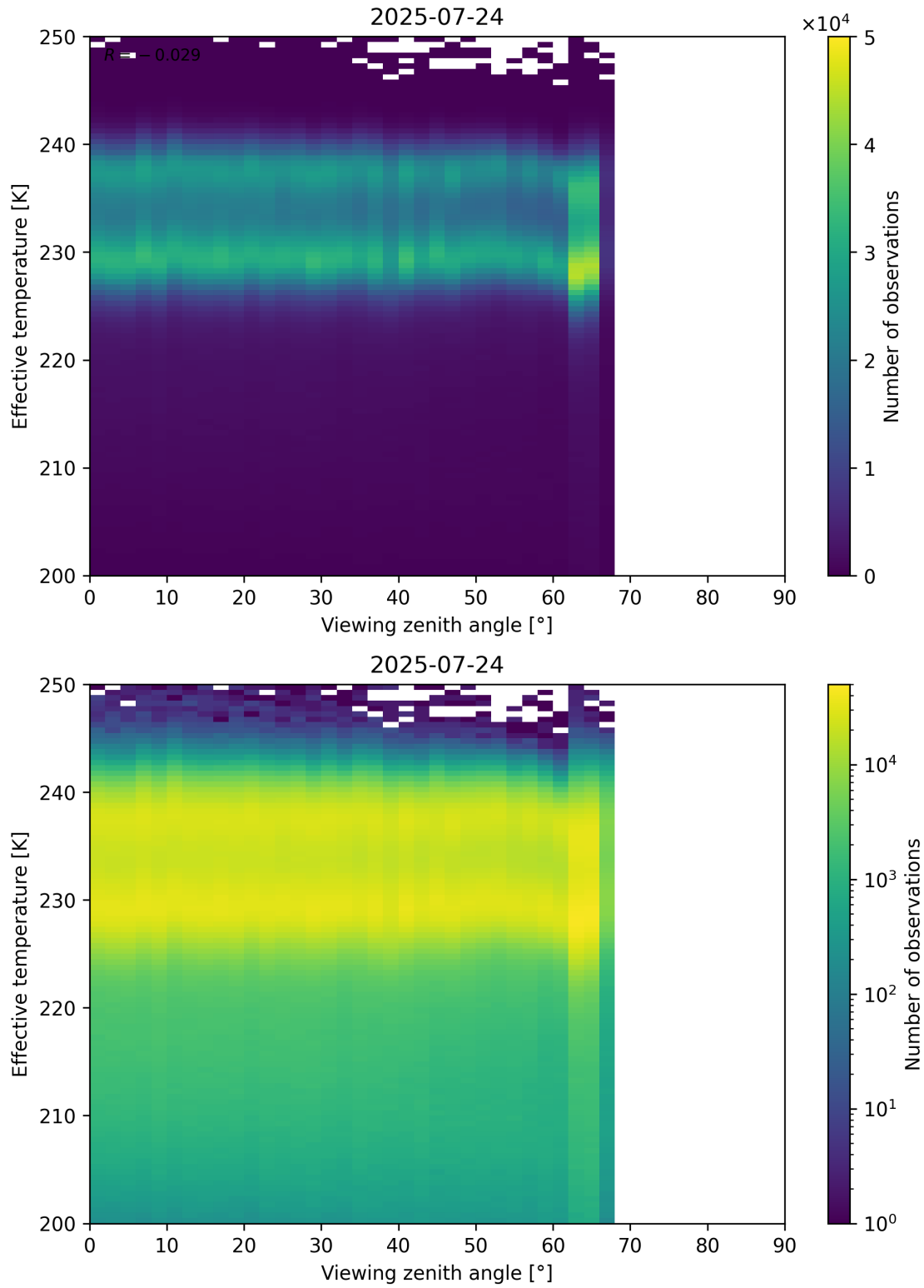
Figure 50: Scatter density plot of “Viewing zenith angle” against “Effective temperature” for 2025-07-24 to 2025-07-25.
