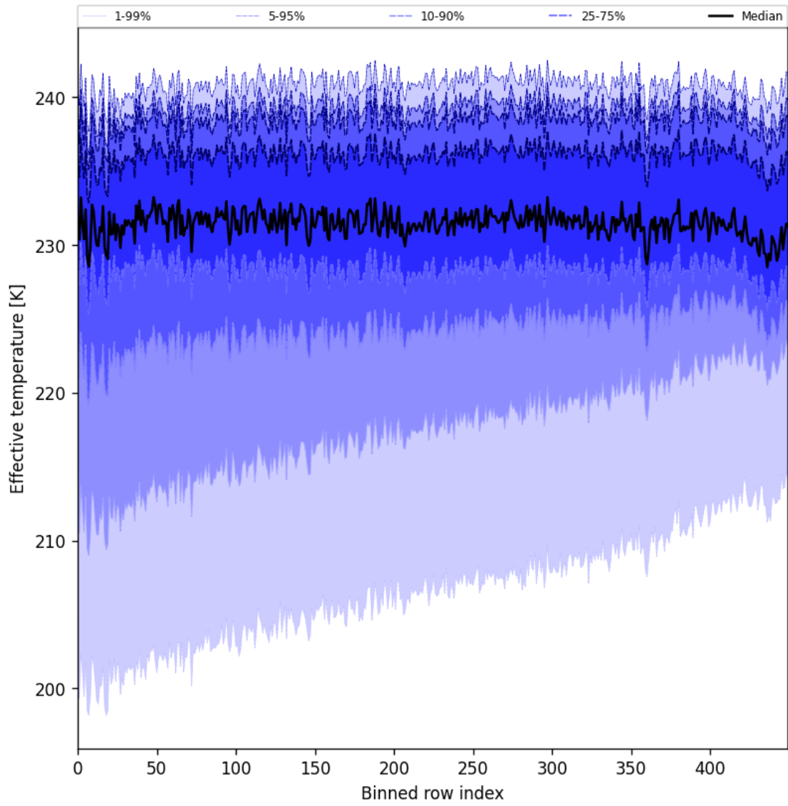
Figure 31: Along track statistics of “Effective temperature” for 2025-07-24 to 2025-07-25
