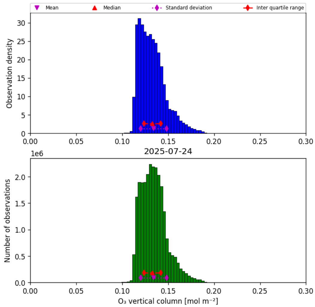
Figure 21: Histogram of “O 3 vertical column” for 2025-07-24 to 2025-07-25
