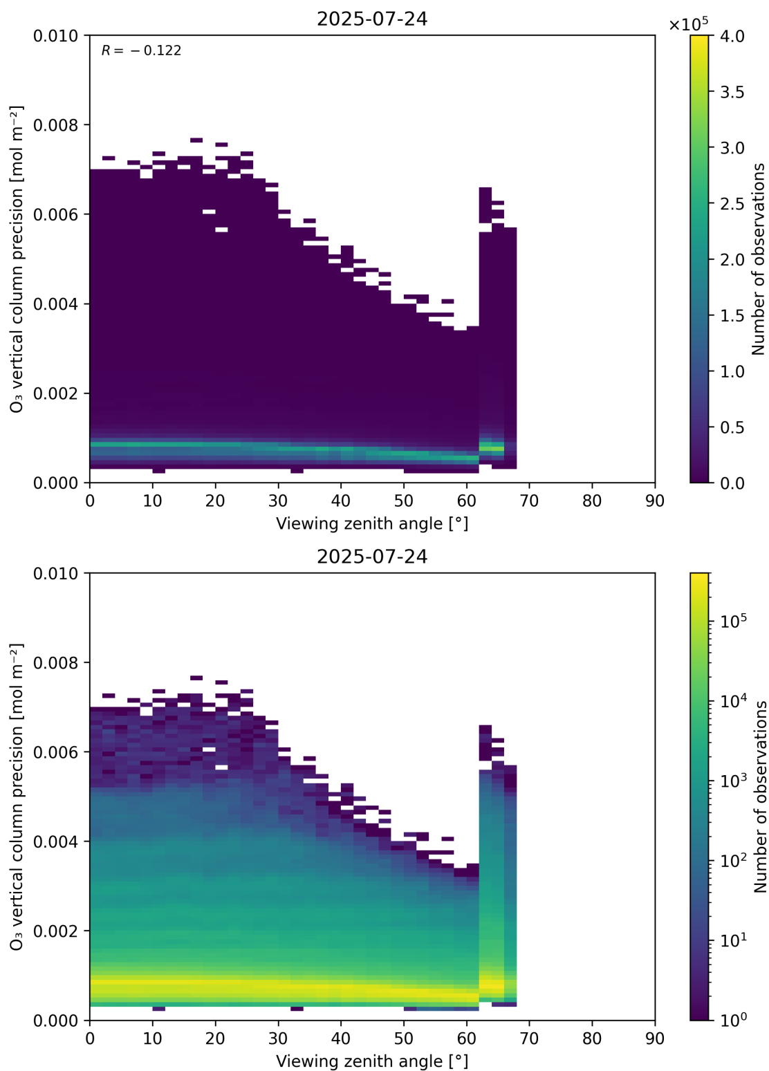
Figure 53: Scatter density plot of “Viewing zenith angle” against “O 3 vertical column precision” for 2025-07-24 to 2025-07-25.
