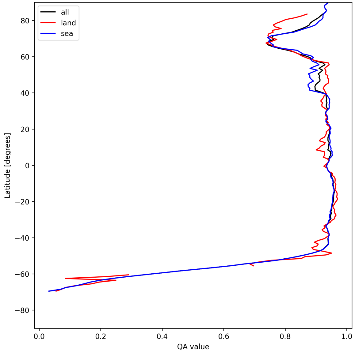
Figure 13: Zonal average of “QA value” for 2025-07-24 to 2025-07-25.
