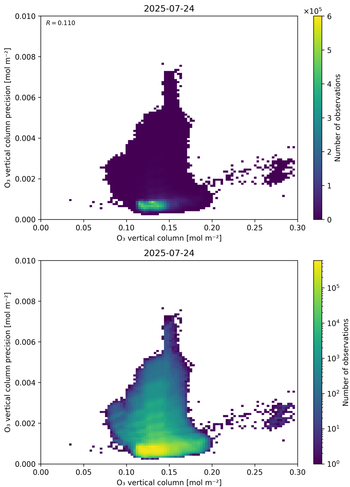
Figure 41: Scatter density plot of “O 3 vertical column” against “O 3 vertical column precision” for 2025-07-24 to 2025-07-25.
