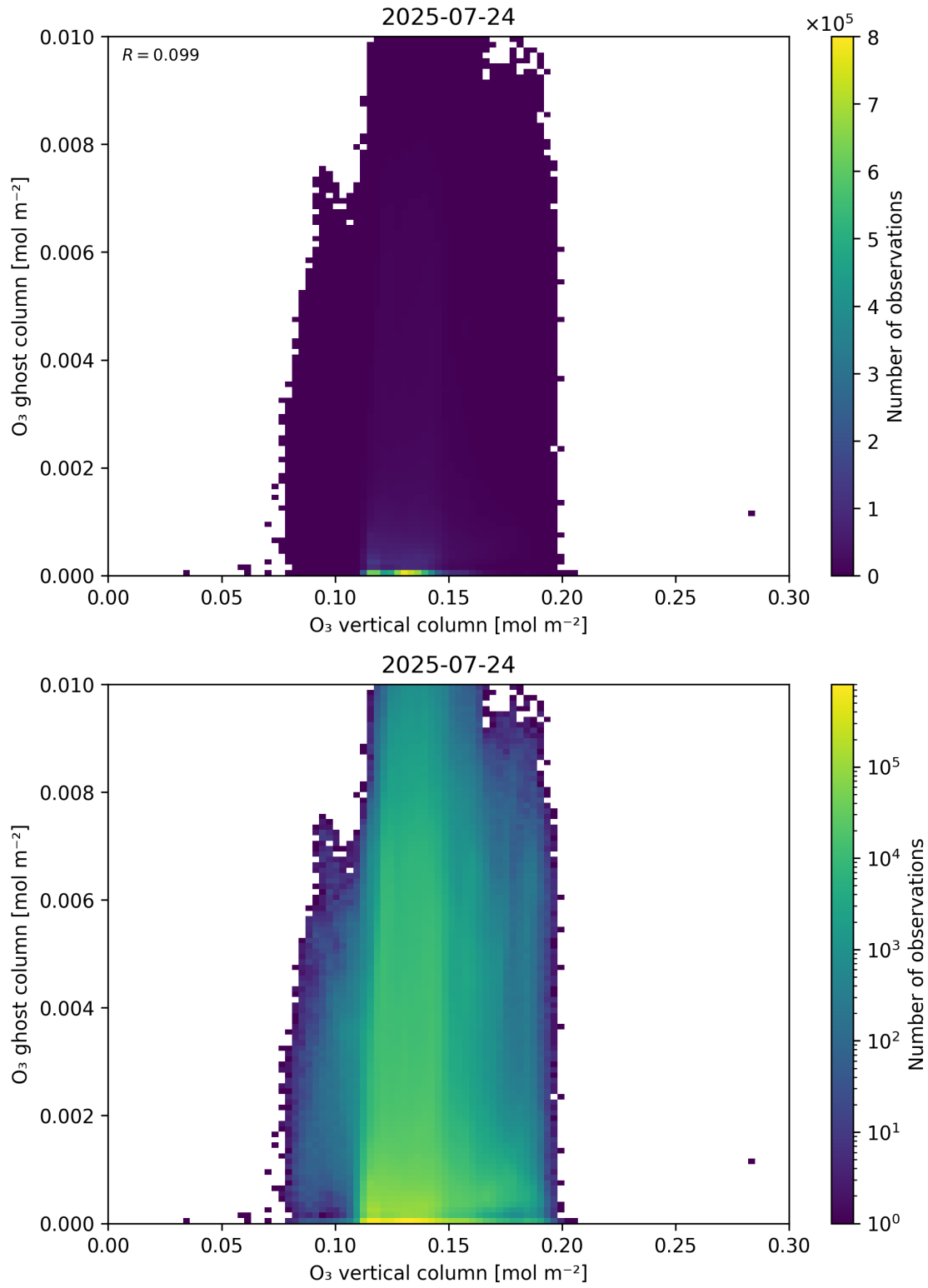
Figure 40: Scatter density plot of “O 3 vertical column” against “O 3 ghost column” for 2025-07-24 to 2025-07-25.
