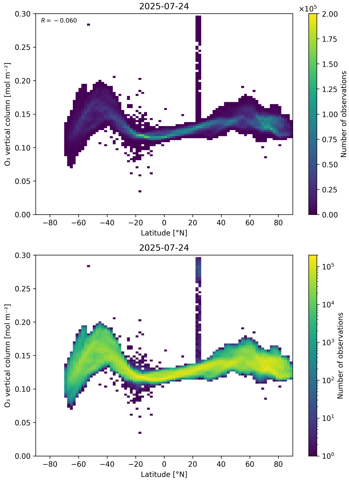
Figure 36: Scatter density plot of “Latitude” against “O 3 vertical column” for 2025-07-24 to 2025-07-25.
