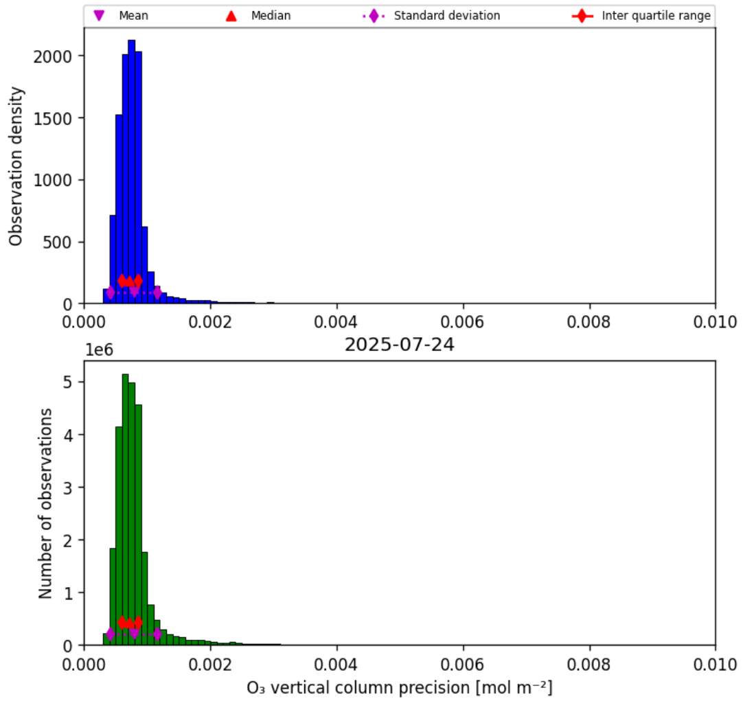
Figure 22: Histogram of “O 3 vertical column precision” for 2025-07-24 to 2025-07-25
