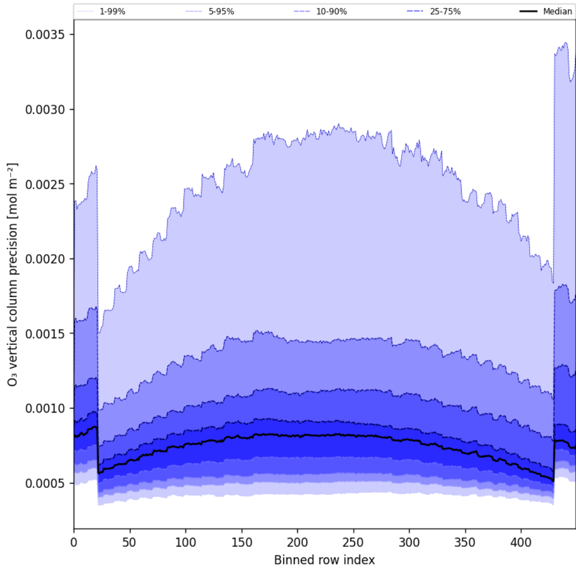
Figure 29: Along track statistics of “O 3 vertical column precision” for 2025-07-24 to 2025-07-25
