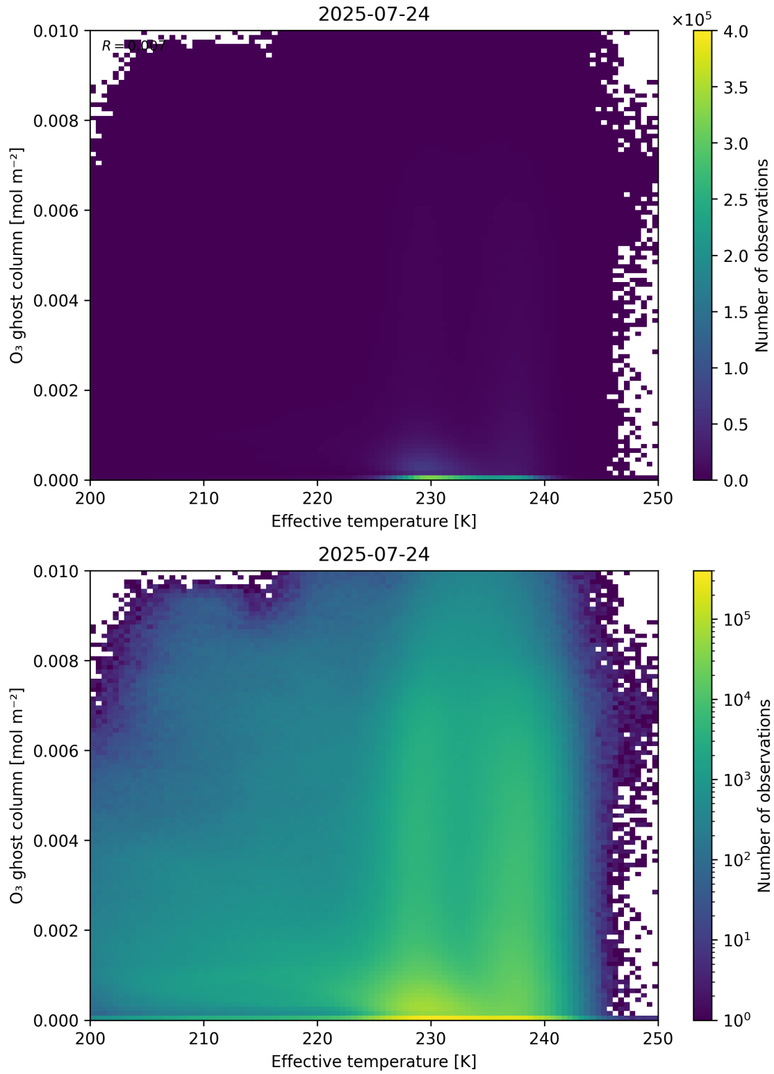
Figure 38: Scatter density plot of “Effective temperature” against “O 3 ghost column” for 2025-07-24 to 2025-07-25.
