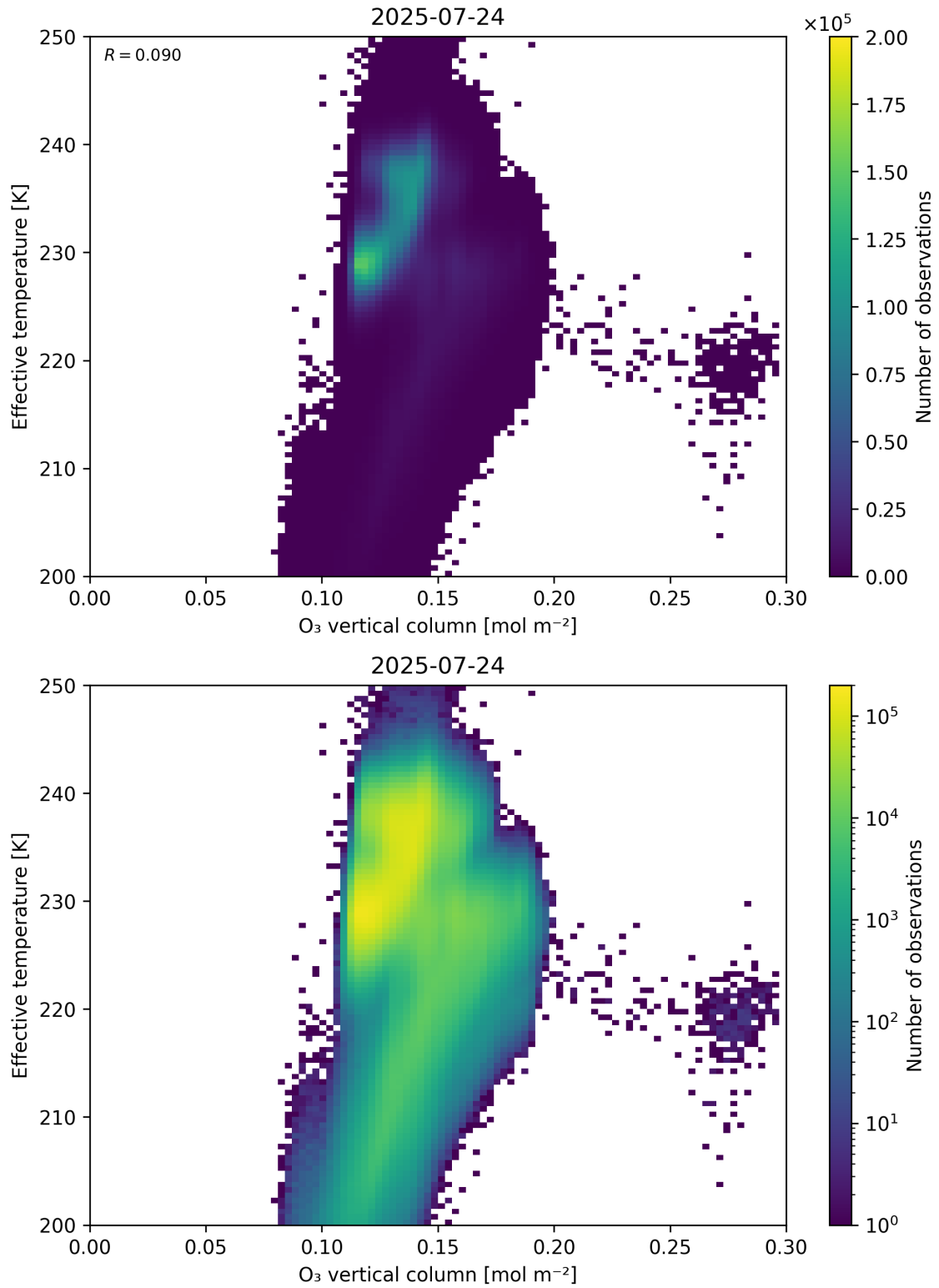
Figure 39: Scatter density plot of “O 3 vertical column” against “Effective temperature” for 2025-07-24 to 2025-07-25.
