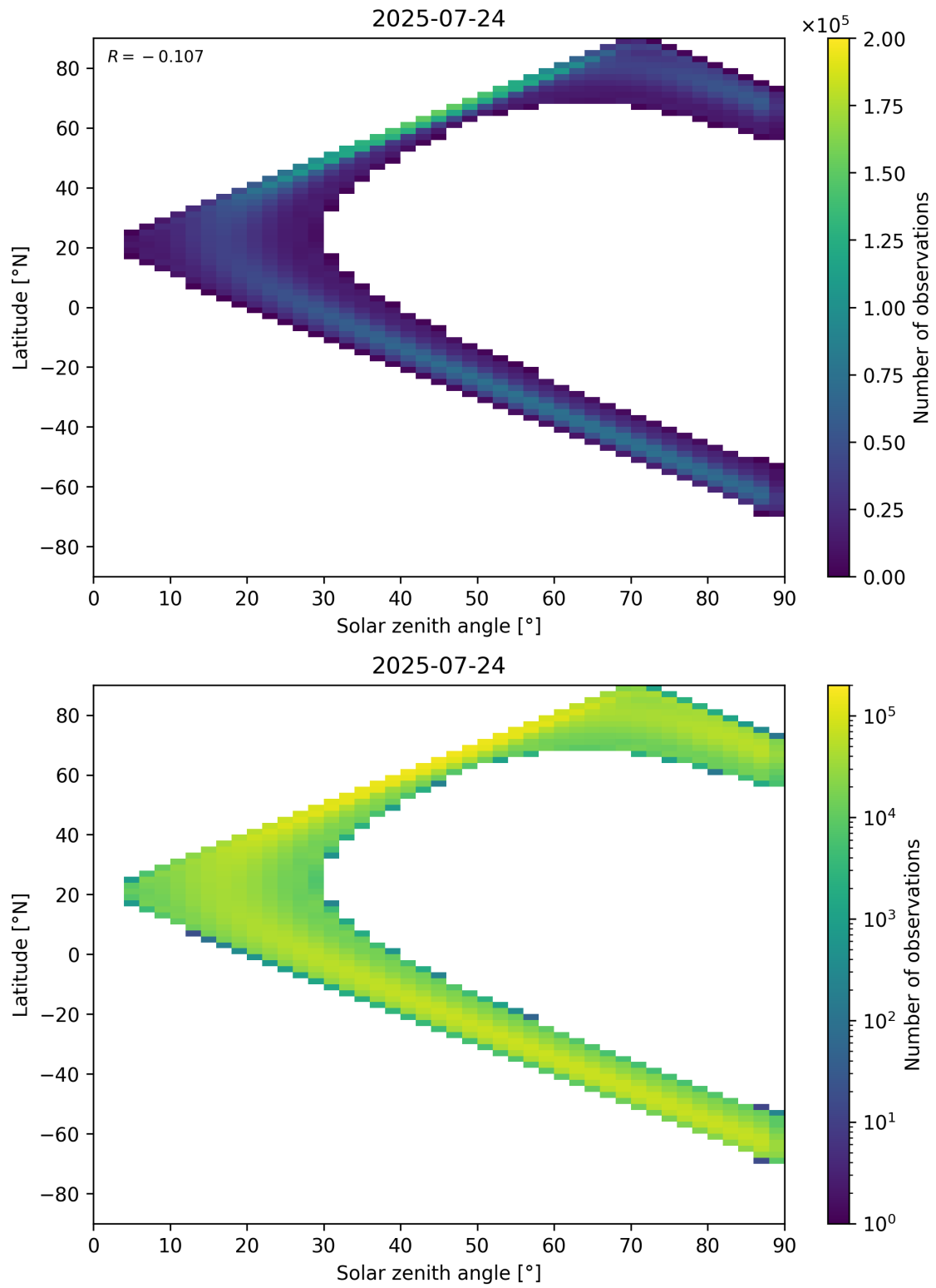
Figure 44: Scatter density plot of “Solar zenith angle” against “Latitude” for 2025-07-24 to 2025-07-25.
