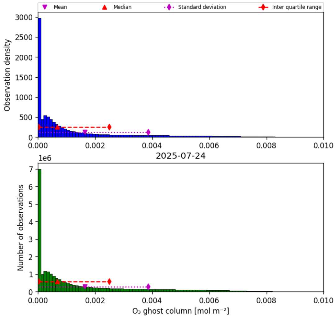
Figure 25: Histogram of “O 3 ghost column” for 2025-07-24 to 2025-07-25
