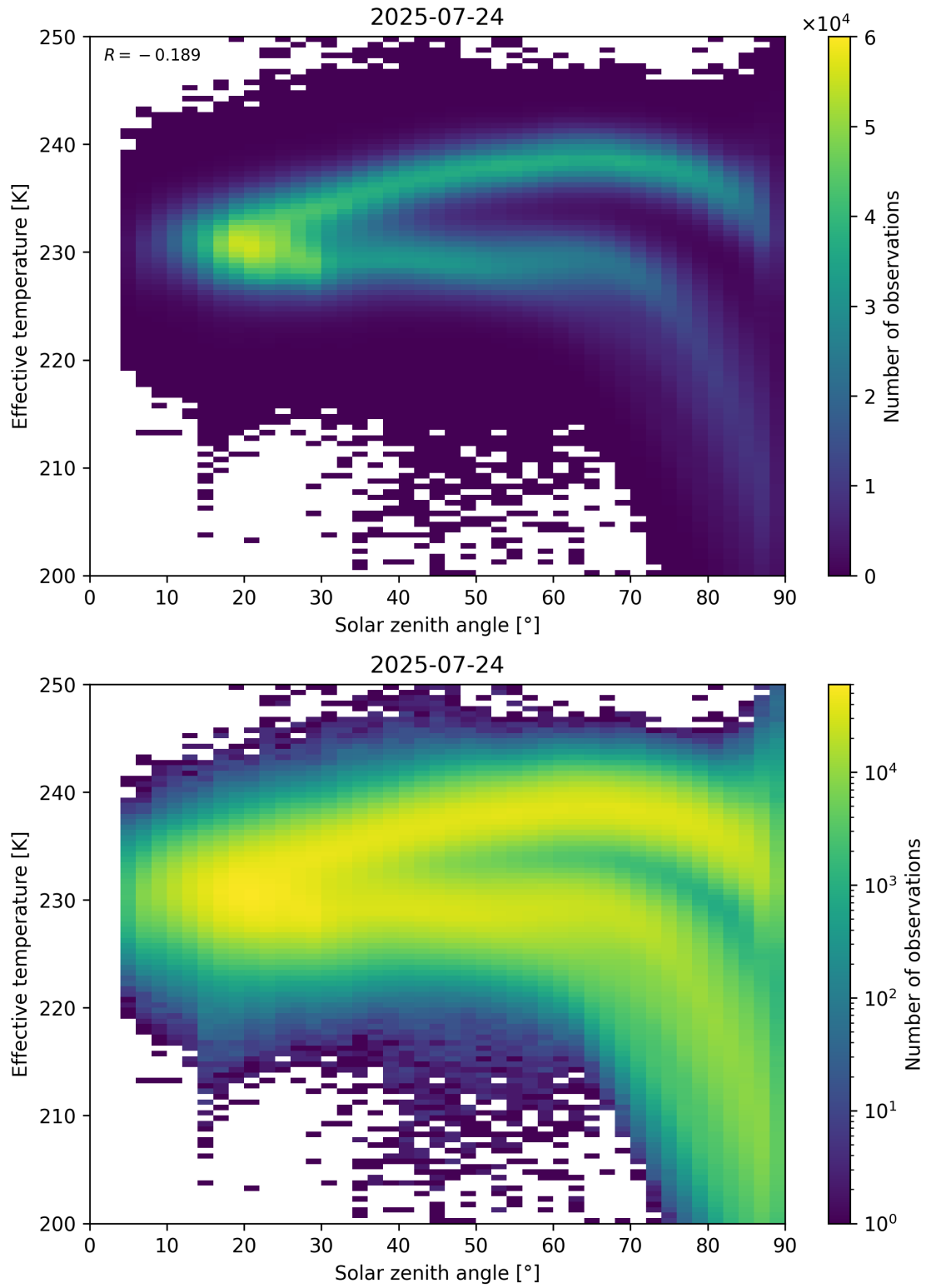
Figure 45: Scatter density plot of “Solar zenith angle” against “Effective temperature” for 2025-07-24 to 2025-07-25.
