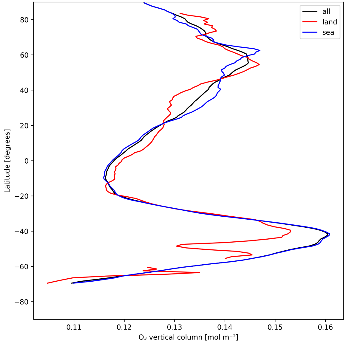
Figure 14: Zonal average of “O 3 vertical column” for 2025-07-24 to 2025-07-25.
