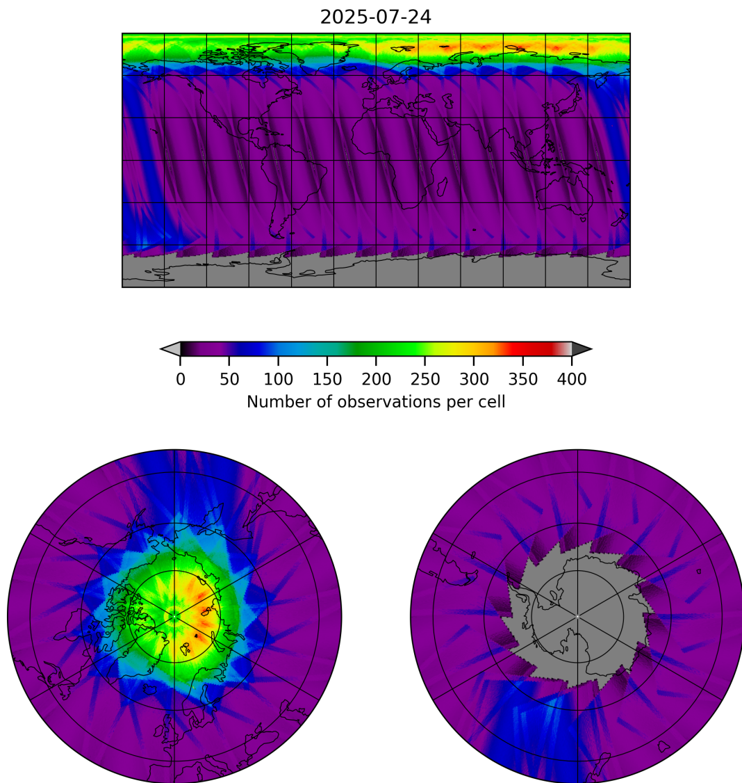
Figure 12: Map of the number of observations for 2025-07-24 to 2025-07-25
