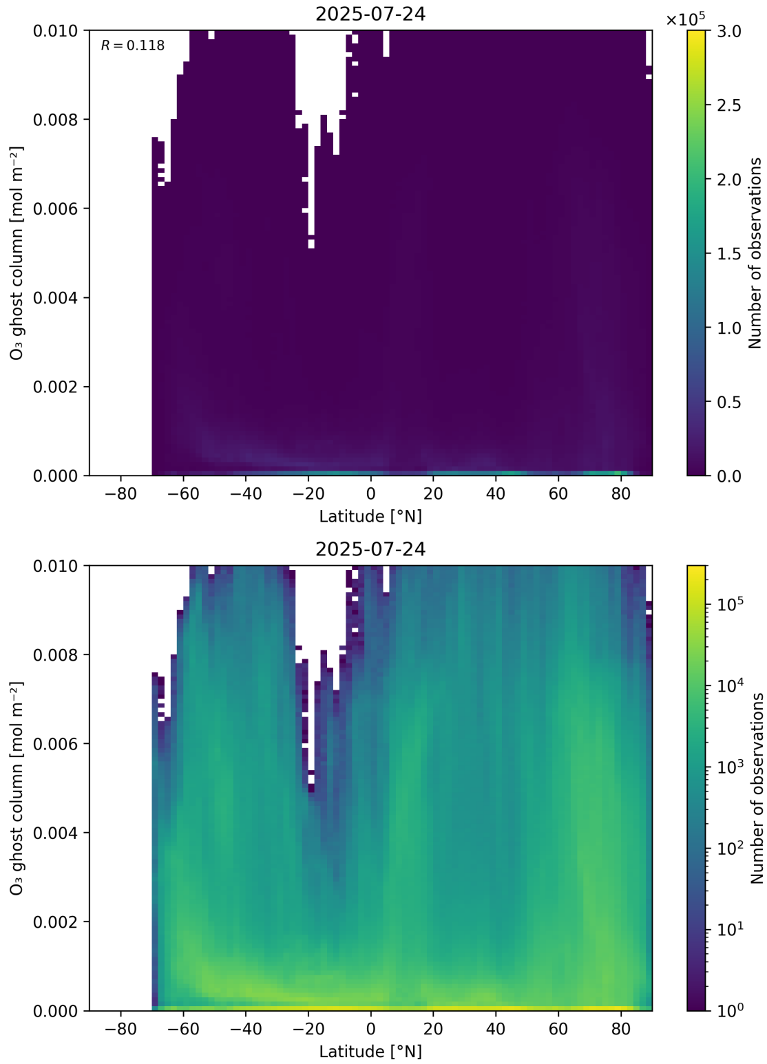
Figure 35: Scatter density plot of “Latitude” against “O 3 ghost column” for 2025-07-24 to 2025-07-25.
