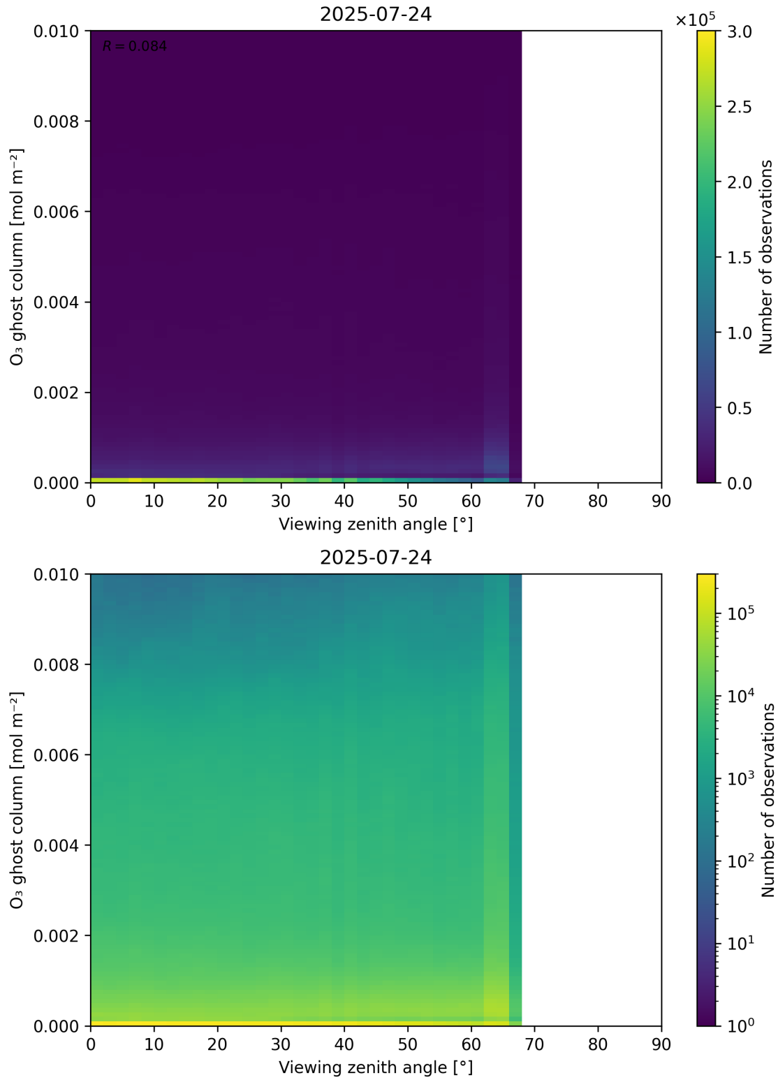
Figure 51: Scatter density plot of “Viewing zenith angle” against “O 3 ghost column” for 2025-07-24 to 2025-07-25.
