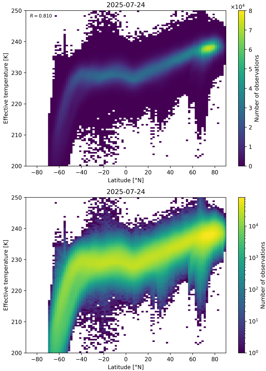
Figure 34: Scatter density plot of “Latitude” against “Effective temperature” for 2025-07-24 to 2025-07-25.
