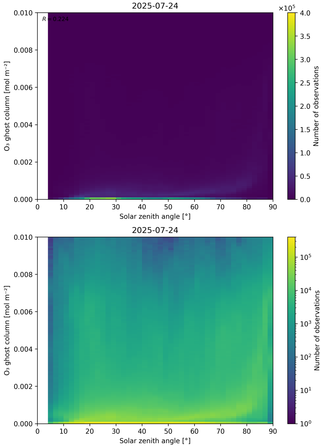
Figure 46: Scatter density plot of “Solar zenith angle” against “O 3 ghost column” for 2025-07-24 to 2025-07-25.
