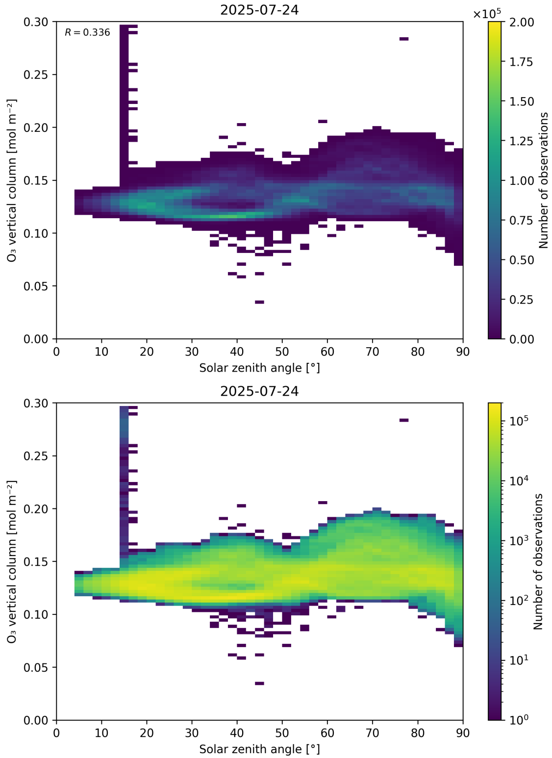
Figure 47: Scatter density plot of “Solar zenith angle” against “O 3 vertical column” for 2025-07-24 to 2025-07-25.
