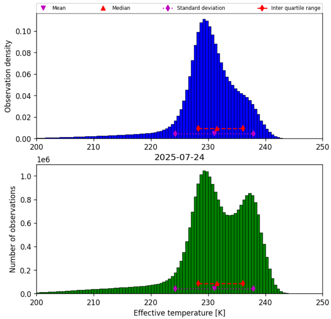
Figure 24: Histogram of “Effective temperature” for 2025-07-24 to 2025-07-25
