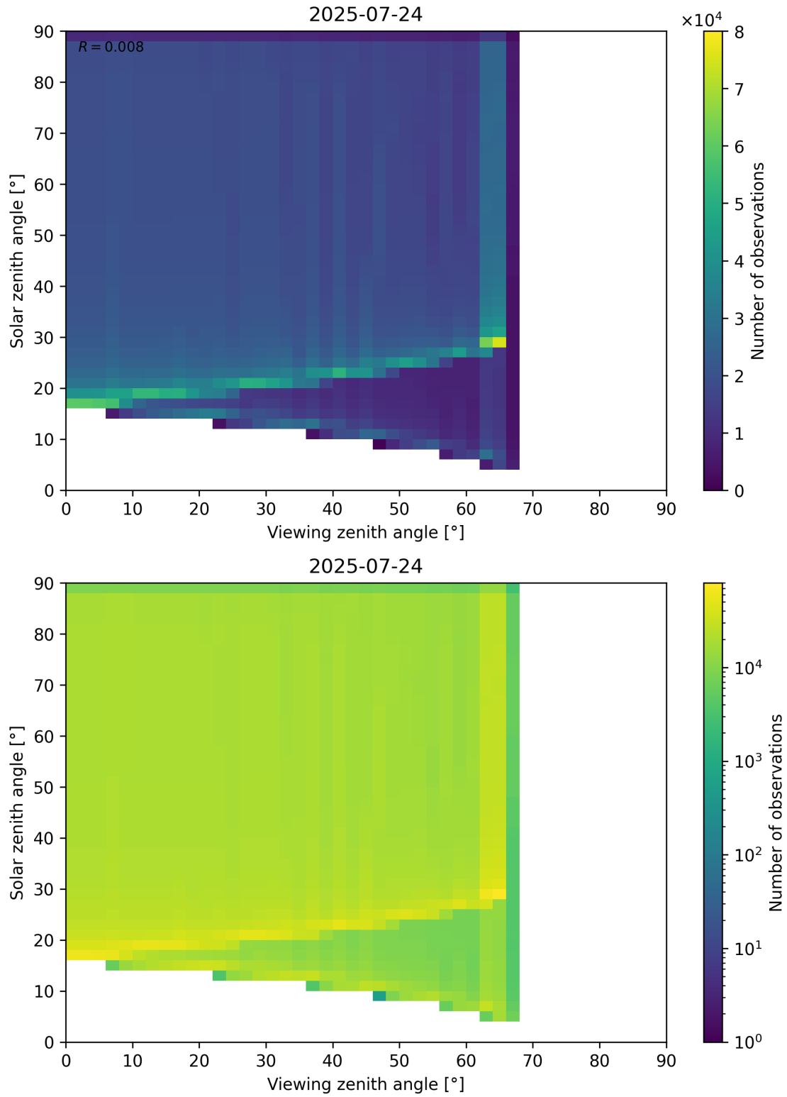
Figure 54: Scatter density plot of “Viewing zenith angle” against “Solar zenith angle” for 2025-07-24 to 2025-07-25.
