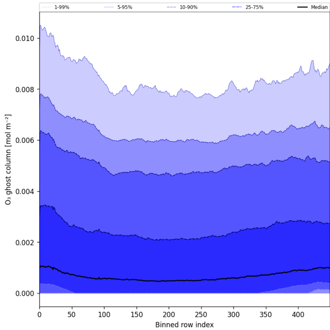
Figure 32: Along track statistics of “O 3 ghost column” for 2025-07-24 to 2025-07-25
