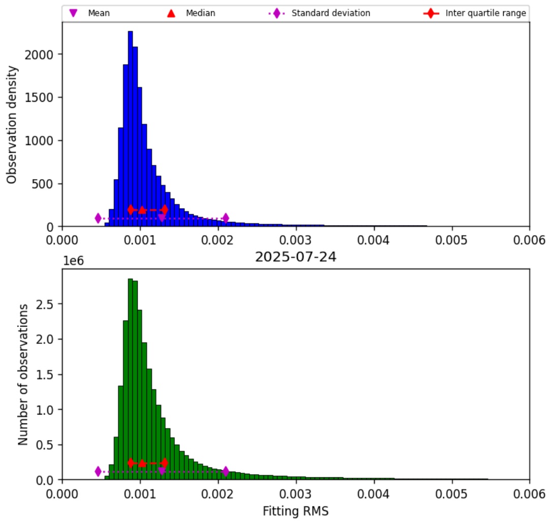
Figure 23: Histogram of “Fitting RMS” for 2025-07-24 to 2025-07-25
