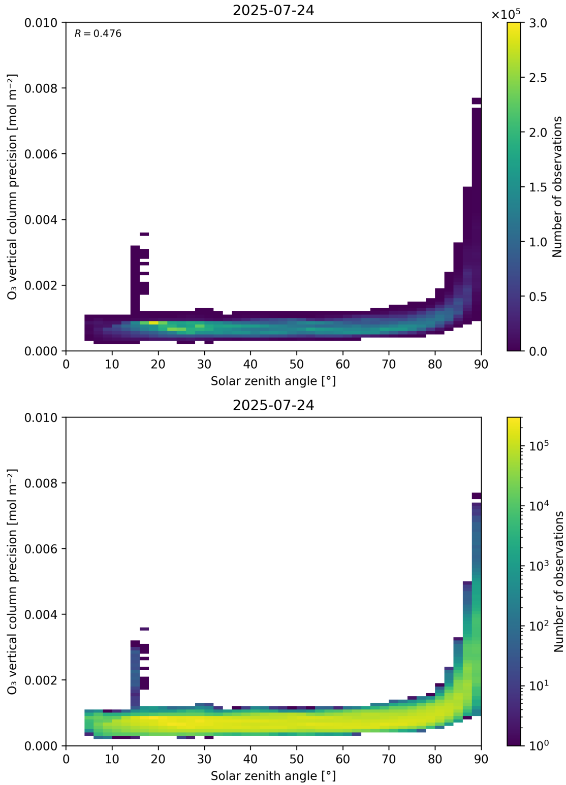
Figure 48: Scatter density plot of “Solar zenith angle” against “O 3 vertical column precision” for 2025-07-24 to 2025-07-25.
