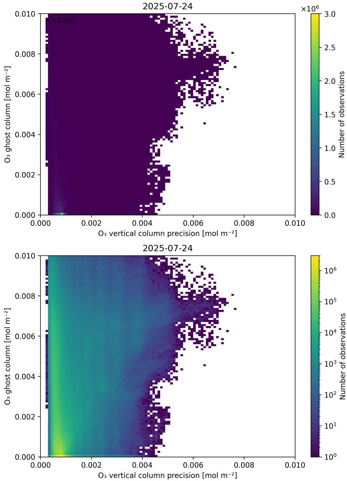
Figure 43: Scatter density plot of “ \text{O}_3 vertical column precision” against “ \text{O}_3 ghost column” for 2025-07-24 to 2025-07-25.
