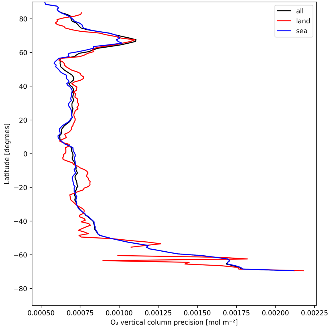
Figure 15: Zonal average of "O 3 vertical column precision" for 2025-07-24 to 2025-07-25.
