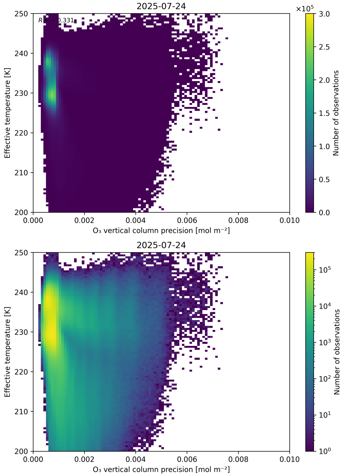
Figure 42: Scatter density plot of “O 3 vertical column precision” against “Effective temperature” for 2025-07-24 to 2025-07-25.
