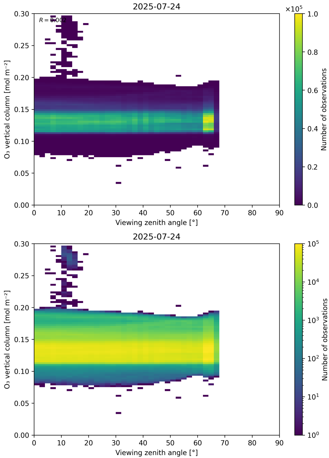
Figure 52: Scatter density plot of “Viewing zenith angle” against “O 3 vertical column” for 2025-07-24 to 2025-07-25.
