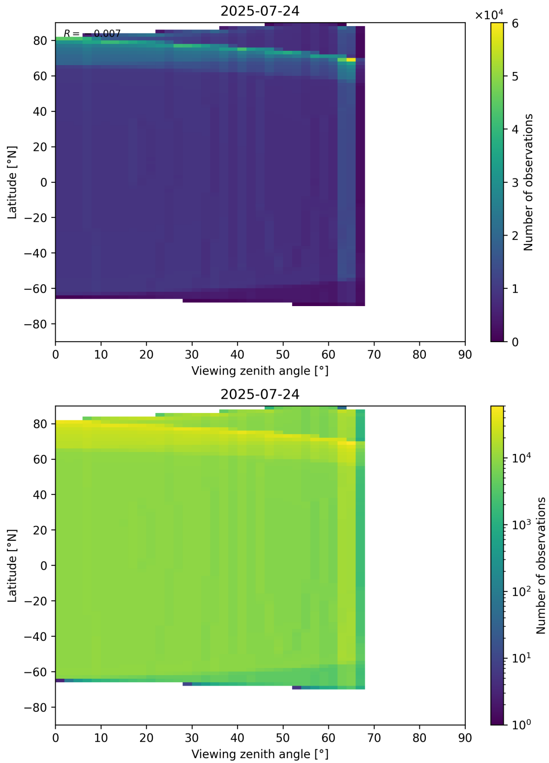
Figure 49: Scatter density plot of “Viewing zenith angle” against “Latitude” for 2025-07-24 to 2025-07-25.
