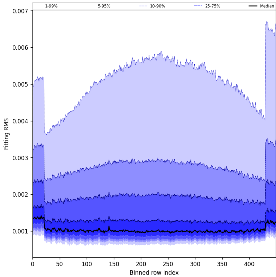
Figure 30: Along track statistics of “Fitting RMS” for 2025-07-24 to 2025-07-25
