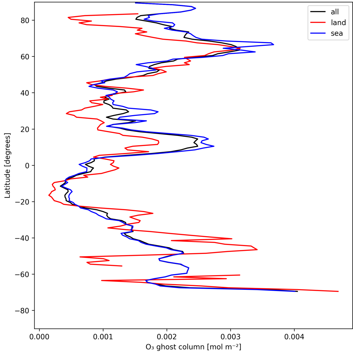
Figure 18: Zonal average of "O 3 ghost column" for 2025-07-24 to 2025-07-25.
