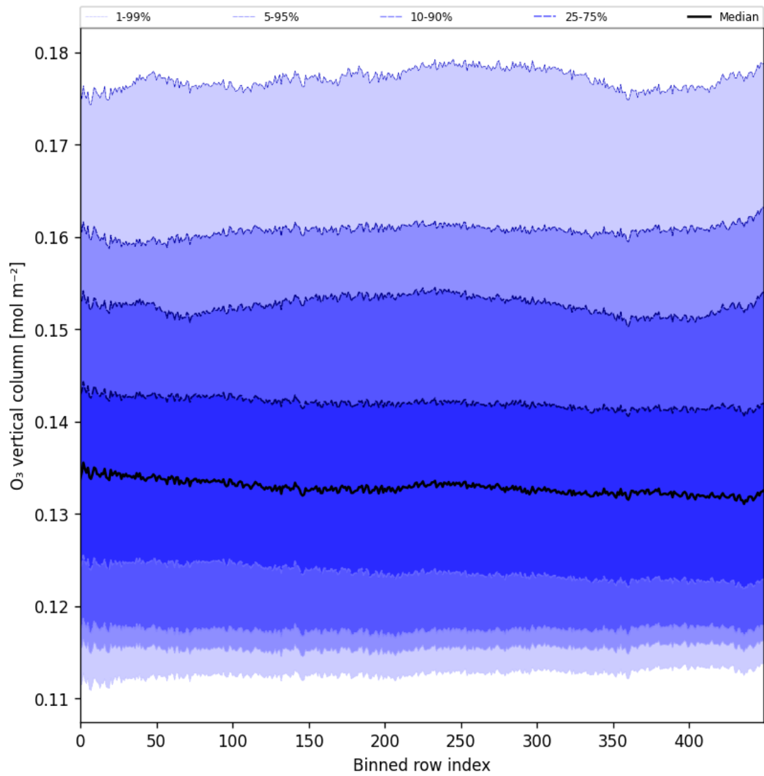
Figure 28: Along track statistics of “O 3 vertical column” for 2025-07-24 to 2025-07-25
