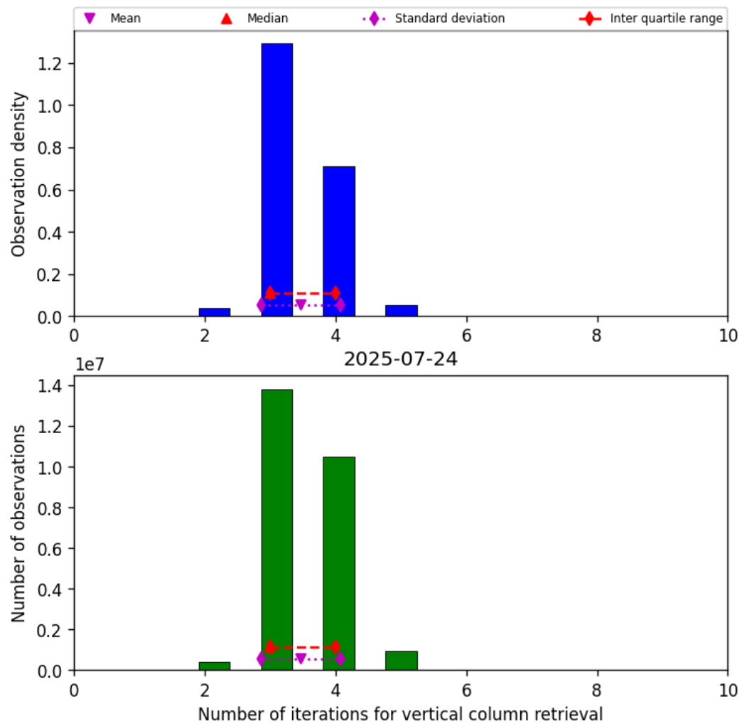
Figure 26: Histogram of “Number of iterations for vertical column retrieval” for 2025-07-24 to 2025-07-25
