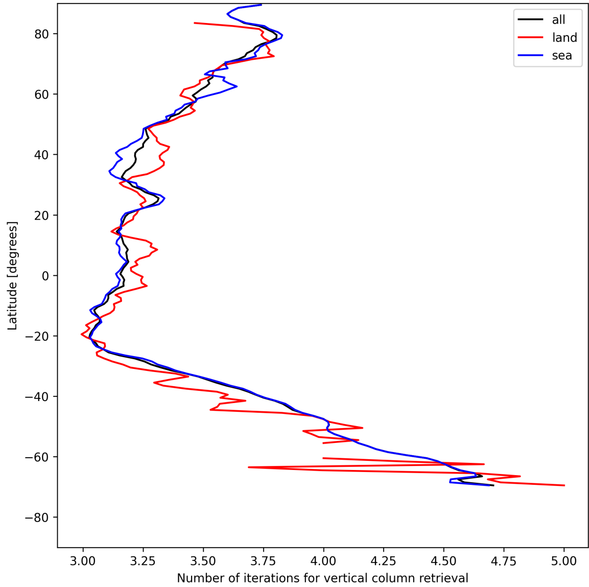
Figure 19: Zonal average of “Number of iterations for vertical column retrieval” for 2025-07-24 to 2025-07-25.
