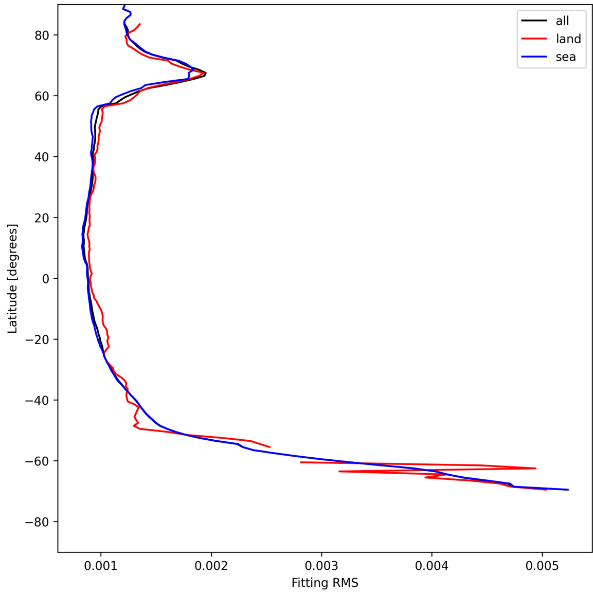
Figure 16: Zonal average of “Fitting RMS” for 2025-07-24 to 2025-07-25.
