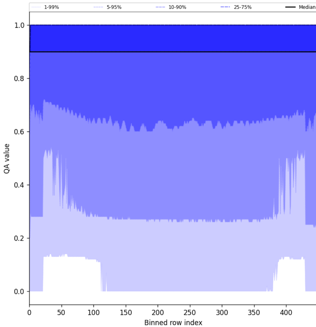
Figure 27: Along track statistics of “QA value” for 2025-07-24 to 2025-07-25
