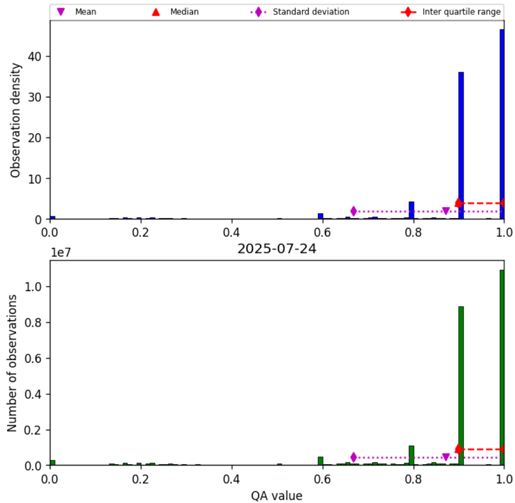
Figure 20: Histogram of “QA value” for 2025-07-24 to 2025-07-25
