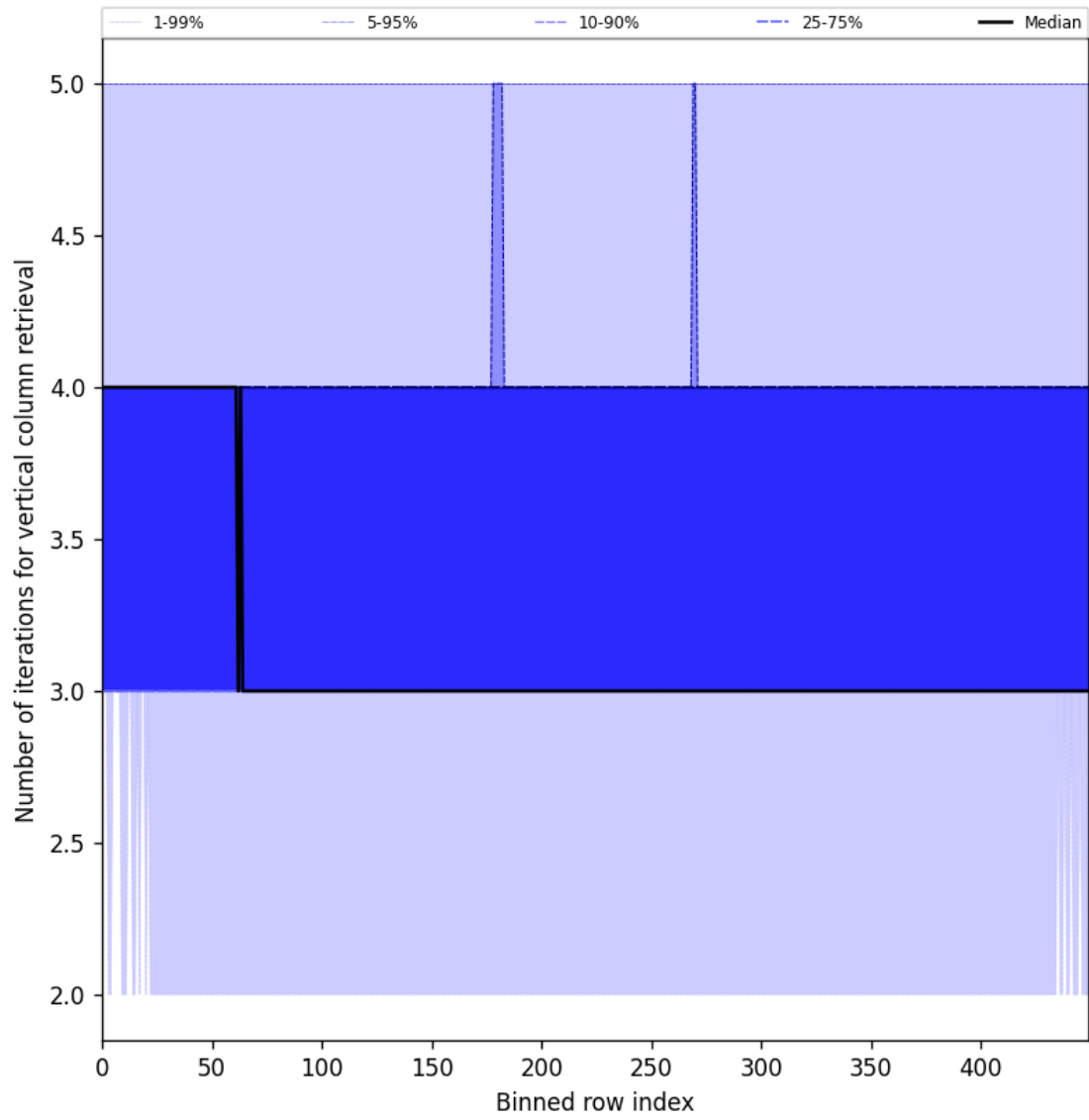
Figure 33: Along track statistics of “Number of iterations for vertical column retrieval” for 2025-07-24 to 2025-07-25
