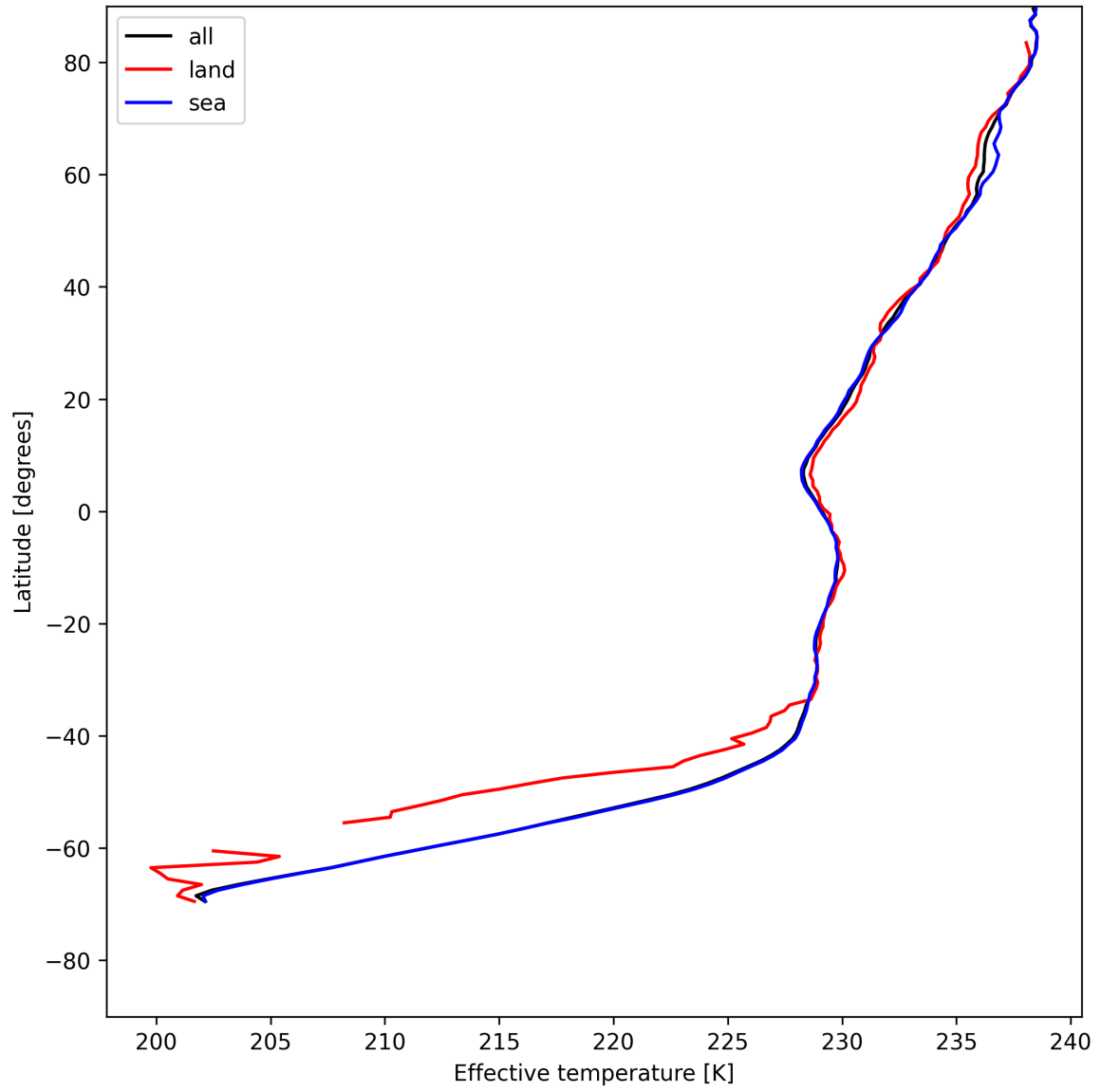
Figure 17: Zonal average of "Effective temperature" for 2025-07-24 to 2025-07-25.
