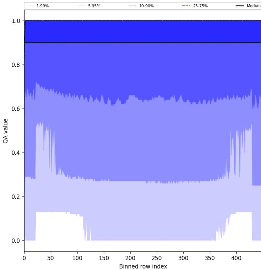
Figure 27: Along track statistics of “QA value” for 2025-07-24 to 2025-07-26
