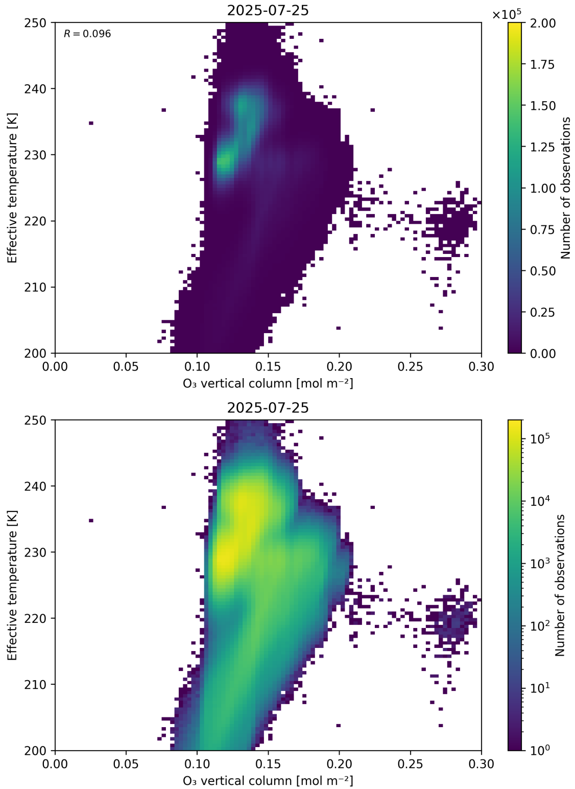
Figure 39: Scatter density plot of “O 3 vertical column” against “Effective temperature” for 2025-07-24 to 2025-07-26.
