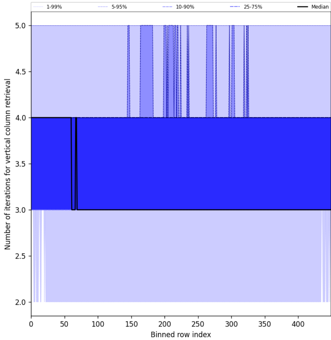
Figure 33: Along track statistics of “Number of iterations for vertical column retrieval” for 2025-07-24 to 2025-07-26
