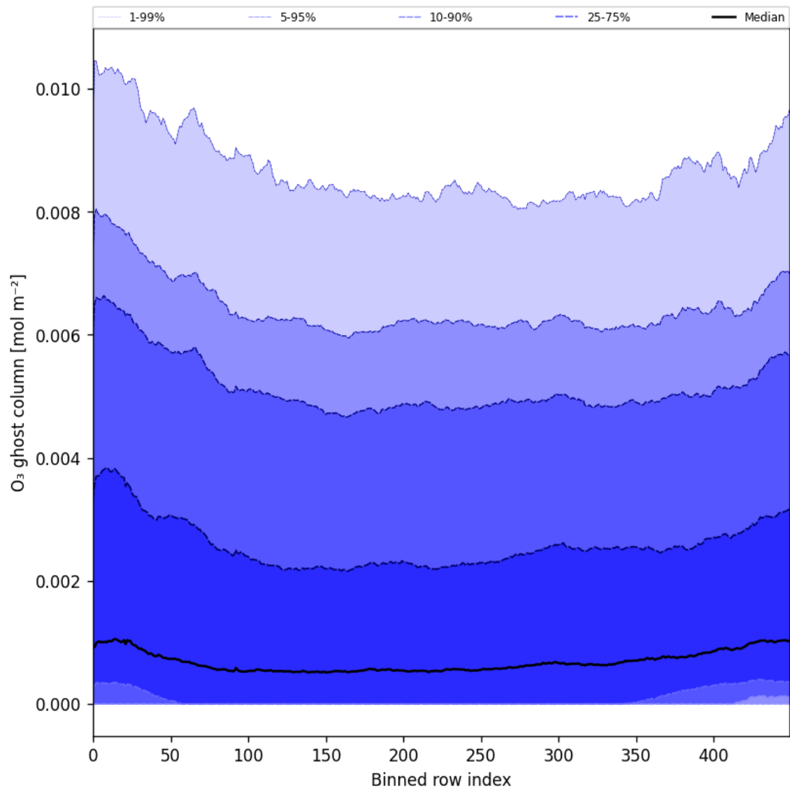
Figure 32: Along track statistics of “O 3 ghost column” for 2025-07-24 to 2025-07-26
