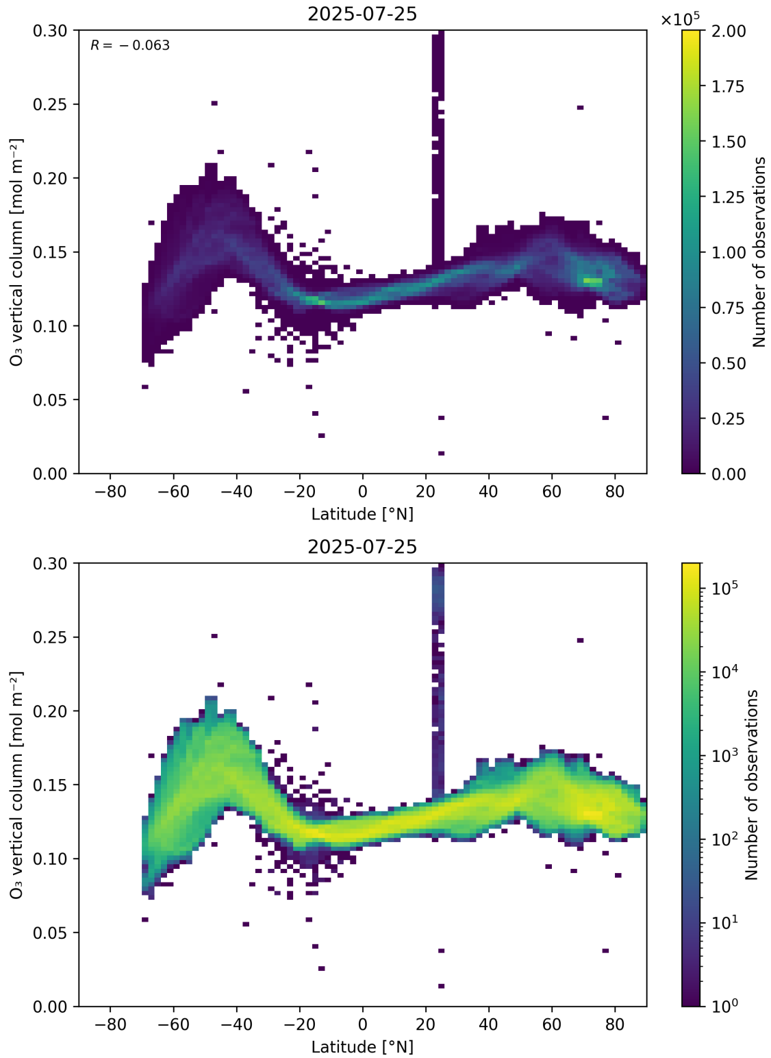
Figure 36: Scatter density plot of “Latitude” against “O 3 vertical column” for 2025-07-24 to 2025-07-26.
