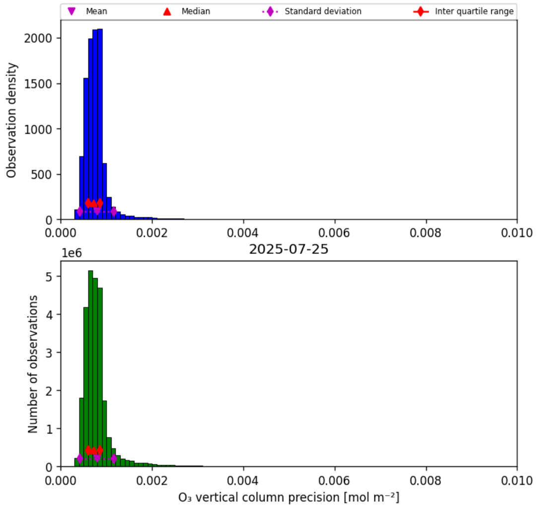
Figure 22: Histogram of “O 3 vertical column precision” for 2025-07-24 to 2025-07-26
