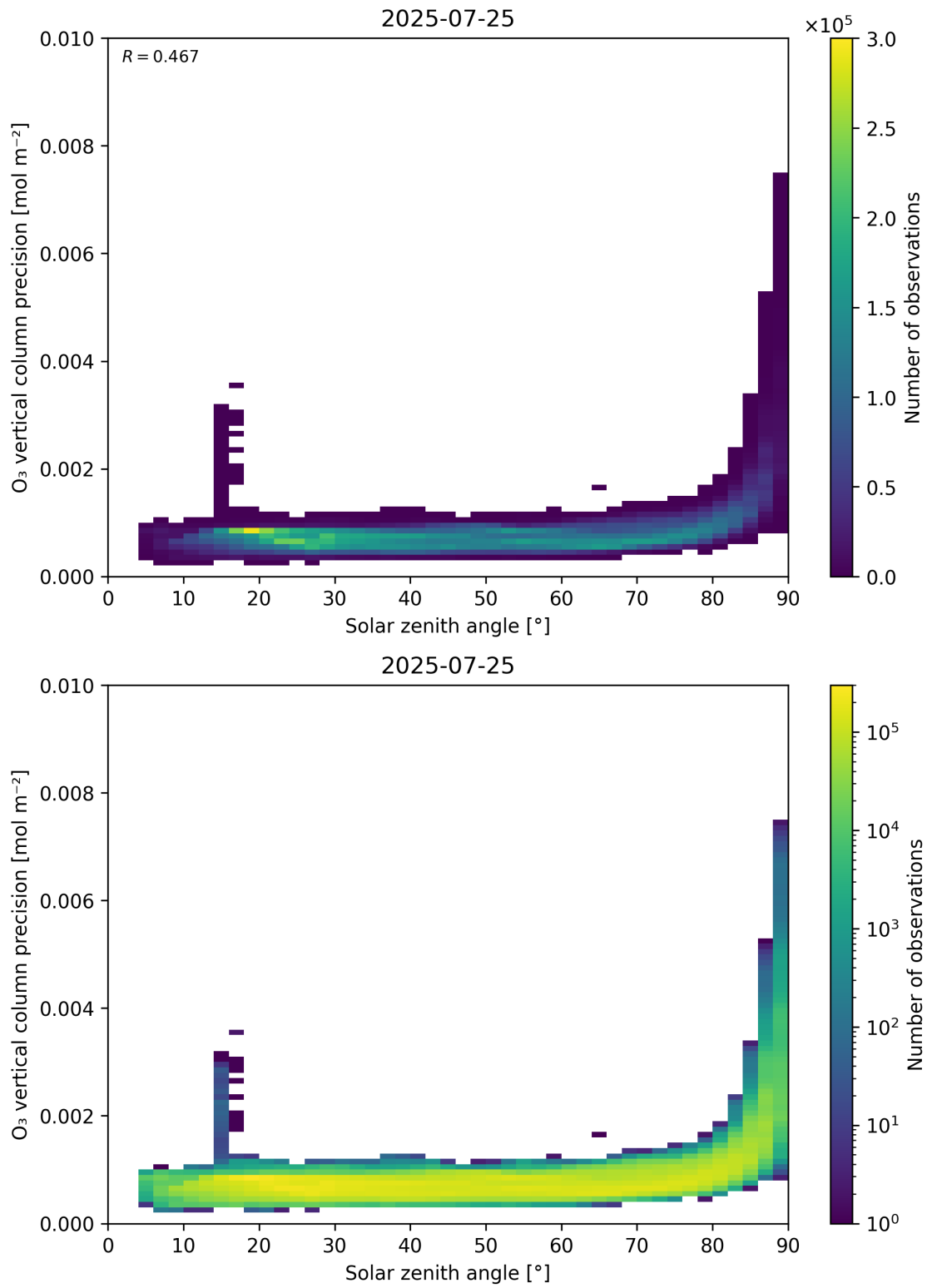
Figure 48: Scatter density plot of “Solar zenith angle” against “O 3 vertical column precision” for 2025-07-24 to 2025-07-26.
