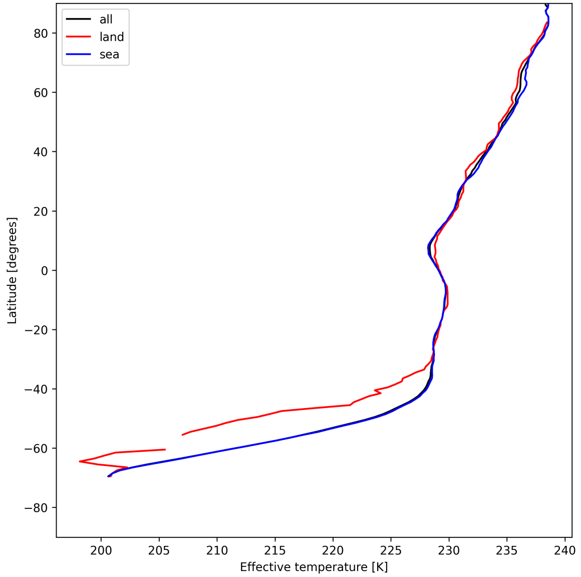
Figure 17: Zonal average of "Effective temperature" for 2025-07-24 to 2025-07-26.
