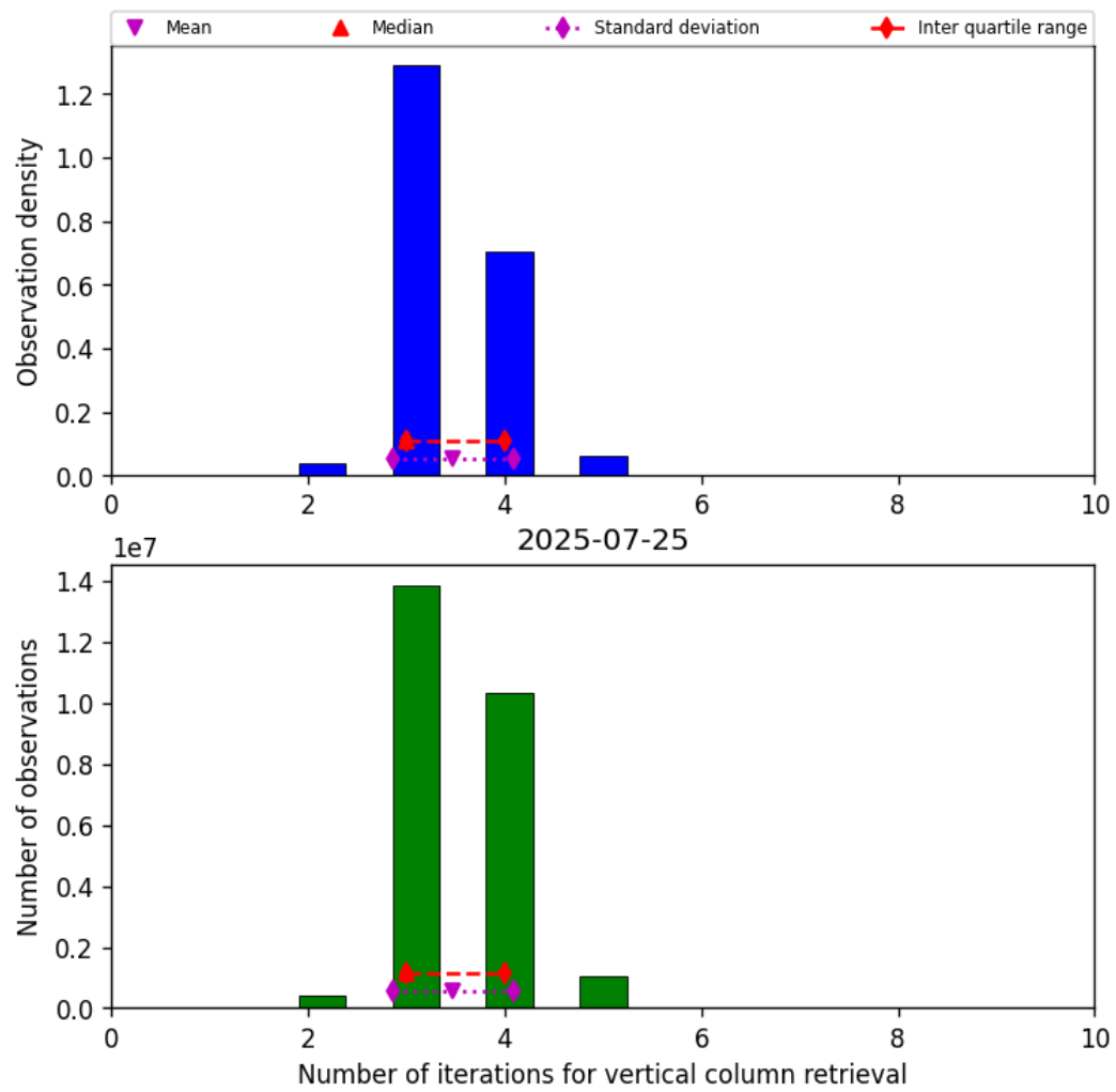
Figure 26: Histogram of “Number of iterations for vertical column retrieval” for 2025-07-24 to 2025-07-26
