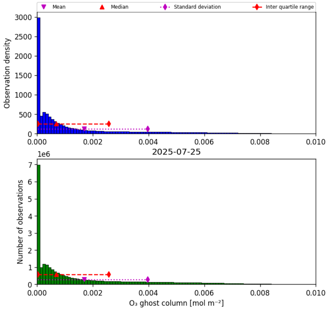
Figure 25: Histogram of “O 3 ghost column” for 2025-07-24 to 2025-07-26
