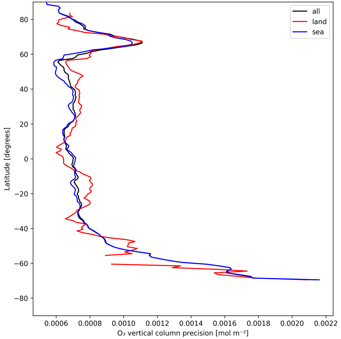
Figure 15: Zonal average of “O 3 vertical column precision” for 2025-07-24 to 2025-07-26.
