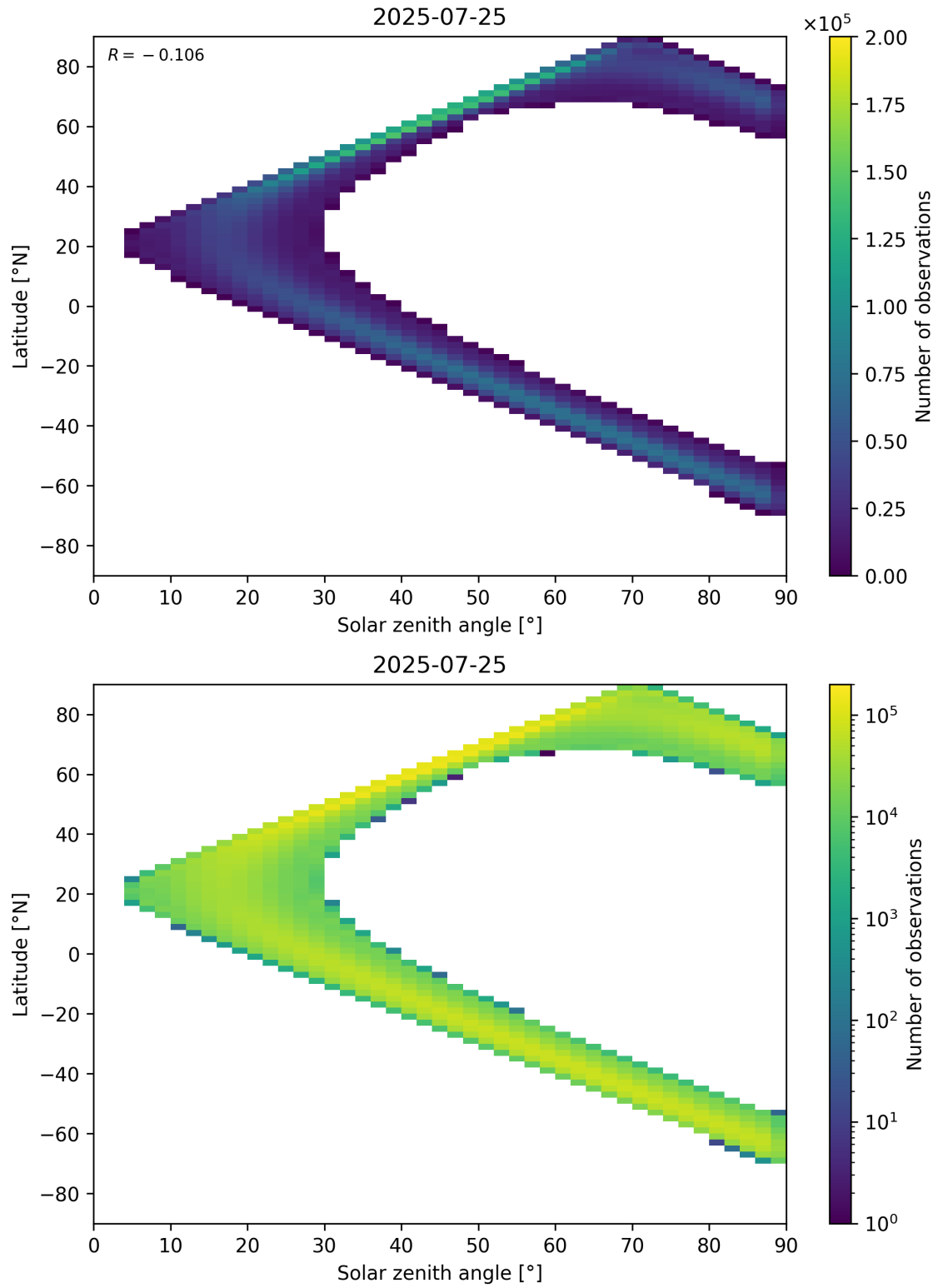
Figure 44: Scatter density plot of “Solar zenith angle” against “Latitude” for 2025-07-24 to 2025-07-26.
