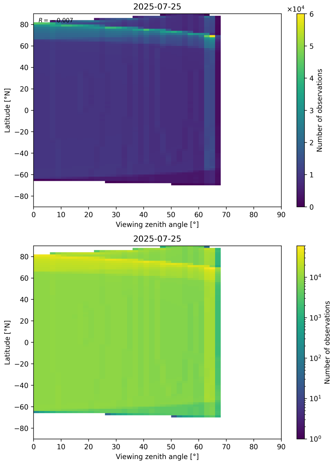
Figure 49: Scatter density plot of “Viewing zenith angle” against “Latitude” for 2025-07-24 to 2025-07-26.
