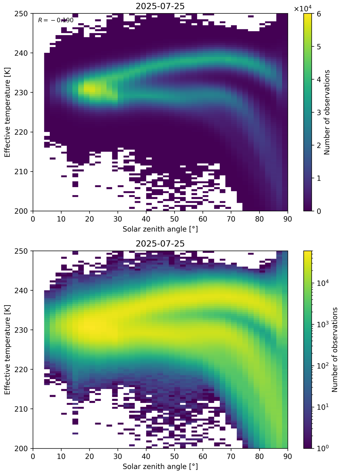
Figure 45: Scatter density plot of “Solar zenith angle” against “Effective temperature” for 2025-07-24 to 2025-07-26.
