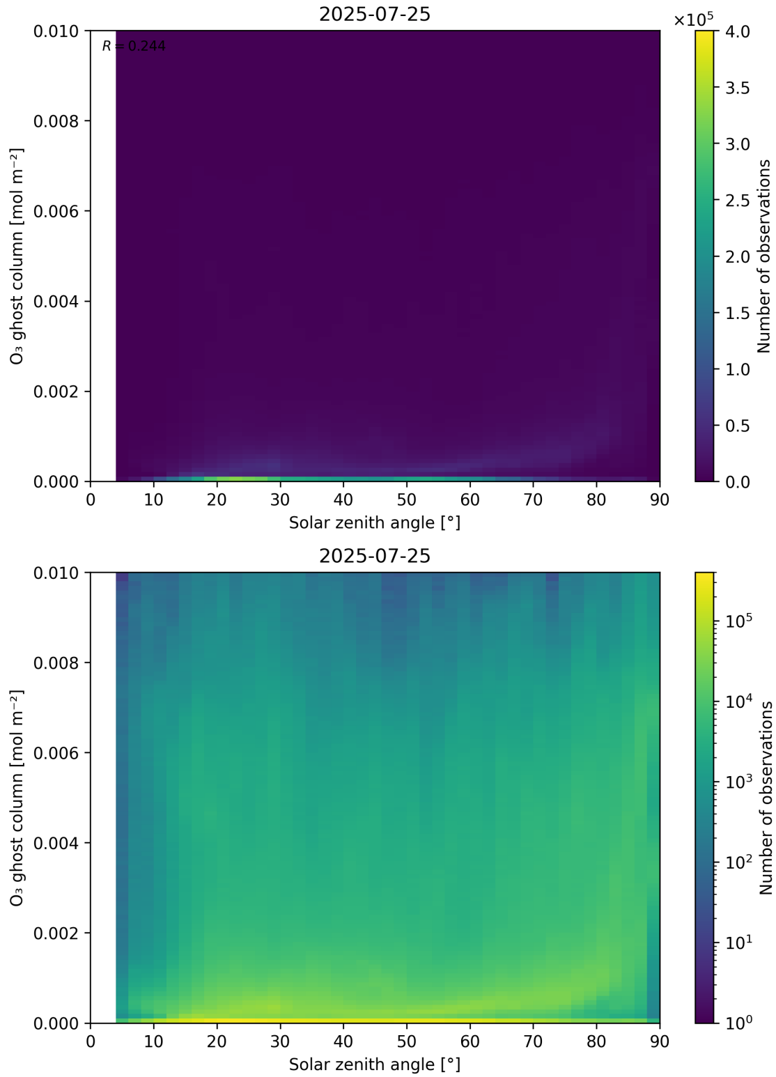
Figure 46: Scatter density plot of “Solar zenith angle” against “O 3 ghost column” for 2025-07-24 to 2025-07-26.
