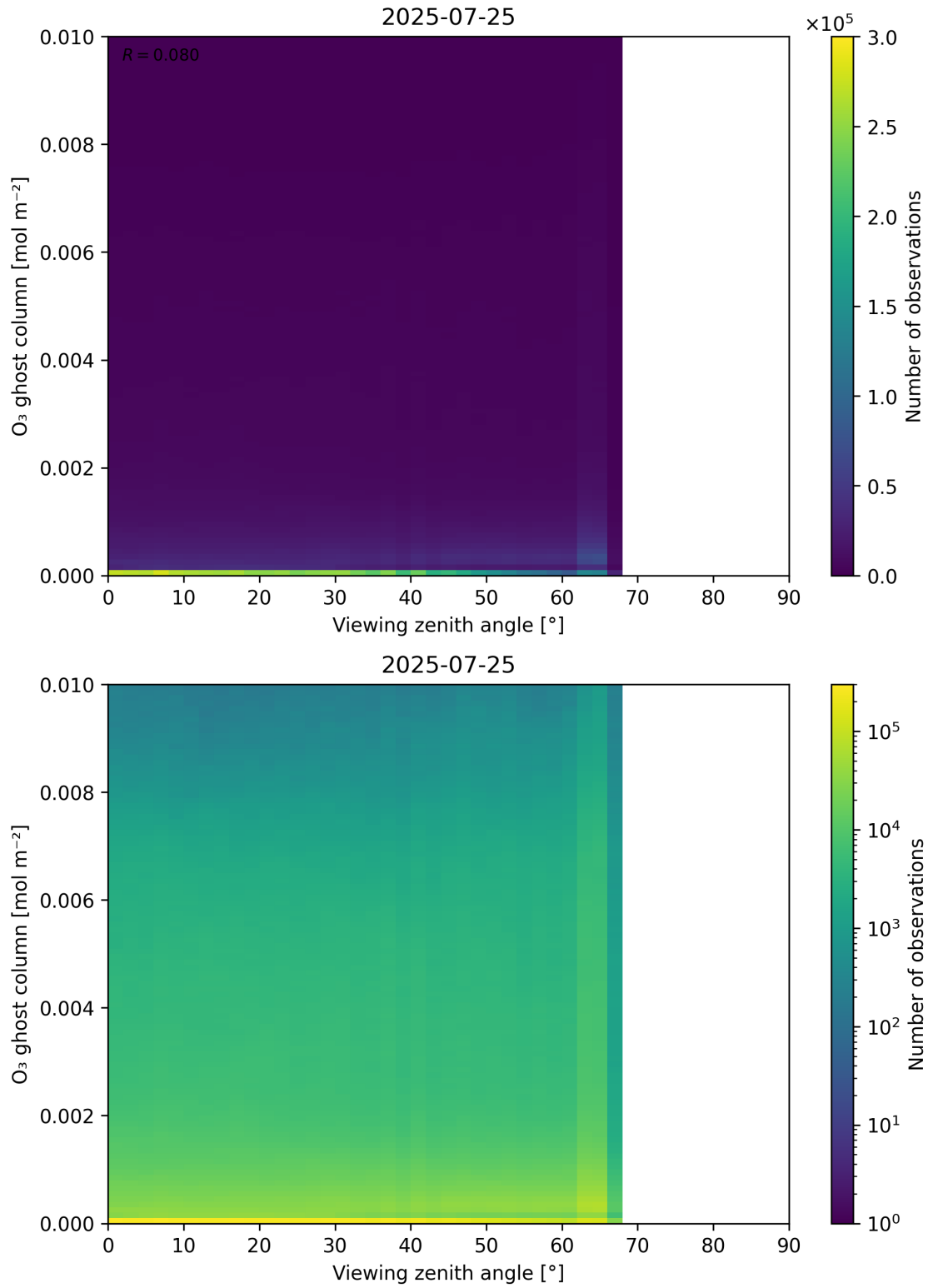
Figure 51: Scatter density plot of “Viewing zenith angle” against “O 3 ghost column” for 2025-07-24 to 2025-07-26.
