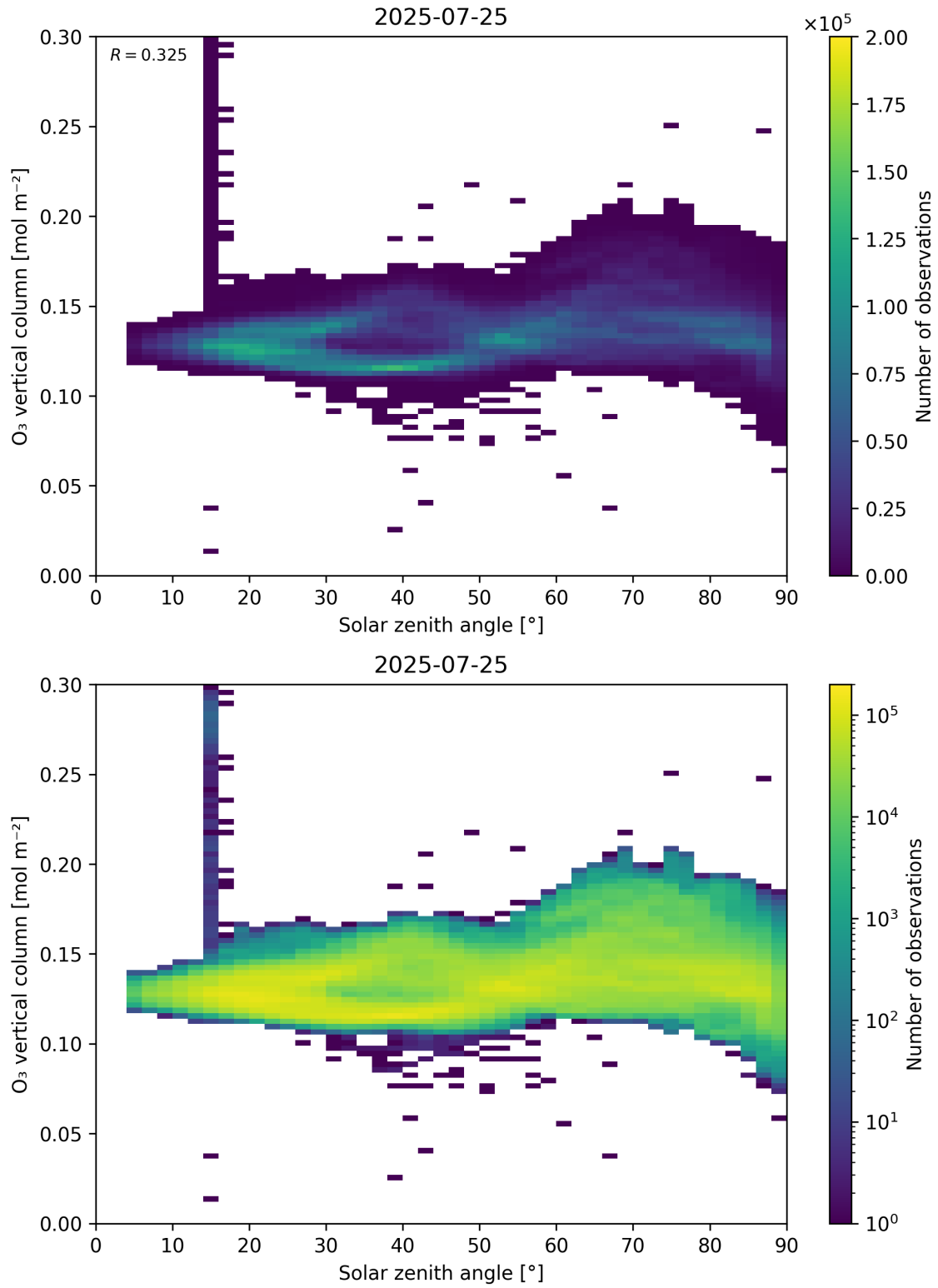
Figure 47: Scatter density plot of “Solar zenith angle” against “O 3 vertical column” for 2025-07-24 to 2025-07-26.
