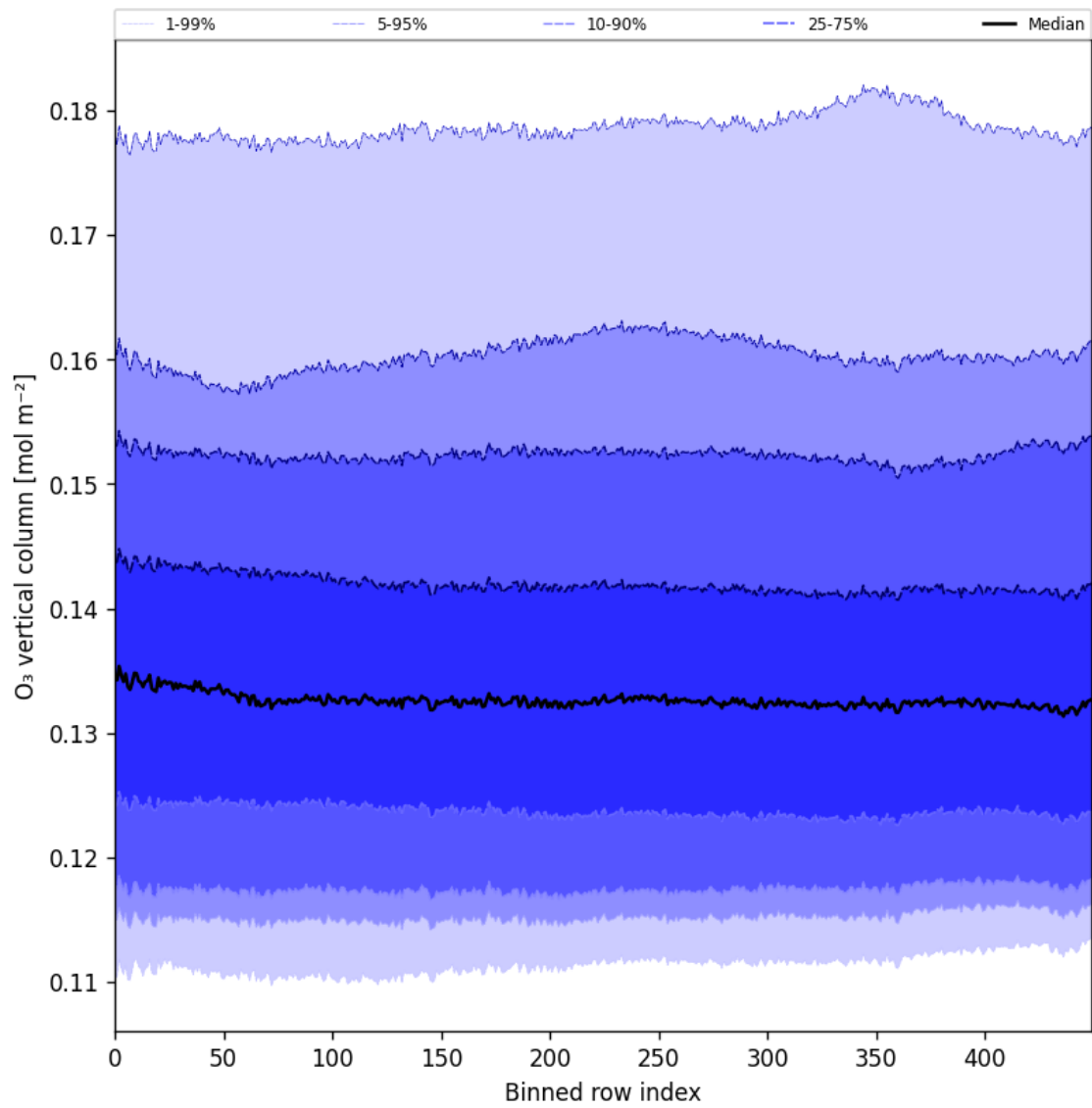
Figure 28: Along track statistics of “O 3 vertical column” for 2025-07-24 to 2025-07-26
