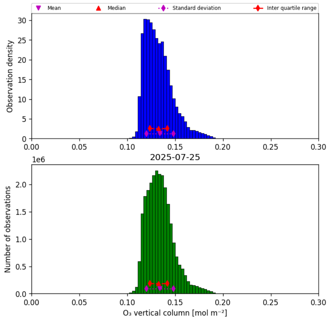
Figure 21: Histogram of “O 3 vertical column” for 2025-07-24 to 2025-07-26
