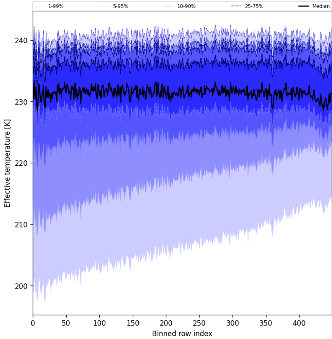
Figure 31: Along track statistics of “Effective temperature” for 2025-07-24 to 2025-07-26
