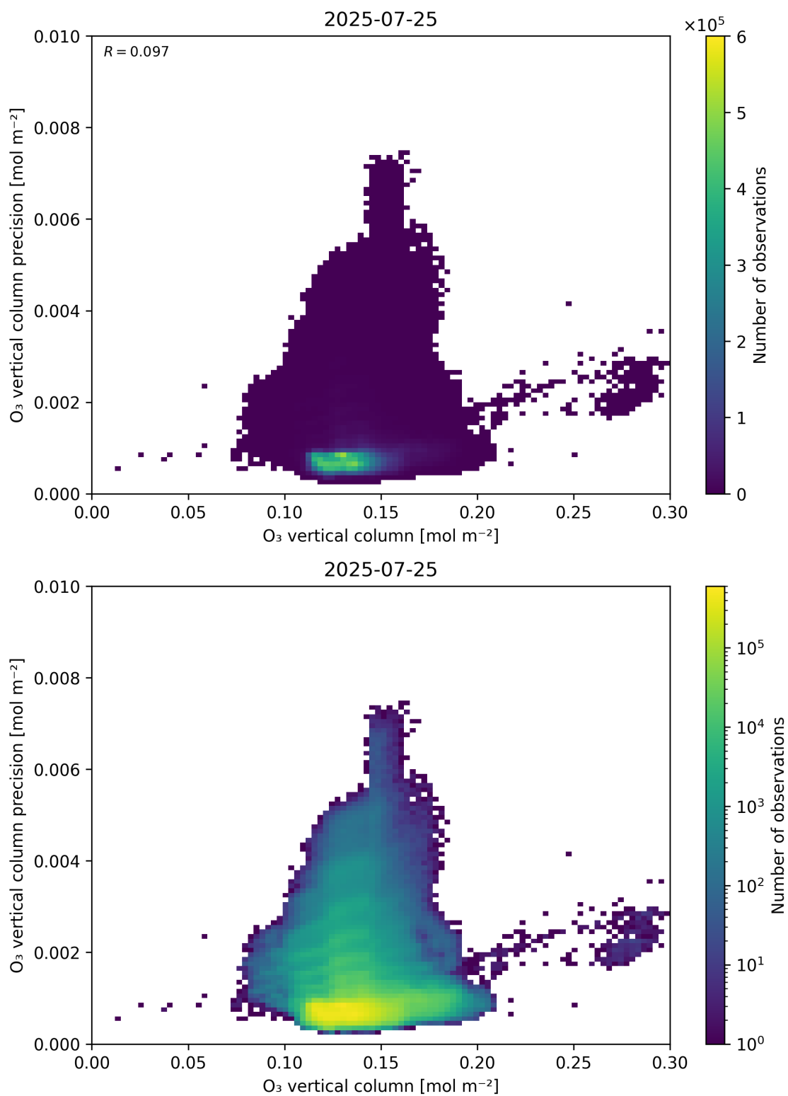
Figure 41: Scatter density plot of “O 3 vertical column” against “O 3 vertical column precision” for 2025-07-24 to 2025-07-26.
