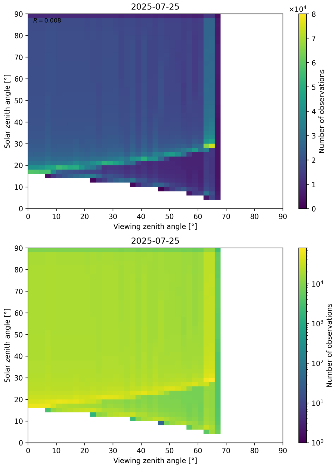
Figure 54: Scatter density plot of “Viewing zenith angle” against “Solar zenith angle” for 2025-07-24 to 2025-07-26.
