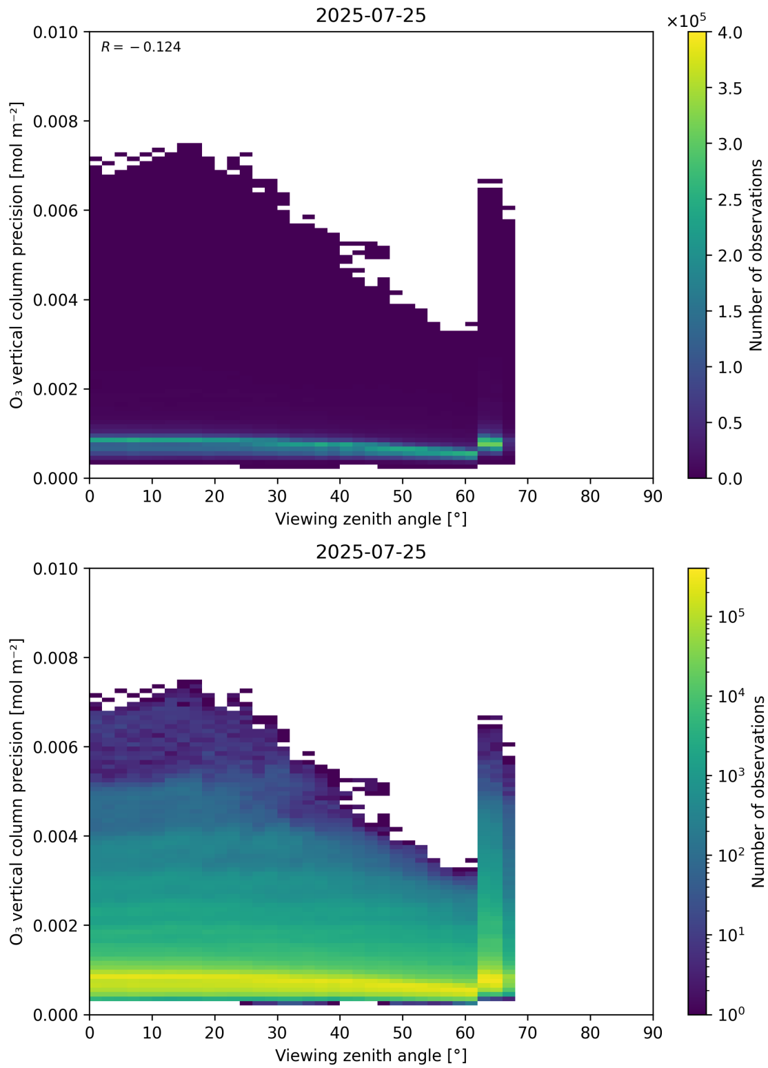
Figure 53: Scatter density plot of “Viewing zenith angle” against “O 3 vertical column precision” for 2025-07-24 to 2025-07-26.
