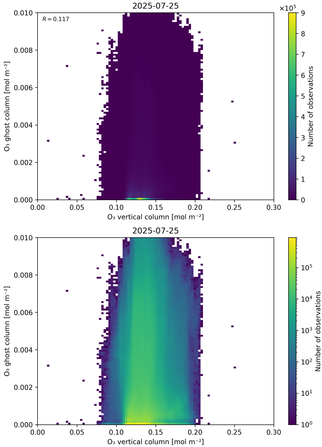
Figure 40: Scatter density plot of “O 3 vertical column” against “O 3 ghost column” for 2025-07-24 to 2025-07-26.
