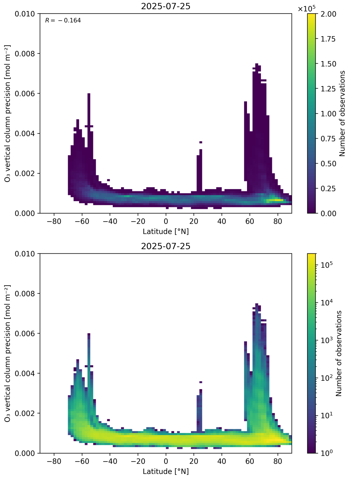
Figure 37: Scatter density plot of “Latitude” against “O 3 vertical column precision” for 2025-07-24 to 2025-07-26.
