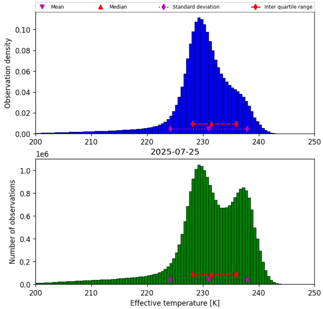
Figure 24: Histogram of “Effective temperature” for 2025-07-24 to 2025-07-26
