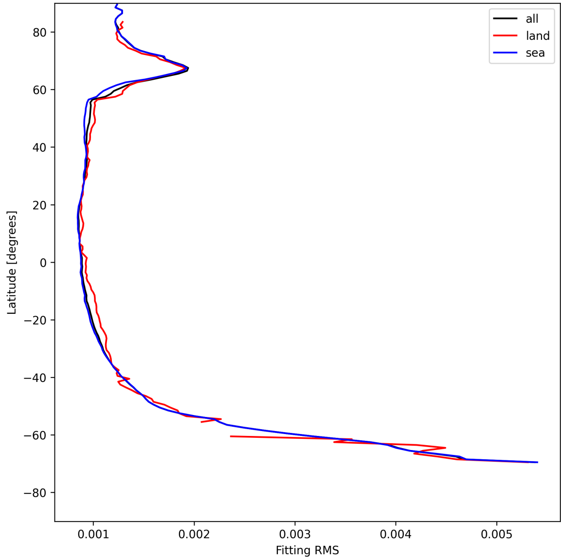
Figure 16: Zonal average of “Fitting RMS” for 2025-07-24 to 2025-07-26.
