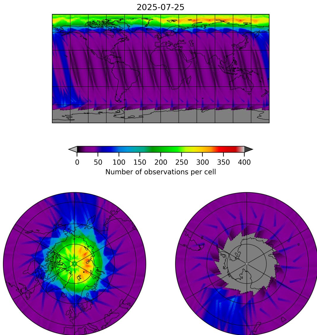
Figure 12: Map of the number of observations for 2025-07-24 to 2025-07-26
