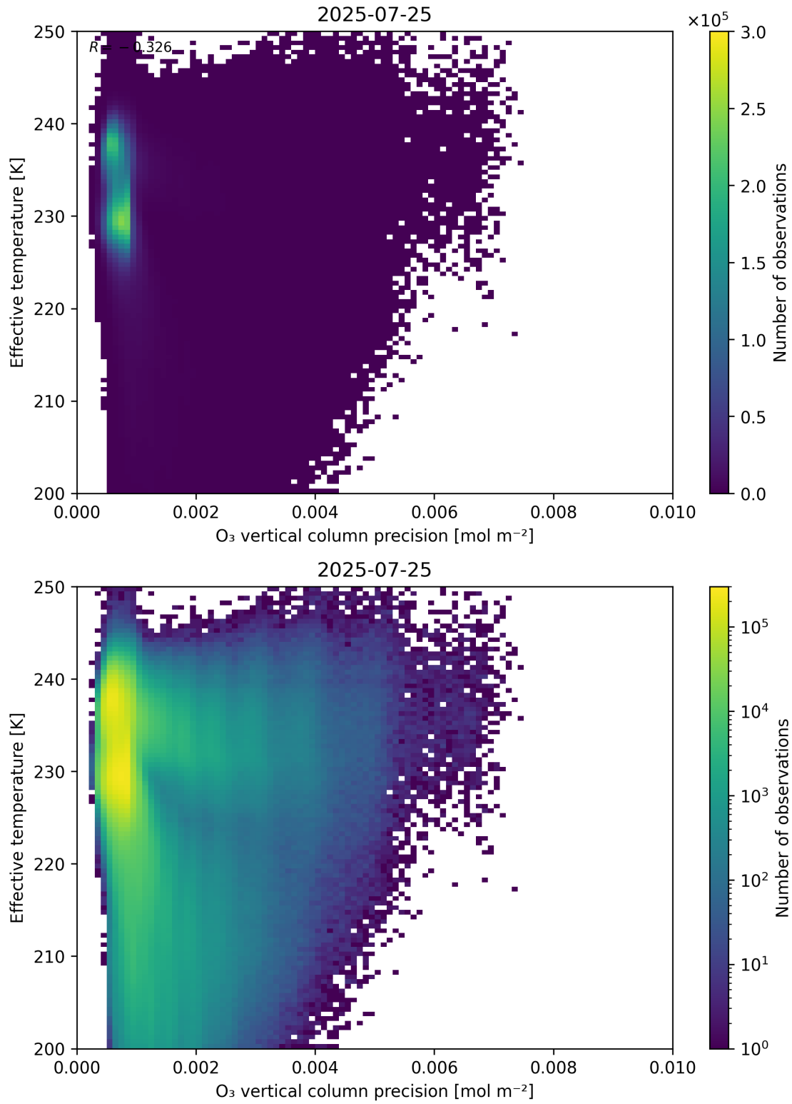
Figure 42: Scatter density plot of “O 3 vertical column precision” against “Effective temperature” for 2025-07-24 to 2025-07-26.
