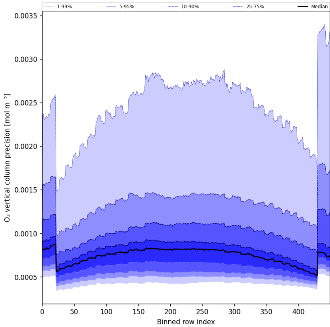
Figure 29: Along track statistics of “O 3 vertical column precision” for 2025-07-24 to 2025-07-26
