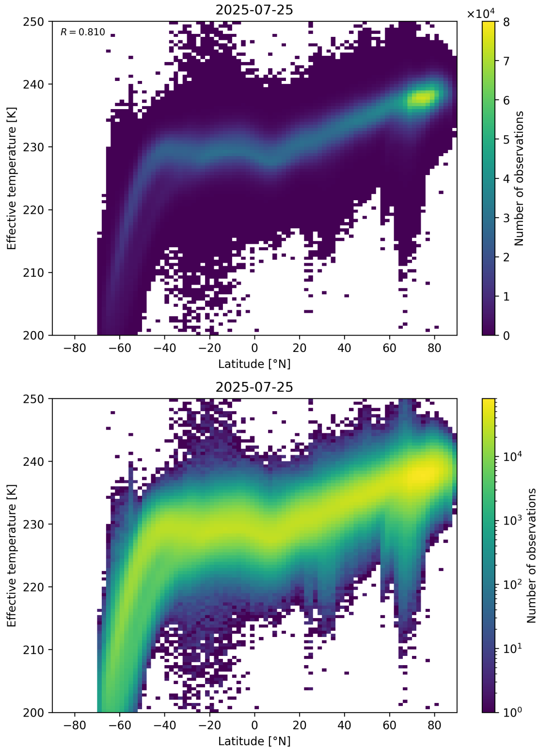
Figure 34: Scatter density plot of “Latitude” against “Effective temperature” for 2025-07-24 to 2025-07-26.
