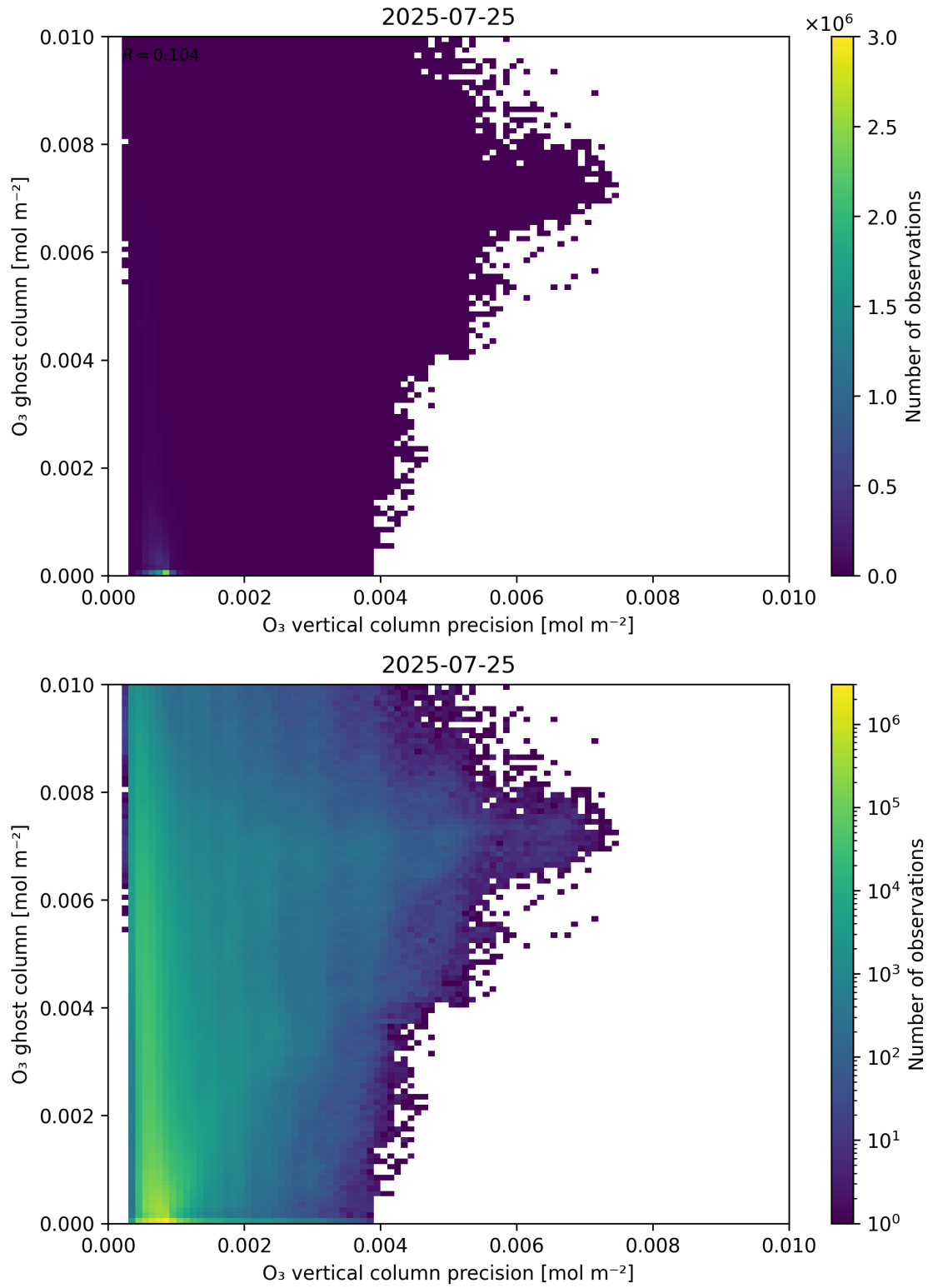
Figure 43: Scatter density plot of “ \text{O}_3 vertical column precision” against “ \text{O}_3 ghost column” for 2025-07-24 to 2025-07-26.
