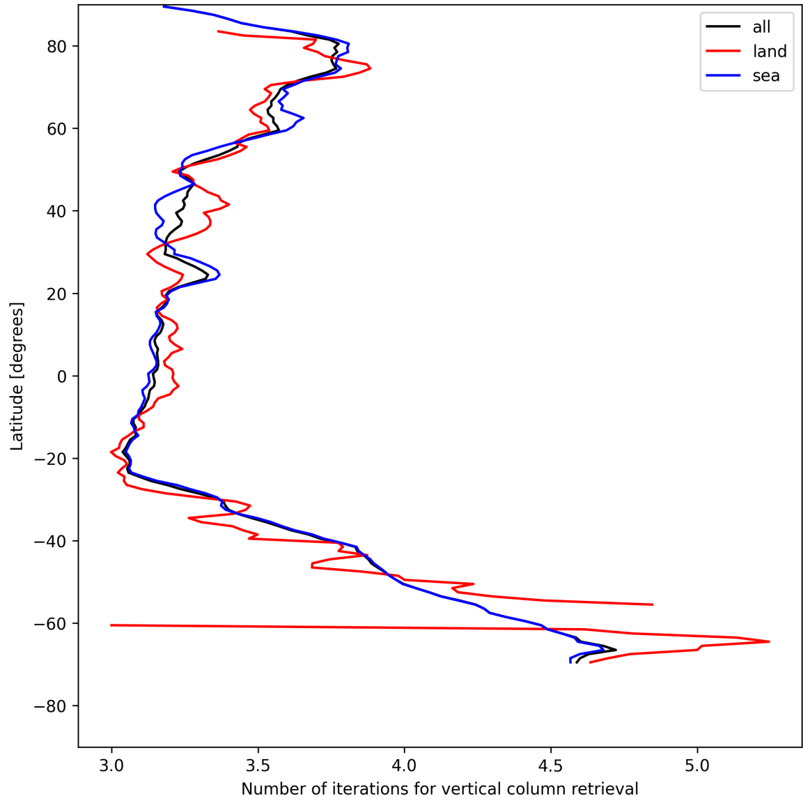
Figure 19: Zonal average of “Number of iterations for vertical column retrieval” for 2025-07-24 to 2025-07-26.
