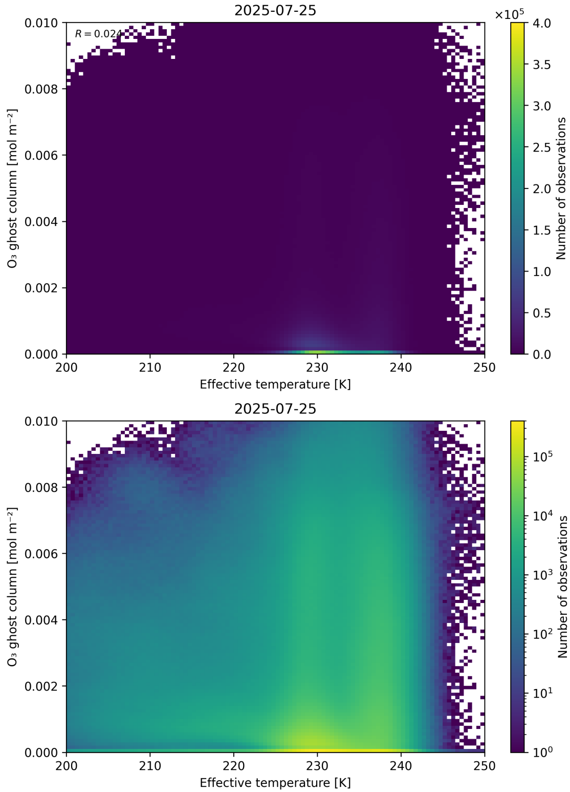
Figure 38: Scatter density plot of “Effective temperature” against “O 3 ghost column” for 2025-07-24 to 2025-07-26.
