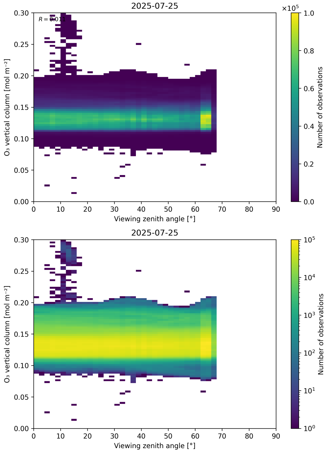
Figure 52: Scatter density plot of “Viewing zenith angle” against “O 3 vertical column” for 2025-07-24 to 2025-07-26.
