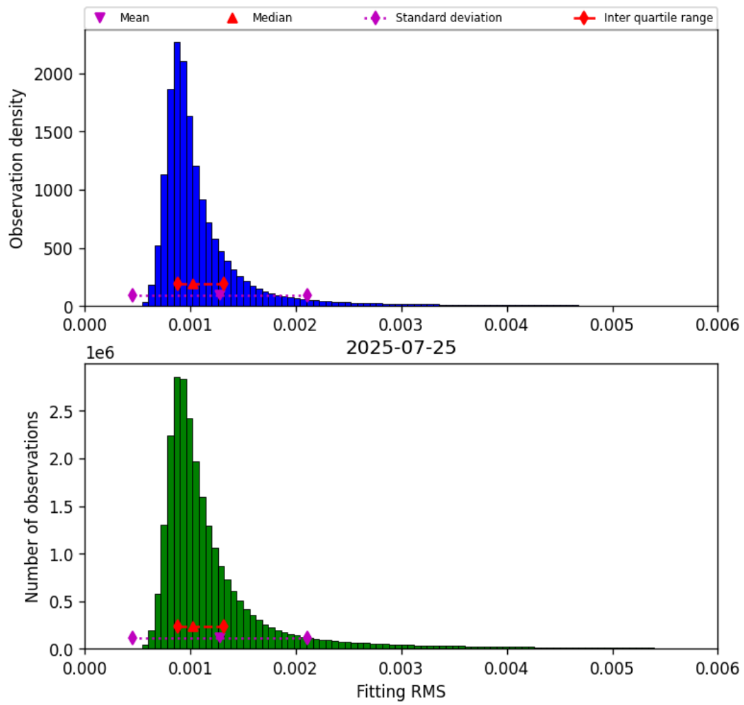
Figure 23: Histogram of “Fitting RMS” for 2025-07-24 to 2025-07-26
