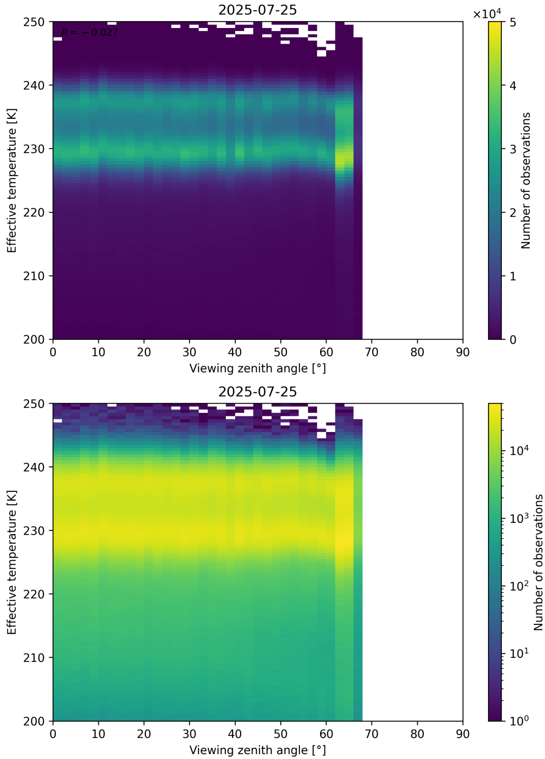
Figure 50: Scatter density plot of “Viewing zenith angle” against “Effective temperature” for 2025-07-24 to 2025-07-26.
