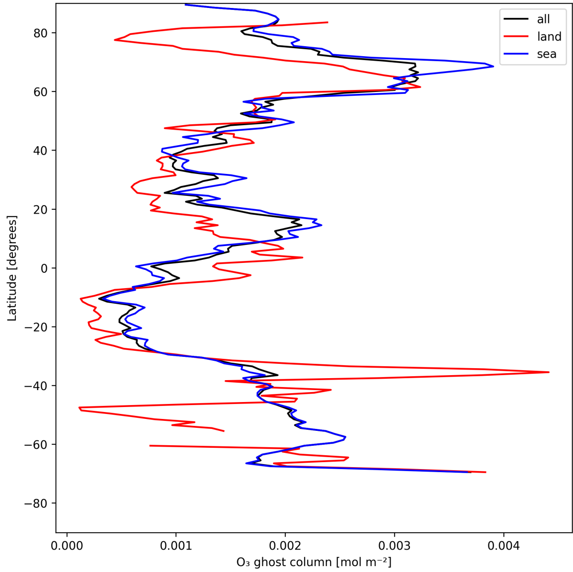
Figure 18: Zonal average of "O 3 ghost column" for 2025-07-24 to 2025-07-26.
