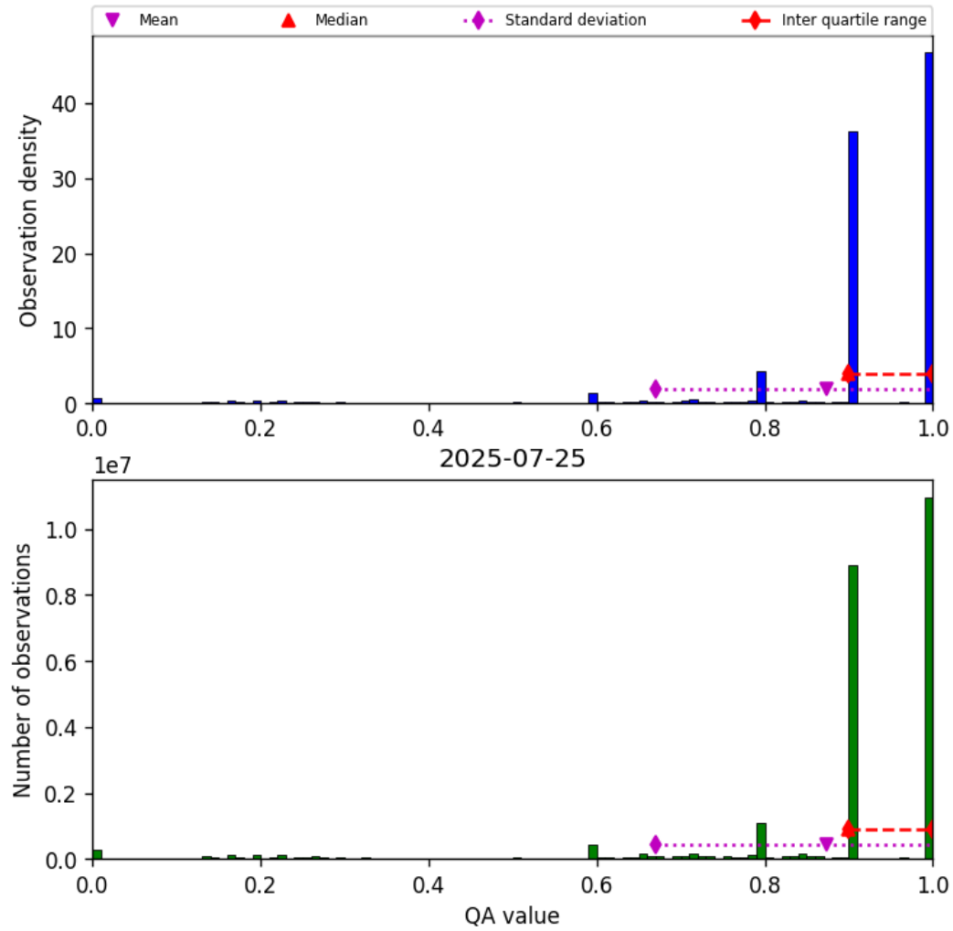
Figure 20: Histogram of “QA value” for 2025-07-24 to 2025-07-26
