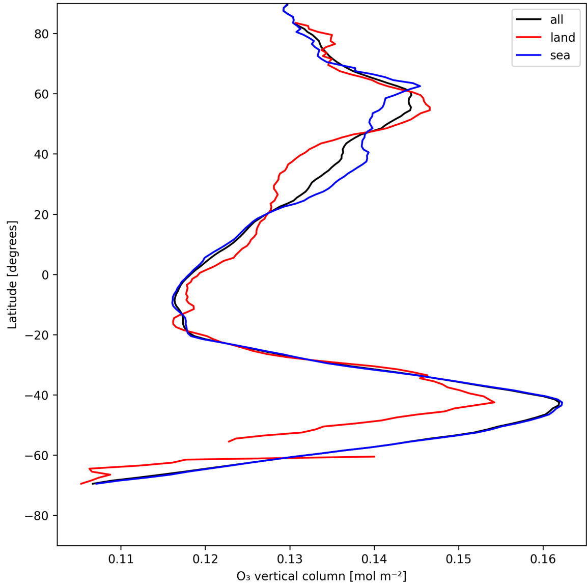
Figure 14: Zonal average of “O 3 vertical column” for 2025-07-24 to 2025-07-26.
