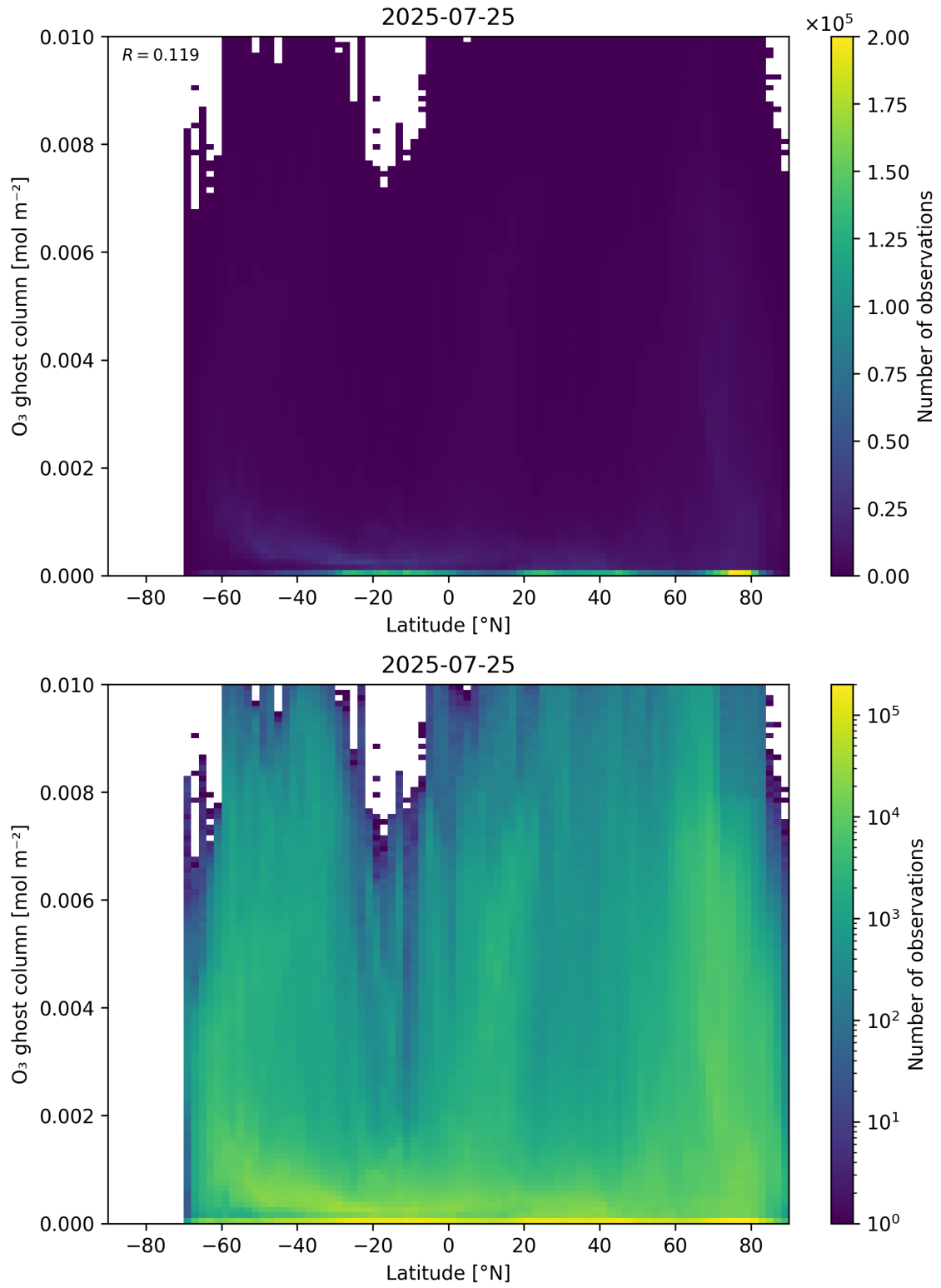
Figure 35: Scatter density plot of “Latitude” against “O 3 ghost column” for 2025-07-24 to 2025-07-26.
