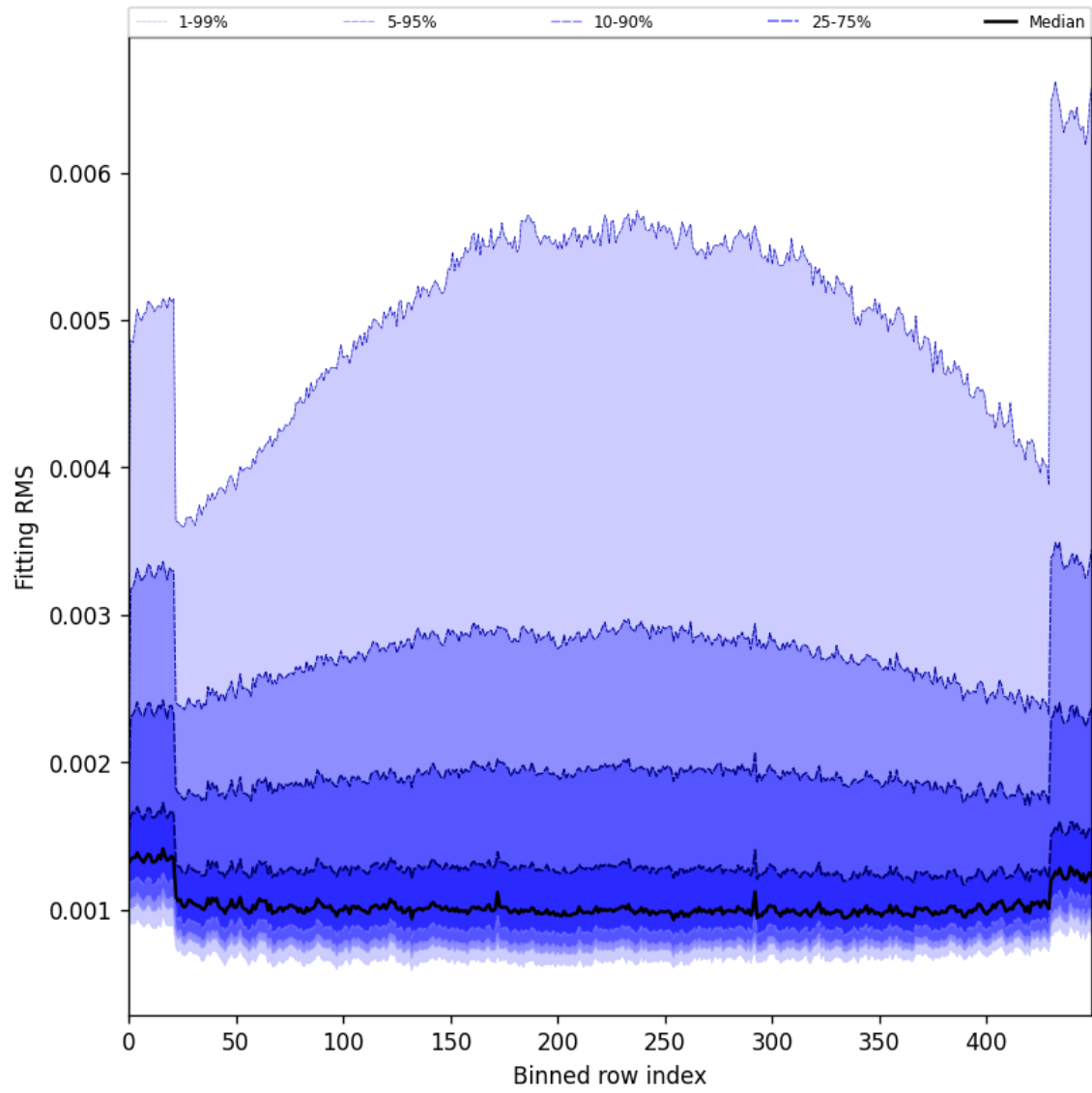
Figure 30: Along track statistics of “Fitting RMS” for 2025-07-24 to 2025-07-26
