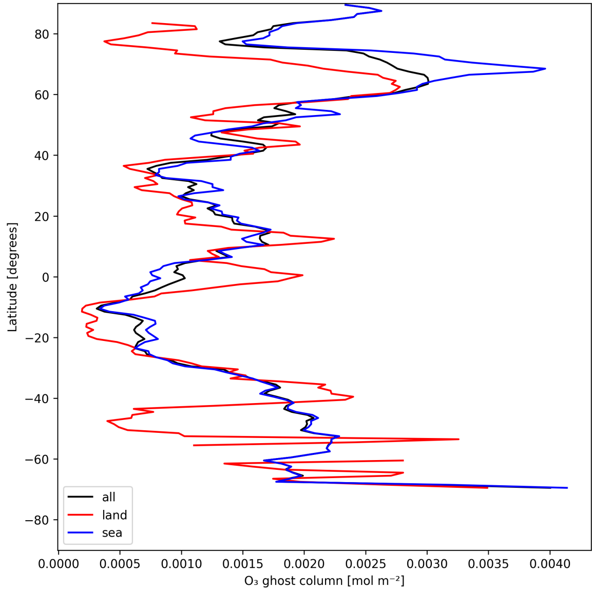
Figure 18: Zonal average of “O 3 ghost column” for 2025-07-25 to 2025-07-27.
