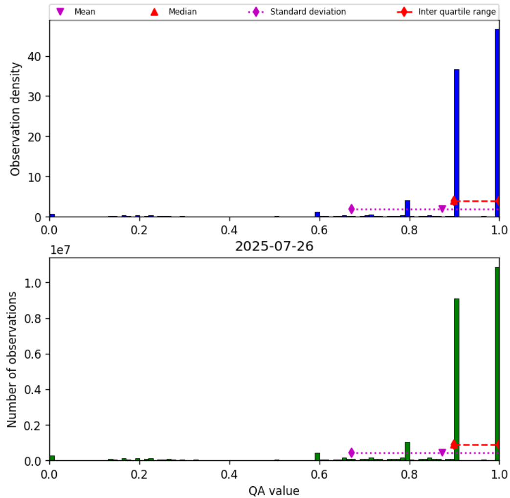
Figure 20: Histogram of “QA value” for 2025-07-25 to 2025-07-27
