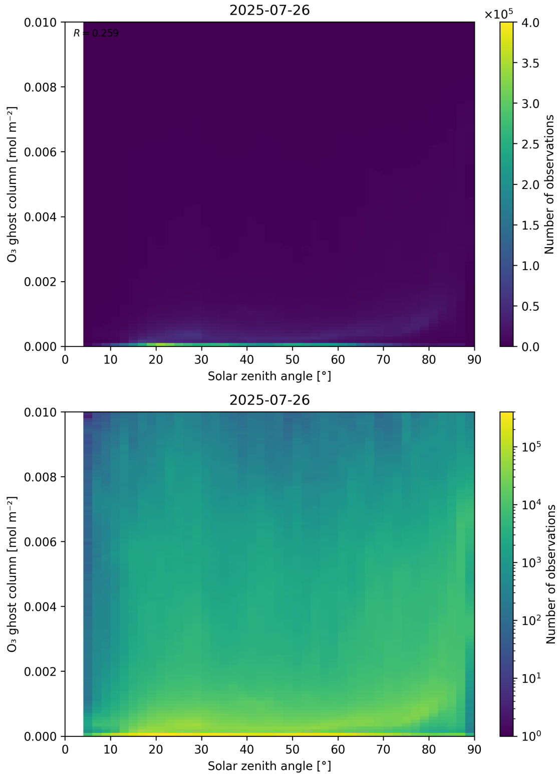
Figure 46: Scatter density plot of “Solar zenith angle” against “O 3 ghost column” for 2025-07-25 to 2025-07-27.
