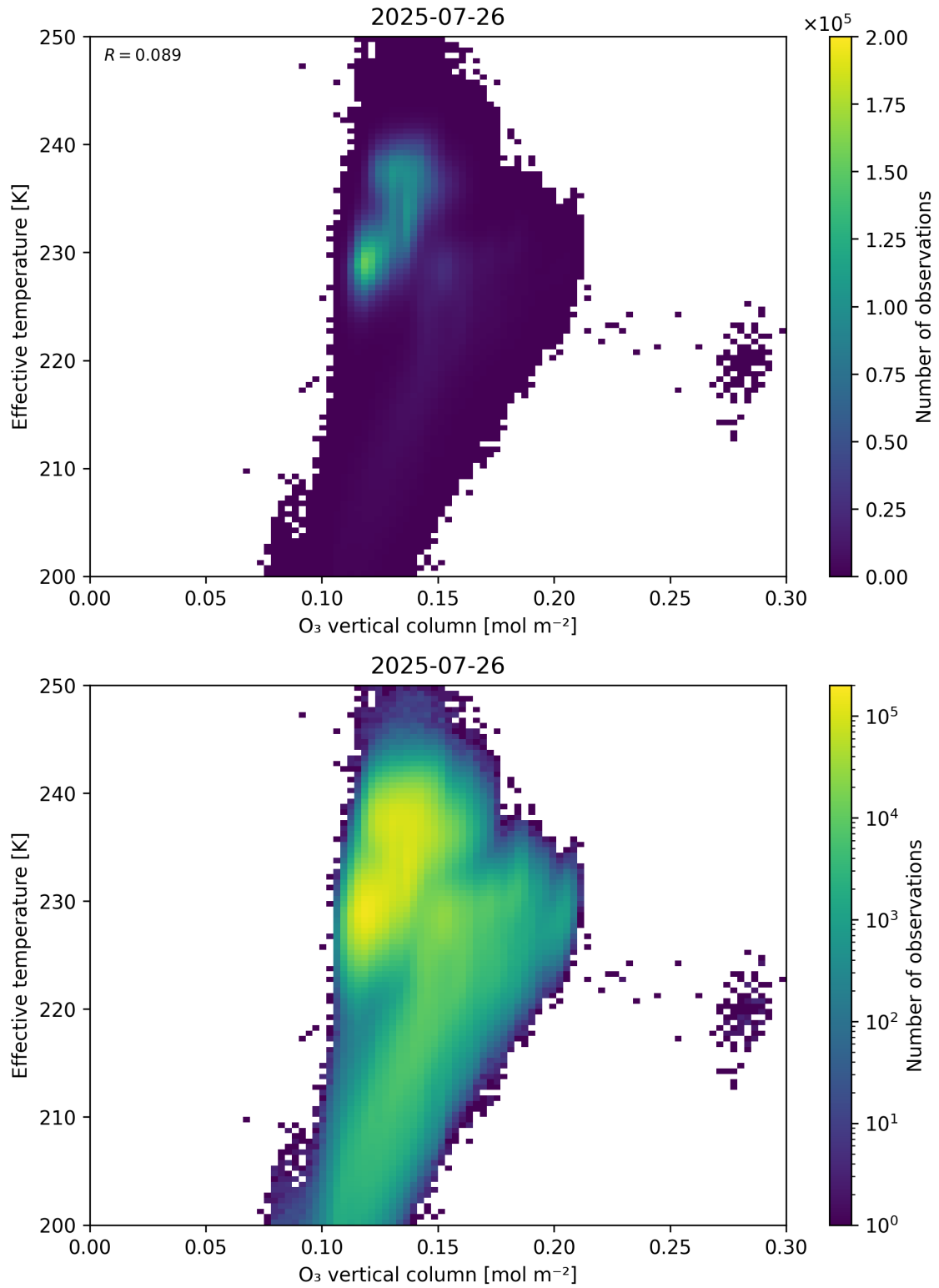
Figure 39: Scatter density plot of “O 3 vertical column” against “Effective temperature” for 2025-07-25 to 2025-07-27.
