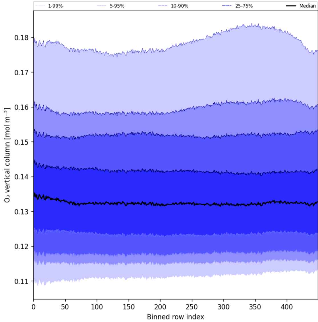
Figure 28: Along track statistics of “O 3 vertical column” for 2025-07-25 to 2025-07-27
