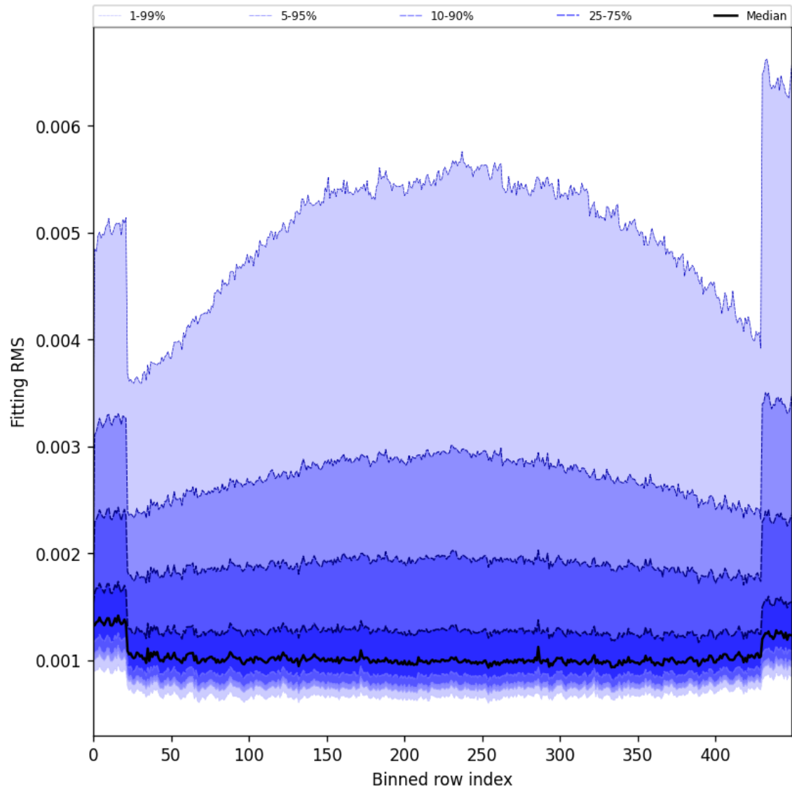
Figure 30: Along track statistics of “Fitting RMS” for 2025-07-25 to 2025-07-27
