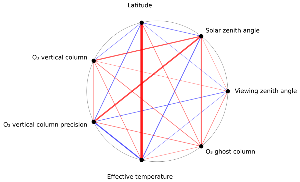
Figure 1: Map of correlation graph for 2025-07-25 to 2025-07-27.
