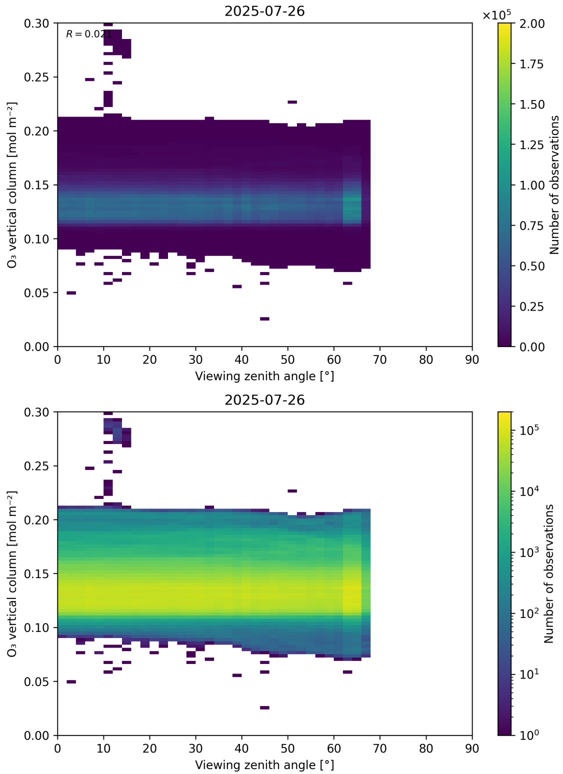
Figure 52: Scatter density plot of “Viewing zenith angle” against “O 3 vertical column” for 2025-07-25 to 2025-07-27.
