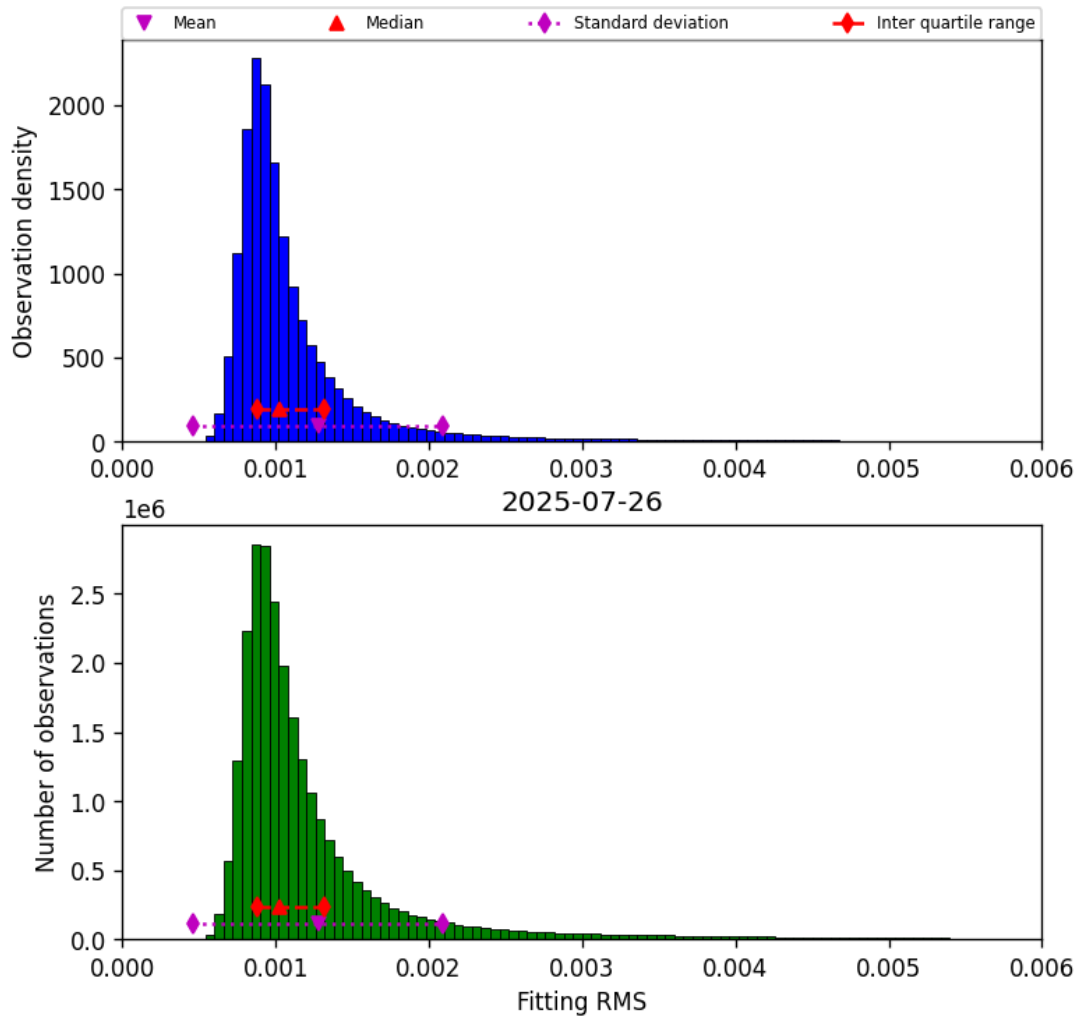
Figure 23: Histogram of “Fitting RMS” for 2025-07-25 to 2025-07-27
