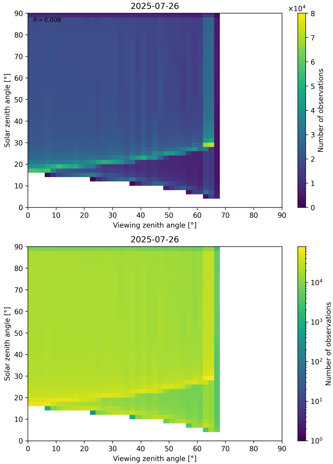
Figure 54: Scatter density plot of “Viewing zenith angle” against “Solar zenith angle” for 2025-07-25 to 2025-07-27.
