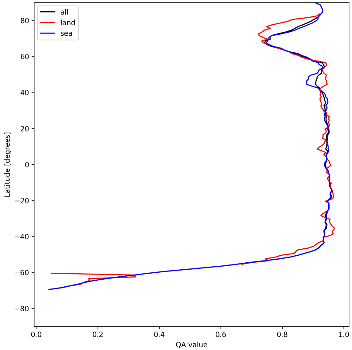
Figure 13: Zonal average of “QA value” for 2025-07-25 to 2025-07-27.
