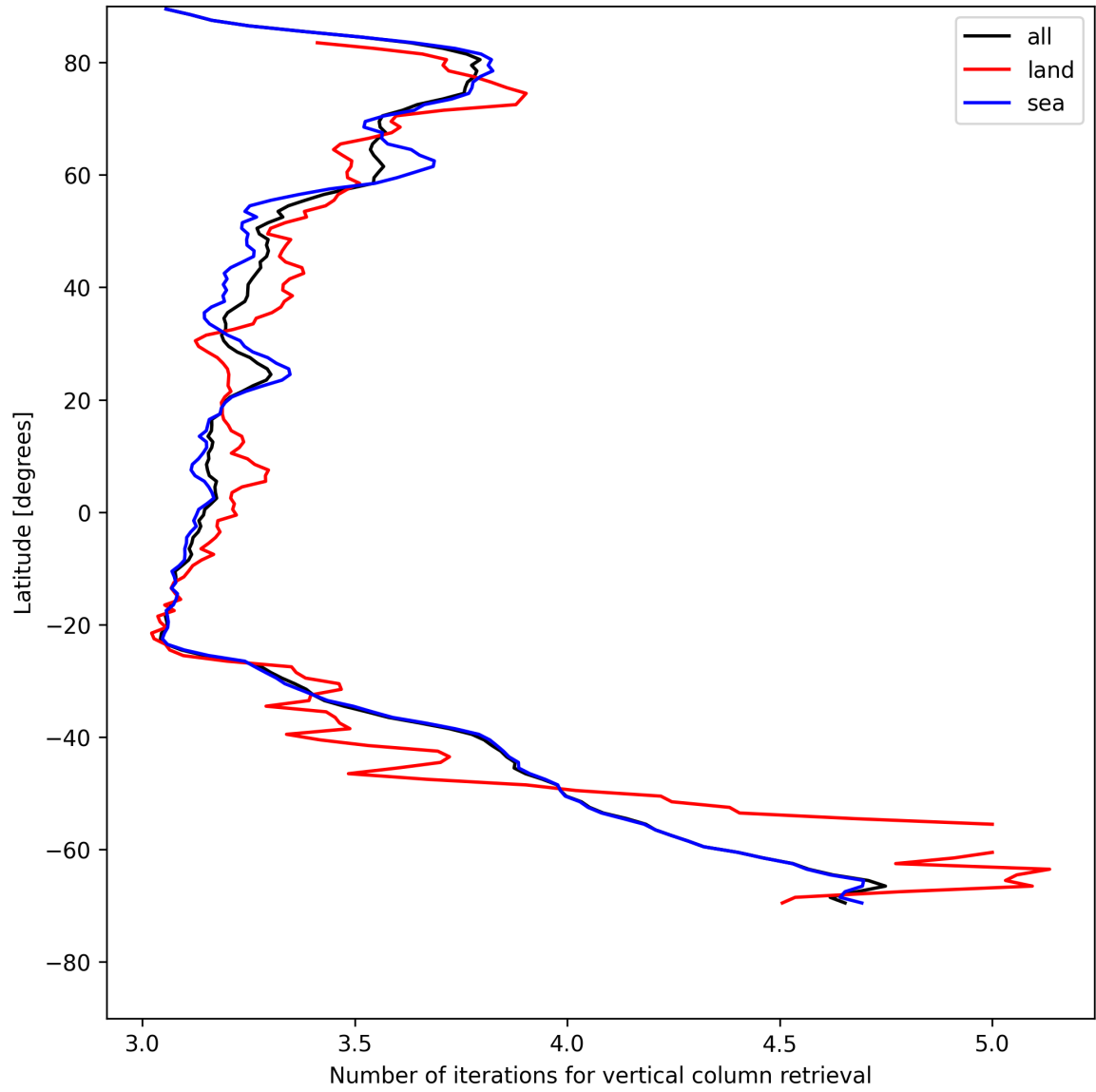
Figure 19: Zonal average of “Number of iterations for vertical column retrieval” for 2025-07-25 to 2025-07-27.
