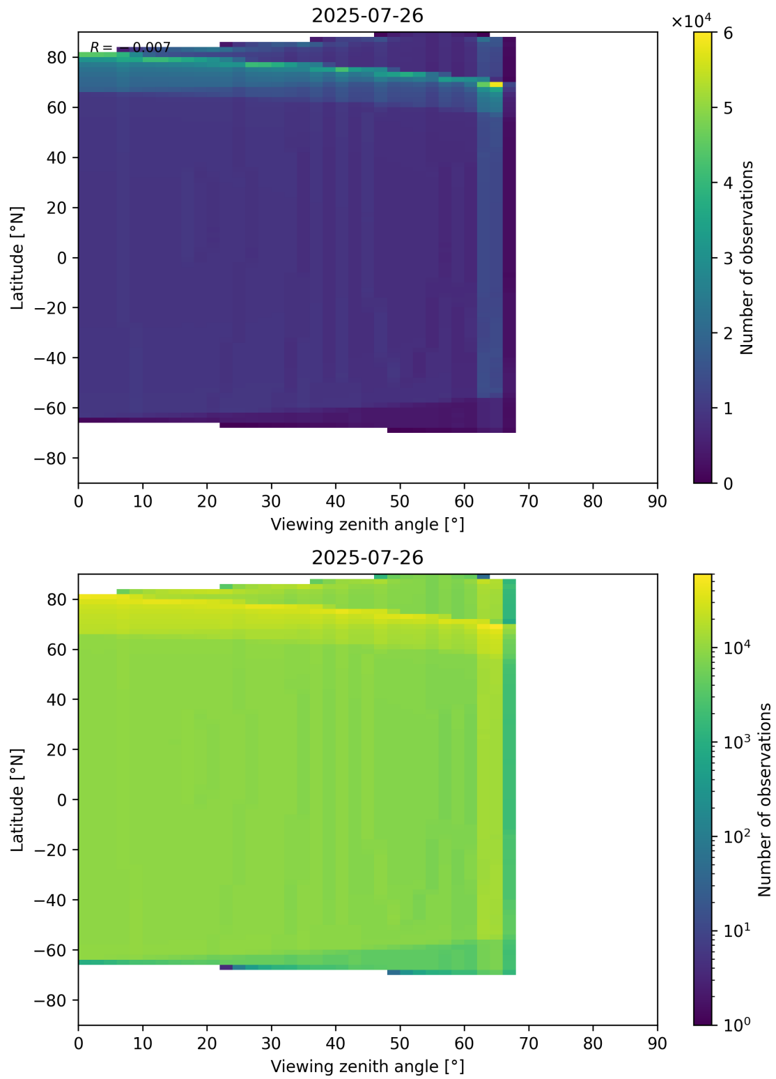
Figure 49: Scatter density plot of “Viewing zenith angle” against “Latitude” for 2025-07-25 to 2025-07-27.
