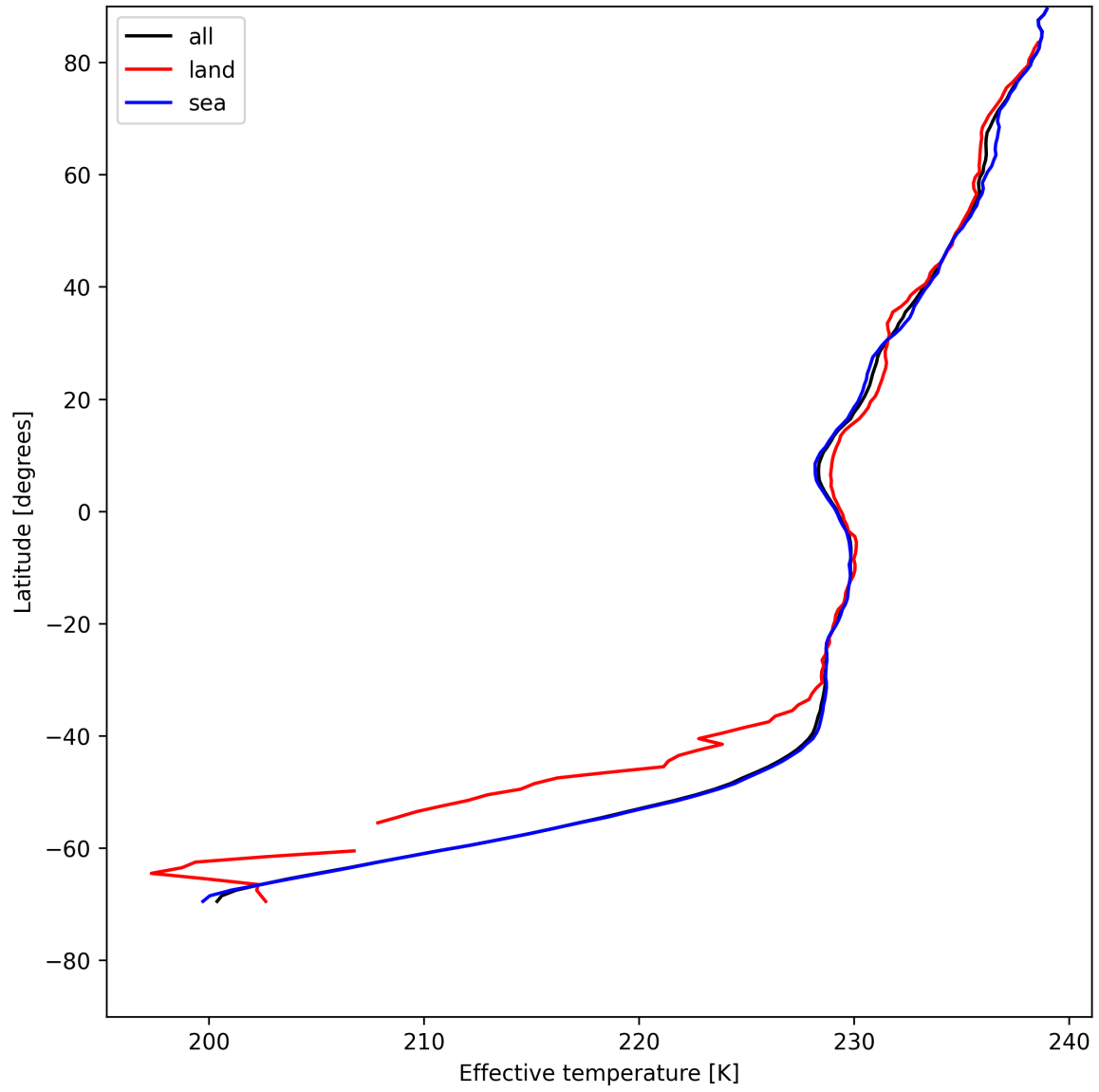
Figure 17: Zonal average of "Effective temperature" for 2025-07-25 to 2025-07-27.
