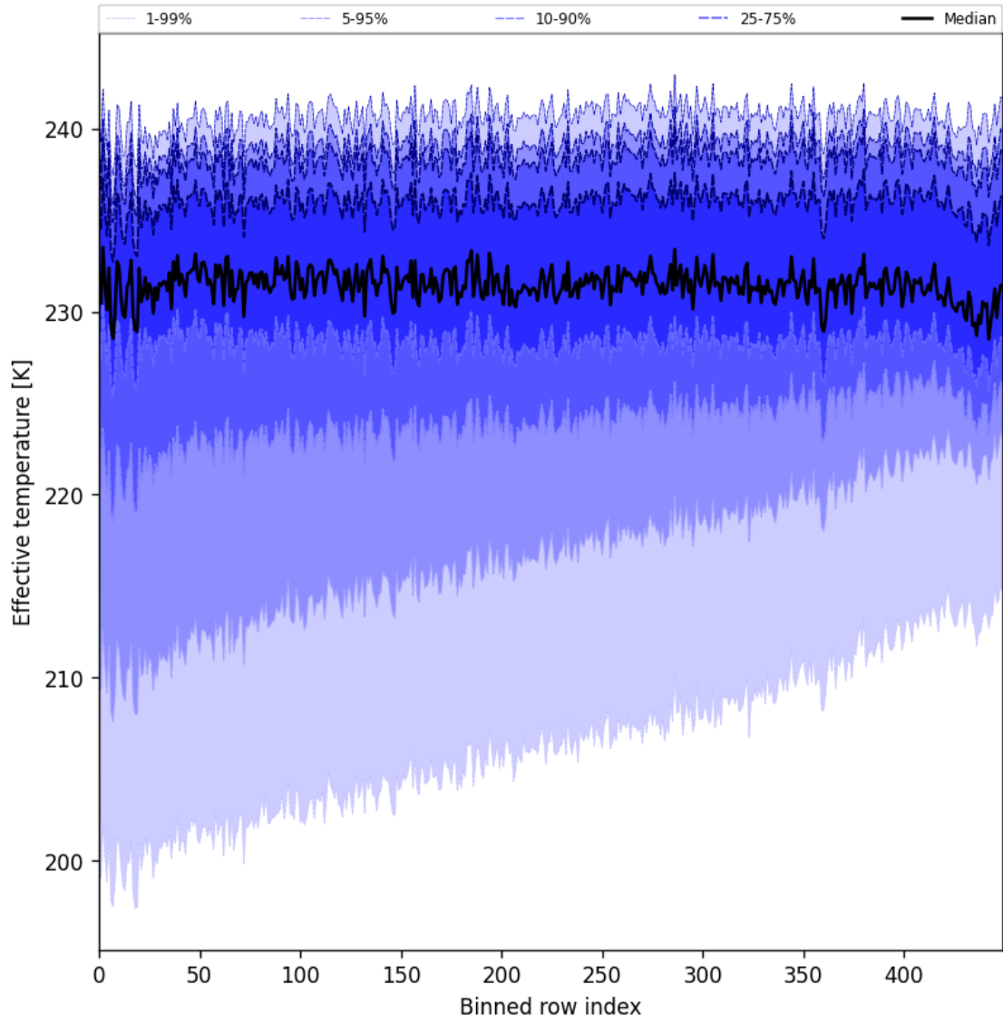
Figure 31: Along track statistics of “Effective temperature” for 2025-07-25 to 2025-07-27
