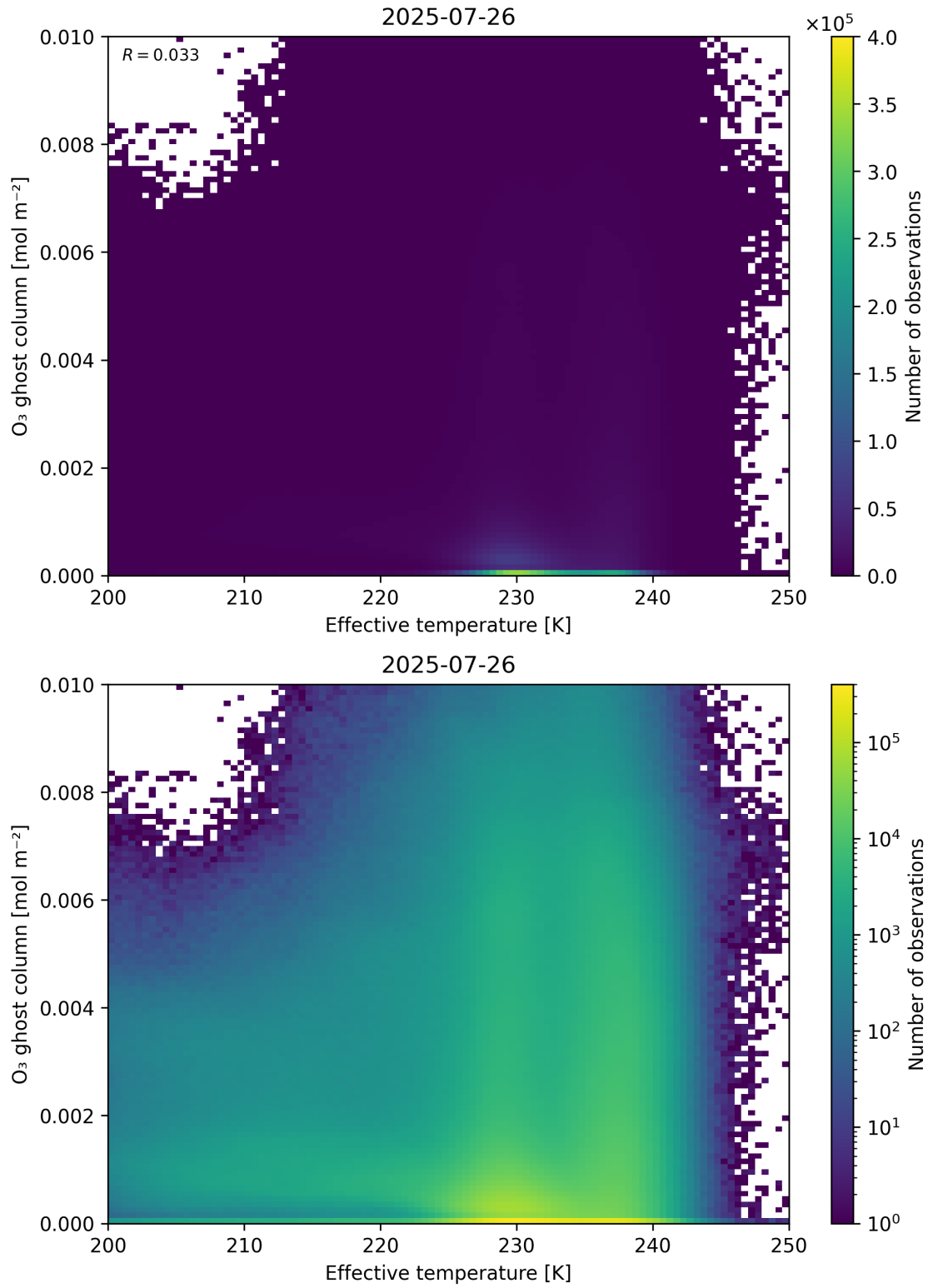
Figure 38: Scatter density plot of “Effective temperature” against “O 3 ghost column” for 2025-07-25 to 2025-07-27.
