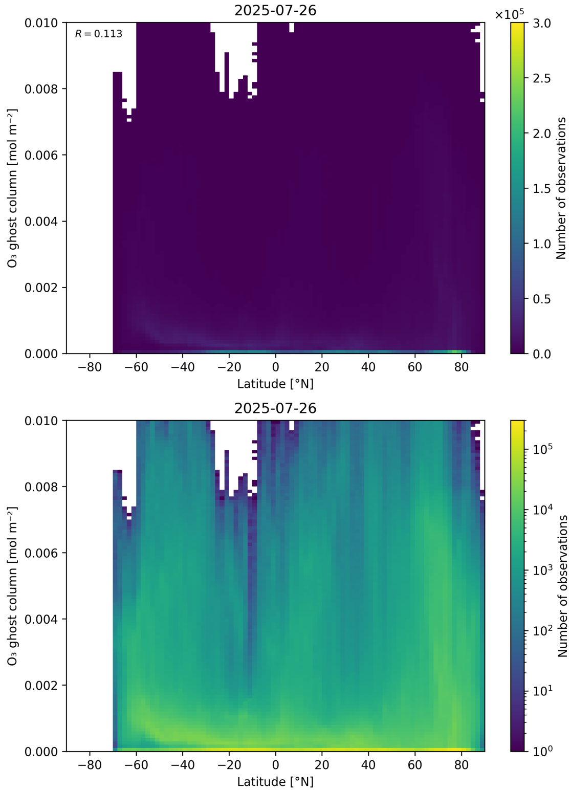
Figure 35: Scatter density plot of “Latitude” against “O 3 ghost column” for 2025-07-25 to 2025-07-27.
