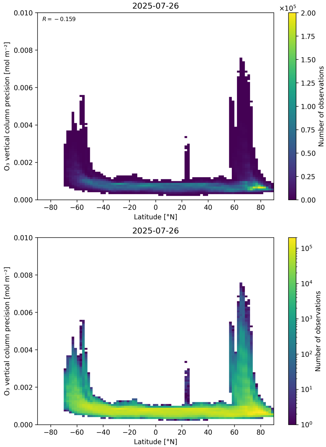
Figure 37: Scatter density plot of “Latitude” against “O 3 vertical column precision” for 2025-07-25 to 2025-07-27.
