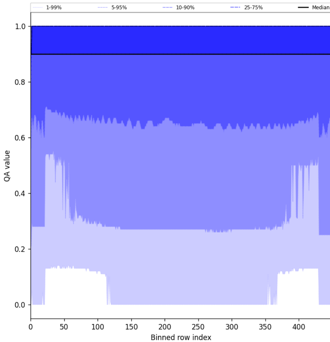
Figure 27: Along track statistics of “QA value” for 2025-07-25 to 2025-07-27
