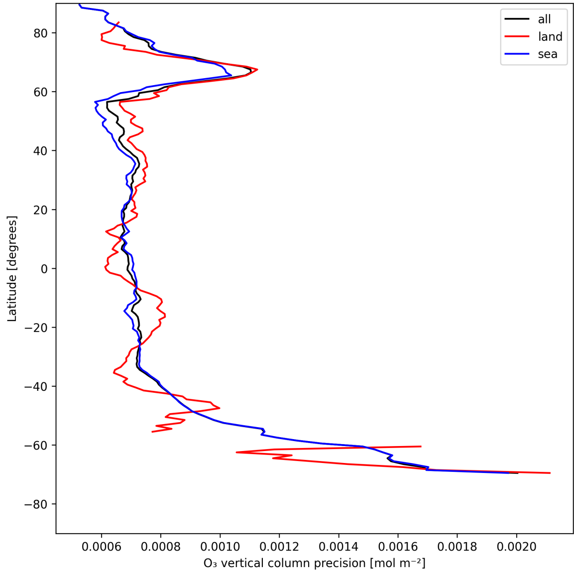
Figure 15: Zonal average of “O 3 vertical column precision” for 2025-07-25 to 2025-07-27.
