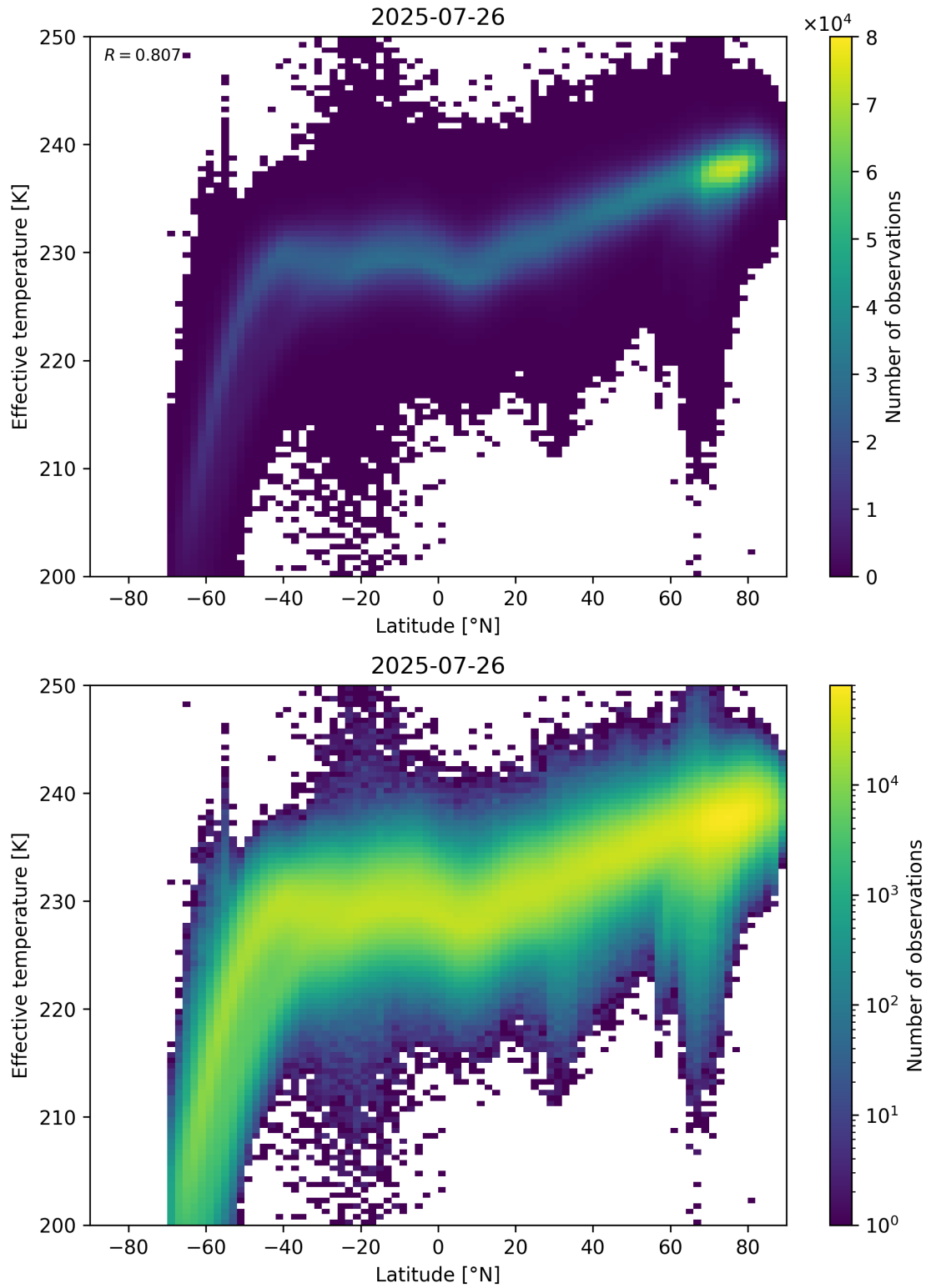
Figure 34: Scatter density plot of “Latitude” against “Effective temperature” for 2025-07-25 to 2025-07-27.
