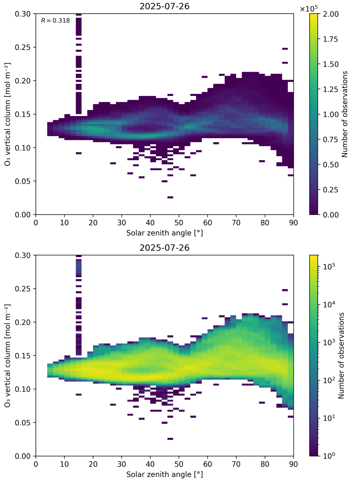
Figure 47: Scatter density plot of “Solar zenith angle” against “O 3 vertical column” for 2025-07-25 to 2025-07-27.
