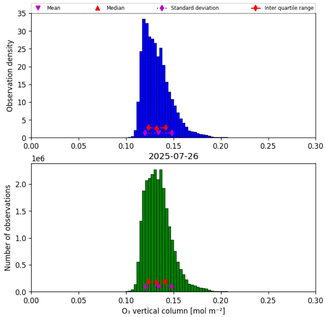
Figure 21: Histogram of “O 3 vertical column” for 2025-07-25 to 2025-07-27
