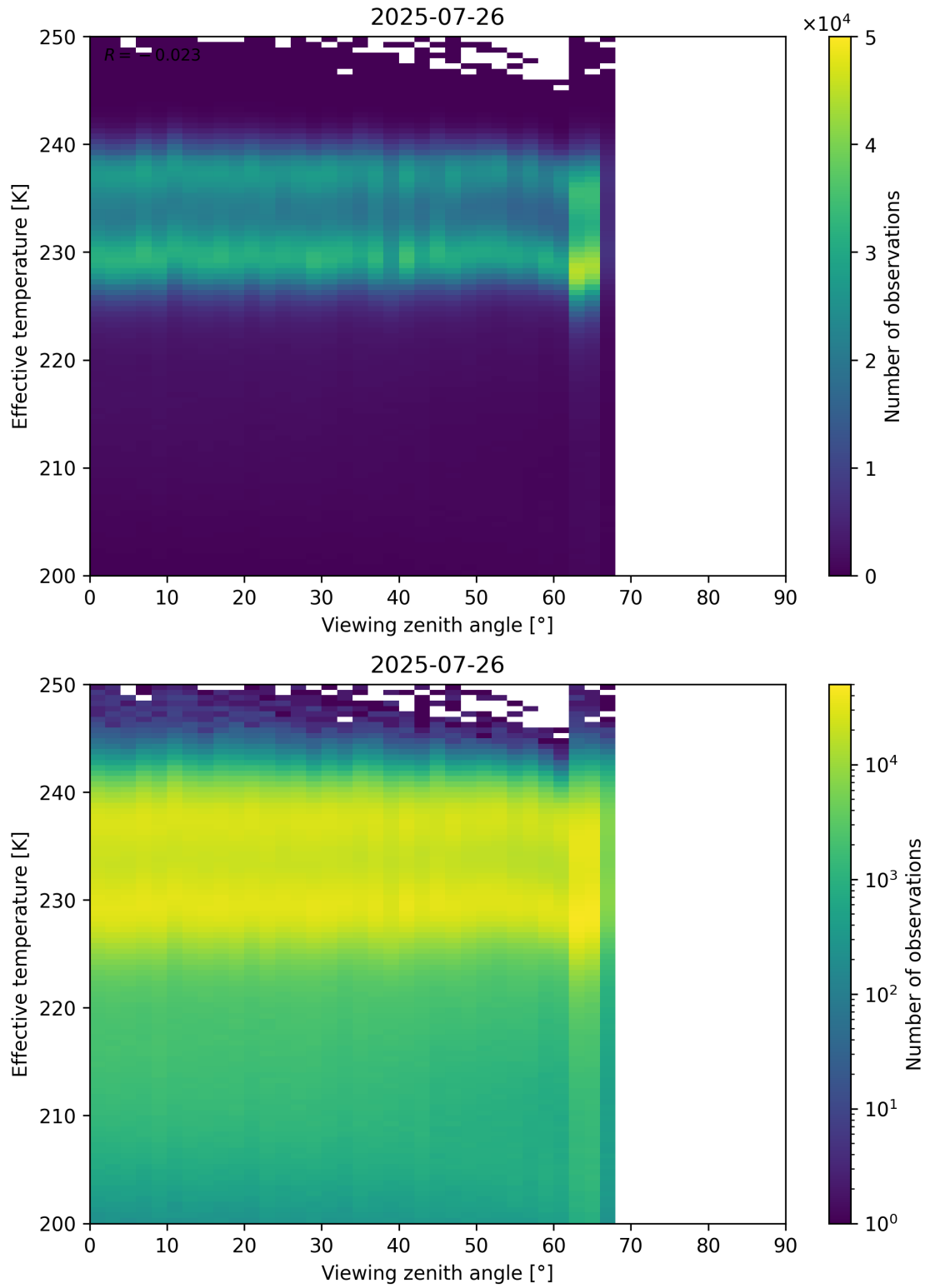
Figure 50: Scatter density plot of “Viewing zenith angle” against “Effective temperature” for 2025-07-25 to 2025-07-27.
