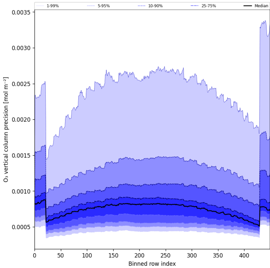
Figure 29: Along track statistics of “O 3 vertical column precision” for 2025-07-25 to 2025-07-27
