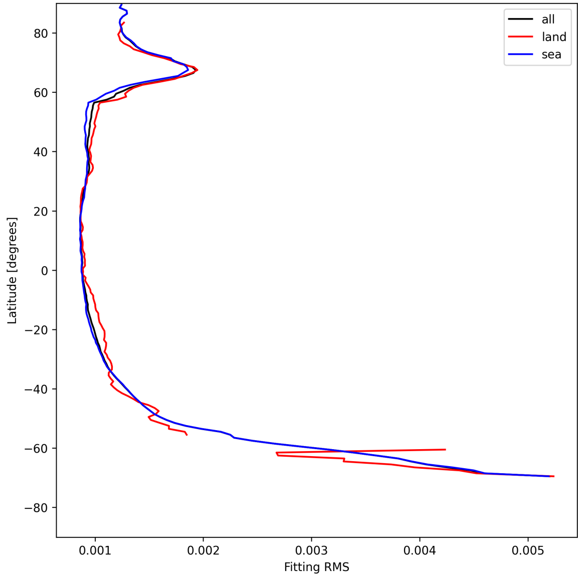
Figure 16: Zonal average of “Fitting RMS” for 2025-07-25 to 2025-07-27.
