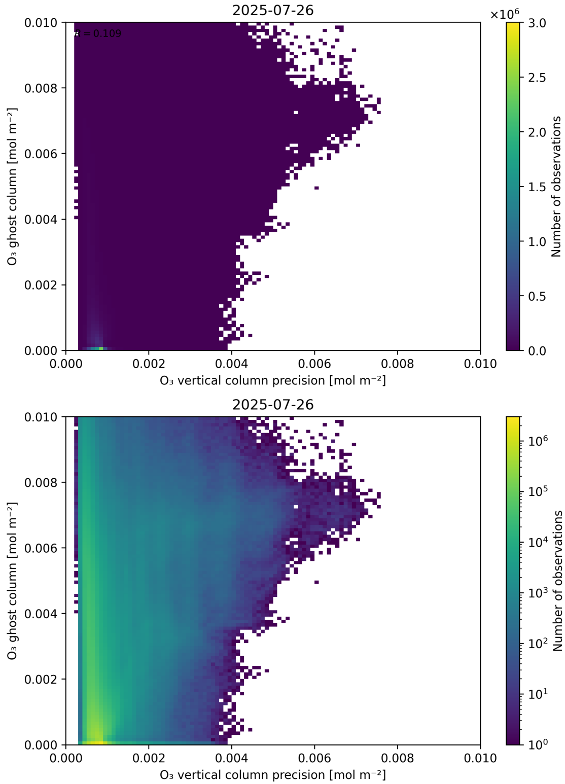
Figure 43: Scatter density plot of “O 3 vertical column precision” against “O 3 ghost column” for 2025-07-25 to 2025-07-27.
