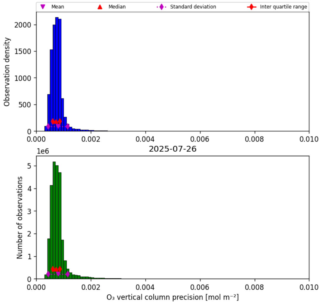
Figure 22: Histogram of "O 3 vertical column precision" for 2025-07-25 to 2025-07-27
