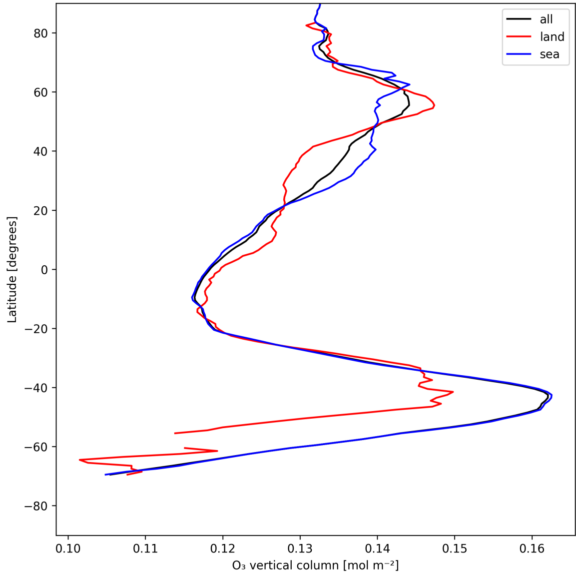
Figure 14: Zonal average of “O 3 vertical column” for 2025-07-25 to 2025-07-27.
