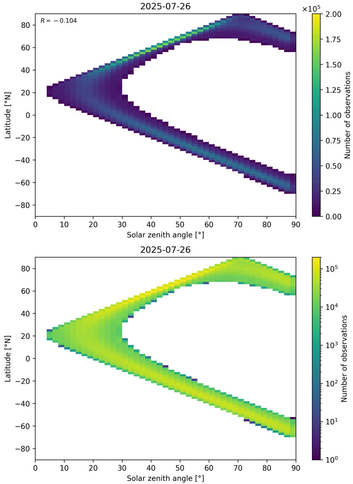
Figure 44: Scatter density plot of “Solar zenith angle” against “Latitude” for 2025-07-25 to 2025-07-27.
