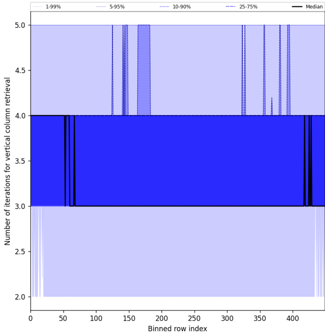
Figure 33: Along track statistics of “Number of iterations for vertical column retrieval” for 2025-07-25 to 2025-07-27
