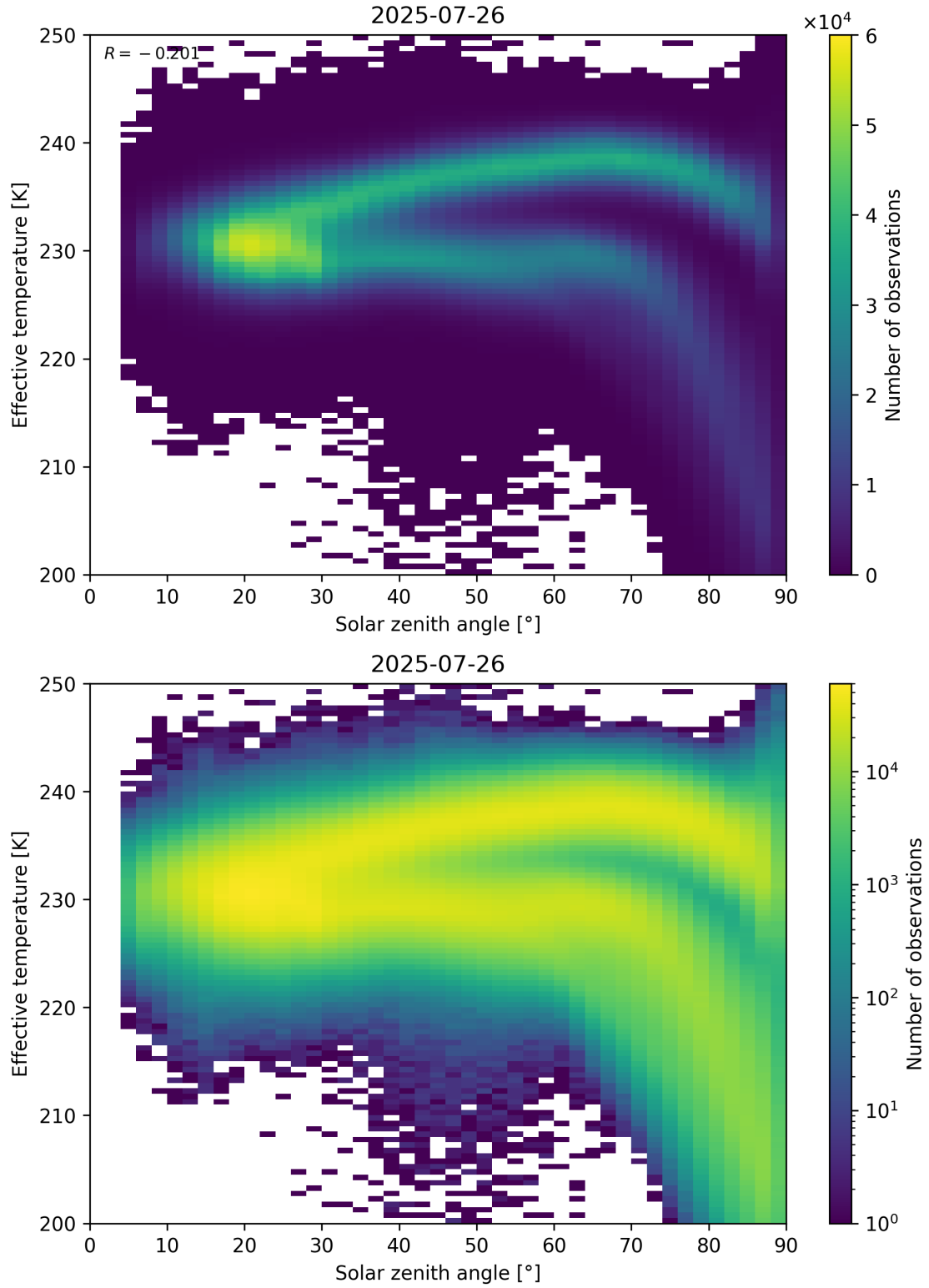
Figure 45: Scatter density plot of “Solar zenith angle” against “Effective temperature” for 2025-07-25 to 2025-07-27.
