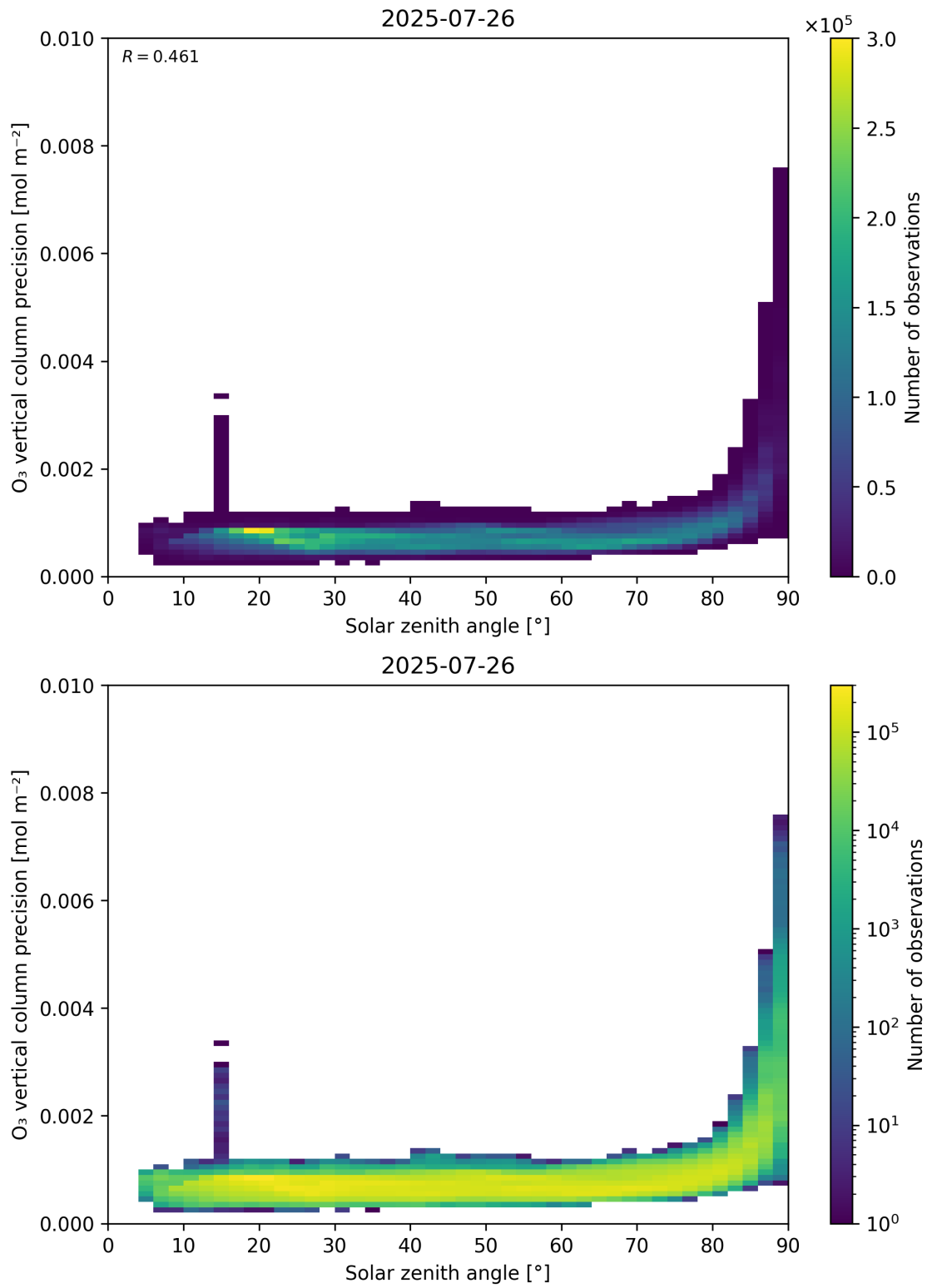
Figure 48: Scatter density plot of “Solar zenith angle” against “O 3 vertical column precision” for 2025-07-25 to 2025-07-27.
