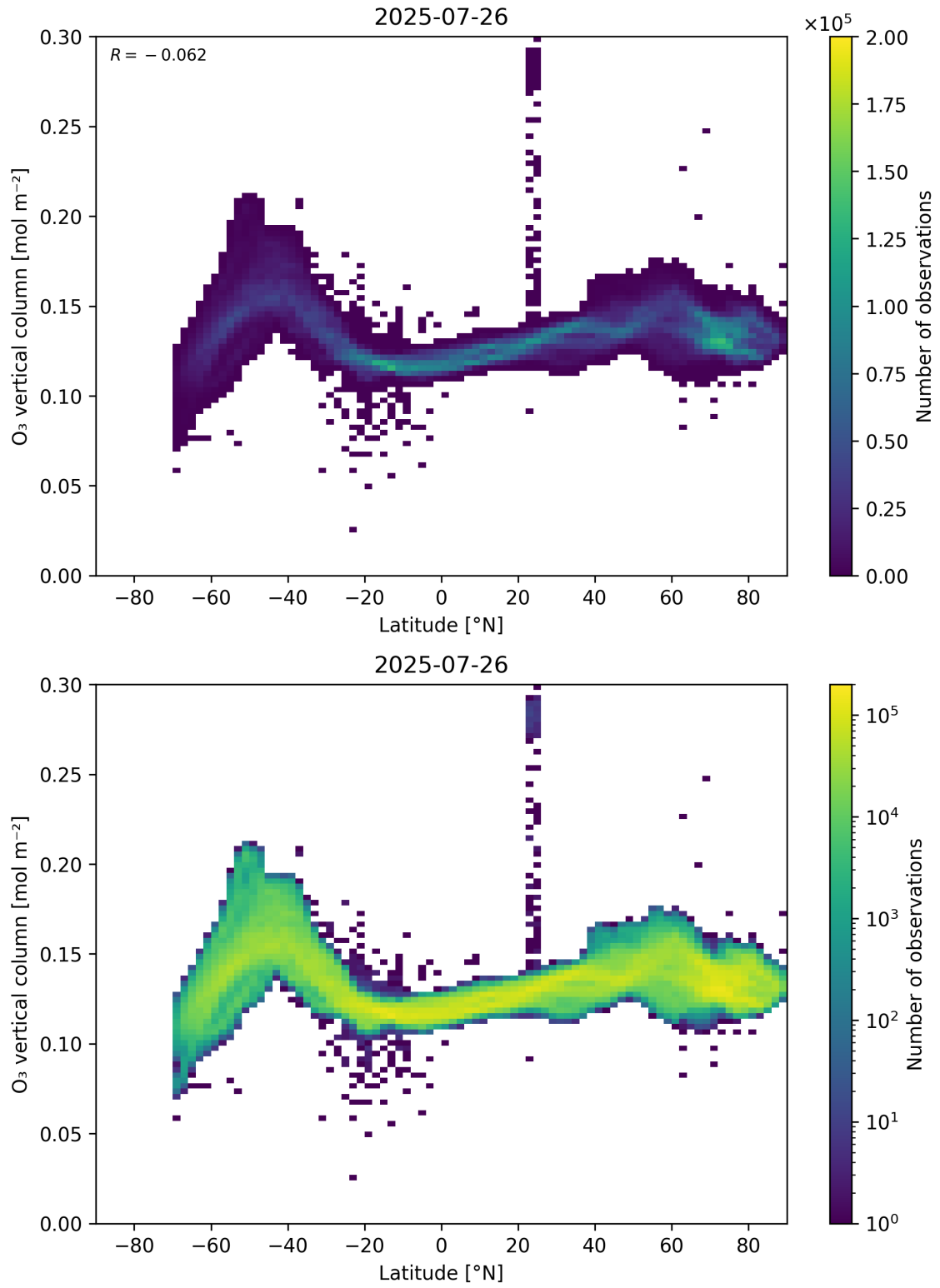
Figure 36: Scatter density plot of “Latitude” against “O 3 vertical column” for 2025-07-25 to 2025-07-27.
