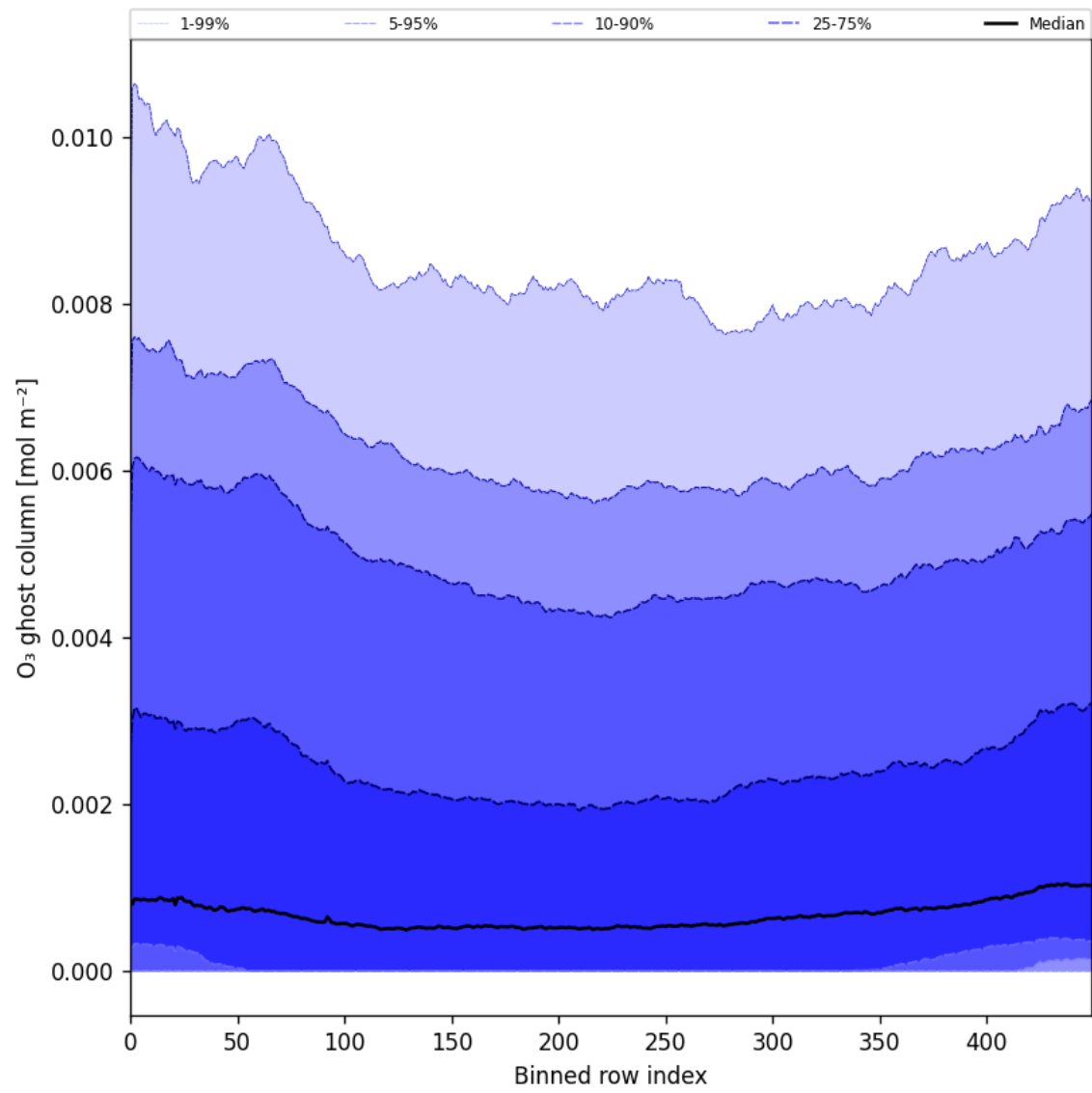
Figure 32: Along track statistics of “O 3 ghost column” for 2025-07-25 to 2025-07-27
