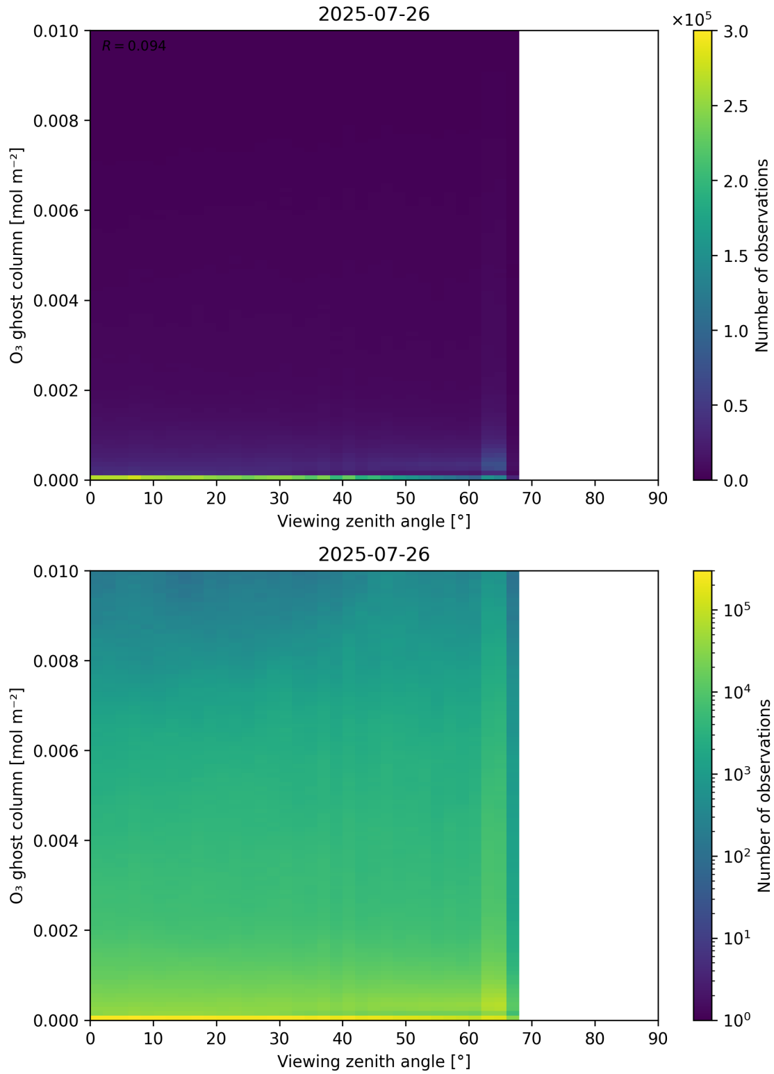
Figure 51: Scatter density plot of “Viewing zenith angle” against “O 3 ghost column” for 2025-07-25 to 2025-07-27.
