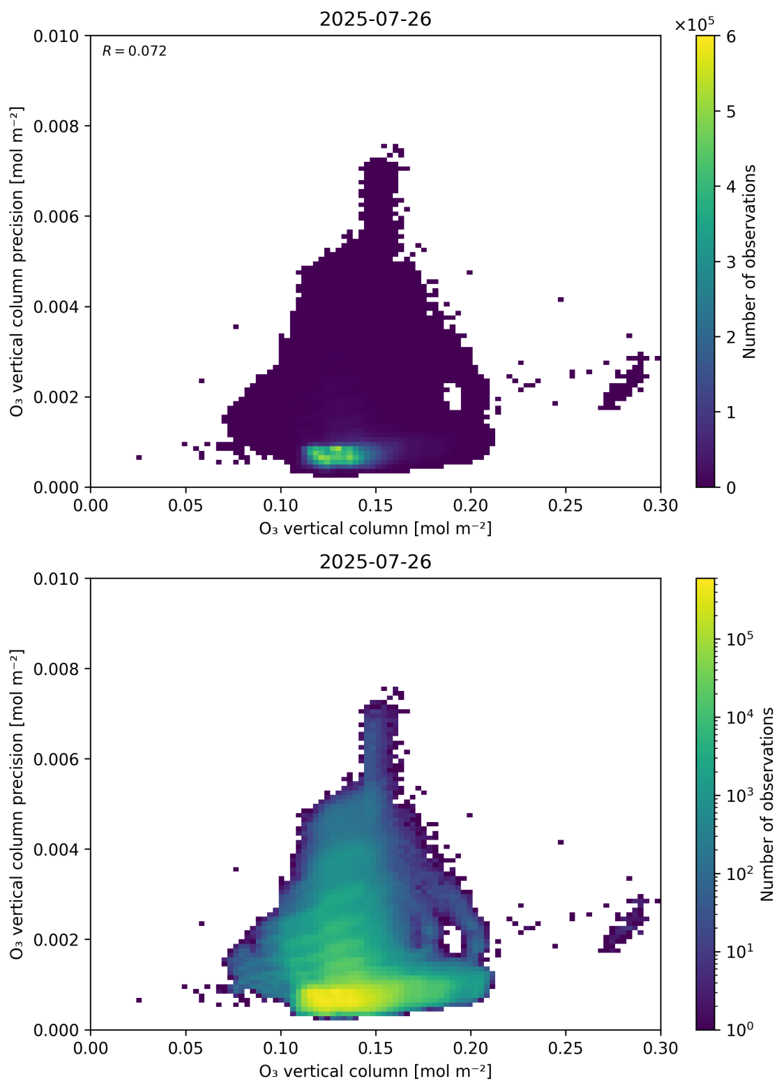
Figure 41: Scatter density plot of “O 3 vertical column” against “O 3 vertical column precision” for 2025-07-25 to 2025-07-27.
