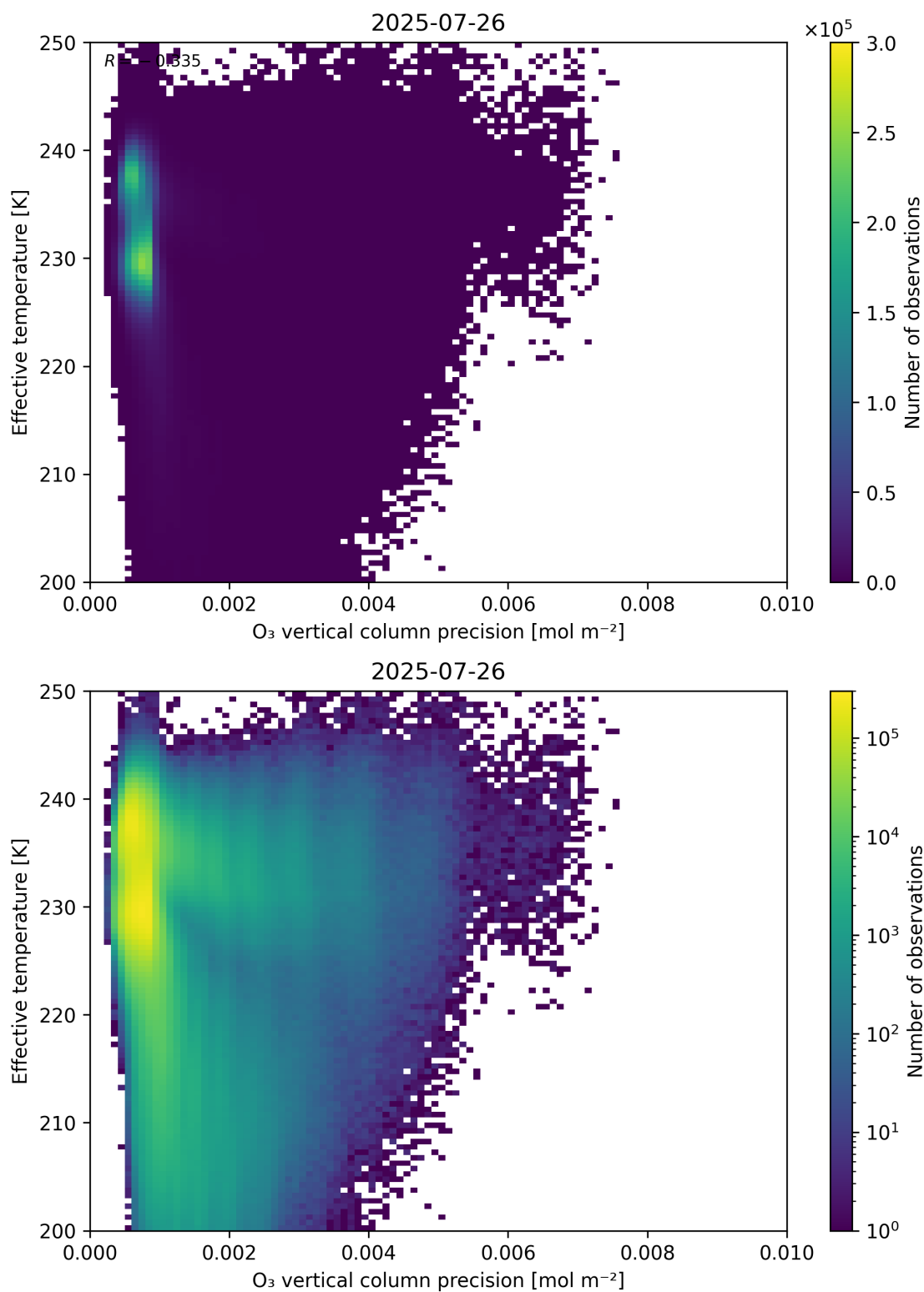
Figure 42: Scatter density plot of “O 3 vertical column precision” against “Effective temperature” for 2025-07-25 to 2025-07-27.
