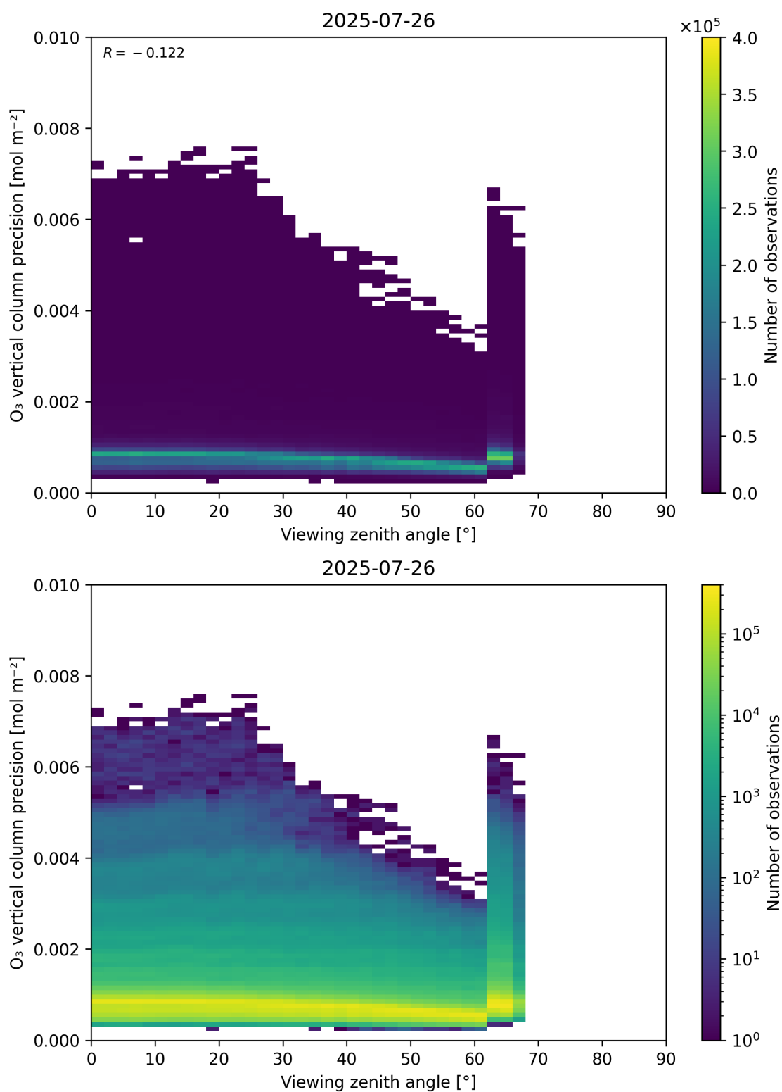
Figure 53: Scatter density plot of “Viewing zenith angle” against “O 3 vertical column precision” for 2025-07-25 to 2025-07-27.
