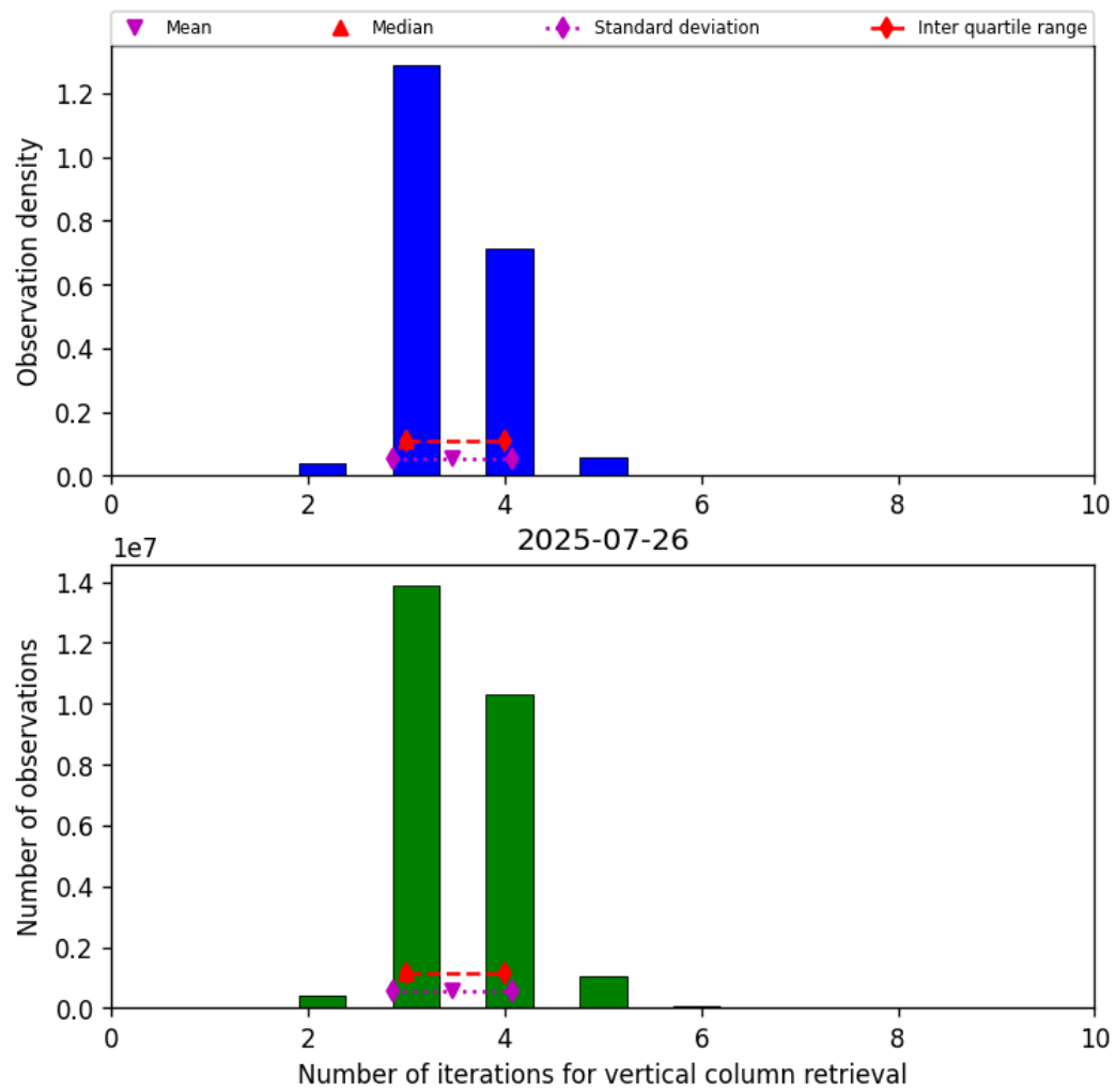
Figure 26: Histogram of “Number of iterations for vertical column retrieval” for 2025-07-25 to 2025-07-27
