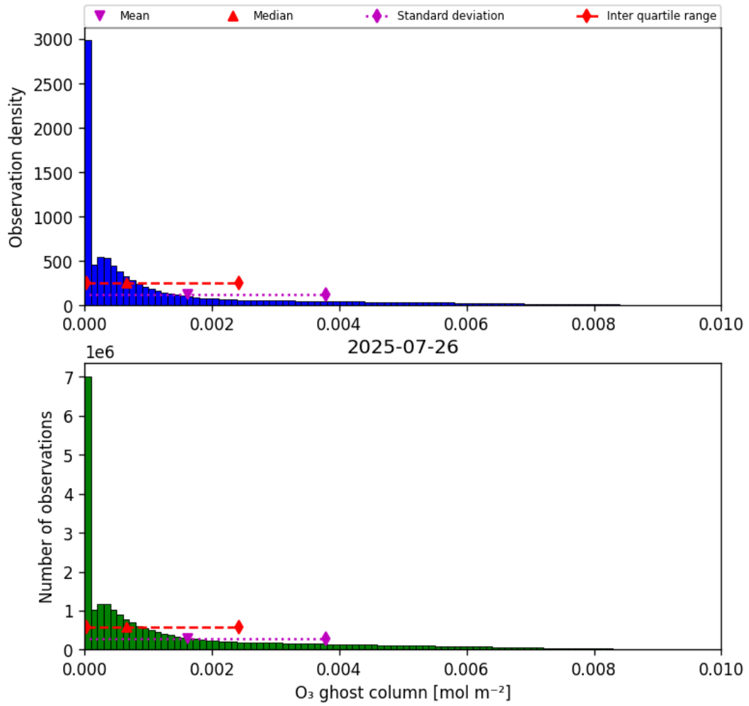
Figure 25: Histogram of “O 3 ghost column” for 2025-07-25 to 2025-07-27
