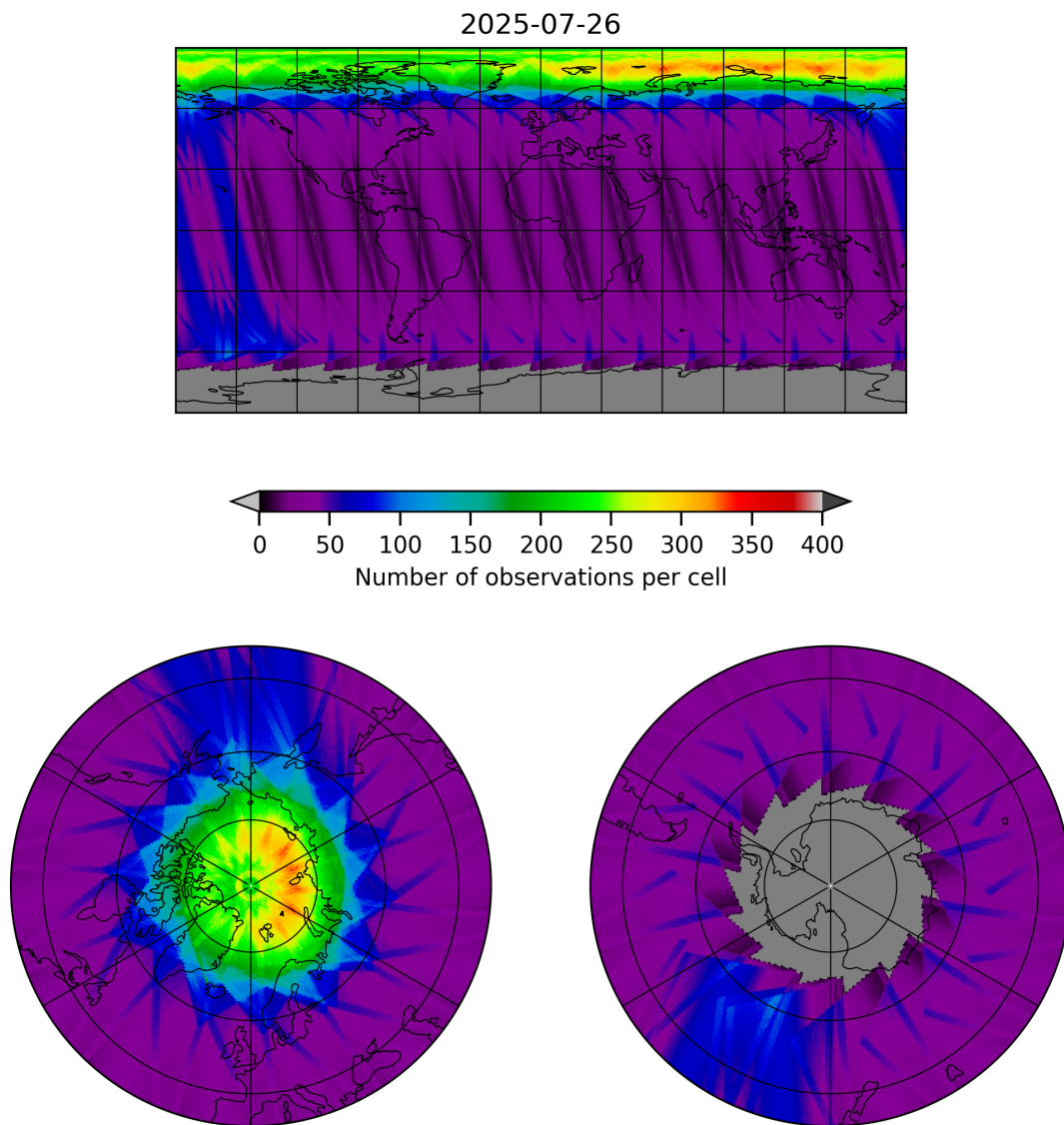
Figure 12: Map of the number of observations for 2025-07-25 to 2025-07-27
