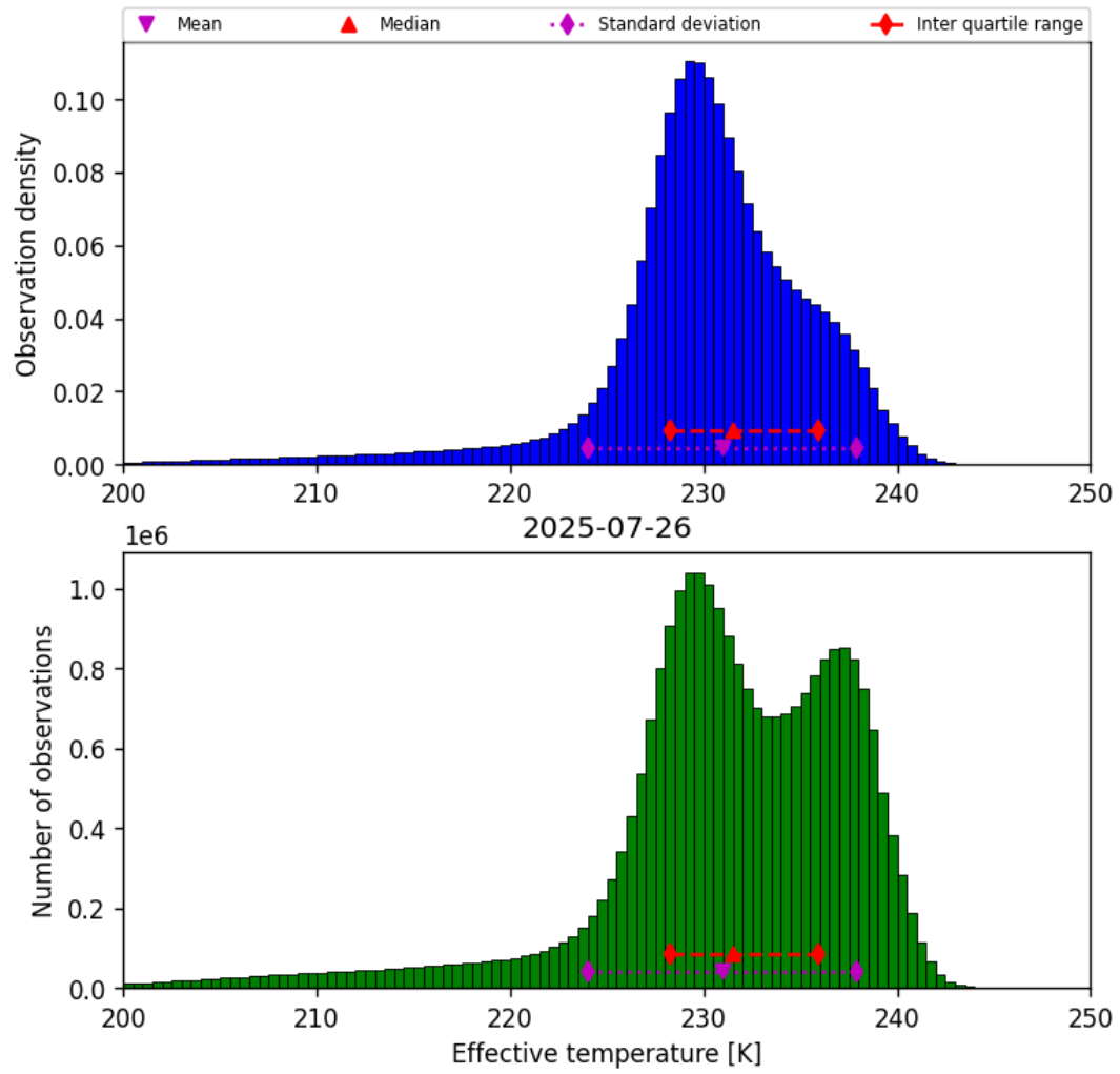
Figure 24: Histogram of “Effective temperature” for 2025-07-25 to 2025-07-27
