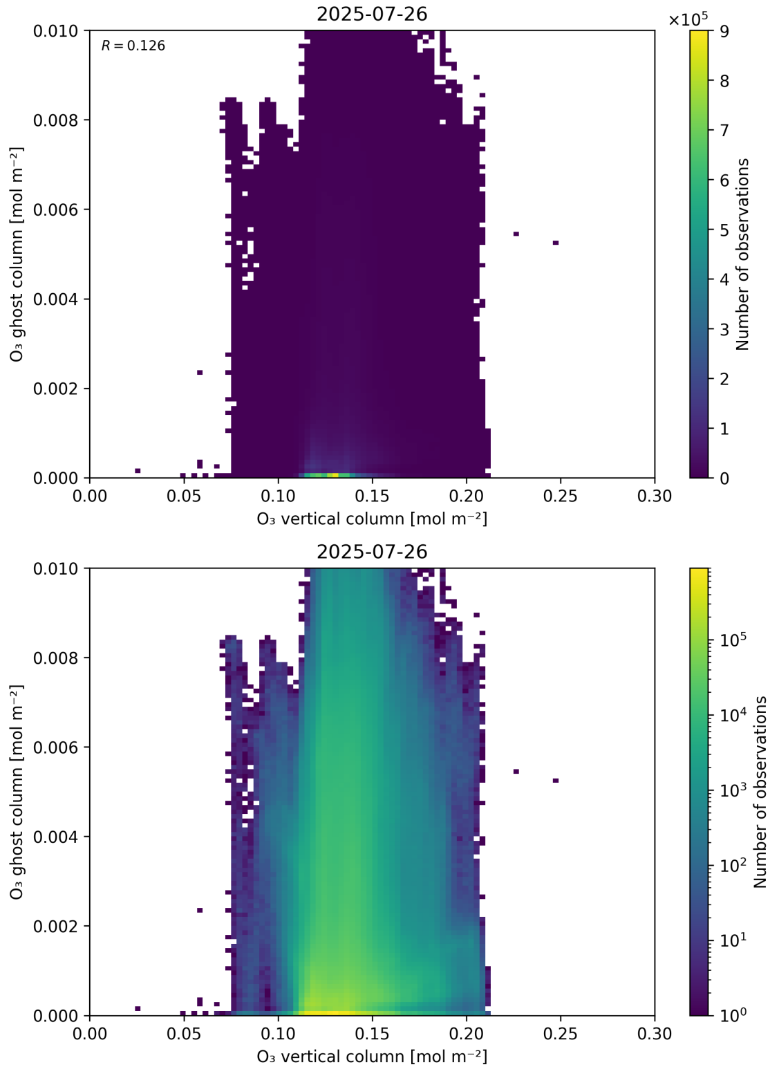
Figure 40: Scatter density plot of “O 3 vertical column” against “O 3 ghost column” for 2025-07-25 to 2025-07-27.
