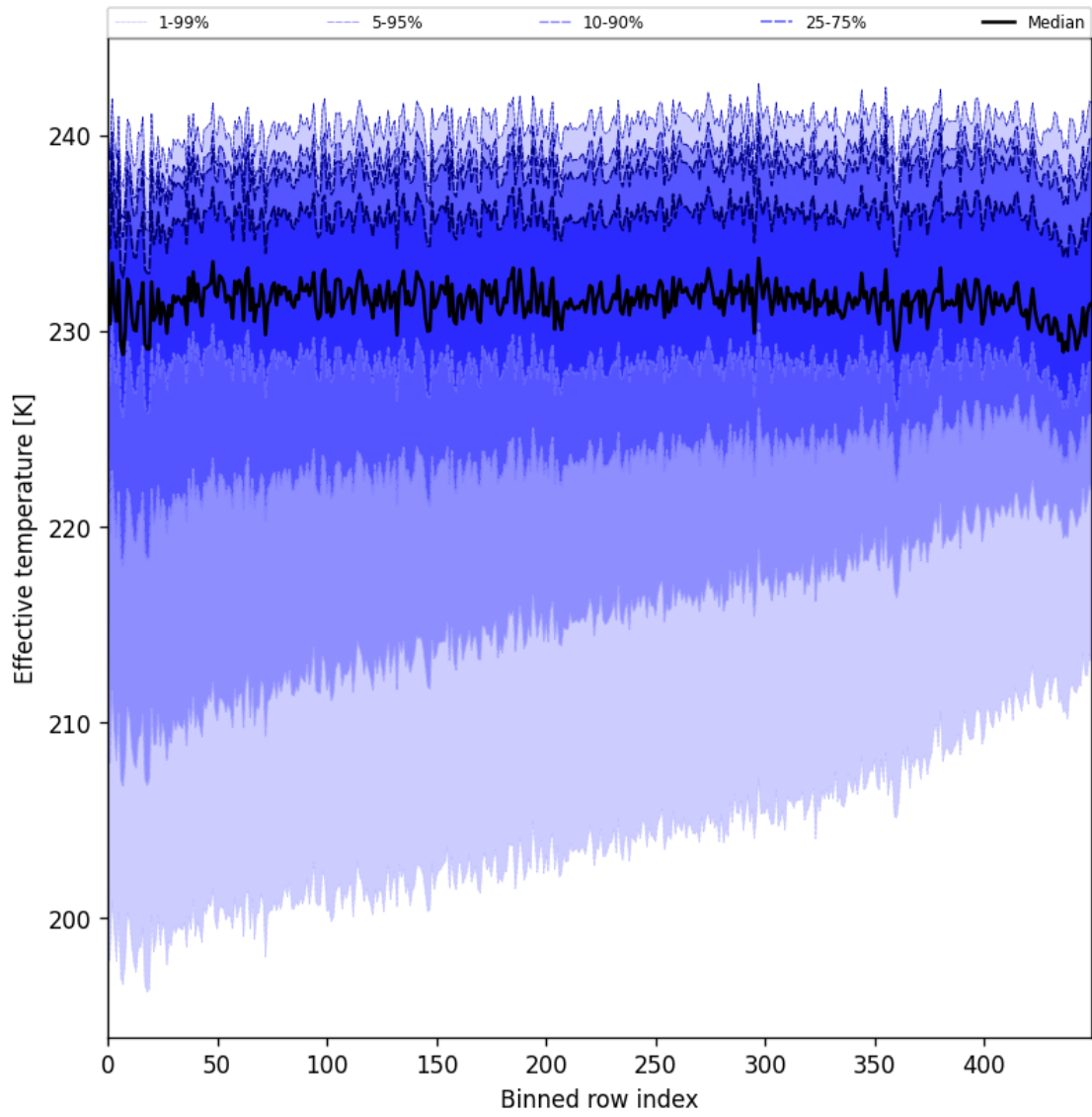
Figure 31: Along track statistics of “Effective temperature” for 2025-07-29 to 2025-07-31
