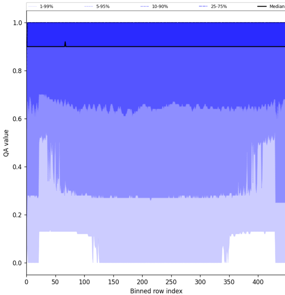
Figure 27: Along track statistics of “QA value” for 2025-07-29 to 2025-07-31
