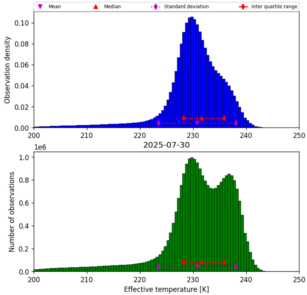
Figure 24: Histogram of “Effective temperature” for 2025-07-29 to 2025-07-31
