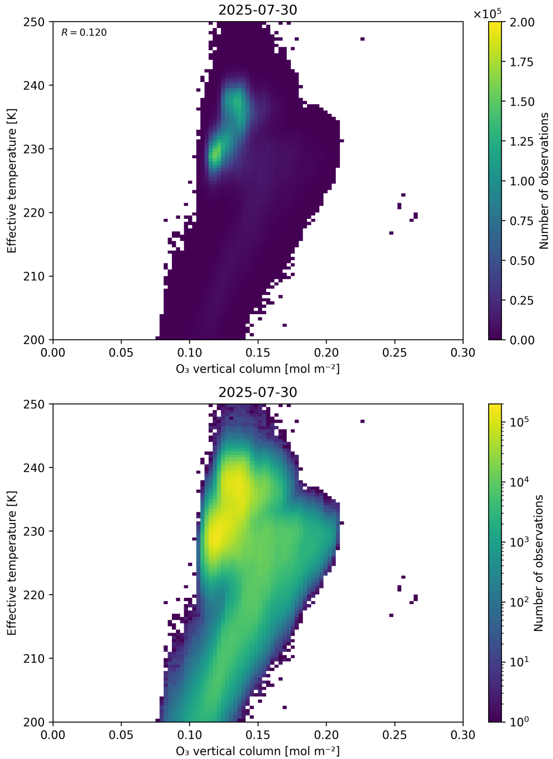
Figure 39: Scatter density plot of “O 3 vertical column” against “Effective temperature” for 2025-07-29 to 2025-07-31.
