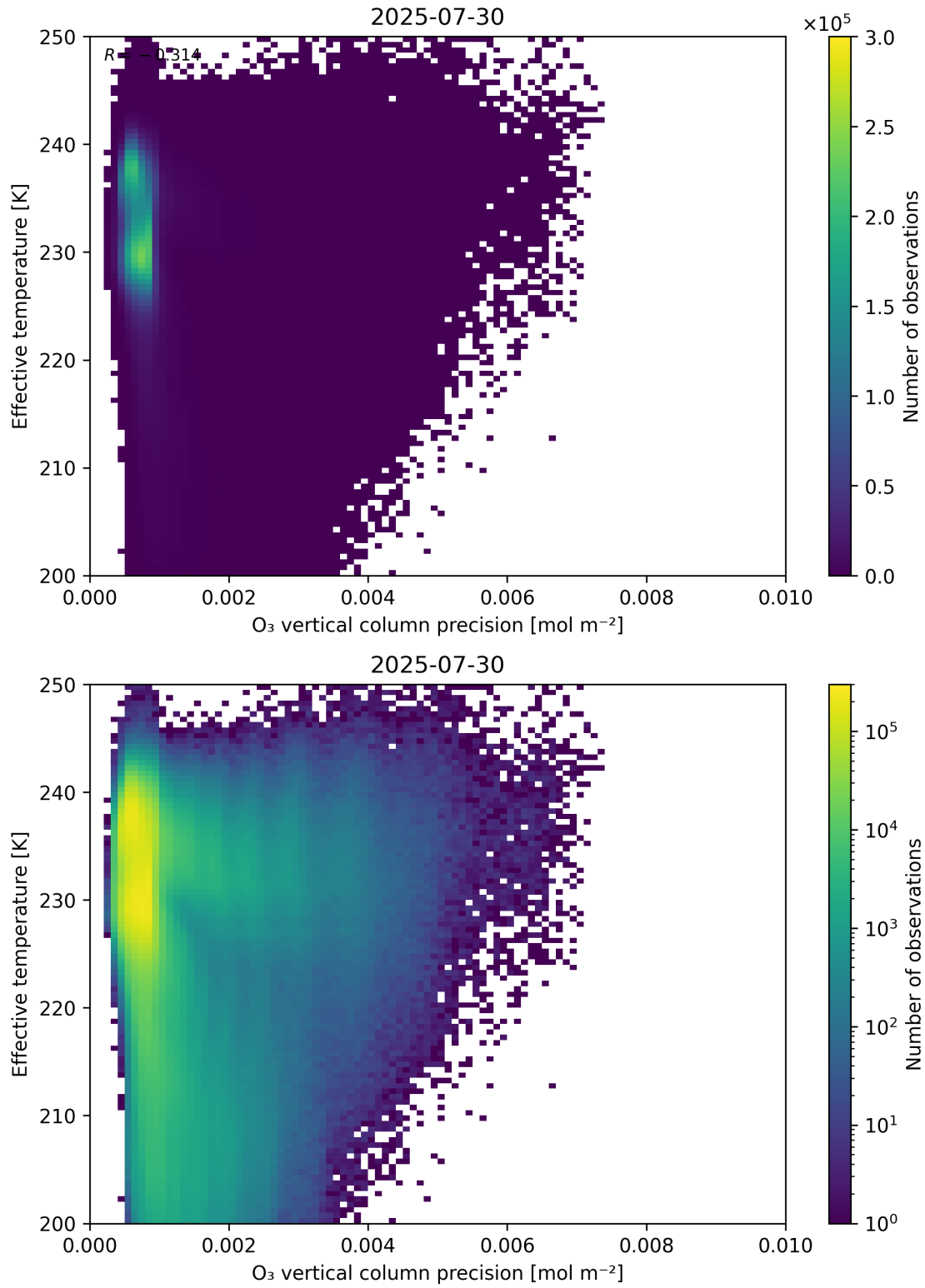
Figure 42: Scatter density plot of “O 3 vertical column precision” against “Effective temperature” for 2025-07-29 to 2025-07-31.
