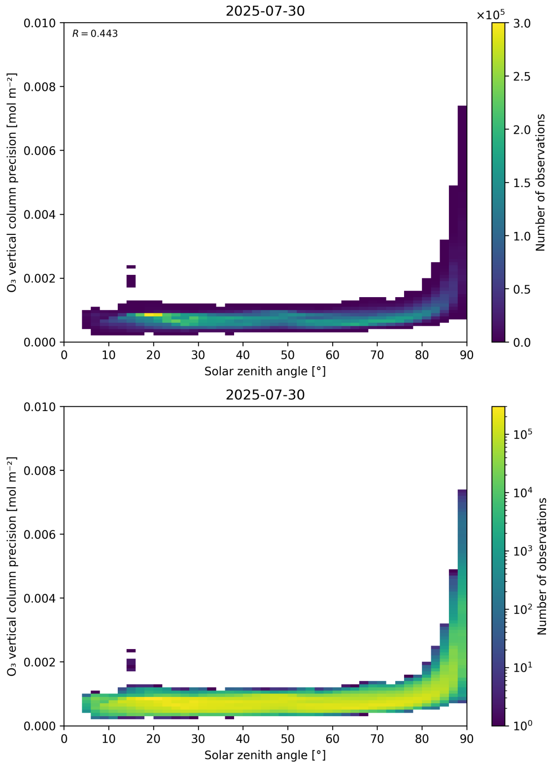
Figure 48: Scatter density plot of “Solar zenith angle” against “O 3 vertical column precision” for 2025-07-29 to 2025-07-31.
