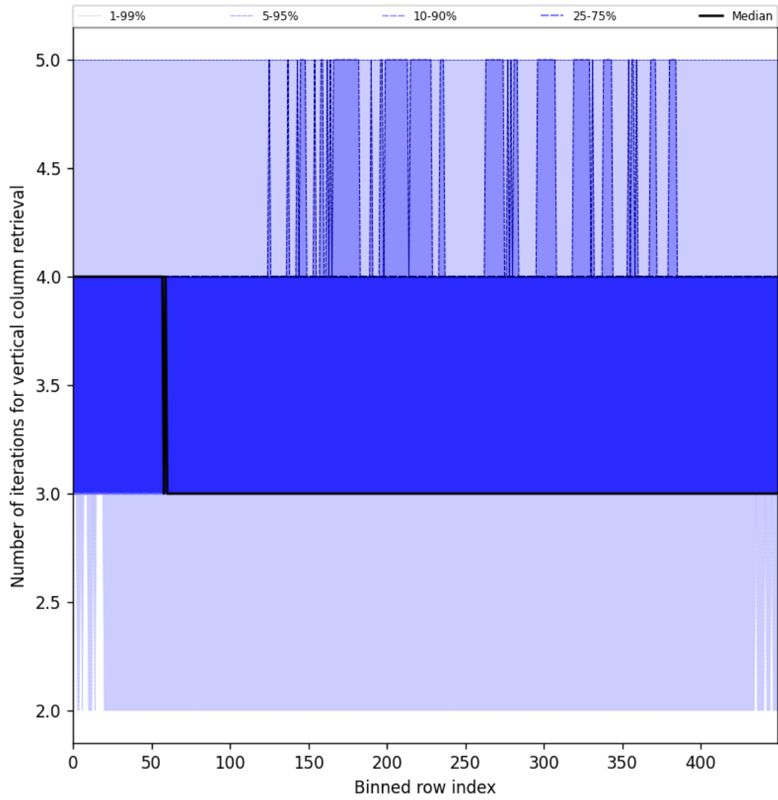
Figure 33: Along track statistics of “Number of iterations for vertical column retrieval” for 2025-07-29 to 2025-07-31
