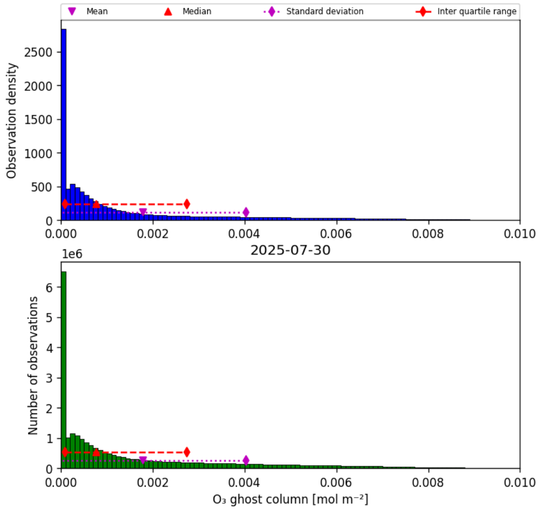
Figure 25: Histogram of “O 3 ghost column” for 2025-07-29 to 2025-07-31
