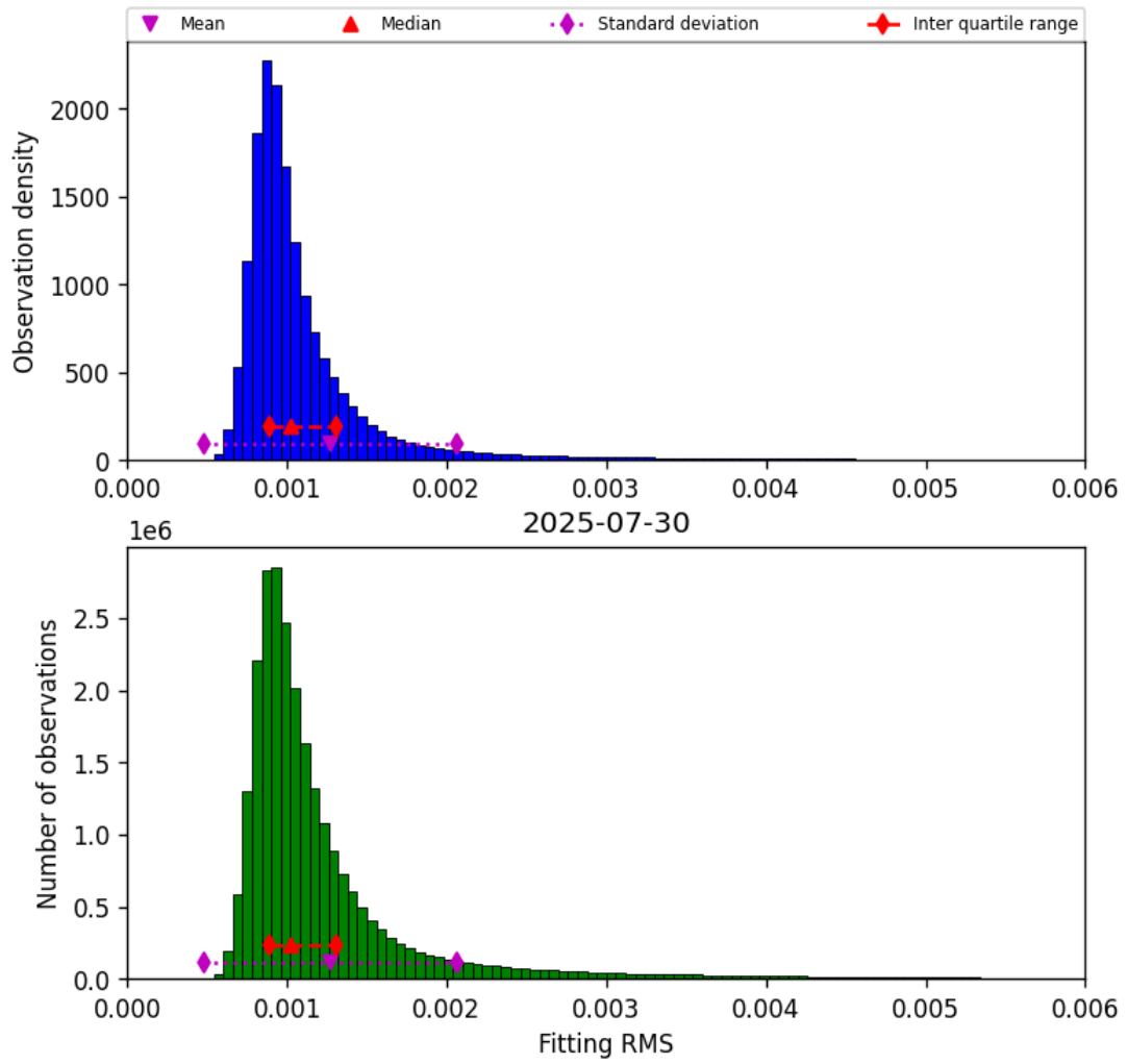
Figure 23: Histogram of “Fitting RMS” for 2025-07-29 to 2025-07-31
