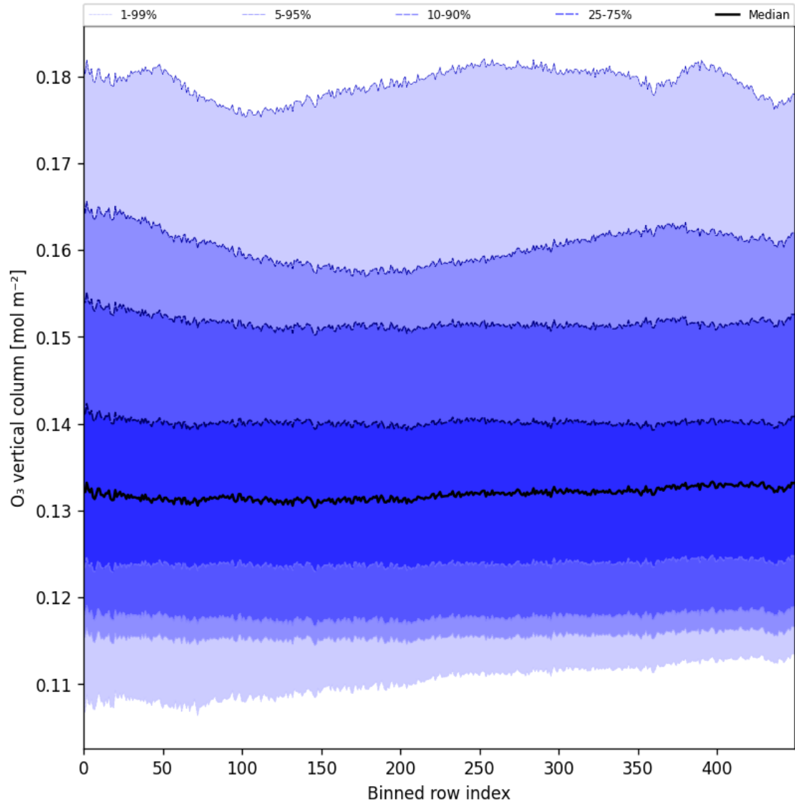
Figure 28: Along track statistics of “O 3 vertical column” for 2025-07-29 to 2025-07-31
