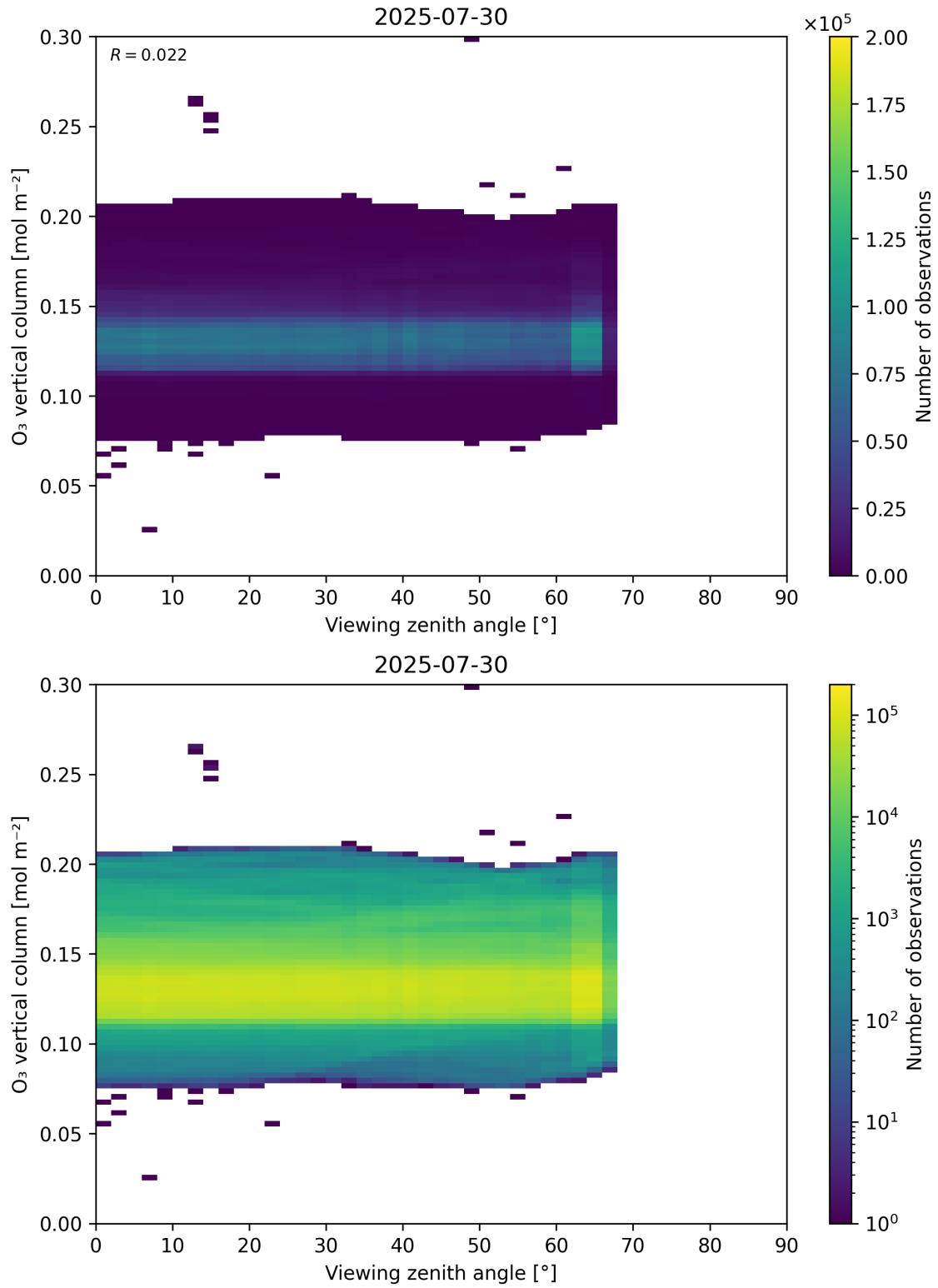
Figure 52: Scatter density plot of “Viewing zenith angle” against “O 3 vertical column” for 2025-07-29 to 2025-07-31.
