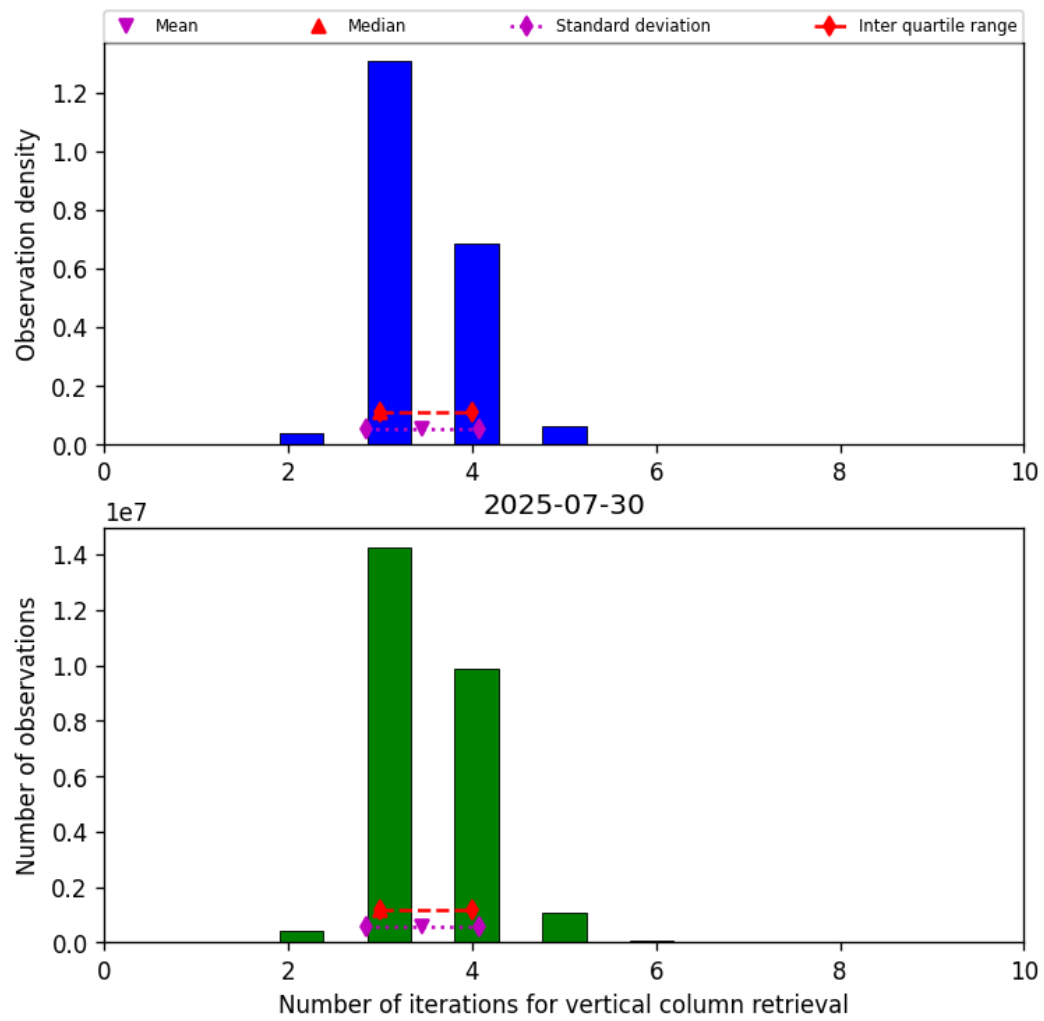
Figure 26: Histogram of “Number of iterations for vertical column retrieval” for 2025-07-29 to 2025-07-31
