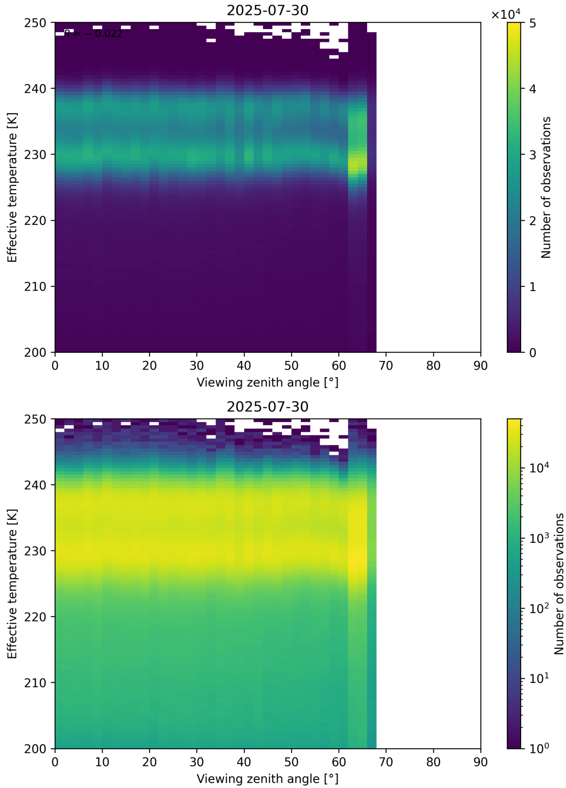
Figure 50: Scatter density plot of “Viewing zenith angle” against “Effective temperature” for 2025-07-29 to 2025-07-31.
