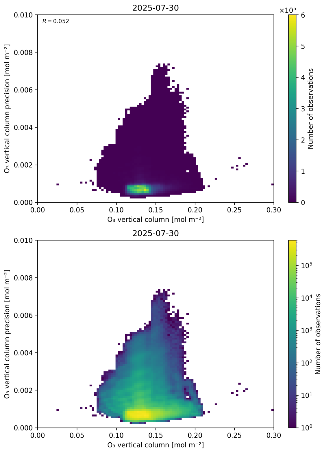
Figure 41: Scatter density plot of “O 3 vertical column” against “O 3 vertical column precision” for 2025-07-29 to 2025-07-31.
