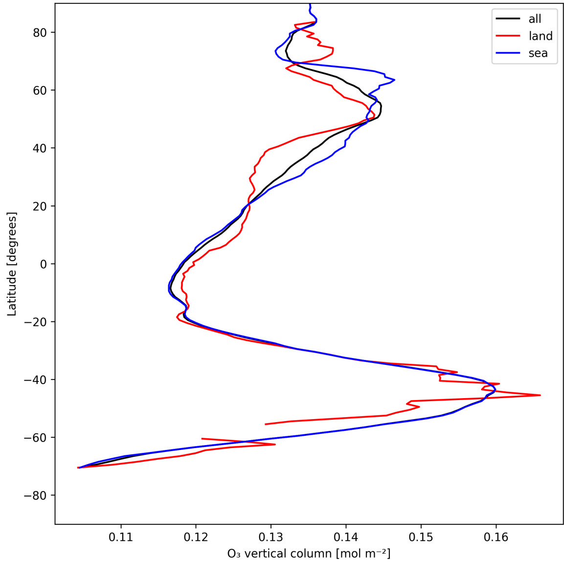
Figure 14: Zonal average of “O 3 vertical column” for 2025-07-29 to 2025-07-31.
