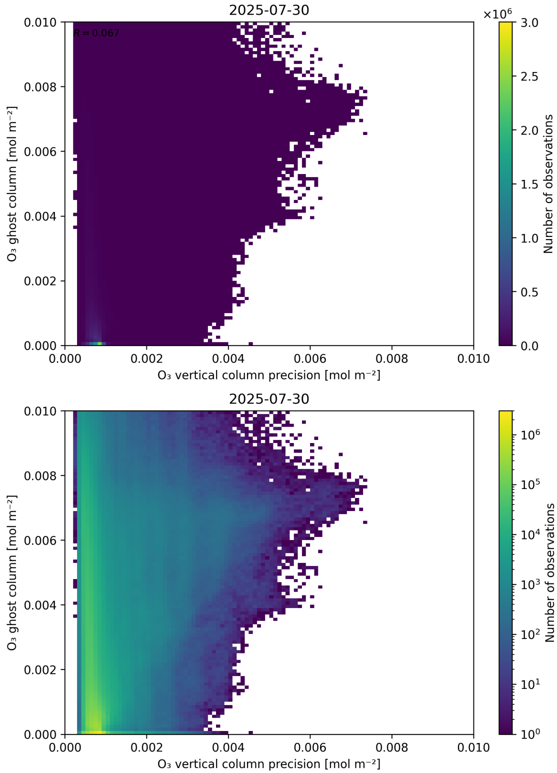
Figure 43: Scatter density plot of “O 3 vertical column precision” against “O 3 ghost column” for 2025-07-29 to 2025-07-31.
