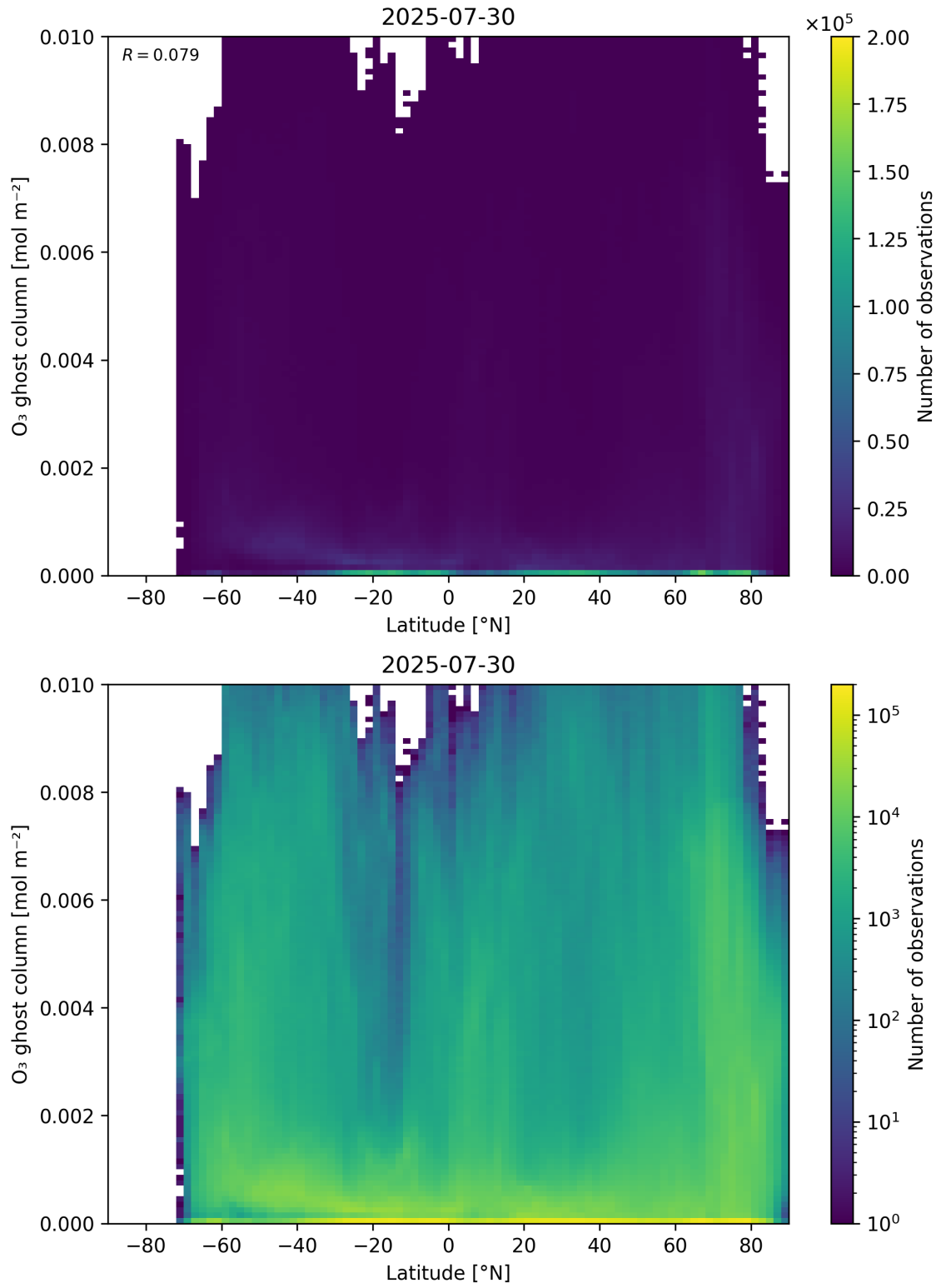
Figure 35: Scatter density plot of “Latitude” against “O 3 ghost column” for 2025-07-29 to 2025-07-31.
