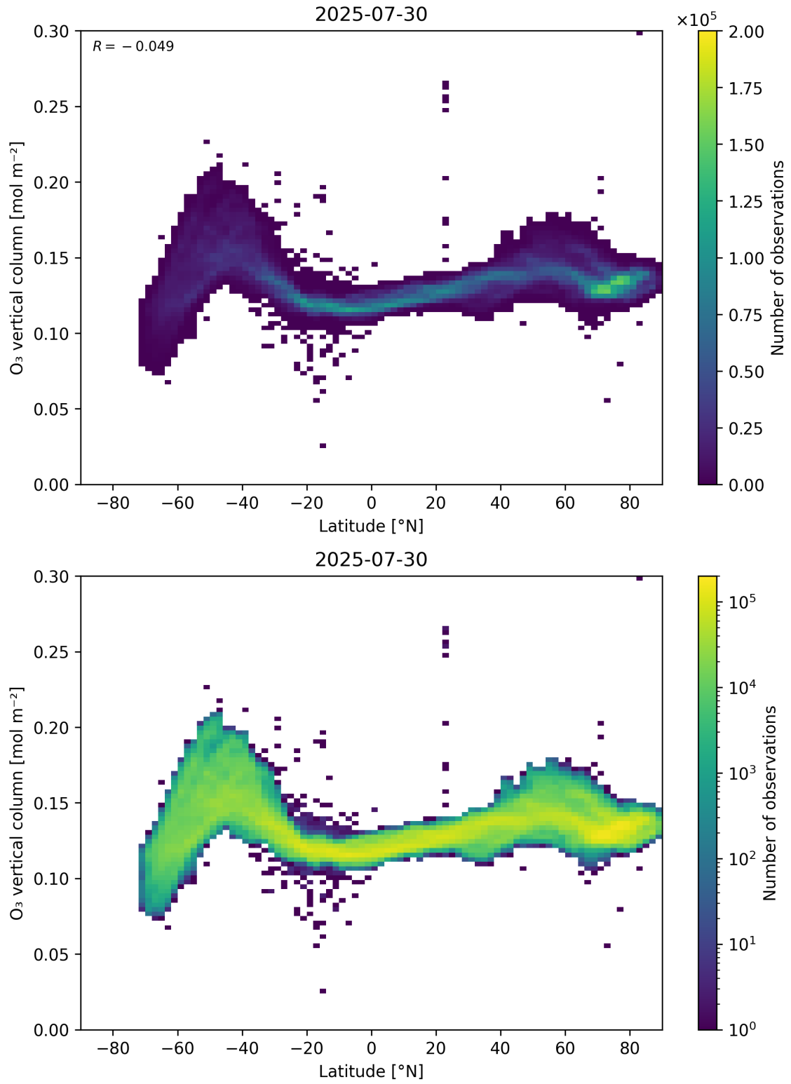
Figure 36: Scatter density plot of “Latitude” against “O 3 vertical column” for 2025-07-29 to 2025-07-31.
