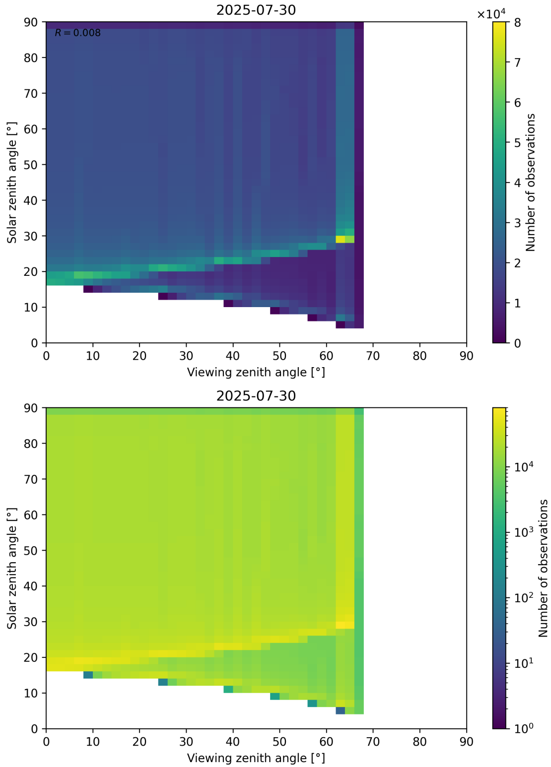
Figure 54: Scatter density plot of “Viewing zenith angle” against “Solar zenith angle” for 2025-07-29 to 2025-07-31.
