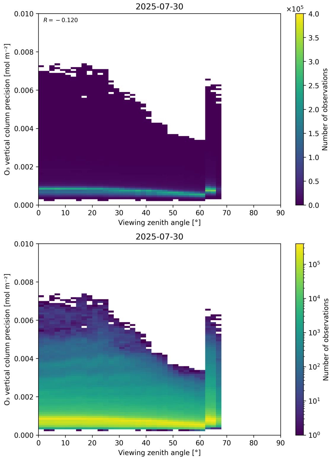
Figure 53: Scatter density plot of “Viewing zenith angle” against “O 3 vertical column precision” for 2025-07-29 to 2025-07-31.
