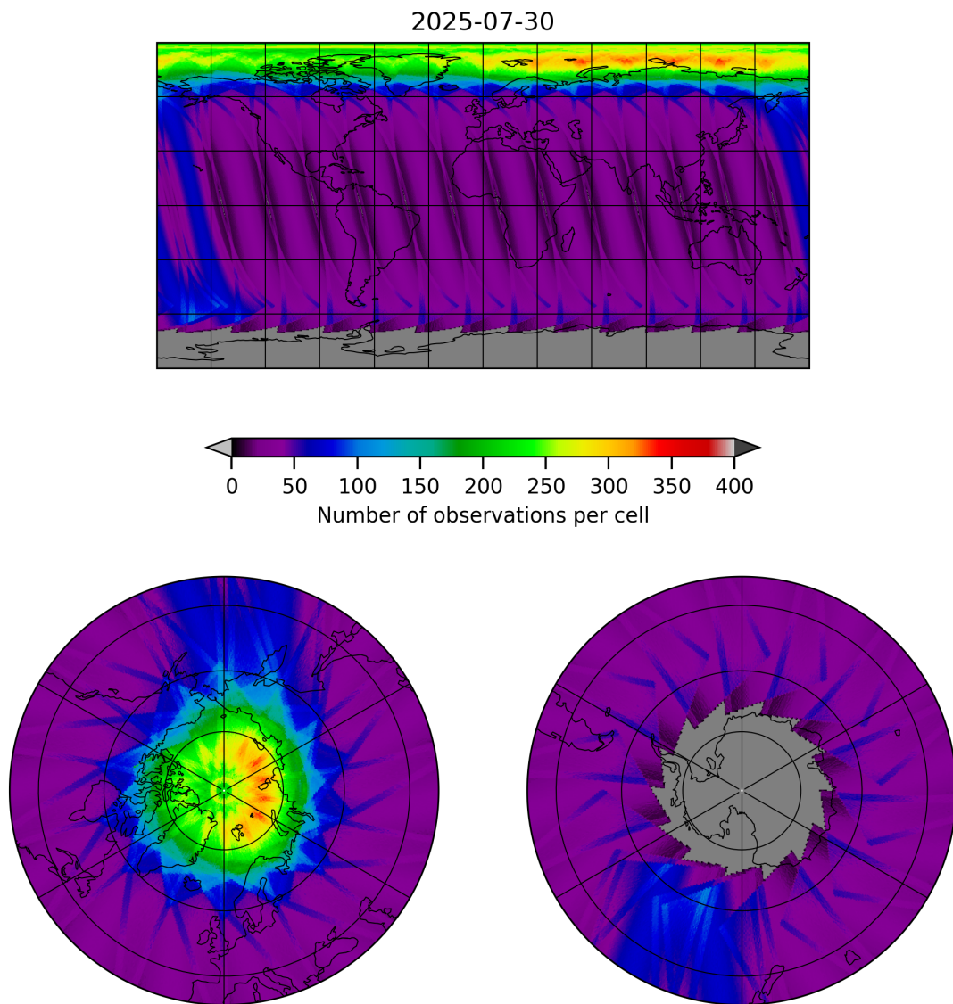
Figure 12: Map of the number of observations for 2025-07-29 to 2025-07-31
