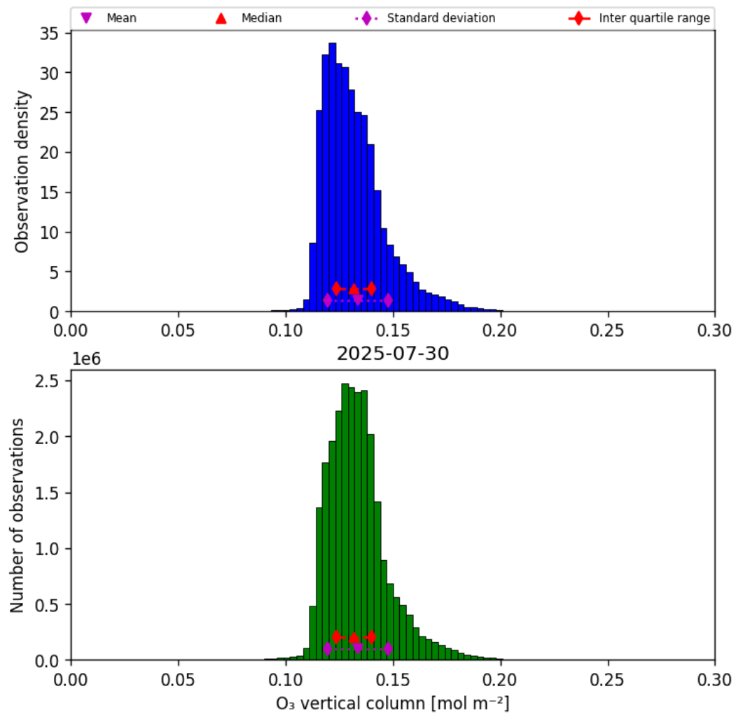
Figure 21: Histogram of “O 3 vertical column” for 2025-07-29 to 2025-07-31
