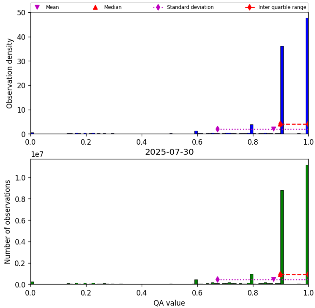
Figure 20: Histogram of “QA value” for 2025-07-29 to 2025-07-31
