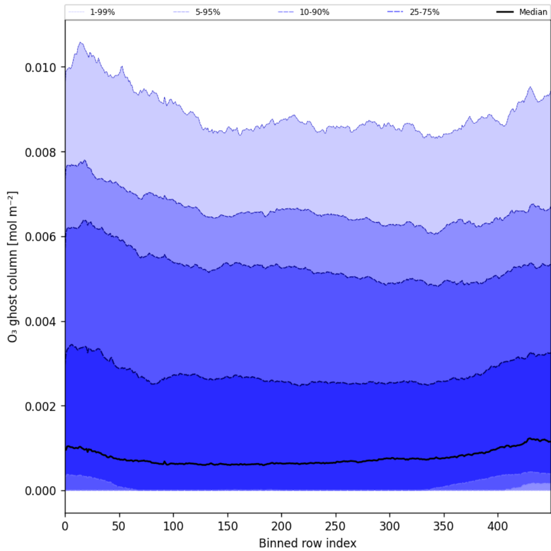
Figure 32: Along track statistics of “O 3 ghost column” for 2025-07-29 to 2025-07-31
