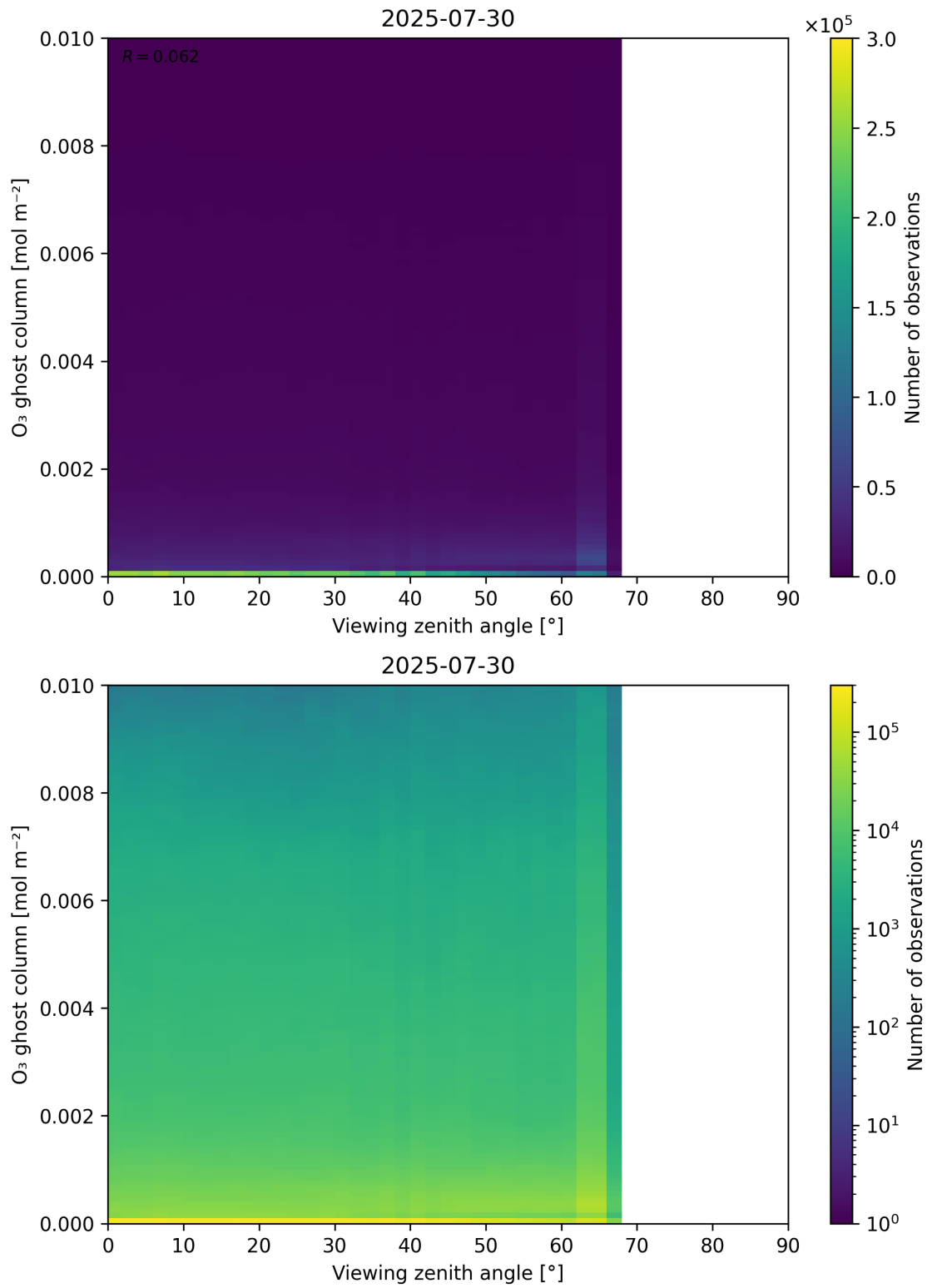
Figure 51: Scatter density plot of “Viewing zenith angle” against “O 3 ghost column” for 2025-07-29 to 2025-07-31.
