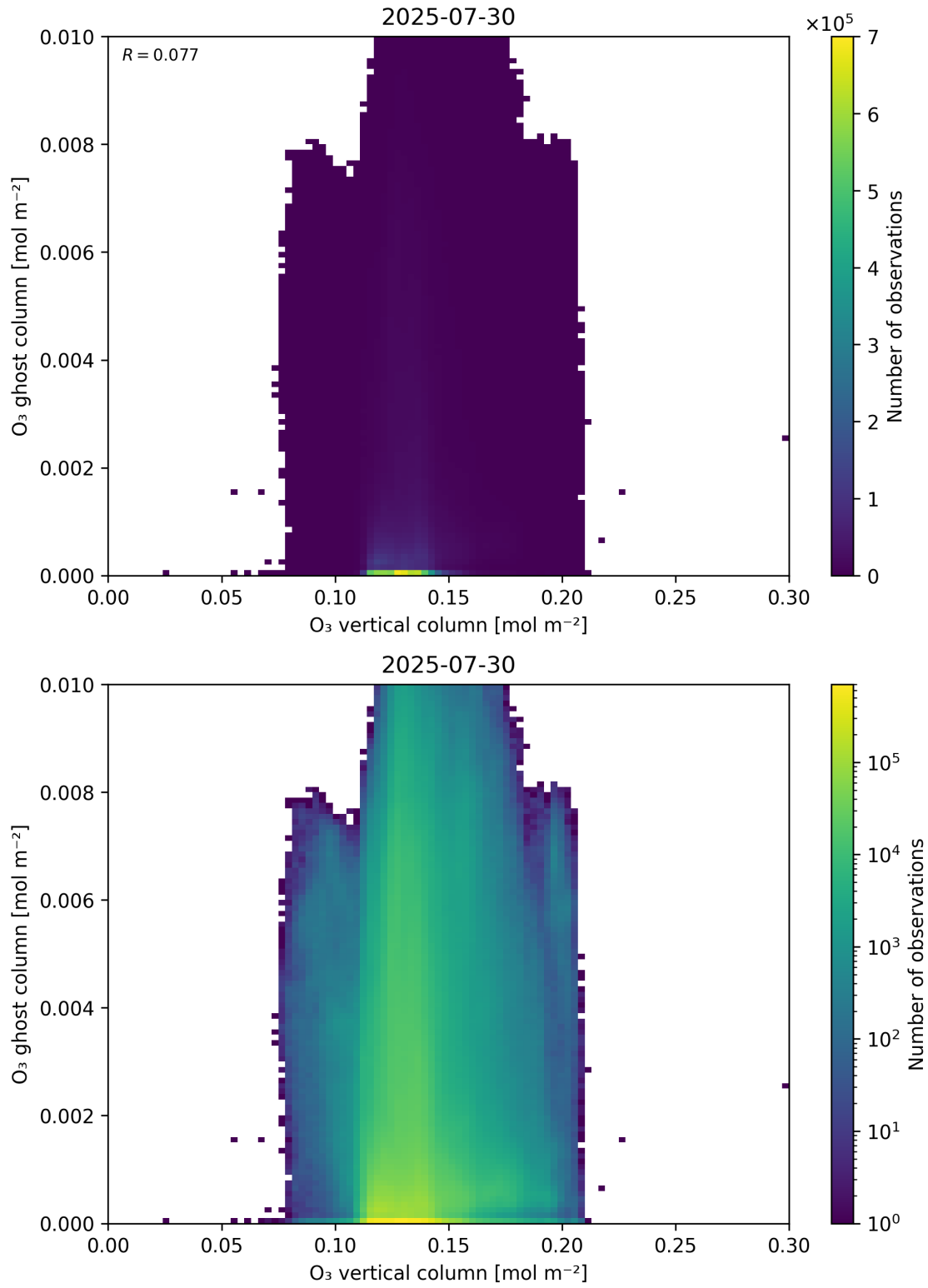
Figure 40: Scatter density plot of “O 3 vertical column” against “O 3 ghost column” for 2025-07-29 to 2025-07-31.
