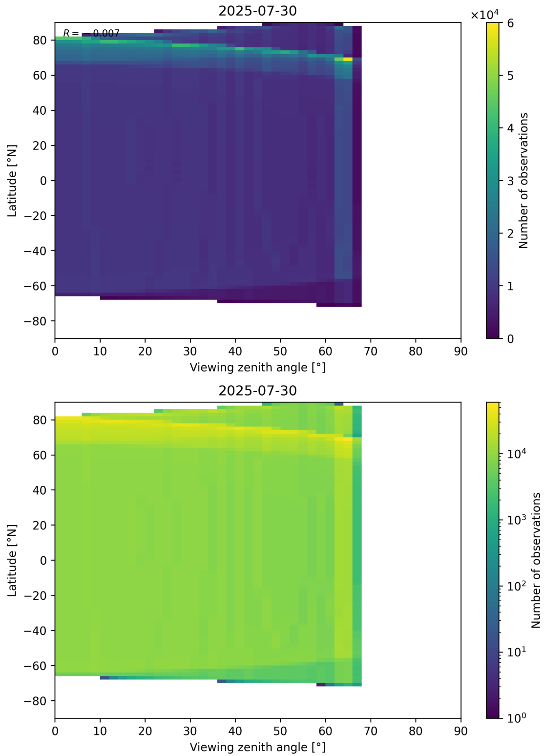
Figure 49: Scatter density plot of “Viewing zenith angle” against “Latitude” for 2025-07-29 to 2025-07-31.
