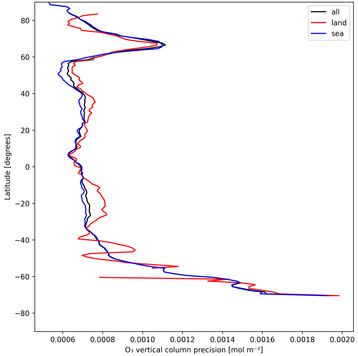
Figure 15: Zonal average of “O 3 vertical column precision” for 2025-07-29 to 2025-07-31.
