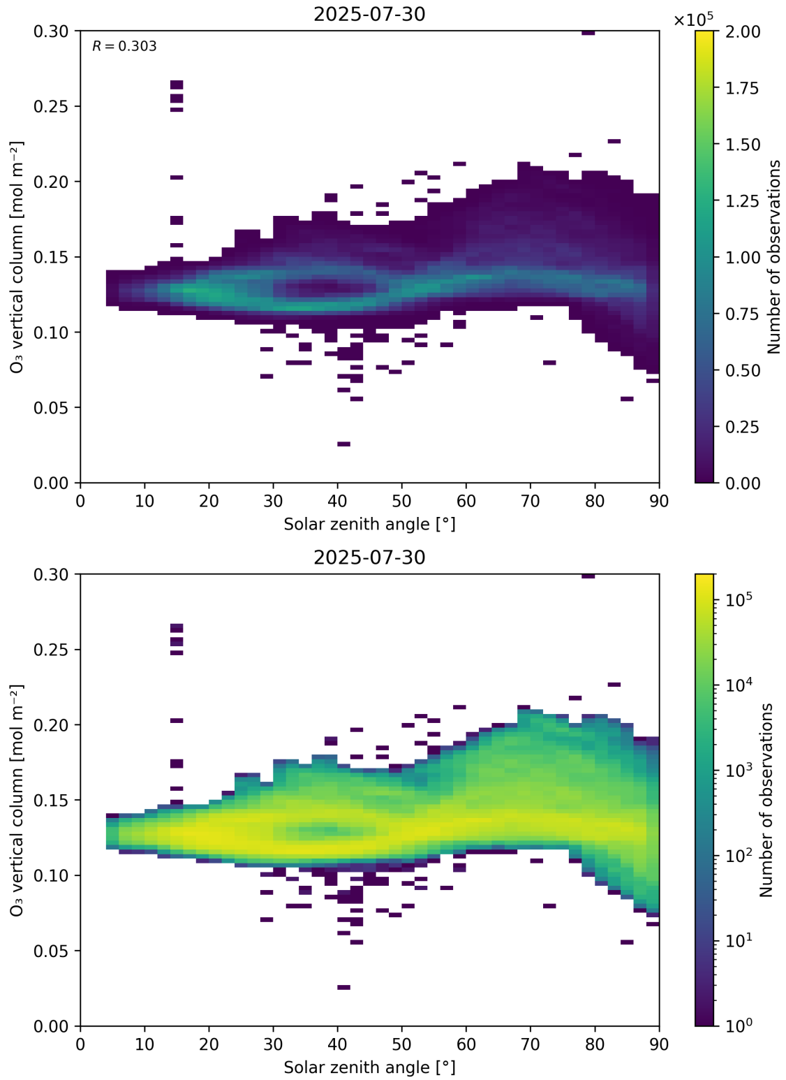
Figure 47: Scatter density plot of “Solar zenith angle” against “O 3 vertical column” for 2025-07-29 to 2025-07-31.
