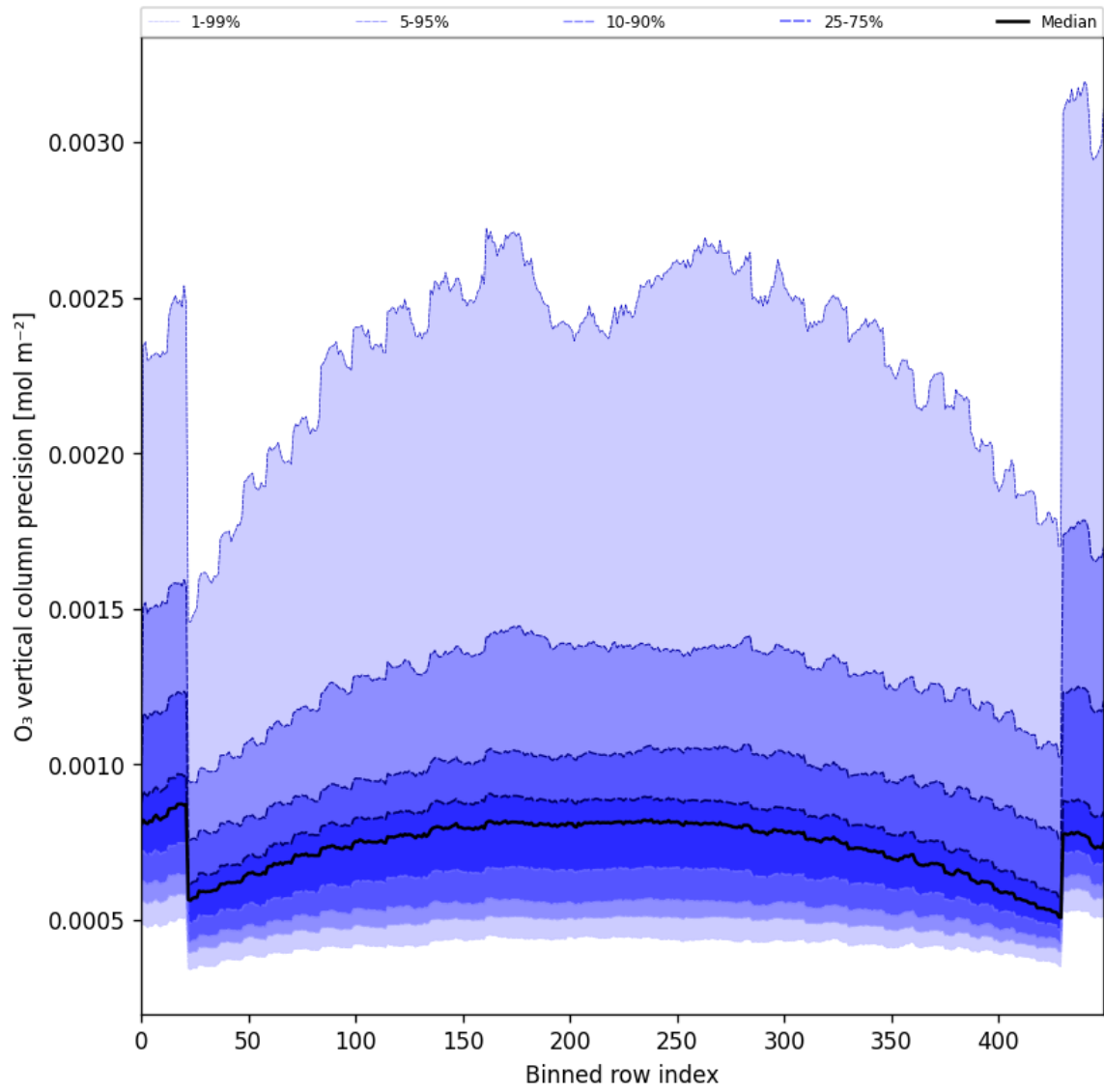
Figure 29: Along track statistics of “O 3 vertical column precision” for 2025-07-29 to 2025-07-31
