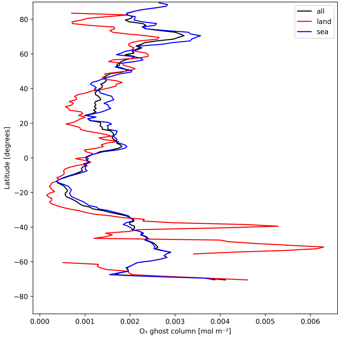
Figure 18: Zonal average of “O 3 ghost column” for 2025-07-29 to 2025-07-31.
