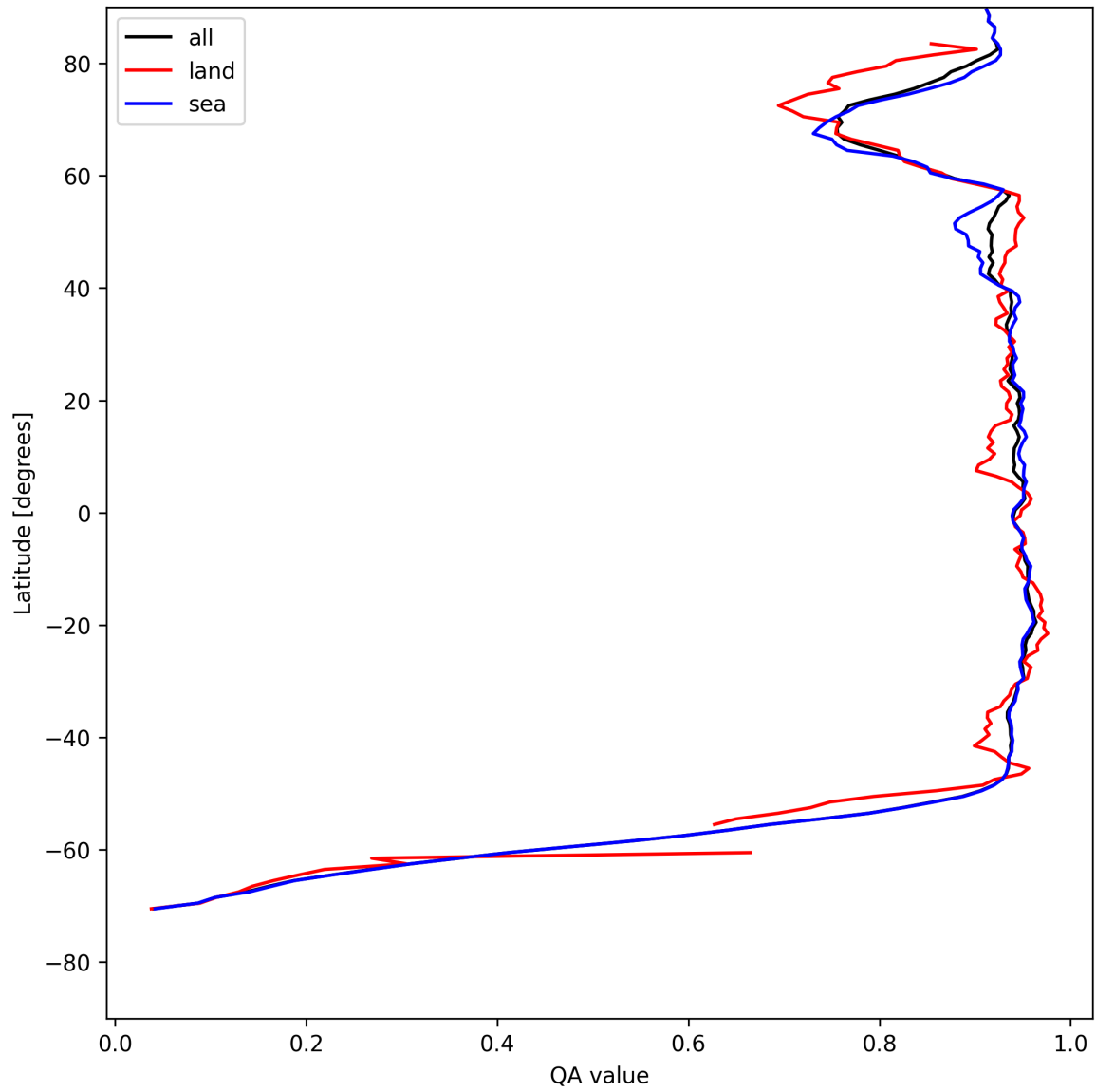
Figure 13: Zonal average of “QA value” for 2025-07-29 to 2025-07-31.
