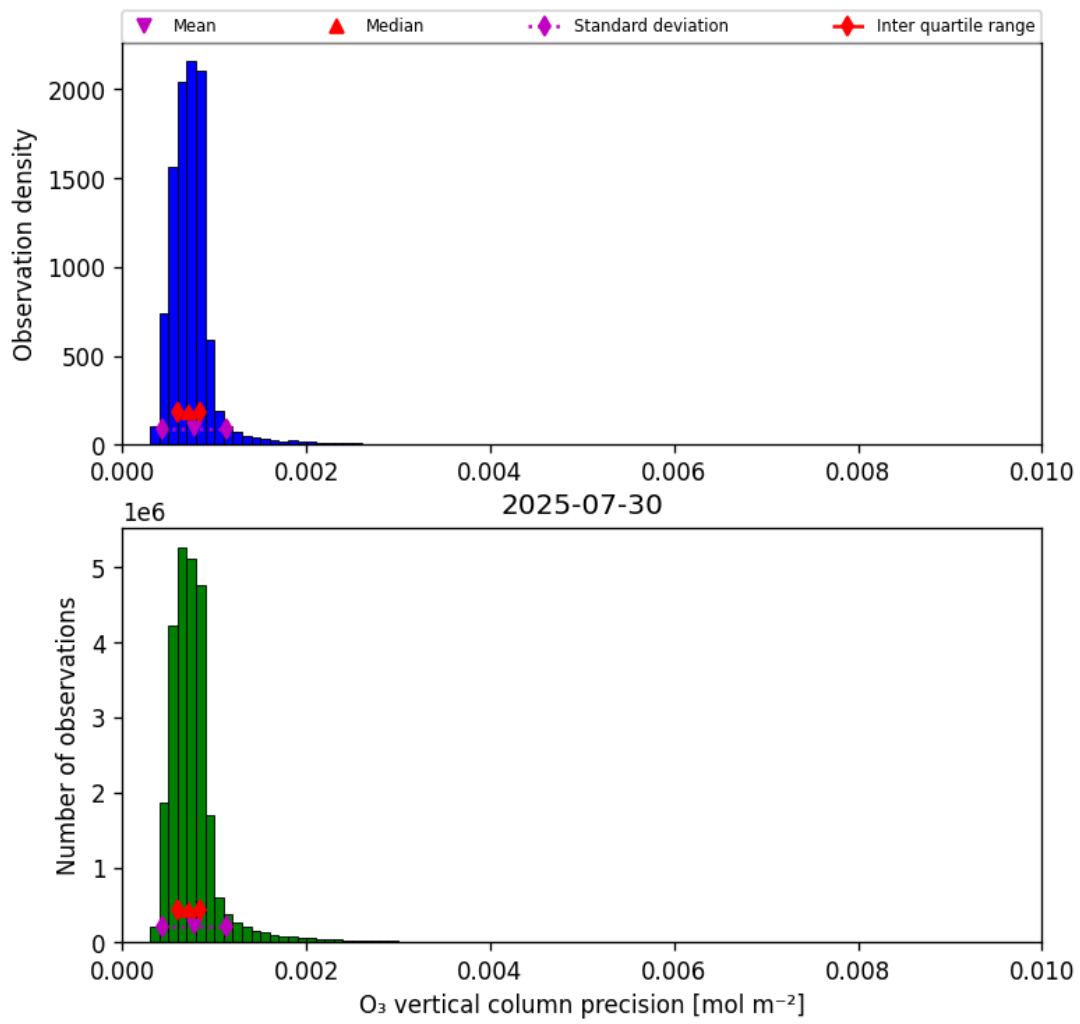
Figure 22: Histogram of “O 3 vertical column precision” for 2025-07-29 to 2025-07-31
