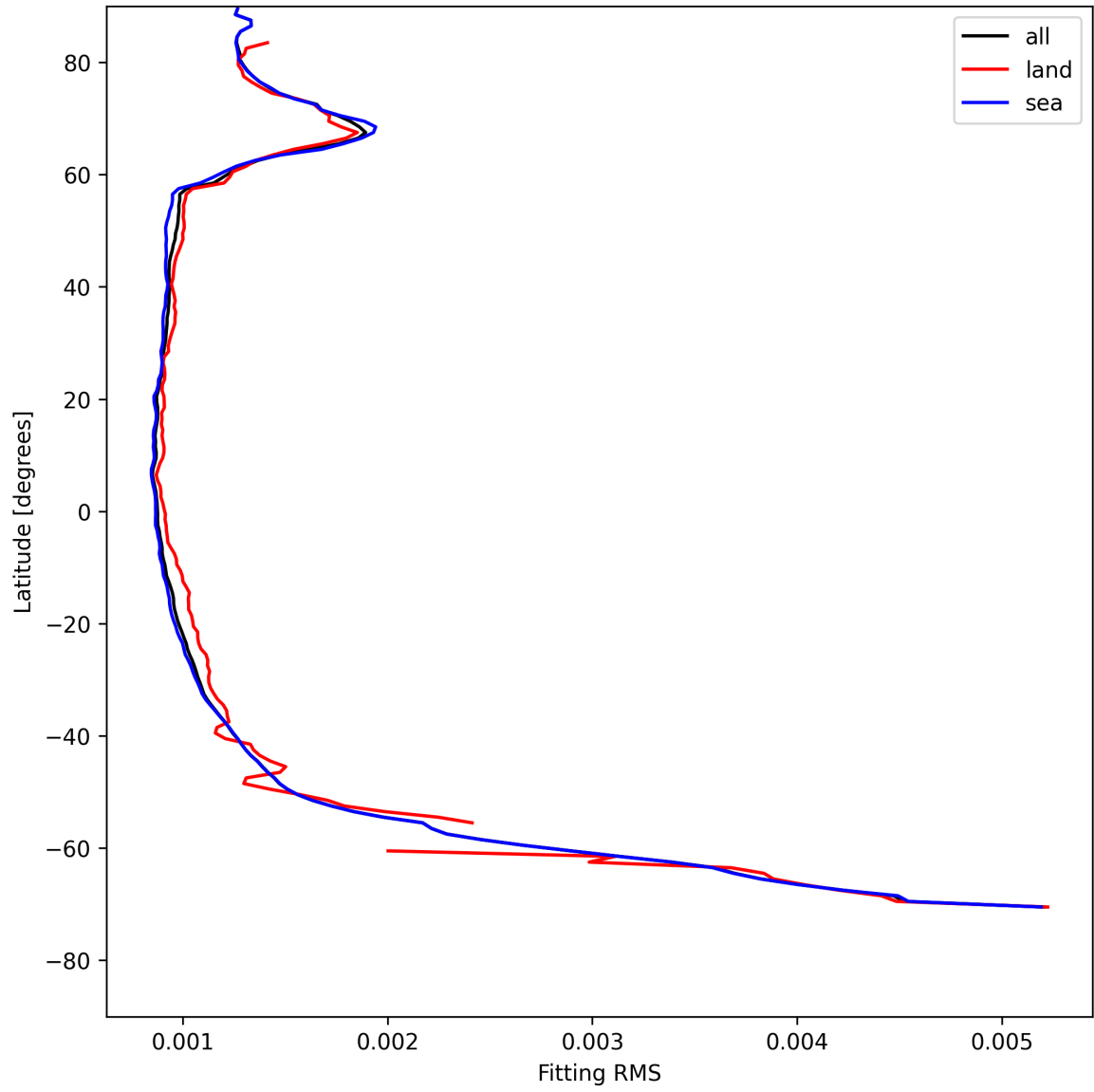
Figure 16: Zonal average of “Fitting RMS” for 2025-07-29 to 2025-07-31.
