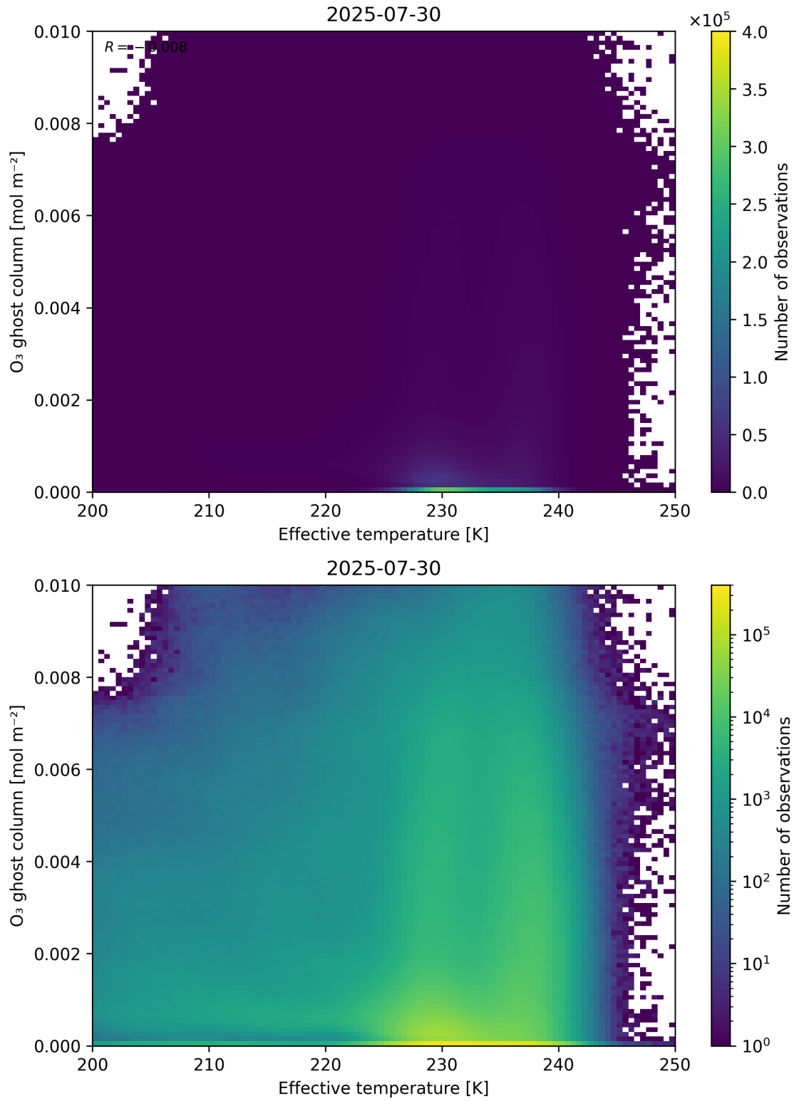
Figure 38: Scatter density plot of “Effective temperature” against “O 3 ghost column” for 2025-07-29 to 2025-07-31.
