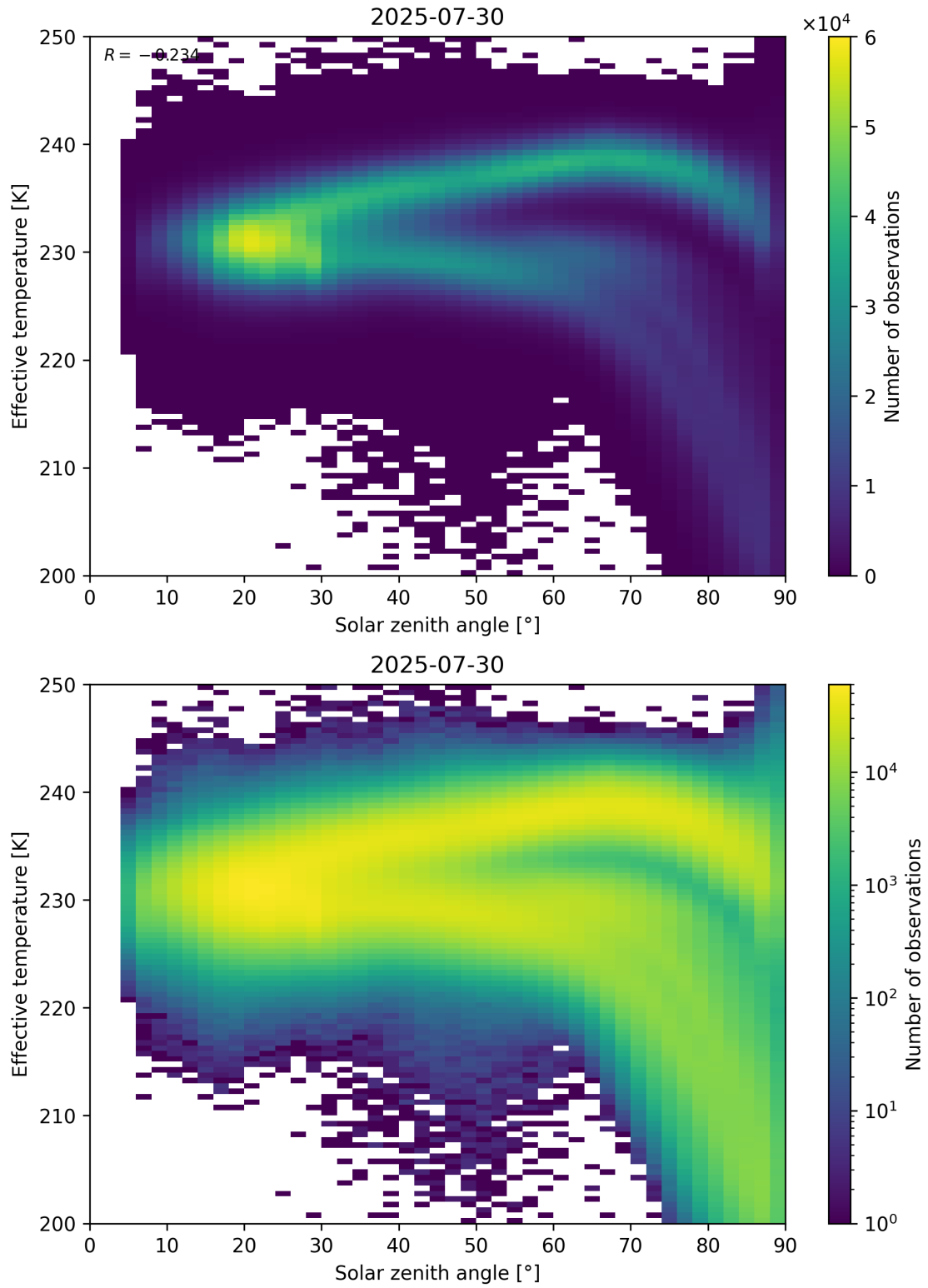
Figure 45: Scatter density plot of “Solar zenith angle” against “Effective temperature” for 2025-07-29 to 2025-07-31.
