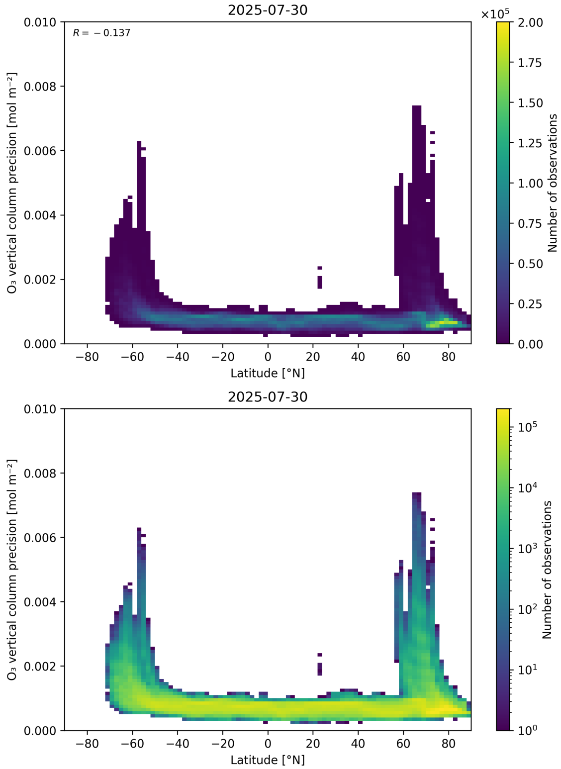
Figure 37: Scatter density plot of “Latitude” against “O 3 vertical column precision” for 2025-07-29 to 2025-07-31.
