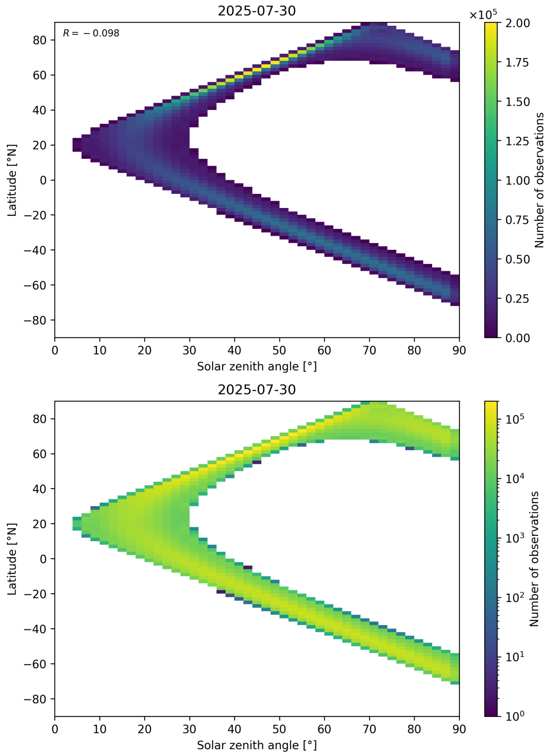
Figure 44: Scatter density plot of “Solar zenith angle” against “Latitude” for 2025-07-29 to 2025-07-31.
