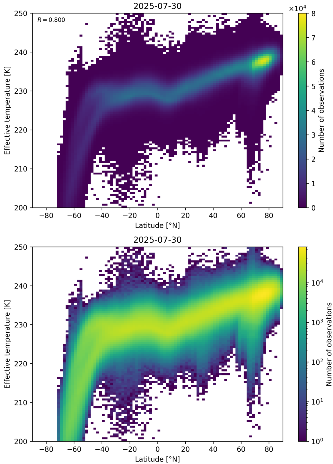
Figure 34: Scatter density plot of “Latitude” against “Effective temperature” for 2025-07-29 to 2025-07-31.
