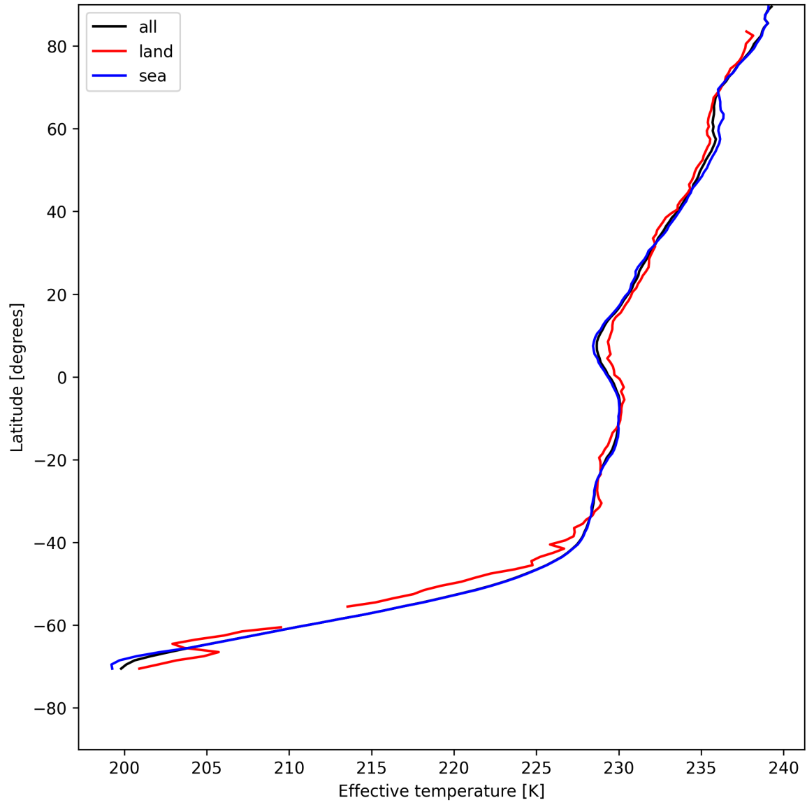
Figure 17: Zonal average of "Effective temperature" for 2025-07-29 to 2025-07-31.
