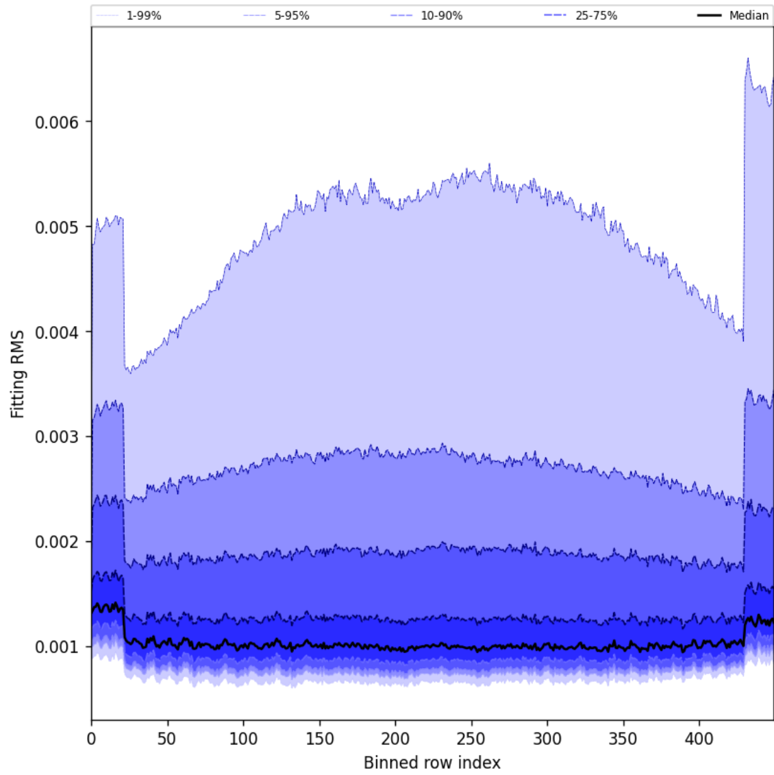
Figure 30: Along track statistics of “Fitting RMS” for 2025-07-29 to 2025-07-31
