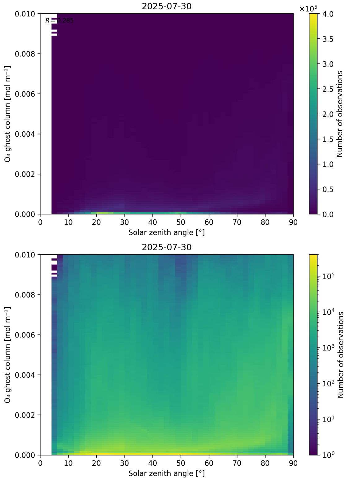
Figure 46: Scatter density plot of “Solar zenith angle” against “O 3 ghost column” for 2025-07-29 to 2025-07-31.
