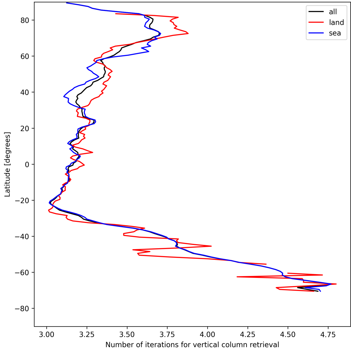
Figure 19: Zonal average of “Number of iterations for vertical column retrieval” for 2025-07-29 to 2025-07-31.
