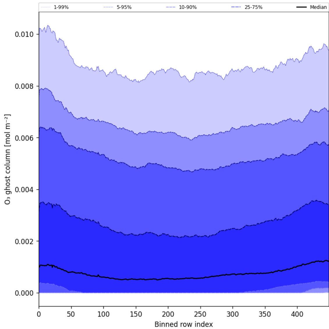
Figure 32: Along track statistics of “O 3 ghost column” for 2025-07-30 to 2025-08-01
