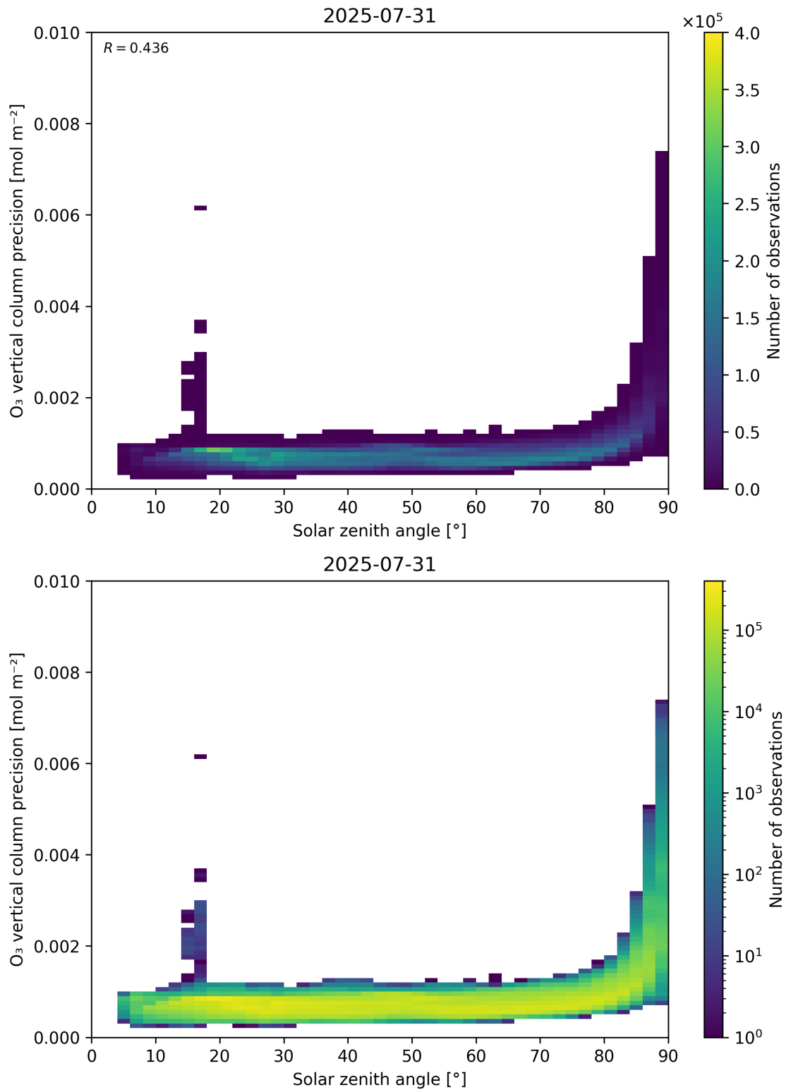
Figure 48: Scatter density plot of “Solar zenith angle” against “O 3 vertical column precision” for 2025-07-30 to 2025-08-01.
