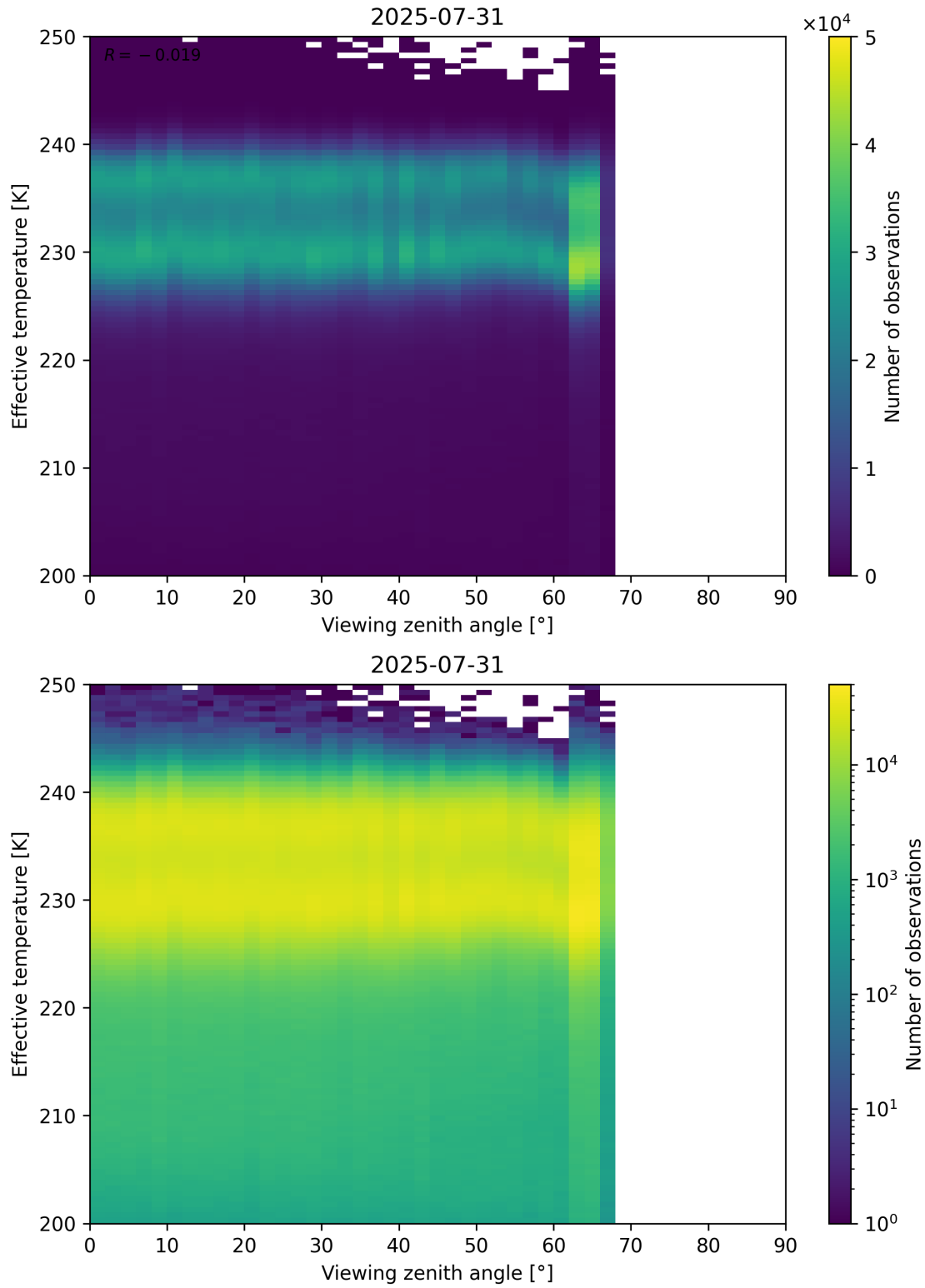
Figure 50: Scatter density plot of “Viewing zenith angle” against “Effective temperature” for 2025-07-30 to 2025-08-01.
