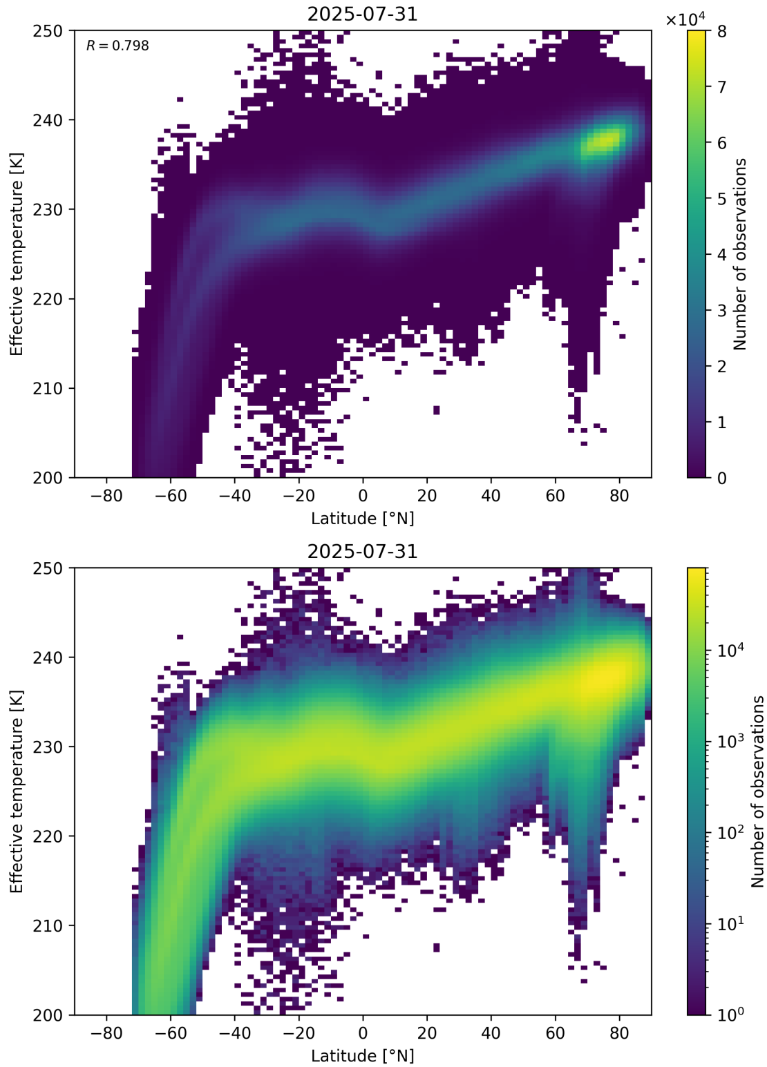
Figure 34: Scatter density plot of “Latitude” against “Effective temperature” for 2025-07-30 to 2025-08-01.
