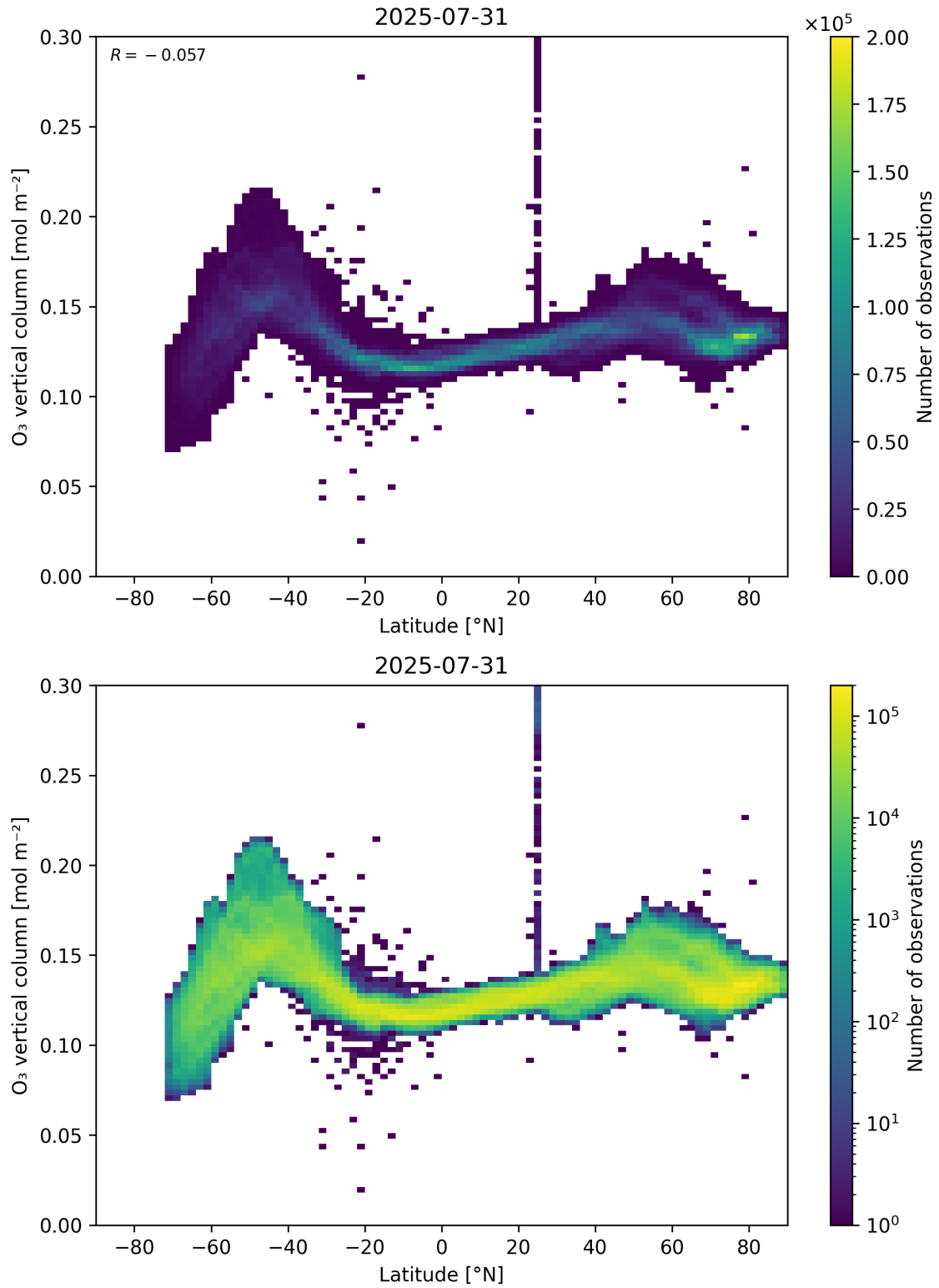
Figure 36: Scatter density plot of “Latitude” against “O 3 vertical column” for 2025-07-30 to 2025-08-01.
