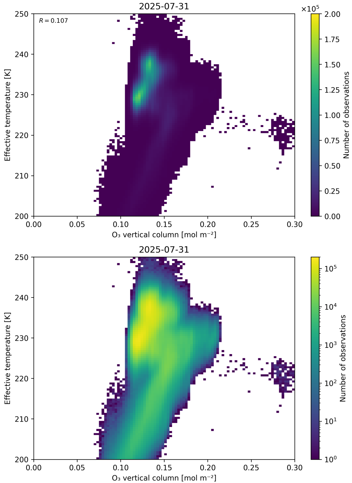
Figure 39: Scatter density plot of “O 3 vertical column” against “Effective temperature” for 2025-07-30 to 2025-08-01.
