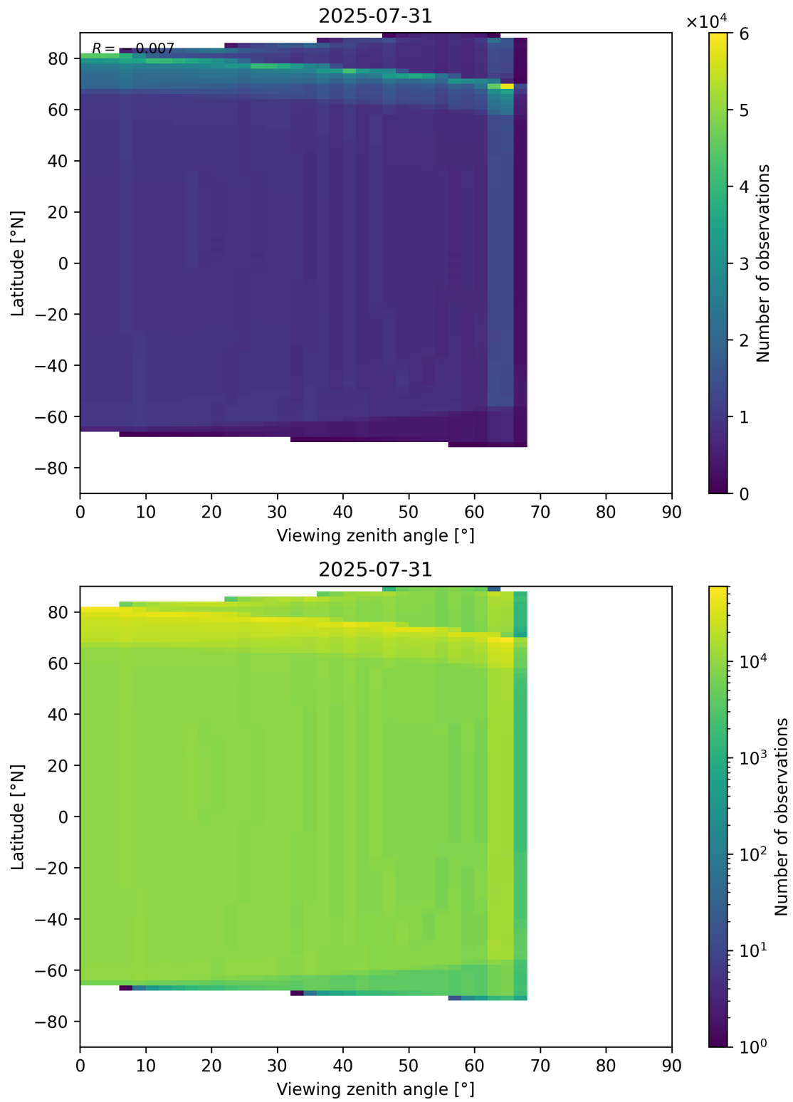
Figure 49: Scatter density plot of “Viewing zenith angle” against “Latitude” for 2025-07-30 to 2025-08-01.
