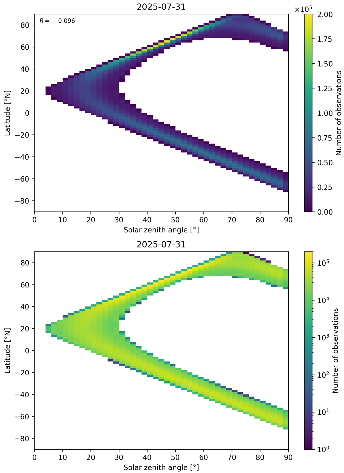
Figure 44: Scatter density plot of “Solar zenith angle” against “Latitude” for 2025-07-30 to 2025-08-01.
