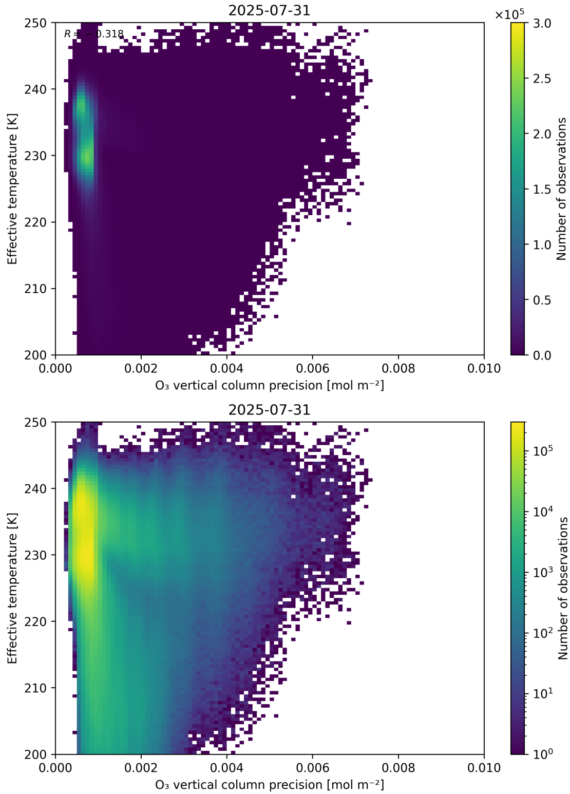
Figure 42: Scatter density plot of “O 3 vertical column precision” against “Effective temperature” for 2025-07-30 to 2025-08-01.
