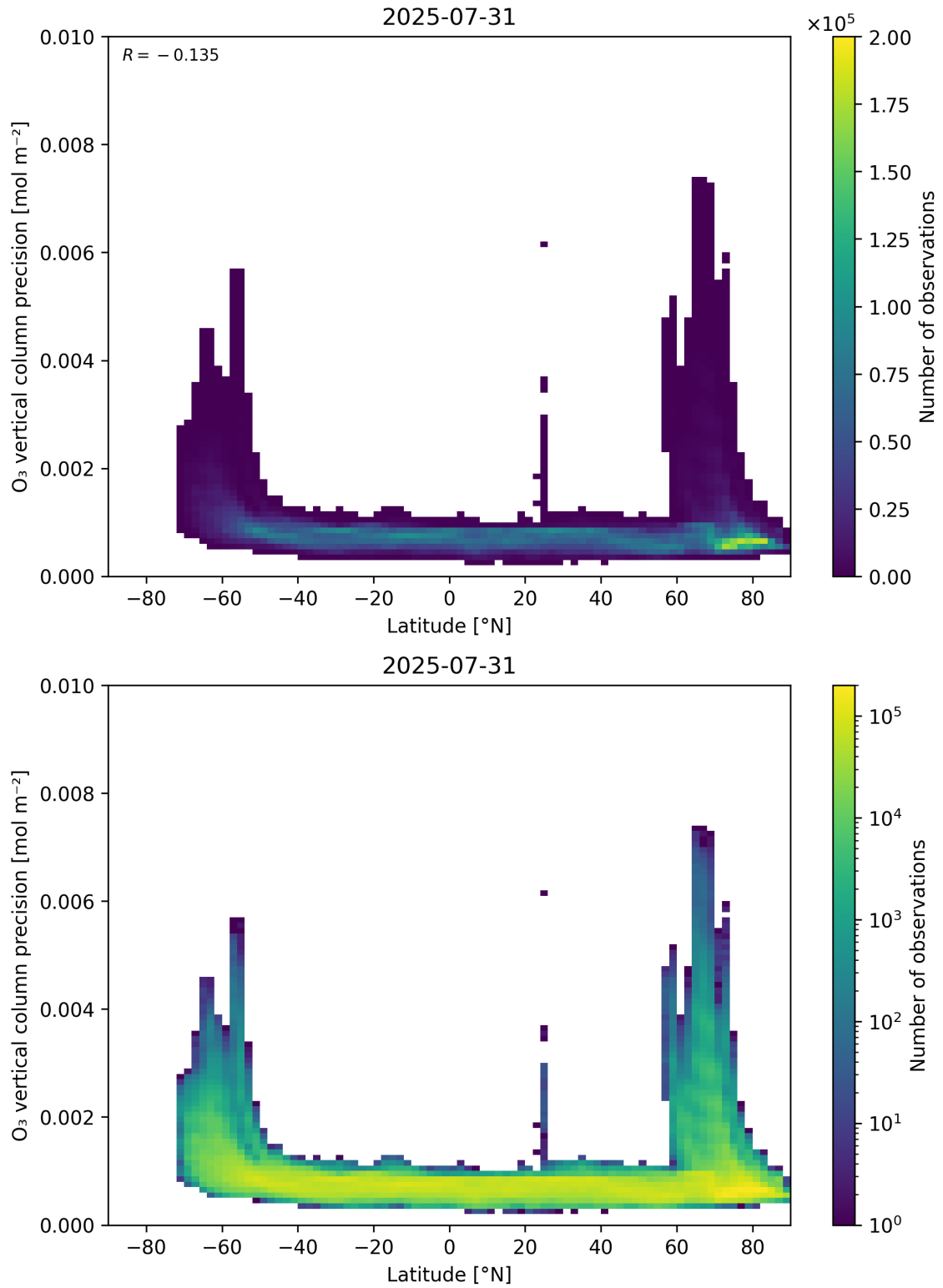
Figure 37: Scatter density plot of “Latitude” against “O 3 vertical column precision” for 2025-07-30 to 2025-08-01.
