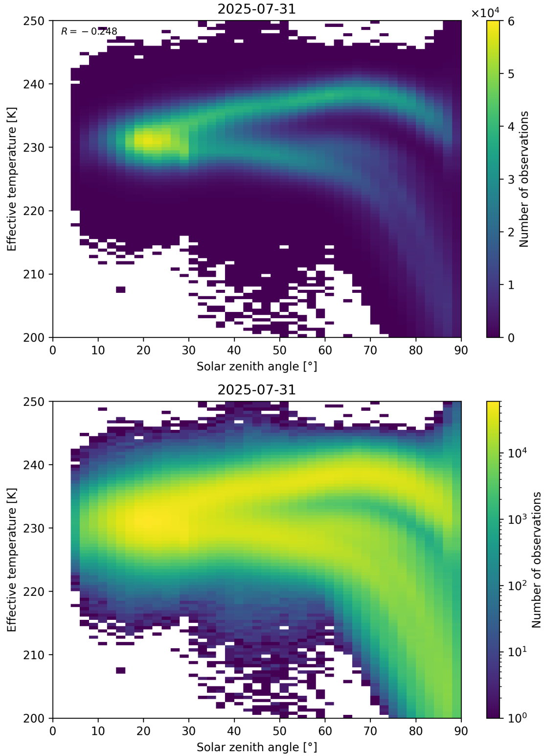
Figure 45: Scatter density plot of “Solar zenith angle” against “Effective temperature” for 2025-07-30 to 2025-08-01.
