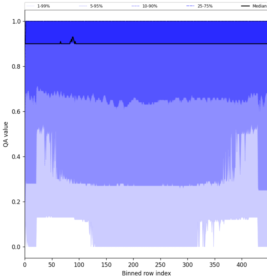
Figure 27: Along track statistics of “QA value” for 2025-07-30 to 2025-08-01
