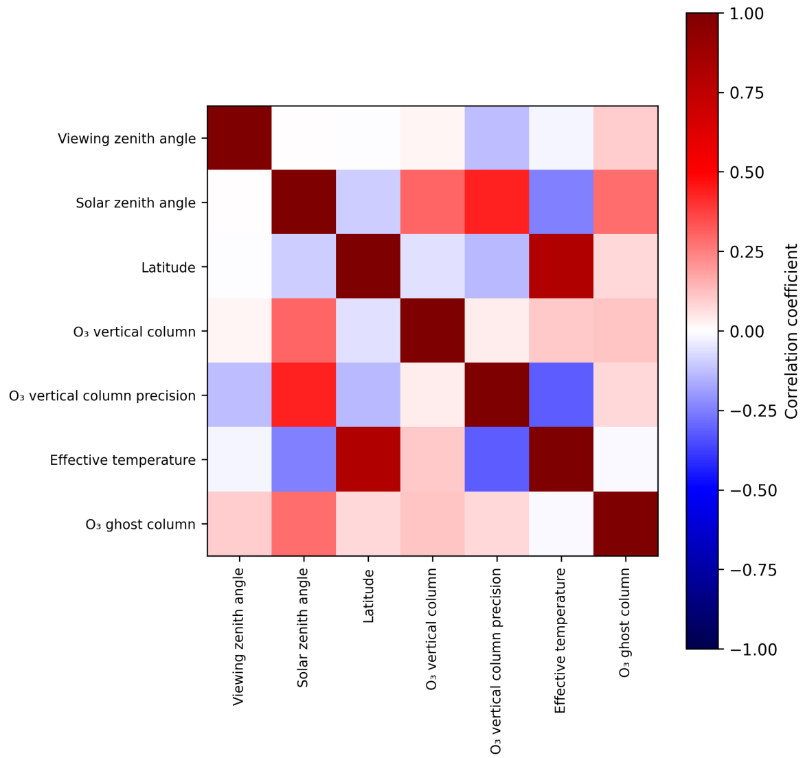
Figure 2: Map of correlation matrix for 2025-07-30 to 2025-08-01.
