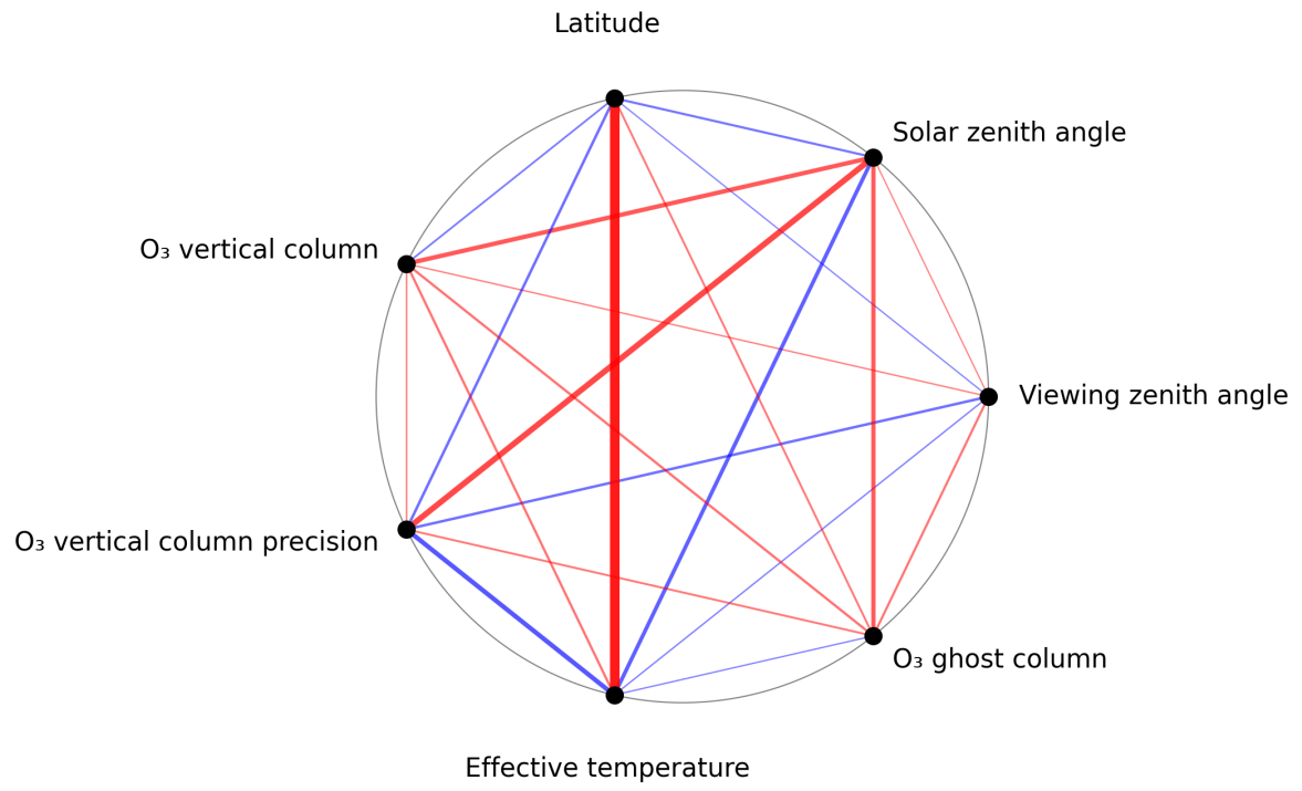
Figure 1: Map of correlation graph for 2025-07-30 to 2025-08-01.
