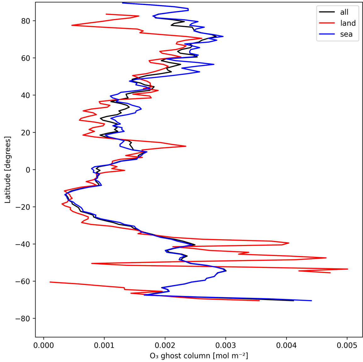
Figure 18: Zonal average of “O 3 ghost column” for 2025-07-30 to 2025-08-01.
