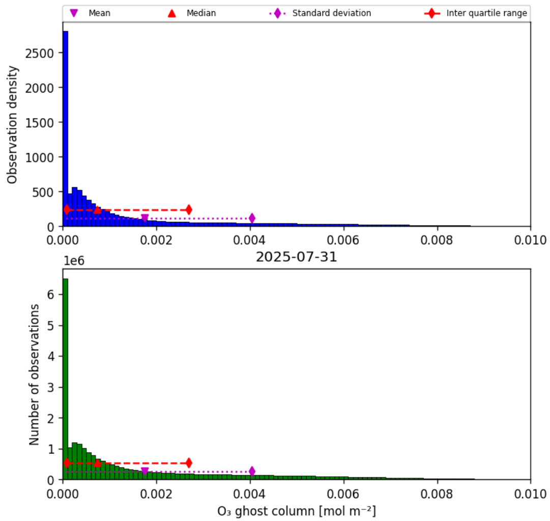
Figure 25: Histogram of “O 3 ghost column” for 2025-07-30 to 2025-08-01
