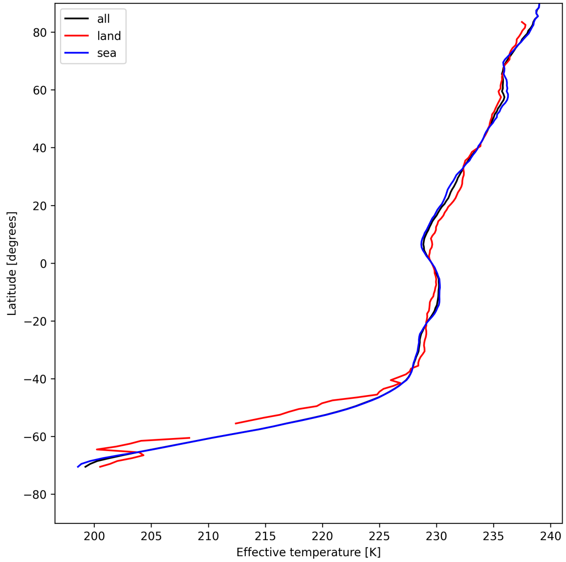
Figure 17: Zonal average of "Effective temperature" for 2025-07-30 to 2025-08-01.
