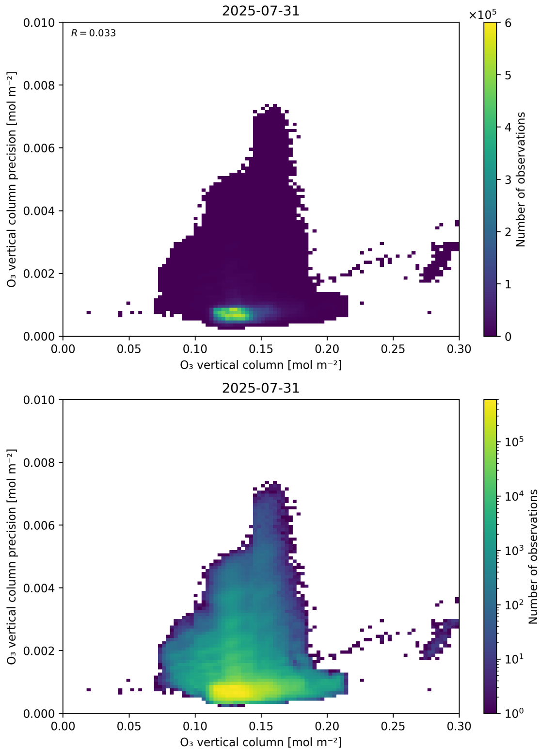
Figure 41: Scatter density plot of “O 3 vertical column” against “O 3 vertical column precision” for 2025-07-30 to 2025-08-01.
