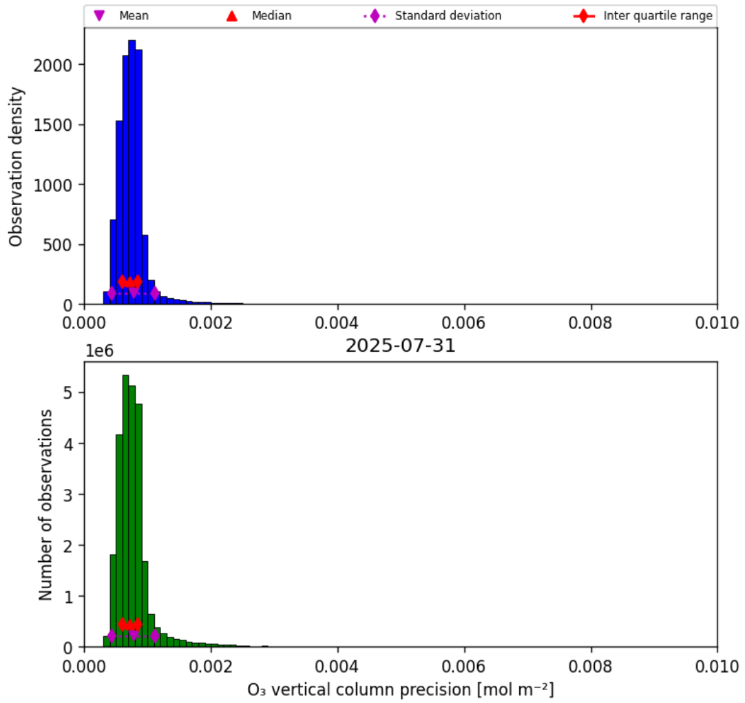
Figure 22: Histogram of “O 3 vertical column precision” for 2025-07-30 to 2025-08-01
