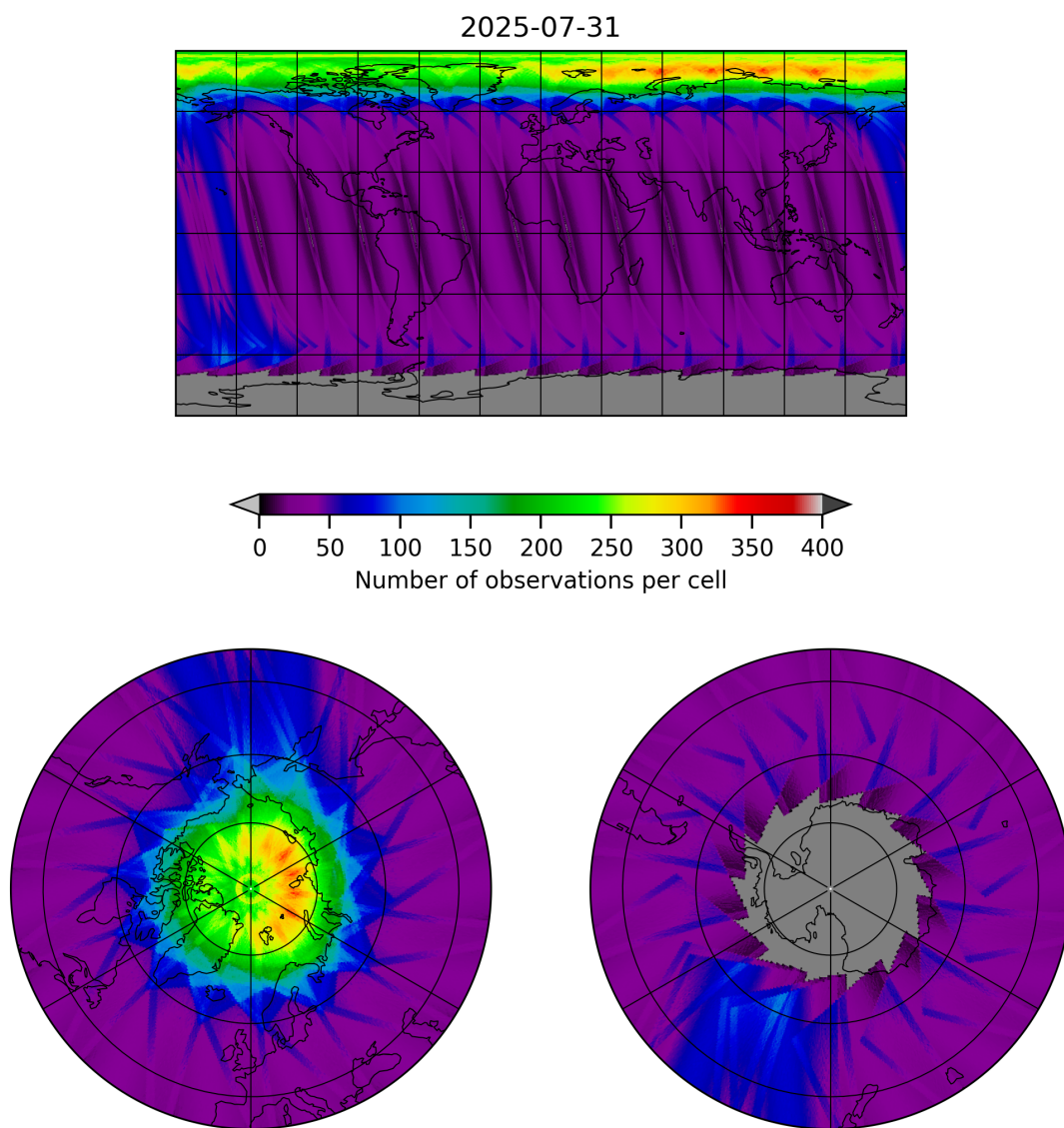
Figure 12: Map of the number of observations for 2025-07-30 to 2025-08-01
