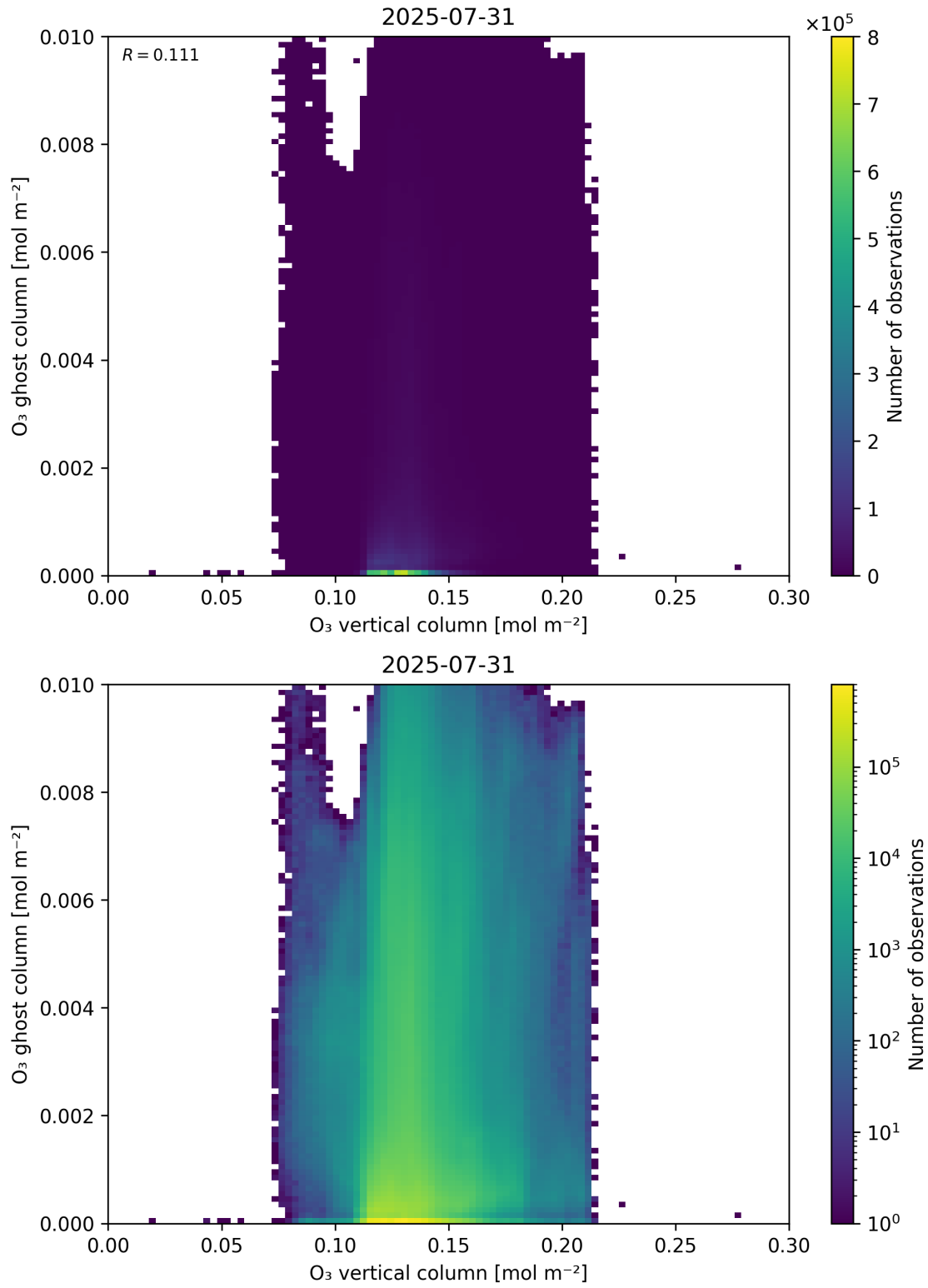
Figure 40: Scatter density plot of “O 3 vertical column” against “O 3 ghost column” for 2025-07-30 to 2025-08-01.
