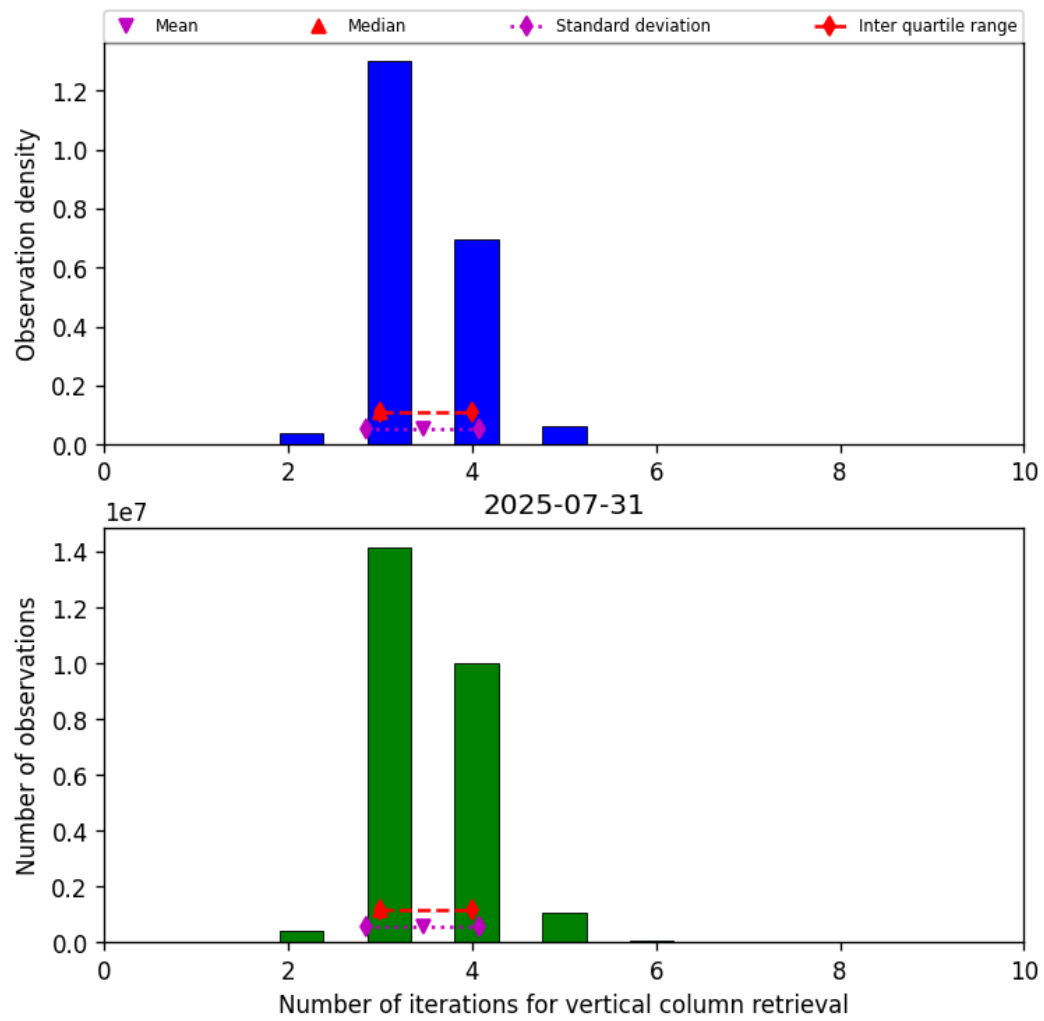
Figure 26: Histogram of “Number of iterations for vertical column retrieval” for 2025-07-30 to 2025-08-01
