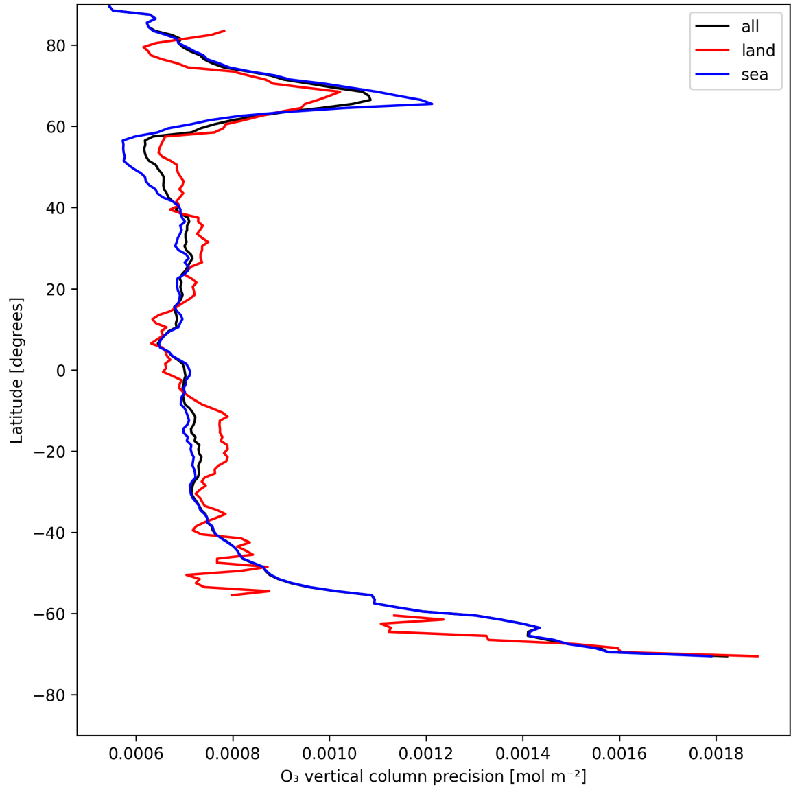
Figure 15: Zonal average of “O 3 vertical column precision” for 2025-07-30 to 2025-08-01.
