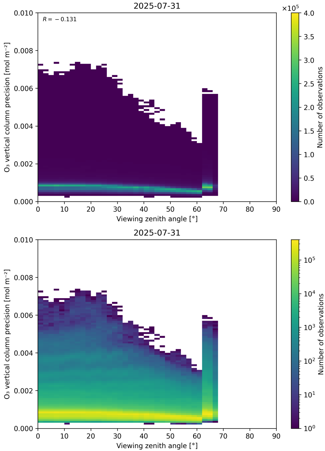
Figure 53: Scatter density plot of “Viewing zenith angle” against “O 3 vertical column precision” for 2025-07-30 to 2025-08-01.
