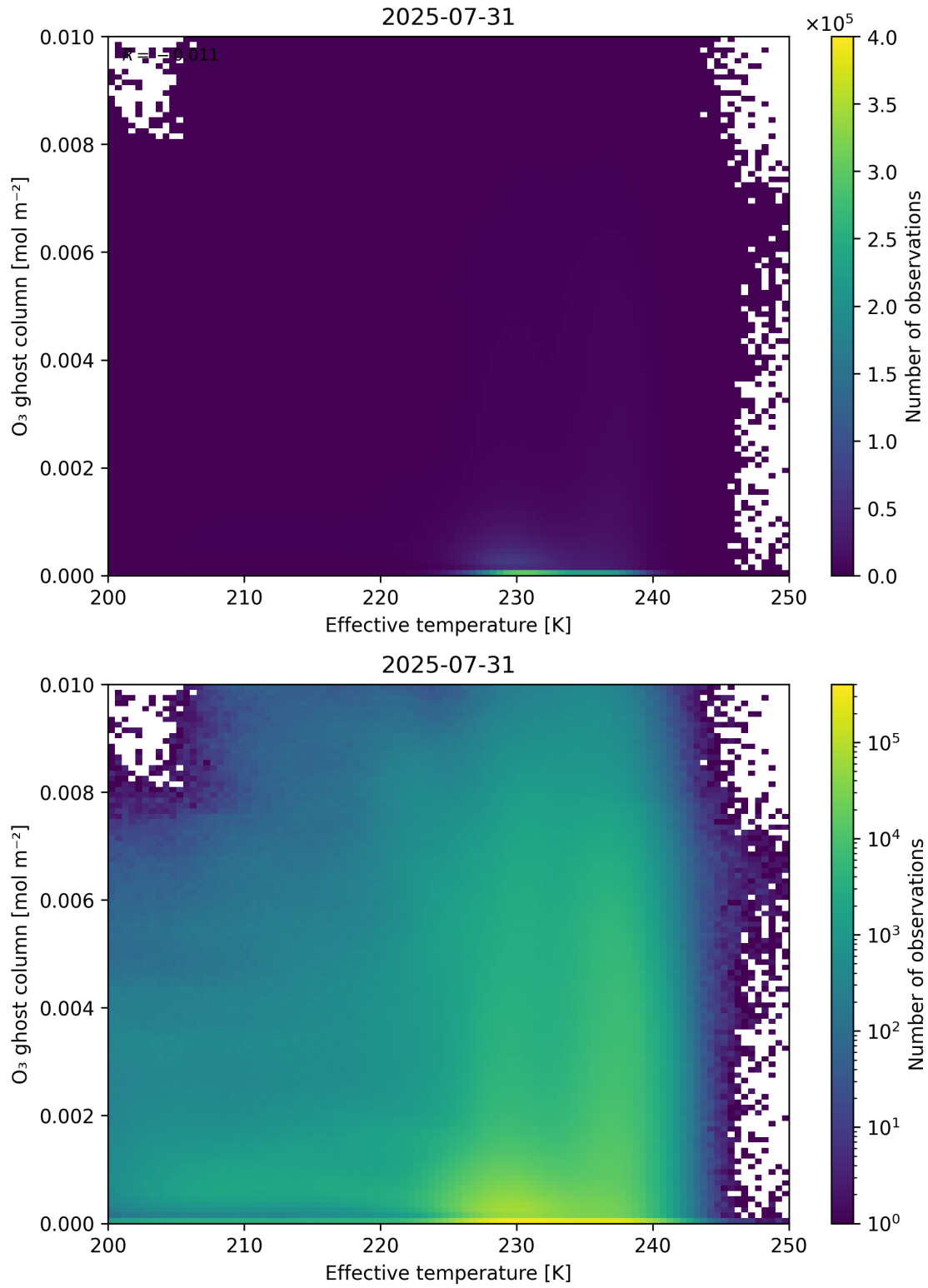
Figure 38: Scatter density plot of “Effective temperature” against “O 3 ghost column” for 2025-07-30 to 2025-08-01.
