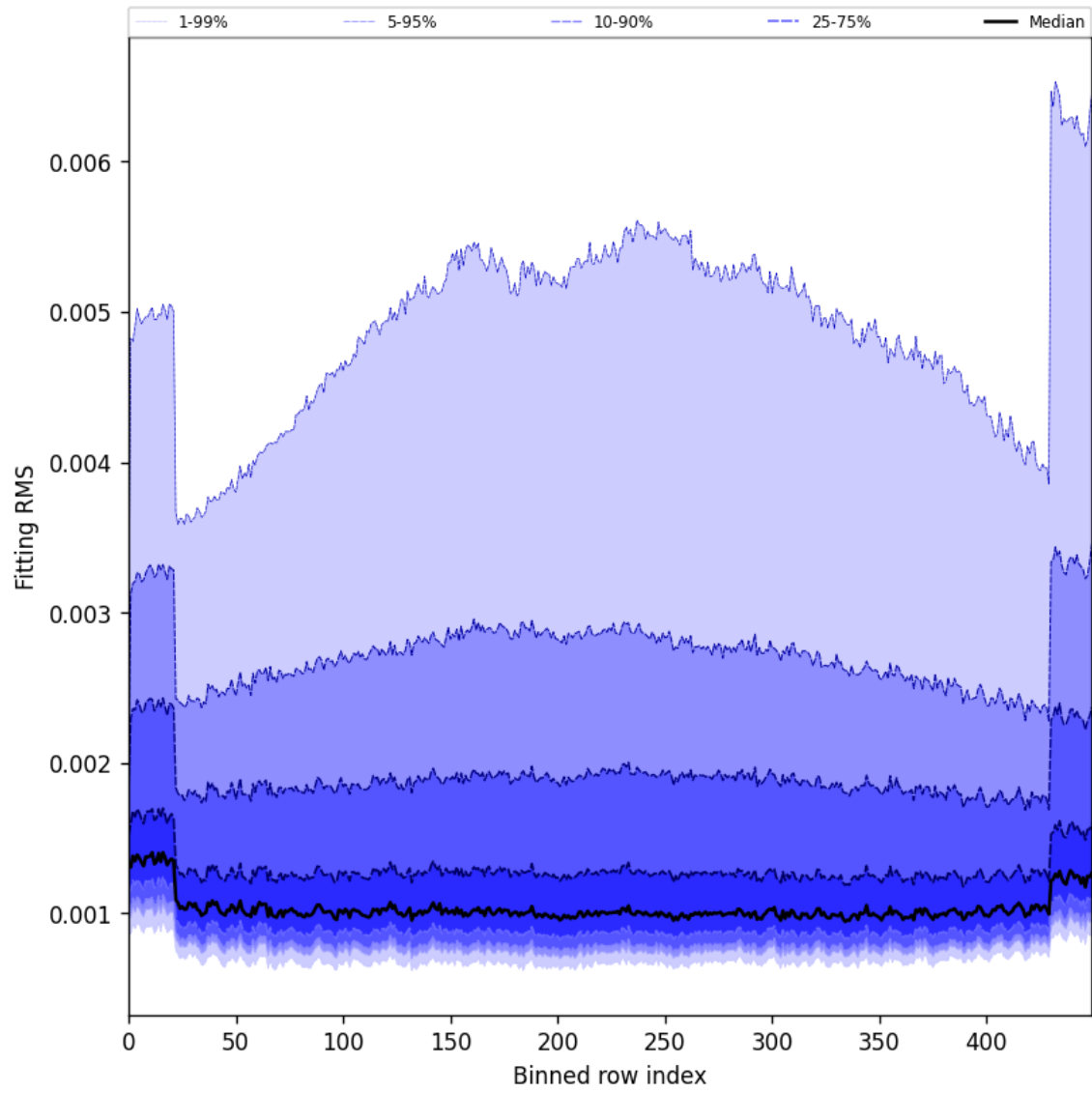
Figure 30: Along track statistics of “Fitting RMS” for 2025-07-30 to 2025-08-01
