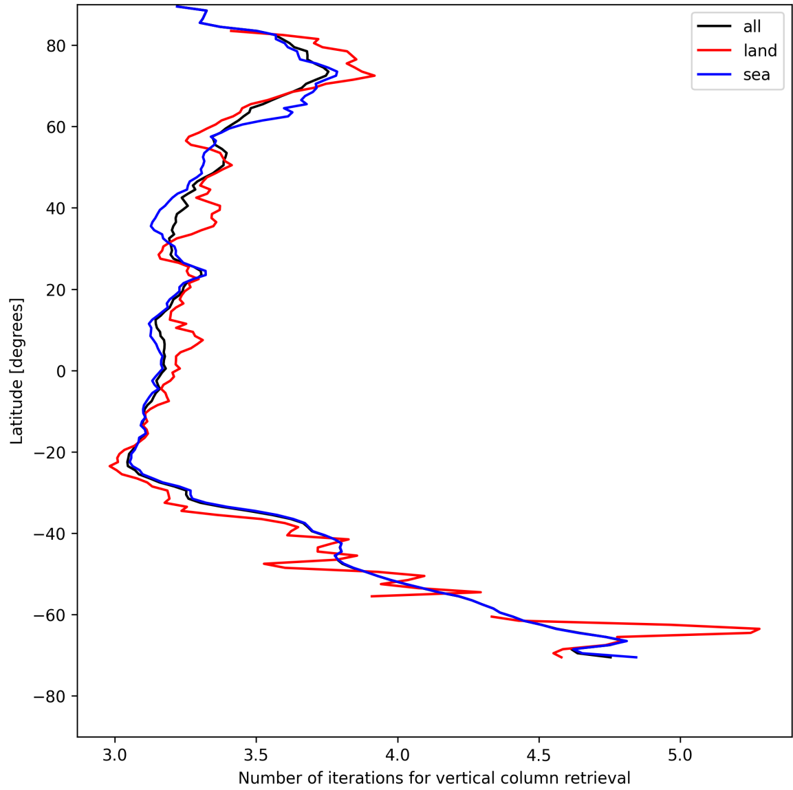
Figure 19: Zonal average of “Number of iterations for vertical column retrieval” for 2025-07-30 to 2025-08-01.
