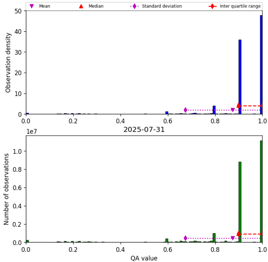
Figure 20: Histogram of “QA value” for 2025-07-30 to 2025-08-01
