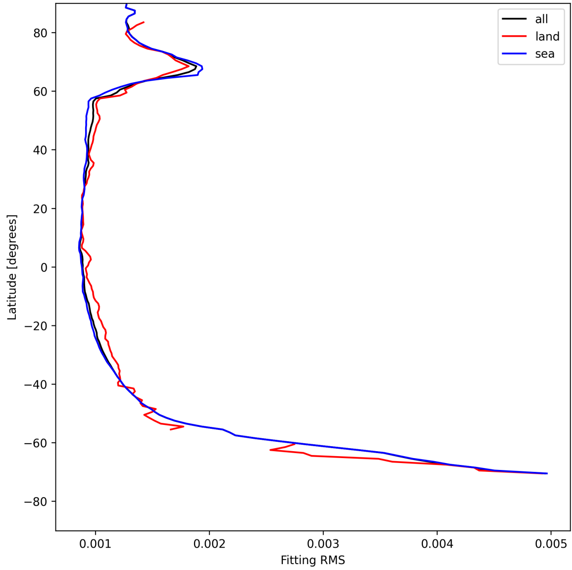
Figure 16: Zonal average of “Fitting RMS” for 2025-07-30 to 2025-08-01.
