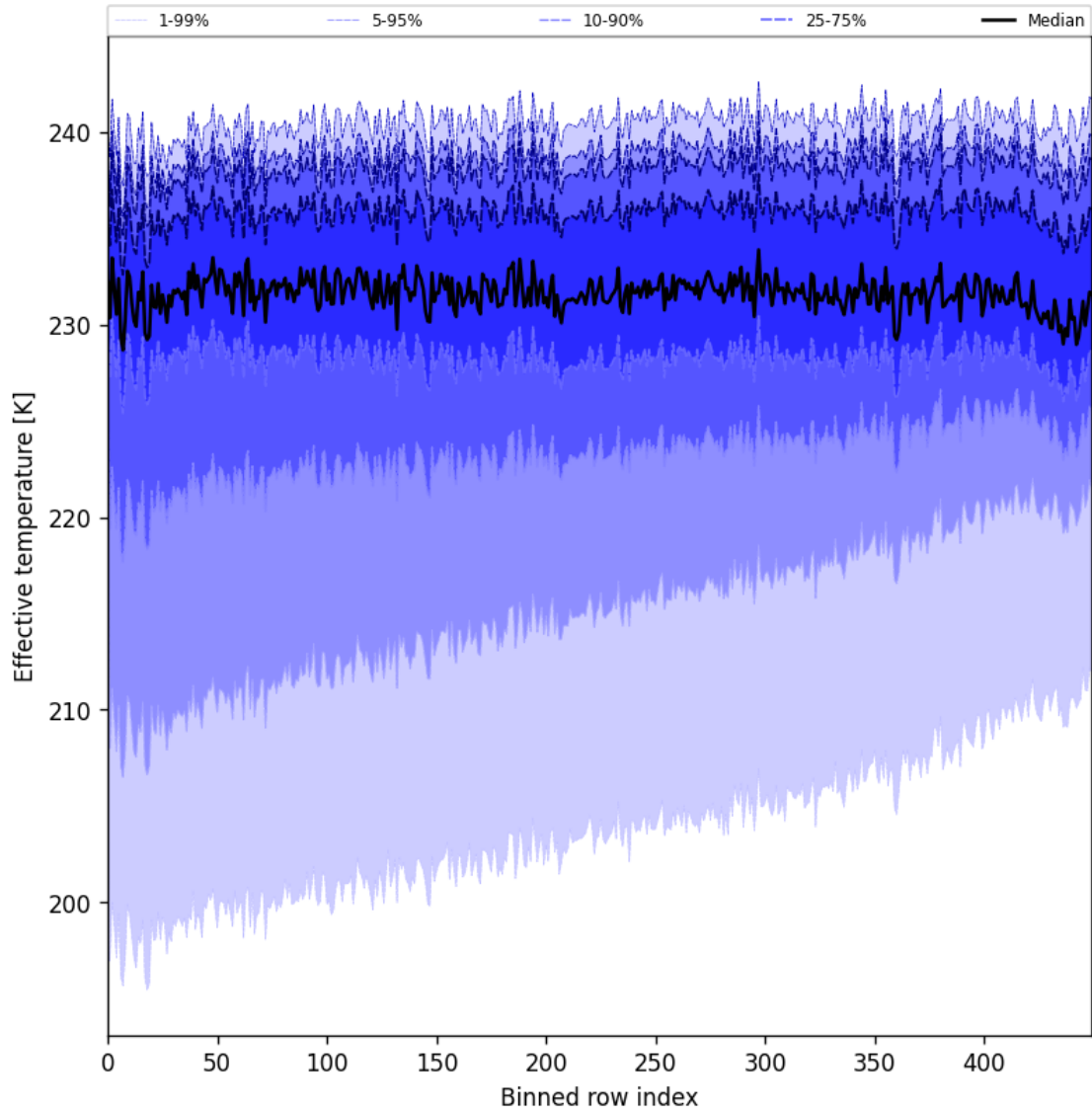
Figure 31: Along track statistics of “Effective temperature” for 2025-07-30 to 2025-08-01
