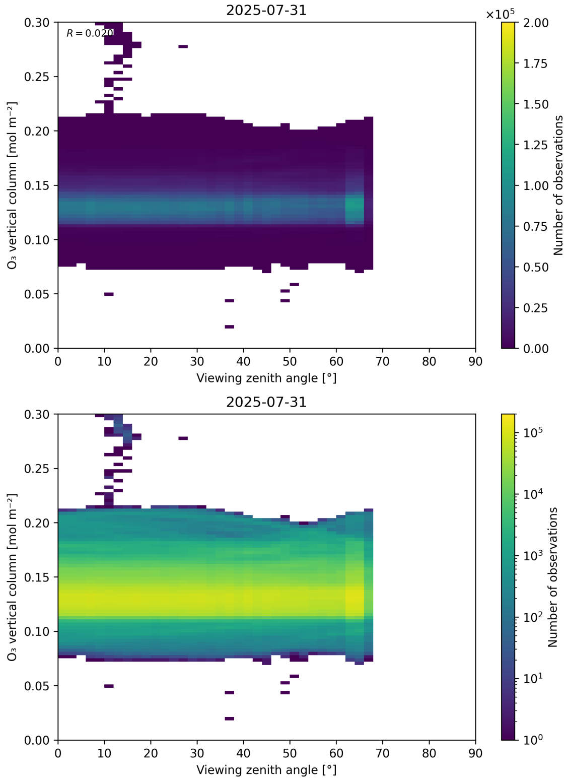
Figure 52: Scatter density plot of “Viewing zenith angle” against “O 3 vertical column” for 2025-07-30 to 2025-08-01.
