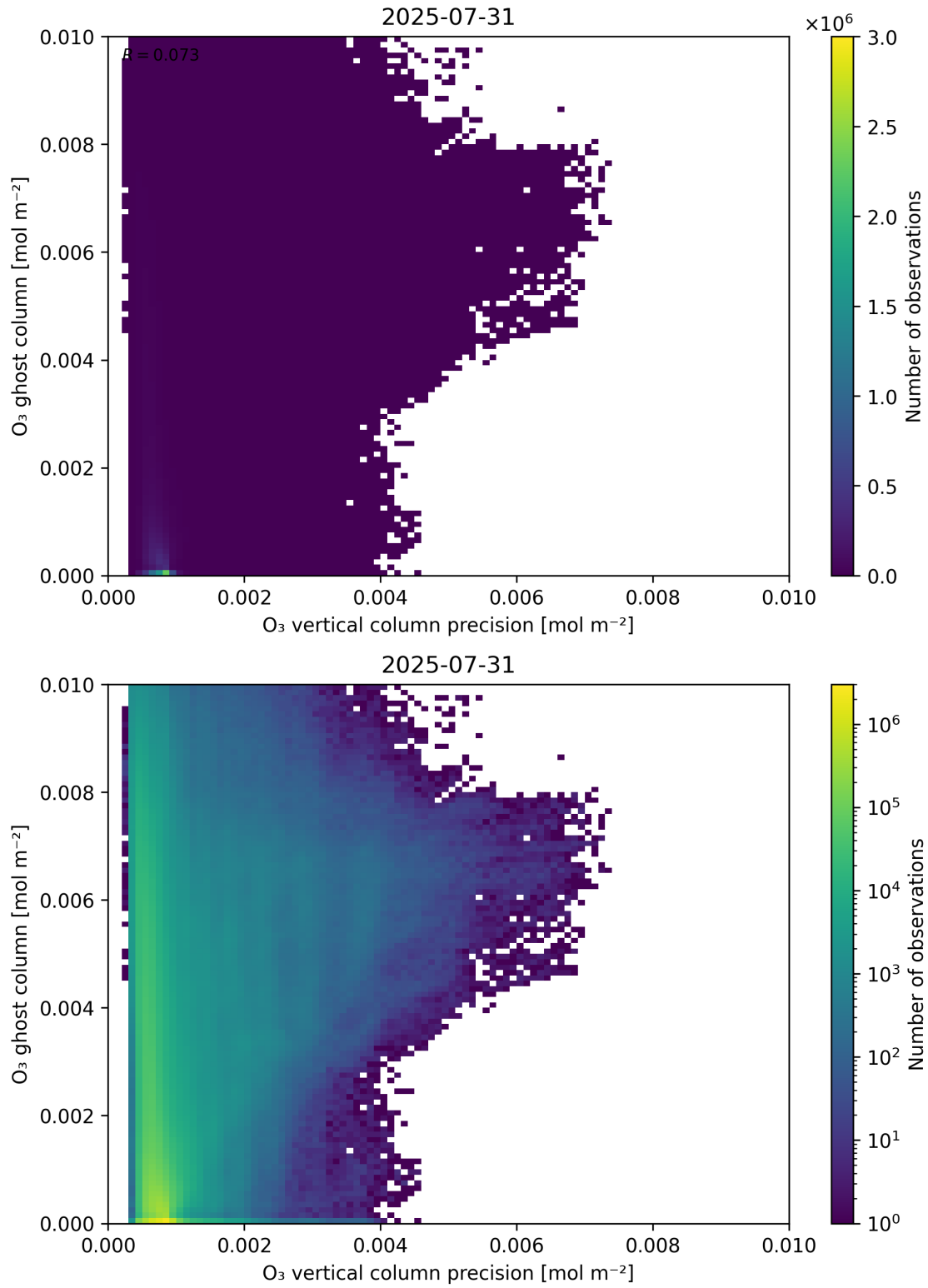
Figure 43: Scatter density plot of “ \text{O}_3 vertical column precision” against “ \text{O}_3 ghost column” for 2025-07-30 to 2025-08-01.
