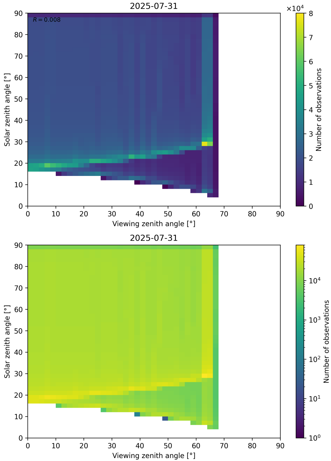
Figure 54: Scatter density plot of “Viewing zenith angle” against “Solar zenith angle” for 2025-07-30 to 2025-08-01.
