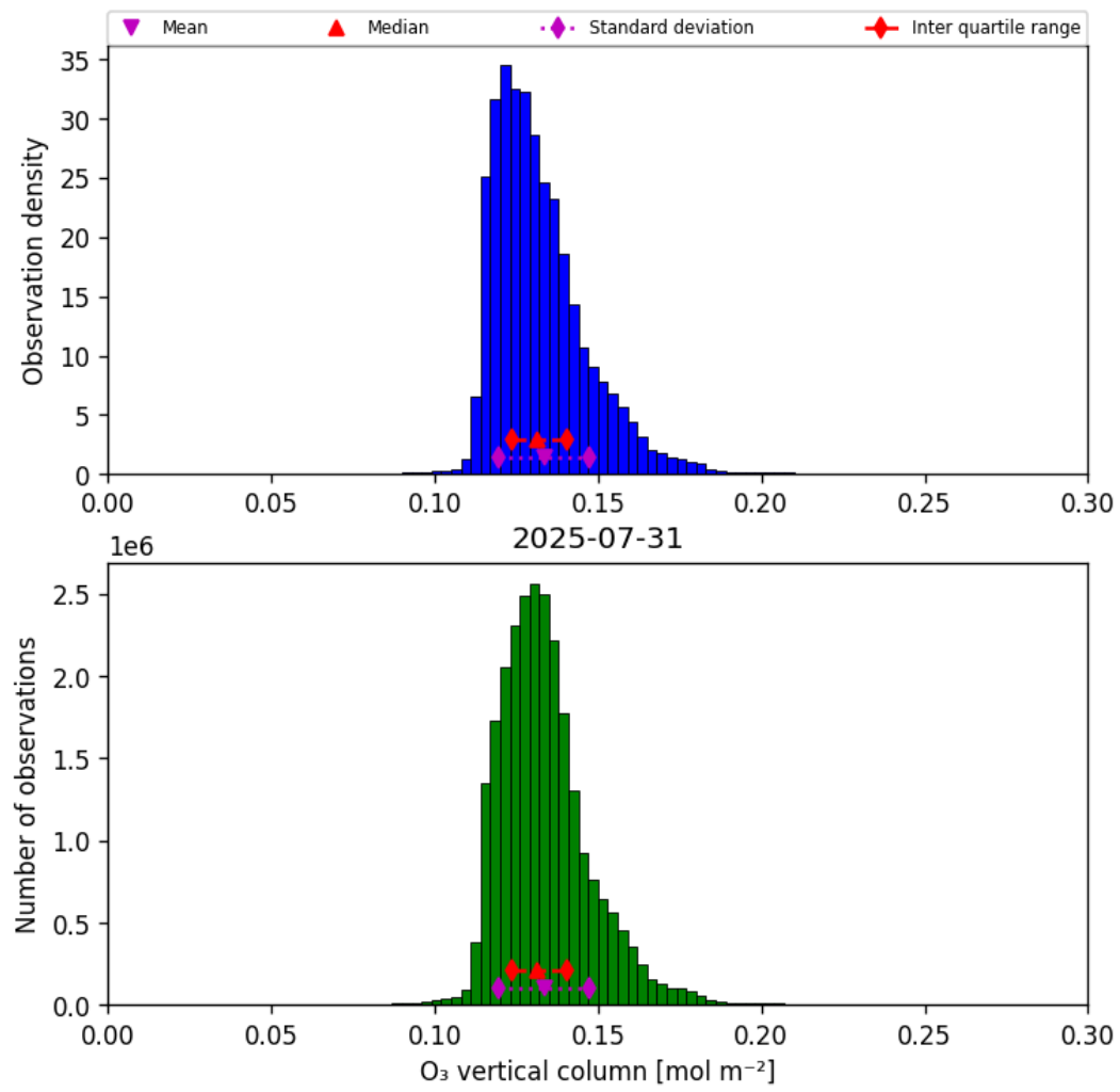
Figure 21: Histogram of “O 3 vertical column” for 2025-07-30 to 2025-08-01
