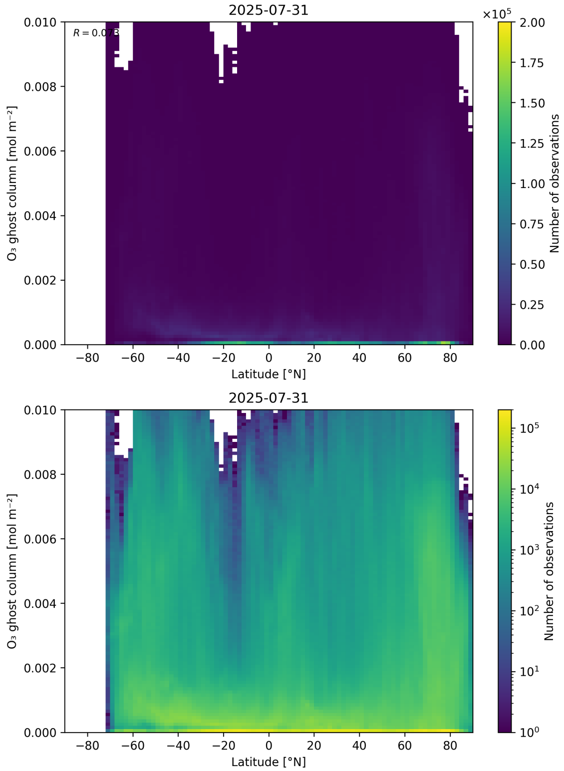
Figure 35: Scatter density plot of “Latitude” against “O 3 ghost column” for 2025-07-30 to 2025-08-01.
