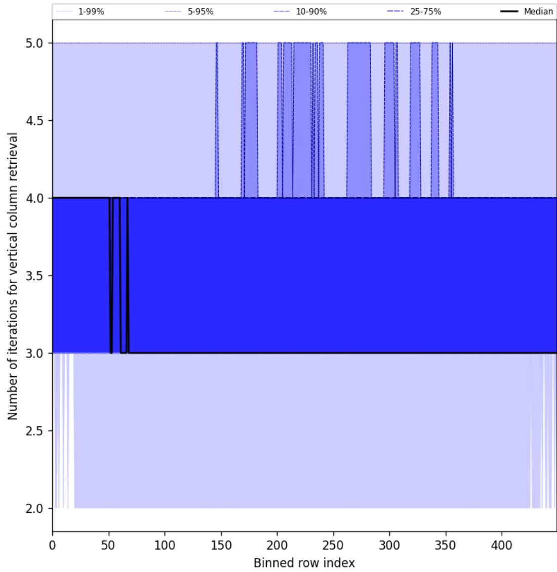
Figure 33: Along track statistics of “Number of iterations for vertical column retrieval” for 2025-07-30 to 2025-08-01
