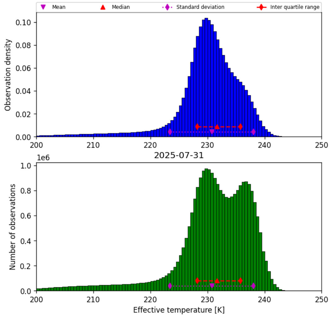
Figure 24: Histogram of “Effective temperature” for 2025-07-30 to 2025-08-01
