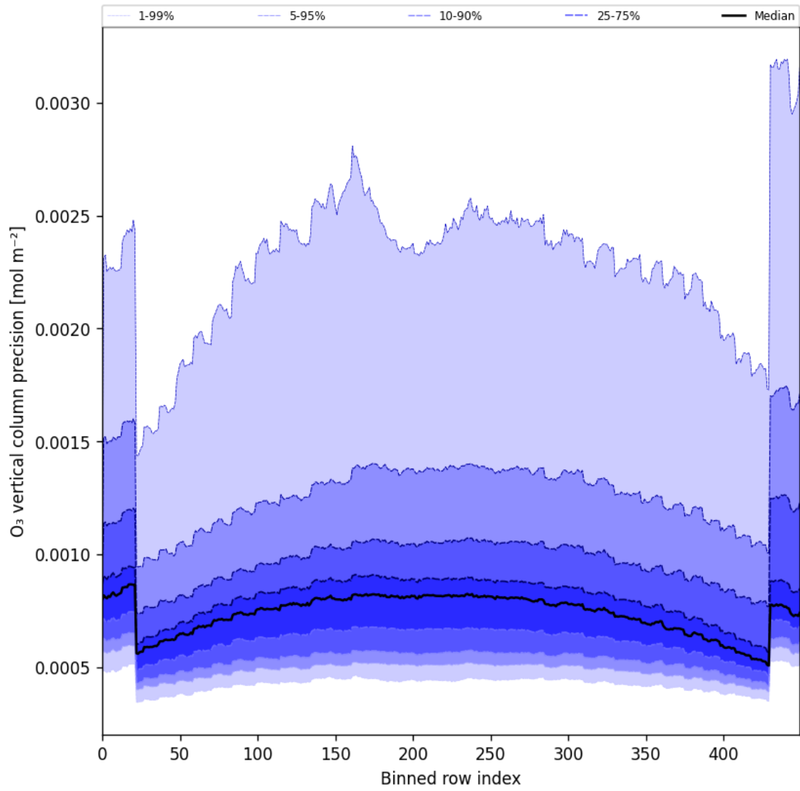
Figure 29: Along track statistics of “O 3 vertical column precision” for 2025-07-30 to 2025-08-01
