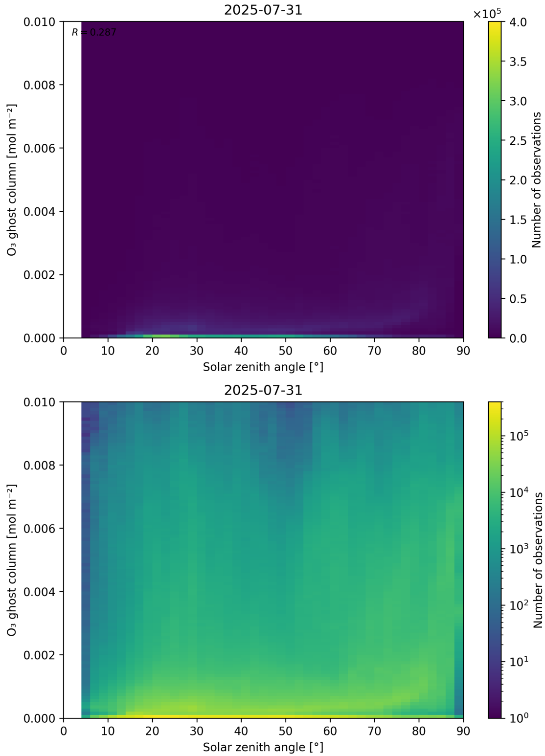
Figure 46: Scatter density plot of “Solar zenith angle” against “O 3 ghost column” for 2025-07-30 to 2025-08-01.
