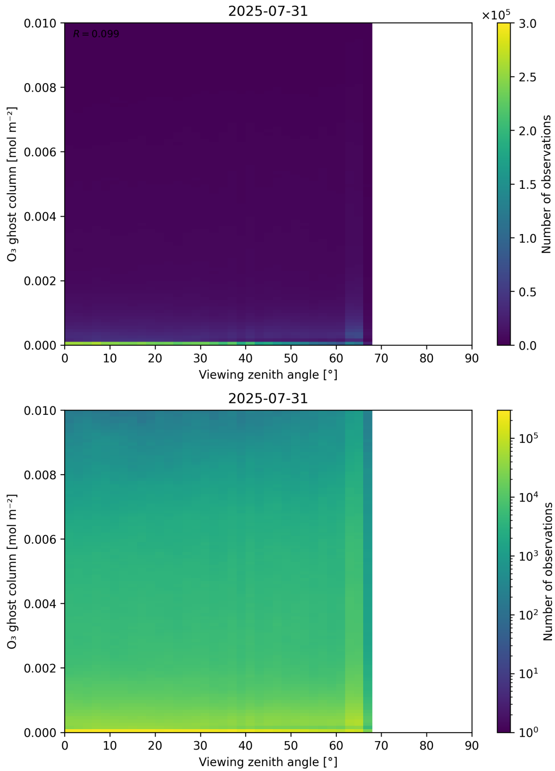
Figure 51: Scatter density plot of “Viewing zenith angle” against “O 3 ghost column” for 2025-07-30 to 2025-08-01.
