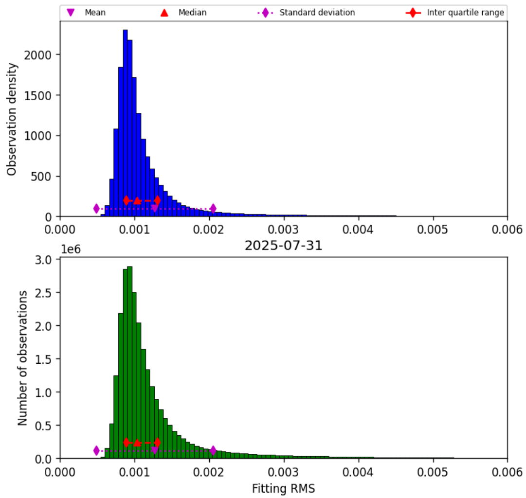
Figure 23: Histogram of “Fitting RMS” for 2025-07-30 to 2025-08-01
