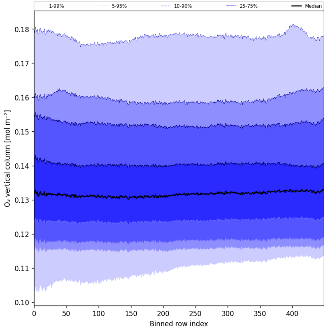
Figure 28: Along track statistics of “O 3 vertical column” for 2025-07-30 to 2025-08-01
