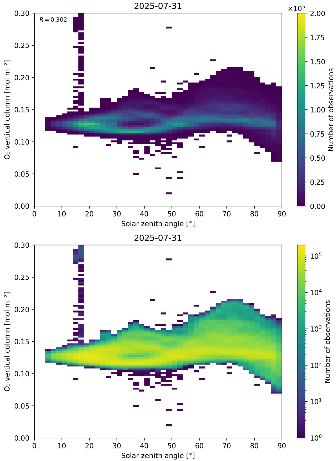
Figure 47: Scatter density plot of “Solar zenith angle” against “O 3 vertical column” for 2025-07-30 to 2025-08-01.
