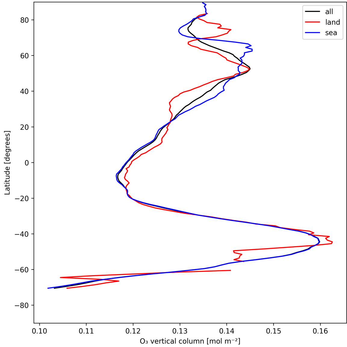
Figure 14: Zonal average of “O 3 vertical column” for 2025-07-30 to 2025-08-01.
